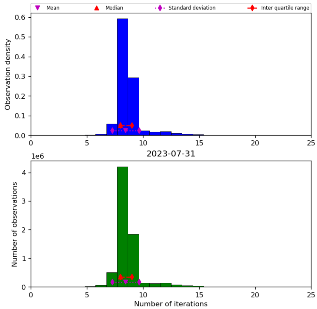
Figure 24: Histogram of “Number of iterations” for 2023-07-30 to 2023-08-01
