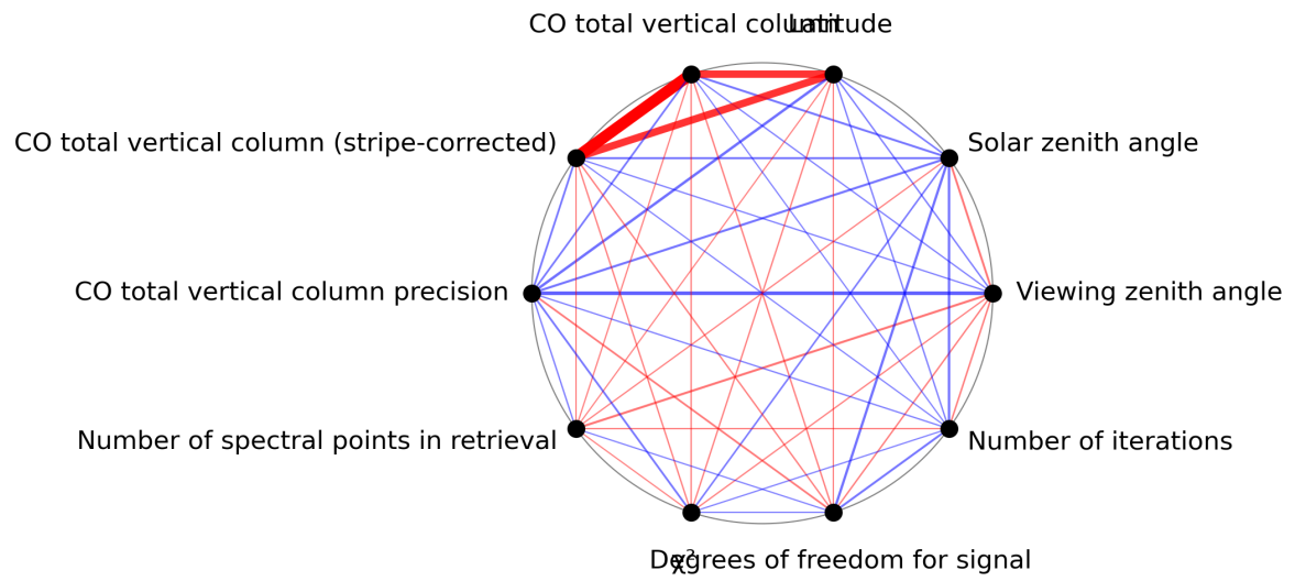
Figure 1: Map of correlation graph for 2023-07-30 to 2023-08-01.
