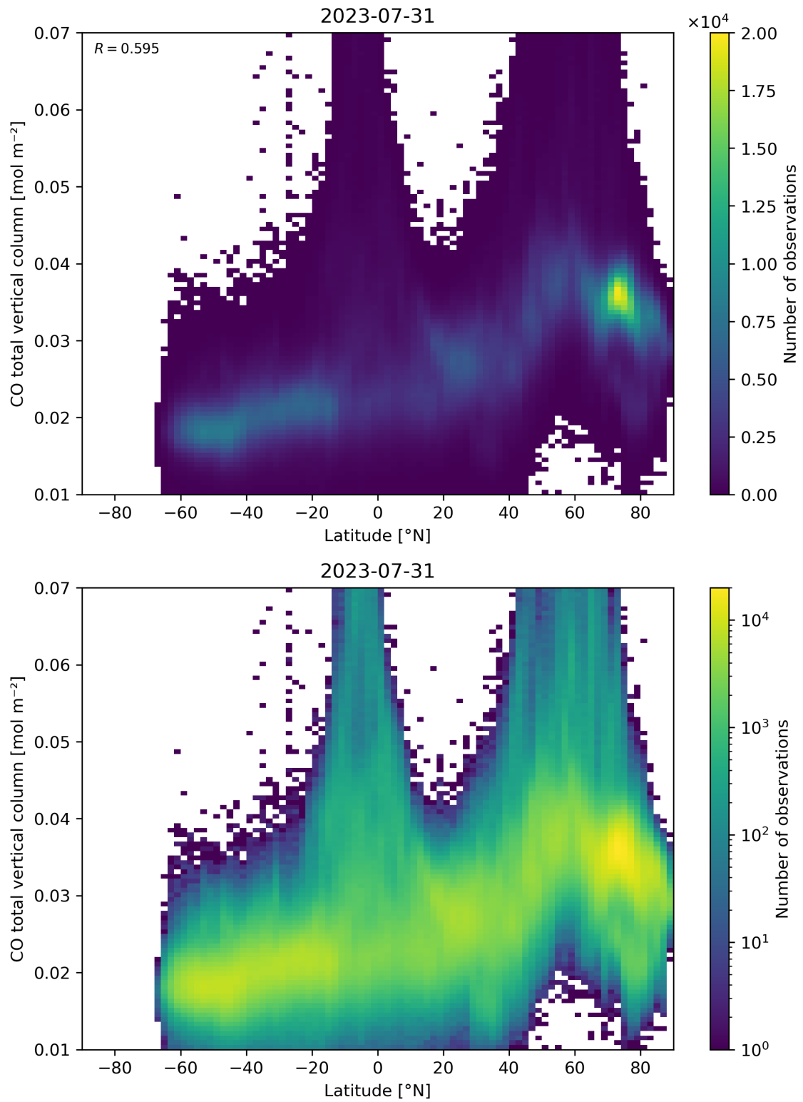
Figure 51: Scatter density plot of “Latitude” against “CO total vertical column” for 2023-07-30 to 2023-08-01.
