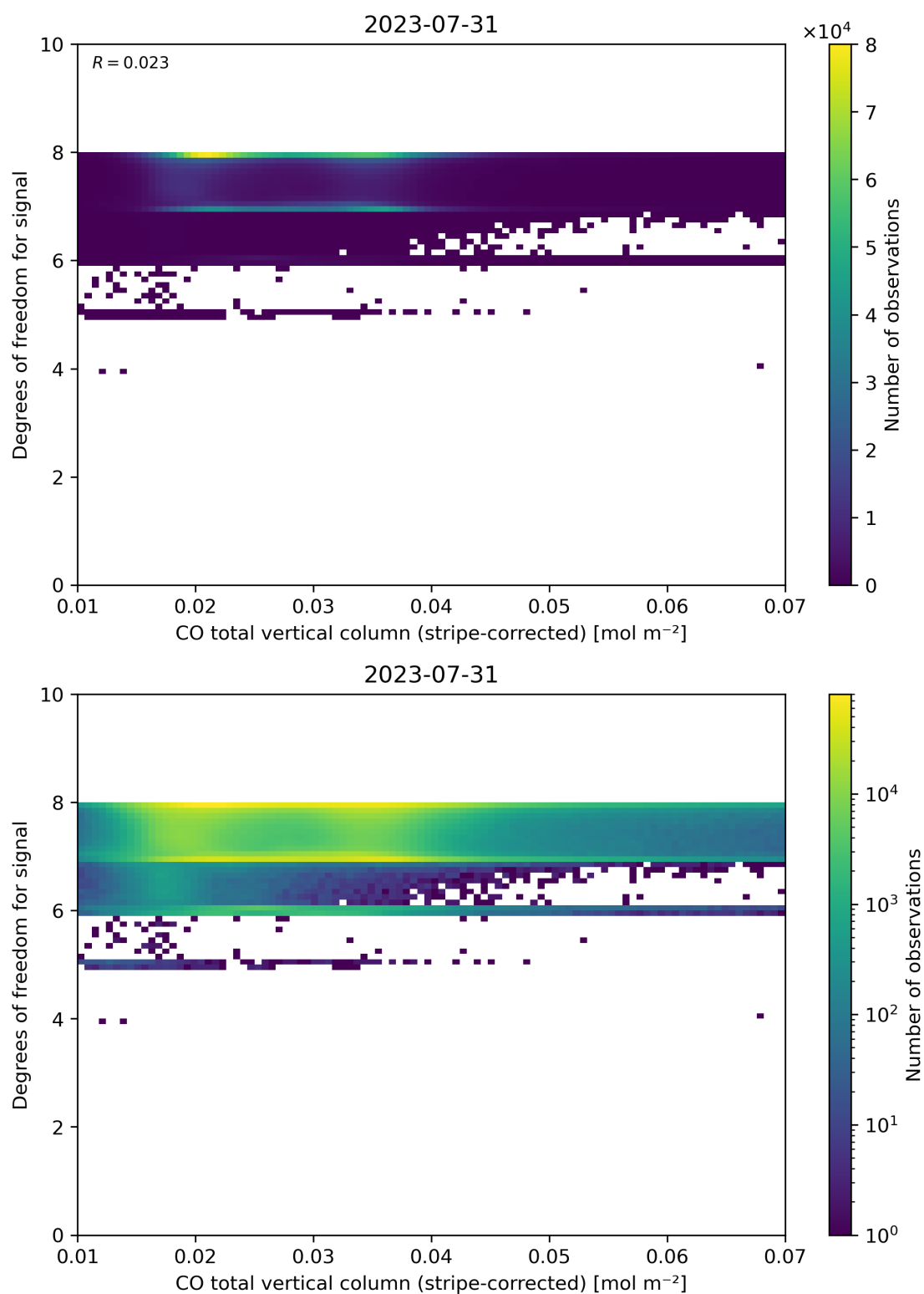
Figure 38: Scatter density plot of “CO total vertical column (stripe-corrected)” against “Degrees of freedom for signal” for 2023-07-30 to 2023-08-01.
