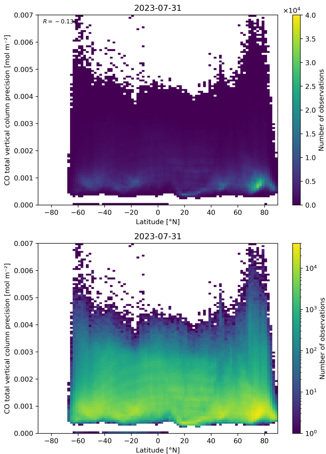
Figure 53: Scatter density plot of “Latitude” against “CO total vertical column precision” for 2023-07-30 to 2023-08-01.
