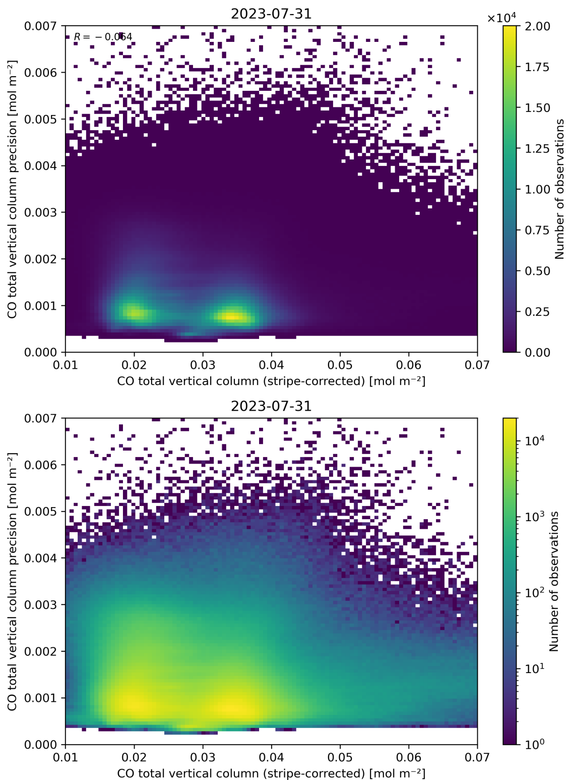
Figure 36: Scatter density plot of “CO total vertical column (stripe-corrected)” against “CO total vertical column precision” for 2023-07-30 to 2023-08-01.
