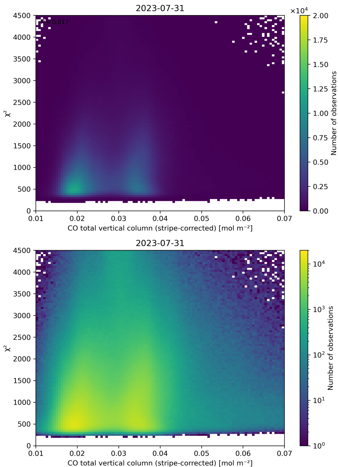
Figure 37: Scatter density plot of “CO total vertical column (stripe-corrected)” against “ \chi^2 ” for 2023-07-30 to 2023-08-01.
