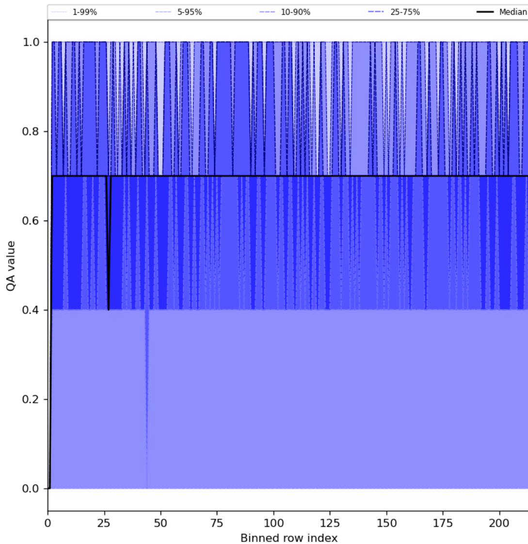
Figure 25: Along track statistics of “QA value” for 2023-07-30 to 2023-08-01
