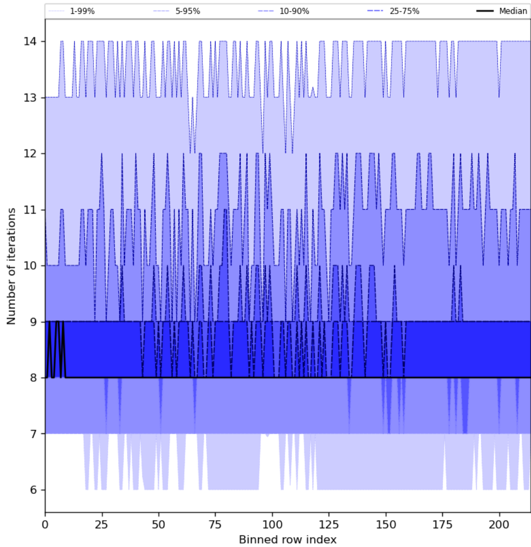
Figure 32: Along track statistics of “Number of iterations” for 2023-07-30 to 2023-08-01
