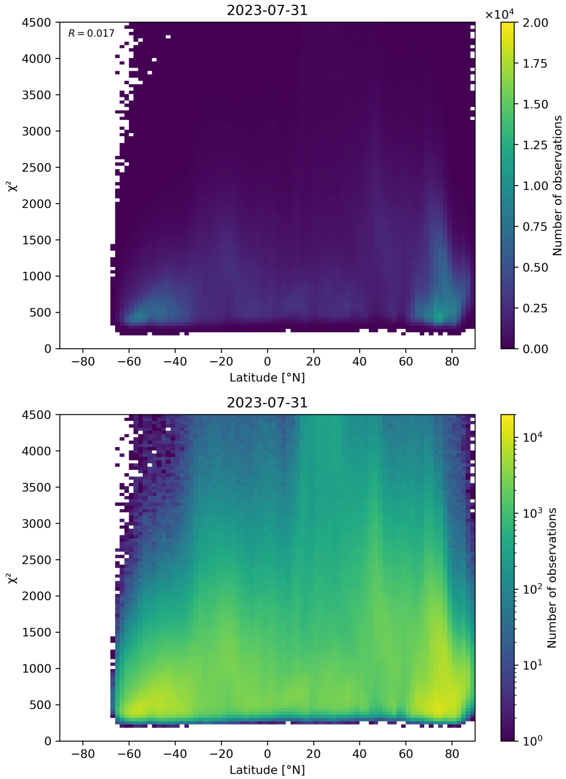
Figure 54: Scatter density plot of “Latitude” against “ \chi^2 ” for 2023-07-30 to 2023-08-01.
