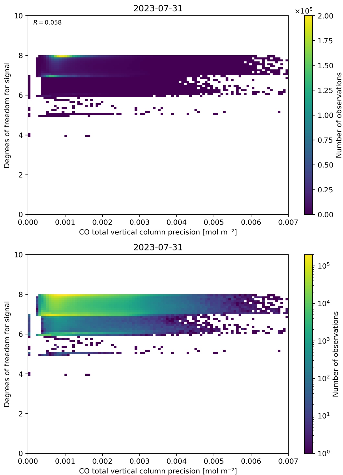
Figure 45: Scatter density plot of “CO total vertical column precision” against “Degrees of freedom for signal” for 2023-07-30 to 2023-08-01.
