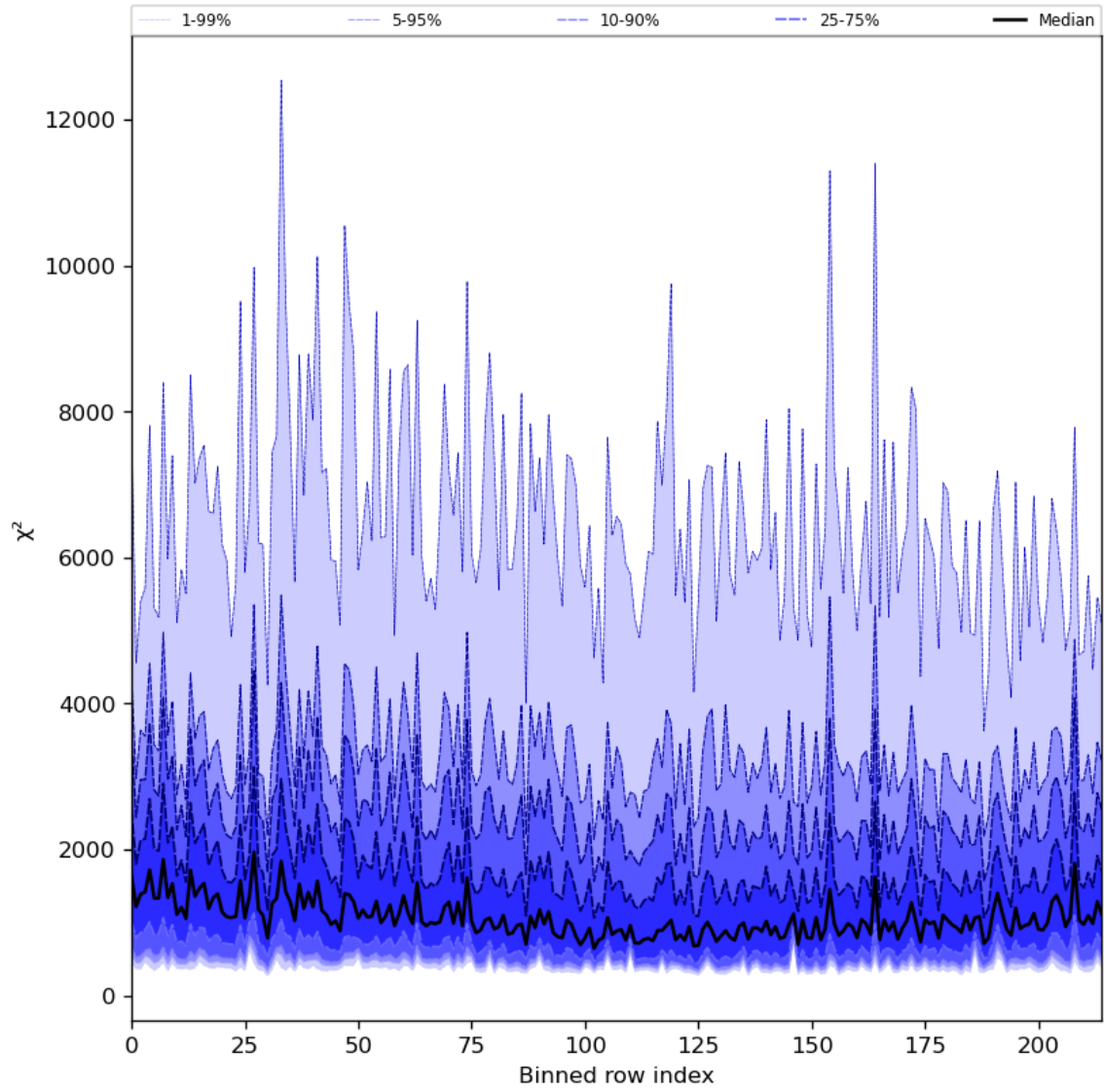
Figure 30: Along track statistics of “ \chi^2 ” for 2023-07-30 to 2023-08-01
