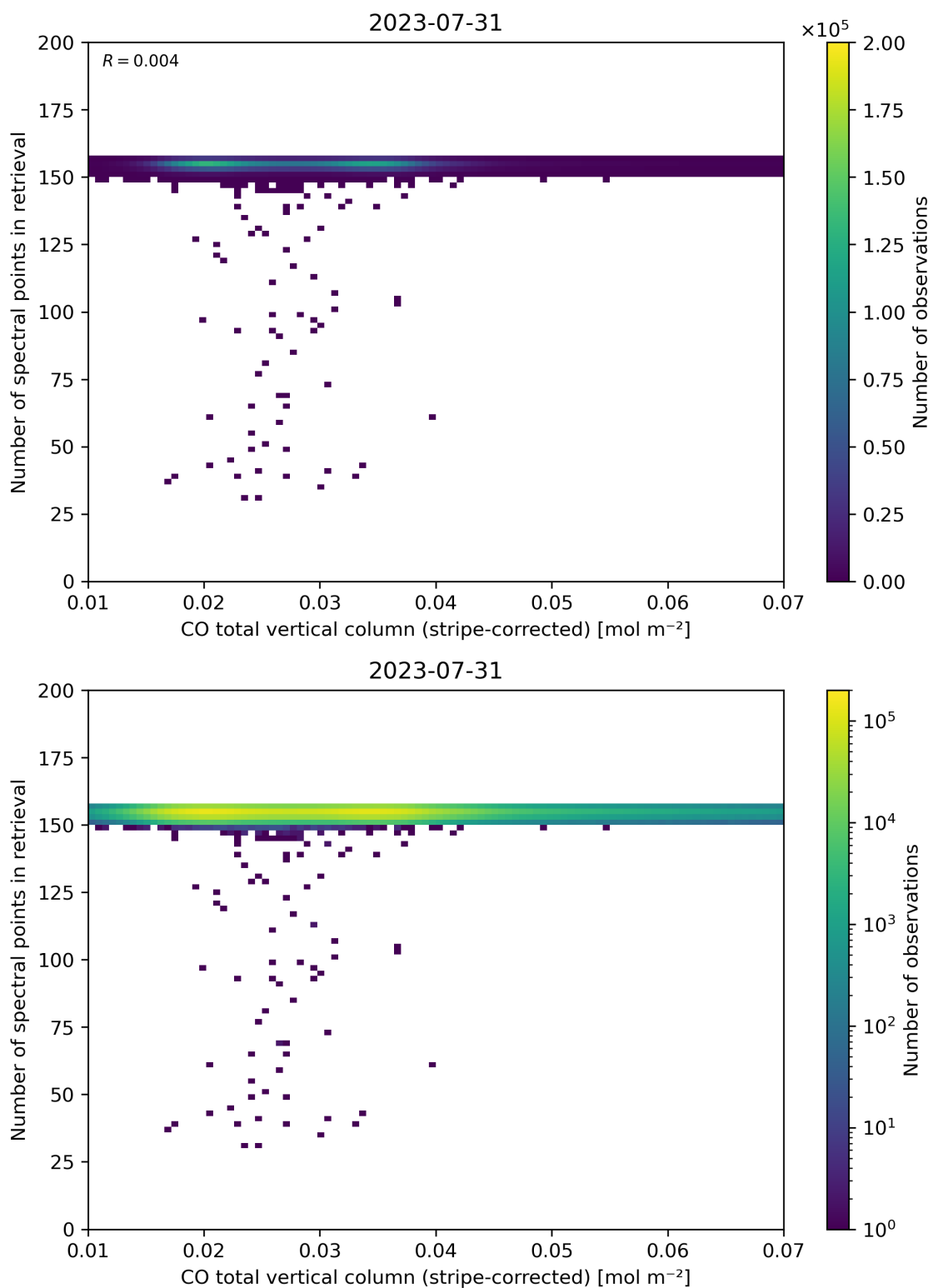
Figure 40: Scatter density plot of “CO total vertical column (stripe-corrected)” against “Number of spectral points in retrieval” for 2023-07-30 to 2023-08-01.
