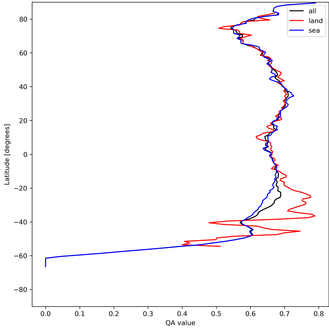
Figure 9: Zonal average of “QA value” for 2023-07-30 to 2023-08-01.
