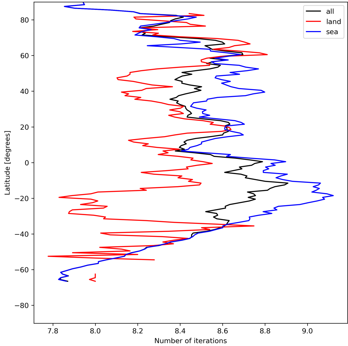
Figure 16: Zonal average of “Number of iterations” for 2023-07-30 to 2023-08-01.
