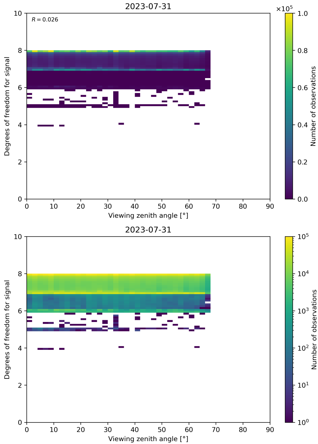
Figure 73: Scatter density plot of “Viewing zenith angle” against “Degrees of freedom for signal” for 2023-07-30 to 2023-08-01.
