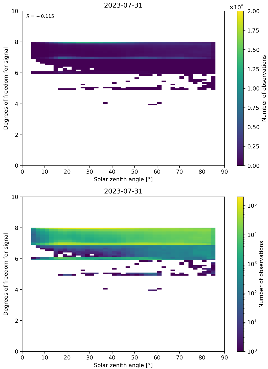
Figure 65: Scatter density plot of “Solar zenith angle” against “Degrees of freedom for signal” for 2023-07-30 to 2023-08-01.
