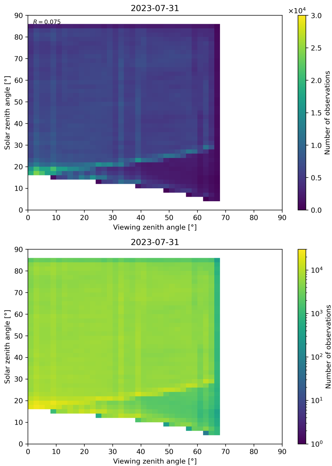
Figure 77: Scatter density plot of “Viewing zenith angle” against “Solar zenith angle” for 2023-07-30 to 2023-08-01.
