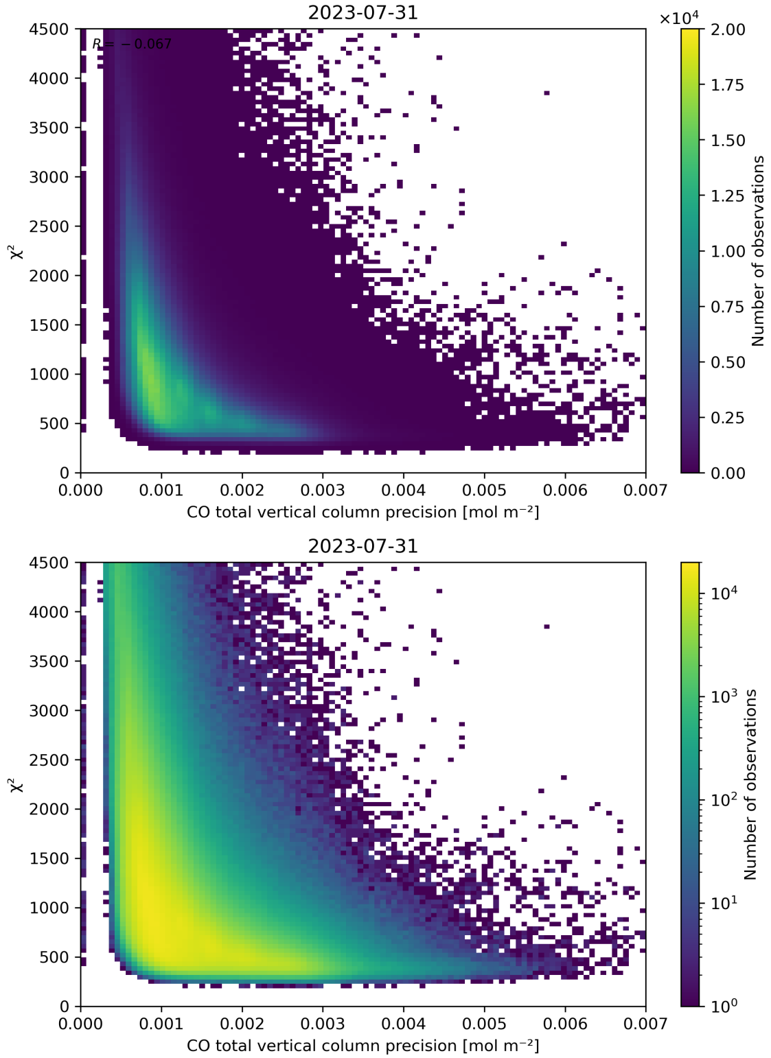
Figure 44: Scatter density plot of “CO total vertical column precision” against “ \chi^2 ” for 2023-07-30 to 2023-08-01.
