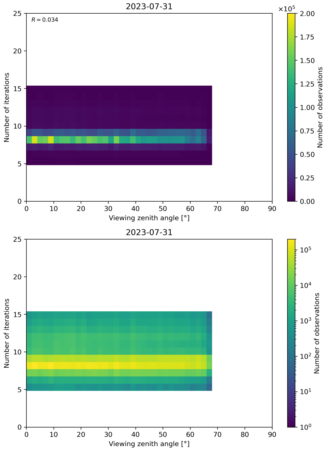
Figure 75: Scatter density plot of “Viewing zenith angle” against “Number of iterations” for 2023-07-30 to 2023-08-01.
