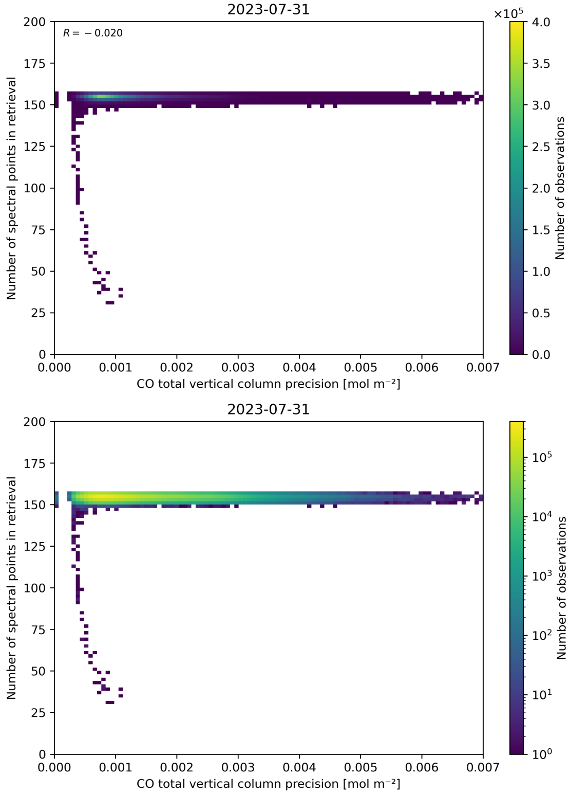
Figure 47: Scatter density plot of “CO total vertical column precision” against “Number of spectral points in retrieval” for 2023-07-30 to 2023-08-01.
