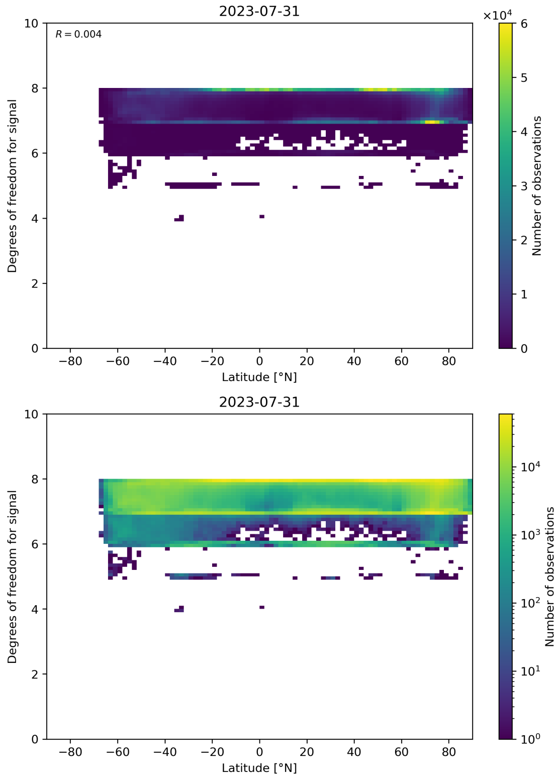
Figure 55: Scatter density plot of “Latitude” against “Degrees of freedom for signal” for 2023-07-30 to 2023-08-01.
