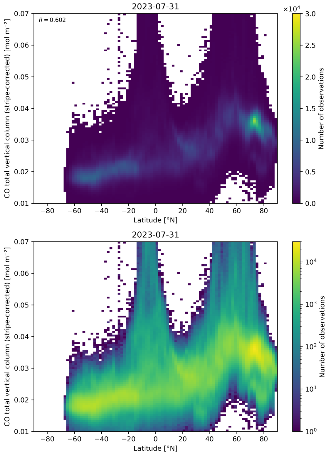
Figure 52: Scatter density plot of “Latitude” against “CO total vertical column (stripe-corrected)” for 2023-07-30 to 2023-08-01.
