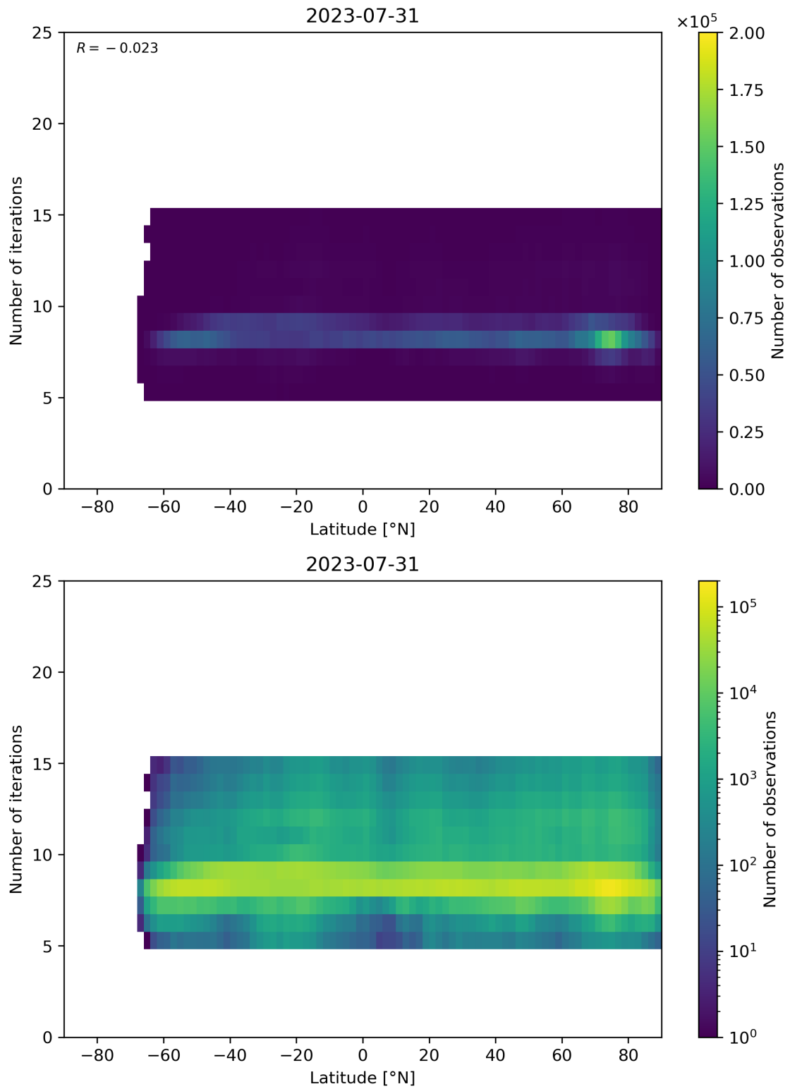
Figure 56: Scatter density plot of “Latitude” against “Number of iterations” for 2023-07-30 to 2023-08-01.
