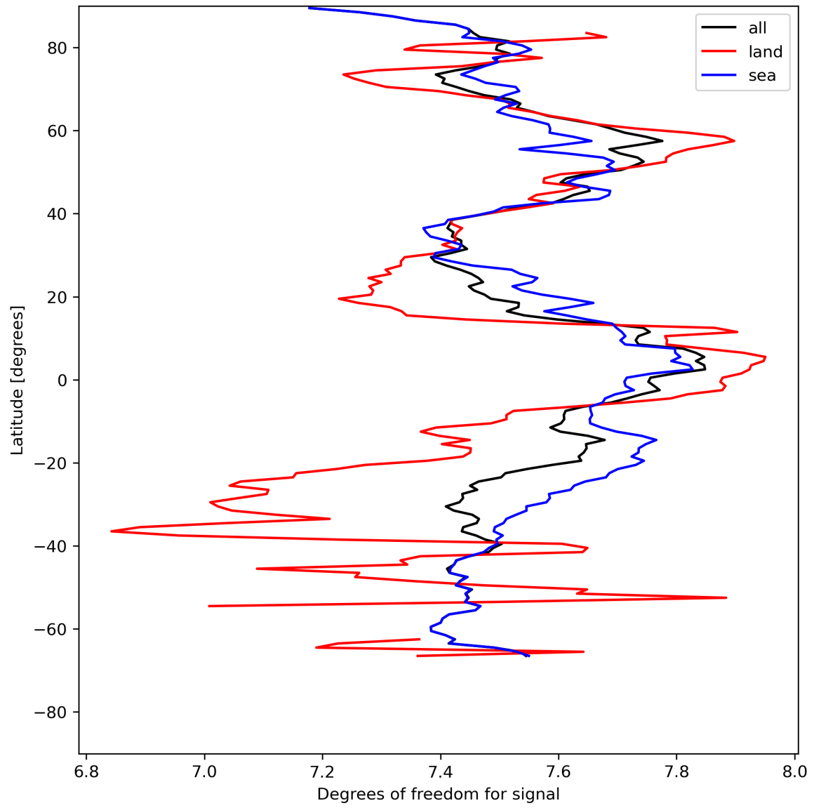
Figure 15: Zonal average of “Degrees of freedom for signal” for 2023-07-30 to 2023-08-01.
