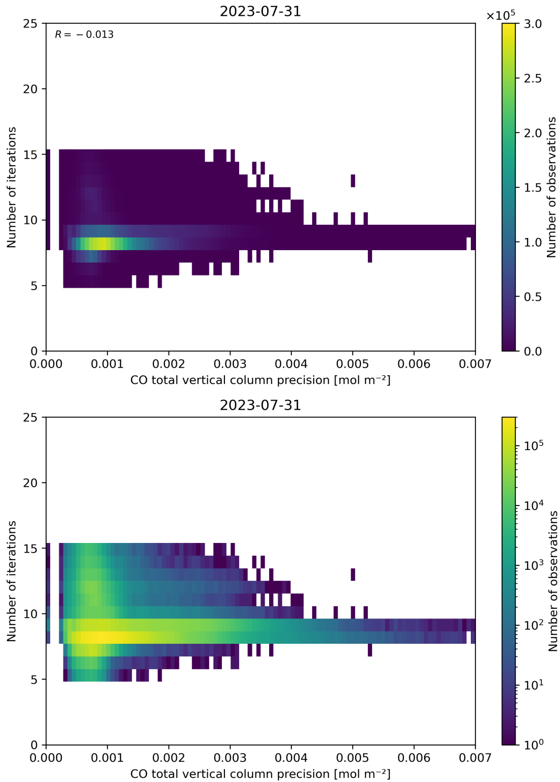
Figure 46: Scatter density plot of “CO total vertical column precision” against “Number of iterations” for 2023-07-30 to 2023-08-01.
