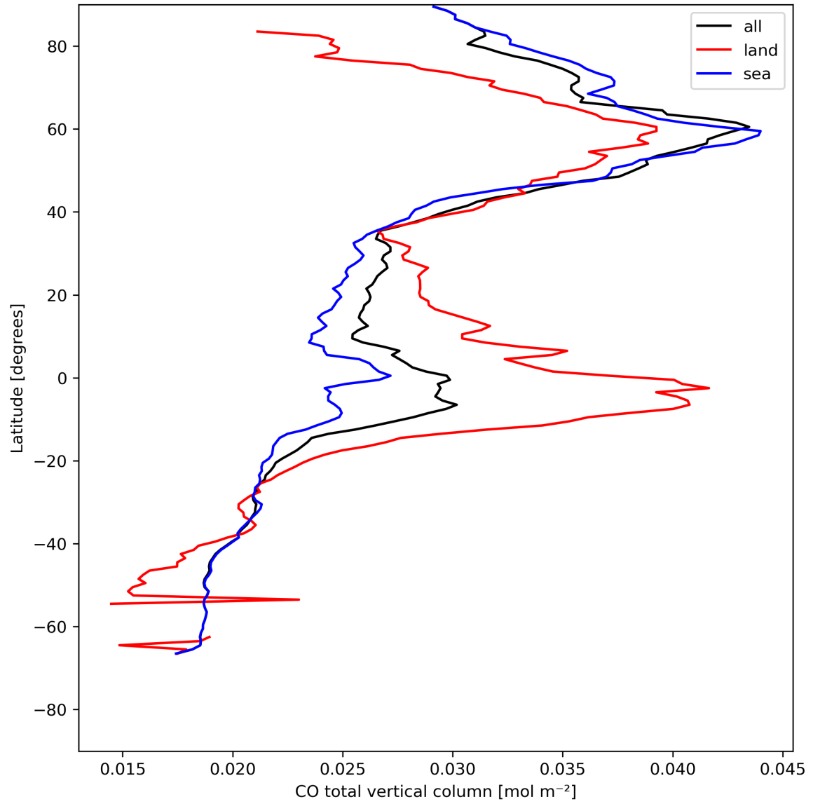
Figure 10: Zonal average of “CO total vertical column” for 2023-07-30 to 2023-08-01.
