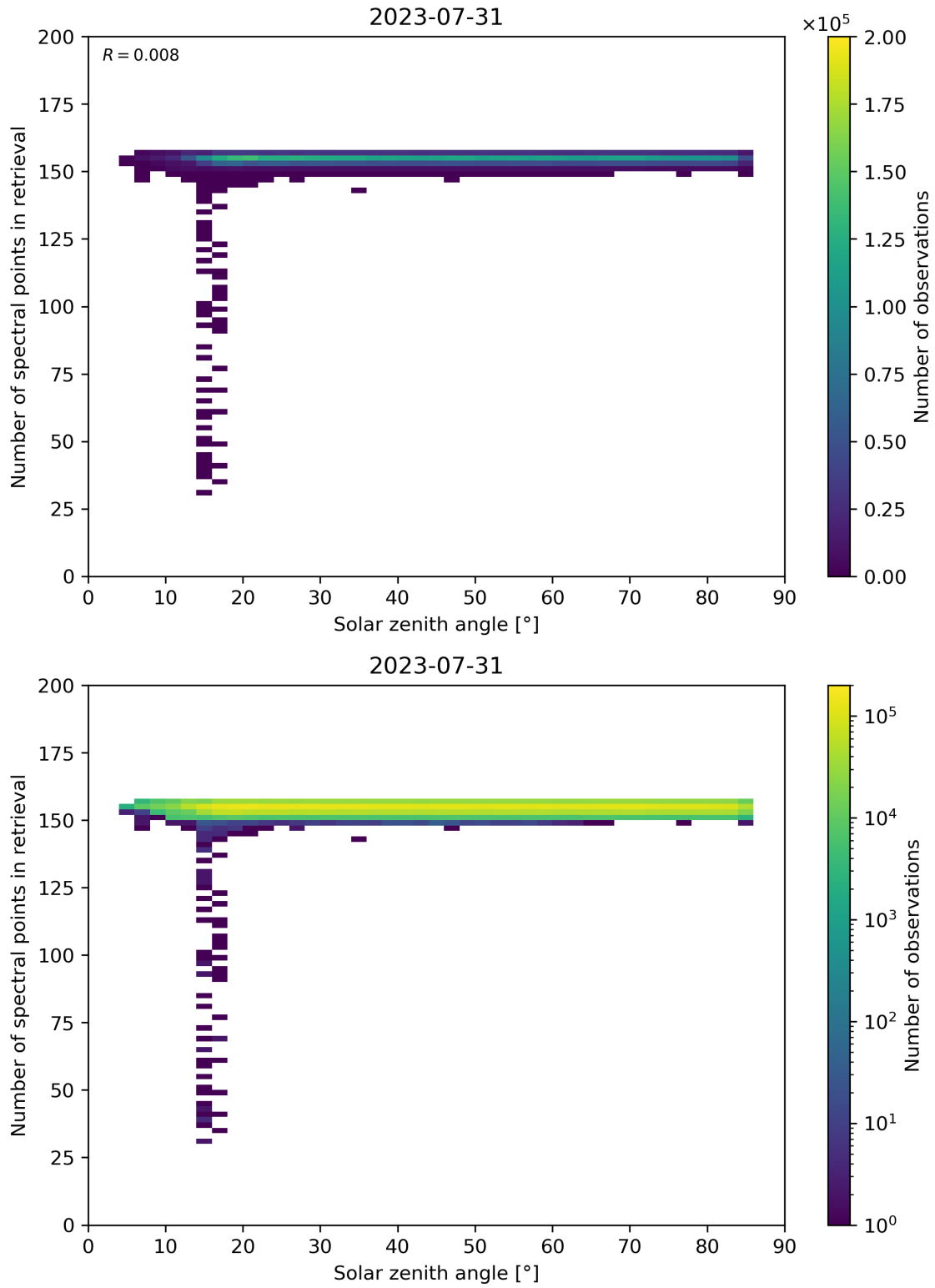
Figure 68: Scatter density plot of “Solar zenith angle” against “Number of spectral points in retrieval” for 2023-07-30 to 2023-08-01.
