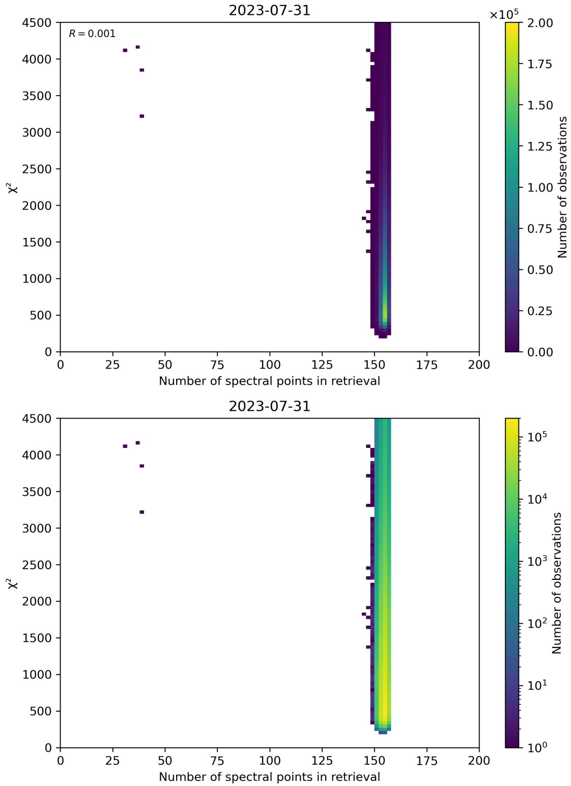
Figure 58: Scatter density plot of “Number of spectral points in retrieval” against “ \chi^2 ” for 2023-07-30 to 2023-08-01.
