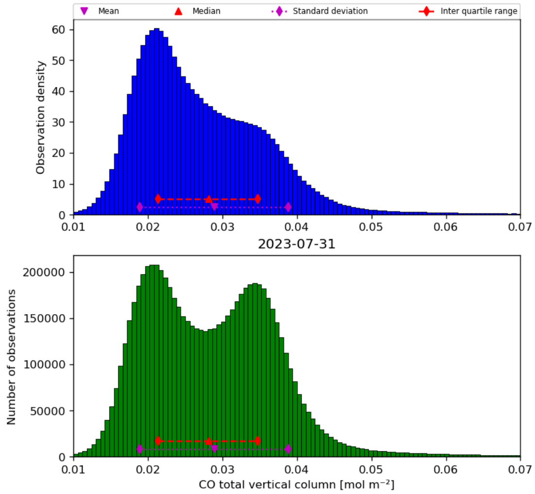
Figure 18: Histogram of “CO total vertical column” for 2023-07-30 to 2023-08-01
