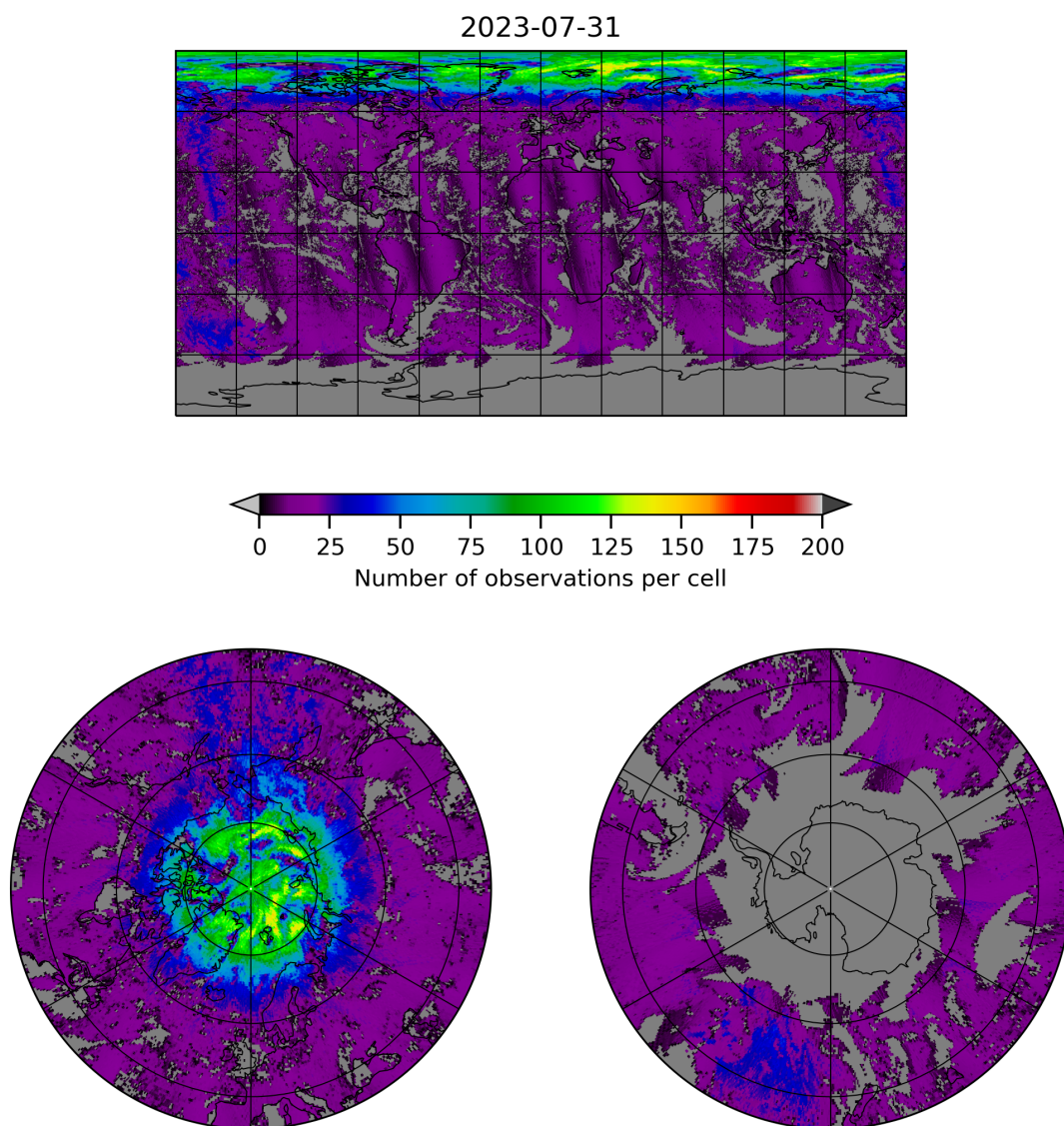
Figure 8: Map of the number of observations for 2023-07-30 to 2023-08-01
