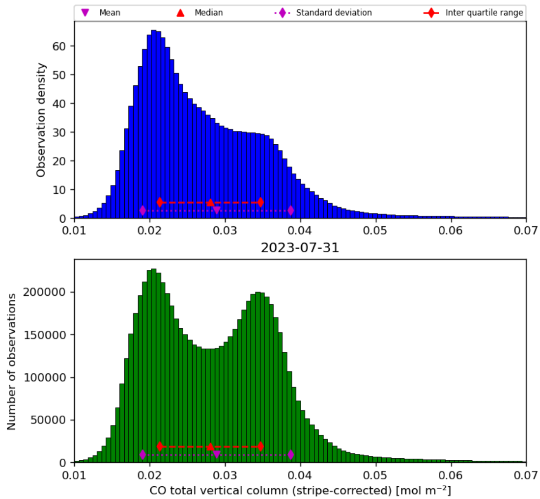
Figure 19: Histogram of “CO total vertical column (stripe-corrected)” for 2023-07-30 to 2023-08-01
