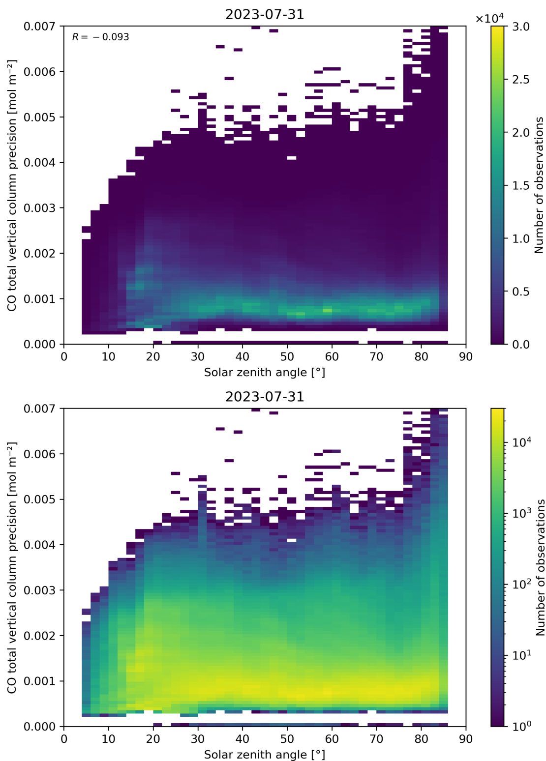
Figure 63: Scatter density plot of “Solar zenith angle” against “CO total vertical column precision” for 2023-07-30 to 2023-08-01.
