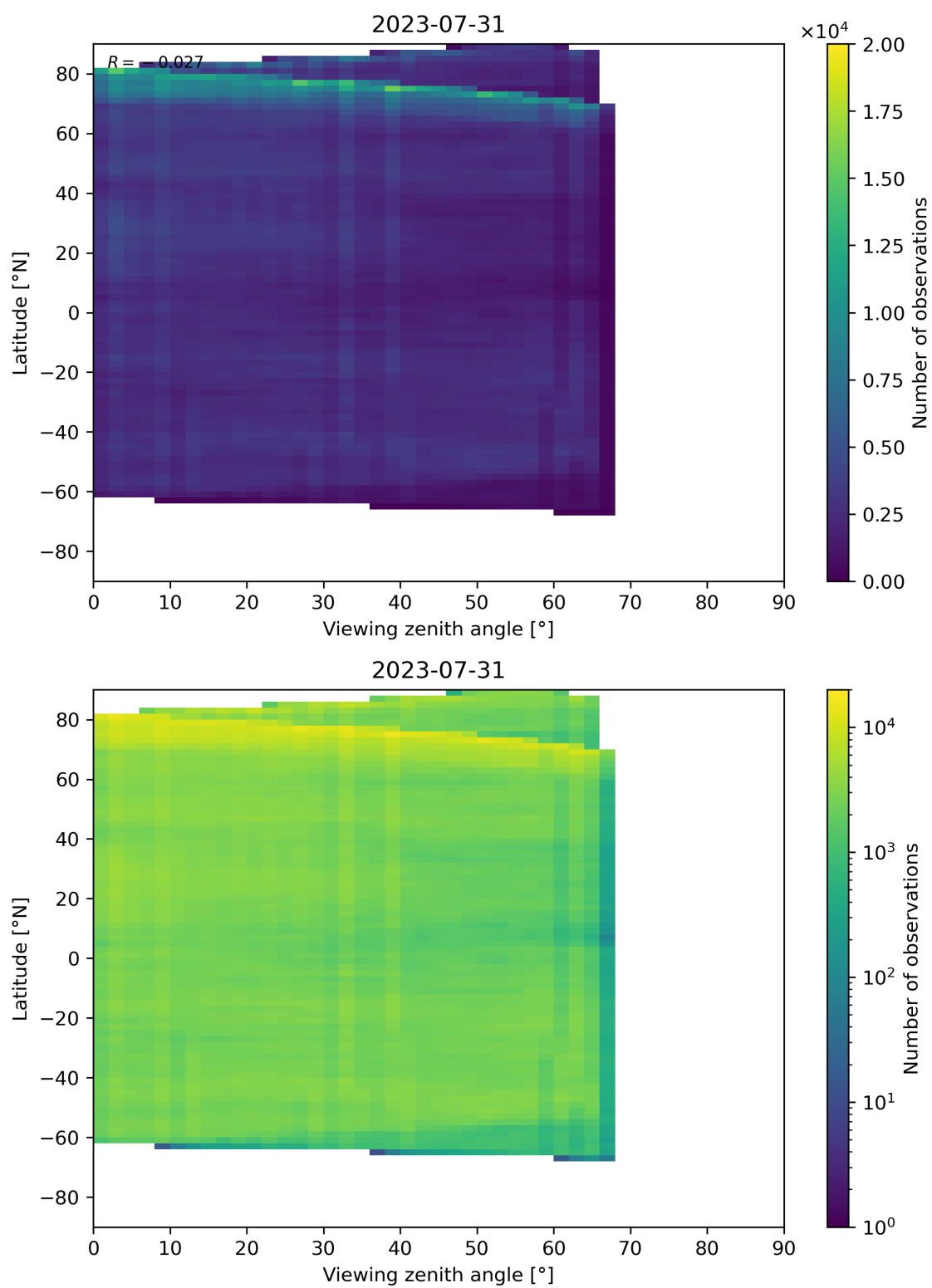
Figure 74: Scatter density plot of “Viewing zenith angle” against “Latitude” for 2023-07-30 to 2023-08-01.
