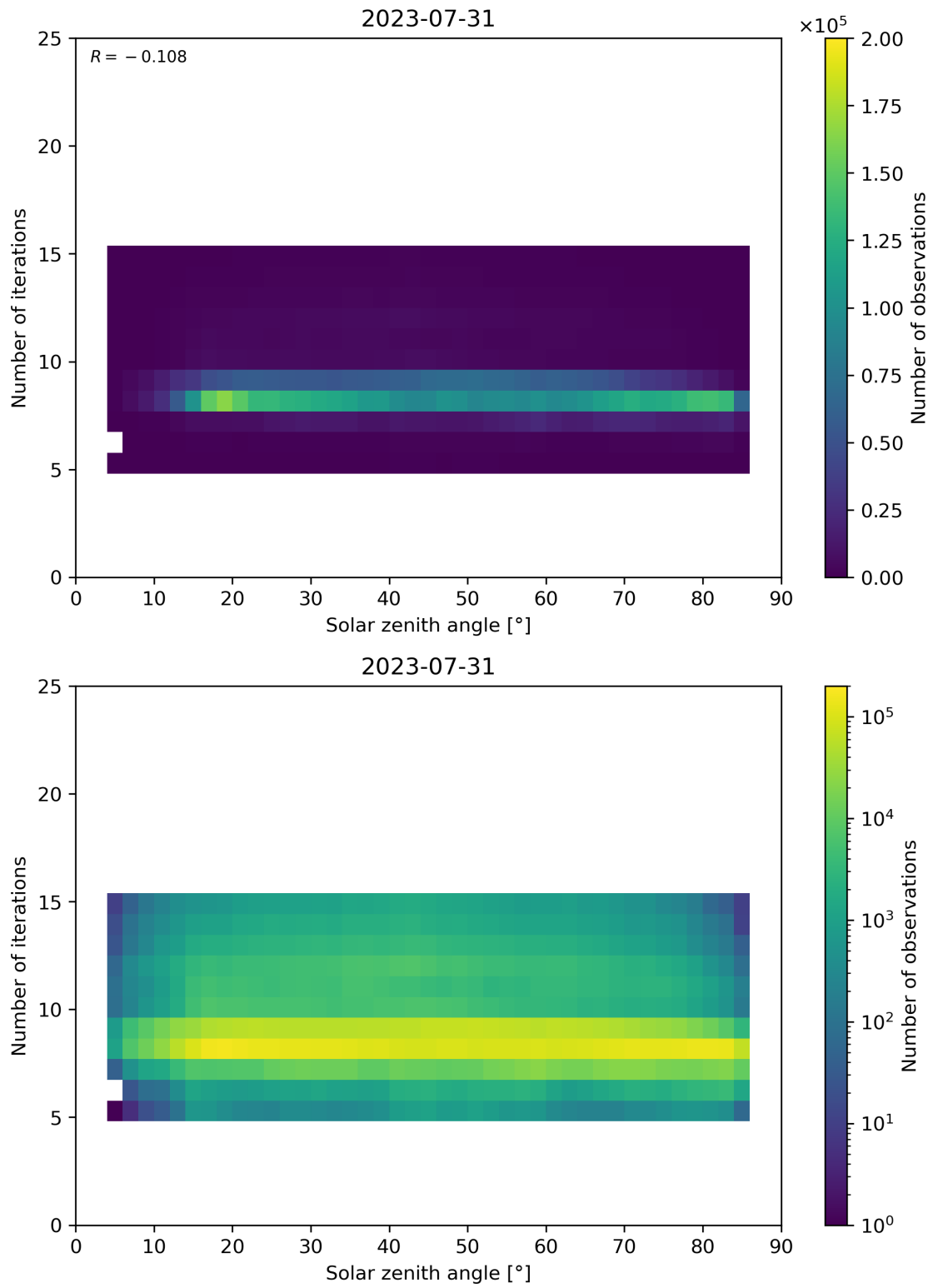
Figure 67: Scatter density plot of “Solar zenith angle” against “Number of iterations” for 2023-07-30 to 2023-08-01.
