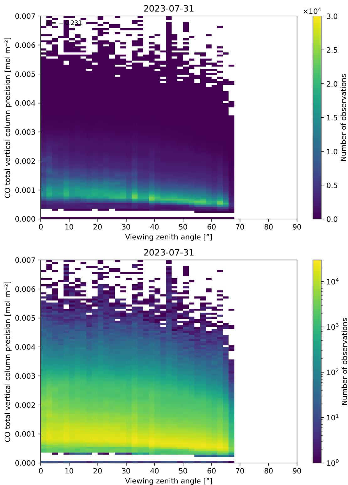
Figure 71: Scatter density plot of “Viewing zenith angle” against “CO total vertical column precision” for 2023-07-30 to 2023-08-01.
