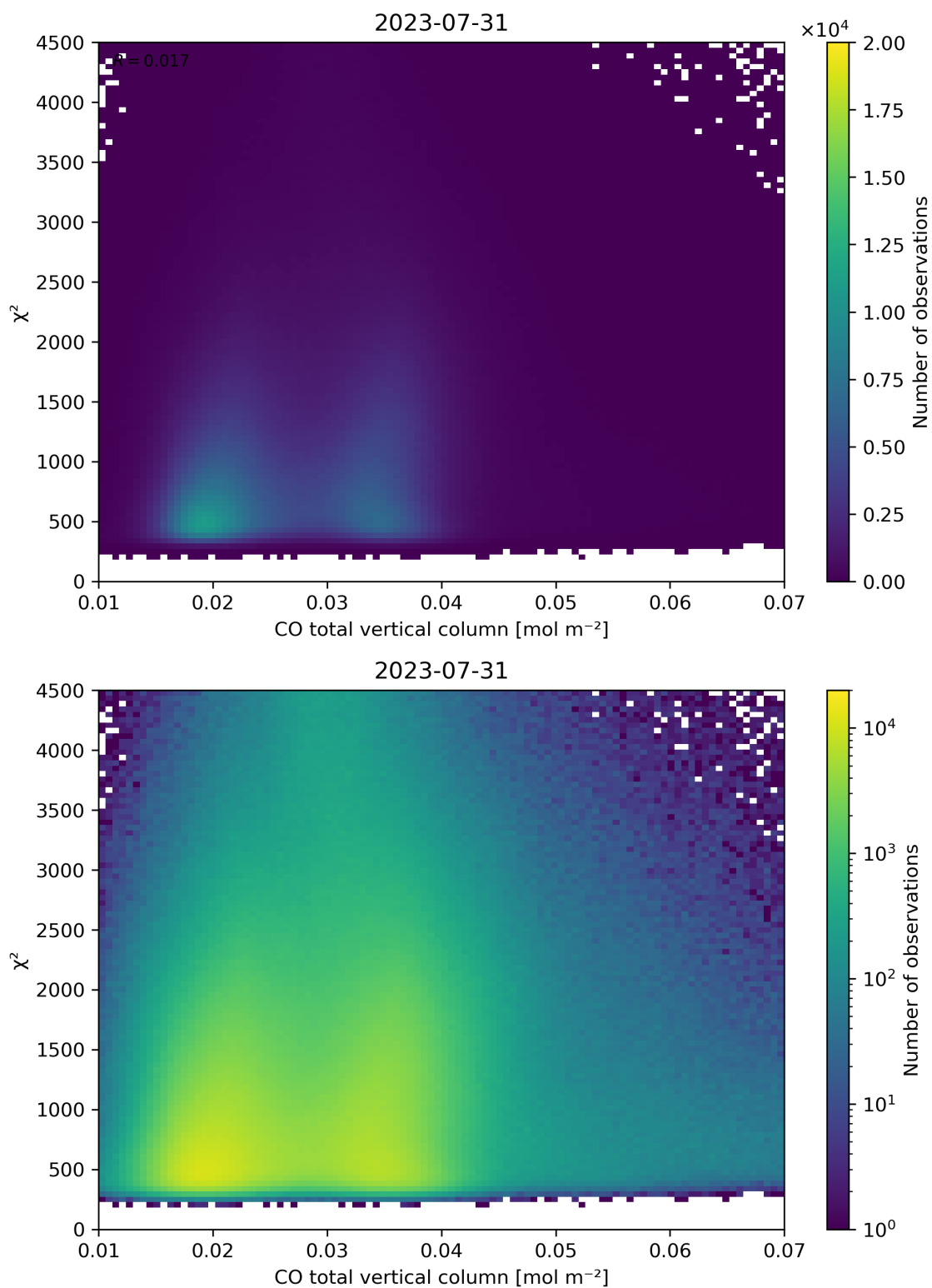
Figure 35: Scatter density plot of “CO total vertical column” against “ \chi^2 ” for 2023-07-30 to 2023-08-01.
