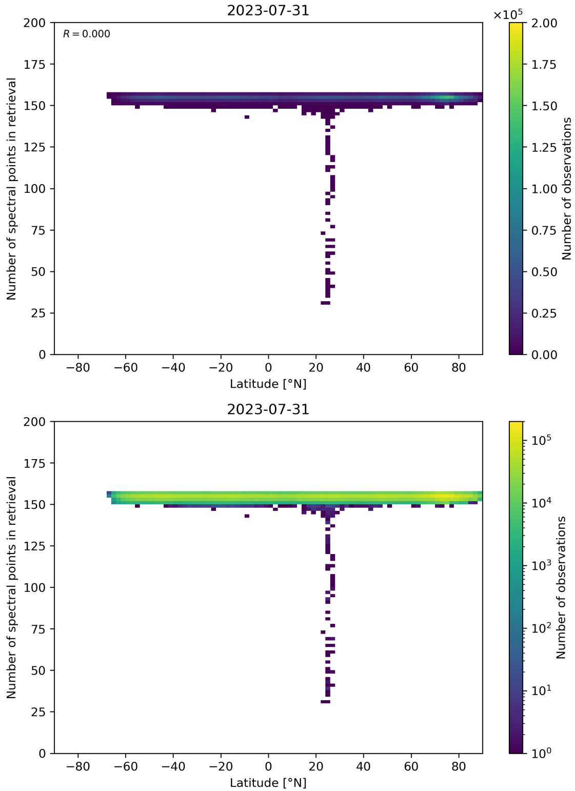
Figure 57: Scatter density plot of “Latitude” against “Number of spectral points in retrieval” for 2023-07-30 to 2023-08-01.
