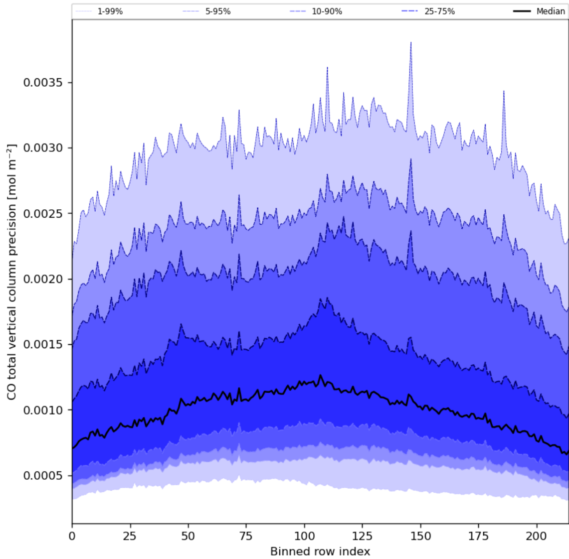
Figure 28: Along track statistics of “CO total vertical column precision” for 2023-07-30 to 2023-08-01
