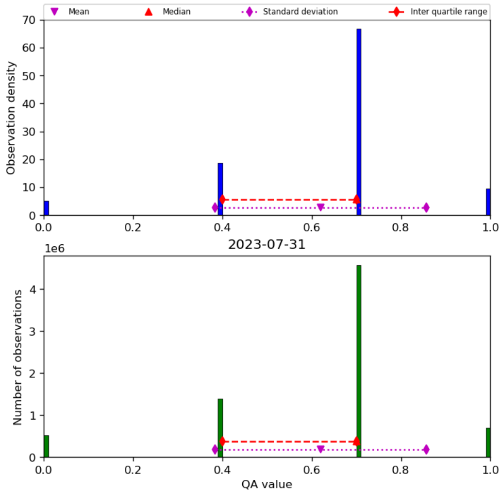
Figure 17: Histogram of “QA value” for 2023-07-30 to 2023-08-01
