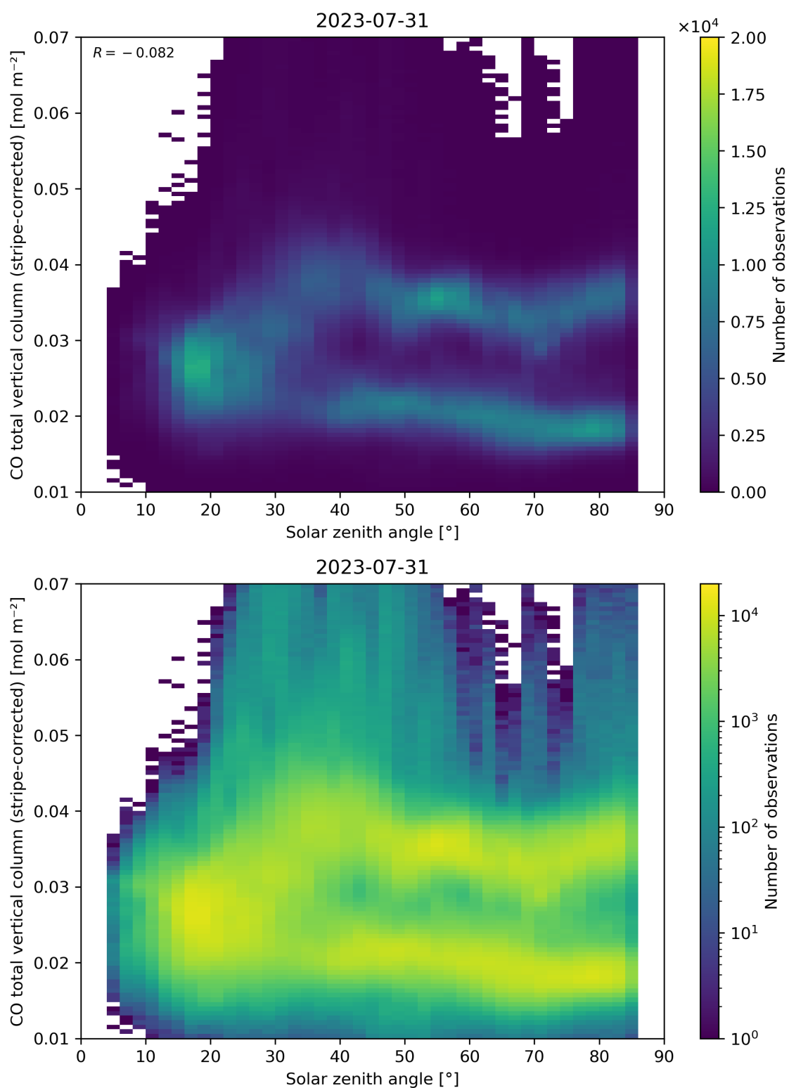
Figure 62: Scatter density plot of “Solar zenith angle” against “CO total vertical column (stripe-corrected)” for 2023-07-30 to 2023-08-01.
