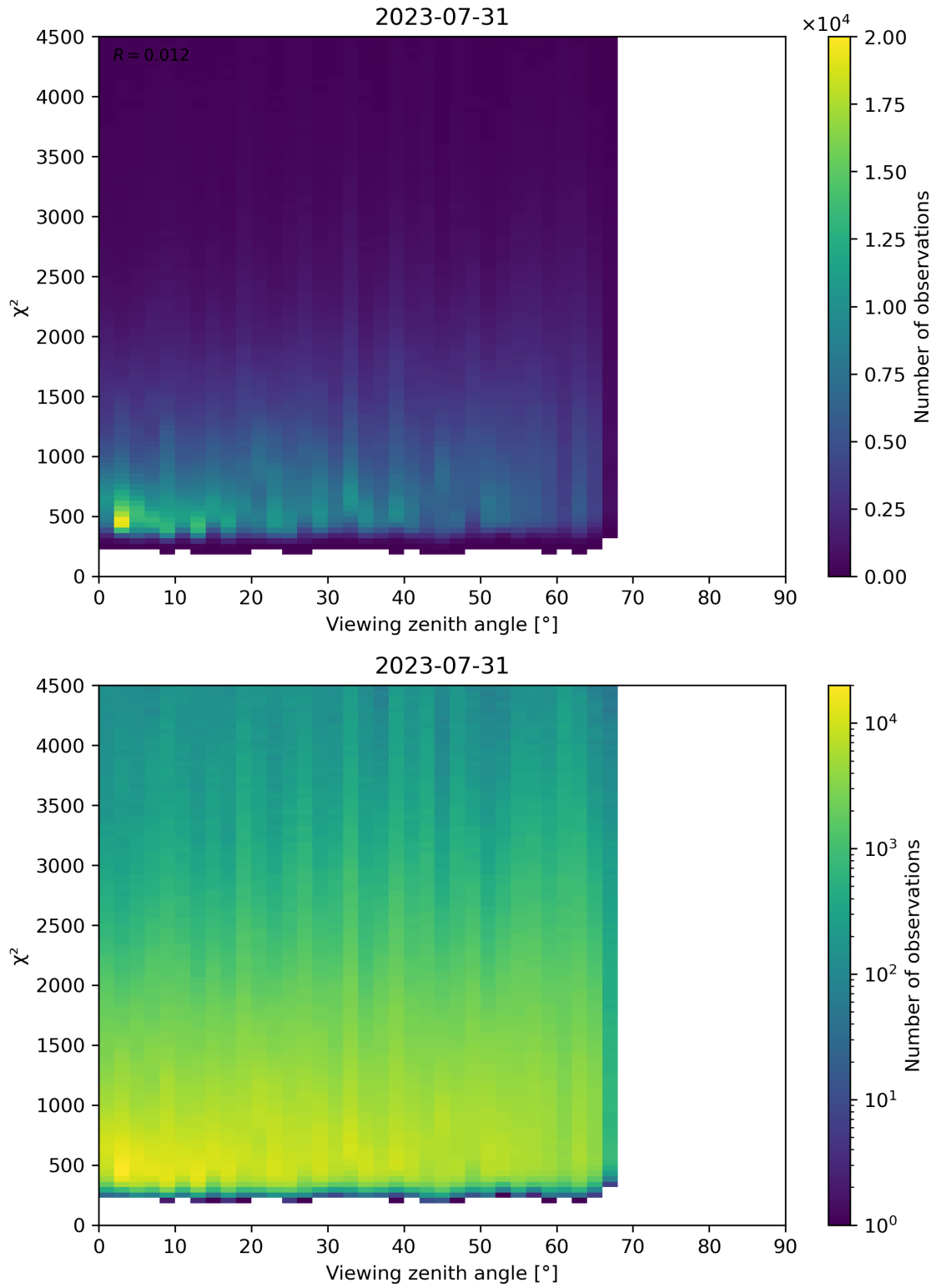
Figure 72: Scatter density plot of “Viewing zenith angle” against “ \chi^2 ” for 2023-07-30 to 2023-08-01.
