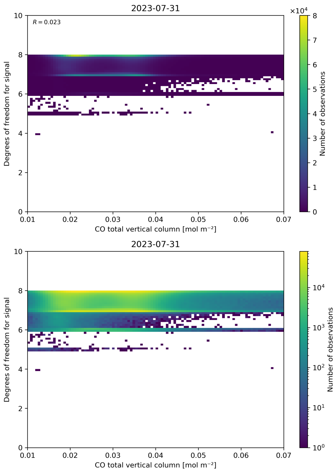
Figure 41: Scatter density plot of “CO total vertical column” against “Degrees of freedom for signal” for 2023-07-30 to 2023-08-01.
