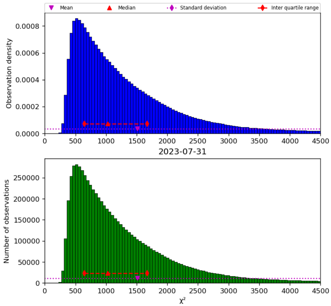
Figure 22: Histogram of " \chi^2 " for 2023-07-30 to 2023-08-01
