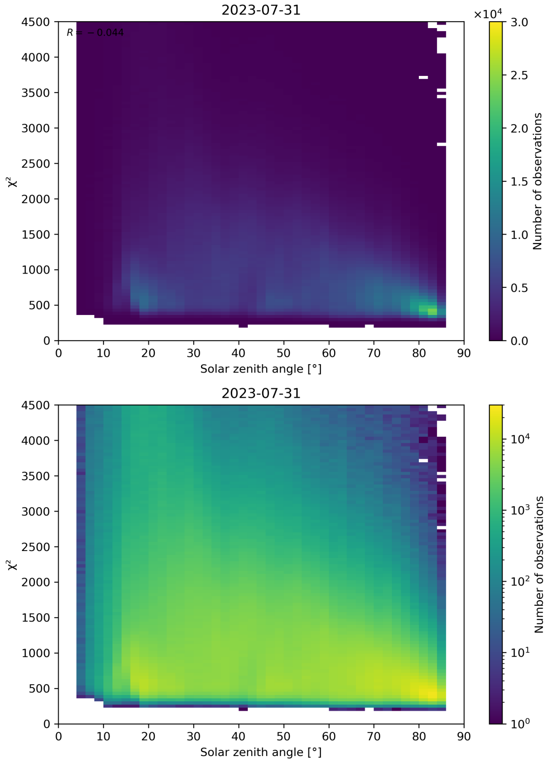
Figure 64: Scatter density plot of “Solar zenith angle” against “ \chi^2 ” for 2023-07-30 to 2023-08-01.
