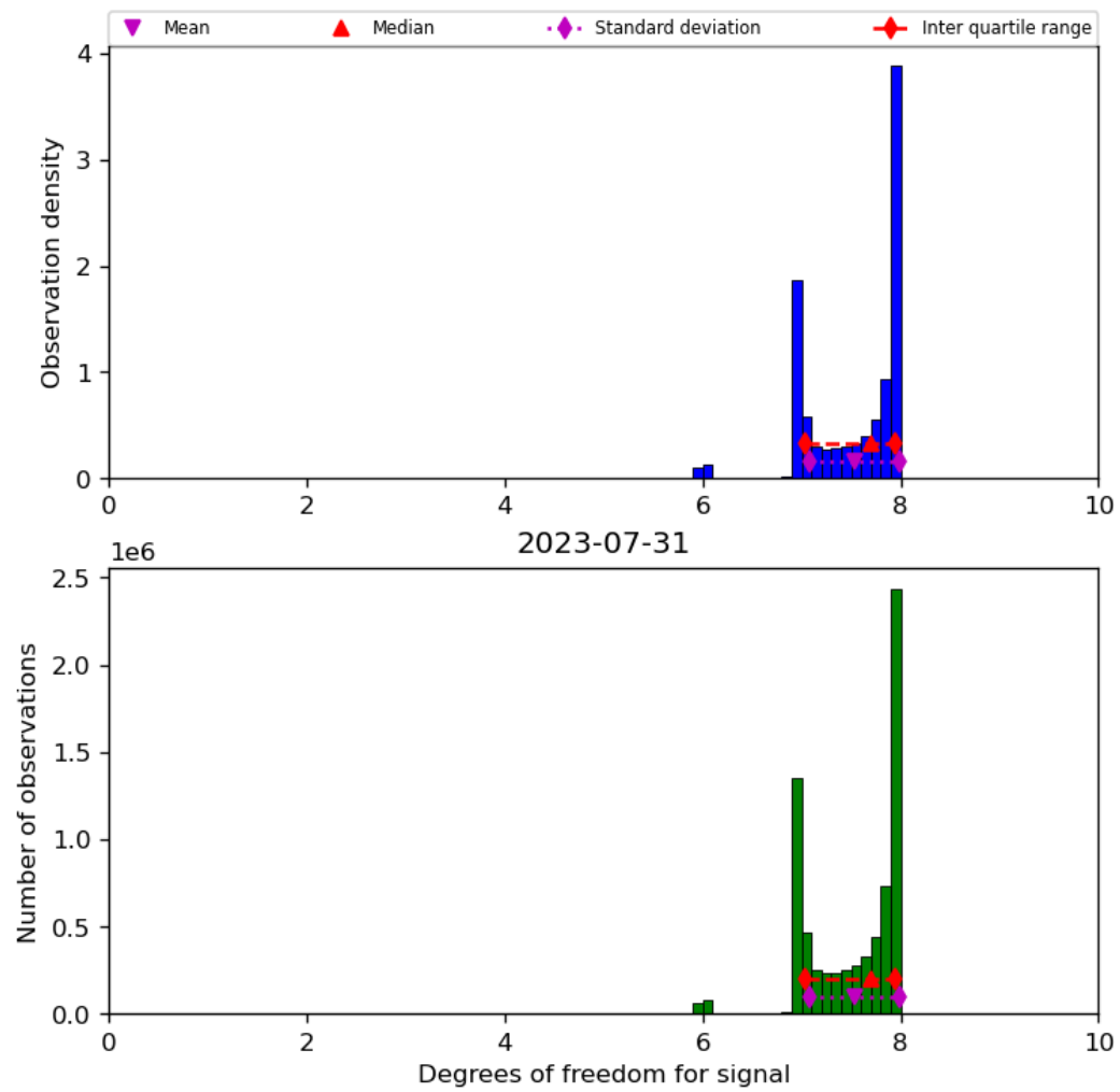
Figure 23: Histogram of “Degrees of freedom for signal” for 2023-07-30 to 2023-08-01
