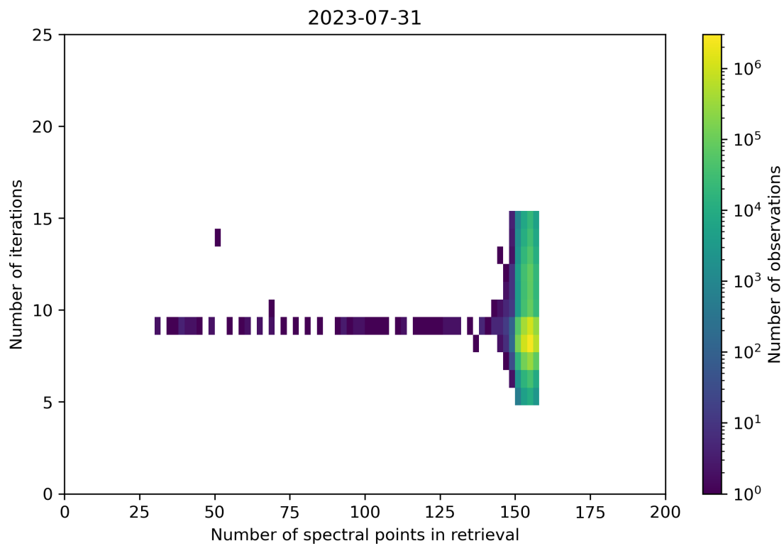
Figure 60: Scatter density plot of “Number of spectral points in retrieval” against “Number of iterations” for 2023-07-30 to 2023-08-01.
