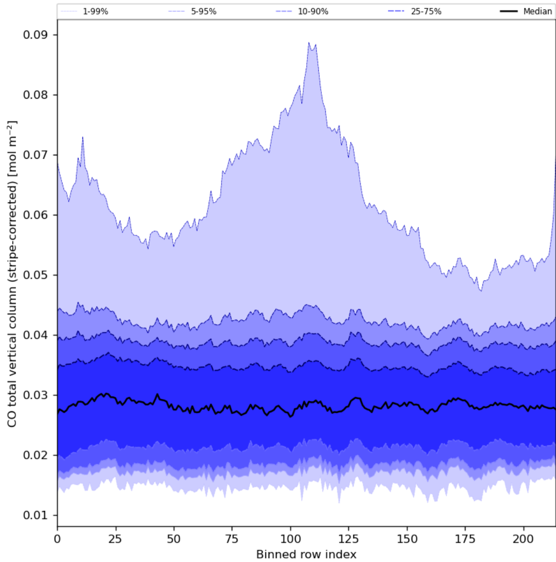
Figure 27: Along track statistics of “CO total vertical column (stripe-corrected)” for 2023-07-30 to 2023-08-01
