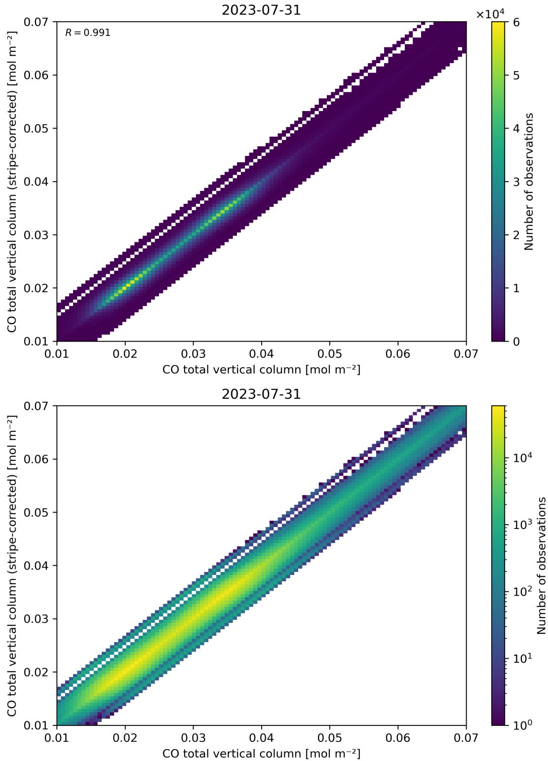
Figure 33: Scatter density plot of “CO total vertical column” against “CO total vertical column (stripe-corrected)” for 2023-07-30 to 2023-08-01.
