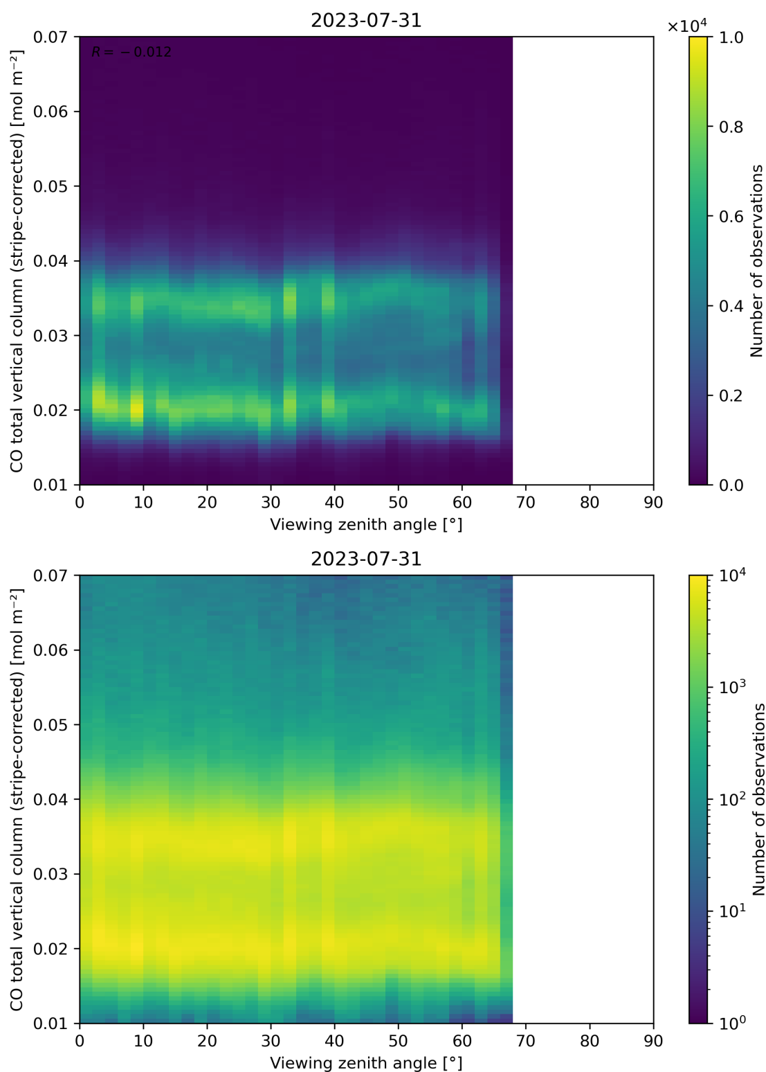
Figure 70: Scatter density plot of “Viewing zenith angle” against “CO total vertical column (stripe-corrected)” for 2023-07-30 to 2023-08-01.
