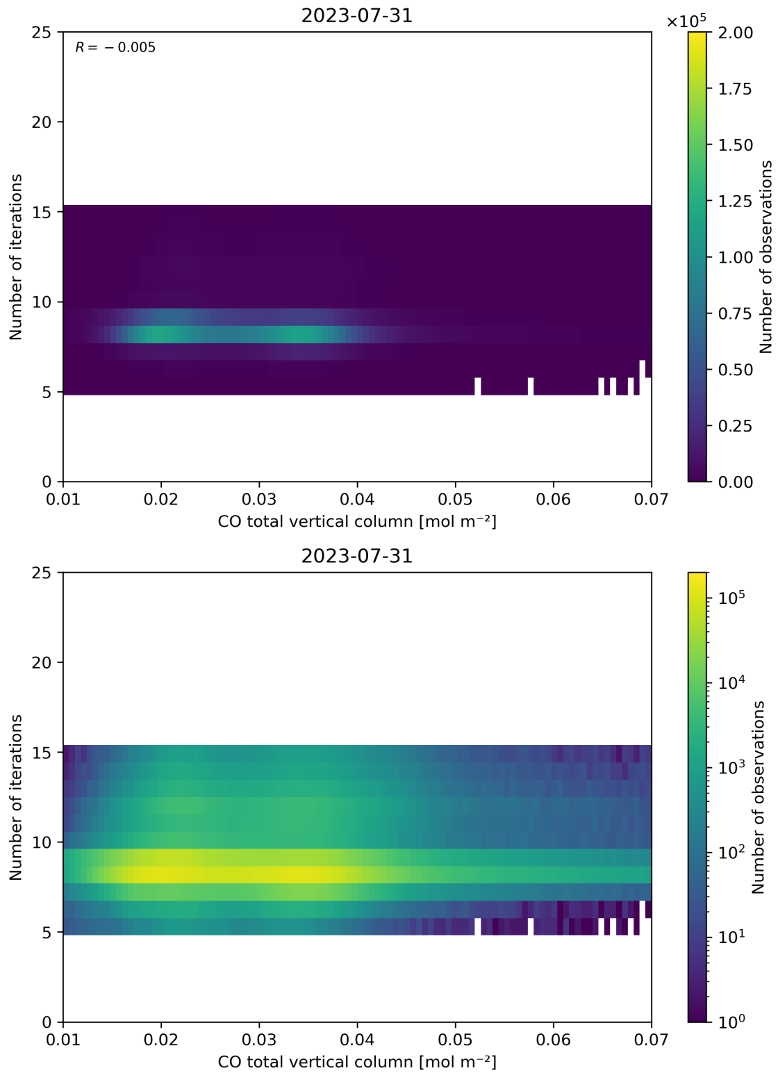
Figure 42: Scatter density plot of “CO total vertical column” against “Number of iterations” for 2023-07-30 to 2023-08-01.
