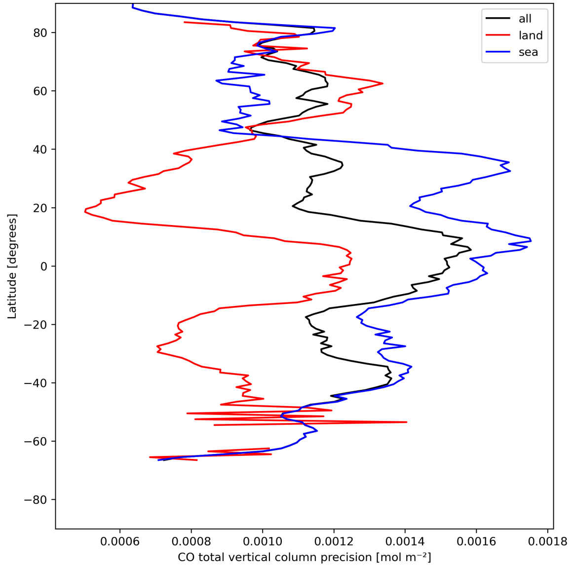
Figure 12: Zonal average of “CO total vertical column precision” for 2023-07-30 to 2023-08-01.
