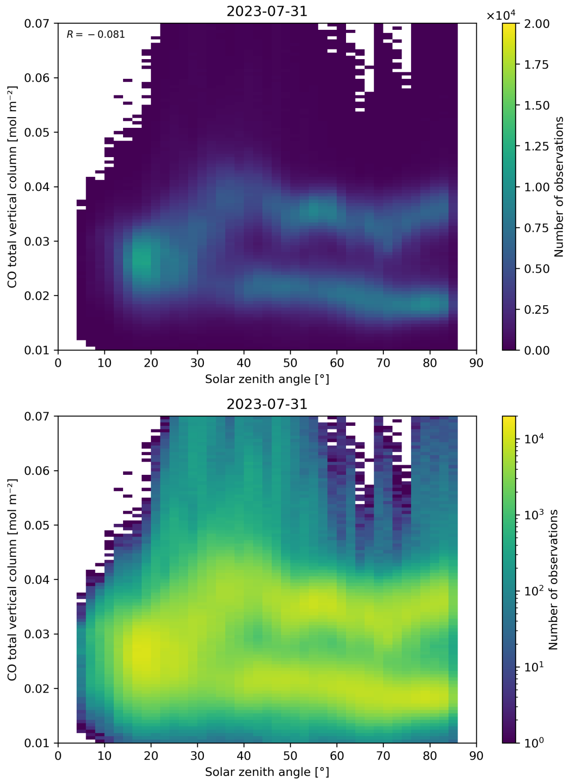
Figure 61: Scatter density plot of “Solar zenith angle” against “CO total vertical column” for 2023-07-30 to 2023-08-01.
