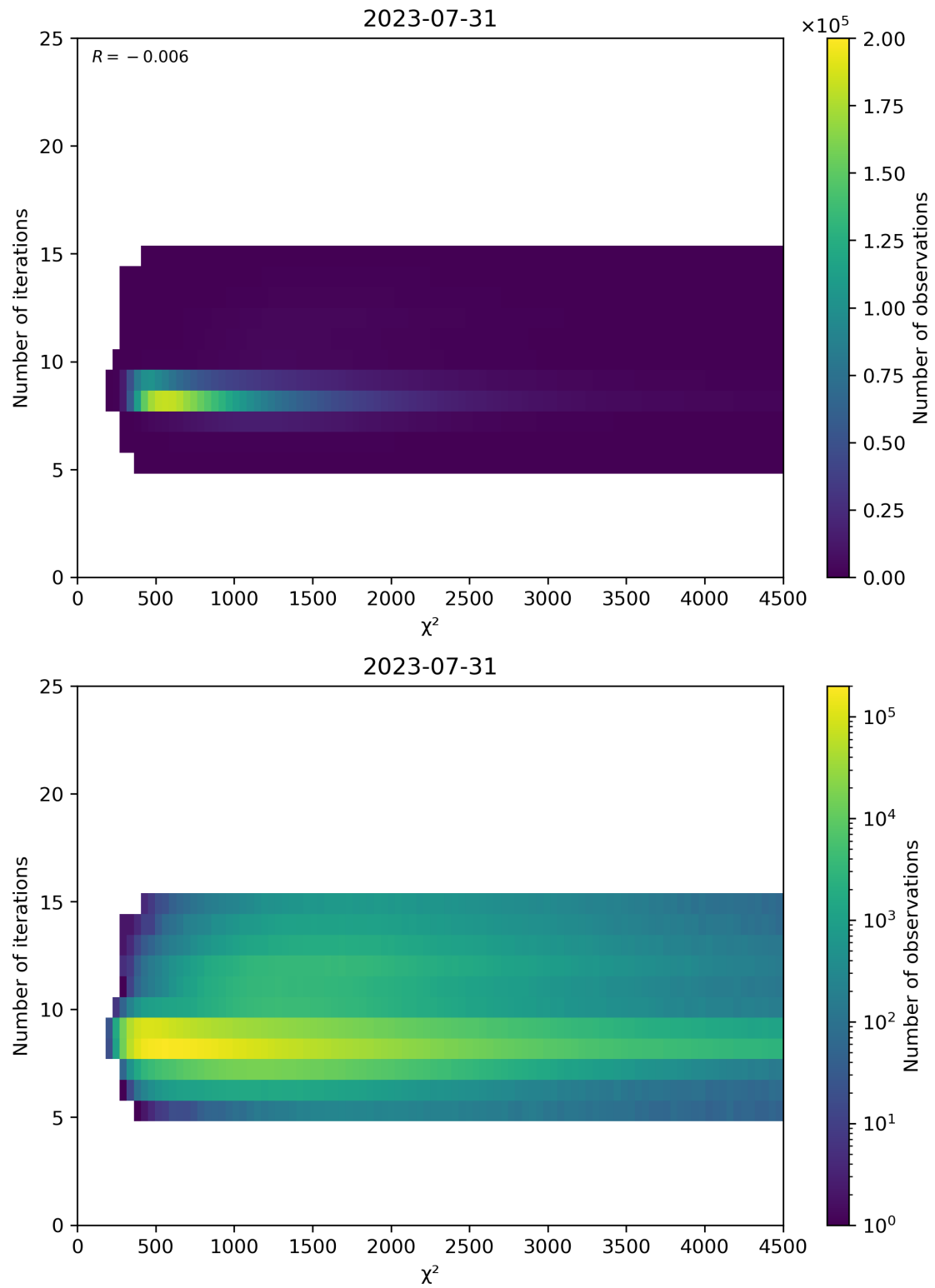
Figure 49: Scatter density plot of “ \chi^2 ” against “Number of iterations” for 2023-07-30 to 2023-08-01.
