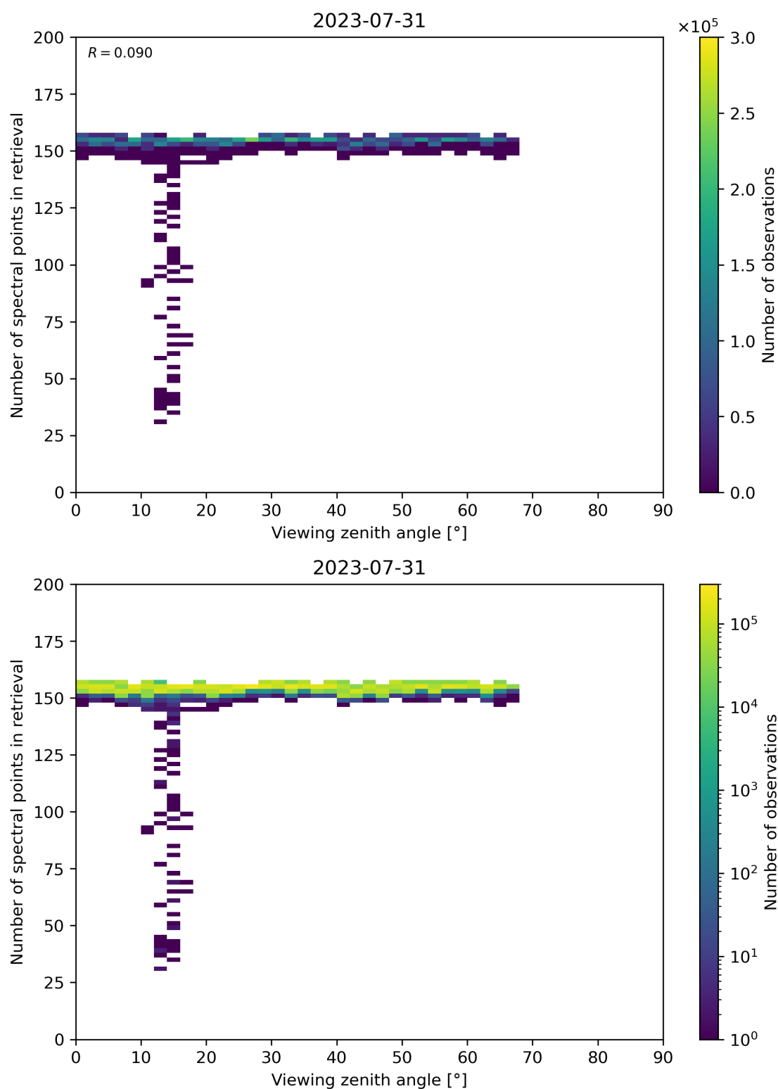
Figure 76: Scatter density plot of “Viewing zenith angle” against “Number of spectral points in retrieval” for 2023-07-30 to 2023-08-01.
