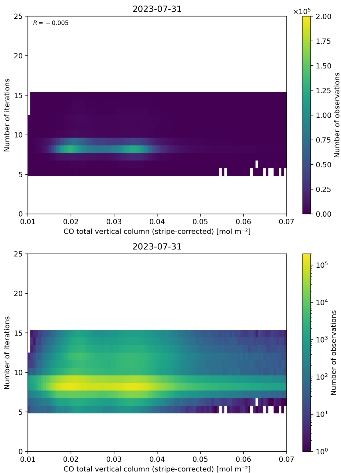
Figure 39: Scatter density plot of “CO total vertical column (stripe-corrected)” against “Number of iterations” for 2023-07-30 to 2023-08-01.
