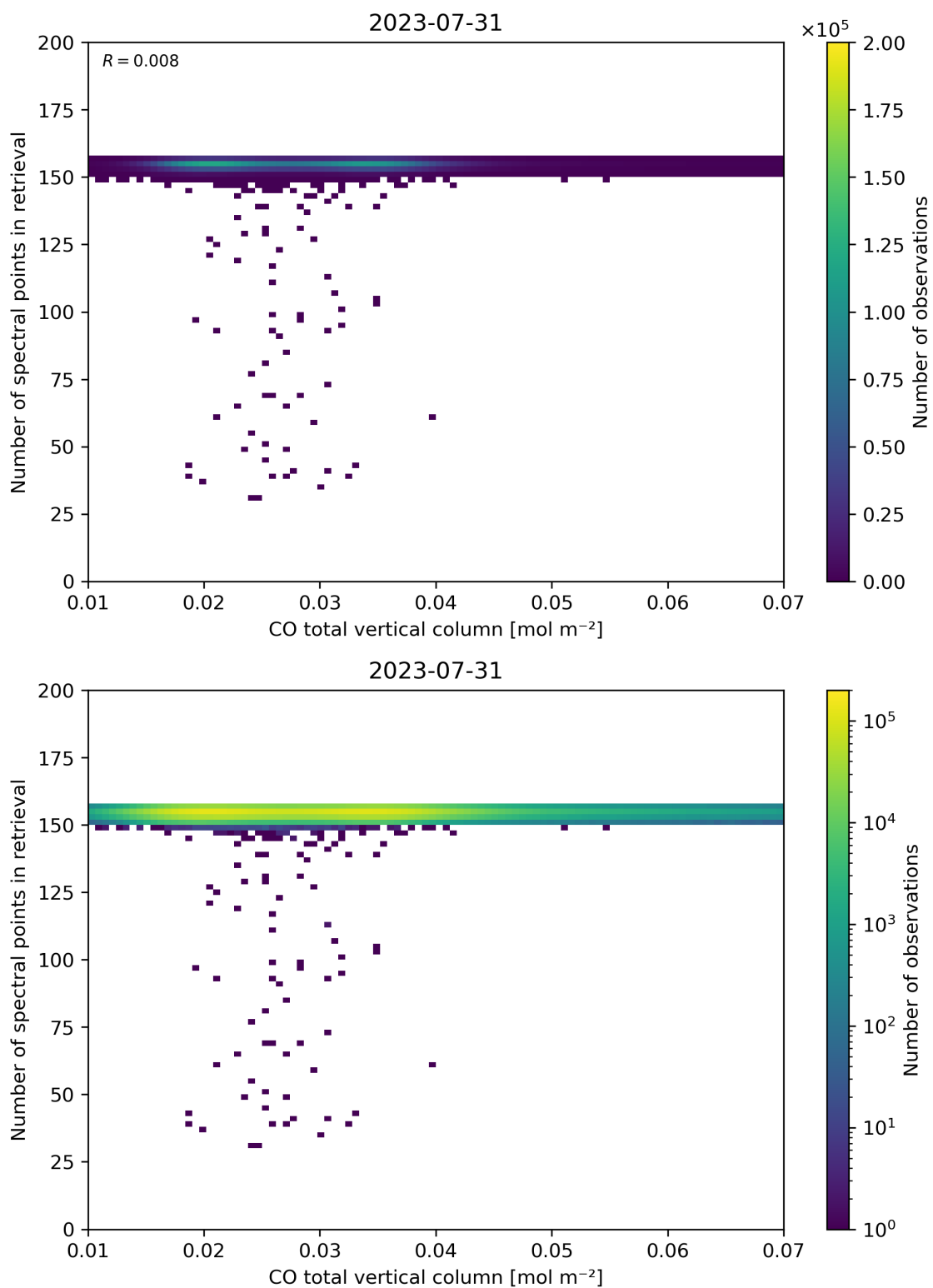
Figure 43: Scatter density plot of “CO total vertical column” against “Number of spectral points in retrieval” for 2023-07-30 to 2023-08-01.
