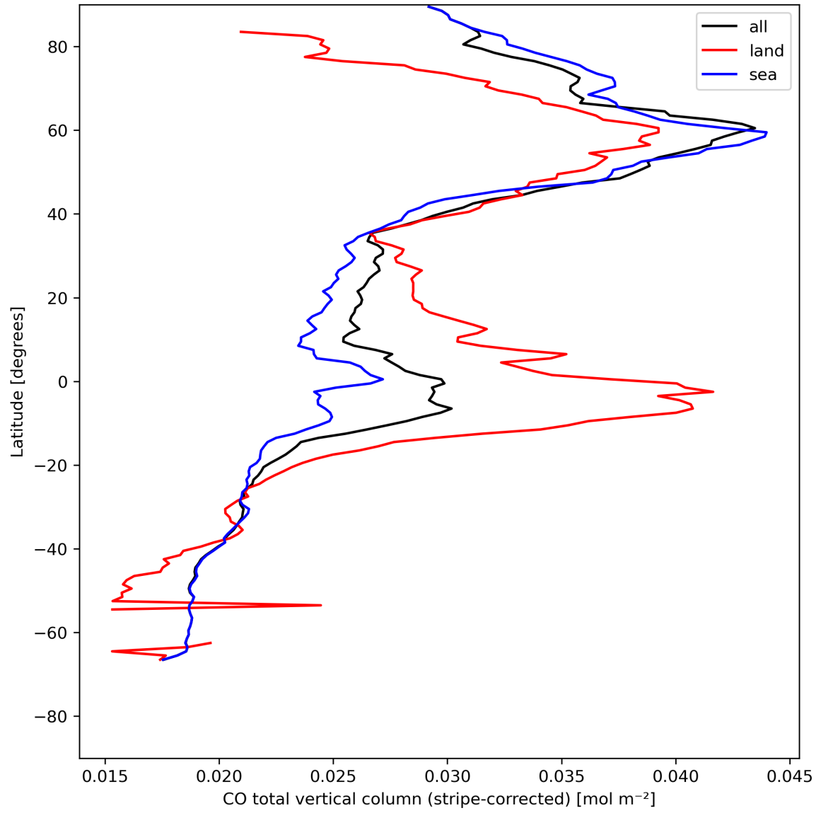
Figure 11: Zonal average of “CO total vertical column (stripe-corrected)” for 2023-07-30 to 2023-08-01.
