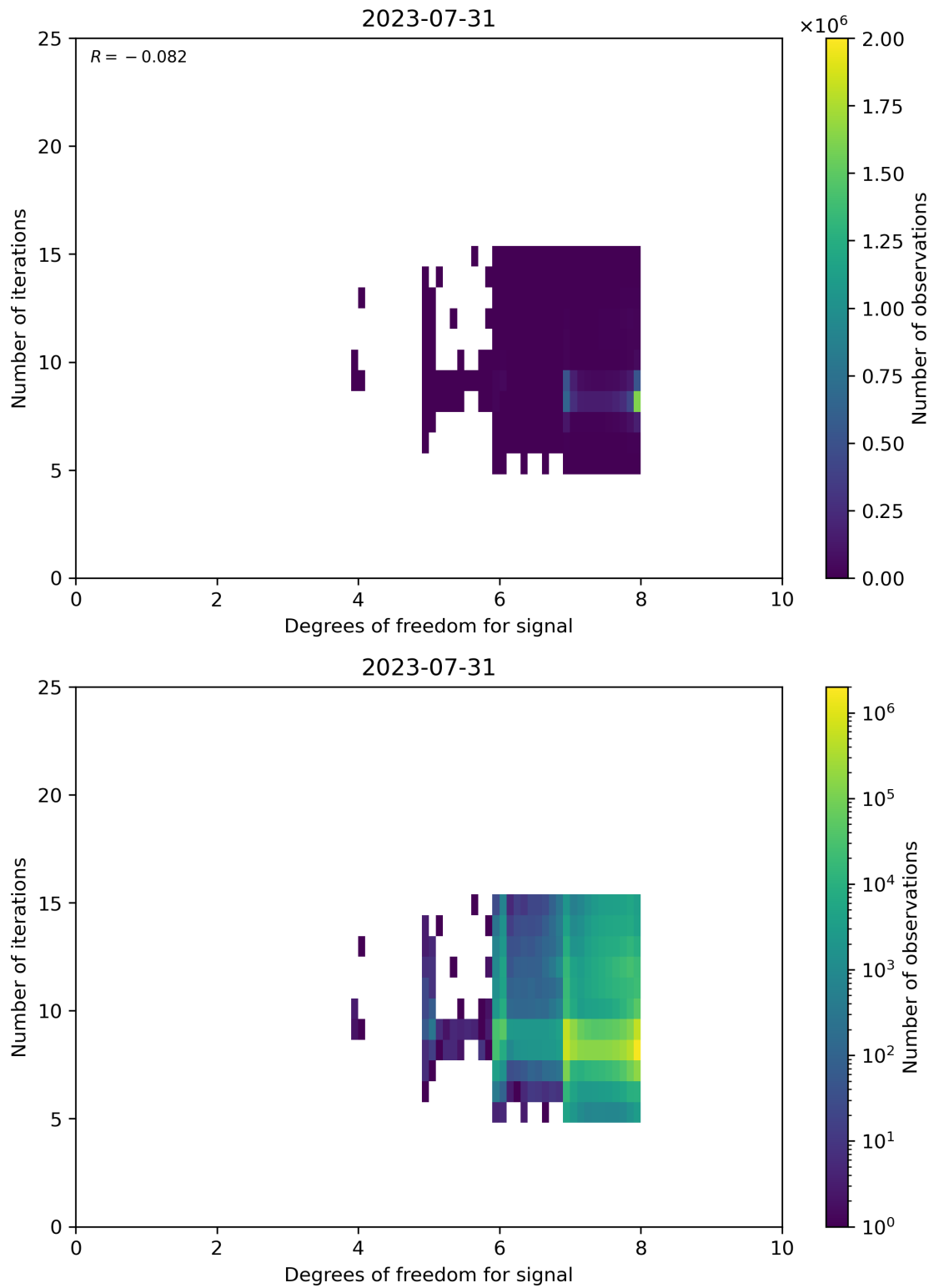
Figure 50: Scatter density plot of “Degrees of freedom for signal” against “Number of iterations” for 2023-07-30 to 2023-08-01.
