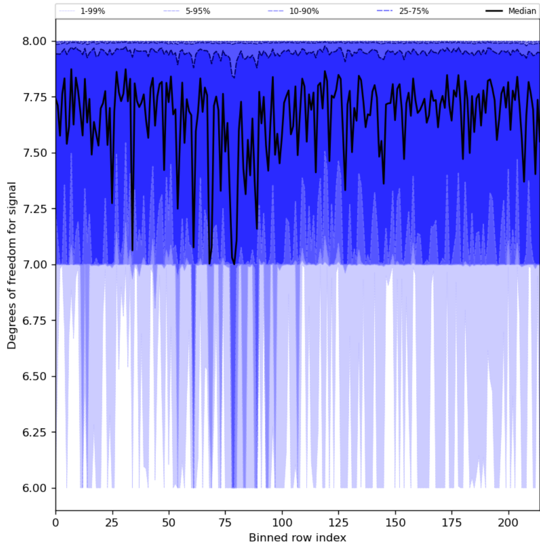
Figure 31: Along track statistics of “Degrees of freedom for signal” for 2023-07-30 to 2023-08-01
