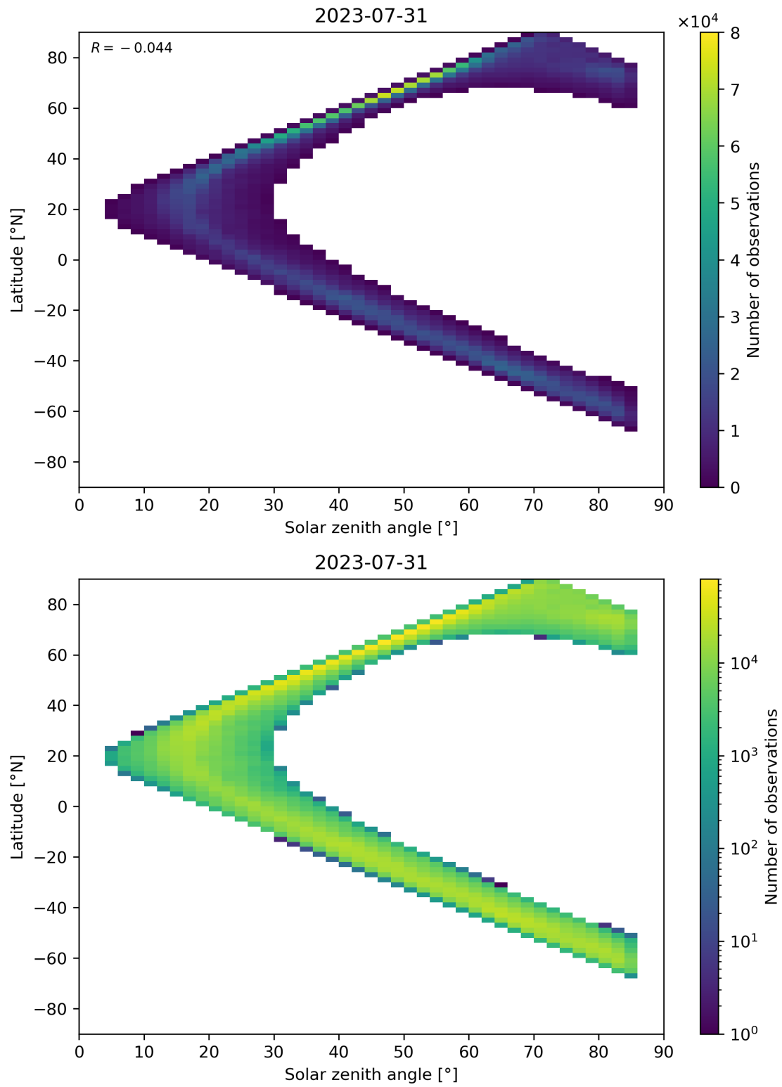
Figure 66: Scatter density plot of “Solar zenith angle” against “Latitude” for 2023-07-30 to 2023-08-01.
