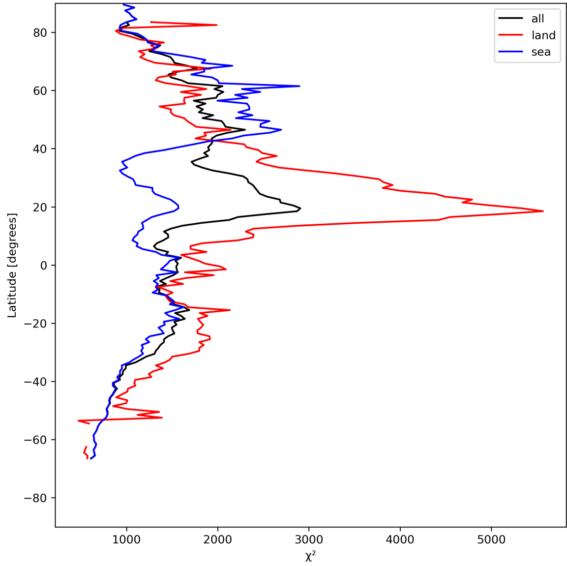
Figure 14: Zonal average of “ \chi^2 ” for 2023-07-30 to 2023-08-01.
