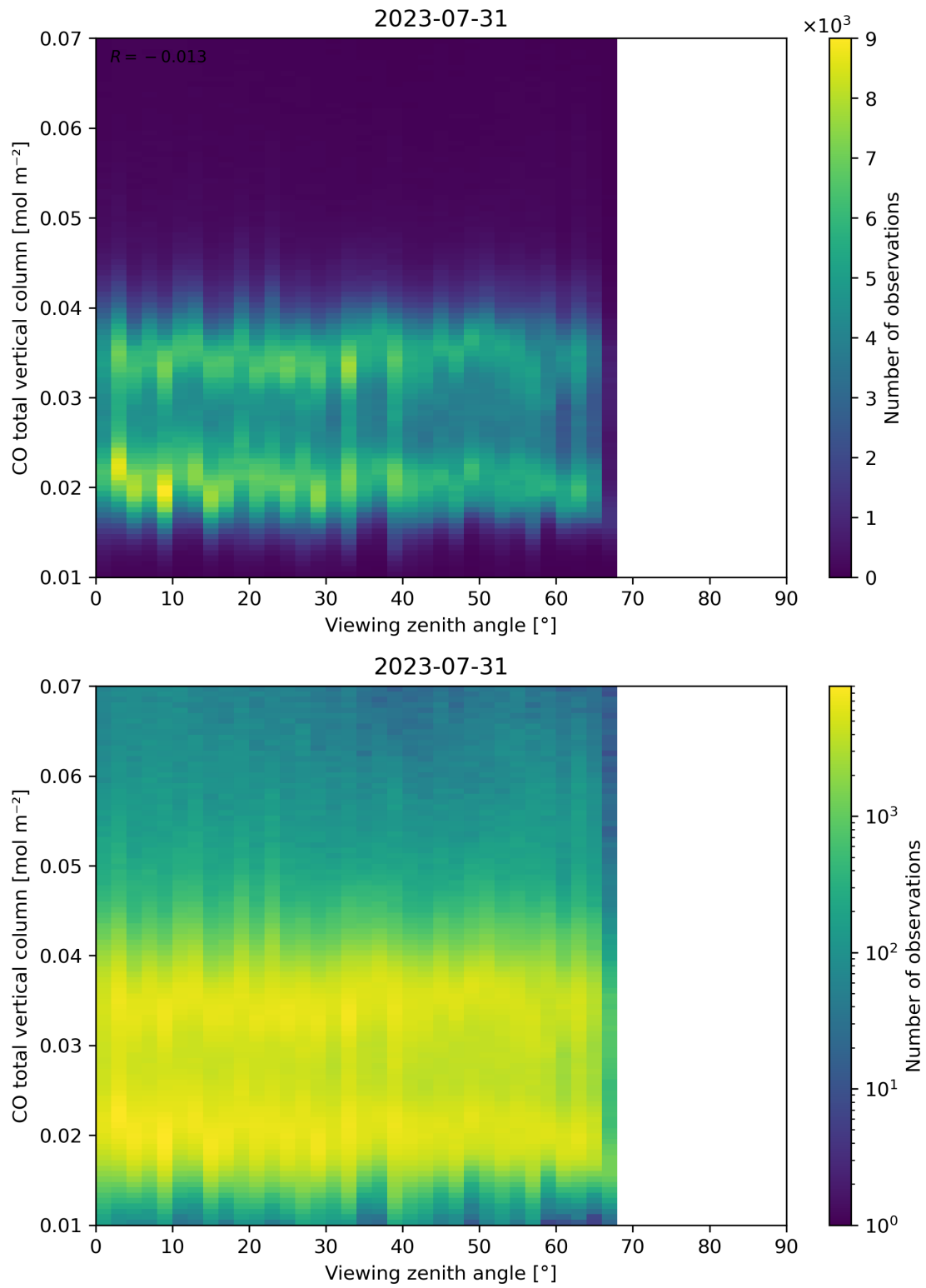
Figure 69: Scatter density plot of “Viewing zenith angle” against “CO total vertical column” for 2023-07-30 to 2023-08-01.
