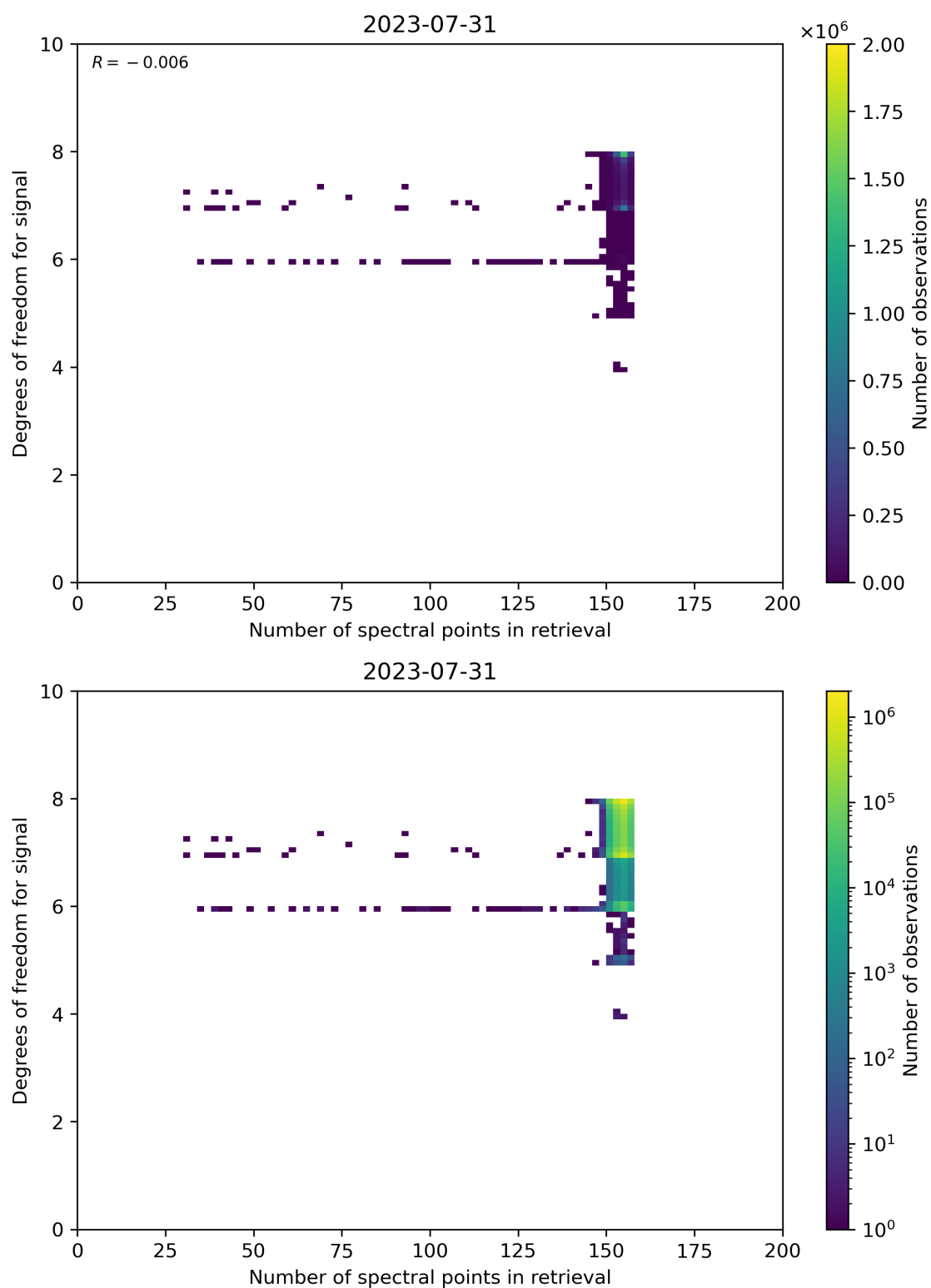
Figure 59: Scatter density plot of “Number of spectral points in retrieval” against “Degrees of freedom for signal” for 2023-07-30 to 2023-08-01.
