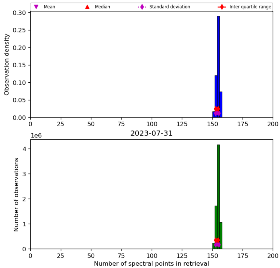
Figure 21: Histogram of “Number of spectral points in retrieval” for 2023-07-30 to 2023-08-01
