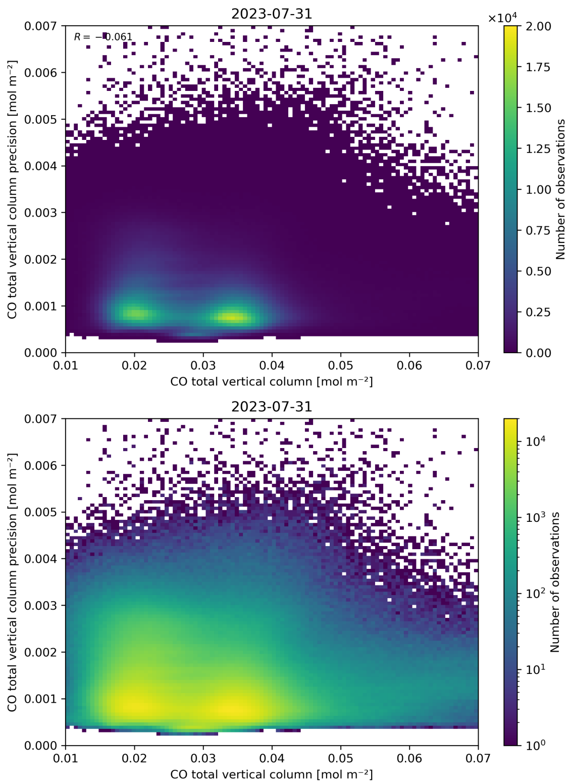
Figure 34: Scatter density plot of “CO total vertical column” against “CO total vertical column precision” for 2023-07-30 to 2023-08-01.
