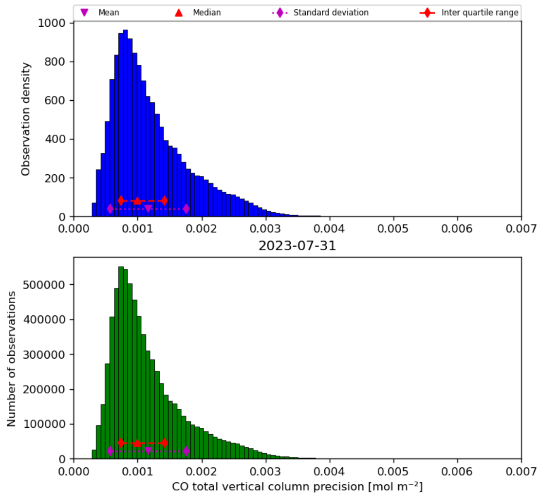
Figure 20: Histogram of “CO total vertical column precision” for 2023-07-30 to 2023-08-01
