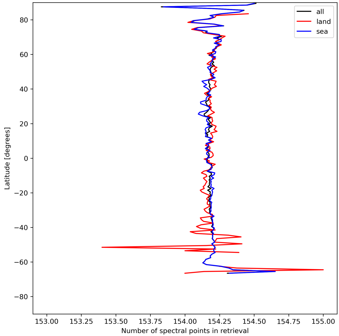
Figure 13: Zonal average of “Number of spectral points in retrieval” for 2023-07-30 to 2023-08-01.
