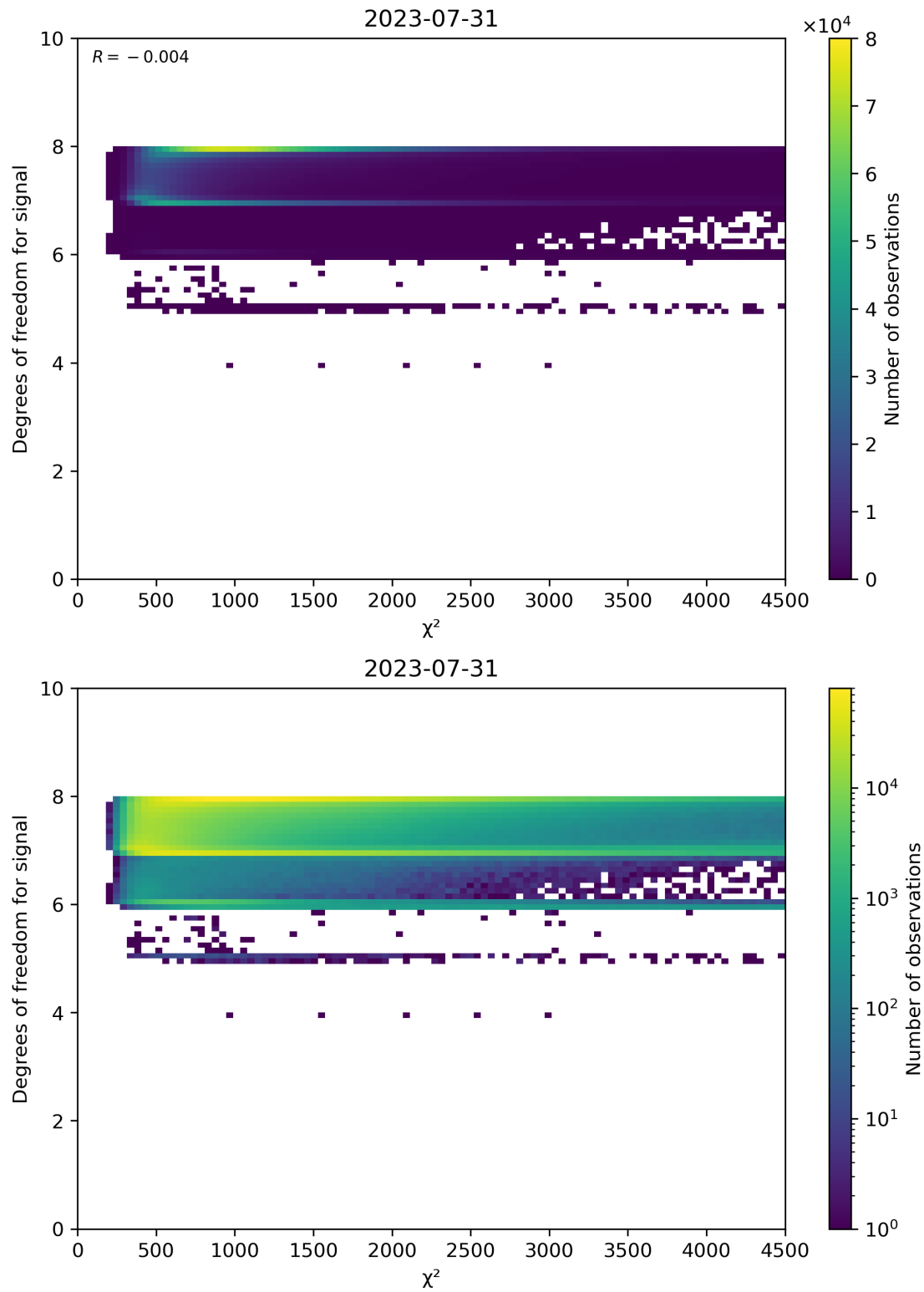
Figure 48: Scatter density plot of " \chi^2 " against "Degrees of freedom for signal" for 2023-07-30 to 2023-08-01.
