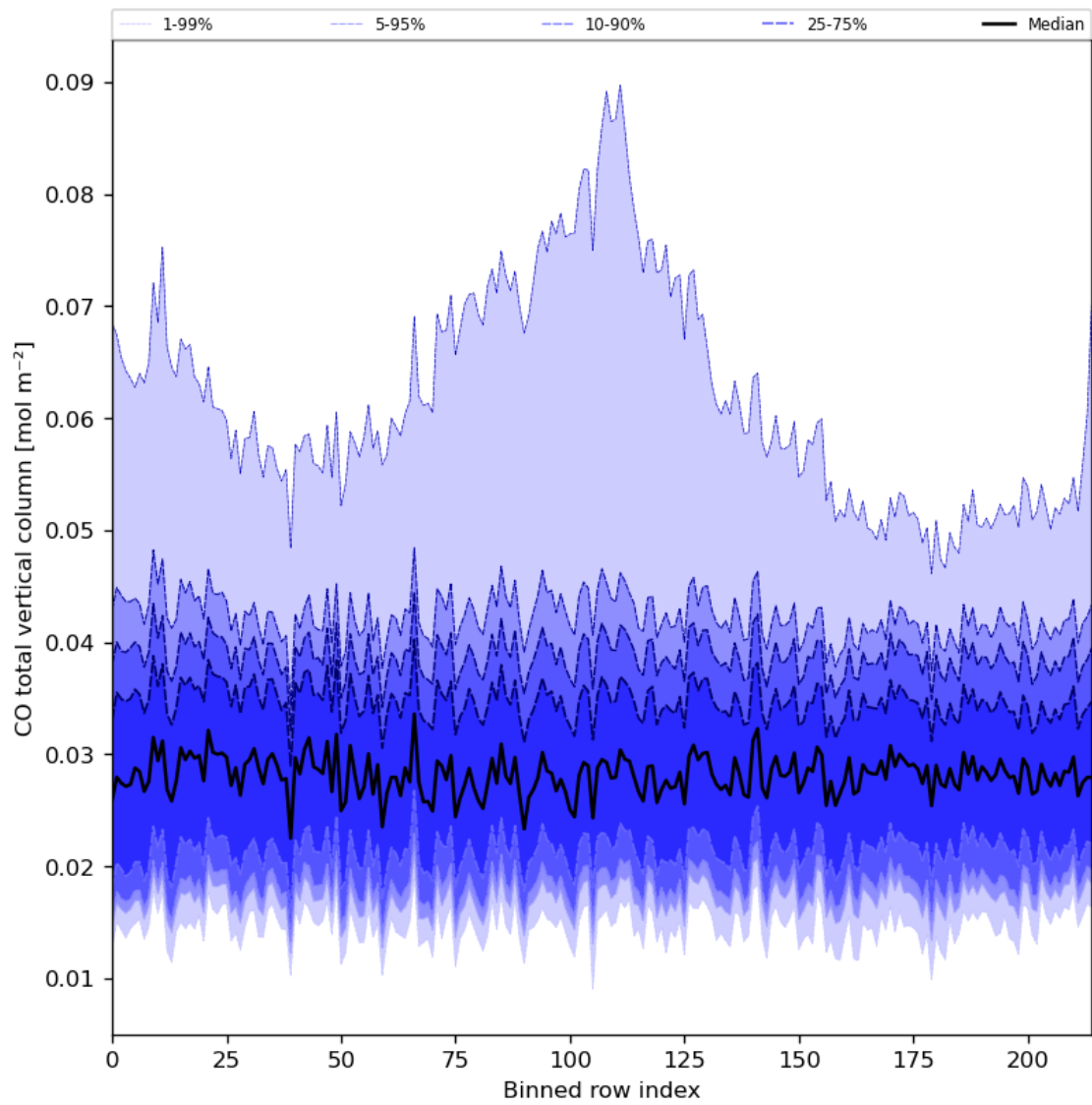
Figure 26: Along track statistics of “CO total vertical column” for 2023-07-30 to 2023-08-01
