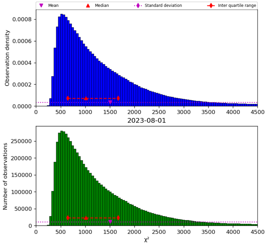
Figure 22: Histogram of “ \chi^2 ” for 2023-07-31 to 2023-08-02
