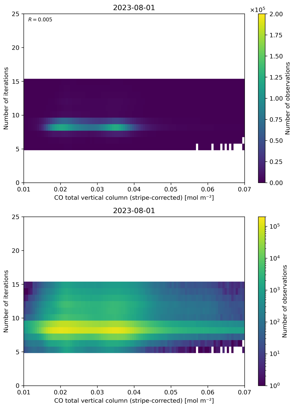
Figure 39: Scatter density plot of “CO total vertical column (stripe-corrected)” against “Number of iterations” for 2023-07-31 to 2023-08-02.
