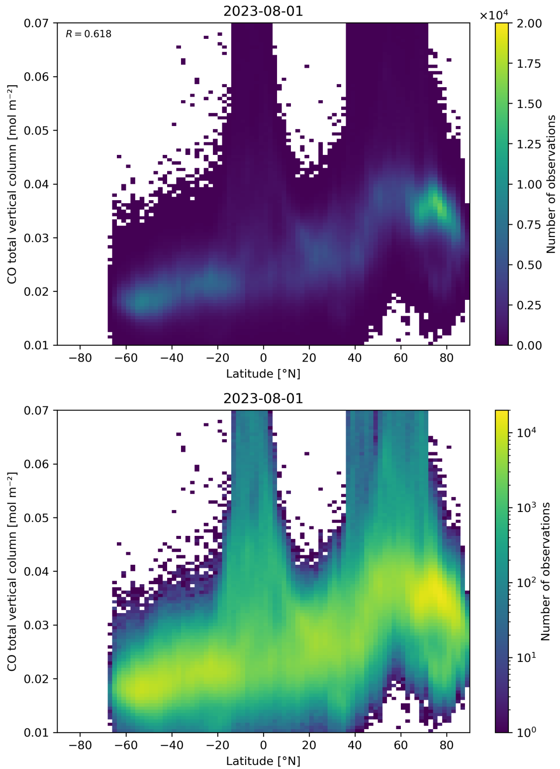
Figure 51: Scatter density plot of “Latitude” against “CO total vertical column” for 2023-07-31 to 2023-08-02.
