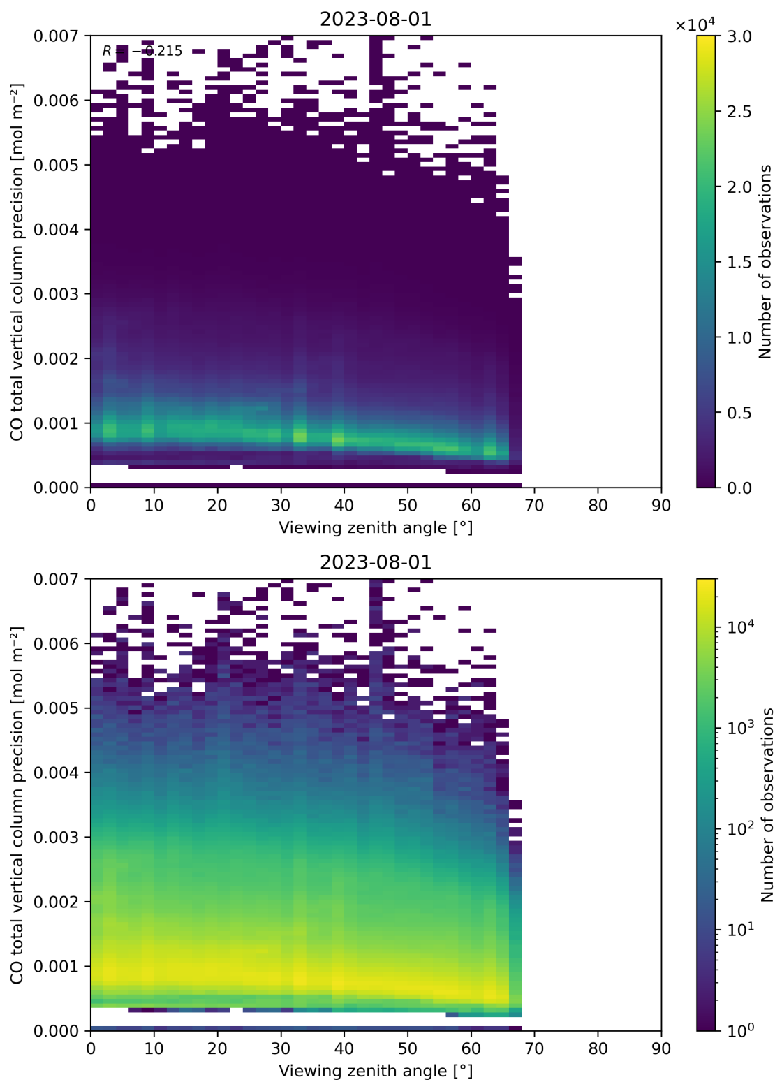
Figure 71: Scatter density plot of “Viewing zenith angle” against “CO total vertical column precision” for 2023-07-31 to 2023-08-02.
