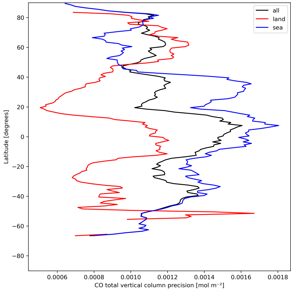
Figure 12: Zonal average of “CO total vertical column precision” for 2023-07-31 to 2023-08-02.
