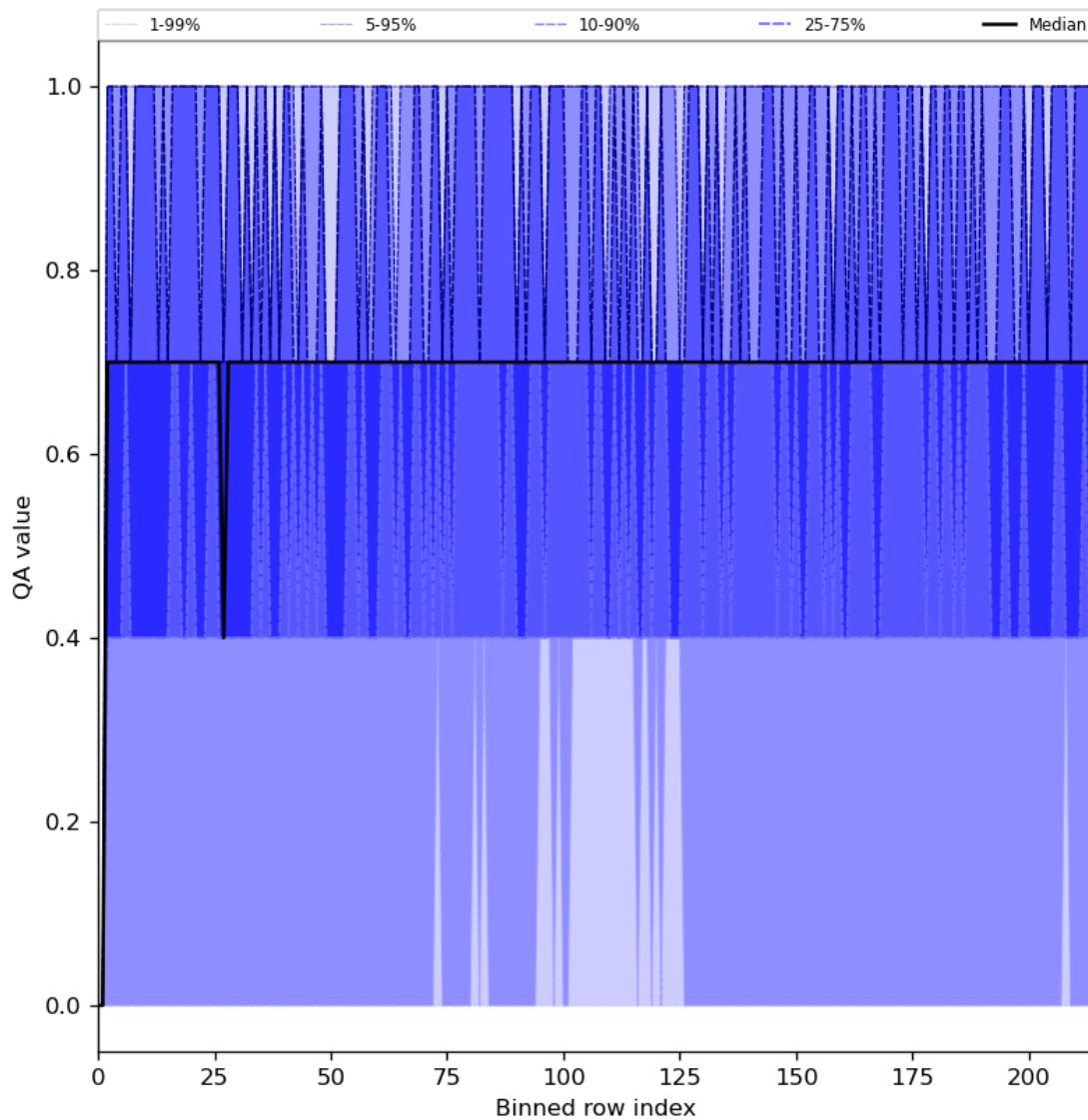
Figure 25: Along track statistics of “QA value” for 2023-07-31 to 2023-08-02
