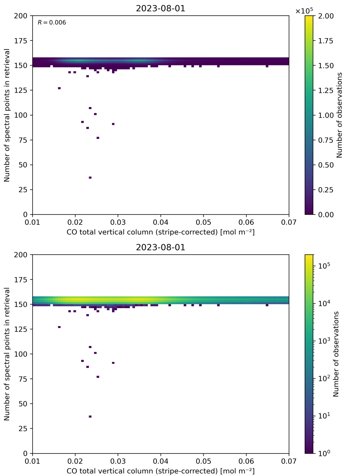
Figure 40: Scatter density plot of “CO total vertical column (stripe-corrected)” against “Number of spectral points in retrieval” for 2023-07-31 to 2023-08-02.
