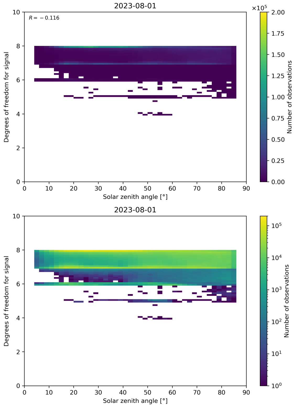
Figure 65: Scatter density plot of “Solar zenith angle” against “Degrees of freedom for signal” for 2023-07-31 to 2023-08-02.
