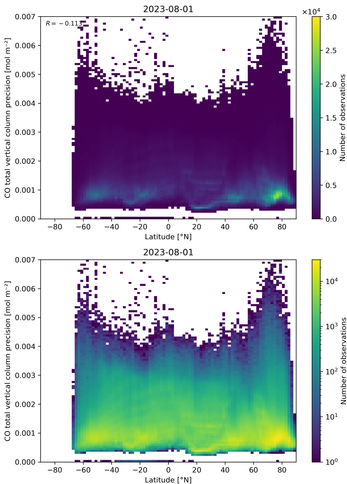
Figure 53: Scatter density plot of “Latitude” against “CO total vertical column precision” for 2023-07-31 to 2023-08-02.
