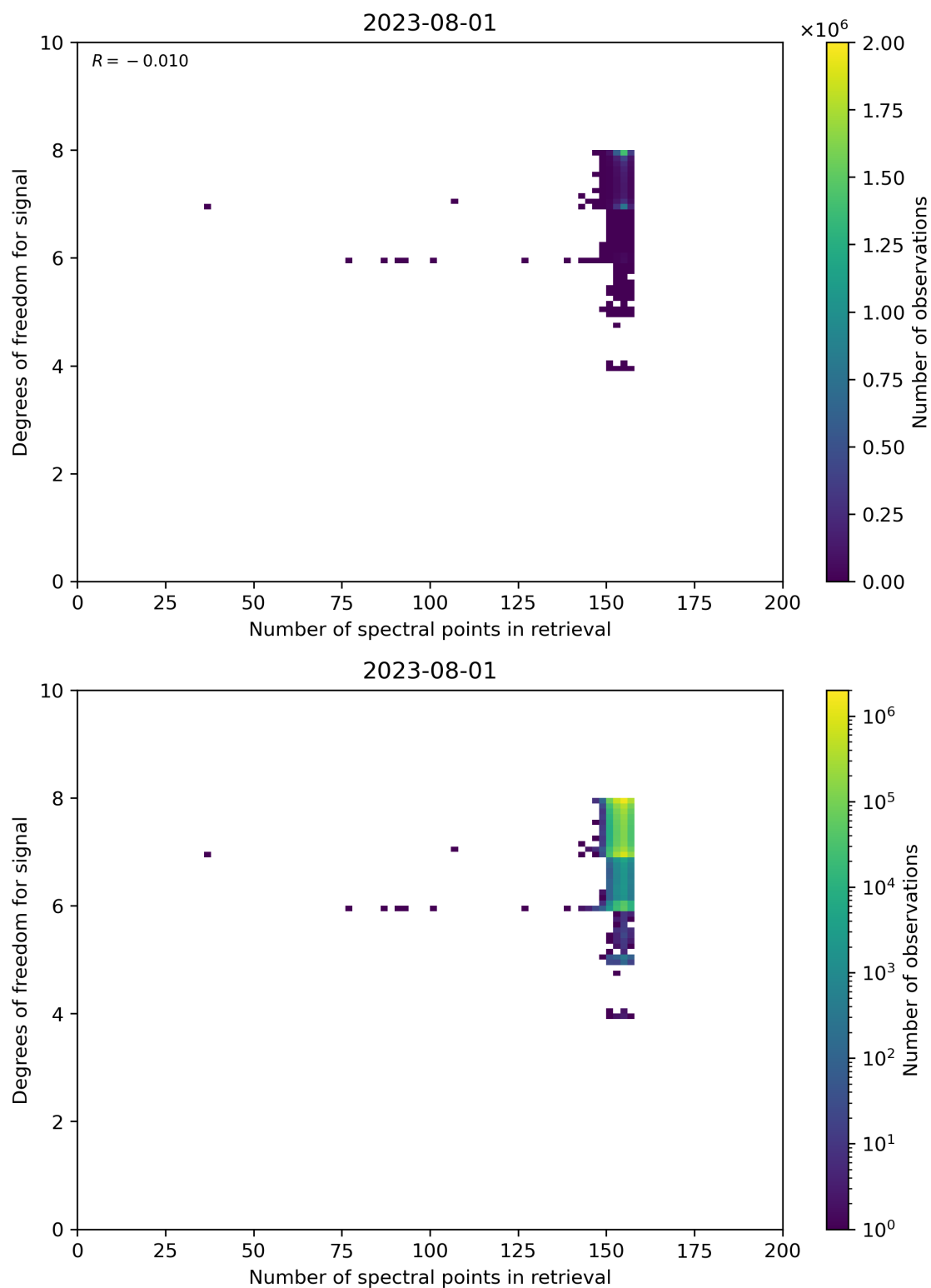
Figure 59: Scatter density plot of “Number of spectral points in retrieval” against “Degrees of freedom for signal” for 2023-07-31 to 2023-08-02.
