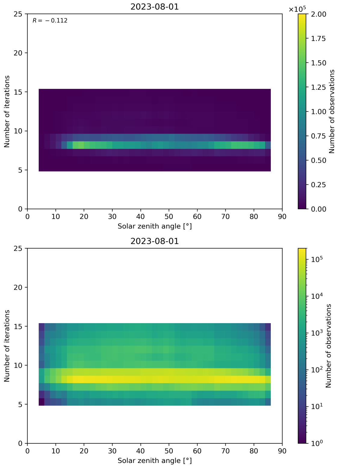
Figure 67: Scatter density plot of “Solar zenith angle” against “Number of iterations” for 2023-07-31 to 2023-08-02.
