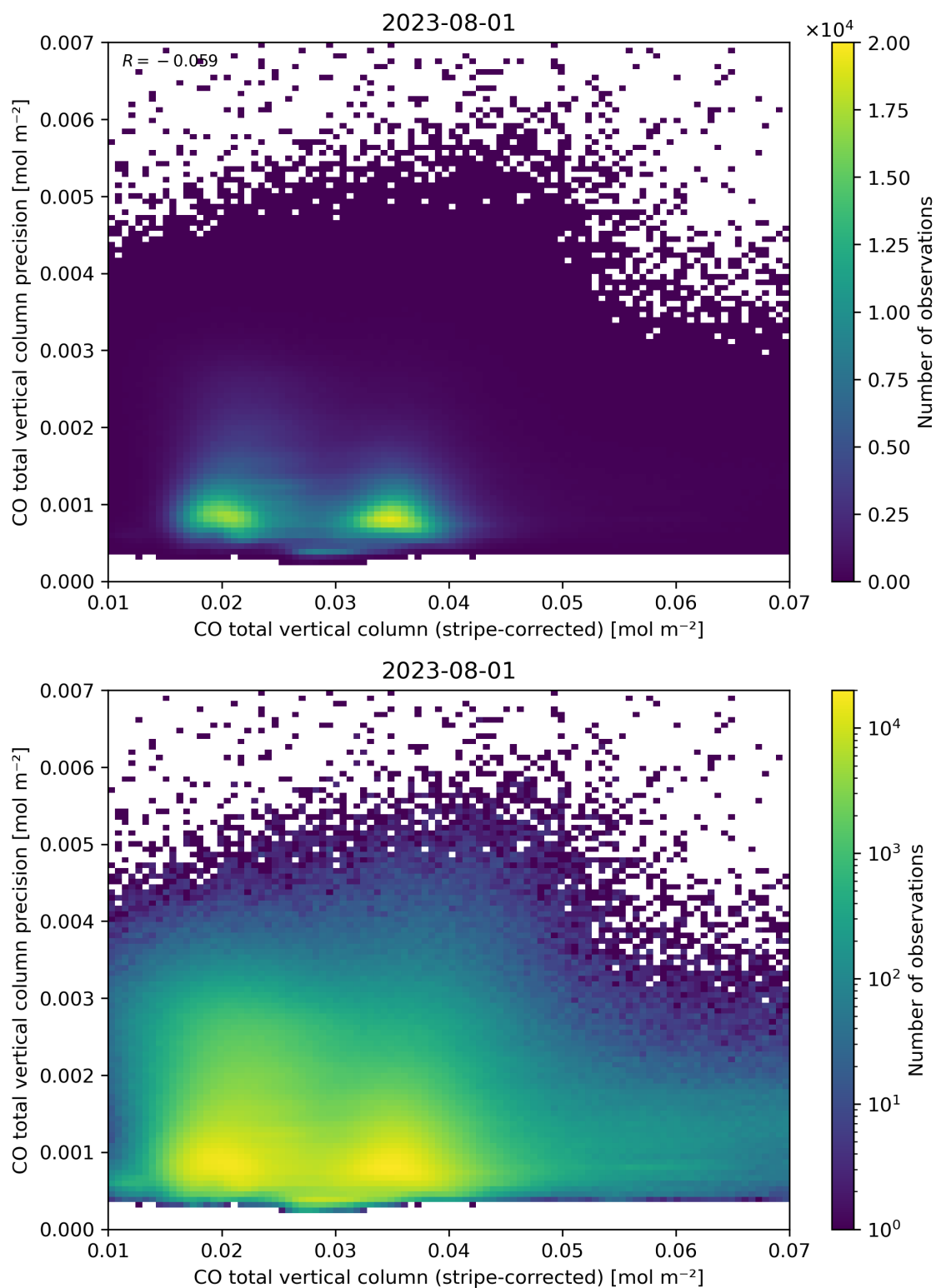
Figure 36: Scatter density plot of “CO total vertical column (stripe-corrected)” against “CO total vertical column precision” for 2023-07-31 to 2023-08-02.
