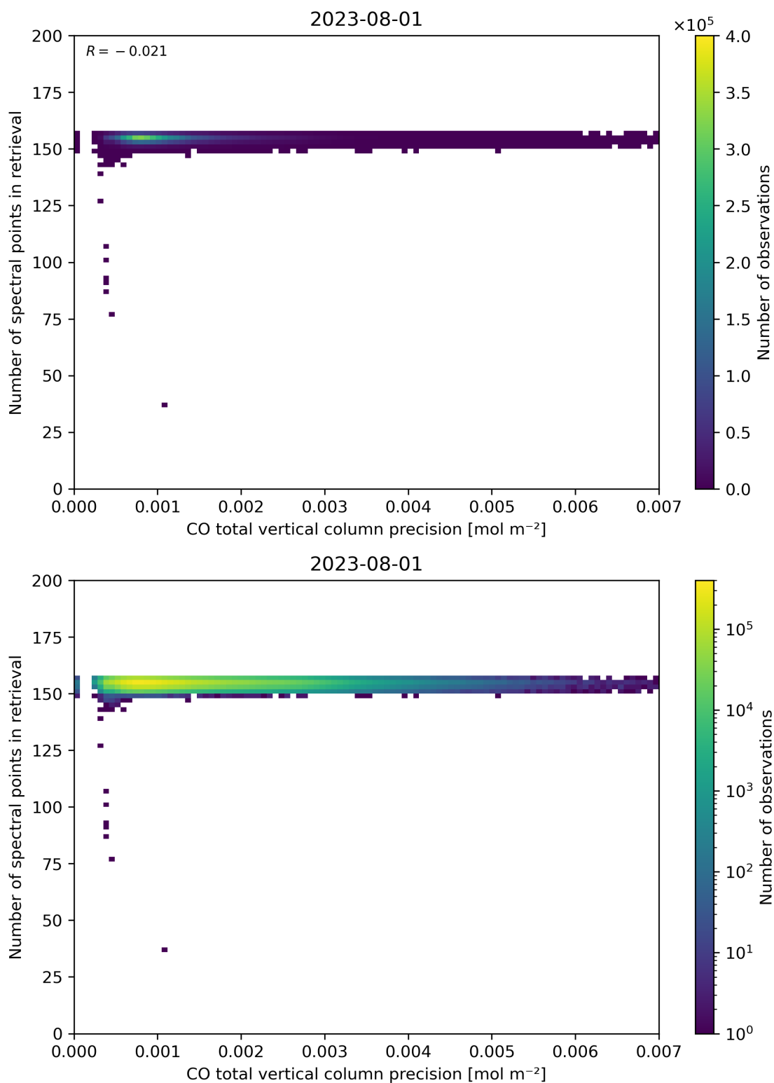
Figure 47: Scatter density plot of “CO total vertical column precision” against “Number of spectral points in retrieval” for 2023-07-31 to 2023-08-02.
