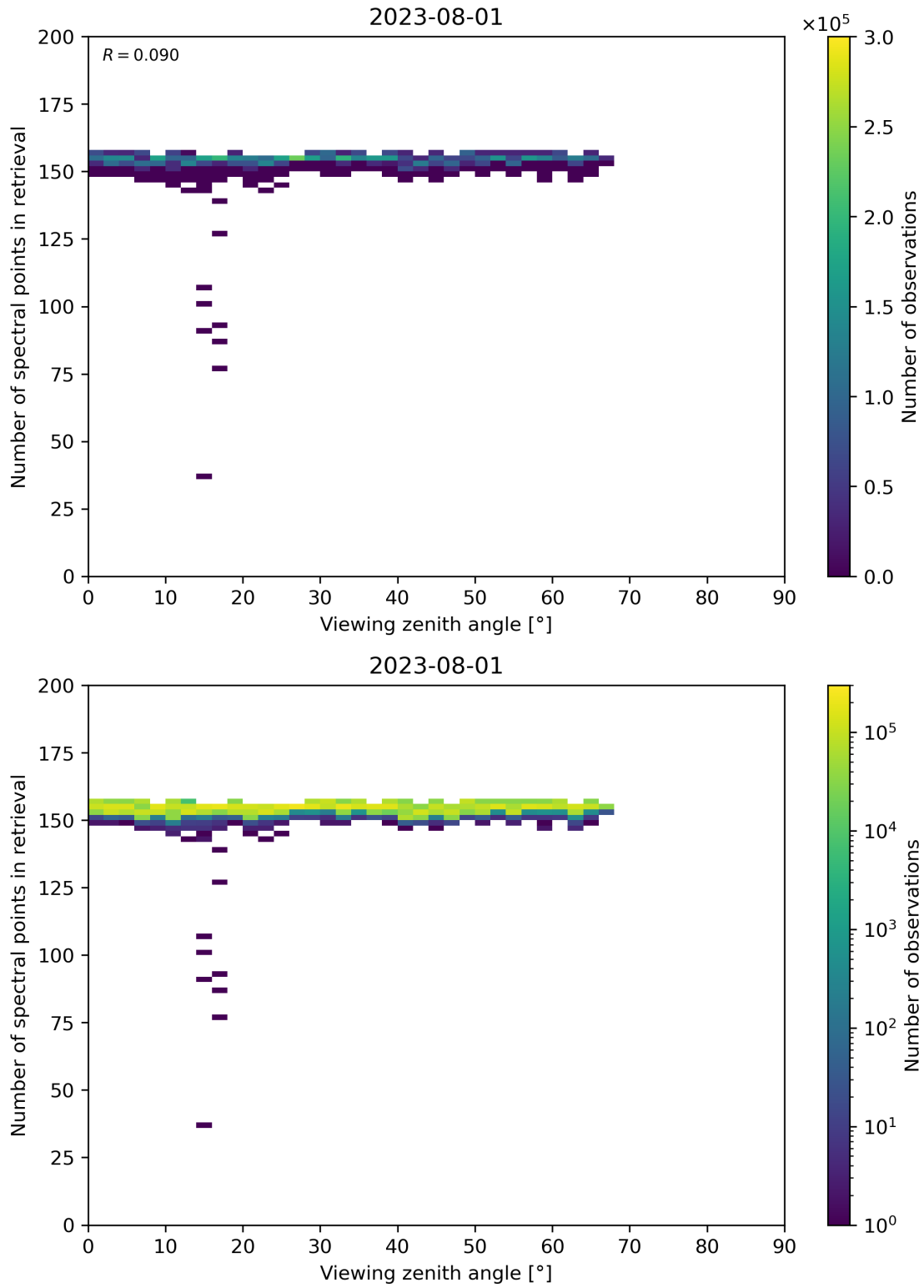
Figure 76: Scatter density plot of “Viewing zenith angle” against “Number of spectral points in retrieval” for 2023-07-31 to 2023-08-02.
