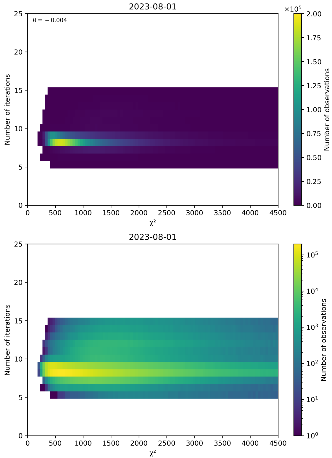
Figure 49: Scatter density plot of “ \chi^2 ” against “Number of iterations” for 2023-07-31 to 2023-08-02.
