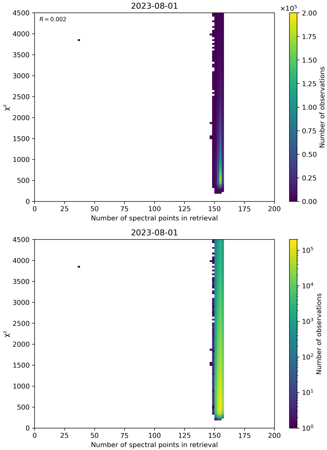
Figure 58: Scatter density plot of “Number of spectral points in retrieval” against “ \chi^2 ” for 2023-07-31 to 2023-08-02.
