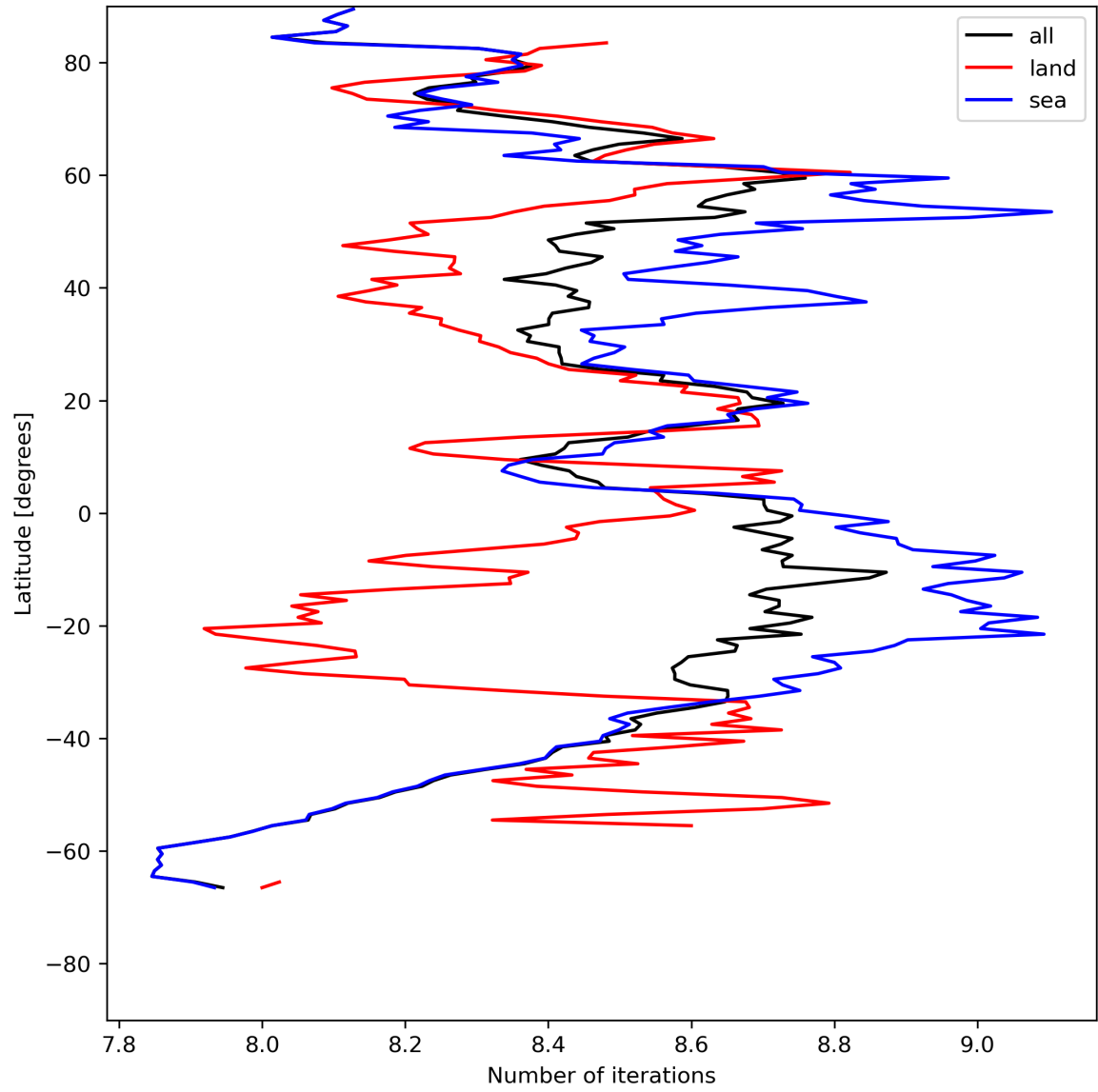
Figure 16: Zonal average of “Number of iterations” for 2023-07-31 to 2023-08-02.
