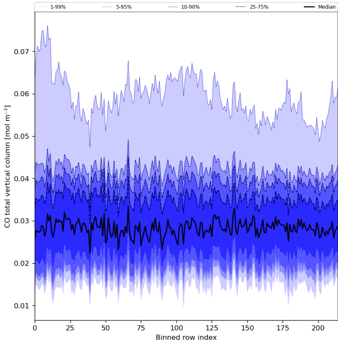
Figure 26: Along track statistics of “CO total vertical column” for 2023-07-31 to 2023-08-02
