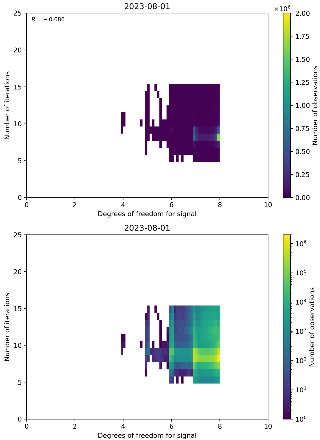
Figure 50: Scatter density plot of “Degrees of freedom for signal” against “Number of iterations” for 2023-07-31 to 2023-08-02.
