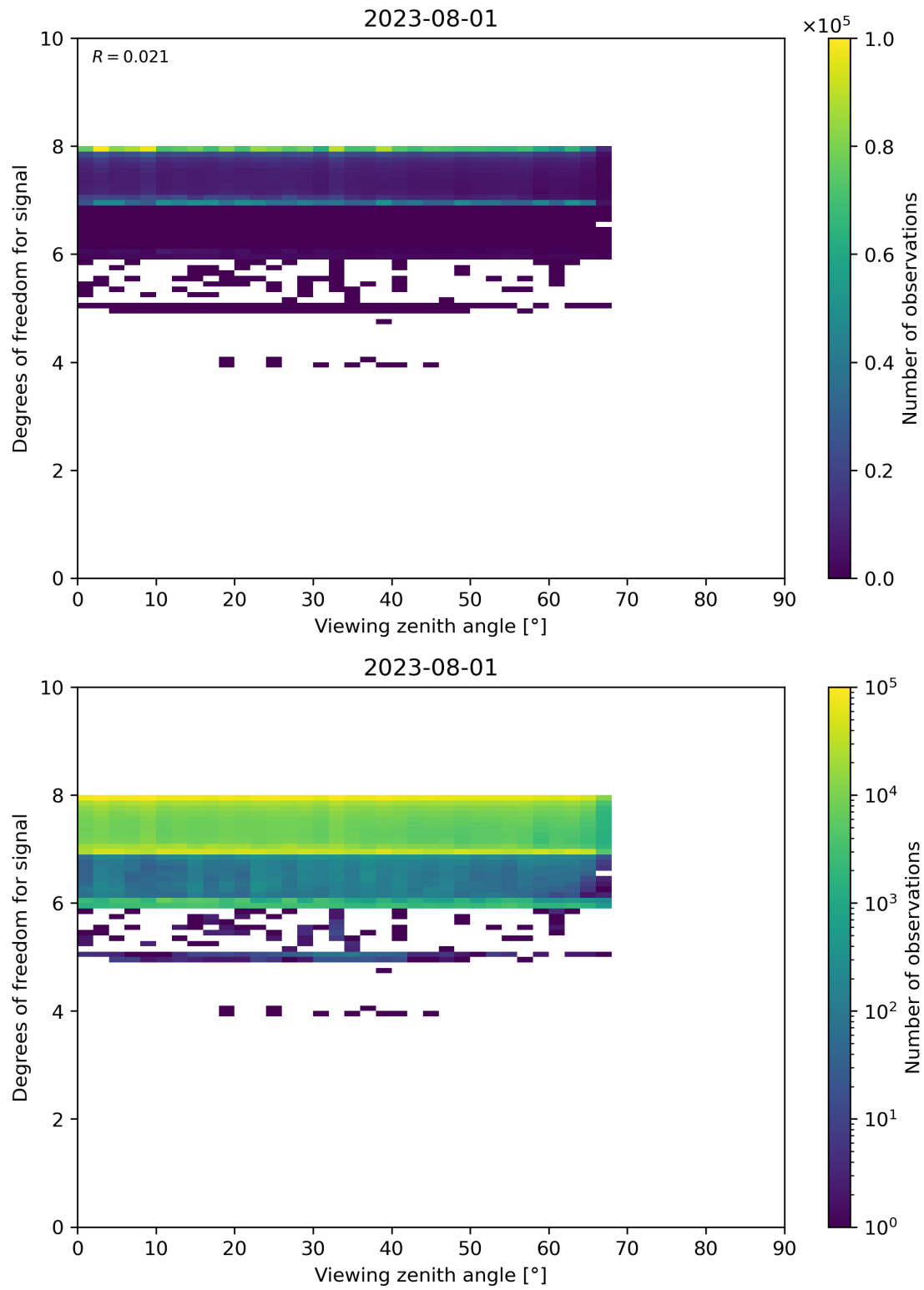
Figure 73: Scatter density plot of “Viewing zenith angle” against “Degrees of freedom for signal” for 2023-07-31 to 2023-08-02.
