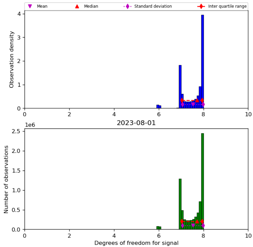
Figure 23: Histogram of “Degrees of freedom for signal” for 2023-07-31 to 2023-08-02
