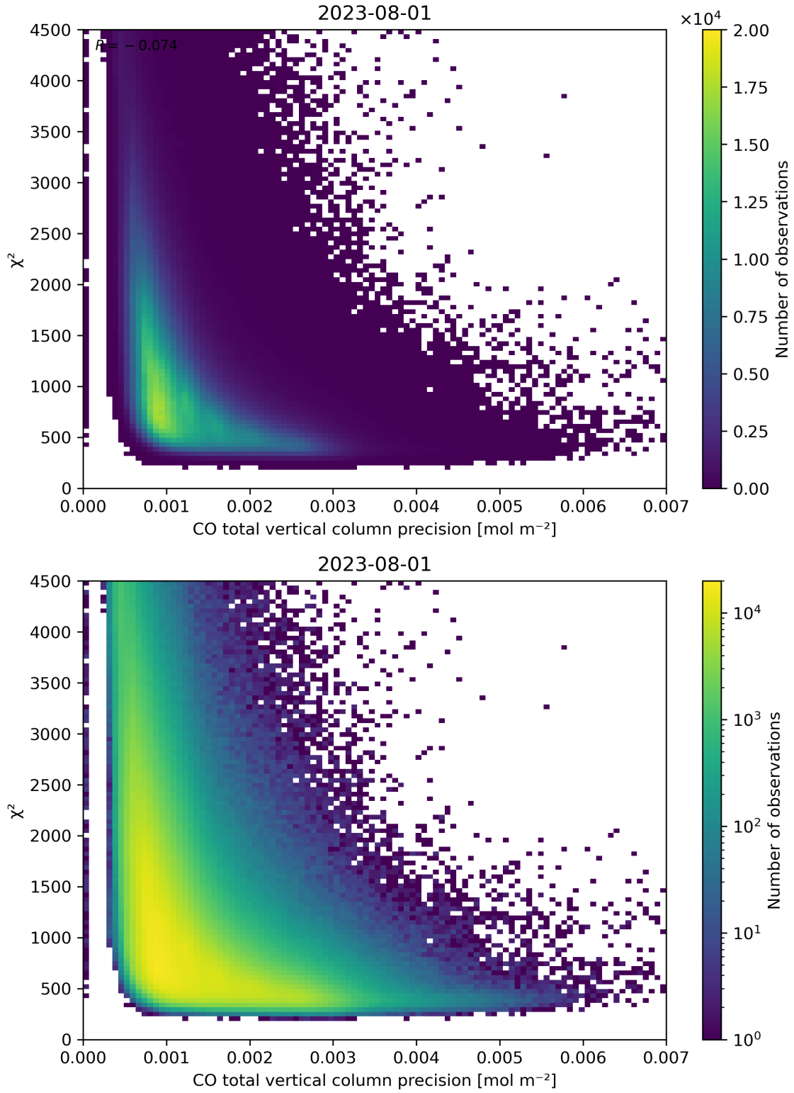
Figure 44: Scatter density plot of “CO total vertical column precision” against “ \chi^2 ” for 2023-07-31 to 2023-08-02.
