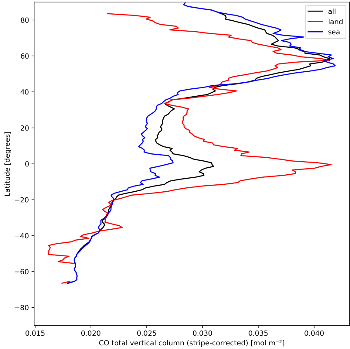
Figure 11: Zonal average of “CO total vertical column (stripe-corrected)” for 2023-07-31 to 2023-08-02.
