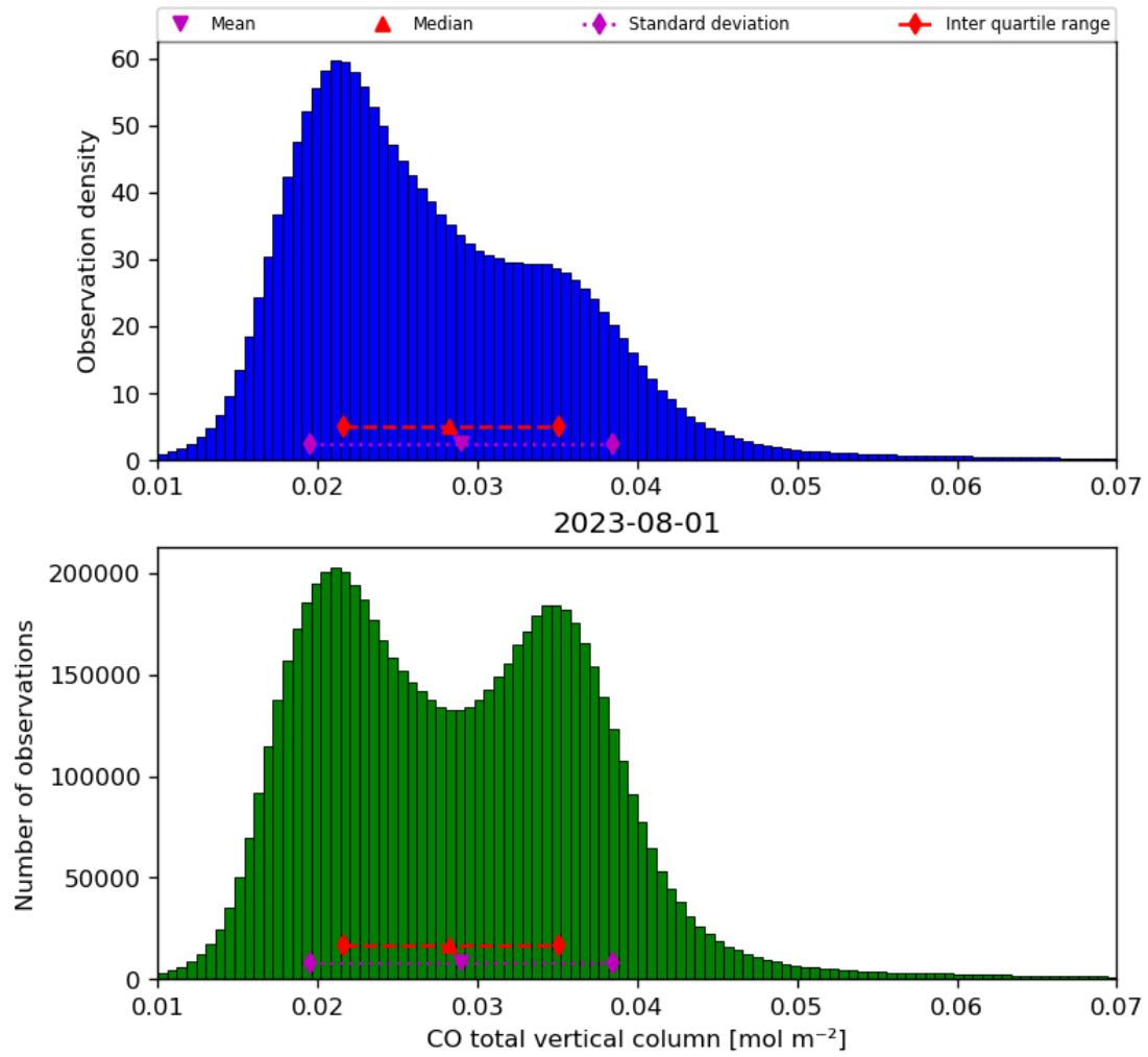
Figure 18: Histogram of “CO total vertical column” for 2023-07-31 to 2023-08-02
