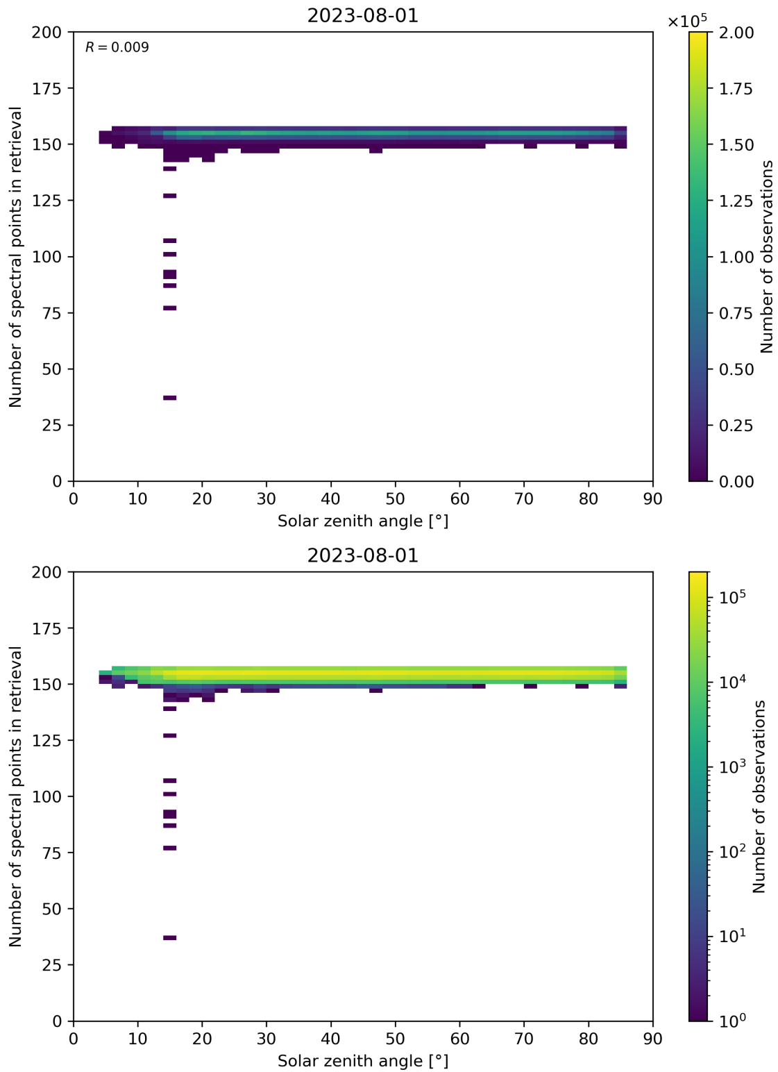
Figure 68: Scatter density plot of “Solar zenith angle” against “Number of spectral points in retrieval” for 2023-07-31 to 2023-08-02.
