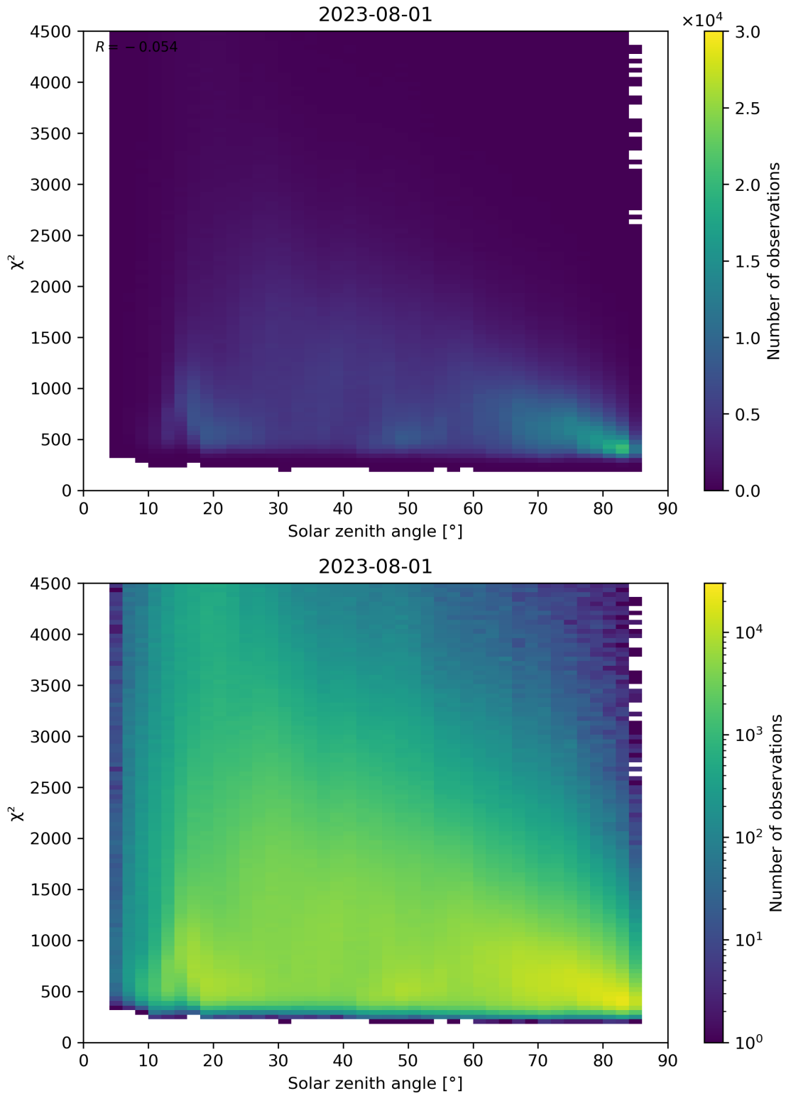
Figure 64: Scatter density plot of “Solar zenith angle” against “ \chi^2 ” for 2023-07-31 to 2023-08-02.
