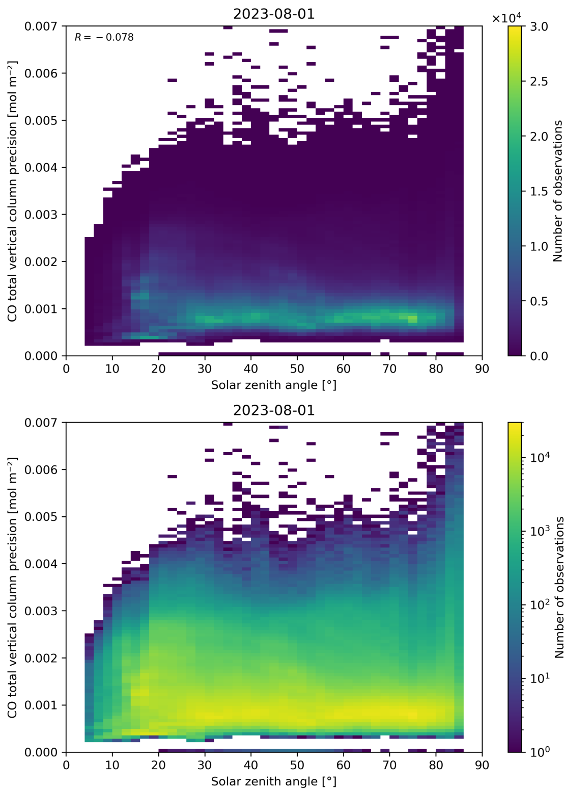
Figure 63: Scatter density plot of “Solar zenith angle” against “CO total vertical column precision” for 2023-07-31 to 2023-08-02.
