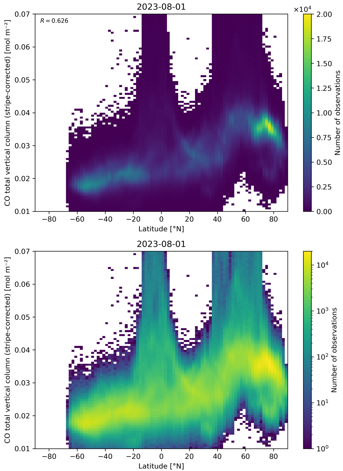
Figure 52: Scatter density plot of “Latitude” against “CO total vertical column (stripe-corrected)” for 2023-07-31 to 2023-08-02.
