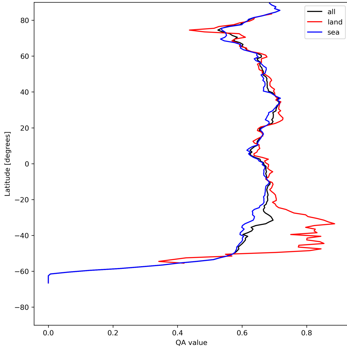
Figure 9: Zonal average of “QA value” for 2023-07-31 to 2023-08-02.
