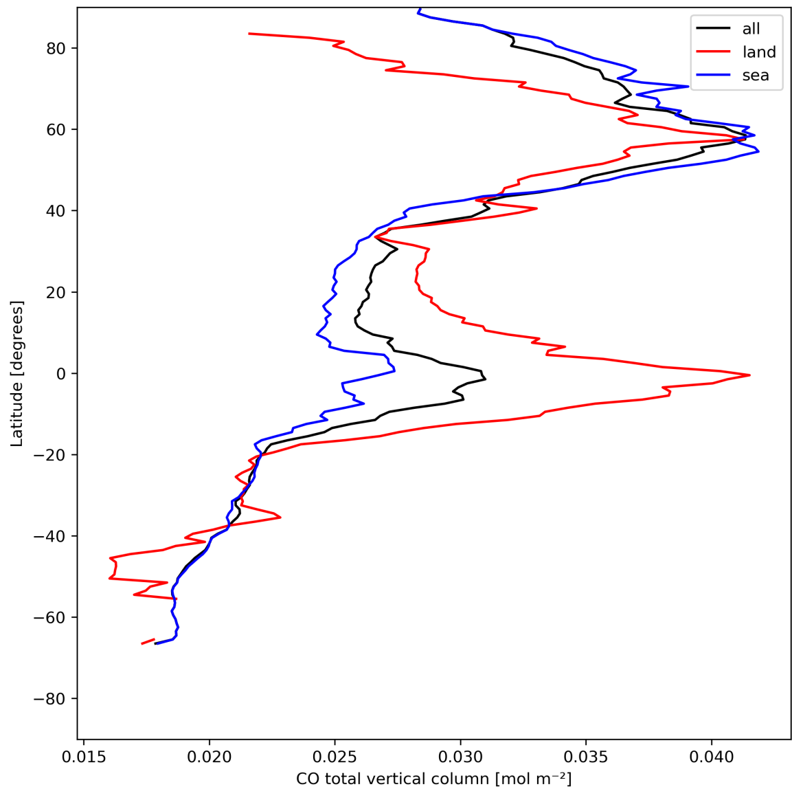
Figure 10: Zonal average of “CO total vertical column” for 2023-07-31 to 2023-08-02.
