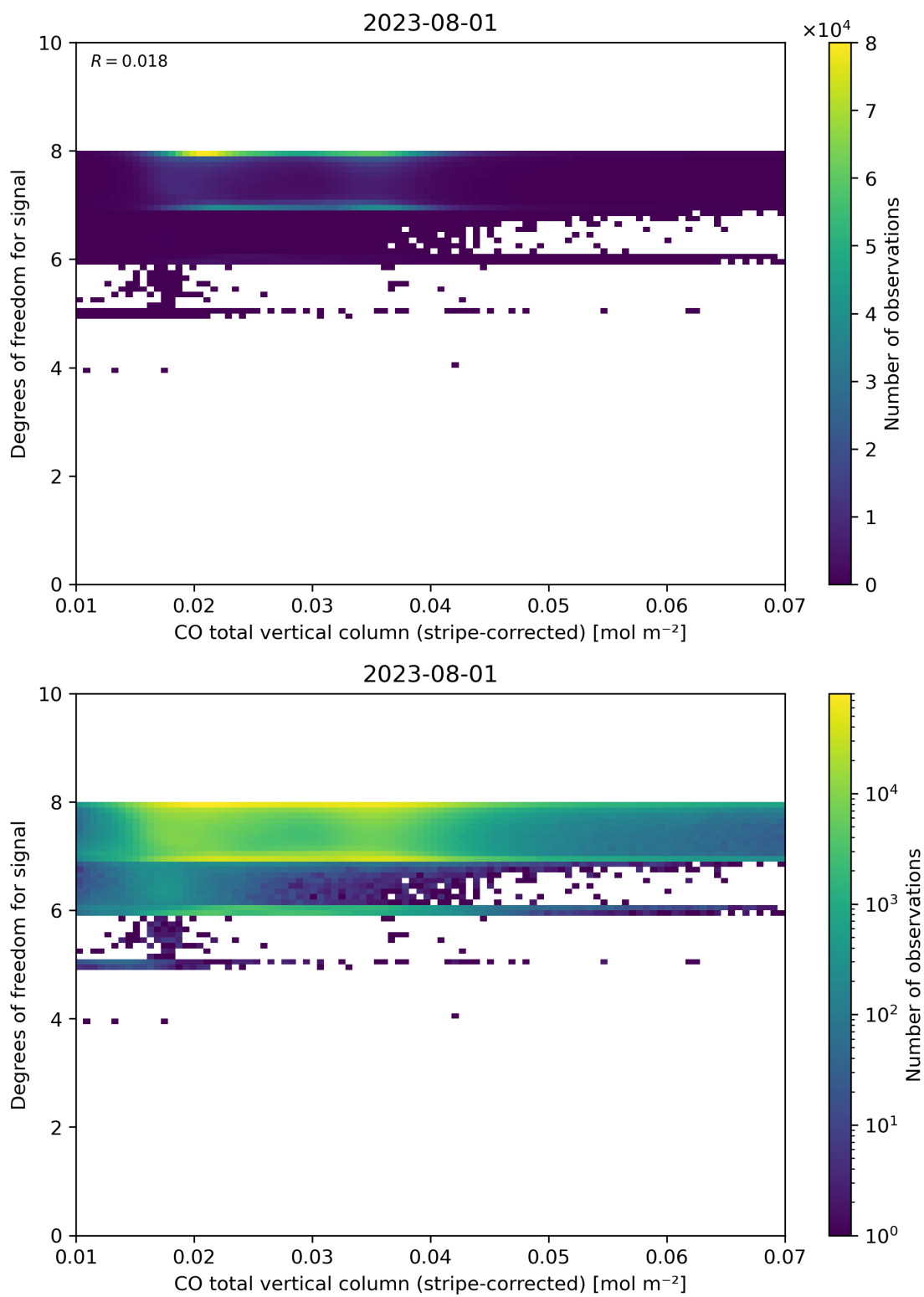
Figure 38: Scatter density plot of “CO total vertical column (stripe-corrected)” against “Degrees of freedom for signal” for 2023-07-31 to 2023-08-02.
