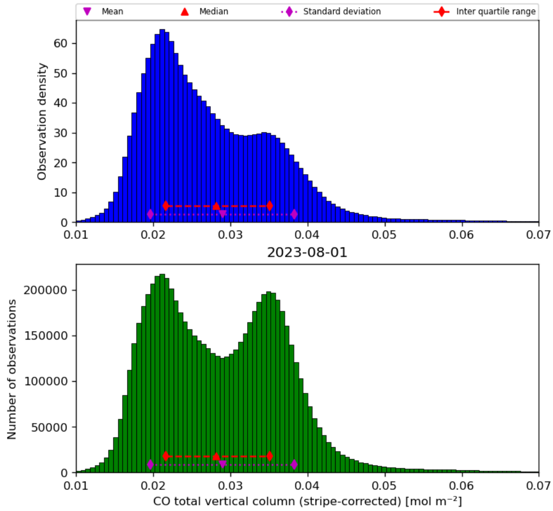
Figure 19: Histogram of “CO total vertical column (stripe-corrected)” for 2023-07-31 to 2023-08-02
