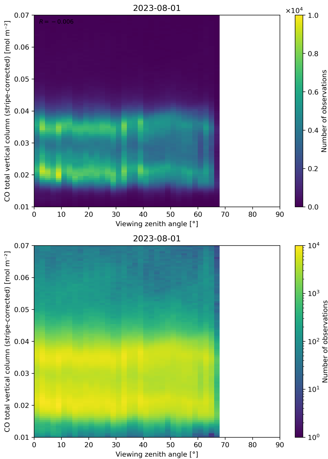
Figure 70: Scatter density plot of “Viewing zenith angle” against “CO total vertical column (stripe-corrected)” for 2023-07-31 to 2023-08-02.
