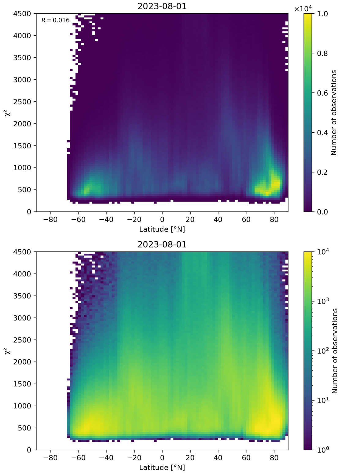
Figure 54: Scatter density plot of “Latitude” against “ \chi^2 ” for 2023-07-31 to 2023-08-02.
