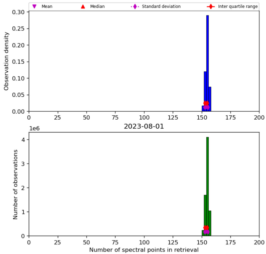
Figure 21: Histogram of “Number of spectral points in retrieval” for 2023-07-31 to 2023-08-02
