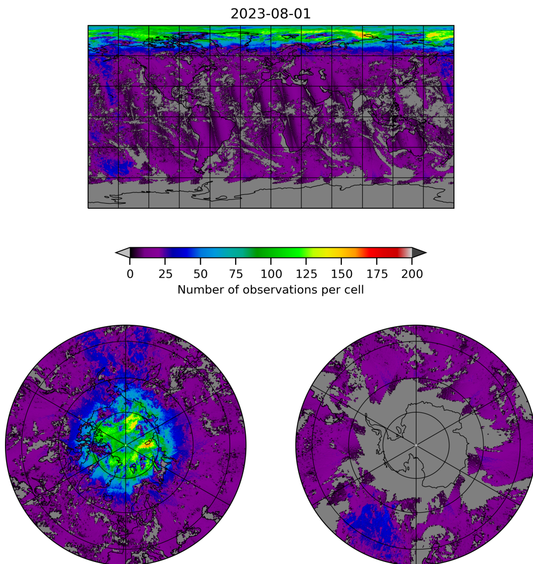
Figure 8: Map of the number of observations for 2023-07-31 to 2023-08-02
