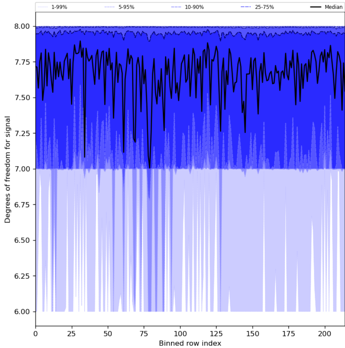
Figure 31: Along track statistics of “Degrees of freedom for signal” for 2023-07-31 to 2023-08-02
