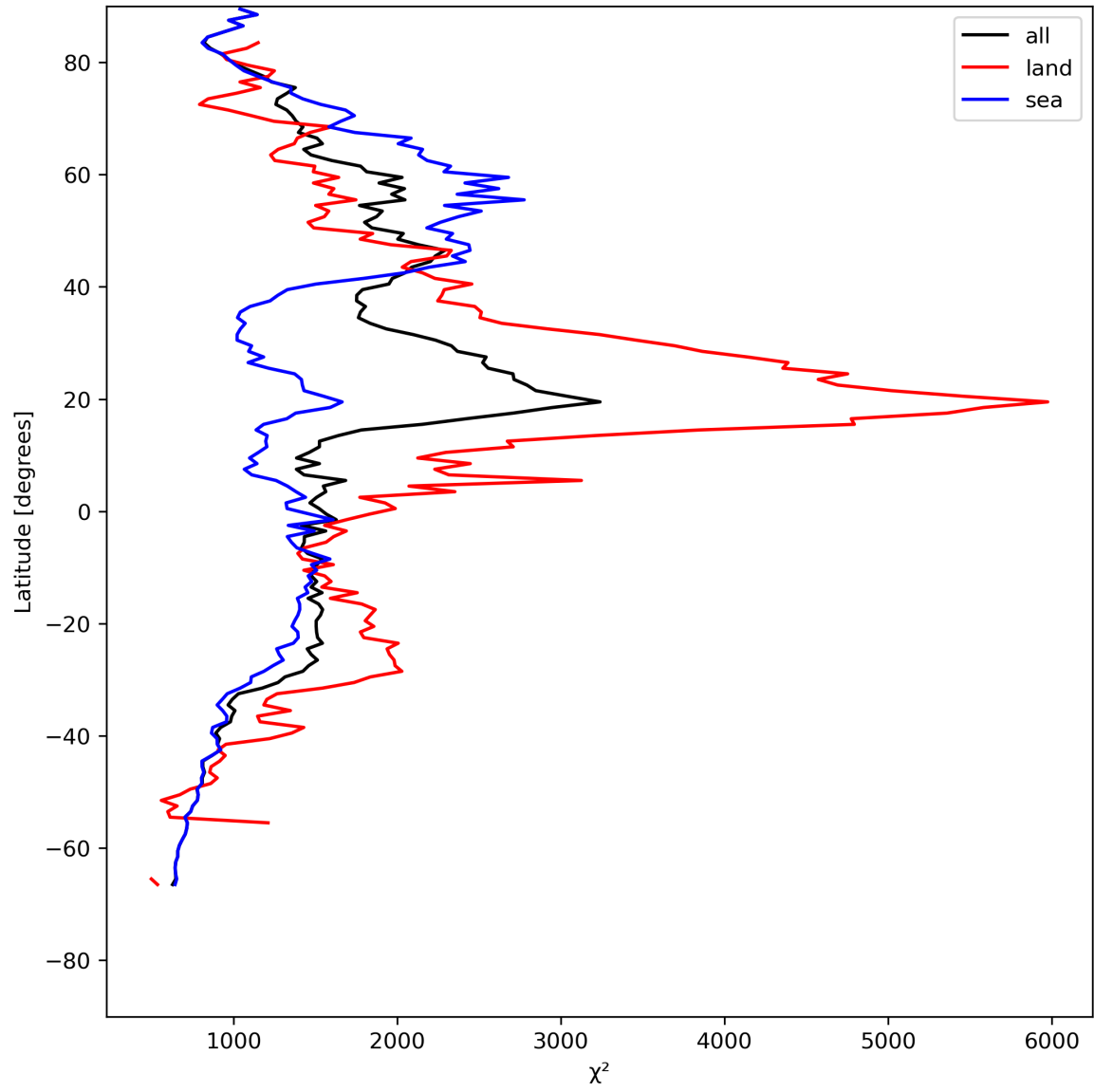
Figure 14: Zonal average of “ \chi^2 ” for 2023-07-31 to 2023-08-02.
