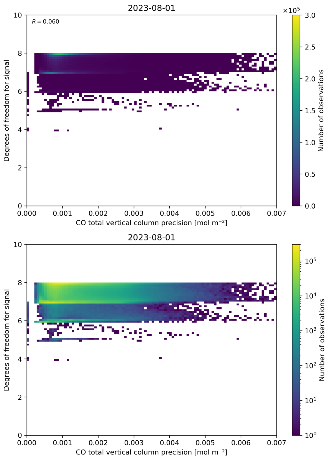
Figure 45: Scatter density plot of “CO total vertical column precision” against “Degrees of freedom for signal” for 2023-07-31 to 2023-08-02.
