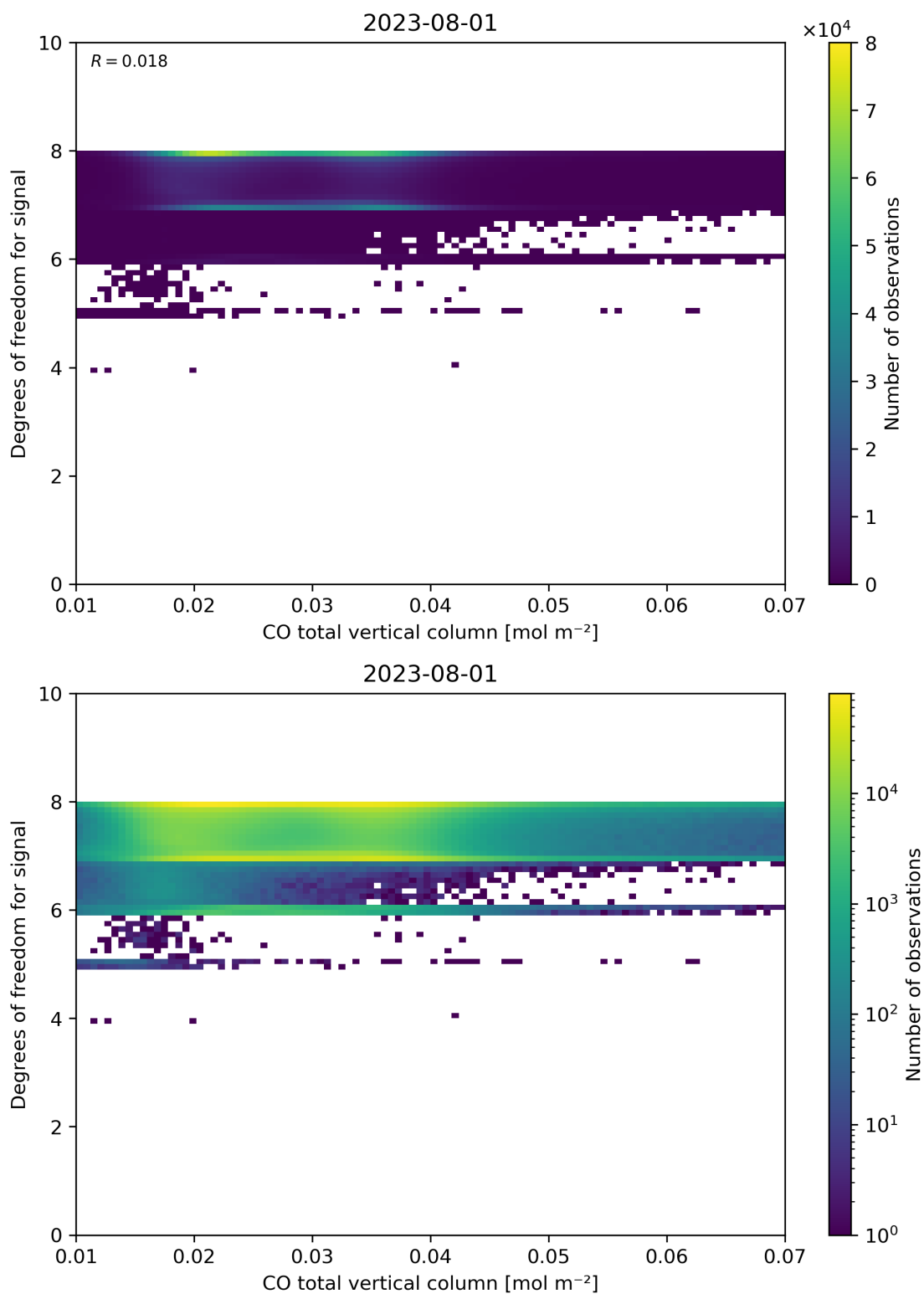
Figure 41: Scatter density plot of “CO total vertical column” against “Degrees of freedom for signal” for 2023-07-31 to 2023-08-02.
