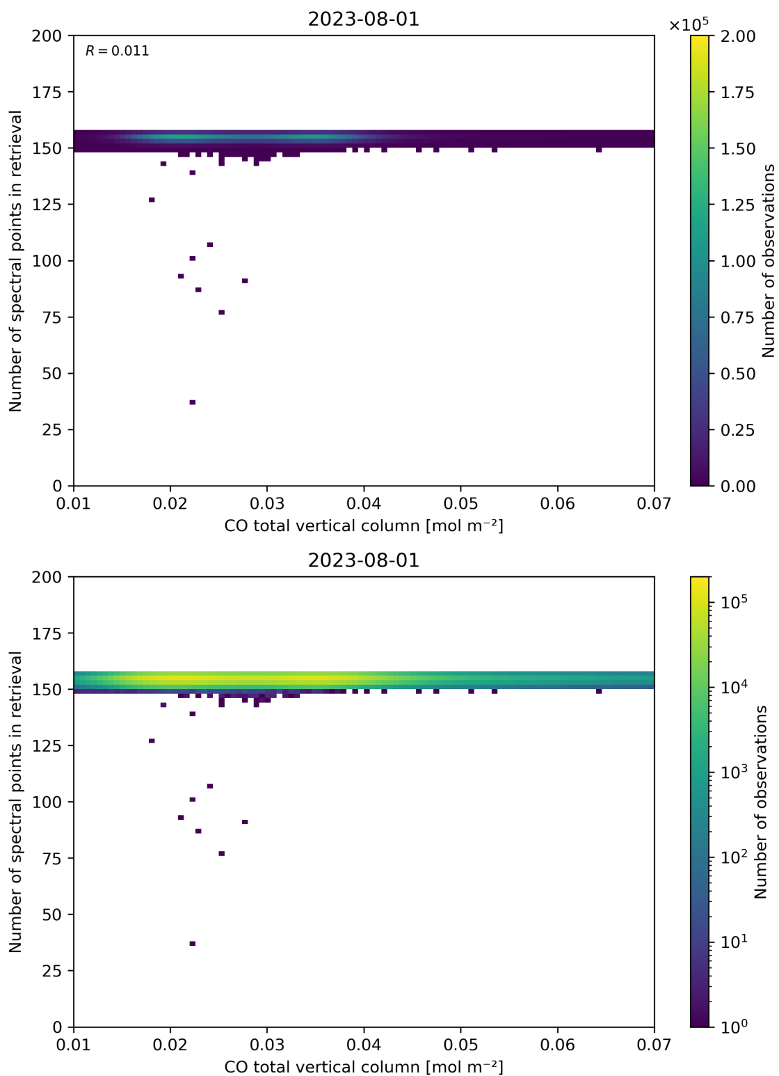
Figure 43: Scatter density plot of “CO total vertical column” against “Number of spectral points in retrieval” for 2023-07-31 to 2023-08-02.
