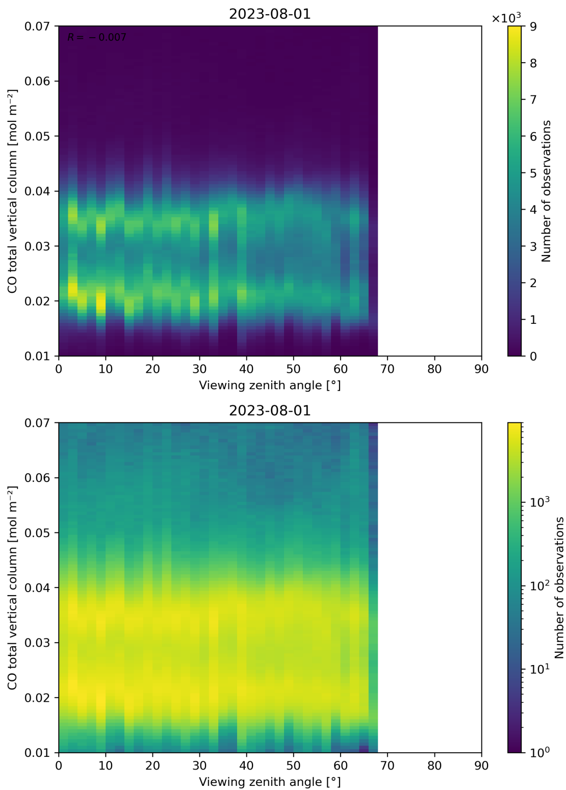
Figure 69: Scatter density plot of “Viewing zenith angle” against “CO total vertical column” for 2023-07-31 to 2023-08-02.
