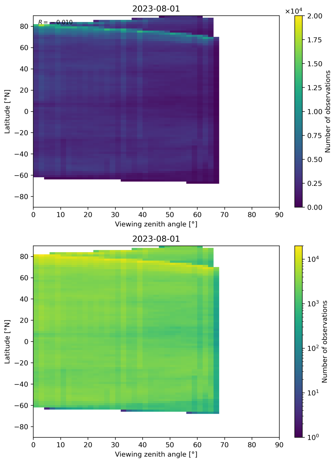
Figure 74: Scatter density plot of “Viewing zenith angle” against “Latitude” for 2023-07-31 to 2023-08-02.
