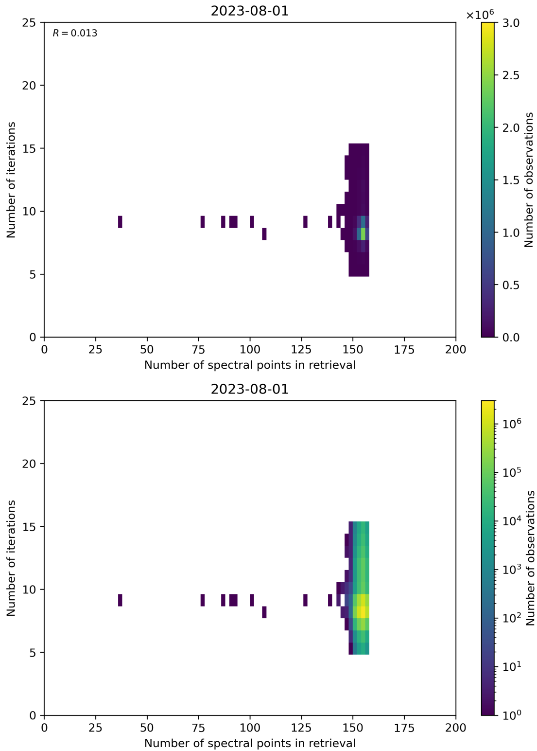
Figure 60: Scatter density plot of “Number of spectral points in retrieval” against “Number of iterations” for 2023-07-31 to 2023-08-02.
