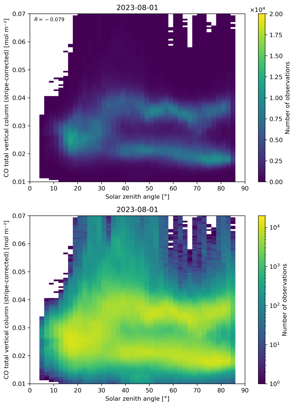
Figure 62: Scatter density plot of “Solar zenith angle” against “CO total vertical column (stripe-corrected)” for 2023-07-31 to 2023-08-02.
