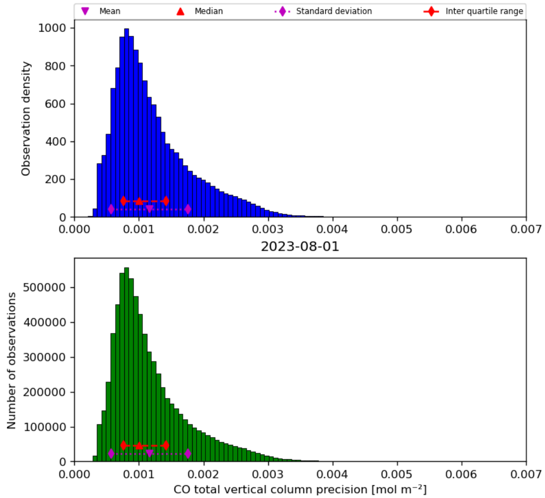
Figure 20: Histogram of “CO total vertical column precision” for 2023-07-31 to 2023-08-02
