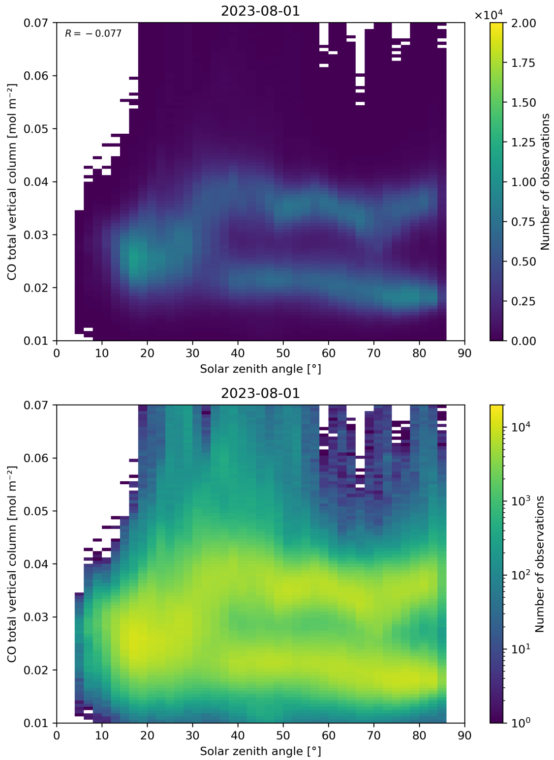
Figure 61: Scatter density plot of “Solar zenith angle” against “CO total vertical column” for 2023-07-31 to 2023-08-02.
