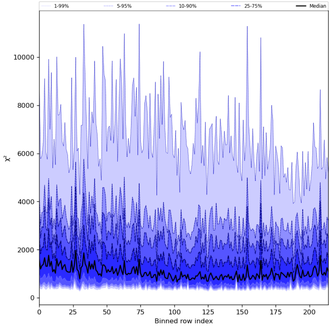
Figure 30: Along track statistics of “ \chi^2 ” for 2023-07-31 to 2023-08-02
