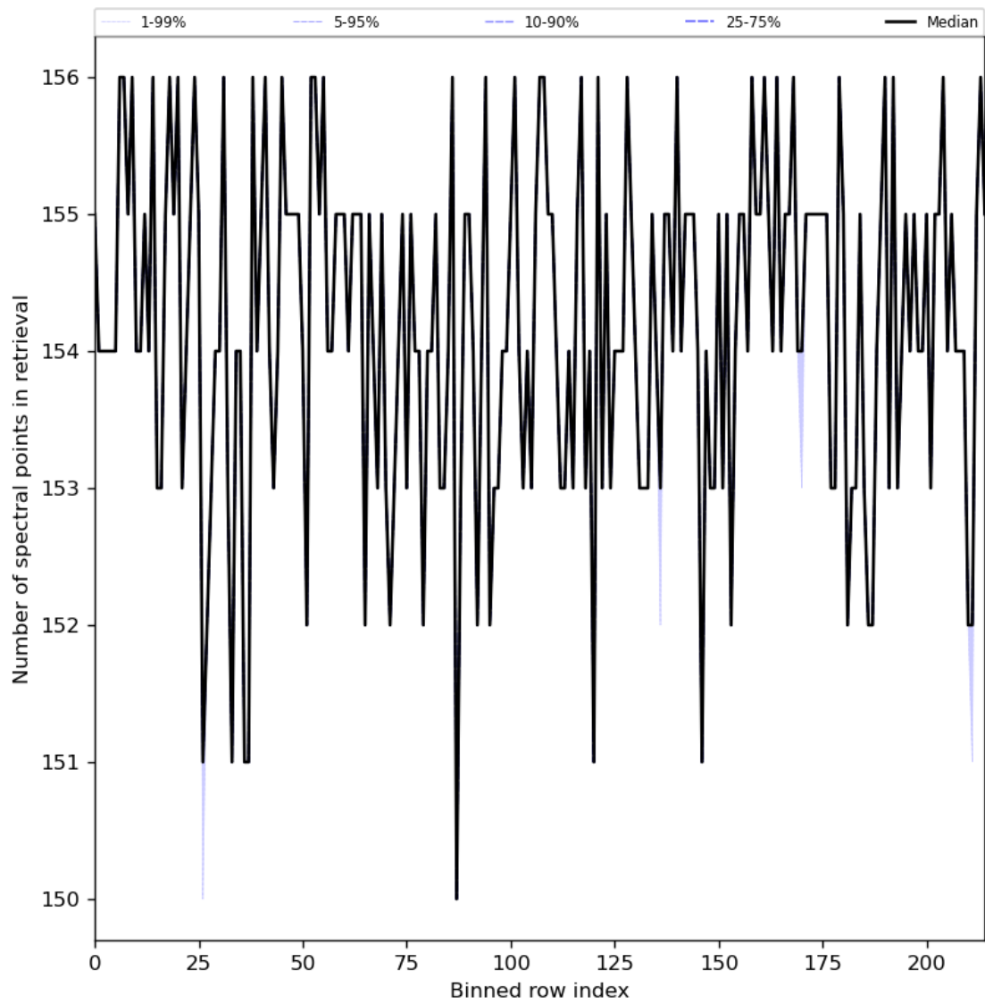
Figure 29: Along track statistics of “Number of spectral points in retrieval” for 2023-07-31 to 2023-08-02
