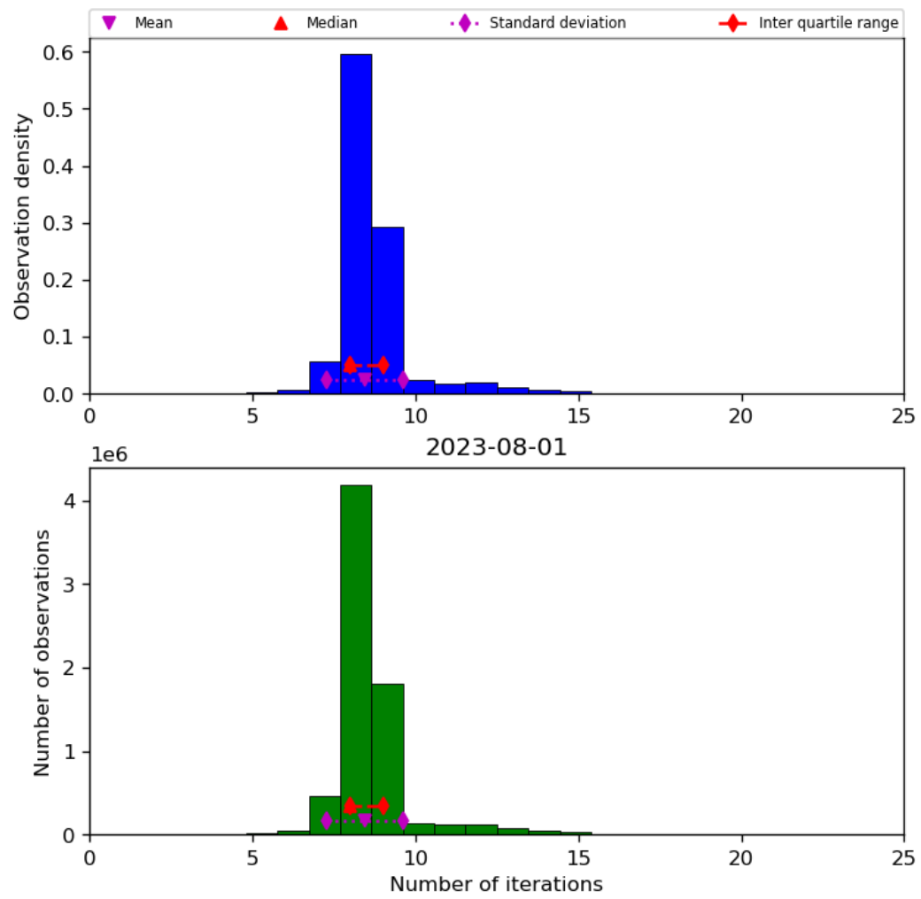
Figure 24: Histogram of "Number of iterations" for 2023-07-31 to 2023-08-02
