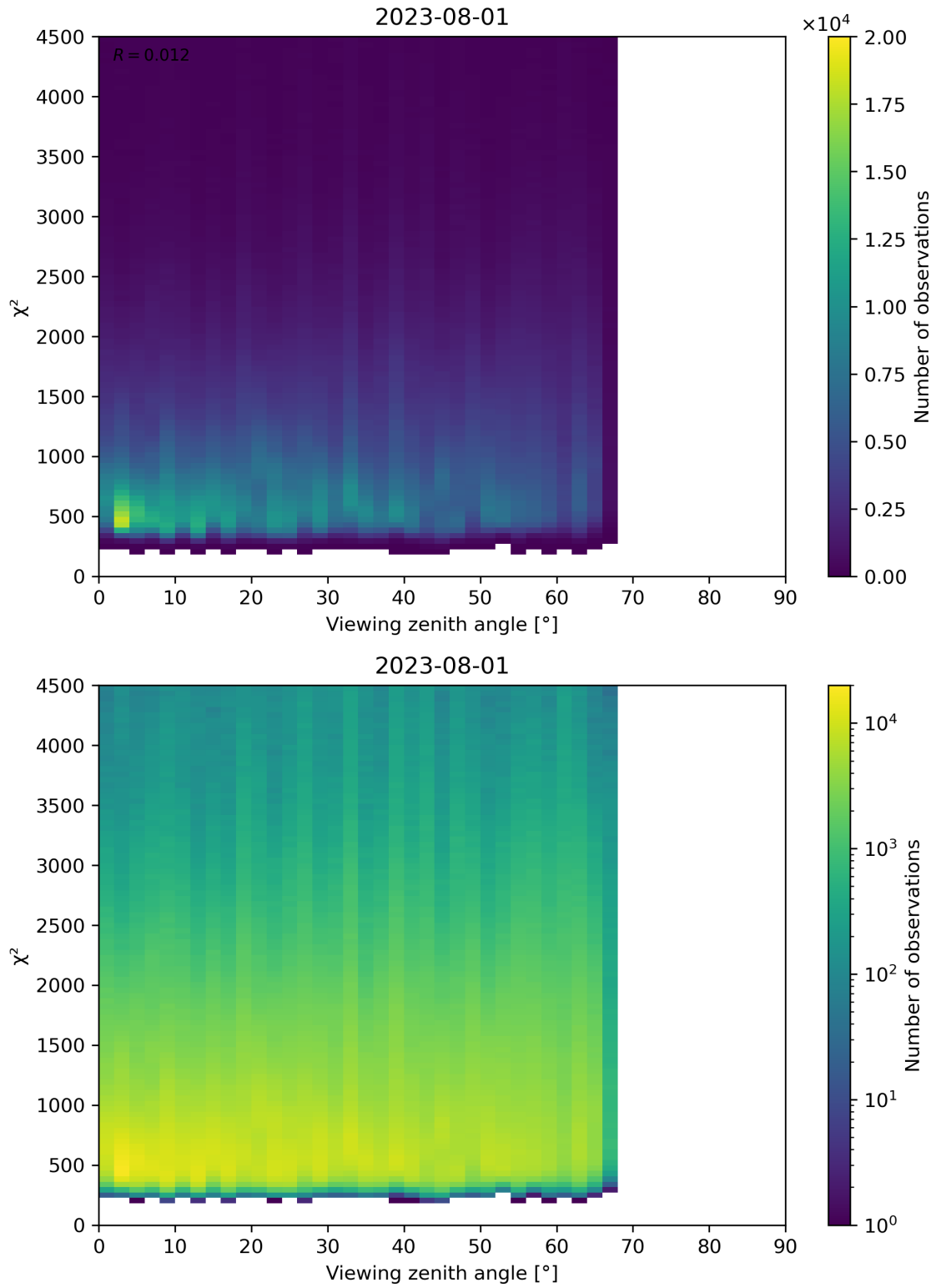
Figure 72: Scatter density plot of “Viewing zenith angle” against “ \chi^2 ” for 2023-07-31 to 2023-08-02.
