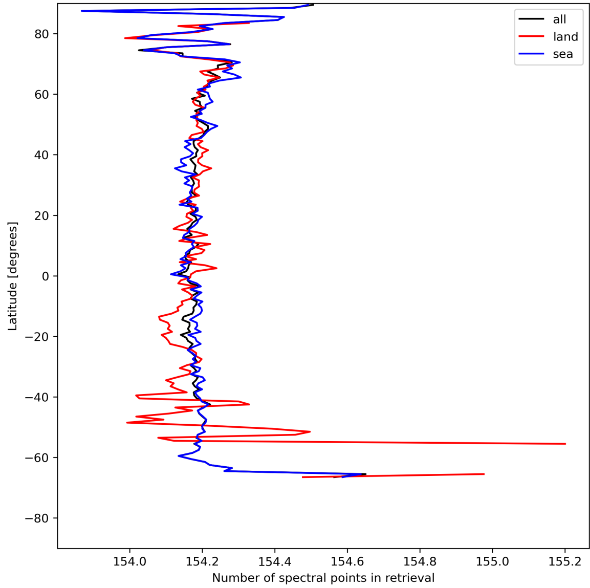
Figure 13: Zonal average of “Number of spectral points in retrieval” for 2023-07-31 to 2023-08-02.
