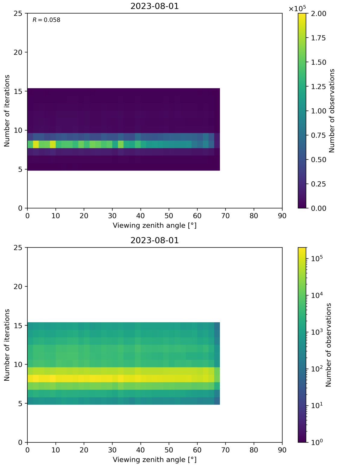
Figure 75: Scatter density plot of “Viewing zenith angle” against “Number of iterations” for 2023-07-31 to 2023-08-02.
