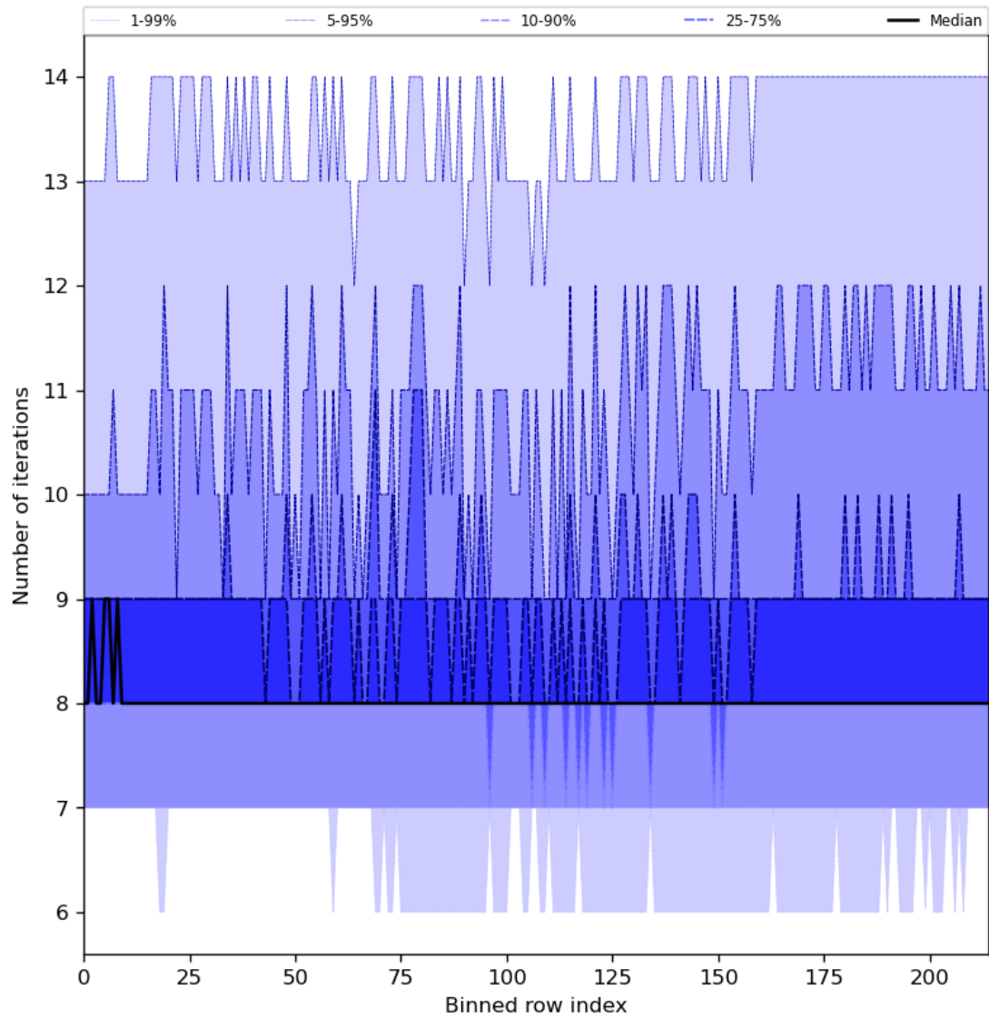
Figure 32: Along track statistics of “Number of iterations” for 2023-07-31 to 2023-08-02
