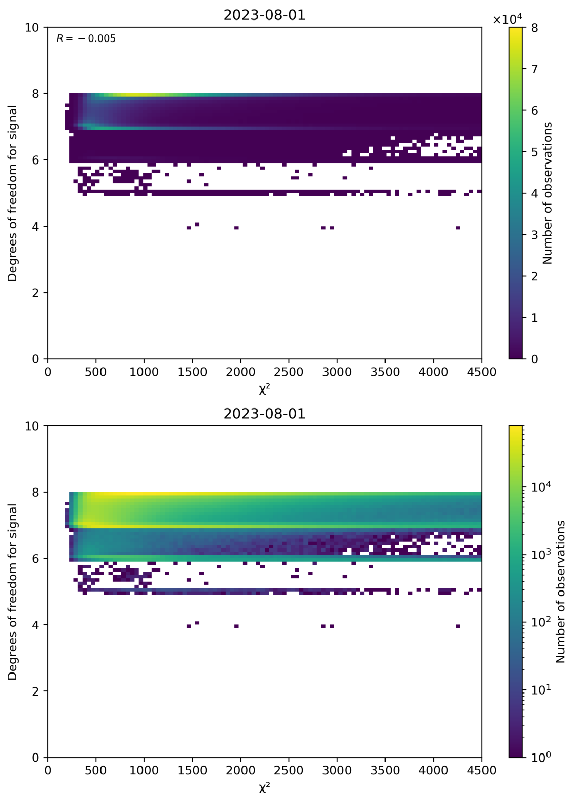
Figure 48: Scatter density plot of “ \chi^2 ” against “Degrees of freedom for signal” for 2023-07-31 to 2023-08-02.
