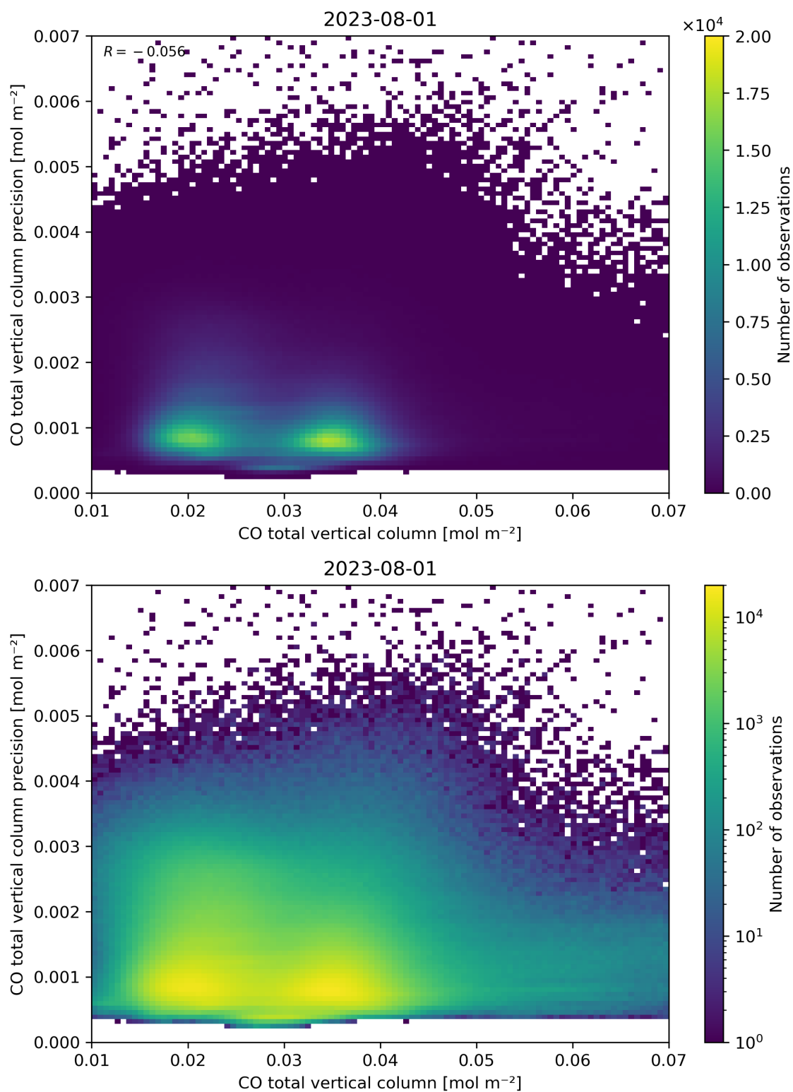
Figure 34: Scatter density plot of “CO total vertical column” against “CO total vertical column precision” for 2023-07-31 to 2023-08-02.
