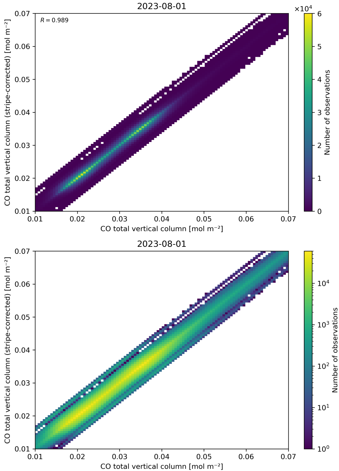
Figure 33: Scatter density plot of “CO total vertical column” against “CO total vertical column (stripe-corrected)” for 2023-07-31 to 2023-08-02.
