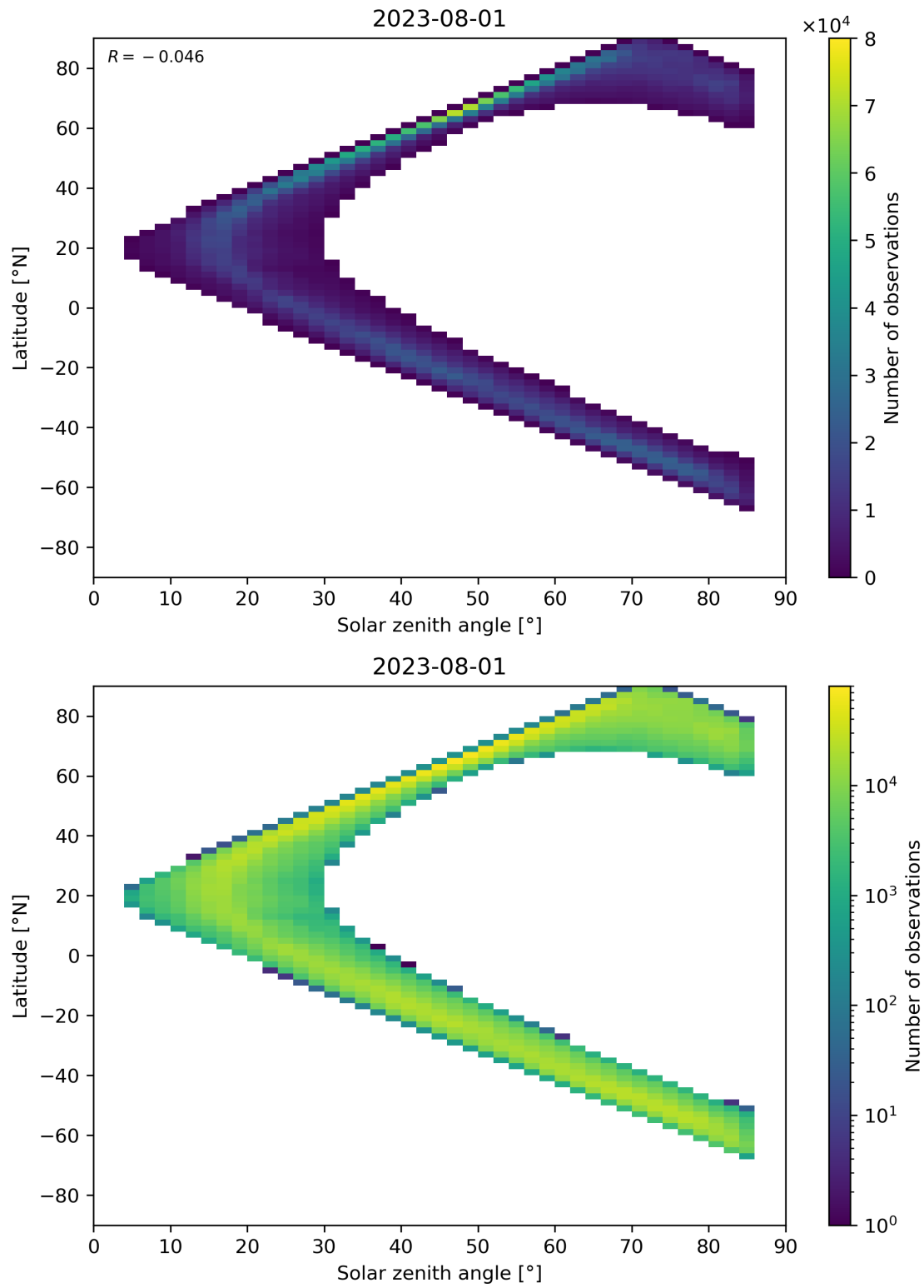
Figure 66: Scatter density plot of “Solar zenith angle” against “Latitude” for 2023-07-31 to 2023-08-02.
