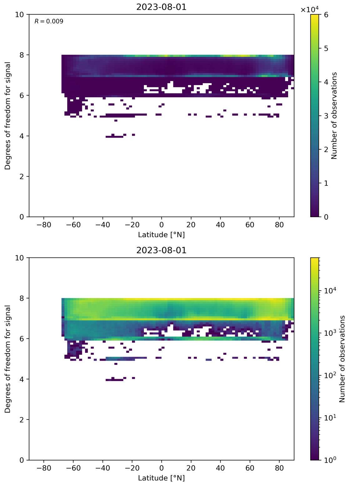
Figure 55: Scatter density plot of “Latitude” against “Degrees of freedom for signal” for 2023-07-31 to 2023-08-02.
