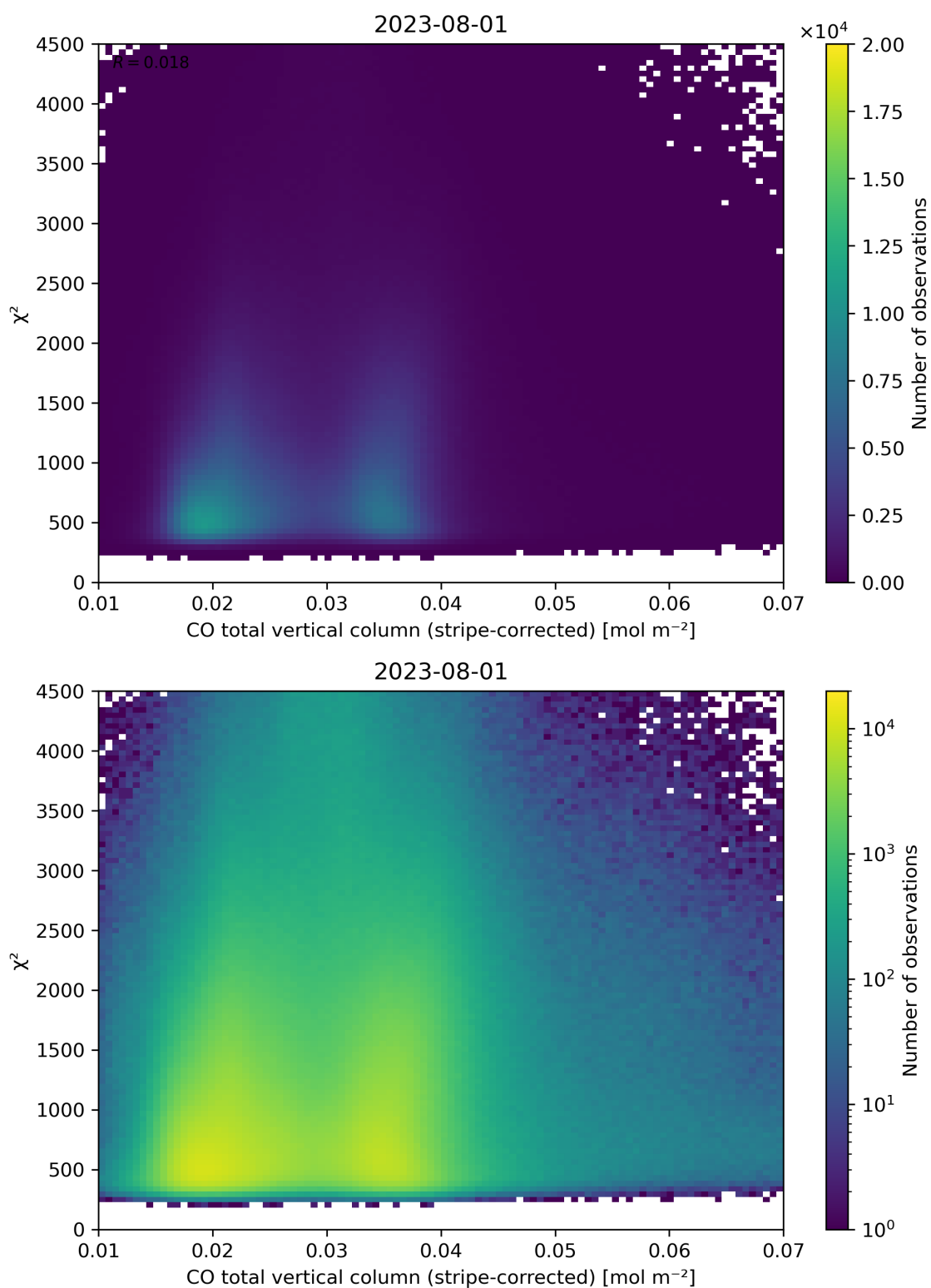
Figure 37: Scatter density plot of “CO total vertical column (stripe-corrected)” against “ \chi^2 ” for 2023-07-31 to 2023-08-02.
