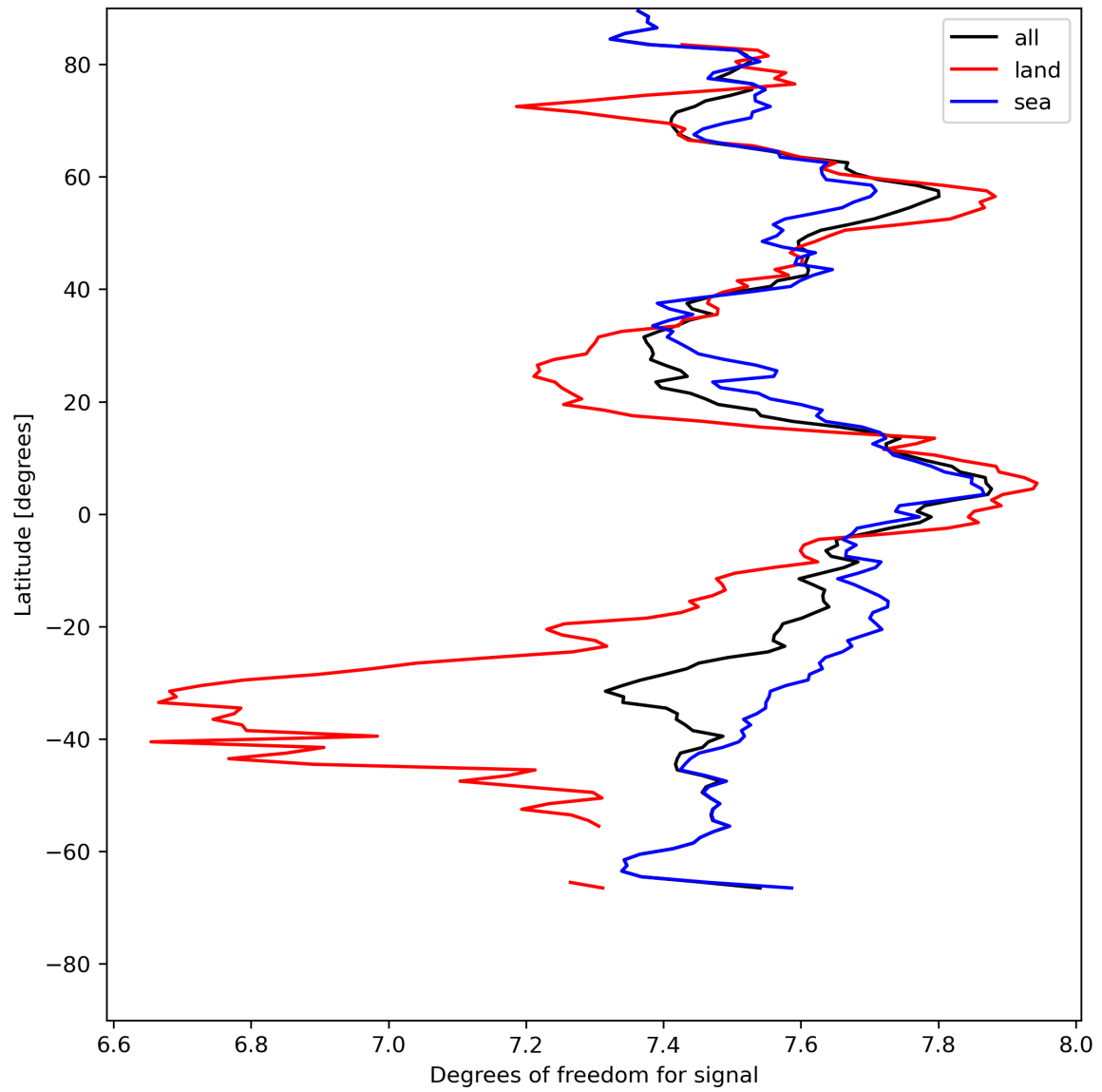
Figure 15: Zonal average of “Degrees of freedom for signal” for 2023-07-31 to 2023-08-02.
