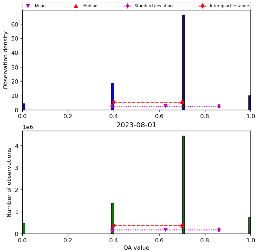
Figure 17: Histogram of “QA value” for 2023-07-31 to 2023-08-02
