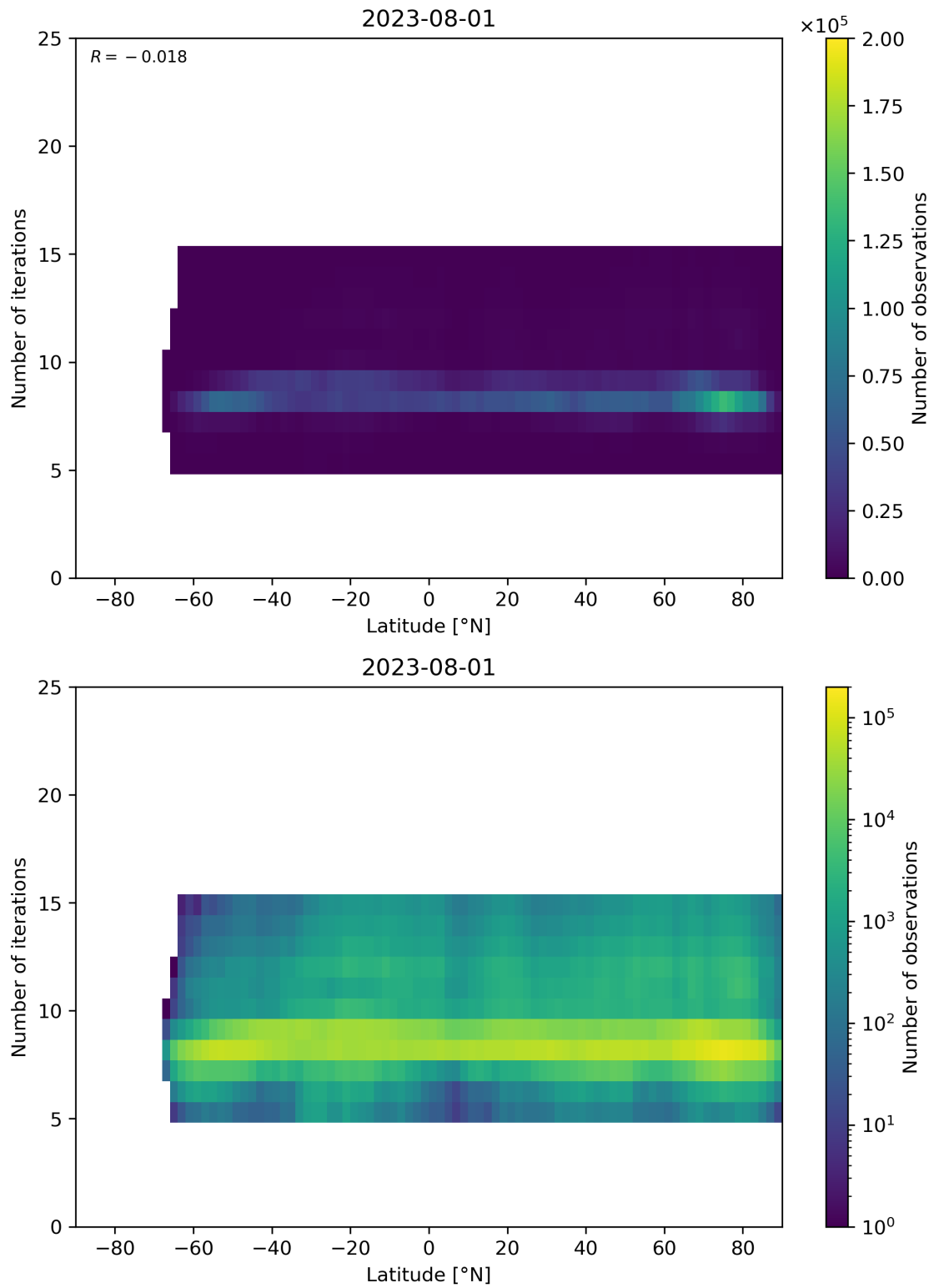
Figure 56: Scatter density plot of “Latitude” against “Number of iterations” for 2023-07-31 to 2023-08-02.
