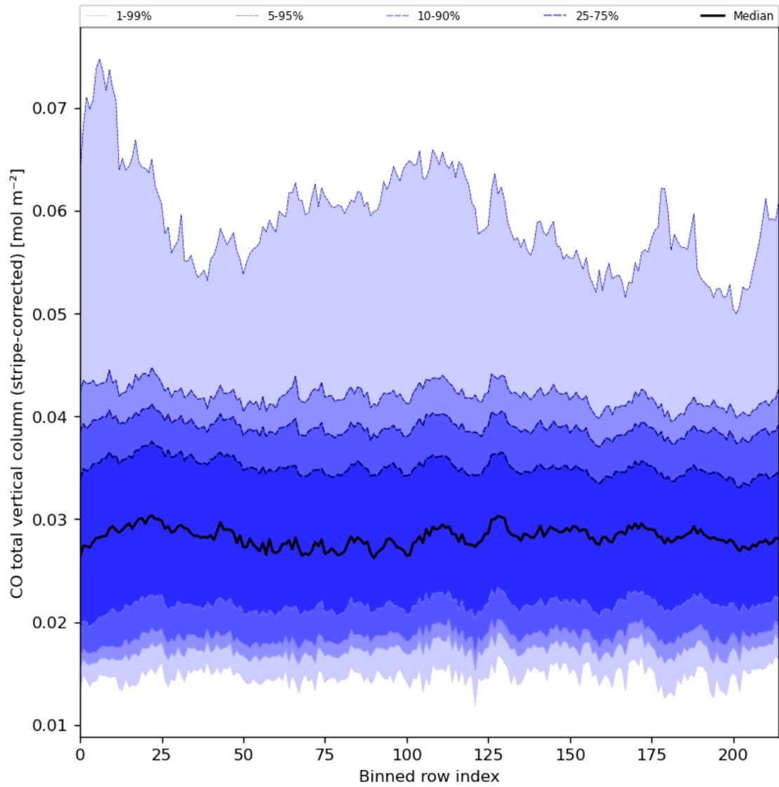
Figure 27: Along track statistics of “CO total vertical column (stripe-corrected)” for 2023-07-31 to 2023-08-02
