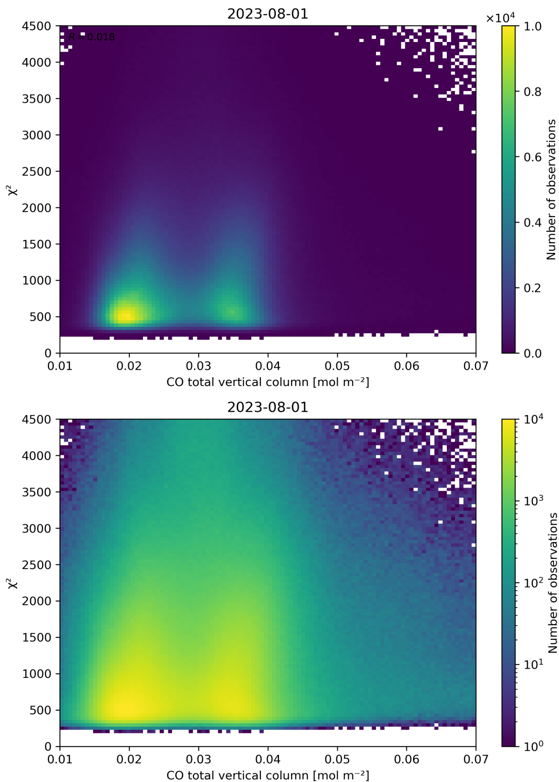
Figure 35: Scatter density plot of “CO total vertical column” against “ \chi^2 ” for 2023-07-31 to 2023-08-02.
