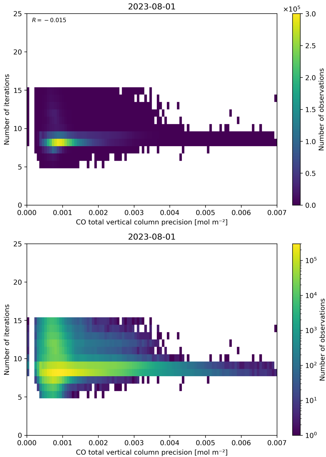
Figure 46: Scatter density plot of “CO total vertical column precision” against “Number of iterations” for 2023-07-31 to 2023-08-02.
