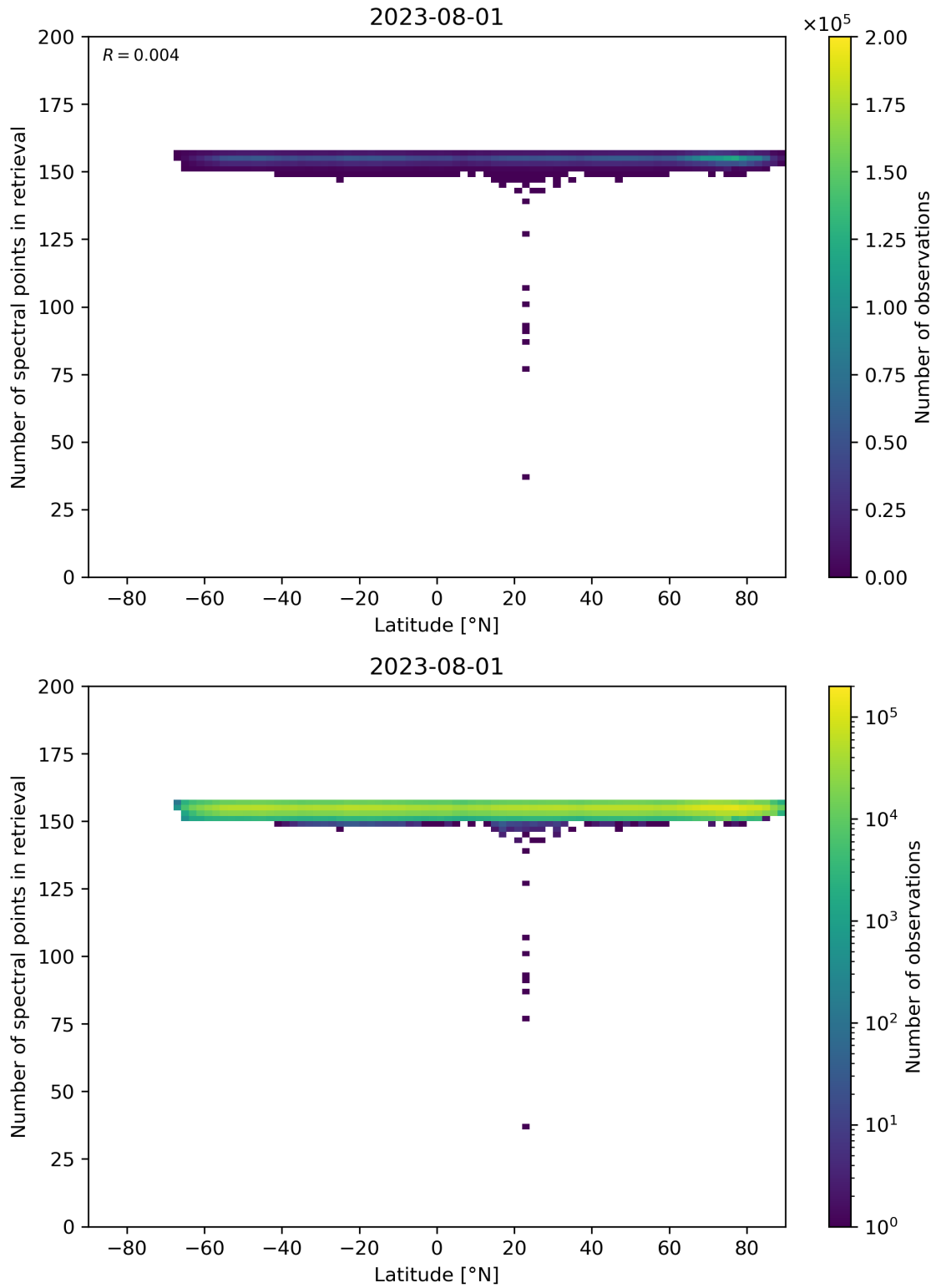
Figure 57: Scatter density plot of “Latitude” against “Number of spectral points in retrieval” for 2023-07-31 to 2023-08-02.
