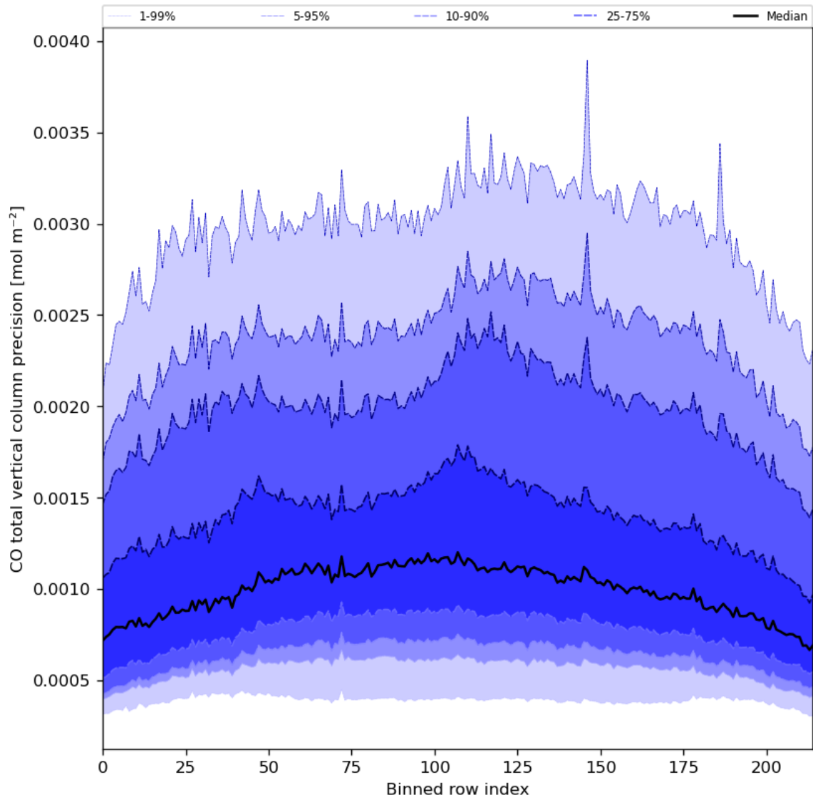
Figure 28: Along track statistics of “CO total vertical column precision” for 2023-07-31 to 2023-08-02
