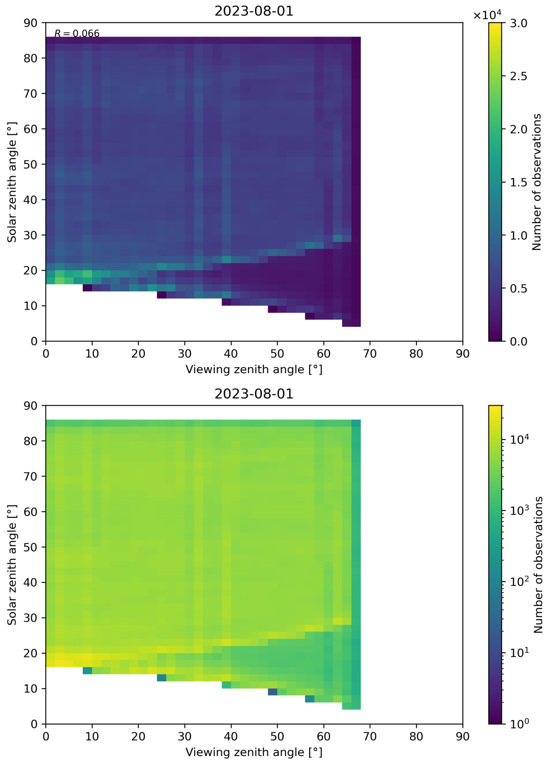
Figure 77: Scatter density plot of “Viewing zenith angle” against “Solar zenith angle” for 2023-07-31 to 2023-08-02.
