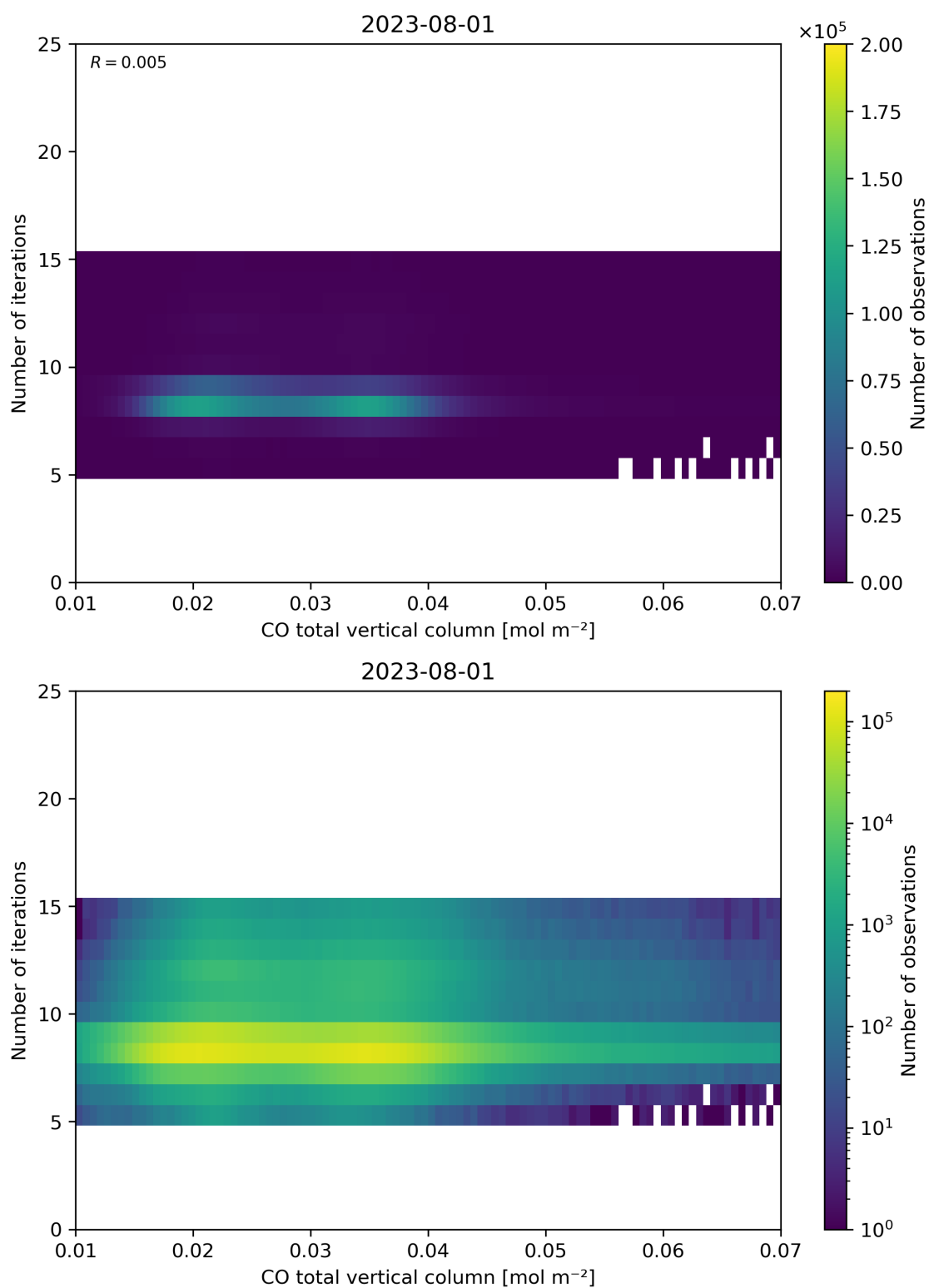
Figure 42: Scatter density plot of “CO total vertical column” against “Number of iterations” for 2023-07-31 to 2023-08-02.
