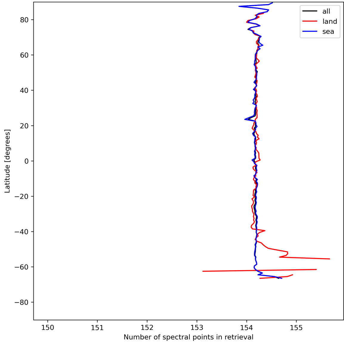
Figure 13: Zonal average of “Number of spectral points in retrieval” for 2023-08-01 to 2023-08-03.
