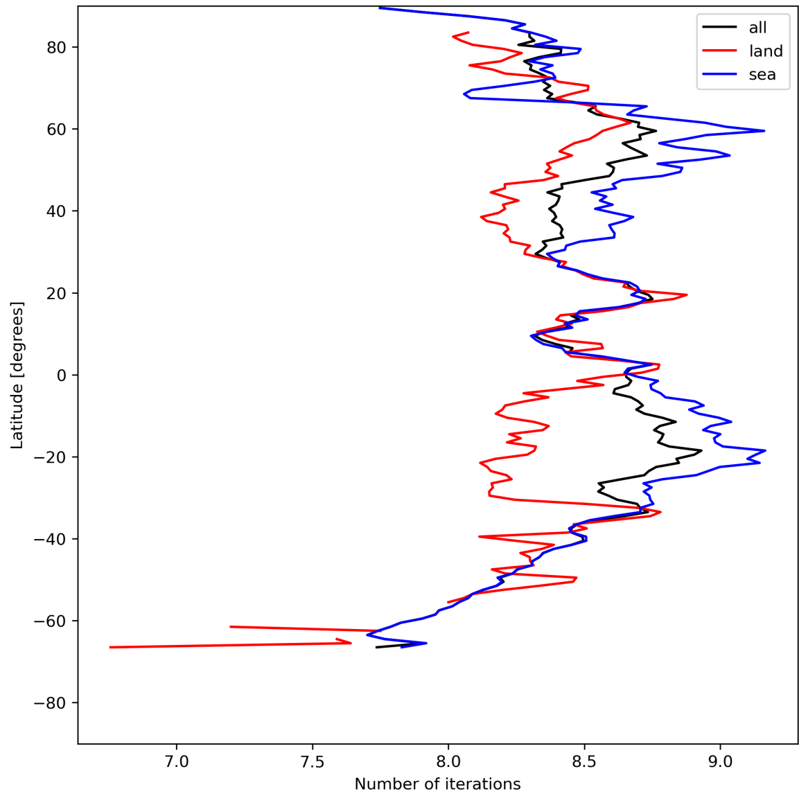
Figure 16: Zonal average of “Number of iterations” for 2023-08-01 to 2023-08-03.
