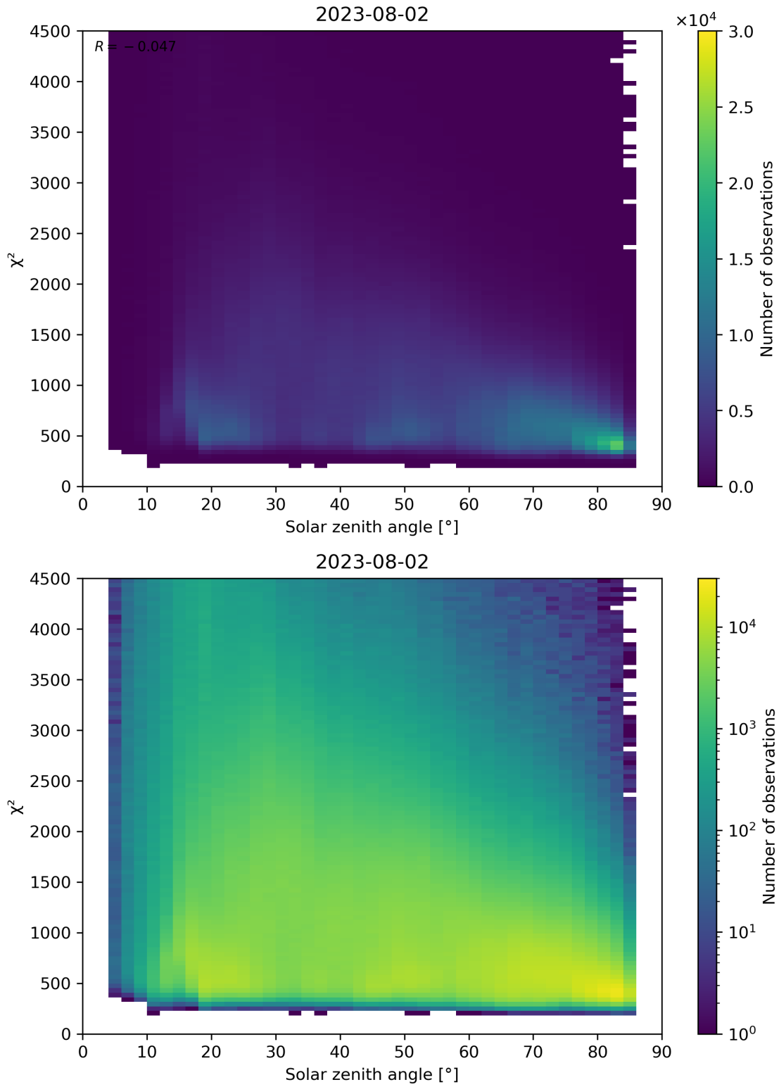
Figure 64: Scatter density plot of “Solar zenith angle” against “ \chi^2 ” for 2023-08-01 to 2023-08-03.
