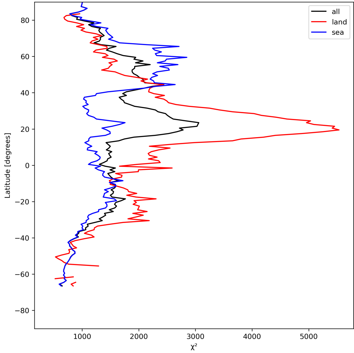
Figure 14: Zonal average of “ \chi^2 ” for 2023-08-01 to 2023-08-03.
