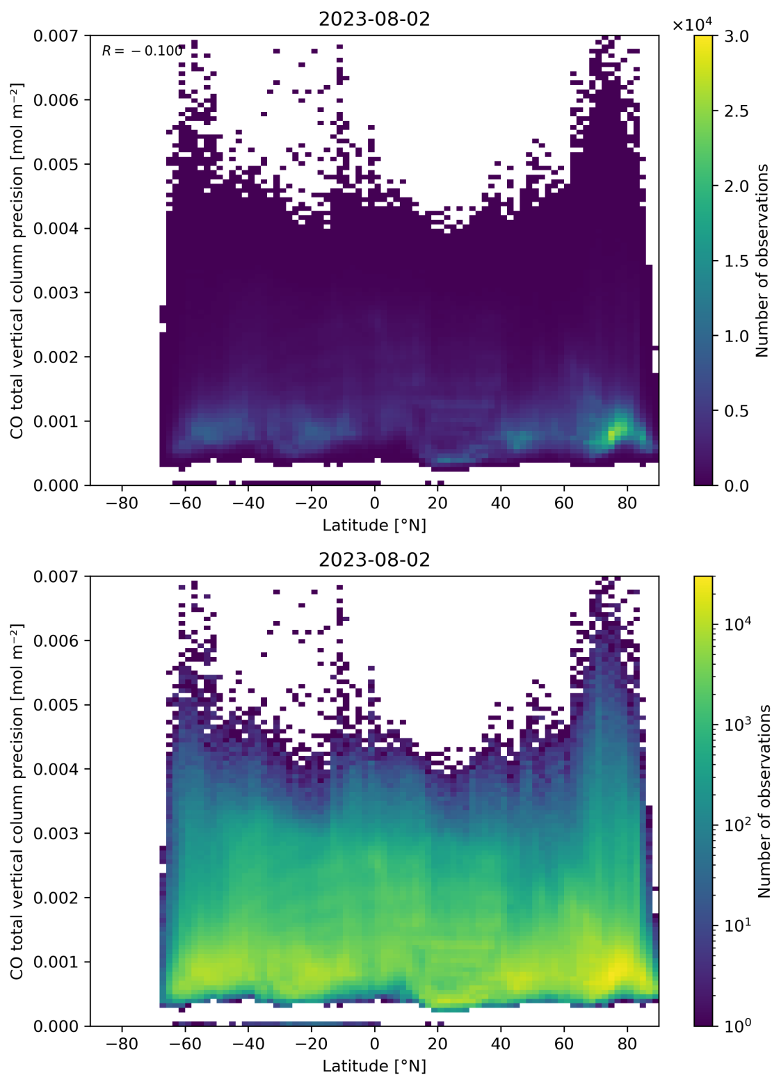
Figure 53: Scatter density plot of “Latitude” against “CO total vertical column precision” for 2023-08-01 to 2023-08-03.
