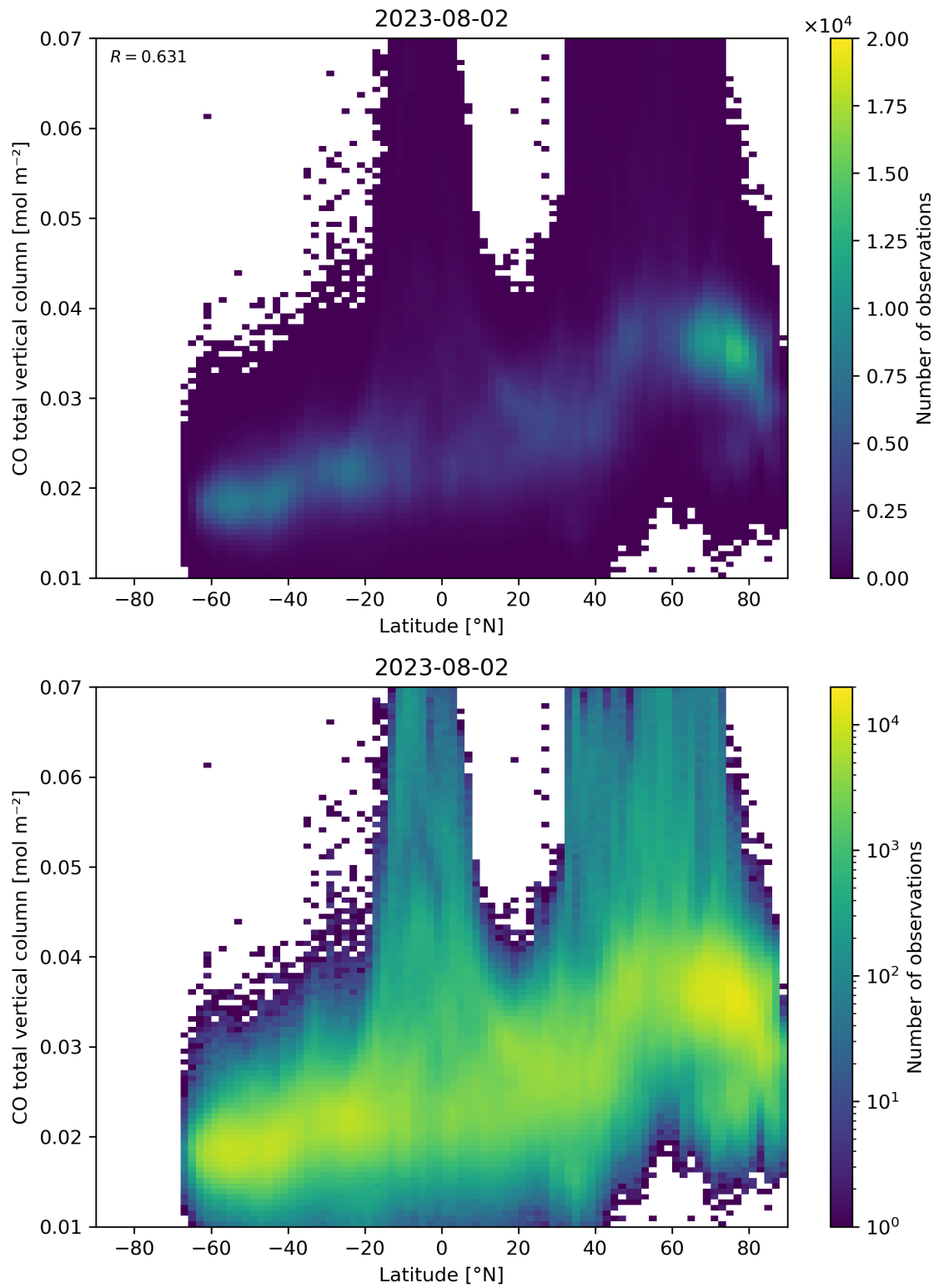
Figure 51: Scatter density plot of “Latitude” against “CO total vertical column” for 2023-08-01 to 2023-08-03.
