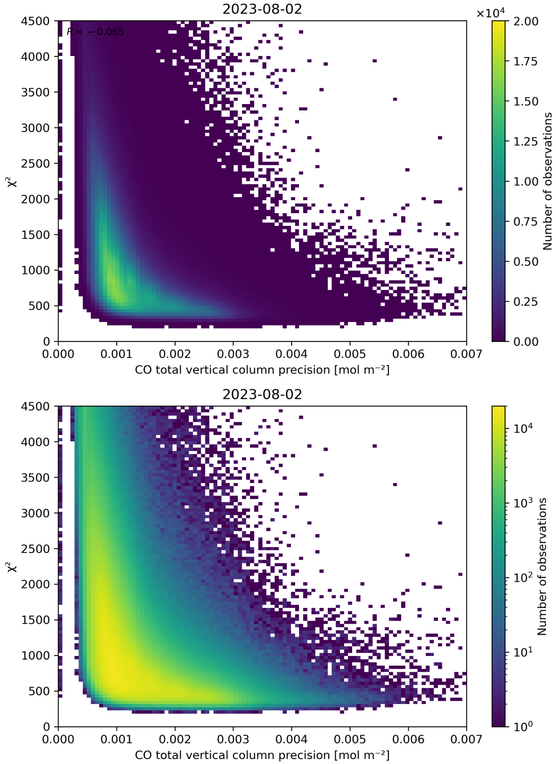
Figure 44: Scatter density plot of “CO total vertical column precision” against “ \chi^2 ” for 2023-08-01 to 2023-08-03.
