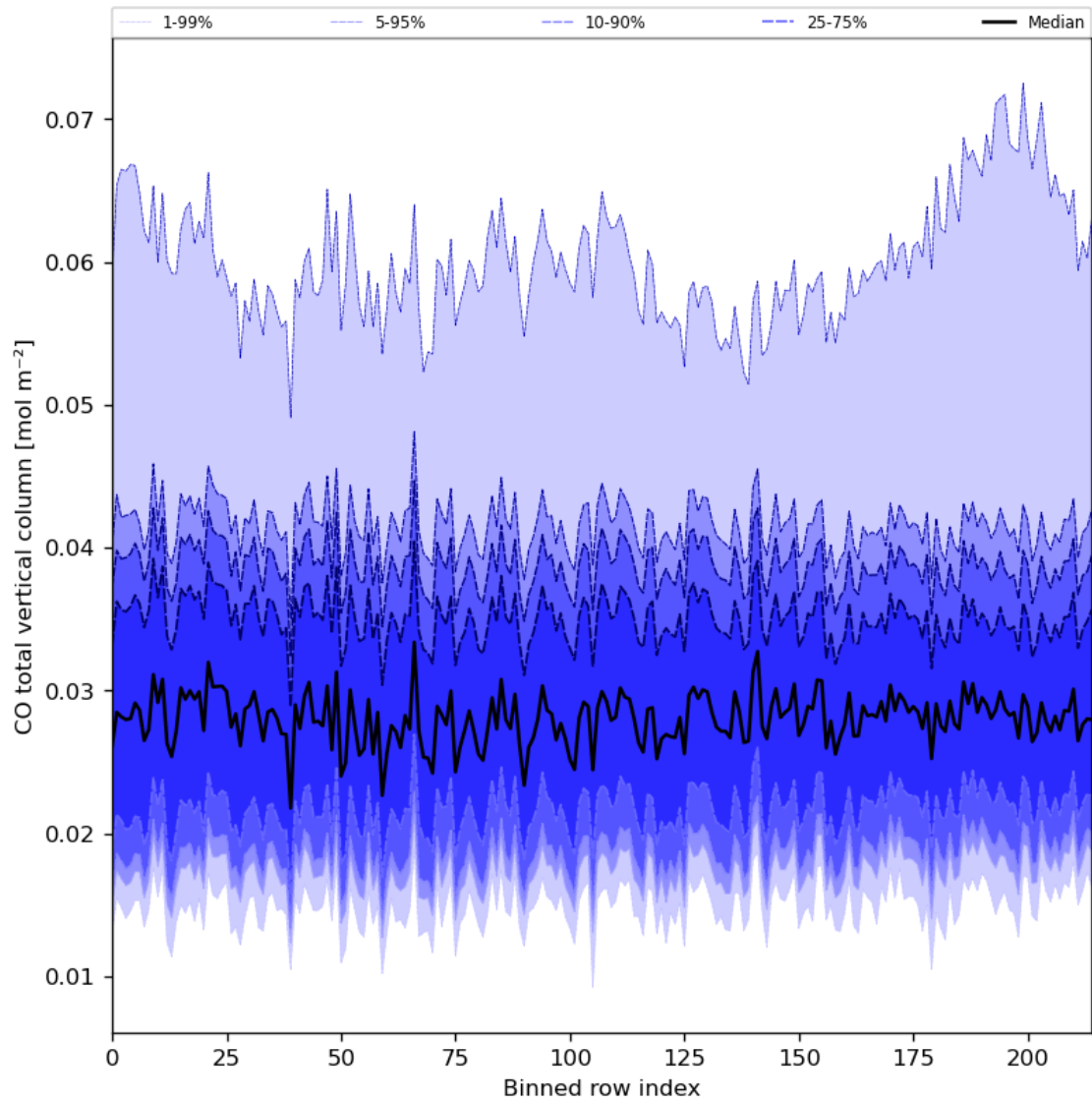
Figure 26: Along track statistics of “CO total vertical column” for 2023-08-01 to 2023-08-03
