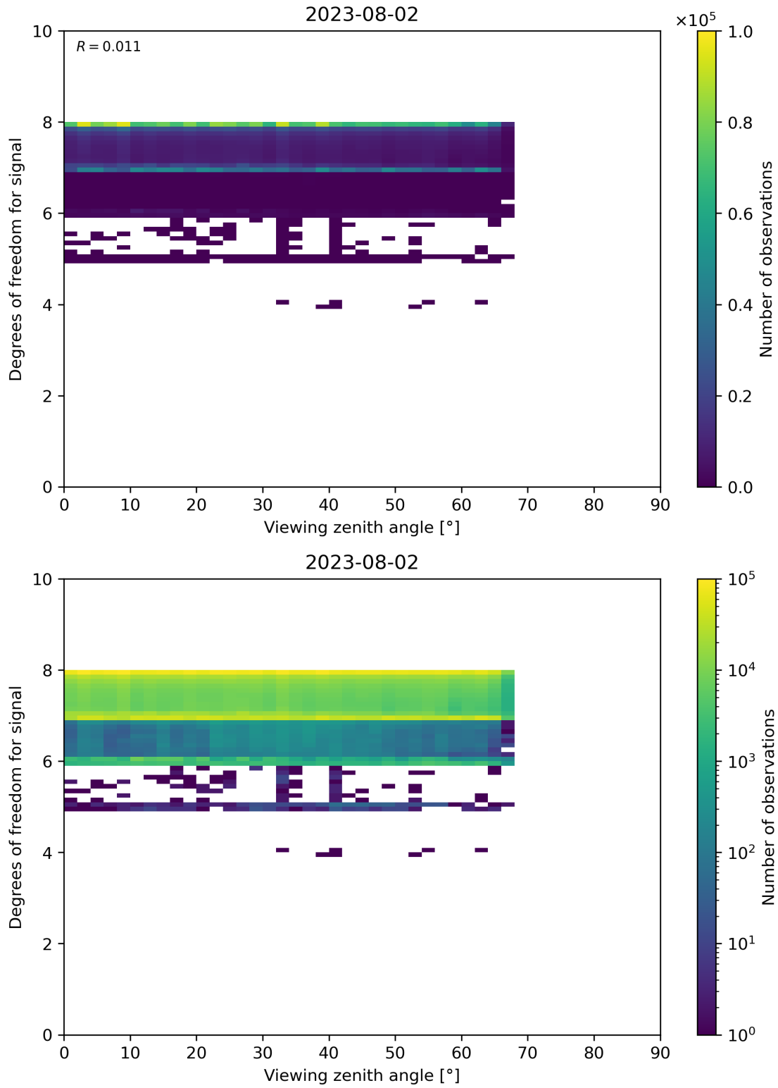
Figure 73: Scatter density plot of “Viewing zenith angle” against “Degrees of freedom for signal” for 2023-08-01 to 2023-08-03.
