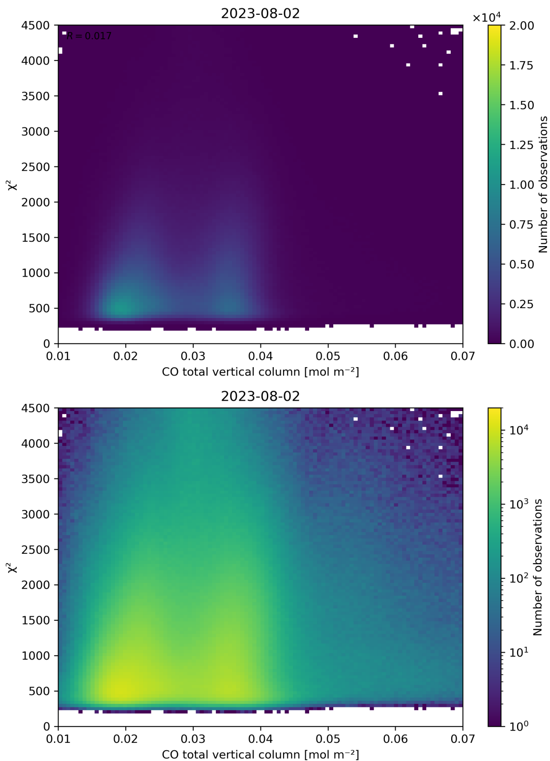
Figure 35: Scatter density plot of “CO total vertical column” against “ \chi^2 ” for 2023-08-01 to 2023-08-03.
