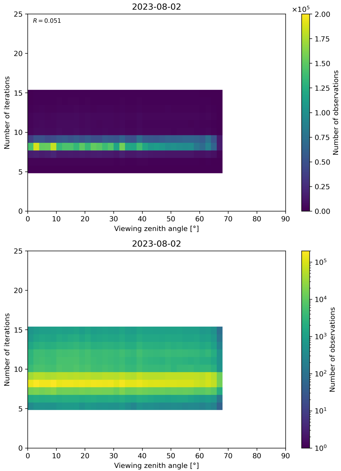
Figure 75: Scatter density plot of “Viewing zenith angle” against “Number of iterations” for 2023-08-01 to 2023-08-03.
