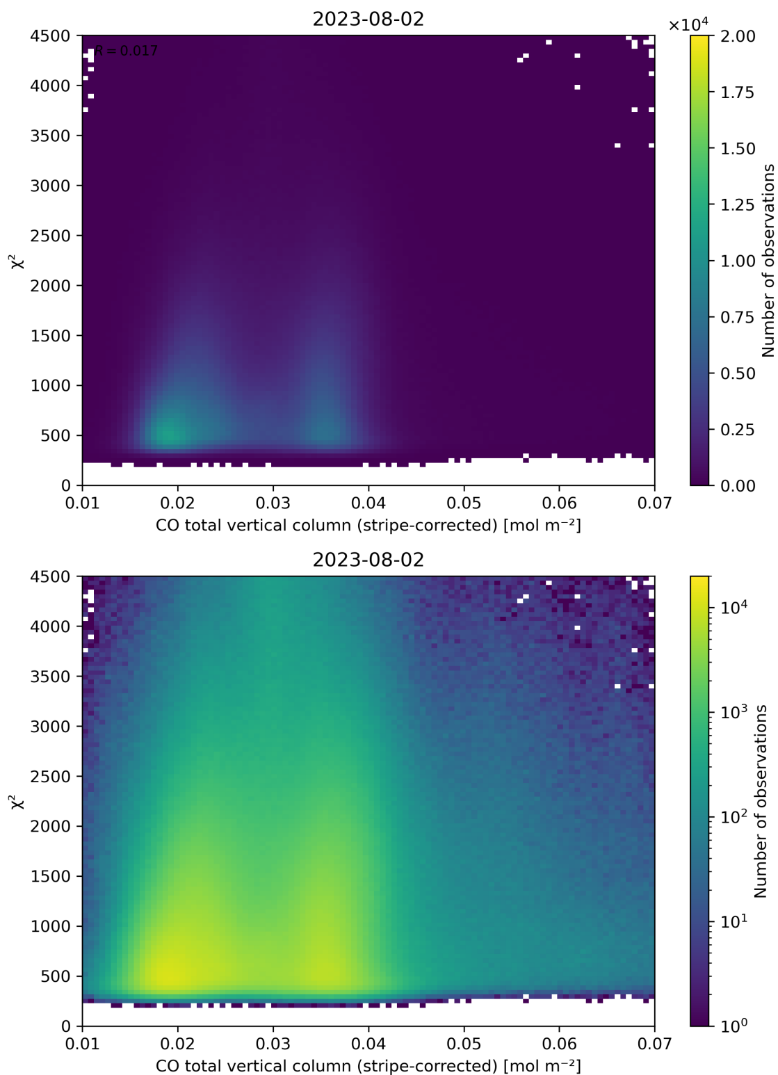
Figure 37: Scatter density plot of “CO total vertical column (stripe-corrected)” against “ \chi^2 ” for 2023-08-01 to 2023-08-03.
