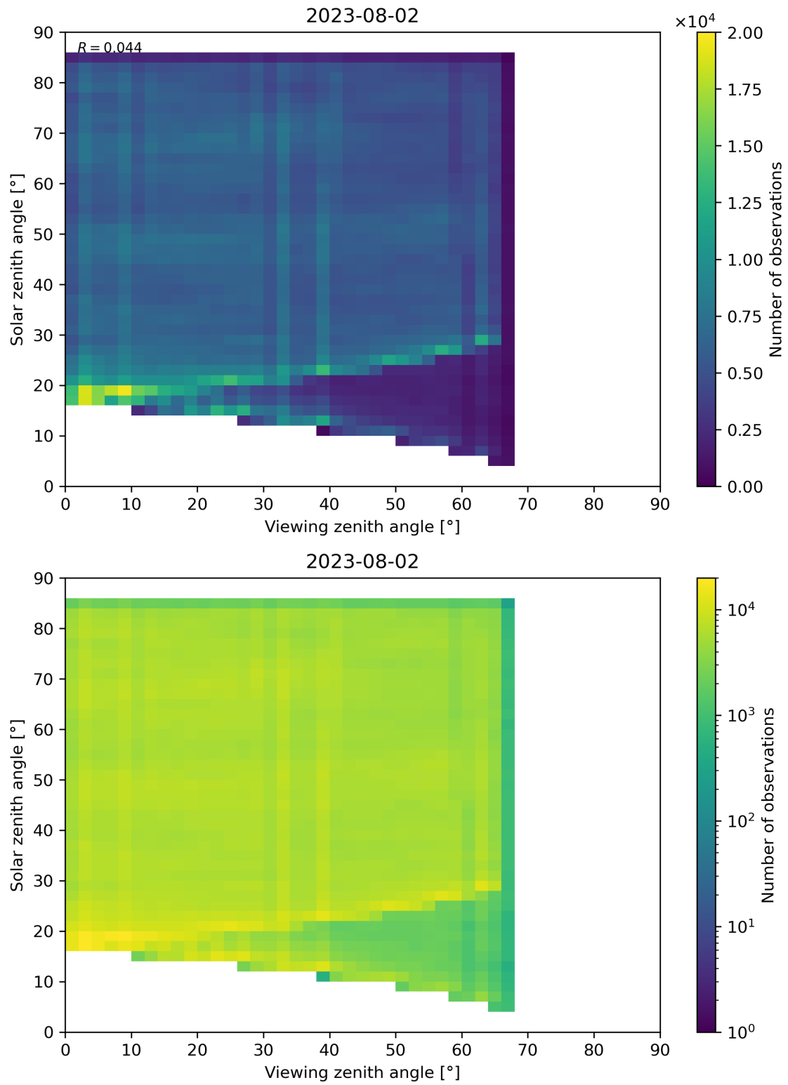
Figure 77: Scatter density plot of “Viewing zenith angle” against “Solar zenith angle” for 2023-08-01 to 2023-08-03.
