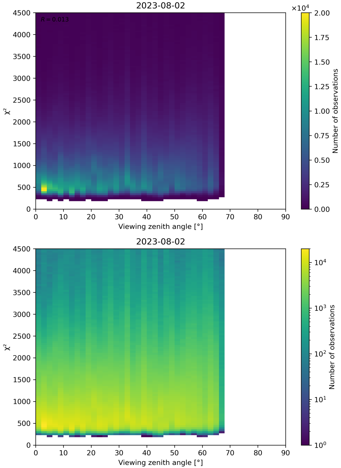
Figure 72: Scatter density plot of “Viewing zenith angle” against “ \chi^2 ” for 2023-08-01 to 2023-08-03.
