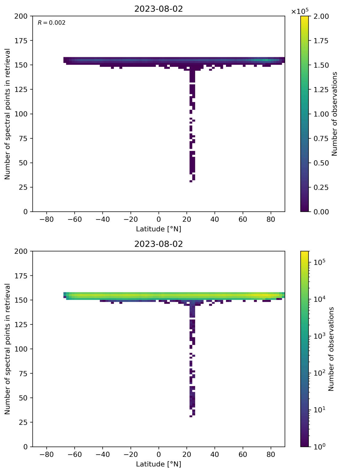
Figure 57: Scatter density plot of “Latitude” against “Number of spectral points in retrieval” for 2023-08-01 to 2023-08-03.
