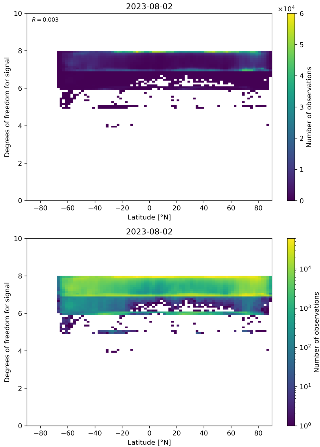
Figure 55: Scatter density plot of “Latitude” against “Degrees of freedom for signal” for 2023-08-01 to 2023-08-03.
