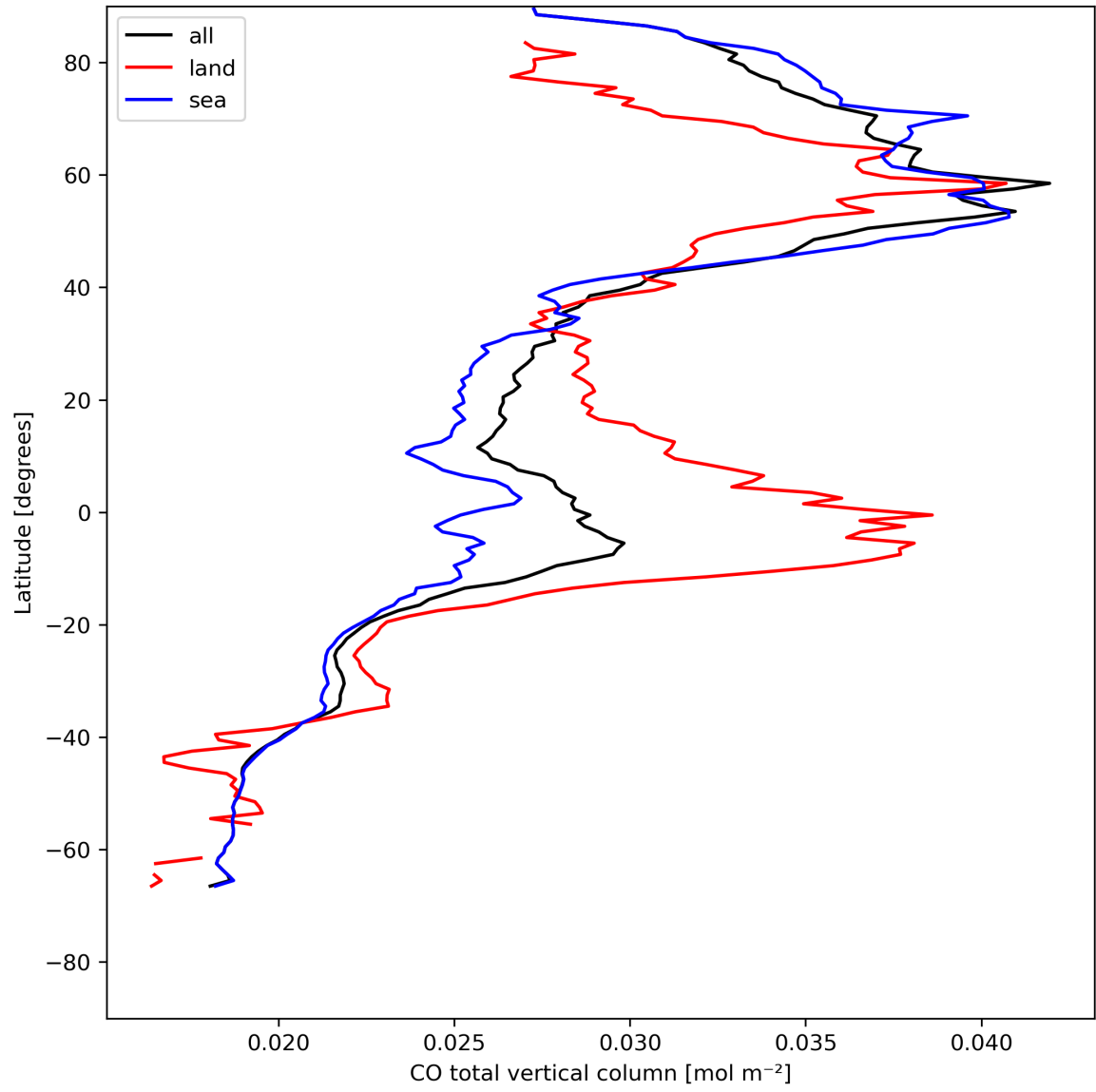
Figure 10: Zonal average of “CO total vertical column” for 2023-08-01 to 2023-08-03.
