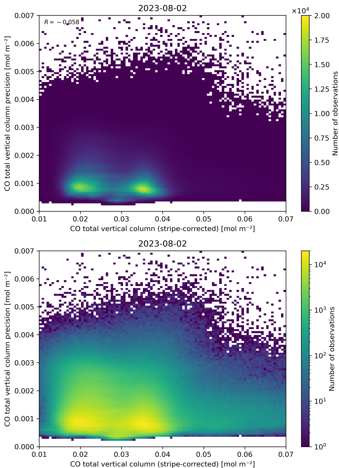
Figure 36: Scatter density plot of “CO total vertical column (stripe-corrected)” against “CO total vertical column precision” for 2023-08-01 to 2023-08-03.
