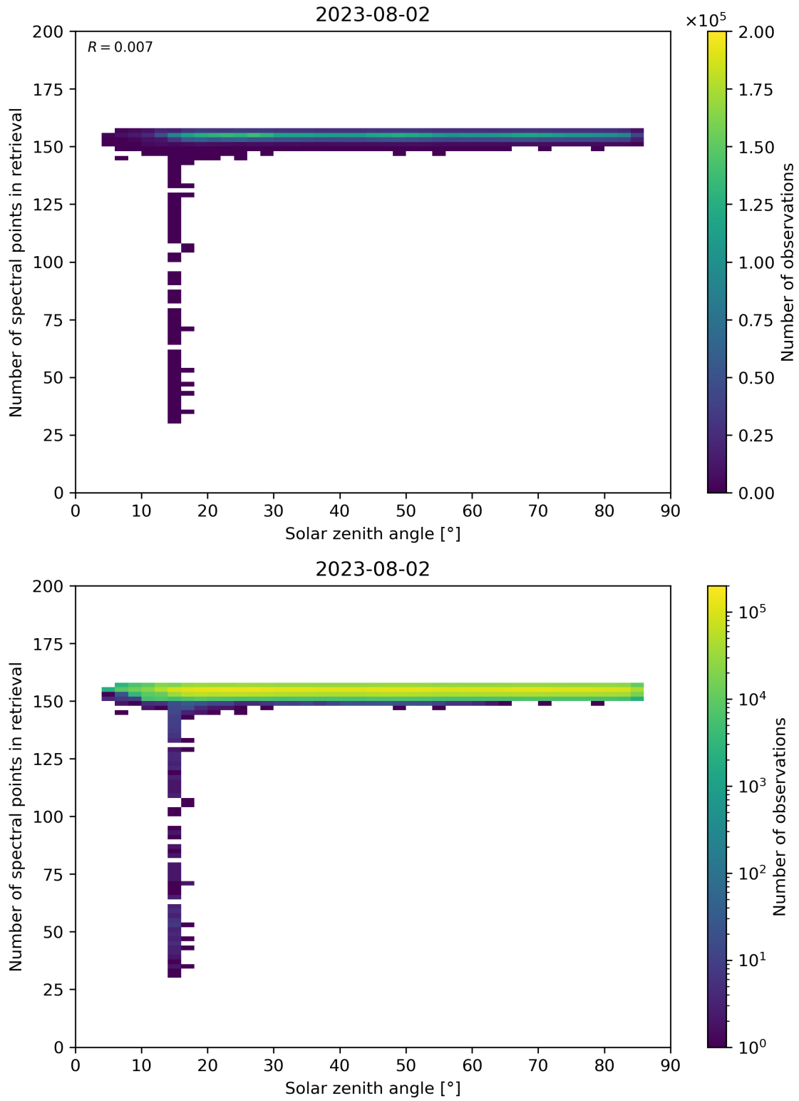
Figure 68: Scatter density plot of “Solar zenith angle” against “Number of spectral points in retrieval” for 2023-08-01 to 2023-08-03.
