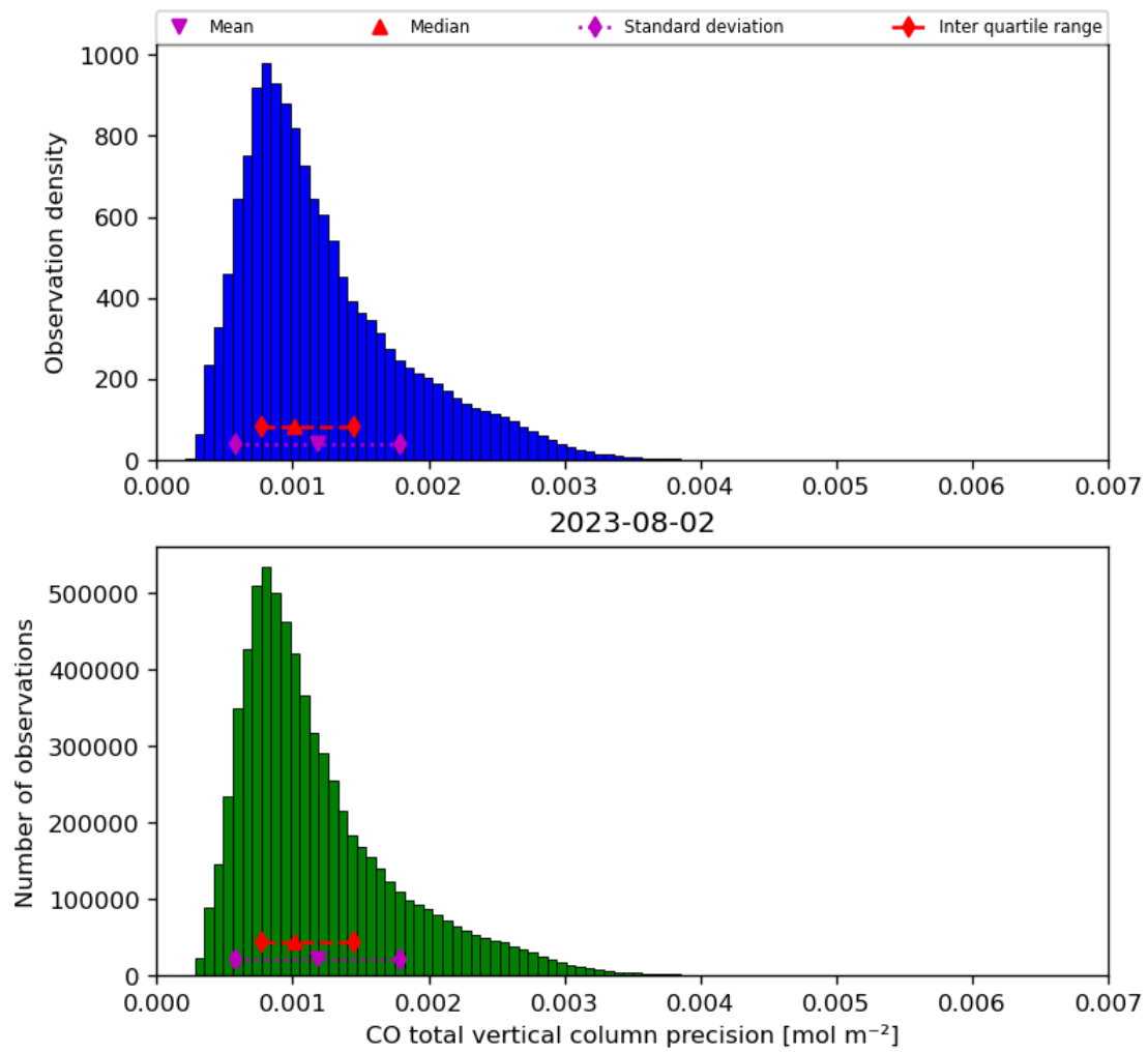
Figure 20: Histogram of “CO total vertical column precision” for 2023-08-01 to 2023-08-03
