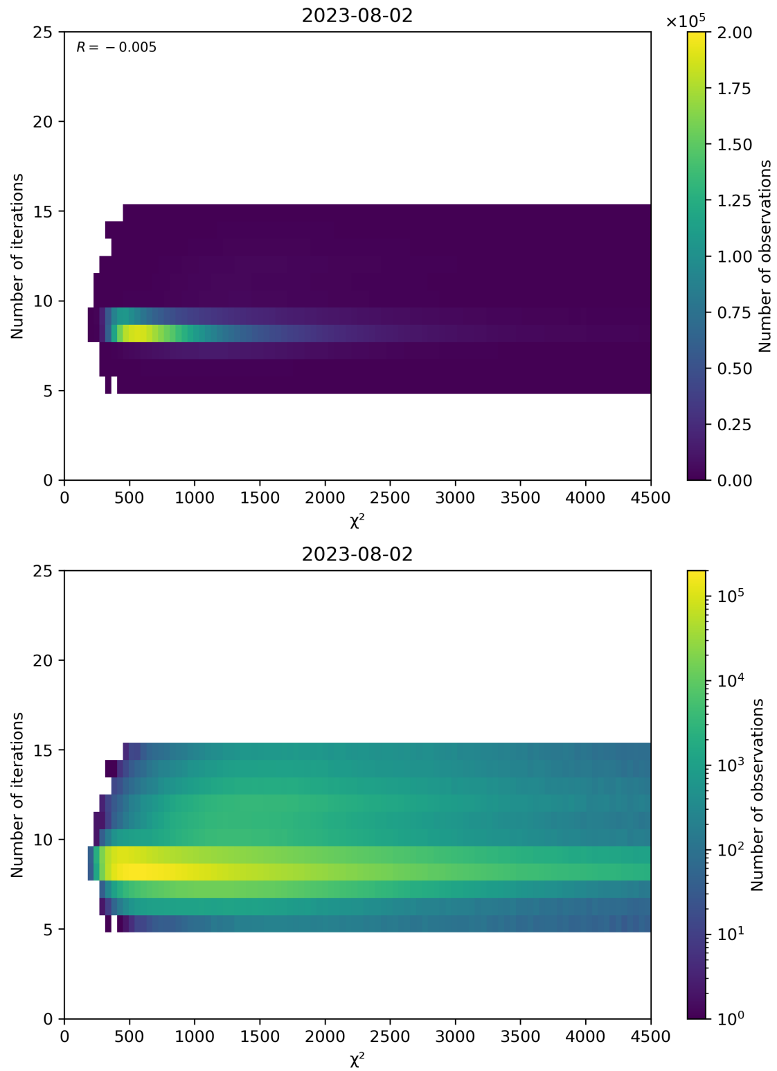
Figure 49: Scatter density plot of “ \chi^2 ” against “Number of iterations” for 2023-08-01 to 2023-08-03.
