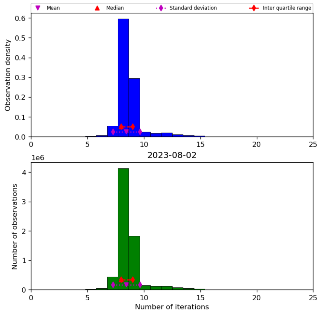
Figure 24: Histogram of "Number of iterations" for 2023-08-01 to 2023-08-03
