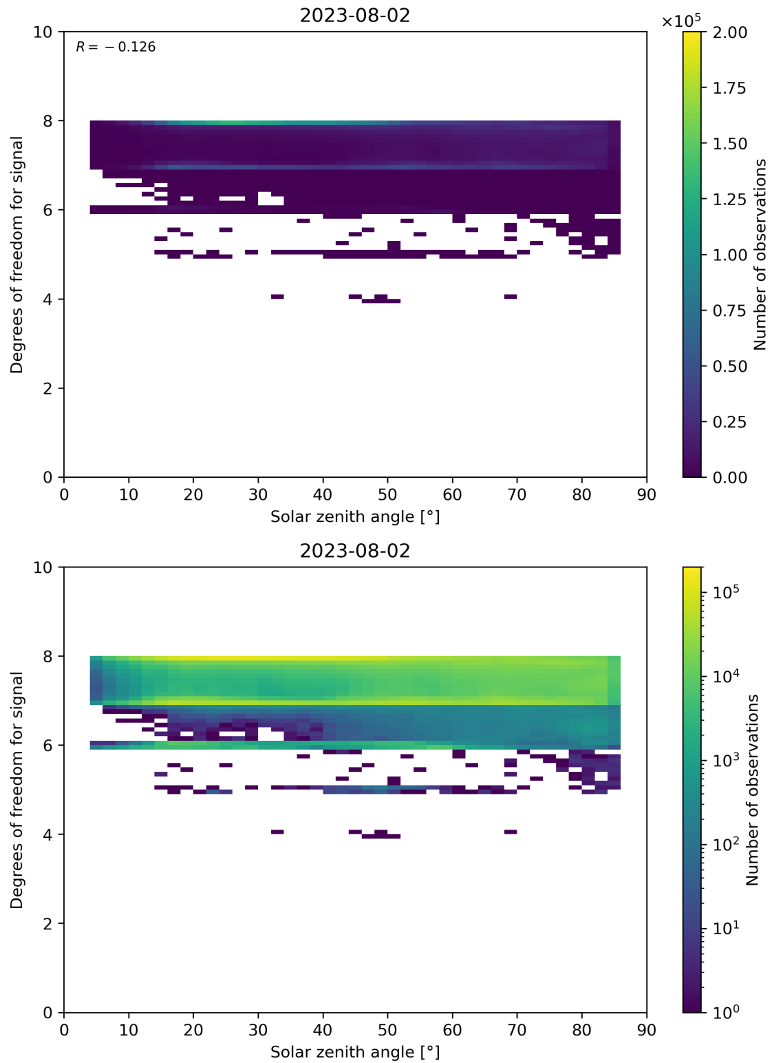
Figure 65: Scatter density plot of “Solar zenith angle” against “Degrees of freedom for signal” for 2023-08-01 to 2023-08-03.
