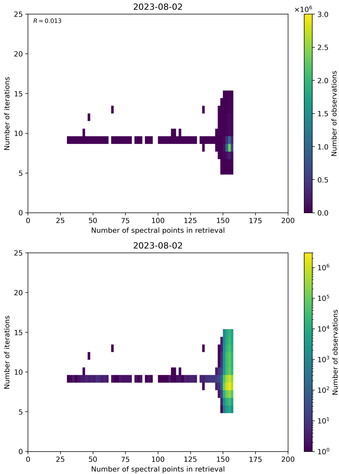
Figure 60: Scatter density plot of “Number of spectral points in retrieval” against “Number of iterations” for 2023-08-01 to 2023-08-03.
