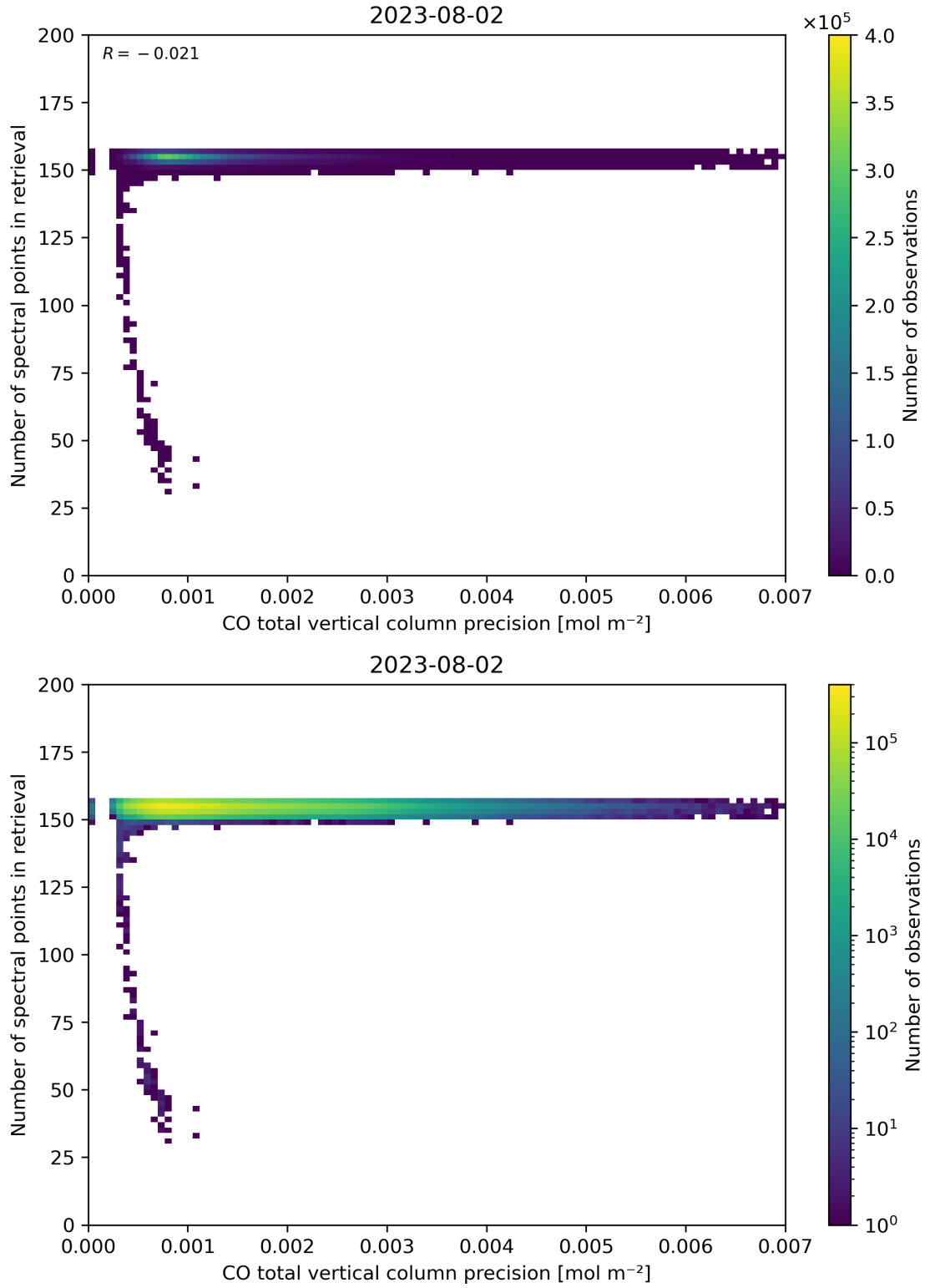
Figure 47: Scatter density plot of “CO total vertical column precision” against “Number of spectral points in retrieval” for 2023-08-01 to 2023-08-03.
