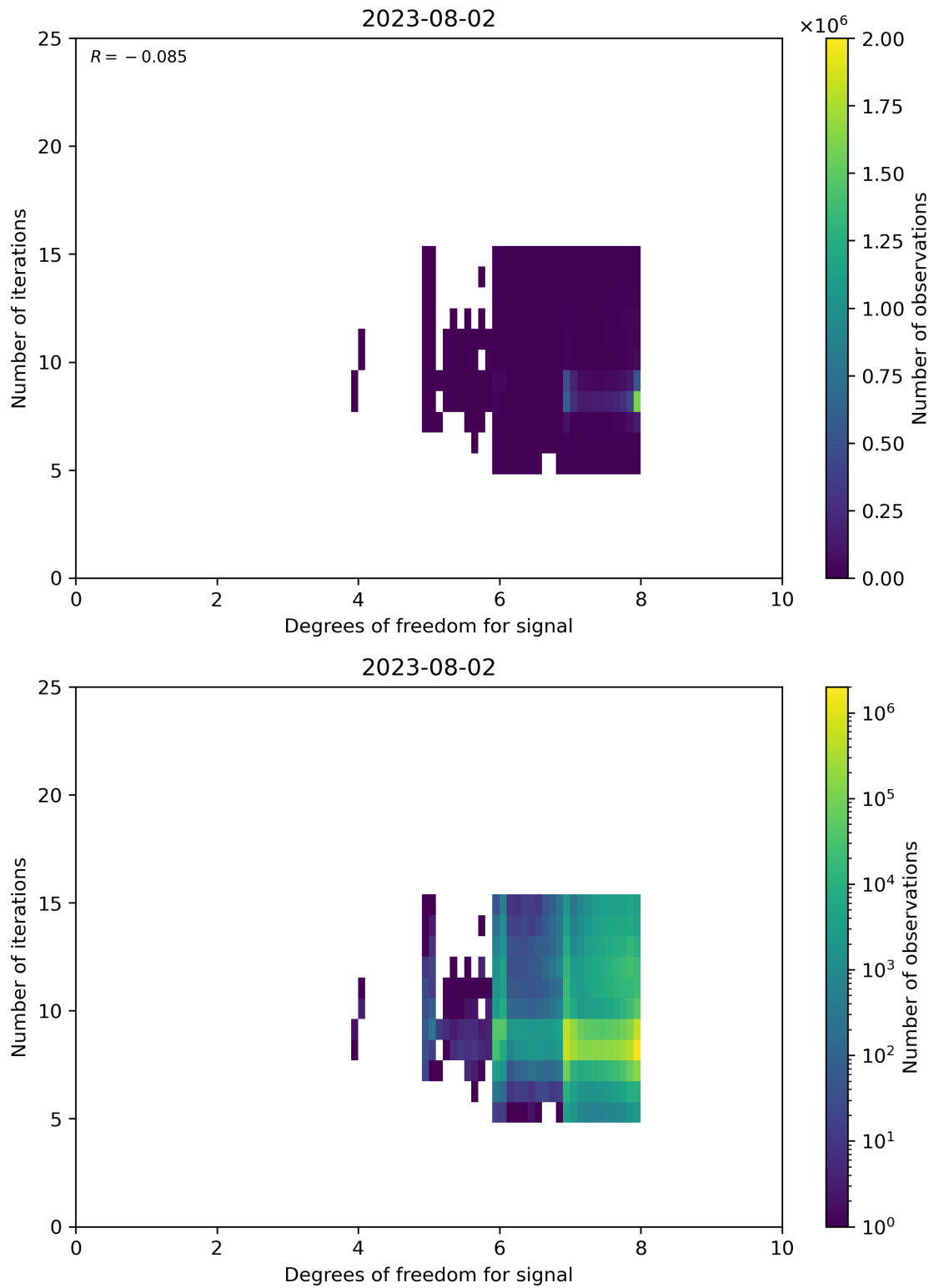
Figure 50: Scatter density plot of “Degrees of freedom for signal” against “Number of iterations” for 2023-08-01 to 2023-08-03.
