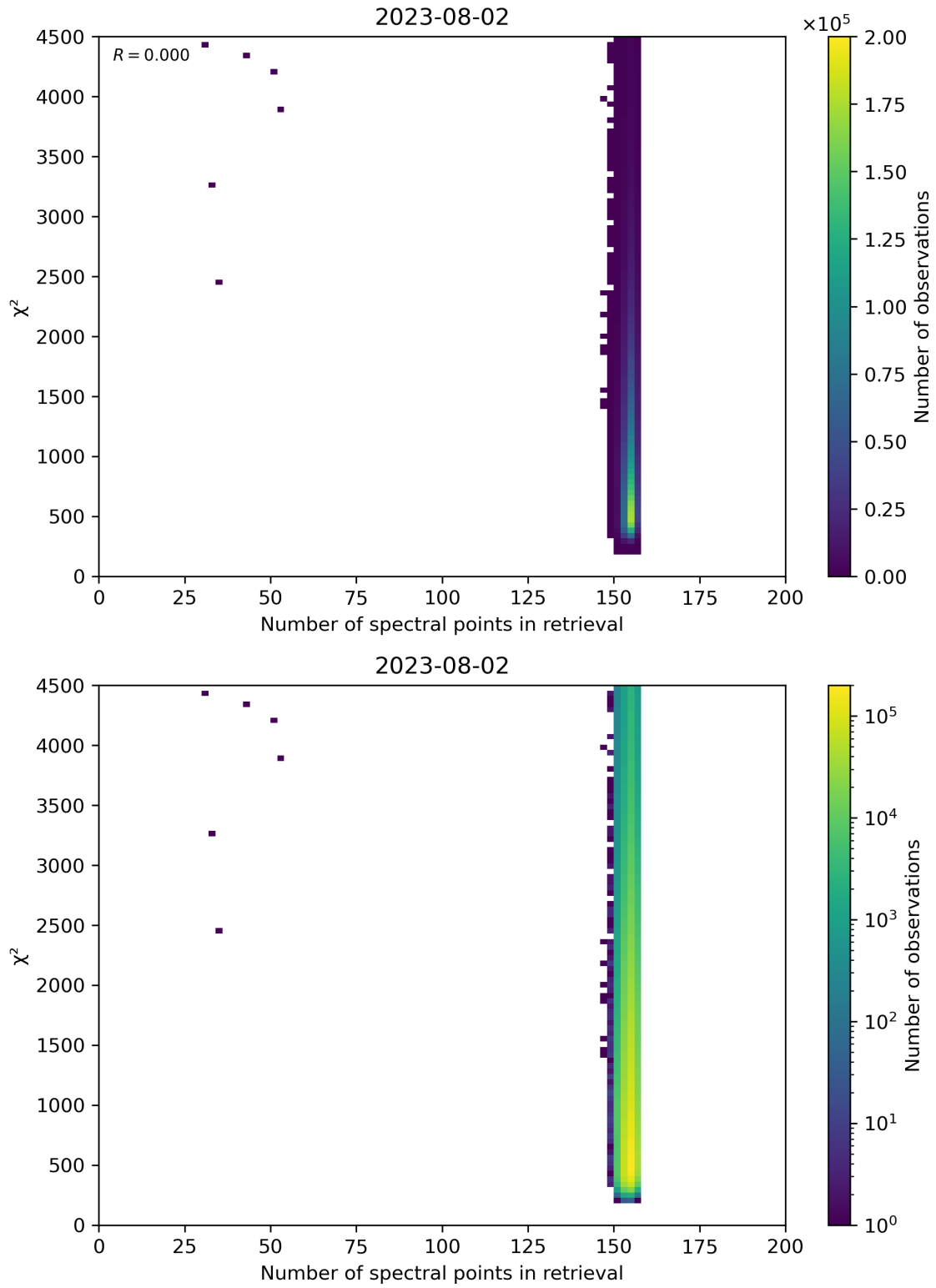
Figure 58: Scatter density plot of “Number of spectral points in retrieval” against “ \chi^2 ” for 2023-08-01 to 2023-08-03.
