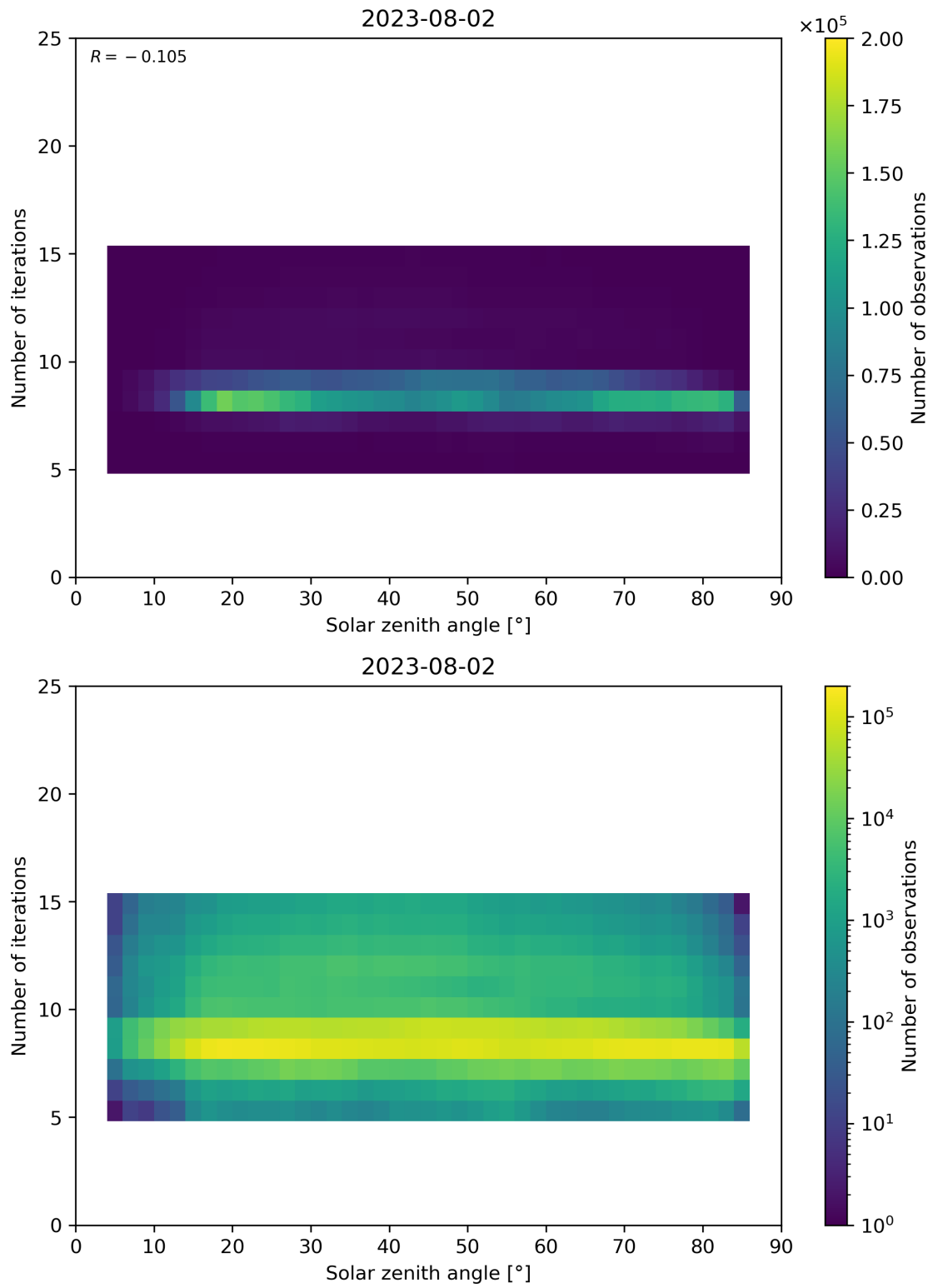
Figure 67: Scatter density plot of “Solar zenith angle” against “Number of iterations” for 2023-08-01 to 2023-08-03.
