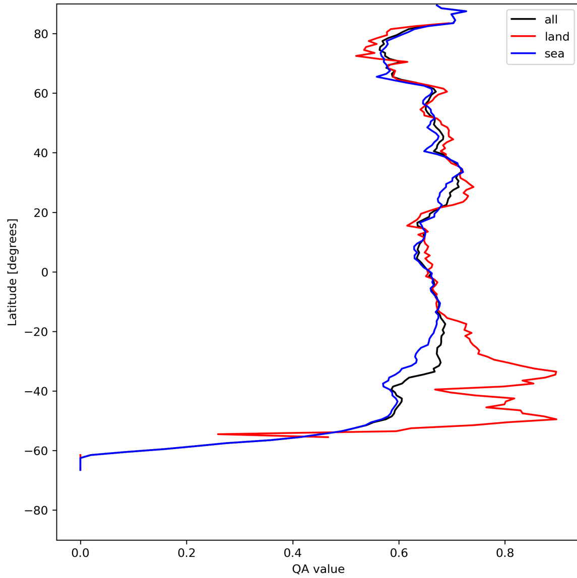
Figure 9: Zonal average of “QA value” for 2023-08-01 to 2023-08-03.
