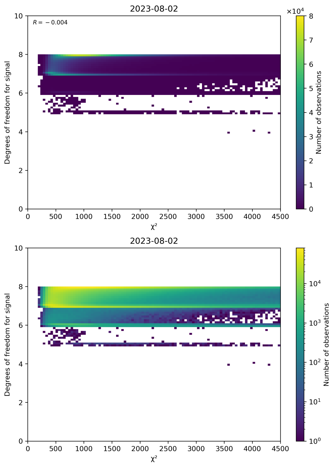
Figure 48: Scatter density plot of “ \chi^2 ” against “Degrees of freedom for signal” for 2023-08-01 to 2023-08-03.
