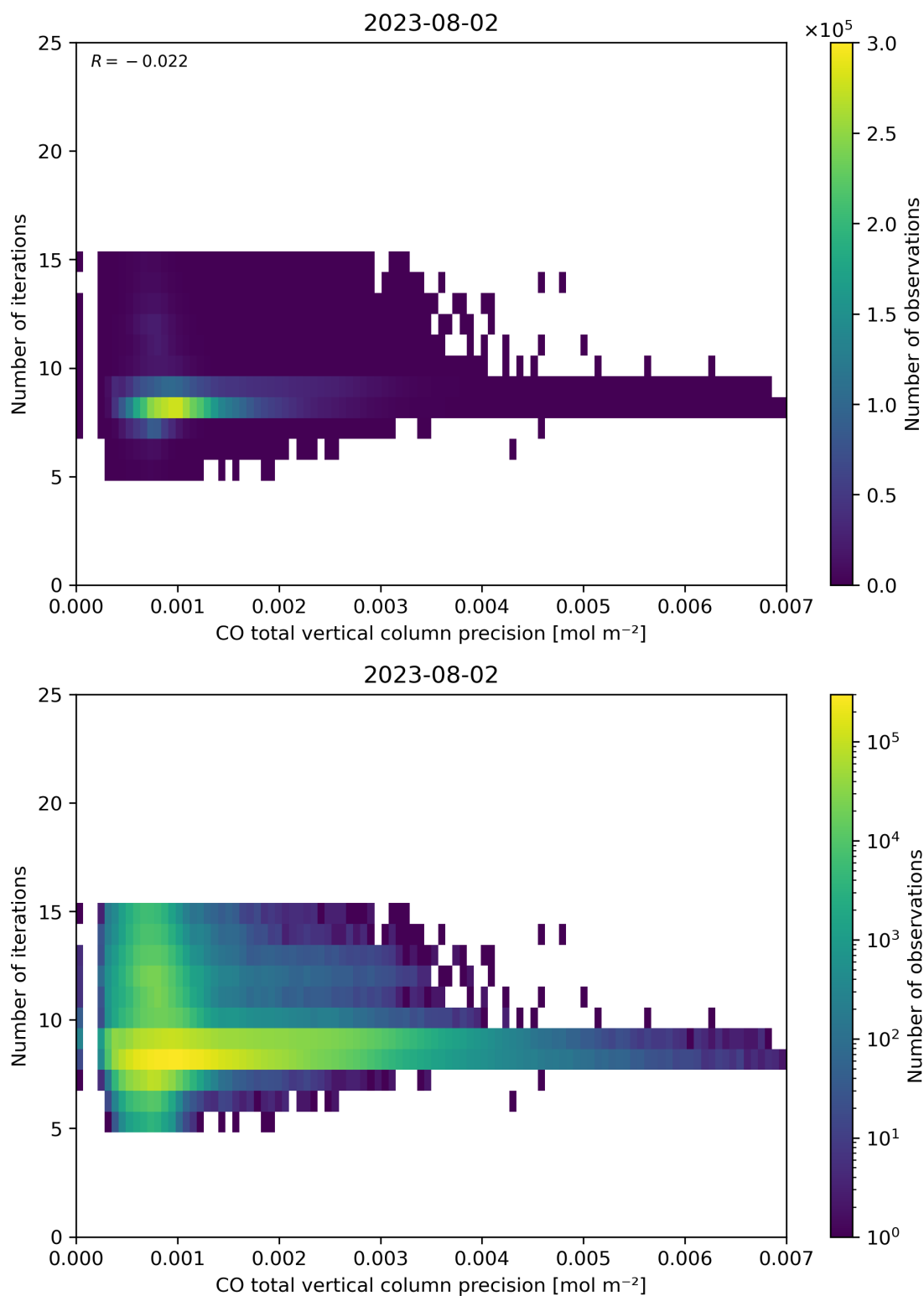
Figure 46: Scatter density plot of “CO total vertical column precision” against “Number of iterations” for 2023-08-01 to 2023-08-03.
