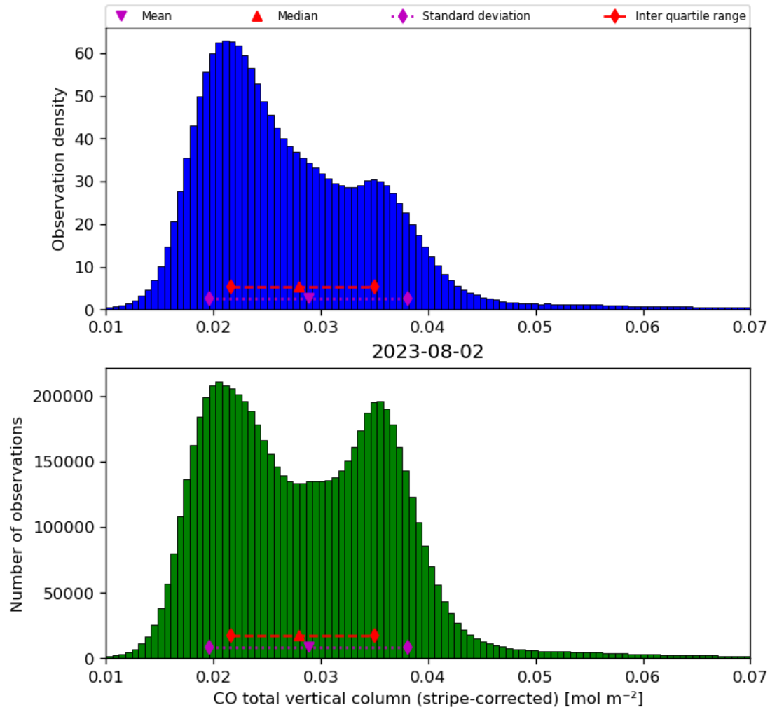
Figure 19: Histogram of “CO total vertical column (stripe-corrected)” for 2023-08-01 to 2023-08-03
