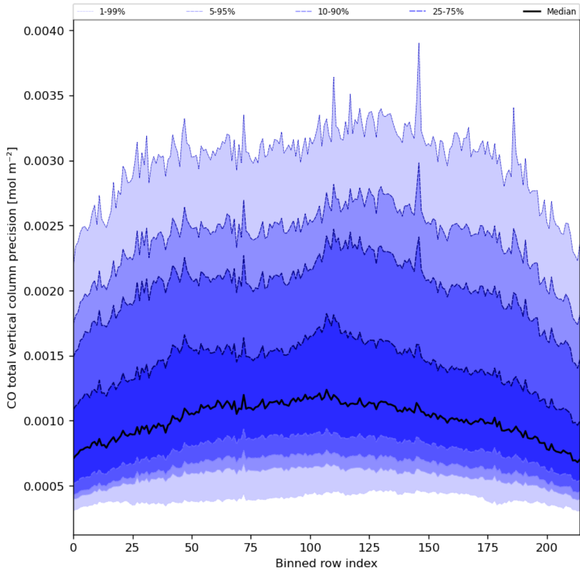
Figure 28: Along track statistics of “CO total vertical column precision” for 2023-08-01 to 2023-08-03
