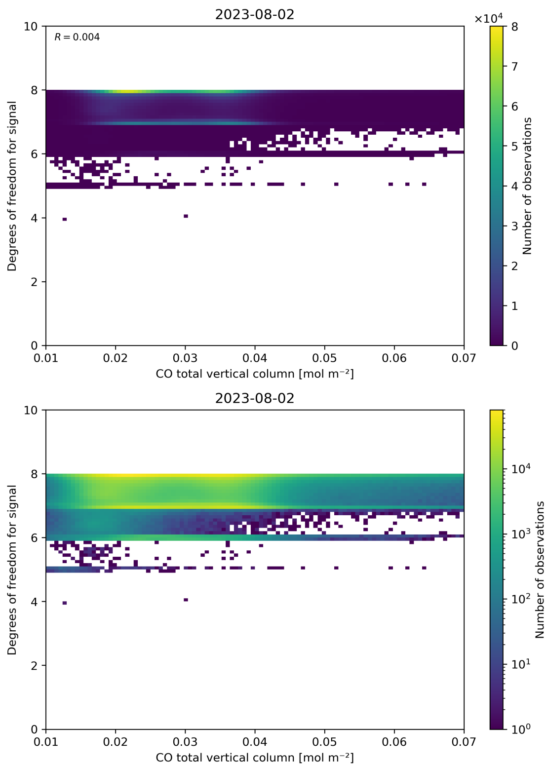
Figure 41: Scatter density plot of “CO total vertical column” against “Degrees of freedom for signal” for 2023-08-01 to 2023-08-03.
