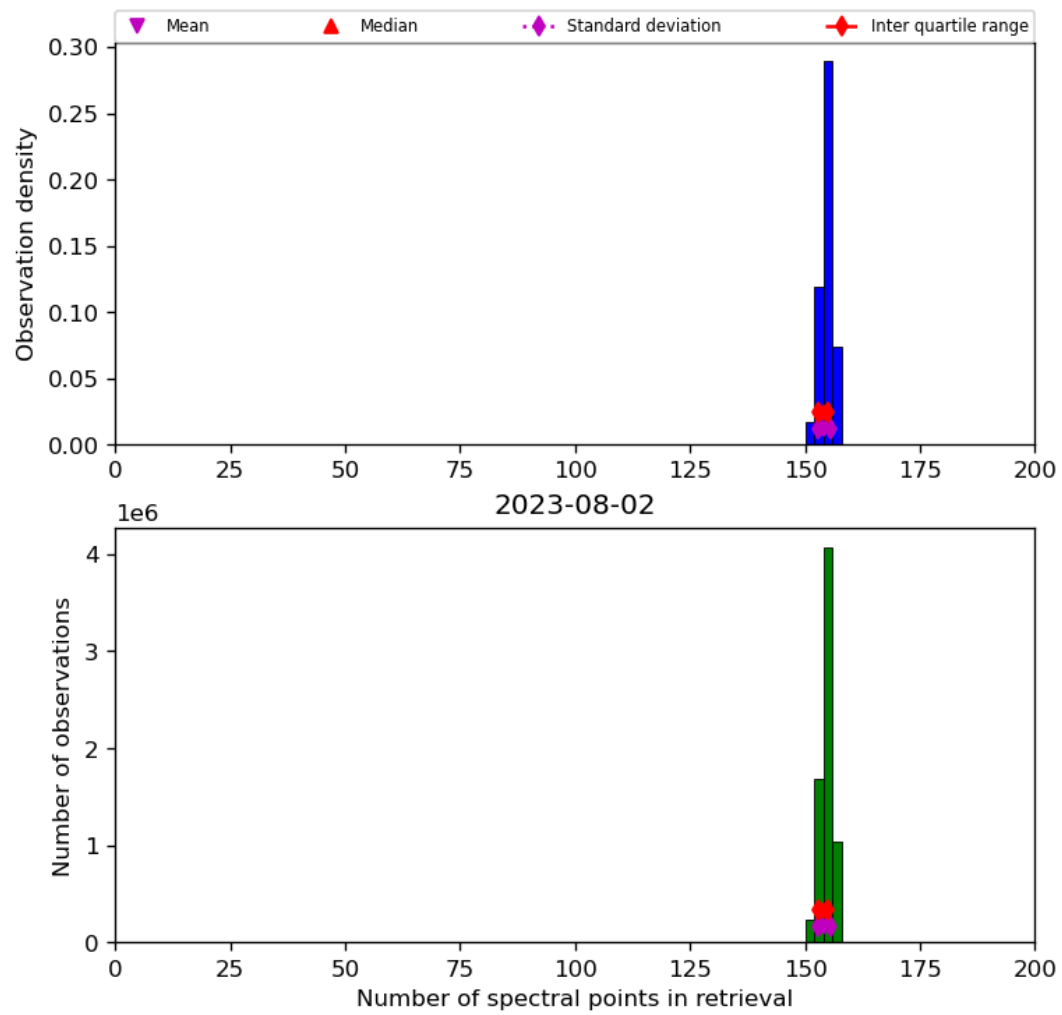
Figure 21: Histogram of “Number of spectral points in retrieval” for 2023-08-01 to 2023-08-03
