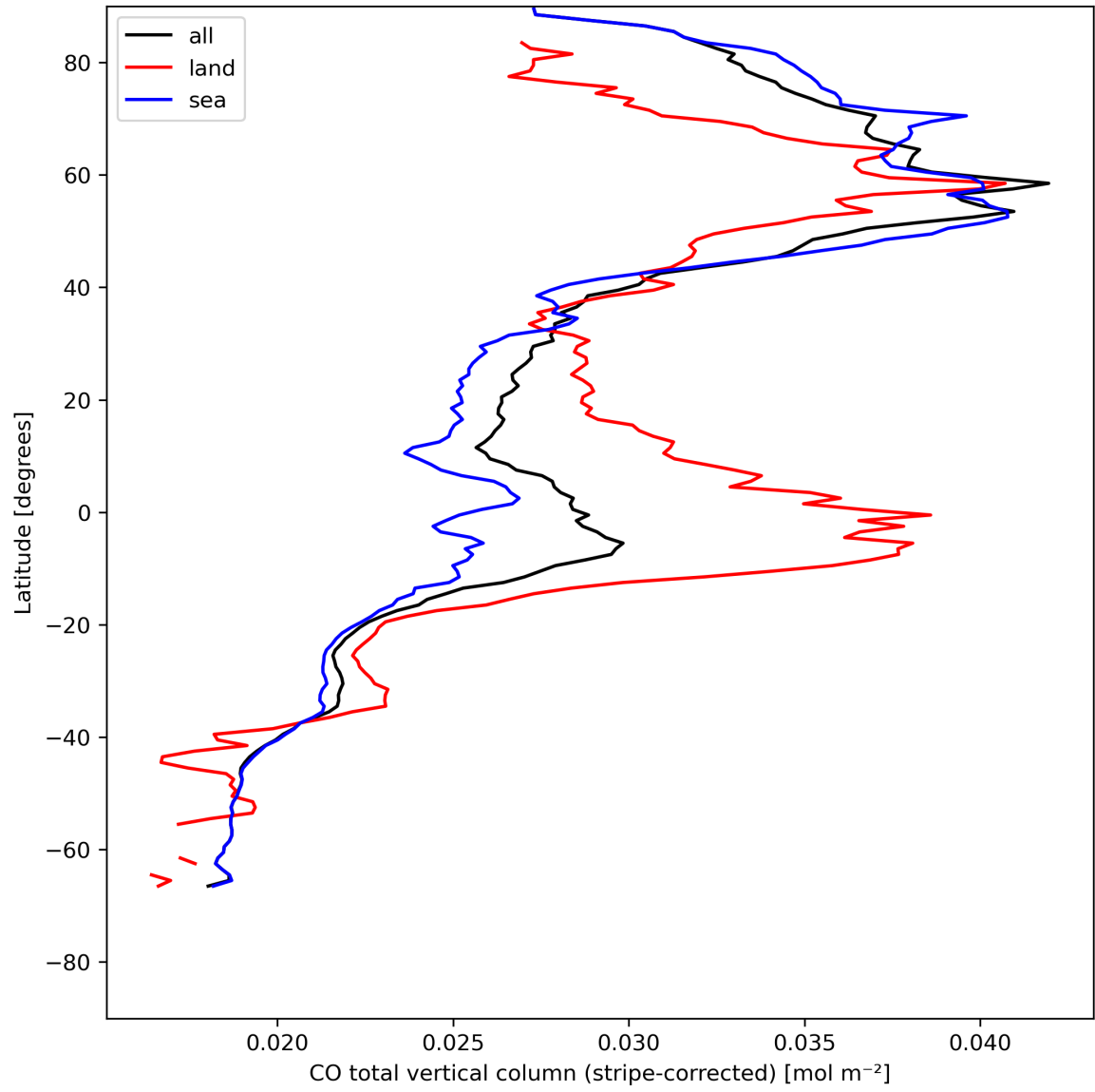
Figure 11: Zonal average of “CO total vertical column (stripe-corrected)” for 2023-08-01 to 2023-08-03.
