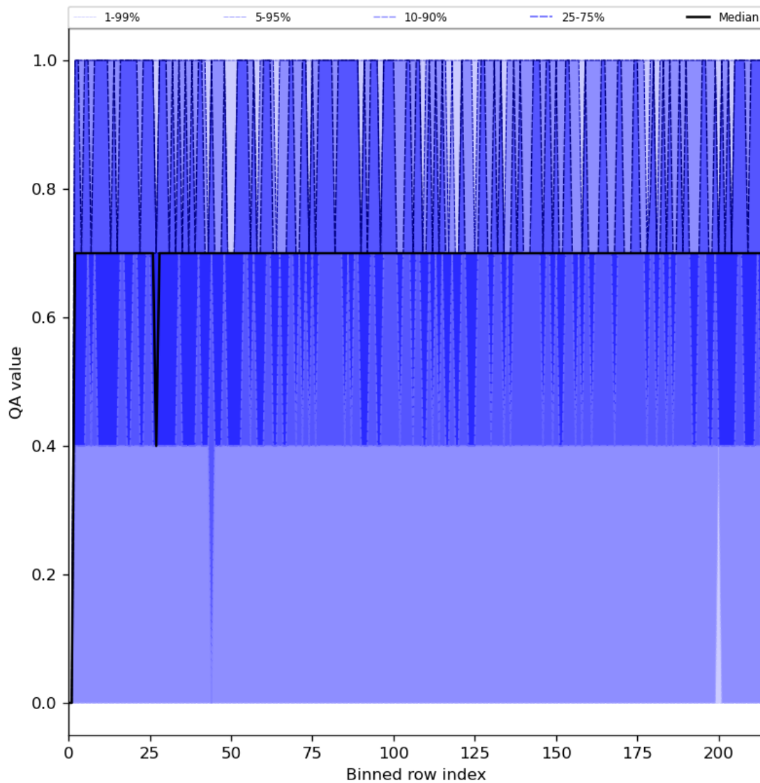
Figure 25: Along track statistics of “QA value” for 2023-08-01 to 2023-08-03
