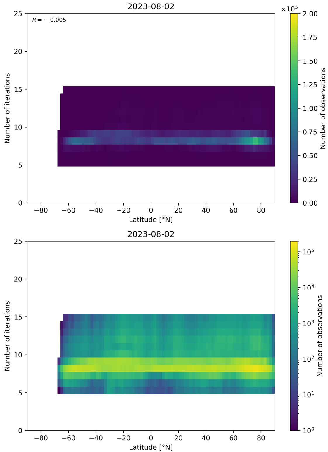
Figure 56: Scatter density plot of “Latitude” against “Number of iterations” for 2023-08-01 to 2023-08-03.
