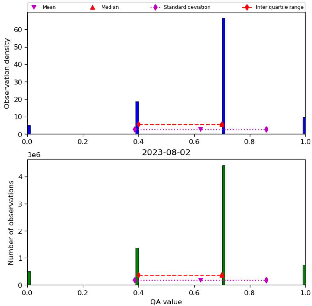
Figure 17: Histogram of “QA value” for 2023-08-01 to 2023-08-03
