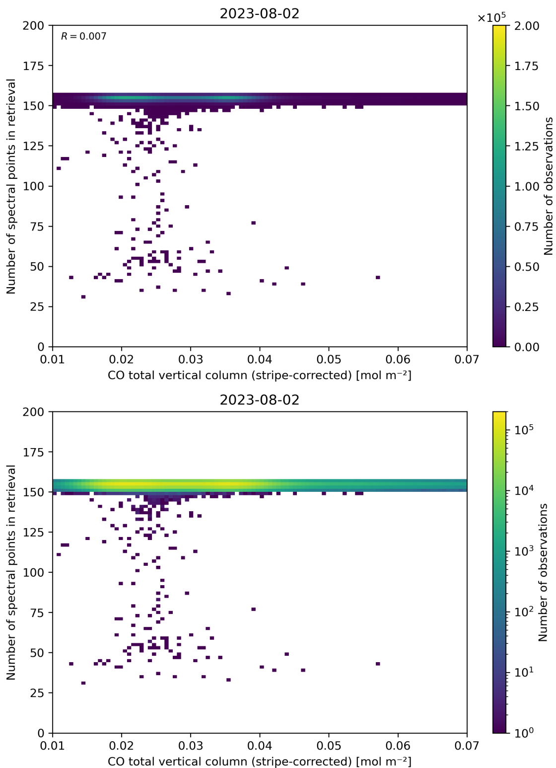
Figure 40: Scatter density plot of “CO total vertical column (stripe-corrected)” against “Number of spectral points in retrieval” for 2023-08-01 to 2023-08-03.
