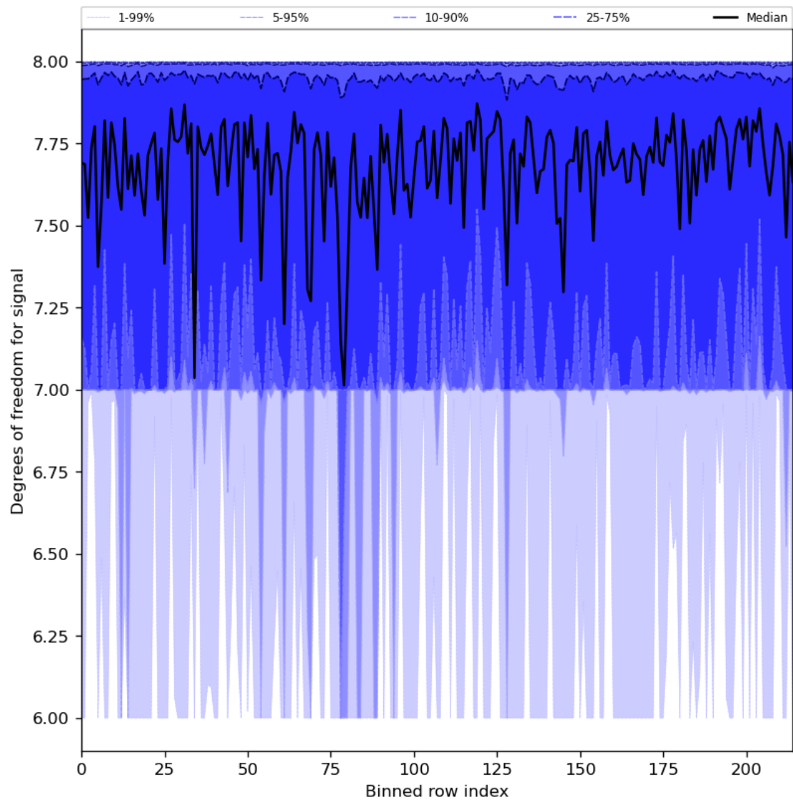
Figure 31: Along track statistics of “Degrees of freedom for signal” for 2023-08-01 to 2023-08-03
