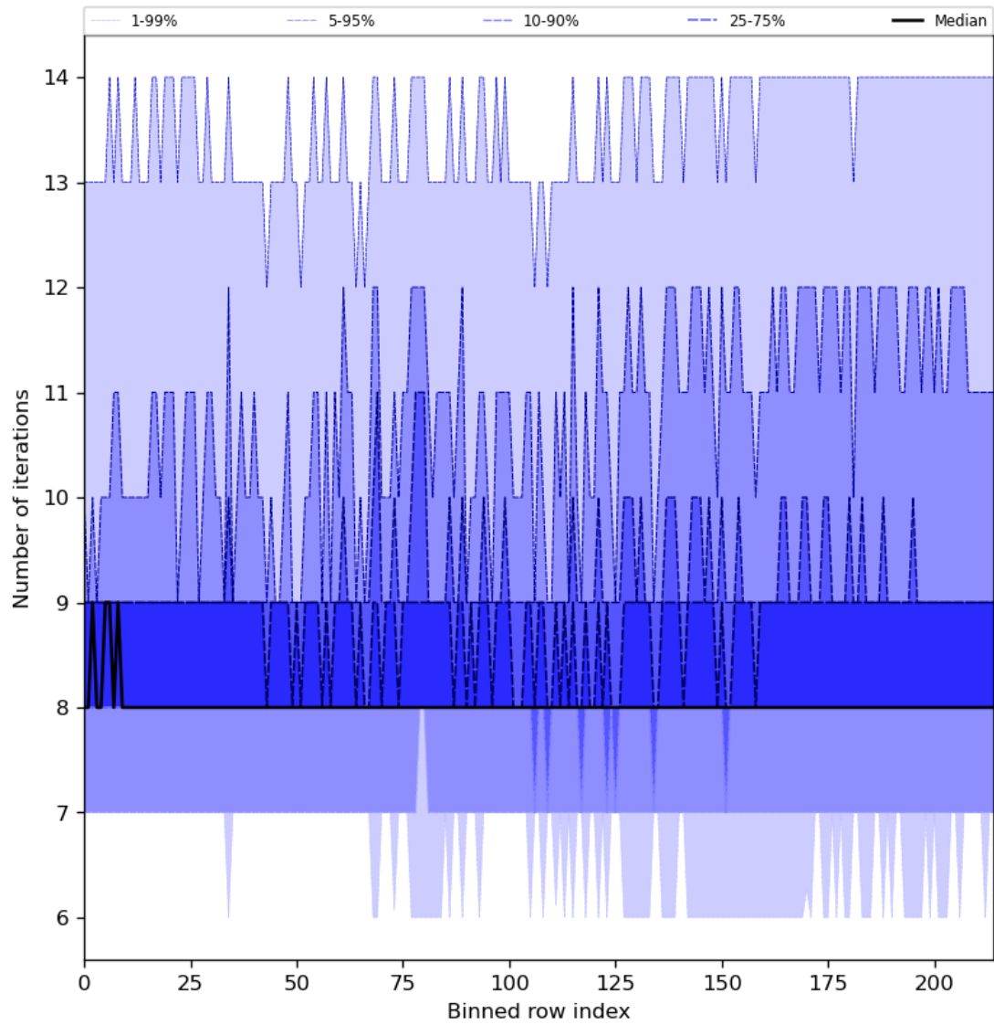
Figure 32: Along track statistics of “Number of iterations” for 2023-08-01 to 2023-08-03
