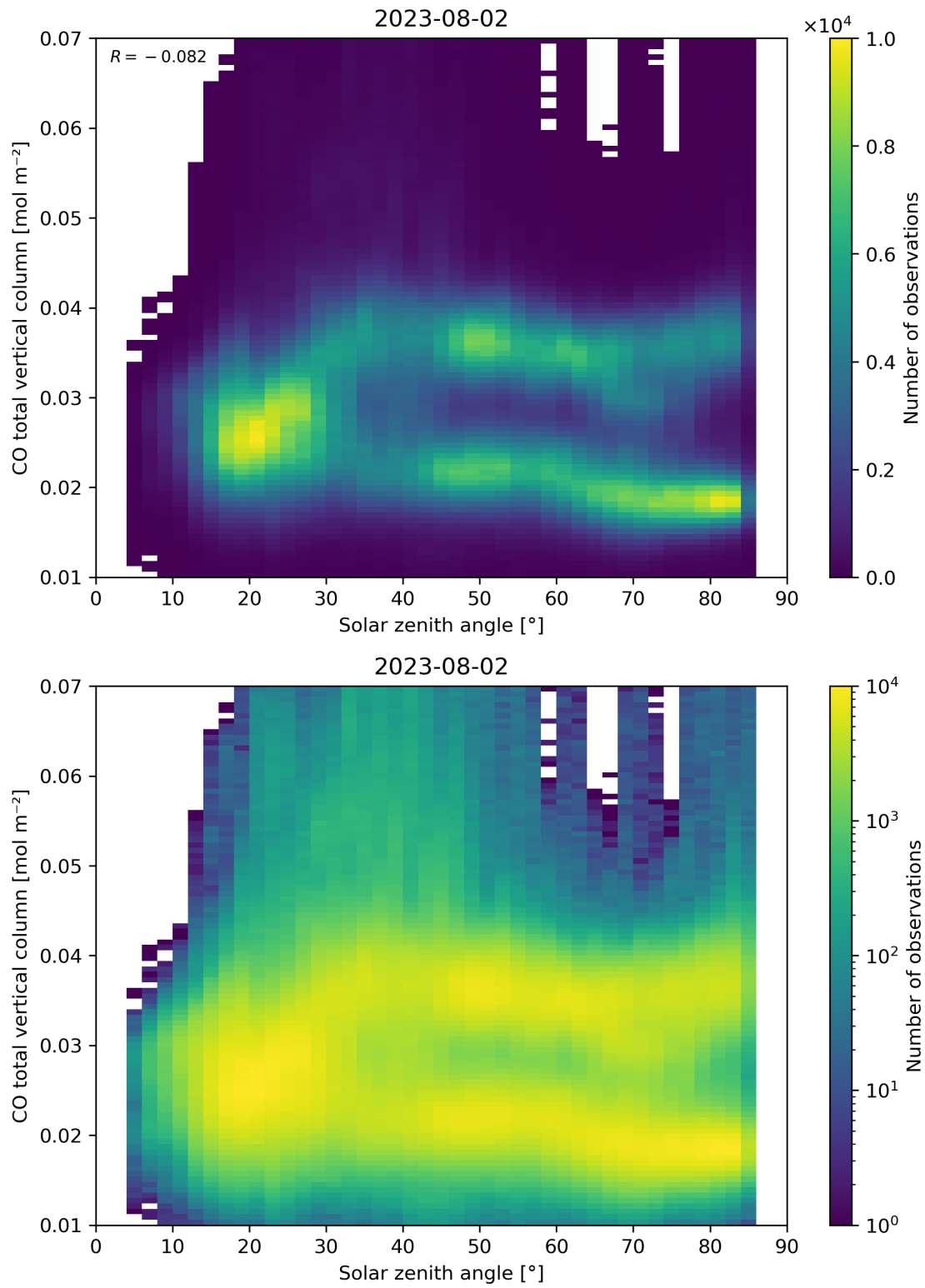
Figure 61: Scatter density plot of “Solar zenith angle” against “CO total vertical column” for 2023-08-01 to 2023-08-03.
