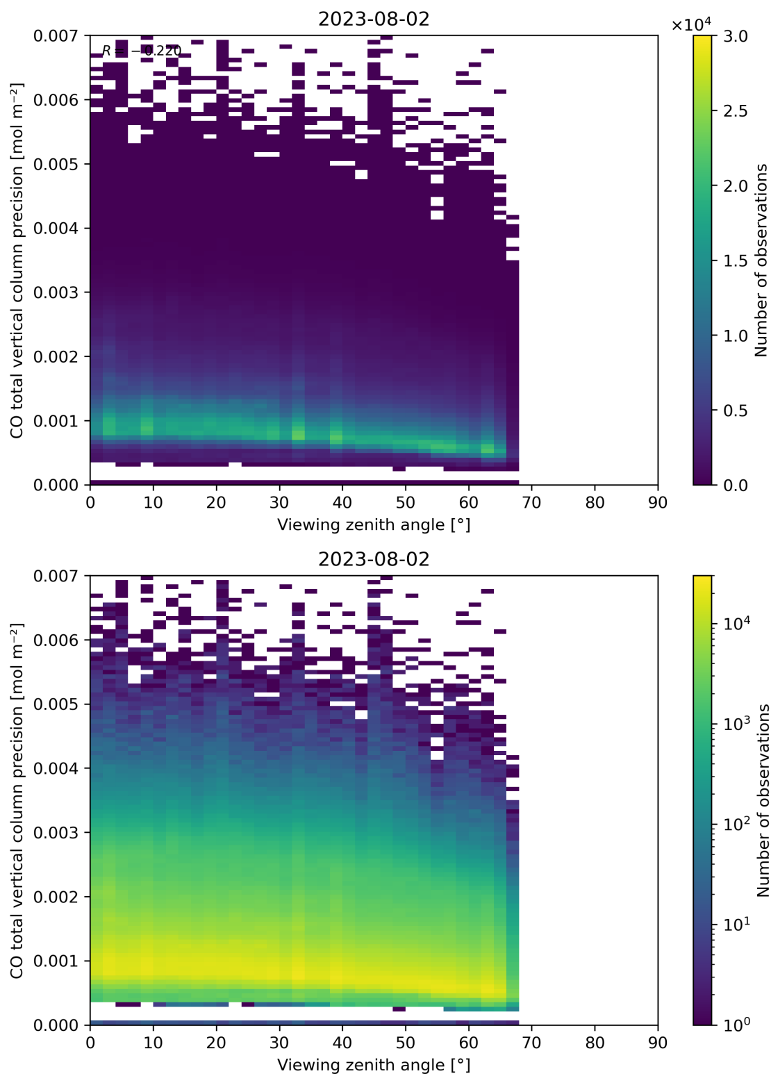
Figure 71: Scatter density plot of “Viewing zenith angle” against “CO total vertical column precision” for 2023-08-01 to 2023-08-03.
