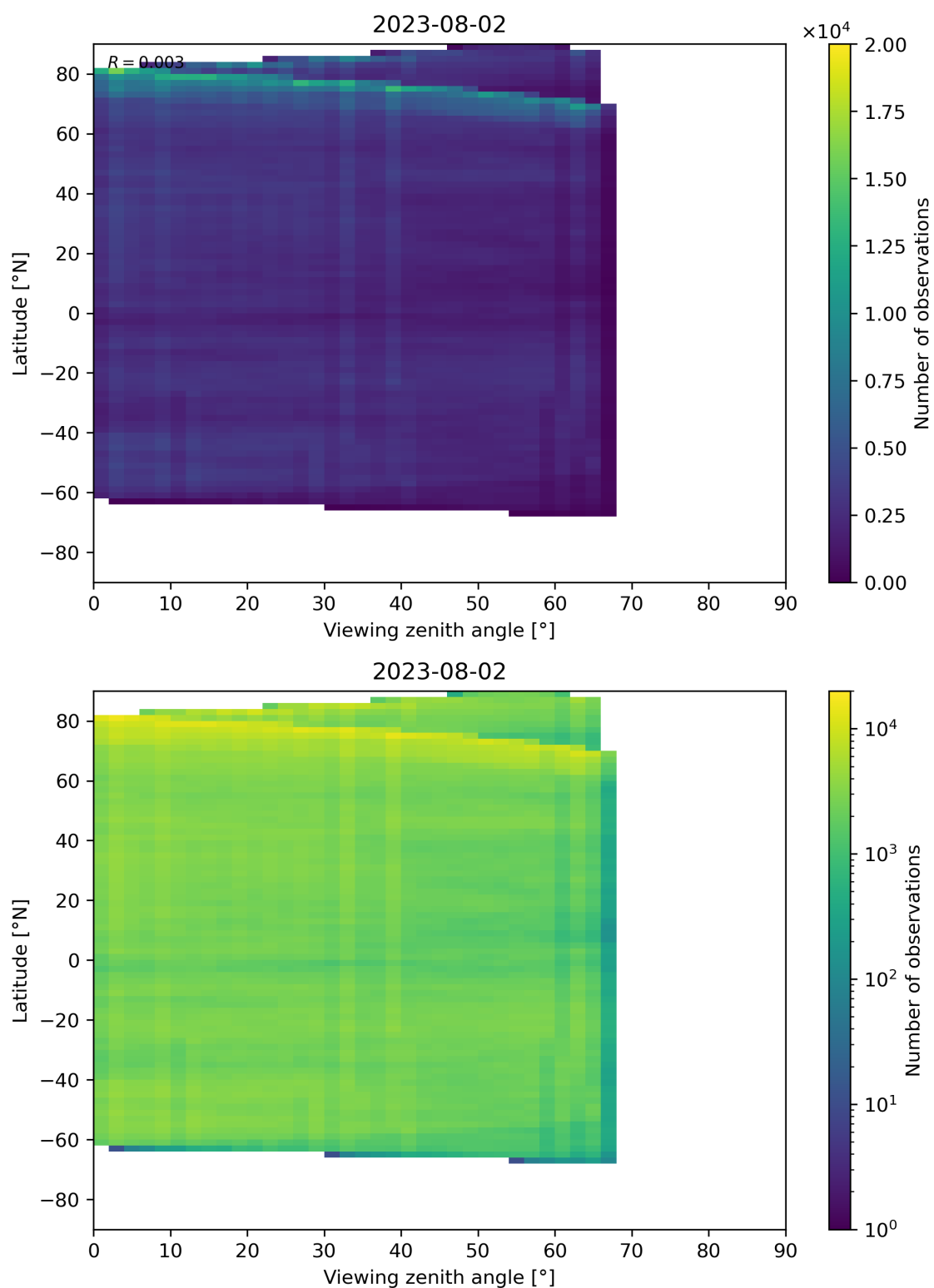
Figure 74: Scatter density plot of “Viewing zenith angle” against “Latitude” for 2023-08-01 to 2023-08-03.
