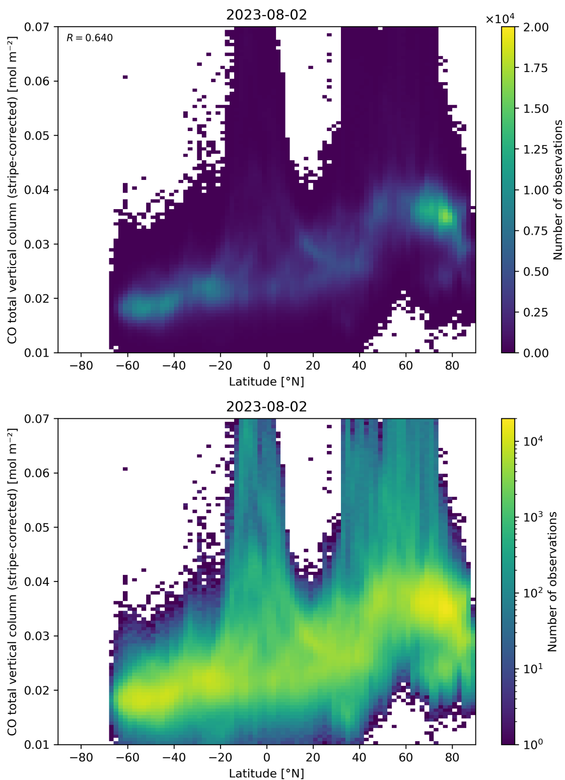
Figure 52: Scatter density plot of “Latitude” against “CO total vertical column (stripe-corrected)” for 2023-08-01 to 2023-08-03.
