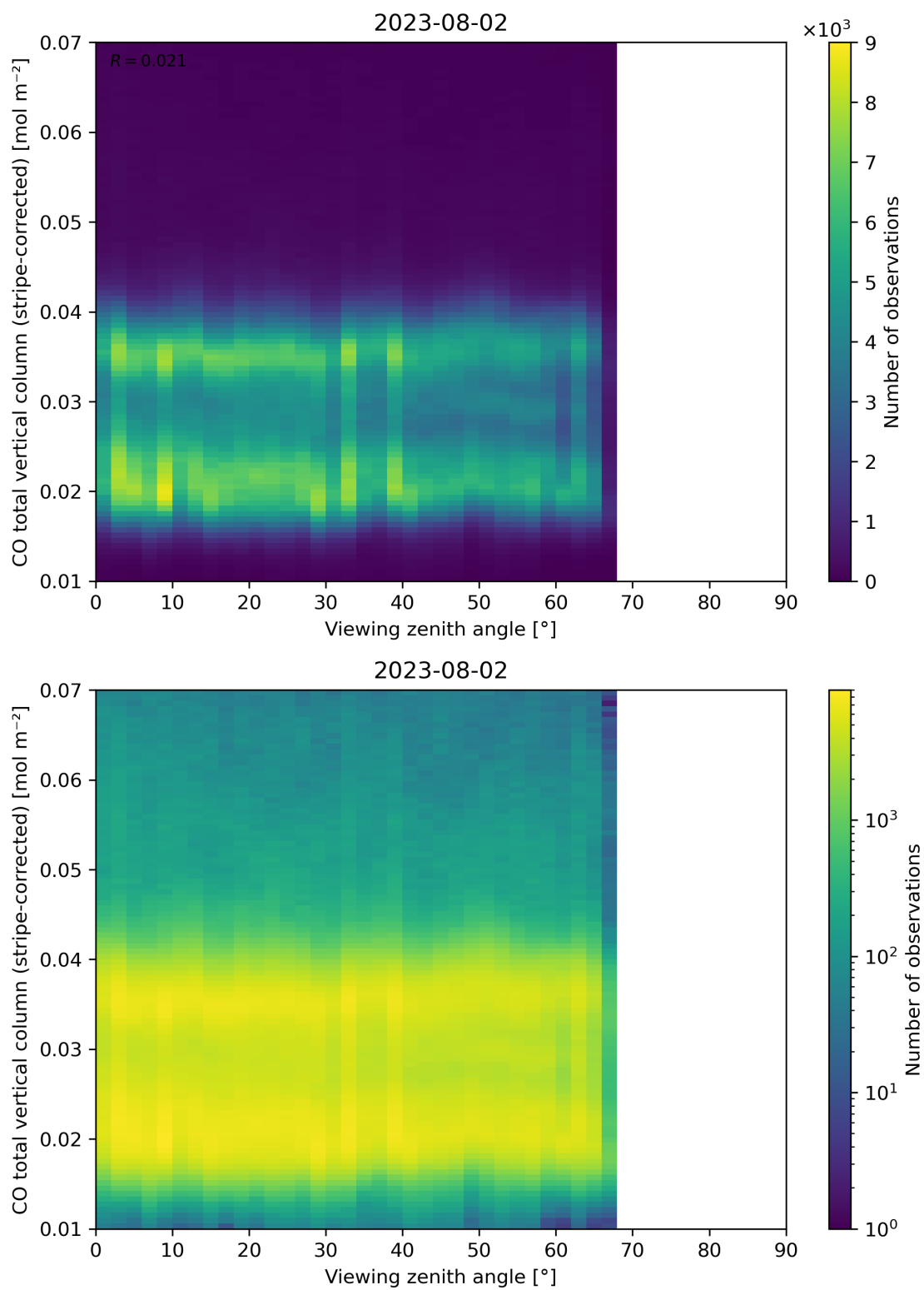
Figure 70: Scatter density plot of “Viewing zenith angle” against “CO total vertical column (stripe-corrected)” for 2023-08-01 to 2023-08-03.
