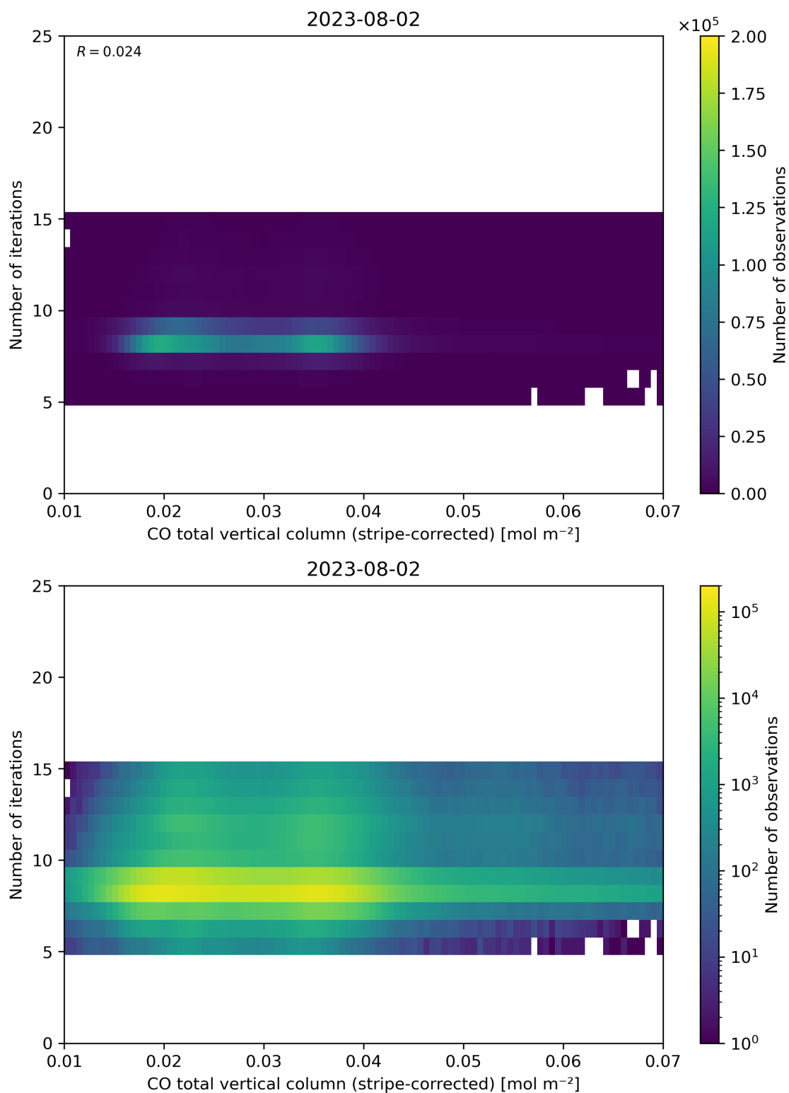
Figure 39: Scatter density plot of “CO total vertical column (stripe-corrected)” against “Number of iterations” for 2023-08-01 to 2023-08-03.
