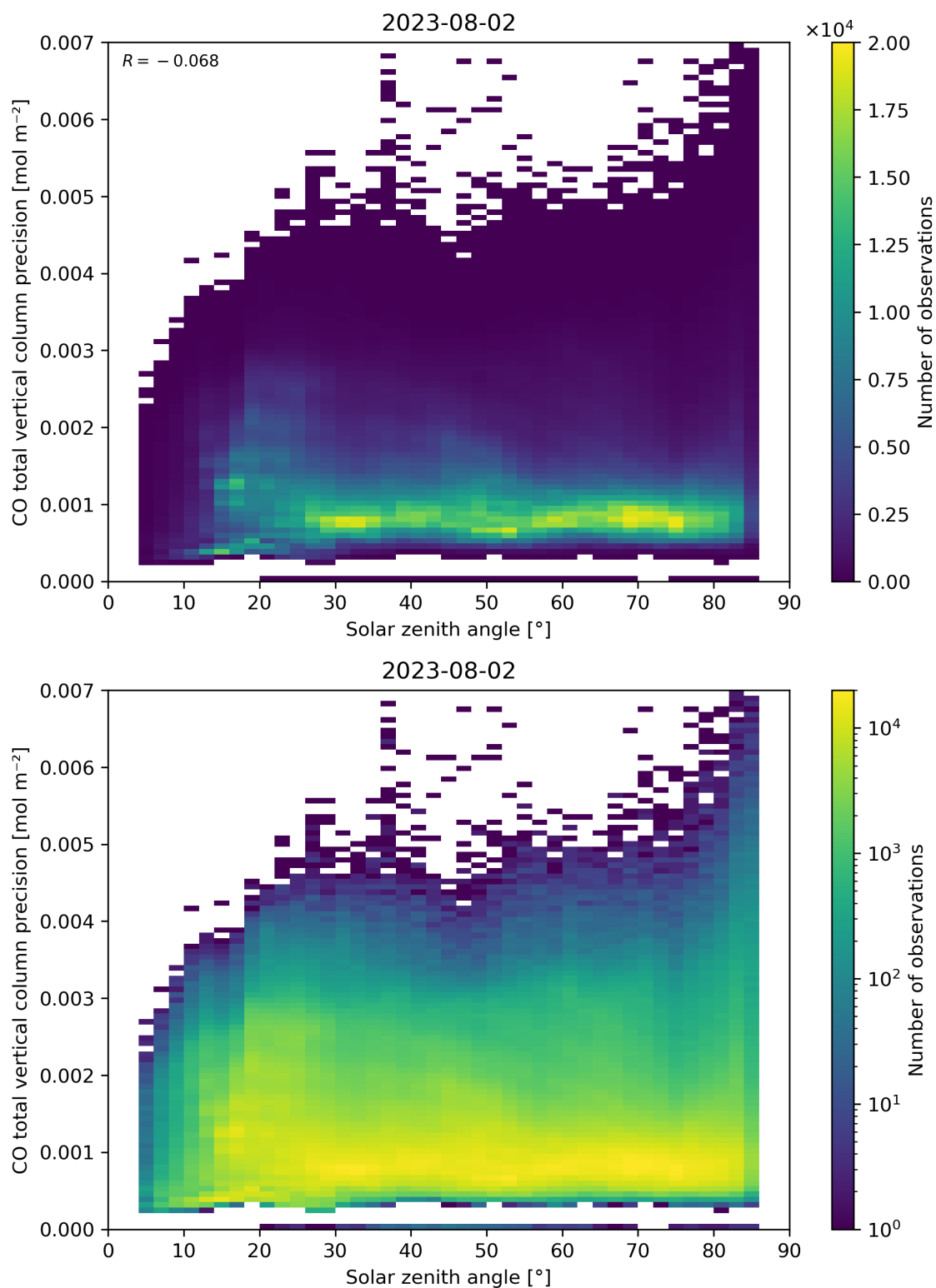
Figure 63: Scatter density plot of “Solar zenith angle” against “CO total vertical column precision” for 2023-08-01 to 2023-08-03.
