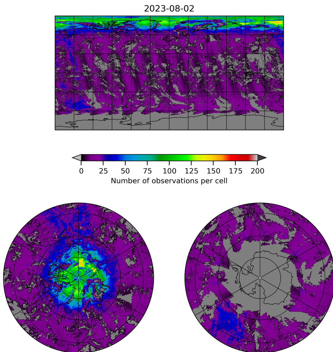
Figure 8: Map of the number of observations for 2023-08-01 to 2023-08-03
