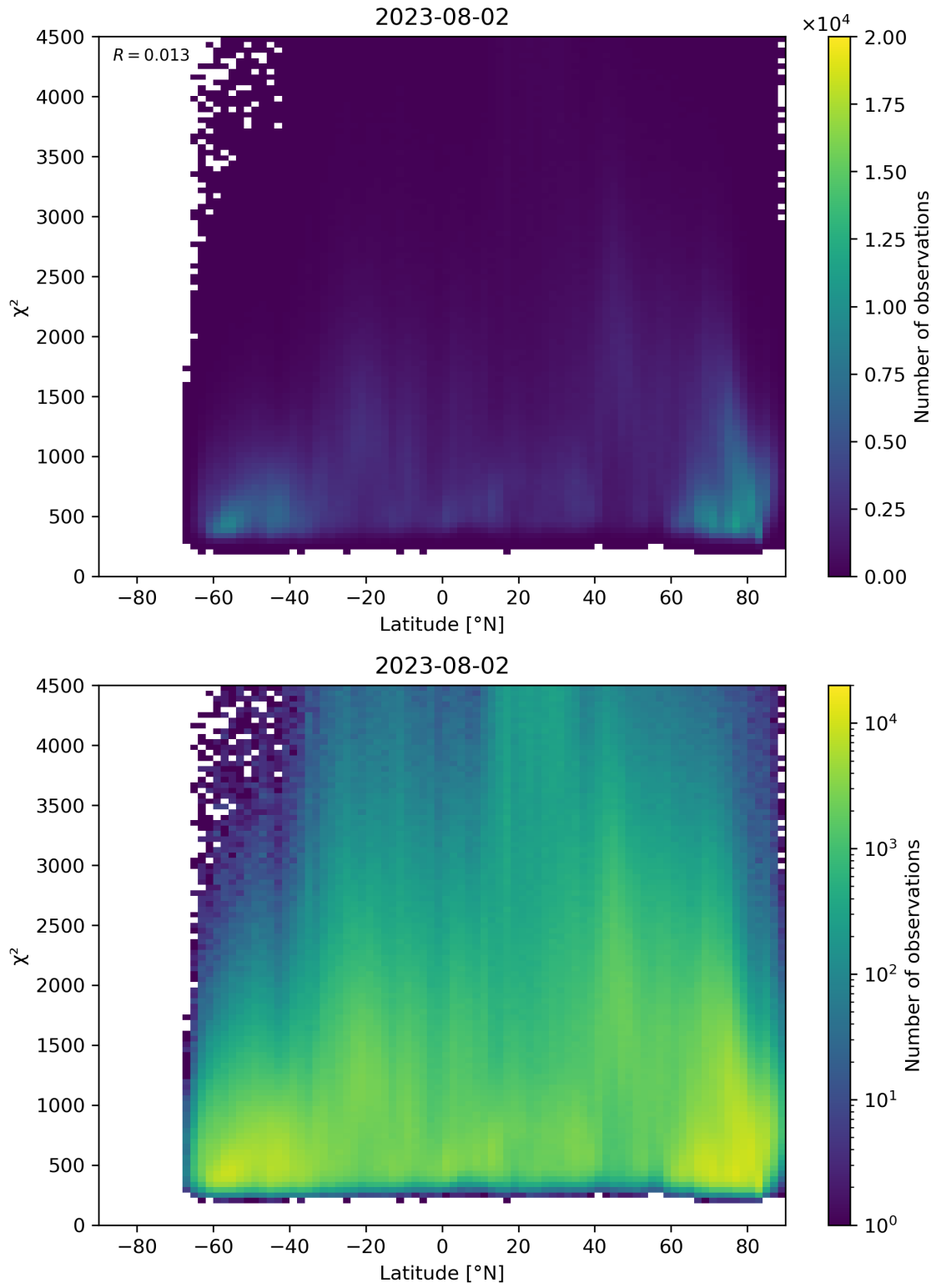
Figure 54: Scatter density plot of “Latitude” against “ \chi^2 ” for 2023-08-01 to 2023-08-03.
