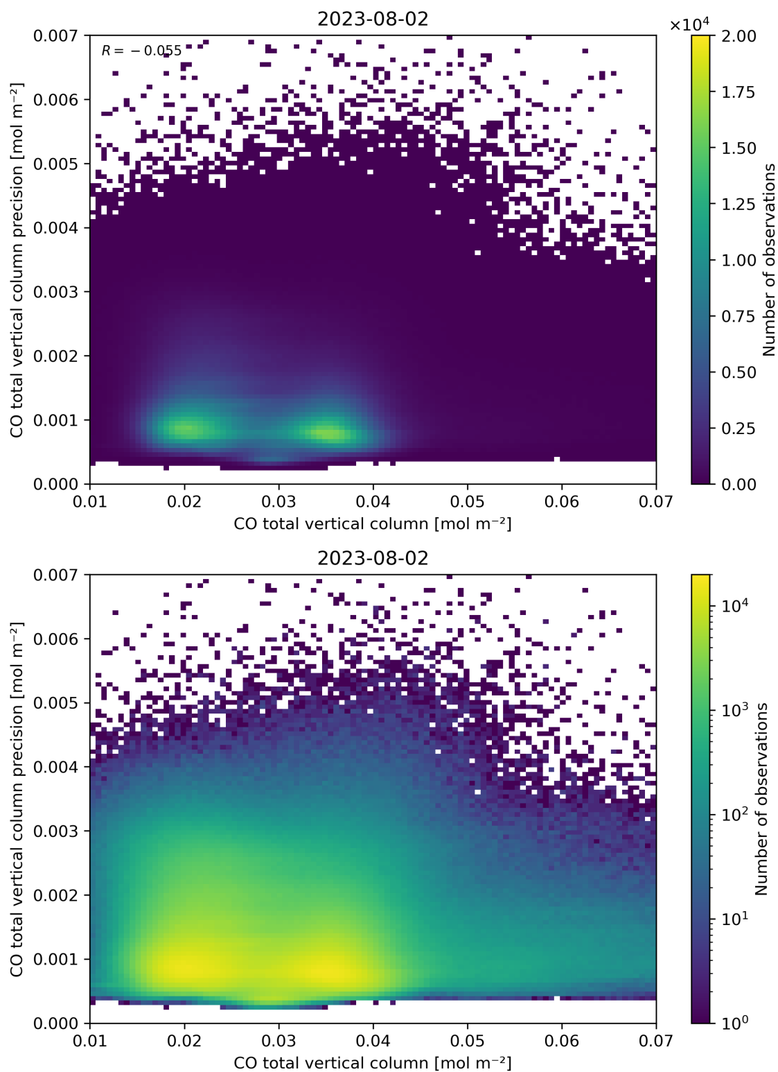
Figure 34: Scatter density plot of “CO total vertical column” against “CO total vertical column precision” for 2023-08-01 to 2023-08-03.
