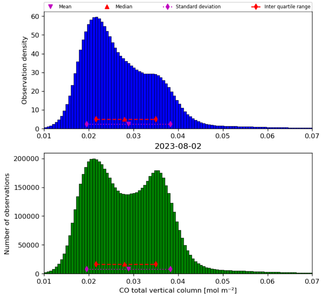
Figure 18: Histogram of “CO total vertical column” for 2023-08-01 to 2023-08-03
