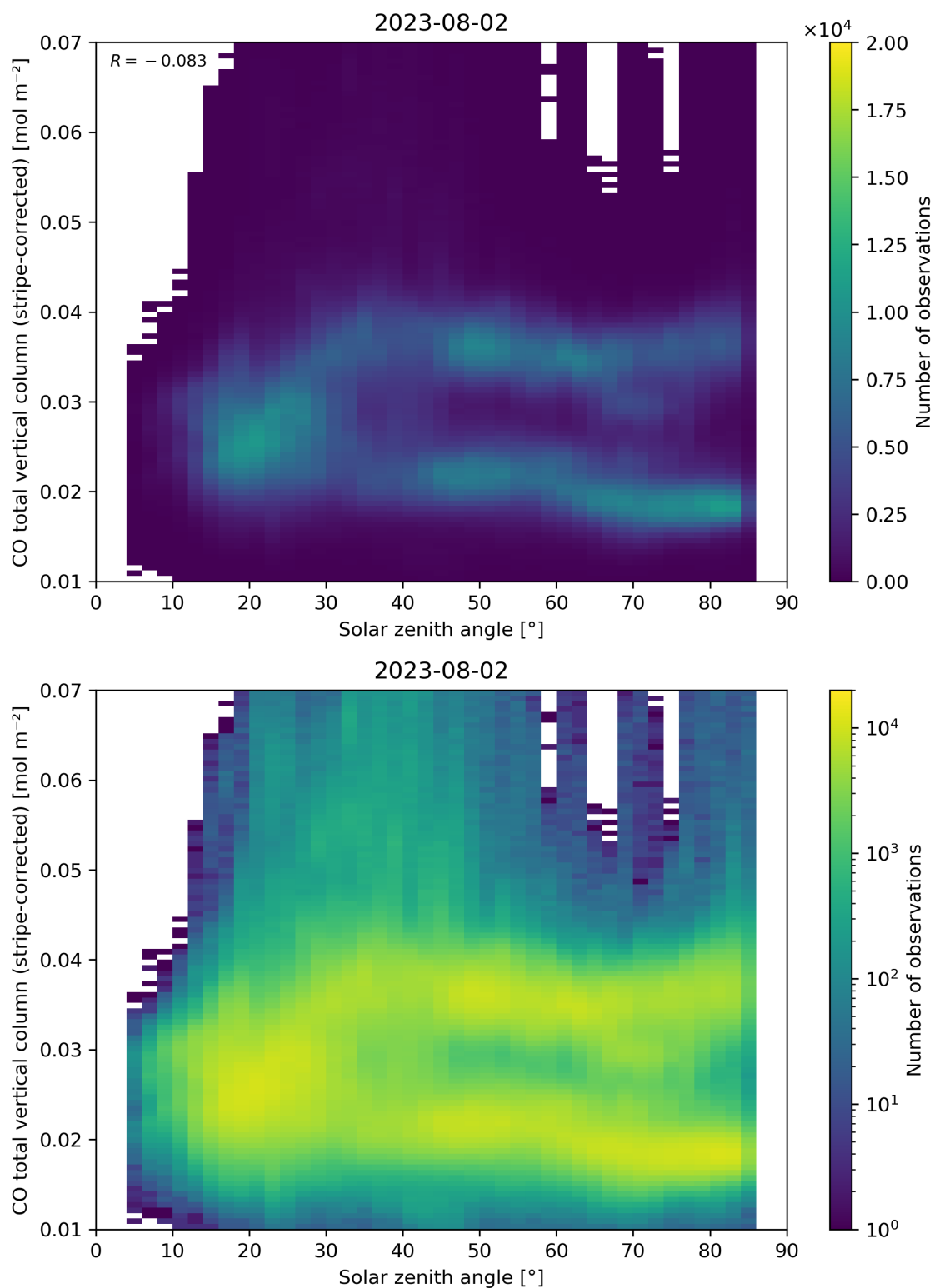
Figure 62: Scatter density plot of “Solar zenith angle” against “CO total vertical column (stripe-corrected)” for 2023-08-01 to 2023-08-03.
