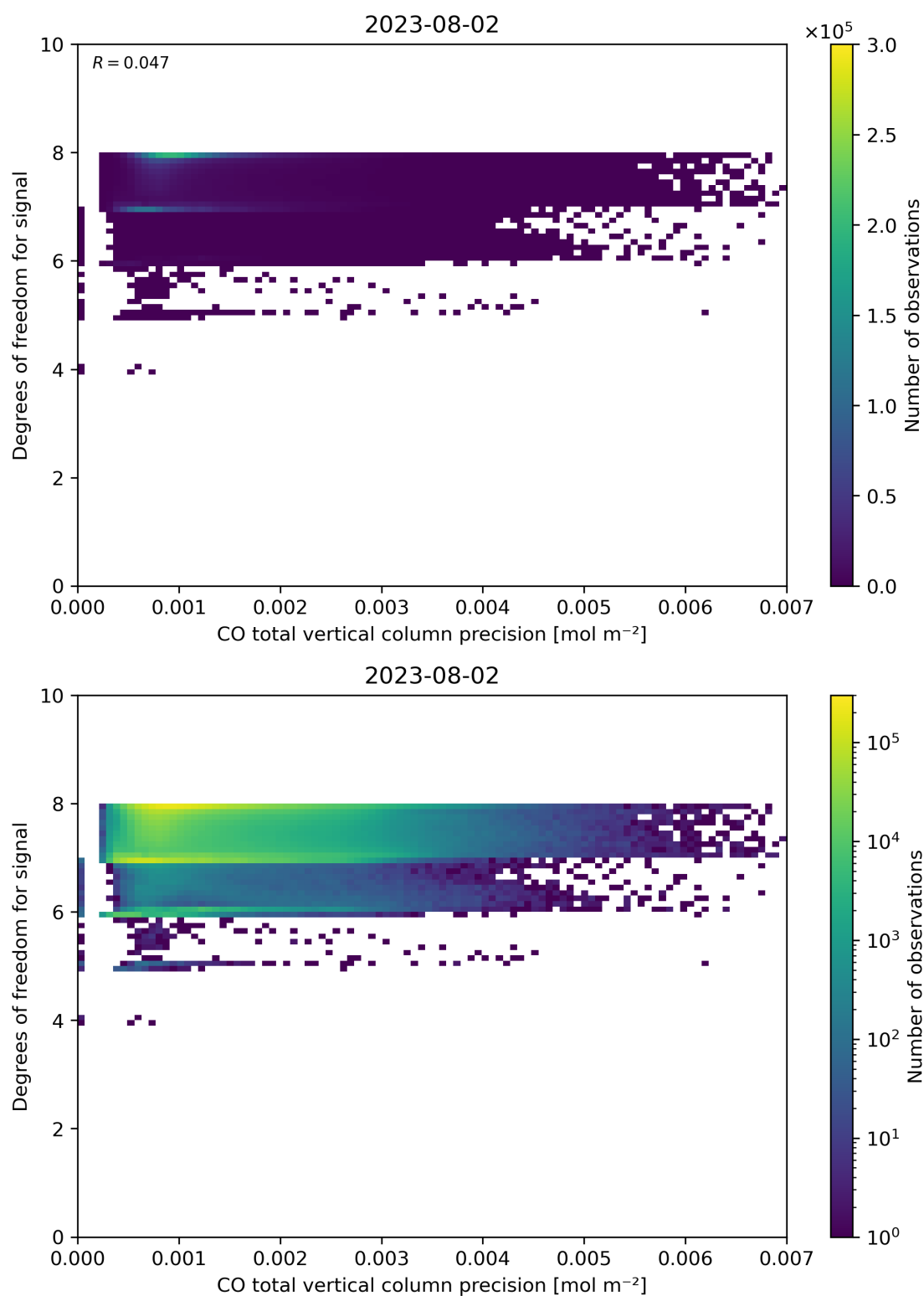
Figure 45: Scatter density plot of “CO total vertical column precision” against “Degrees of freedom for signal” for 2023-08-01 to 2023-08-03.
