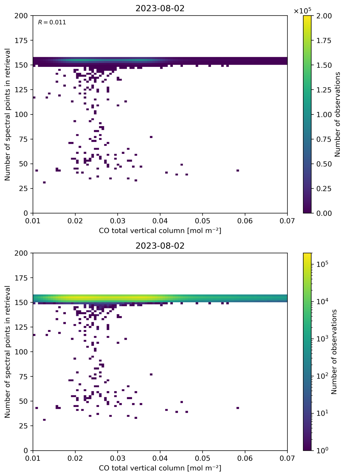
Figure 43: Scatter density plot of “CO total vertical column” against “Number of spectral points in retrieval” for 2023-08-01 to 2023-08-03.
