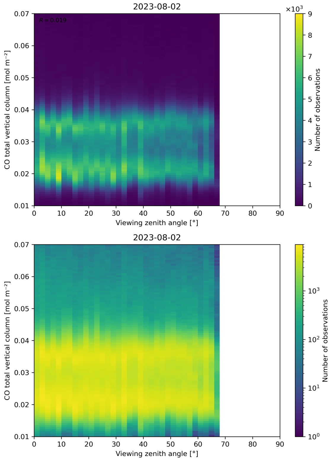
Figure 69: Scatter density plot of “Viewing zenith angle” against “CO total vertical column” for 2023-08-01 to 2023-08-03.
