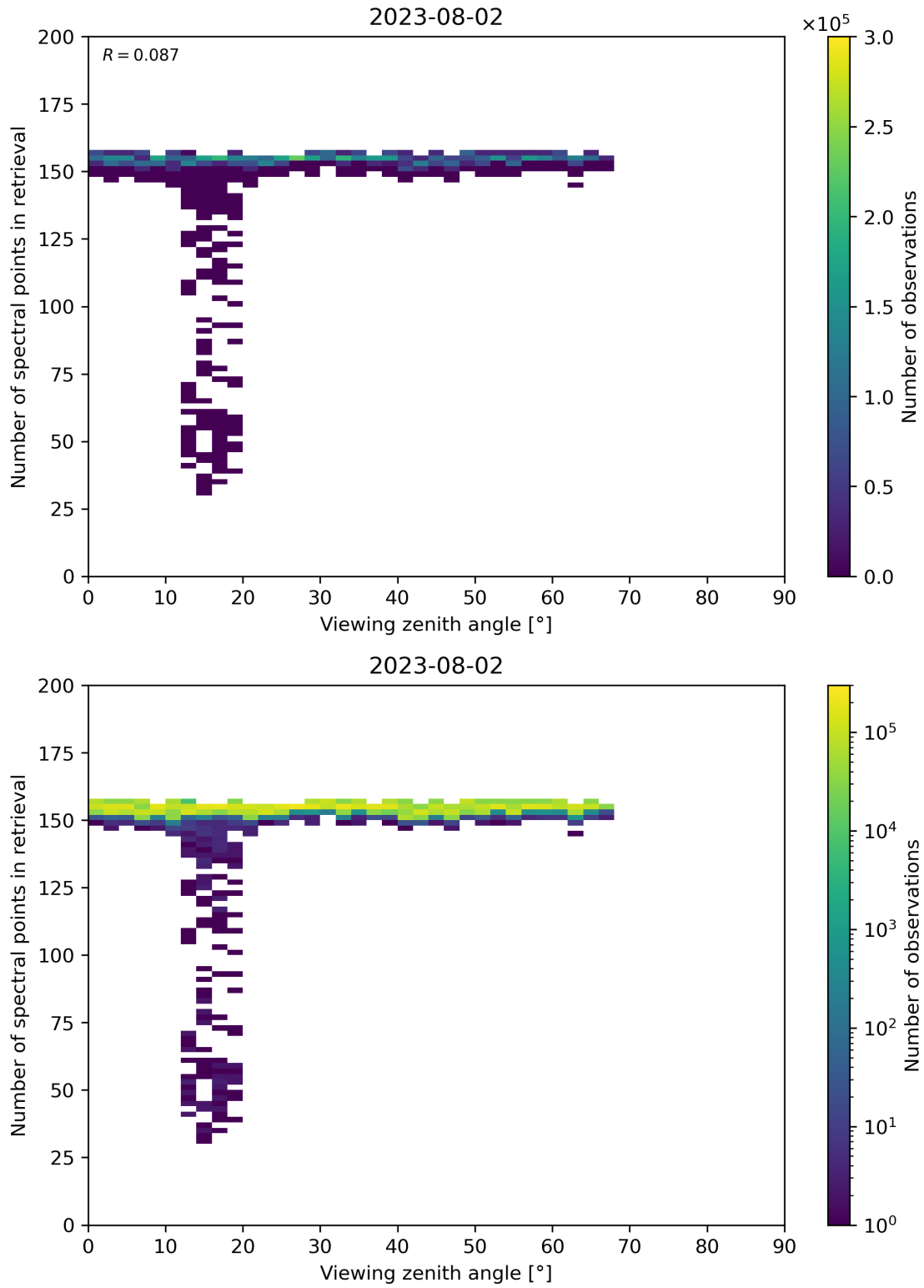
Figure 76: Scatter density plot of “Viewing zenith angle” against “Number of spectral points in retrieval” for 2023-08-01 to 2023-08-03.
