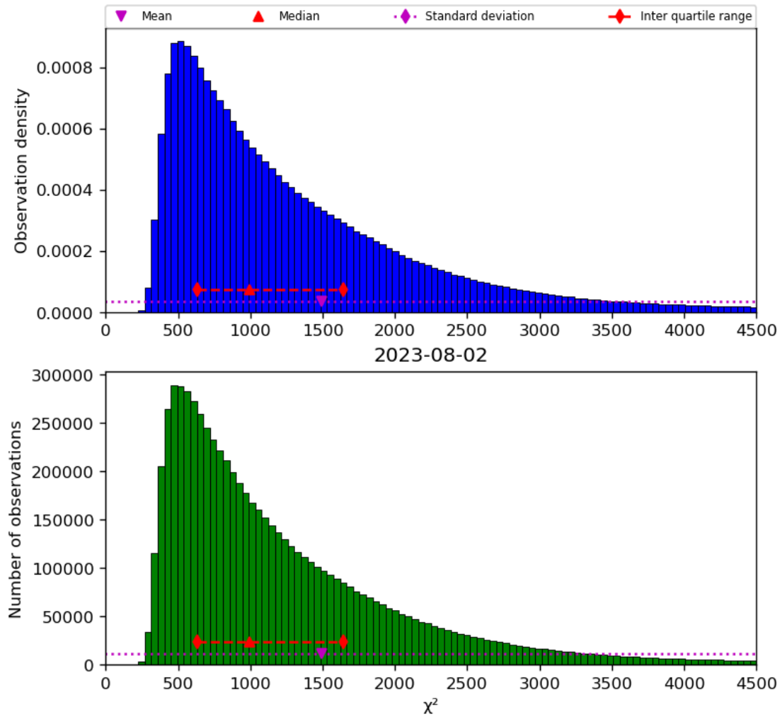
Figure 22: Histogram of “ \chi^2 ” for 2023-08-01 to 2023-08-03
