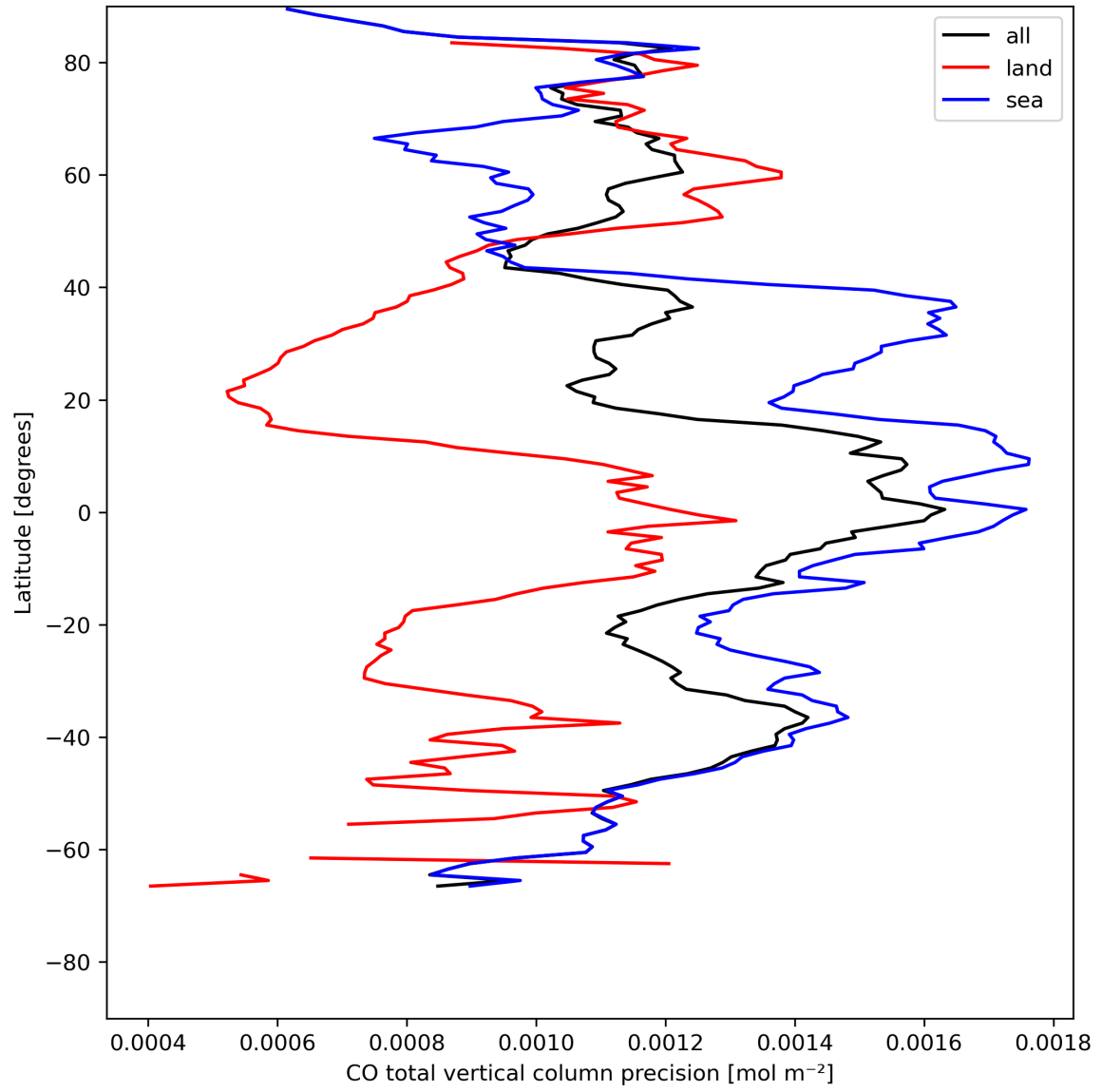
Figure 12: Zonal average of “CO total vertical column precision” for 2023-08-01 to 2023-08-03.
