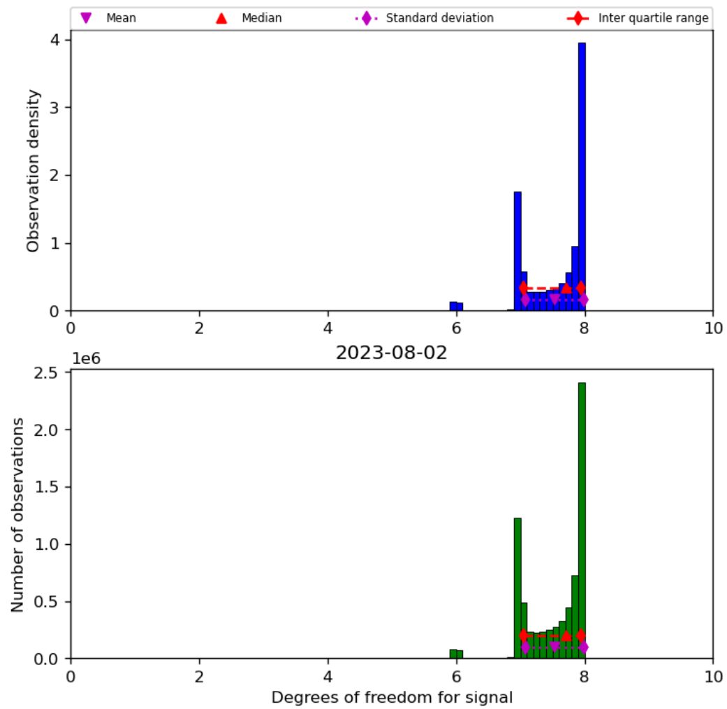
Figure 23: Histogram of “Degrees of freedom for signal” for 2023-08-01 to 2023-08-03
