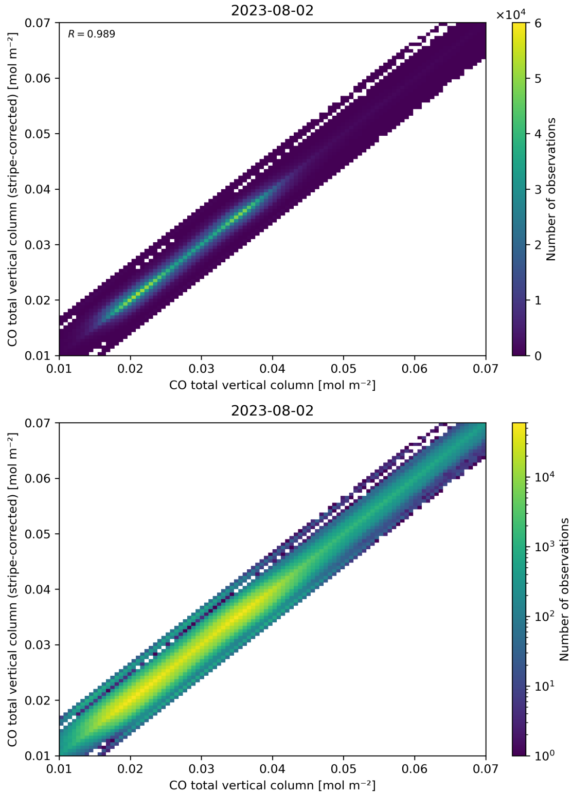
Figure 33: Scatter density plot of “CO total vertical column” against “CO total vertical column (stripe-corrected)” for 2023-08-01 to 2023-08-03.
