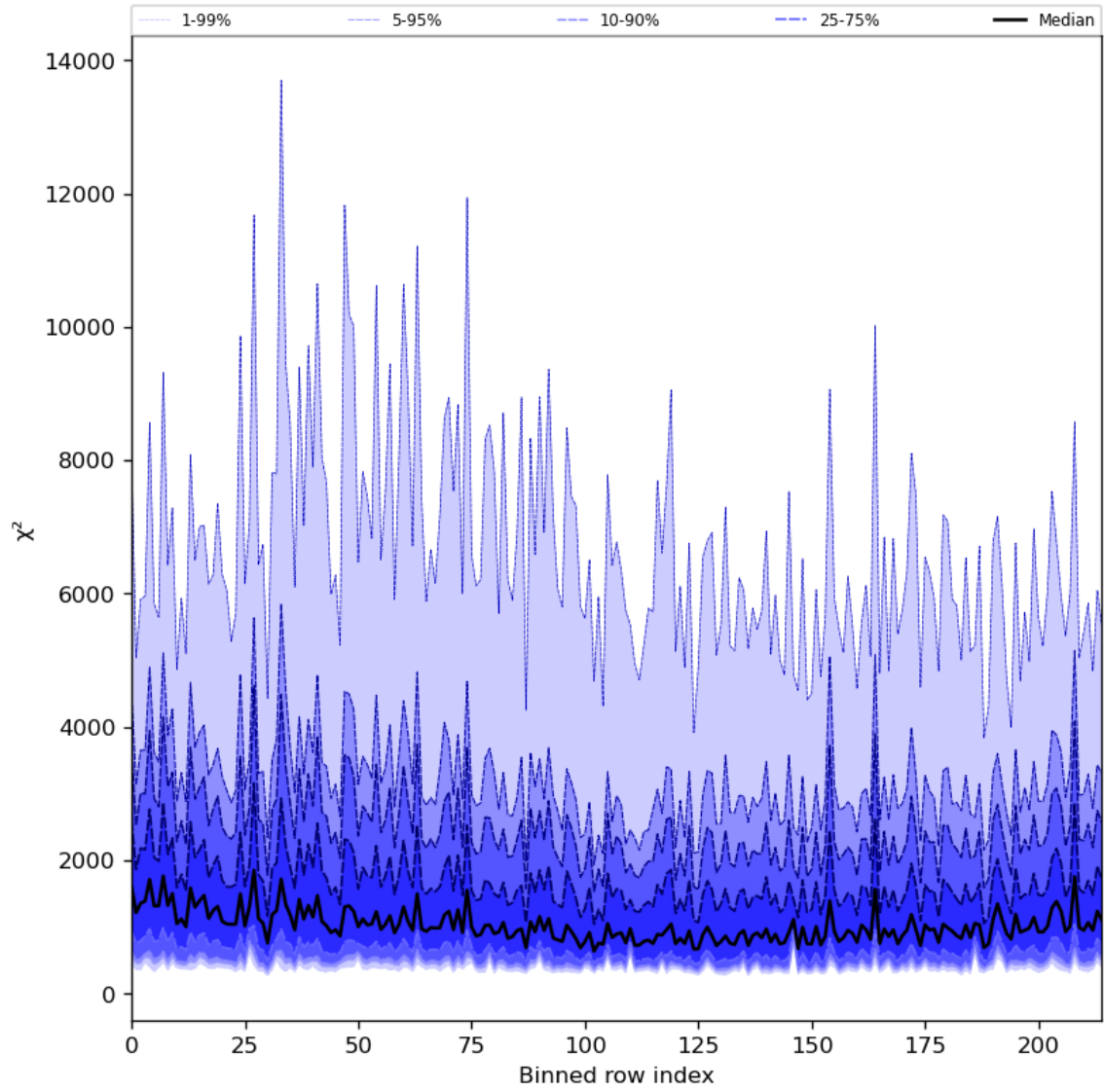
Figure 30: Along track statistics of “ \chi^2 ” for 2023-08-01 to 2023-08-03
