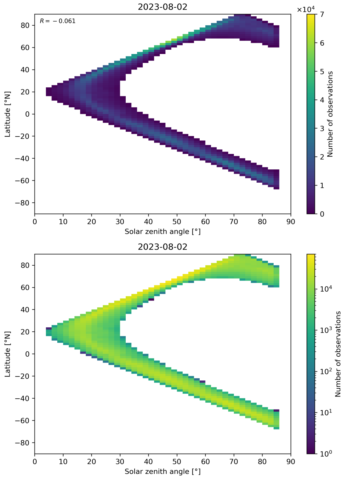
Figure 66: Scatter density plot of “Solar zenith angle” against “Latitude” for 2023-08-01 to 2023-08-03.
