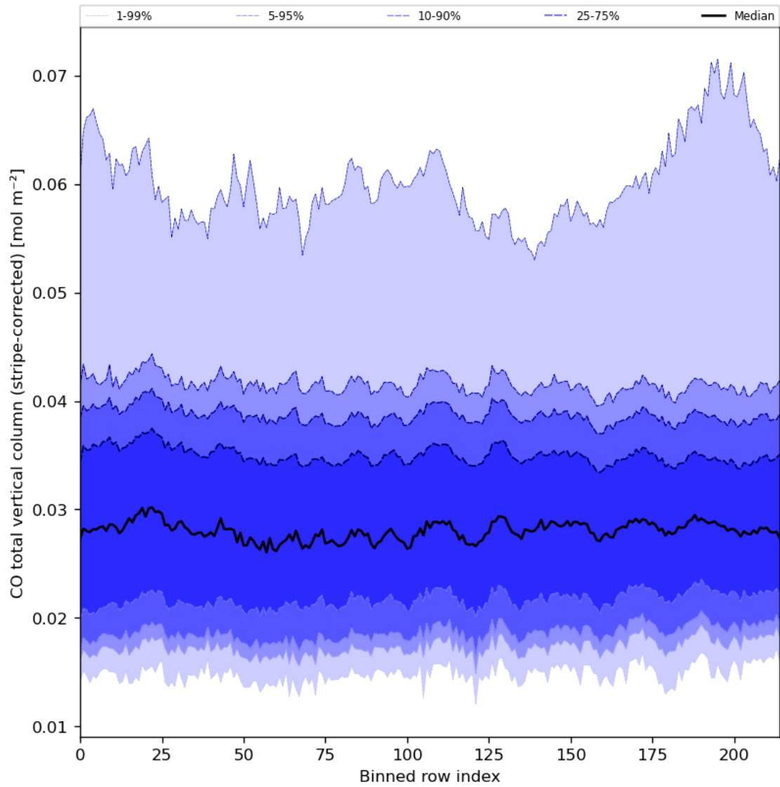
Figure 27: Along track statistics of “CO total vertical column (stripe-corrected)” for 2023-08-01 to 2023-08-03
