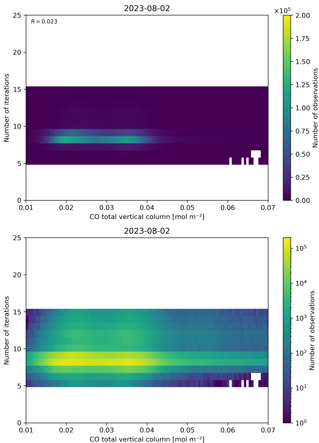
Figure 42: Scatter density plot of “CO total vertical column” against “Number of iterations” for 2023-08-01 to 2023-08-03.
