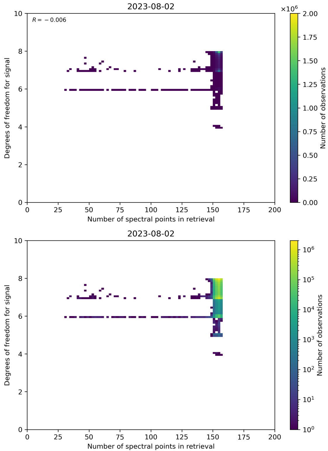
Figure 59: Scatter density plot of “Number of spectral points in retrieval” against “Degrees of freedom for signal” for 2023-08-01 to 2023-08-03.
