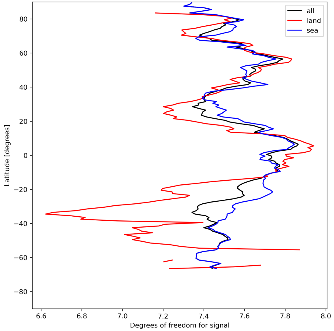
Figure 15: Zonal average of “Degrees of freedom for signal” for 2023-08-01 to 2023-08-03.
