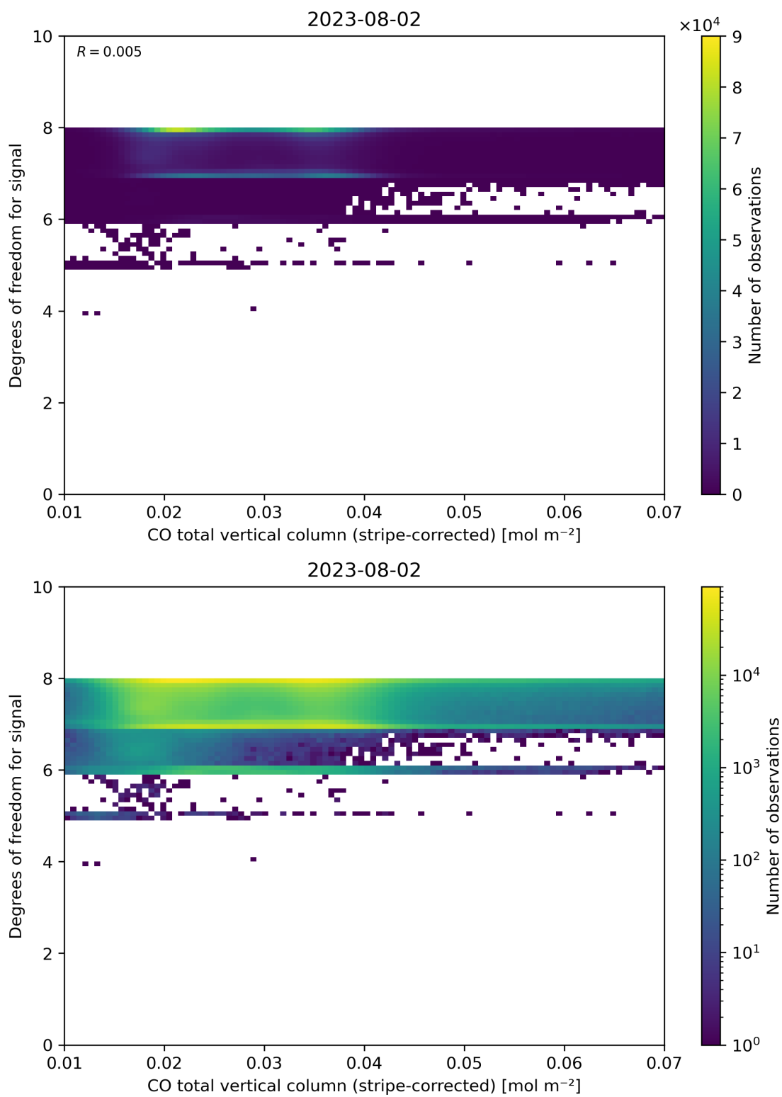
Figure 38: Scatter density plot of “CO total vertical column (stripe-corrected)” against “Degrees of freedom for signal” for 2023-08-01 to 2023-08-03.
