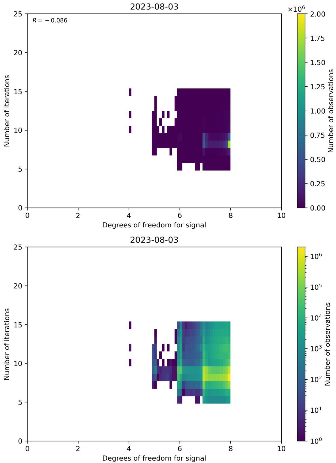
Figure 50: Scatter density plot of “Degrees of freedom for signal” against “Number of iterations” for 2023-08-02 to 2023-08-04.
