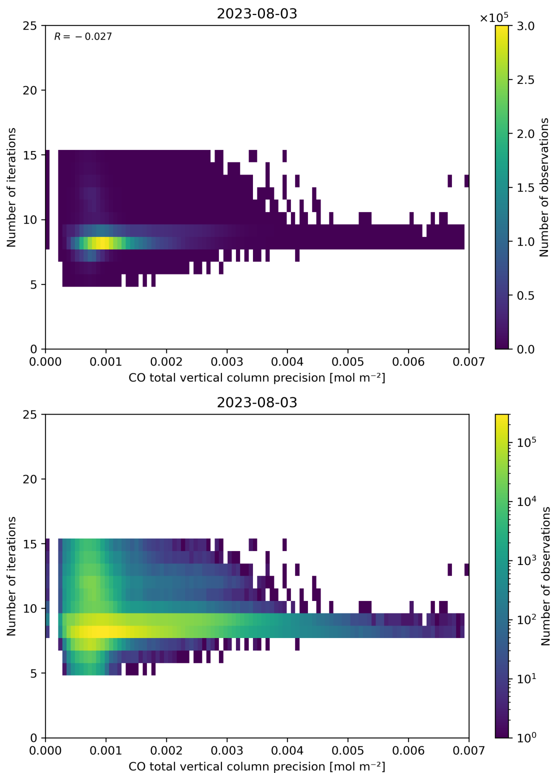
Figure 46: Scatter density plot of “CO total vertical column precision” against “Number of iterations” for 2023-08-02 to 2023-08-04.
