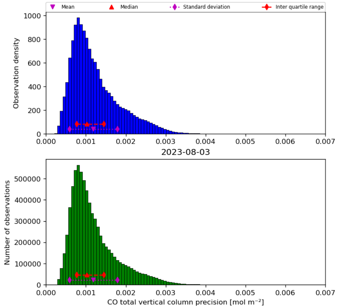
Figure 20: Histogram of “CO total vertical column precision” for 2023-08-02 to 2023-08-04
