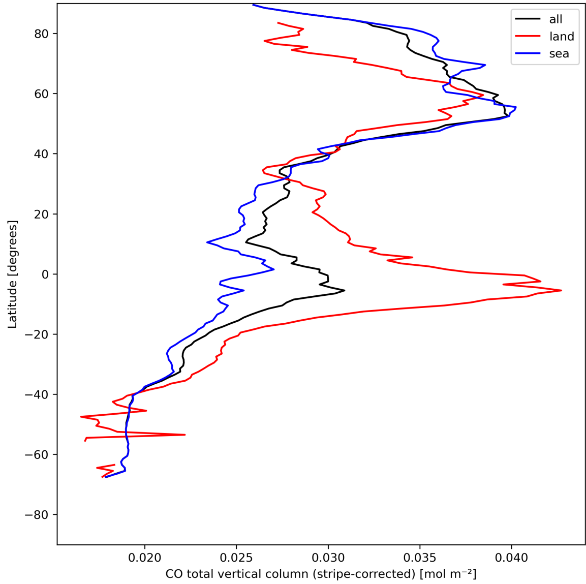
Figure 11: Zonal average of “CO total vertical column (stripe-corrected)” for 2023-08-02 to 2023-08-04.
