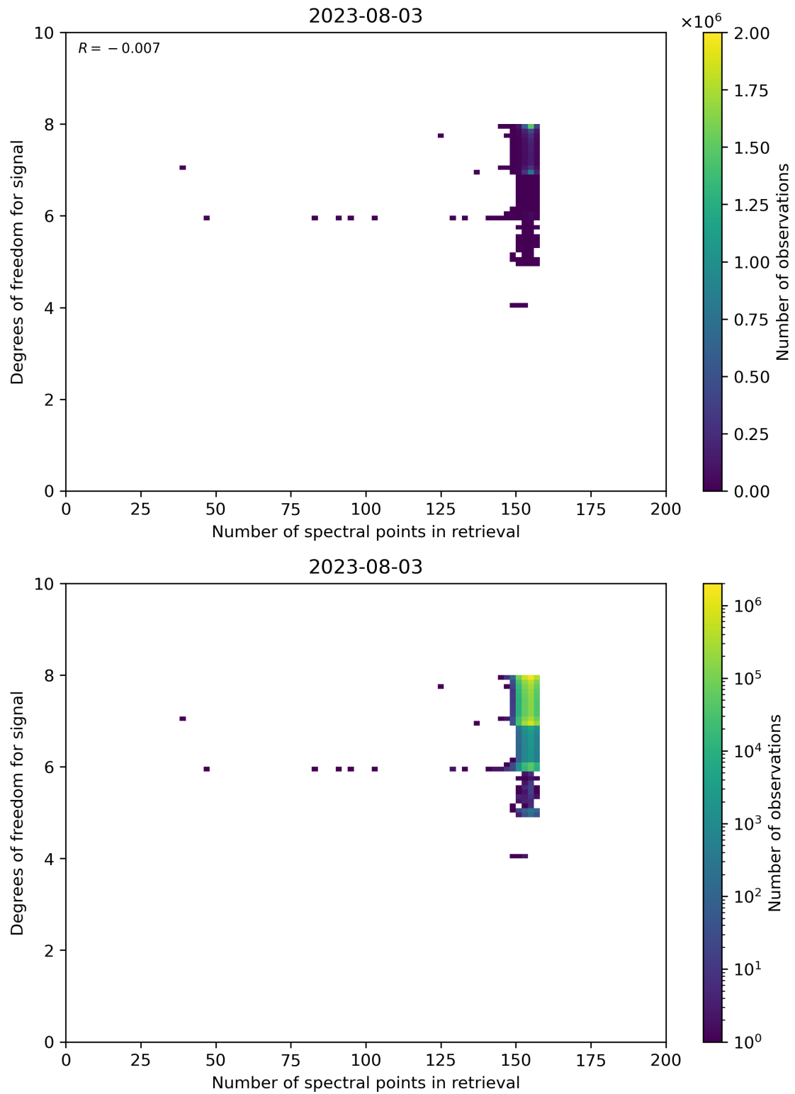
Figure 59: Scatter density plot of “Number of spectral points in retrieval” against “Degrees of freedom for signal” for 2023-08-02 to 2023-08-04.
