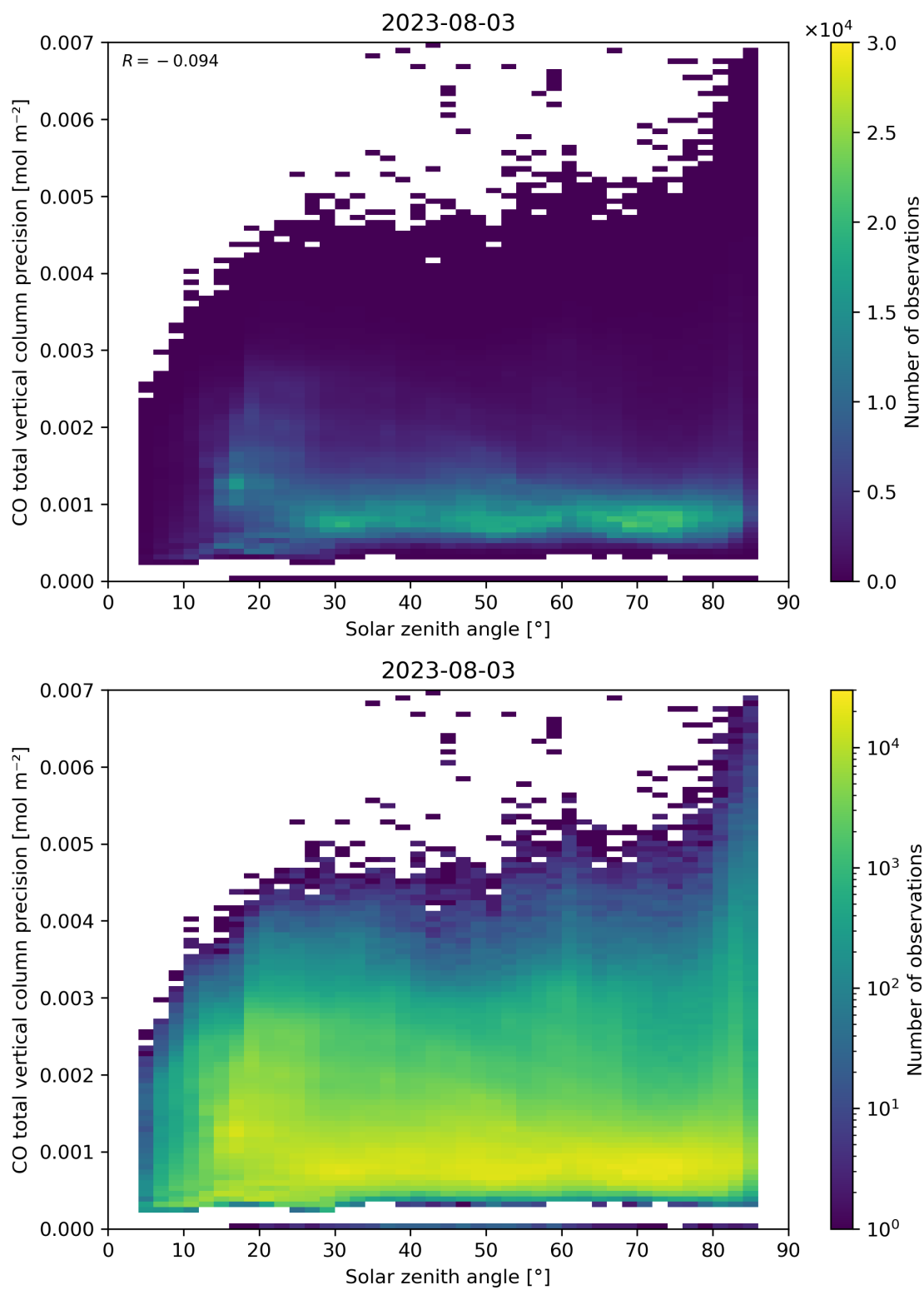
Figure 63: Scatter density plot of “Solar zenith angle” against “CO total vertical column precision” for 2023-08-02 to 2023-08-04.
