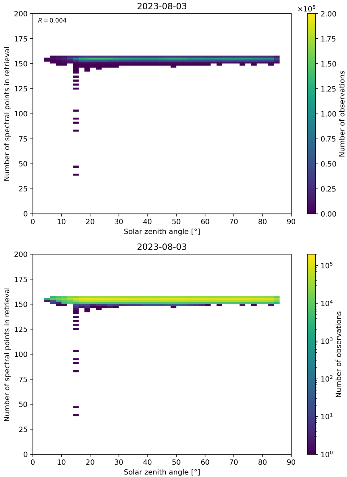
Figure 68: Scatter density plot of “Solar zenith angle” against “Number of spectral points in retrieval” for 2023-08-02 to 2023-08-04.
