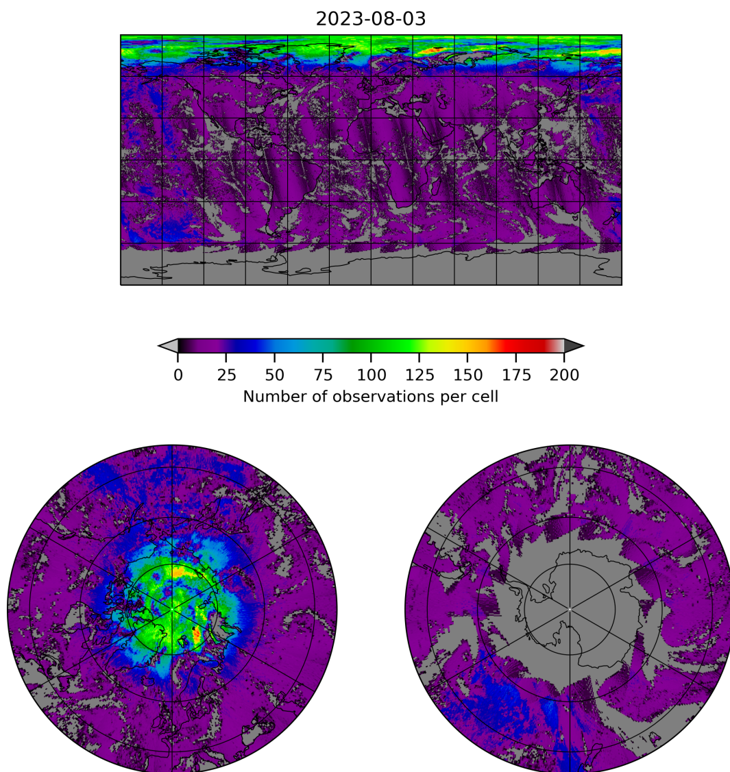
Figure 8: Map of the number of observations for 2023-08-02 to 2023-08-04
