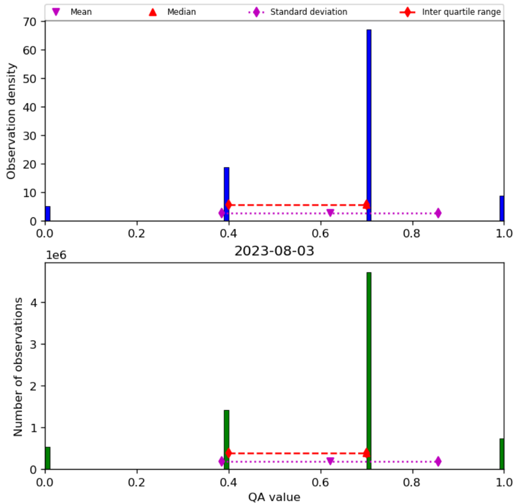
Figure 17: Histogram of “QA value” for 2023-08-02 to 2023-08-04
