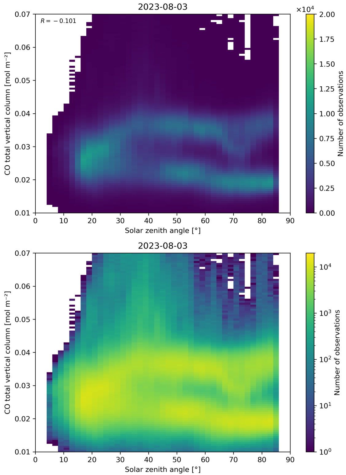
Figure 61: Scatter density plot of “Solar zenith angle” against “CO total vertical column” for 2023-08-02 to 2023-08-04.
