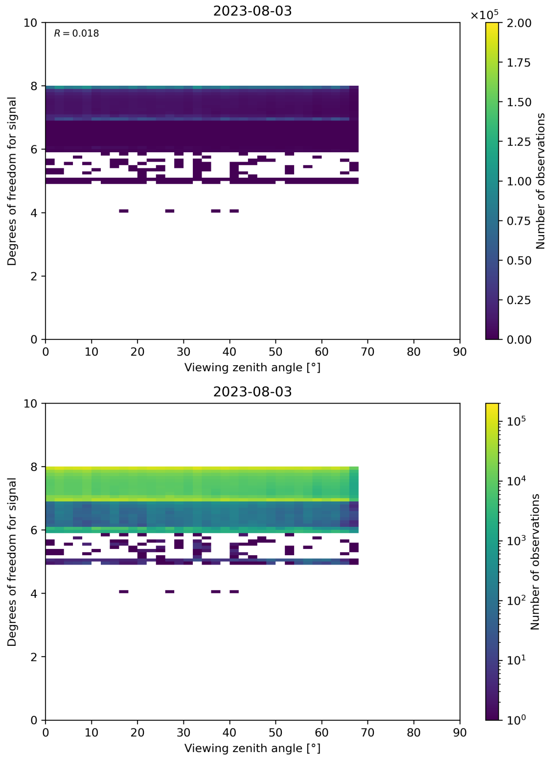
Figure 73: Scatter density plot of “Viewing zenith angle” against “Degrees of freedom for signal” for 2023-08-02 to 2023-08-04.
