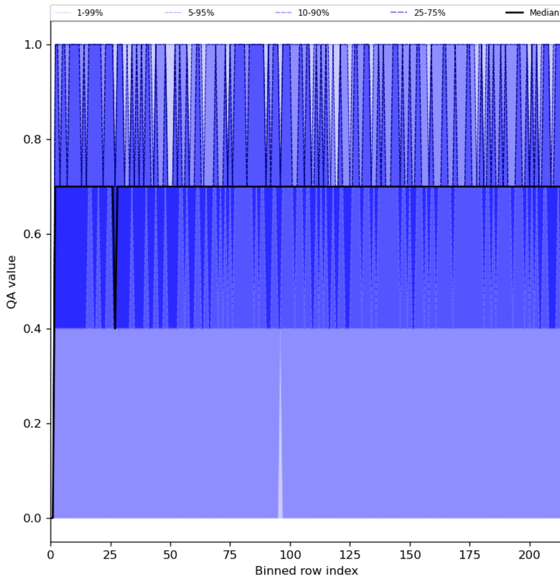
Figure 25: Along track statistics of “QA value” for 2023-08-02 to 2023-08-04
