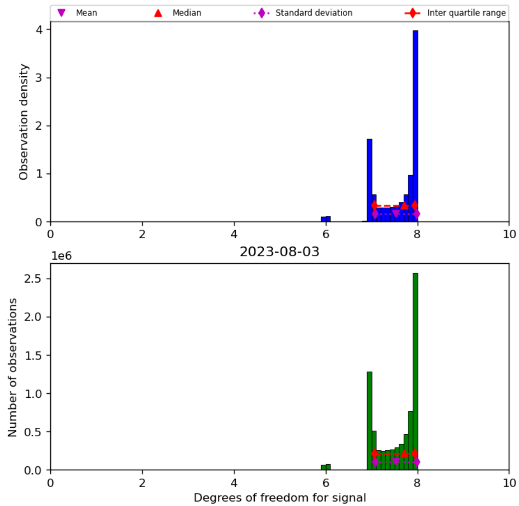
Figure 23: Histogram of “Degrees of freedom for signal” for 2023-08-02 to 2023-08-04
