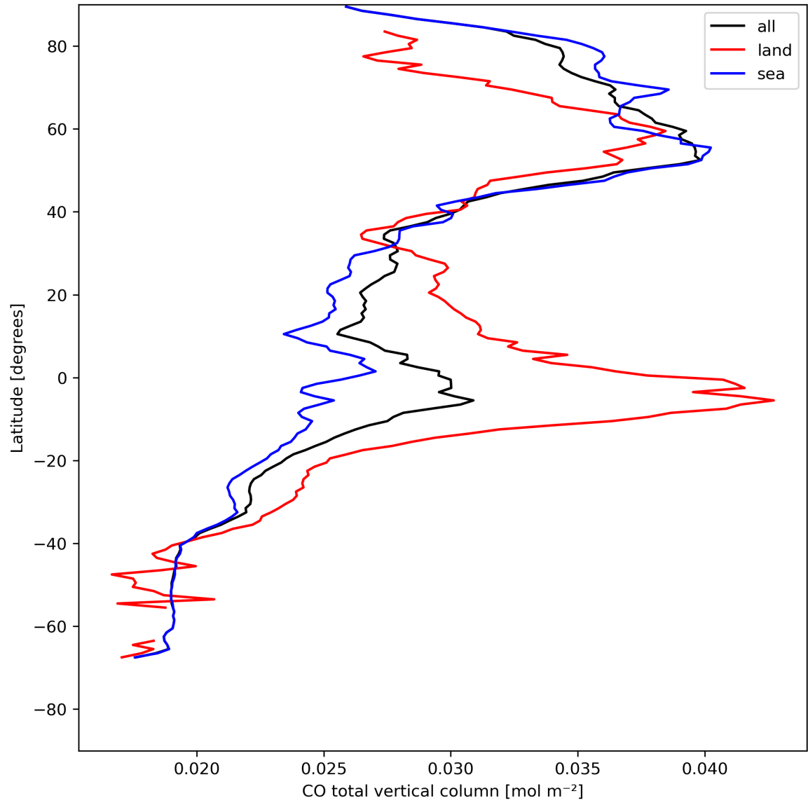
Figure 10: Zonal average of “CO total vertical column” for 2023-08-02 to 2023-08-04.
