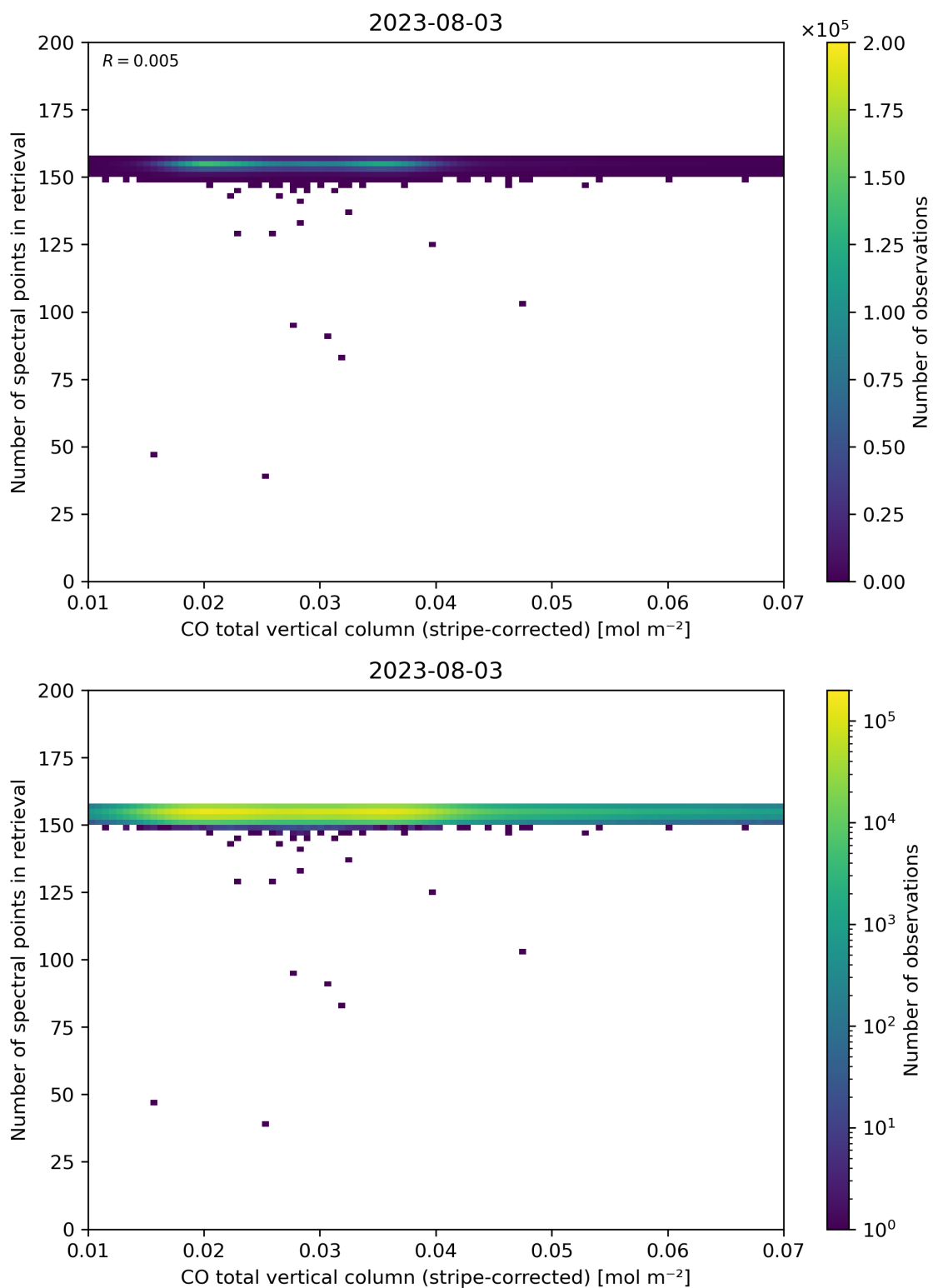
Figure 40: Scatter density plot of “CO total vertical column (stripe-corrected)” against “Number of spectral points in retrieval” for 2023-08-02 to 2023-08-04.
