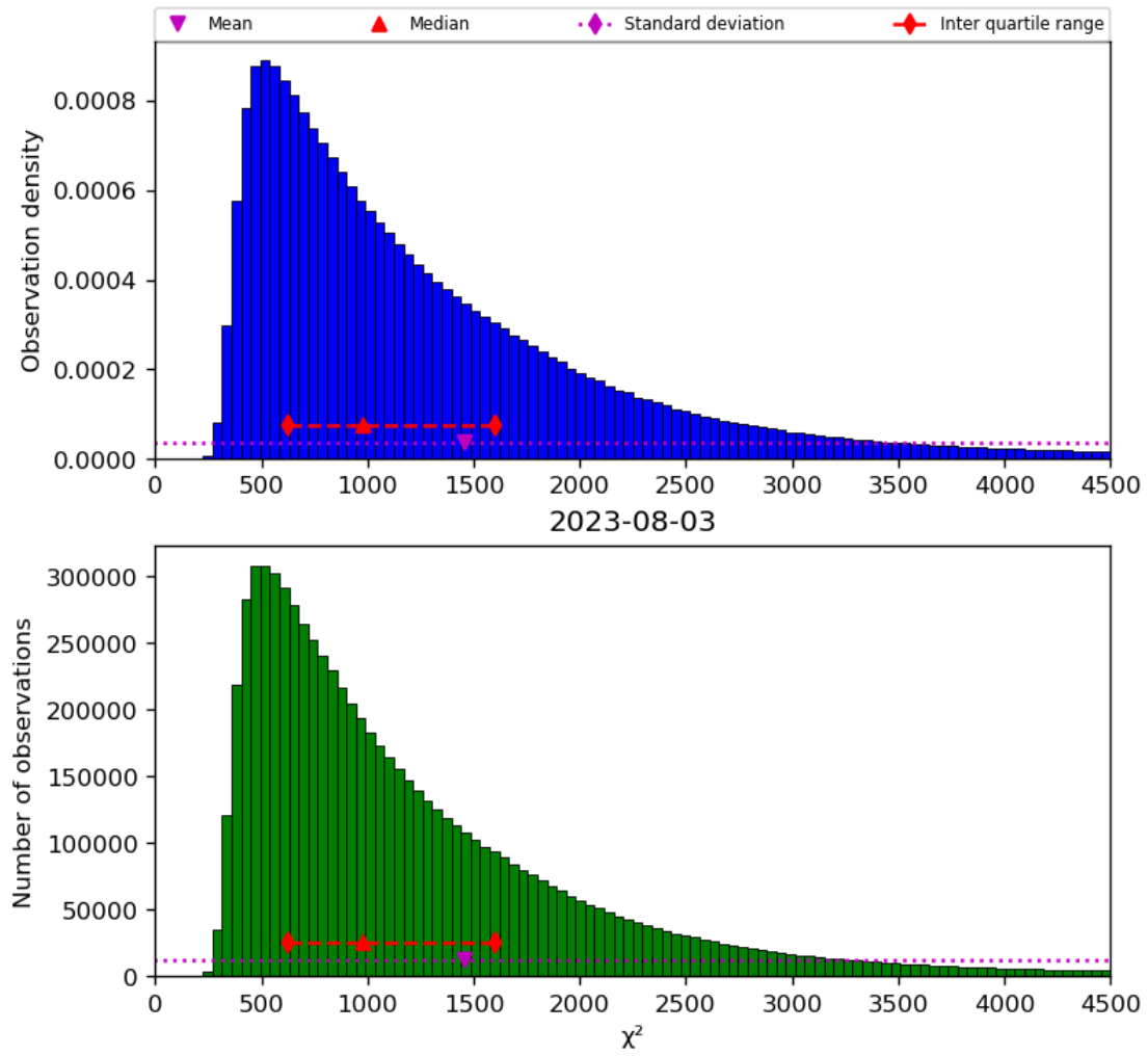
Figure 22: Histogram of " \chi^2 " for 2023-08-02 to 2023-08-04
