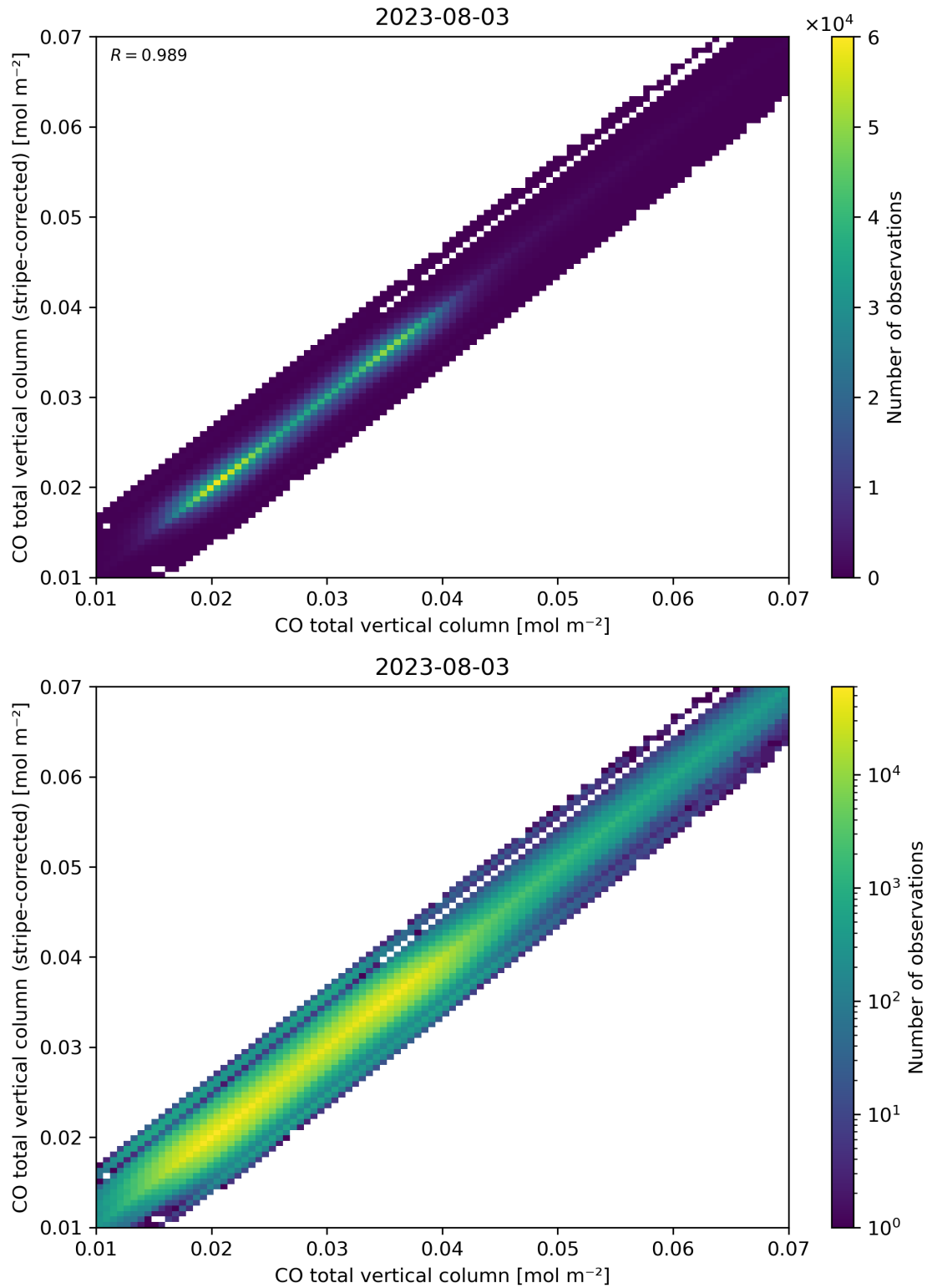
Figure 33: Scatter density plot of “CO total vertical column” against “CO total vertical column (stripe-corrected)” for 2023-08-02 to 2023-08-04.
