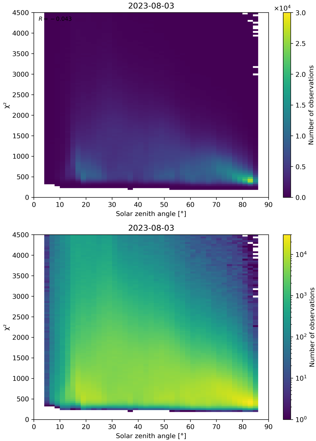
Figure 64: Scatter density plot of “Solar zenith angle” against “ \chi^2 ” for 2023-08-02 to 2023-08-04.
