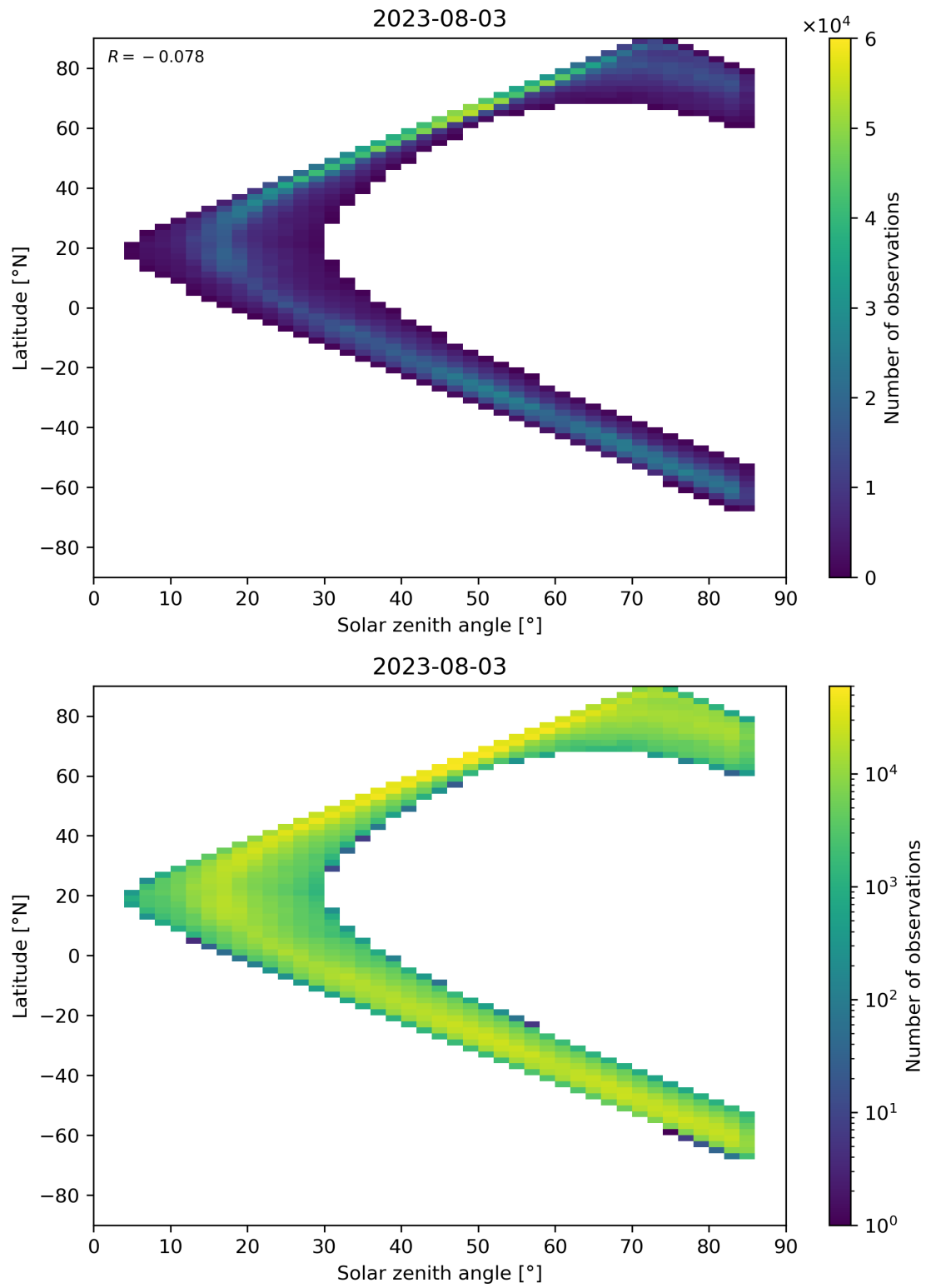
Figure 66: Scatter density plot of “Solar zenith angle” against “Latitude” for 2023-08-02 to 2023-08-04.
