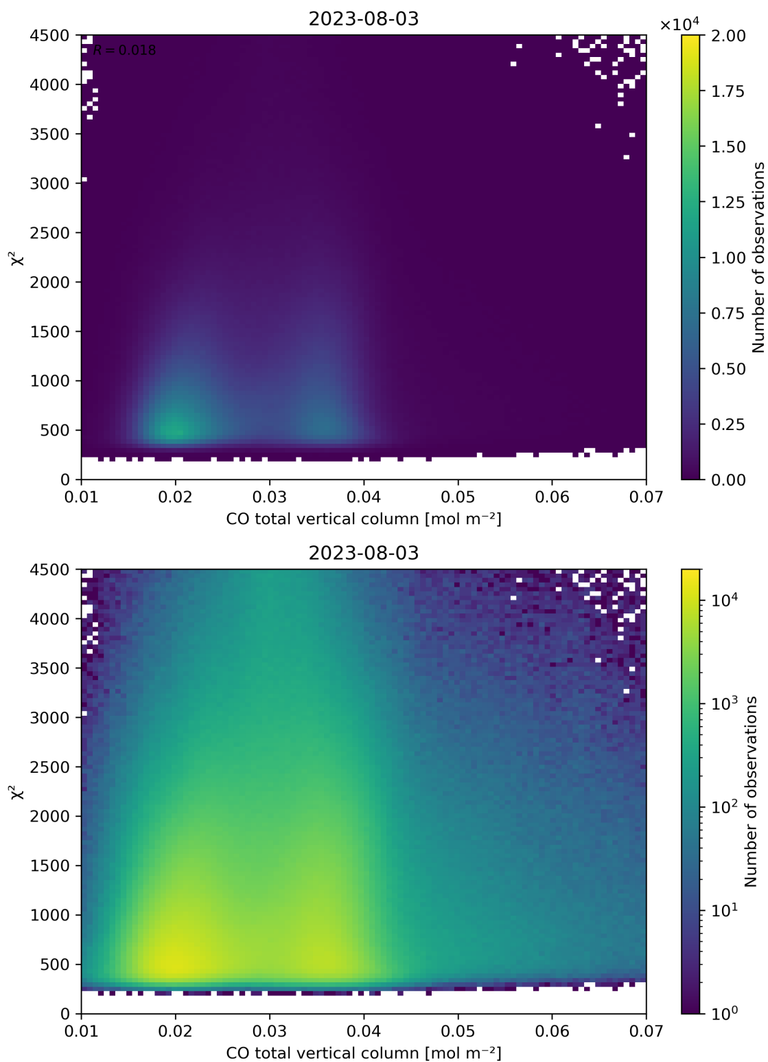
Figure 35: Scatter density plot of “CO total vertical column” against “ \chi^2 ” for 2023-08-02 to 2023-08-04.
