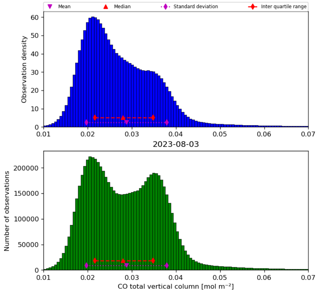
Figure 18: Histogram of “CO total vertical column” for 2023-08-02 to 2023-08-04
