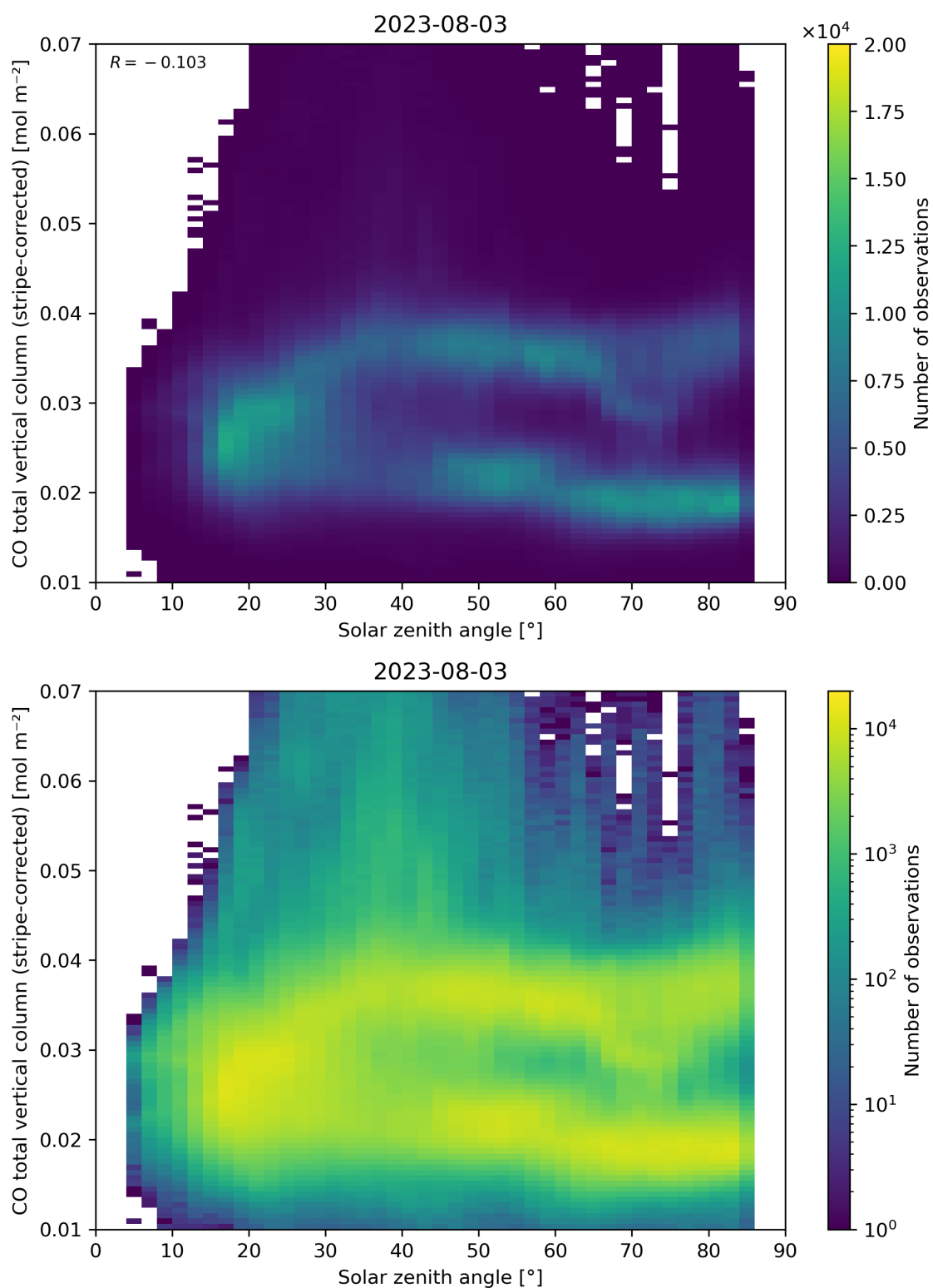
Figure 62: Scatter density plot of “Solar zenith angle” against “CO total vertical column (stripe-corrected)” for 2023-08-02 to 2023-08-04.
