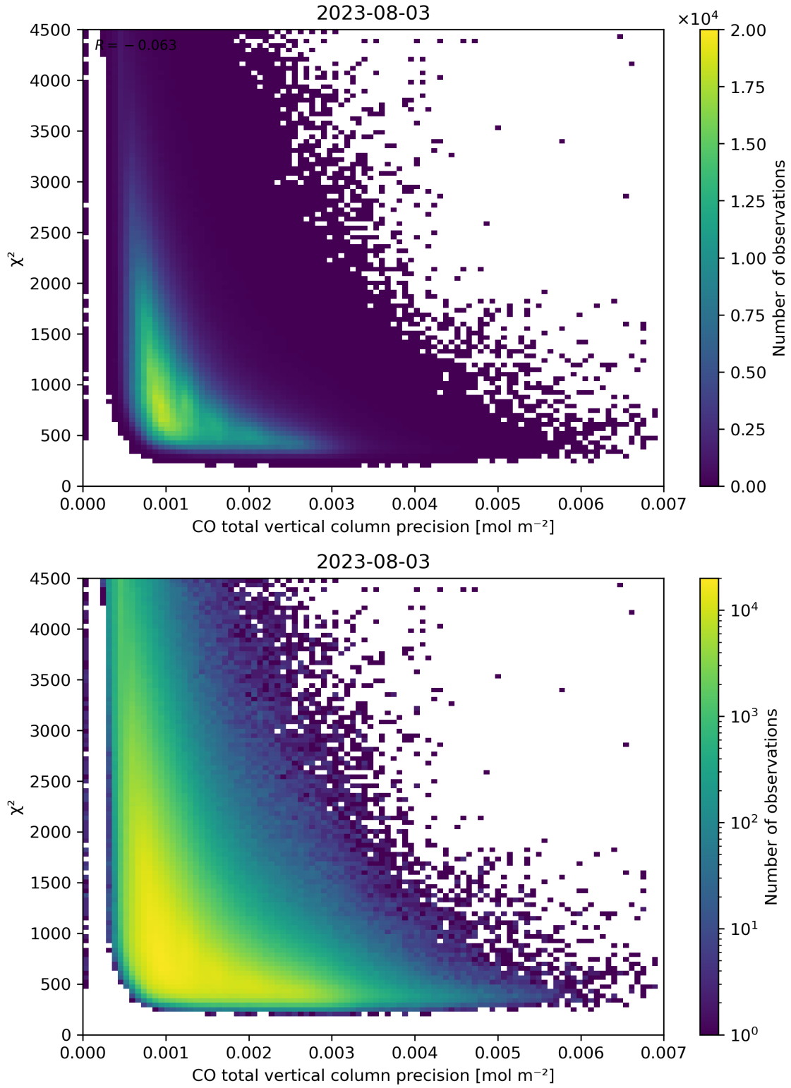
Figure 44: Scatter density plot of “CO total vertical column precision” against “ \chi^2 ” for 2023-08-02 to 2023-08-04.
