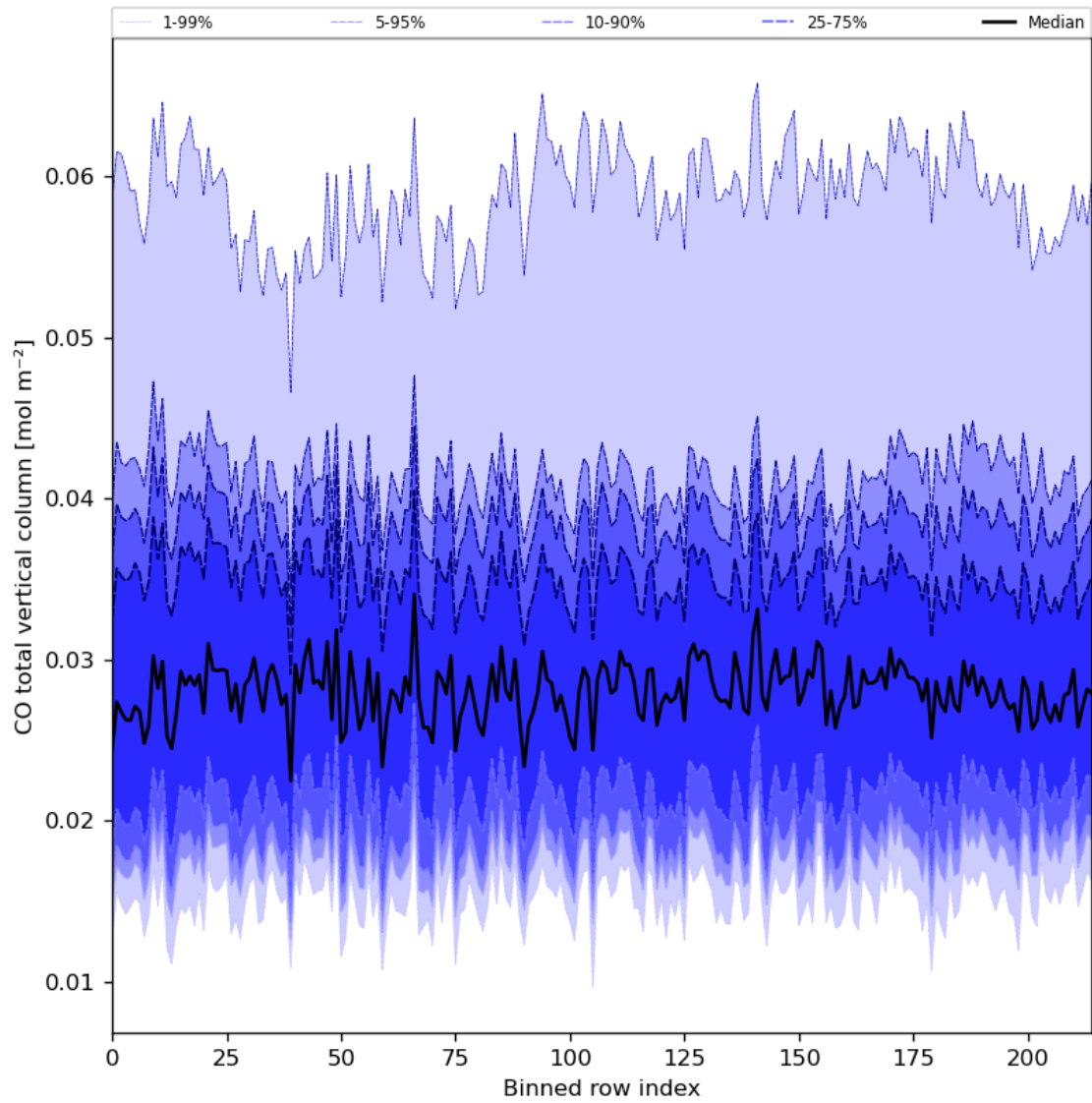
Figure 26: Along track statistics of “CO total vertical column” for 2023-08-02 to 2023-08-04
