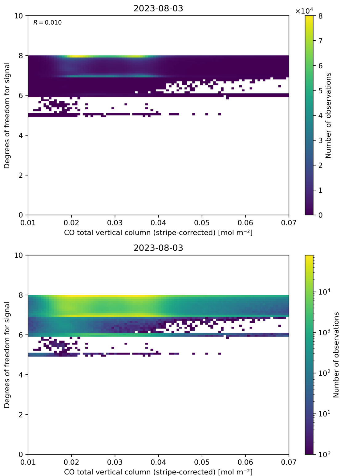
Figure 38: Scatter density plot of “CO total vertical column (stripe-corrected)” against “Degrees of freedom for signal” for 2023-08-02 to 2023-08-04.
