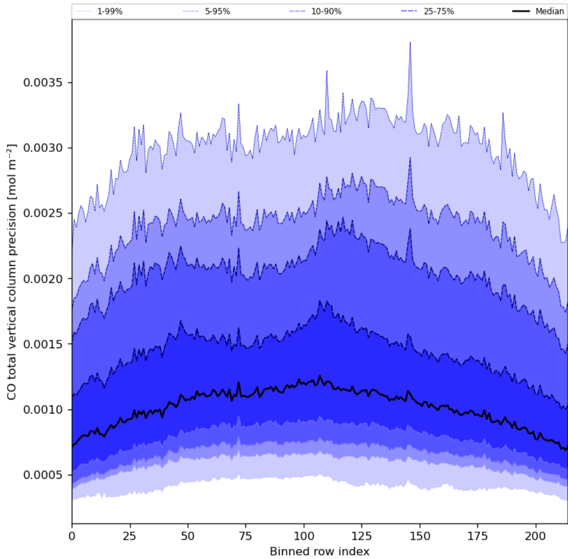
Figure 28: Along track statistics of “CO total vertical column precision” for 2023-08-02 to 2023-08-04
