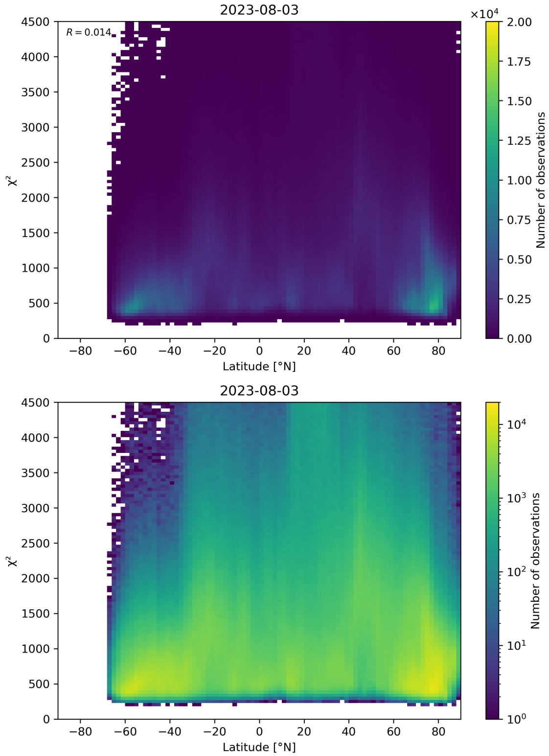
Figure 54: Scatter density plot of “Latitude” against “ \chi^2 ” for 2023-08-02 to 2023-08-04.
