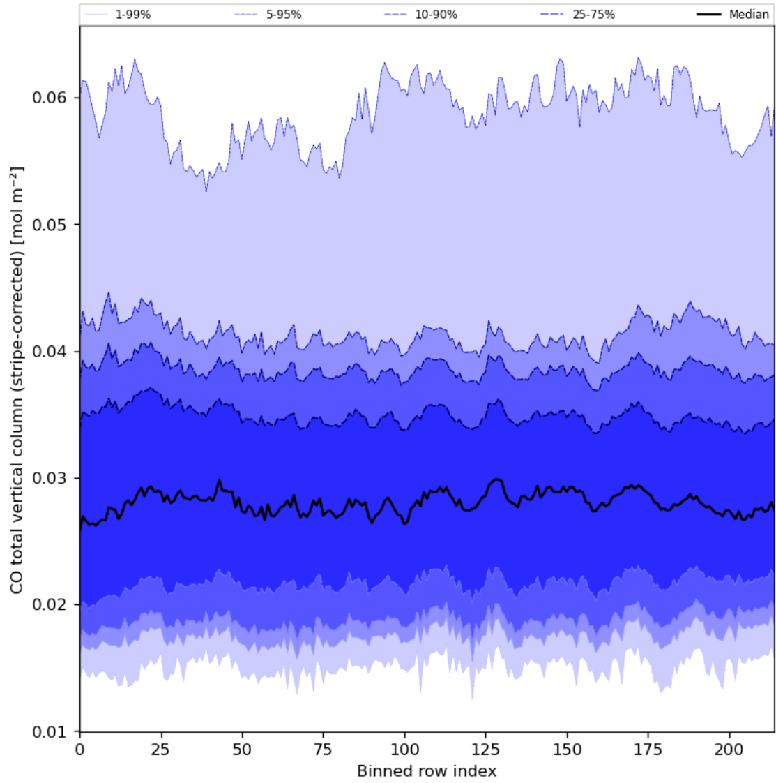
Figure 27: Along track statistics of “CO total vertical column (stripe-corrected)” for 2023-08-02 to 2023-08-04
