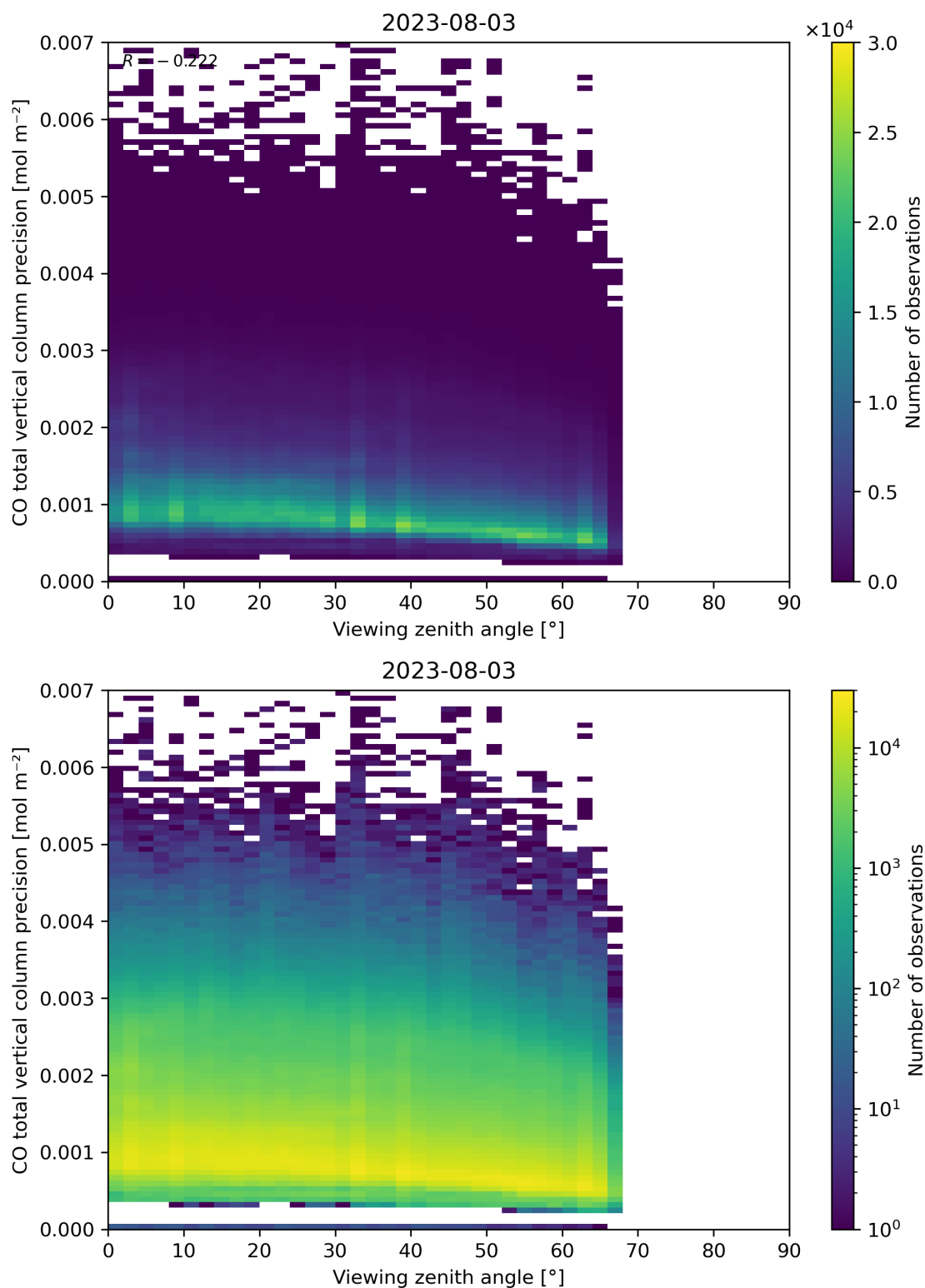
Figure 71: Scatter density plot of “Viewing zenith angle” against “CO total vertical column precision” for 2023-08-02 to 2023-08-04.
