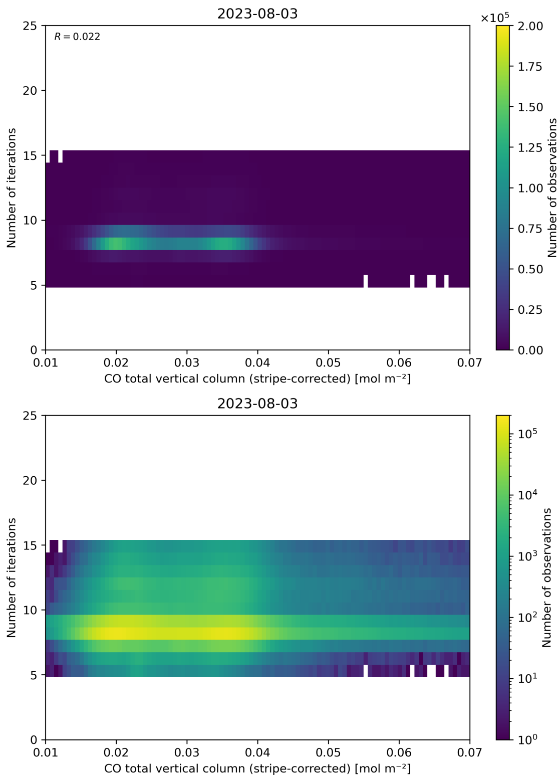
Figure 39: Scatter density plot of “CO total vertical column (stripe-corrected)” against “Number of iterations” for 2023-08-02 to 2023-08-04.
