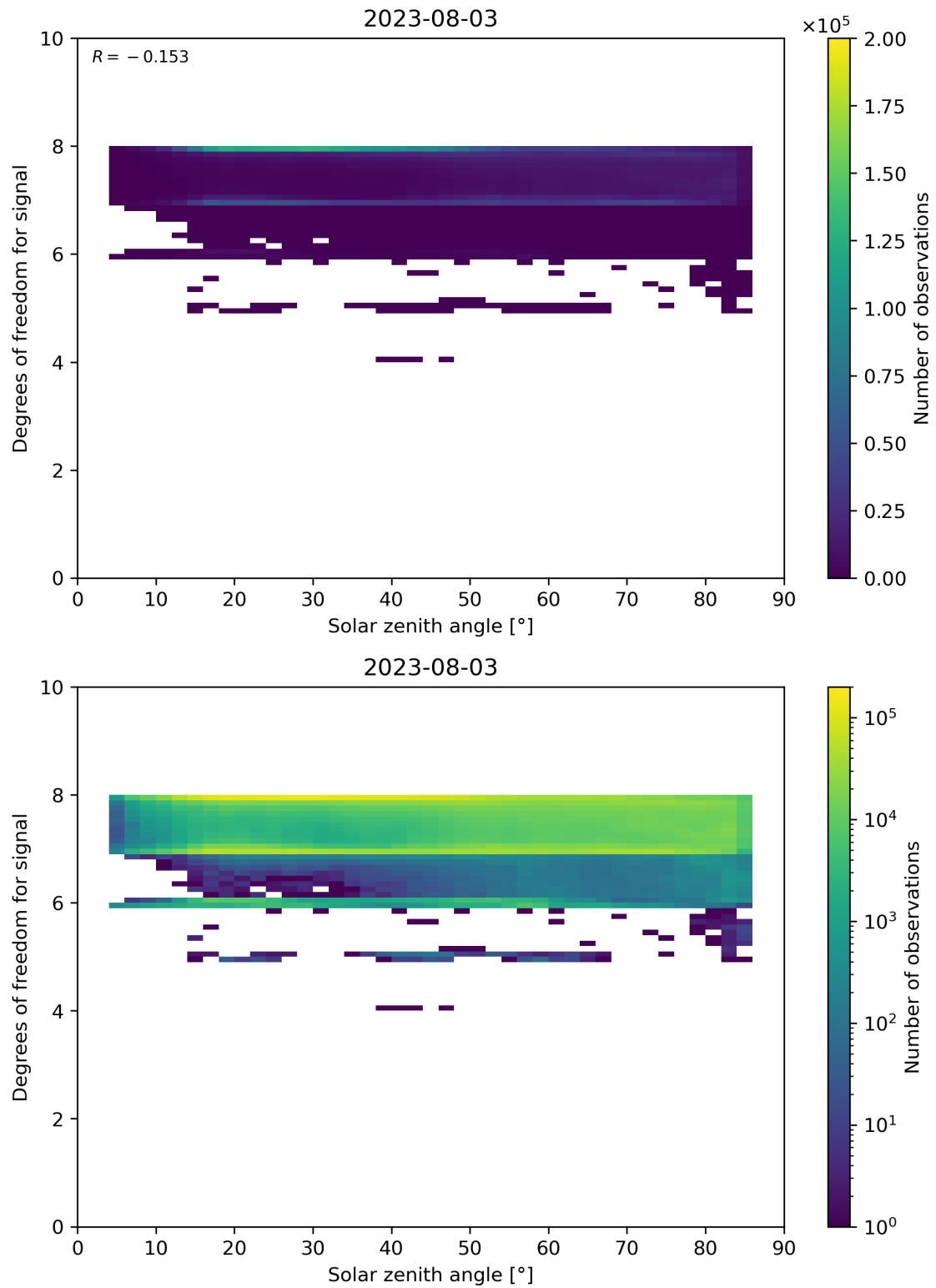
Figure 65: Scatter density plot of “Solar zenith angle” against “Degrees of freedom for signal” for 2023-08-02 to 2023-08-04.
