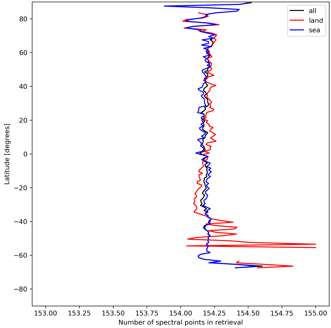
Figure 13: Zonal average of “Number of spectral points in retrieval” for 2023-08-02 to 2023-08-04.
