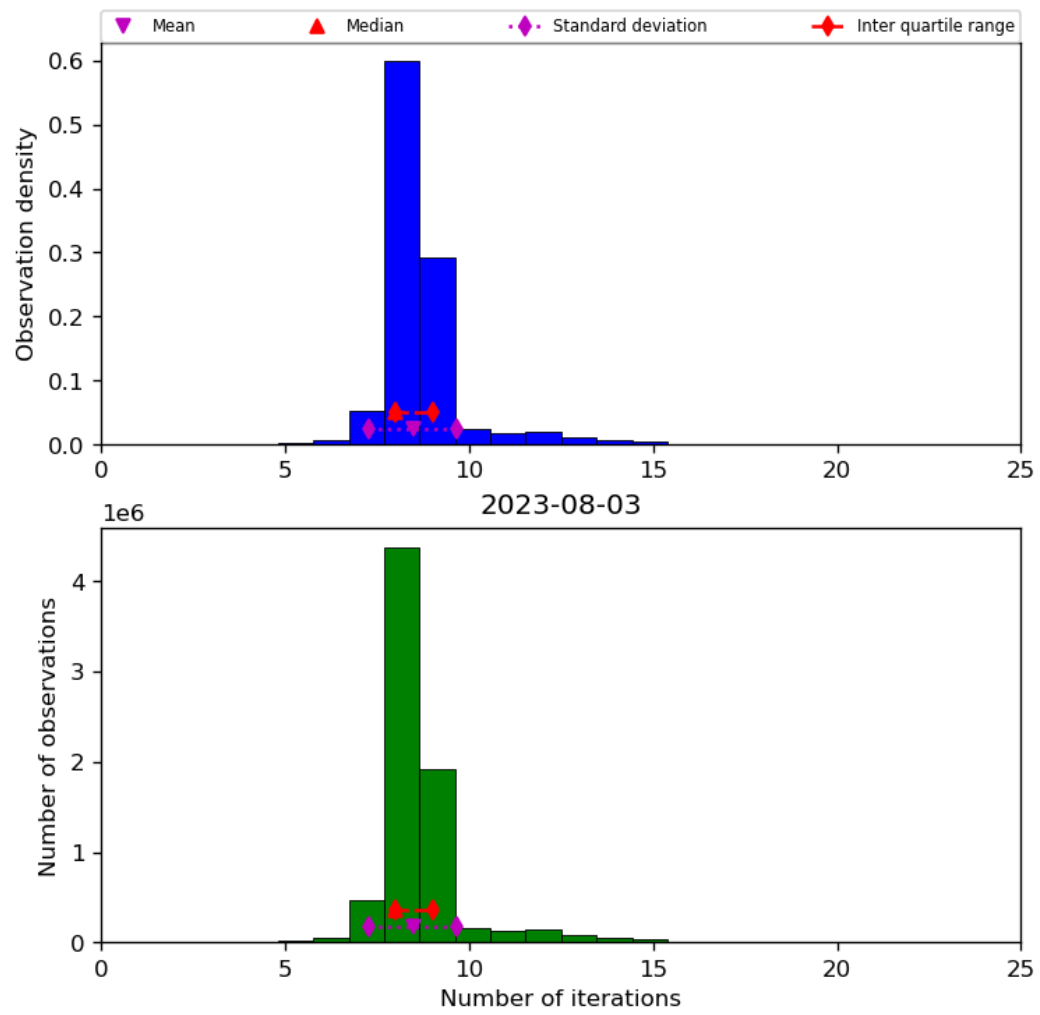
Figure 24: Histogram of "Number of iterations" for 2023-08-02 to 2023-08-04
