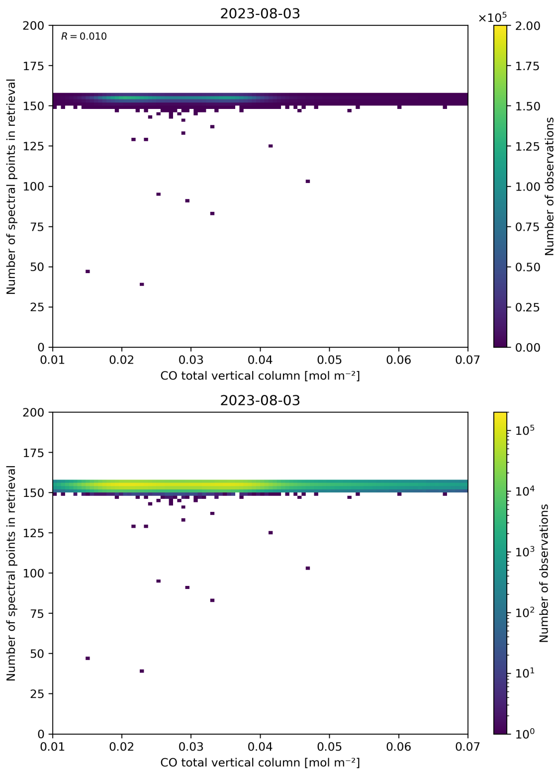
Figure 43: Scatter density plot of “CO total vertical column” against “Number of spectral points in retrieval” for 2023-08-02 to 2023-08-04.
