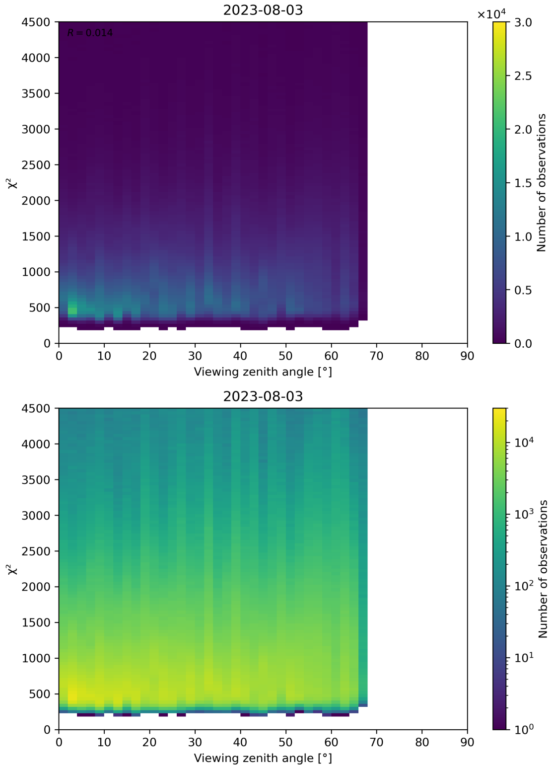
Figure 72: Scatter density plot of “Viewing zenith angle” against “ \chi^2 ” for 2023-08-02 to 2023-08-04.
