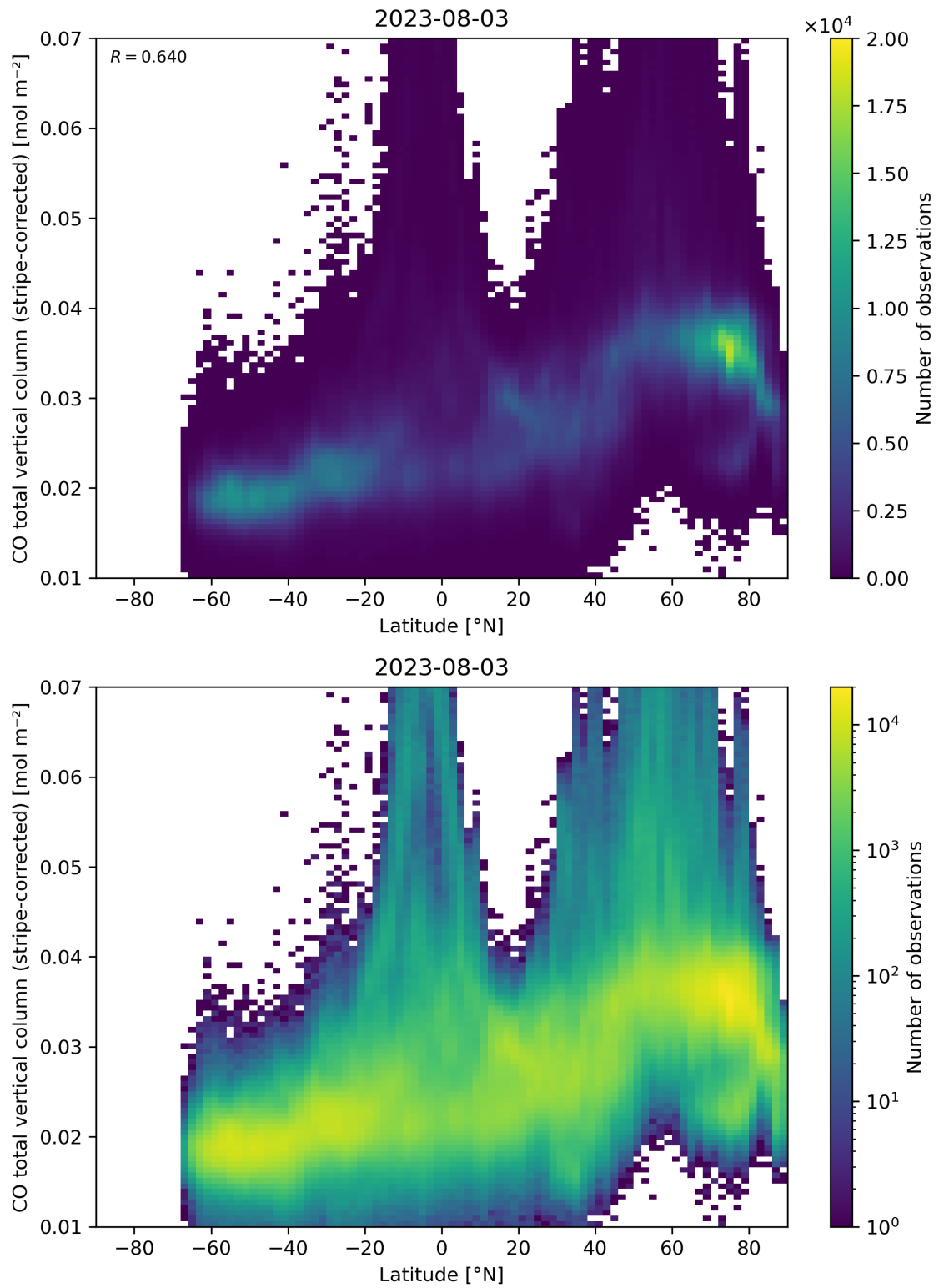
Figure 52: Scatter density plot of “Latitude” against “CO total vertical column (stripe-corrected)” for 2023-08-02 to 2023-08-04.
