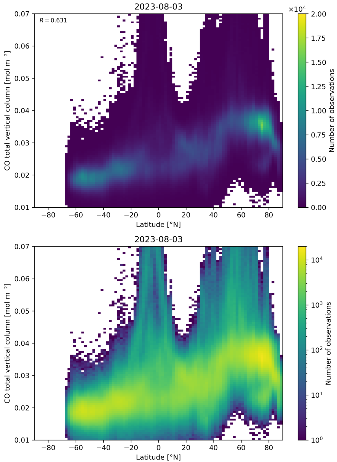
Figure 51: Scatter density plot of “Latitude” against “CO total vertical column” for 2023-08-02 to 2023-08-04.
