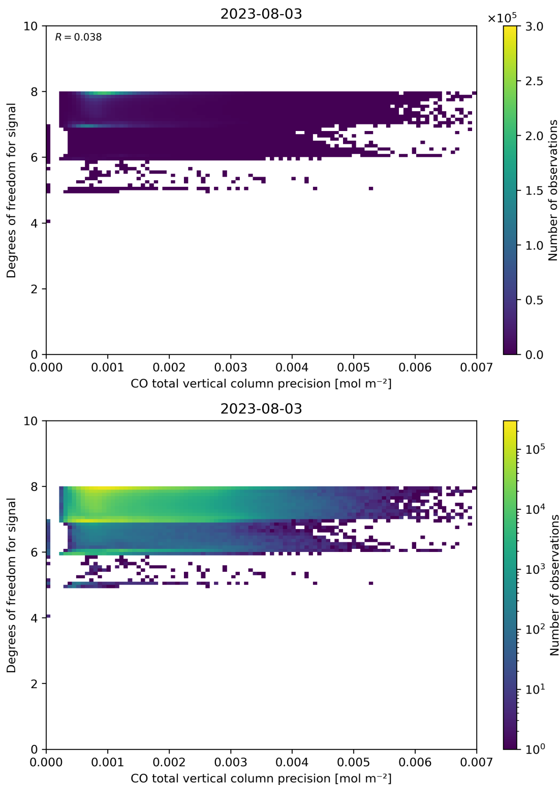
Figure 45: Scatter density plot of “CO total vertical column precision” against “Degrees of freedom for signal” for 2023-08-02 to 2023-08-04.
