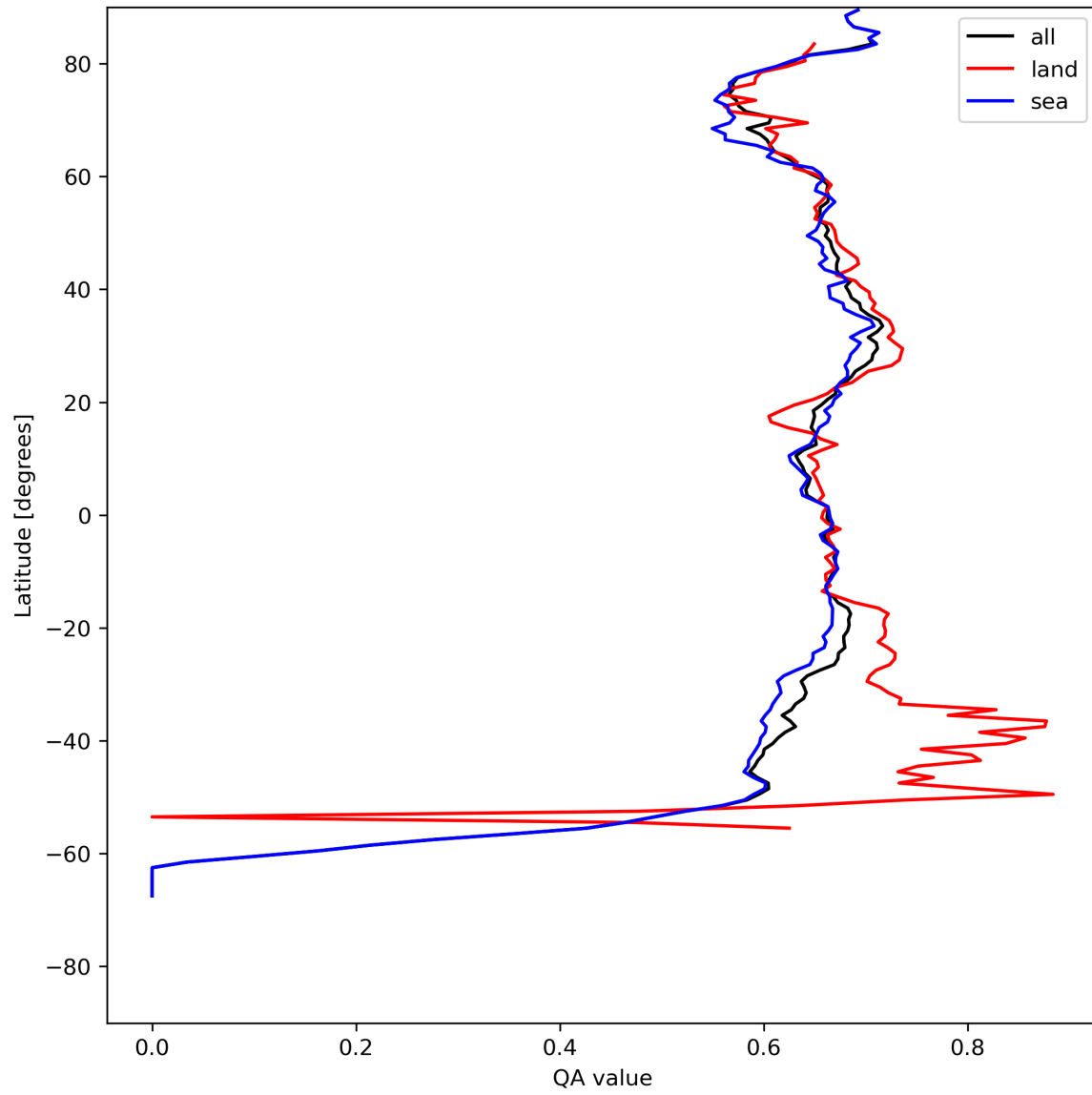
Figure 9: Zonal average of “QA value” for 2023-08-02 to 2023-08-04.
