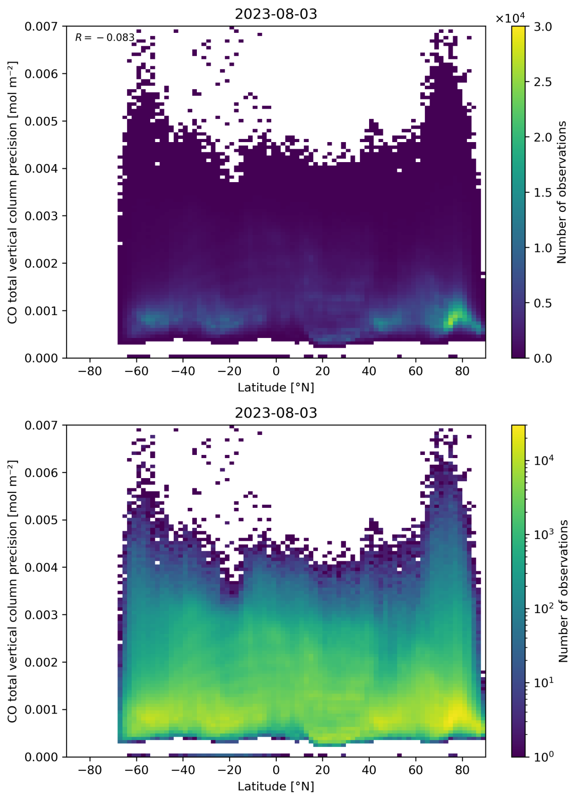
Figure 53: Scatter density plot of “Latitude” against “CO total vertical column precision” for 2023-08-02 to 2023-08-04.
