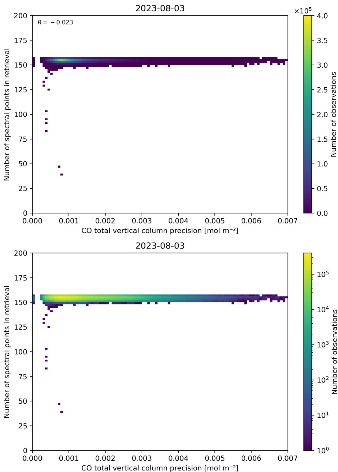
Figure 47: Scatter density plot of “CO total vertical column precision” against “Number of spectral points in retrieval” for 2023-08-02 to 2023-08-04.
