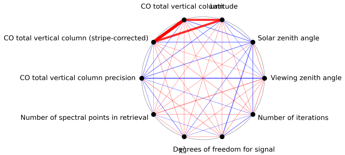
Figure 1: Map of correlation graph for 2023-08-02 to 2023-08-04.
