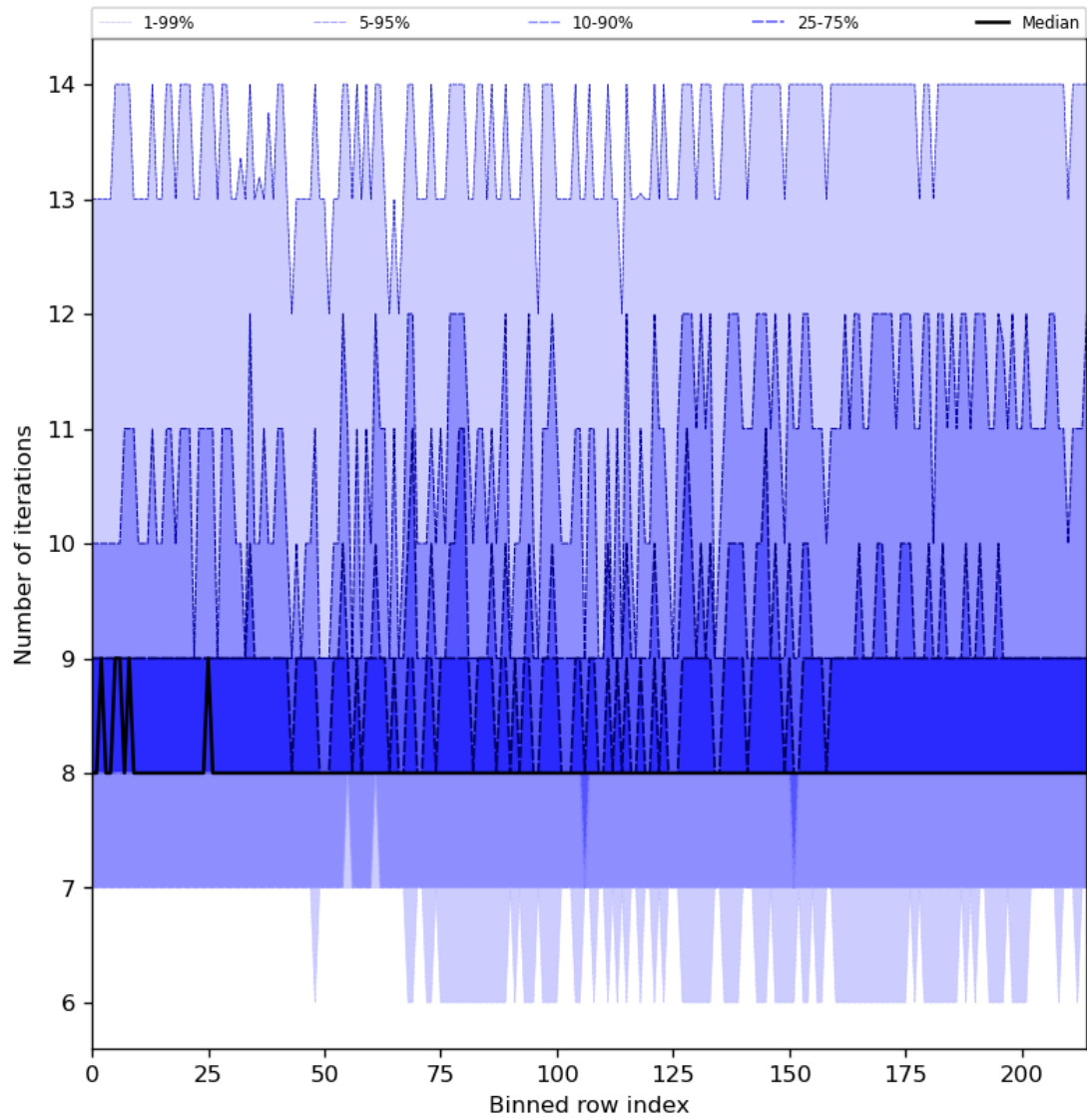
Figure 32: Along track statistics of “Number of iterations” for 2023-08-02 to 2023-08-04
