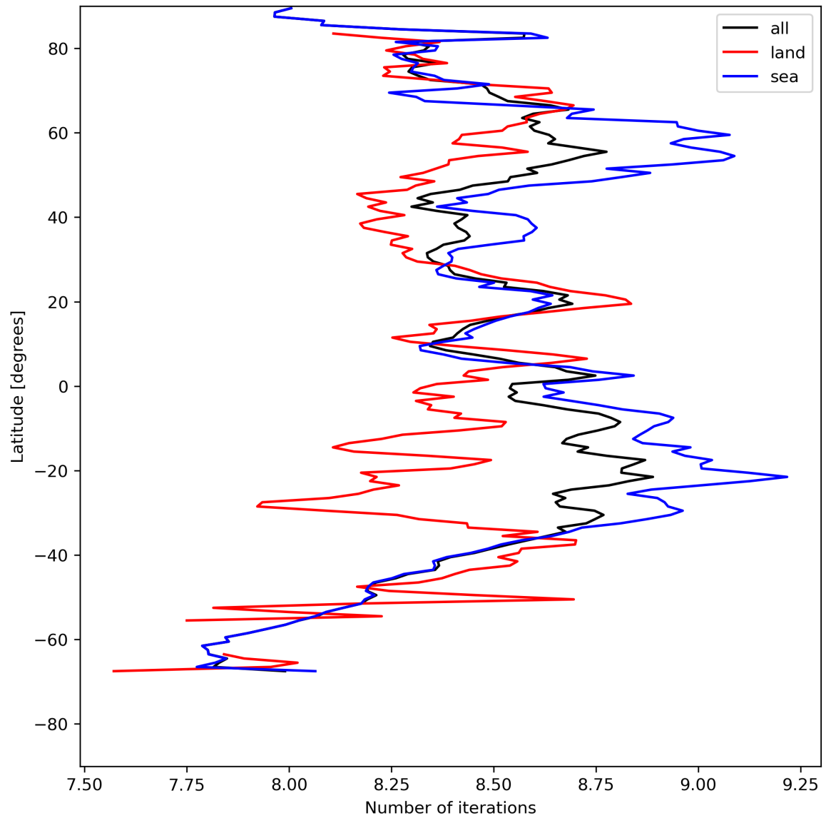
Figure 16: Zonal average of “Number of iterations” for 2023-08-02 to 2023-08-04.
