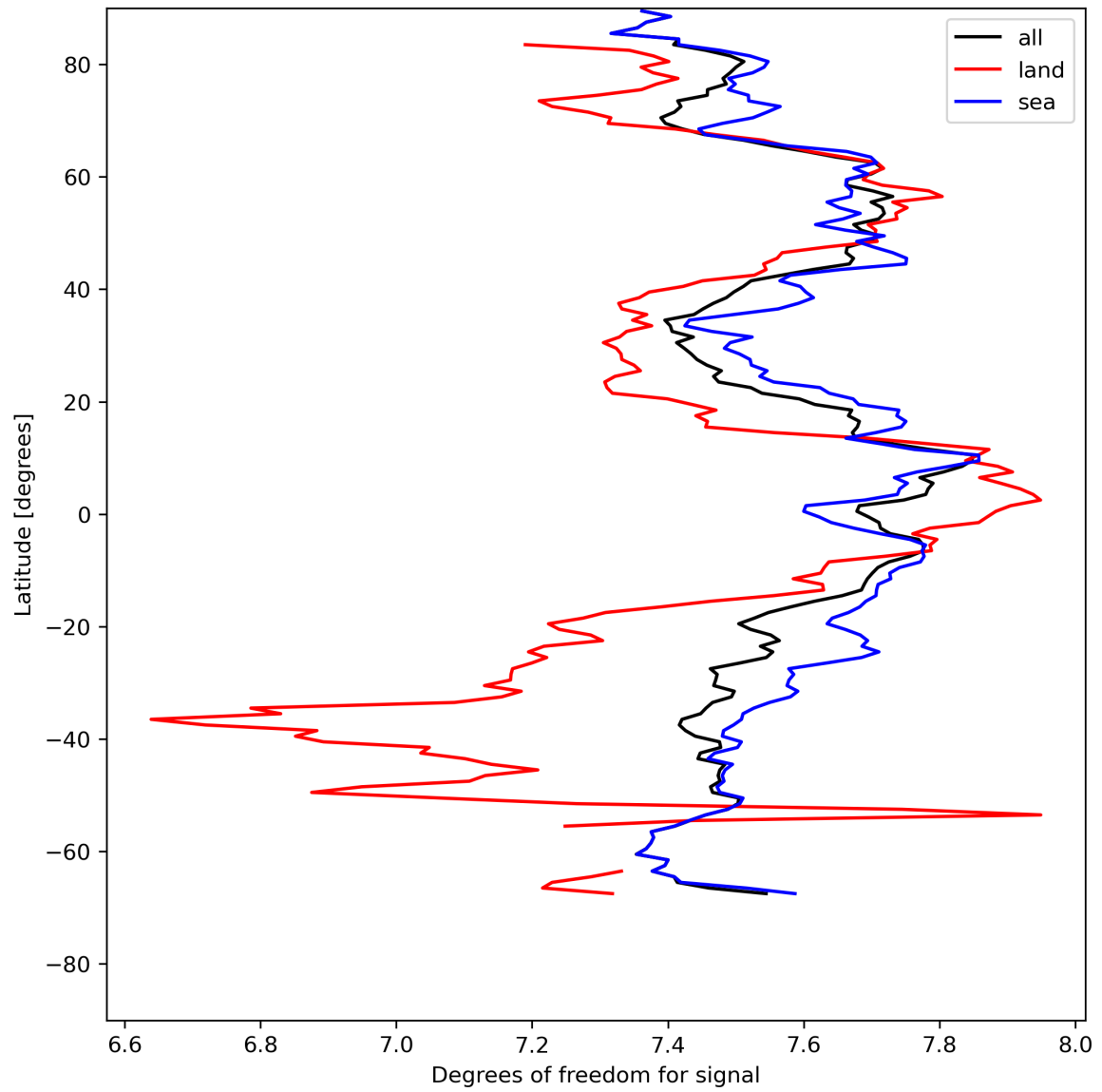
Figure 15: Zonal average of “Degrees of freedom for signal” for 2023-08-02 to 2023-08-04.
