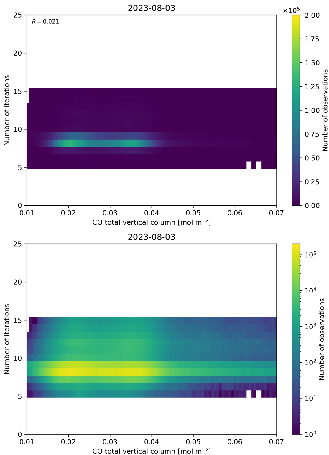
Figure 42: Scatter density plot of “CO total vertical column” against “Number of iterations” for 2023-08-02 to 2023-08-04.
