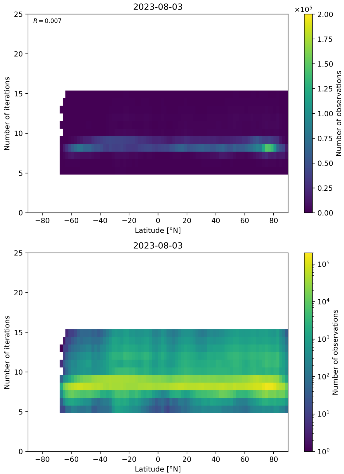
Figure 56: Scatter density plot of “Latitude” against “Number of iterations” for 2023-08-02 to 2023-08-04.
