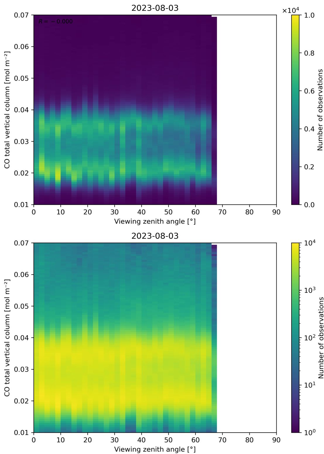
Figure 69: Scatter density plot of “Viewing zenith angle” against “CO total vertical column” for 2023-08-02 to 2023-08-04.
