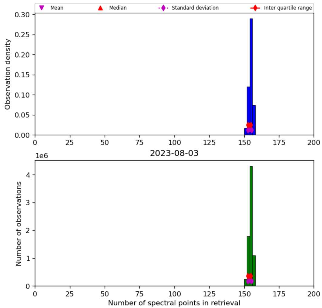
Figure 21: Histogram of “Number of spectral points in retrieval” for 2023-08-02 to 2023-08-04
