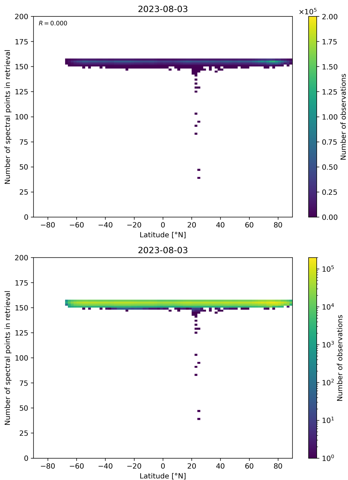
Figure 57: Scatter density plot of “Latitude” against “Number of spectral points in retrieval” for 2023-08-02 to 2023-08-04.
