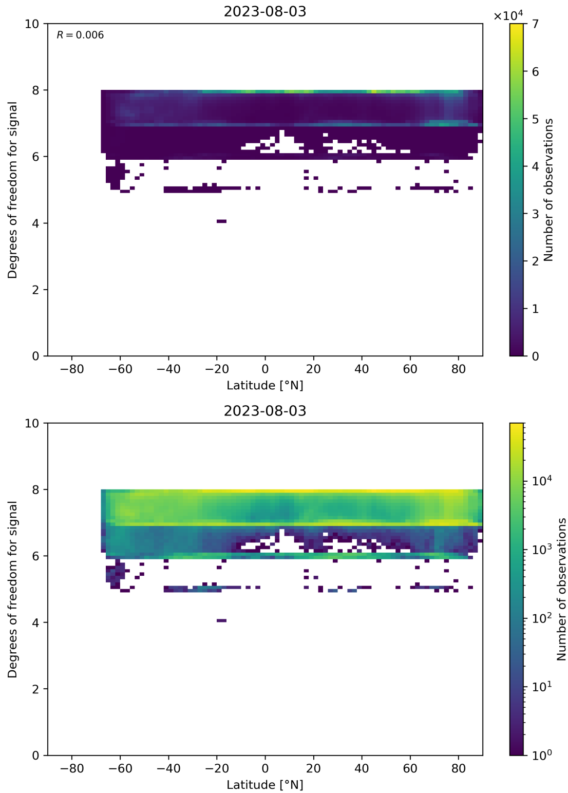
Figure 55: Scatter density plot of “Latitude” against “Degrees of freedom for signal” for 2023-08-02 to 2023-08-04.
