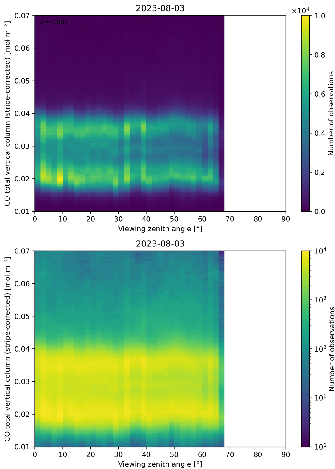
Figure 70: Scatter density plot of “Viewing zenith angle” against “CO total vertical column (stripe-corrected)” for 2023-08-02 to 2023-08-04.
