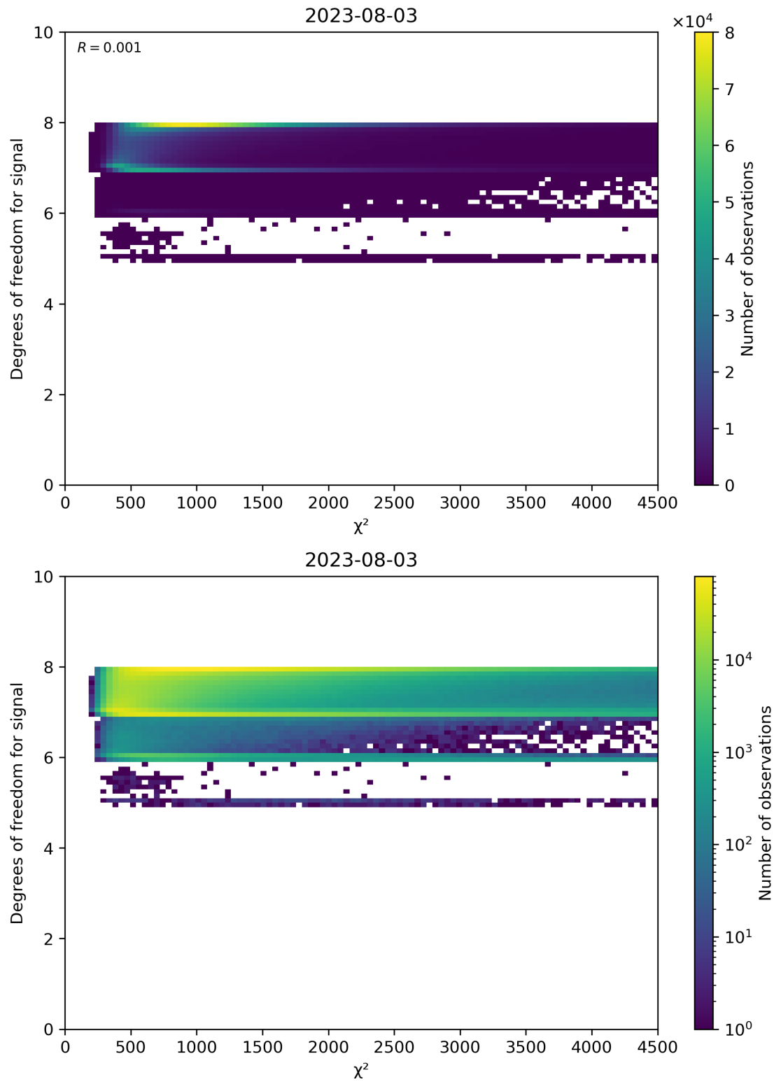
Figure 48: Scatter density plot of “ \chi^2 ” against “Degrees of freedom for signal” for 2023-08-02 to 2023-08-04.
