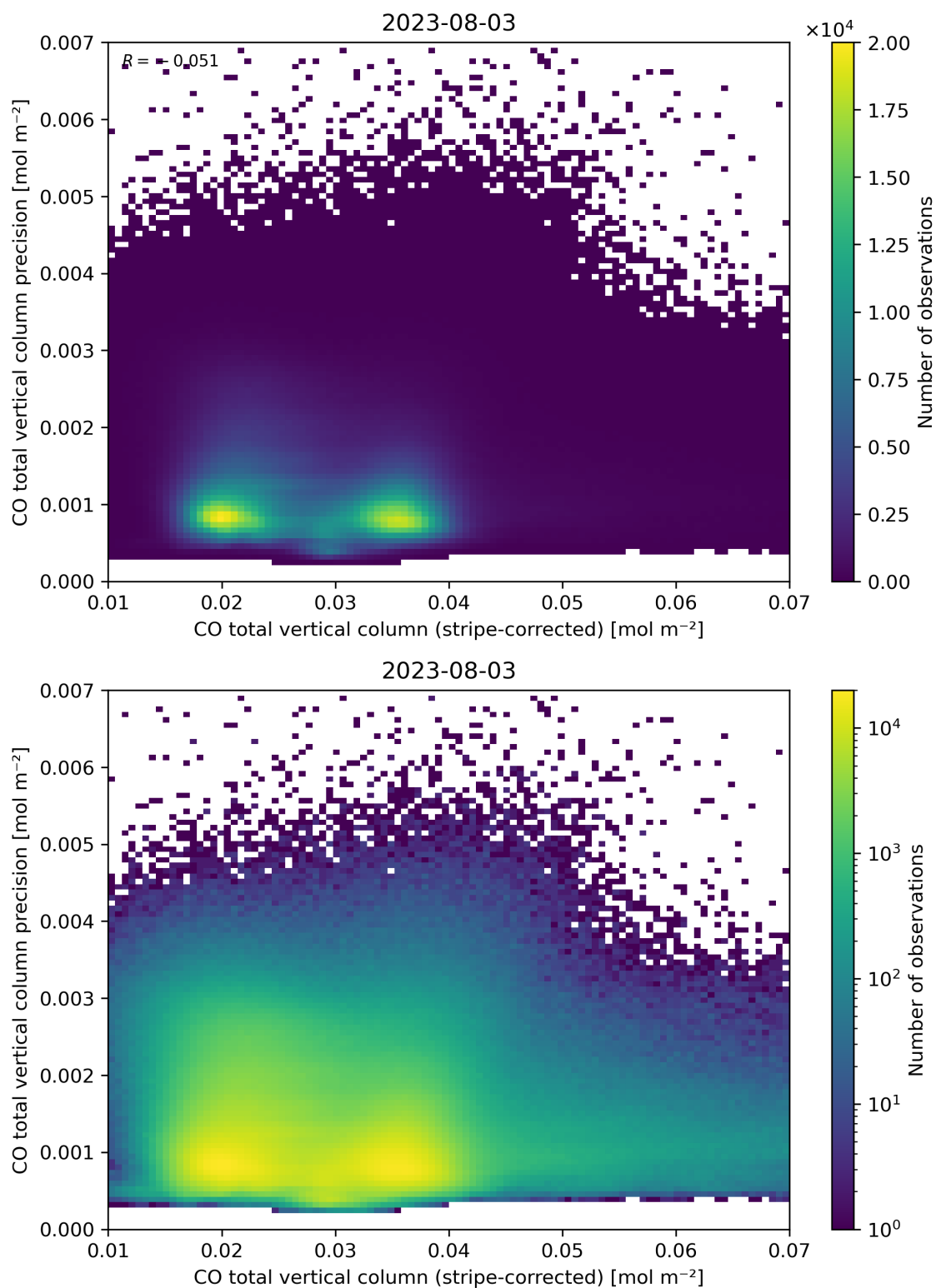
Figure 36: Scatter density plot of “CO total vertical column (stripe-corrected)” against “CO total vertical column precision” for 2023-08-02 to 2023-08-04.
