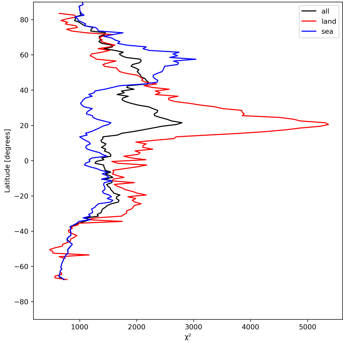
Figure 14: Zonal average of “ \chi^2 ” for 2023-08-02 to 2023-08-04.
