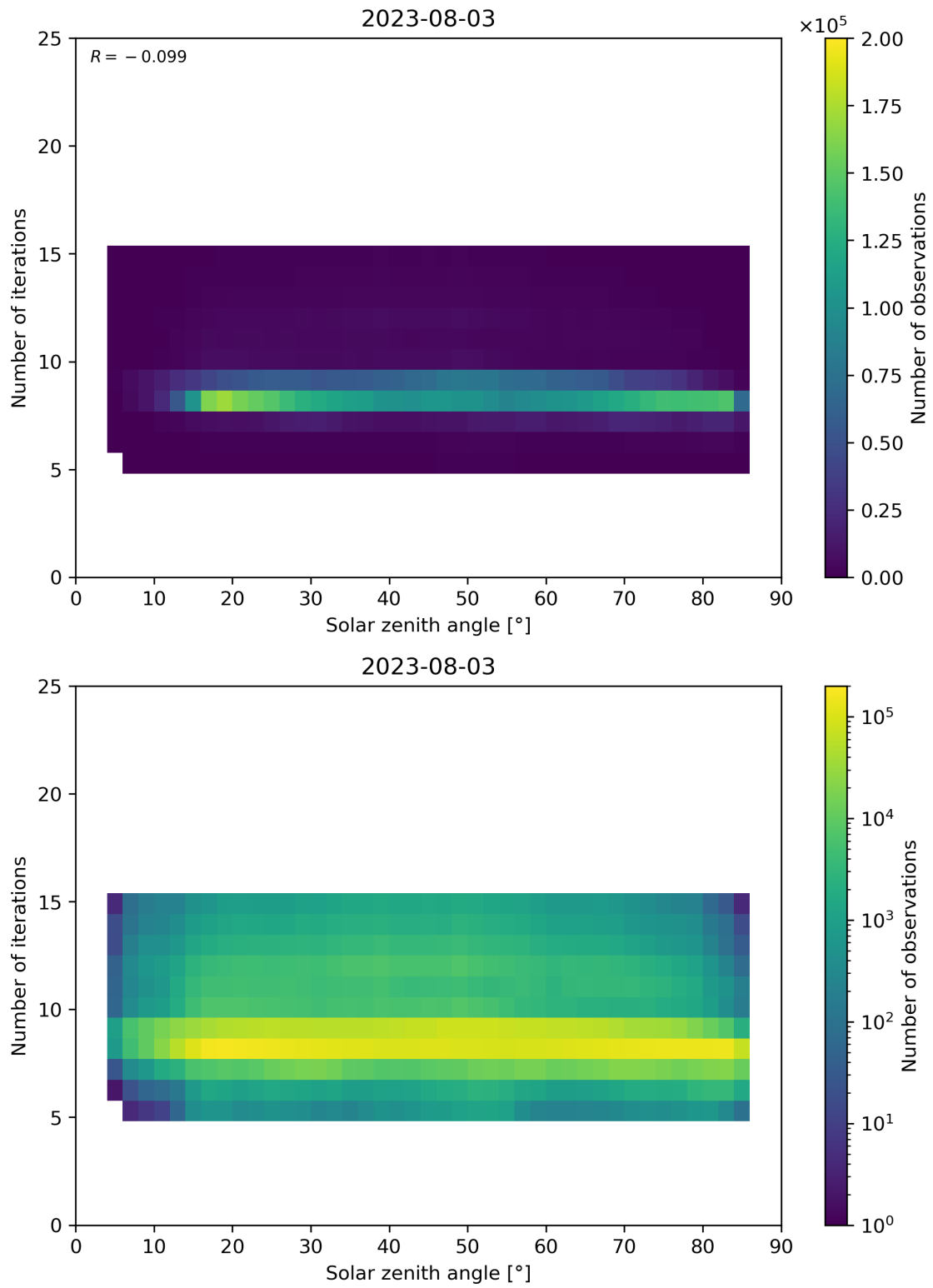
Figure 67: Scatter density plot of “Solar zenith angle” against “Number of iterations” for 2023-08-02 to 2023-08-04.
