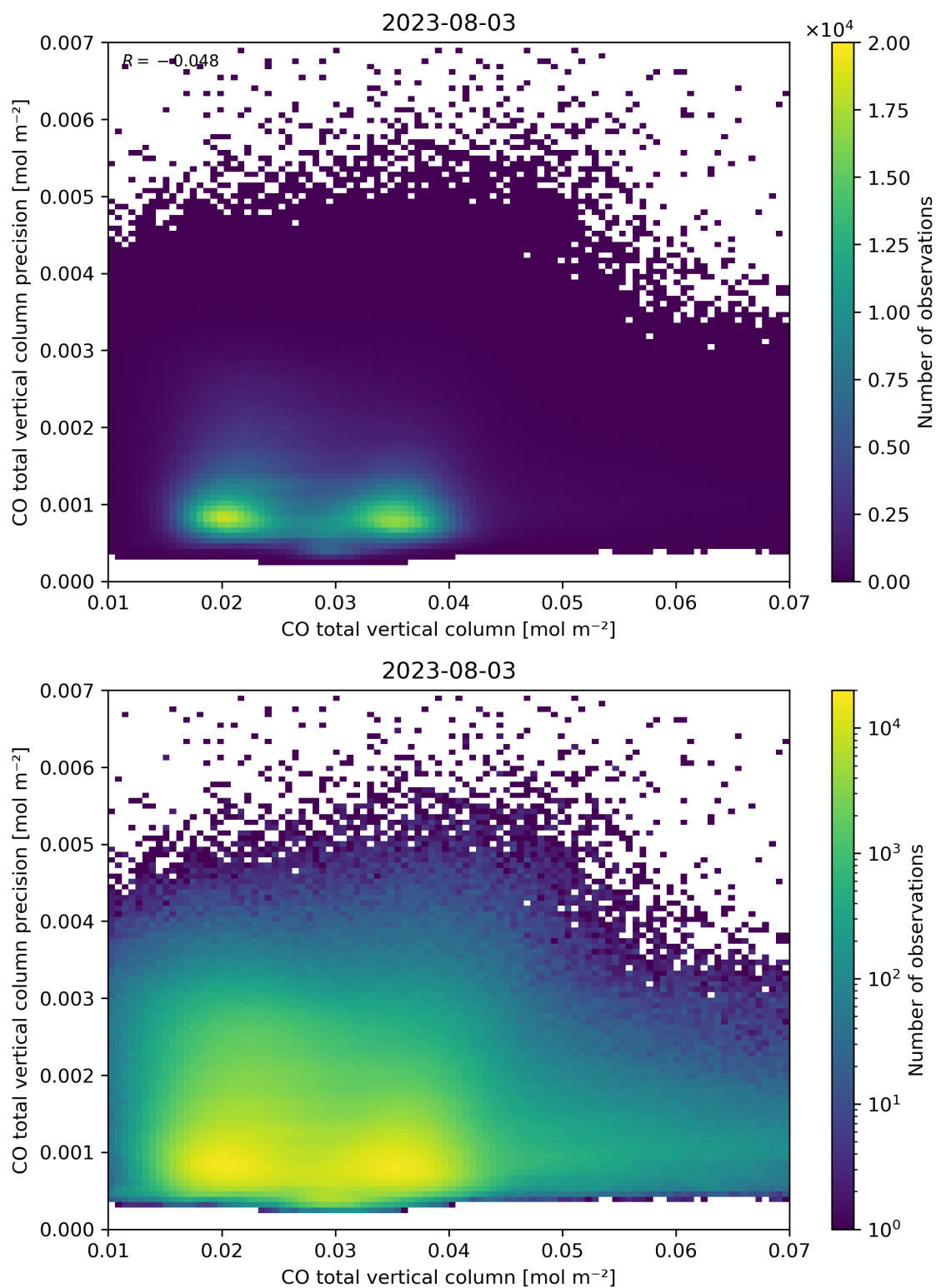
Figure 34: Scatter density plot of “CO total vertical column” against “CO total vertical column precision” for 2023-08-02 to 2023-08-04.
