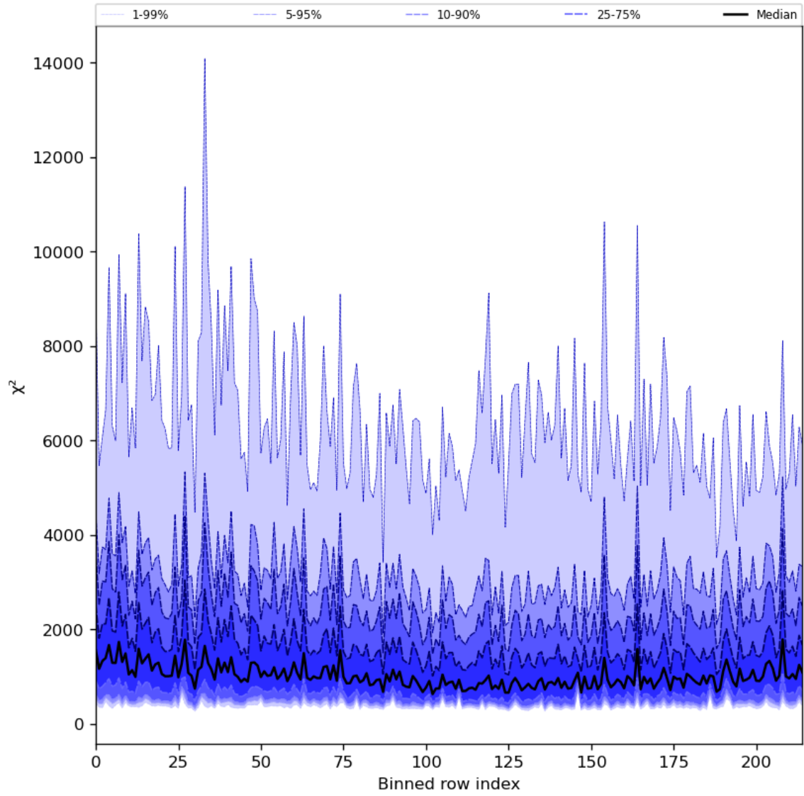
Figure 30: Along track statistics of “ \chi^2 ” for 2023-08-02 to 2023-08-04
