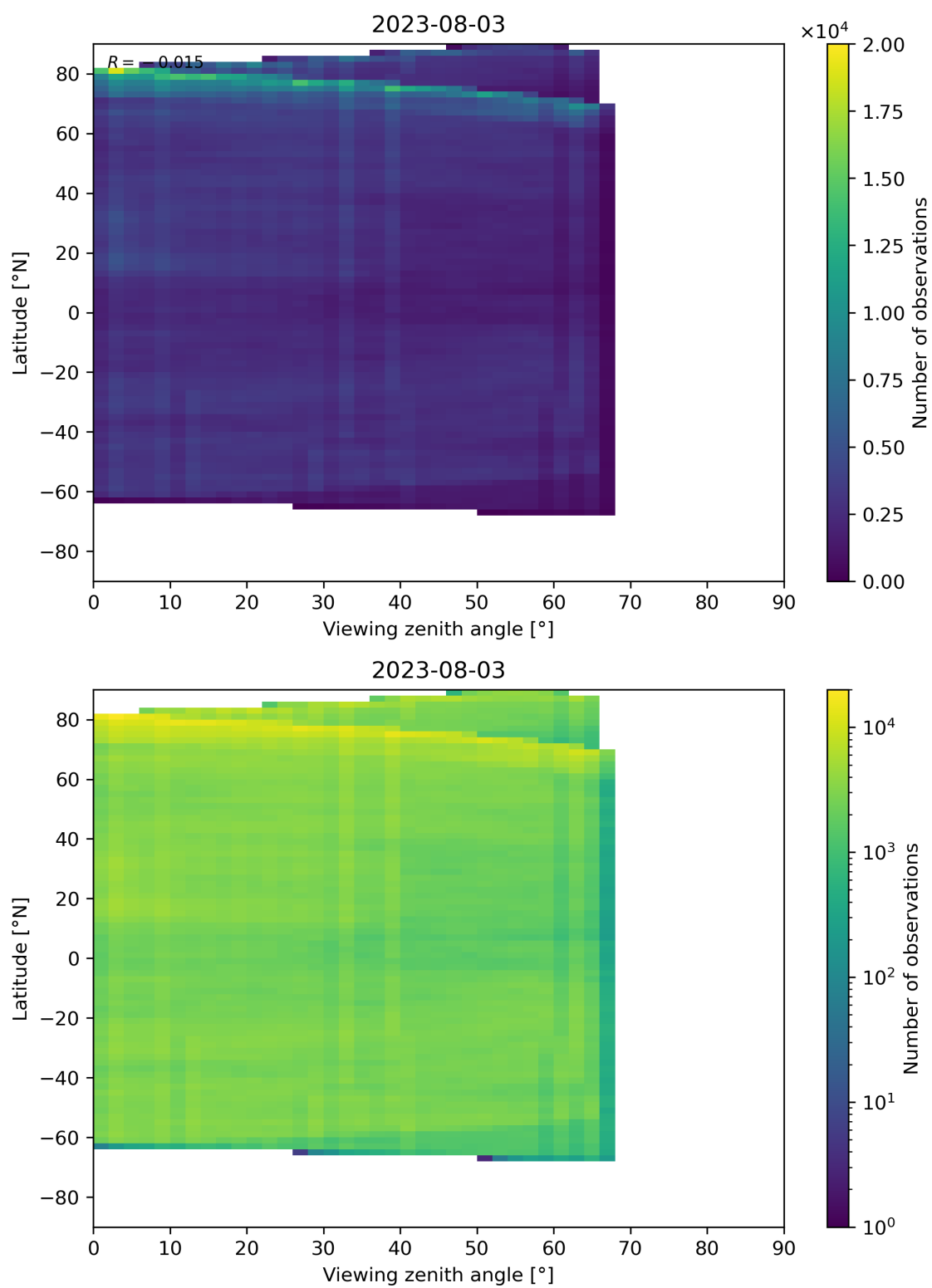
Figure 74: Scatter density plot of “Viewing zenith angle” against “Latitude” for 2023-08-02 to 2023-08-04.
