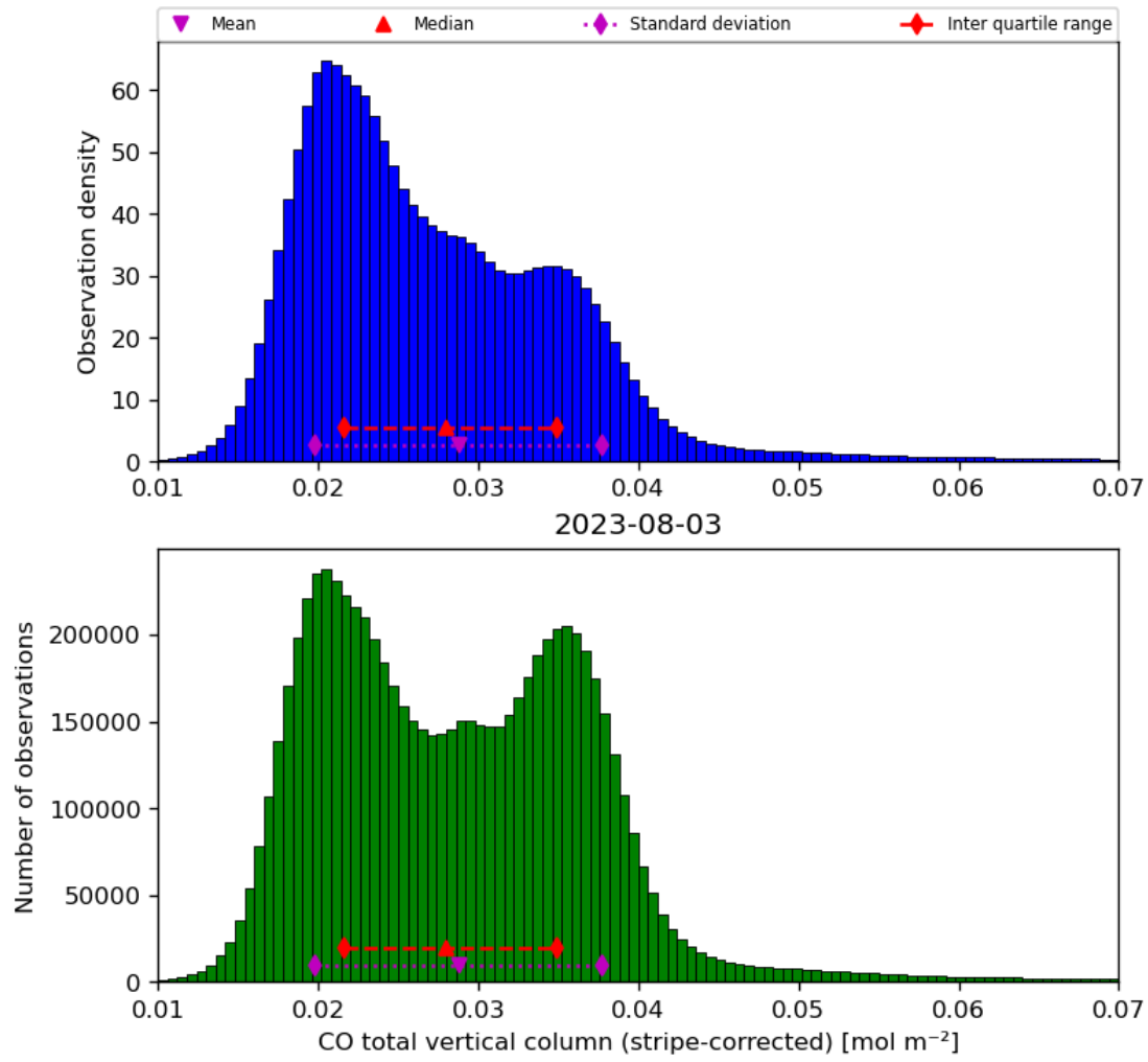
Figure 19: Histogram of “CO total vertical column (stripe-corrected)” for 2023-08-02 to 2023-08-04
