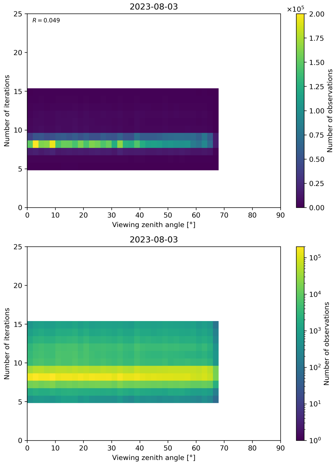
Figure 75: Scatter density plot of “Viewing zenith angle” against “Number of iterations” for 2023-08-02 to 2023-08-04.
