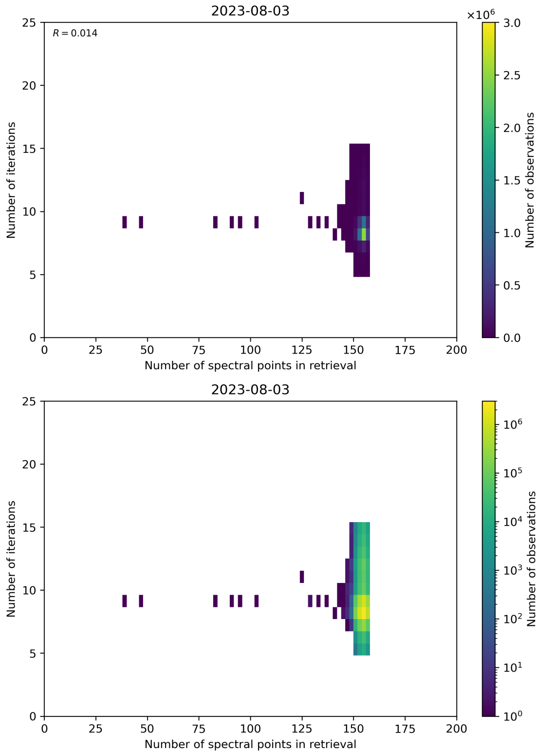
Figure 60: Scatter density plot of “Number of spectral points in retrieval” against “Number of iterations” for 2023-08-02 to 2023-08-04.
