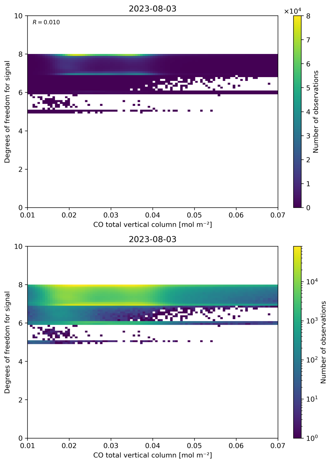
Figure 41: Scatter density plot of “CO total vertical column” against “Degrees of freedom for signal” for 2023-08-02 to 2023-08-04.
