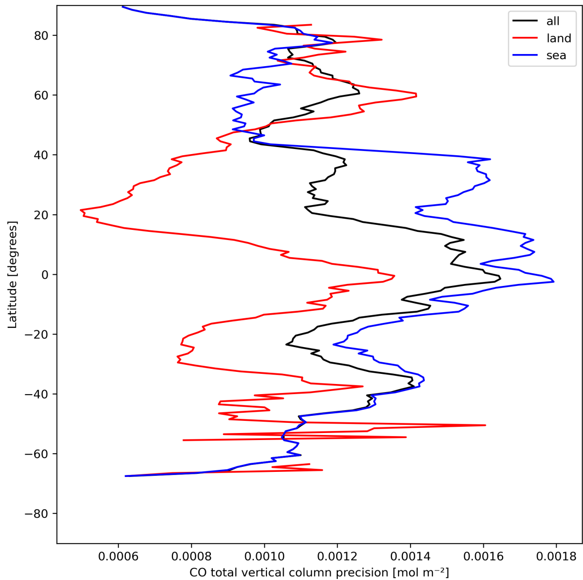
Figure 12: Zonal average of “CO total vertical column precision” for 2023-08-02 to 2023-08-04.
