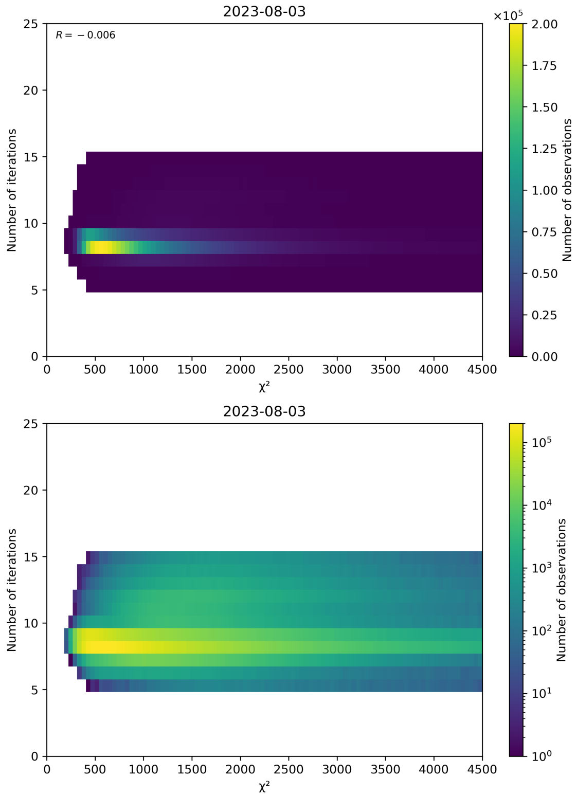
Figure 49: Scatter density plot of “ \chi^2 ” against “Number of iterations” for 2023-08-02 to 2023-08-04.
