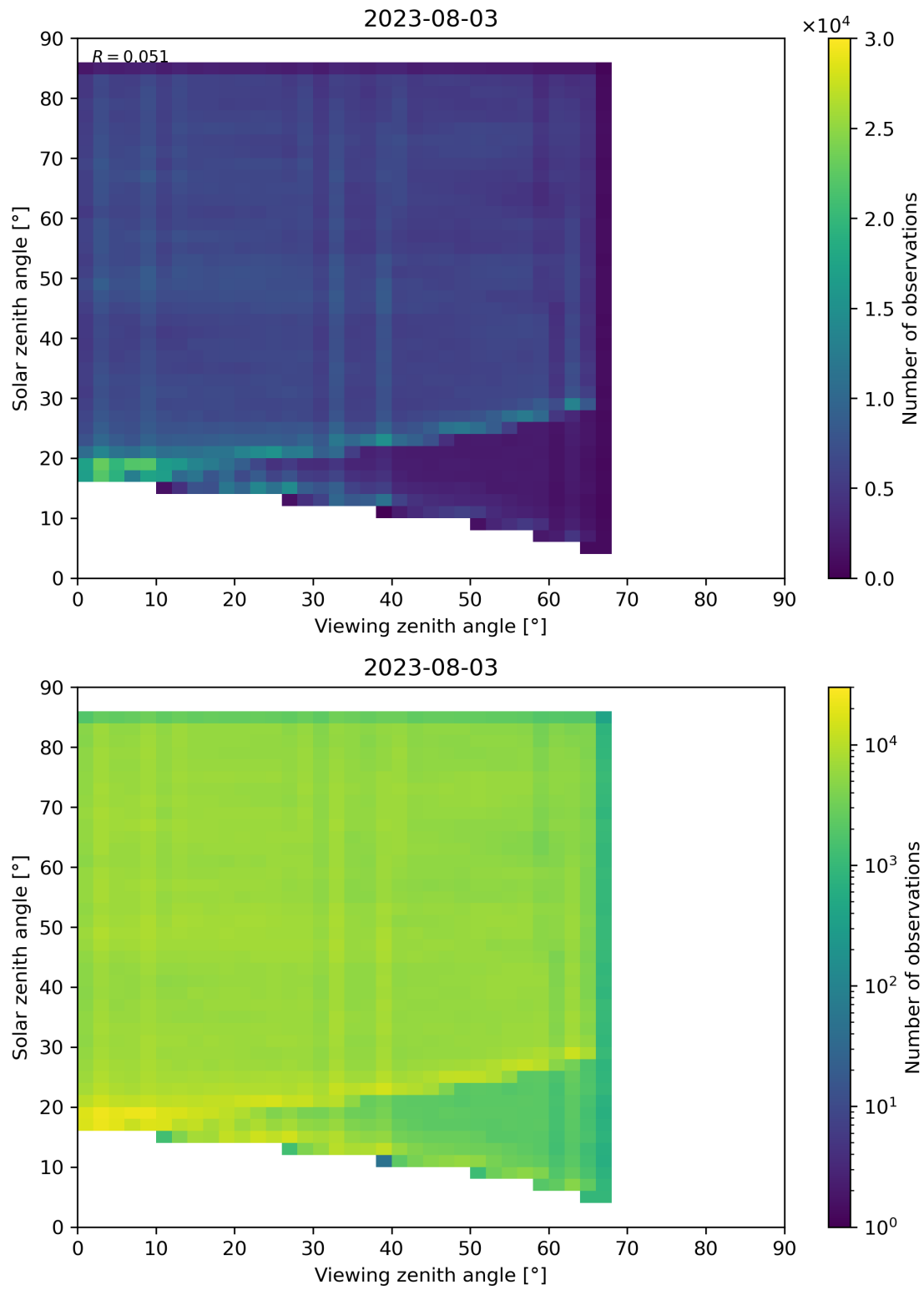
Figure 77: Scatter density plot of “Viewing zenith angle” against “Solar zenith angle” for 2023-08-02 to 2023-08-04.
