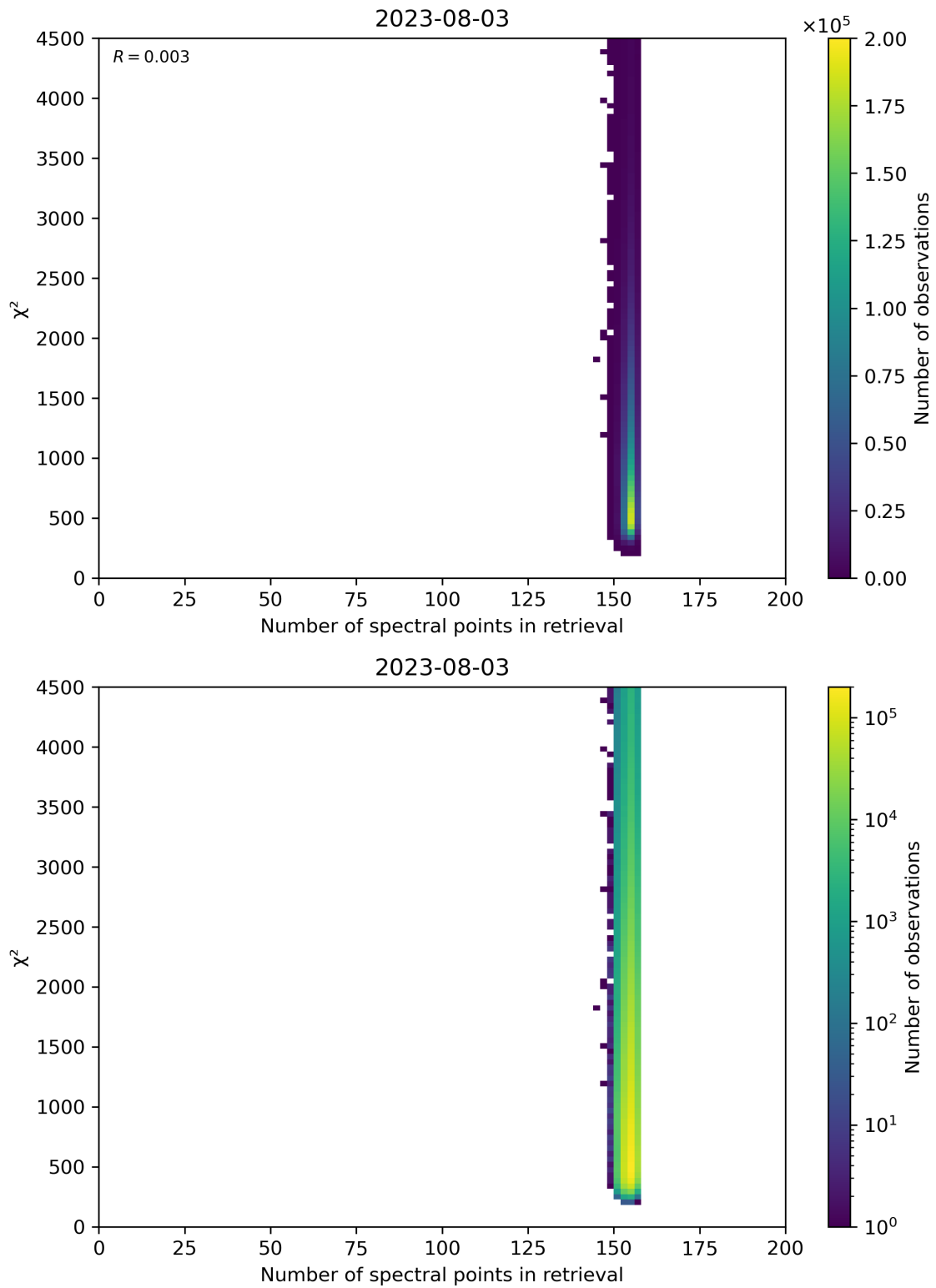
Figure 58: Scatter density plot of “Number of spectral points in retrieval” against “ \chi^2 ” for 2023-08-02 to 2023-08-04.
