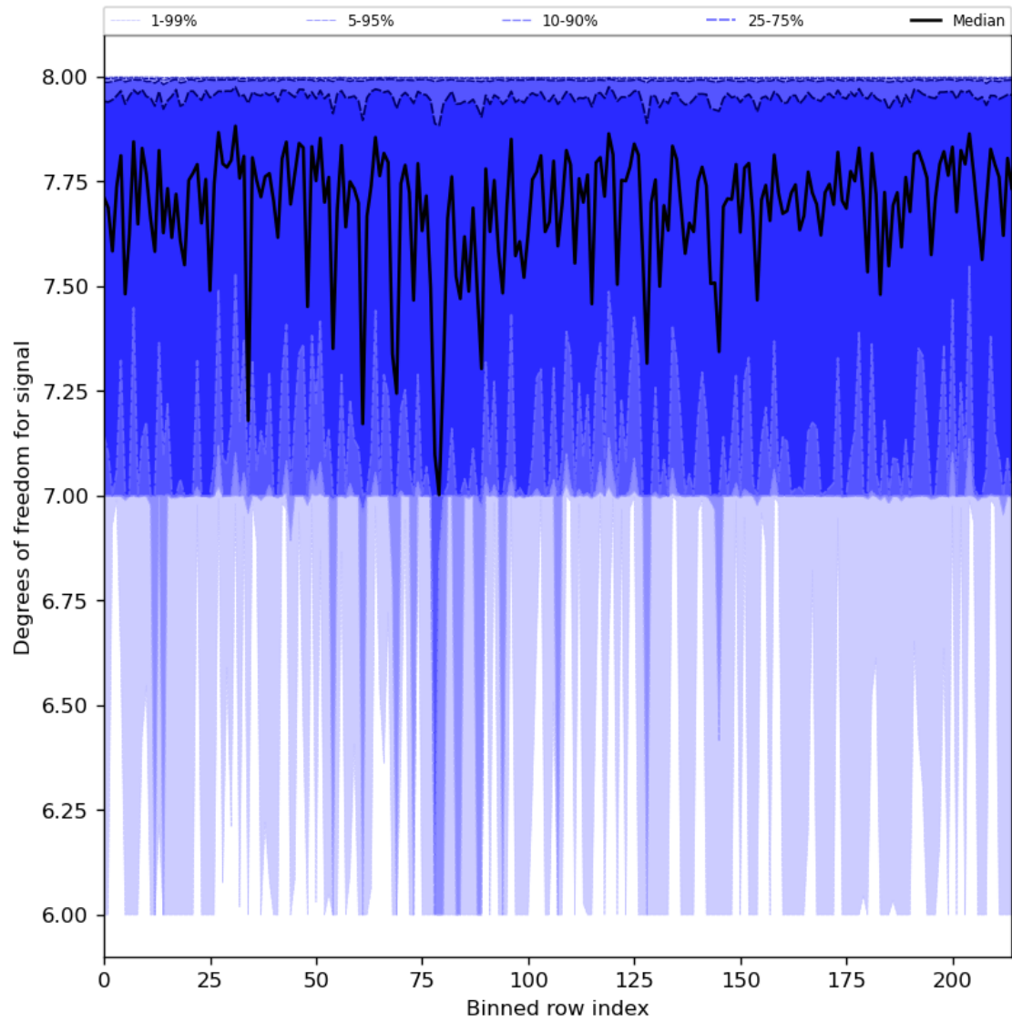
Figure 31: Along track statistics of “Degrees of freedom for signal” for 2023-08-02 to 2023-08-04
