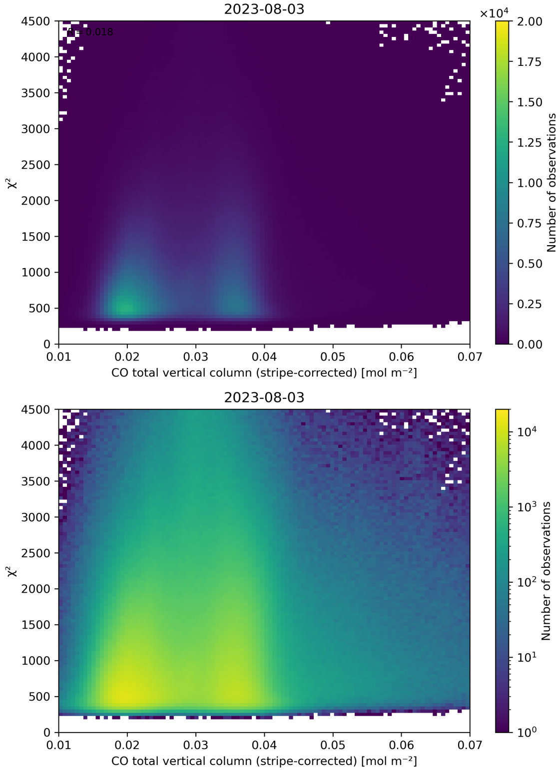
Figure 37: Scatter density plot of “CO total vertical column (stripe-corrected)” against “ \chi^2 ” for 2023-08-02 to 2023-08-04.
