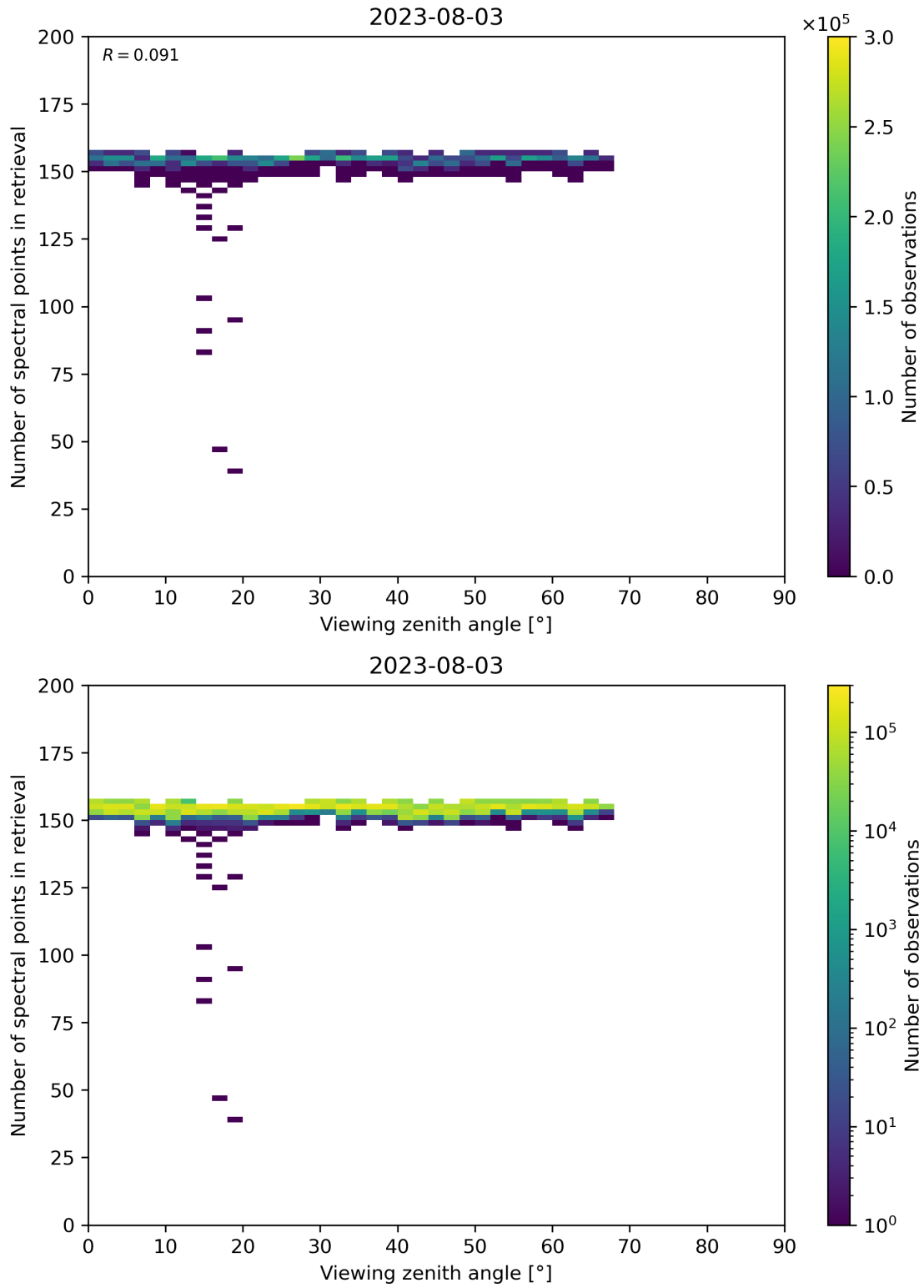
Figure 76: Scatter density plot of “Viewing zenith angle” against “Number of spectral points in retrieval” for 2023-08-02 to 2023-08-04.
