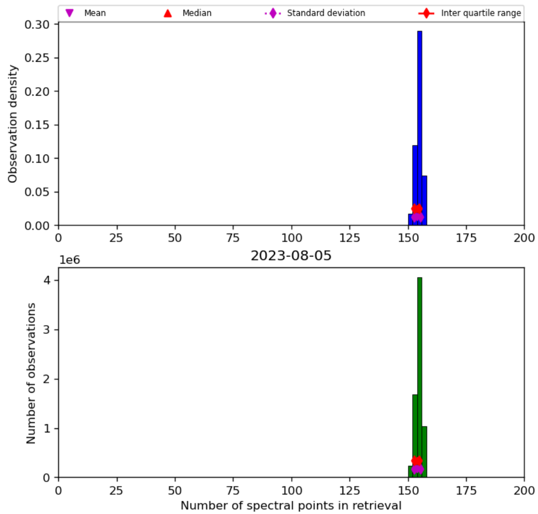
Figure 21: Histogram of “Number of spectral points in retrieval” for 2023-08-04 to 2023-08-06
