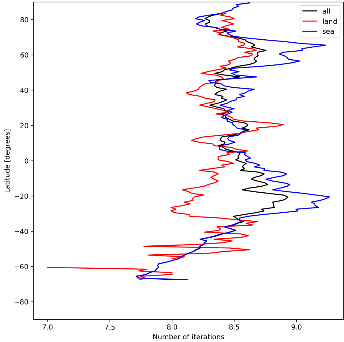
Figure 16: Zonal average of “Number of iterations” for 2023-08-04 to 2023-08-06.
