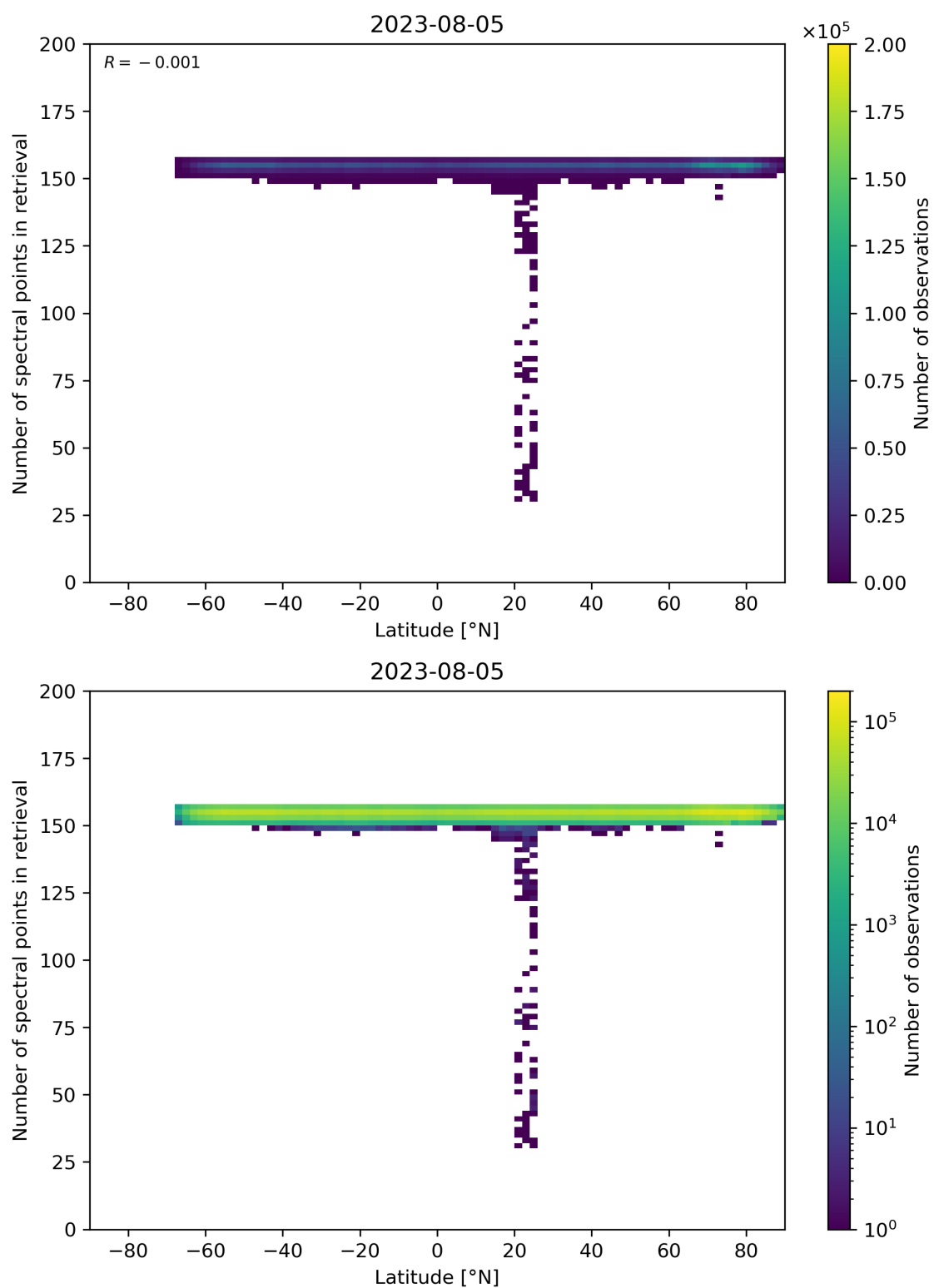
Figure 57: Scatter density plot of “Latitude” against “Number of spectral points in retrieval” for 2023-08-04 to 2023-08-06.
