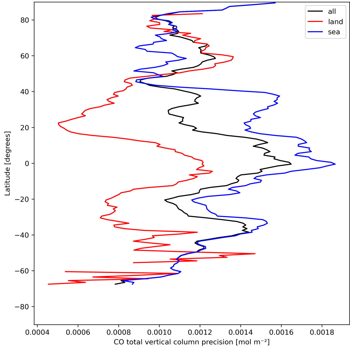
Figure 12: Zonal average of “CO total vertical column precision” for 2023-08-04 to 2023-08-06.
