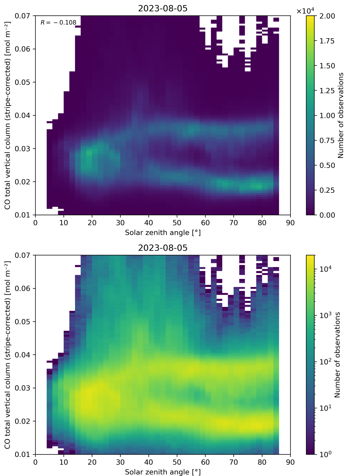
Figure 62: Scatter density plot of “Solar zenith angle” against “CO total vertical column (stripe-corrected)” for 2023-08-04 to 2023-08-06.
