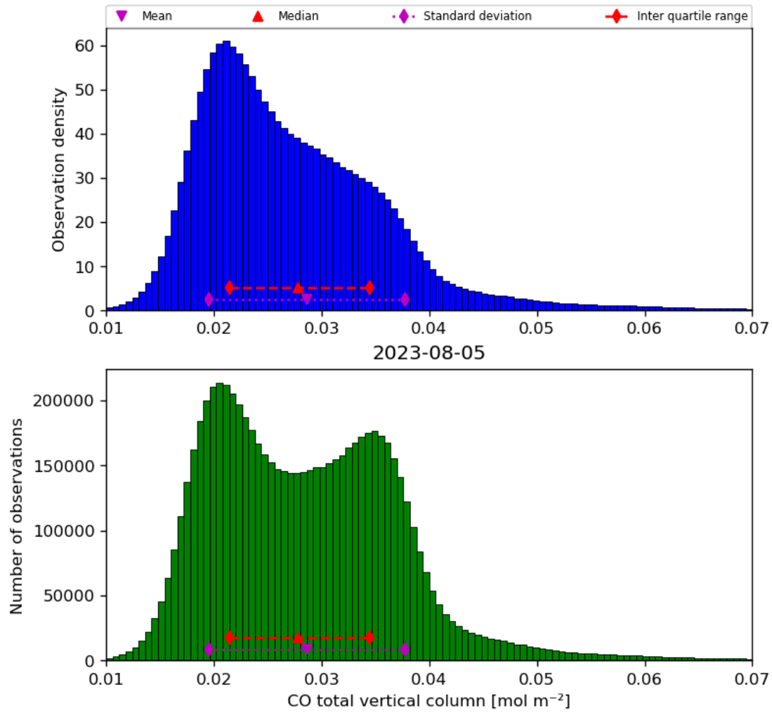
Figure 18: Histogram of “CO total vertical column” for 2023-08-04 to 2023-08-06
