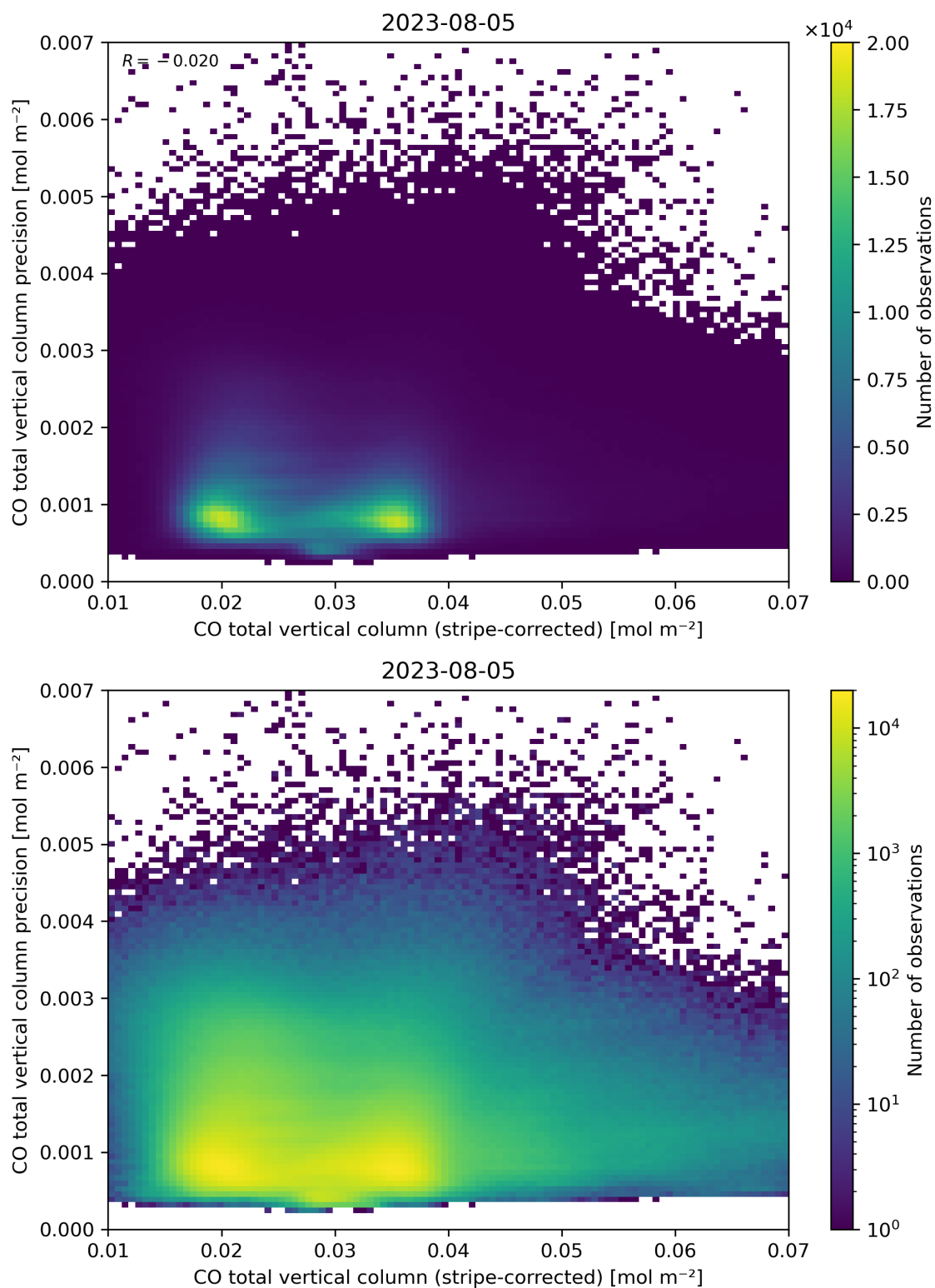
Figure 36: Scatter density plot of “CO total vertical column (stripe-corrected)” against “CO total vertical column precision” for 2023-08-04 to 2023-08-06.
