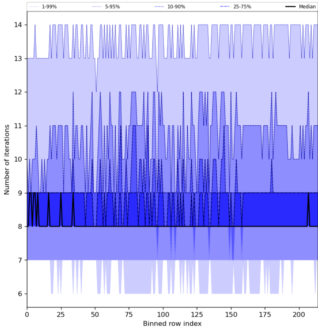
Figure 32: Along track statistics of “Number of iterations” for 2023-08-04 to 2023-08-06
