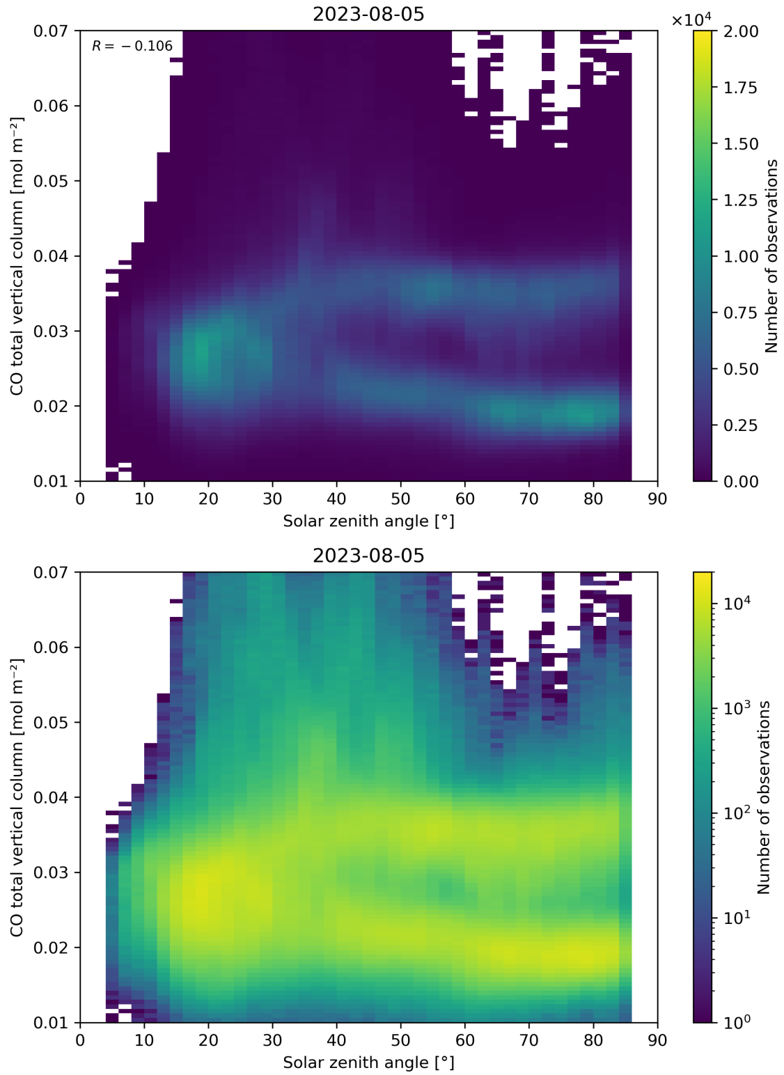
Figure 61: Scatter density plot of “Solar zenith angle” against “CO total vertical column” for 2023-08-04 to 2023-08-06.
