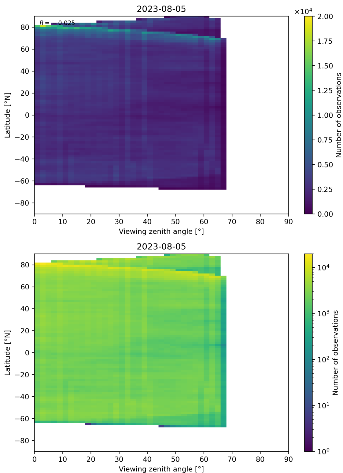
Figure 74: Scatter density plot of “Viewing zenith angle” against “Latitude” for 2023-08-04 to 2023-08-06.
