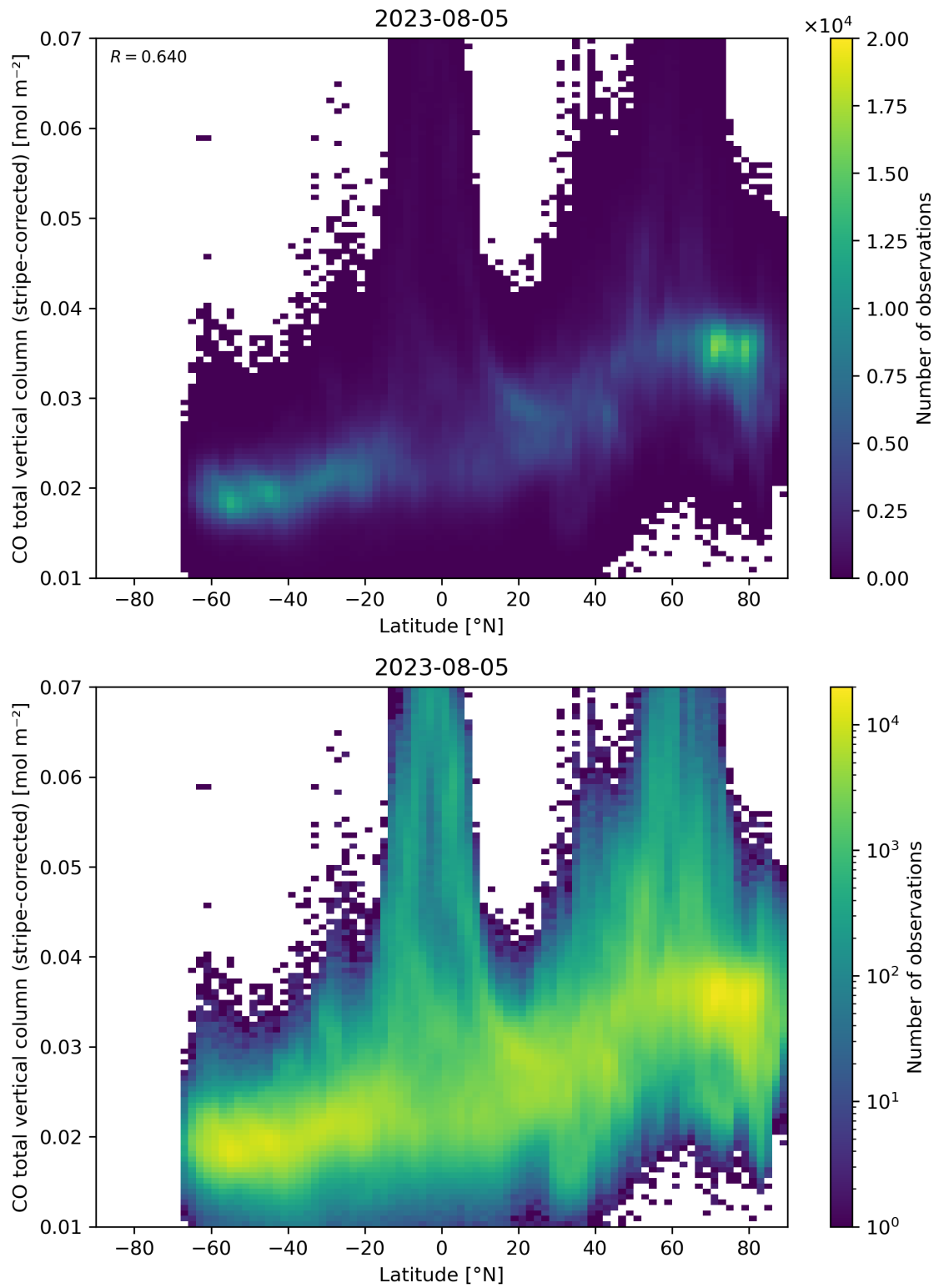
Figure 52: Scatter density plot of “Latitude” against “CO total vertical column (stripe-corrected)” for 2023-08-04 to 2023-08-06.
