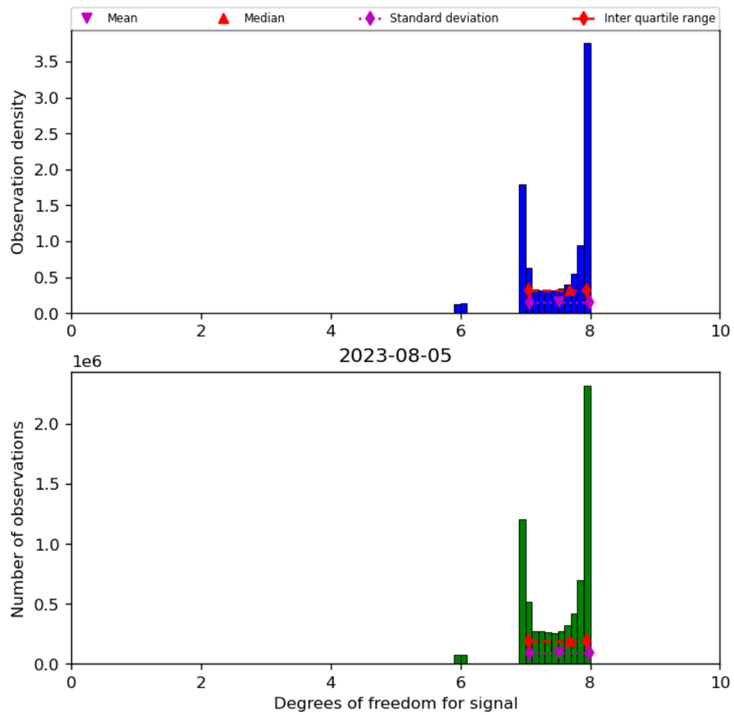
Figure 23: Histogram of “Degrees of freedom for signal” for 2023-08-04 to 2023-08-06
