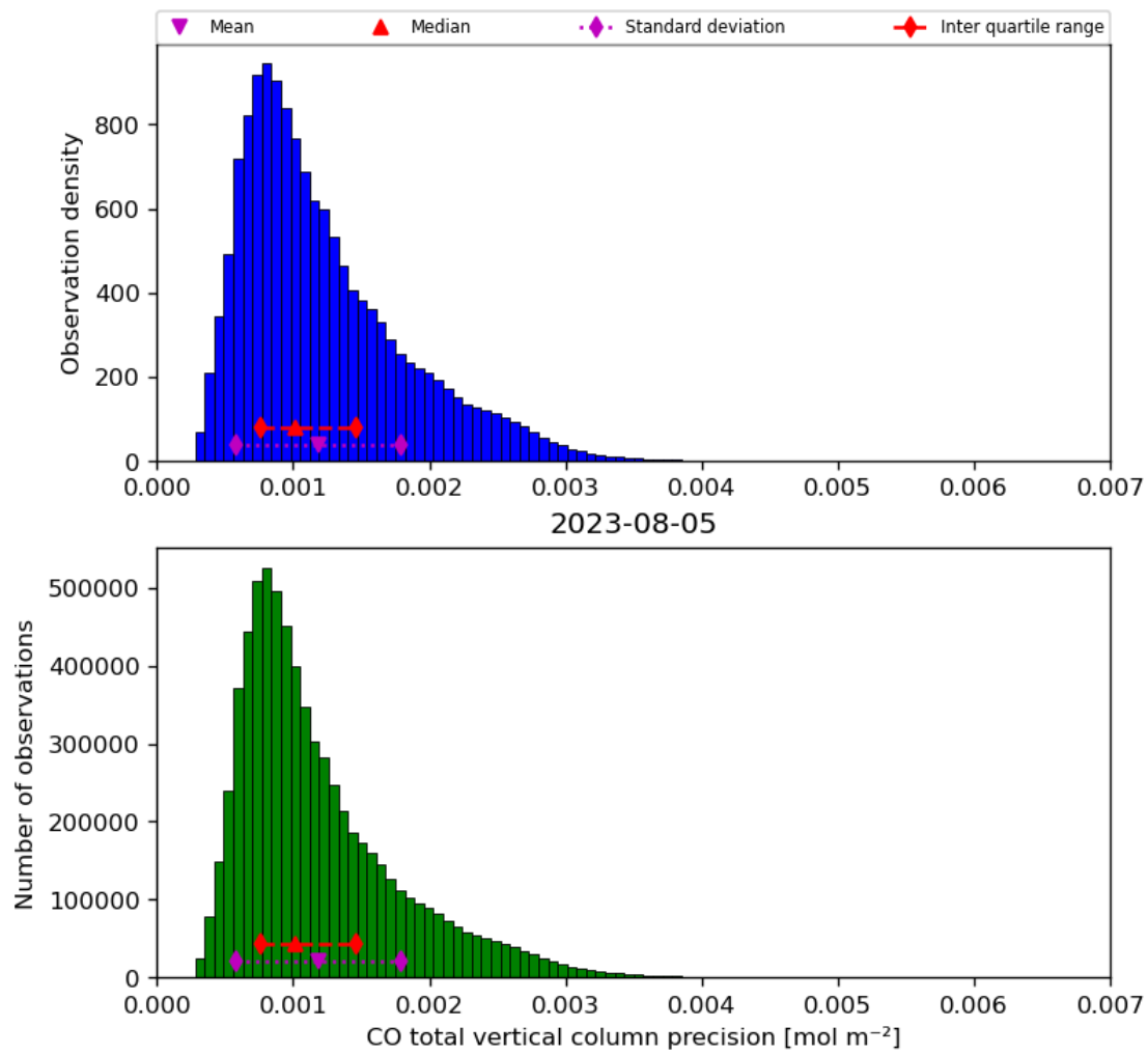
Figure 20: Histogram of “CO total vertical column precision” for 2023-08-04 to 2023-08-06
