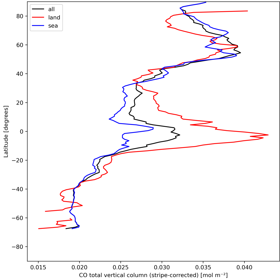
Figure 11: Zonal average of “CO total vertical column (stripe-corrected)” for 2023-08-04 to 2023-08-06.
