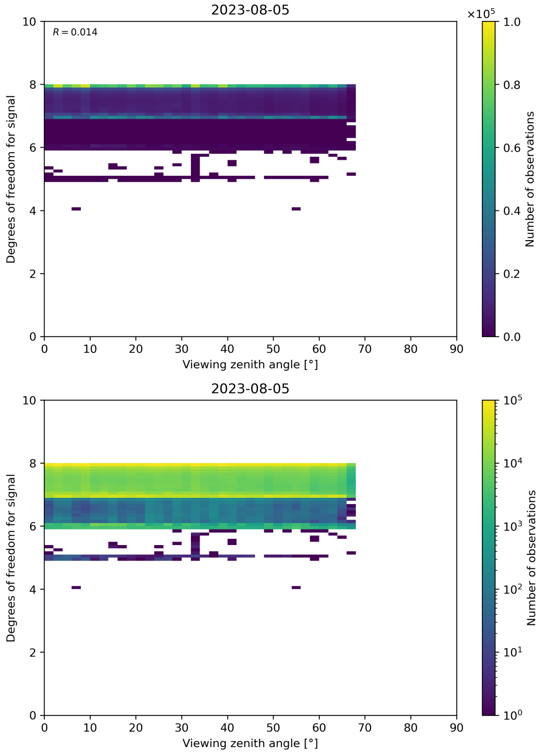
Figure 73: Scatter density plot of “Viewing zenith angle” against “Degrees of freedom for signal” for 2023-08-04 to 2023-08-06.
