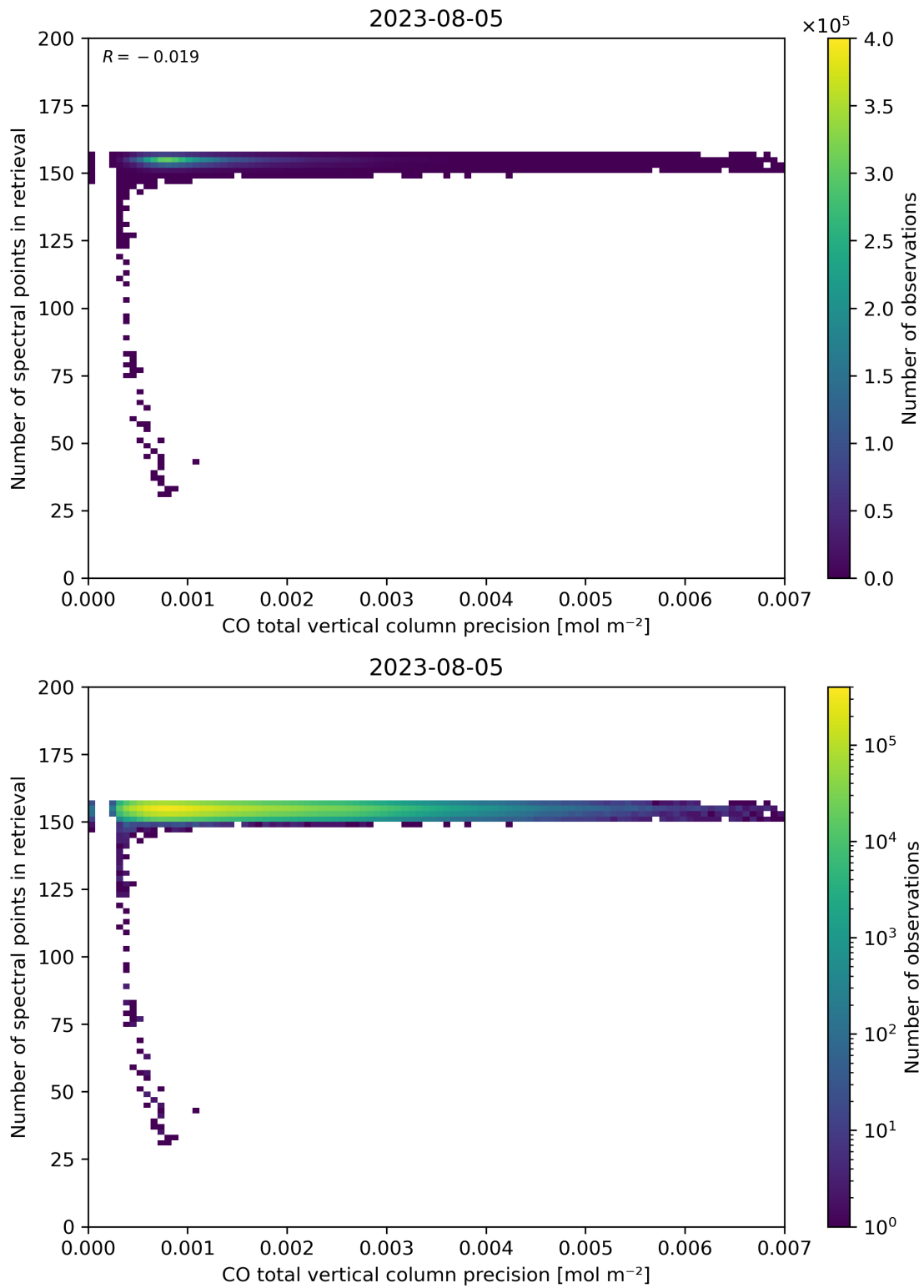
Figure 47: Scatter density plot of “CO total vertical column precision” against “Number of spectral points in retrieval” for 2023-08-04 to 2023-08-06.
