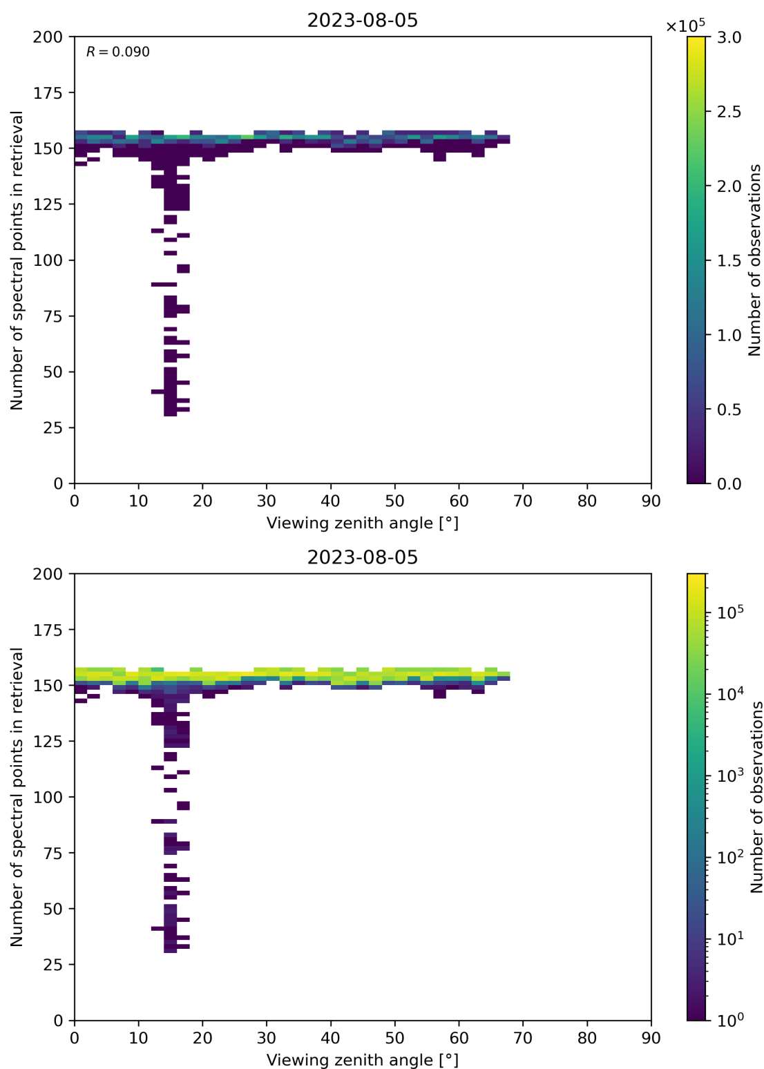
Figure 76: Scatter density plot of “Viewing zenith angle” against “Number of spectral points in retrieval” for 2023-08-04 to 2023-08-06.
