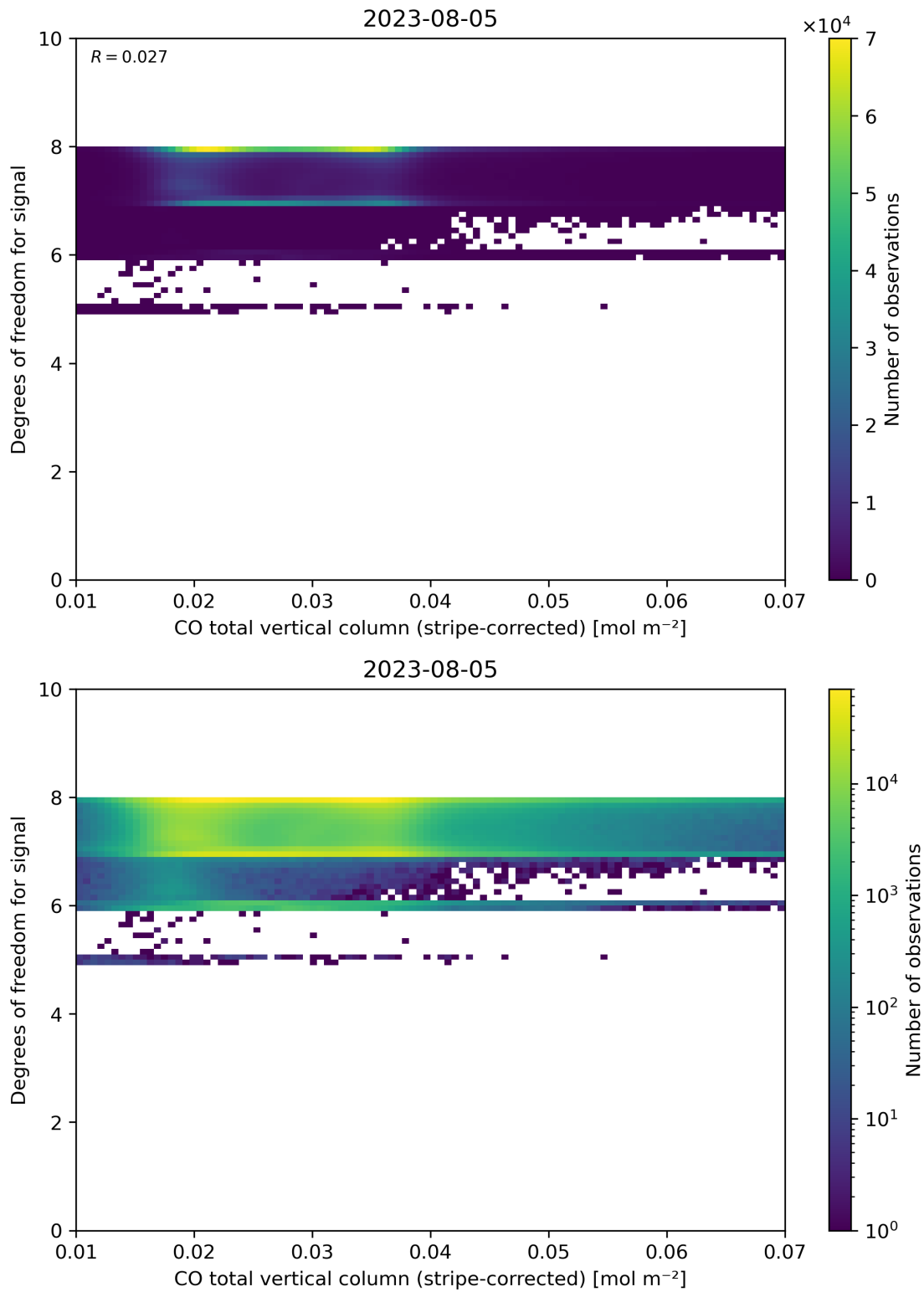
Figure 38: Scatter density plot of “CO total vertical column (stripe-corrected)” against “Degrees of freedom for signal” for 2023-08-04 to 2023-08-06.
