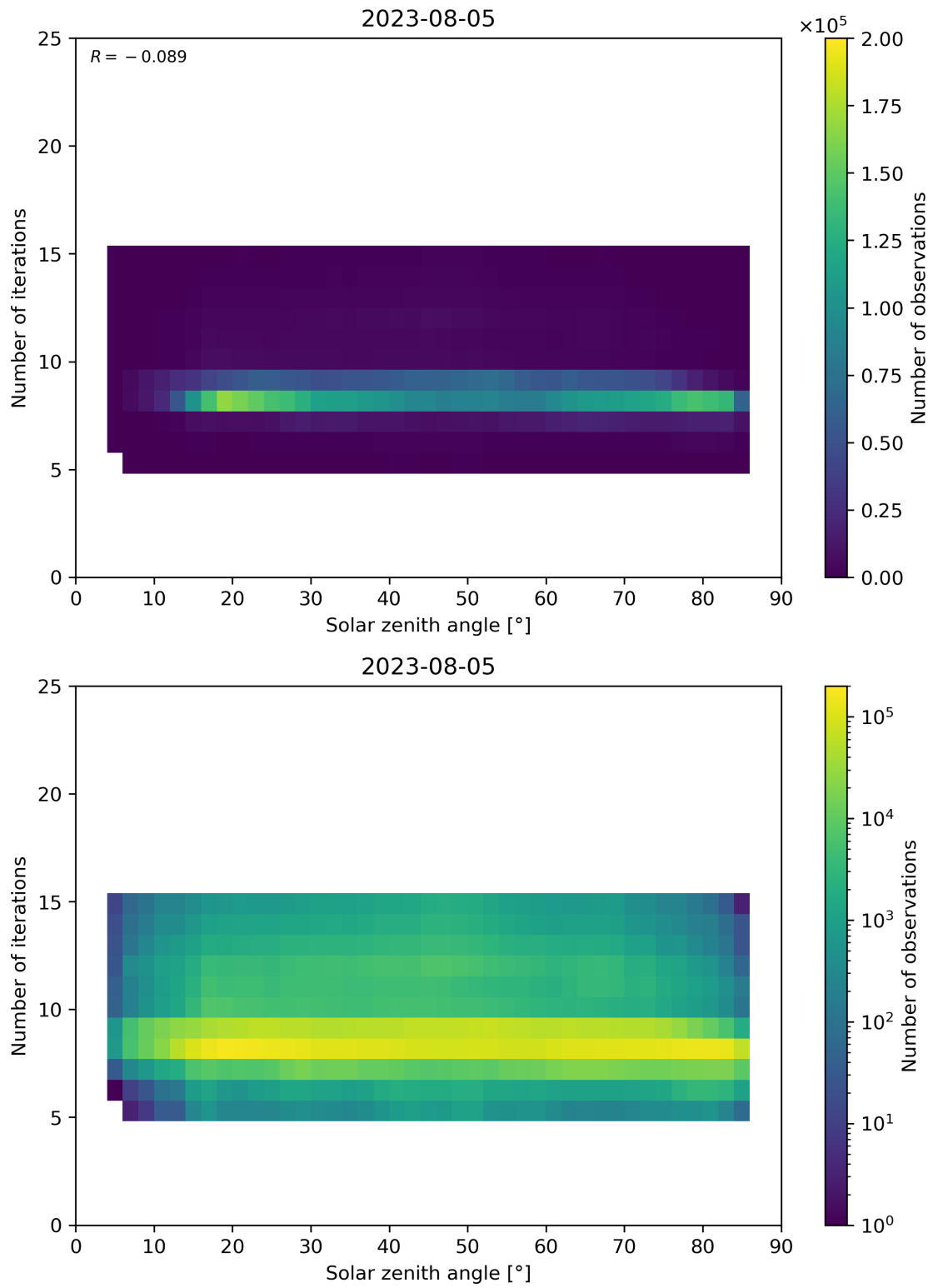
Figure 67: Scatter density plot of “Solar zenith angle” against “Number of iterations” for 2023-08-04 to 2023-08-06.
