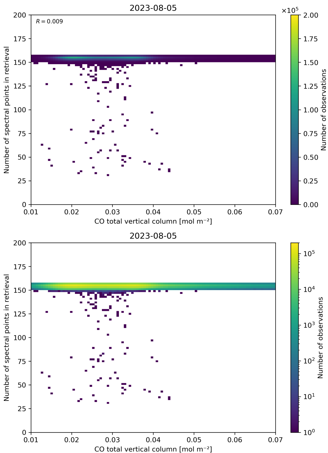
Figure 43: Scatter density plot of “CO total vertical column” against “Number of spectral points in retrieval” for 2023-08-04 to 2023-08-06.
