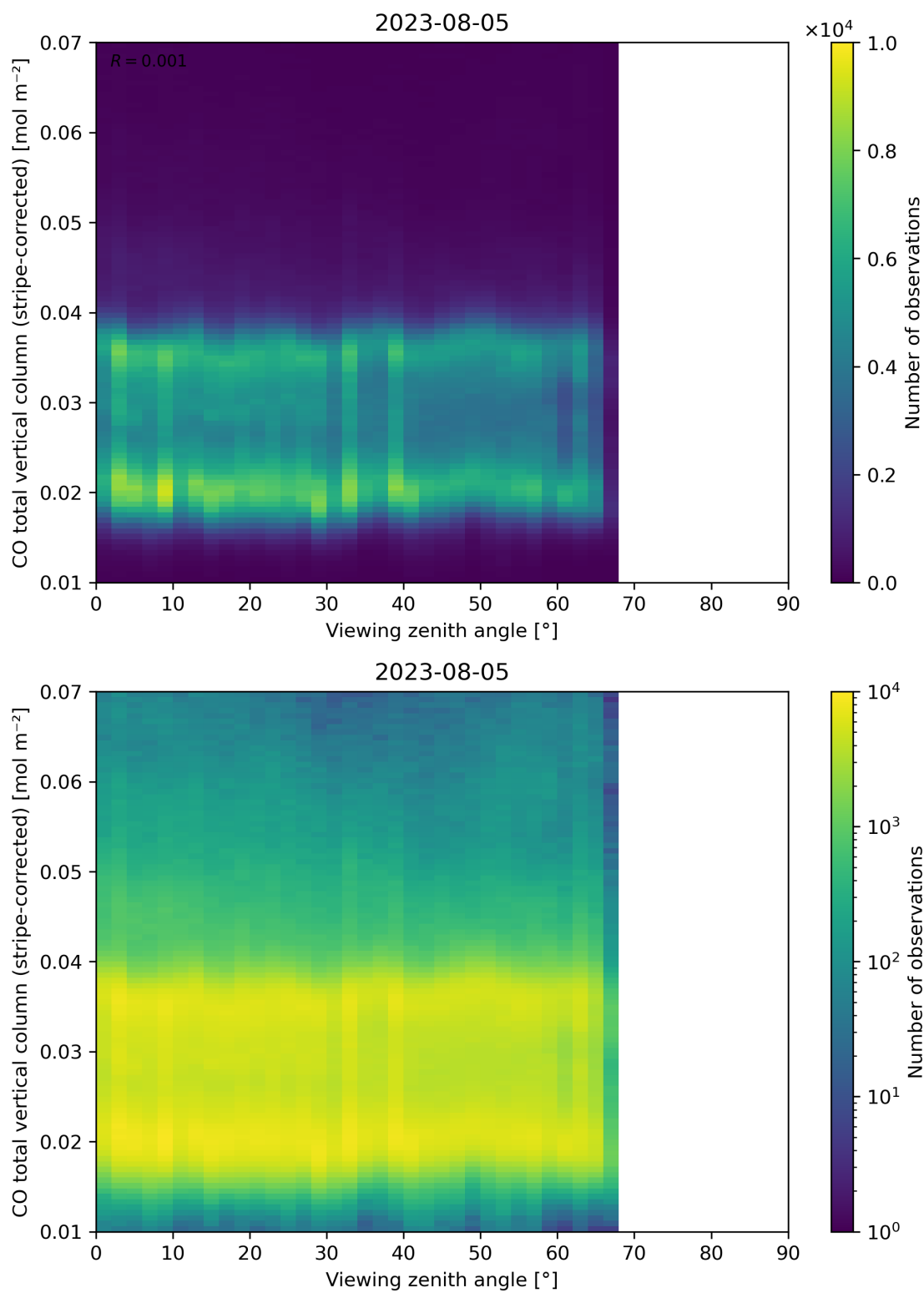
Figure 70: Scatter density plot of “Viewing zenith angle” against “CO total vertical column (stripe-corrected)” for 2023-08-04 to 2023-08-06.
