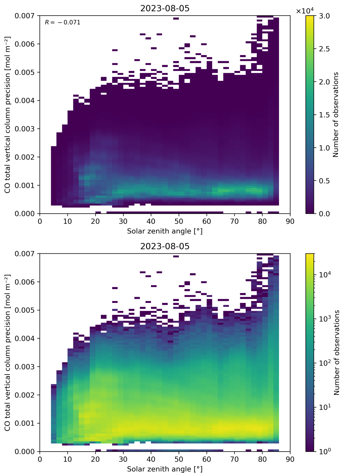
Figure 63: Scatter density plot of “Solar zenith angle” against “CO total vertical column precision” for 2023-08-04 to 2023-08-06.
