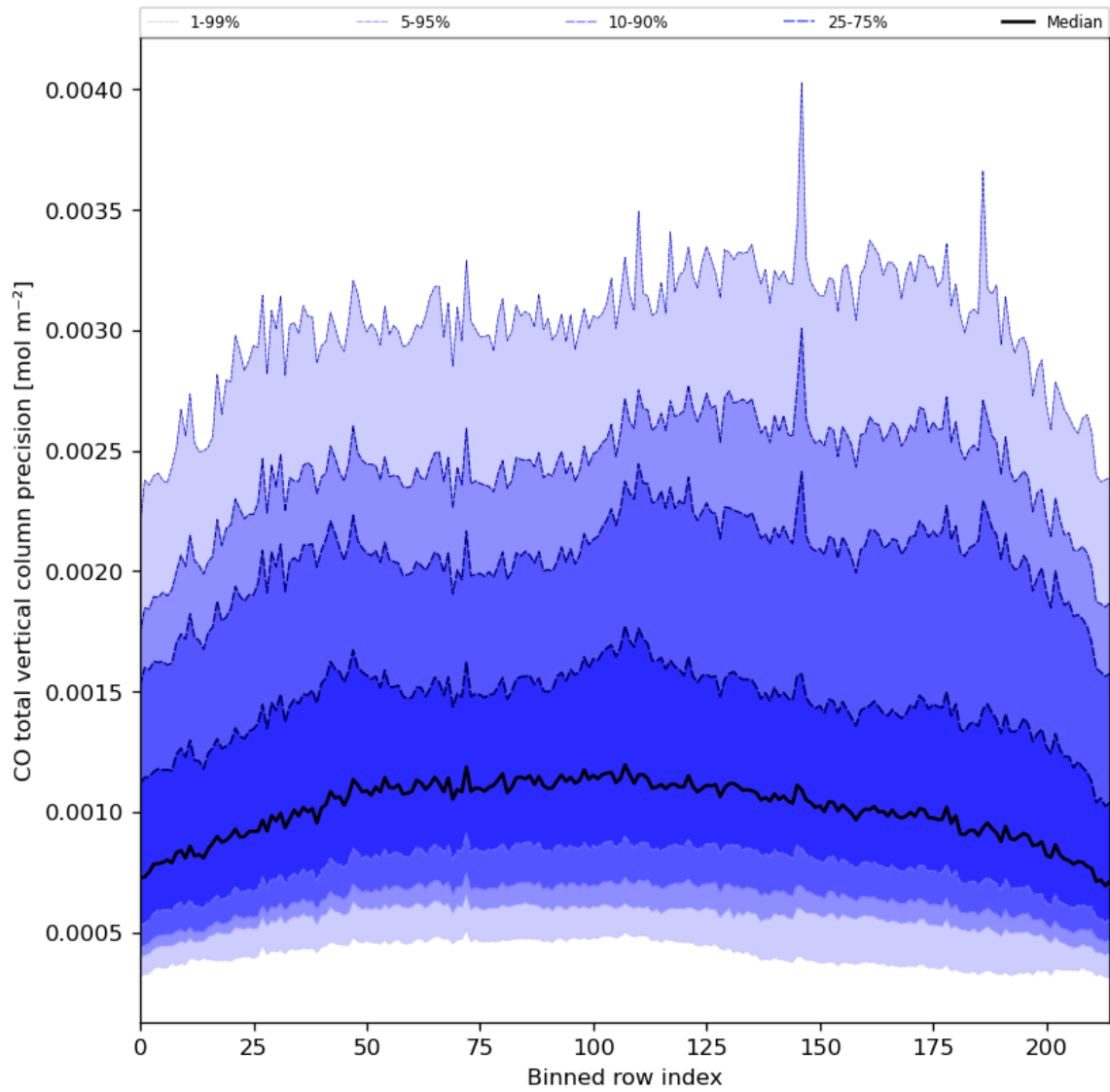
Figure 28: Along track statistics of “CO total vertical column precision” for 2023-08-04 to 2023-08-06
