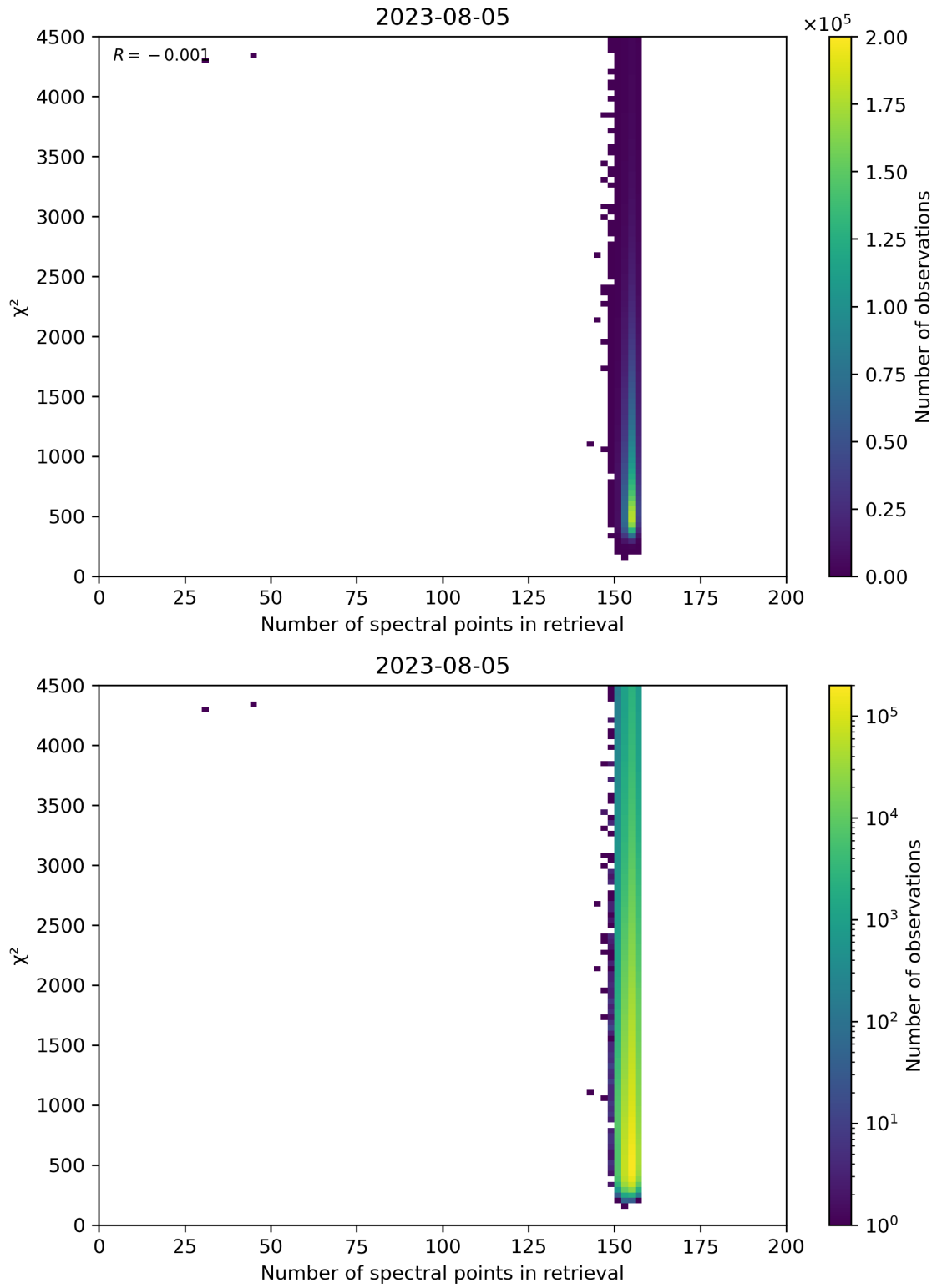
Figure 58: Scatter density plot of “Number of spectral points in retrieval” against “ \chi^2 ” for 2023-08-04 to 2023-08-06.
