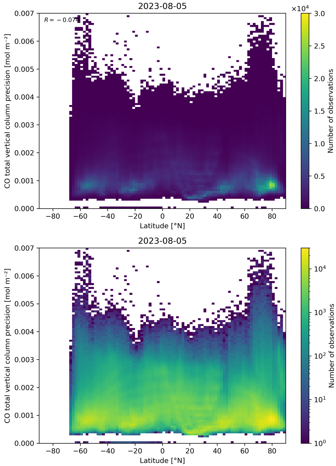
Figure 53: Scatter density plot of “Latitude” against “CO total vertical column precision” for 2023-08-04 to 2023-08-06.
