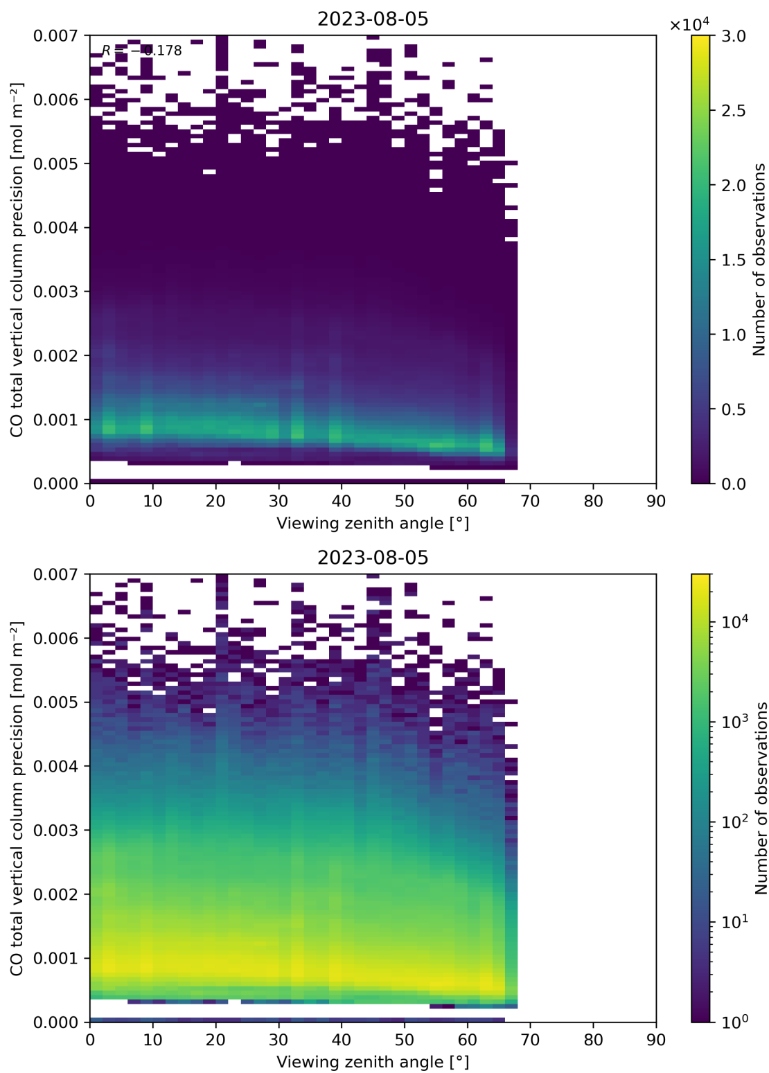
Figure 71: Scatter density plot of “Viewing zenith angle” against “CO total vertical column precision” for 2023-08-04 to 2023-08-06.
