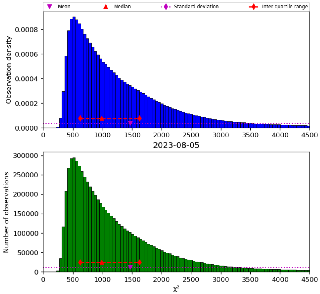
Figure 22: Histogram of “ \chi^2 ” for 2023-08-04 to 2023-08-06
