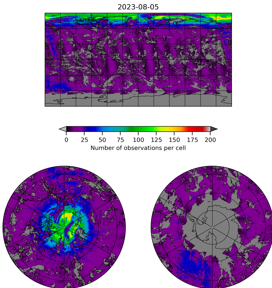
Figure 8: Map of the number of observations for 2023-08-04 to 2023-08-06
