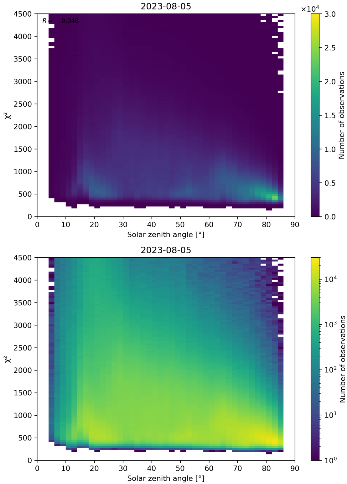
Figure 64: Scatter density plot of “Solar zenith angle” against “ \chi^2 ” for 2023-08-04 to 2023-08-06.
