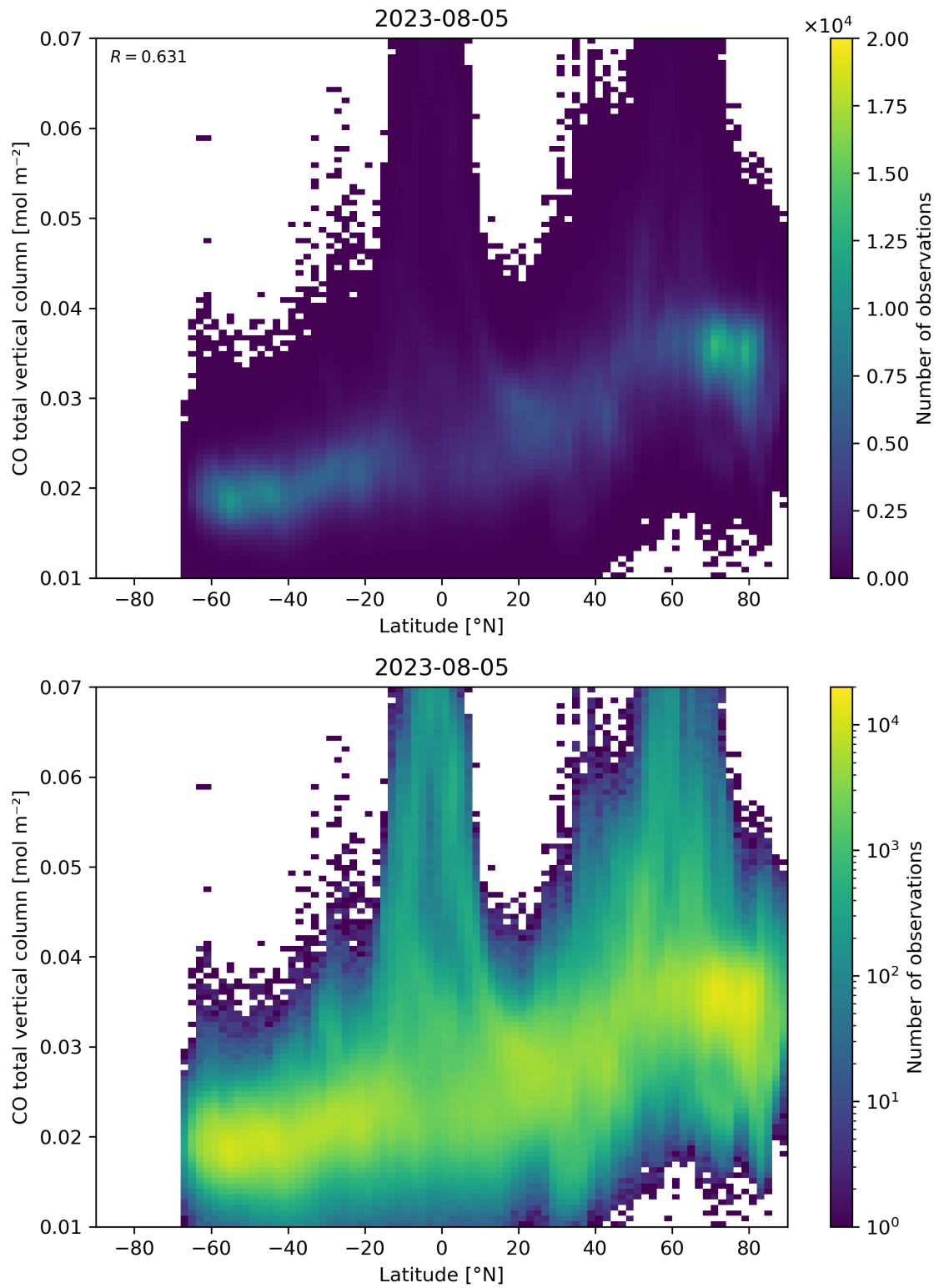
Figure 51: Scatter density plot of “Latitude” against “CO total vertical column” for 2023-08-04 to 2023-08-06.
