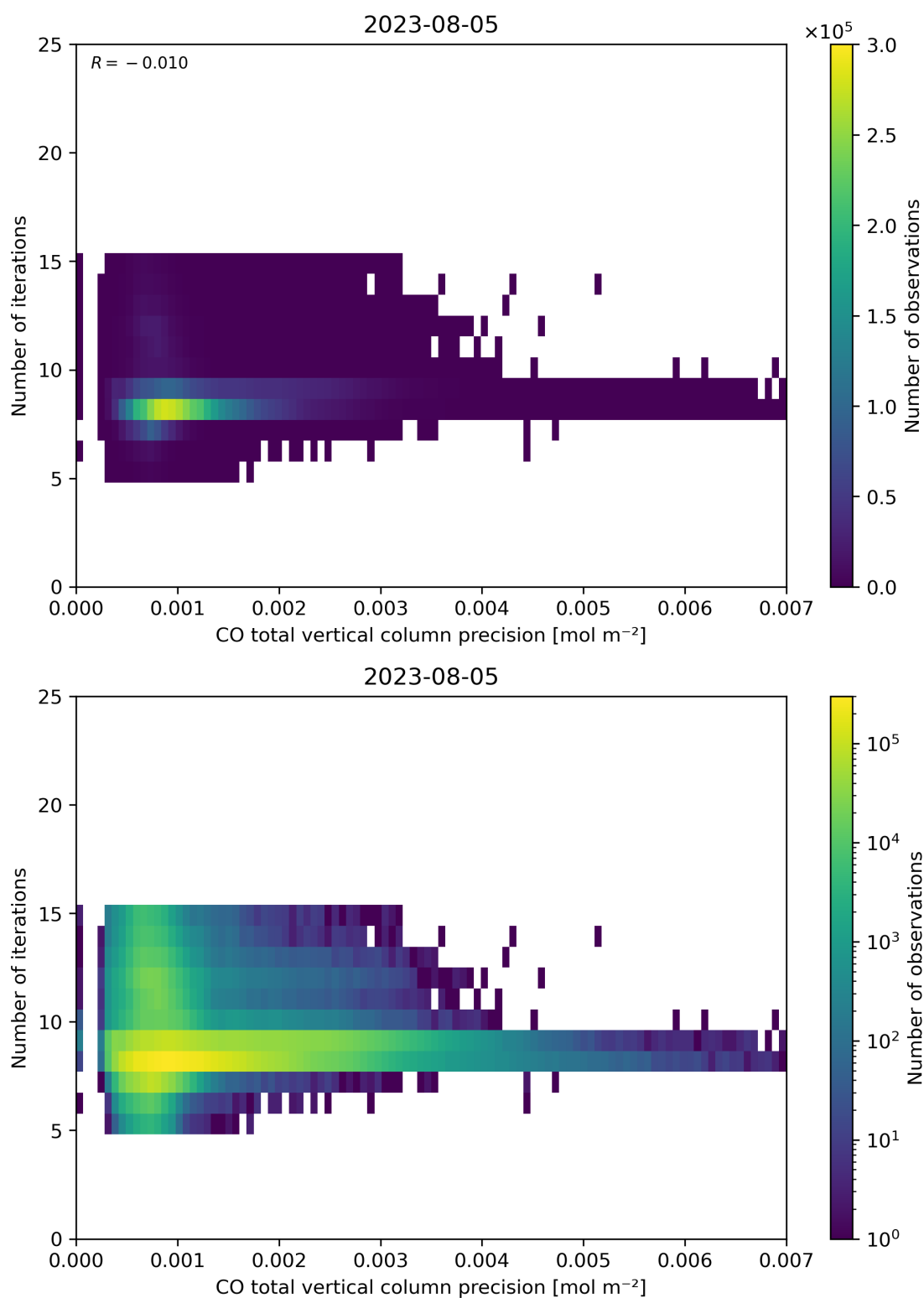
Figure 46: Scatter density plot of “CO total vertical column precision” against “Number of iterations” for 2023-08-04 to 2023-08-06.
