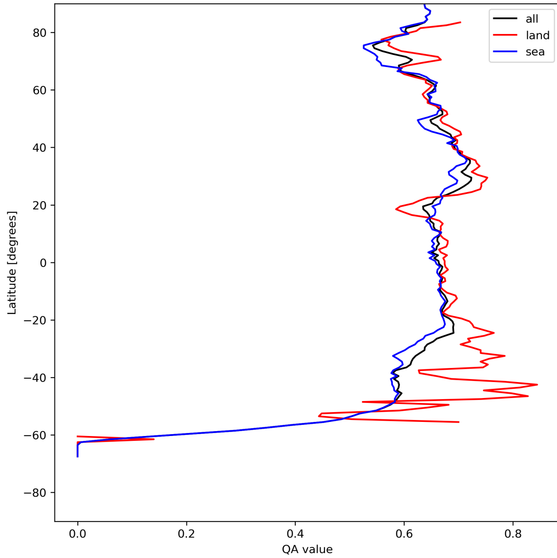
Figure 9: Zonal average of “QA value” for 2023-08-04 to 2023-08-06.
