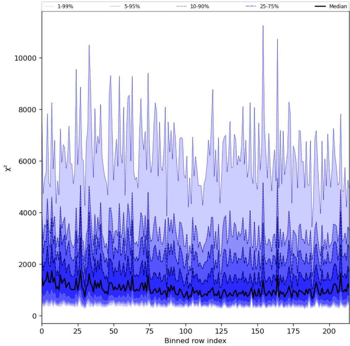
Figure 30: Along track statistics of “ \chi^2 ” for 2023-08-04 to 2023-08-06
