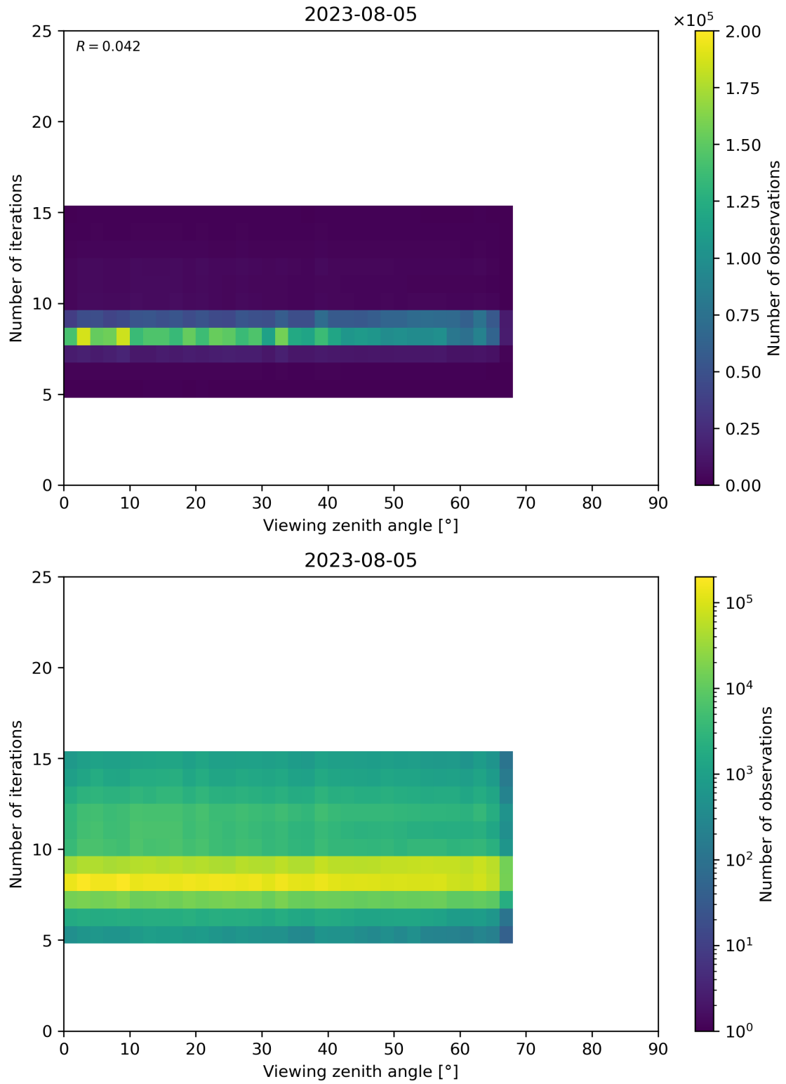
Figure 75: Scatter density plot of “Viewing zenith angle” against “Number of iterations” for 2023-08-04 to 2023-08-06.
