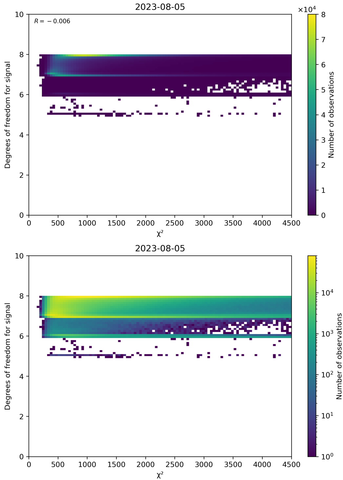
Figure 48: Scatter density plot of “ \chi^2 ” against “Degrees of freedom for signal” for 2023-08-04 to 2023-08-06.
