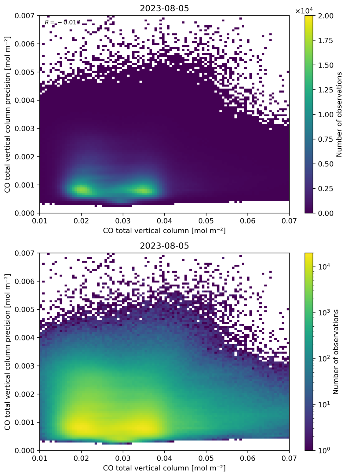
Figure 34: Scatter density plot of “CO total vertical column” against “CO total vertical column precision” for 2023-08-04 to 2023-08-06.
