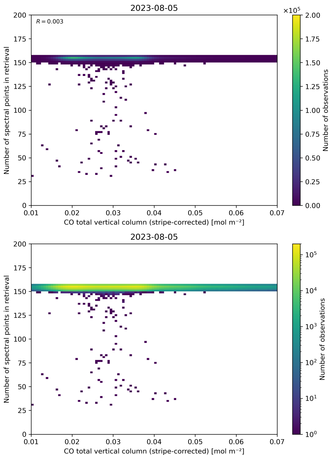
Figure 40: Scatter density plot of “CO total vertical column (stripe-corrected)” against “Number of spectral points in retrieval” for 2023-08-04 to 2023-08-06.
