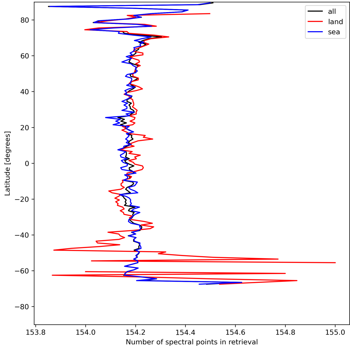
Figure 13: Zonal average of “Number of spectral points in retrieval” for 2023-08-04 to 2023-08-06.
