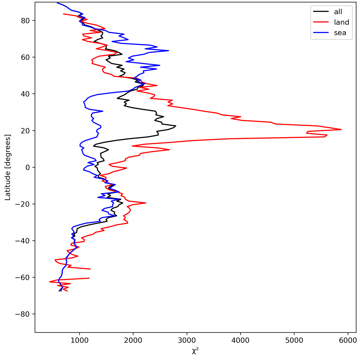
Figure 14: Zonal average of “ \chi^2 ” for 2023-08-04 to 2023-08-06.
