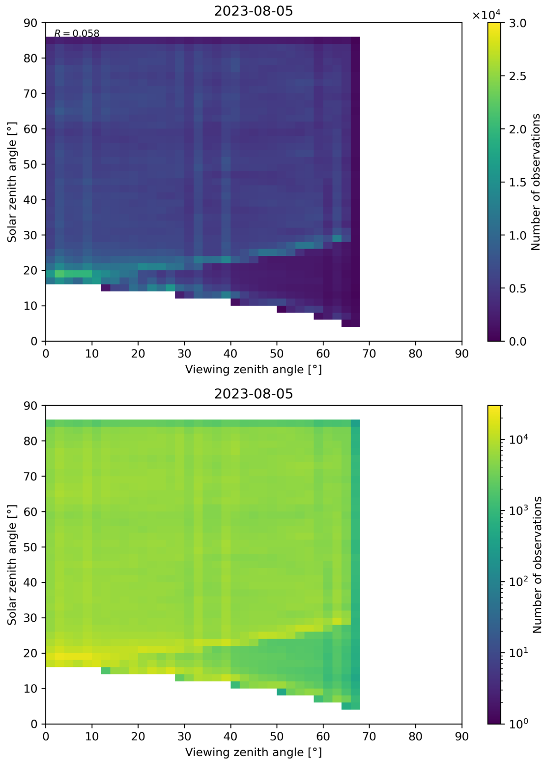
Figure 77: Scatter density plot of “Viewing zenith angle” against “Solar zenith angle” for 2023-08-04 to 2023-08-06.
