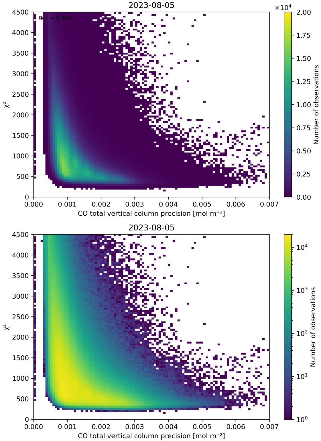
Figure 44: Scatter density plot of “CO total vertical column precision” against “ \chi^2 ” for 2023-08-04 to 2023-08-06.
