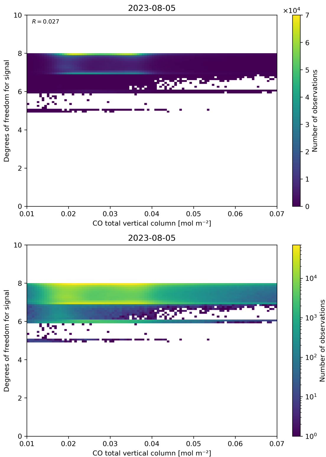
Figure 41: Scatter density plot of “CO total vertical column” against “Degrees of freedom for signal” for 2023-08-04 to 2023-08-06.
