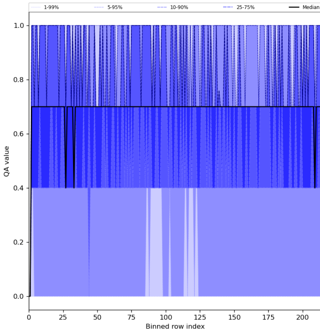
Figure 25: Along track statistics of “QA value” for 2023-08-04 to 2023-08-06
