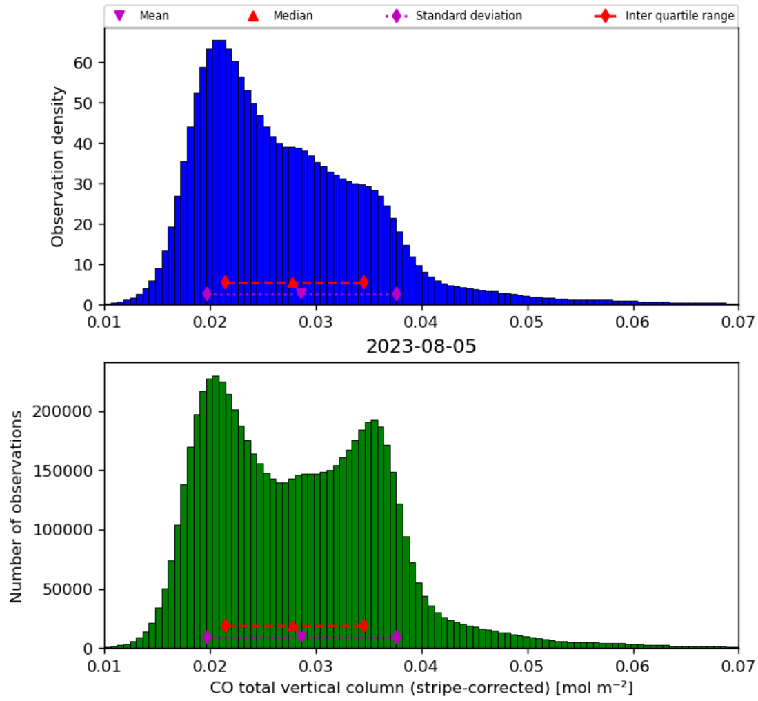
Figure 19: Histogram of “CO total vertical column (stripe-corrected)” for 2023-08-04 to 2023-08-06
