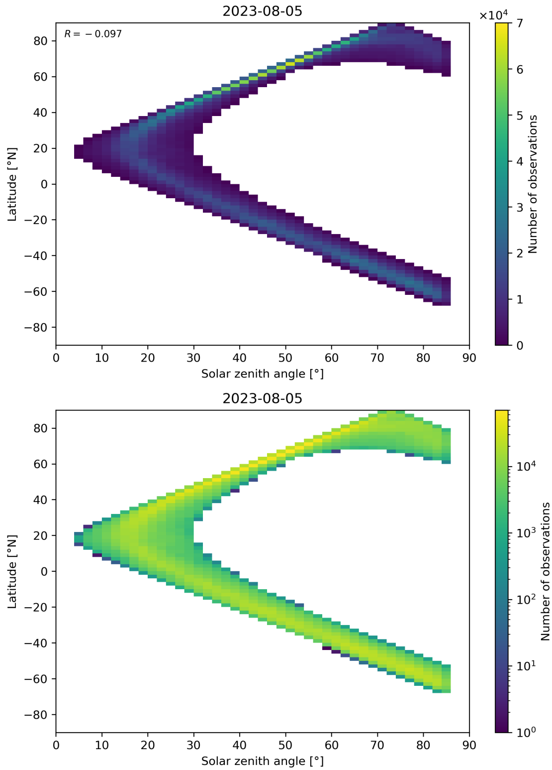
Figure 66: Scatter density plot of “Solar zenith angle” against “Latitude” for 2023-08-04 to 2023-08-06.
