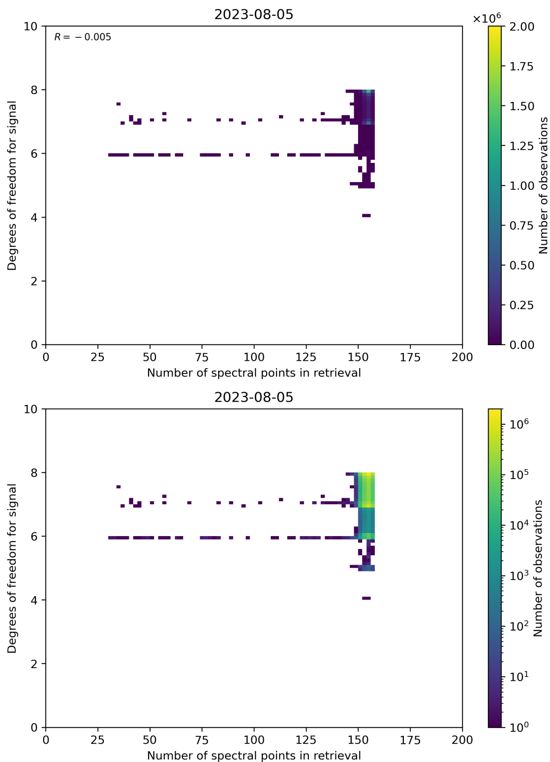
Figure 59: Scatter density plot of “Number of spectral points in retrieval” against “Degrees of freedom for signal” for 2023-08-04 to 2023-08-06.
