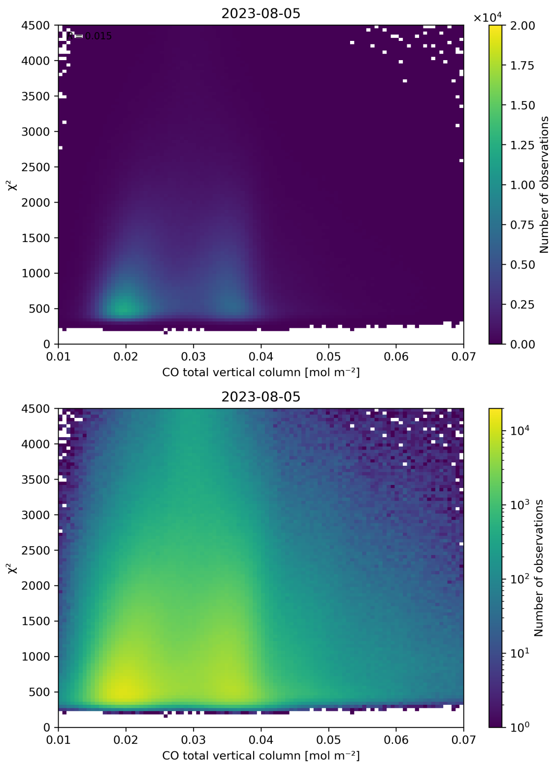
Figure 35: Scatter density plot of “CO total vertical column” against “ \chi^2 ” for 2023-08-04 to 2023-08-06.
