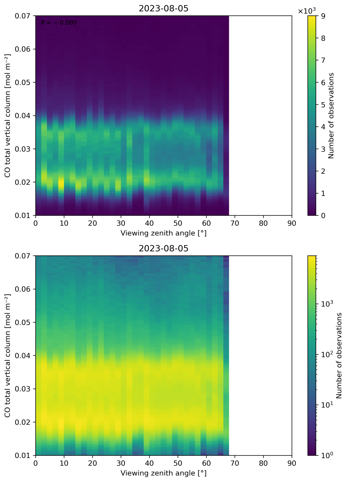
Figure 69: Scatter density plot of “Viewing zenith angle” against “CO total vertical column” for 2023-08-04 to 2023-08-06.
