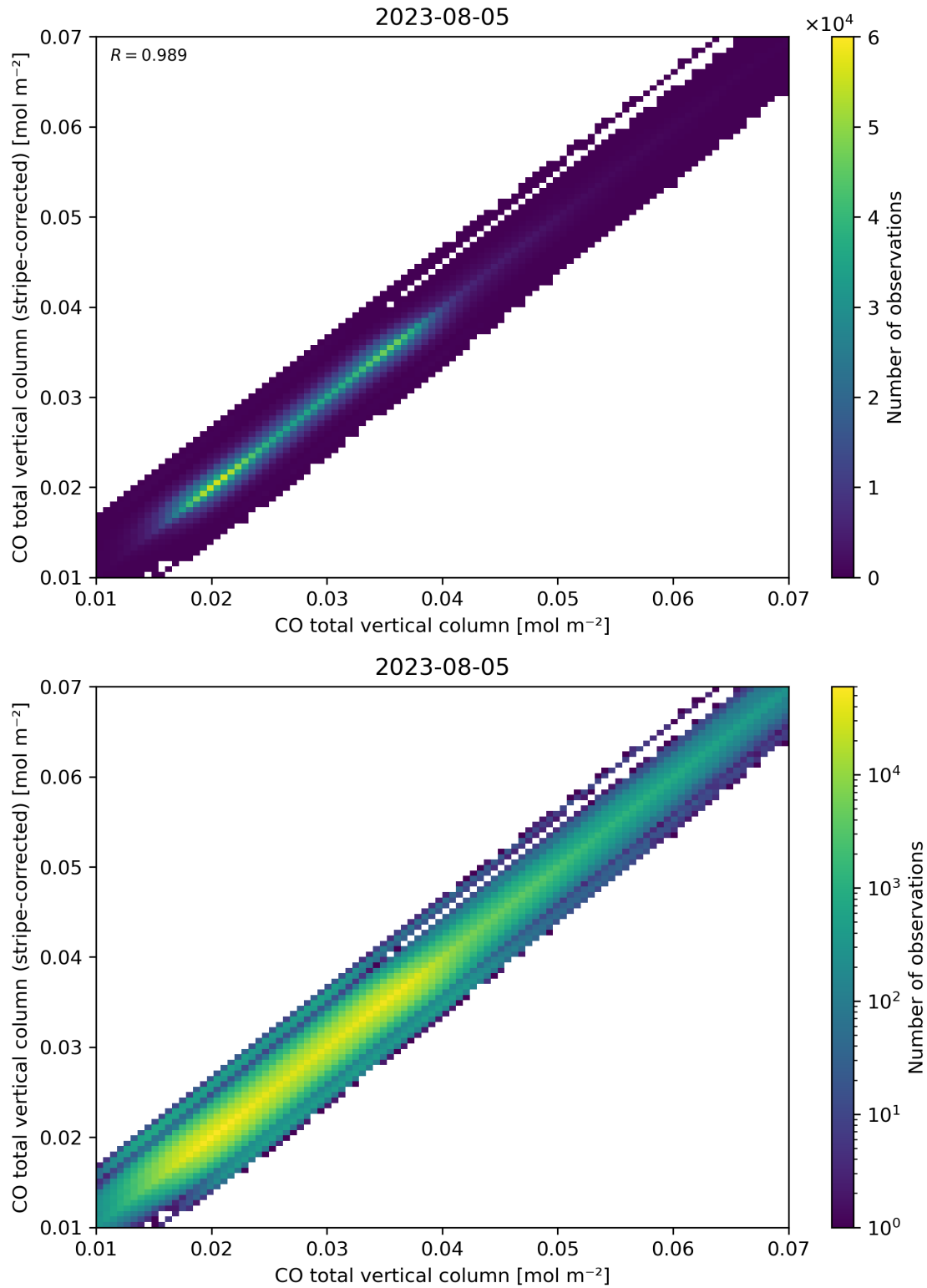
Figure 33: Scatter density plot of “CO total vertical column” against “CO total vertical column (stripe-corrected)” for 2023-08-04 to 2023-08-06.
