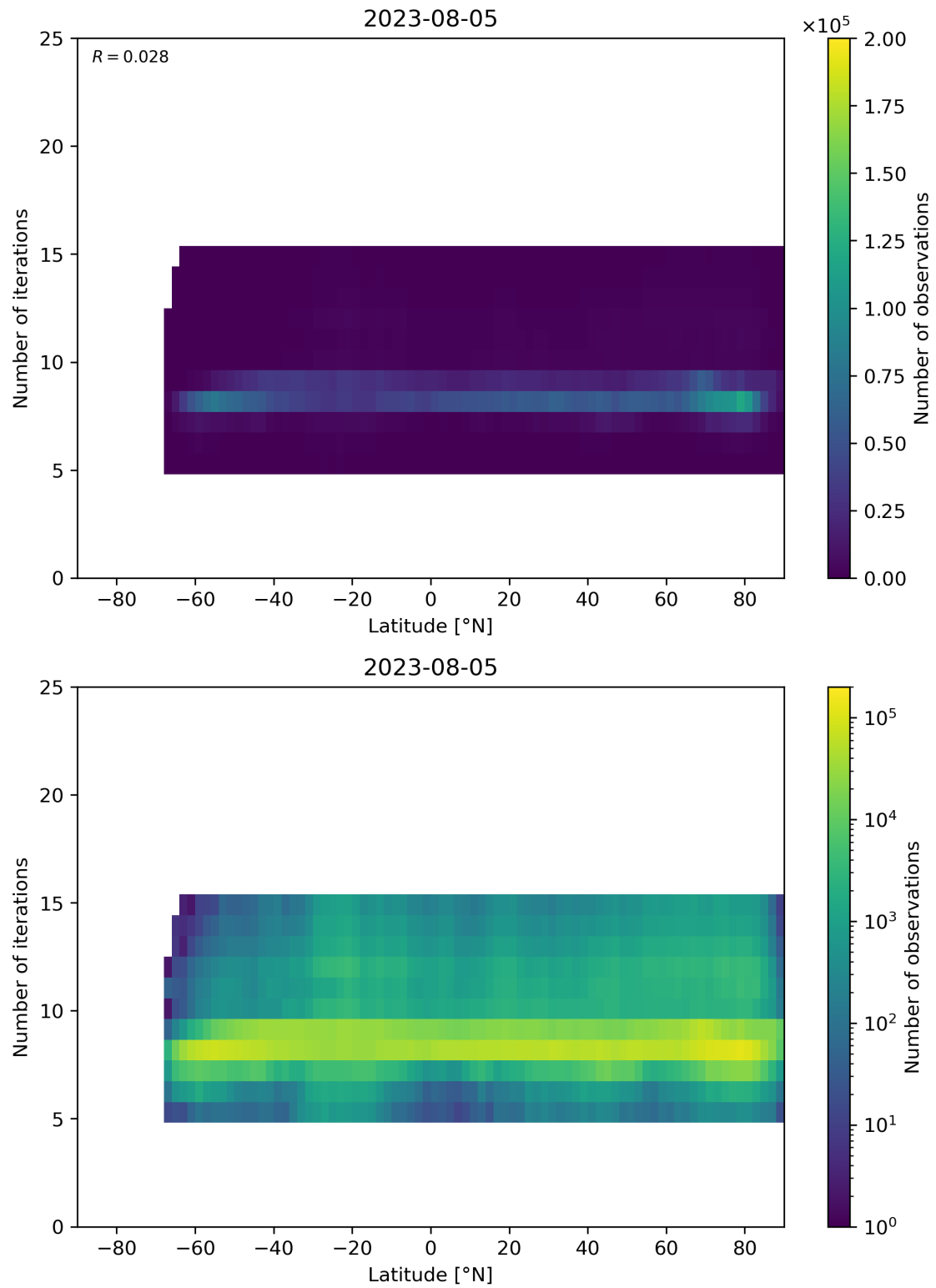
Figure 56: Scatter density plot of “Latitude” against “Number of iterations” for 2023-08-04 to 2023-08-06.
