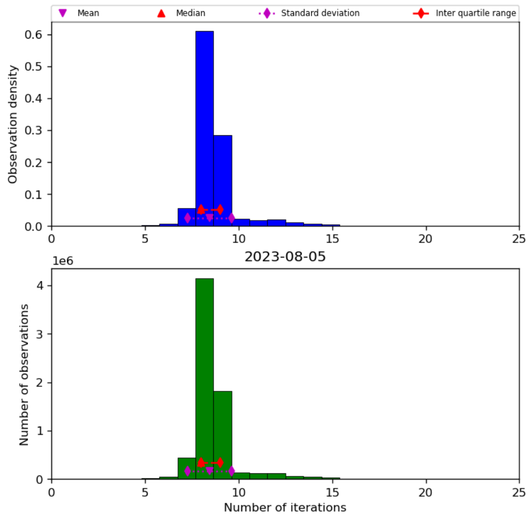
Figure 24: Histogram of “Number of iterations” for 2023-08-04 to 2023-08-06
