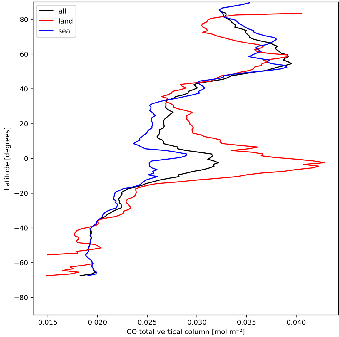
Figure 10: Zonal average of “CO total vertical column” for 2023-08-04 to 2023-08-06.
