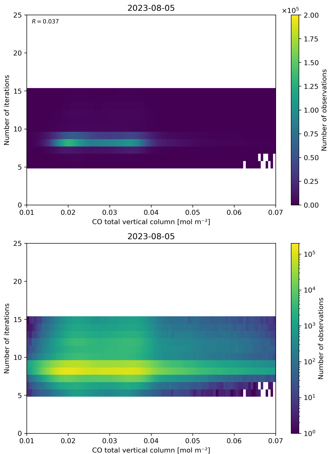
Figure 42: Scatter density plot of “CO total vertical column” against “Number of iterations” for 2023-08-04 to 2023-08-06.
