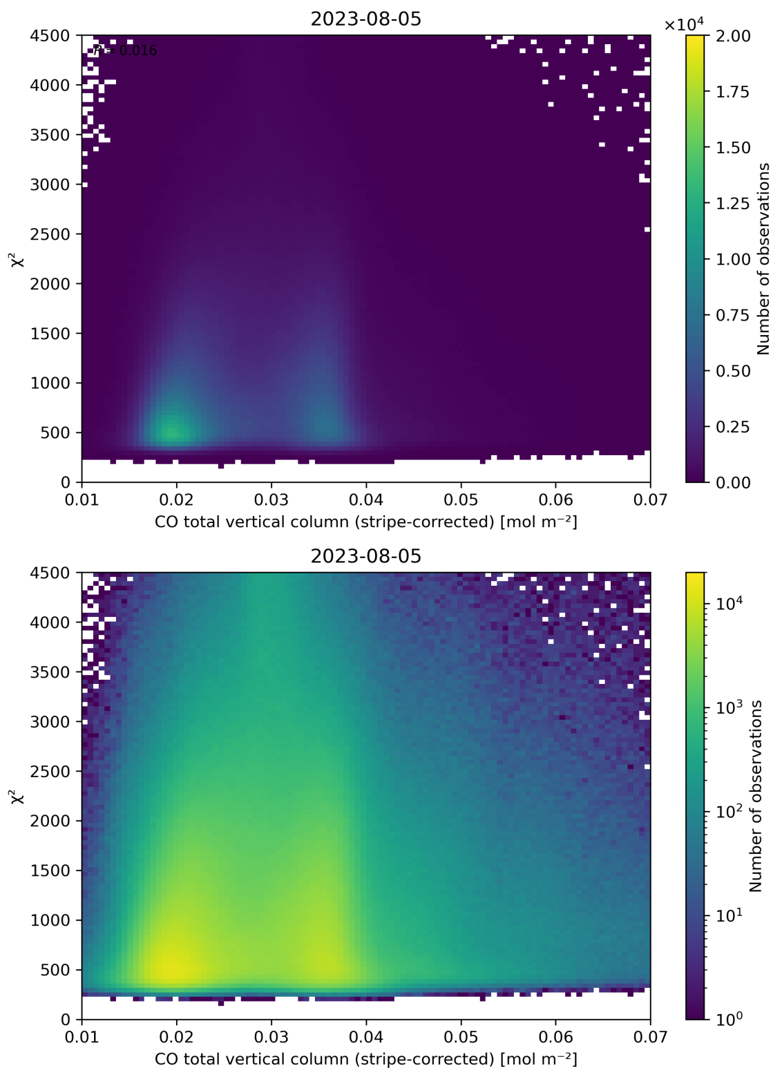
Figure 37: Scatter density plot of “CO total vertical column (stripe-corrected)” against “ \chi^2 ” for 2023-08-04 to 2023-08-06.
