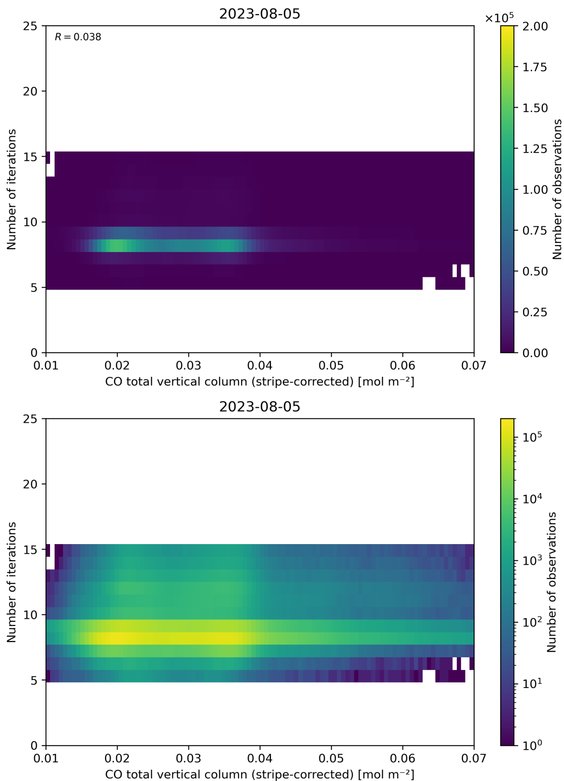
Figure 39: Scatter density plot of “CO total vertical column (stripe-corrected)” against “Number of iterations” for 2023-08-04 to 2023-08-06.
