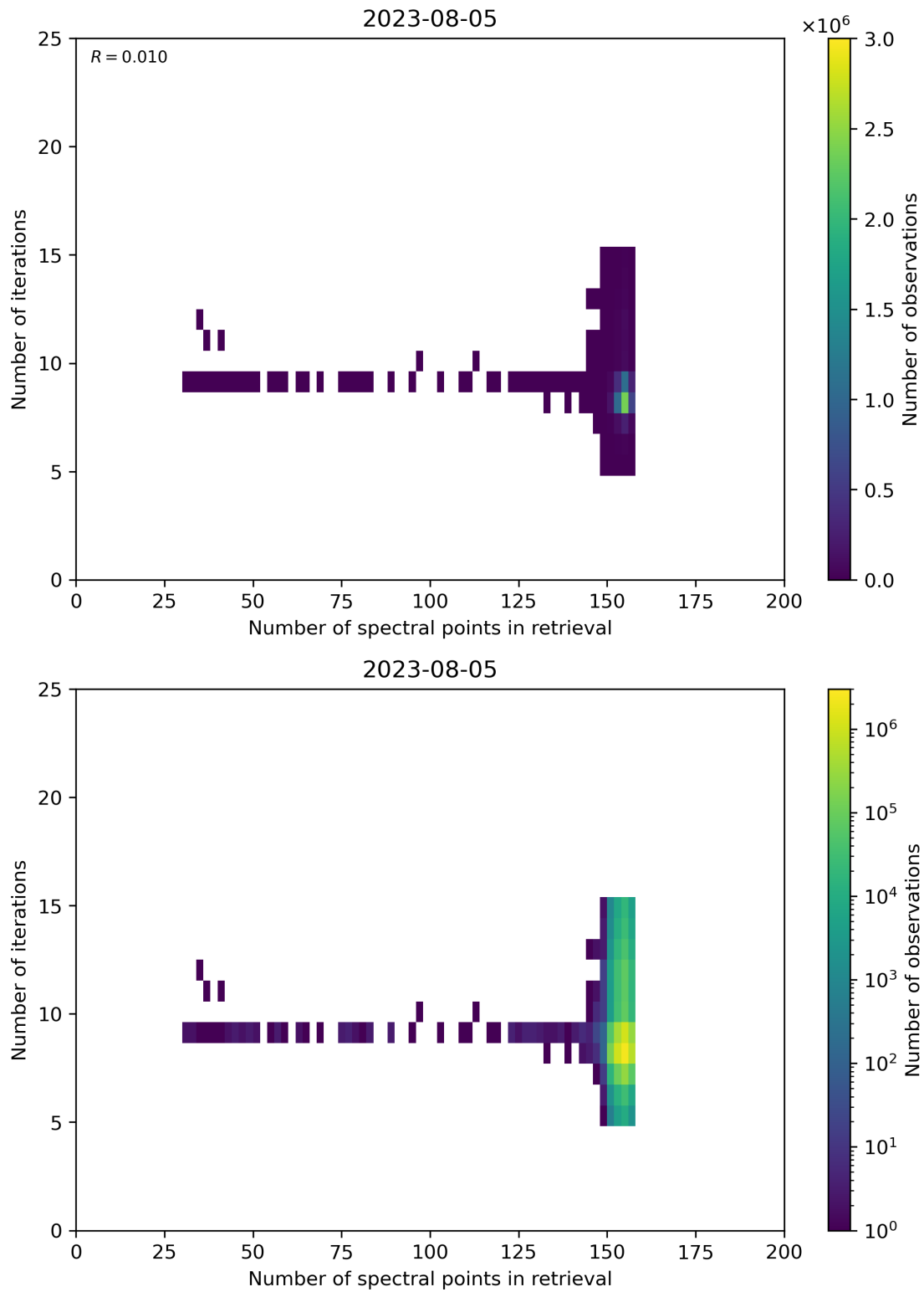
Figure 60: Scatter density plot of “Number of spectral points in retrieval” against “Number of iterations” for 2023-08-04 to 2023-08-06.
