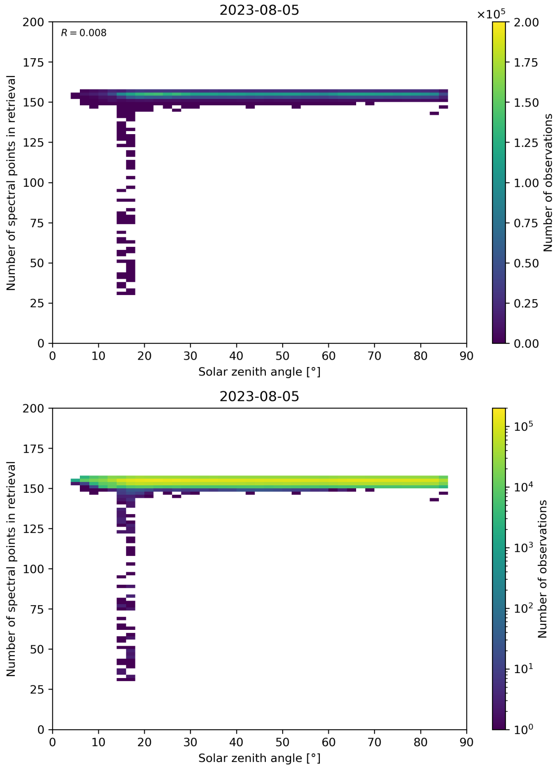
Figure 68: Scatter density plot of “Solar zenith angle” against “Number of spectral points in retrieval” for 2023-08-04 to 2023-08-06.
