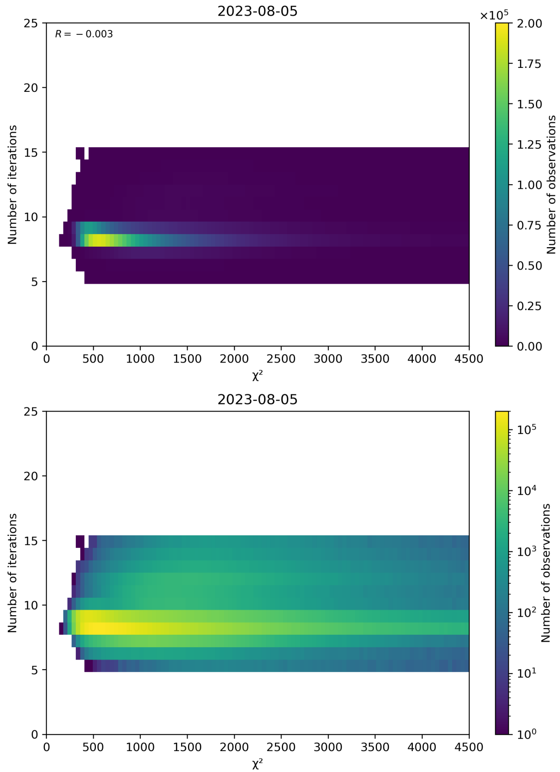
Figure 49: Scatter density plot of “ \chi^2 ” against “Number of iterations” for 2023-08-04 to 2023-08-06.
