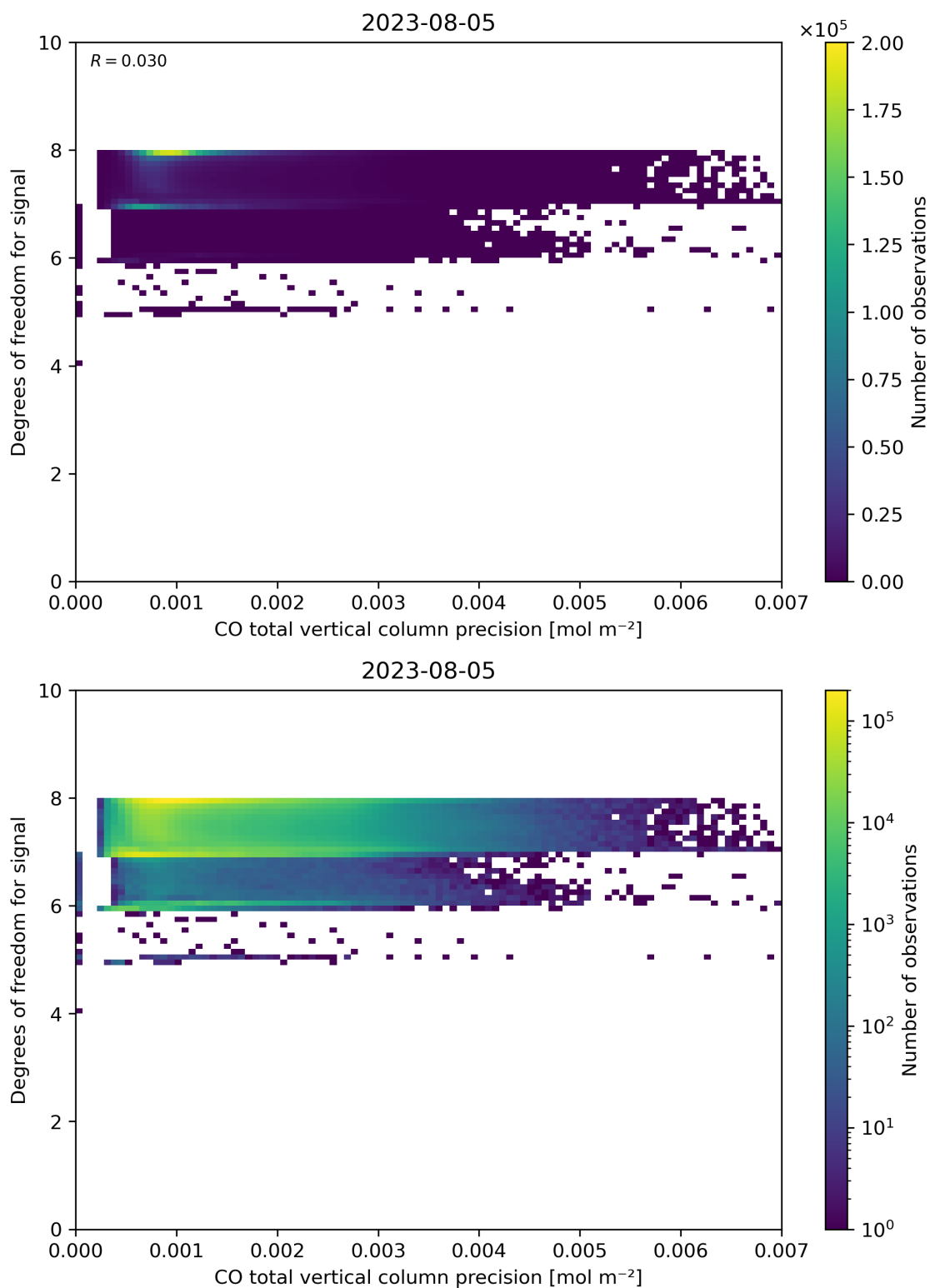
Figure 45: Scatter density plot of “CO total vertical column precision” against “Degrees of freedom for signal” for 2023-08-04 to 2023-08-06.
