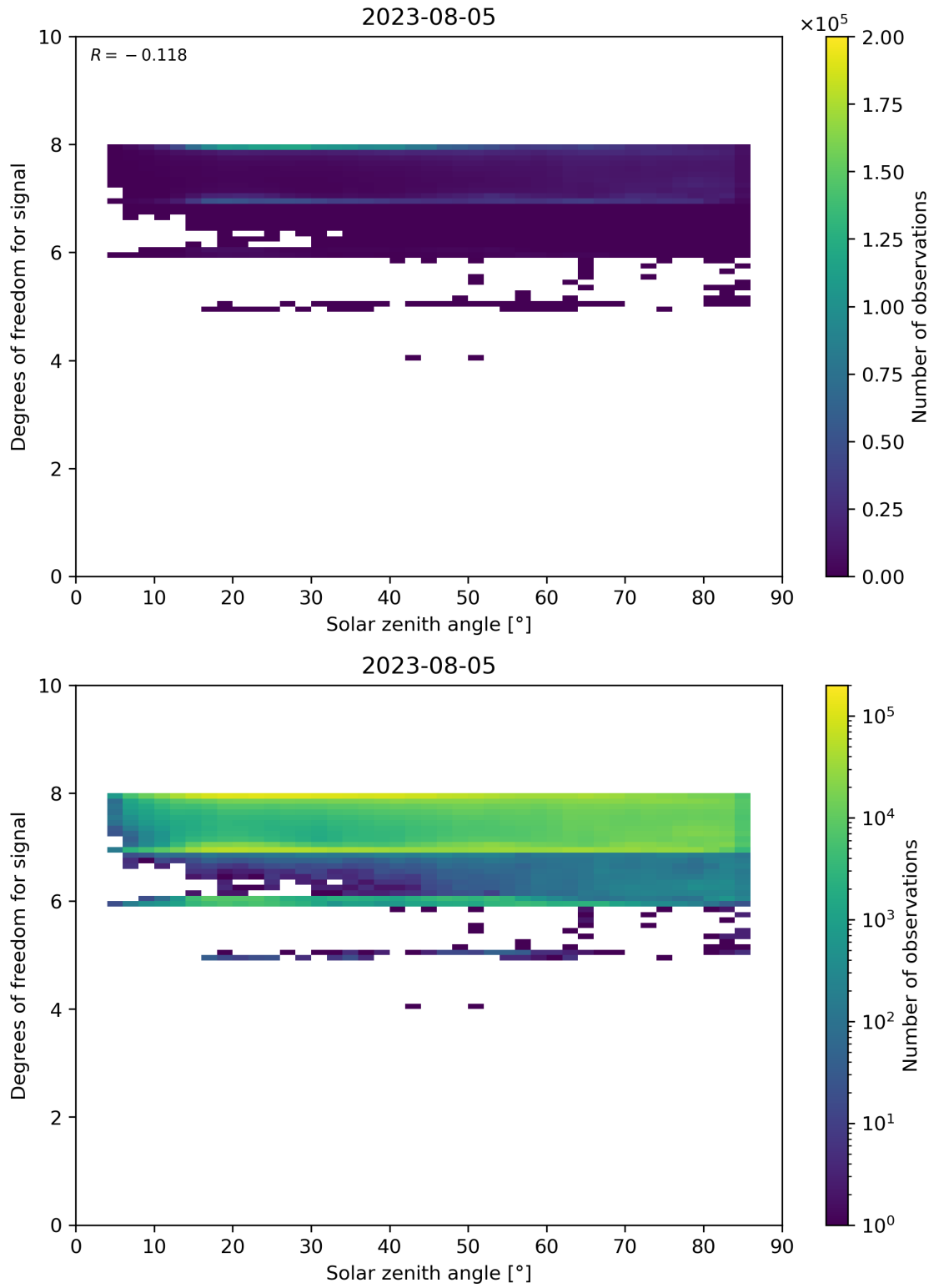
Figure 65: Scatter density plot of “Solar zenith angle” against “Degrees of freedom for signal” for 2023-08-04 to 2023-08-06.
