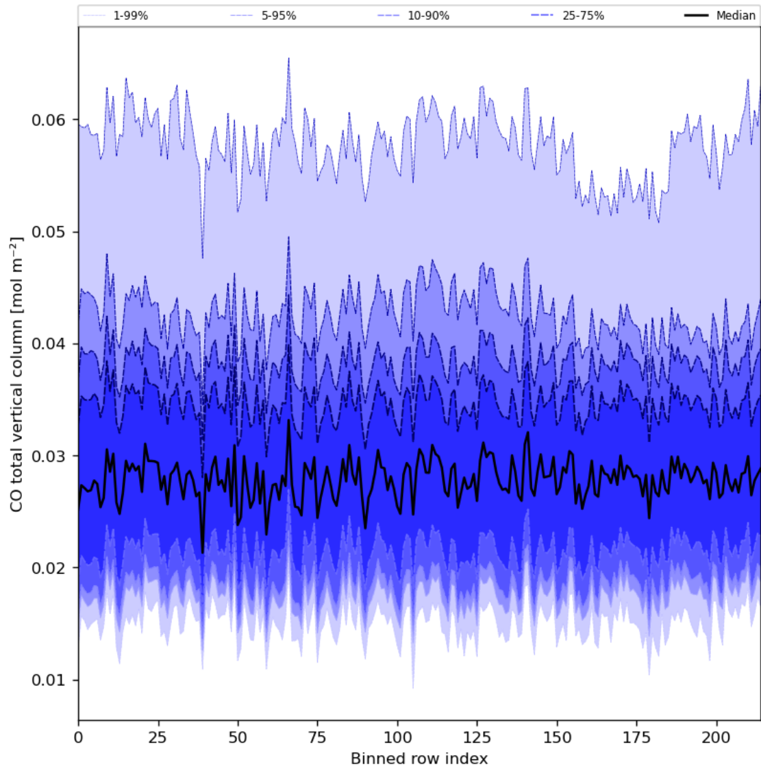
Figure 26: Along track statistics of “CO total vertical column” for 2023-08-04 to 2023-08-06
