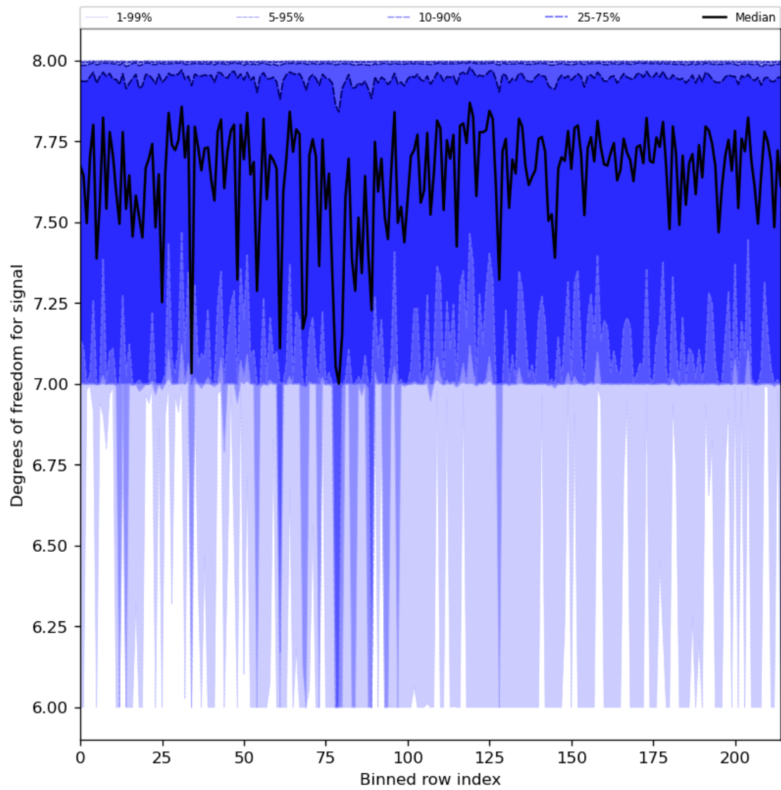
Figure 31: Along track statistics of “Degrees of freedom for signal” for 2023-08-04 to 2023-08-06
