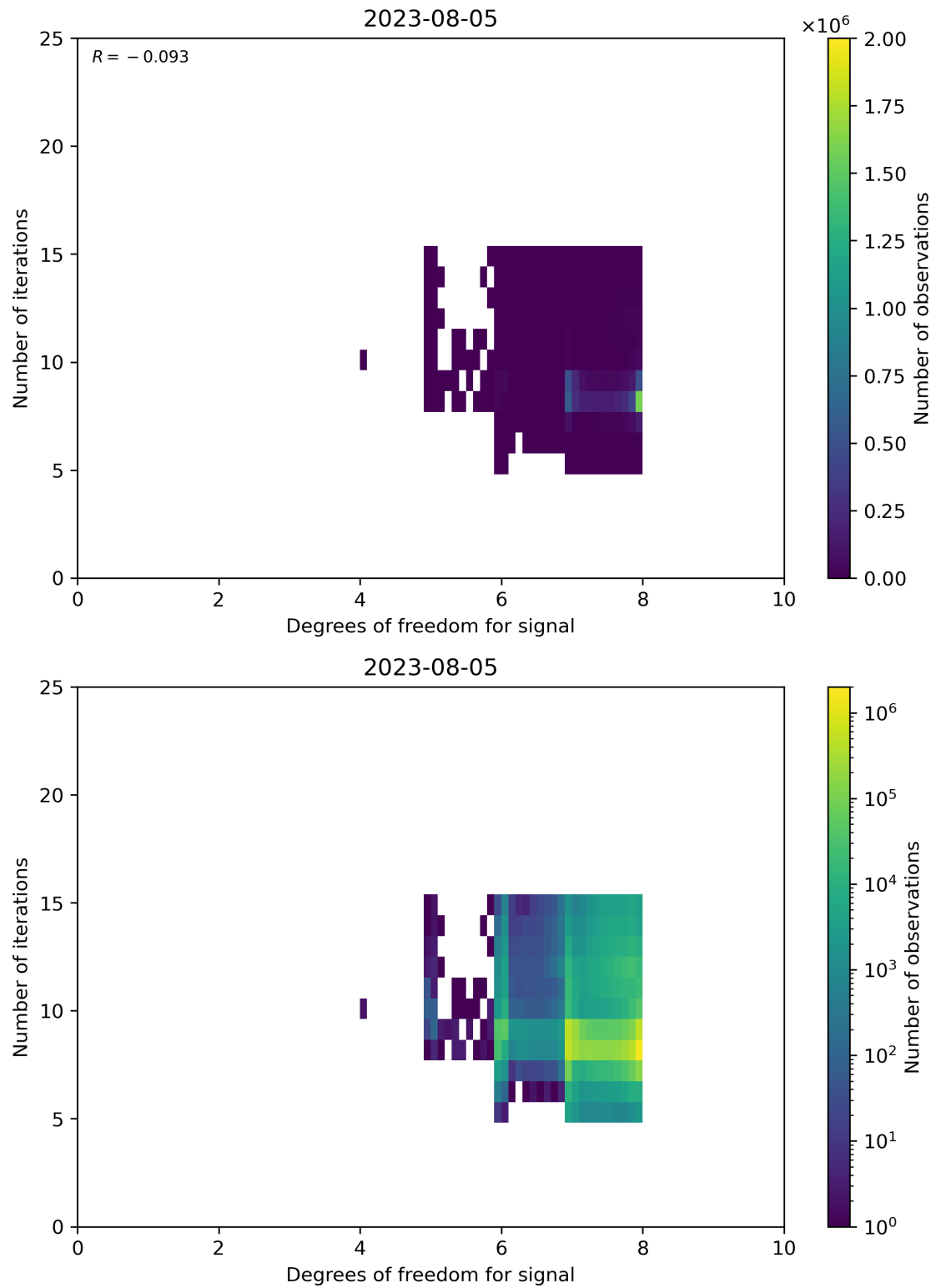
Figure 50: Scatter density plot of “Degrees of freedom for signal” against “Number of iterations” for 2023-08-04 to 2023-08-06.
