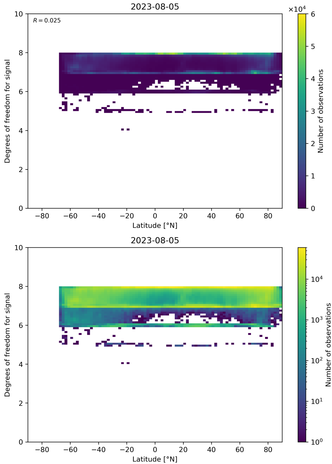
Figure 55: Scatter density plot of “Latitude” against “Degrees of freedom for signal” for 2023-08-04 to 2023-08-06.
