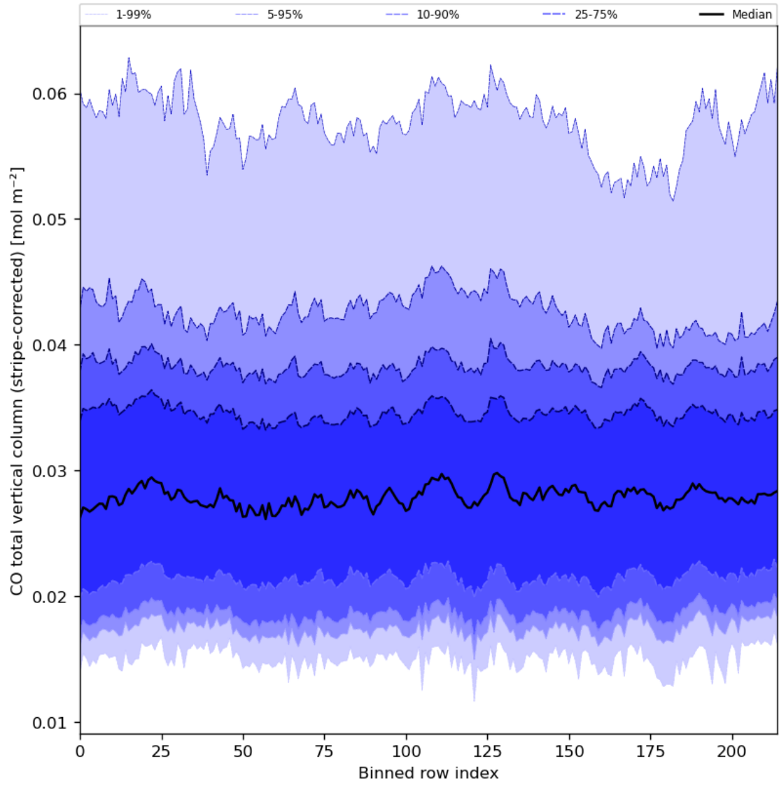
Figure 27: Along track statistics of “CO total vertical column (stripe-corrected)” for 2023-08-04 to 2023-08-06
