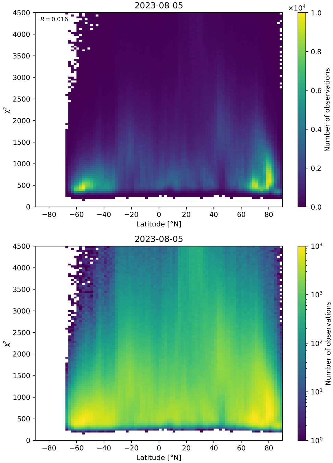
Figure 54: Scatter density plot of “Latitude” against “ \chi^2 ” for 2023-08-04 to 2023-08-06.
