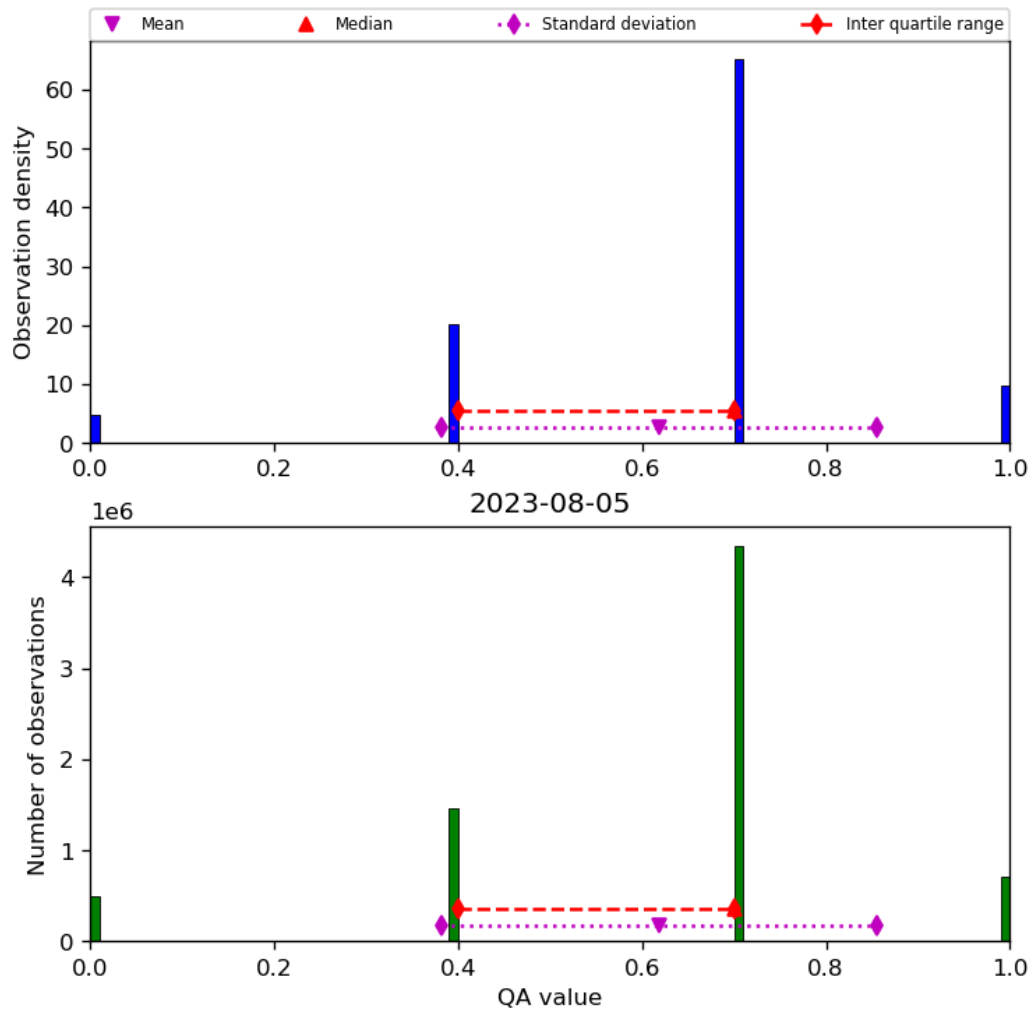
Figure 17: Histogram of “QA value” for 2023-08-04 to 2023-08-06
