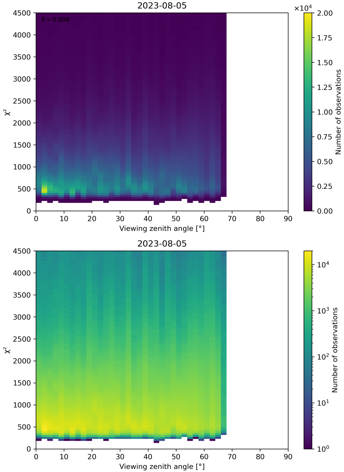
Figure 72: Scatter density plot of “Viewing zenith angle” against “ \chi^2 ” for 2023-08-04 to 2023-08-06.
