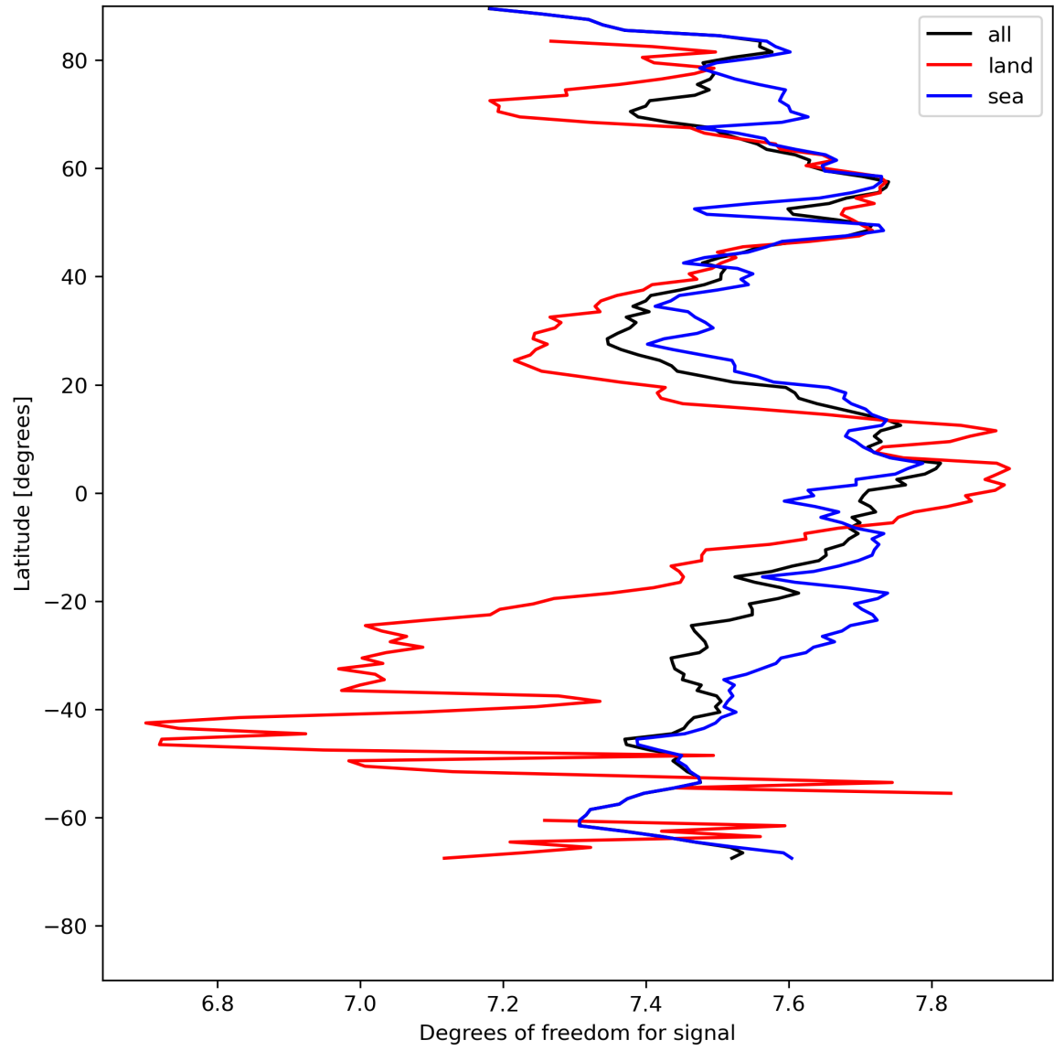
Figure 15: Zonal average of “Degrees of freedom for signal” for 2023-08-04 to 2023-08-06.
