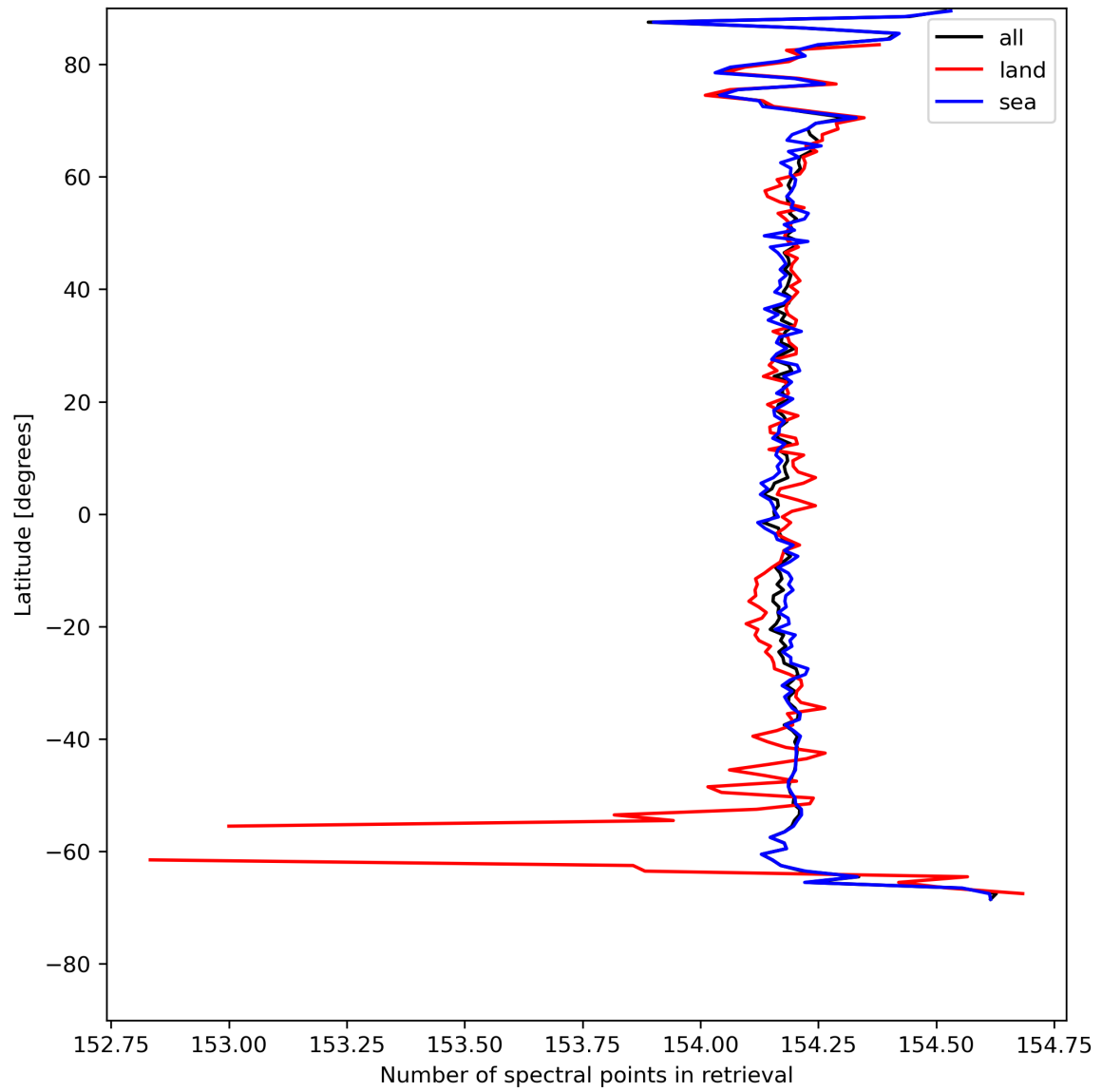
Figure 13: Zonal average of “Number of spectral points in retrieval” for 2023-08-05 to 2023-08-07.
