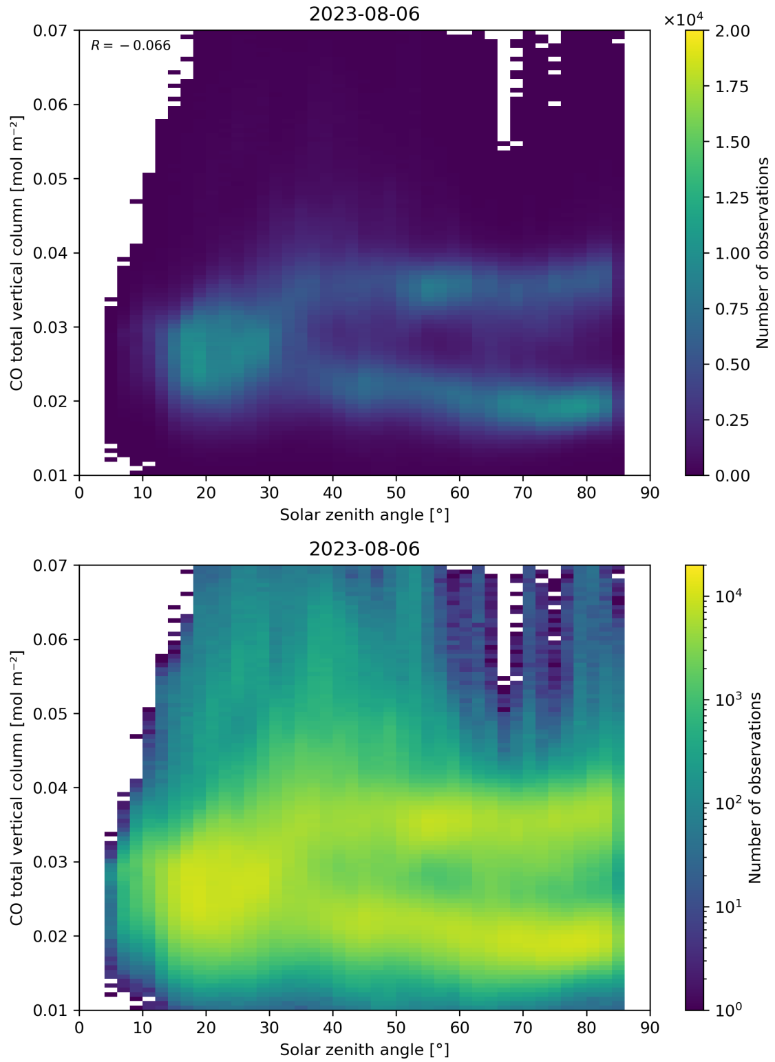
Figure 61: Scatter density plot of “Solar zenith angle” against “CO total vertical column” for 2023-08-05 to 2023-08-07.
