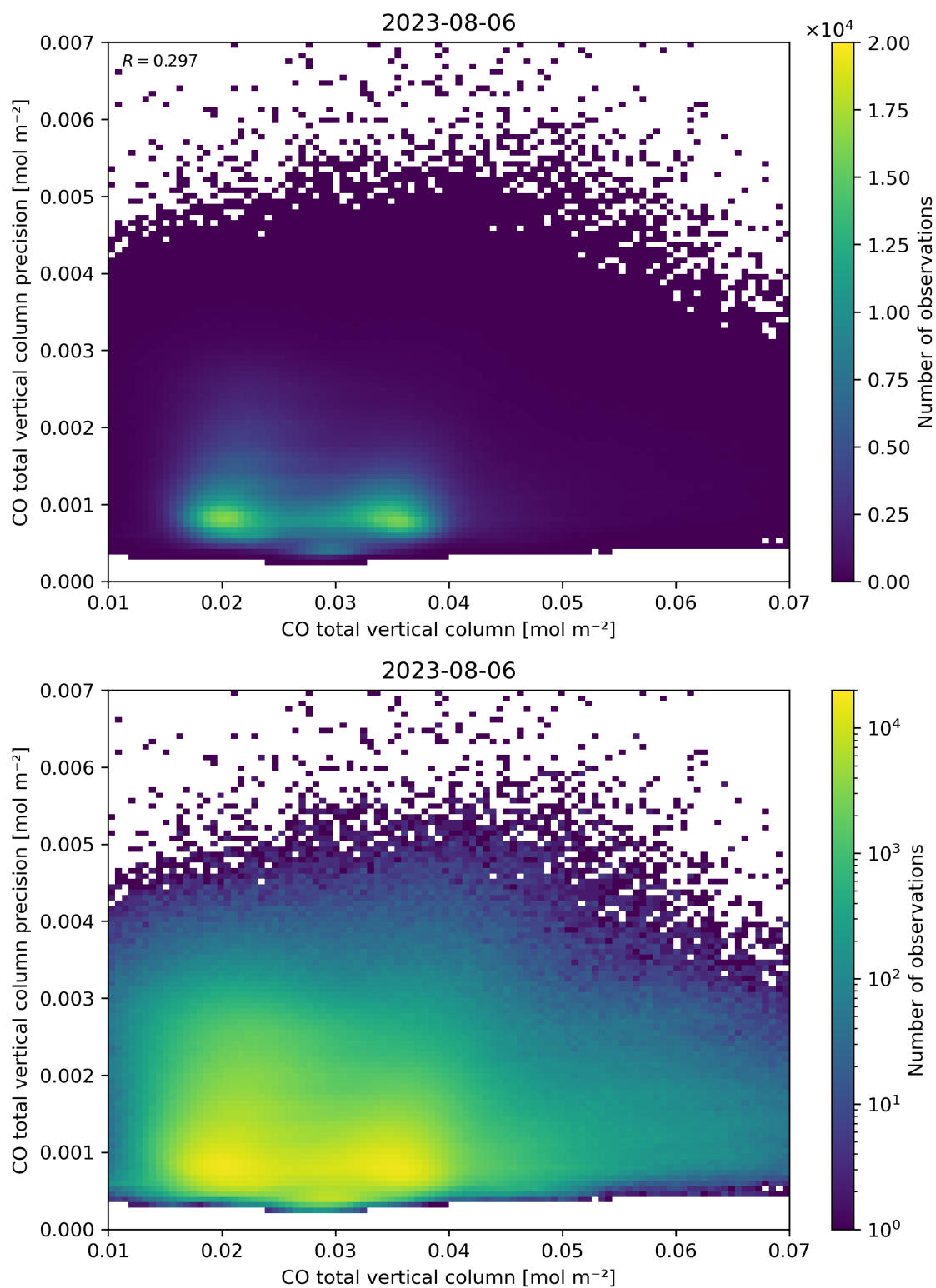
Figure 34: Scatter density plot of “CO total vertical column” against “CO total vertical column precision” for 2023-08-05 to 2023-08-07.
