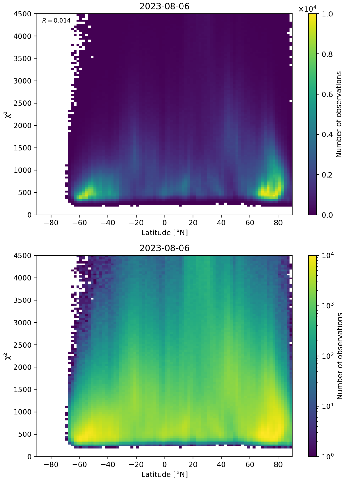
Figure 54: Scatter density plot of “Latitude” against “ \chi^2 ” for 2023-08-05 to 2023-08-07.
