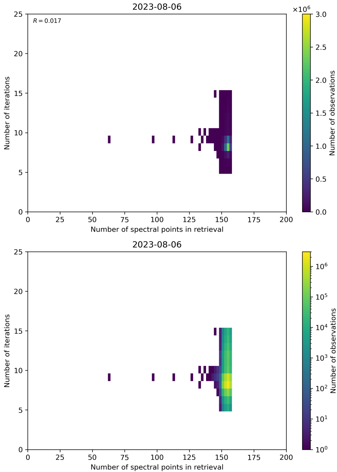
Figure 60: Scatter density plot of “Number of spectral points in retrieval” against “Number of iterations” for 2023-08-05 to 2023-08-07.
