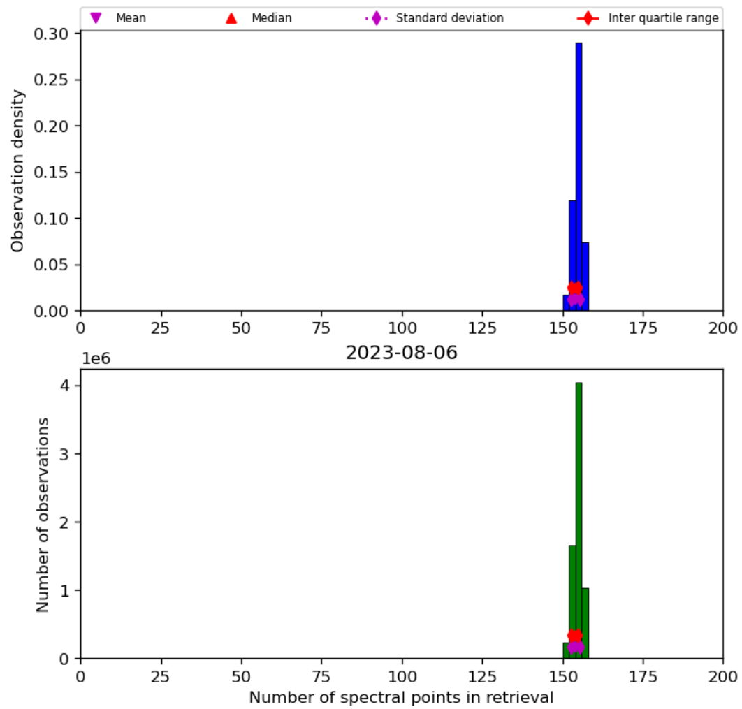
Figure 21: Histogram of “Number of spectral points in retrieval” for 2023-08-05 to 2023-08-07
