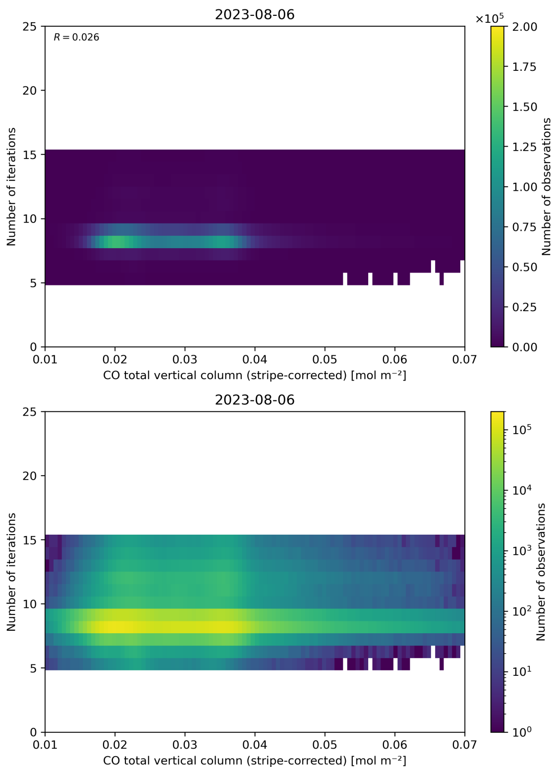
Figure 39: Scatter density plot of “CO total vertical column (stripe-corrected)” against “Number of iterations” for 2023-08-05 to 2023-08-07.
