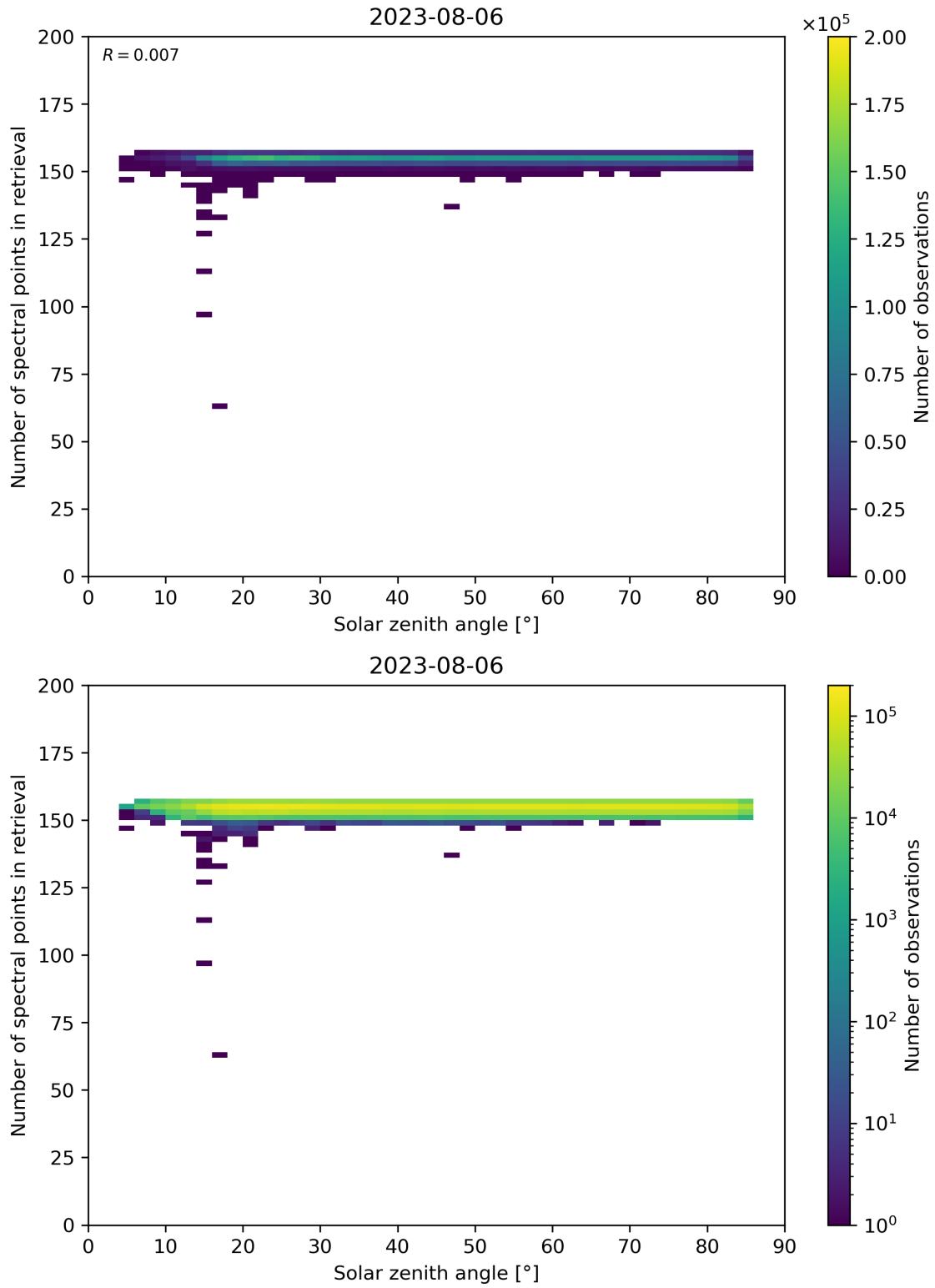
Figure 68: Scatter density plot of “Solar zenith angle” against “Number of spectral points in retrieval” for 2023-08-05 to 2023-08-07.
