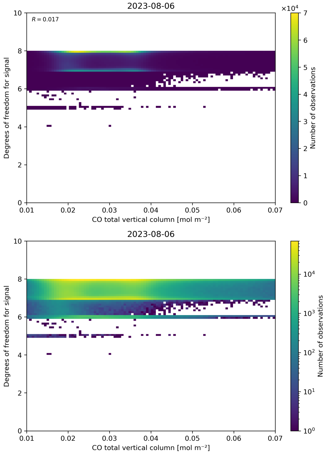
Figure 41: Scatter density plot of “CO total vertical column” against “Degrees of freedom for signal” for 2023-08-05 to 2023-08-07.
