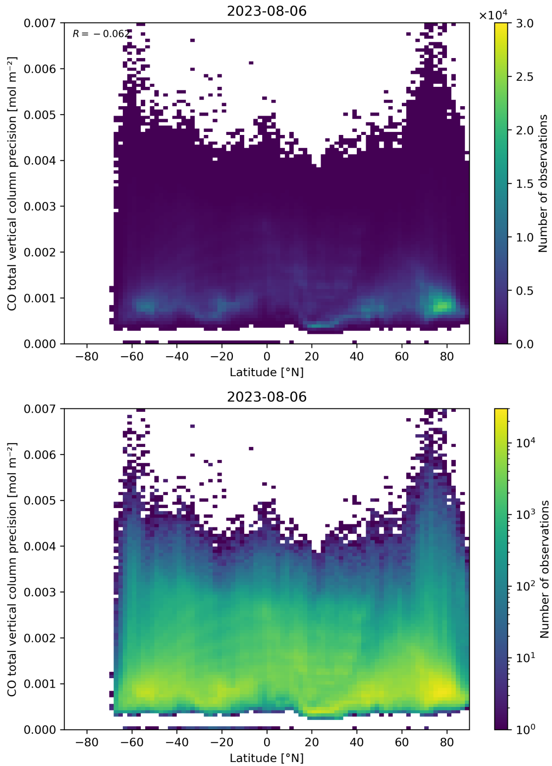
Figure 53: Scatter density plot of “Latitude” against “CO total vertical column precision” for 2023-08-05 to 2023-08-07.
