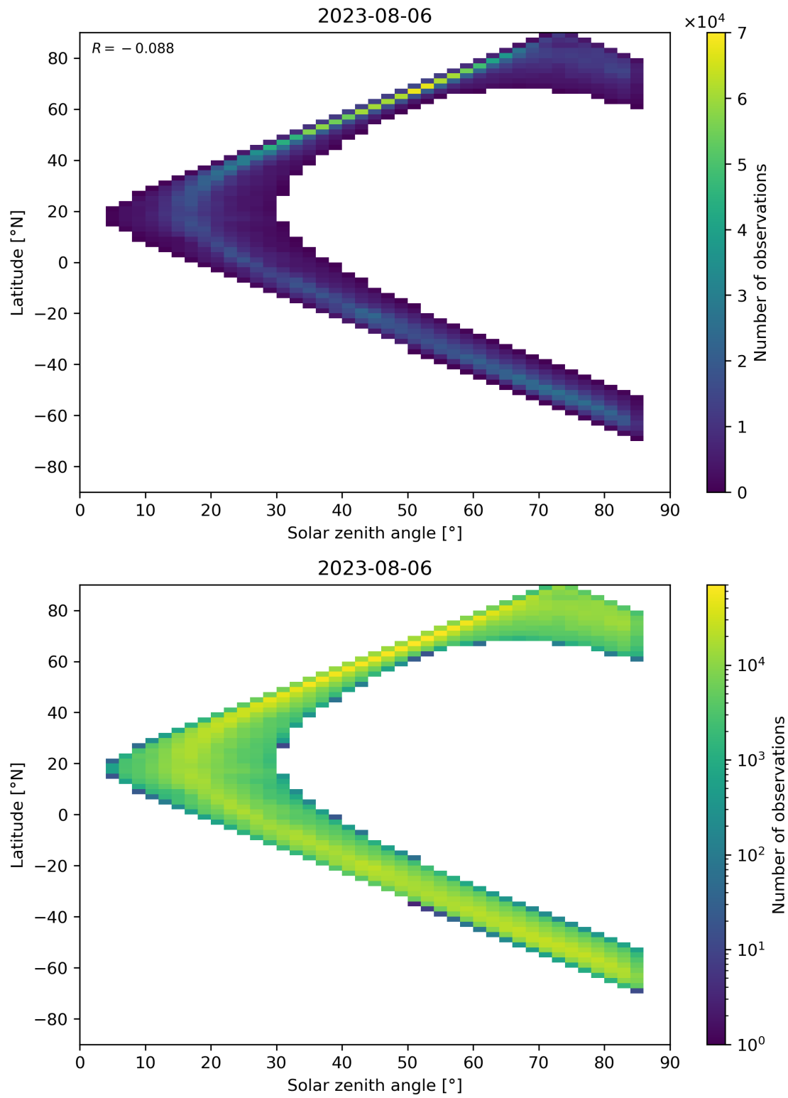
Figure 66: Scatter density plot of “Solar zenith angle” against “Latitude” for 2023-08-05 to 2023-08-07.
