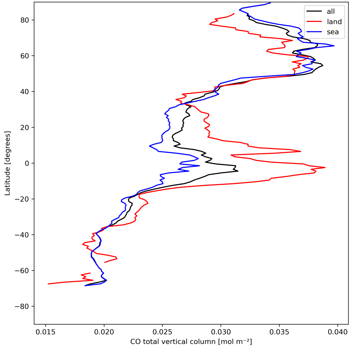
Figure 10: Zonal average of “CO total vertical column” for 2023-08-05 to 2023-08-07.
