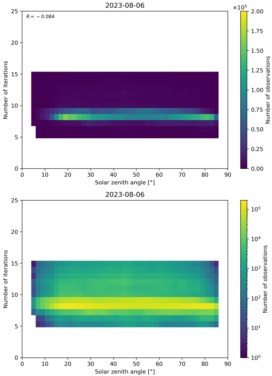
Figure 67: Scatter density plot of “Solar zenith angle” against “Number of iterations” for 2023-08-05 to 2023-08-07.
