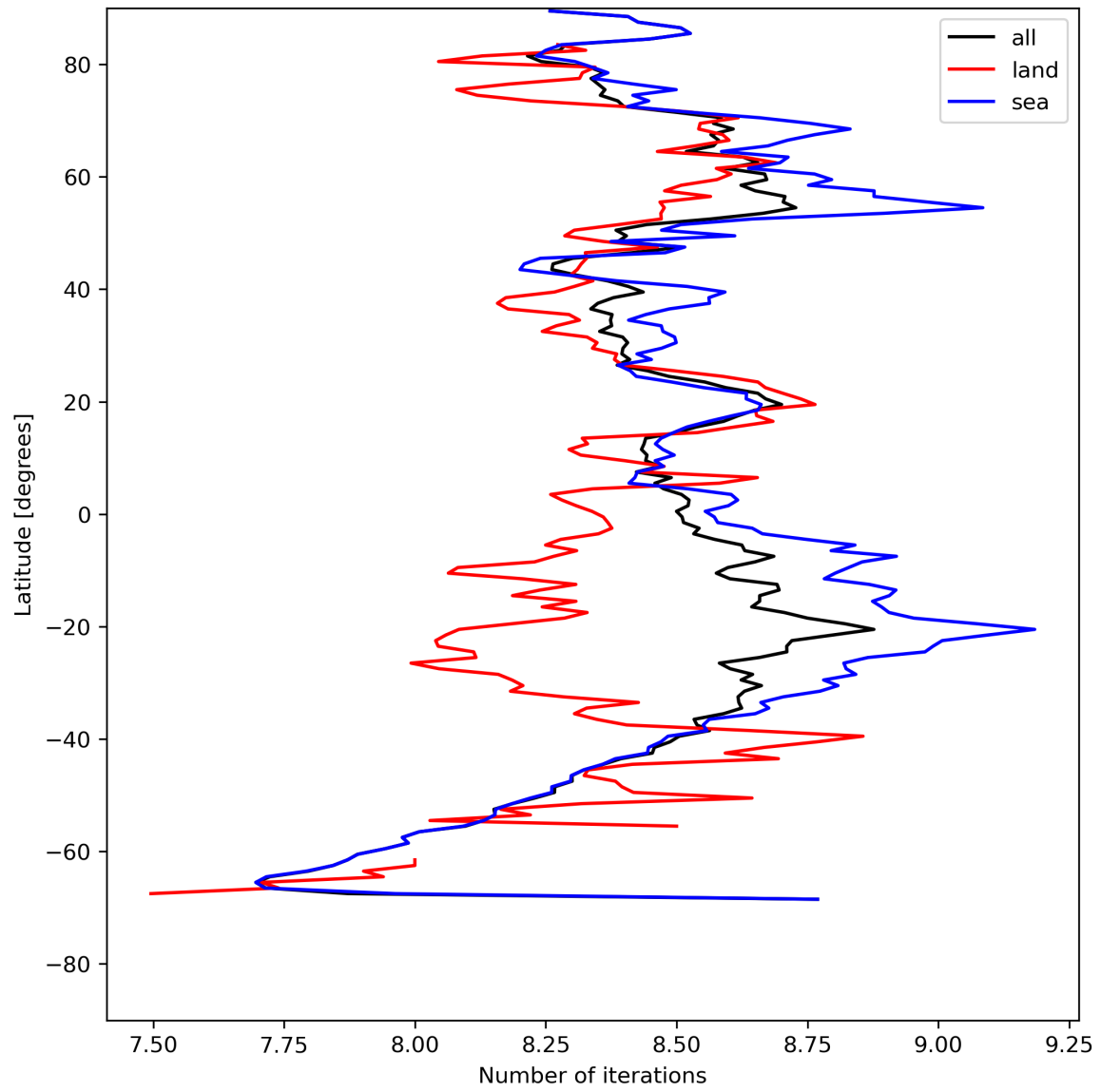
Figure 16: Zonal average of “Number of iterations” for 2023-08-05 to 2023-08-07.
