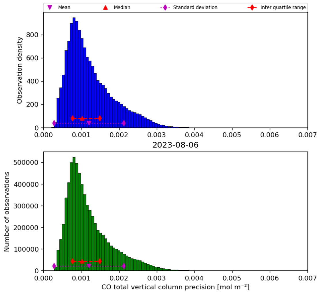
Figure 20: Histogram of “CO total vertical column precision” for 2023-08-05 to 2023-08-07
