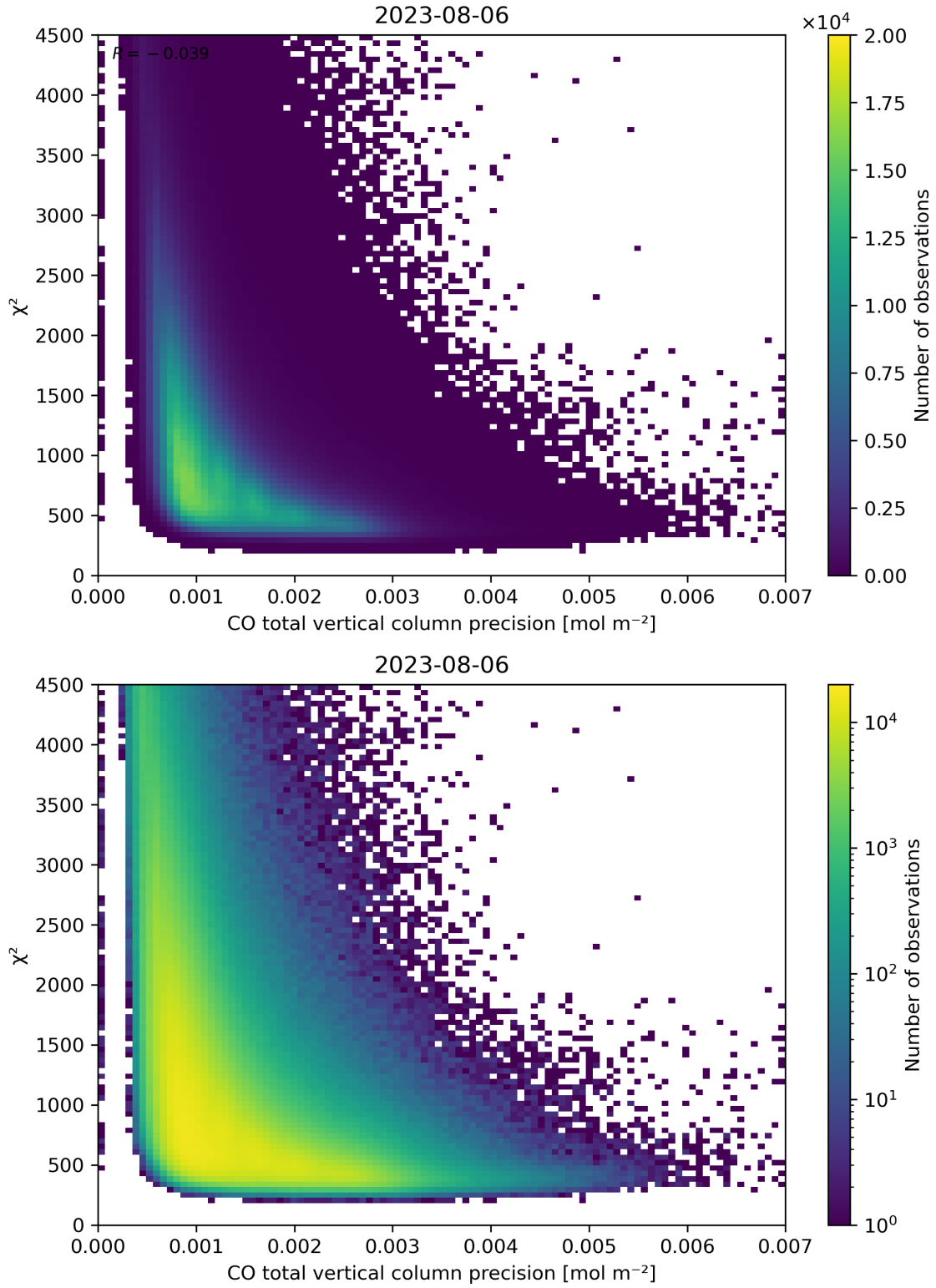
Figure 44: Scatter density plot of “CO total vertical column precision” against “ \chi^2 ” for 2023-08-05 to 2023-08-07.
