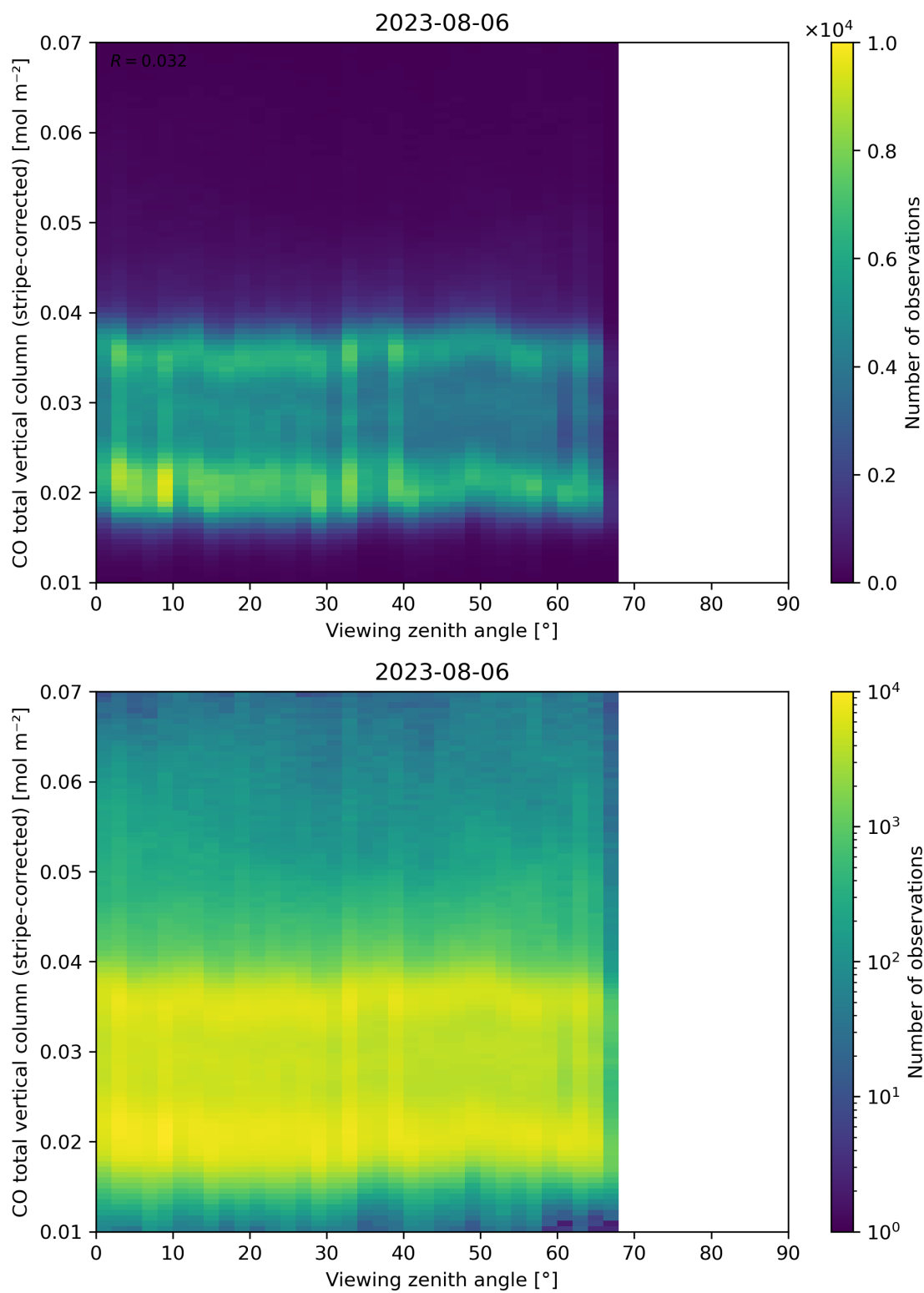
Figure 70: Scatter density plot of “Viewing zenith angle” against “CO total vertical column (stripe-corrected)” for 2023-08-05 to 2023-08-07.
