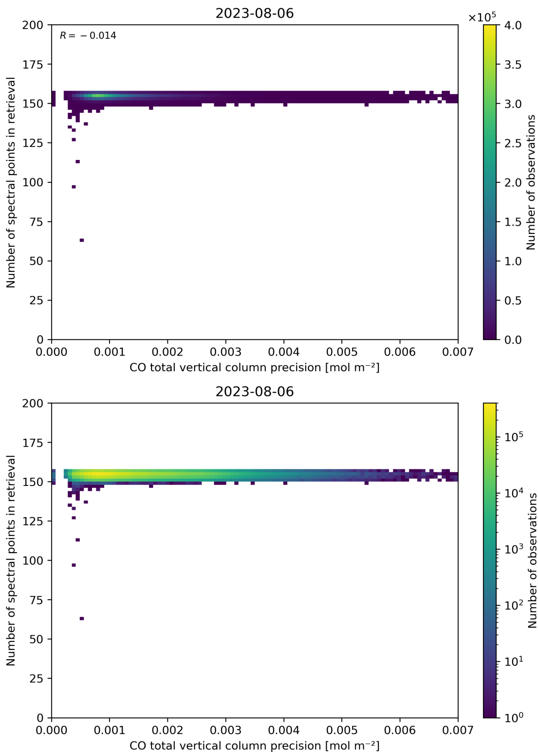
Figure 47: Scatter density plot of “CO total vertical column precision” against “Number of spectral points in retrieval” for 2023-08-05 to 2023-08-07.
