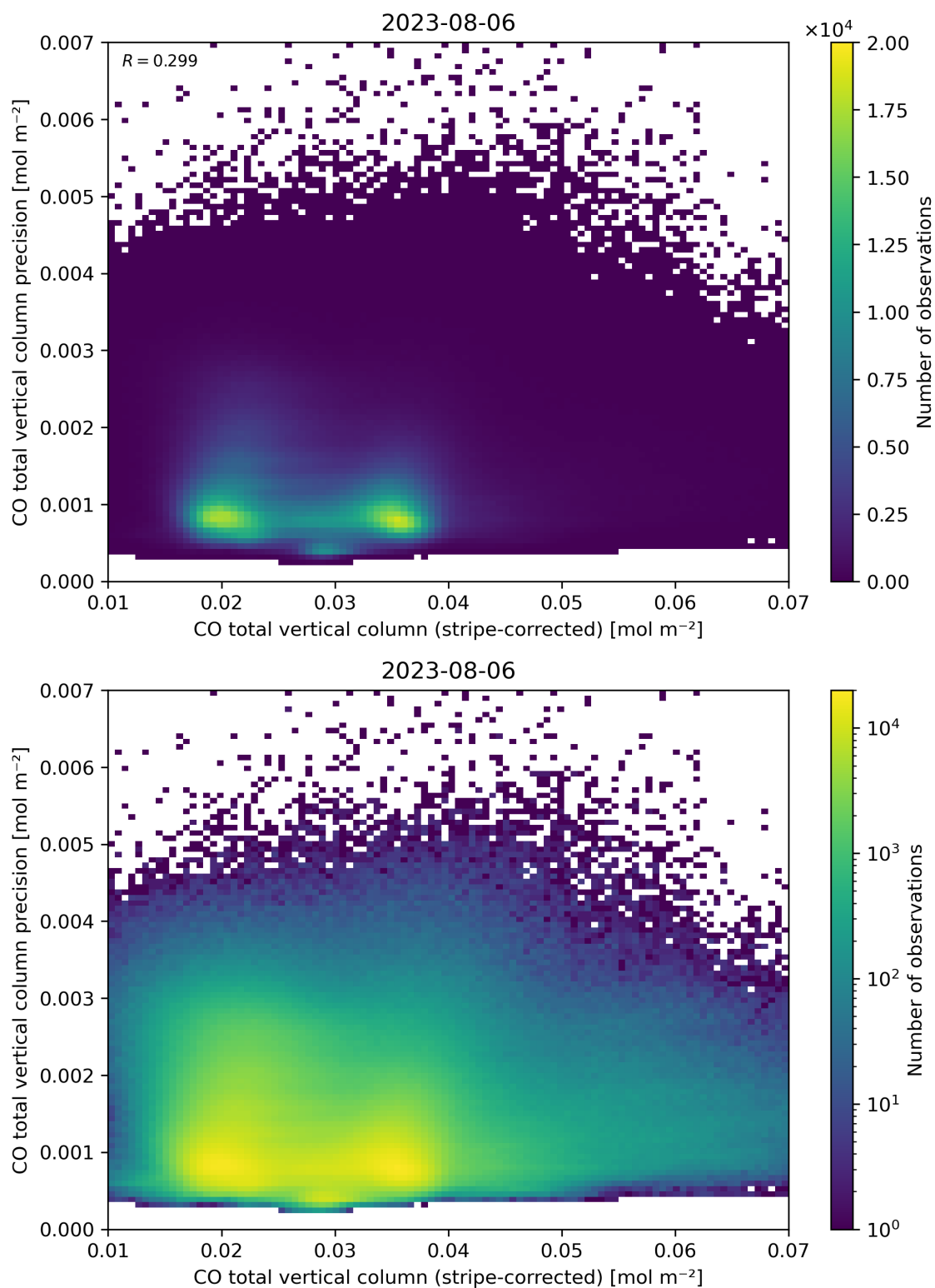
Figure 36: Scatter density plot of “CO total vertical column (stripe-corrected)” against “CO total vertical column precision” for 2023-08-05 to 2023-08-07.
