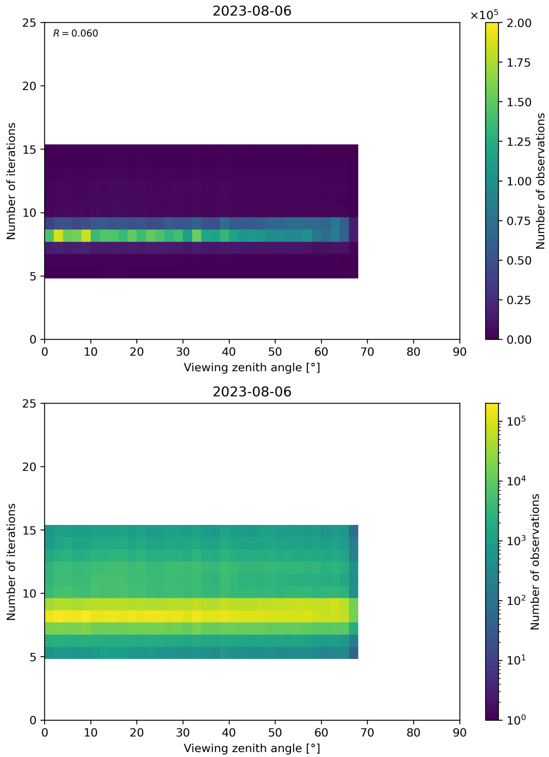
Figure 75: Scatter density plot of “Viewing zenith angle” against “Number of iterations” for 2023-08-05 to 2023-08-07.
