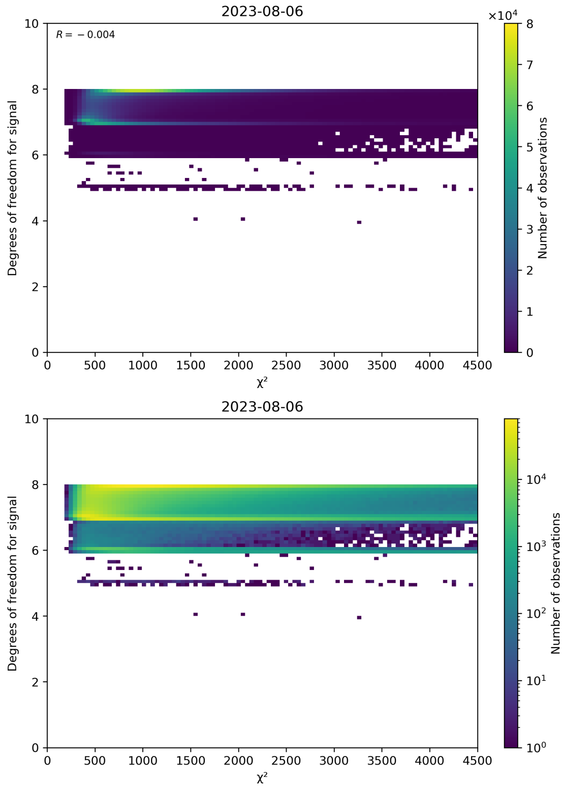
Figure 48: Scatter density plot of " \chi^2 " against "Degrees of freedom for signal" for 2023-08-05 to 2023-08-07.
