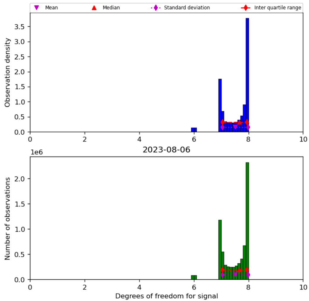
Figure 23: Histogram of “Degrees of freedom for signal” for 2023-08-05 to 2023-08-07
