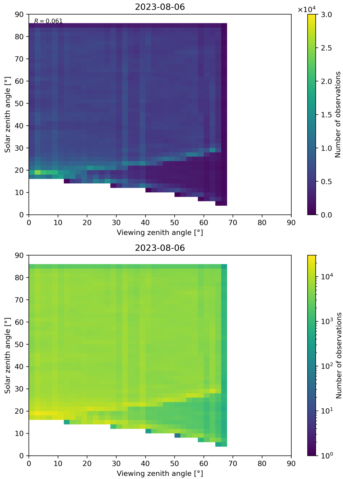
Figure 77: Scatter density plot of “Viewing zenith angle” against “Solar zenith angle” for 2023-08-05 to 2023-08-07.
