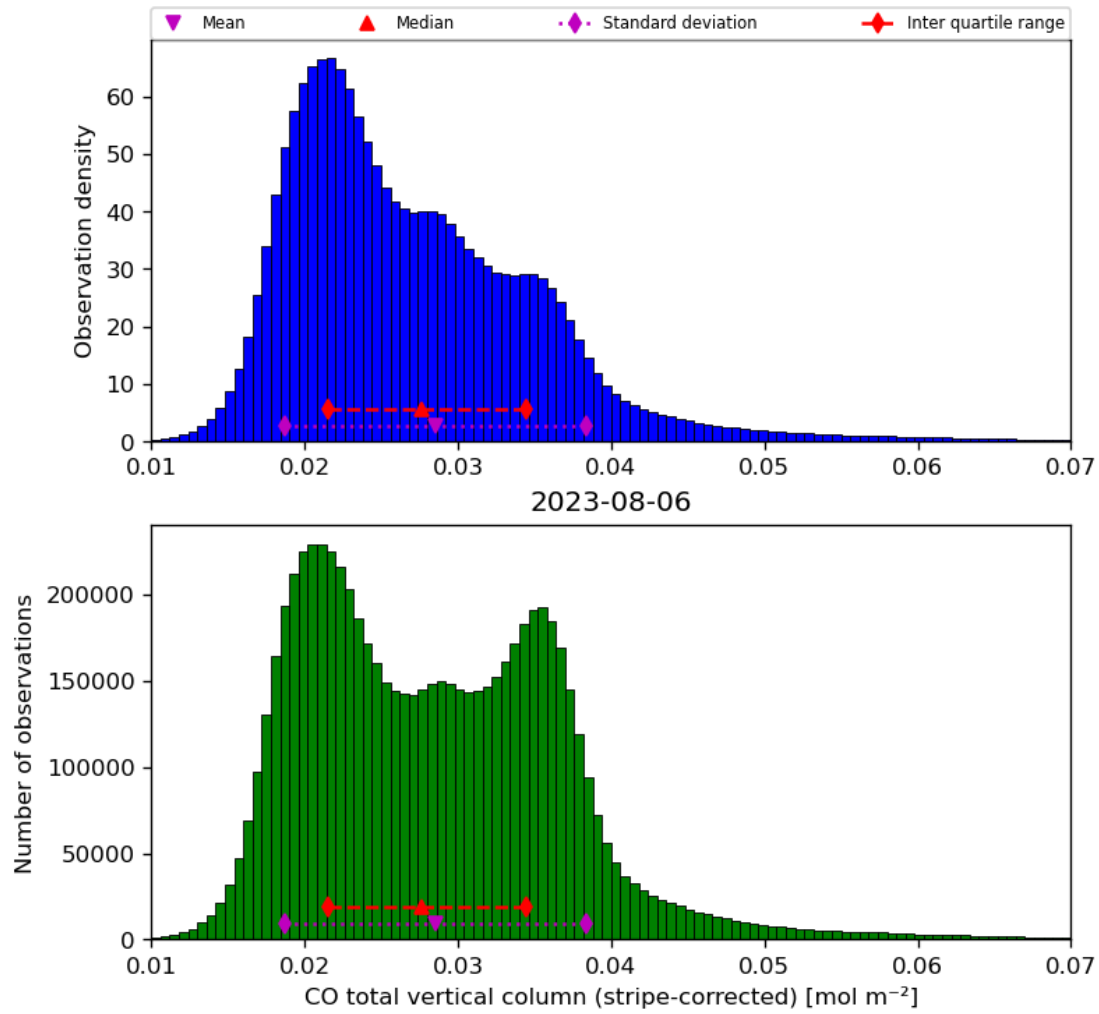
Figure 19: Histogram of “CO total vertical column (stripe-corrected)” for 2023-08-05 to 2023-08-07
