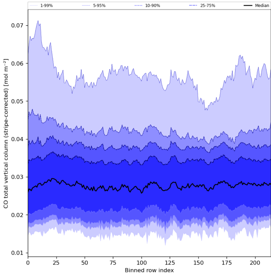
Figure 27: Along track statistics of “CO total vertical column (stripe-corrected)” for 2023-08-05 to 2023-08-07
