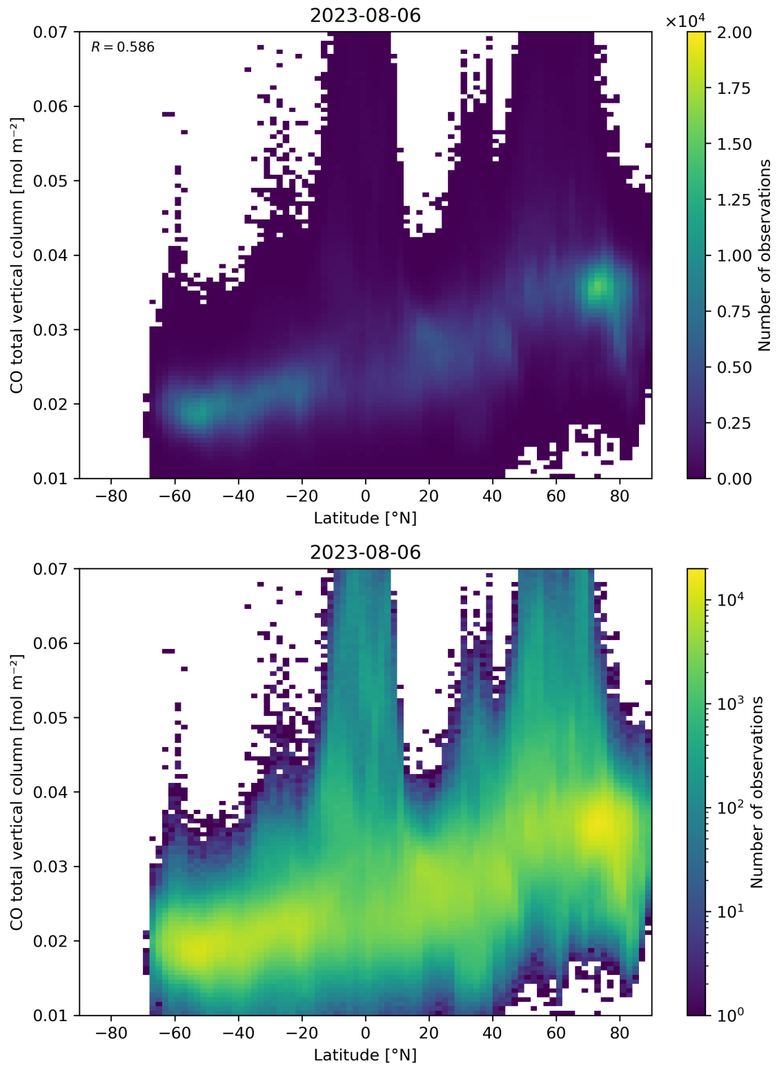
Figure 51: Scatter density plot of “Latitude” against “CO total vertical column” for 2023-08-05 to 2023-08-07.
