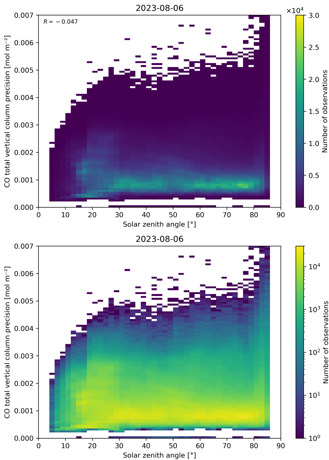
Figure 63: Scatter density plot of “Solar zenith angle” against “CO total vertical column precision” for 2023-08-05 to 2023-08-07.
