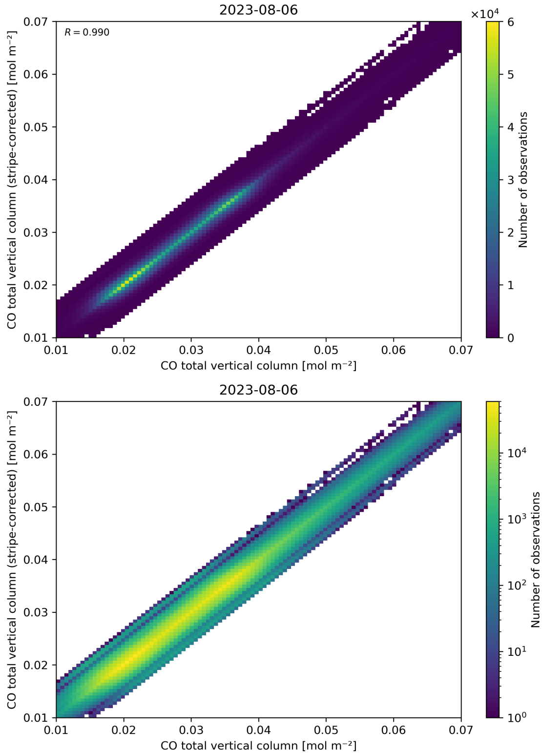
Figure 33: Scatter density plot of “CO total vertical column” against “CO total vertical column (stripe-corrected)” for 2023-08-05 to 2023-08-07.
