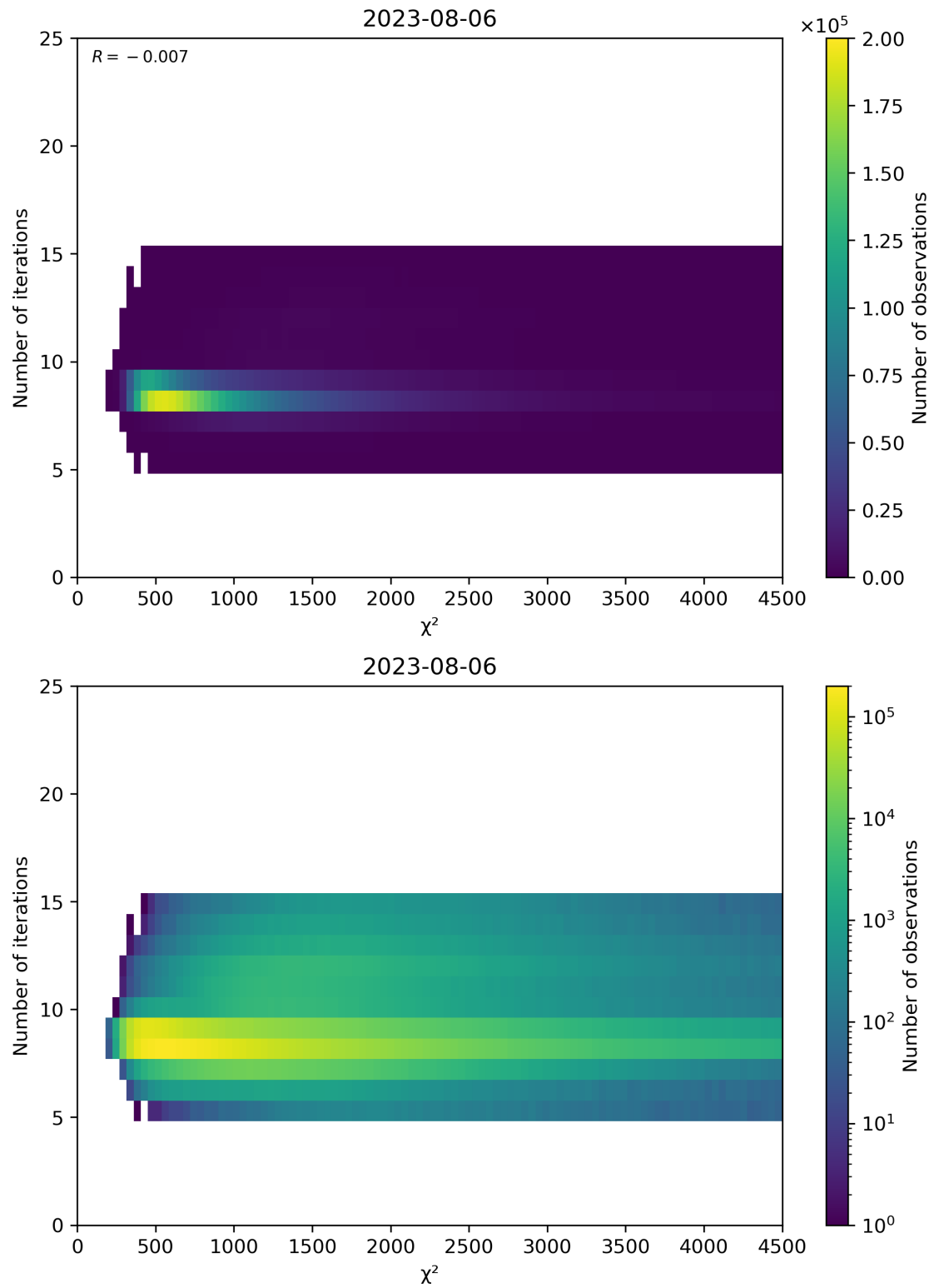
Figure 49: Scatter density plot of “ \chi^2 ” against “Number of iterations” for 2023-08-05 to 2023-08-07.
