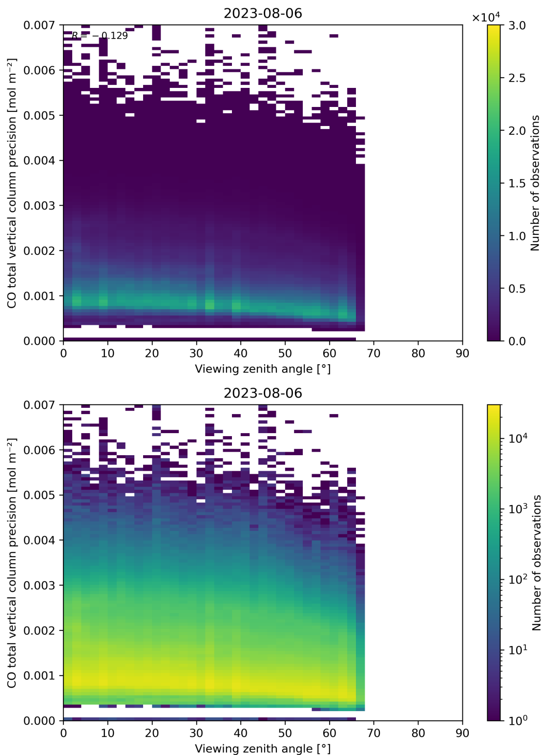
Figure 71: Scatter density plot of “Viewing zenith angle” against “CO total vertical column precision” for 2023-08-05 to 2023-08-07.
