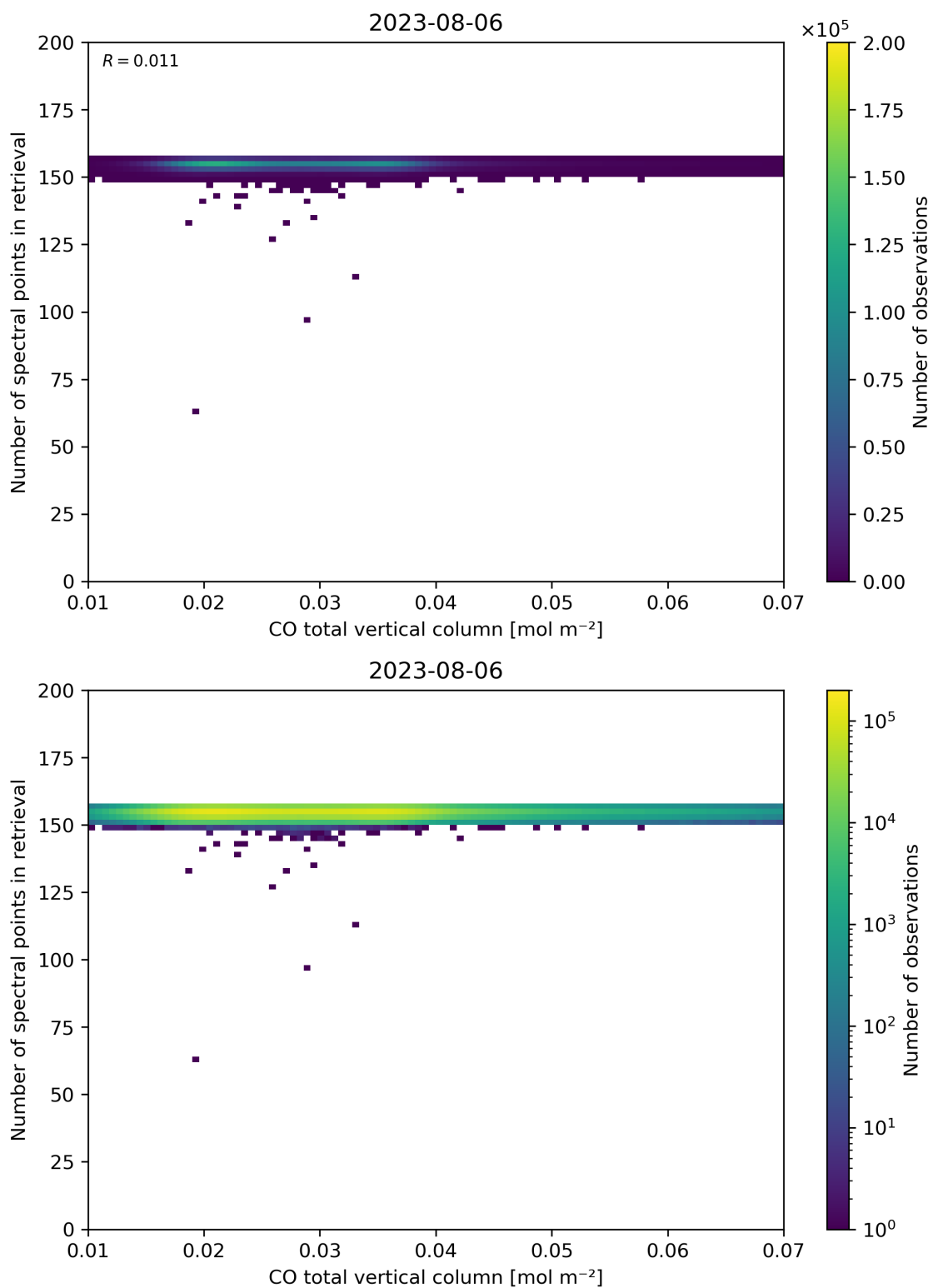
Figure 43: Scatter density plot of “CO total vertical column” against “Number of spectral points in retrieval” for 2023-08-05 to 2023-08-07.
