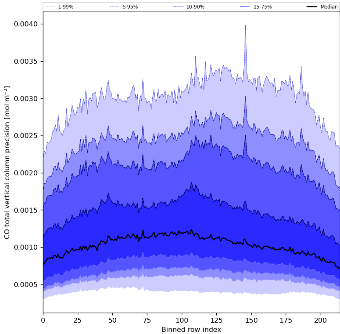
Figure 28: Along track statistics of “CO total vertical column precision” for 2023-08-05 to 2023-08-07
