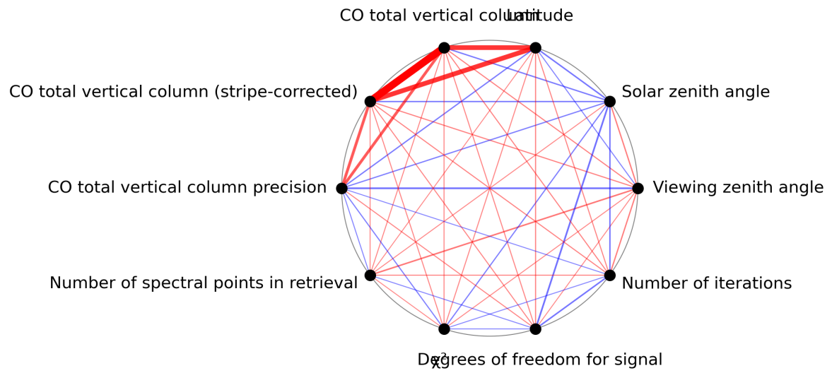
Figure 1: Map of correlation graph for 2023-08-05 to 2023-08-07.
