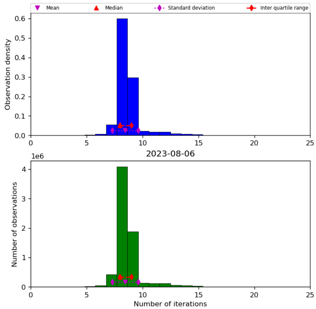
Figure 24: Histogram of “Number of iterations” for 2023-08-05 to 2023-08-07
