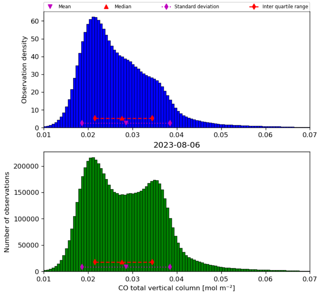
Figure 18: Histogram of “CO total vertical column” for 2023-08-05 to 2023-08-07
