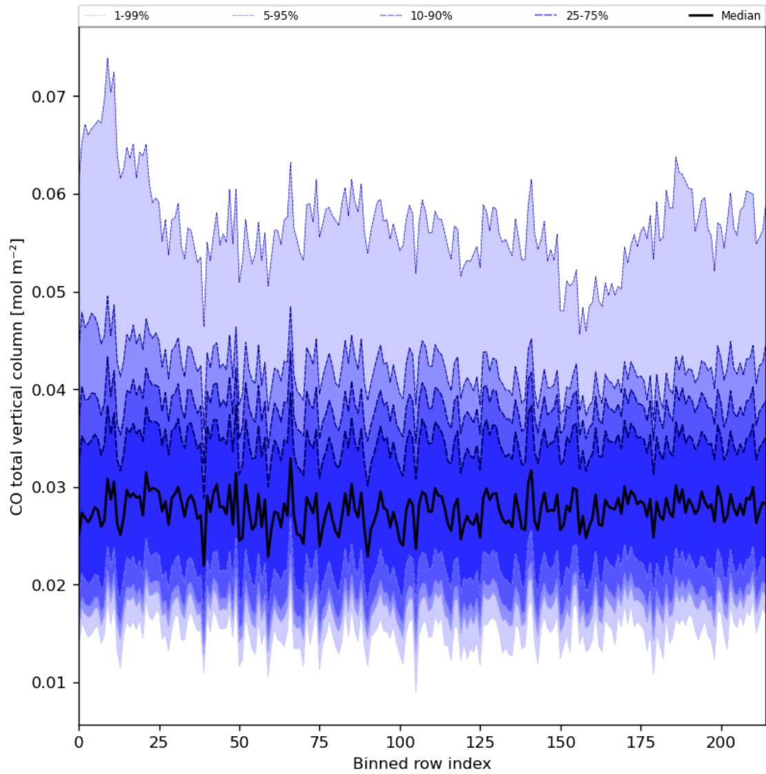
Figure 26: Along track statistics of “CO total vertical column” for 2023-08-05 to 2023-08-07
