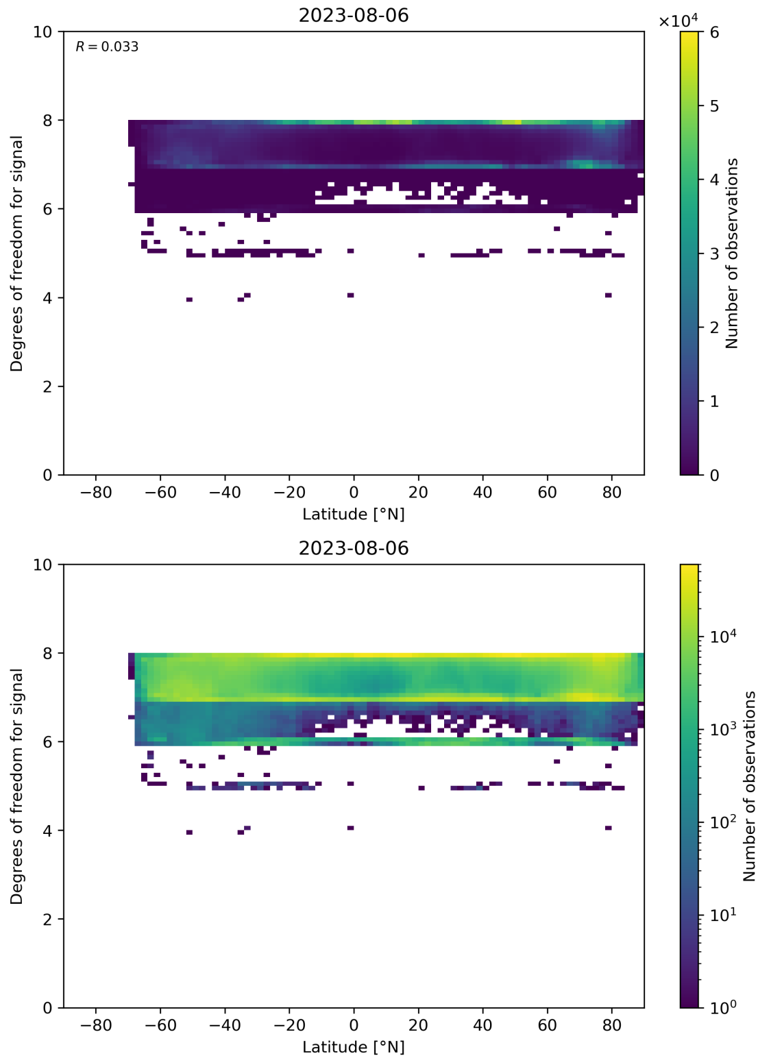
Figure 55: Scatter density plot of “Latitude” against “Degrees of freedom for signal” for 2023-08-05 to 2023-08-07.
