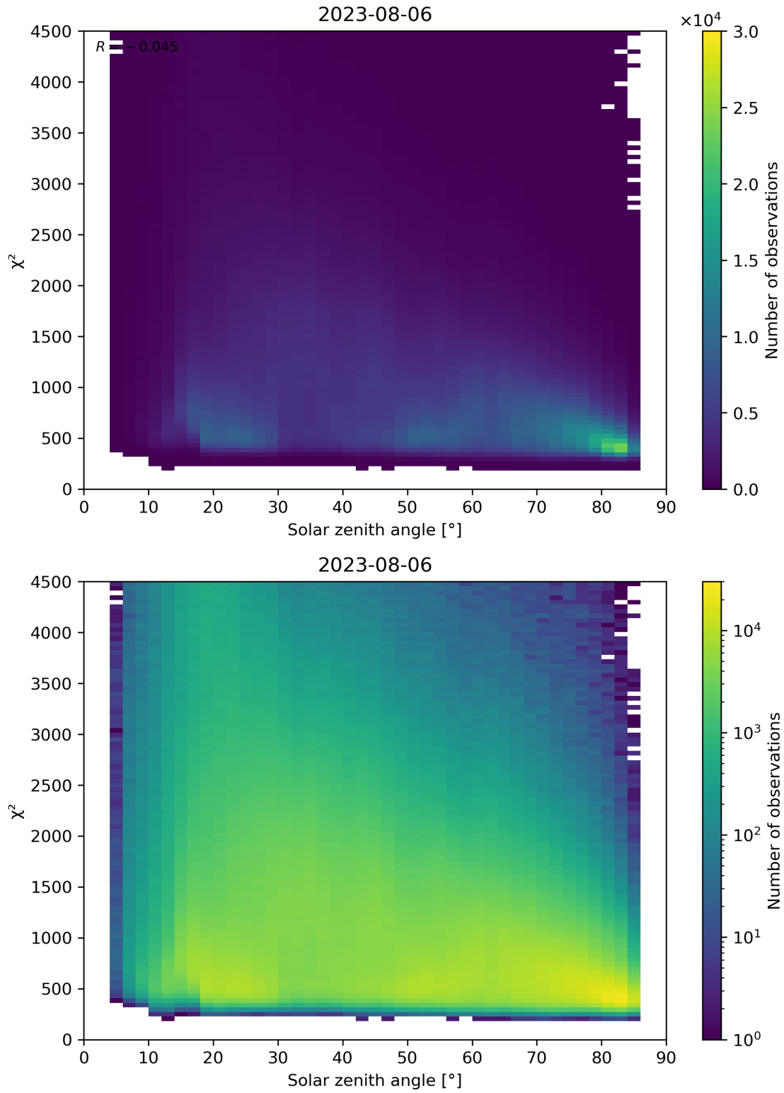
Figure 64: Scatter density plot of “Solar zenith angle” against “ \chi^2 ” for 2023-08-05 to 2023-08-07.
