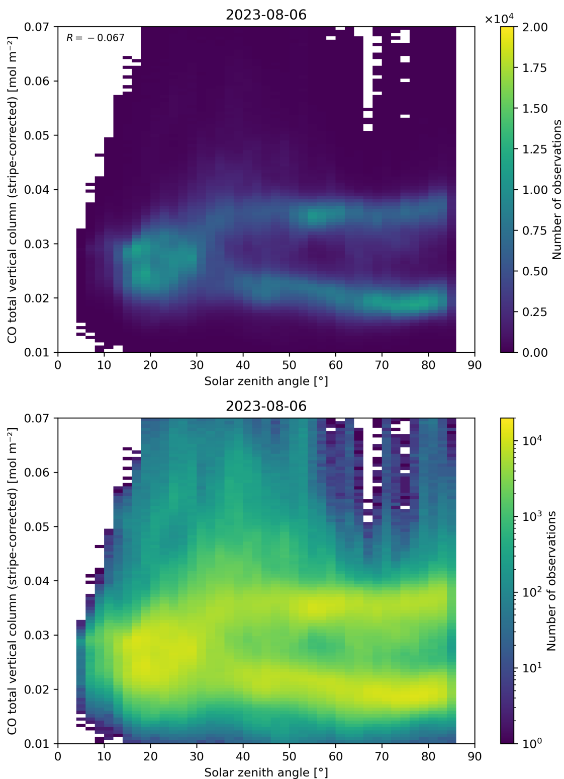
Figure 62: Scatter density plot of “Solar zenith angle” against “CO total vertical column (stripe-corrected)” for 2023-08-05 to 2023-08-07.
