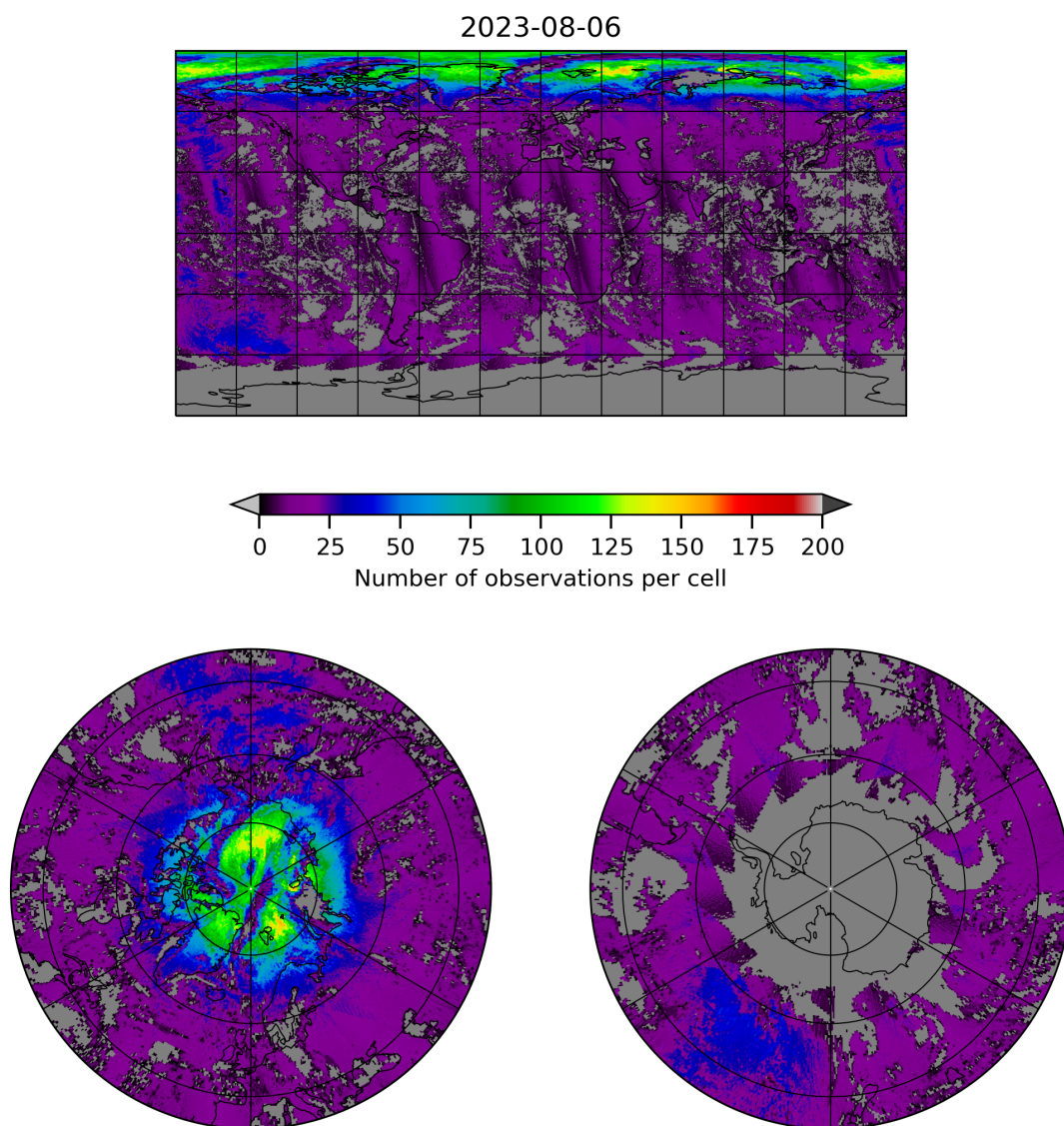
Figure 8: Map of the number of observations for 2023-08-05 to 2023-08-07
