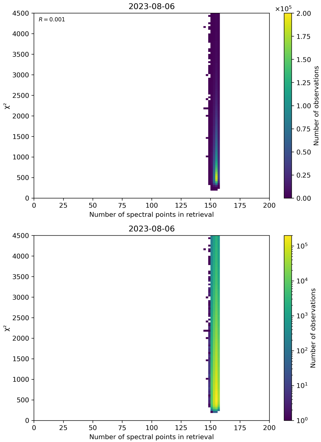
Figure 58: Scatter density plot of “Number of spectral points in retrieval” against “ \chi^2 ” for 2023-08-05 to 2023-08-07.
