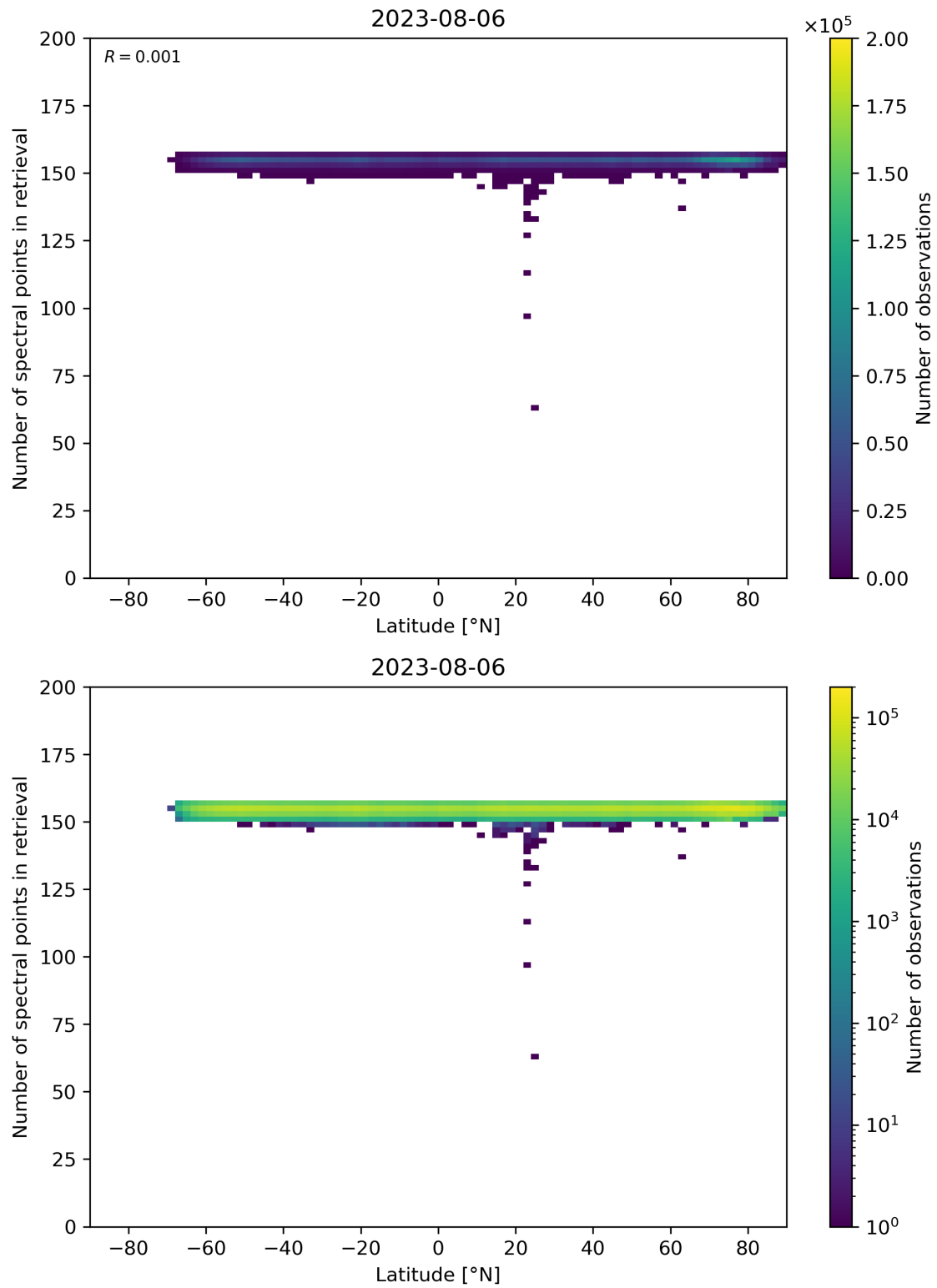
Figure 57: Scatter density plot of “Latitude” against “Number of spectral points in retrieval” for 2023-08-05 to 2023-08-07.
