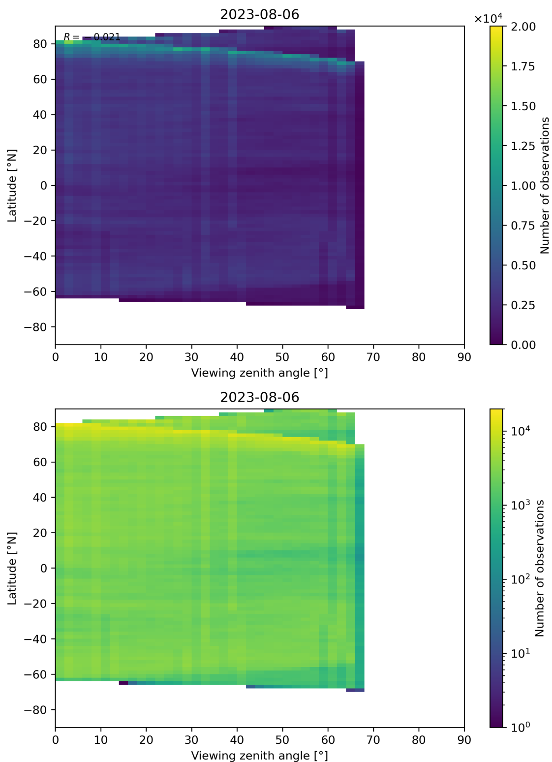
Figure 74: Scatter density plot of “Viewing zenith angle” against “Latitude” for 2023-08-05 to 2023-08-07.
