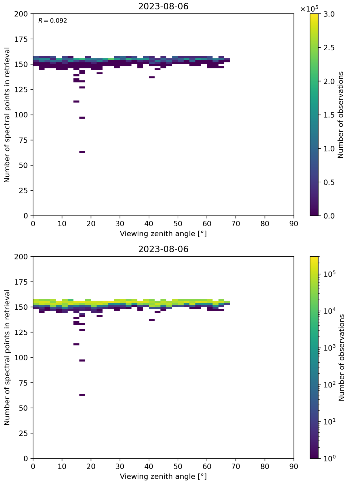
Figure 76: Scatter density plot of “Viewing zenith angle” against “Number of spectral points in retrieval” for 2023-08-05 to 2023-08-07.
