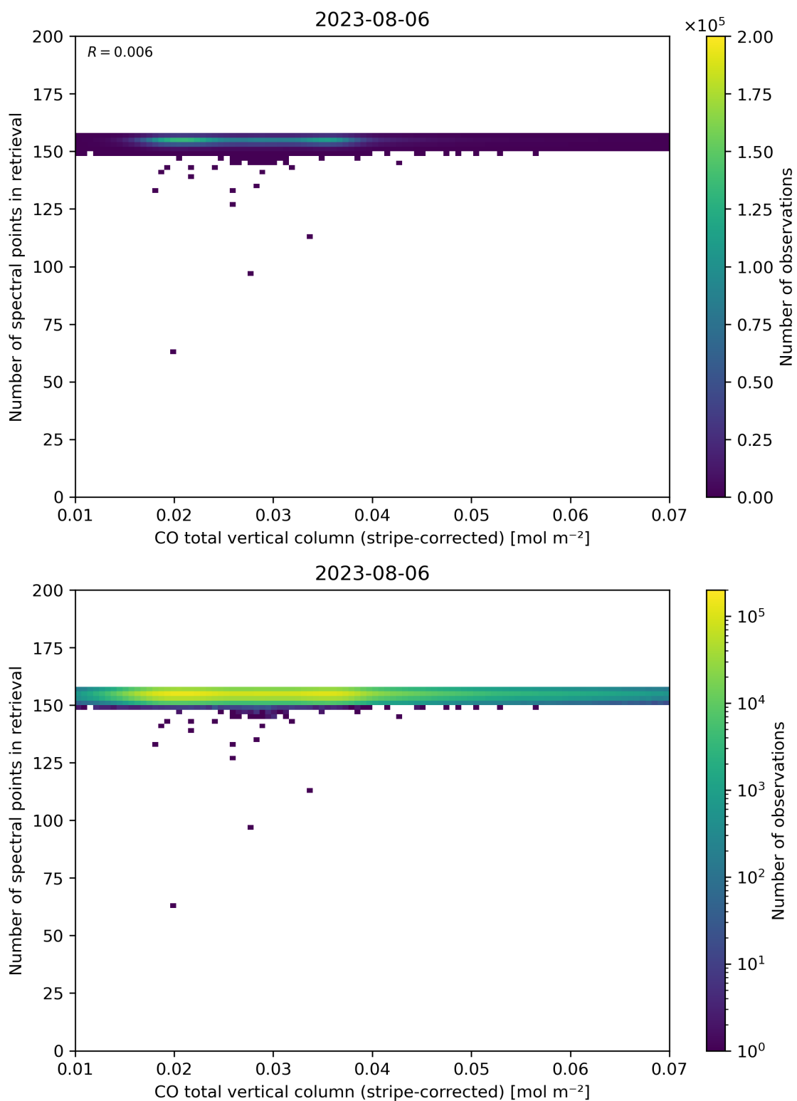
Figure 40: Scatter density plot of “CO total vertical column (stripe-corrected)” against “Number of spectral points in retrieval” for 2023-08-05 to 2023-08-07.
