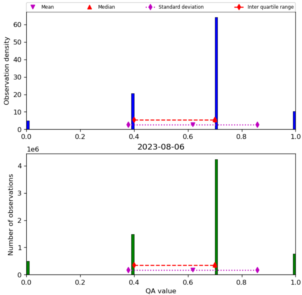
Figure 17: Histogram of “QA value” for 2023-08-05 to 2023-08-07
