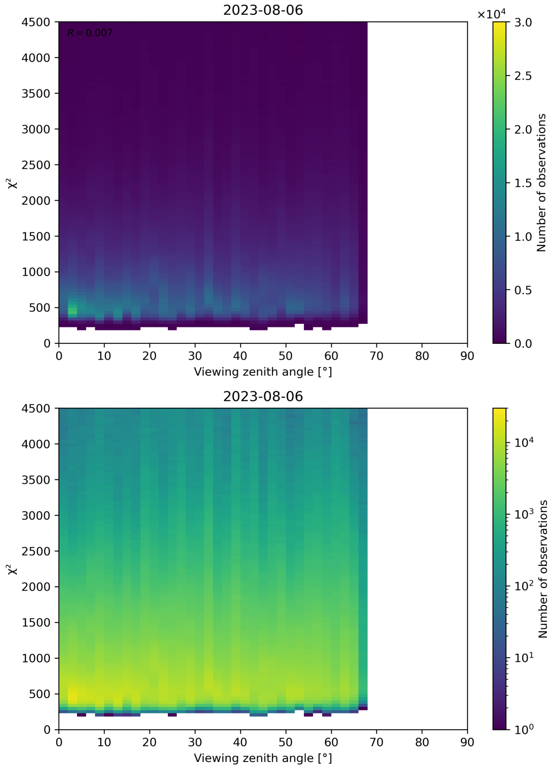
Figure 72: Scatter density plot of “Viewing zenith angle” against “ \chi^2 ” for 2023-08-05 to 2023-08-07.
