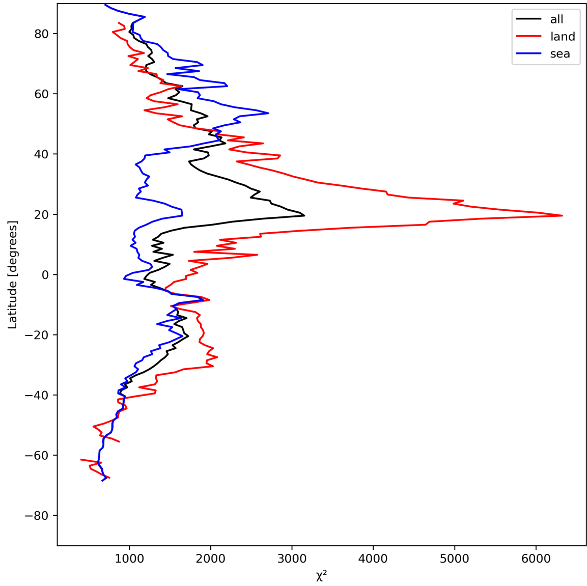
Figure 14: Zonal average of “ \chi^2 ” for 2023-08-05 to 2023-08-07.
