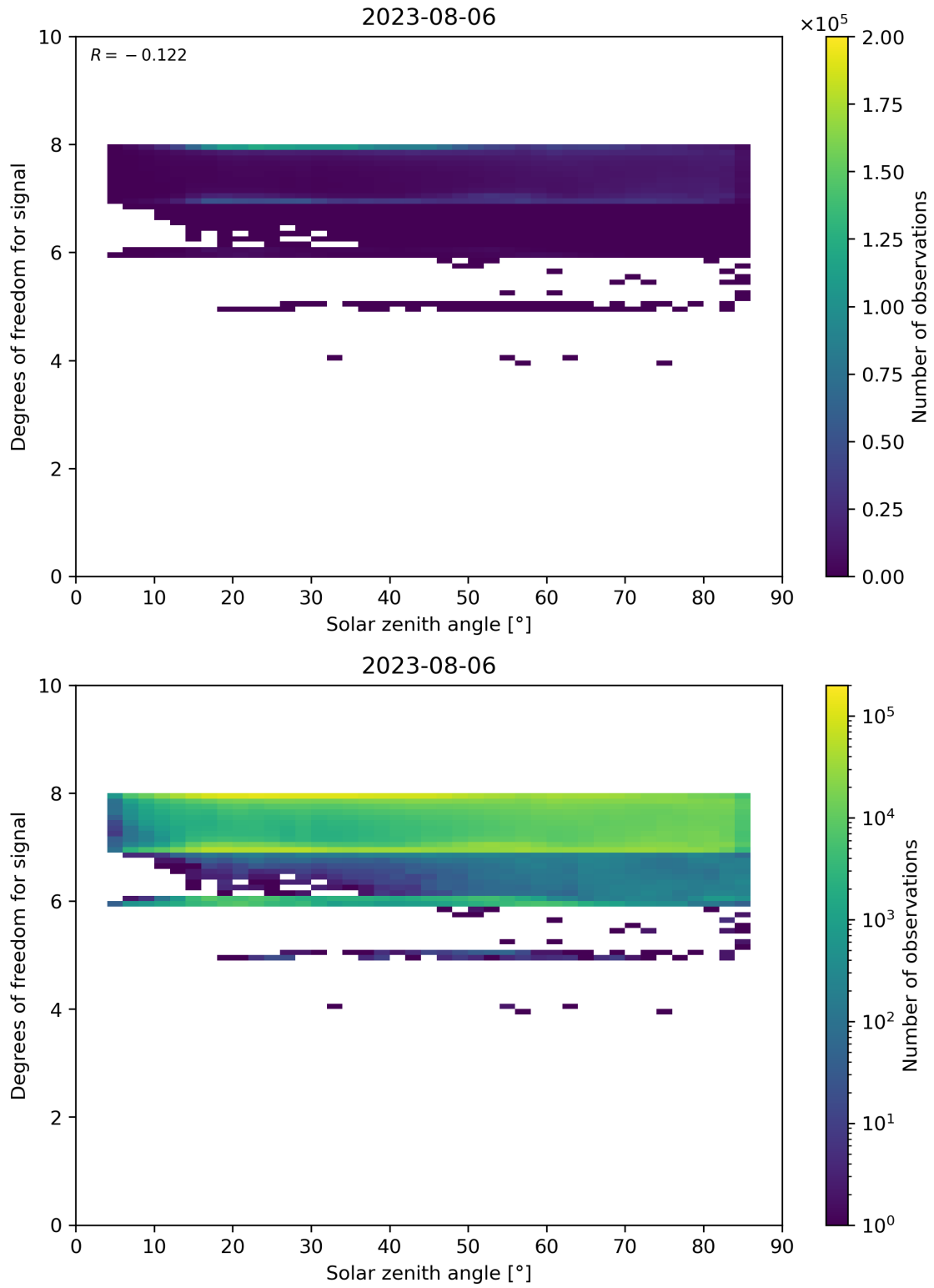
Figure 65: Scatter density plot of “Solar zenith angle” against “Degrees of freedom for signal” for 2023-08-05 to 2023-08-07.
