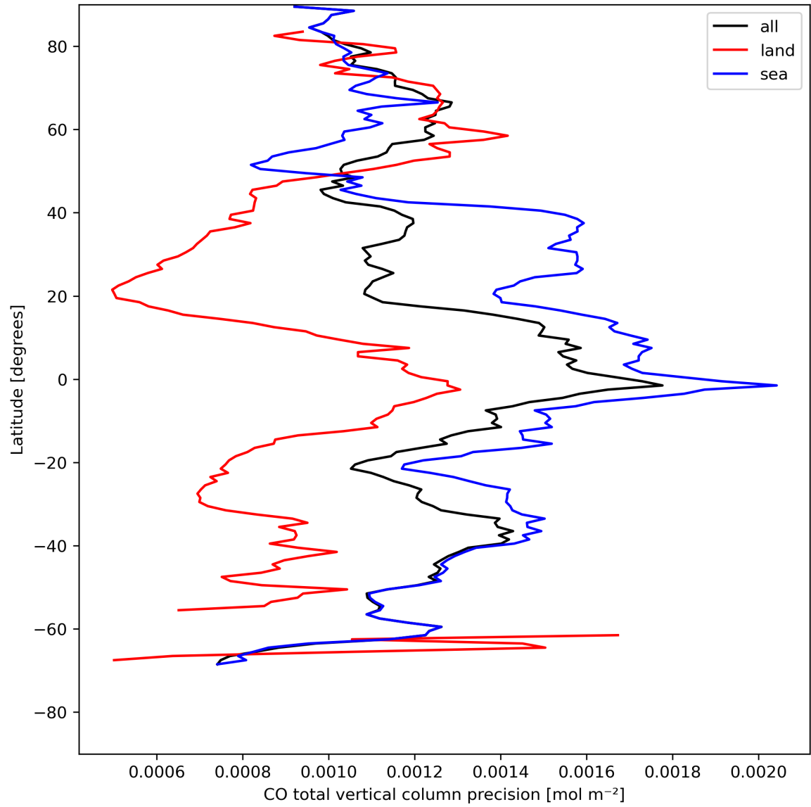
Figure 12: Zonal average of “CO total vertical column precision” for 2023-08-05 to 2023-08-07.
