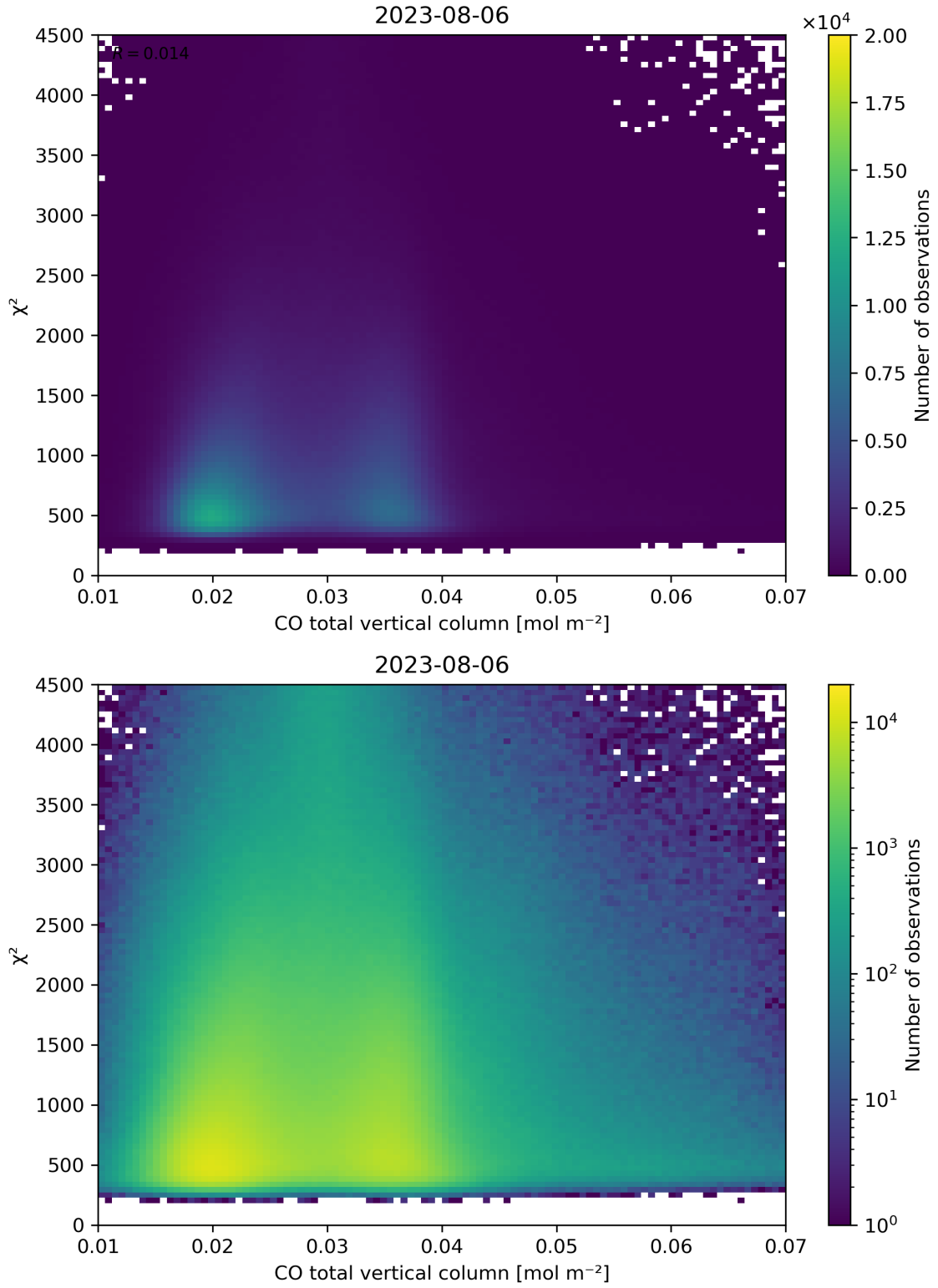
Figure 35: Scatter density plot of “CO total vertical column” against “ \chi^2 ” for 2023-08-05 to 2023-08-07.
