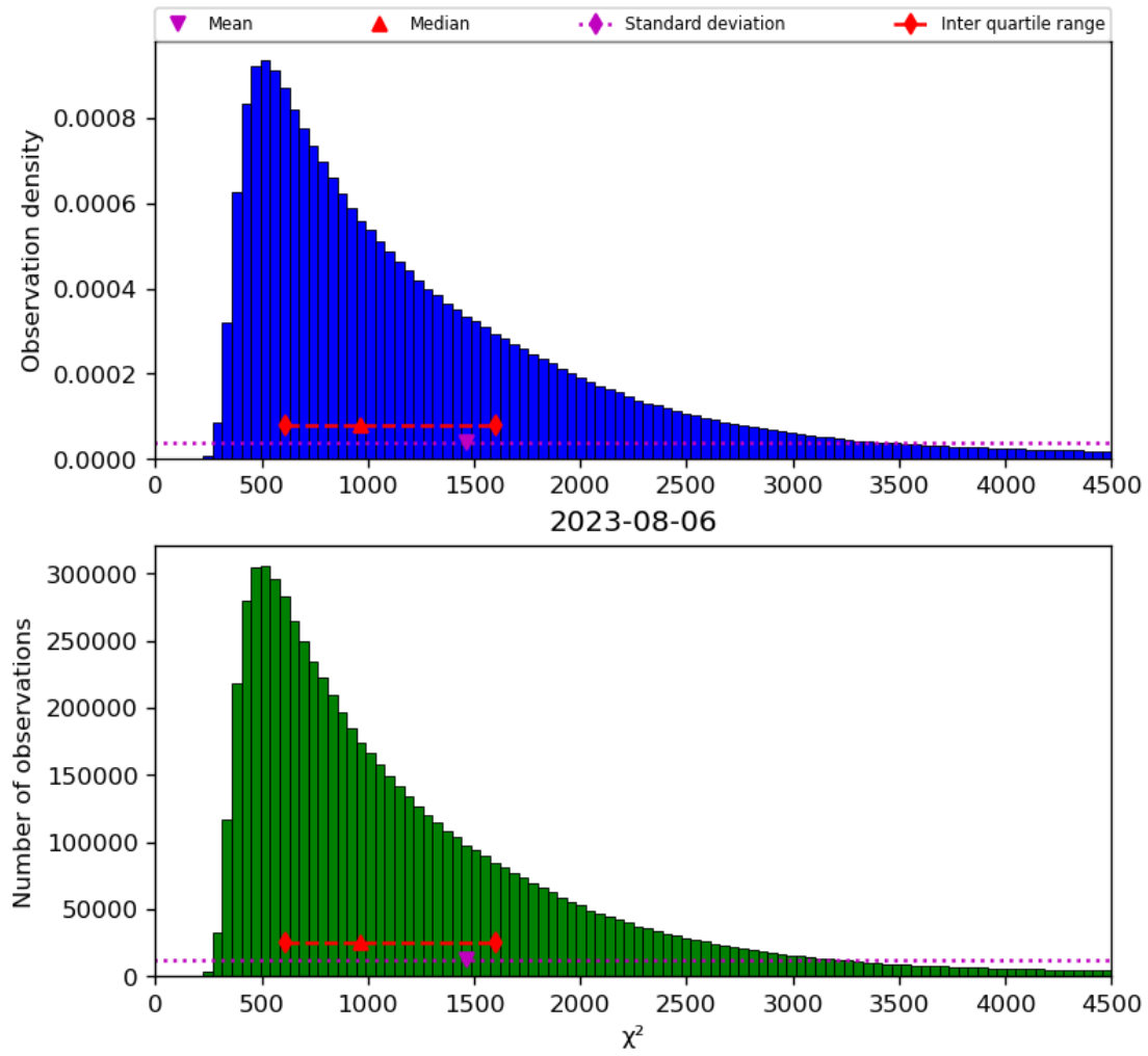
Figure 22: Histogram of “ \chi^2 ” for 2023-08-05 to 2023-08-07
