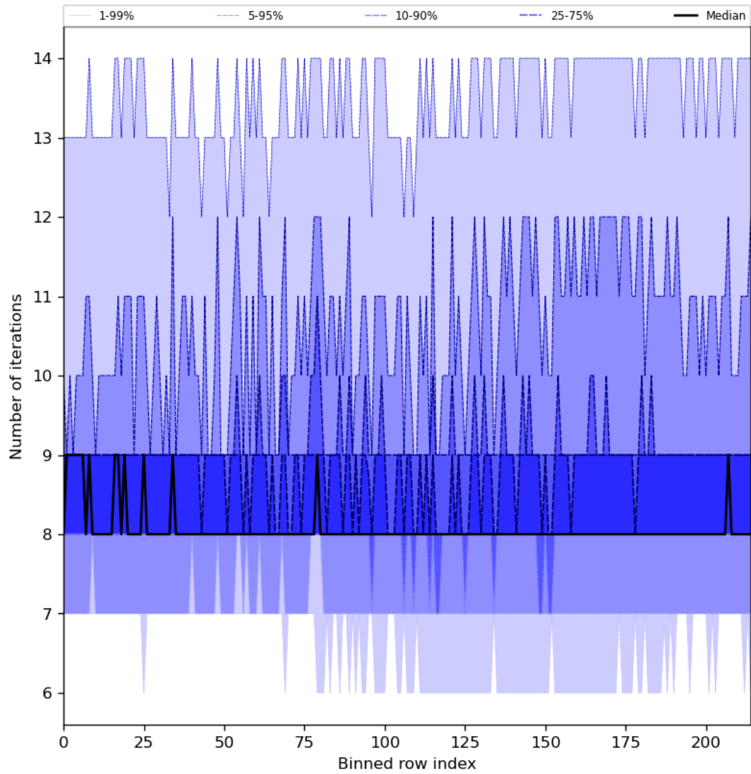
Figure 32: Along track statistics of “Number of iterations” for 2023-08-05 to 2023-08-07
