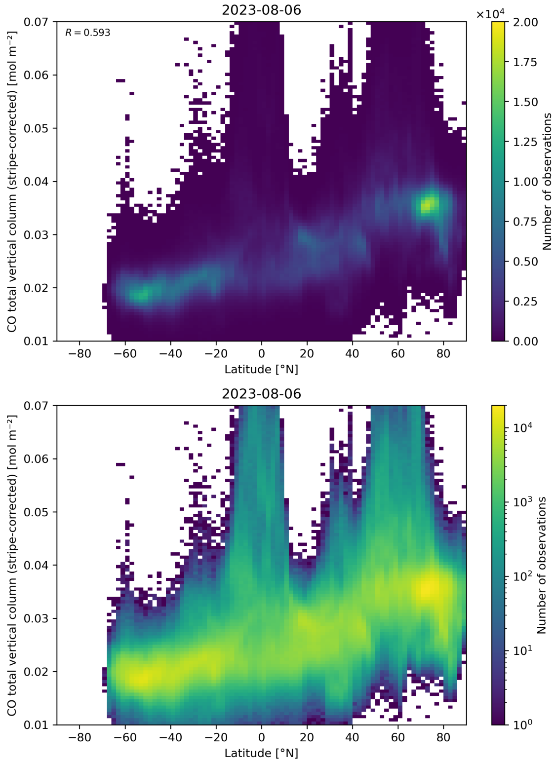
Figure 52: Scatter density plot of “Latitude” against “CO total vertical column (stripe-corrected)” for 2023-08-05 to 2023-08-07.
