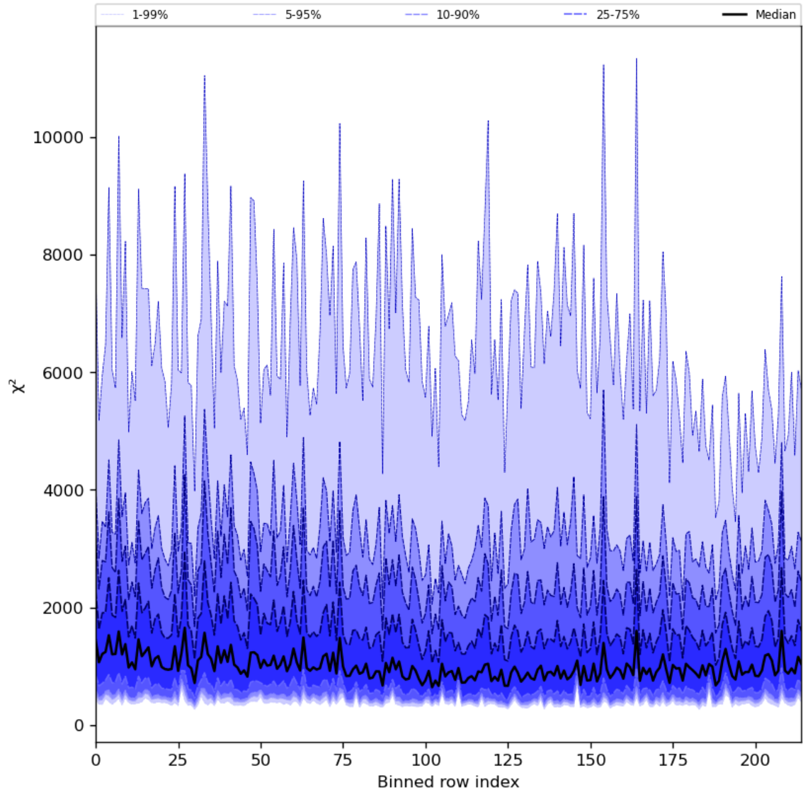
Figure 30: Along track statistics of “ \chi^2 ” for 2023-08-05 to 2023-08-07
