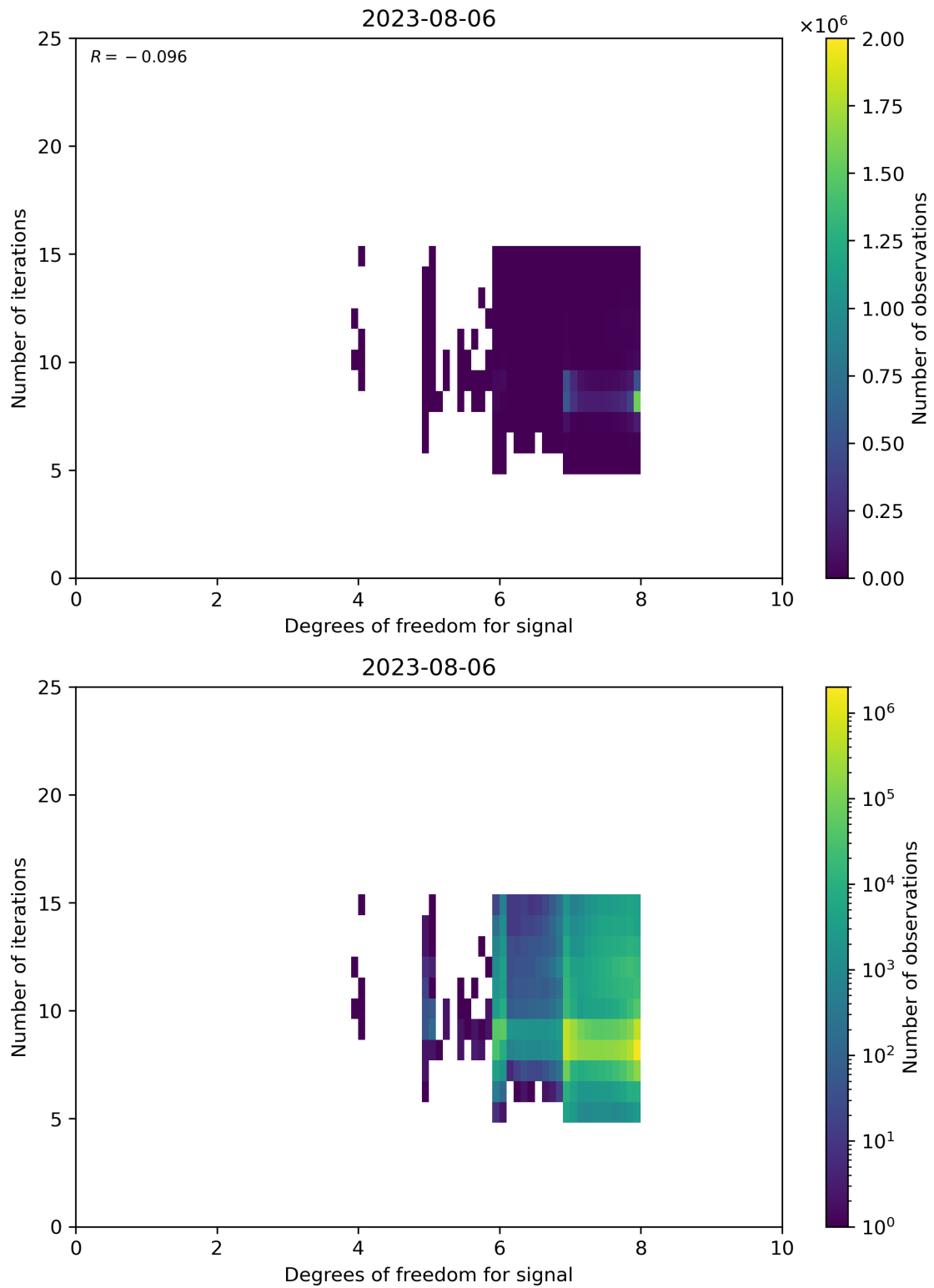
Figure 50: Scatter density plot of “Degrees of freedom for signal” against “Number of iterations” for 2023-08-05 to 2023-08-07.
