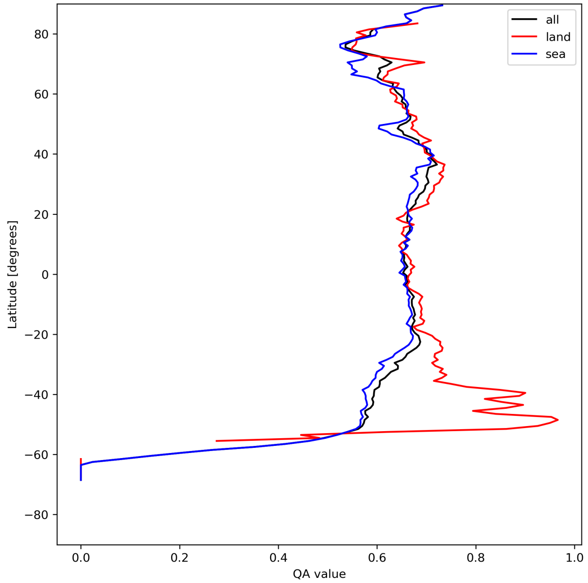
Figure 9: Zonal average of “QA value” for 2023-08-05 to 2023-08-07.
