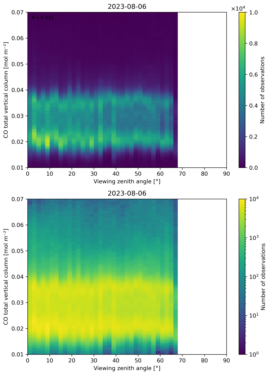
Figure 69: Scatter density plot of “Viewing zenith angle” against “CO total vertical column” for 2023-08-05 to 2023-08-07.
