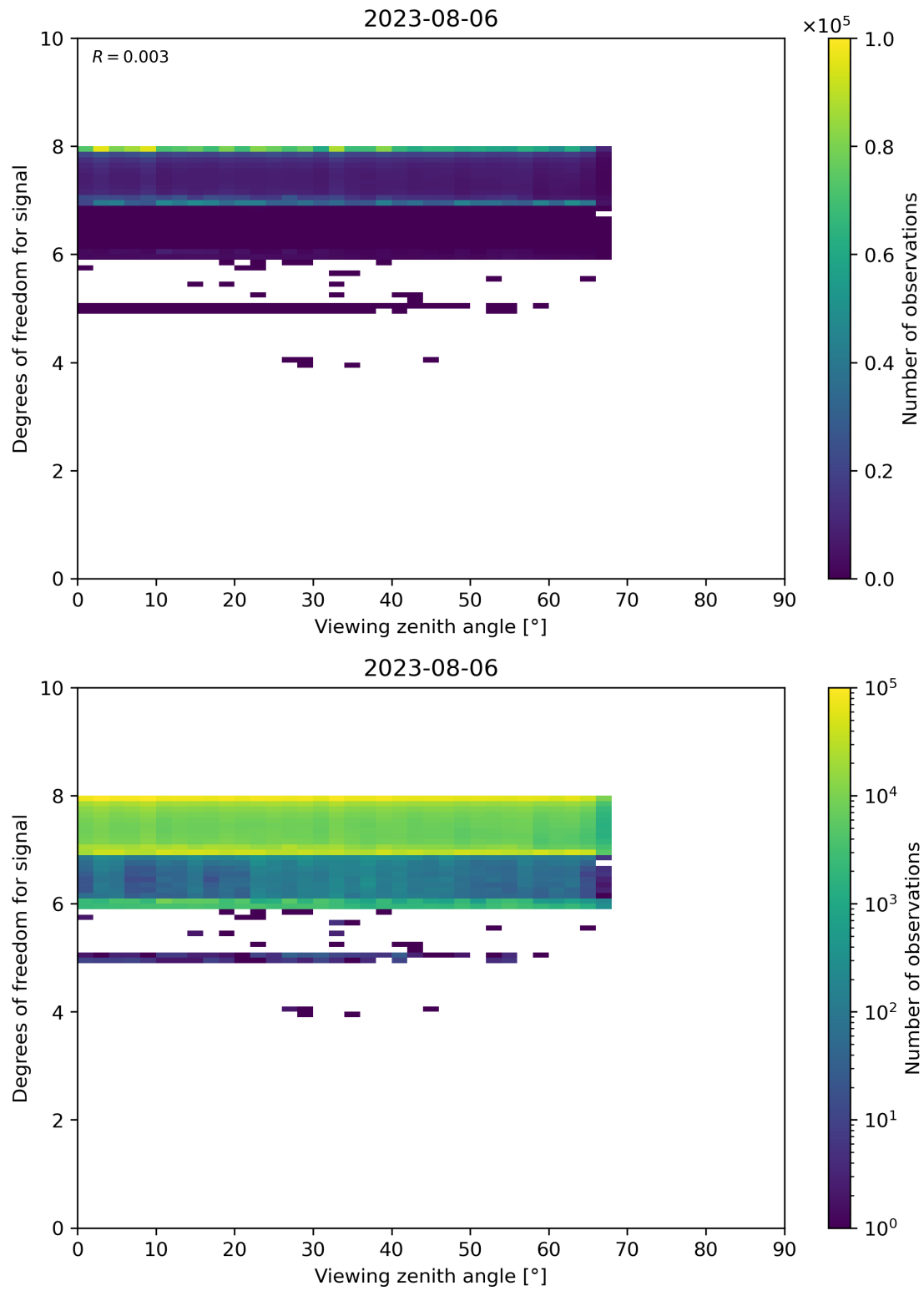
Figure 73: Scatter density plot of “Viewing zenith angle” against “Degrees of freedom for signal” for 2023-08-05 to 2023-08-07.
