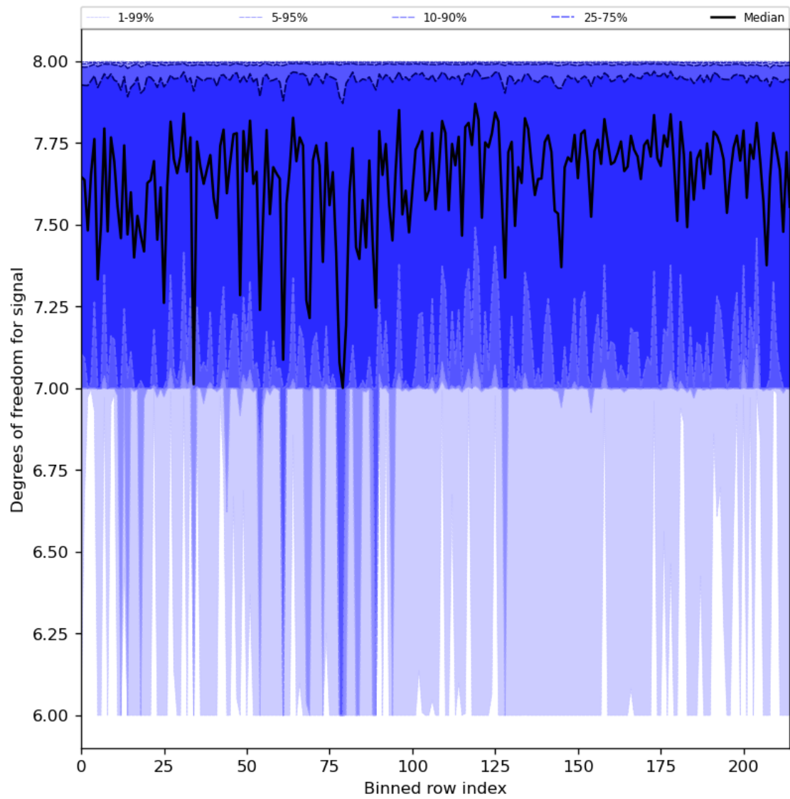
Figure 31: Along track statistics of “Degrees of freedom for signal” for 2023-08-05 to 2023-08-07
