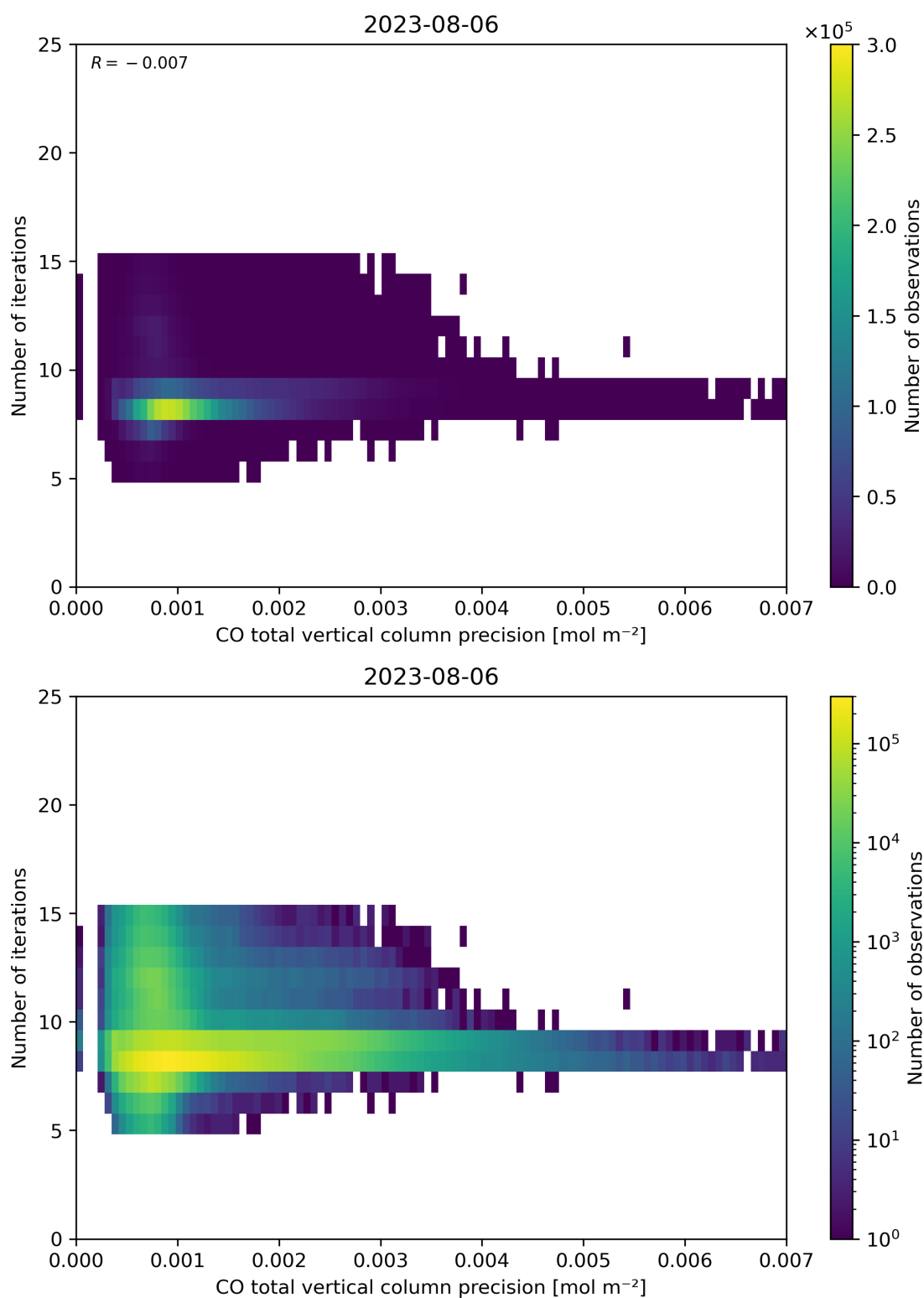
Figure 46: Scatter density plot of “CO total vertical column precision” against “Number of iterations” for 2023-08-05 to 2023-08-07.
