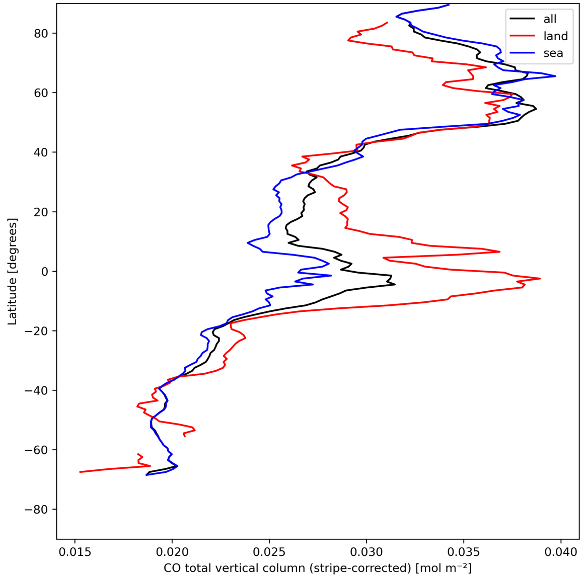
Figure 11: Zonal average of “CO total vertical column (stripe-corrected)” for 2023-08-05 to 2023-08-07.
