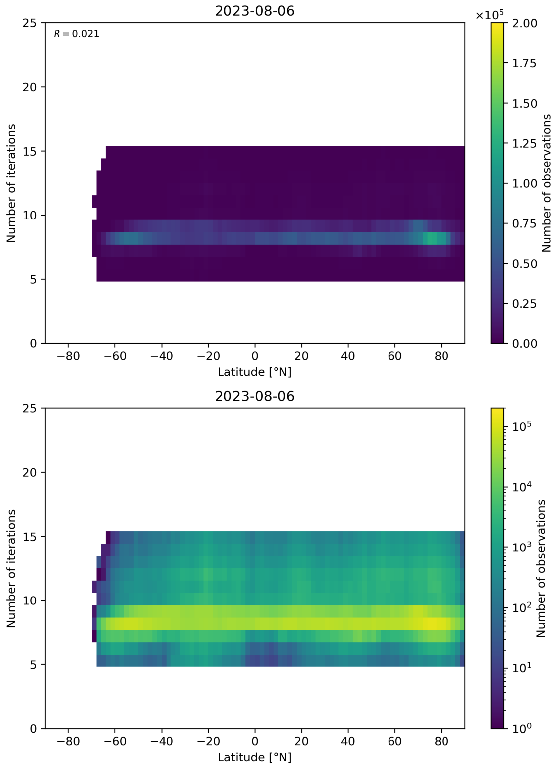
Figure 56: Scatter density plot of “Latitude” against “Number of iterations” for 2023-08-05 to 2023-08-07.
