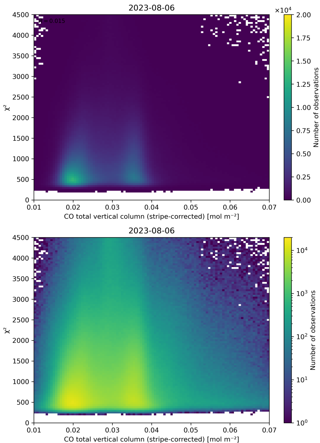
Figure 37: Scatter density plot of “CO total vertical column (stripe-corrected)” against “ \chi^2 ” for 2023-08-05 to 2023-08-07.
