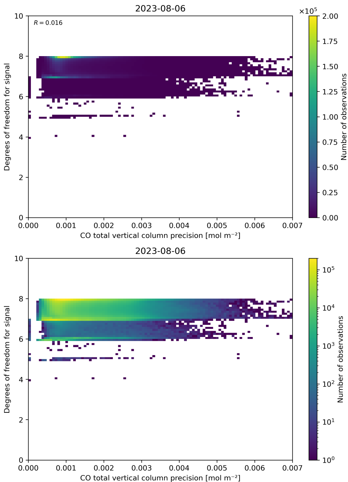
Figure 45: Scatter density plot of “CO total vertical column precision” against “Degrees of freedom for signal” for 2023-08-05 to 2023-08-07.
