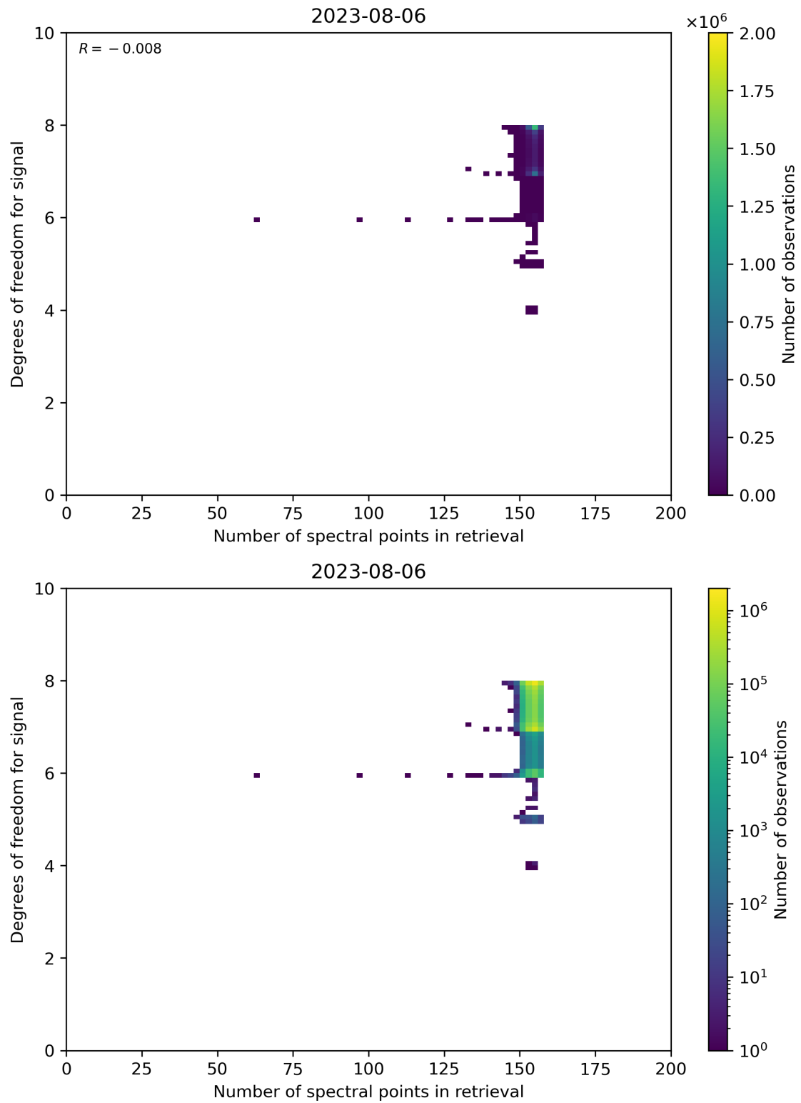
Figure 59: Scatter density plot of “Number of spectral points in retrieval” against “Degrees of freedom for signal” for 2023-08-05 to 2023-08-07.
