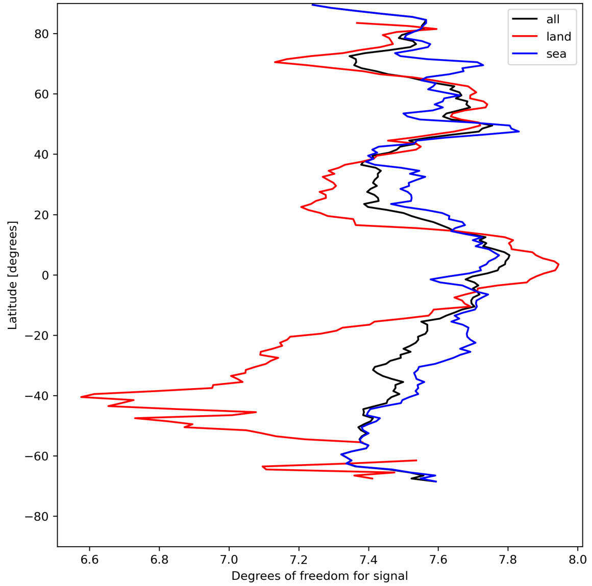
Figure 15: Zonal average of “Degrees of freedom for signal” for 2023-08-05 to 2023-08-07.
