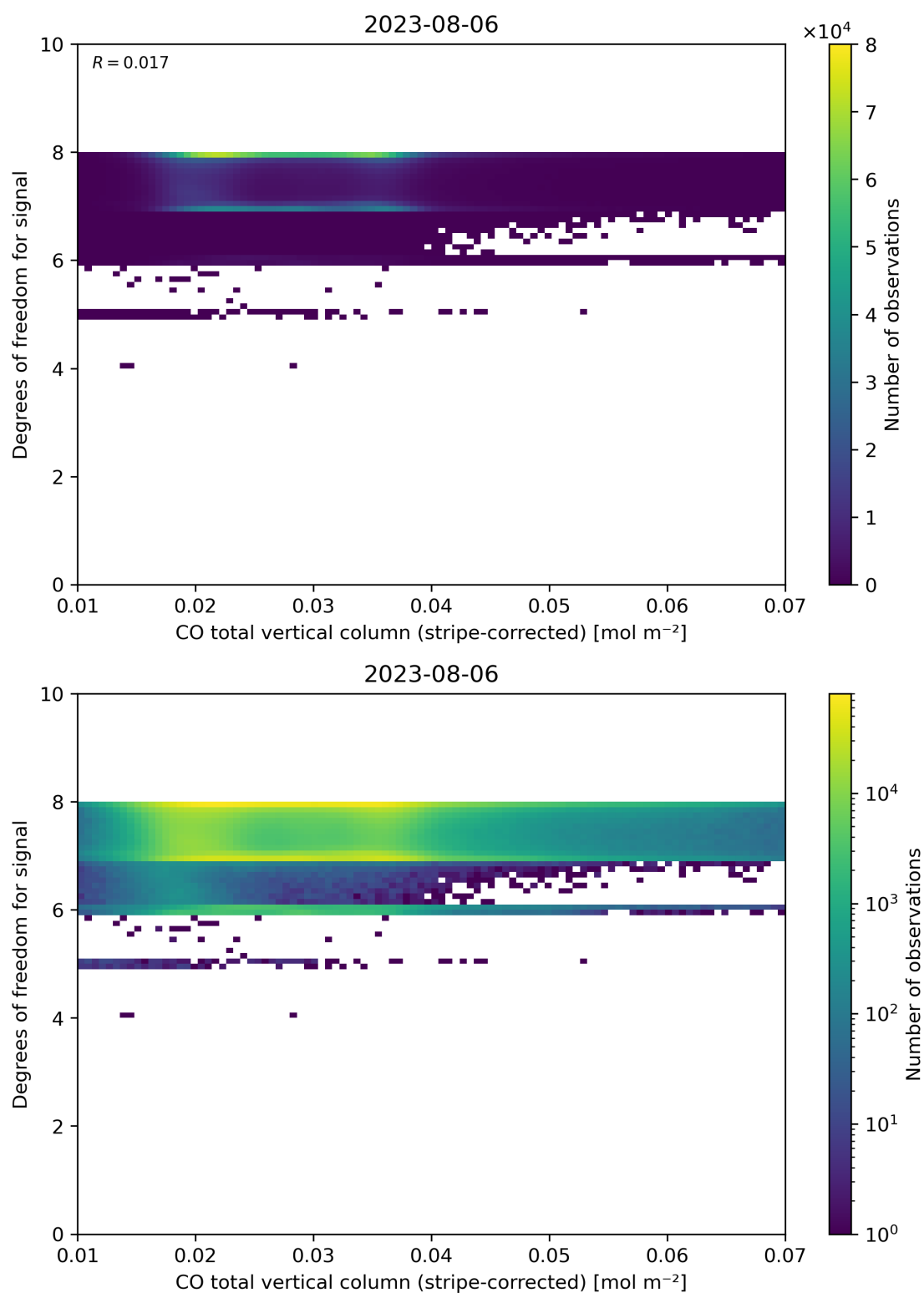
Figure 38: Scatter density plot of “CO total vertical column (stripe-corrected)” against “Degrees of freedom for signal” for 2023-08-05 to 2023-08-07.
