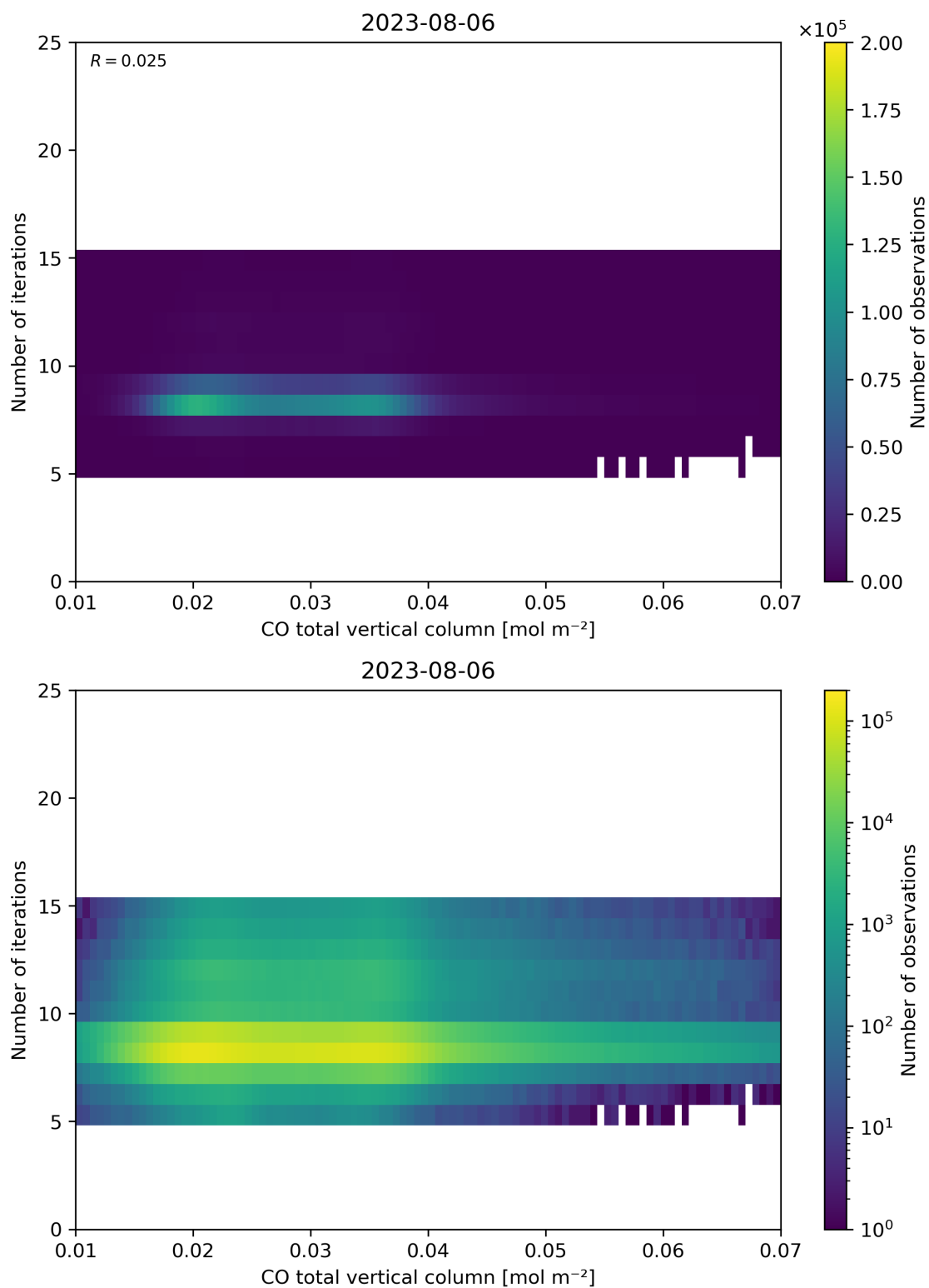
Figure 42: Scatter density plot of “CO total vertical column” against “Number of iterations” for 2023-08-05 to 2023-08-07.
