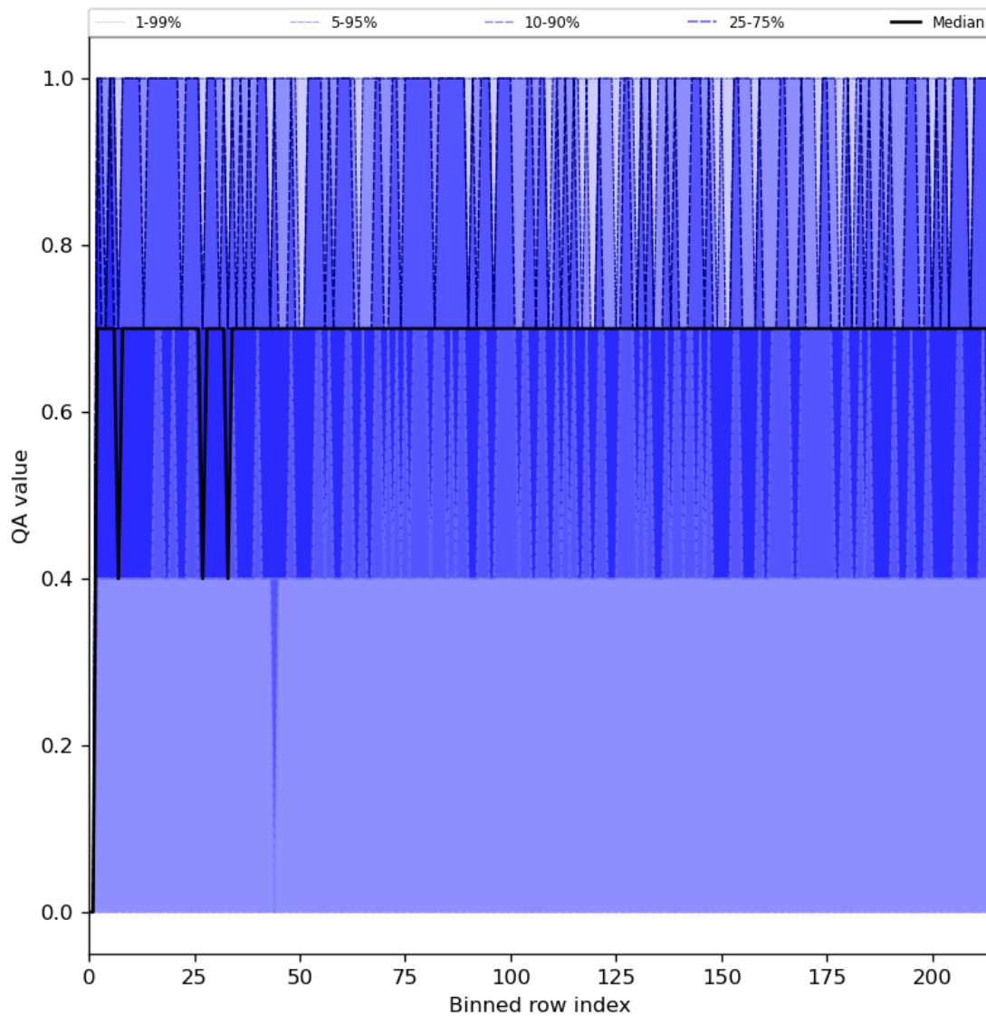
Figure 25: Along track statistics of “QA value” for 2023-08-05 to 2023-08-07
