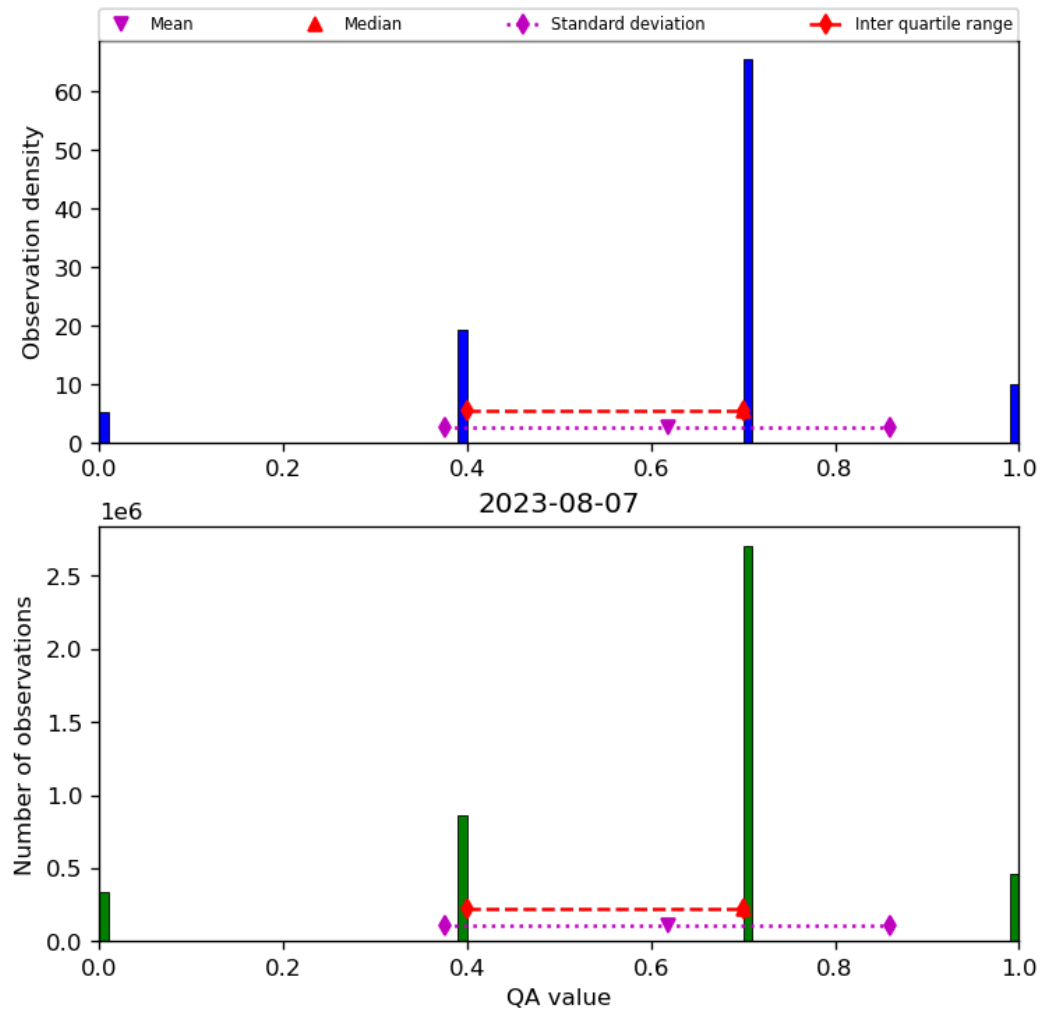
Figure 17: Histogram of “QA value” for 2023-08-06 to 2023-08-08
