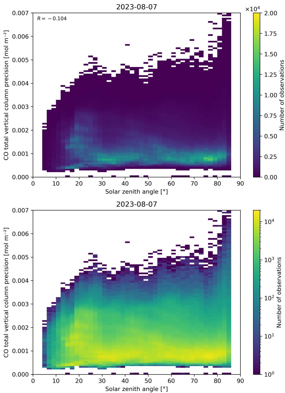
Figure 63: Scatter density plot of “Solar zenith angle” against “CO total vertical column precision” for 2023-08-06 to 2023-08-08.
