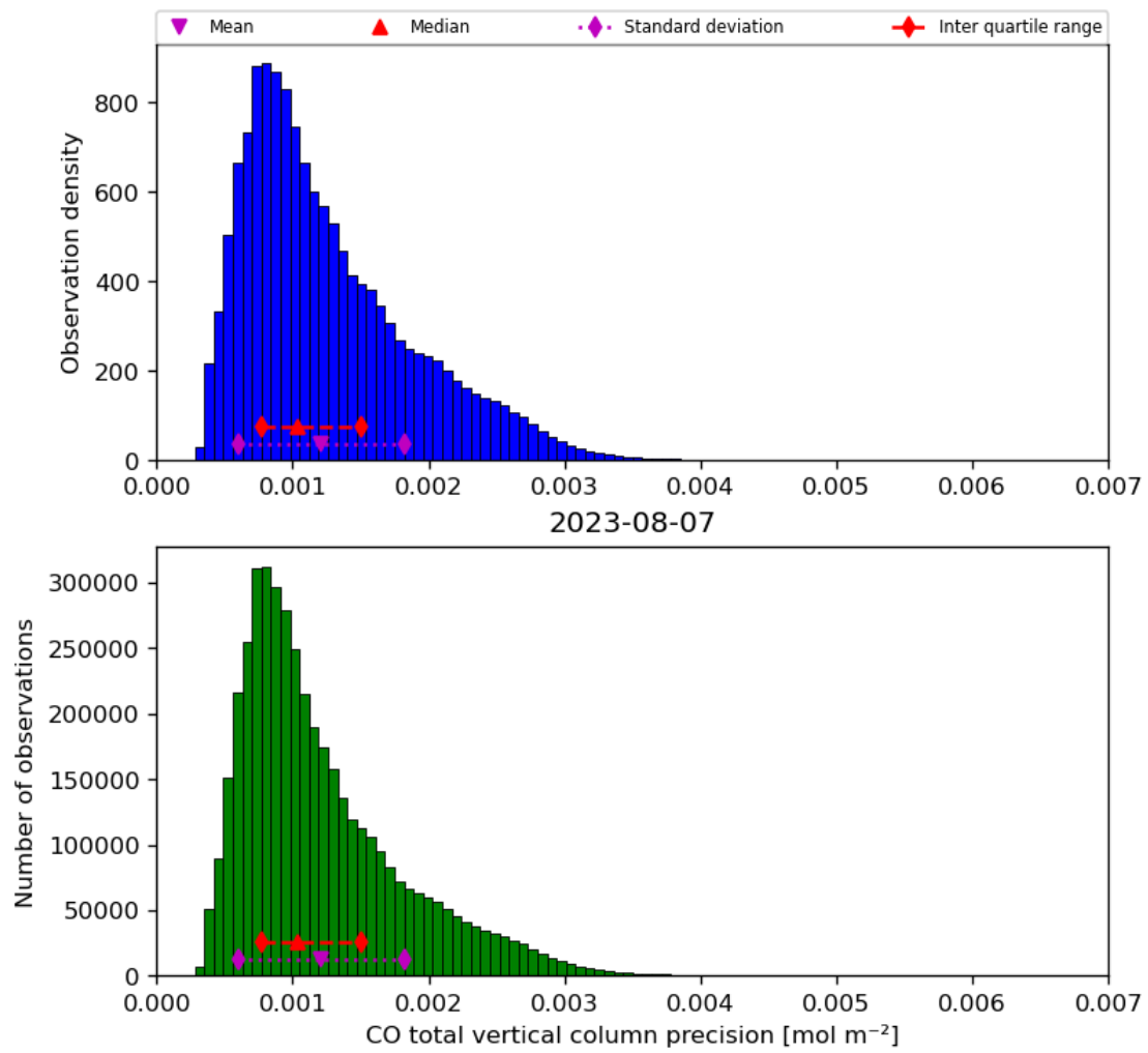
Figure 20: Histogram of “CO total vertical column precision” for 2023-08-06 to 2023-08-08
