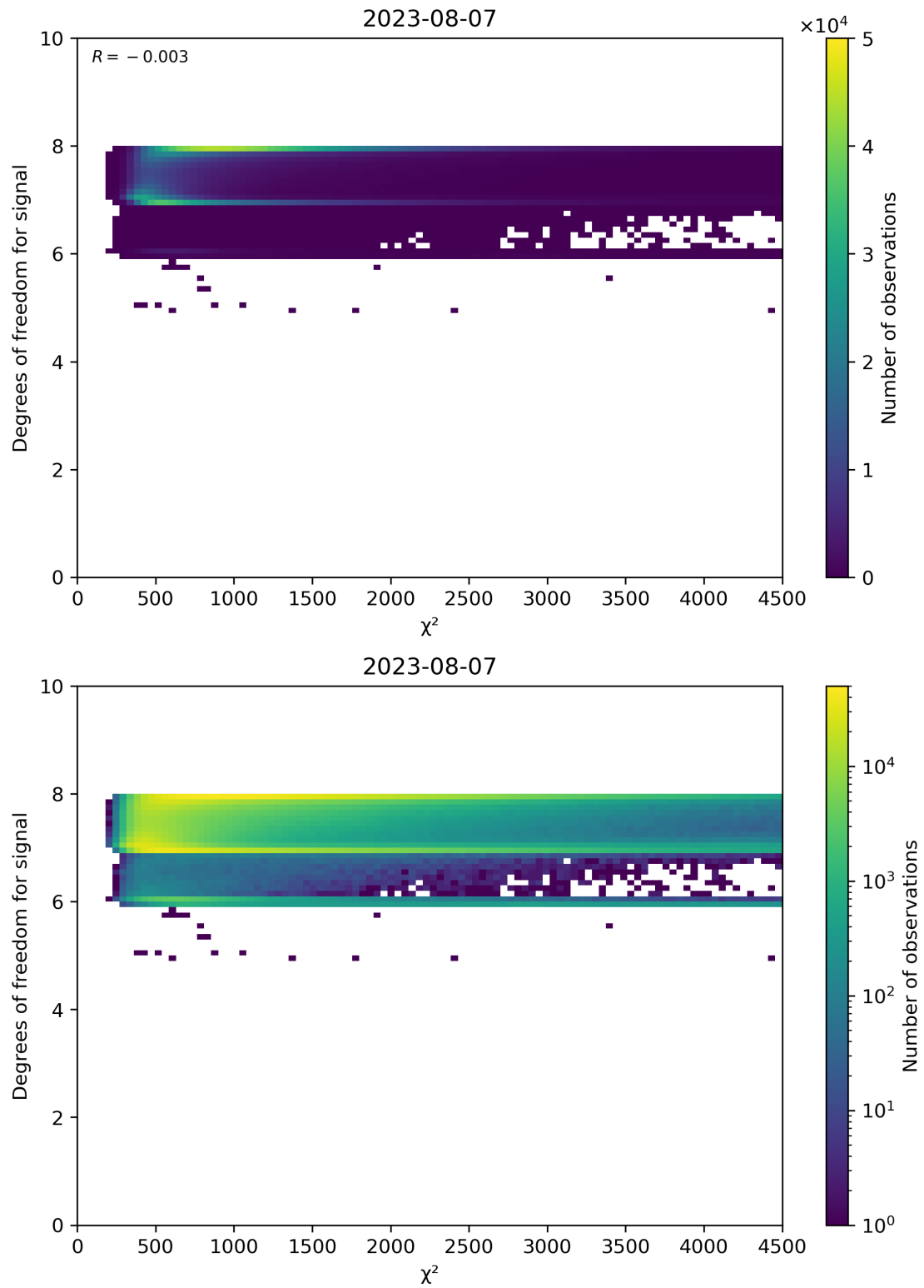
Figure 48: Scatter density plot of “ \chi^2 ” against “Degrees of freedom for signal” for 2023-08-06 to 2023-08-08.
