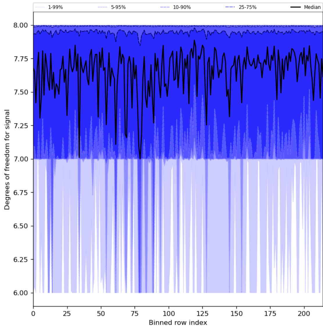
Figure 31: Along track statistics of “Degrees of freedom for signal” for 2023-08-06 to 2023-08-08
