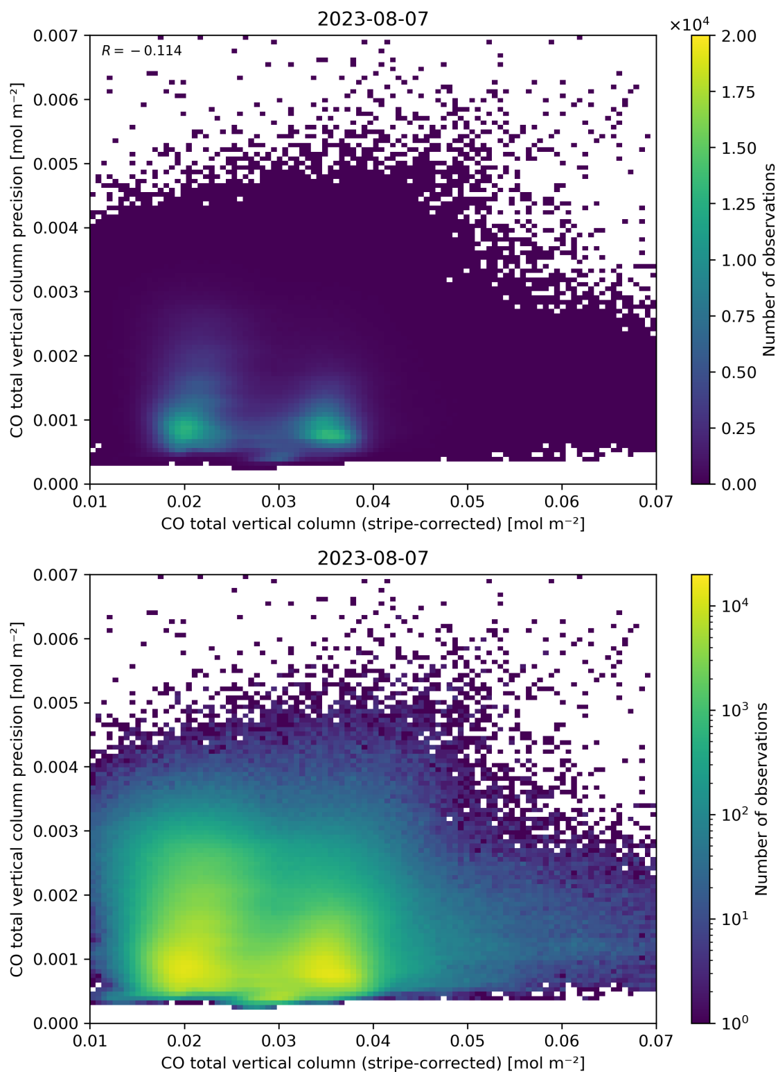
Figure 36: Scatter density plot of “CO total vertical column (stripe-corrected)” against “CO total vertical column precision” for 2023-08-06 to 2023-08-08.
