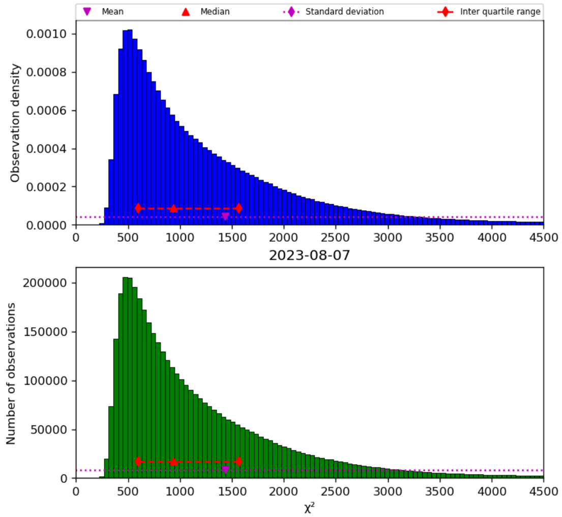
Figure 22: Histogram of “ \chi^2 ” for 2023-08-06 to 2023-08-08
