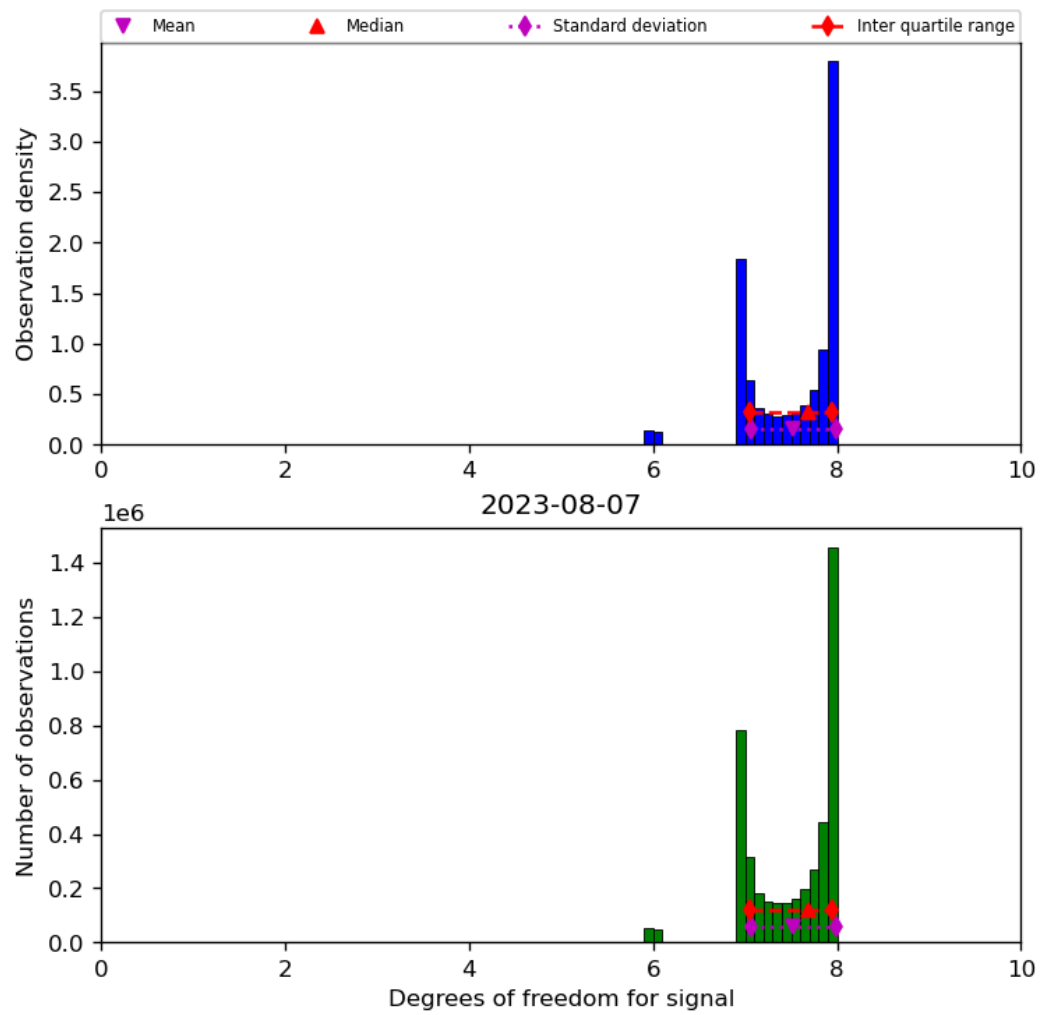
Figure 23: Histogram of “Degrees of freedom for signal” for 2023-08-06 to 2023-08-08
