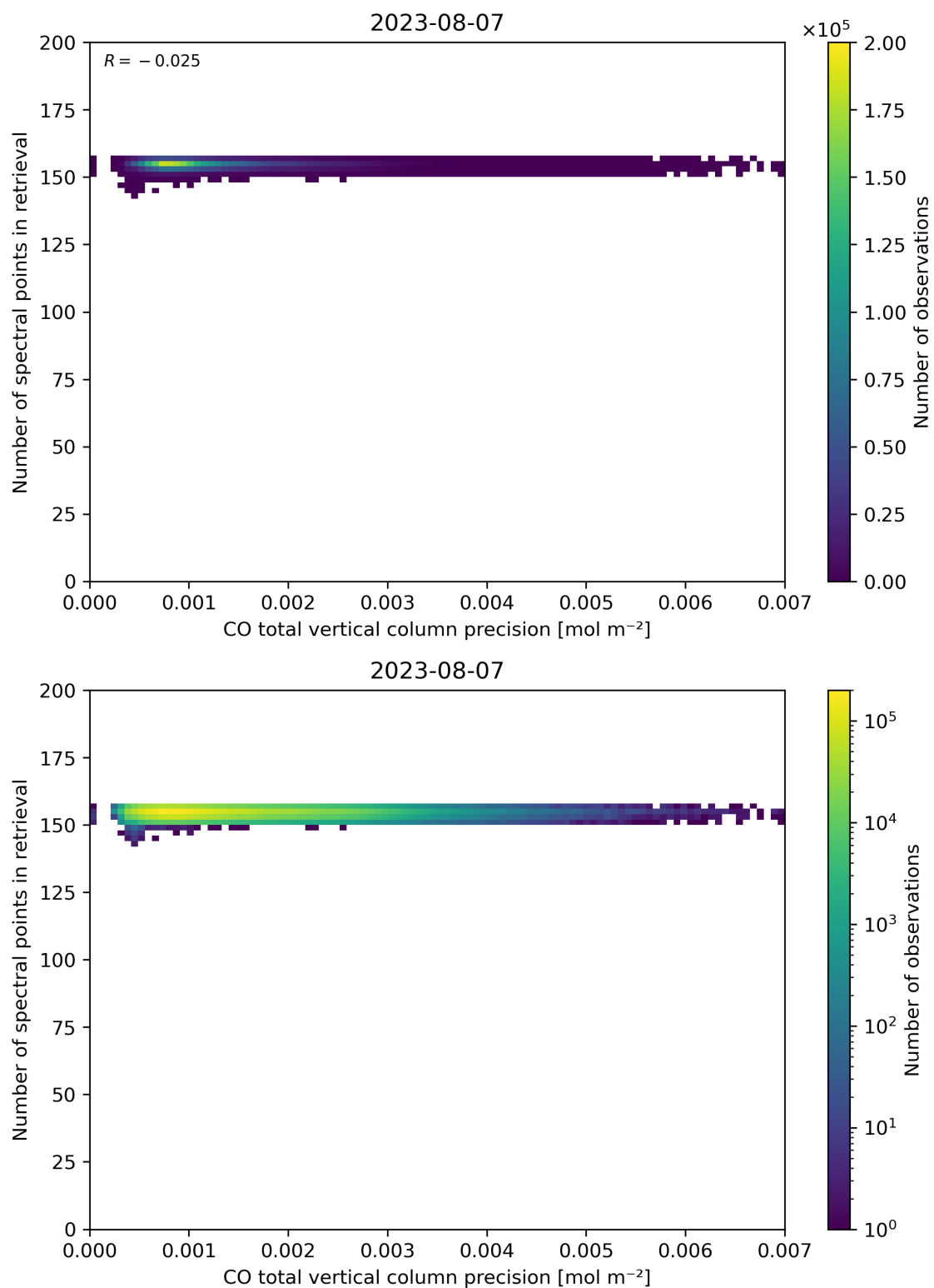
Figure 47: Scatter density plot of “CO total vertical column precision” against “Number of spectral points in retrieval” for 2023-08-06 to 2023-08-08.
