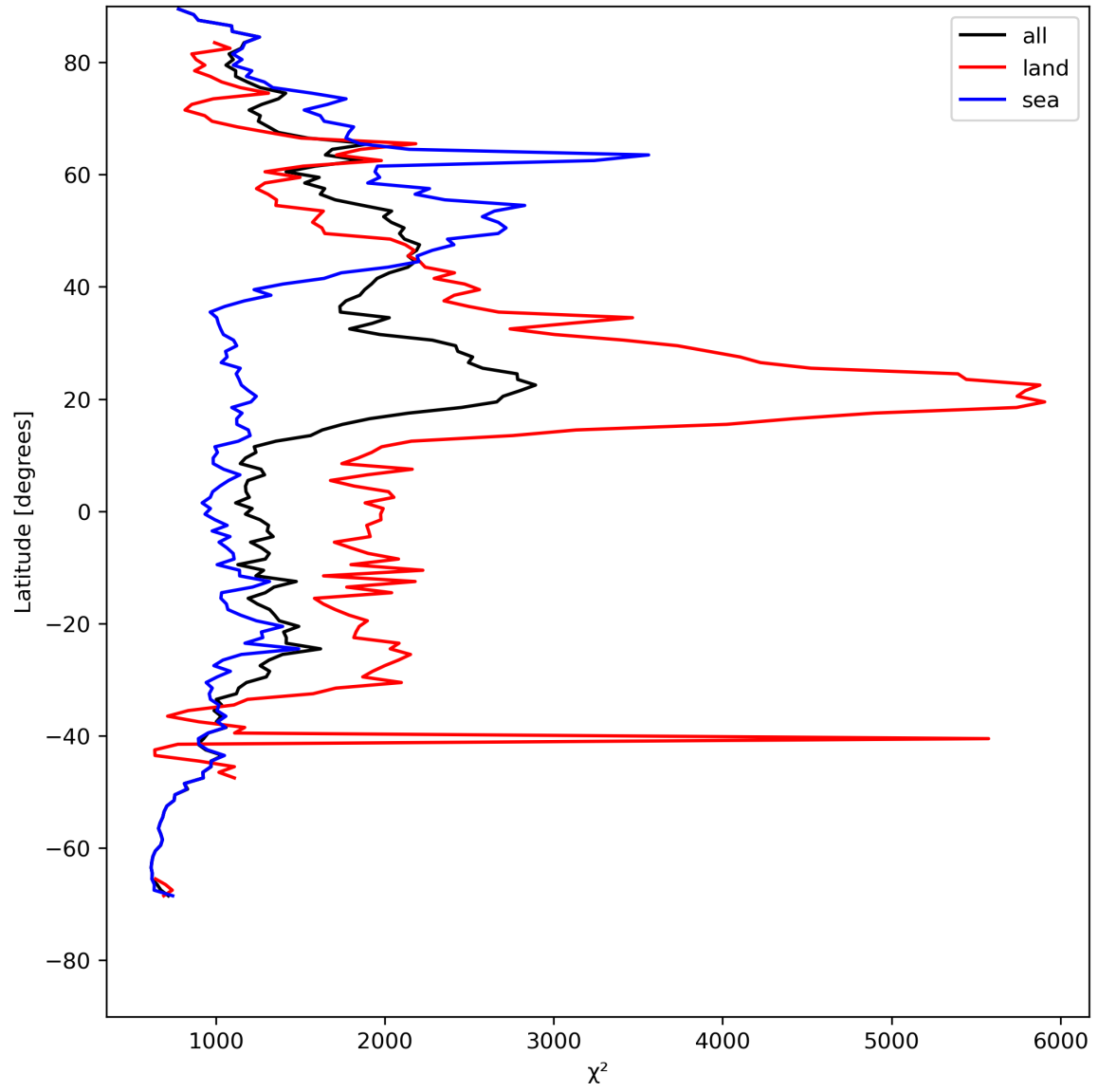
Figure 14: Zonal average of “ \chi^2 ” for 2023-08-06 to 2023-08-08.
