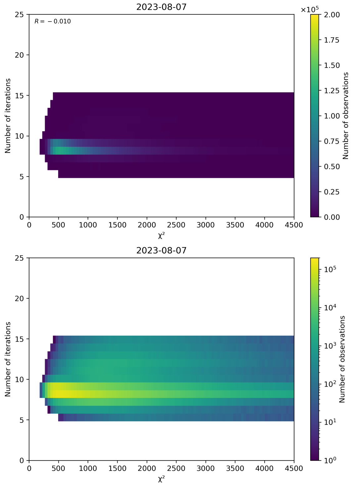
Figure 49: Scatter density plot of “ \chi^2 ” against “Number of iterations” for 2023-08-06 to 2023-08-08.
