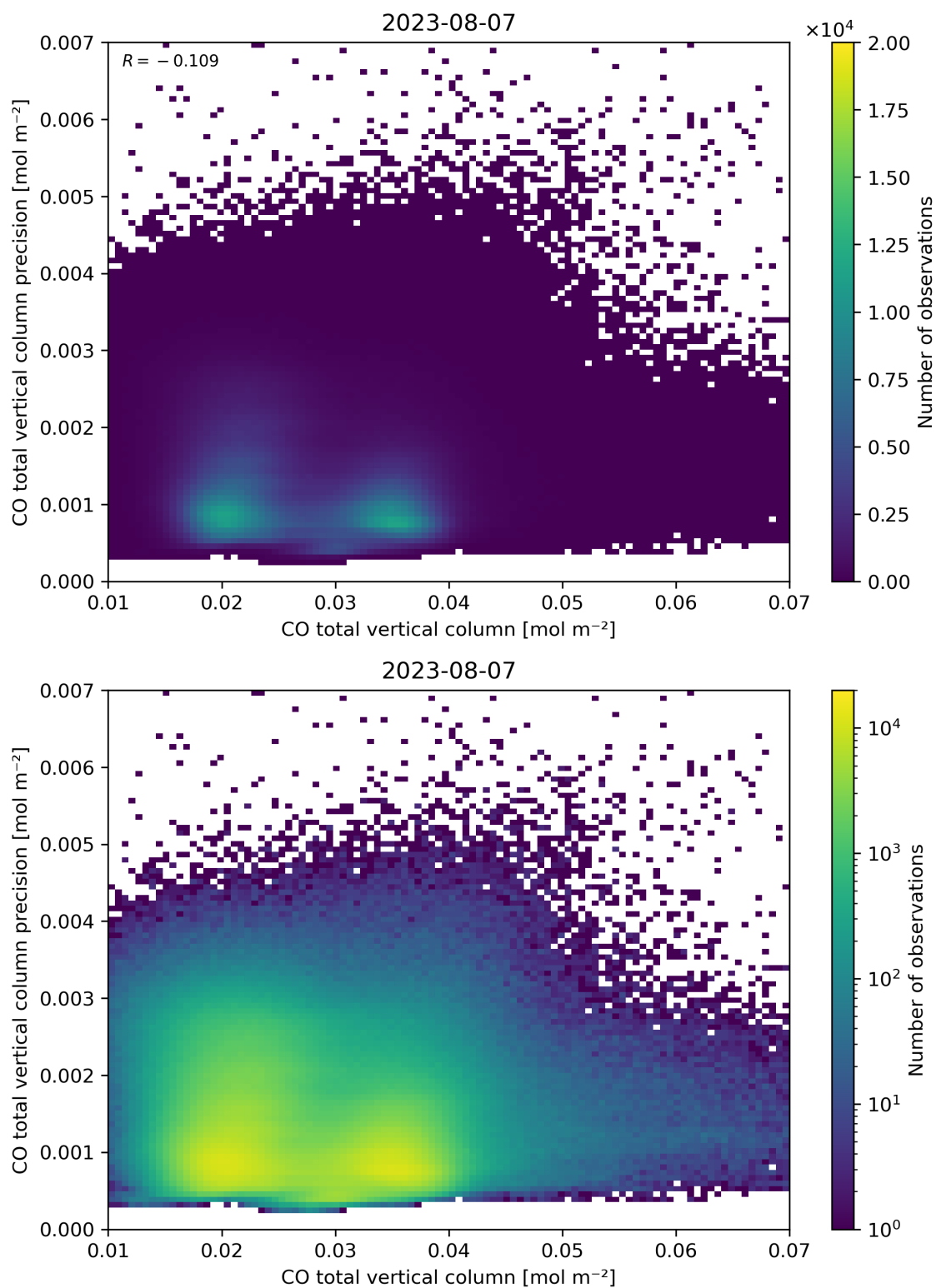
Figure 34: Scatter density plot of “CO total vertical column” against “CO total vertical column precision” for 2023-08-06 to 2023-08-08.
