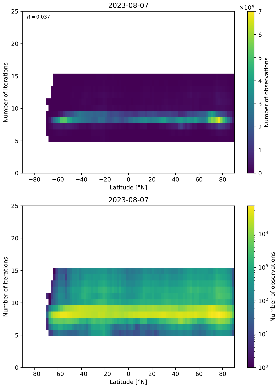
Figure 56: Scatter density plot of “Latitude” against “Number of iterations” for 2023-08-06 to 2023-08-08.
