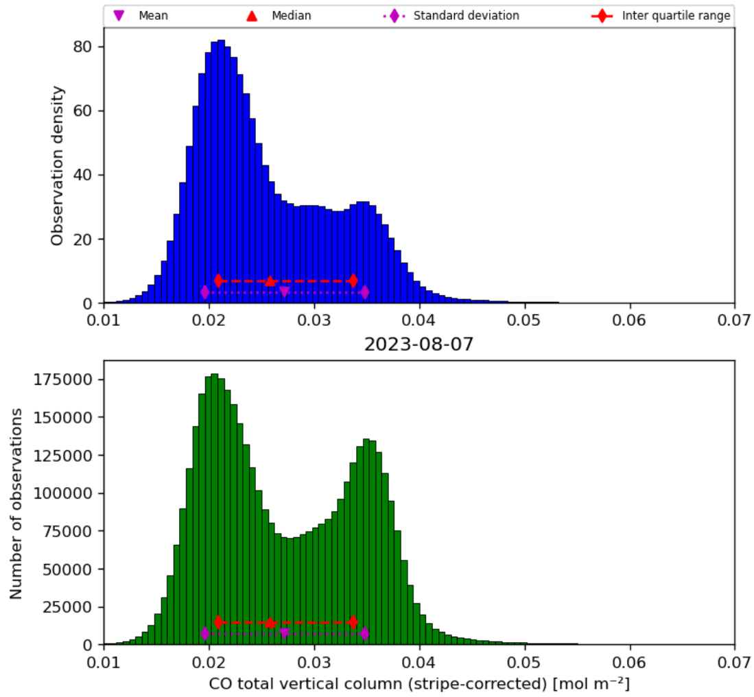
Figure 19: Histogram of “CO total vertical column (stripe-corrected)” for 2023-08-06 to 2023-08-08
