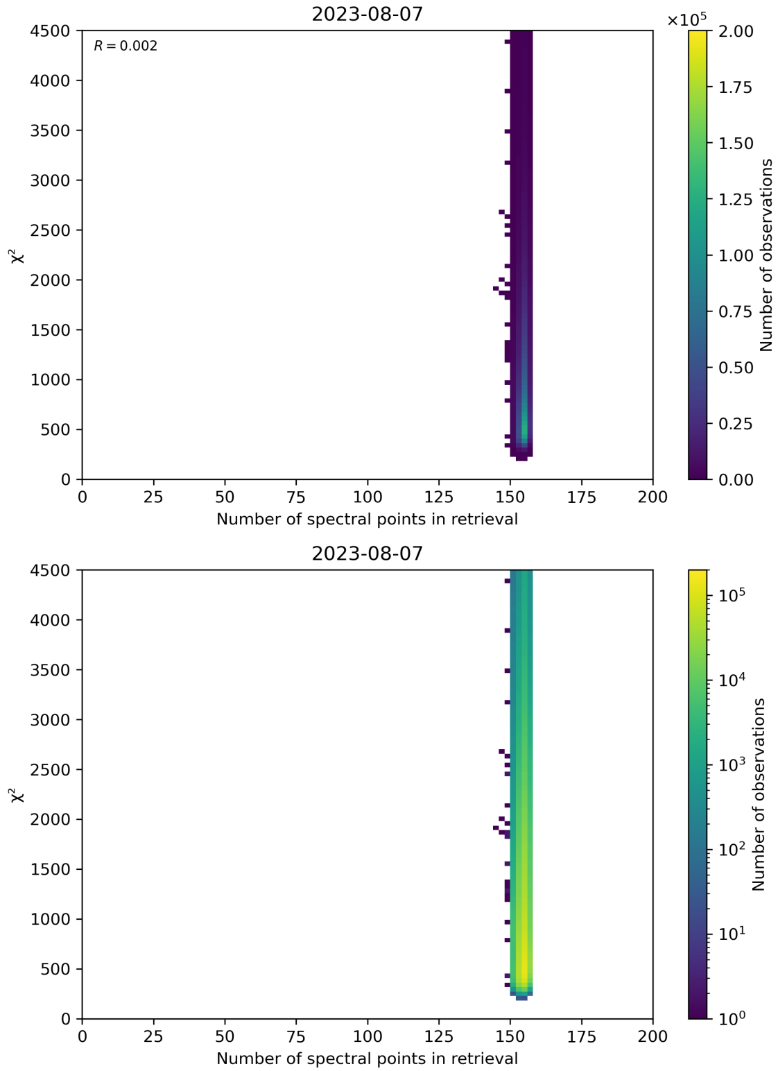
Figure 58: Scatter density plot of “Number of spectral points in retrieval” against “ \chi^2 ” for 2023-08-06 to 2023-08-08.
