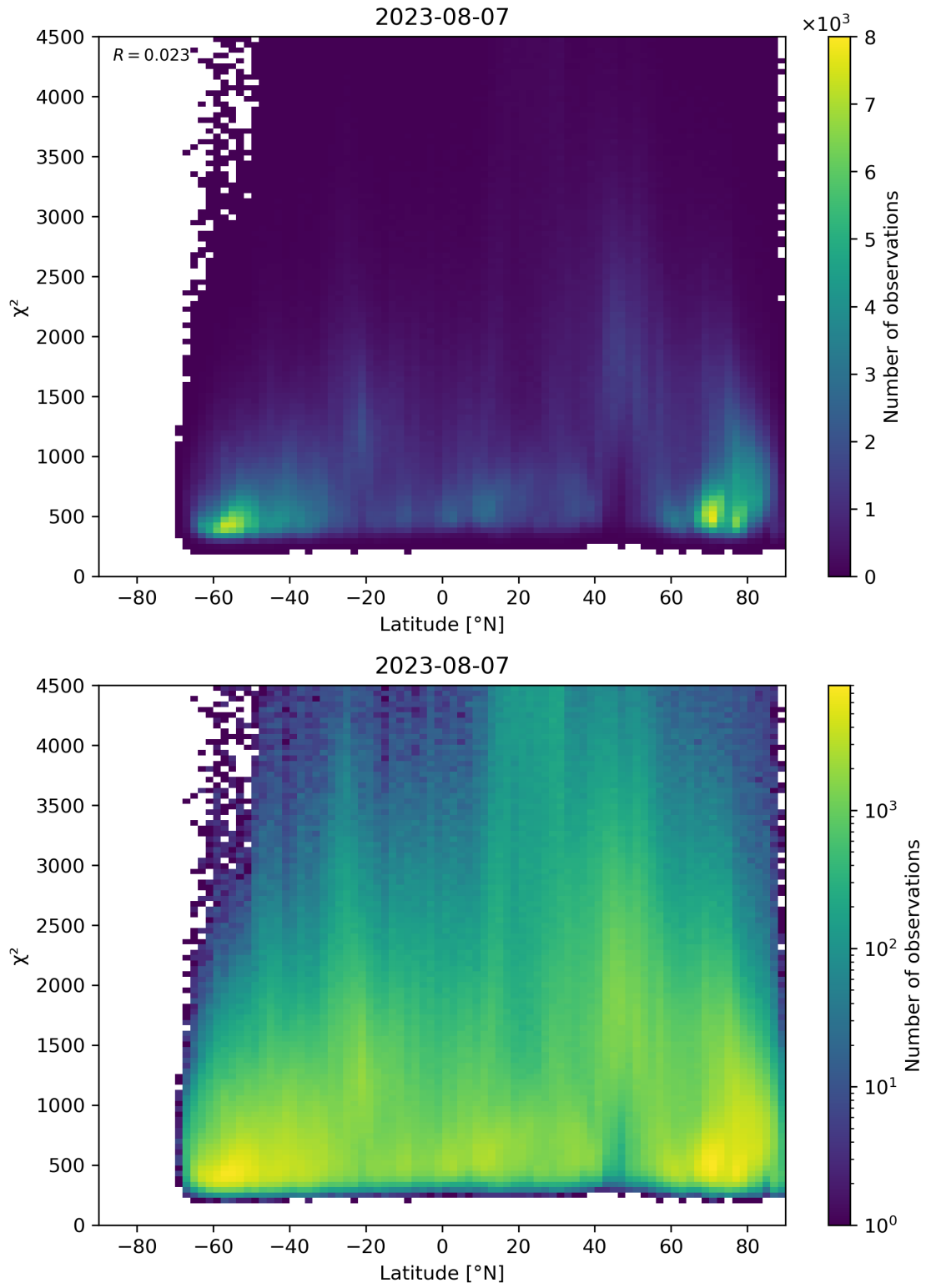
Figure 54: Scatter density plot of “Latitude” against “ \chi^2 ” for 2023-08-06 to 2023-08-08.
