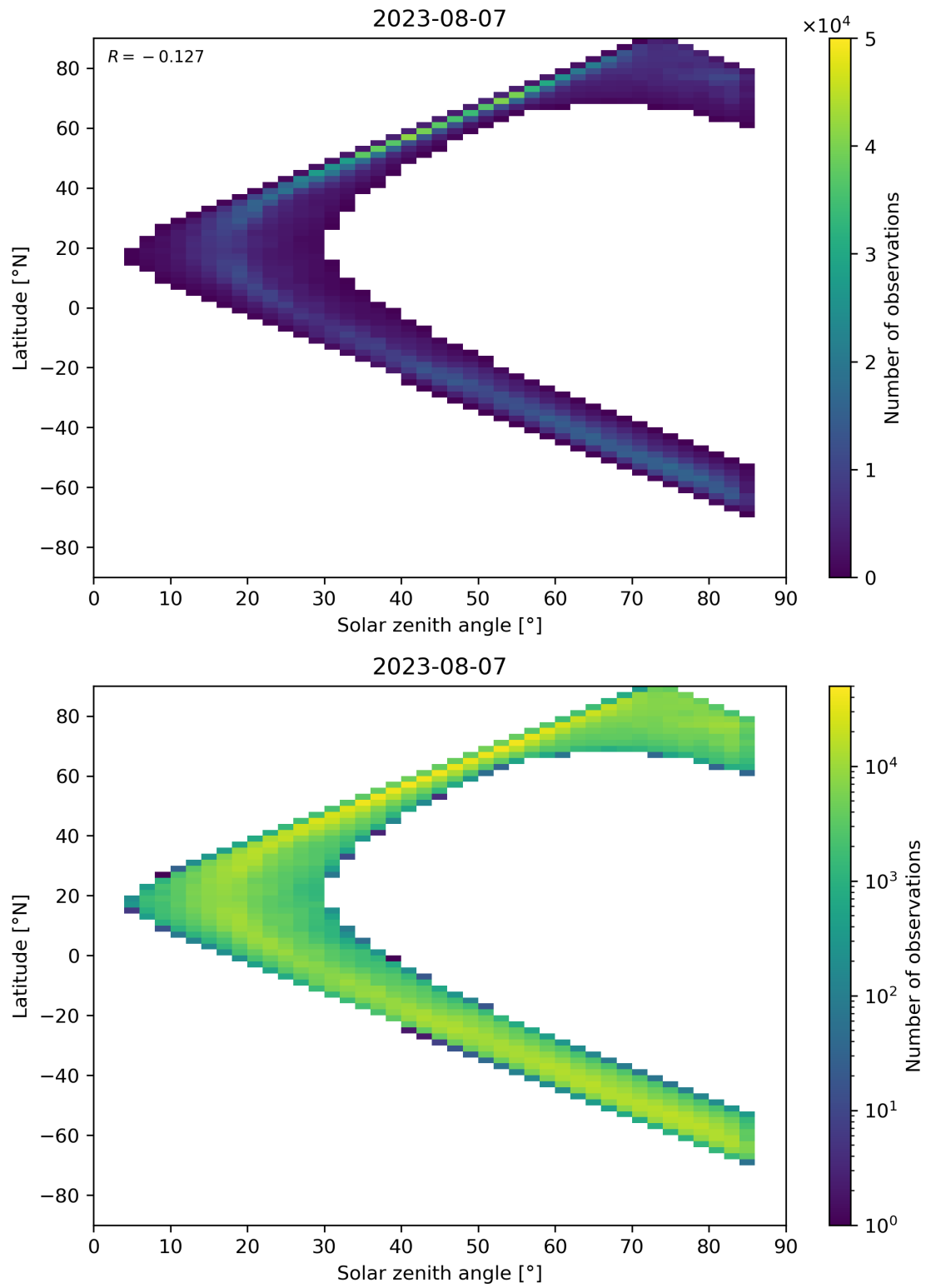
Figure 66: Scatter density plot of “Solar zenith angle” against “Latitude” for 2023-08-06 to 2023-08-08.
