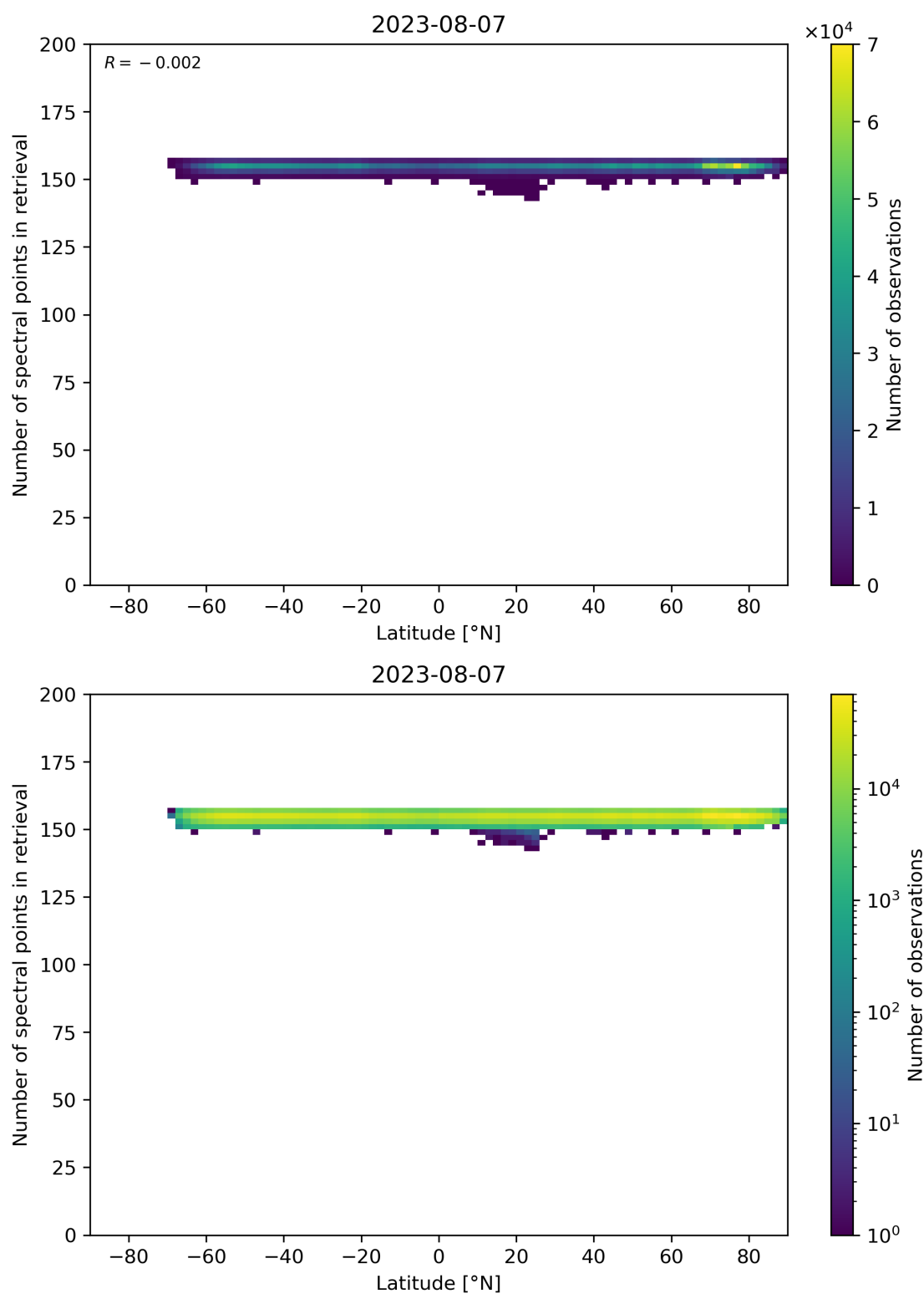
Figure 57: Scatter density plot of “Latitude” against “Number of spectral points in retrieval” for 2023-08-06 to 2023-08-08.
