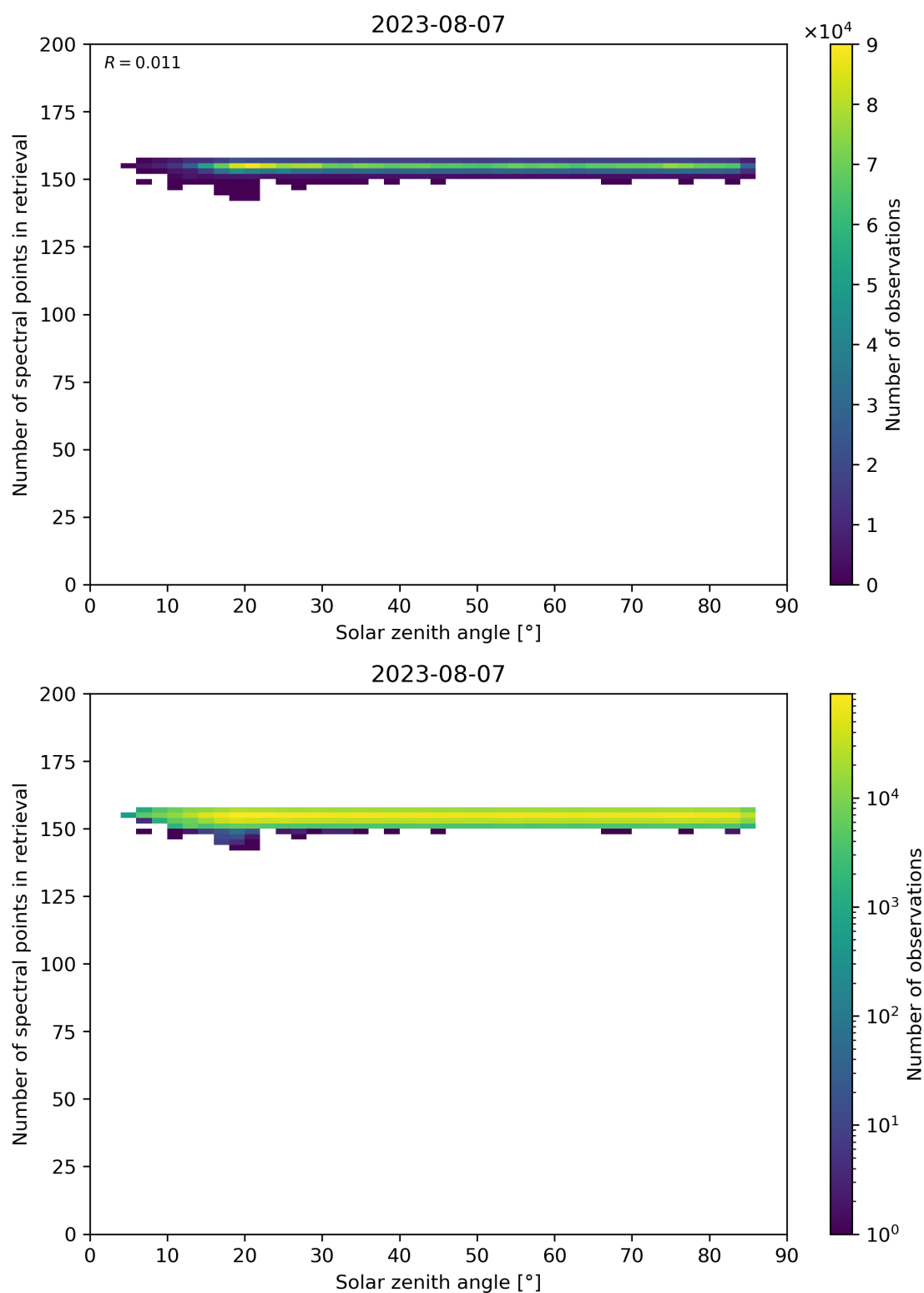
Figure 68: Scatter density plot of “Solar zenith angle” against “Number of spectral points in retrieval” for 2023-08-06 to 2023-08-08.
