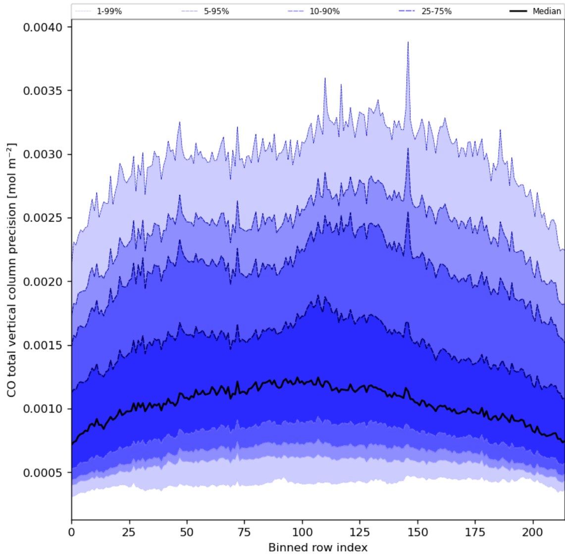
Figure 28: Along track statistics of “CO total vertical column precision” for 2023-08-06 to 2023-08-08
