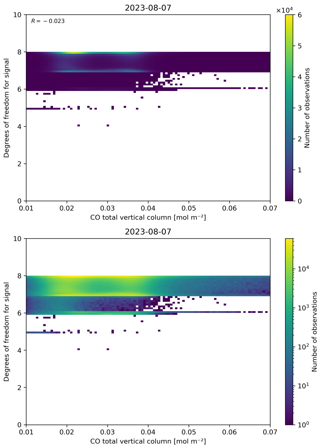
Figure 41: Scatter density plot of “CO total vertical column” against “Degrees of freedom for signal” for 2023-08-06 to 2023-08-08.
