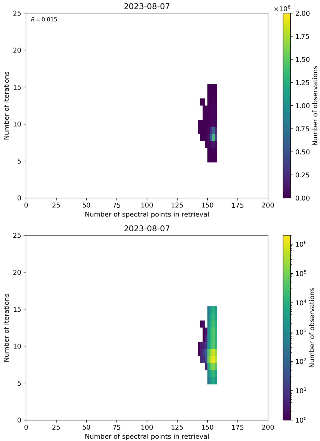
Figure 60: Scatter density plot of “Number of spectral points in retrieval” against “Number of iterations” for 2023-08-06 to 2023-08-08.
