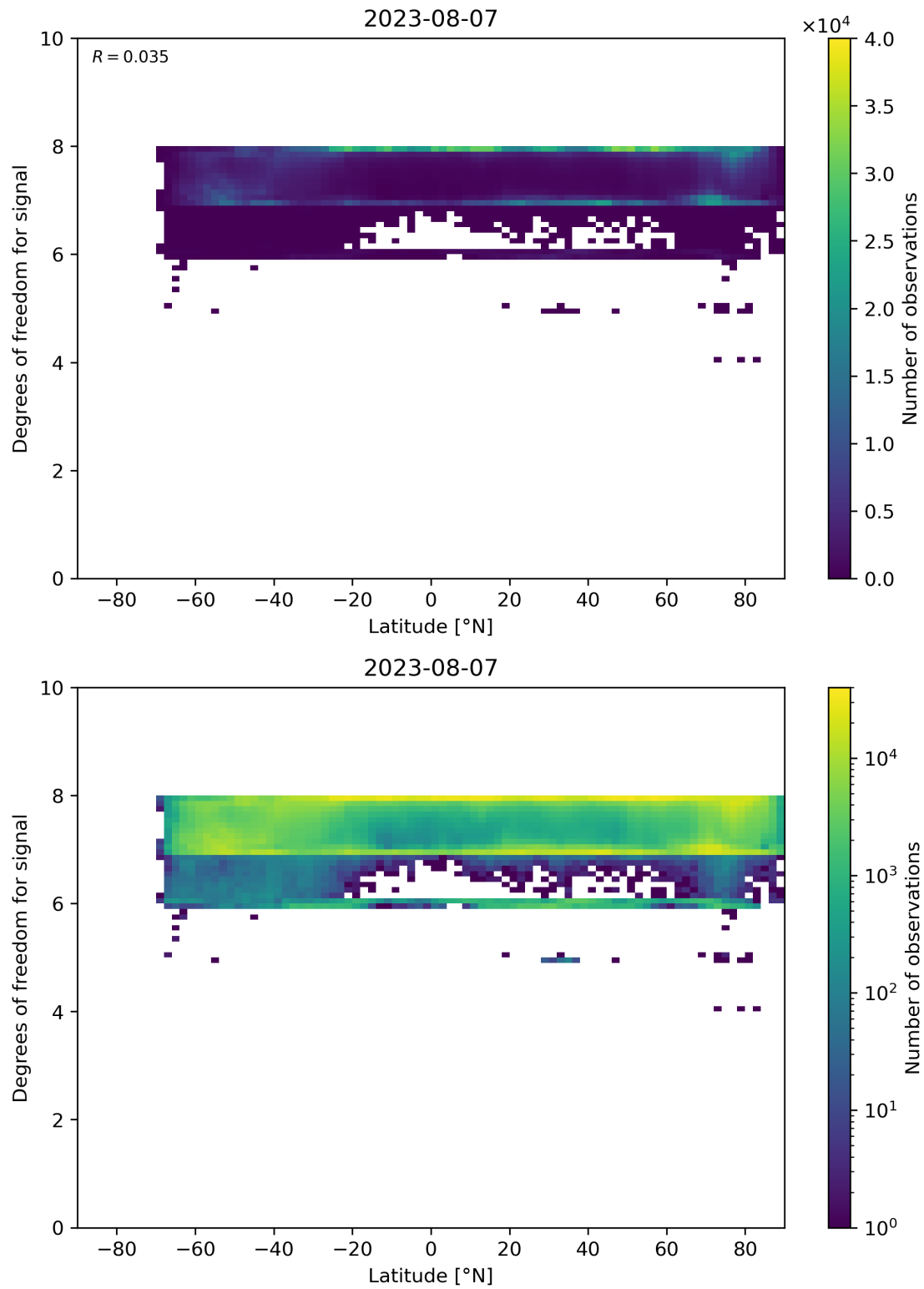
Figure 55: Scatter density plot of “Latitude” against “Degrees of freedom for signal” for 2023-08-06 to 2023-08-08.
