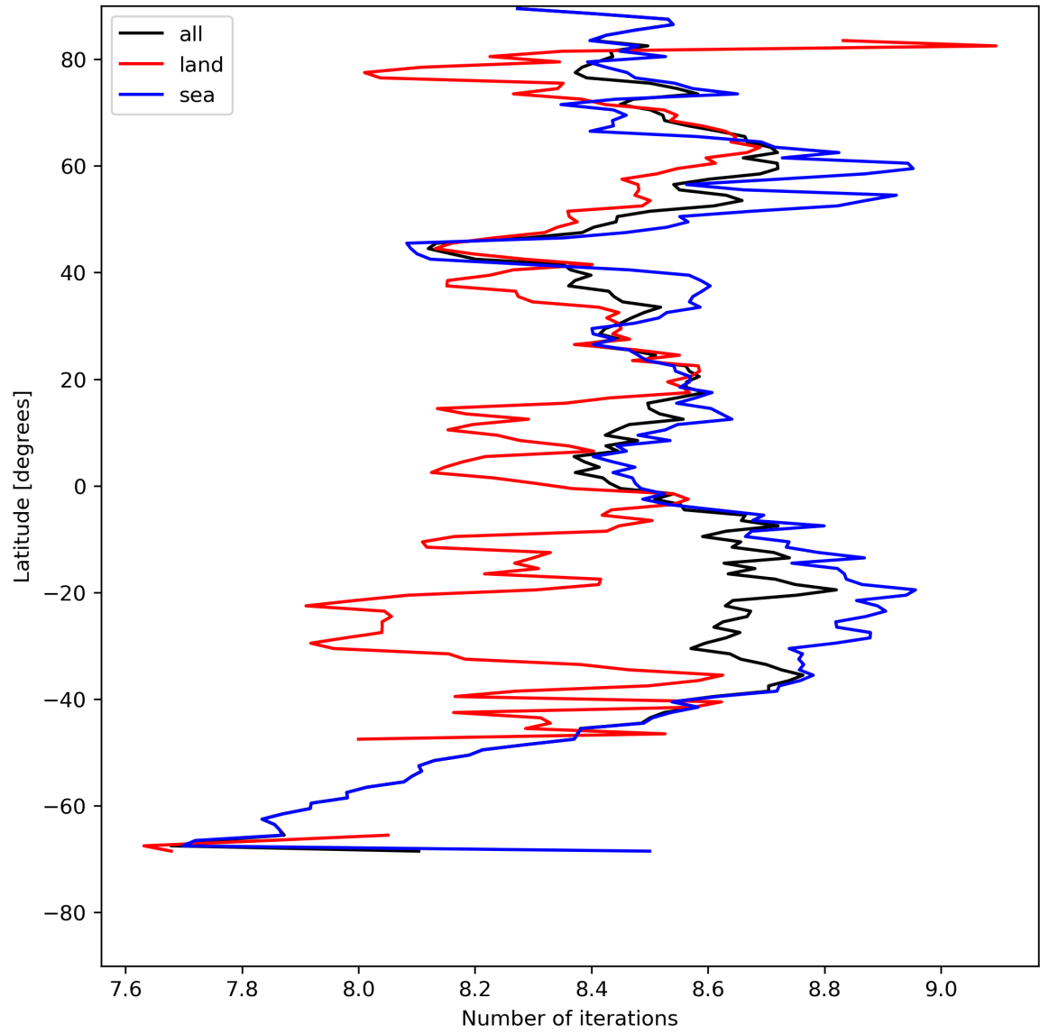
Figure 16: Zonal average of “Number of iterations” for 2023-08-06 to 2023-08-08.
