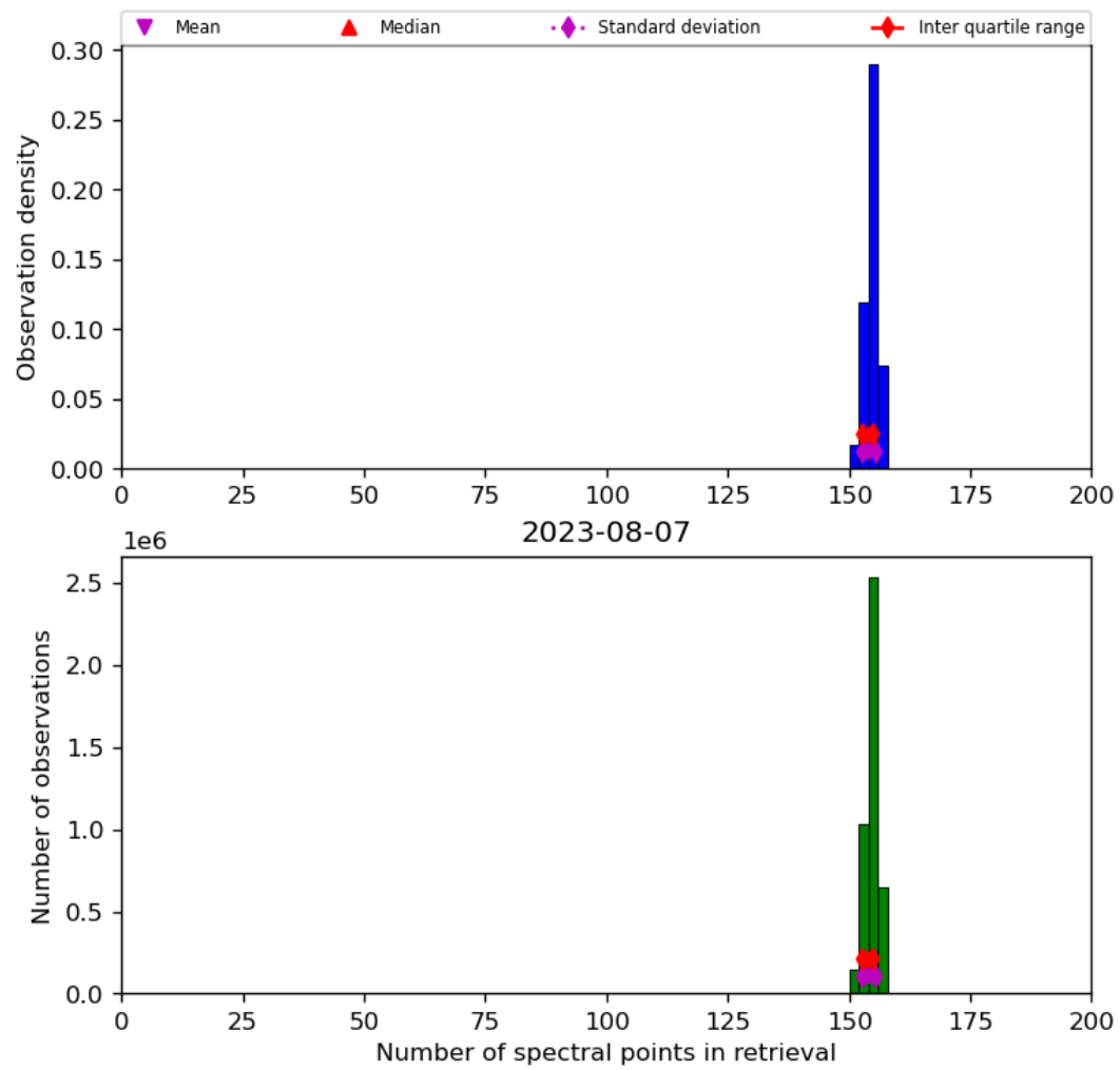
Figure 21: Histogram of “Number of spectral points in retrieval” for 2023-08-06 to 2023-08-08
