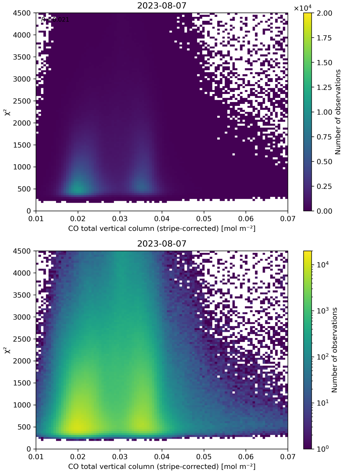
Figure 37: Scatter density plot of “CO total vertical column (stripe-corrected)” against “ \chi^2 ” for 2023-08-06 to 2023-08-08.
