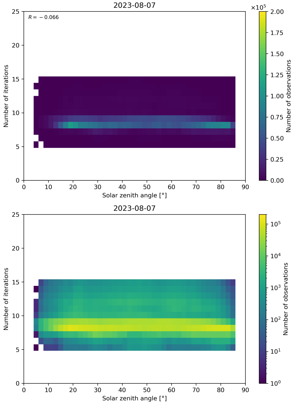
Figure 67: Scatter density plot of “Solar zenith angle” against “Number of iterations” for 2023-08-06 to 2023-08-08.
