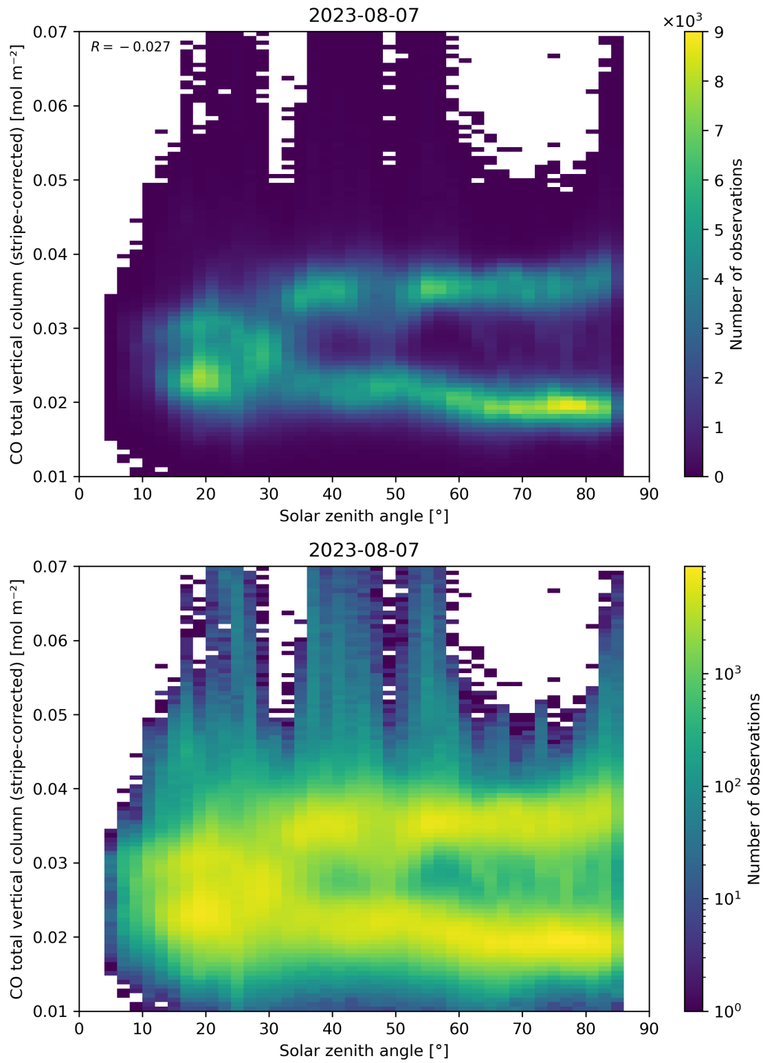
Figure 62: Scatter density plot of “Solar zenith angle” against “CO total vertical column (stripe-corrected)” for 2023-08-06 to 2023-08-08.
