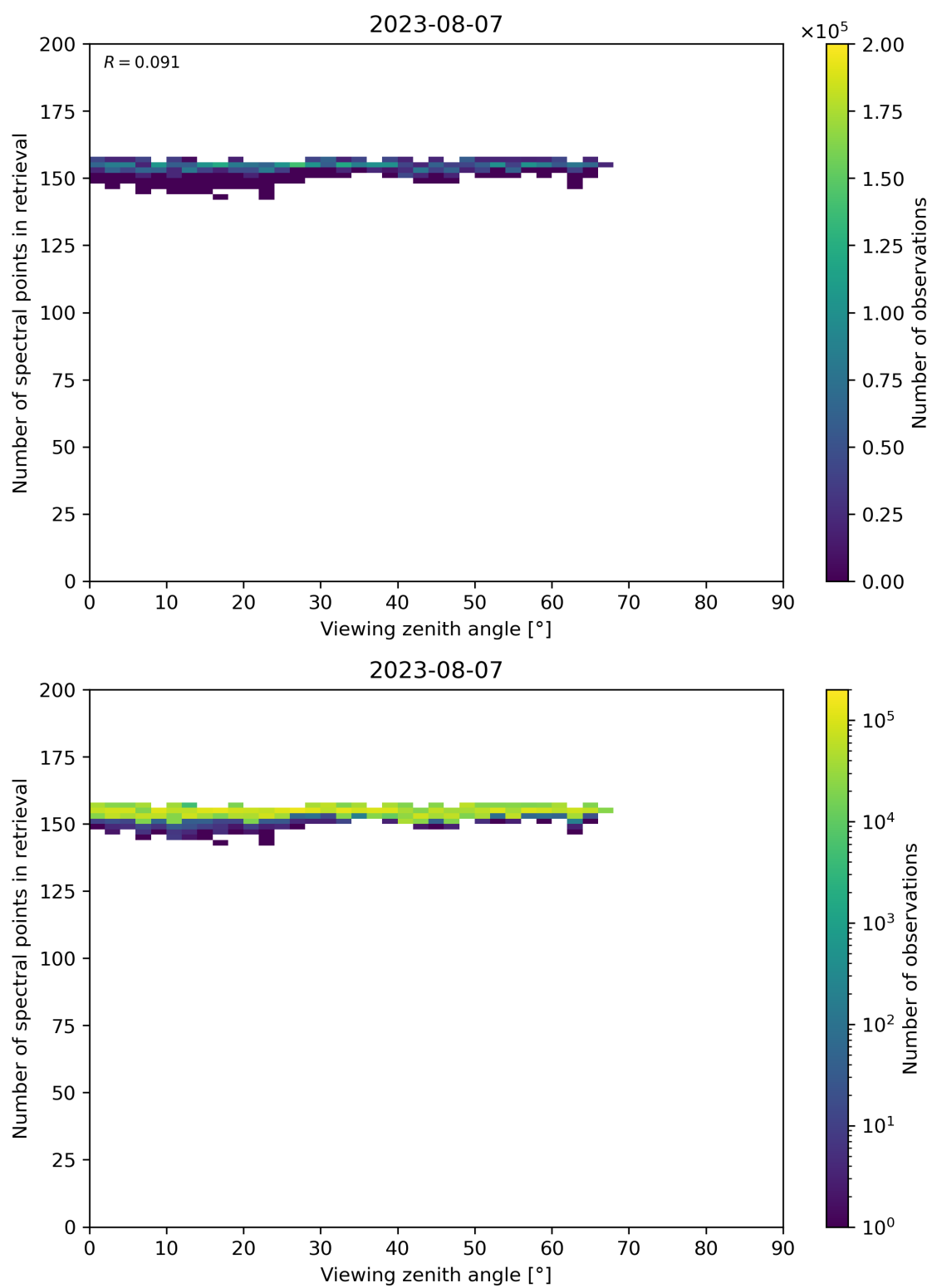
Figure 76: Scatter density plot of “Viewing zenith angle” against “Number of spectral points in retrieval” for 2023-08-06 to 2023-08-08.
