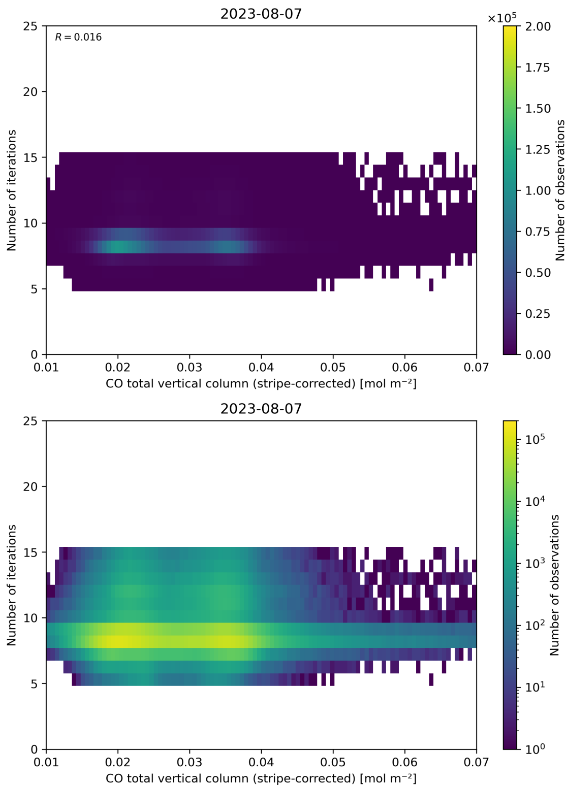
Figure 39: Scatter density plot of “CO total vertical column (stripe-corrected)” against “Number of iterations” for 2023-08-06 to 2023-08-08.
