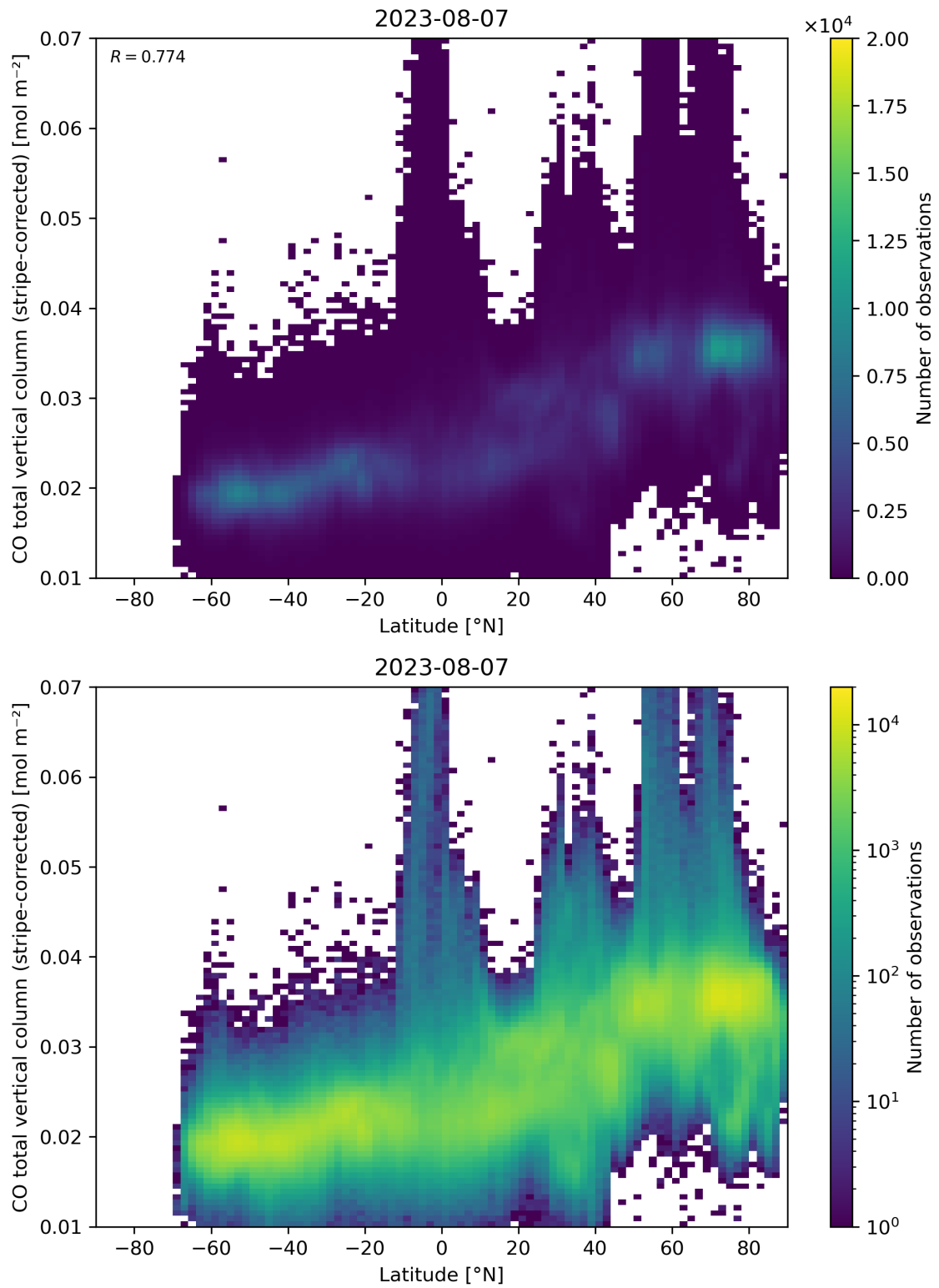
Figure 52: Scatter density plot of “Latitude” against “CO total vertical column (stripe-corrected)” for 2023-08-06 to 2023-08-08.
