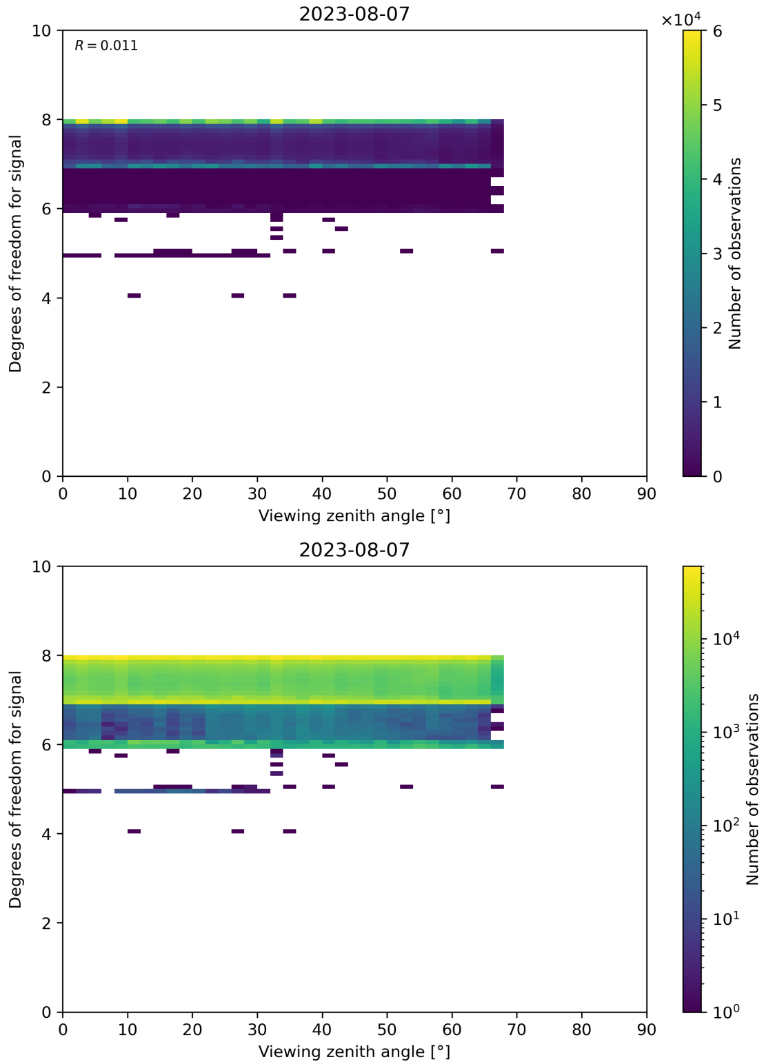
Figure 73: Scatter density plot of “Viewing zenith angle” against “Degrees of freedom for signal” for 2023-08-06 to 2023-08-08.
