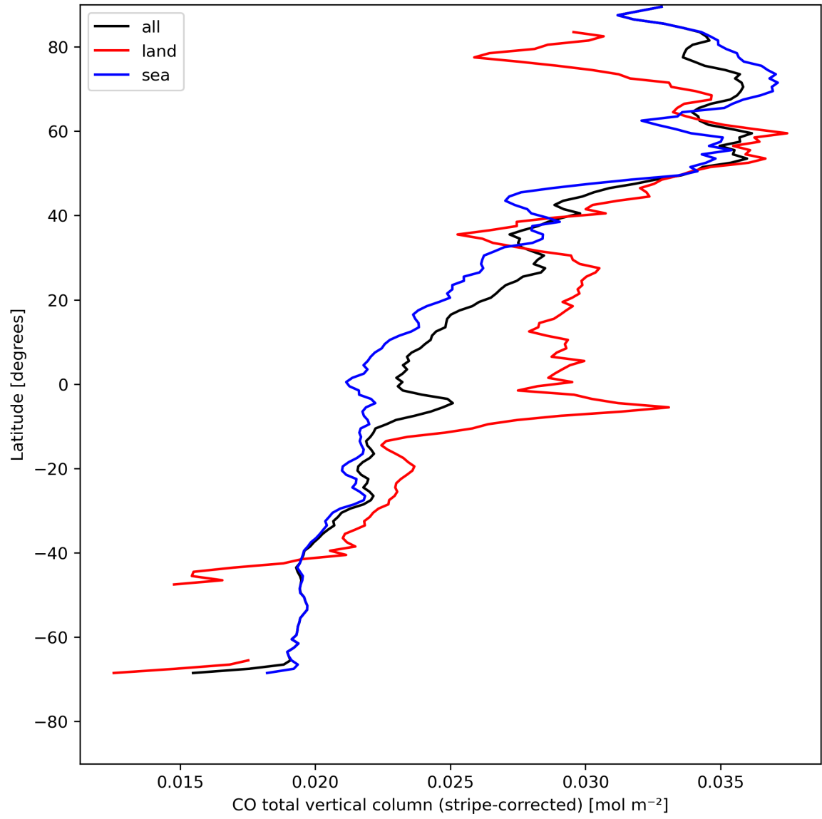
Figure 11: Zonal average of “CO total vertical column (stripe-corrected)” for 2023-08-06 to 2023-08-08.
