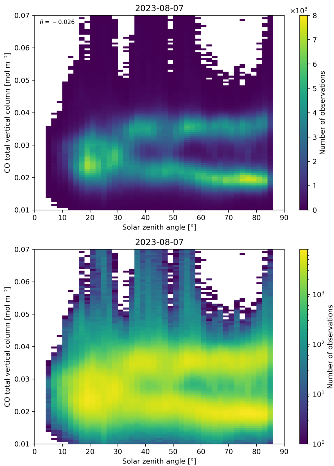
Figure 61: Scatter density plot of “Solar zenith angle” against “CO total vertical column” for 2023-08-06 to 2023-08-08.
