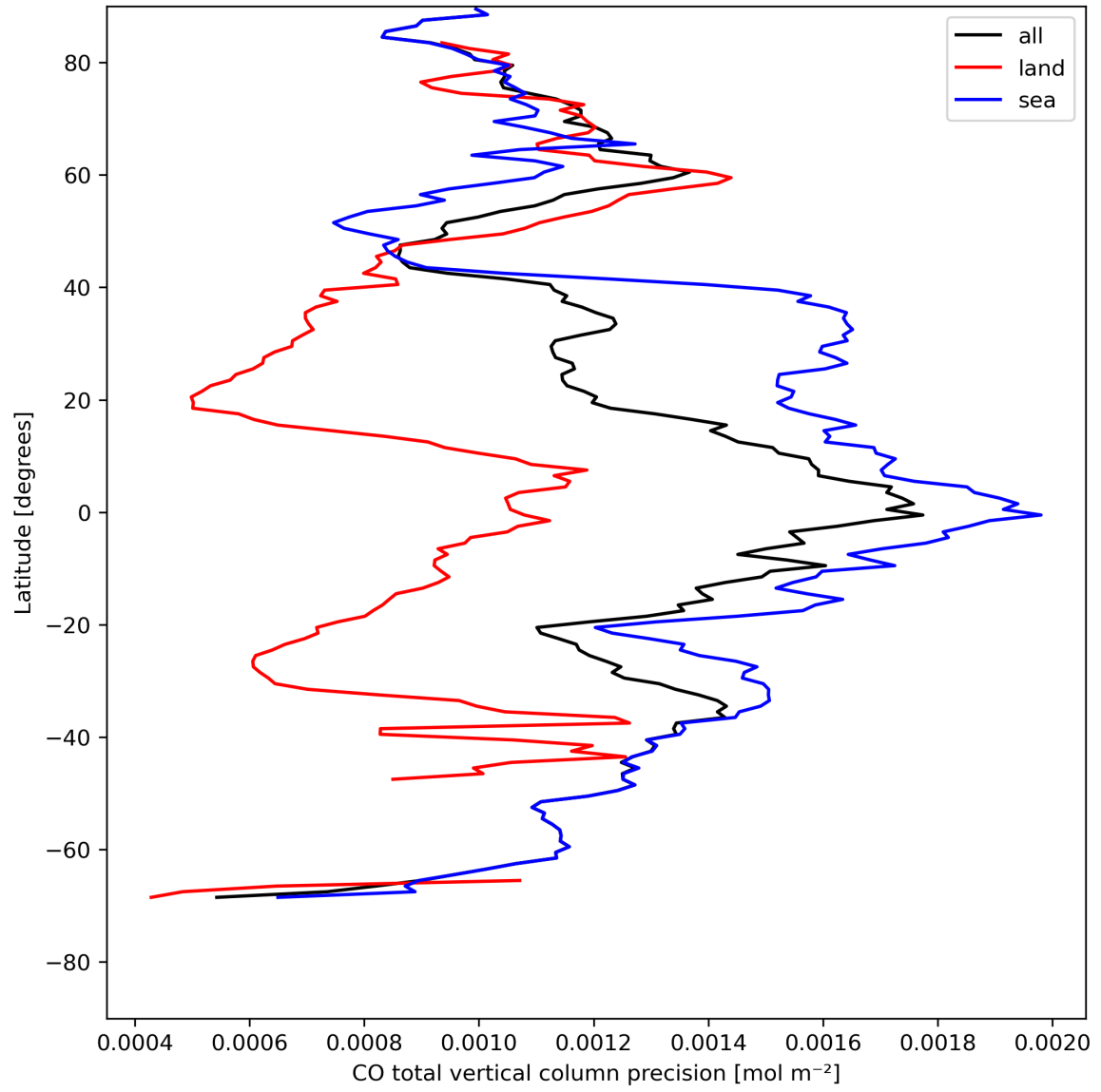
Figure 12: Zonal average of “CO total vertical column precision” for 2023-08-06 to 2023-08-08.
