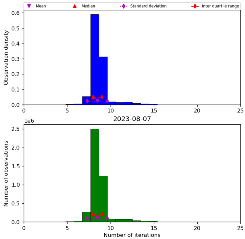
Figure 24: Histogram of “Number of iterations” for 2023-08-06 to 2023-08-08
