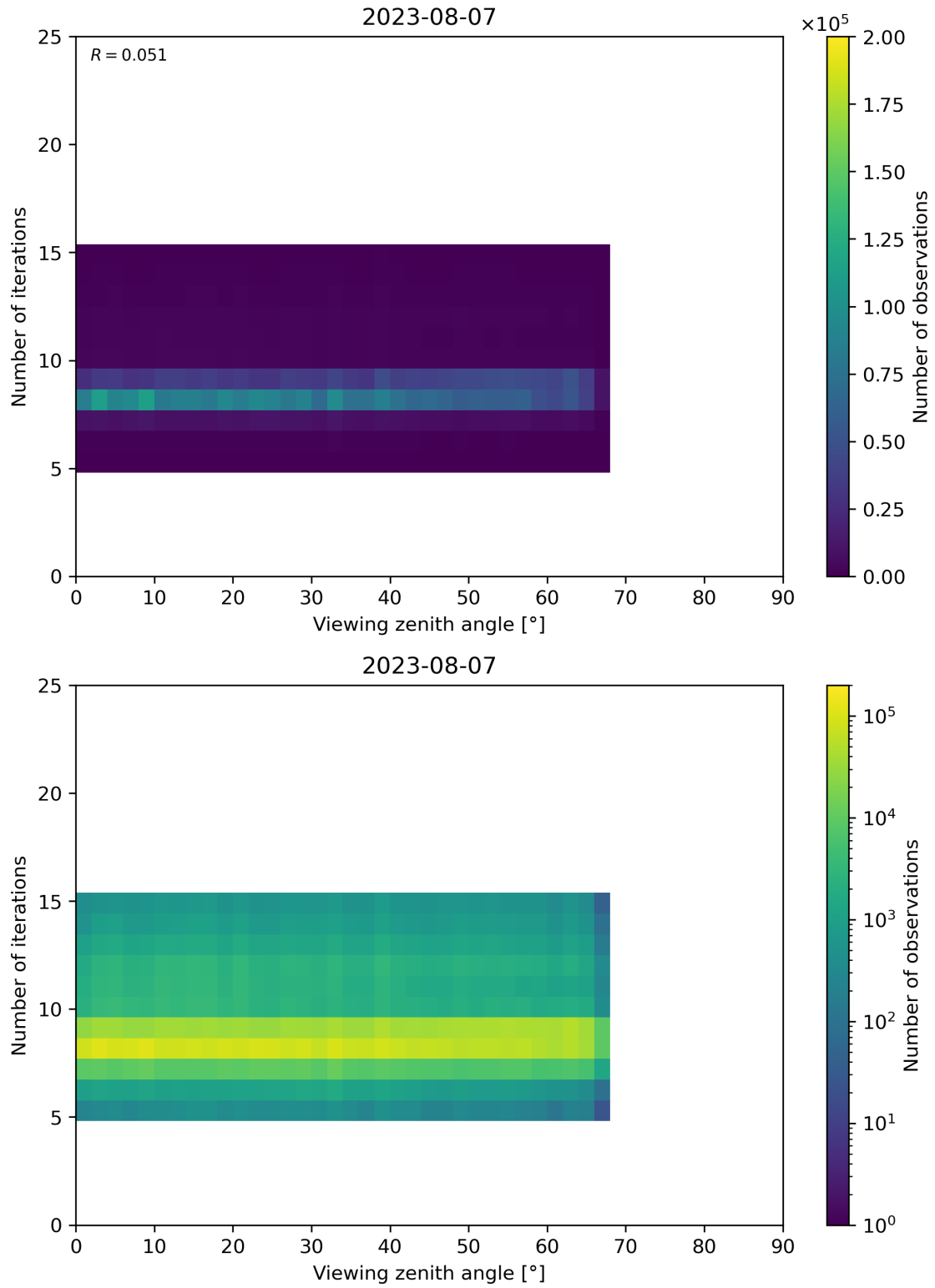
Figure 75: Scatter density plot of “Viewing zenith angle” against “Number of iterations” for 2023-08-06 to 2023-08-08.
