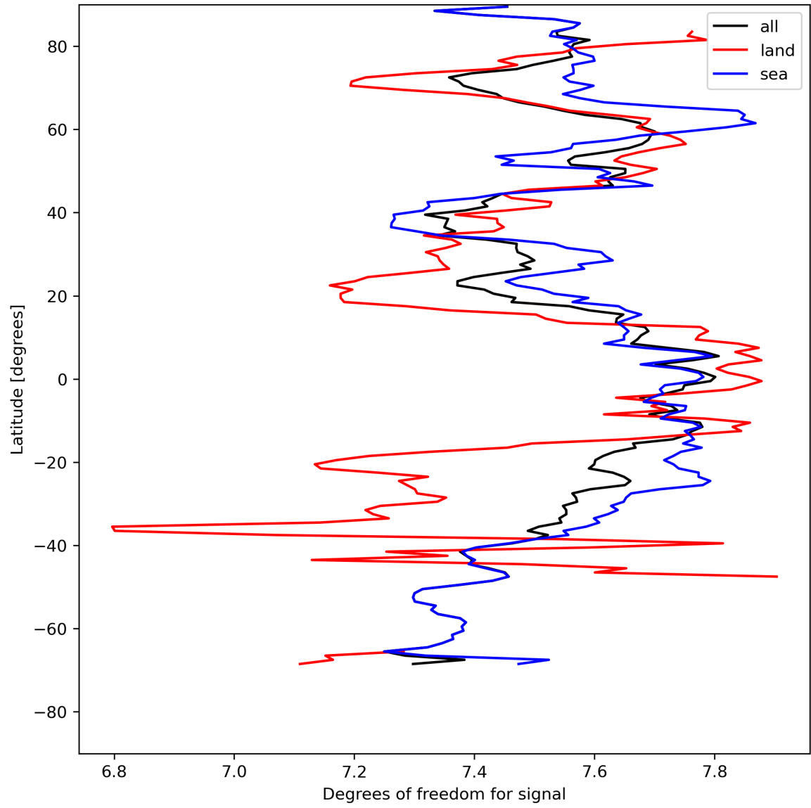
Figure 15: Zonal average of “Degrees of freedom for signal” for 2023-08-06 to 2023-08-08.
