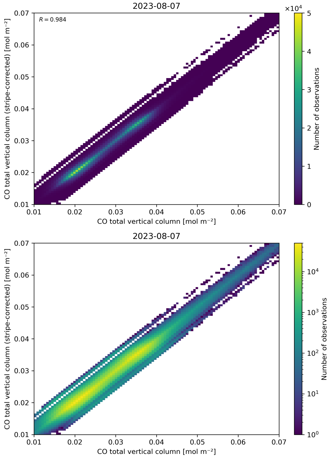
Figure 33: Scatter density plot of “CO total vertical column” against “CO total vertical column (stripe-corrected)” for 2023-08-06 to 2023-08-08.
