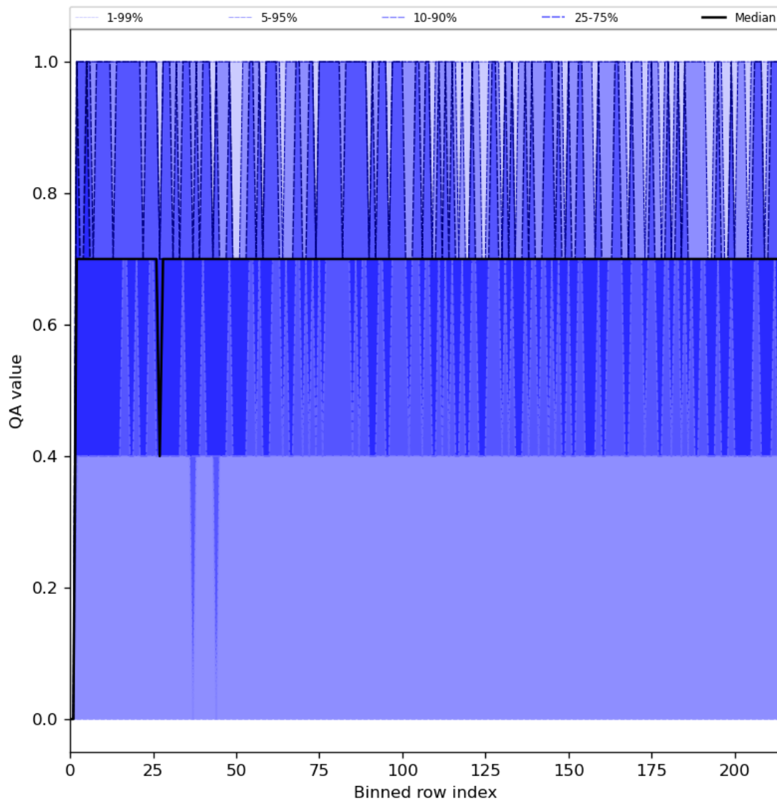
Figure 25: Along track statistics of “QA value” for 2023-08-06 to 2023-08-08
