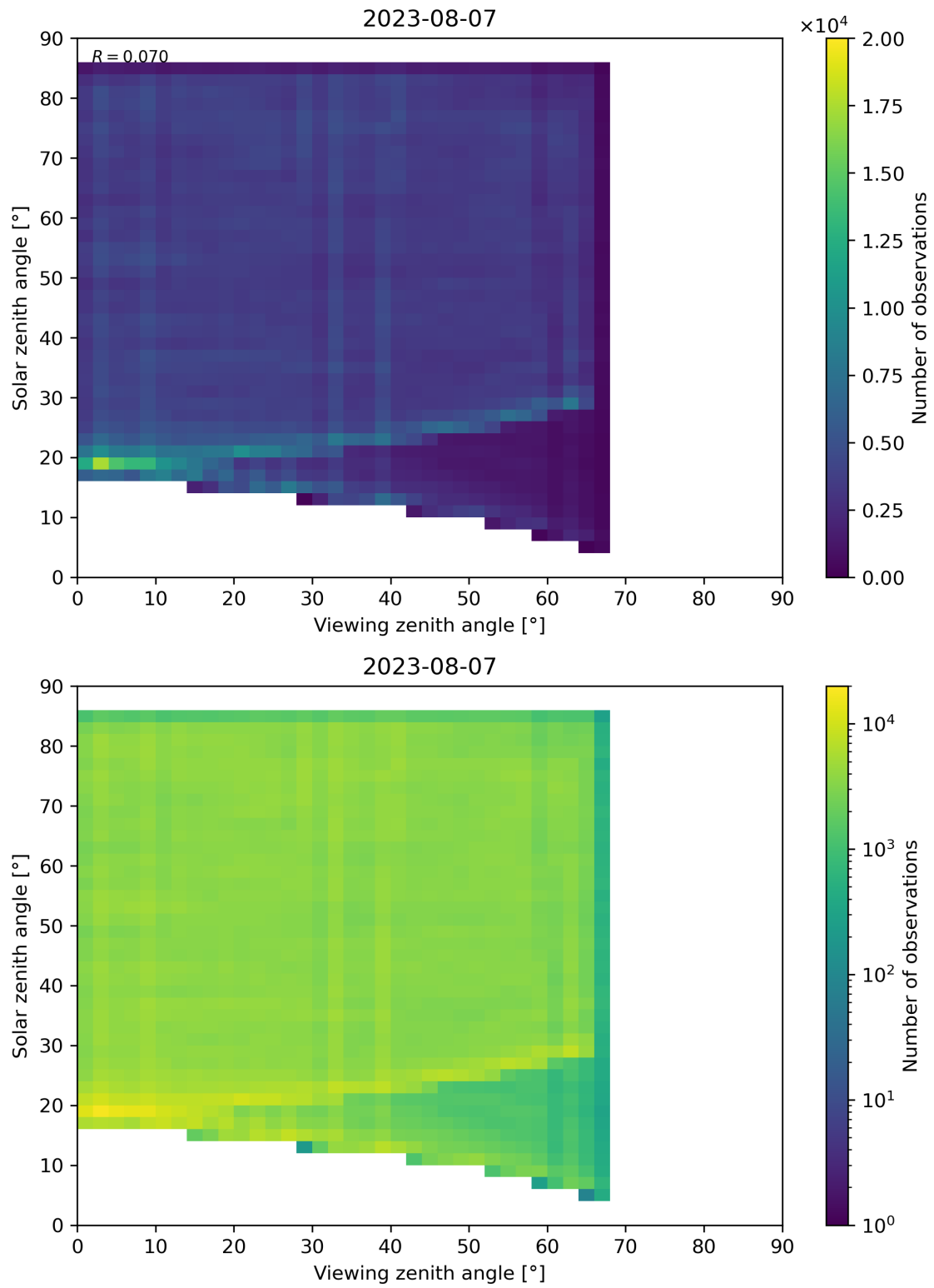
Figure 77: Scatter density plot of “Viewing zenith angle” against “Solar zenith angle” for 2023-08-06 to 2023-08-08.
