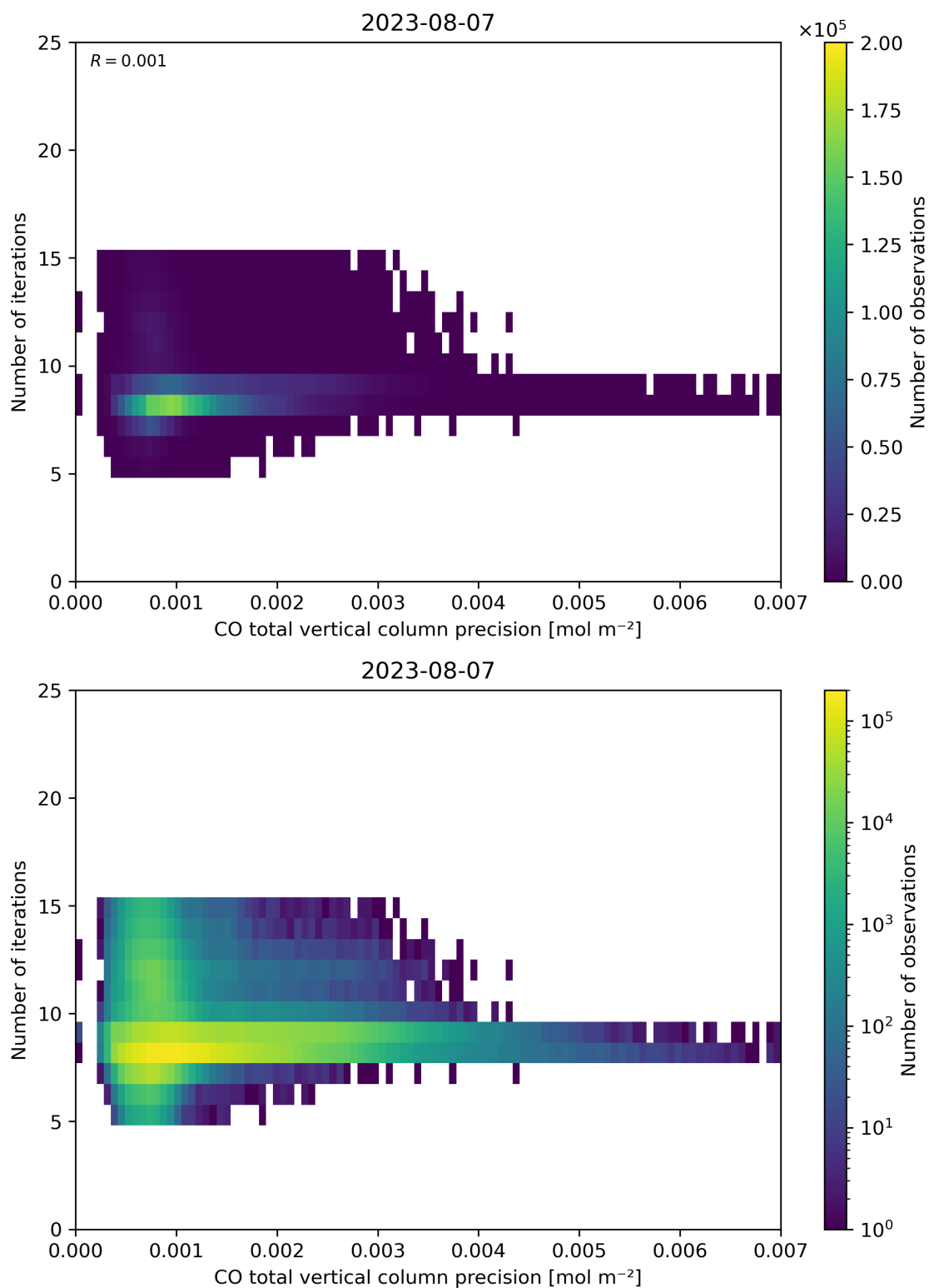
Figure 46: Scatter density plot of “CO total vertical column precision” against “Number of iterations” for 2023-08-06 to 2023-08-08.
