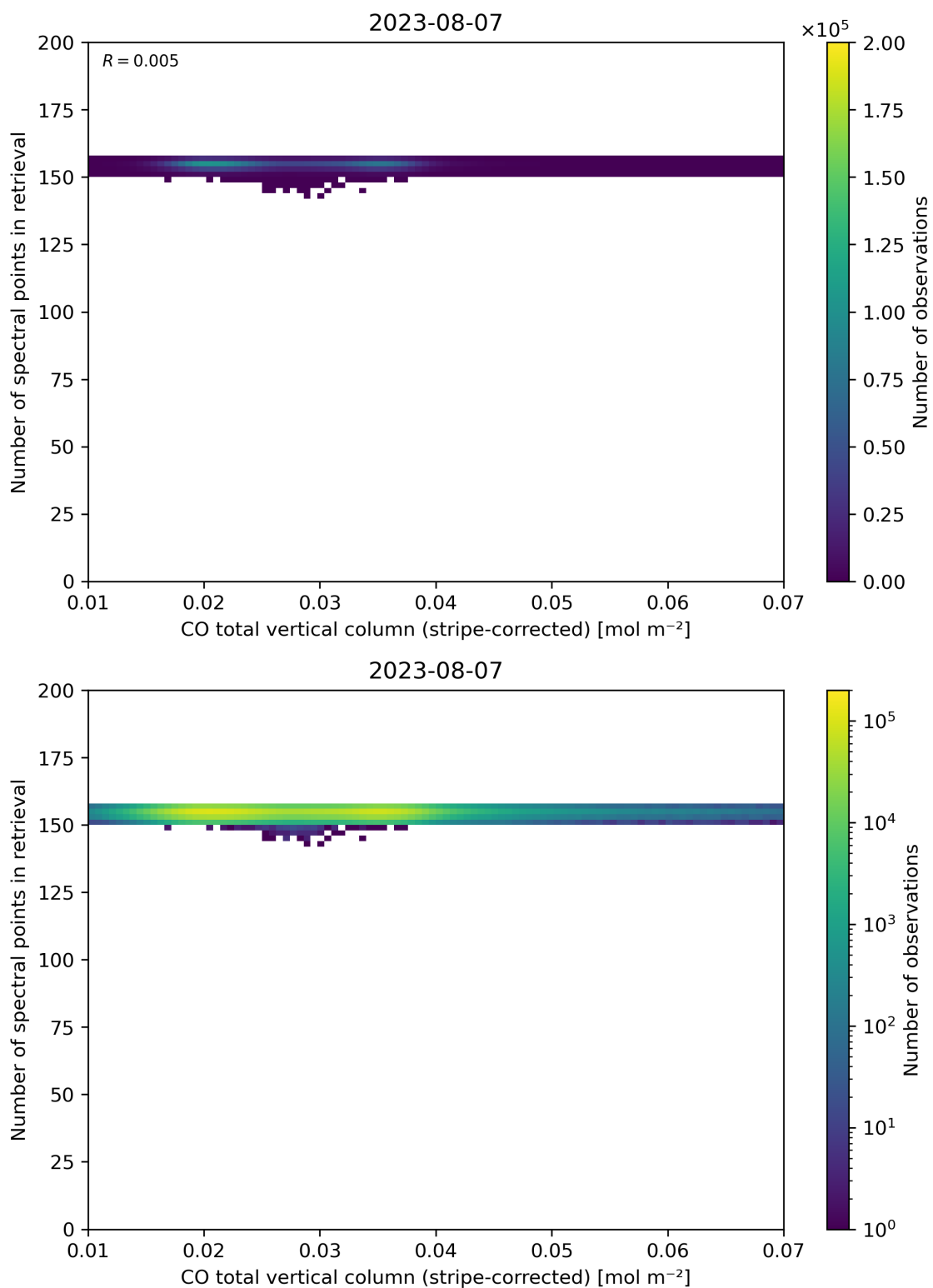
Figure 40: Scatter density plot of “CO total vertical column (stripe-corrected)” against “Number of spectral points in retrieval” for 2023-08-06 to 2023-08-08.
