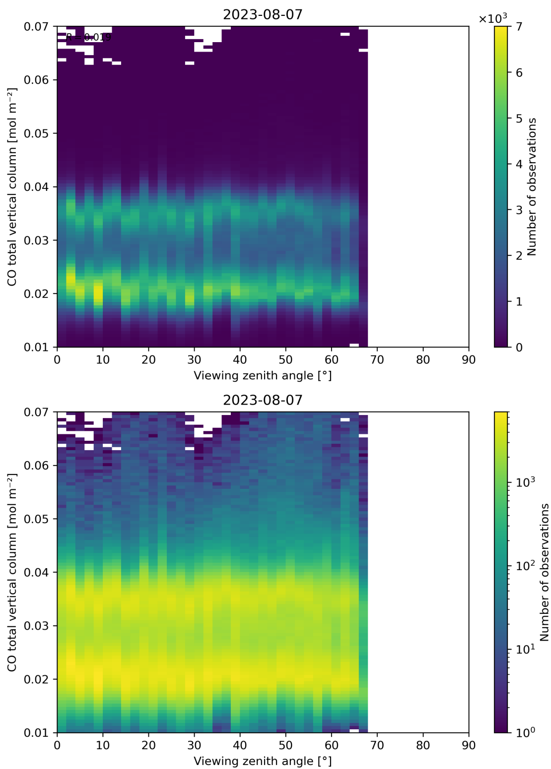
Figure 69: Scatter density plot of “Viewing zenith angle” against “CO total vertical column” for 2023-08-06 to 2023-08-08.
