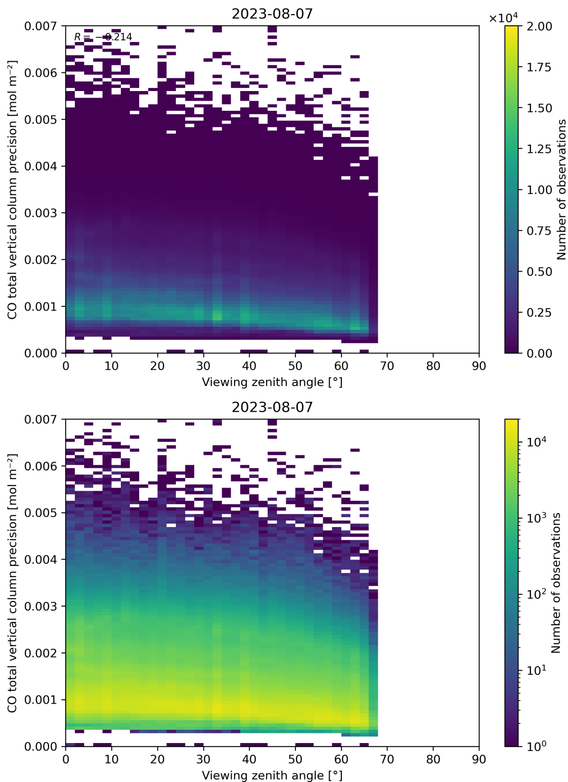
Figure 71: Scatter density plot of “Viewing zenith angle” against “CO total vertical column precision” for 2023-08-06 to 2023-08-08.
