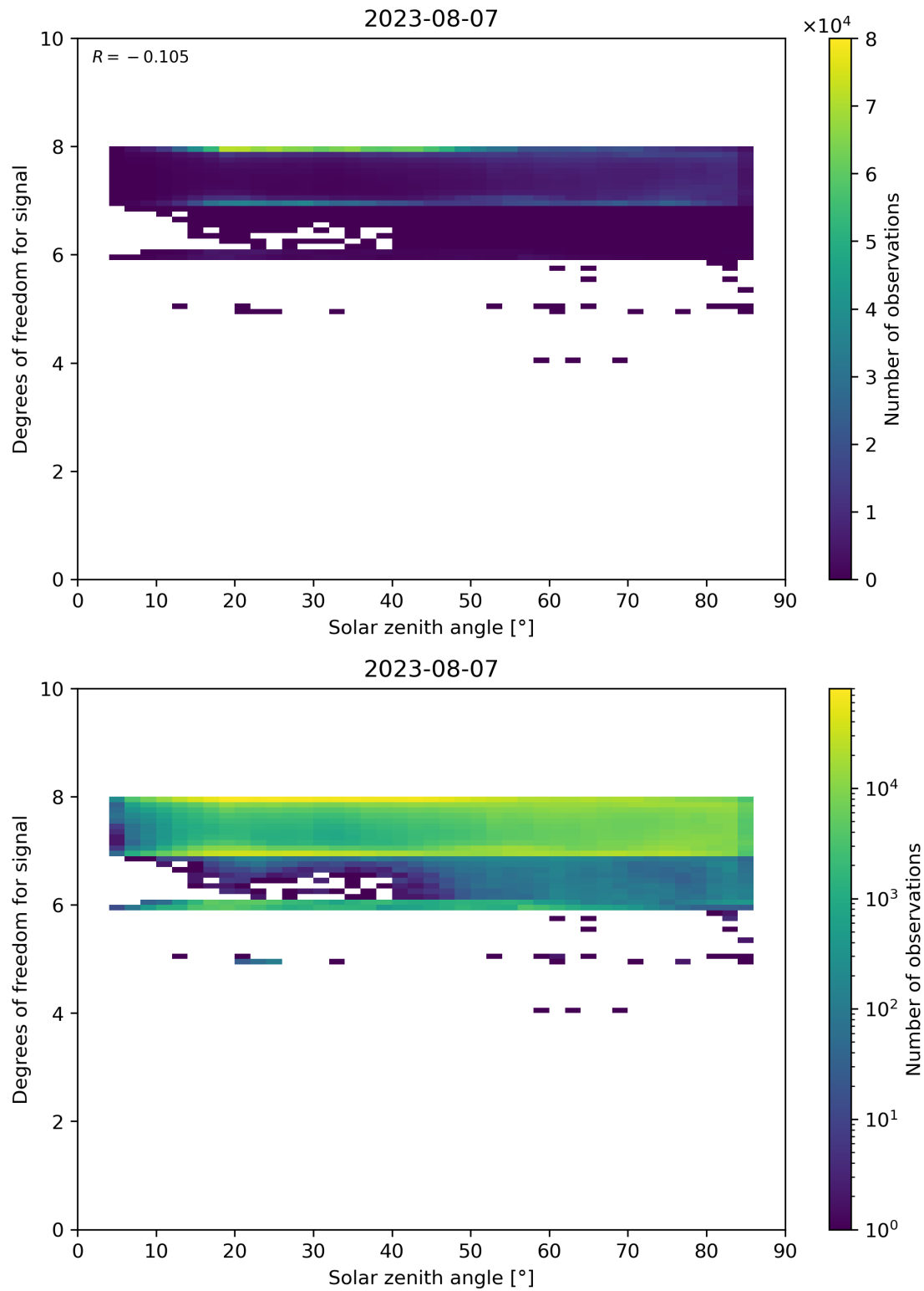
Figure 65: Scatter density plot of “Solar zenith angle” against “Degrees of freedom for signal” for 2023-08-06 to 2023-08-08.
