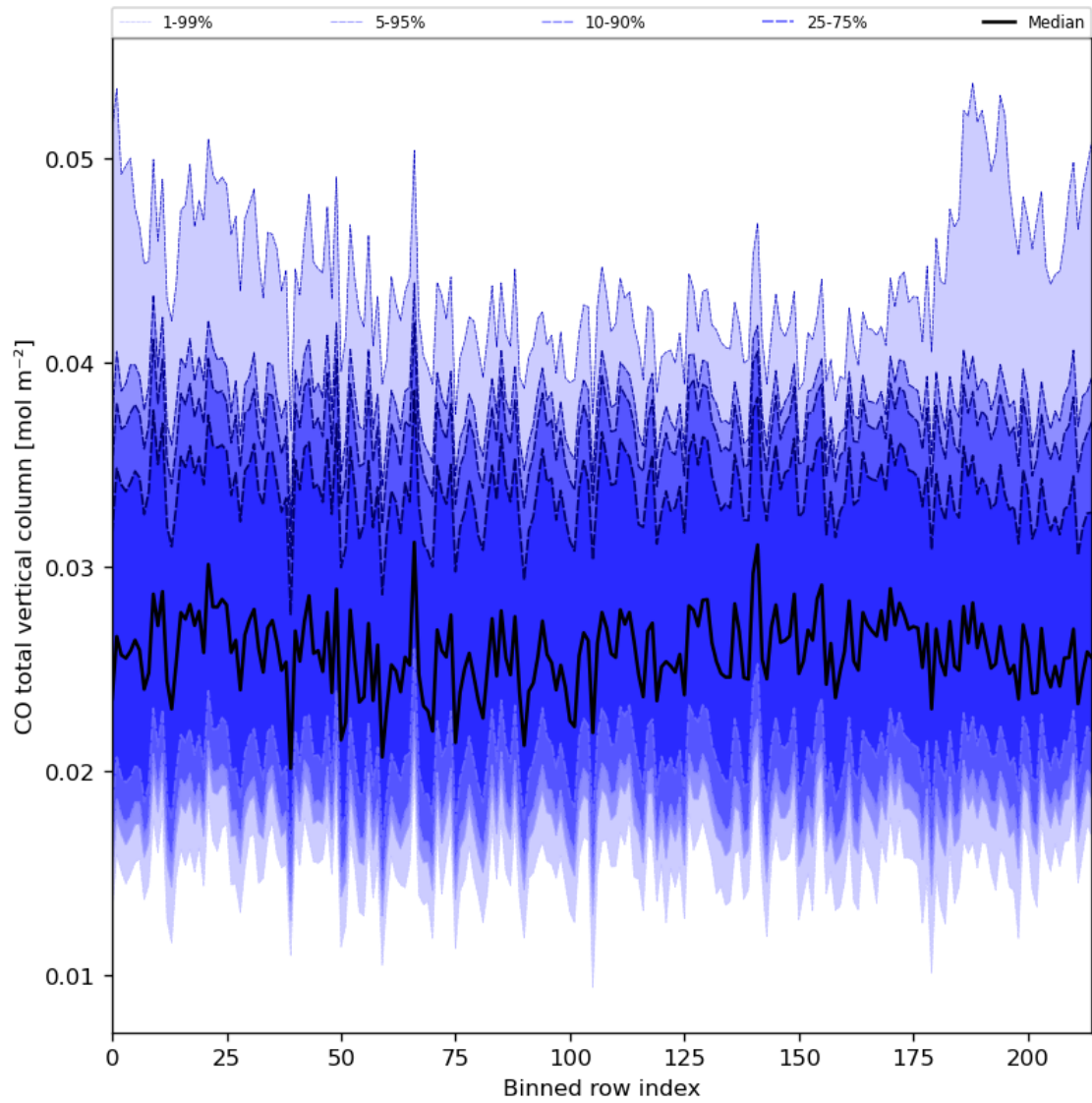
Figure 26: Along track statistics of “CO total vertical column” for 2023-08-06 to 2023-08-08
