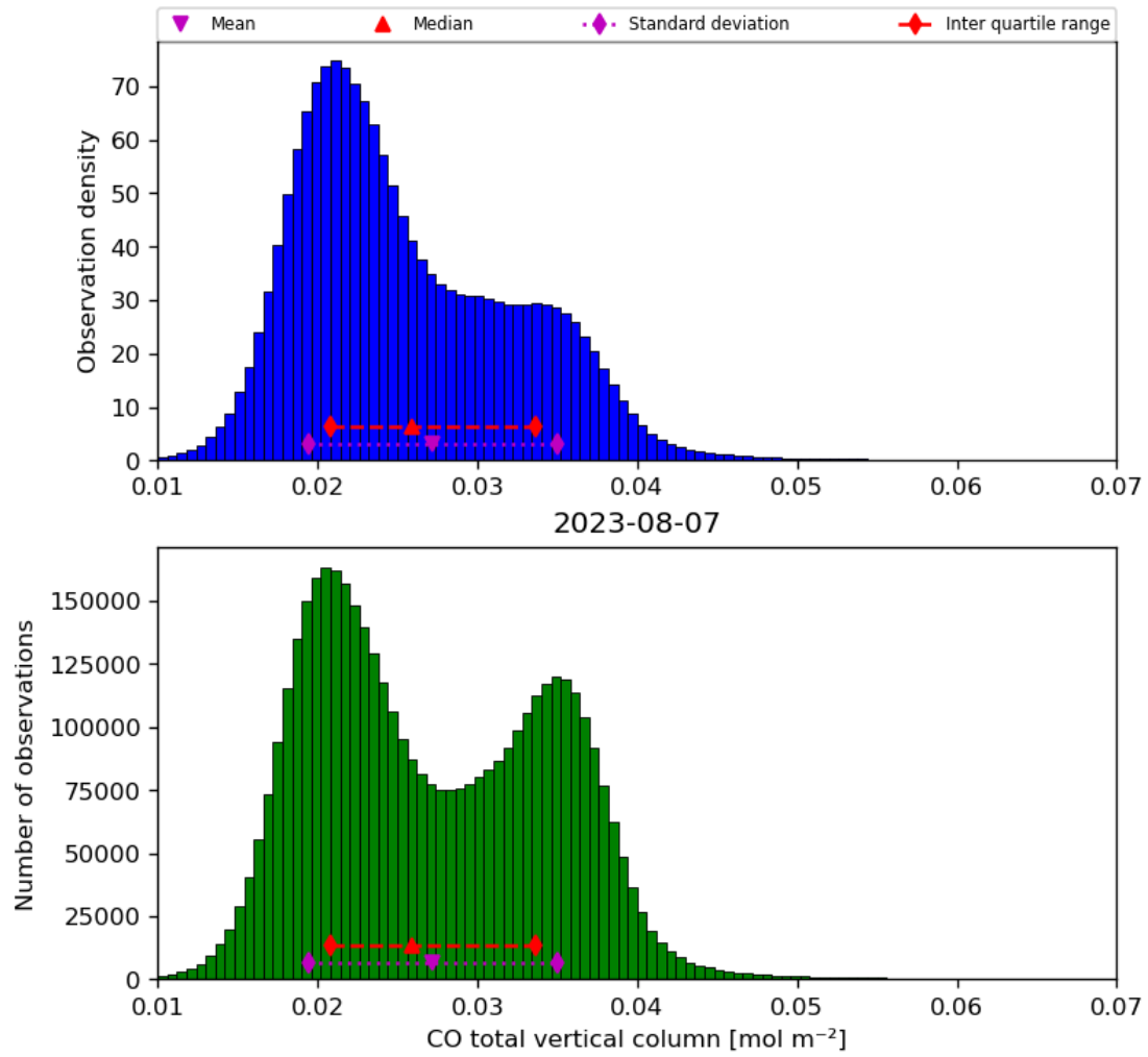
Figure 18: Histogram of “CO total vertical column” for 2023-08-06 to 2023-08-08
