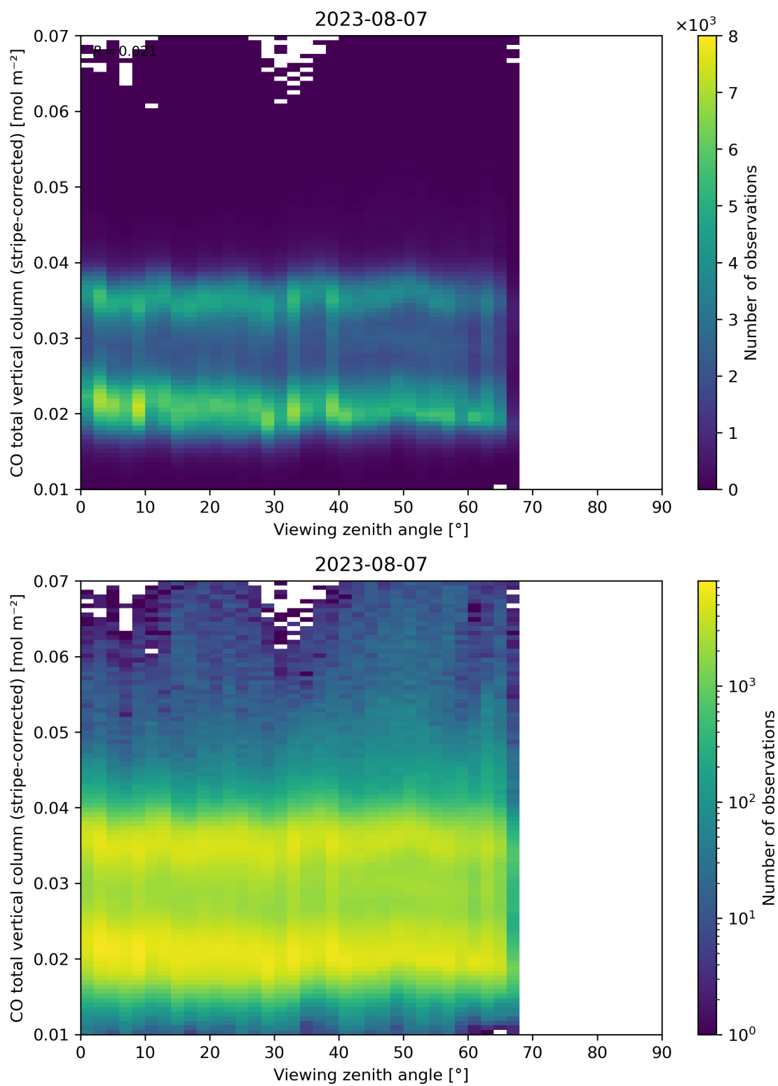
Figure 70: Scatter density plot of “Viewing zenith angle” against “CO total vertical column (stripe-corrected)” for 2023-08-06 to 2023-08-08.
