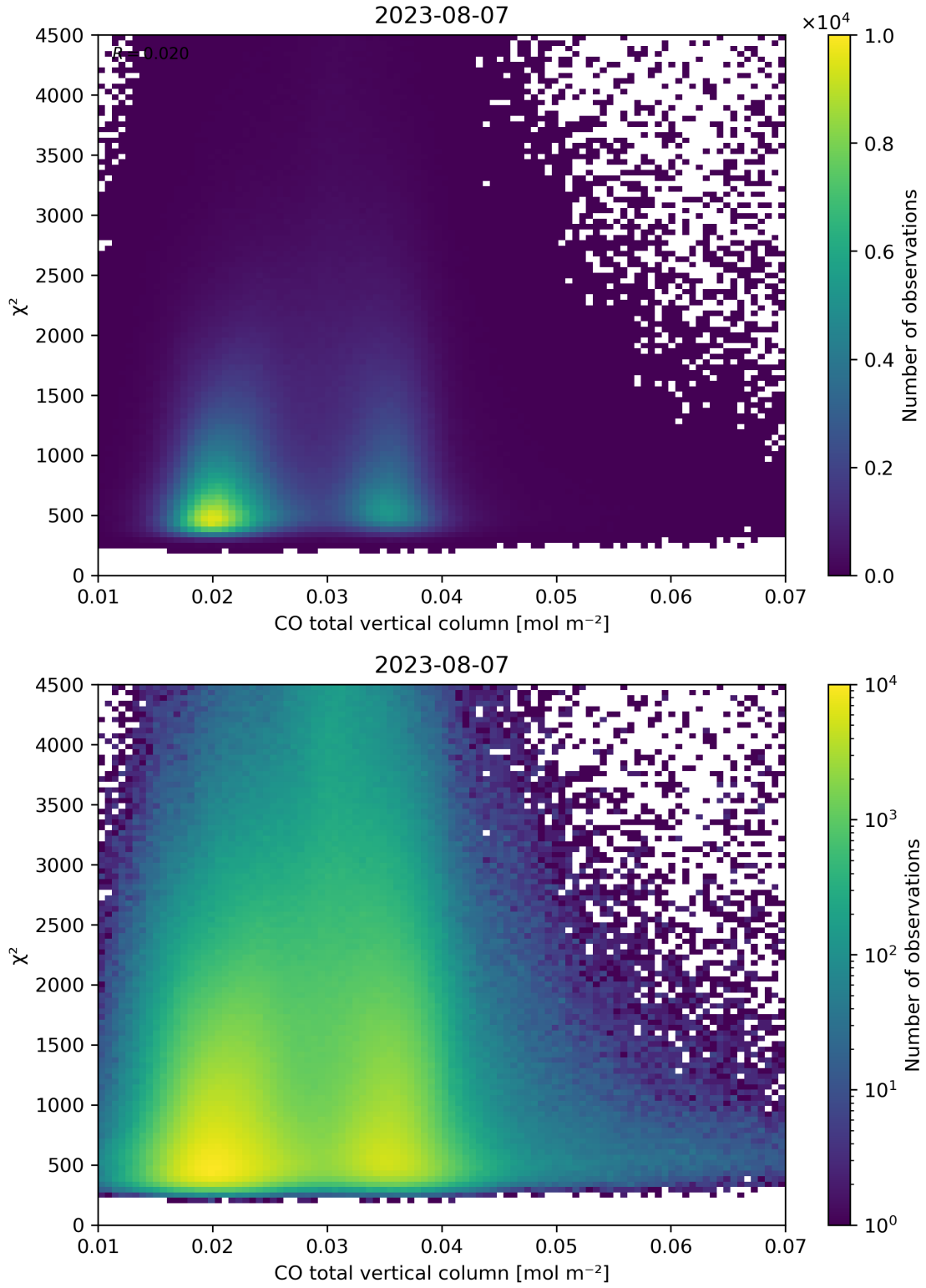
Figure 35: Scatter density plot of “CO total vertical column” against “ \chi^2 ” for 2023-08-06 to 2023-08-08.
