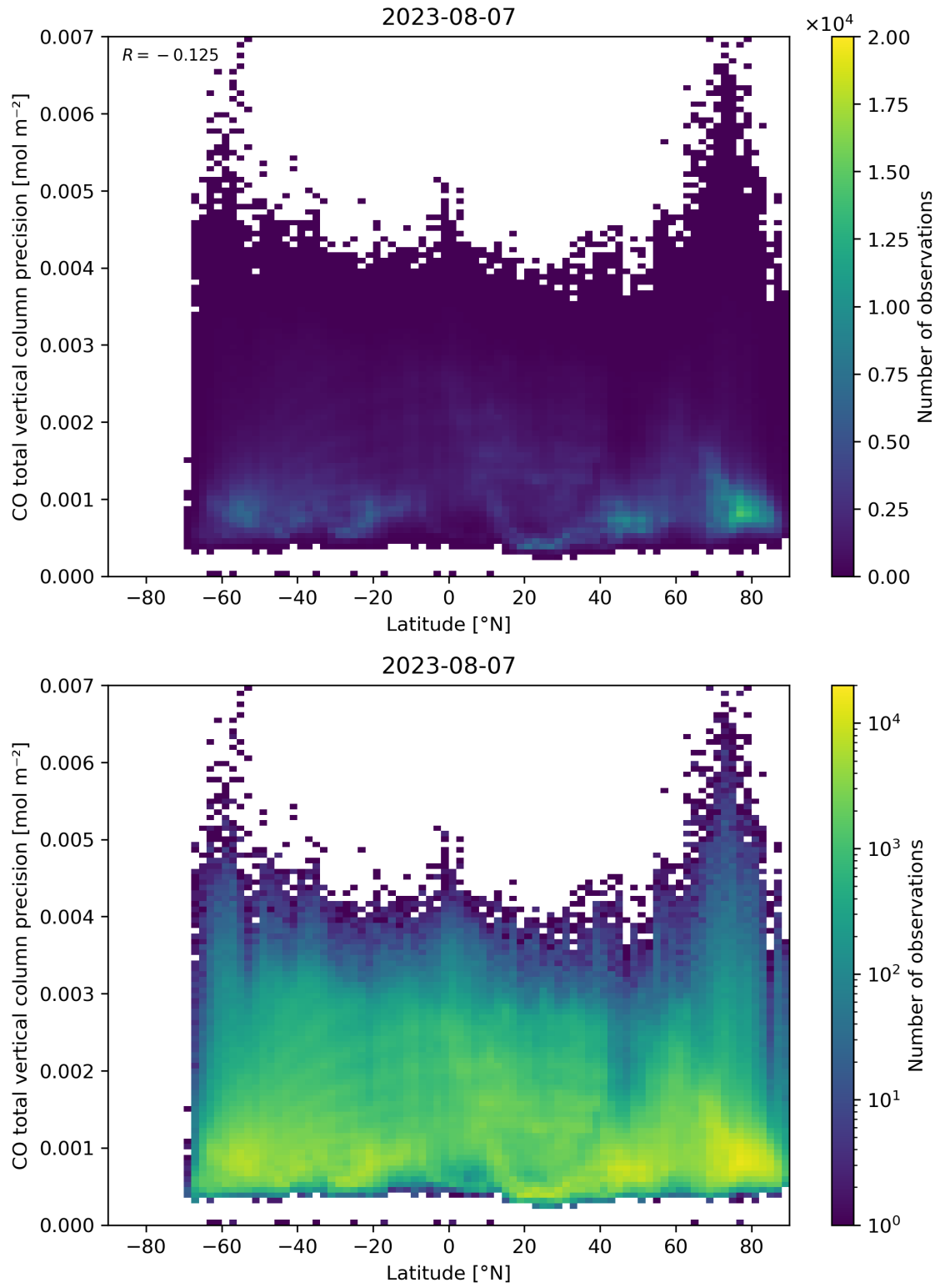
Figure 53: Scatter density plot of “Latitude” against “CO total vertical column precision” for 2023-08-06 to 2023-08-08.
