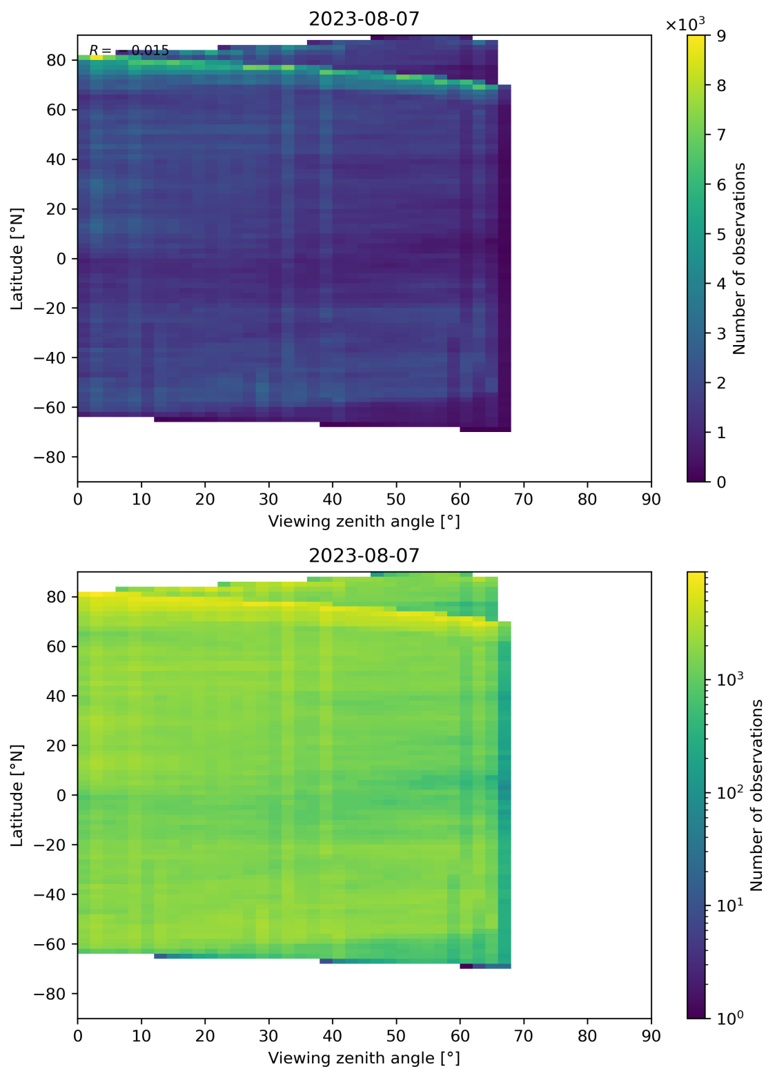
Figure 74: Scatter density plot of “Viewing zenith angle” against “Latitude” for 2023-08-06 to 2023-08-08.
