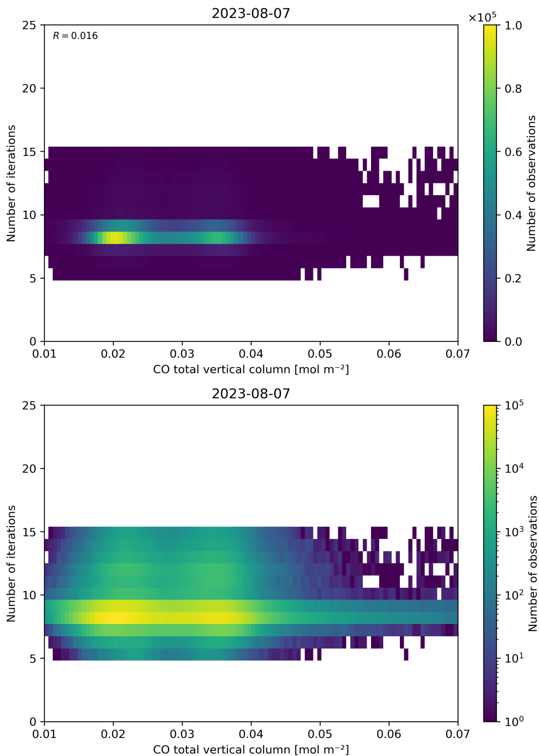
Figure 42: Scatter density plot of “CO total vertical column” against “Number of iterations” for 2023-08-06 to 2023-08-08.
