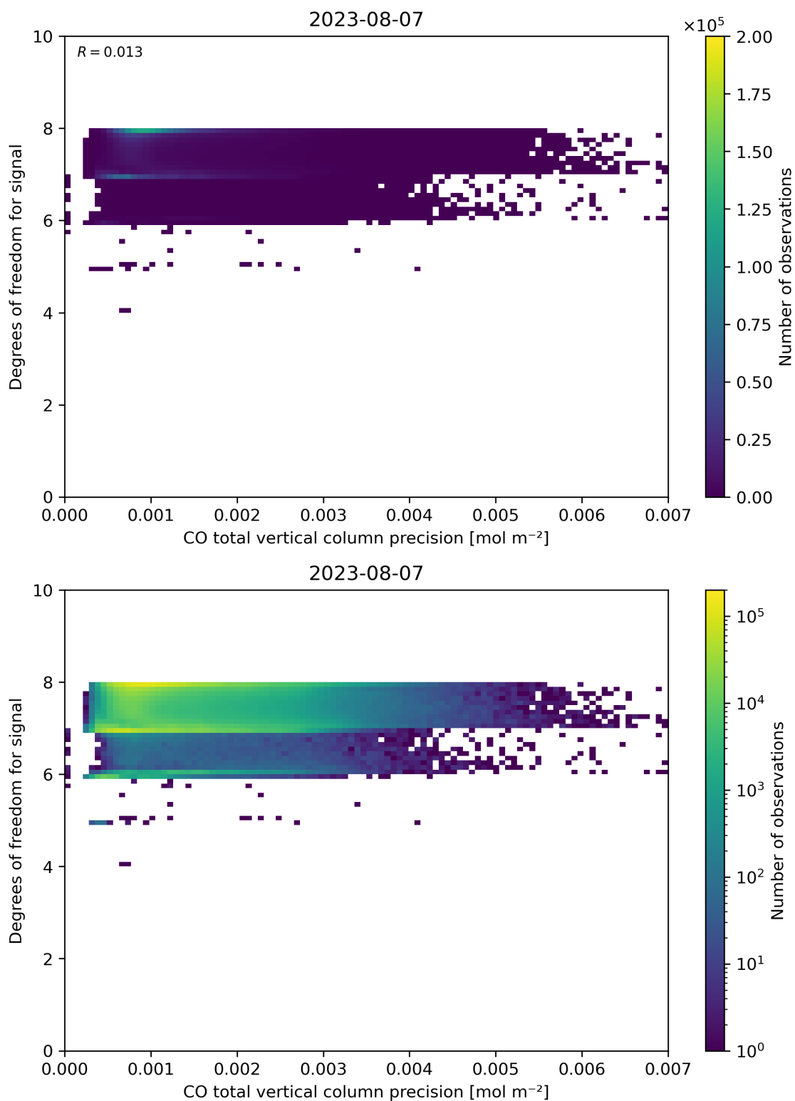
Figure 45: Scatter density plot of “CO total vertical column precision” against “Degrees of freedom for signal” for 2023-08-06 to 2023-08-08.
