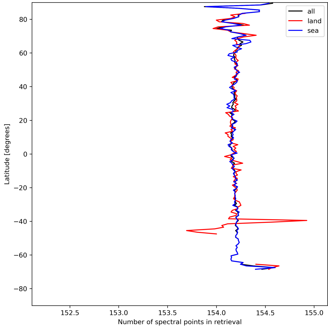
Figure 13: Zonal average of “Number of spectral points in retrieval” for 2023-08-06 to 2023-08-08.
