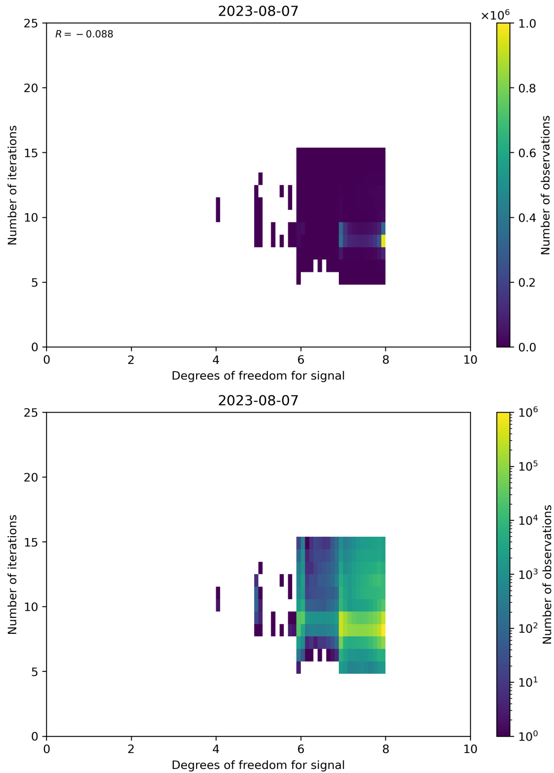
Figure 50: Scatter density plot of “Degrees of freedom for signal” against “Number of iterations” for 2023-08-06 to 2023-08-08.
