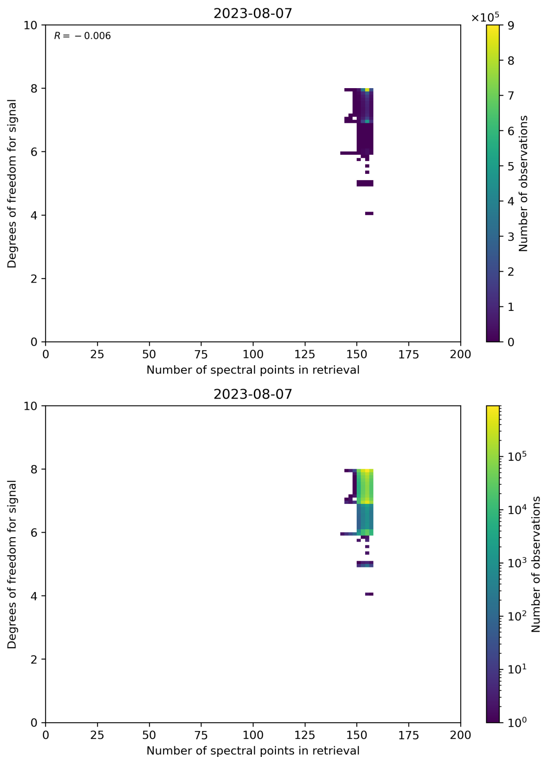
Figure 59: Scatter density plot of “Number of spectral points in retrieval” against “Degrees of freedom for signal” for 2023-08-06 to 2023-08-08.
