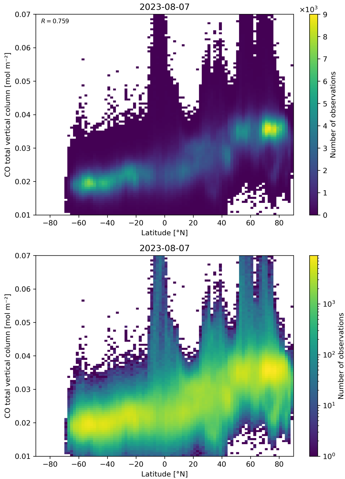
Figure 51: Scatter density plot of “Latitude” against “CO total vertical column” for 2023-08-06 to 2023-08-08.
