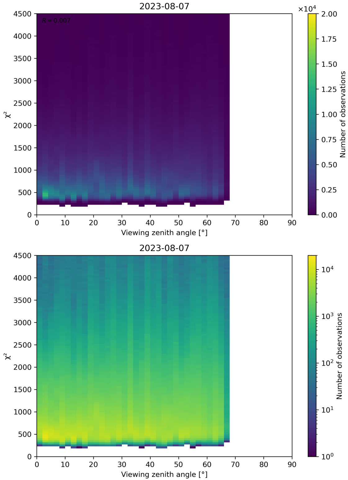
Figure 72: Scatter density plot of “Viewing zenith angle” against “ \chi^2 ” for 2023-08-06 to 2023-08-08.
