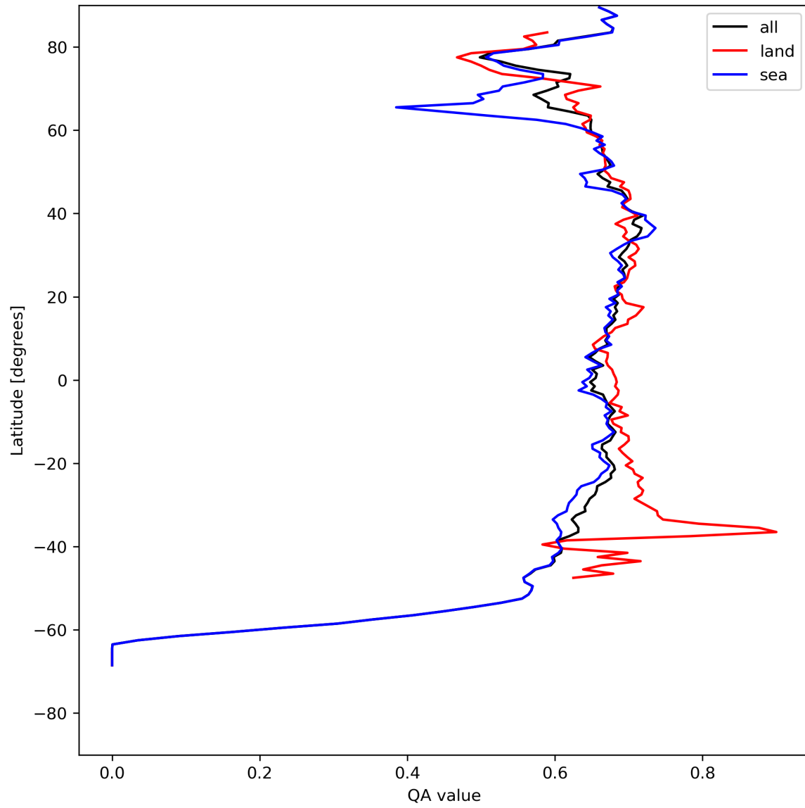
Figure 9: Zonal average of “QA value” for 2023-08-06 to 2023-08-08.
