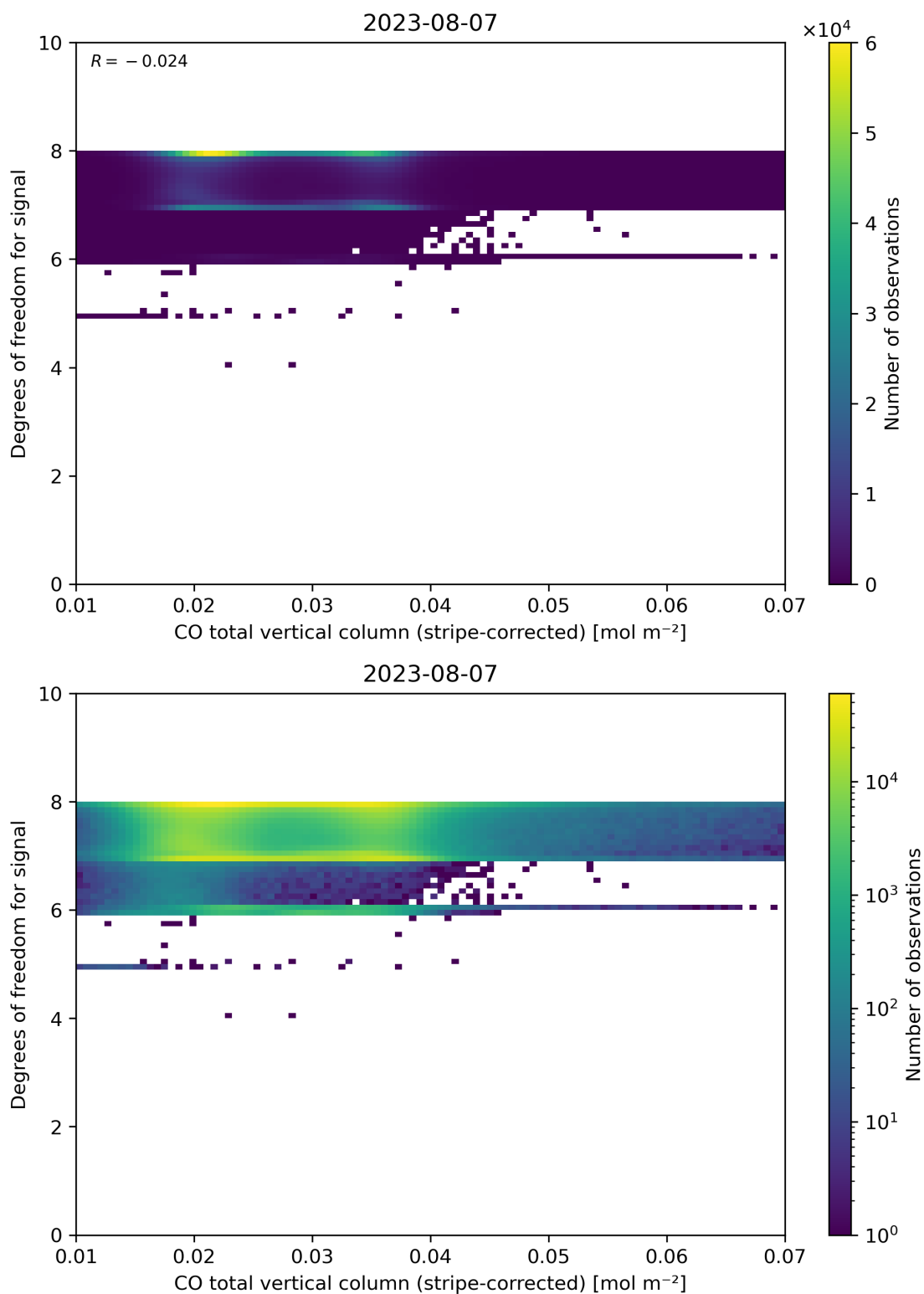
Figure 38: Scatter density plot of “CO total vertical column (stripe-corrected)” against “Degrees of freedom for signal” for 2023-08-06 to 2023-08-08.
