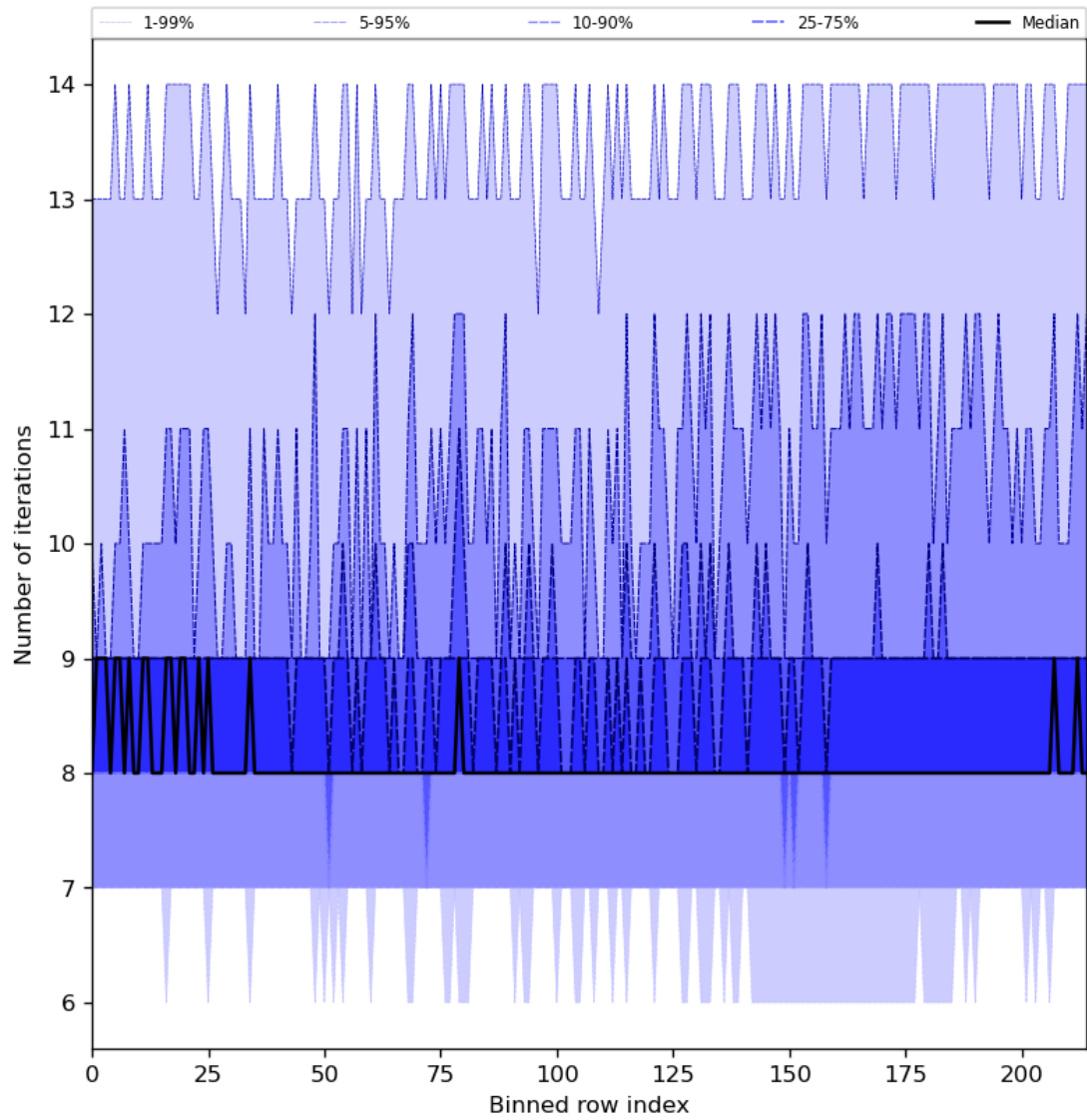
Figure 32: Along track statistics of “Number of iterations” for 2023-08-06 to 2023-08-08
