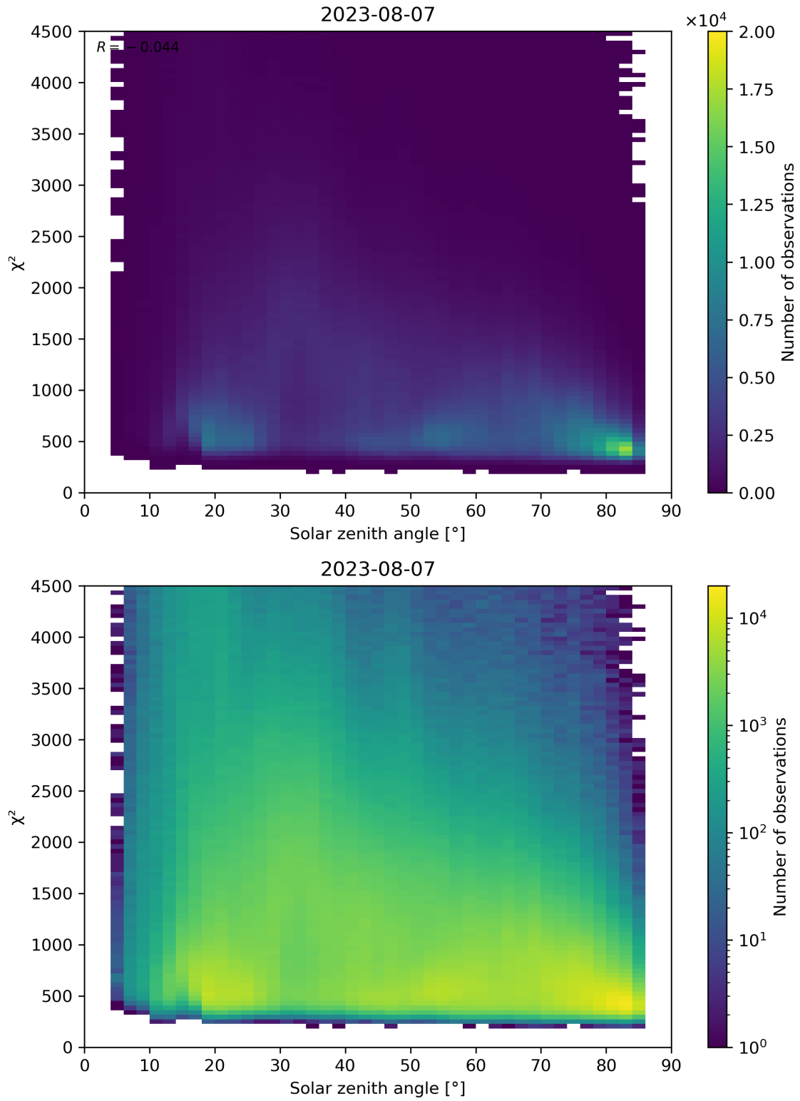
Figure 64: Scatter density plot of “Solar zenith angle” against “ \chi^2 ” for 2023-08-06 to 2023-08-08.
