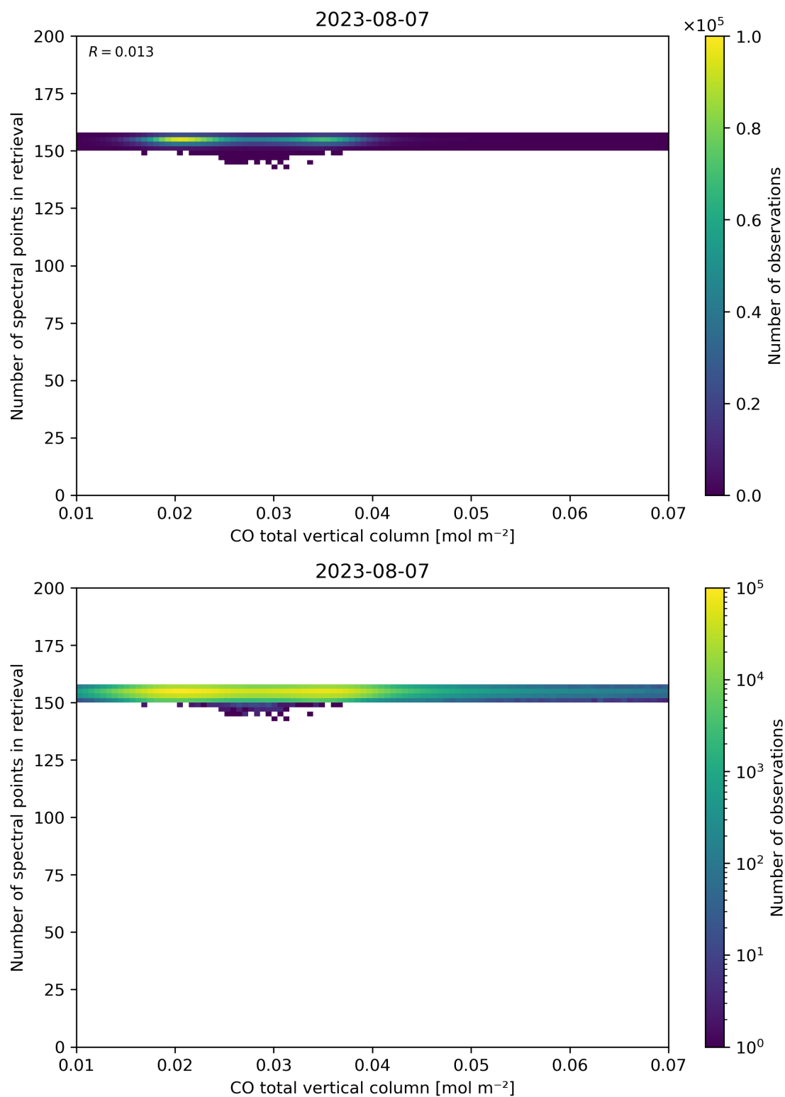
Figure 43: Scatter density plot of “CO total vertical column” against “Number of spectral points in retrieval” for 2023-08-06 to 2023-08-08.
