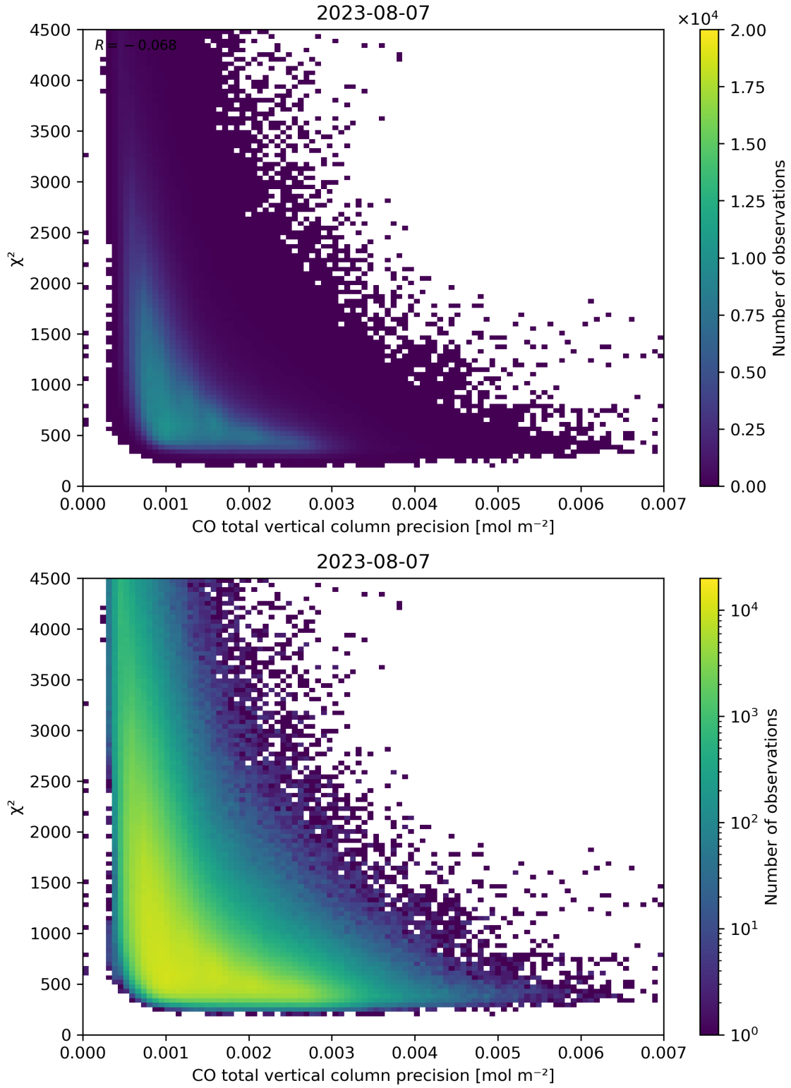
Figure 44: Scatter density plot of “CO total vertical column precision” against “ \chi^2 ” for 2023-08-06 to 2023-08-08.
