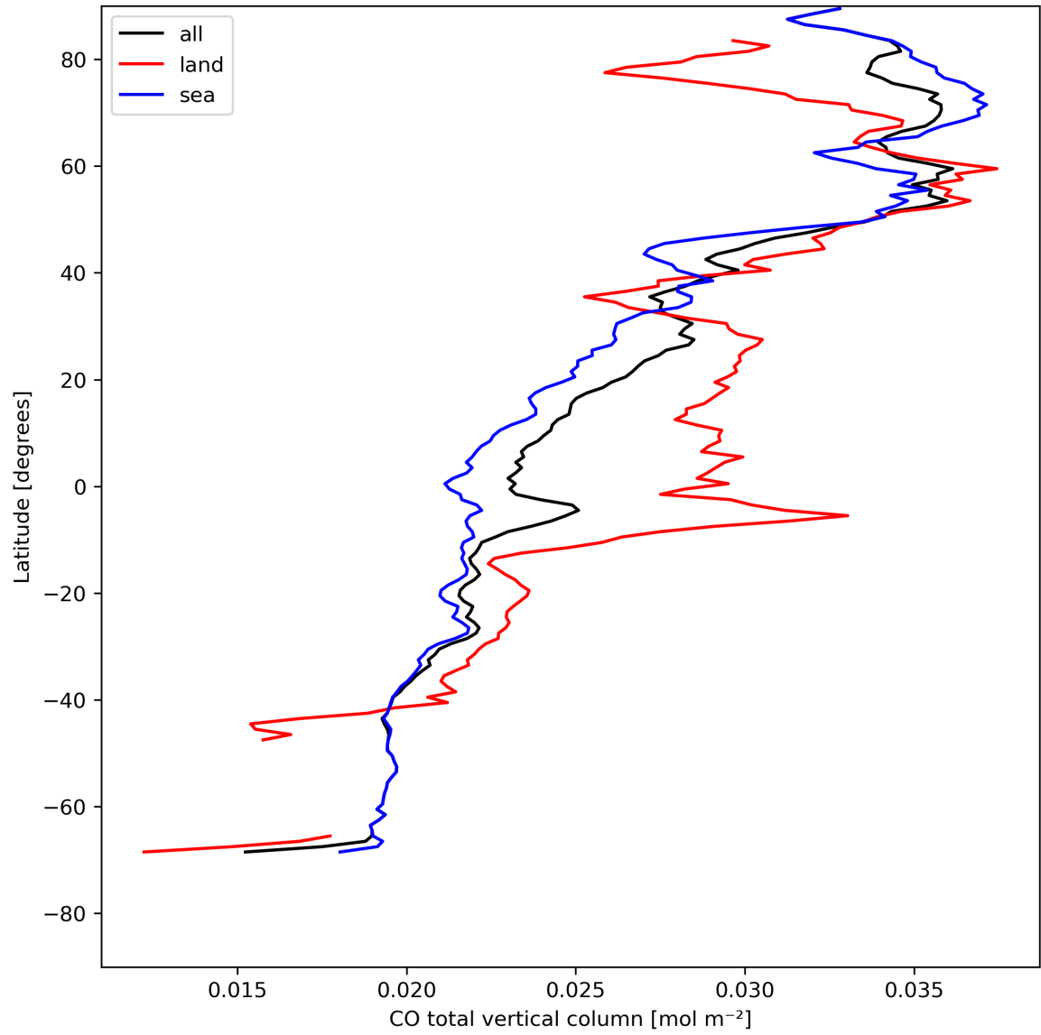
Figure 10: Zonal average of “CO total vertical column” for 2023-08-06 to 2023-08-08.
