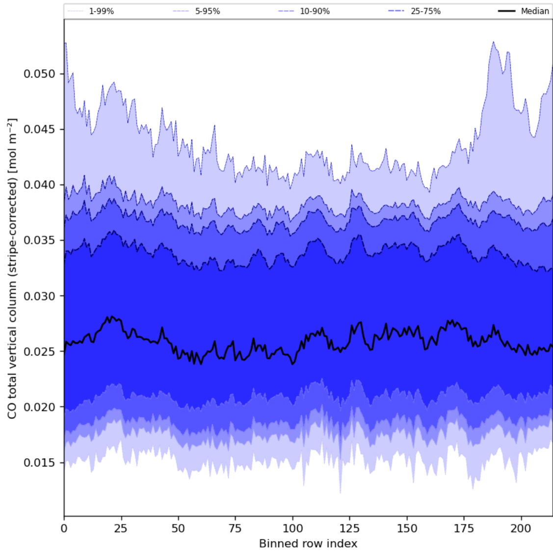
Figure 27: Along track statistics of “CO total vertical column (stripe-corrected)” for 2023-08-06 to 2023-08-08
