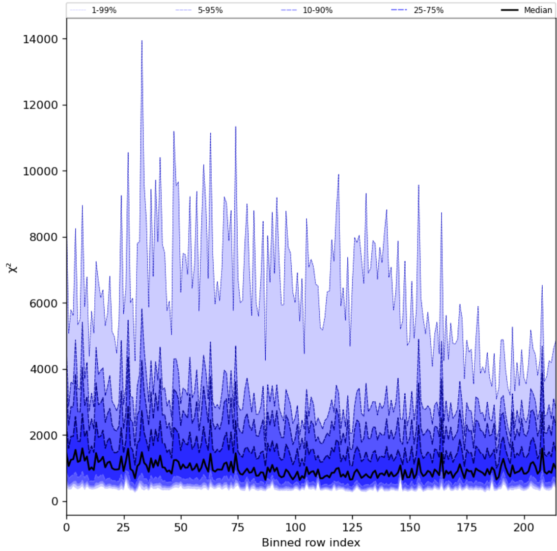
Figure 30: Along track statistics of “ \chi^2 ” for 2023-08-06 to 2023-08-08
