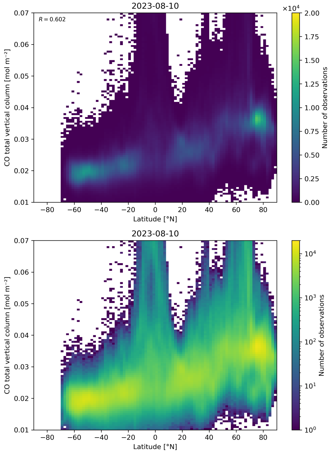
Figure 51: Scatter density plot of “Latitude” against “CO total vertical column” for 2023-08-09 to 2023-08-11.
