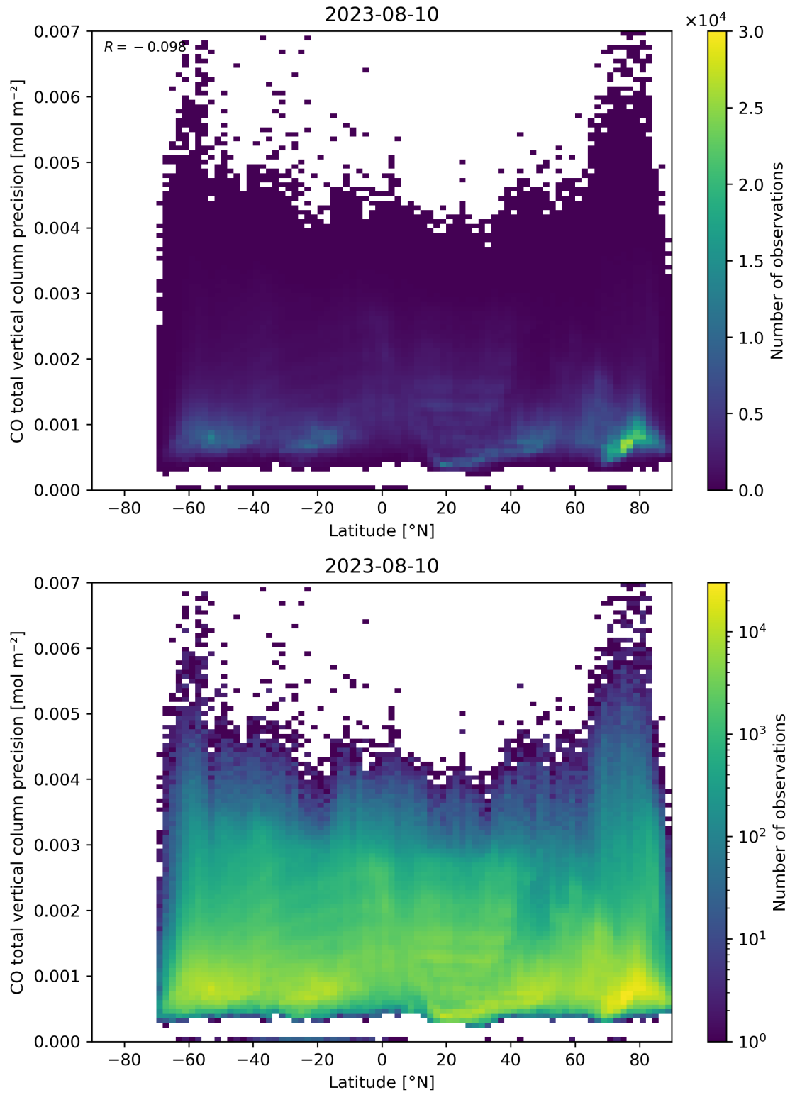
Figure 53: Scatter density plot of “Latitude” against “CO total vertical column precision” for 2023-08-09 to 2023-08-11.
