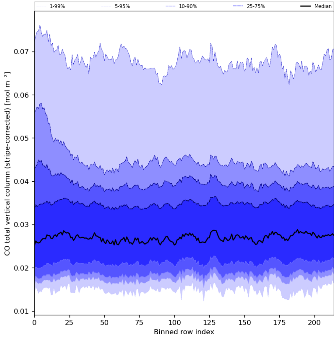
Figure 27: Along track statistics of “CO total vertical column (stripe-corrected)” for 2023-08-09 to 2023-08-11
