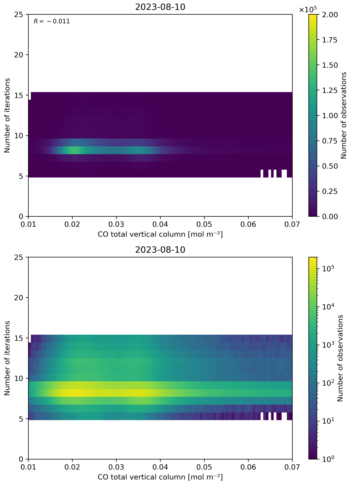
Figure 42: Scatter density plot of “CO total vertical column” against “Number of iterations” for 2023-08-09 to 2023-08-11.
