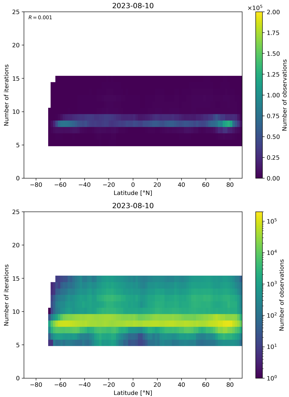
Figure 56: Scatter density plot of “Latitude” against “Number of iterations” for 2023-08-09 to 2023-08-11.
