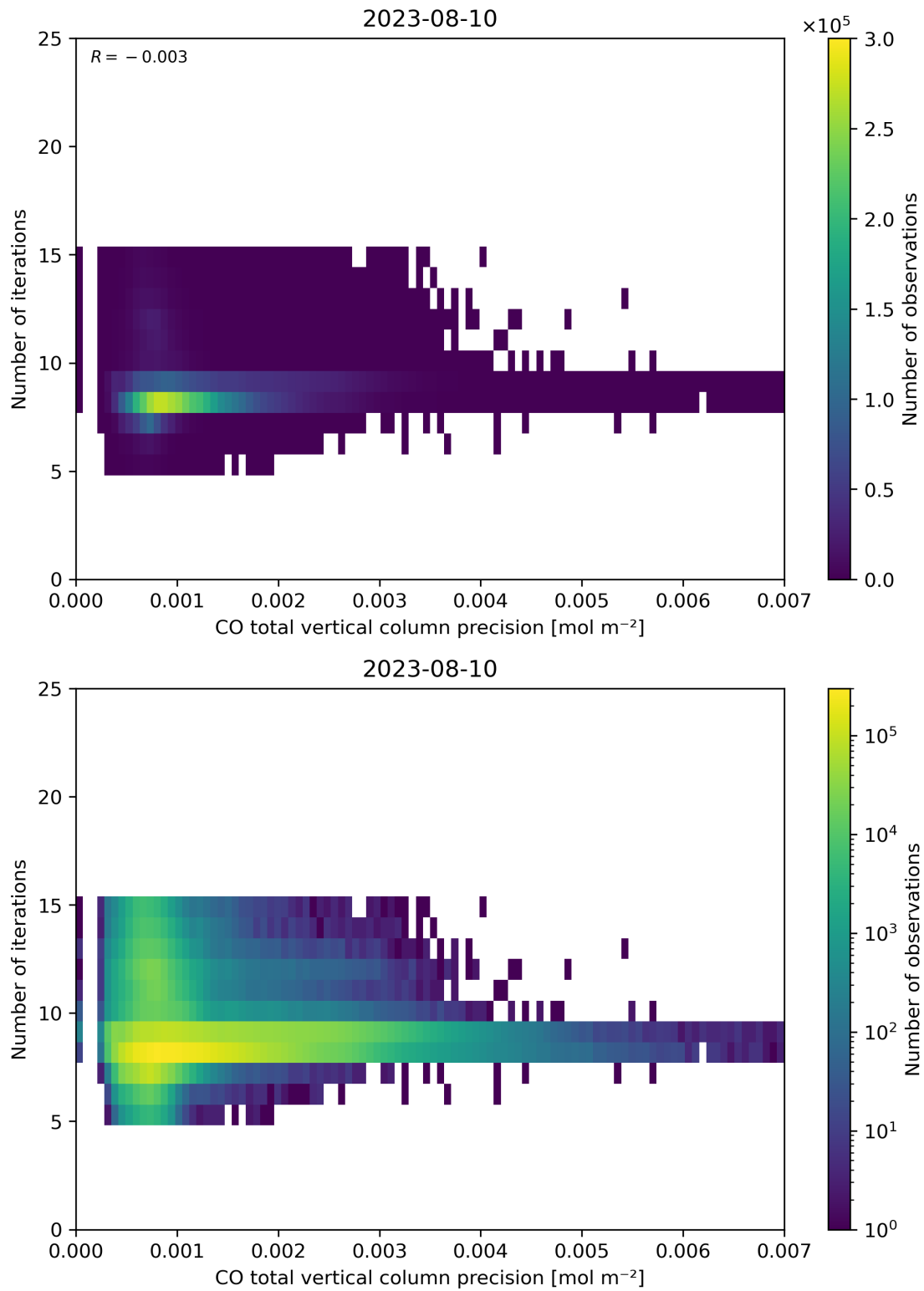
Figure 46: Scatter density plot of “CO total vertical column precision” against “Number of iterations” for 2023-08-09 to 2023-08-11.
