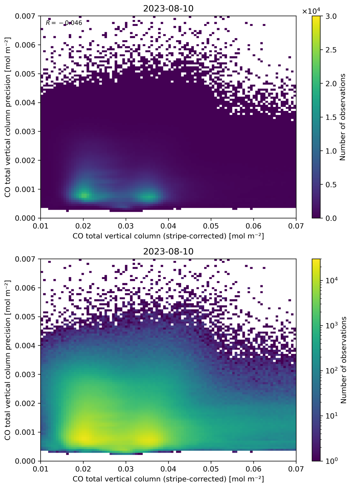
Figure 36: Scatter density plot of “CO total vertical column (stripe-corrected)” against “CO total vertical column precision” for 2023-08-09 to 2023-08-11.
