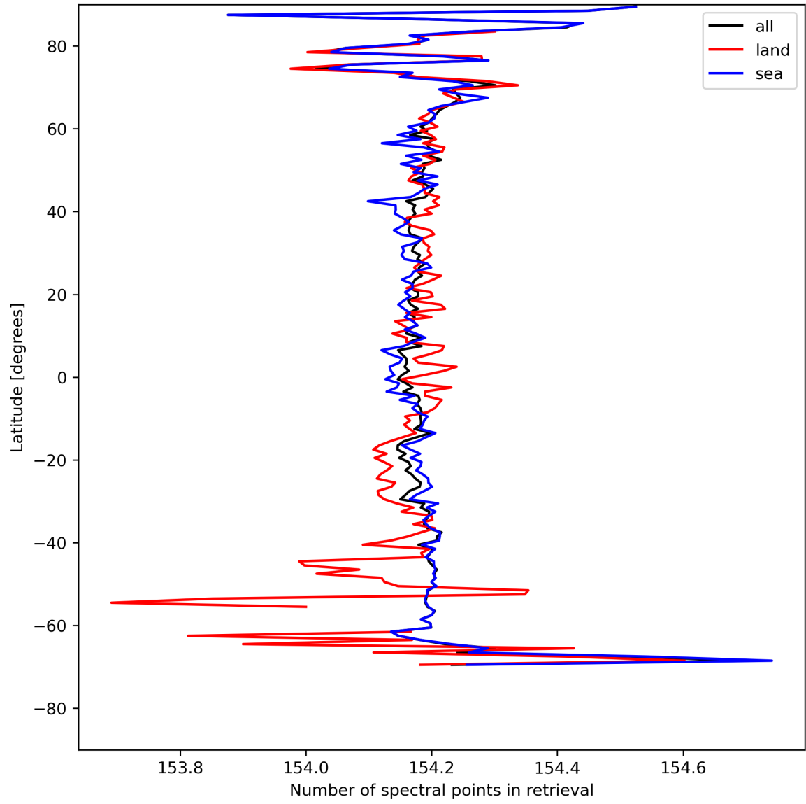
Figure 13: Zonal average of “Number of spectral points in retrieval” for 2023-08-09 to 2023-08-11.
