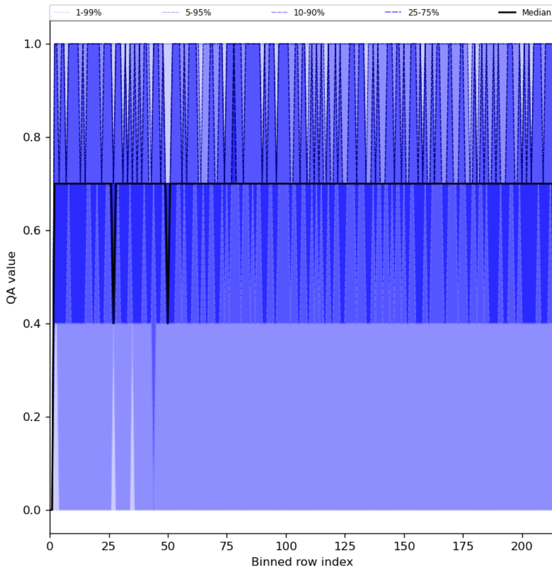
Figure 25: Along track statistics of “QA value” for 2023-08-09 to 2023-08-11
