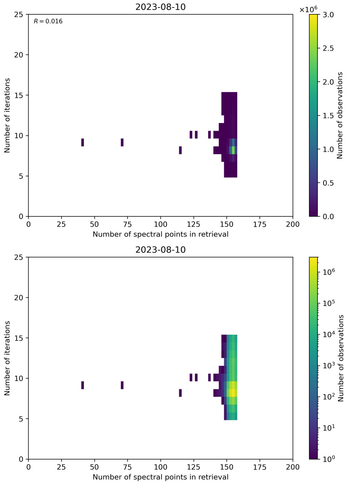
Figure 60: Scatter density plot of “Number of spectral points in retrieval” against “Number of iterations” for 2023-08-09 to 2023-08-11.
