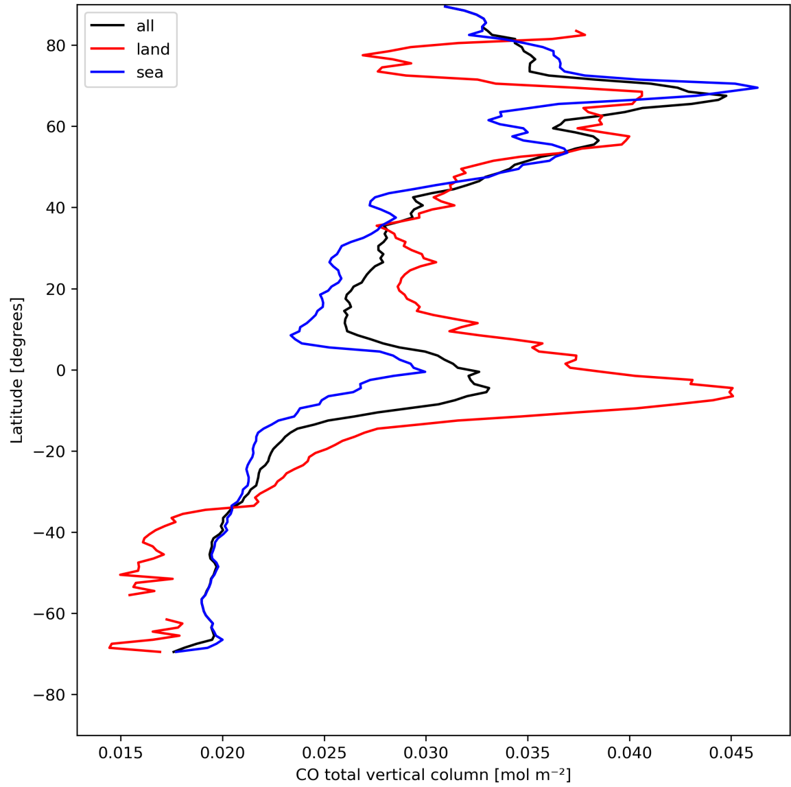
Figure 10: Zonal average of “CO total vertical column” for 2023-08-09 to 2023-08-11.
