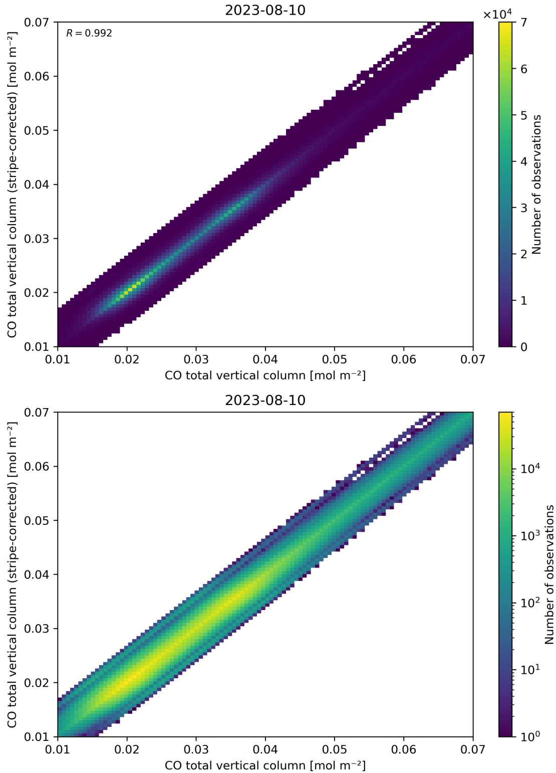
Figure 33: Scatter density plot of “CO total vertical column” against “CO total vertical column (stripe-corrected)” for 2023-08-09 to 2023-08-11.
