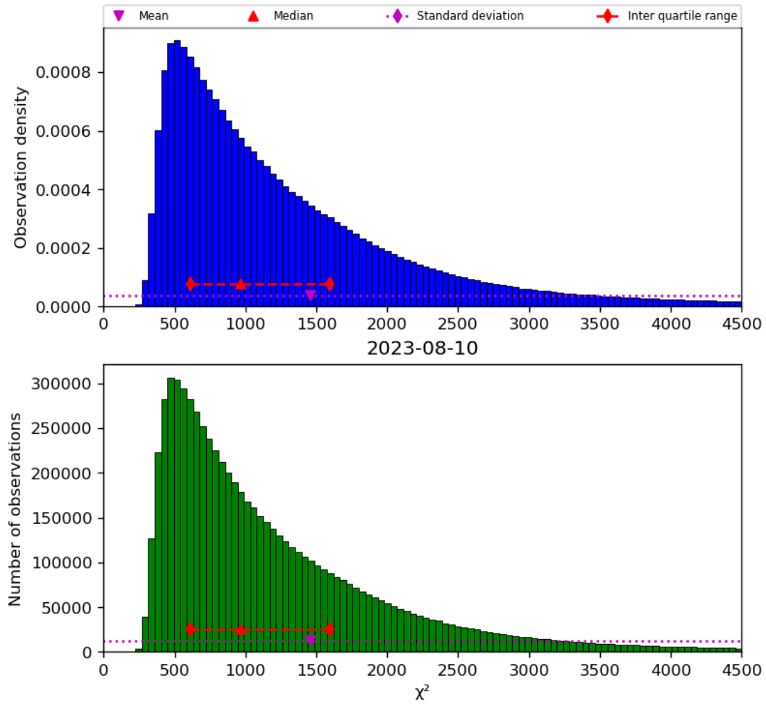
Figure 22: Histogram of “ \chi^2 ” for 2023-08-09 to 2023-08-11
