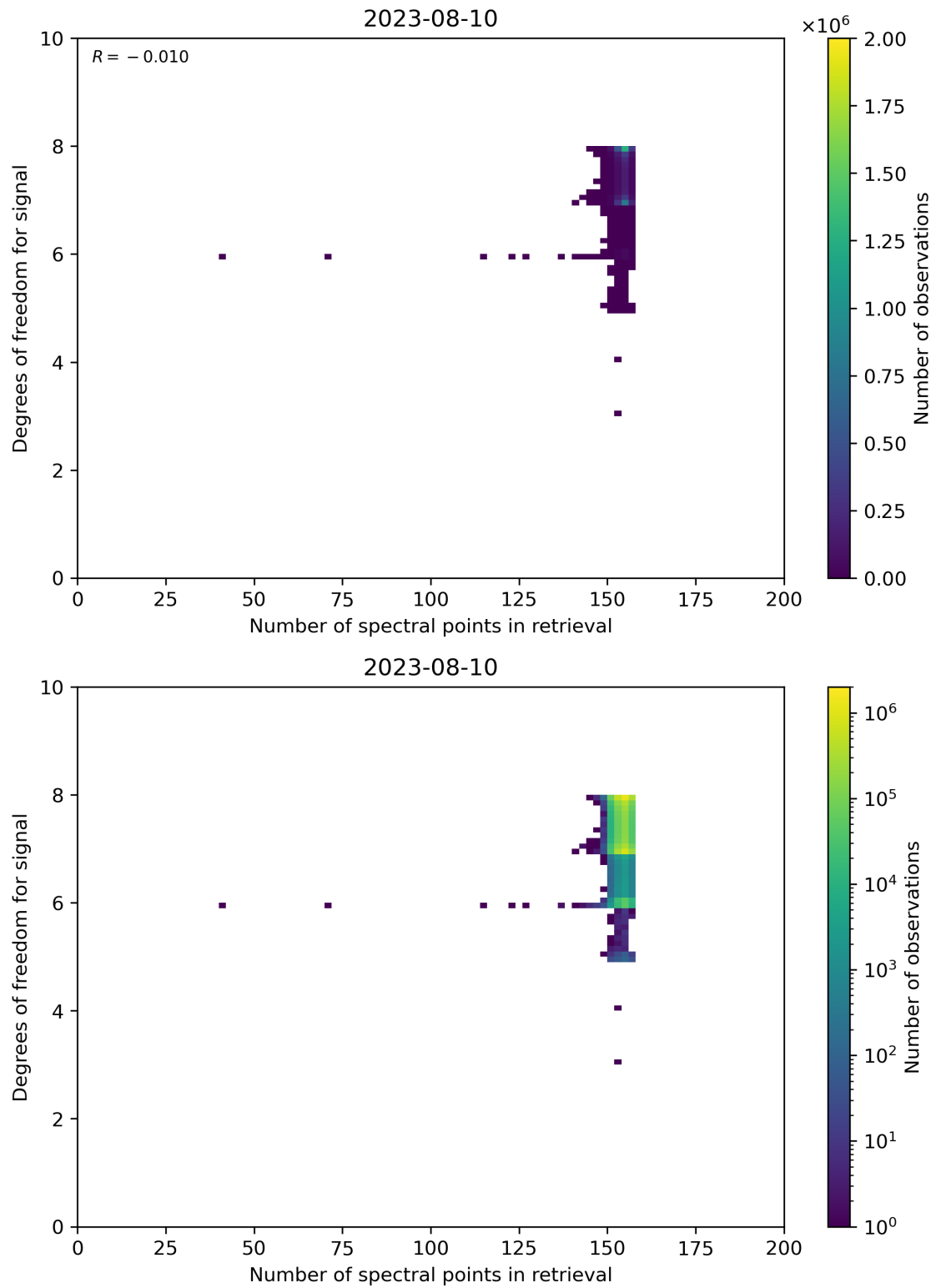
Figure 59: Scatter density plot of “Number of spectral points in retrieval” against “Degrees of freedom for signal” for 2023-08-09 to 2023-08-11.
