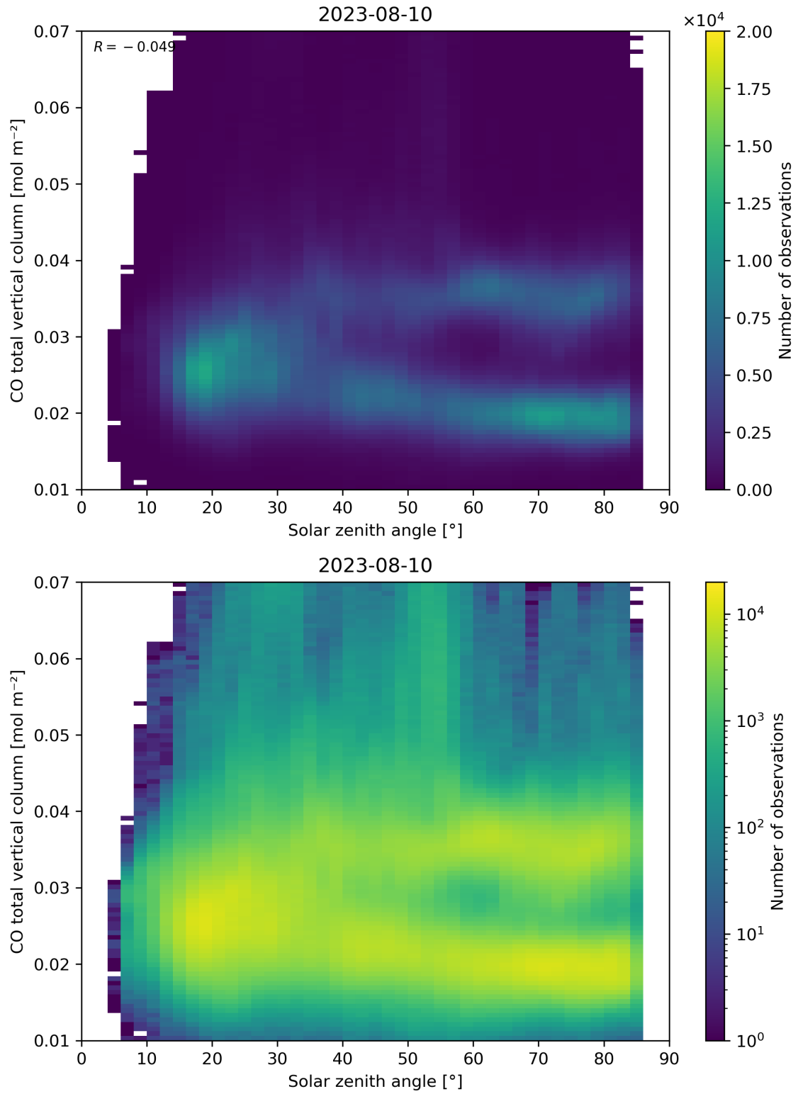
Figure 61: Scatter density plot of “Solar zenith angle” against “CO total vertical column” for 2023-08-09 to 2023-08-11.
