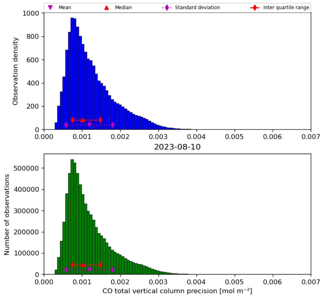
Figure 20: Histogram of “CO total vertical column precision” for 2023-08-09 to 2023-08-11
