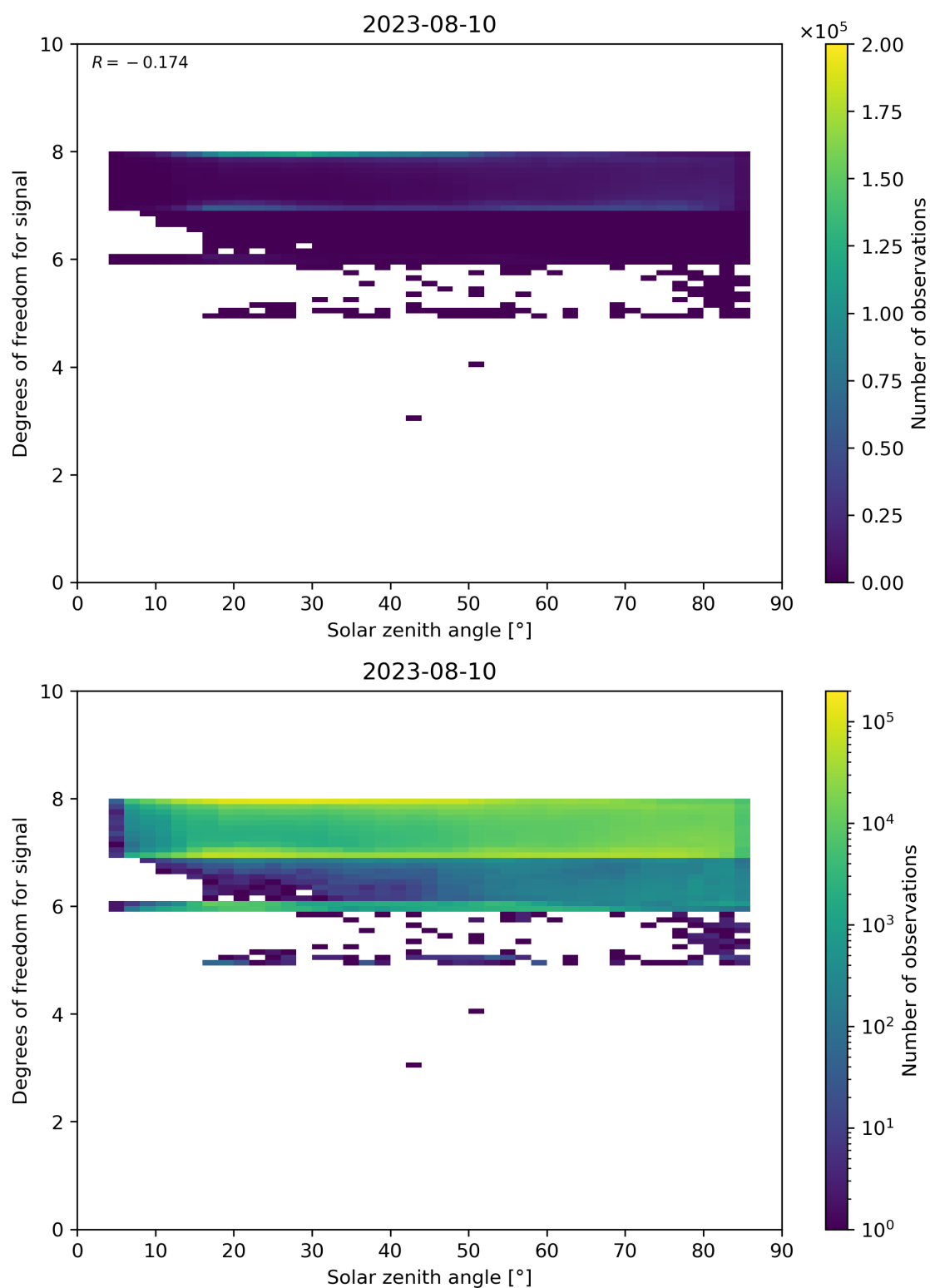
Figure 65: Scatter density plot of “Solar zenith angle” against “Degrees of freedom for signal” for 2023-08-09 to 2023-08-11.
