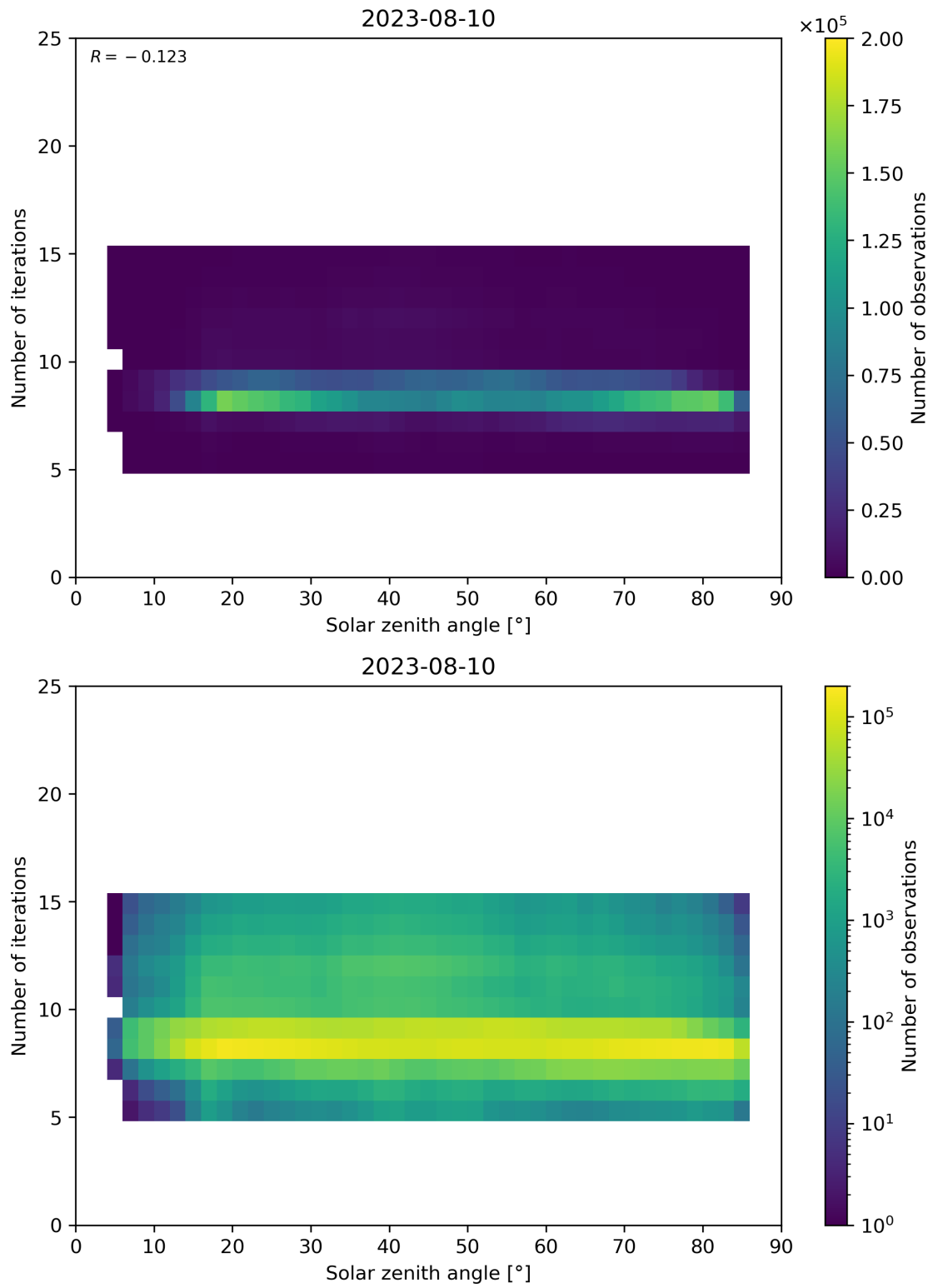
Figure 67: Scatter density plot of “Solar zenith angle” against “Number of iterations” for 2023-08-09 to 2023-08-11.
