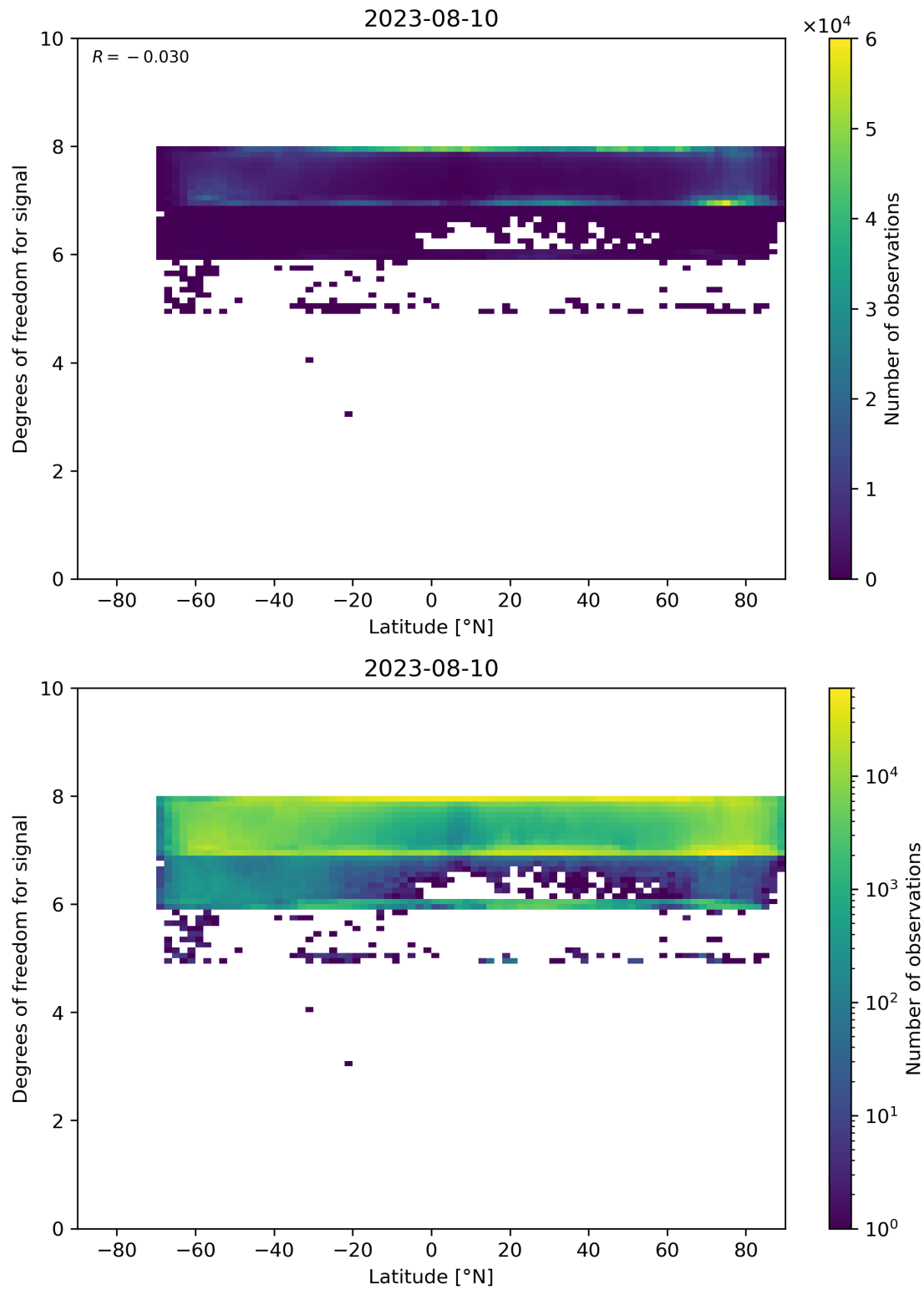
Figure 55: Scatter density plot of “Latitude” against “Degrees of freedom for signal” for 2023-08-09 to 2023-08-11.
