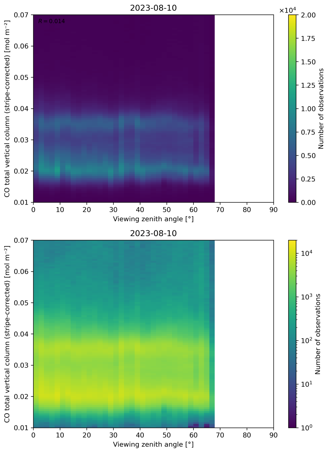
Figure 70: Scatter density plot of “Viewing zenith angle” against “CO total vertical column (stripe-corrected)” for 2023-08-09 to 2023-08-11.
