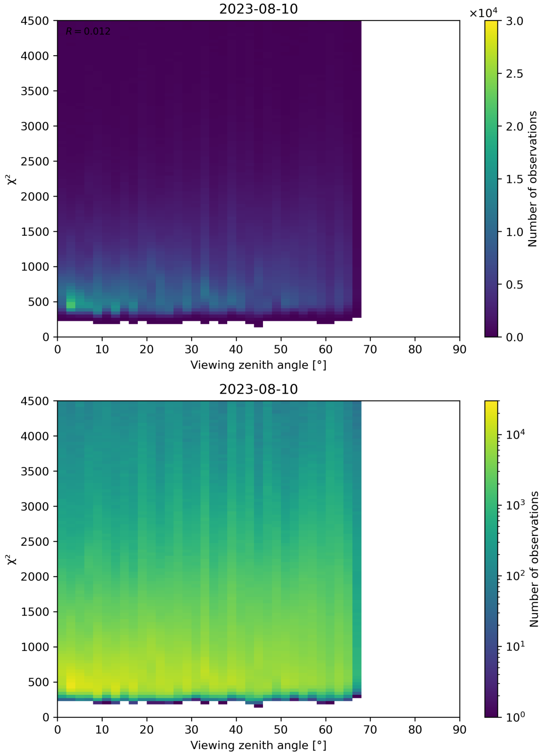
Figure 72: Scatter density plot of “Viewing zenith angle” against “ \chi^2 ” for 2023-08-09 to 2023-08-11.
