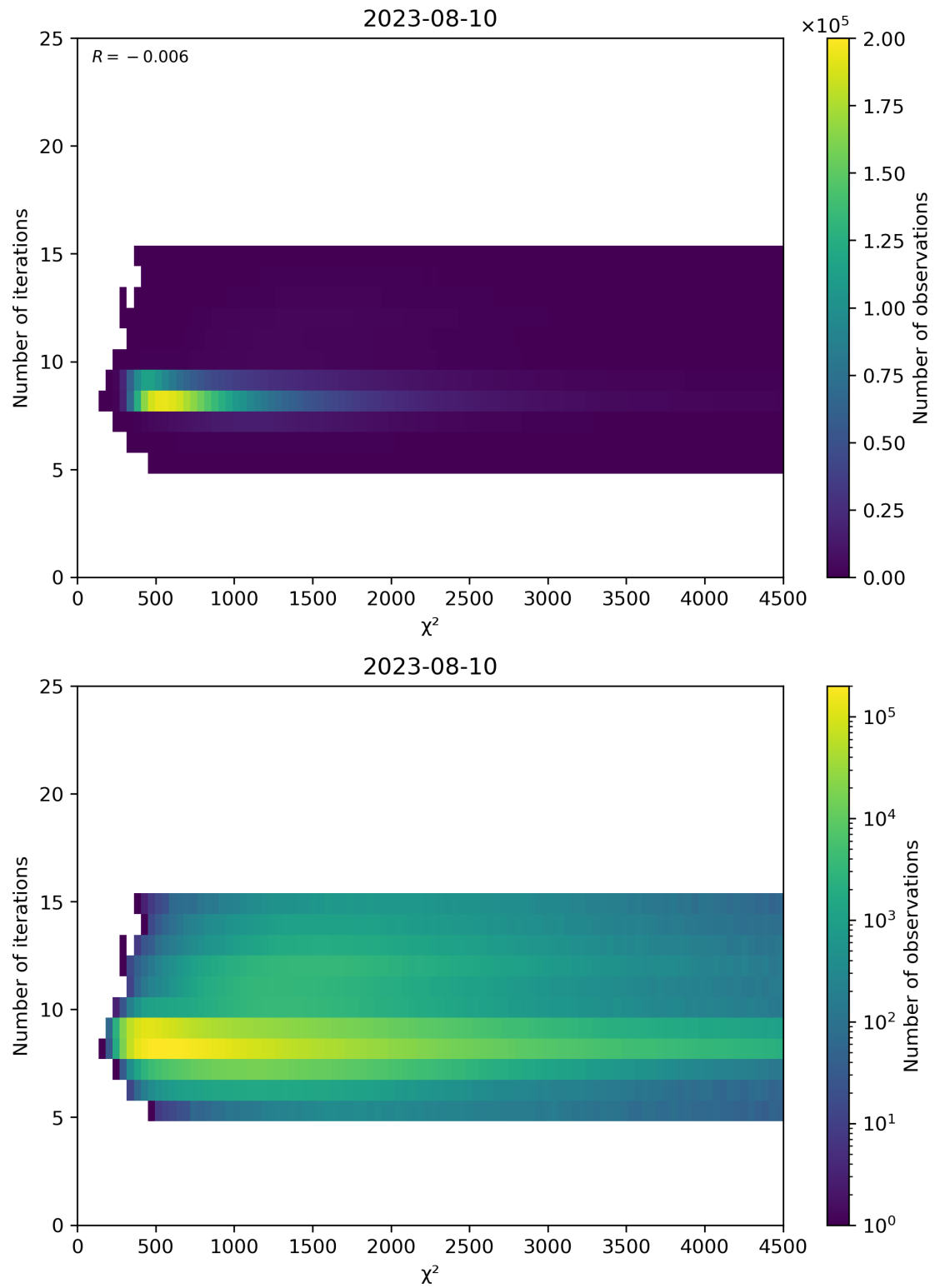
Figure 49: Scatter density plot of “ \chi^2 ” against “Number of iterations” for 2023-08-09 to 2023-08-11.
