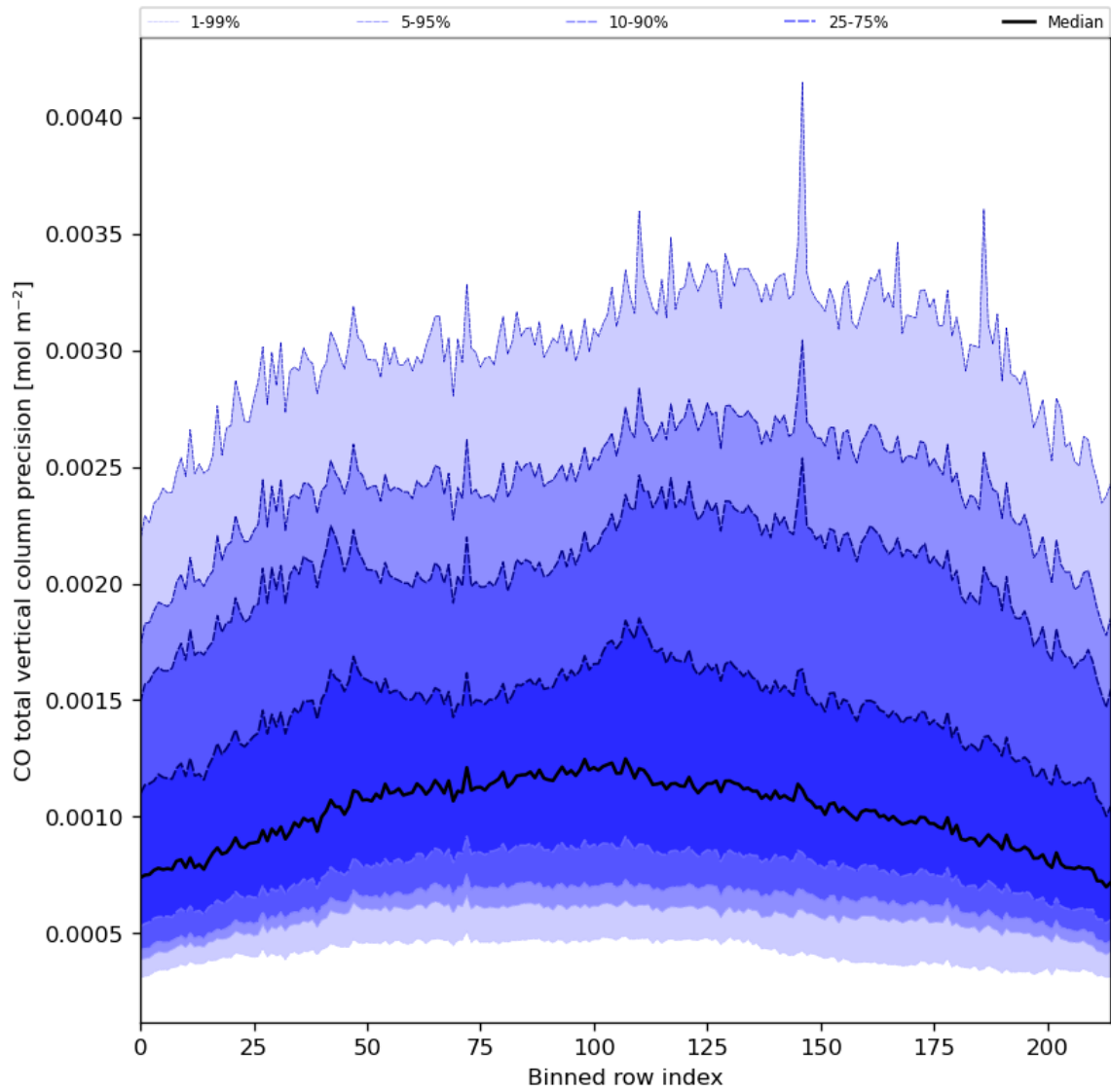
Figure 28: Along track statistics of “CO total vertical column precision” for 2023-08-09 to 2023-08-11
