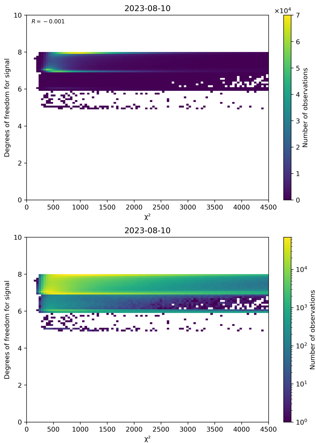
Figure 48: Scatter density plot of " \chi^2 " against "Degrees of freedom for signal" for 2023-08-09 to 2023-08-11.
