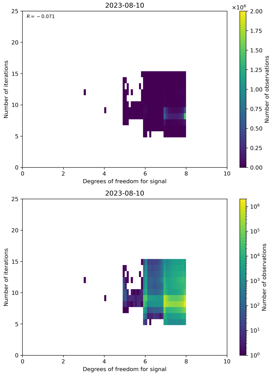
Figure 50: Scatter density plot of “Degrees of freedom for signal” against “Number of iterations” for 2023-08-09 to 2023-08-11.
