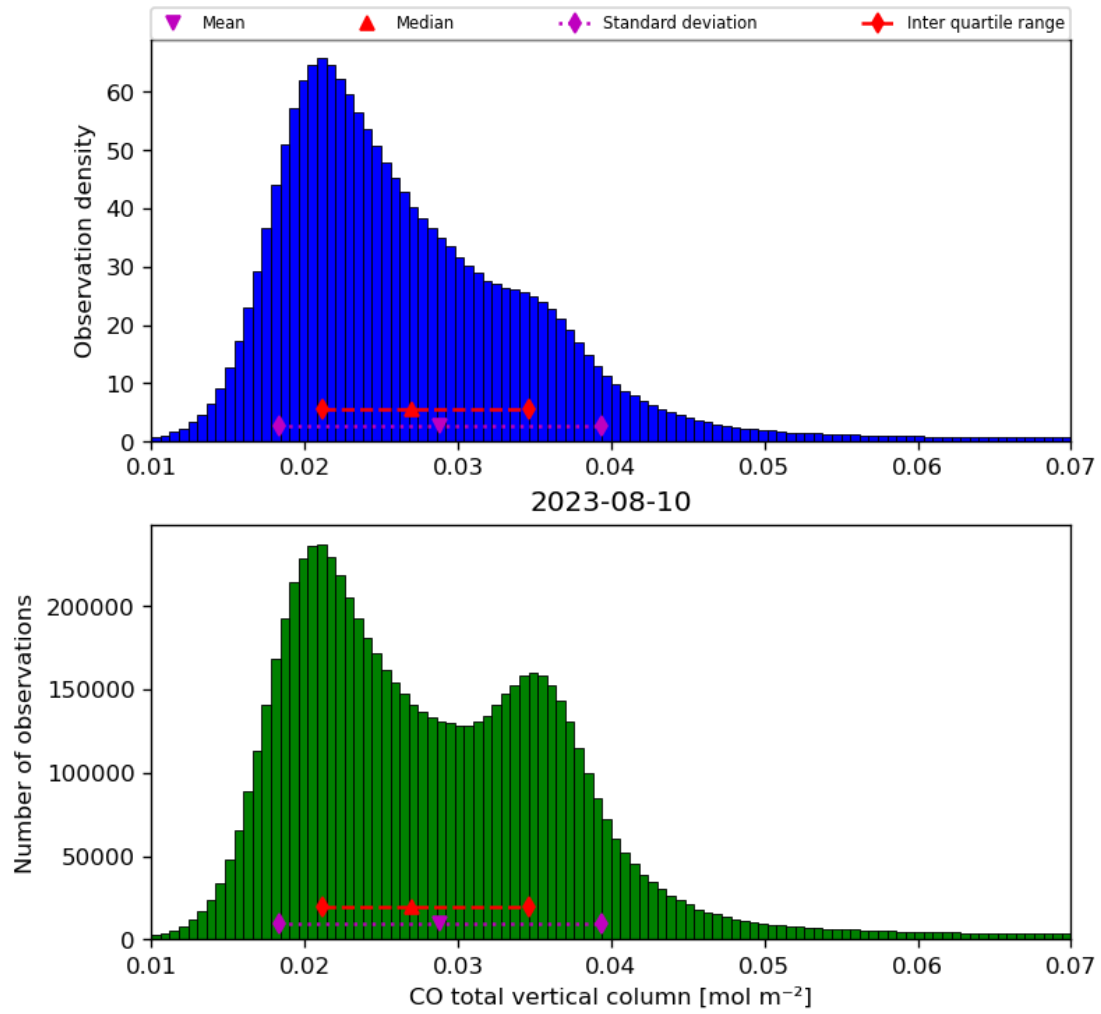
Figure 18: Histogram of “CO total vertical column” for 2023-08-09 to 2023-08-11
