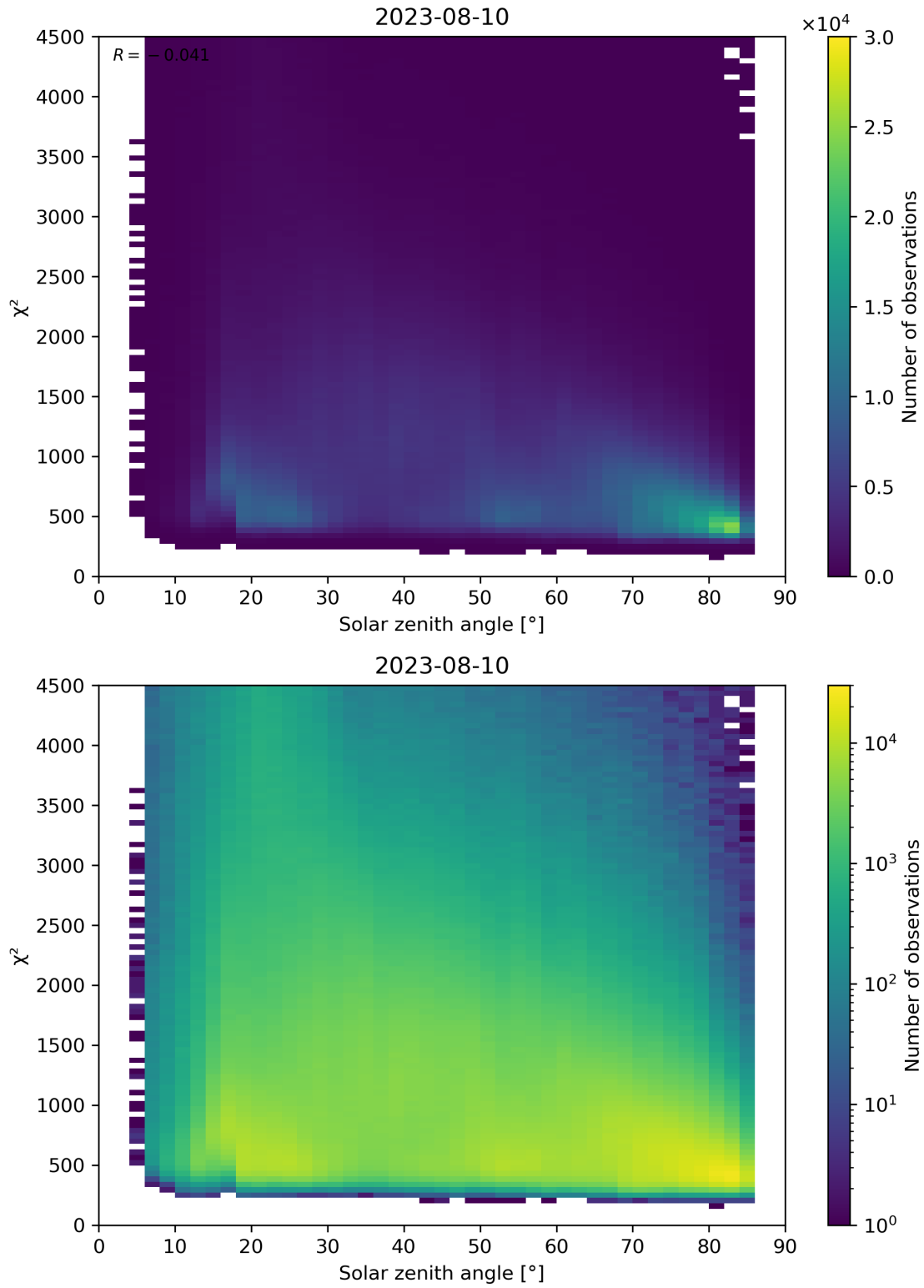
Figure 64: Scatter density plot of “Solar zenith angle” against “ \chi^2 ” for 2023-08-09 to 2023-08-11.
