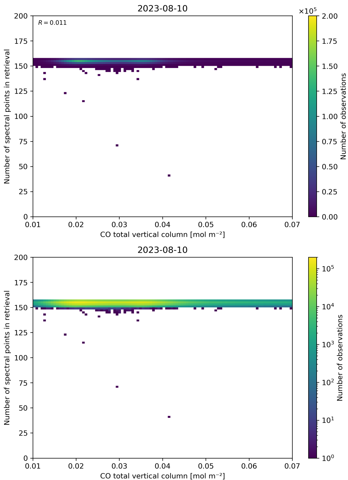
Figure 43: Scatter density plot of “CO total vertical column” against “Number of spectral points in retrieval” for 2023-08-09 to 2023-08-11.
