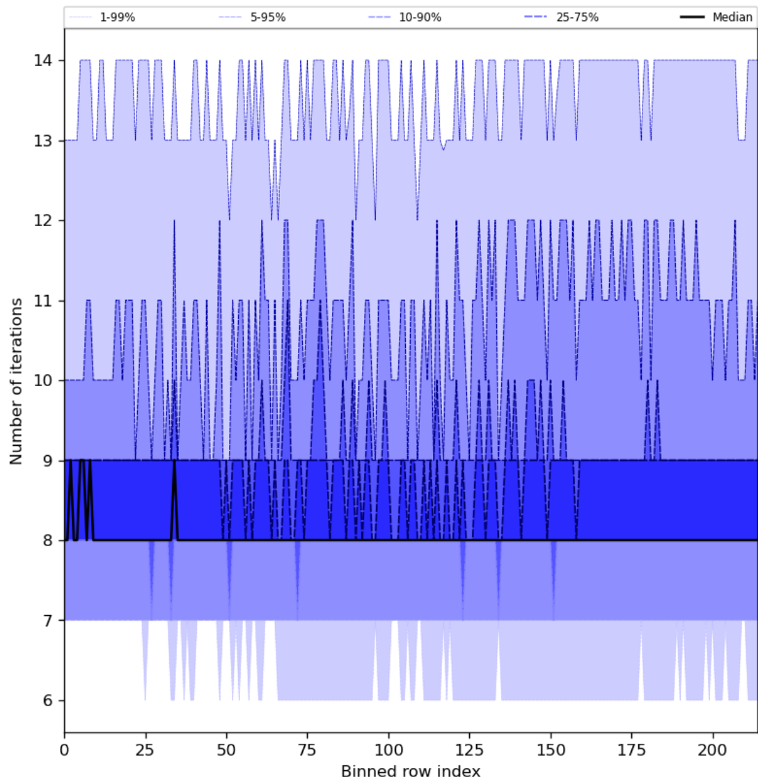
Figure 32: Along track statistics of “Number of iterations” for 2023-08-09 to 2023-08-11
