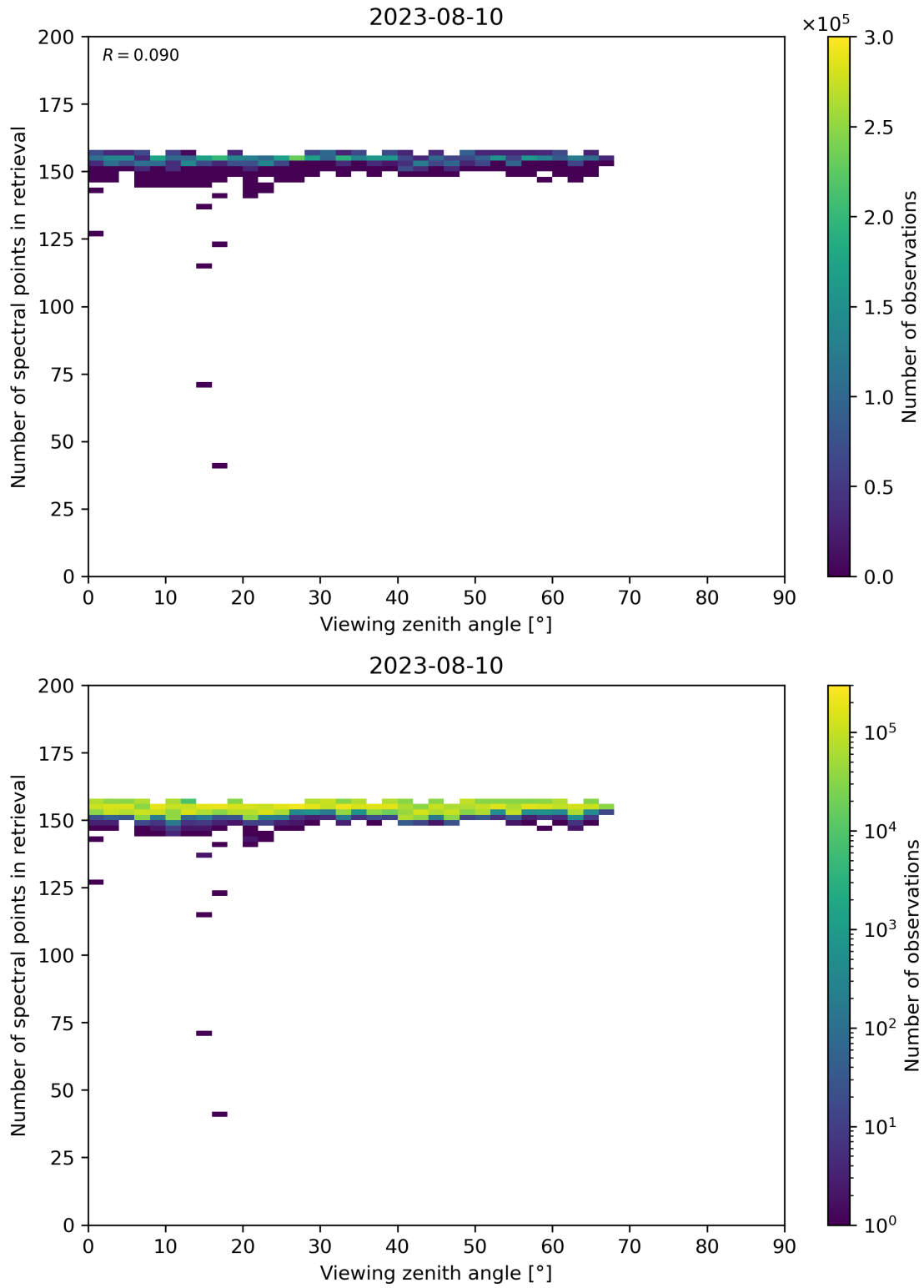
Figure 76: Scatter density plot of “Viewing zenith angle” against “Number of spectral points in retrieval” for 2023-08-09 to 2023-08-11.
