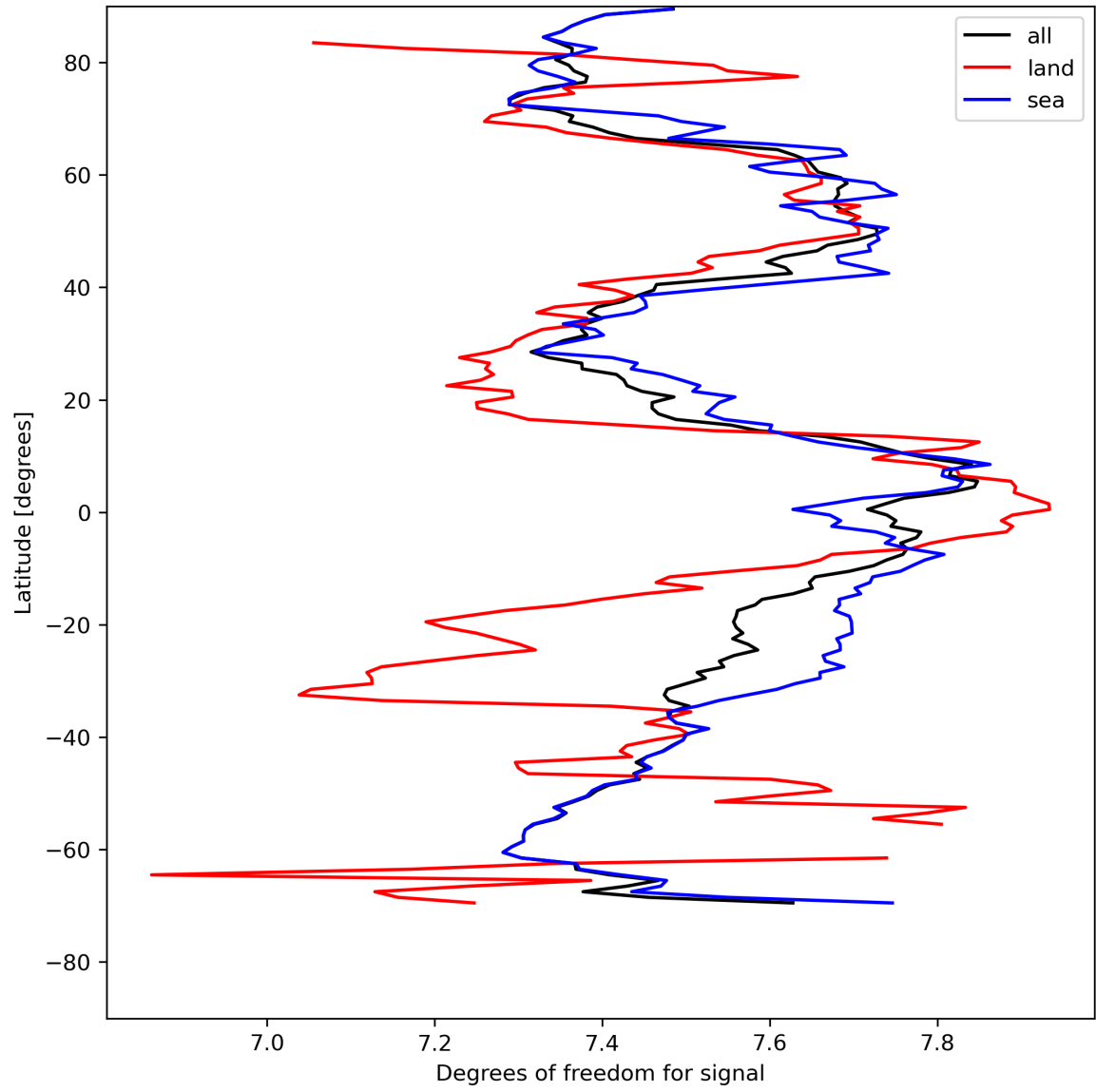
Figure 15: Zonal average of “Degrees of freedom for signal” for 2023-08-09 to 2023-08-11.
