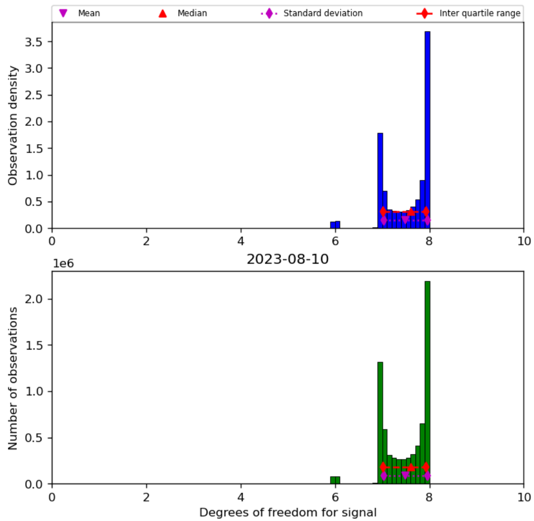
Figure 23: Histogram of “Degrees of freedom for signal” for 2023-08-09 to 2023-08-11
