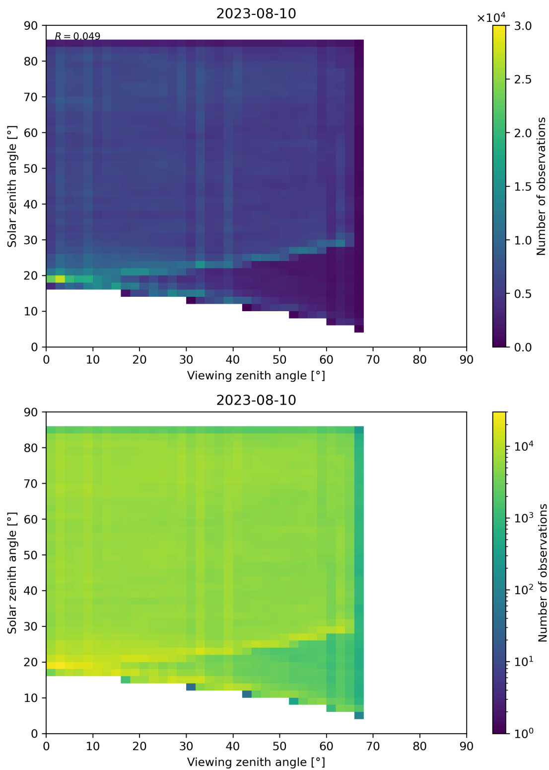
Figure 77: Scatter density plot of “Viewing zenith angle” against “Solar zenith angle” for 2023-08-09 to 2023-08-11.
