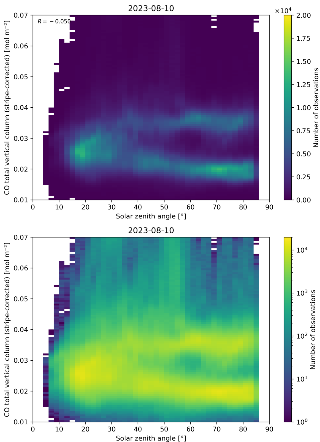
Figure 62: Scatter density plot of “Solar zenith angle” against “CO total vertical column (stripe-corrected)” for 2023-08-09 to 2023-08-11.
