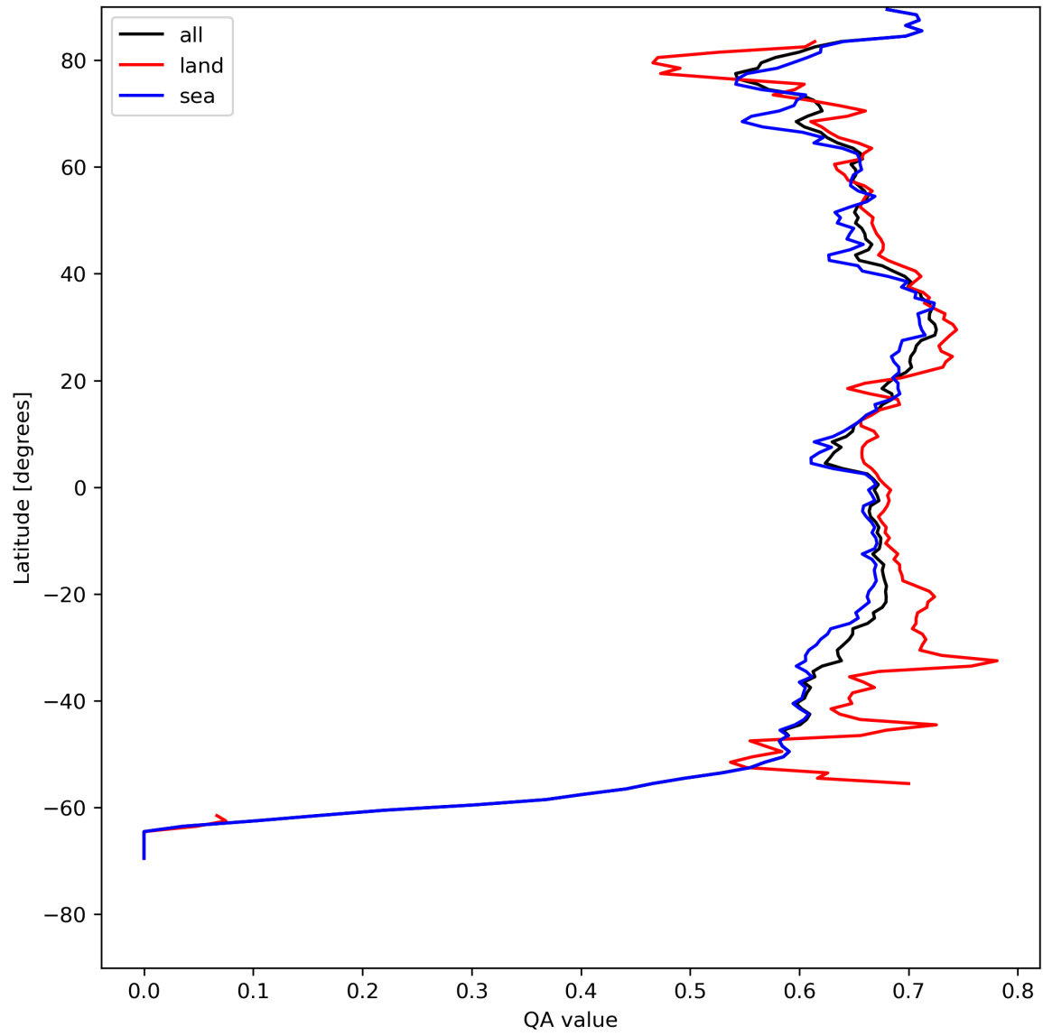
Figure 9: Zonal average of “QA value” for 2023-08-09 to 2023-08-11.
