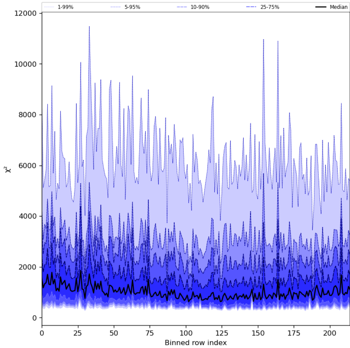
Figure 30: Along track statistics of “ \chi^2 ” for 2023-08-09 to 2023-08-11
