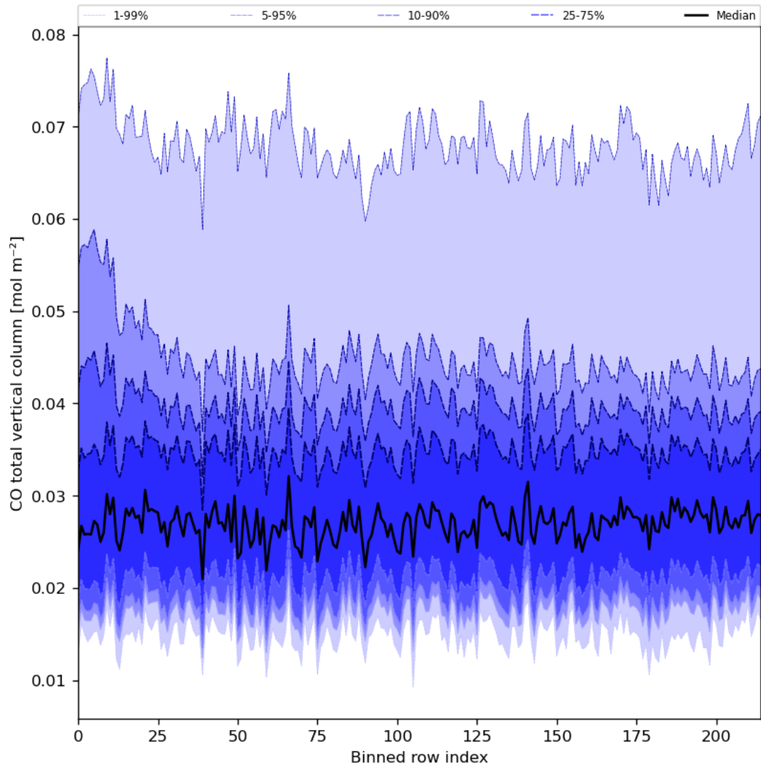
Figure 26: Along track statistics of “CO total vertical column” for 2023-08-09 to 2023-08-11
