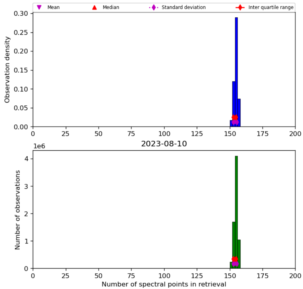
Figure 21: Histogram of “Number of spectral points in retrieval” for 2023-08-09 to 2023-08-11
