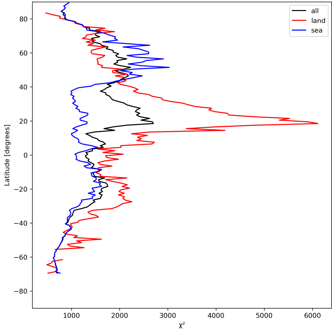
Figure 14: Zonal average of “ \chi^2 ” for 2023-08-09 to 2023-08-11.
