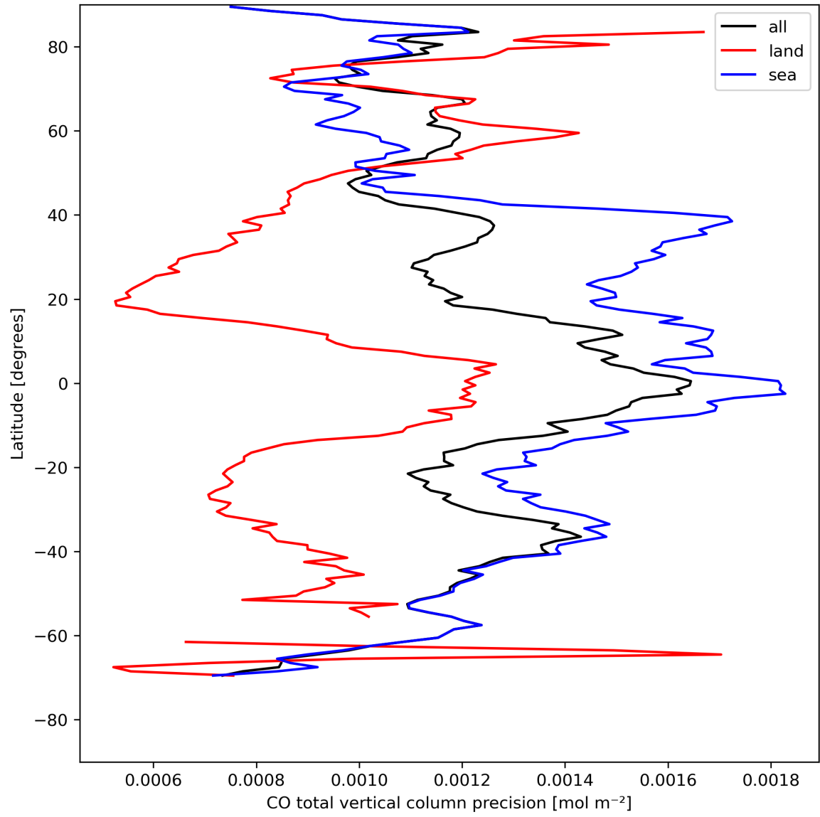
Figure 12: Zonal average of “CO total vertical column precision” for 2023-08-09 to 2023-08-11.
