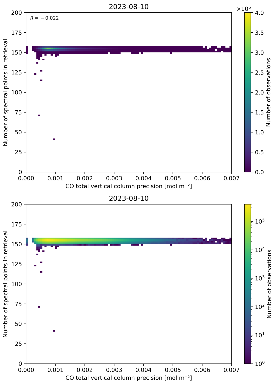
Figure 47: Scatter density plot of “CO total vertical column precision” against “Number of spectral points in retrieval” for 2023-08-09 to 2023-08-11.
