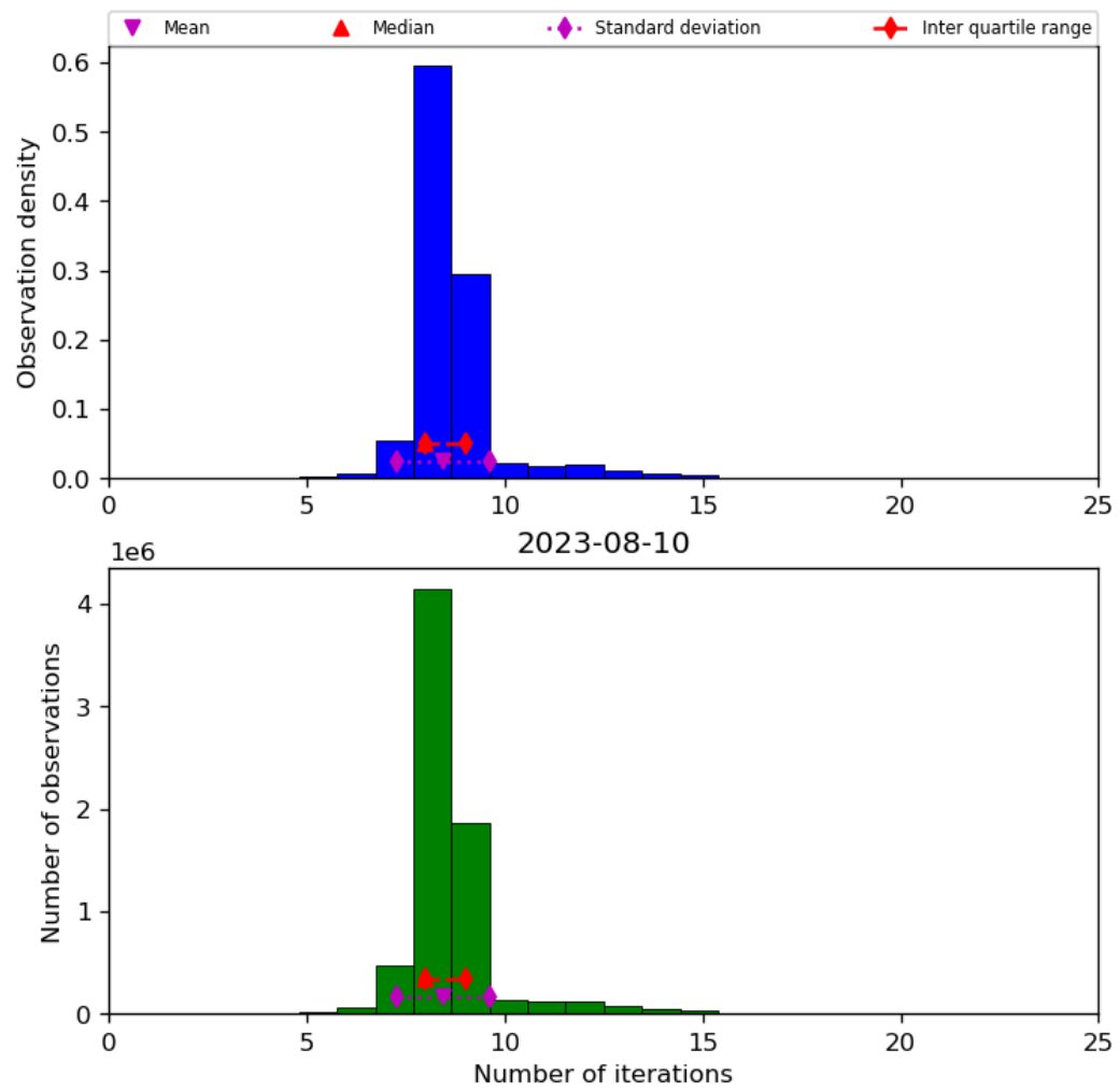
Figure 24: Histogram of “Number of iterations” for 2023-08-09 to 2023-08-11
