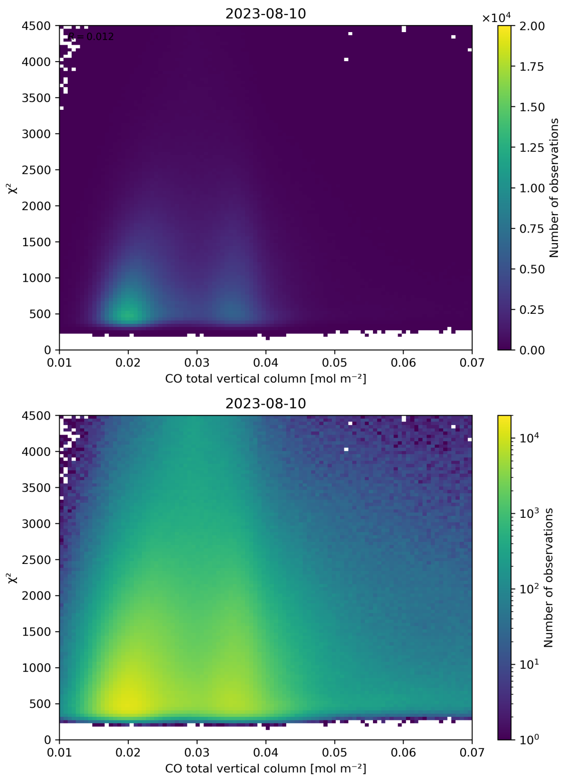
Figure 35: Scatter density plot of “CO total vertical column” against “ \chi^2 ” for 2023-08-09 to 2023-08-11.
