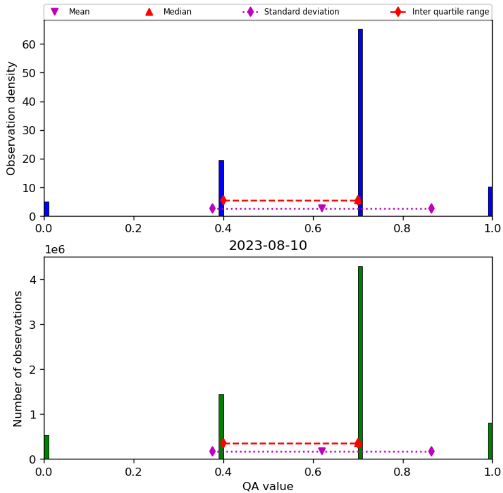
Figure 17: Histogram of “QA value” for 2023-08-09 to 2023-08-11
