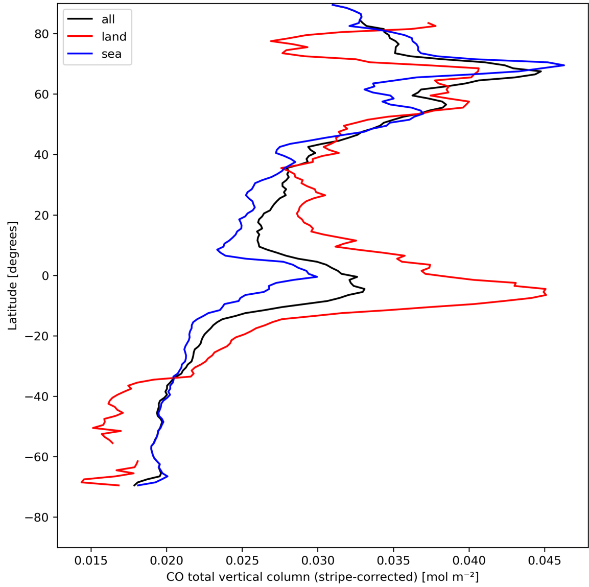
Figure 11: Zonal average of “CO total vertical column (stripe-corrected)” for 2023-08-09 to 2023-08-11.
