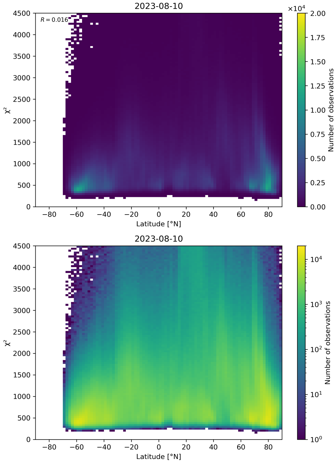
Figure 54: Scatter density plot of “Latitude” against “ \chi^2 ” for 2023-08-09 to 2023-08-11.
