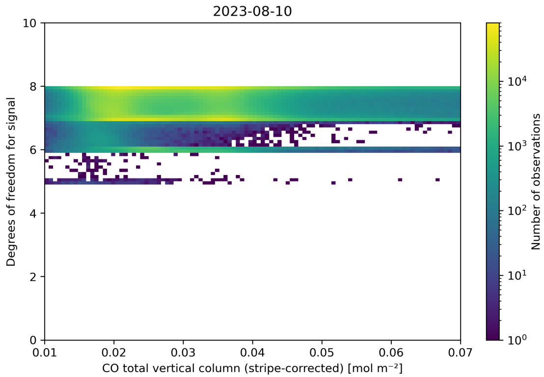
Figure 38: Scatter density plot of “CO total vertical column (stripe-corrected)” against “Degrees of freedom for signal” for 2023-08-09 to 2023-08-11.
