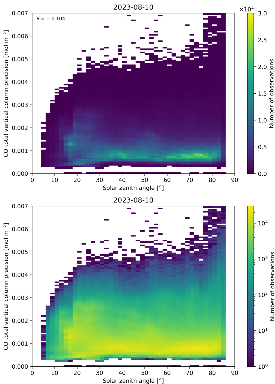
Figure 63: Scatter density plot of “Solar zenith angle” against “CO total vertical column precision” for 2023-08-09 to 2023-08-11.
