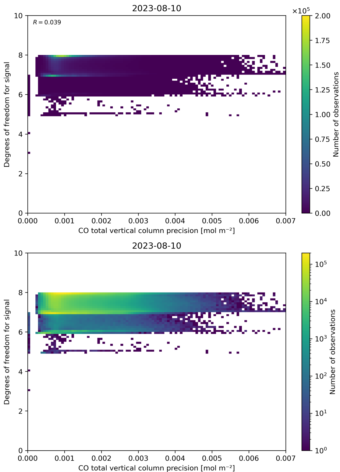
Figure 45: Scatter density plot of “CO total vertical column precision” against “Degrees of freedom for signal” for 2023-08-09 to 2023-08-11.
