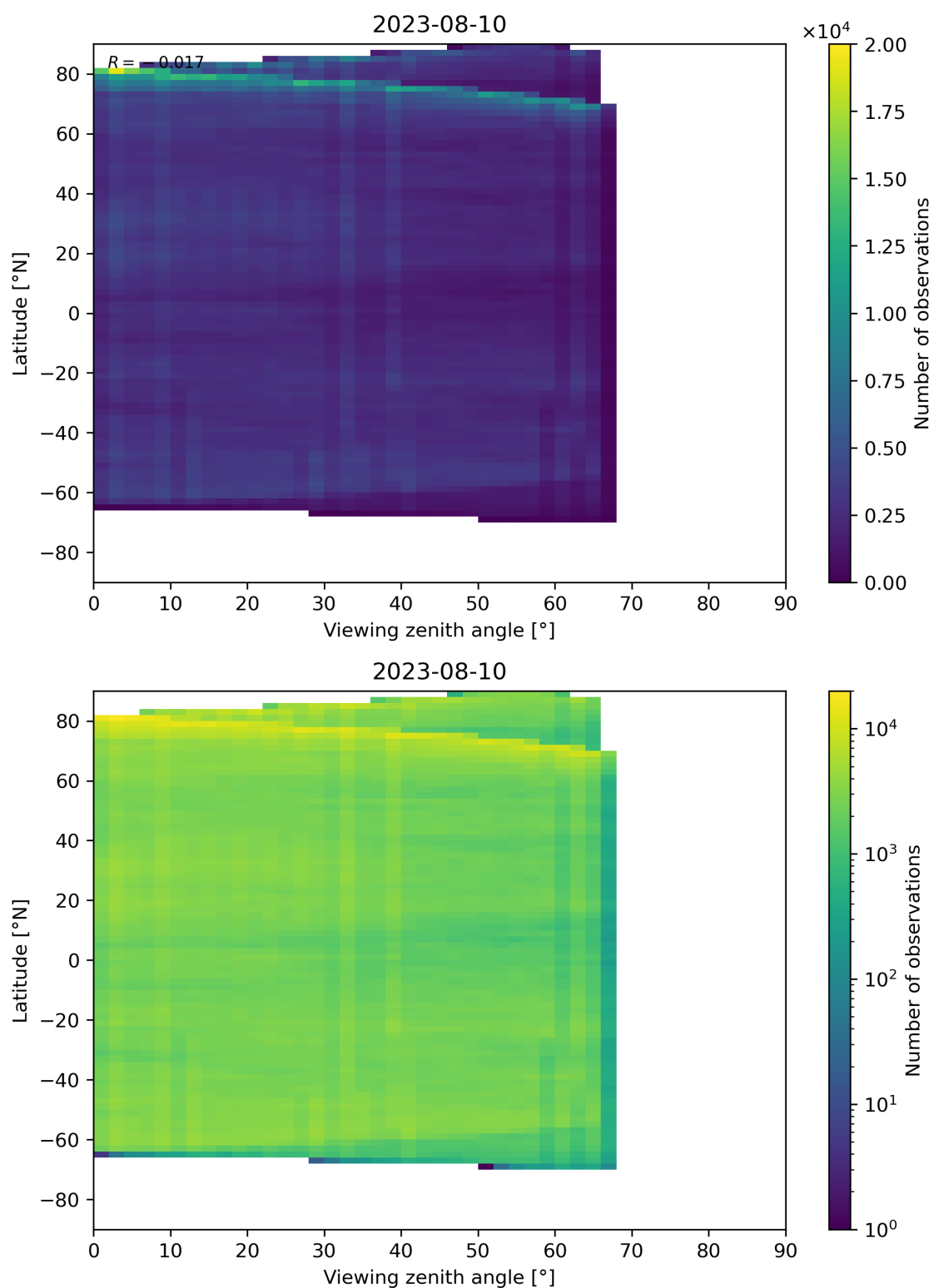
Figure 74: Scatter density plot of “Viewing zenith angle” against “Latitude” for 2023-08-09 to 2023-08-11.
