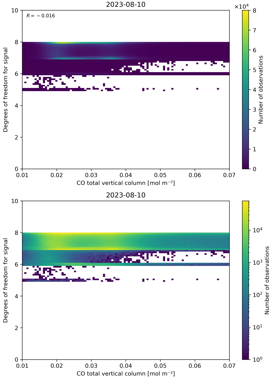
Figure 41: Scatter density plot of “CO total vertical column” against “Degrees of freedom for signal” for 2023-08-09 to 2023-08-11.
