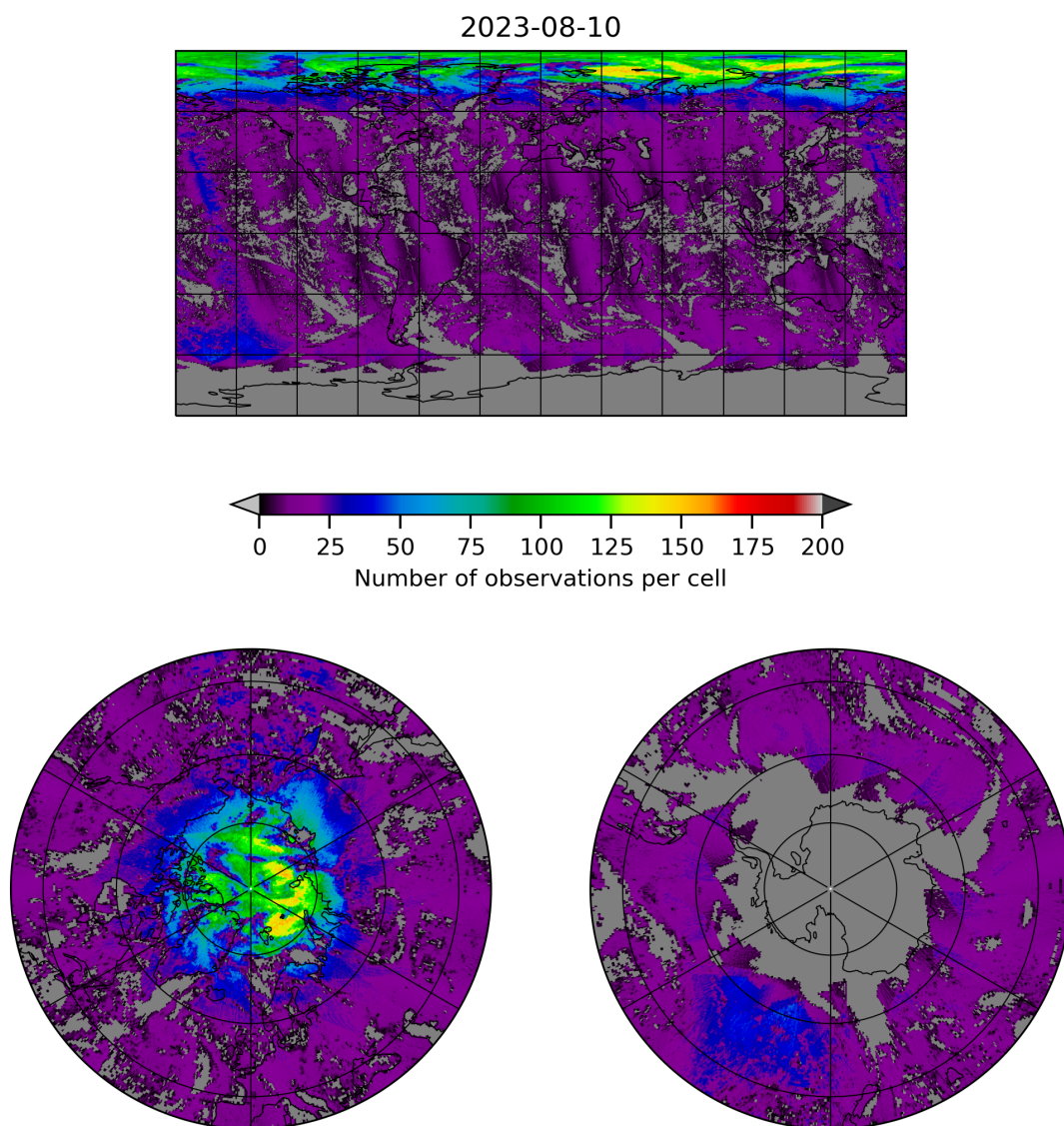
Figure 8: Map of the number of observations for 2023-08-09 to 2023-08-11
