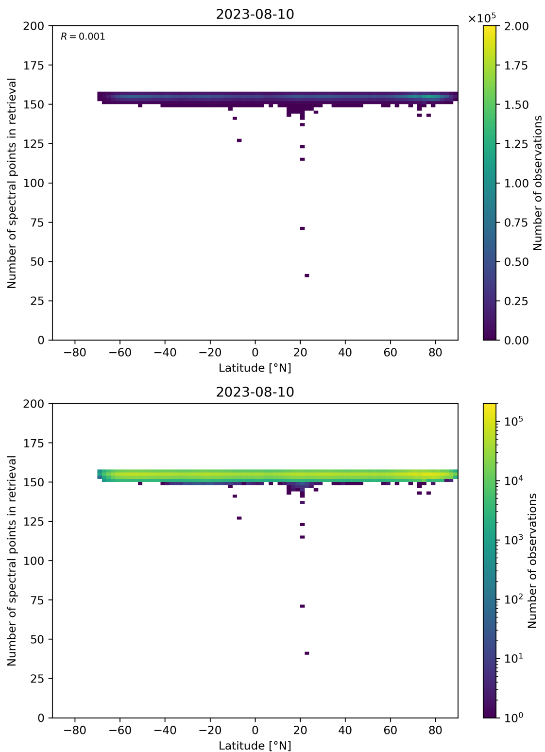
Figure 57: Scatter density plot of “Latitude” against “Number of spectral points in retrieval” for 2023-08-09 to 2023-08-11.
