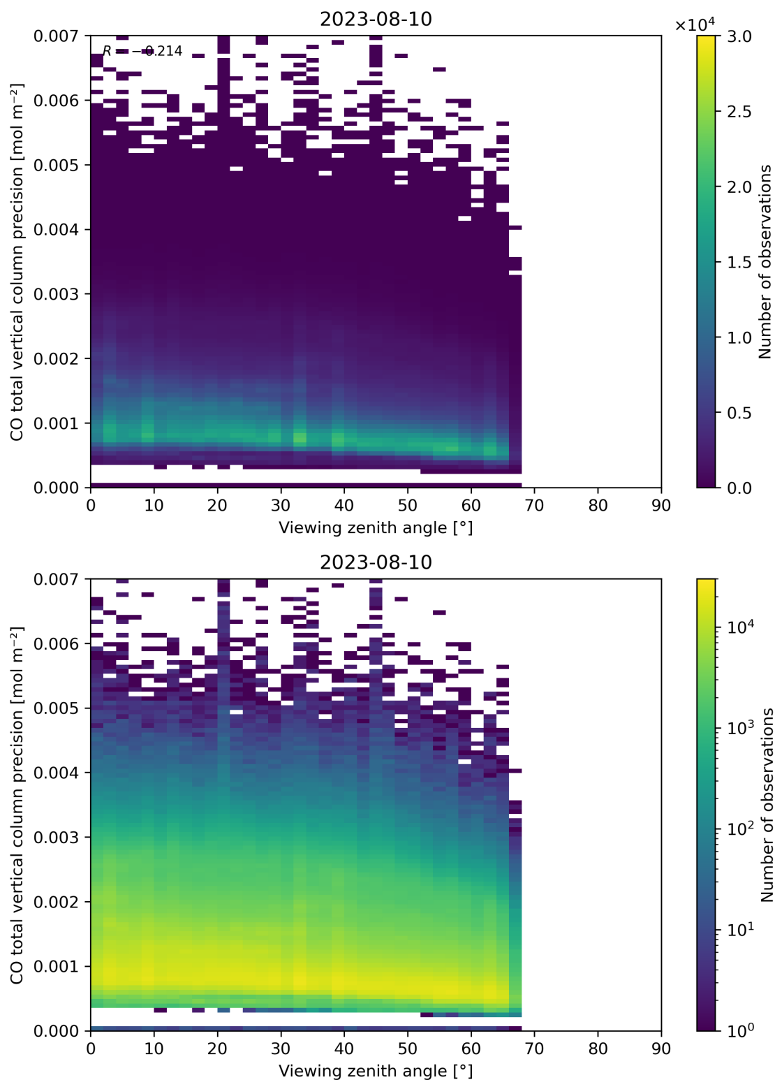
Figure 71: Scatter density plot of “Viewing zenith angle” against “CO total vertical column precision” for 2023-08-09 to 2023-08-11.
