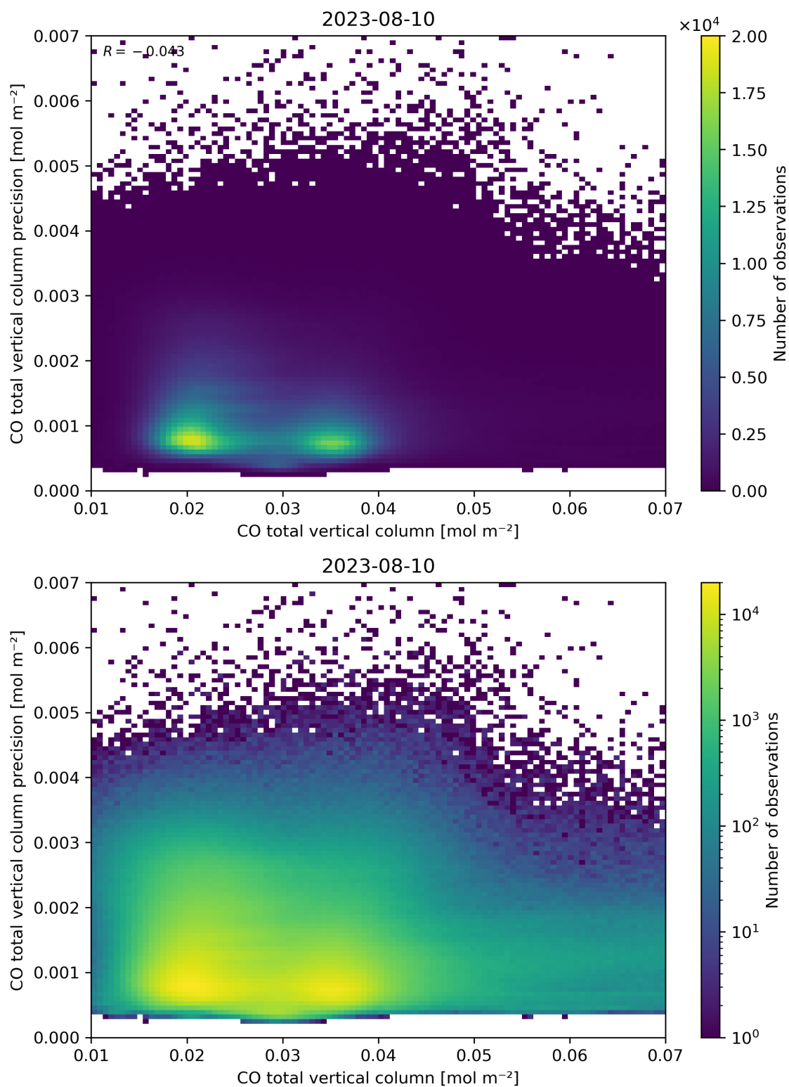
Figure 34: Scatter density plot of “CO total vertical column” against “CO total vertical column precision” for 2023-08-09 to 2023-08-11.
