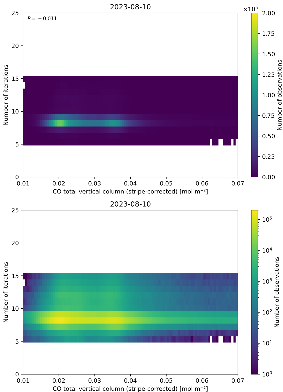
Figure 39: Scatter density plot of “CO total vertical column (stripe-corrected)” against “Number of iterations” for 2023-08-09 to 2023-08-11.
