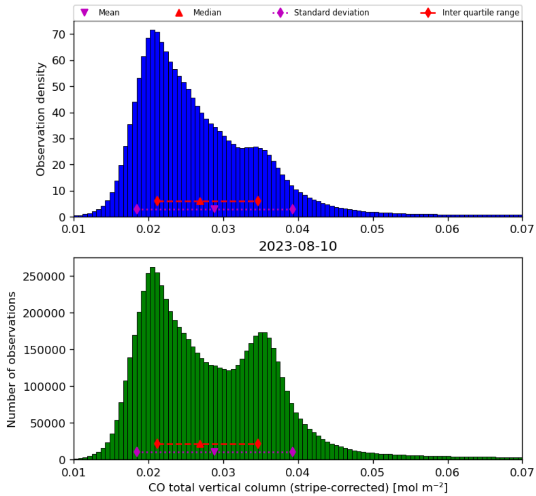
Figure 19: Histogram of “CO total vertical column (stripe-corrected)” for 2023-08-09 to 2023-08-11
