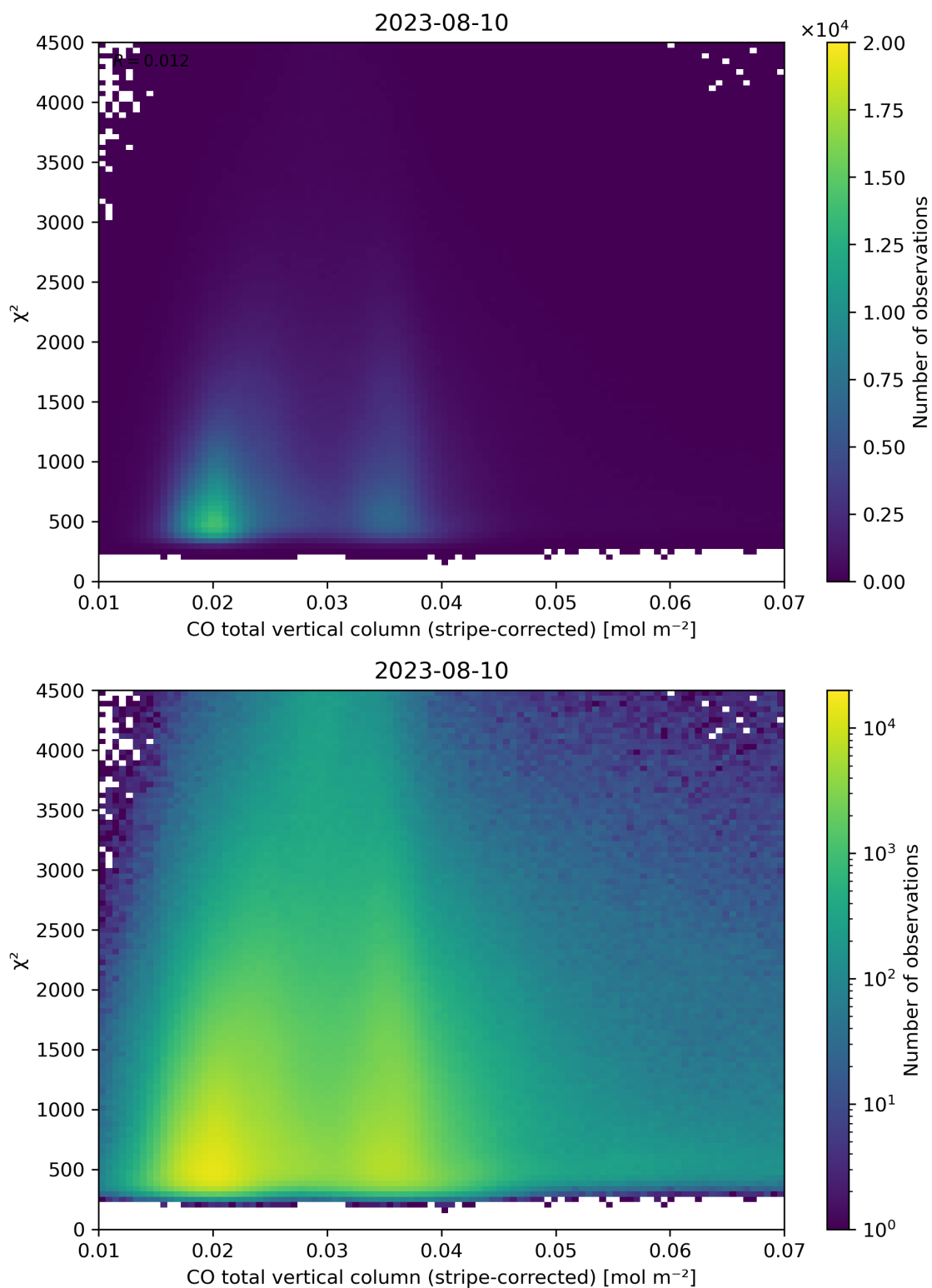
Figure 37: Scatter density plot of “CO total vertical column (stripe-corrected)” against “ \chi^2 ” for 2023-08-09 to 2023-08-11.
