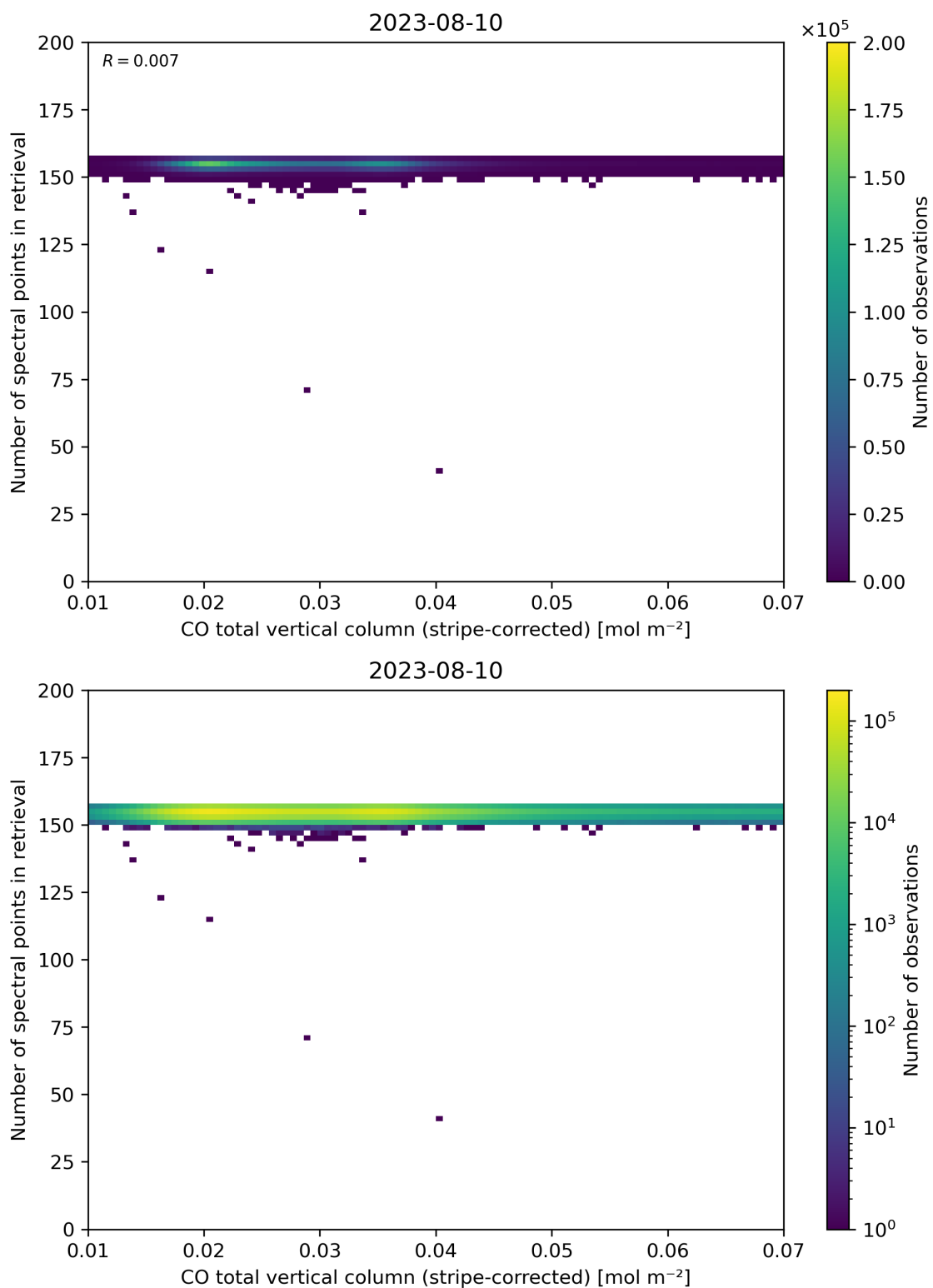
Figure 40: Scatter density plot of “CO total vertical column (stripe-corrected)” against “Number of spectral points in retrieval” for 2023-08-09 to 2023-08-11.
