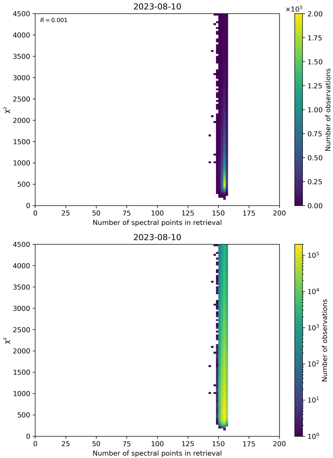
Figure 58: Scatter density plot of “Number of spectral points in retrieval” against “ \chi^2 ” for 2023-08-09 to 2023-08-11.
