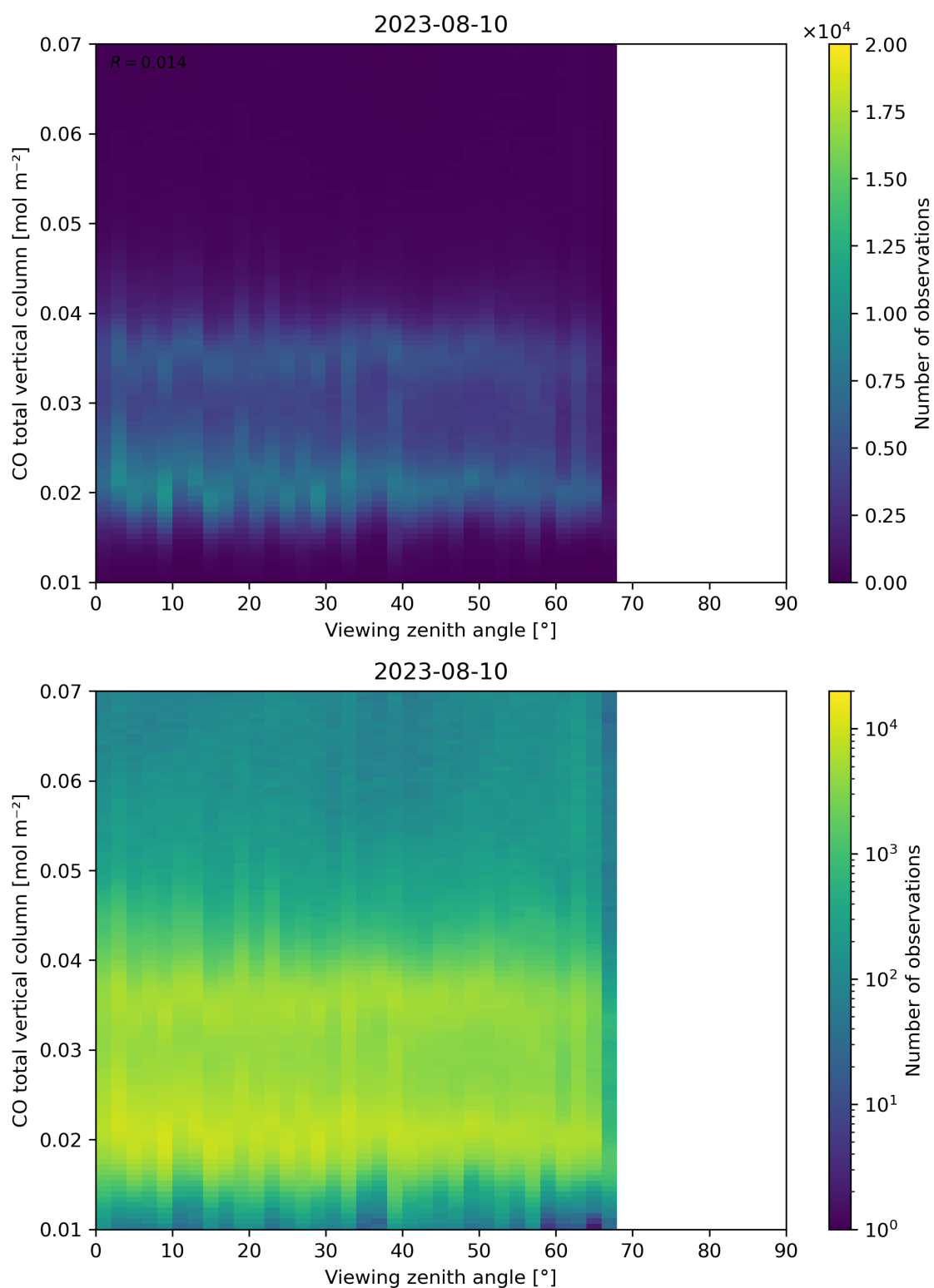
Figure 69: Scatter density plot of “Viewing zenith angle” against “CO total vertical column” for 2023-08-09 to 2023-08-11.
