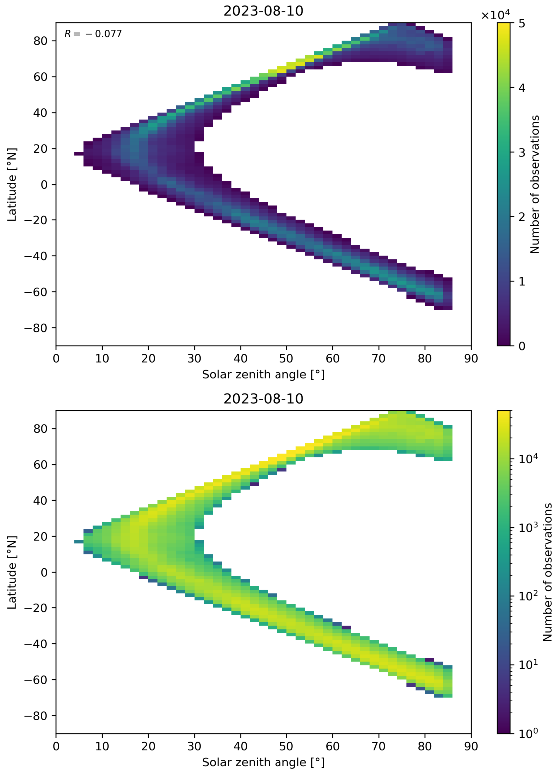
Figure 66: Scatter density plot of “Solar zenith angle” against “Latitude” for 2023-08-09 to 2023-08-11.
