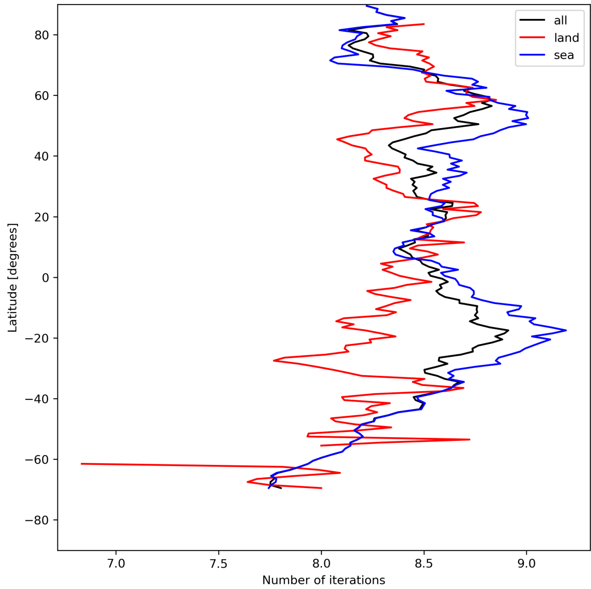
Figure 16: Zonal average of “Number of iterations” for 2023-08-09 to 2023-08-11.
