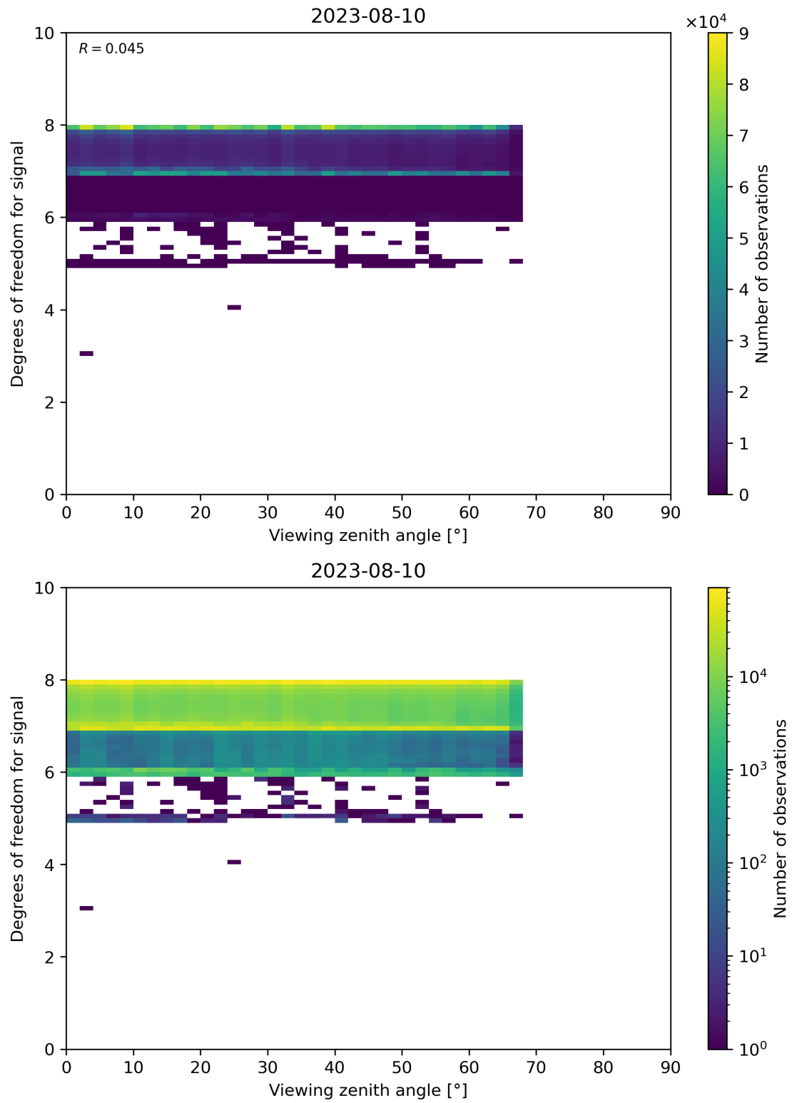
Figure 73: Scatter density plot of “Viewing zenith angle” against “Degrees of freedom for signal” for 2023-08-09 to 2023-08-11.
