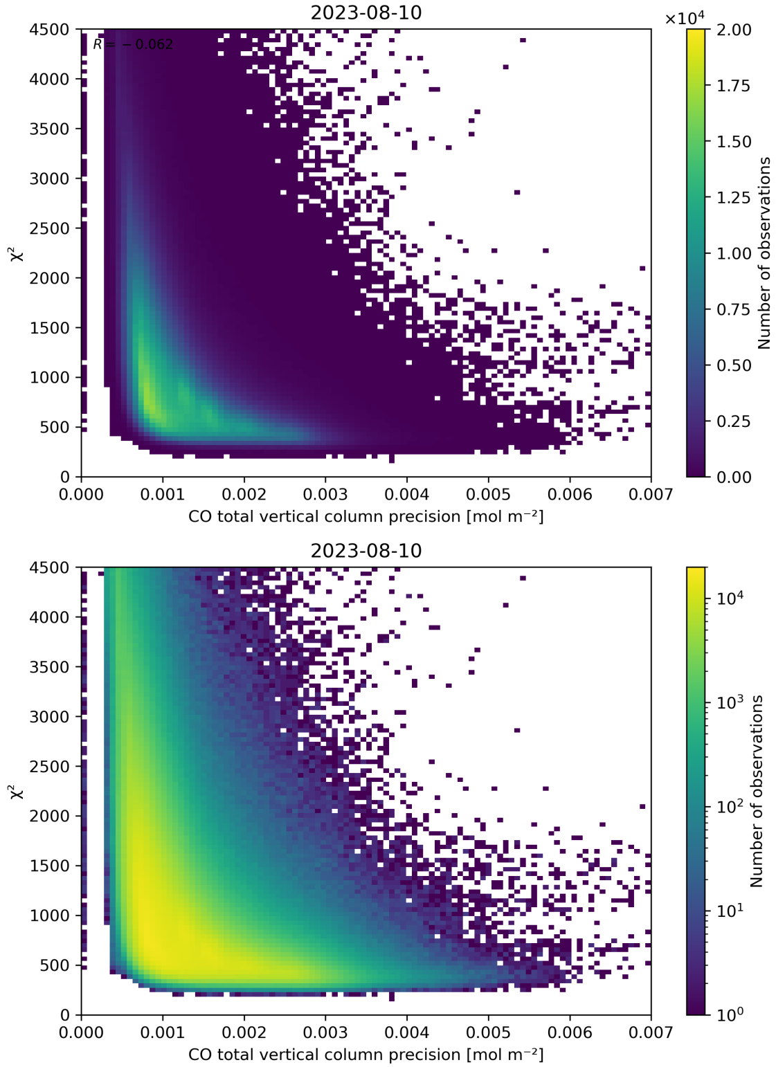
Figure 44: Scatter density plot of “CO total vertical column precision” against “ \chi^2 ” for 2023-08-09 to 2023-08-11.
