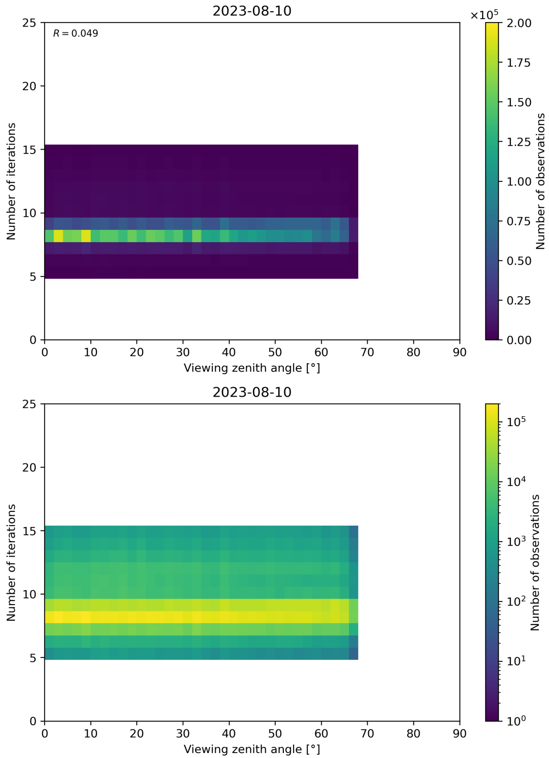
Figure 75: Scatter density plot of “Viewing zenith angle” against “Number of iterations” for 2023-08-09 to 2023-08-11.
