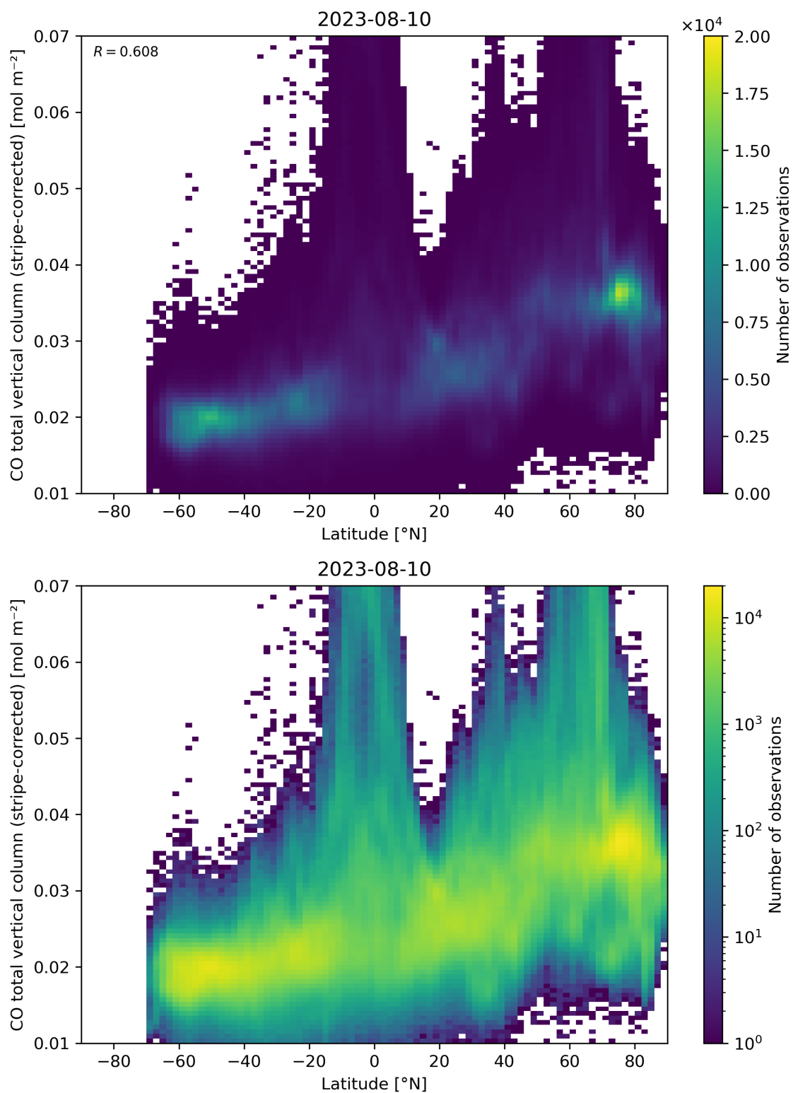
Figure 52: Scatter density plot of “Latitude” against “CO total vertical column (stripe-corrected)” for 2023-08-09 to 2023-08-11.
