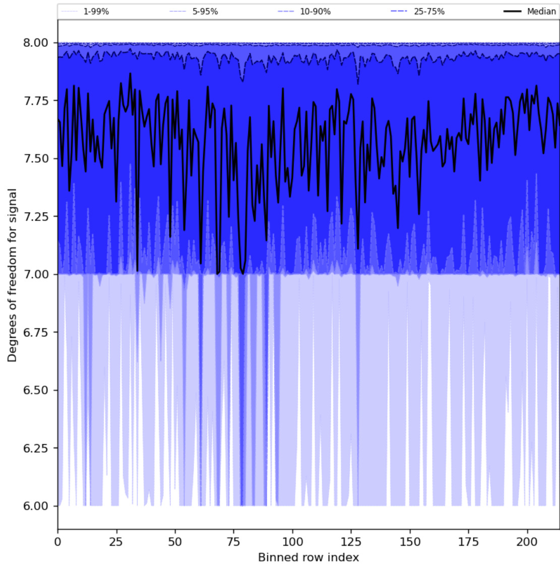
Figure 31: Along track statistics of “Degrees of freedom for signal” for 2023-08-09 to 2023-08-11
