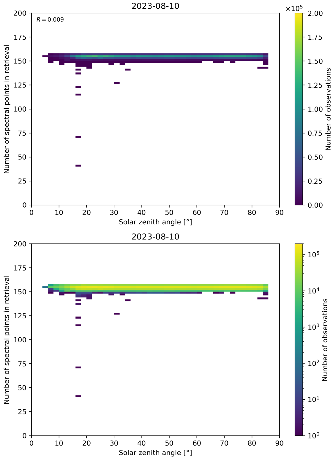
Figure 68: Scatter density plot of “Solar zenith angle” against “Number of spectral points in retrieval” for 2023-08-09 to 2023-08-11.
