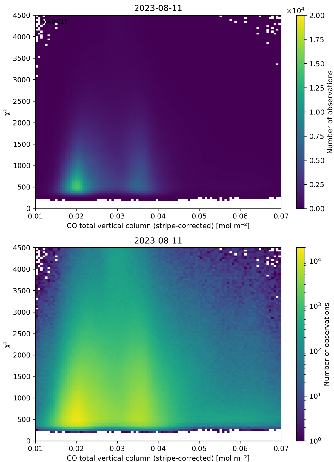
Figure 37: Scatter density plot of “CO total vertical column (stripe-corrected)” against “ \chi^2 ” for 2023-08-10 to 2023-08-12.
