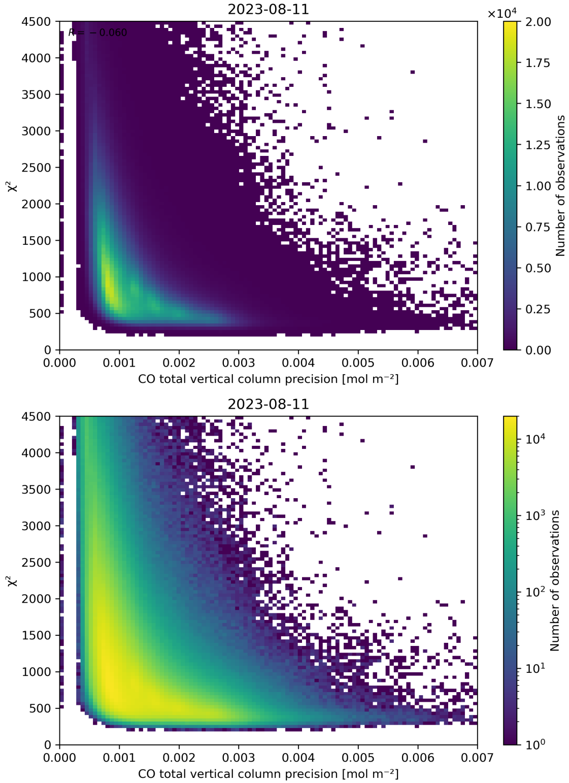
Figure 44: Scatter density plot of “CO total vertical column precision” against “ \chi^2 ” for 2023-08-10 to 2023-08-12.
