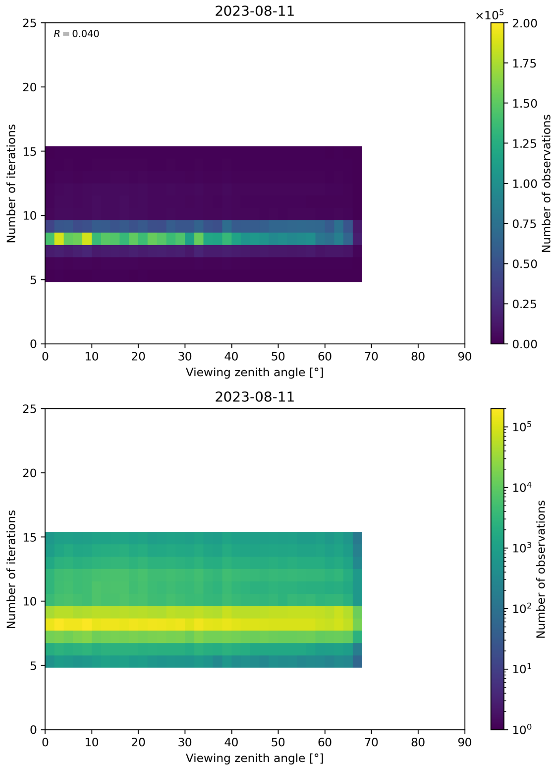
Figure 75: Scatter density plot of “Viewing zenith angle” against “Number of iterations” for 2023-08-10 to 2023-08-12.
