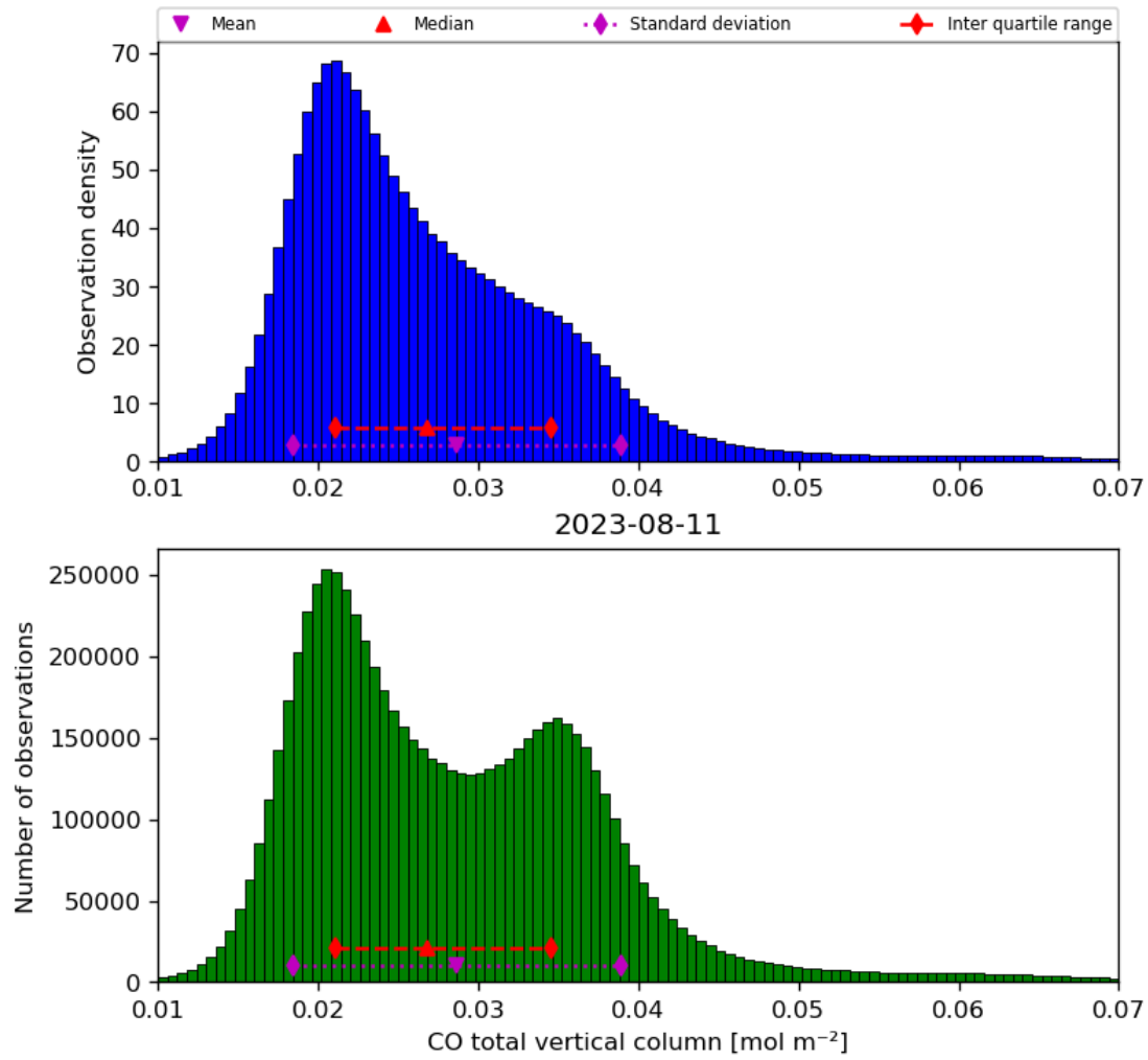
Figure 18: Histogram of “CO total vertical column” for 2023-08-10 to 2023-08-12
