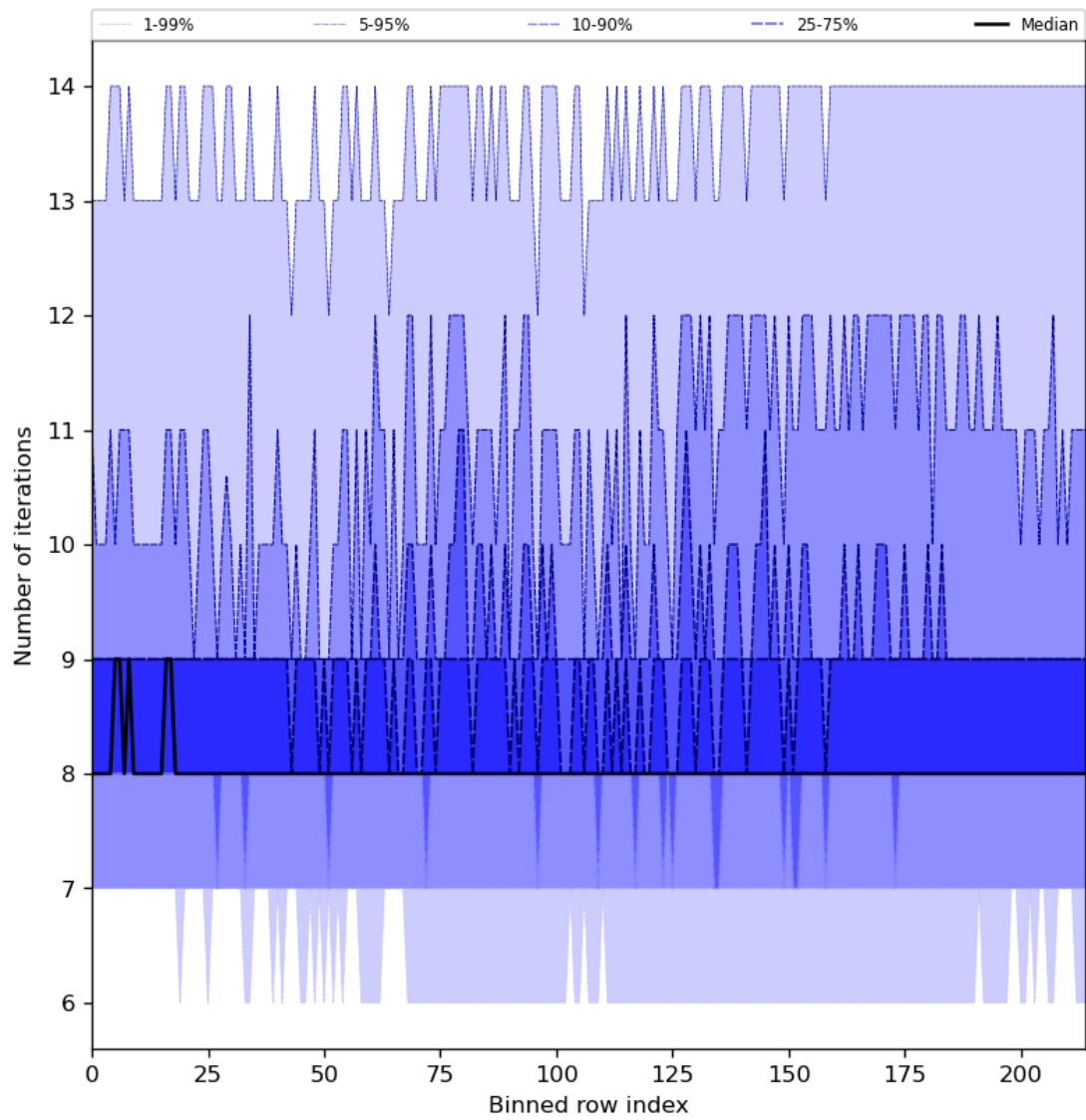
Figure 32: Along track statistics of “Number of iterations” for 2023-08-10 to 2023-08-12
