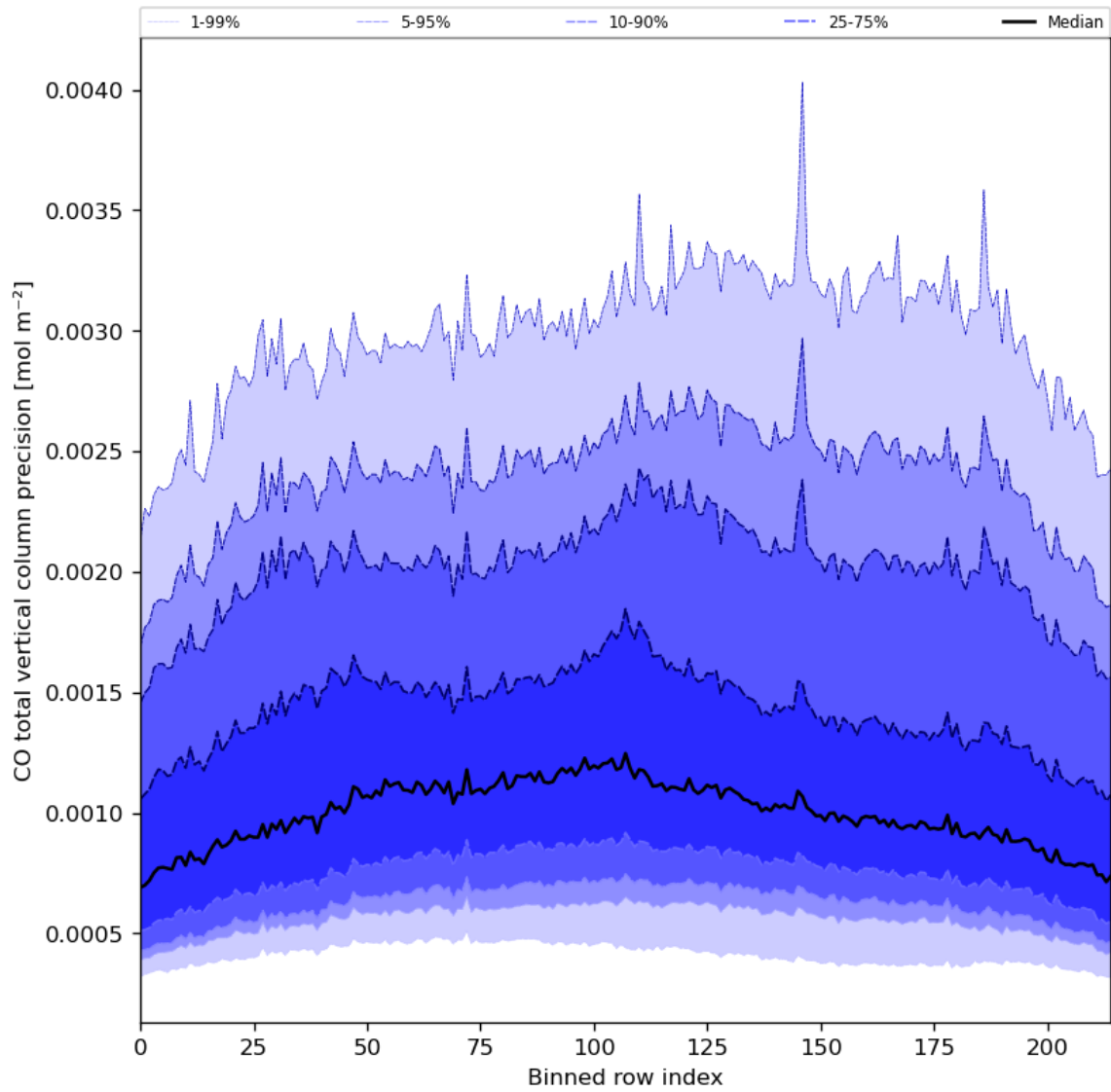
Figure 28: Along track statistics of “CO total vertical column precision” for 2023-08-10 to 2023-08-12
