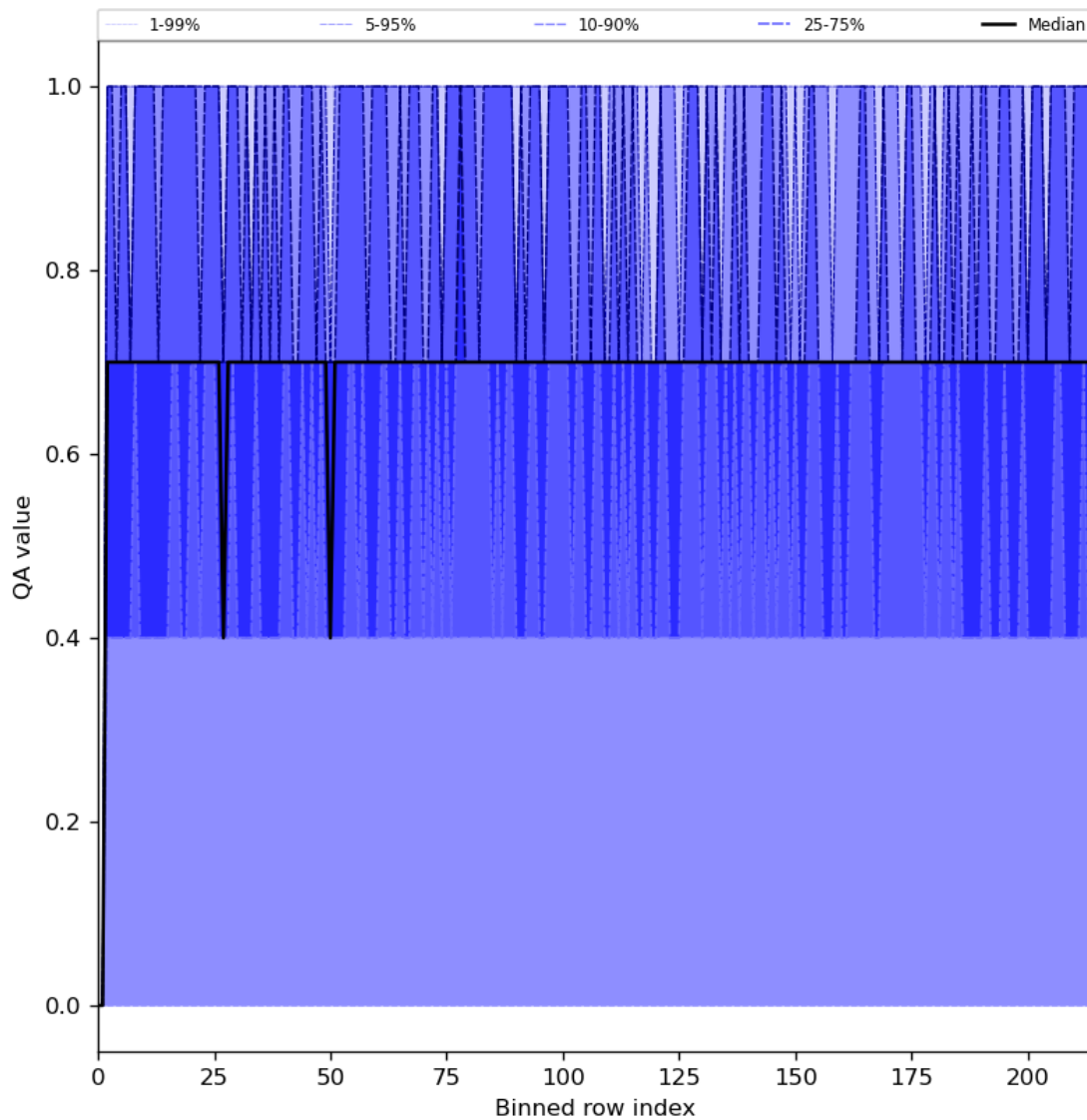
Figure 25: Along track statistics of “QA value” for 2023-08-10 to 2023-08-12
