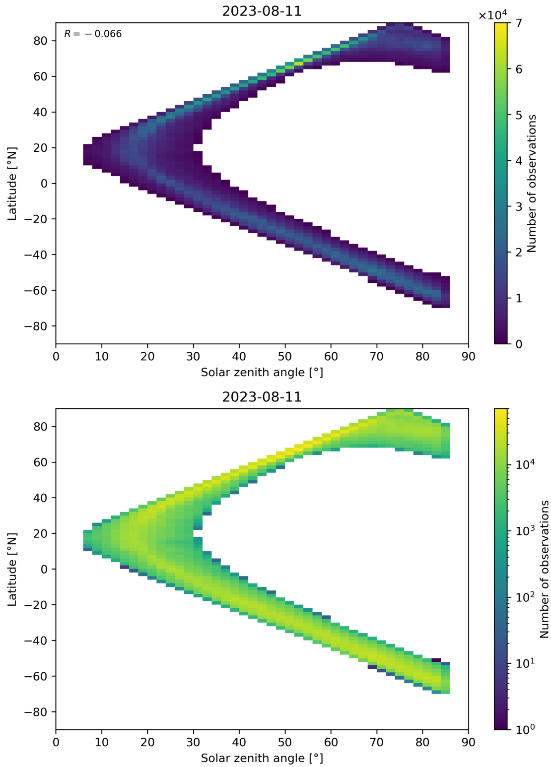
Figure 66: Scatter density plot of “Solar zenith angle” against “Latitude” for 2023-08-10 to 2023-08-12.
