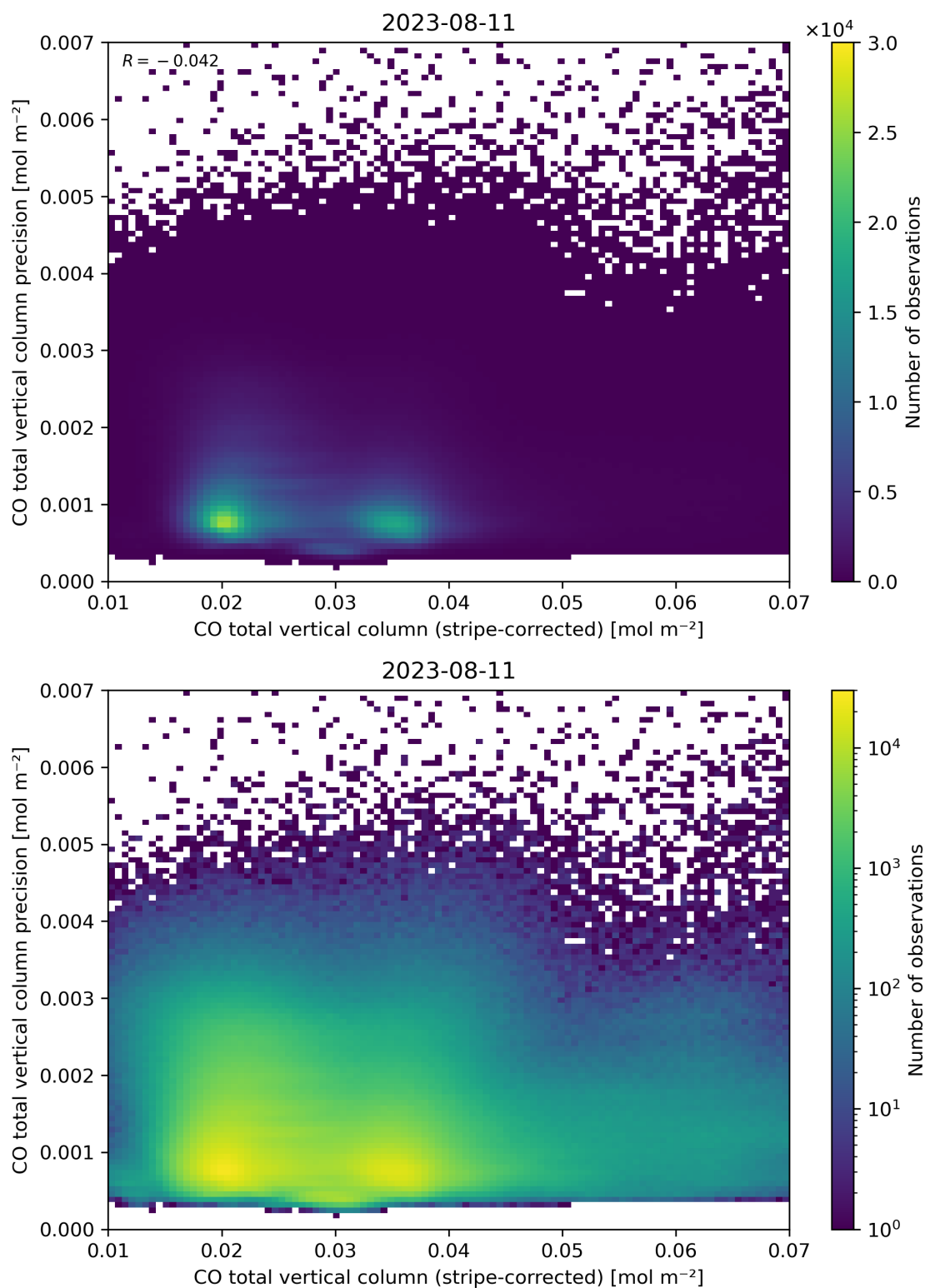
Figure 36: Scatter density plot of “CO total vertical column (stripe-corrected)” against “CO total vertical column precision” for 2023-08-10 to 2023-08-12.
