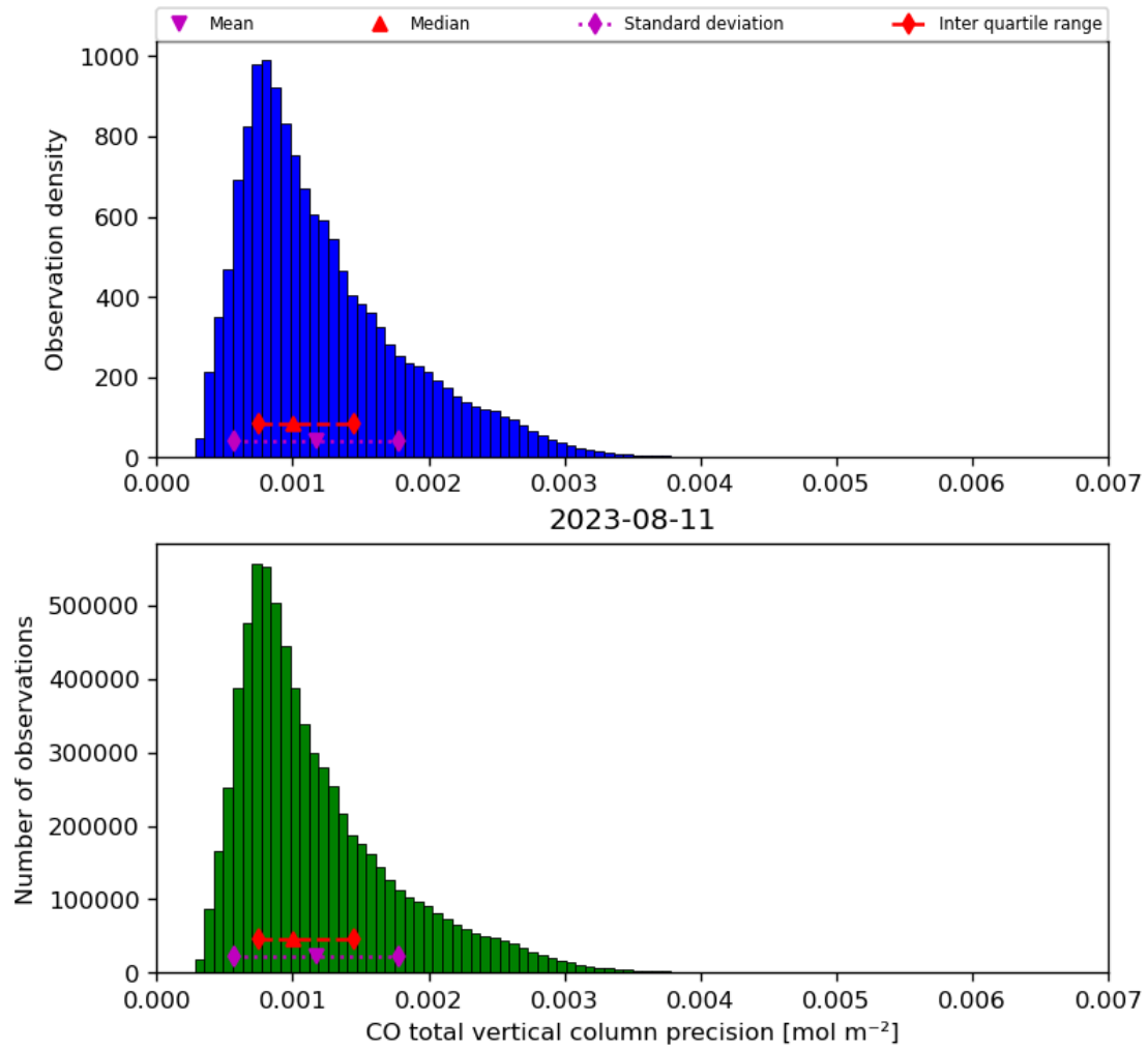
Figure 20: Histogram of “CO total vertical column precision” for 2023-08-10 to 2023-08-12
