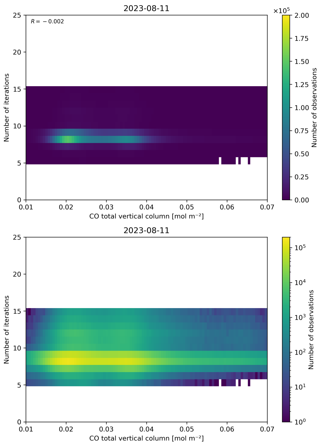
Figure 42: Scatter density plot of “CO total vertical column” against “Number of iterations” for 2023-08-10 to 2023-08-12.
