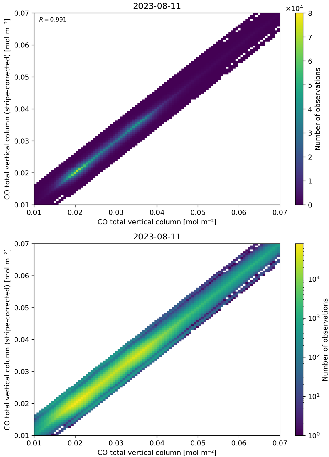
Figure 33: Scatter density plot of “CO total vertical column” against “CO total vertical column (stripe-corrected)” for 2023-08-10 to 2023-08-12.
