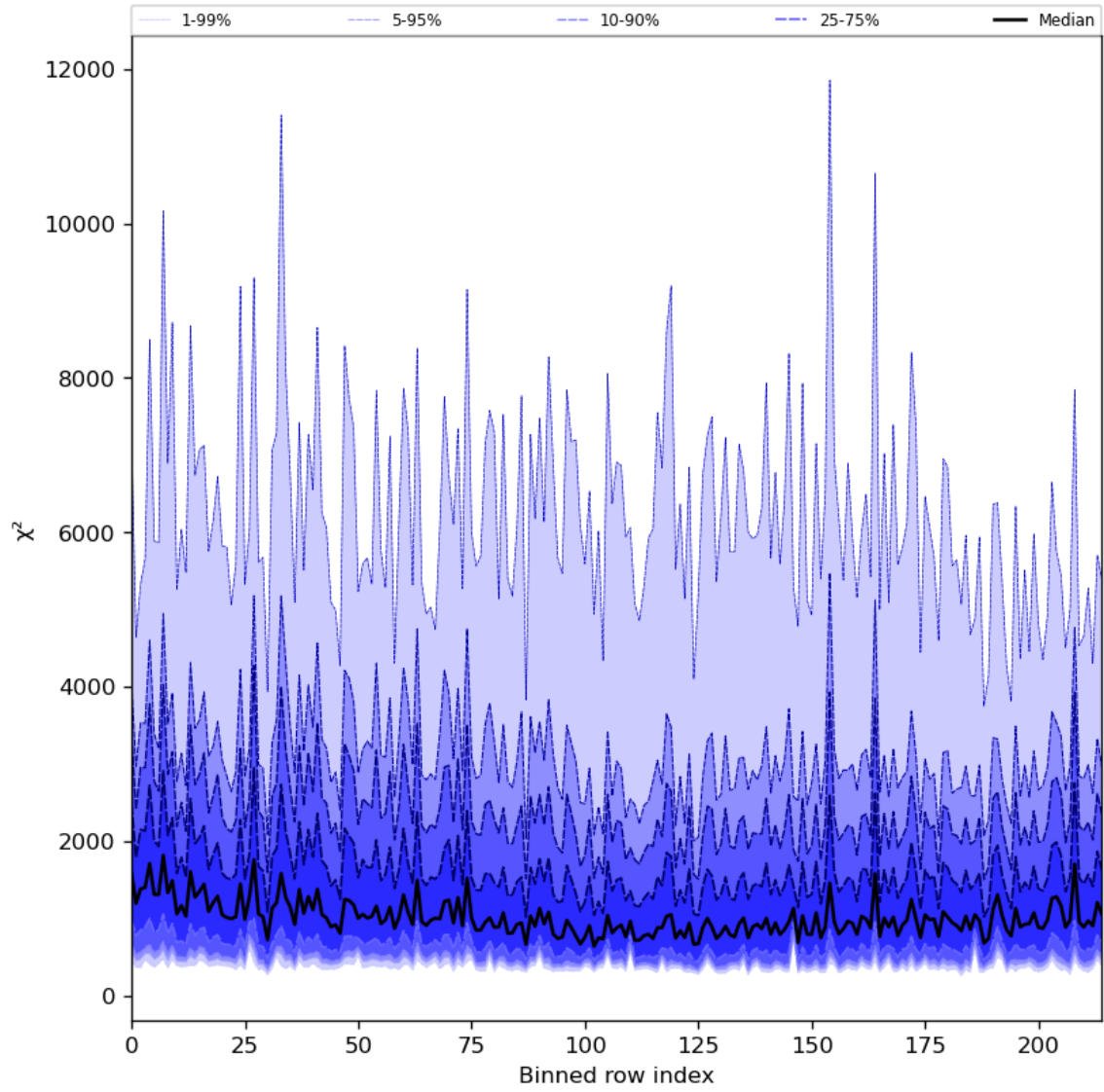
Figure 30: Along track statistics of “ \chi^2 ” for 2023-08-10 to 2023-08-12
