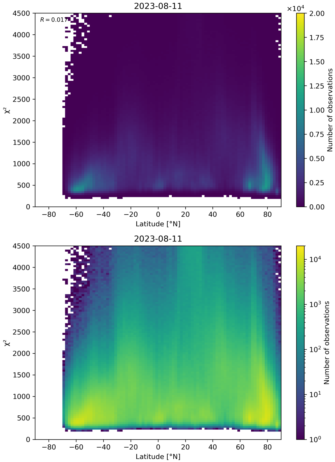
Figure 54: Scatter density plot of “Latitude” against “ \chi^2 ” for 2023-08-10 to 2023-08-12.
