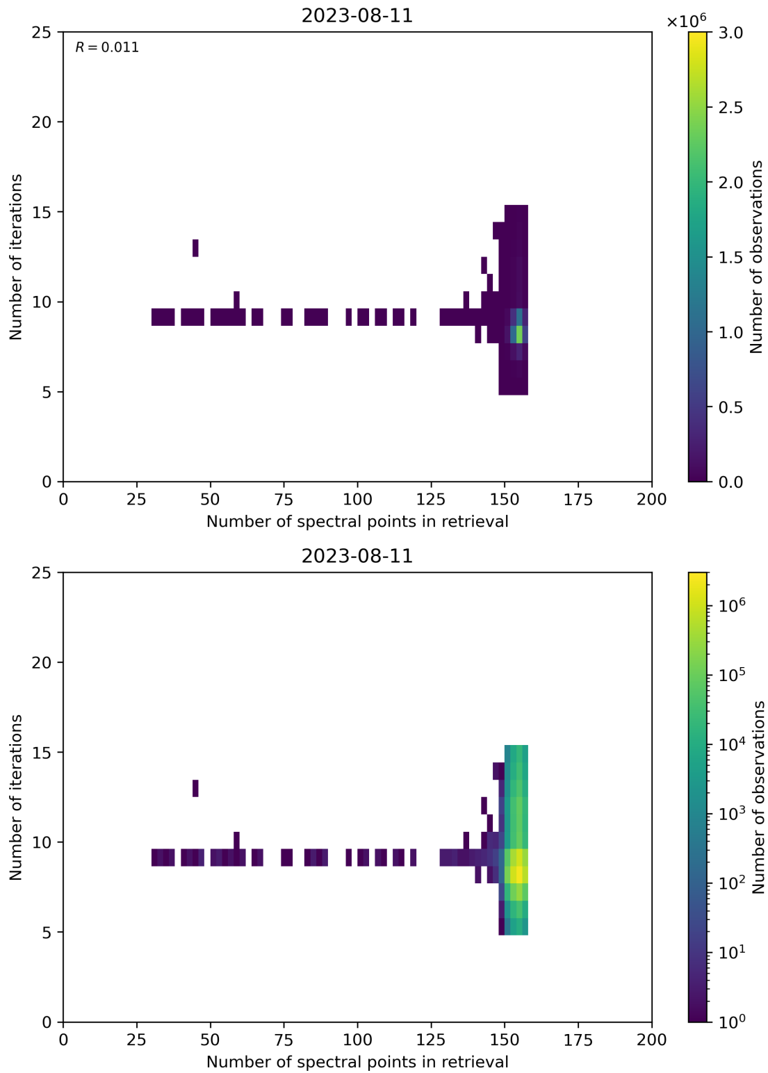
Figure 60: Scatter density plot of “Number of spectral points in retrieval” against “Number of iterations” for 2023-08-10 to 2023-08-12.
