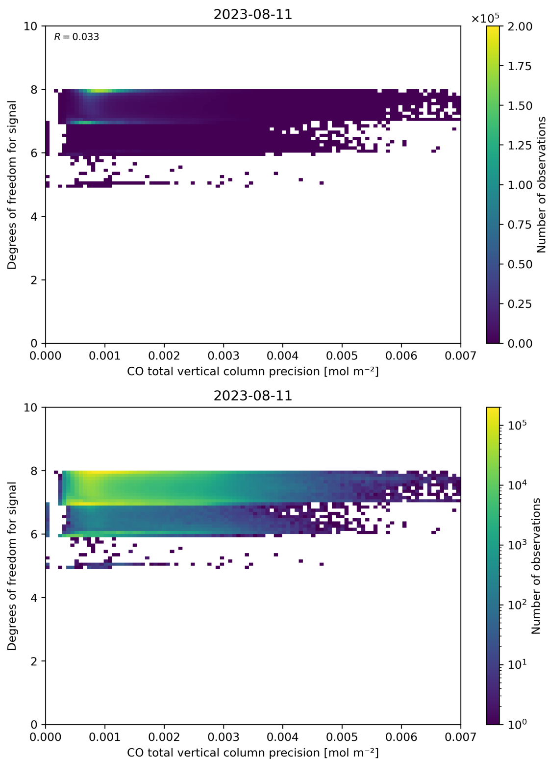
Figure 45: Scatter density plot of “CO total vertical column precision” against “Degrees of freedom for signal” for 2023-08-10 to 2023-08-12.
