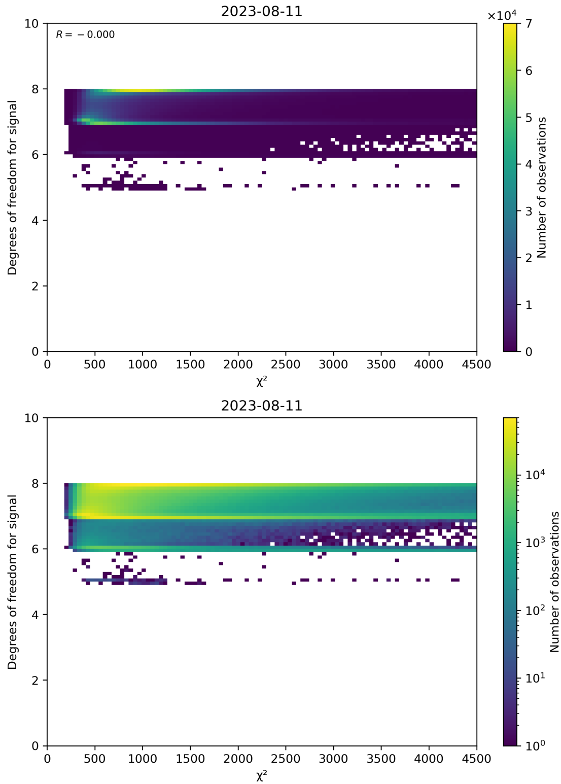
Figure 48: Scatter density plot of " \chi^2 " against "Degrees of freedom for signal" for 2023-08-10 to 2023-08-12.
