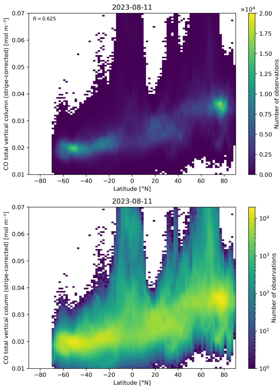
Figure 52: Scatter density plot of “Latitude” against “CO total vertical column (stripe-corrected)” for 2023-08-10 to 2023-08-12.
