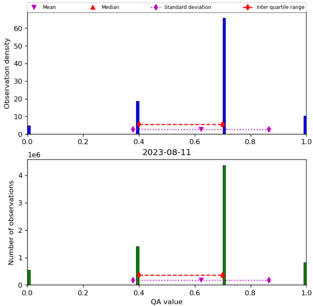
Figure 17: Histogram of “QA value” for 2023-08-10 to 2023-08-12
