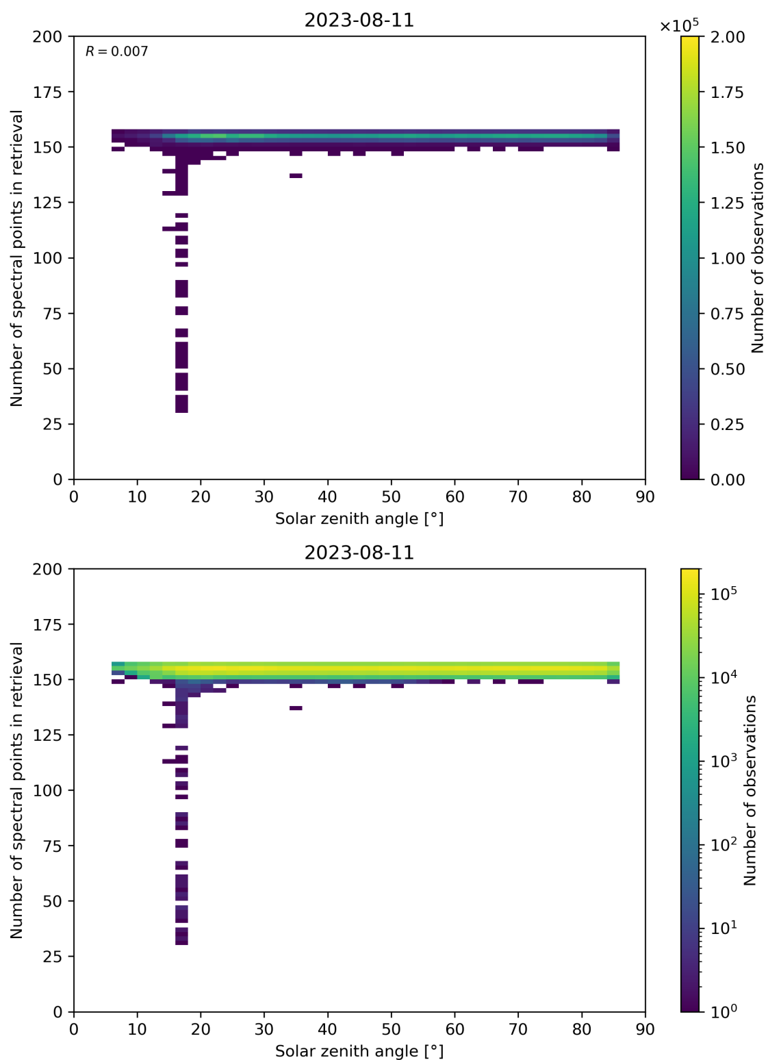
Figure 68: Scatter density plot of “Solar zenith angle” against “Number of spectral points in retrieval” for 2023-08-10 to 2023-08-12.
