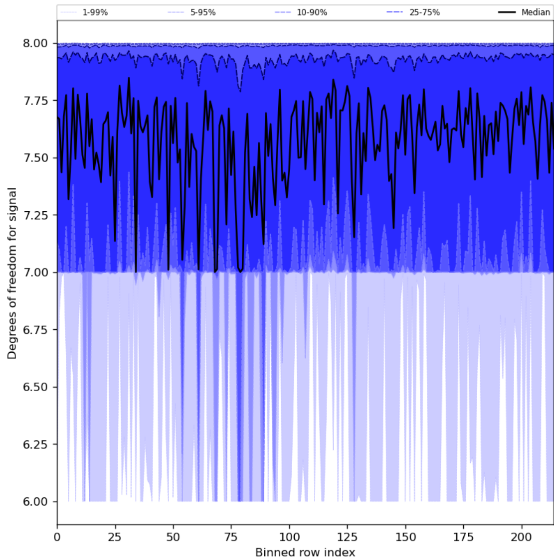
Figure 31: Along track statistics of “Degrees of freedom for signal” for 2023-08-10 to 2023-08-12
