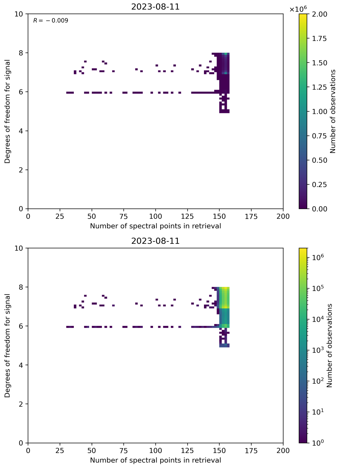
Figure 59: Scatter density plot of “Number of spectral points in retrieval” against “Degrees of freedom for signal” for 2023-08-10 to 2023-08-12.
