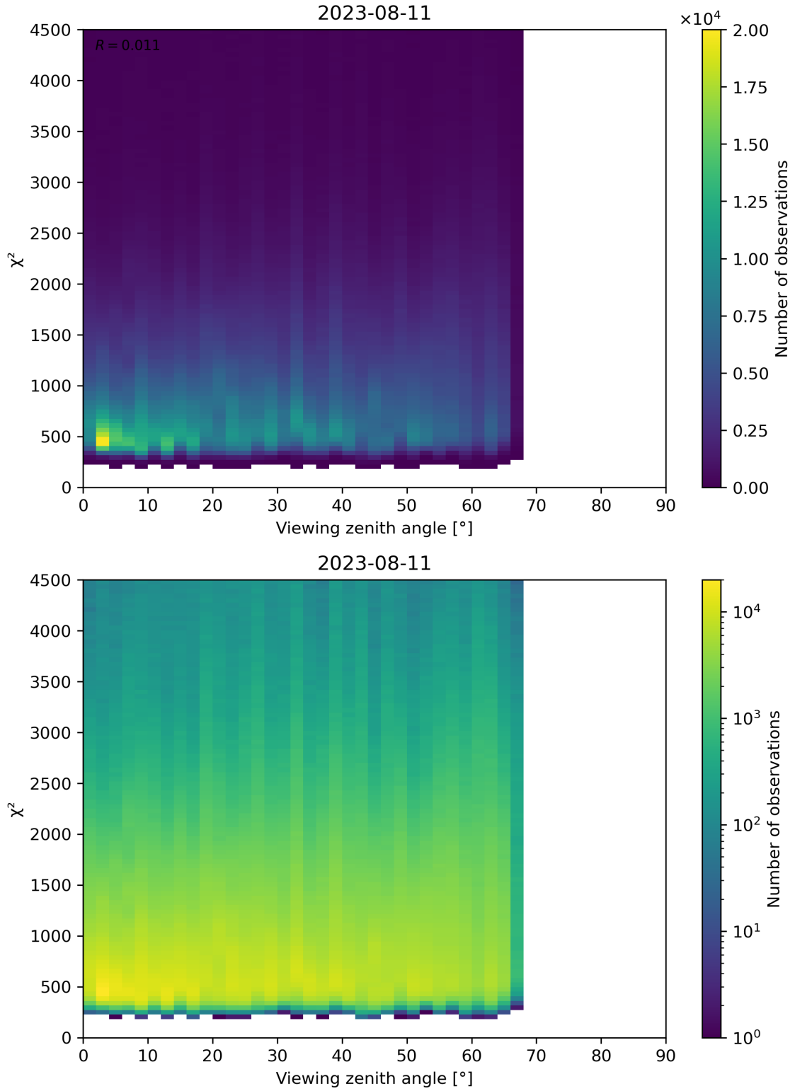
Figure 72: Scatter density plot of “Viewing zenith angle” against “ \chi^2 ” for 2023-08-10 to 2023-08-12.
