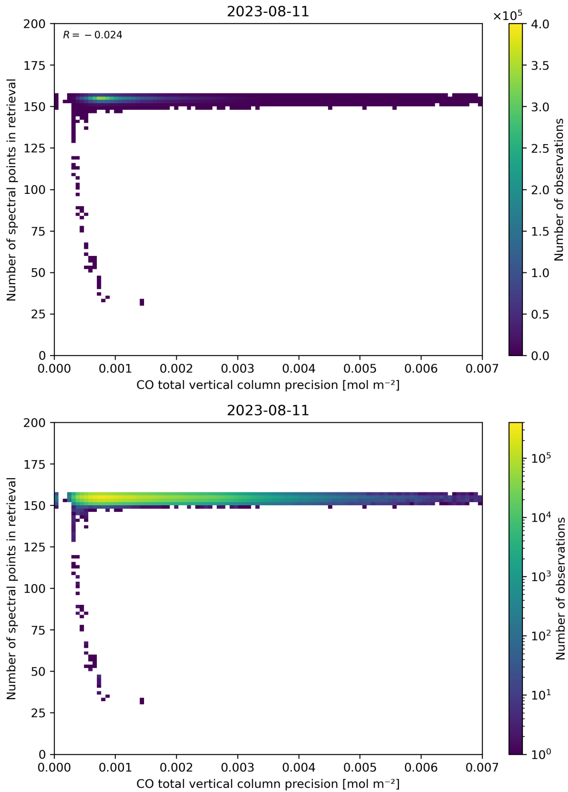
Figure 47: Scatter density plot of “CO total vertical column precision” against “Number of spectral points in retrieval” for 2023-08-10 to 2023-08-12.
