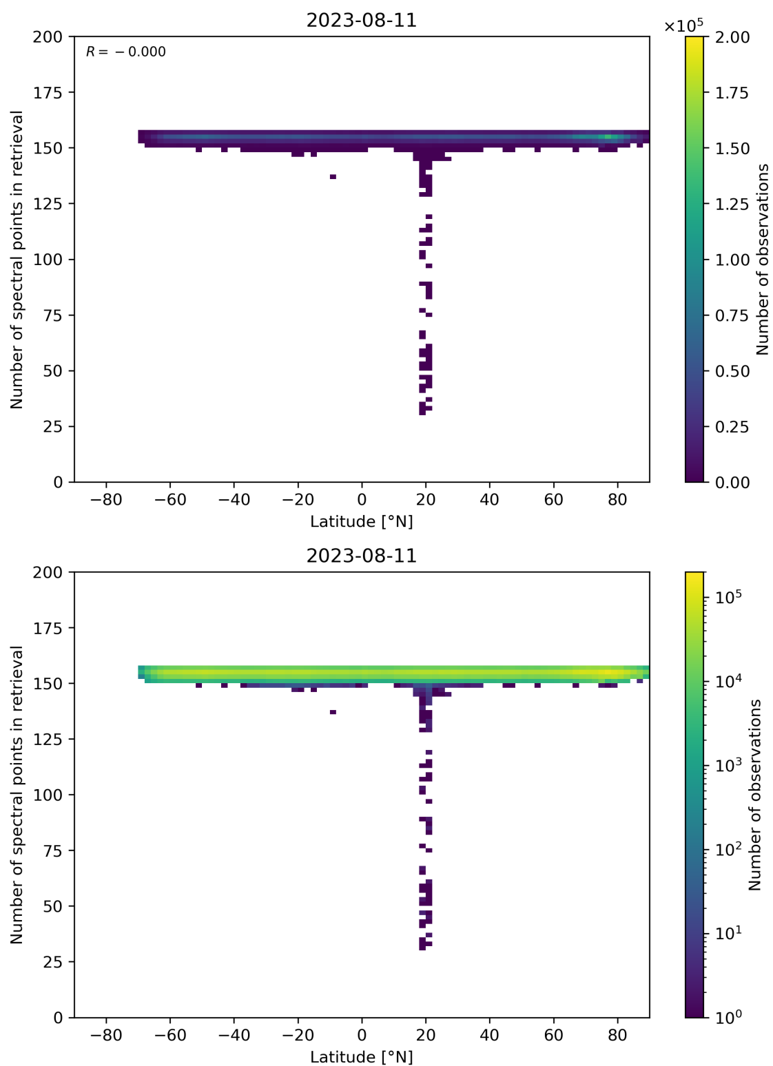
Figure 57: Scatter density plot of “Latitude” against “Number of spectral points in retrieval” for 2023-08-10 to 2023-08-12.
