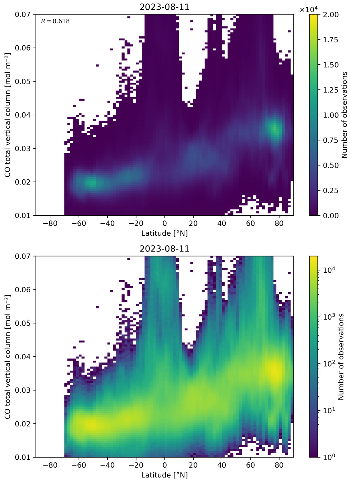
Figure 51: Scatter density plot of “Latitude” against “CO total vertical column” for 2023-08-10 to 2023-08-12.
