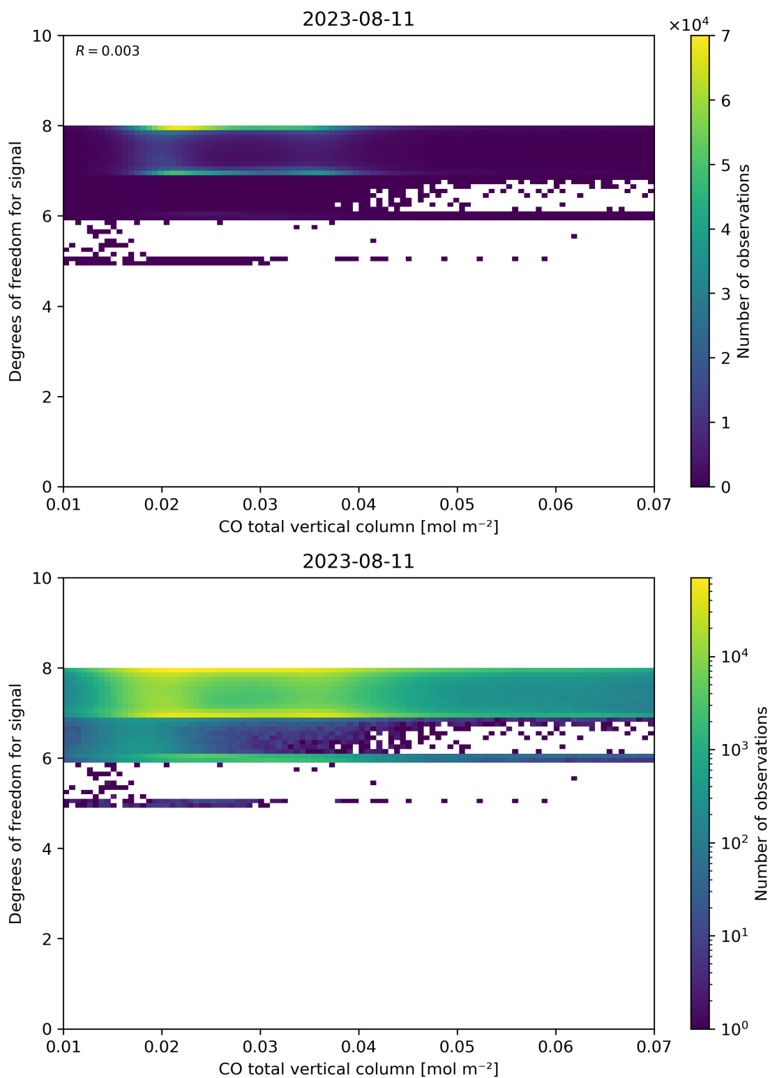
Figure 41: Scatter density plot of “CO total vertical column” against “Degrees of freedom for signal” for 2023-08-10 to 2023-08-12.
