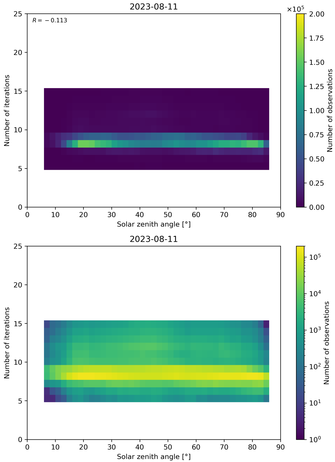
Figure 67: Scatter density plot of “Solar zenith angle” against “Number of iterations” for 2023-08-10 to 2023-08-12.
