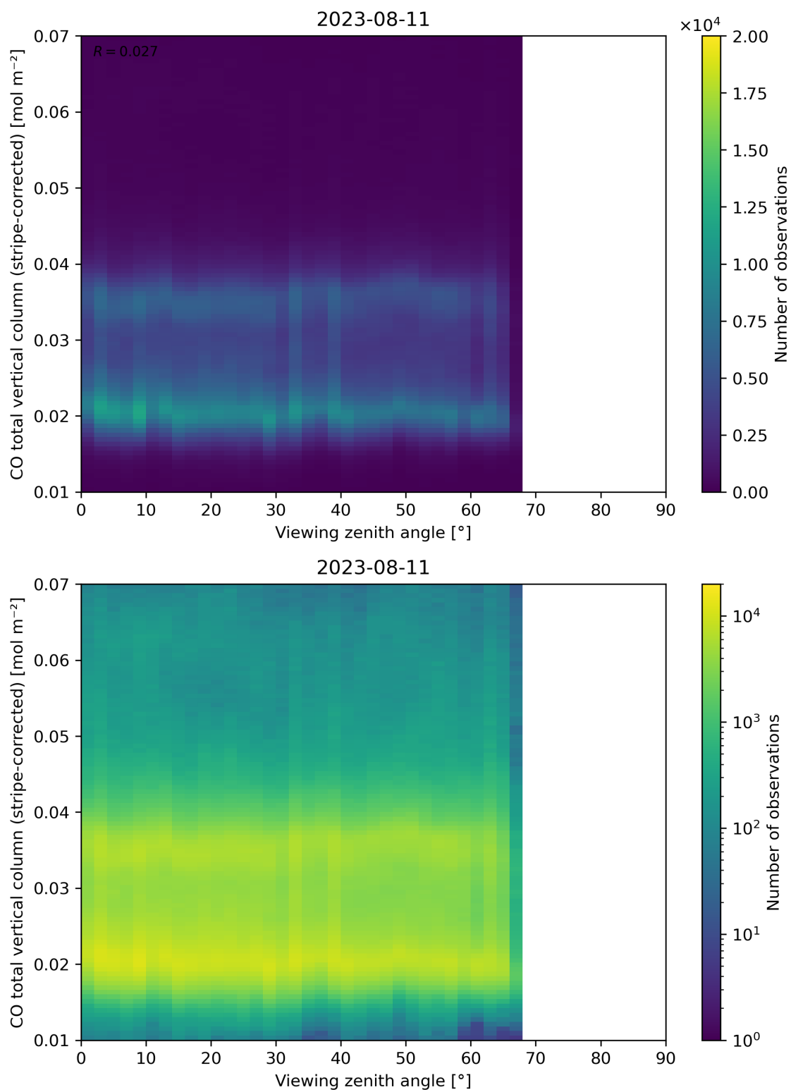
Figure 70: Scatter density plot of “Viewing zenith angle” against “CO total vertical column (stripe-corrected)” for 2023-08-10 to 2023-08-12.
