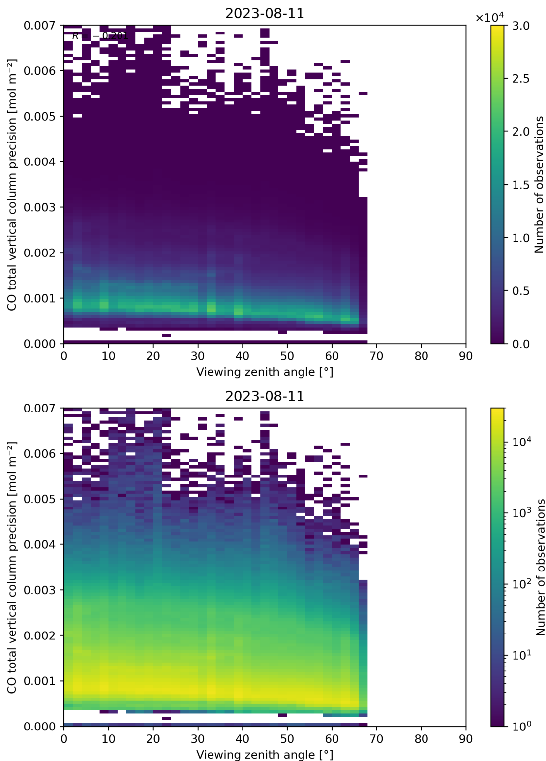
Figure 71: Scatter density plot of “Viewing zenith angle” against “CO total vertical column precision” for 2023-08-10 to 2023-08-12.
