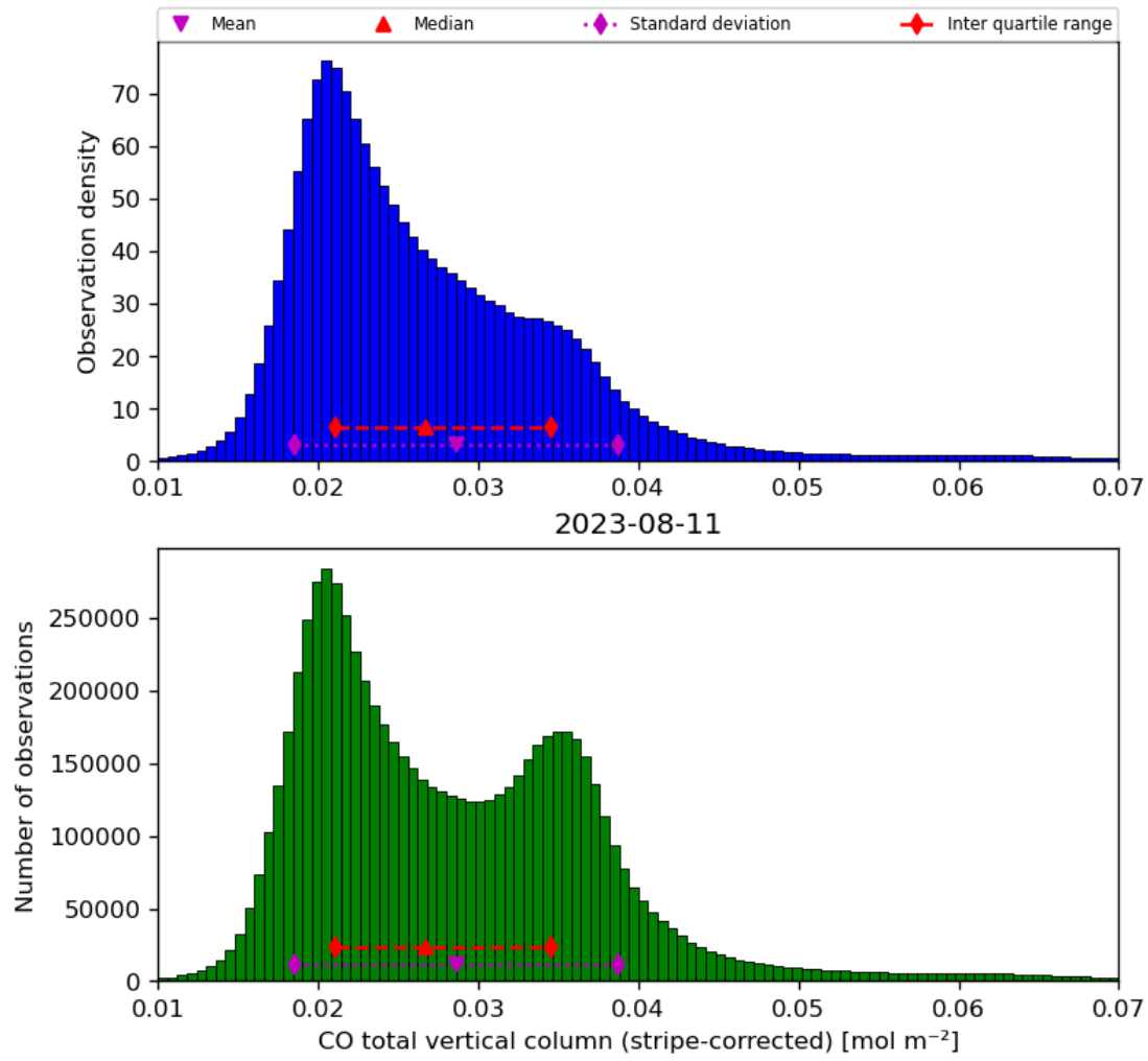
Figure 19: Histogram of “CO total vertical column (stripe-corrected)” for 2023-08-10 to 2023-08-12
