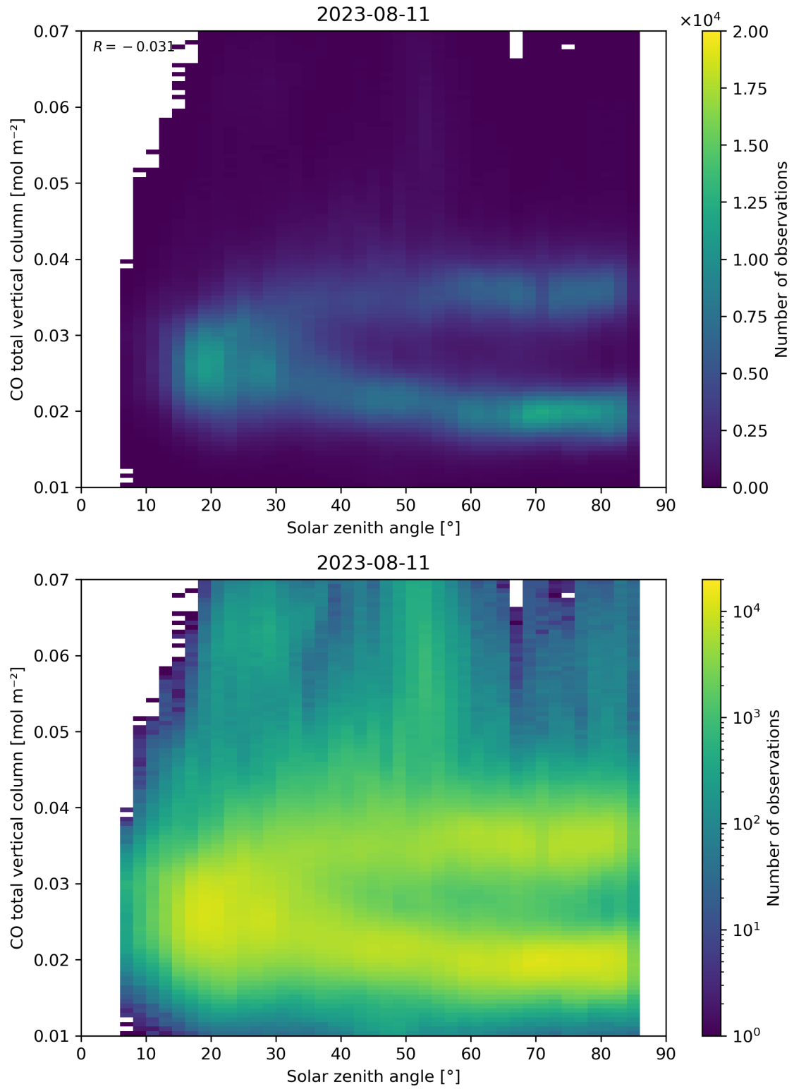
Figure 61: Scatter density plot of “Solar zenith angle” against “CO total vertical column” for 2023-08-10 to 2023-08-12.
