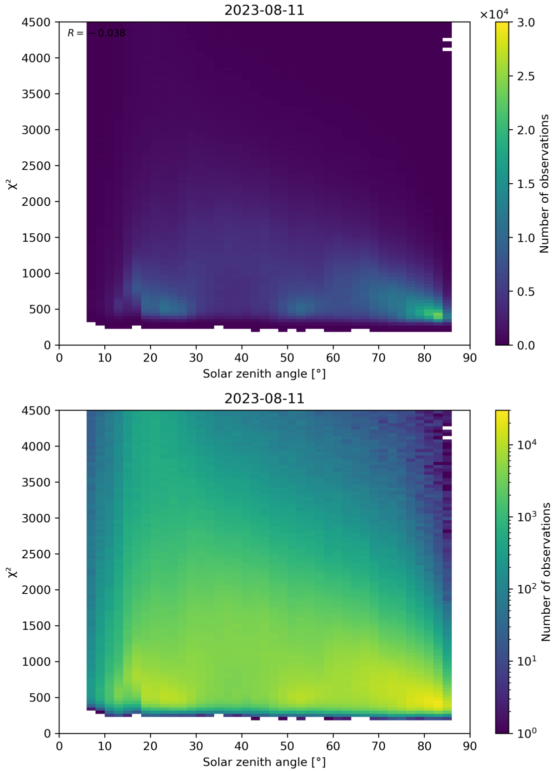
Figure 64: Scatter density plot of “Solar zenith angle” against “ \chi^2 ” for 2023-08-10 to 2023-08-12.
