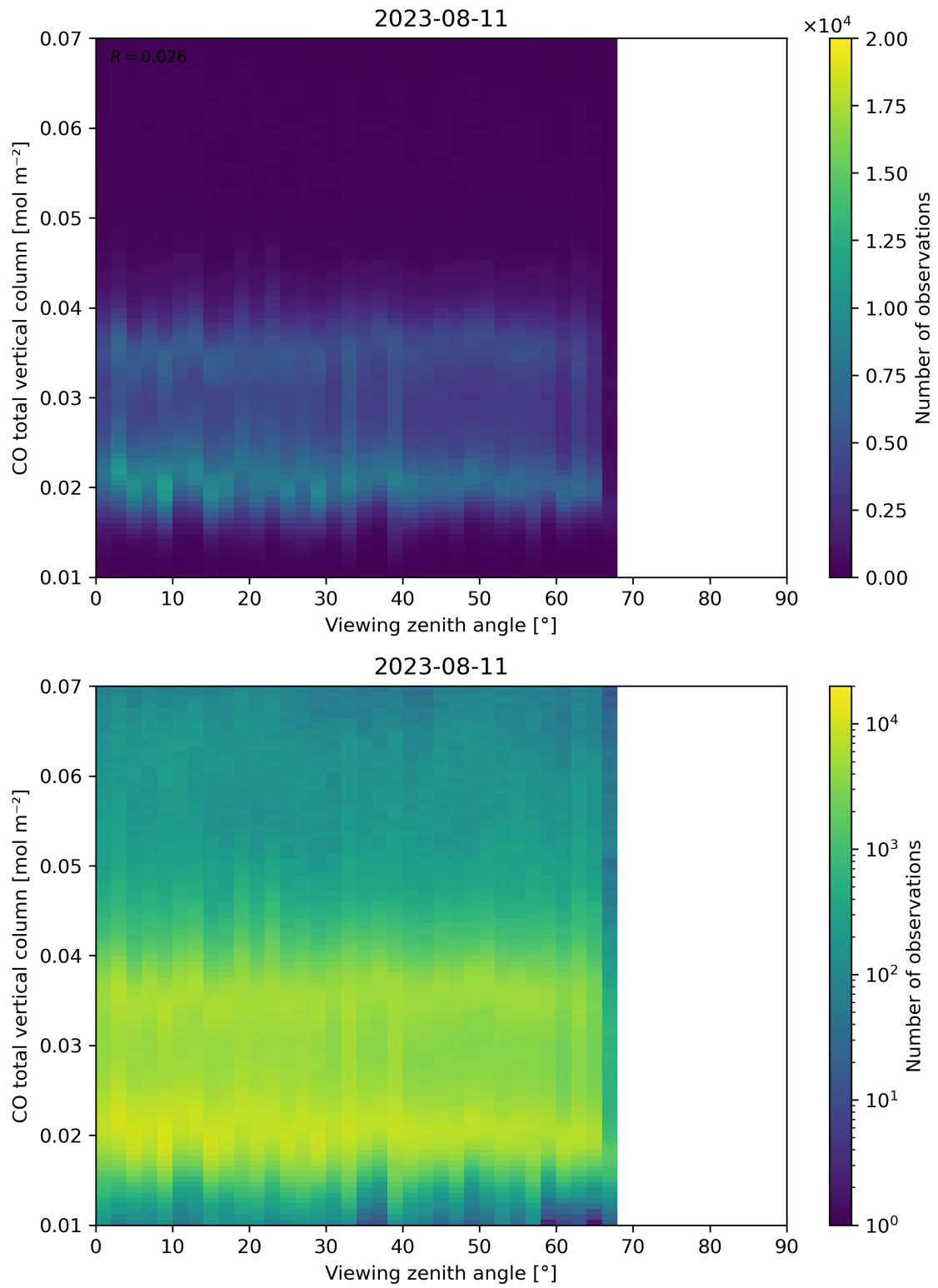
Figure 69: Scatter density plot of “Viewing zenith angle” against “CO total vertical column” for 2023-08-10 to 2023-08-12.
