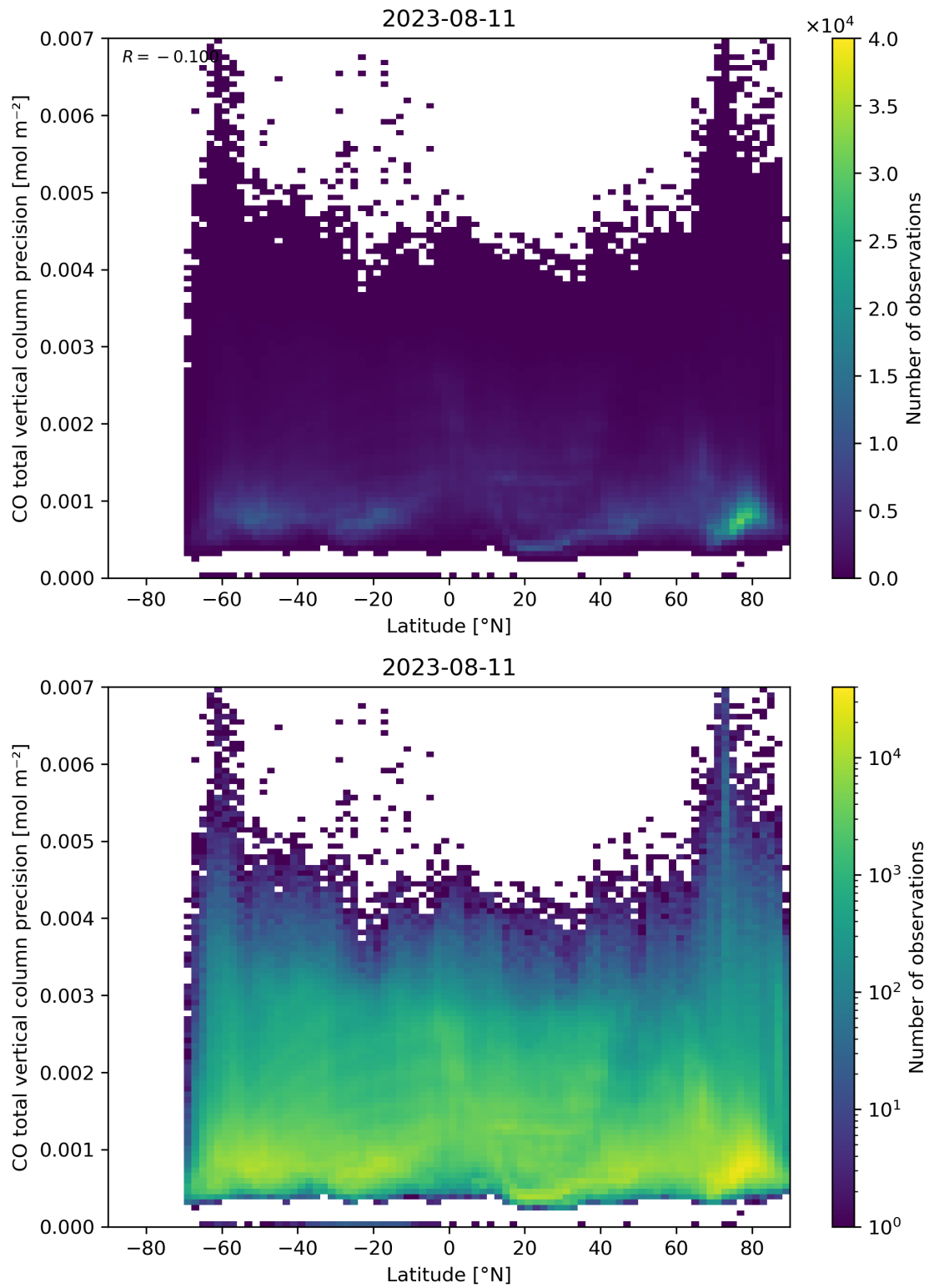
Figure 53: Scatter density plot of “Latitude” against “CO total vertical column precision” for 2023-08-10 to 2023-08-12.
