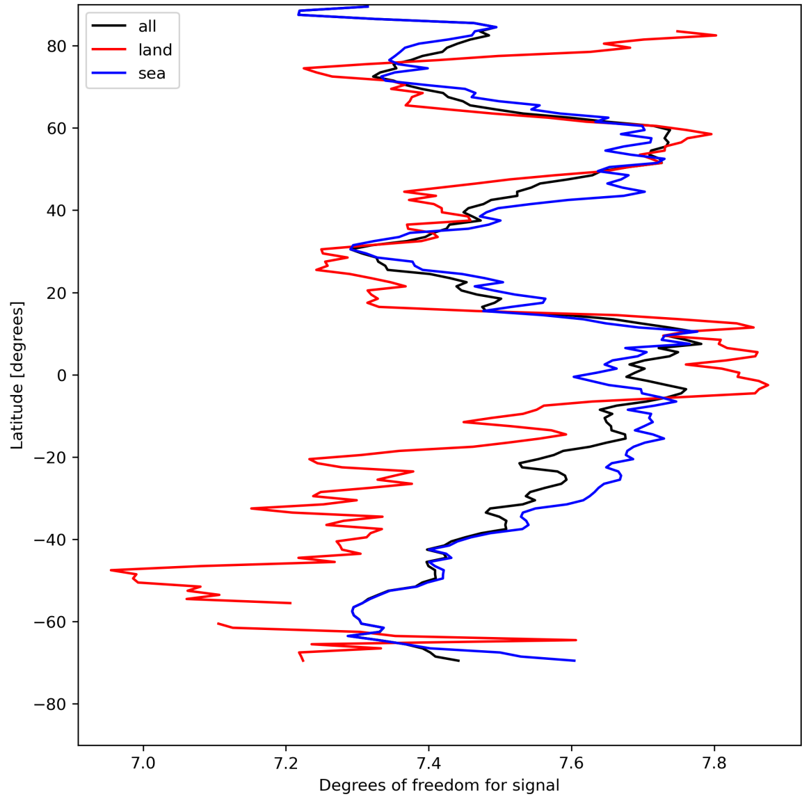
Figure 15: Zonal average of “Degrees of freedom for signal” for 2023-08-10 to 2023-08-12.
