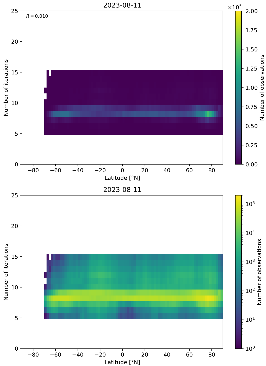
Figure 56: Scatter density plot of “Latitude” against “Number of iterations” for 2023-08-10 to 2023-08-12.
