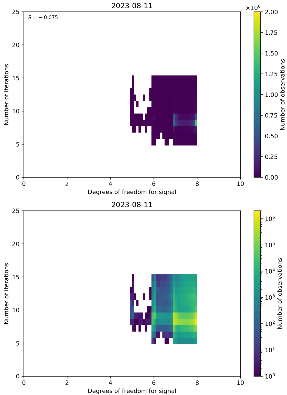
Figure 50: Scatter density plot of “Degrees of freedom for signal” against “Number of iterations” for 2023-08-10 to 2023-08-12.
