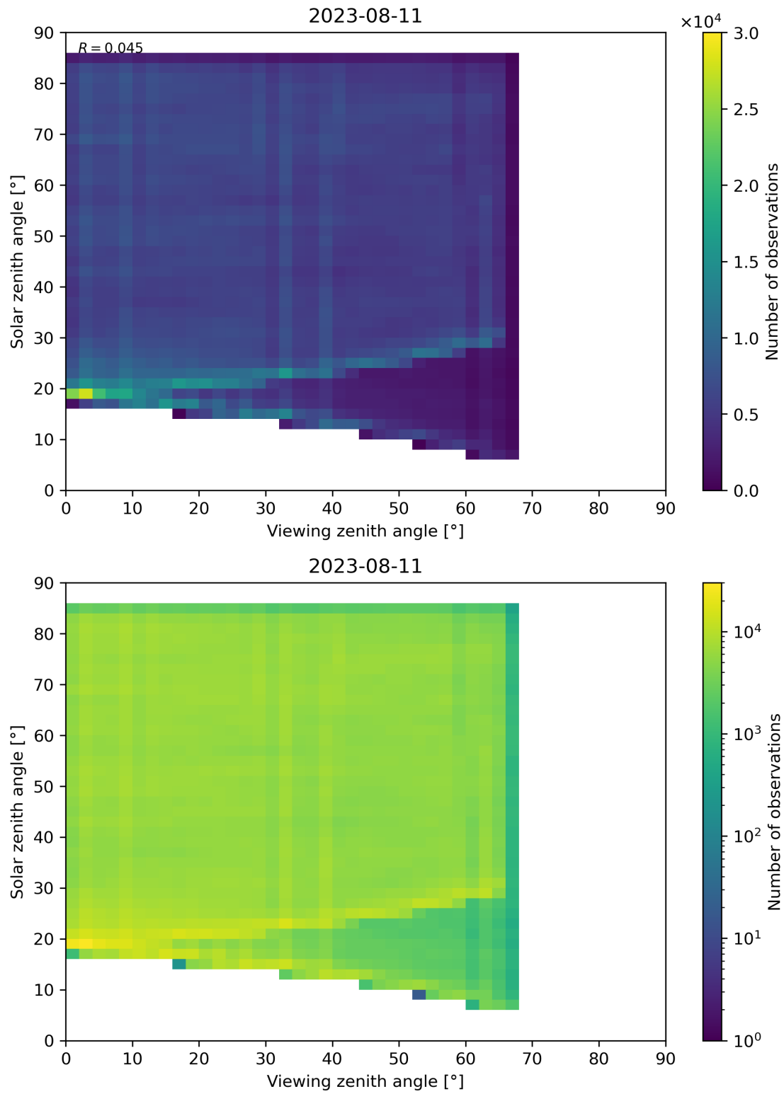
Figure 77: Scatter density plot of “Viewing zenith angle” against “Solar zenith angle” for 2023-08-10 to 2023-08-12.
