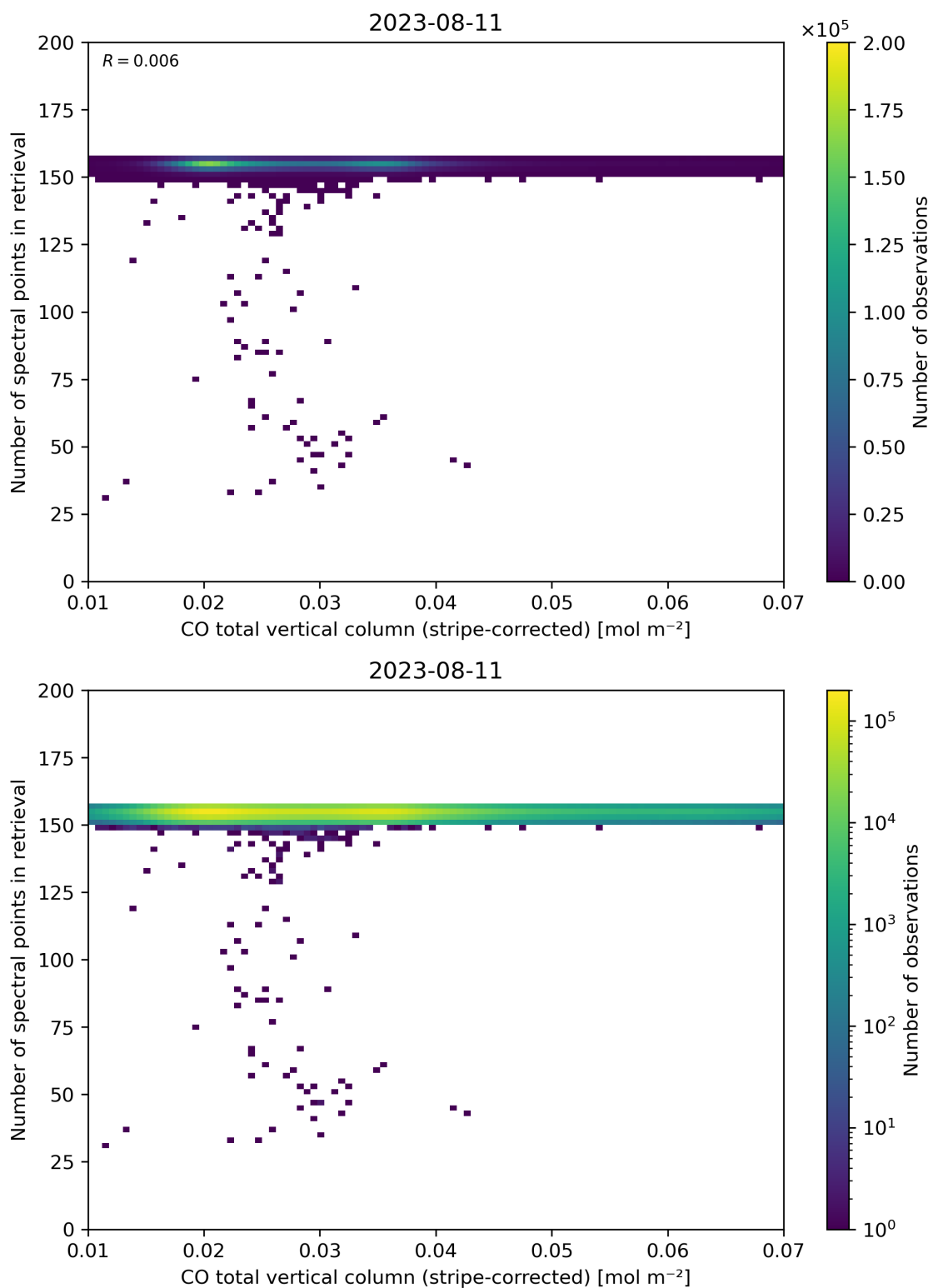
Figure 40: Scatter density plot of “CO total vertical column (stripe-corrected)” against “Number of spectral points in retrieval” for 2023-08-10 to 2023-08-12.
