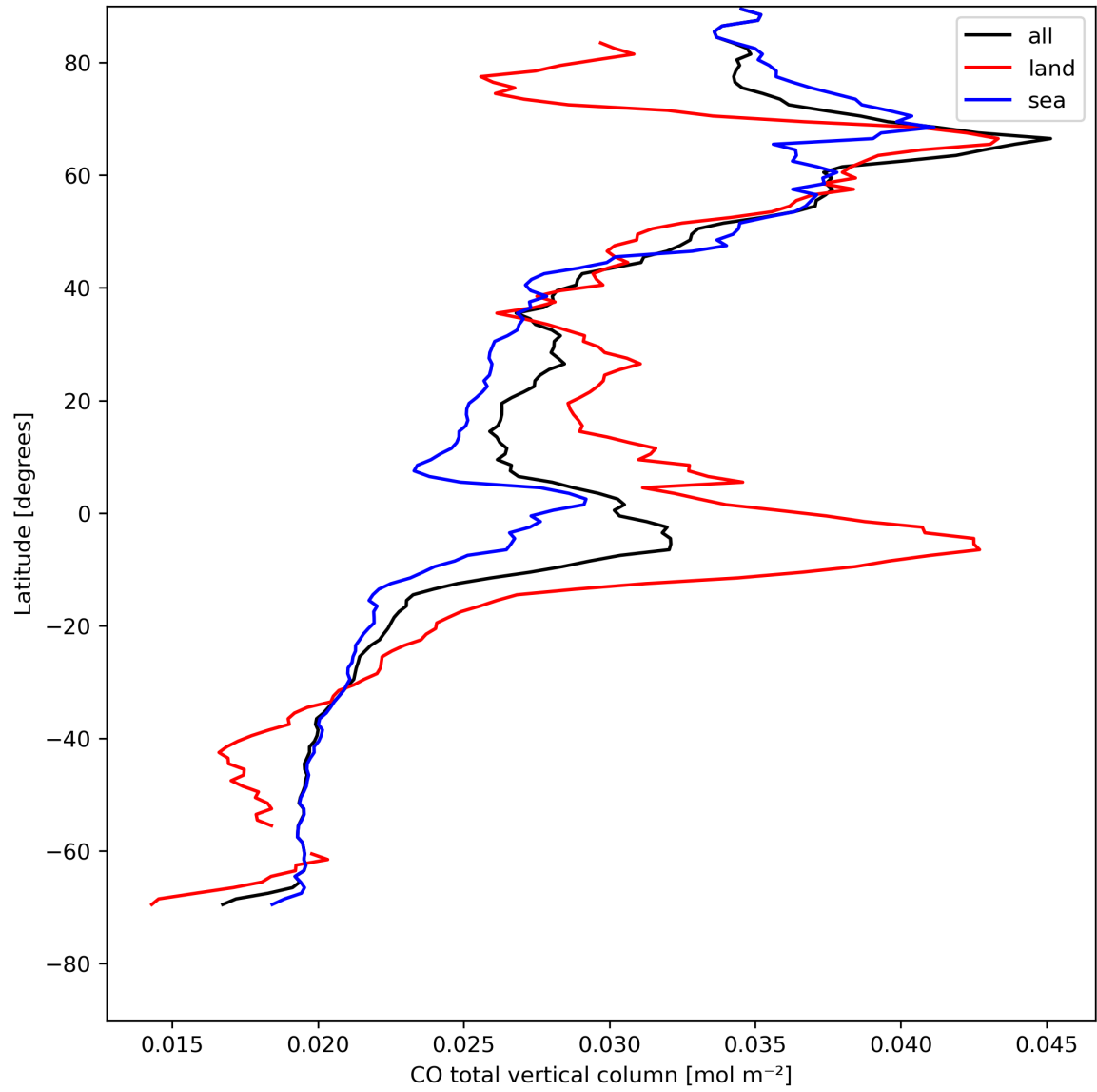
Figure 10: Zonal average of “CO total vertical column” for 2023-08-10 to 2023-08-12.
