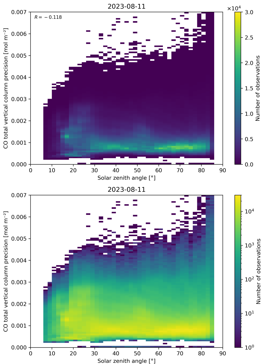
Figure 63: Scatter density plot of “Solar zenith angle” against “CO total vertical column precision” for 2023-08-10 to 2023-08-12.
