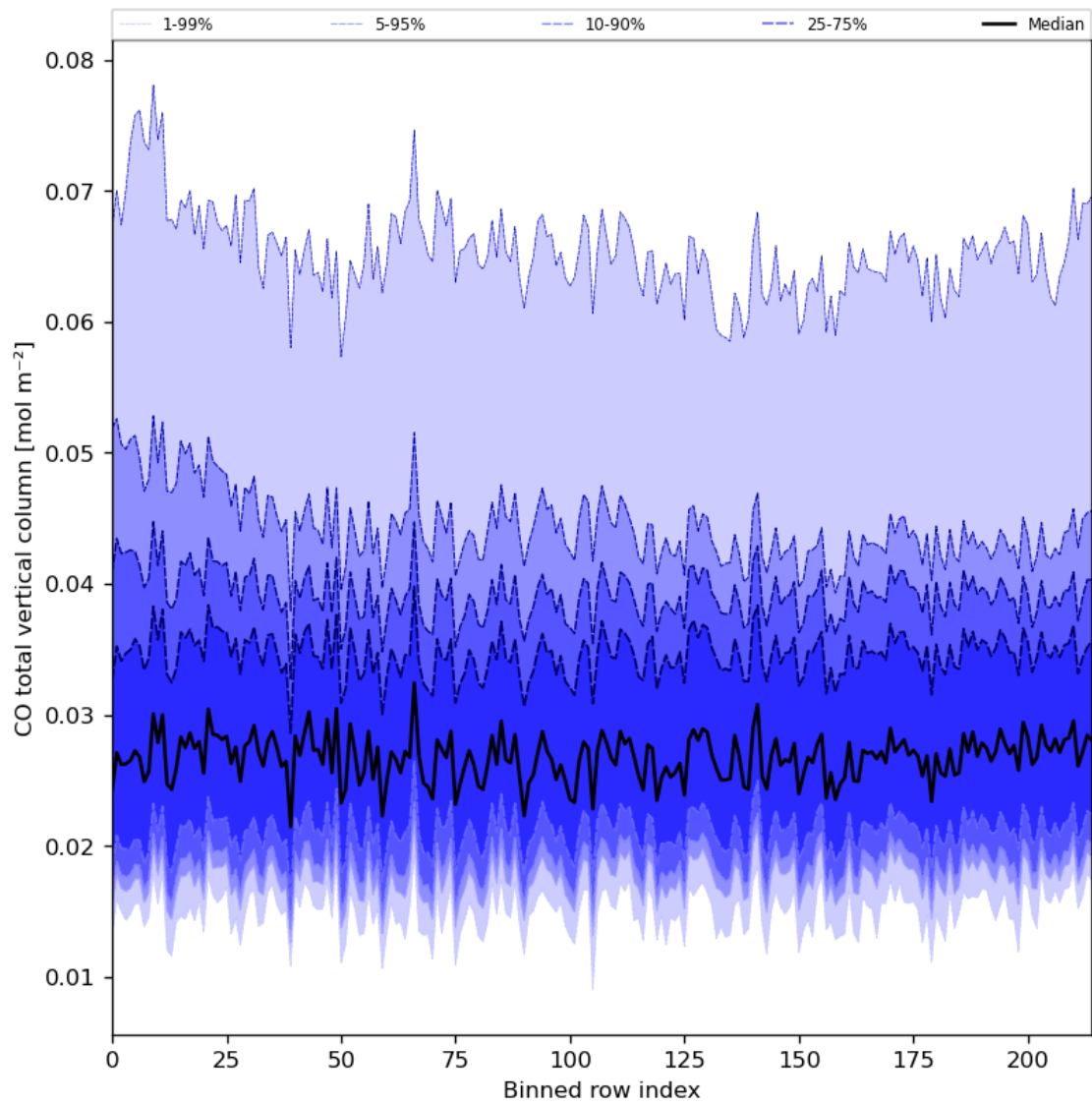
Figure 26: Along track statistics of “CO total vertical column” for 2023-08-10 to 2023-08-12
