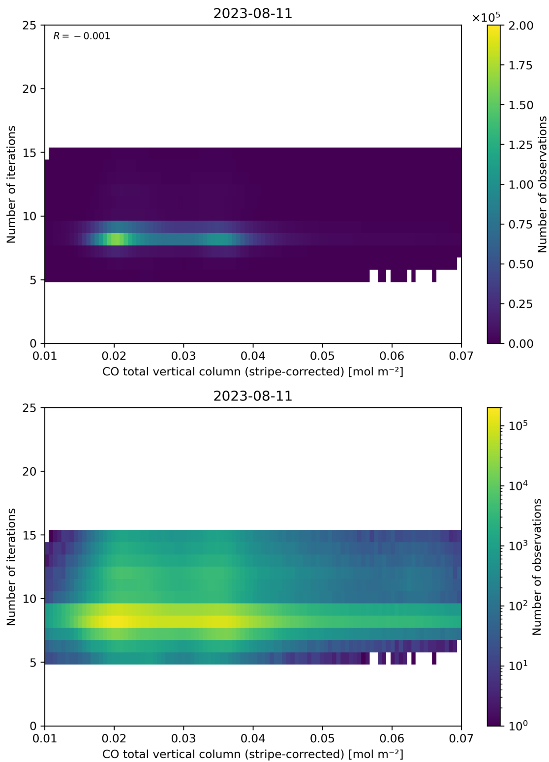
Figure 39: Scatter density plot of “CO total vertical column (stripe-corrected)” against “Number of iterations” for 2023-08-10 to 2023-08-12.
