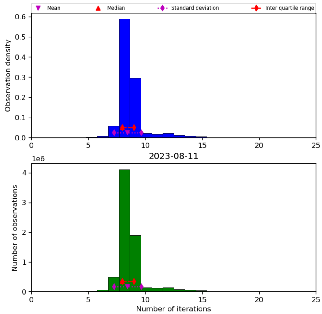
Figure 24: Histogram of “Number of iterations” for 2023-08-10 to 2023-08-12
