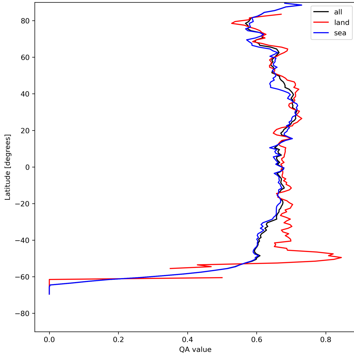
Figure 9: Zonal average of “QA value” for 2023-08-10 to 2023-08-12.
