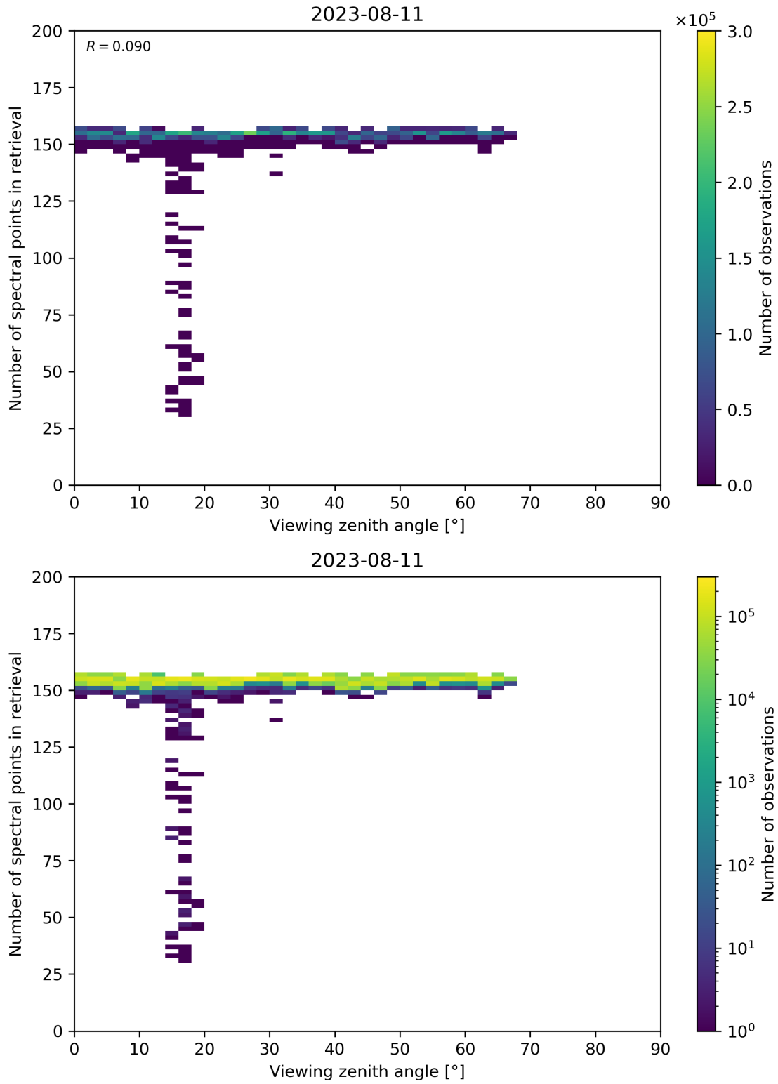
Figure 76: Scatter density plot of “Viewing zenith angle” against “Number of spectral points in retrieval” for 2023-08-10 to 2023-08-12.
