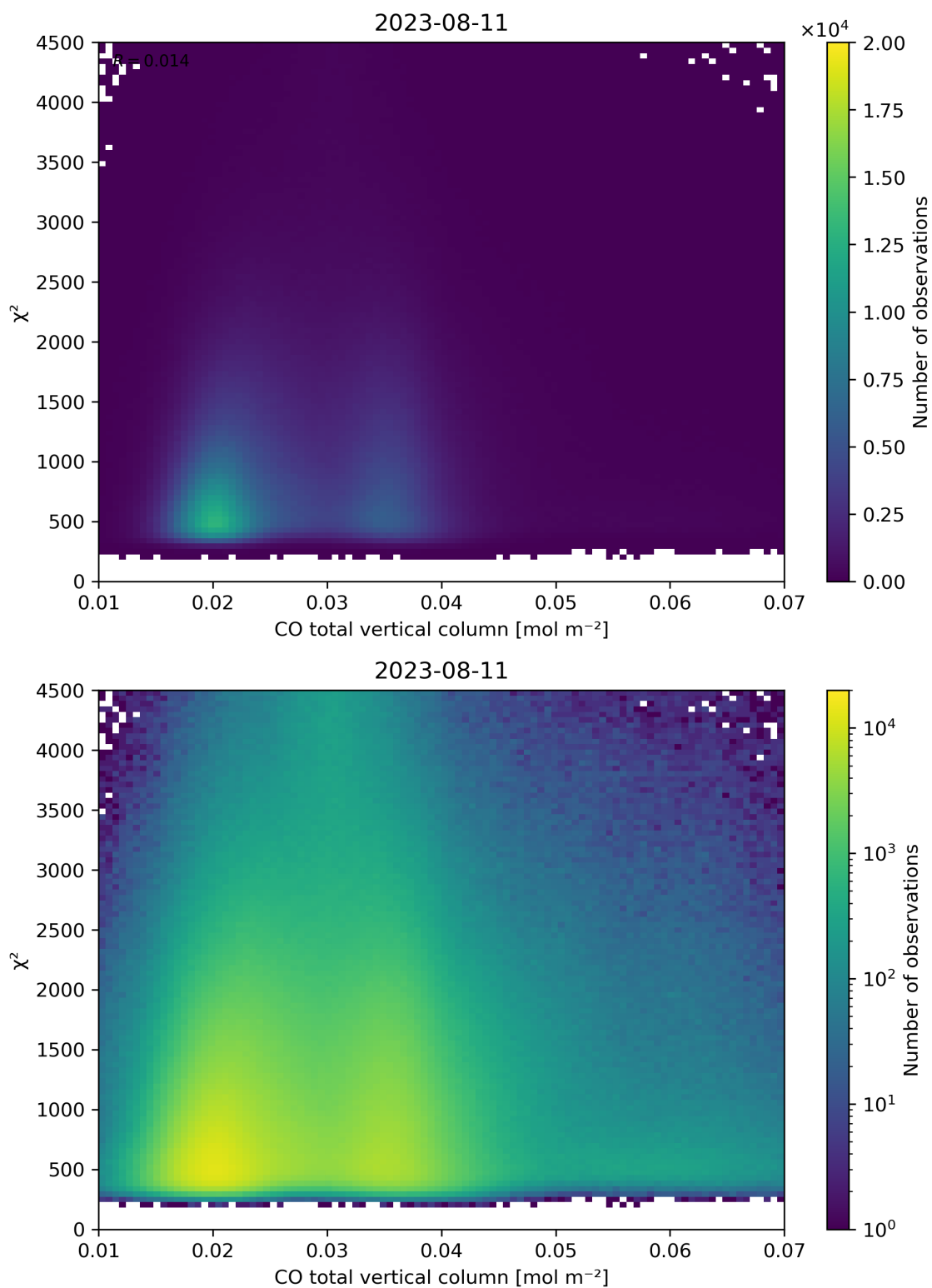
Figure 35: Scatter density plot of “CO total vertical column” against “ \chi^2 ” for 2023-08-10 to 2023-08-12.
