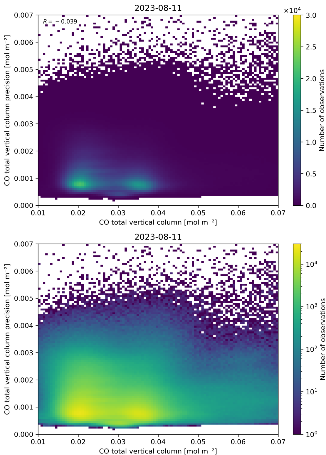
Figure 34: Scatter density plot of “CO total vertical column” against “CO total vertical column precision” for 2023-08-10 to 2023-08-12.
