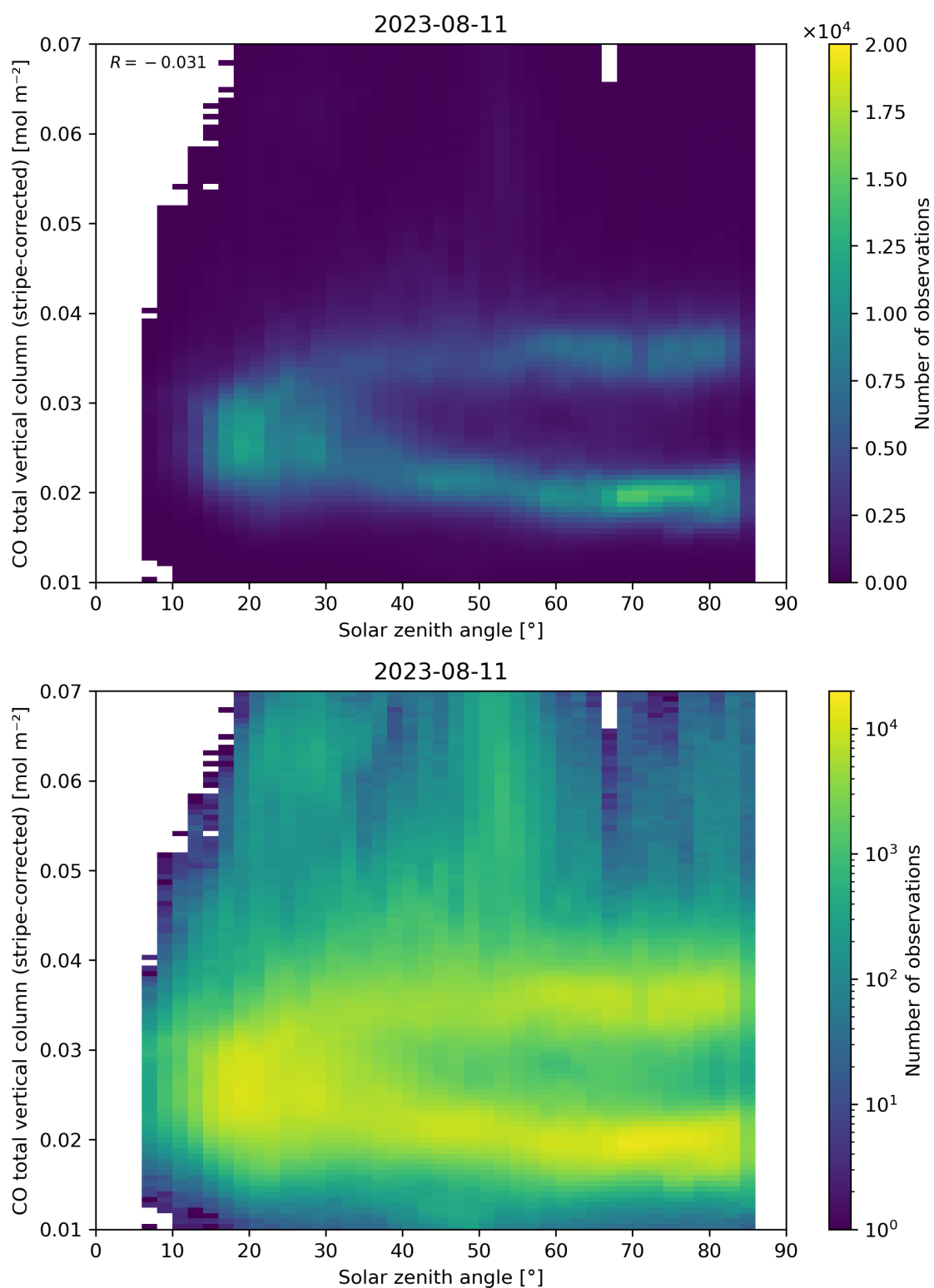
Figure 62: Scatter density plot of “Solar zenith angle” against “CO total vertical column (stripe-corrected)” for 2023-08-10 to 2023-08-12.
