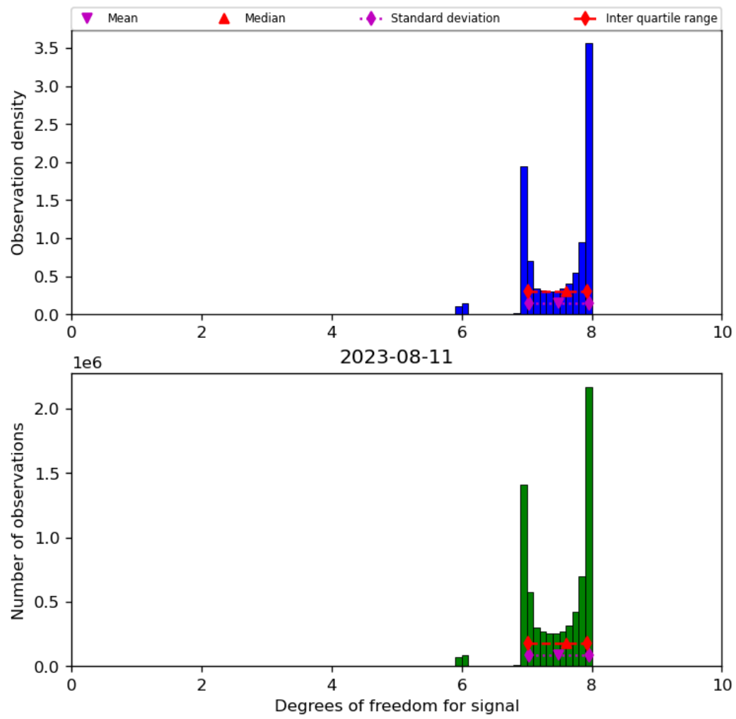
Figure 23: Histogram of “Degrees of freedom for signal” for 2023-08-10 to 2023-08-12
