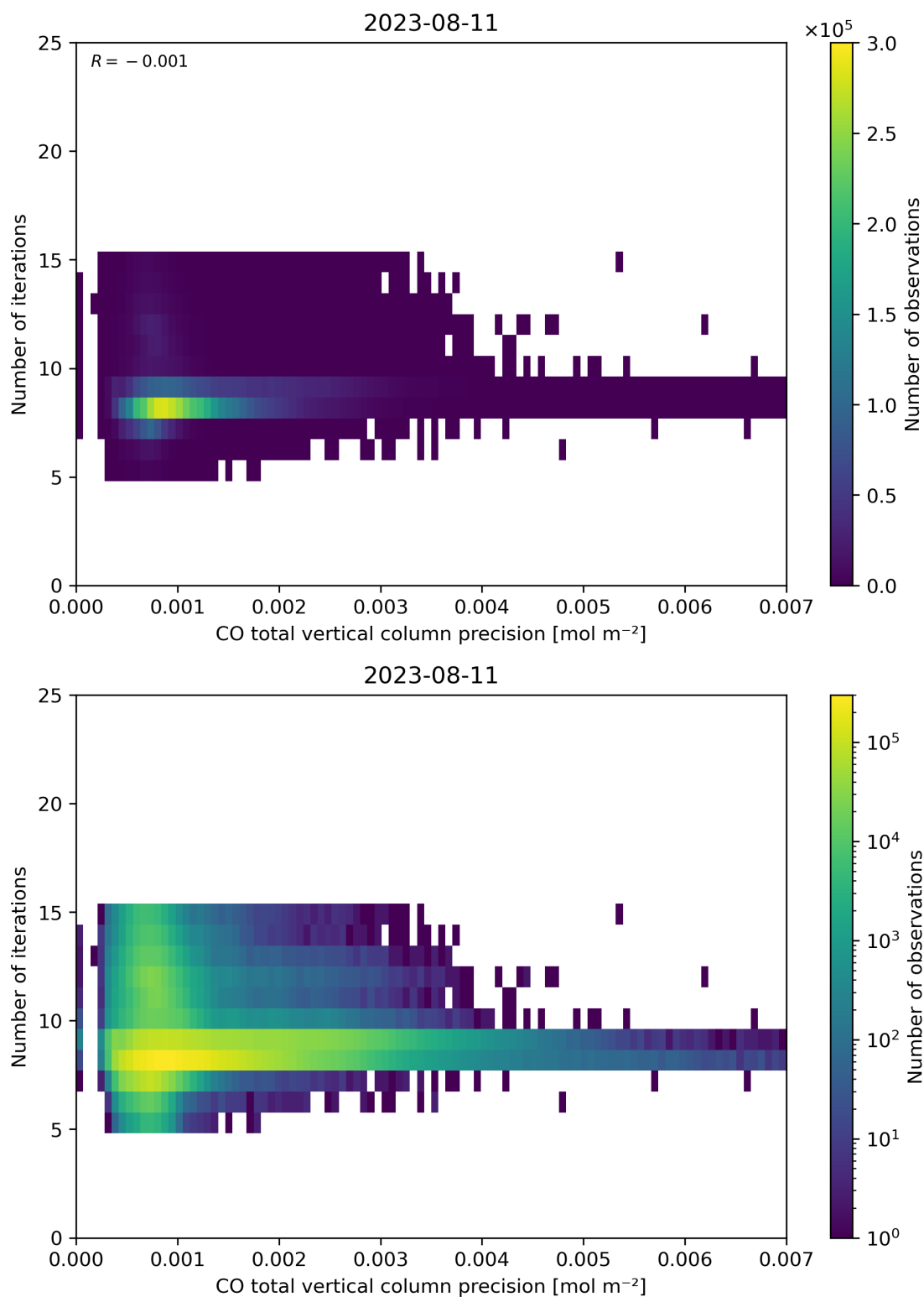
Figure 46: Scatter density plot of “CO total vertical column precision” against “Number of iterations” for 2023-08-10 to 2023-08-12.
