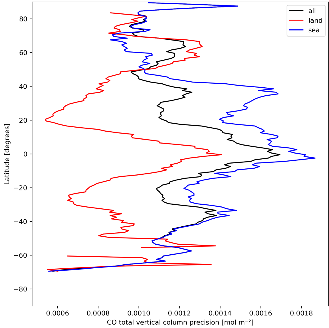
Figure 12: Zonal average of “CO total vertical column precision” for 2023-08-10 to 2023-08-12.
