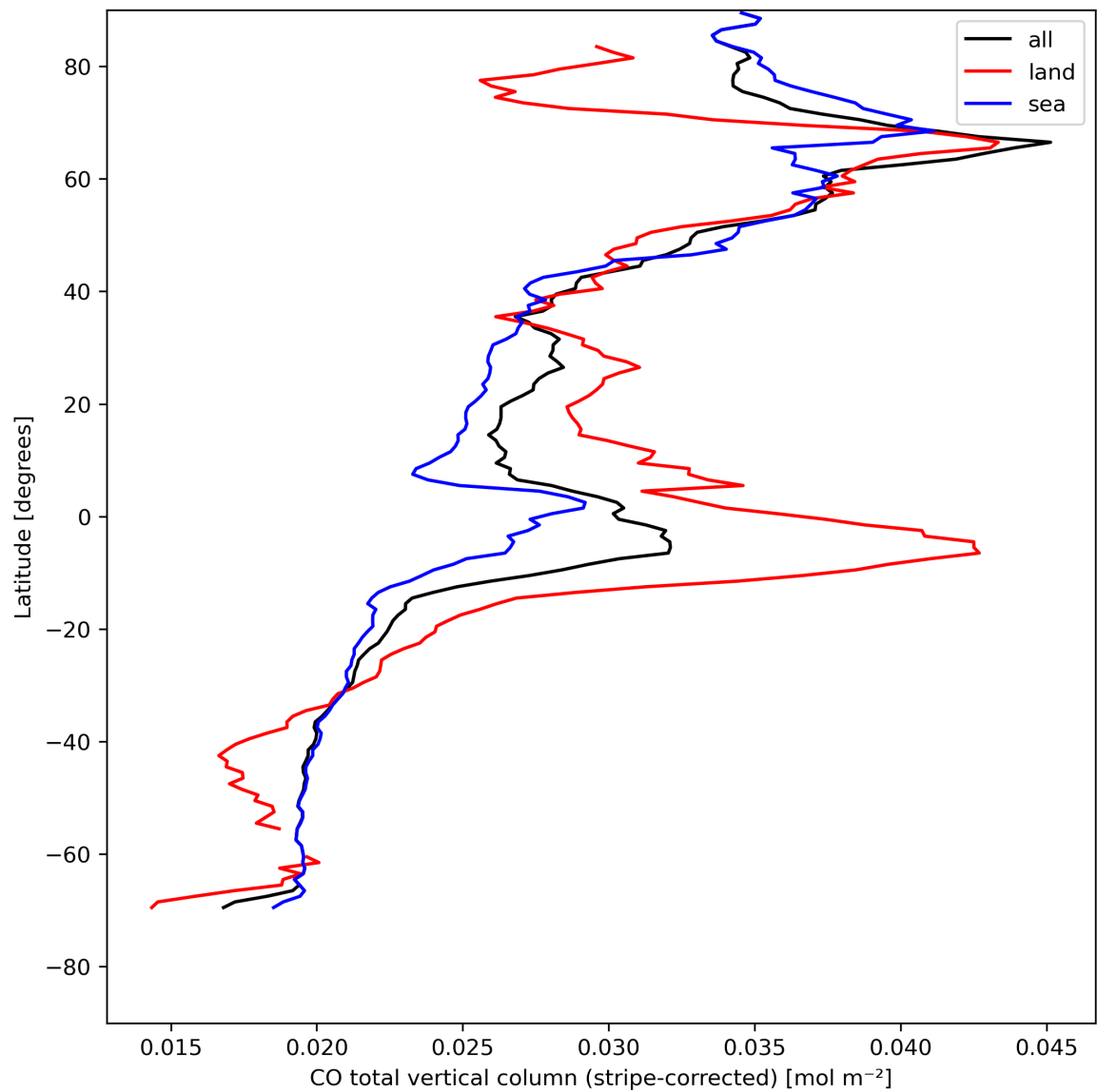
Figure 11: Zonal average of “CO total vertical column (stripe-corrected)” for 2023-08-10 to 2023-08-12.
