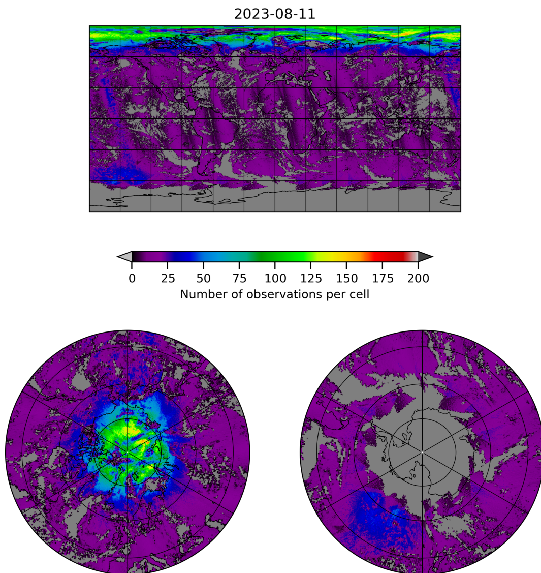
Figure 8: Map of the number of observations for 2023-08-10 to 2023-08-12
