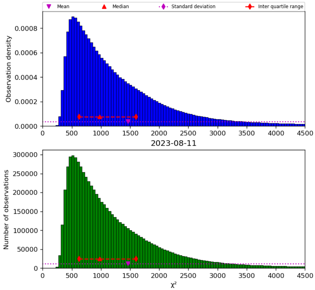
Figure 22: Histogram of “ \chi^2 ” for 2023-08-10 to 2023-08-12
