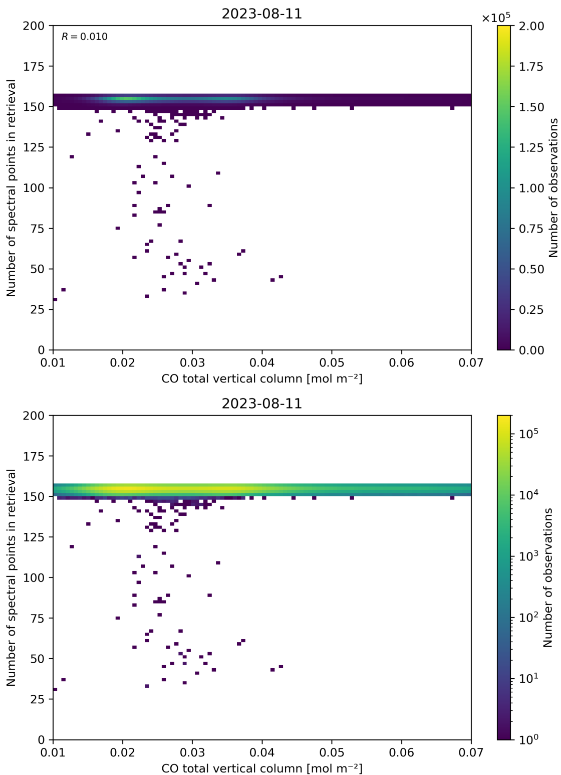
Figure 43: Scatter density plot of “CO total vertical column” against “Number of spectral points in retrieval” for 2023-08-10 to 2023-08-12.
