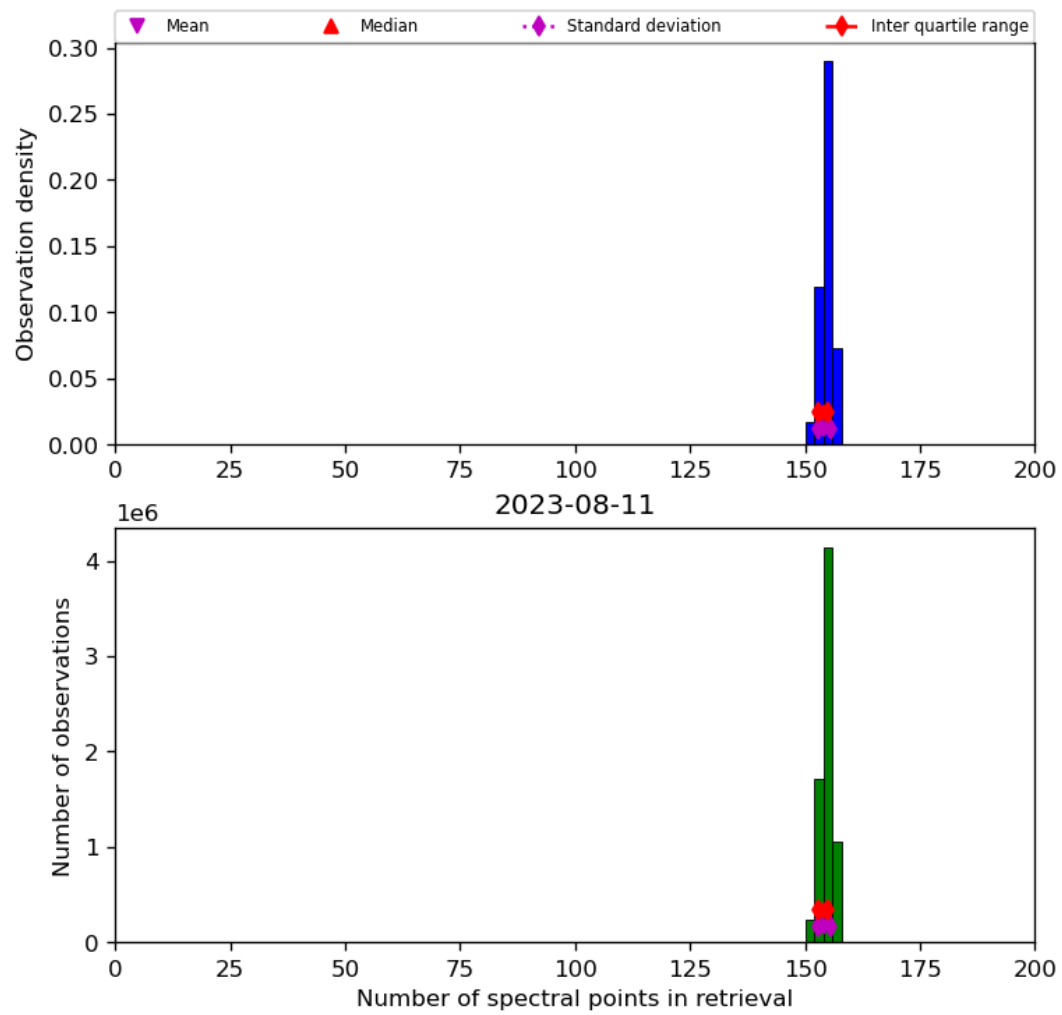
Figure 21: Histogram of “Number of spectral points in retrieval” for 2023-08-10 to 2023-08-12
