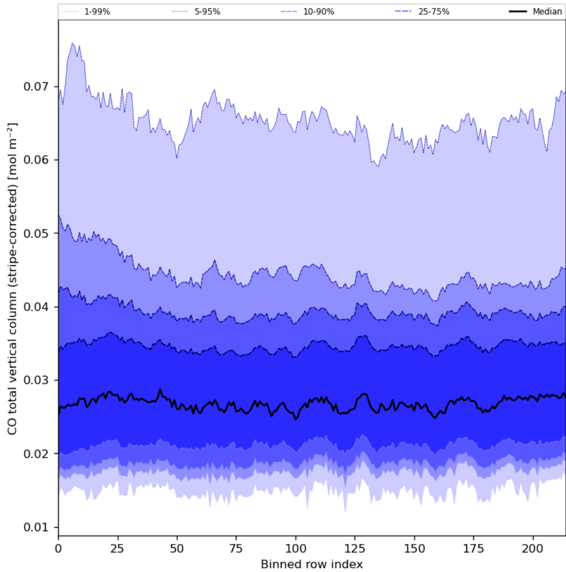
Figure 27: Along track statistics of "CO total vertical column (stripe-corrected)" for 2023-08-10 to 2023-08-12
