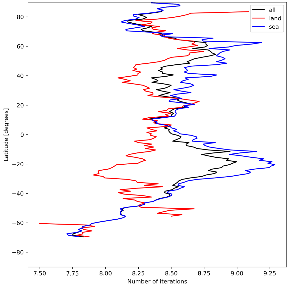
Figure 16: Zonal average of “Number of iterations” for 2023-08-10 to 2023-08-12.
