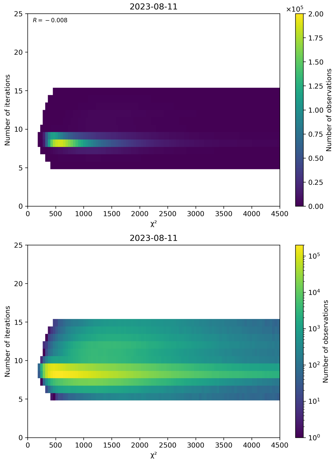
Figure 49: Scatter density plot of “ \chi^2 ” against “Number of iterations” for 2023-08-10 to 2023-08-12.
