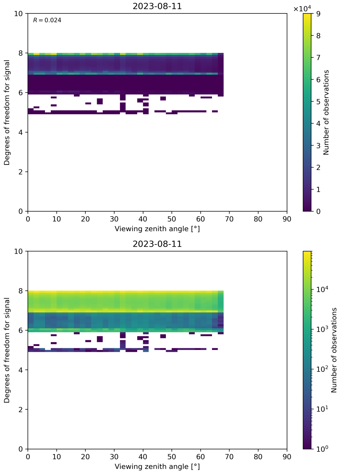
Figure 73: Scatter density plot of “Viewing zenith angle” against “Degrees of freedom for signal” for 2023-08-10 to 2023-08-12.
