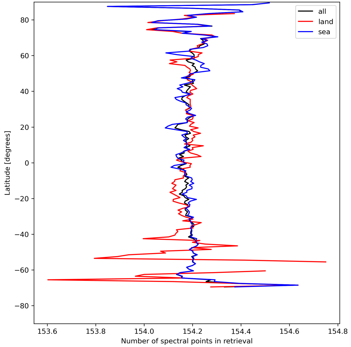
Figure 13: Zonal average of “Number of spectral points in retrieval” for 2023-08-10 to 2023-08-12.
