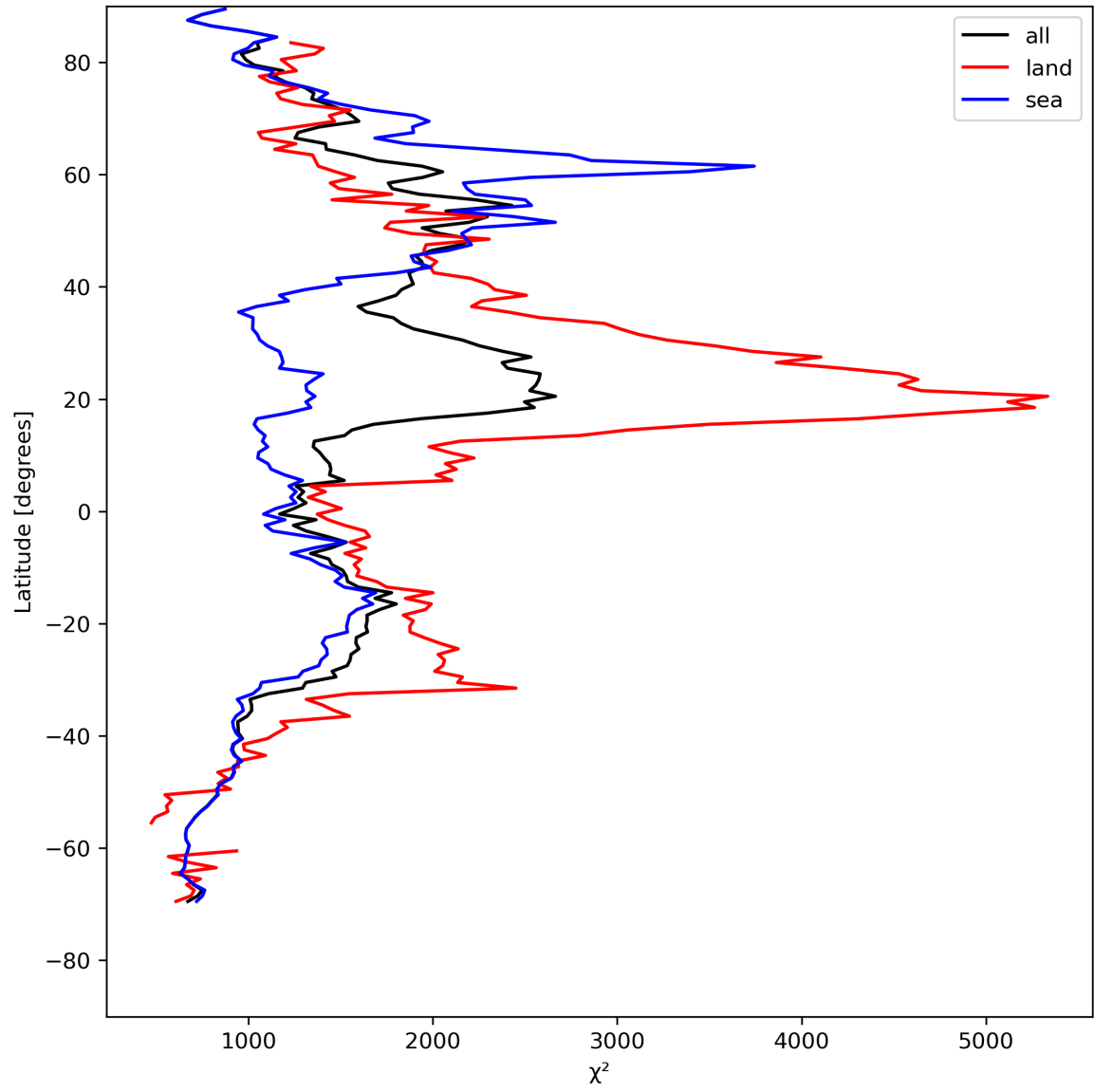
Figure 14: Zonal average of “ \chi^2 ” for 2023-08-10 to 2023-08-12.
