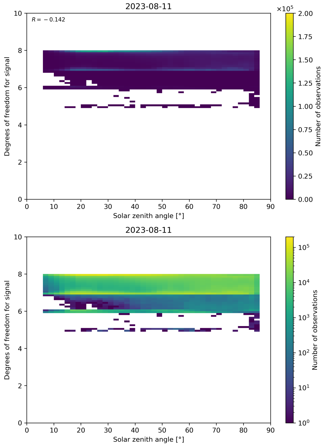
Figure 65: Scatter density plot of “Solar zenith angle” against “Degrees of freedom for signal” for 2023-08-10 to 2023-08-12.
