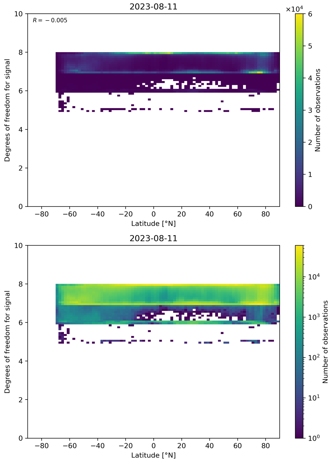
Figure 55: Scatter density plot of “Latitude” against “Degrees of freedom for signal” for 2023-08-10 to 2023-08-12.
