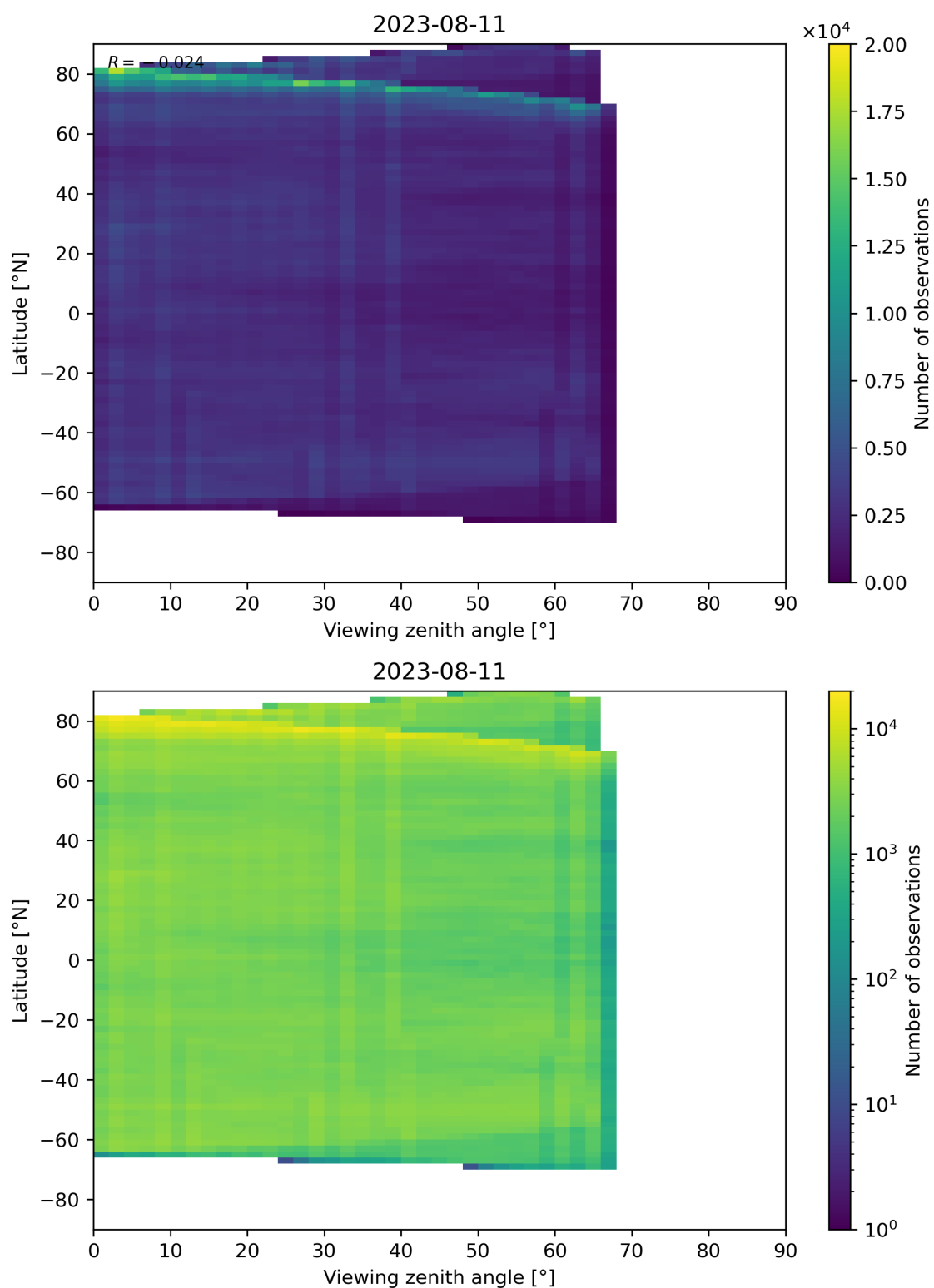
Figure 74: Scatter density plot of “Viewing zenith angle” against “Latitude” for 2023-08-10 to 2023-08-12.
