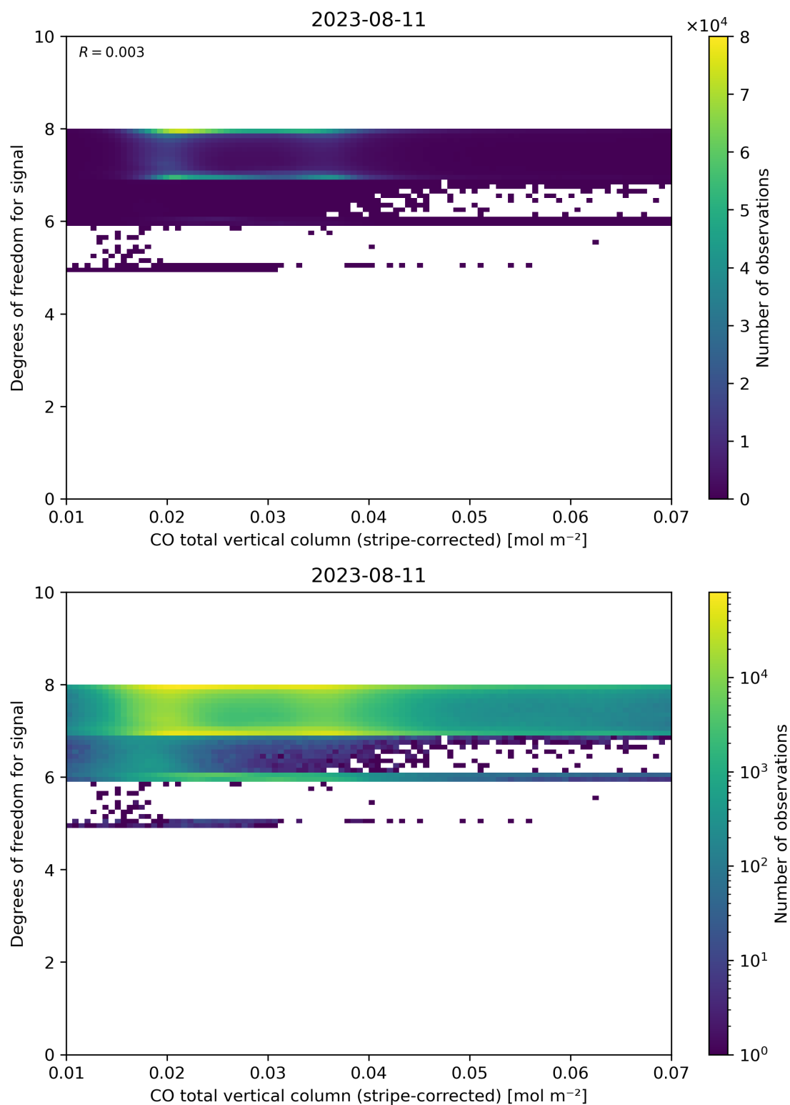
Figure 38: Scatter density plot of “CO total vertical column (stripe-corrected)” against “Degrees of freedom for signal” for 2023-08-10 to 2023-08-12.
