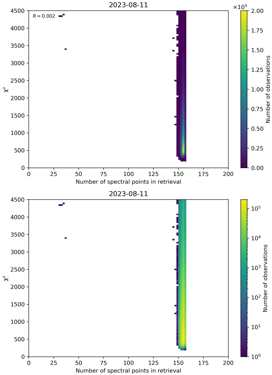
Figure 58: Scatter density plot of “Number of spectral points in retrieval” against “ \chi^2 ” for 2023-08-10 to 2023-08-12.
