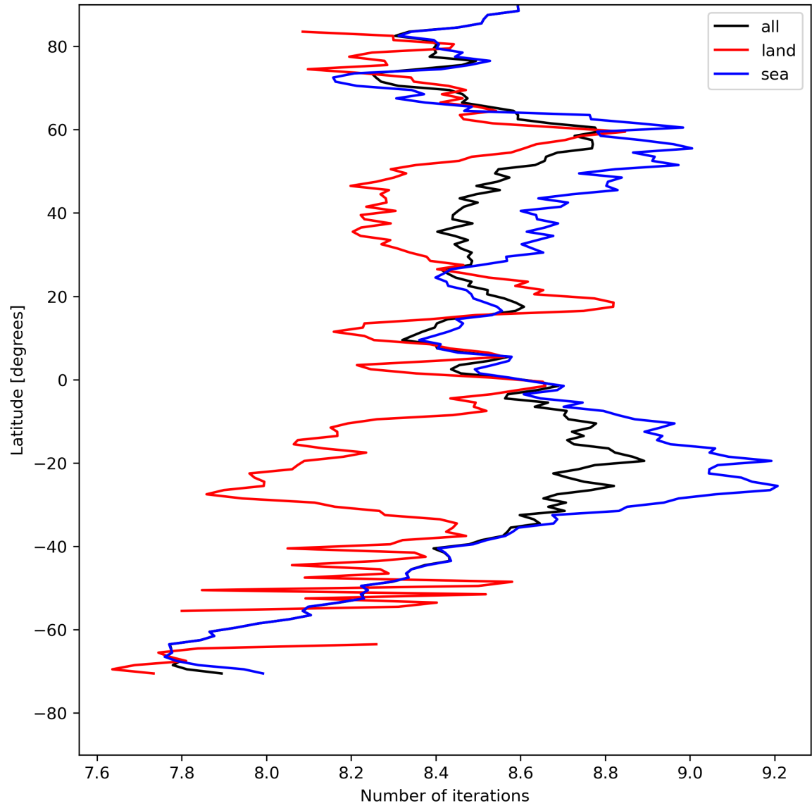
Figure 16: Zonal average of “Number of iterations” for 2023-08-14 to 2023-08-15.
