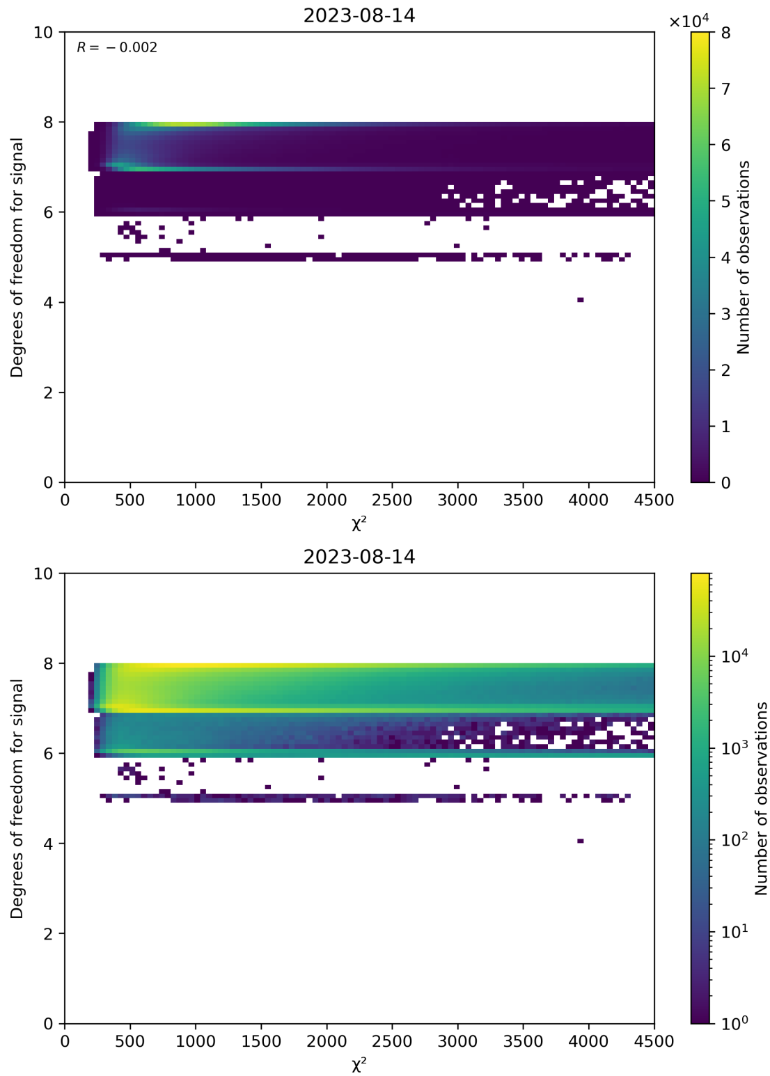
Figure 48: Scatter density plot of “ \chi^2 ” against “Degrees of freedom for signal” for 2023-08-14 to 2023-08-15.
