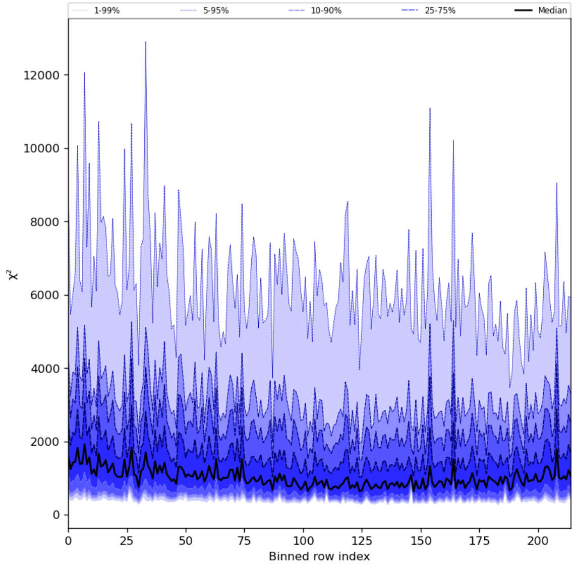
Figure 30: Along track statistics of “ \chi^2 ” for 2023-08-14 to 2023-08-15
