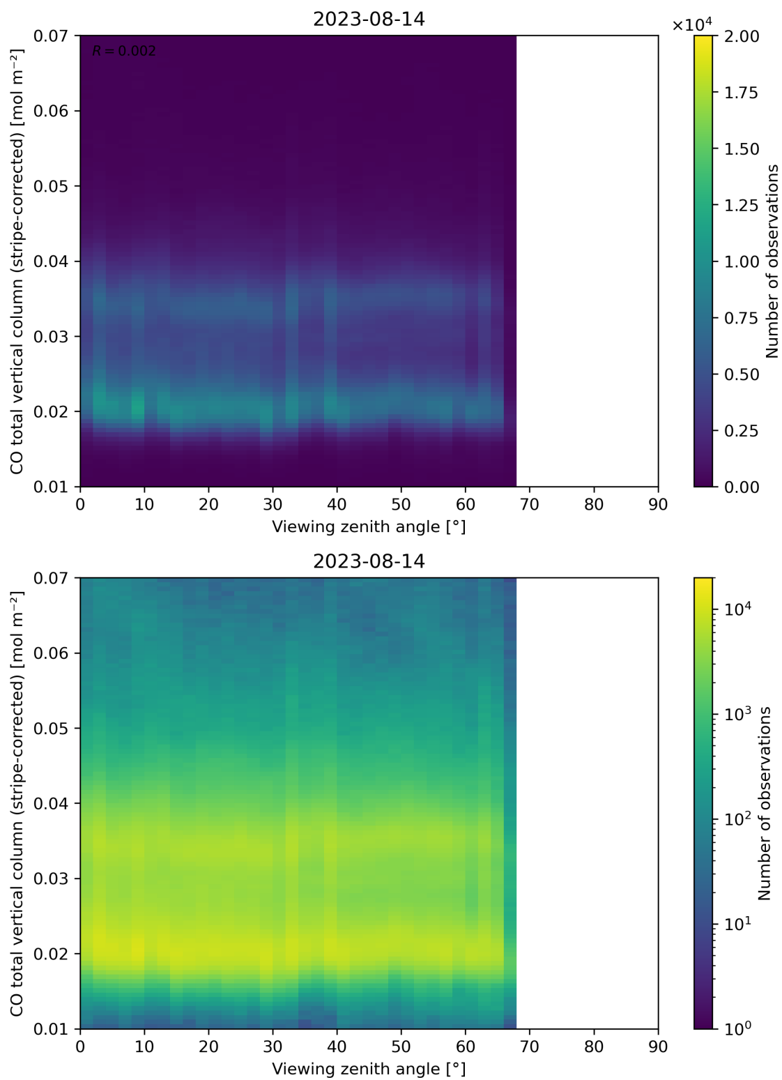
Figure 70: Scatter density plot of “Viewing zenith angle” against “CO total vertical column (stripe-corrected)” for 2023-08-14 to 2023-08-15.
