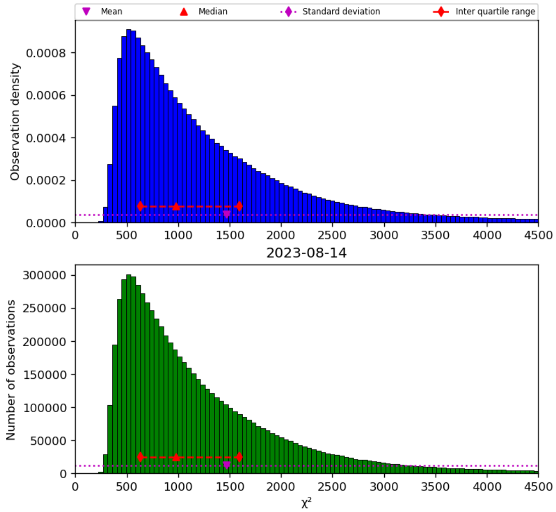
Figure 22: Histogram of “ \chi^2 ” for 2023-08-14 to 2023-08-15
