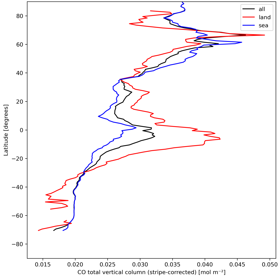
Figure 11: Zonal average of “CO total vertical column (stripe-corrected)” for 2023-08-14 to 2023-08-15.
