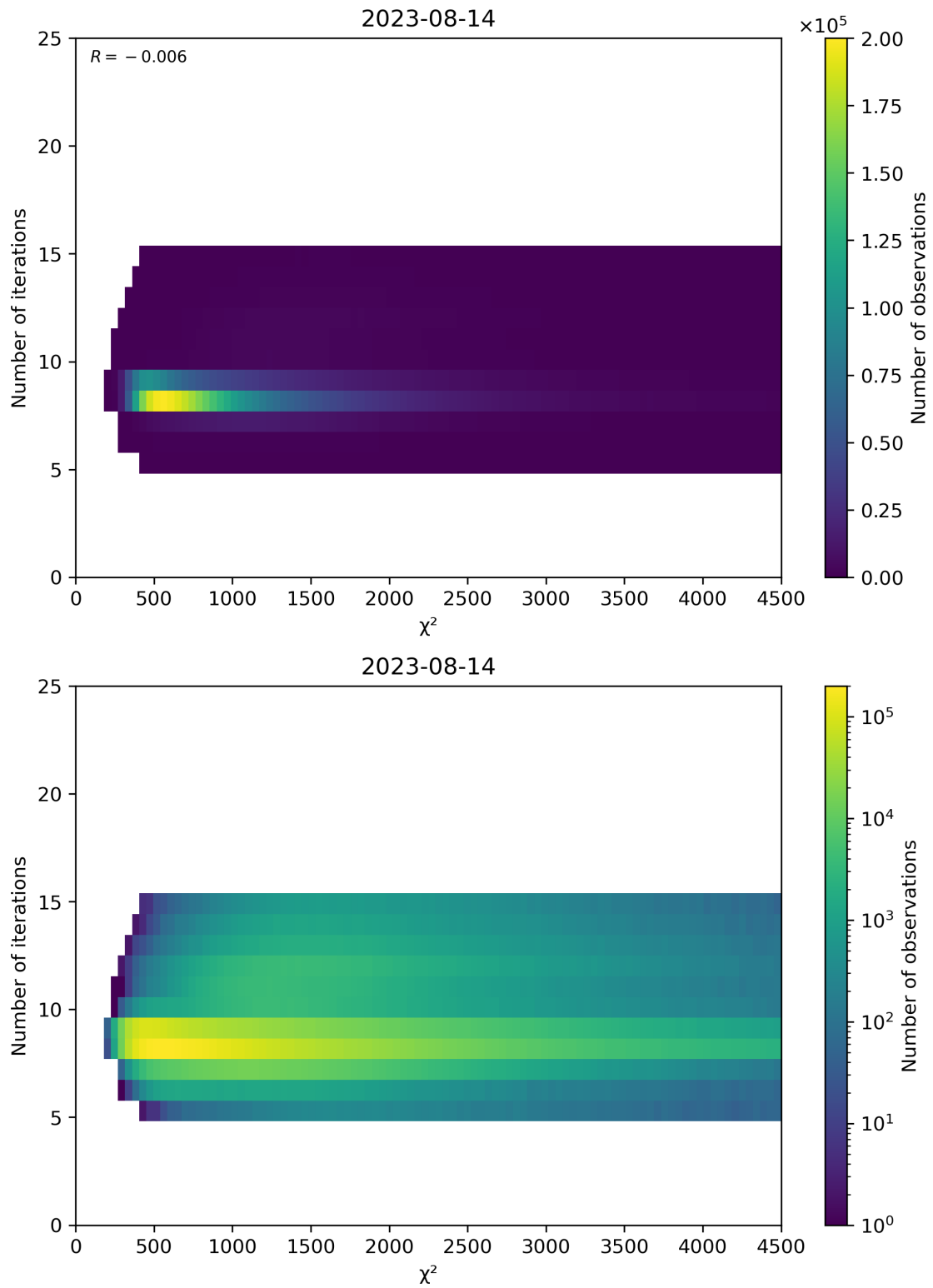
Figure 49: Scatter density plot of “ \chi^2 ” against “Number of iterations” for 2023-08-14 to 2023-08-15.
