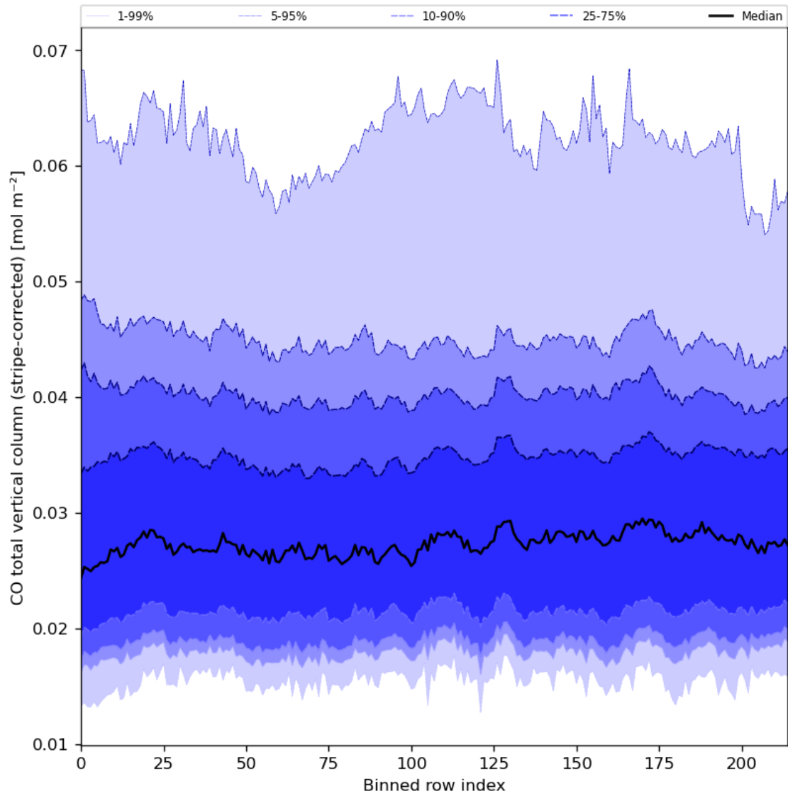
Figure 27: Along track statistics of “CO total vertical column (stripe-corrected)” for 2023-08-14 to 2023-08-15
