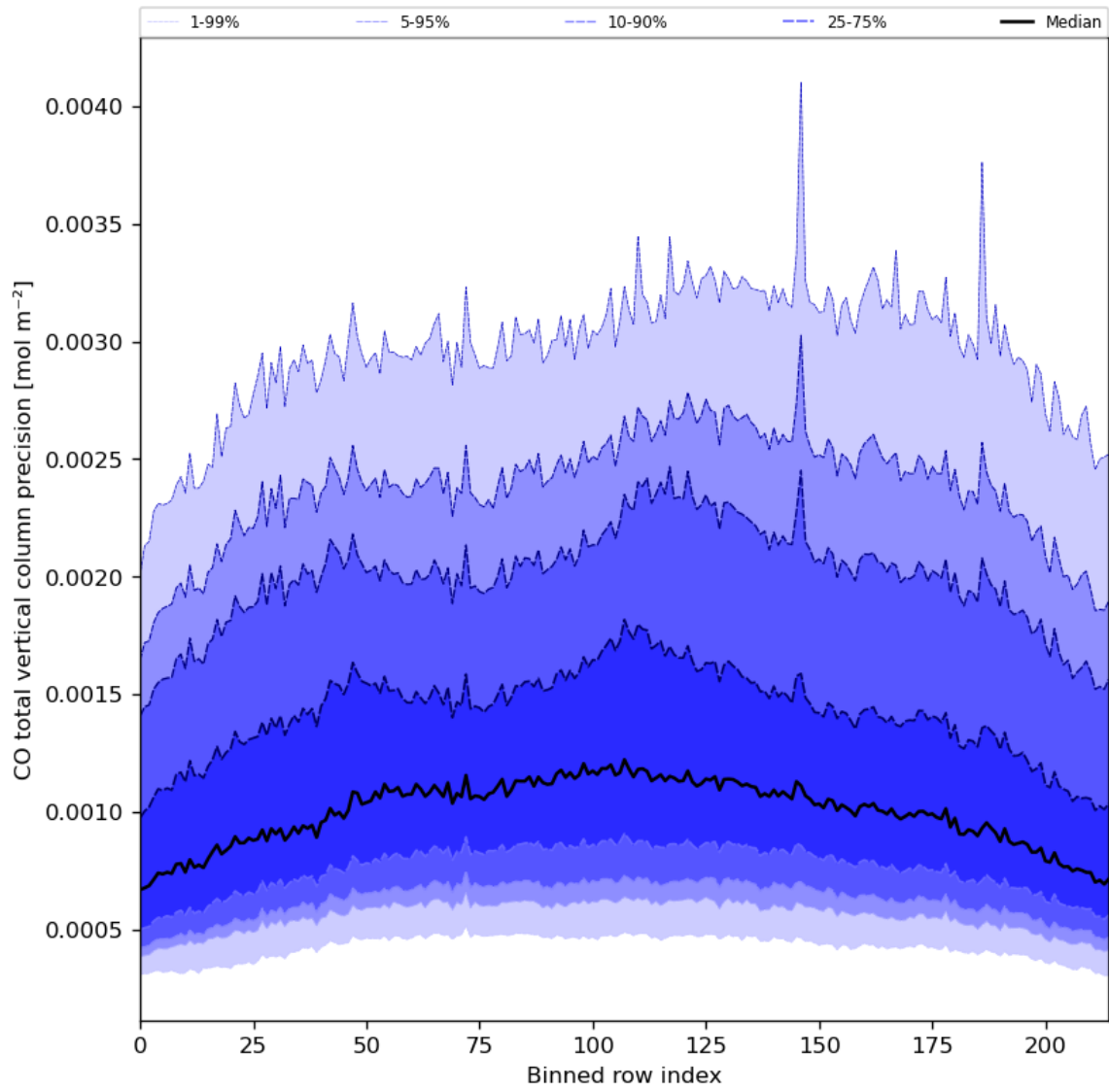
Figure 28: Along track statistics of “CO total vertical column precision” for 2023-08-14 to 2023-08-15
