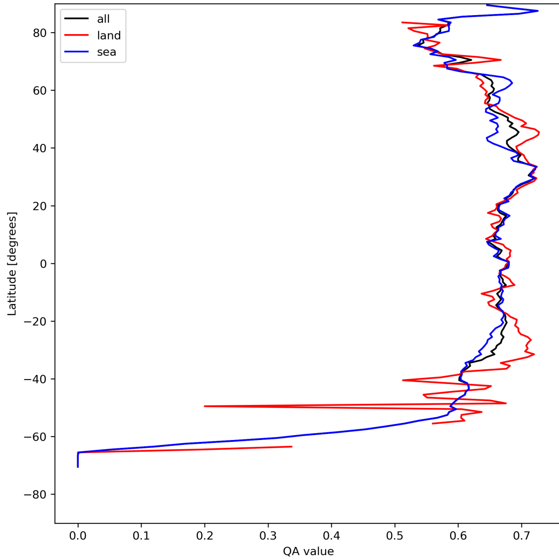
Figure 9: Zonal average of “QA value” for 2023-08-14 to 2023-08-15.
