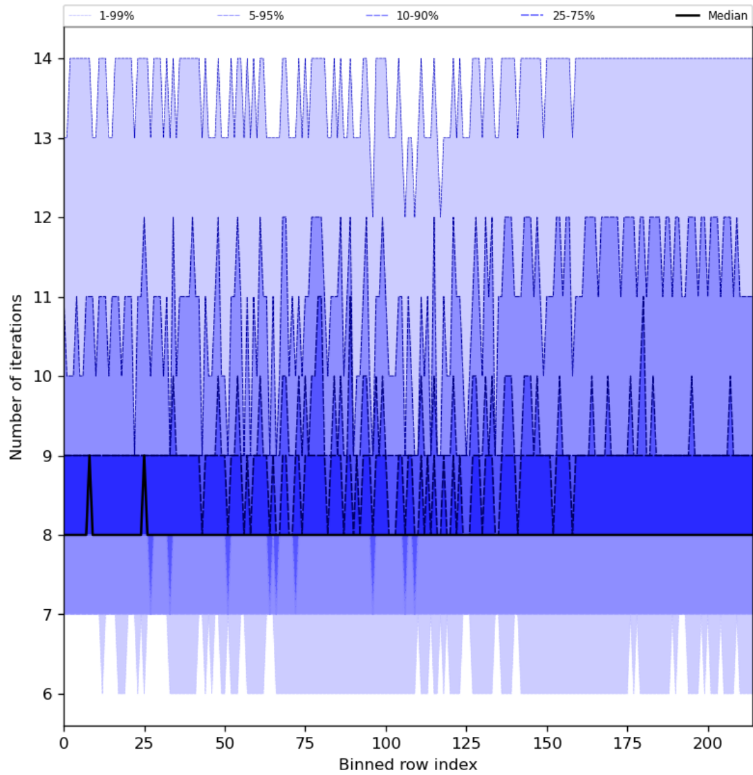
Figure 32: Along track statistics of “Number of iterations” for 2023-08-14 to 2023-08-15
