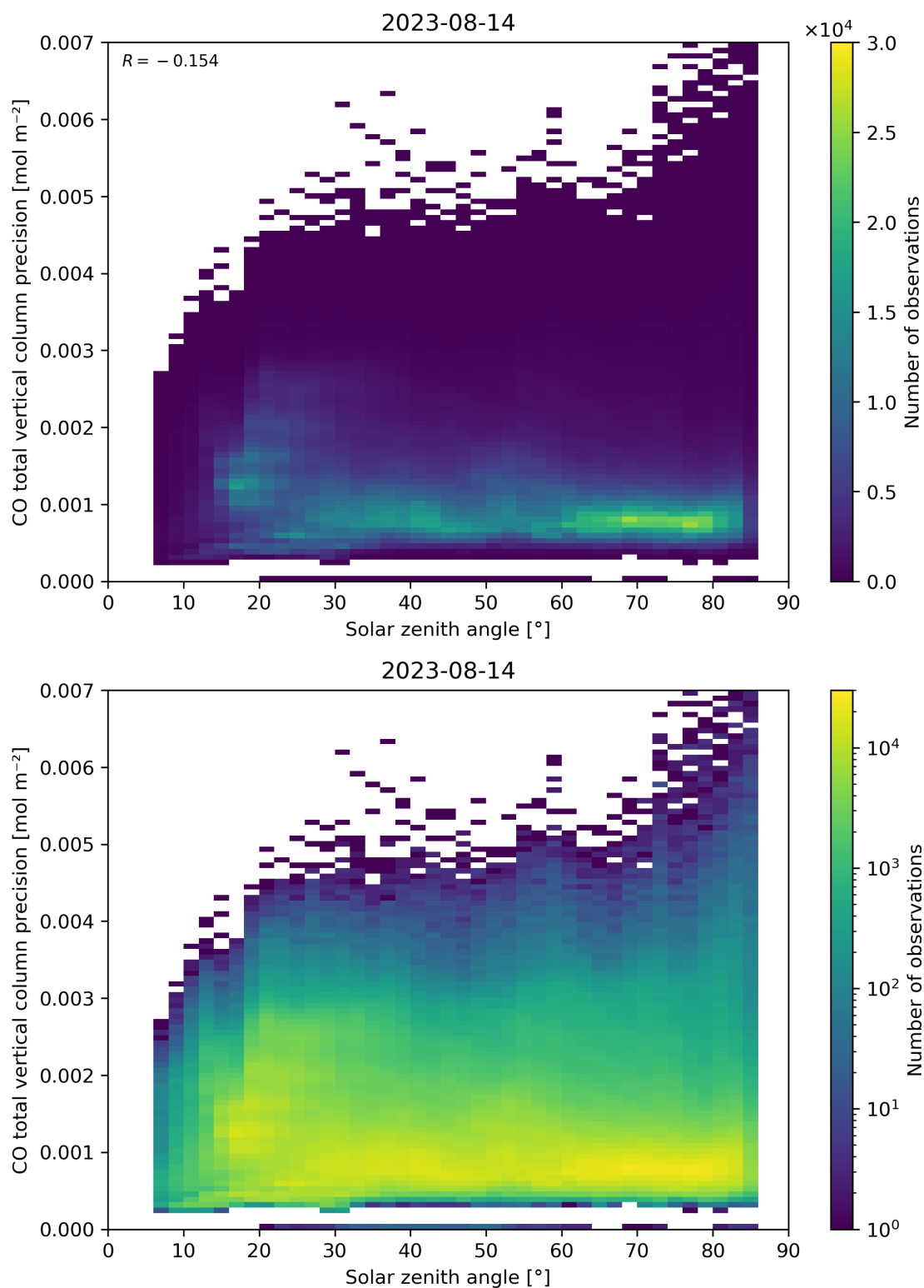
Figure 63: Scatter density plot of “Solar zenith angle” against “CO total vertical column precision” for 2023-08-14 to 2023-08-15.
