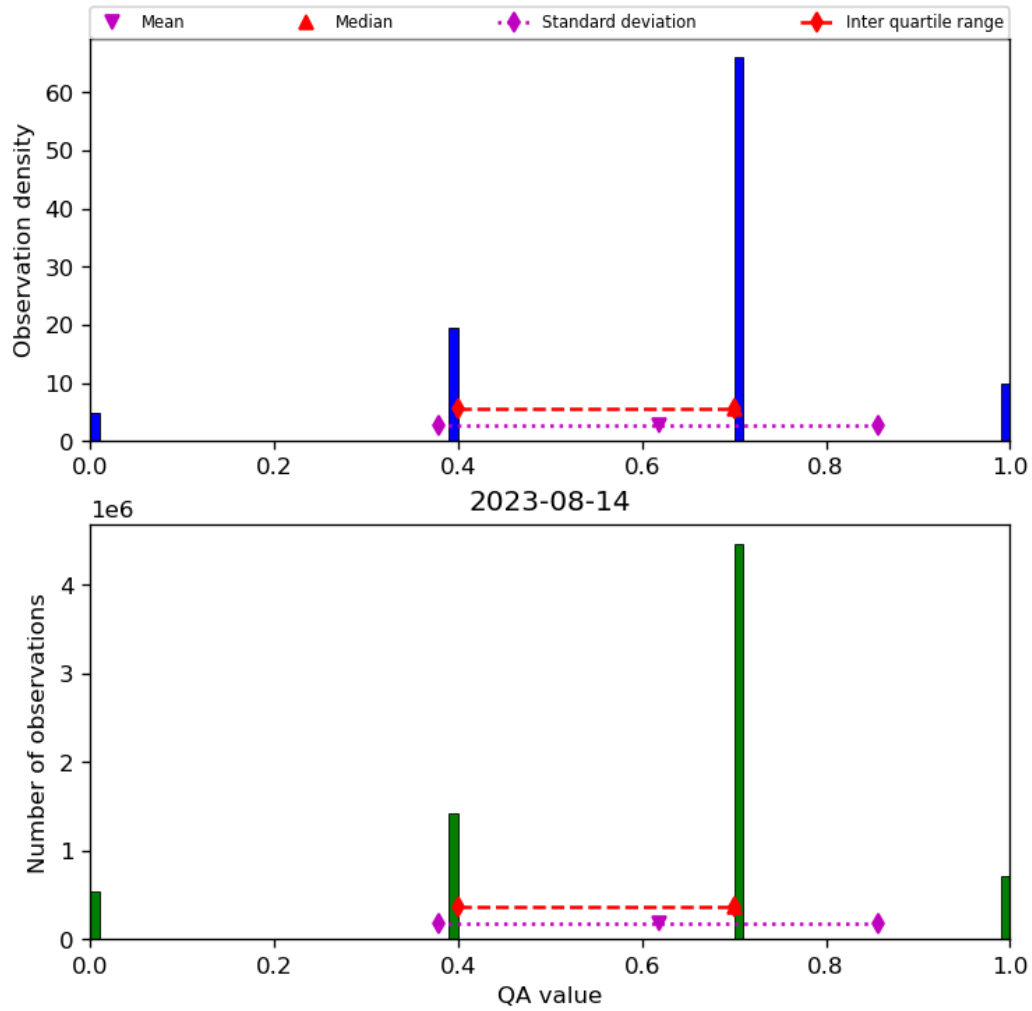
Figure 17: Histogram of “QA value” for 2023-08-14 to 2023-08-15
