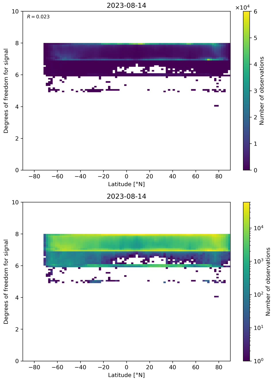
Figure 55: Scatter density plot of “Latitude” against “Degrees of freedom for signal” for 2023-08-14 to 2023-08-15.
