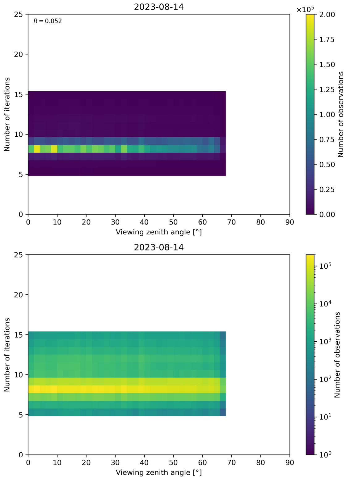
Figure 75: Scatter density plot of “Viewing zenith angle” against “Number of iterations” for 2023-08-14 to 2023-08-15.
