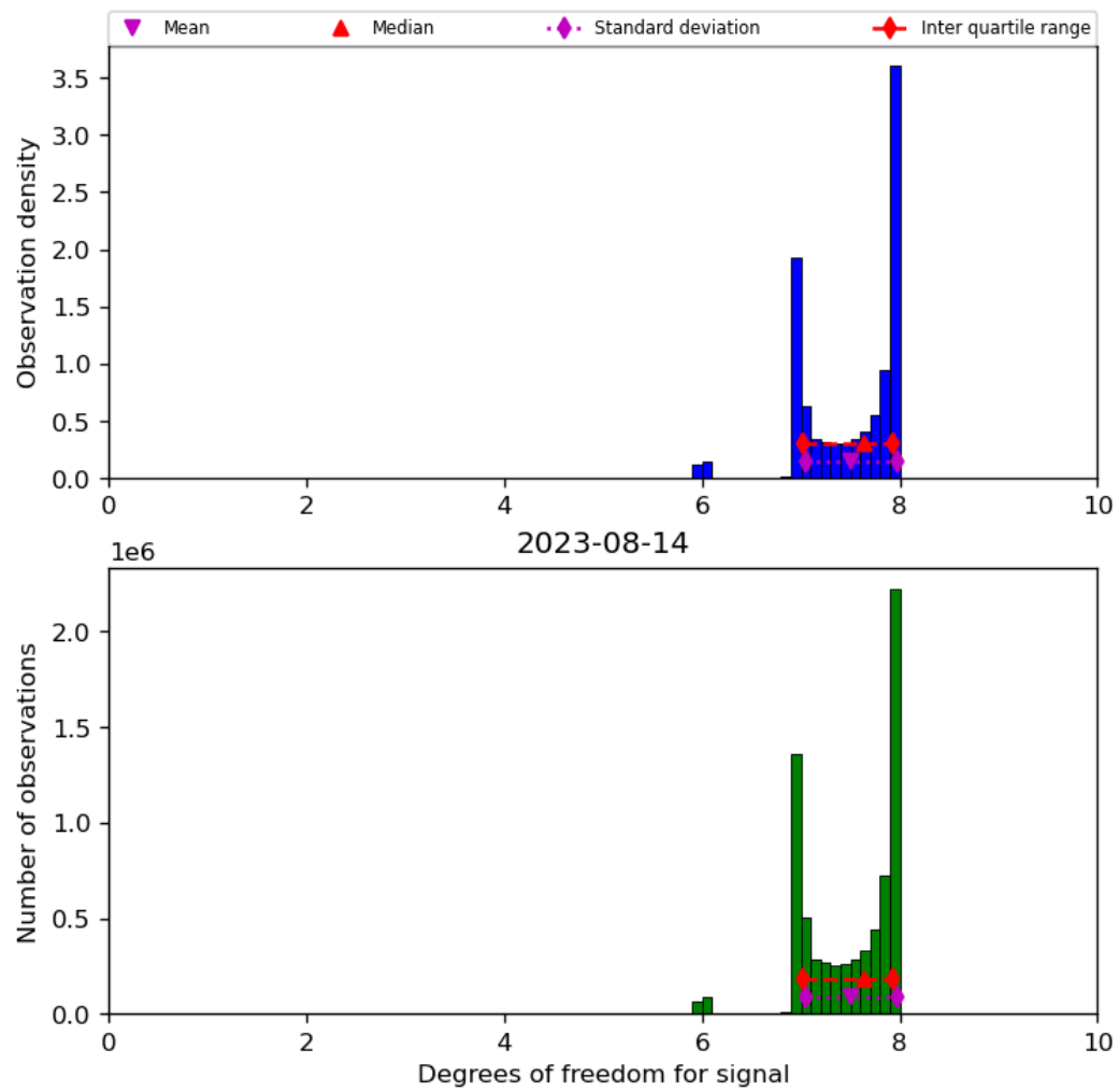
Figure 23: Histogram of “Degrees of freedom for signal” for 2023-08-14 to 2023-08-15
