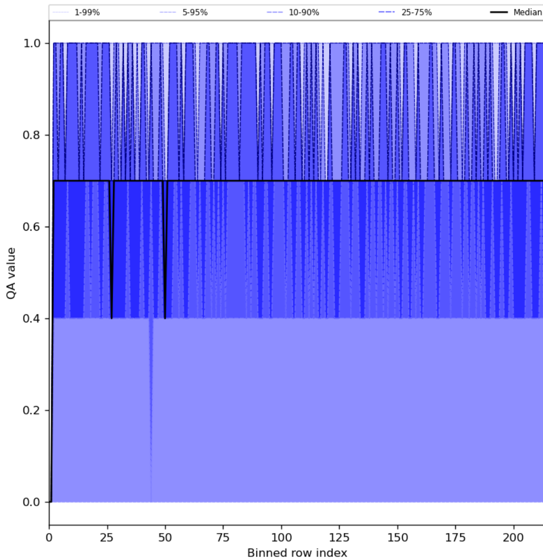
Figure 25: Along track statistics of “QA value” for 2023-08-14 to 2023-08-15
