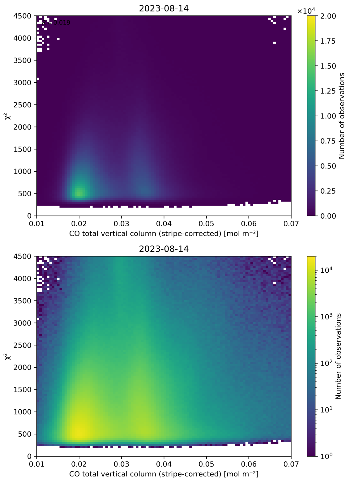
Figure 37: Scatter density plot of “CO total vertical column (stripe-corrected)” against “ \chi^2 ” for 2023-08-14 to 2023-08-15.
