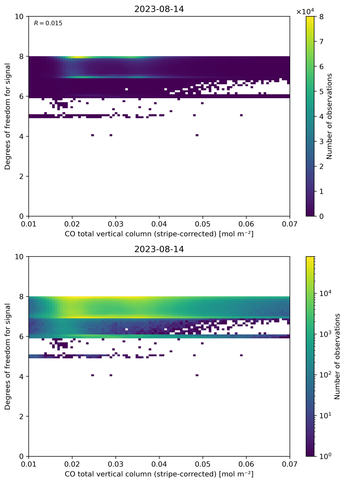
Figure 38: Scatter density plot of “CO total vertical column (stripe-corrected)” against “Degrees of freedom for signal” for 2023-08-14 to 2023-08-15.
