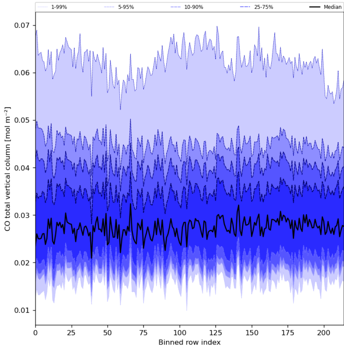
Figure 26: Along track statistics of “CO total vertical column” for 2023-08-14 to 2023-08-15
