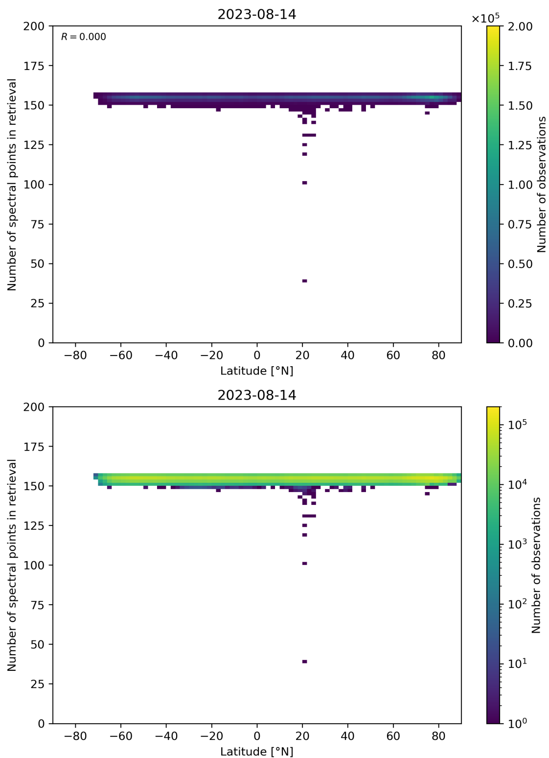
Figure 57: Scatter density plot of “Latitude” against “Number of spectral points in retrieval” for 2023-08-14 to 2023-08-15.
