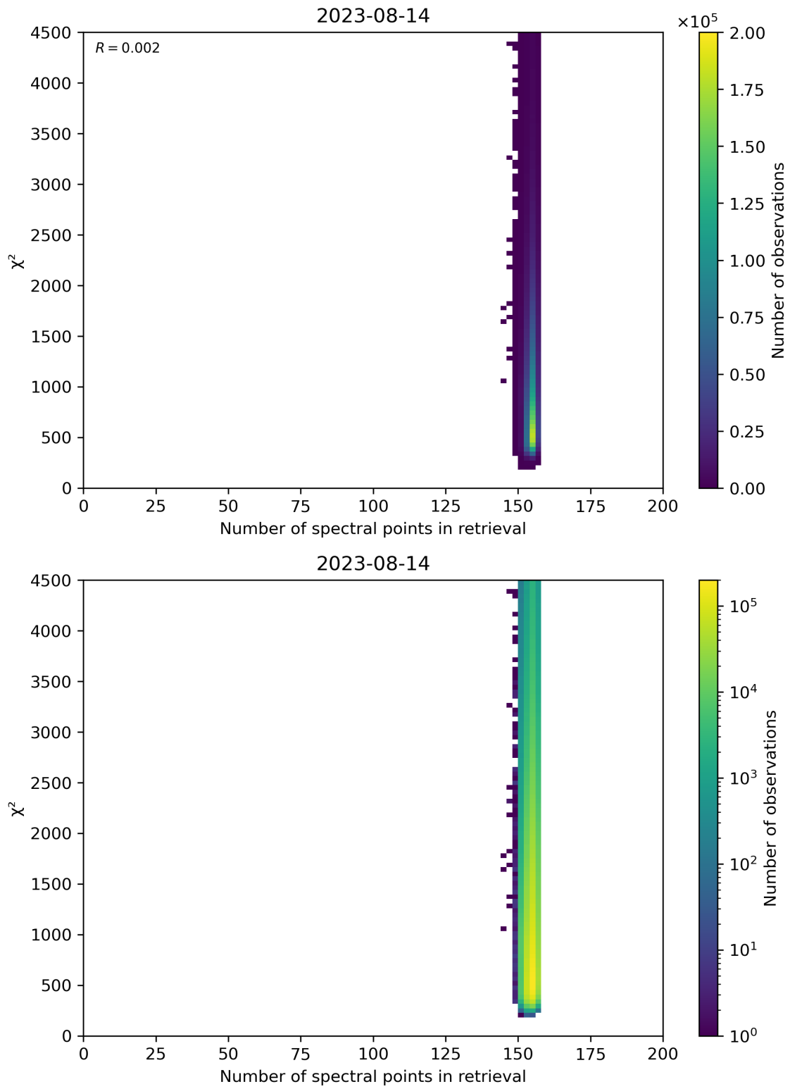
Figure 58: Scatter density plot of “Number of spectral points in retrieval” against “ \chi^2 ” for 2023-08-14 to 2023-08-15.
