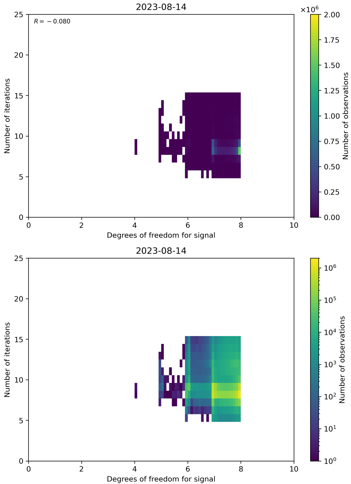
Figure 50: Scatter density plot of “Degrees of freedom for signal” against “Number of iterations” for 2023-08-14 to 2023-08-15.
