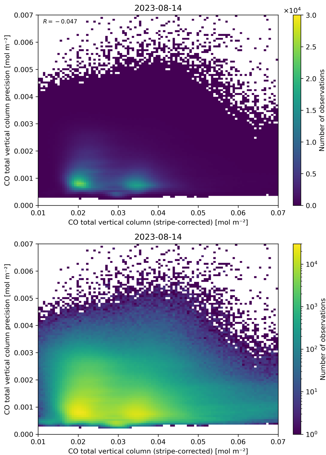
Figure 36: Scatter density plot of “CO total vertical column (stripe-corrected)” against “CO total vertical column precision” for 2023-08-14 to 2023-08-15.
