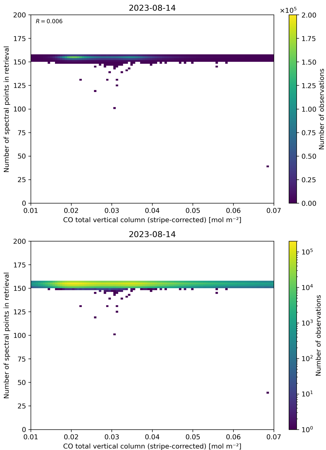
Figure 40: Scatter density plot of “CO total vertical column (stripe-corrected)” against “Number of spectral points in retrieval” for 2023-08-14 to 2023-08-15.
