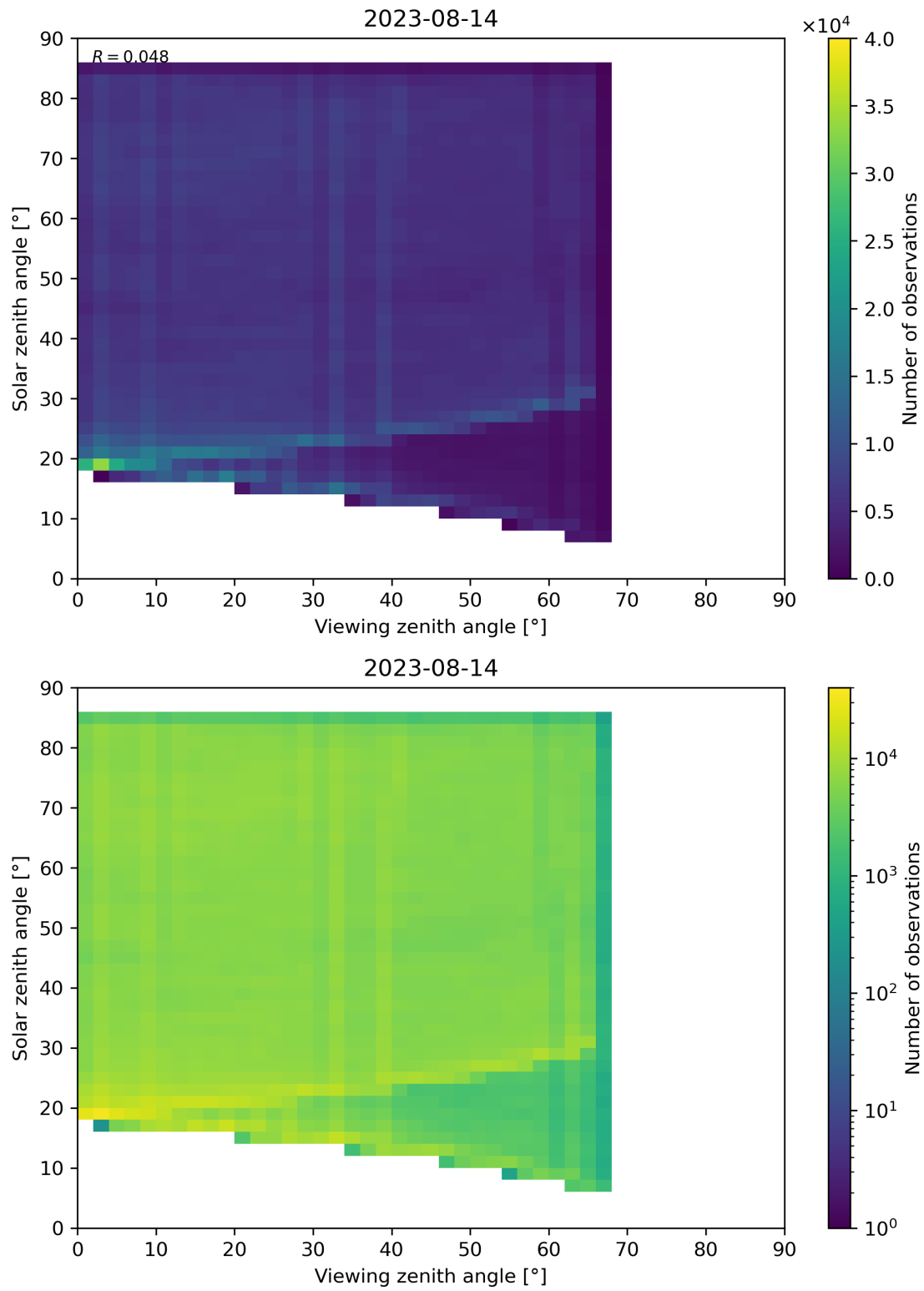
Figure 77: Scatter density plot of “Viewing zenith angle” against “Solar zenith angle” for 2023-08-14 to 2023-08-15.
