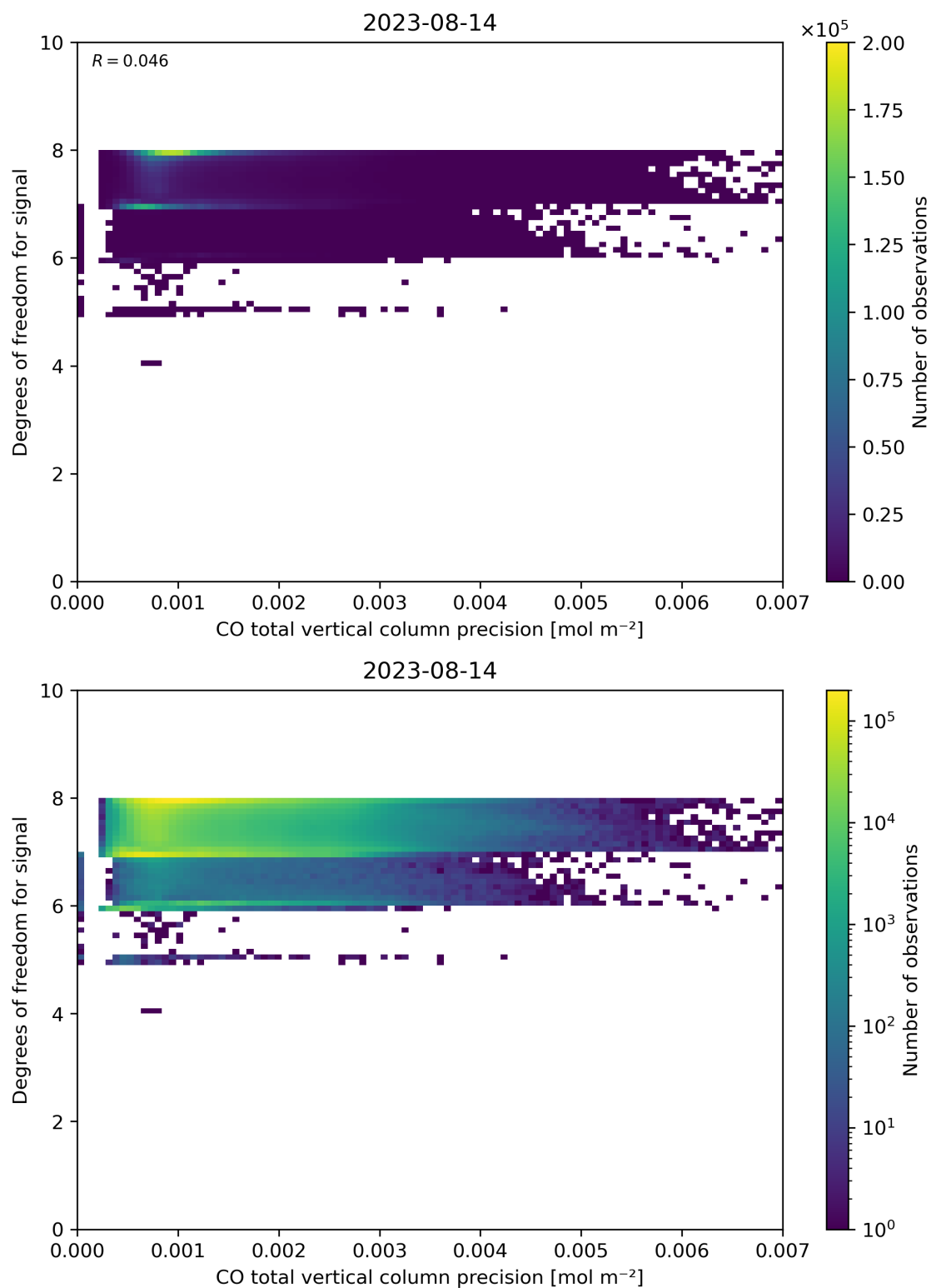
Figure 45: Scatter density plot of “CO total vertical column precision” against “Degrees of freedom for signal” for 2023-08-14 to 2023-08-15.
