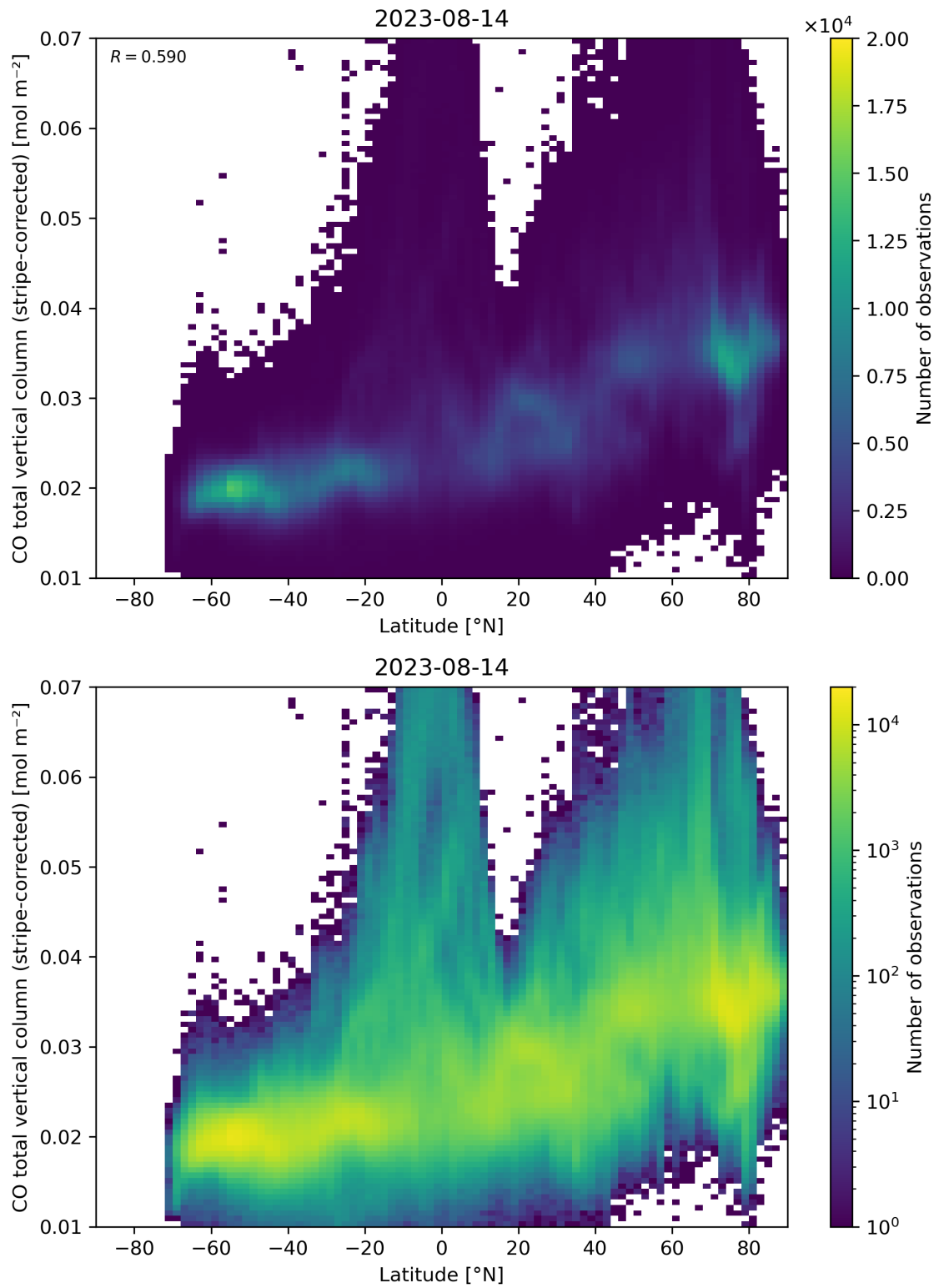
Figure 52: Scatter density plot of “Latitude” against “CO total vertical column (stripe-corrected)” for 2023-08-14 to 2023-08-15.
