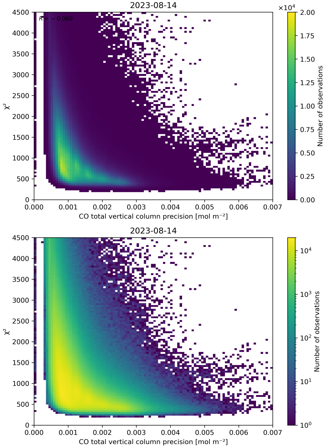
Figure 44: Scatter density plot of “CO total vertical column precision” against “ \chi^2 ” for 2023-08-14 to 2023-08-15.
