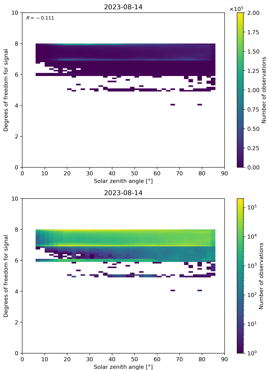
Figure 65: Scatter density plot of “Solar zenith angle” against “Degrees of freedom for signal” for 2023-08-14 to 2023-08-15.
