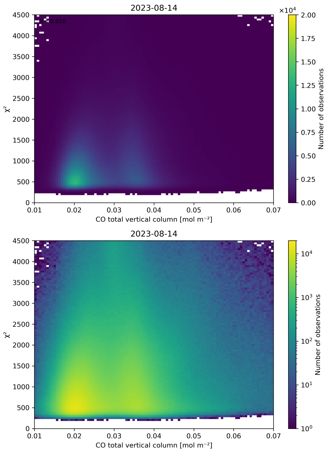
Figure 35: Scatter density plot of “CO total vertical column” against “ \chi^2 ” for 2023-08-14 to 2023-08-15.
