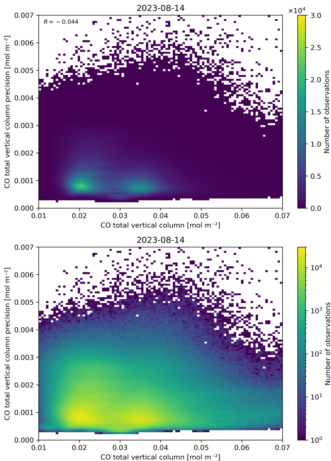
Figure 34: Scatter density plot of “CO total vertical column” against “CO total vertical column precision” for 2023-08-14 to 2023-08-15.
