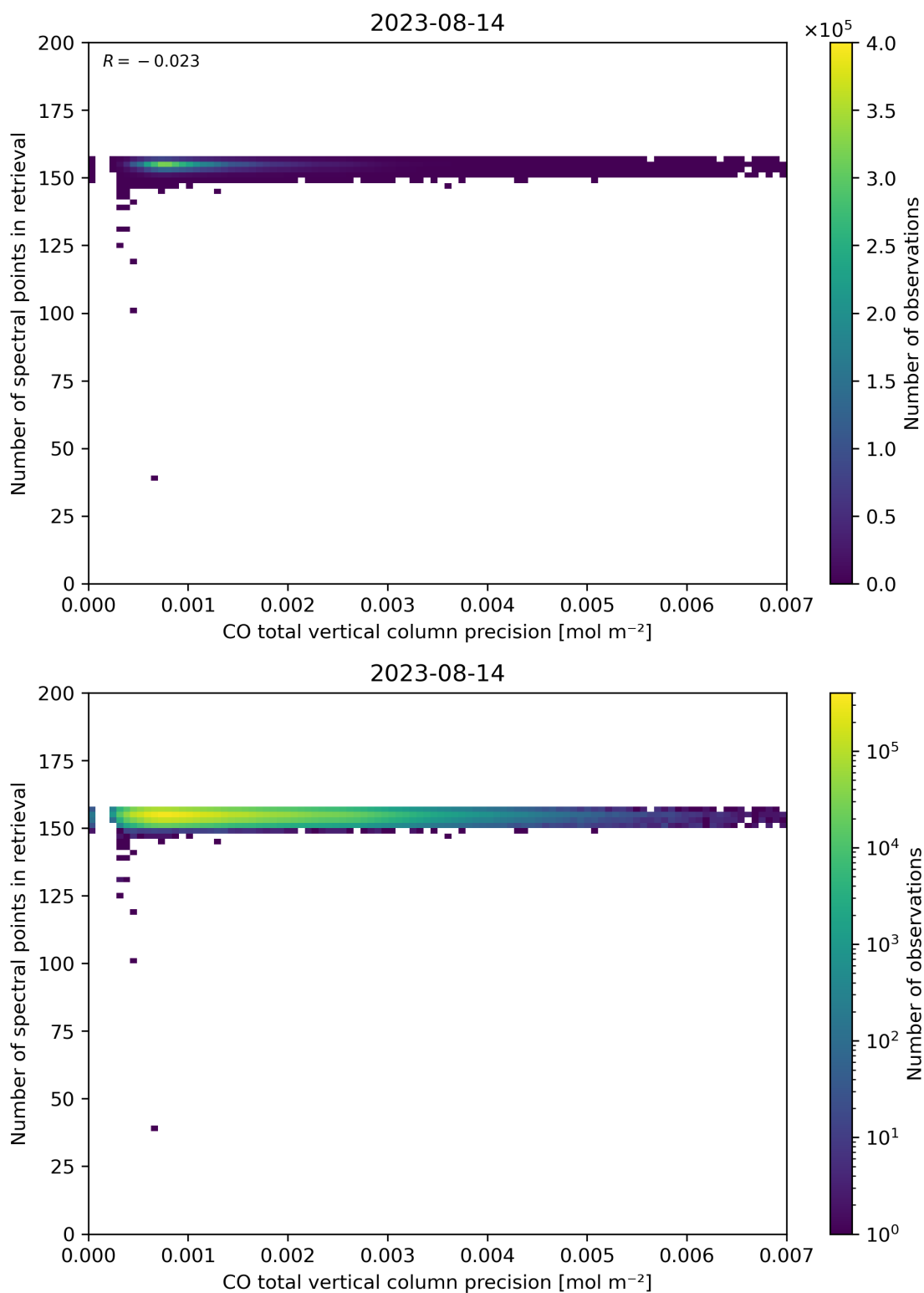
Figure 47: Scatter density plot of “CO total vertical column precision” against “Number of spectral points in retrieval” for 2023-08-14 to 2023-08-15.
