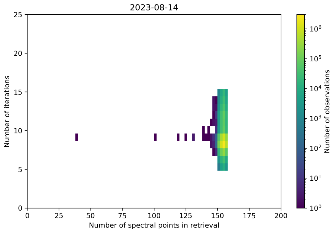
Figure 60: Scatter density plot of “Number of spectral points in retrieval” against “Number of iterations” for 2023-08-14 to 2023-08-15.
