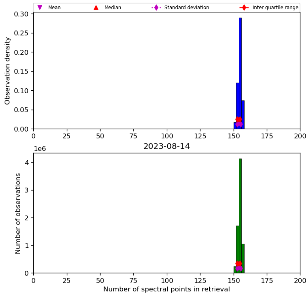
Figure 21: Histogram of “Number of spectral points in retrieval” for 2023-08-14 to 2023-08-15
