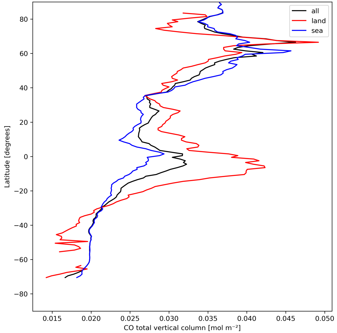
Figure 10: Zonal average of “CO total vertical column” for 2023-08-14 to 2023-08-15.
