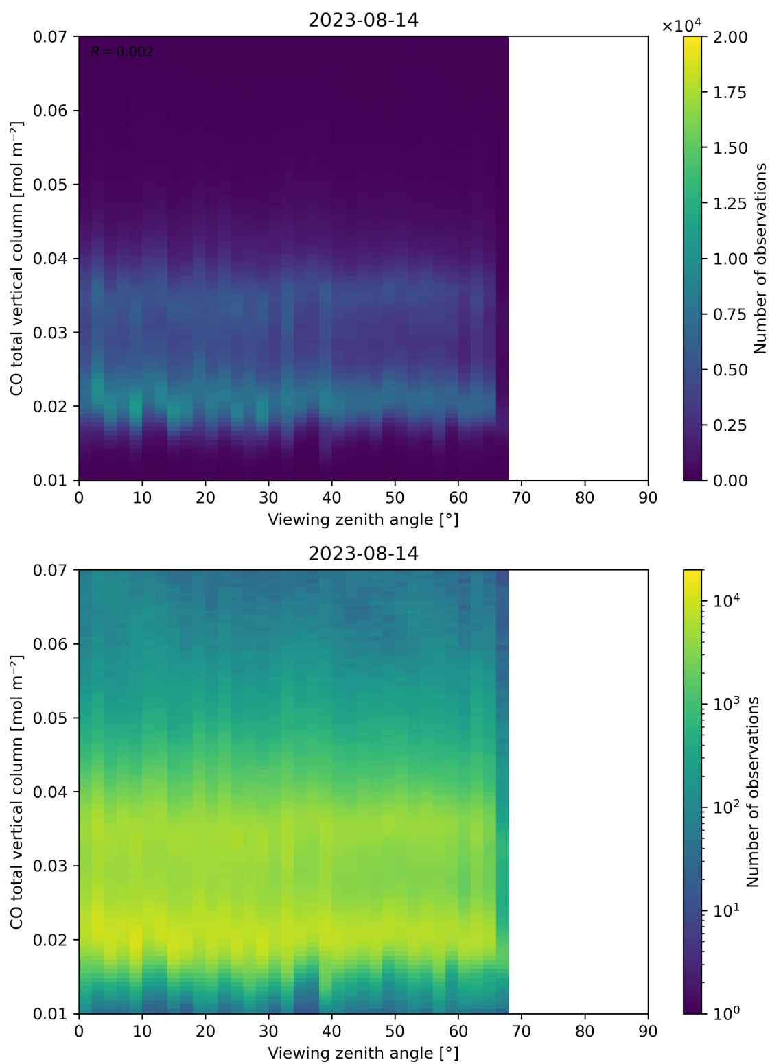
Figure 69: Scatter density plot of “Viewing zenith angle” against “CO total vertical column” for 2023-08-14 to 2023-08-15.
