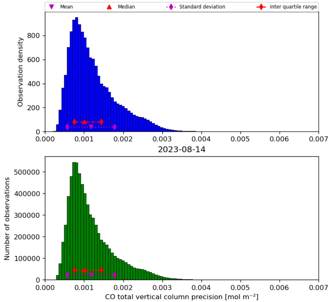
Figure 20: Histogram of “CO total vertical column precision” for 2023-08-14 to 2023-08-15
