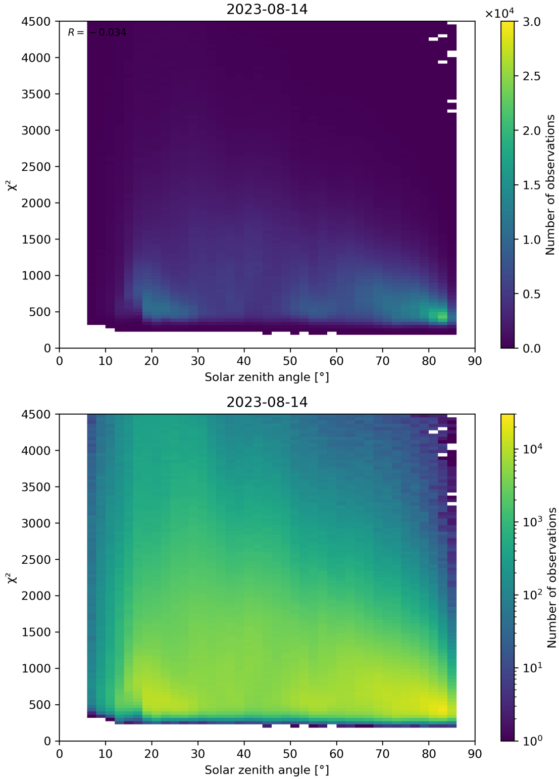
Figure 64: Scatter density plot of “Solar zenith angle” against “ \chi^2 ” for 2023-08-14 to 2023-08-15.
