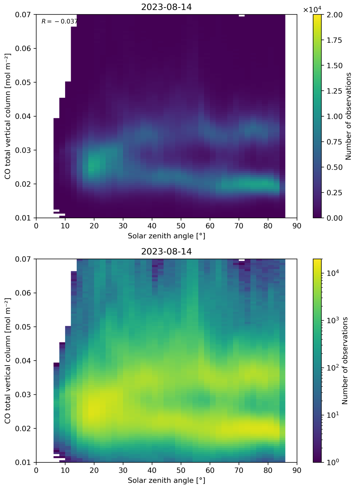
Figure 61: Scatter density plot of “Solar zenith angle” against “CO total vertical column” for 2023-08-14 to 2023-08-15.
