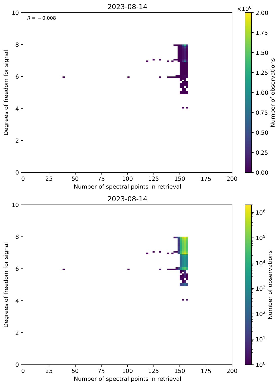
Figure 59: Scatter density plot of “Number of spectral points in retrieval” against “Degrees of freedom for signal” for 2023-08-14 to 2023-08-15.
