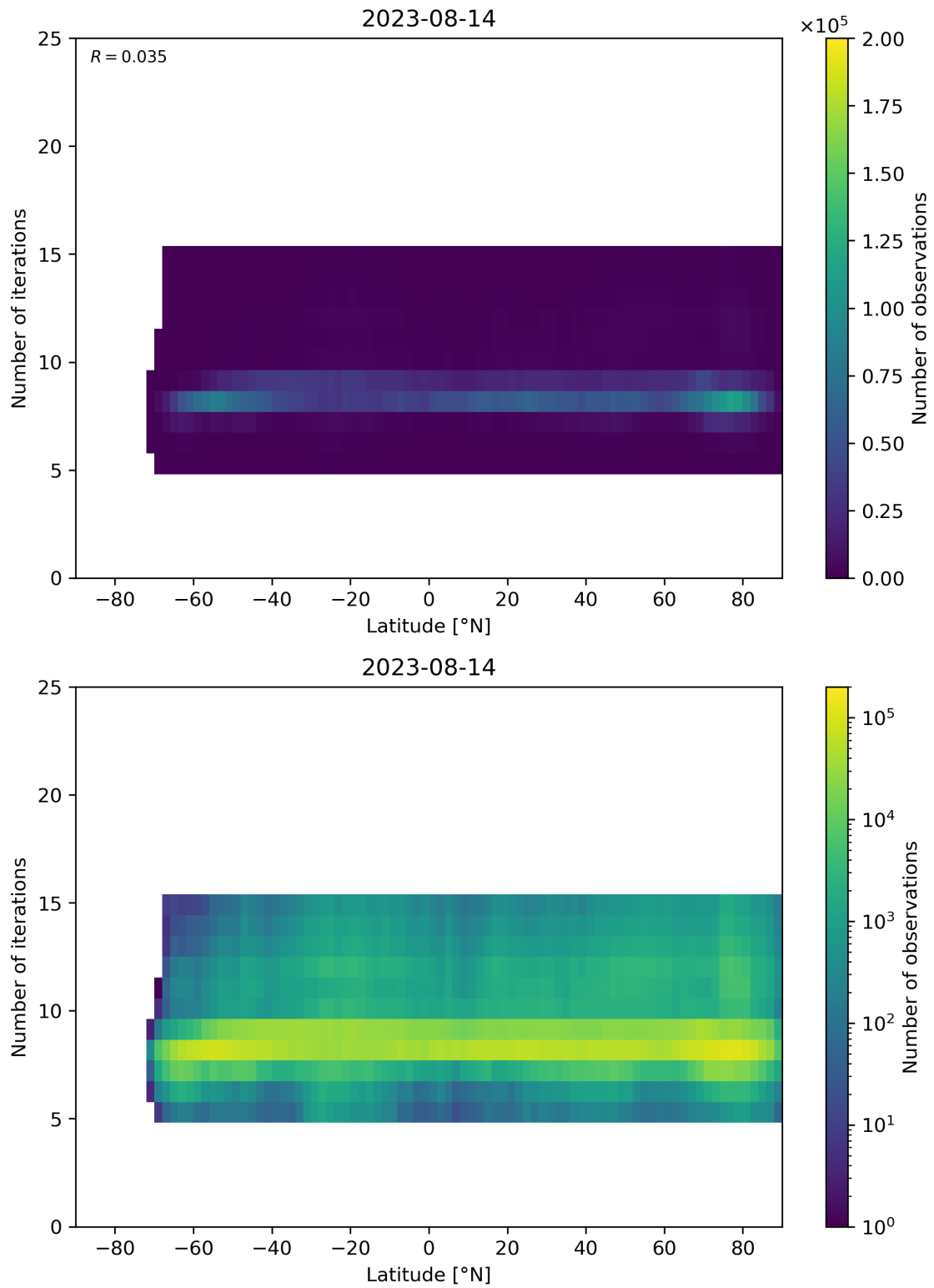
Figure 56: Scatter density plot of “Latitude” against “Number of iterations” for 2023-08-14 to 2023-08-15.
