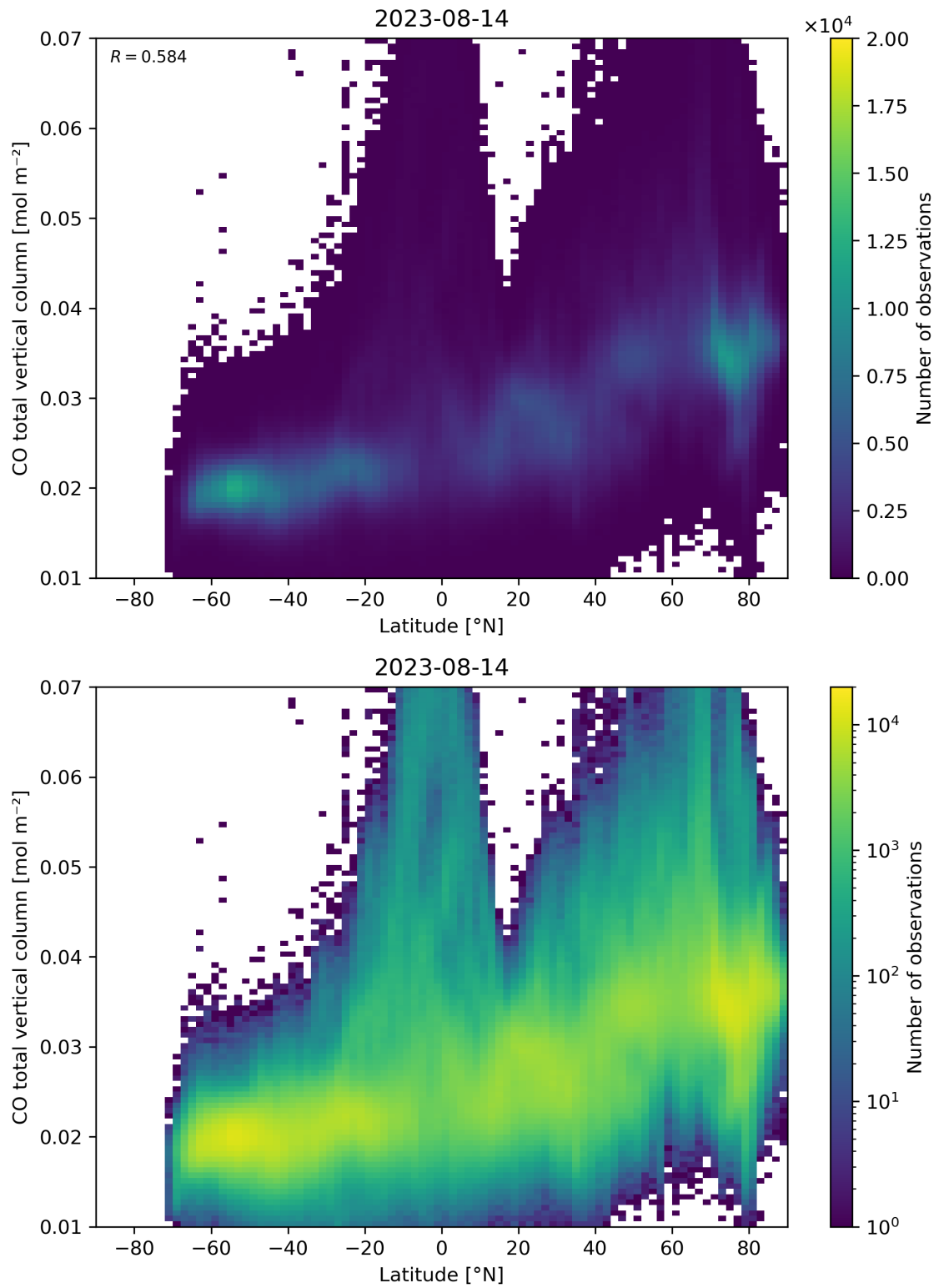
Figure 51: Scatter density plot of “Latitude” against “CO total vertical column” for 2023-08-14 to 2023-08-15.
