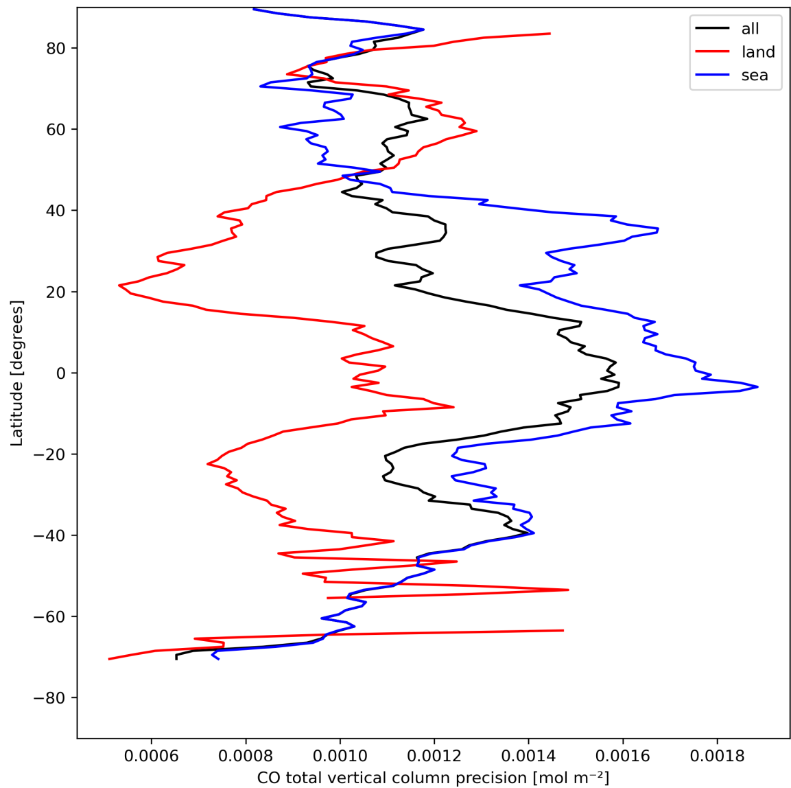
Figure 12: Zonal average of “CO total vertical column precision” for 2023-08-14 to 2023-08-15.
