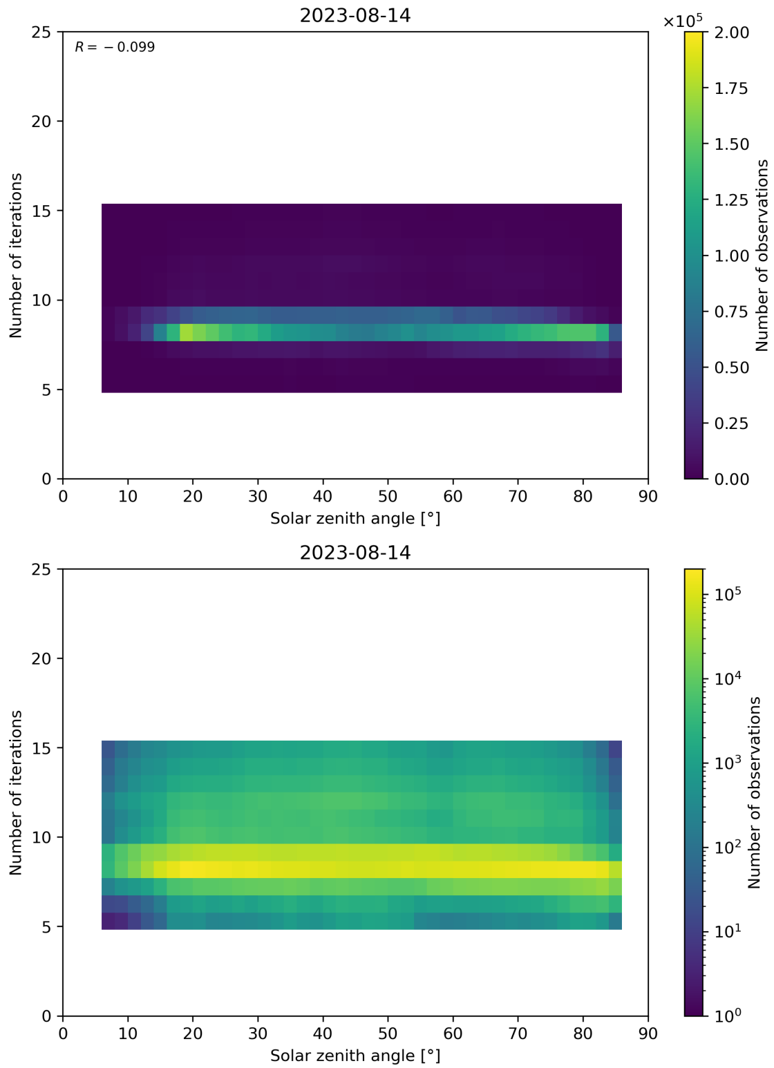
Figure 67: Scatter density plot of “Solar zenith angle” against “Number of iterations” for 2023-08-14 to 2023-08-15.
