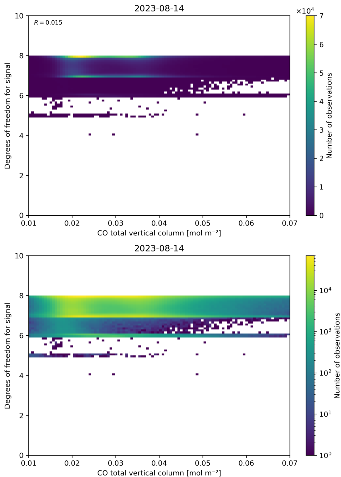
Figure 41: Scatter density plot of “CO total vertical column” against “Degrees of freedom for signal” for 2023-08-14 to 2023-08-15.
