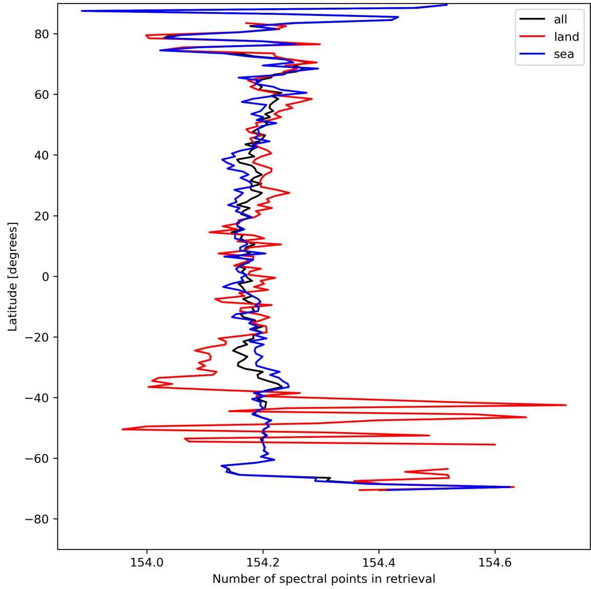
Figure 13: Zonal average of “Number of spectral points in retrieval” for 2023-08-14 to 2023-08-15.
