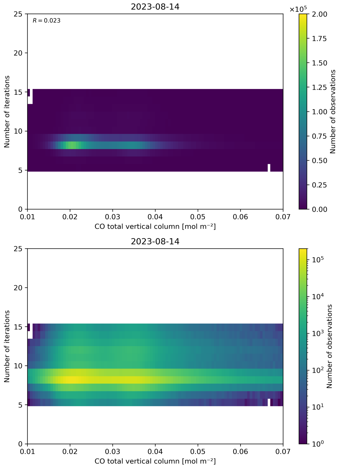
Figure 42: Scatter density plot of “CO total vertical column” against “Number of iterations” for 2023-08-14 to 2023-08-15.
