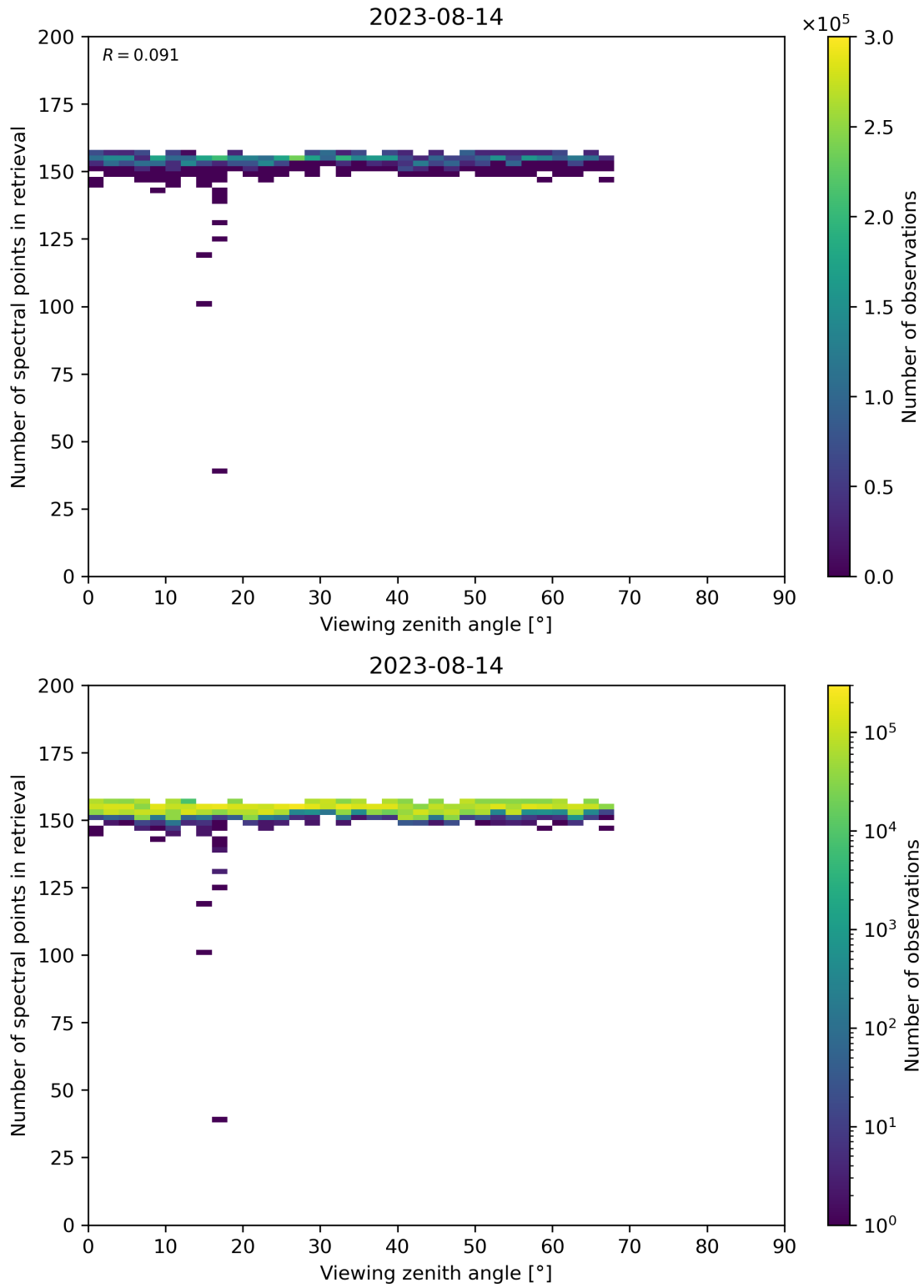
Figure 76: Scatter density plot of “Viewing zenith angle” against “Number of spectral points in retrieval” for 2023-08-14 to 2023-08-15.
