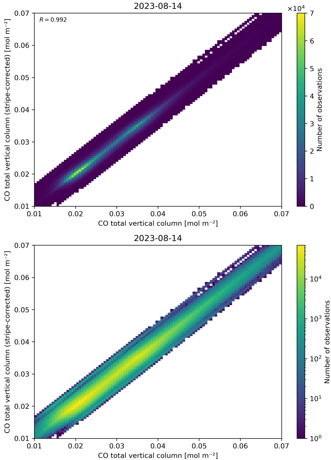
Figure 33: Scatter density plot of “CO total vertical column” against “CO total vertical column (stripe-corrected)” for 2023-08-14 to 2023-08-15.
