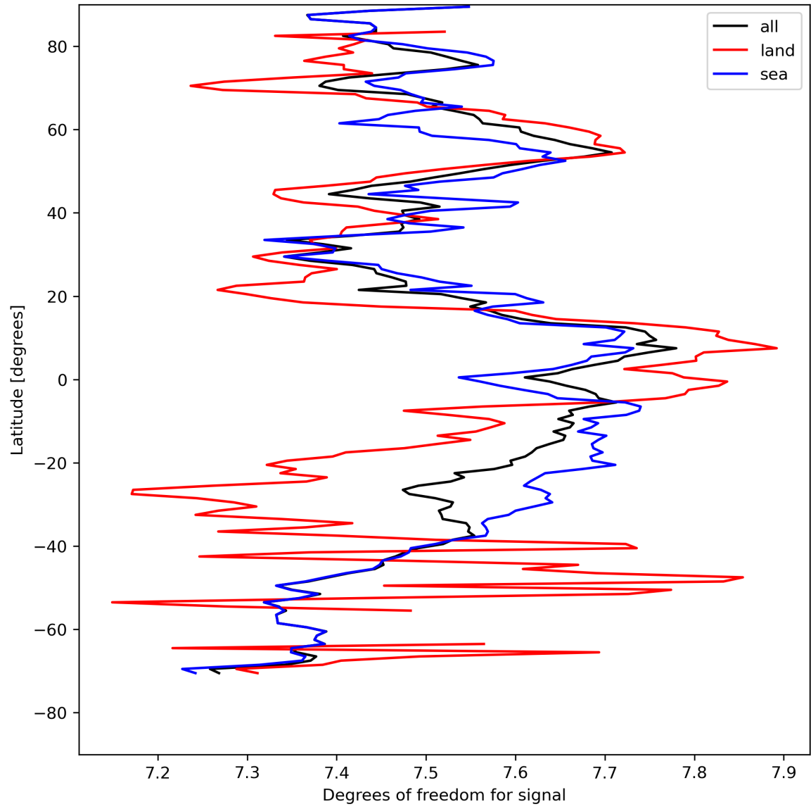
Figure 15: Zonal average of “Degrees of freedom for signal” for 2023-08-14 to 2023-08-15.
