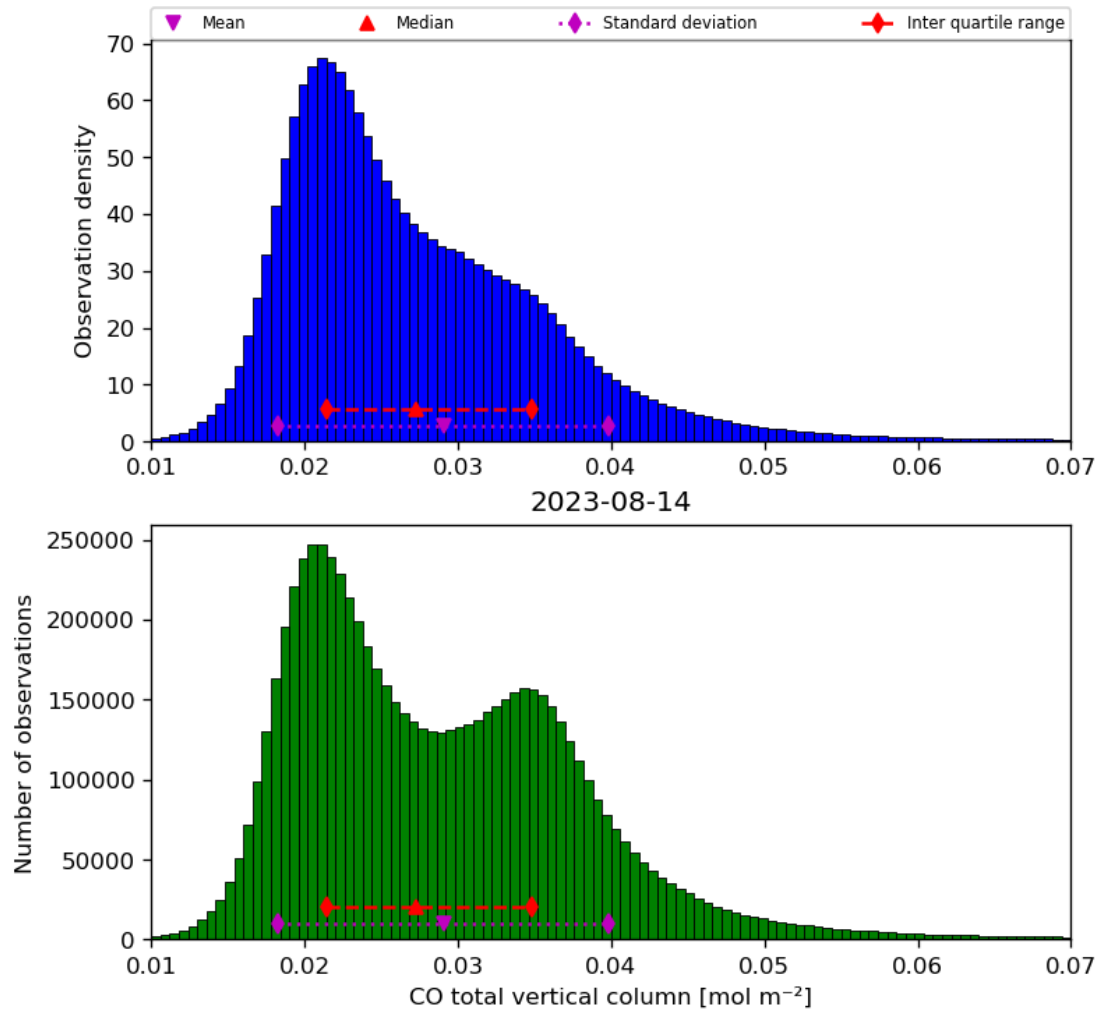
Figure 18: Histogram of “CO total vertical column” for 2023-08-14 to 2023-08-15
