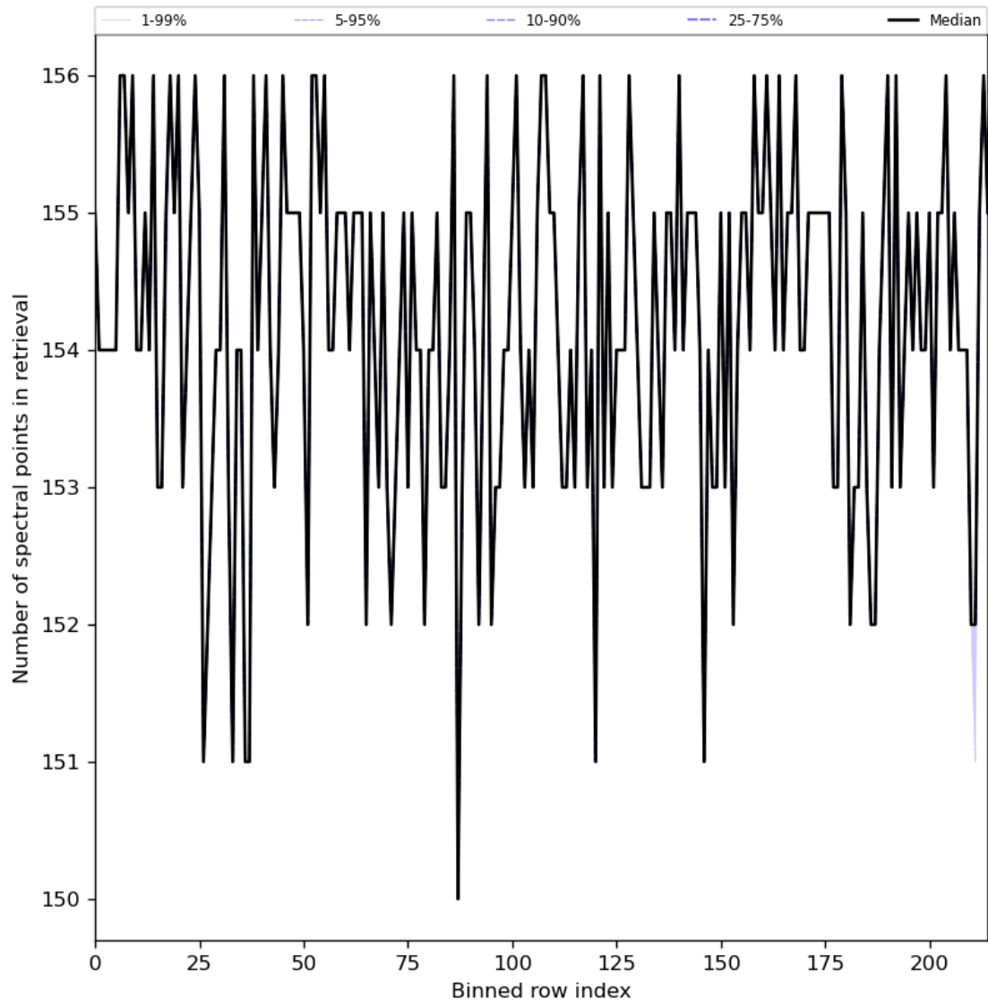
Figure 29: Along track statistics of “Number of spectral points in retrieval” for 2023-08-14 to 2023-08-15
