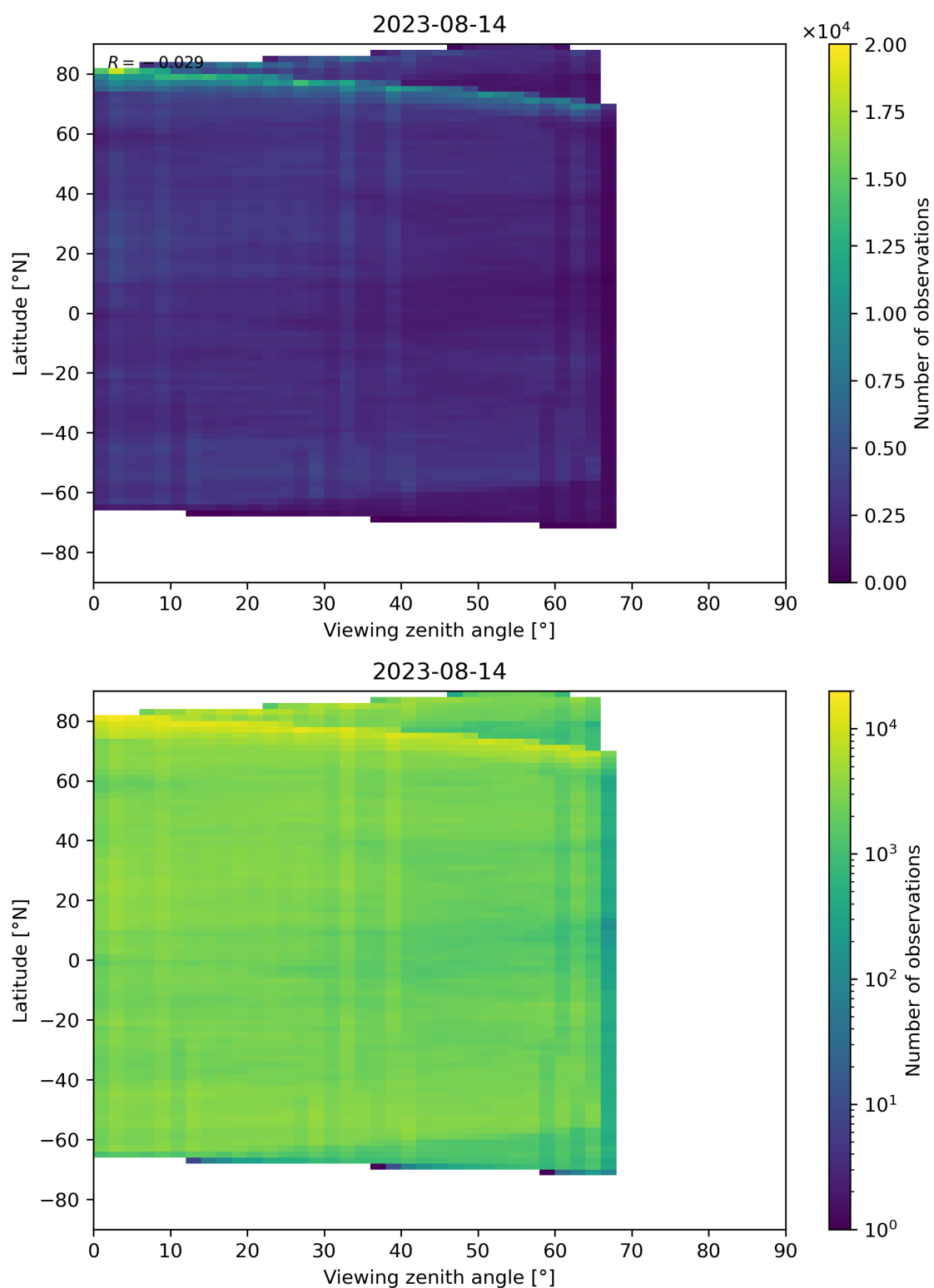
Figure 74: Scatter density plot of “Viewing zenith angle” against “Latitude” for 2023-08-14 to 2023-08-15.
