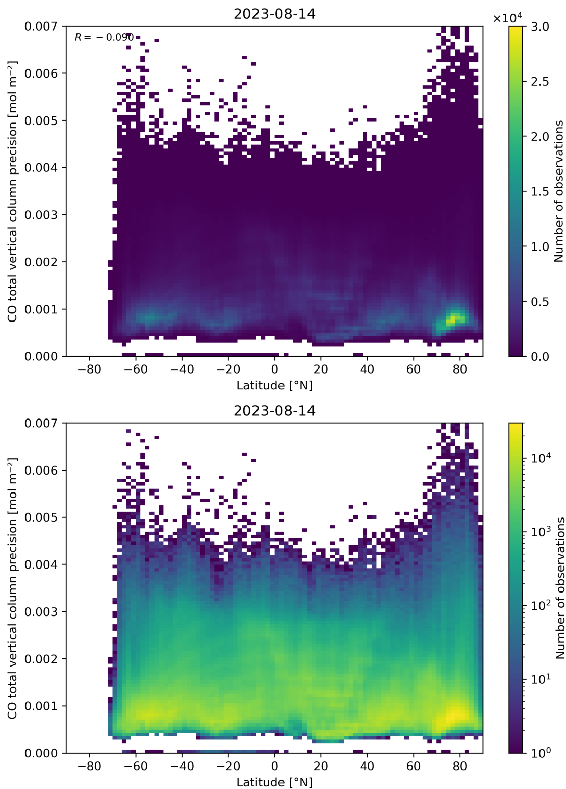
Figure 53: Scatter density plot of “Latitude” against “CO total vertical column precision” for 2023-08-14 to 2023-08-15.
