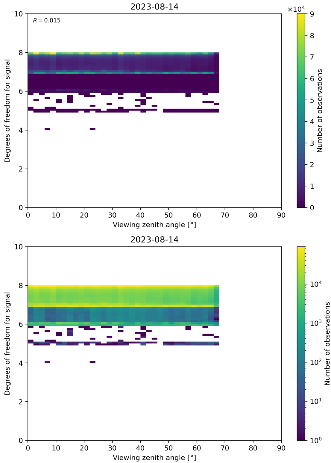
Figure 73: Scatter density plot of “Viewing zenith angle” against “Degrees of freedom for signal” for 2023-08-14 to 2023-08-15.
