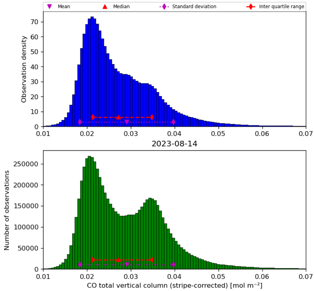
Figure 19: Histogram of “CO total vertical column (stripe-corrected)” for 2023-08-14 to 2023-08-15
