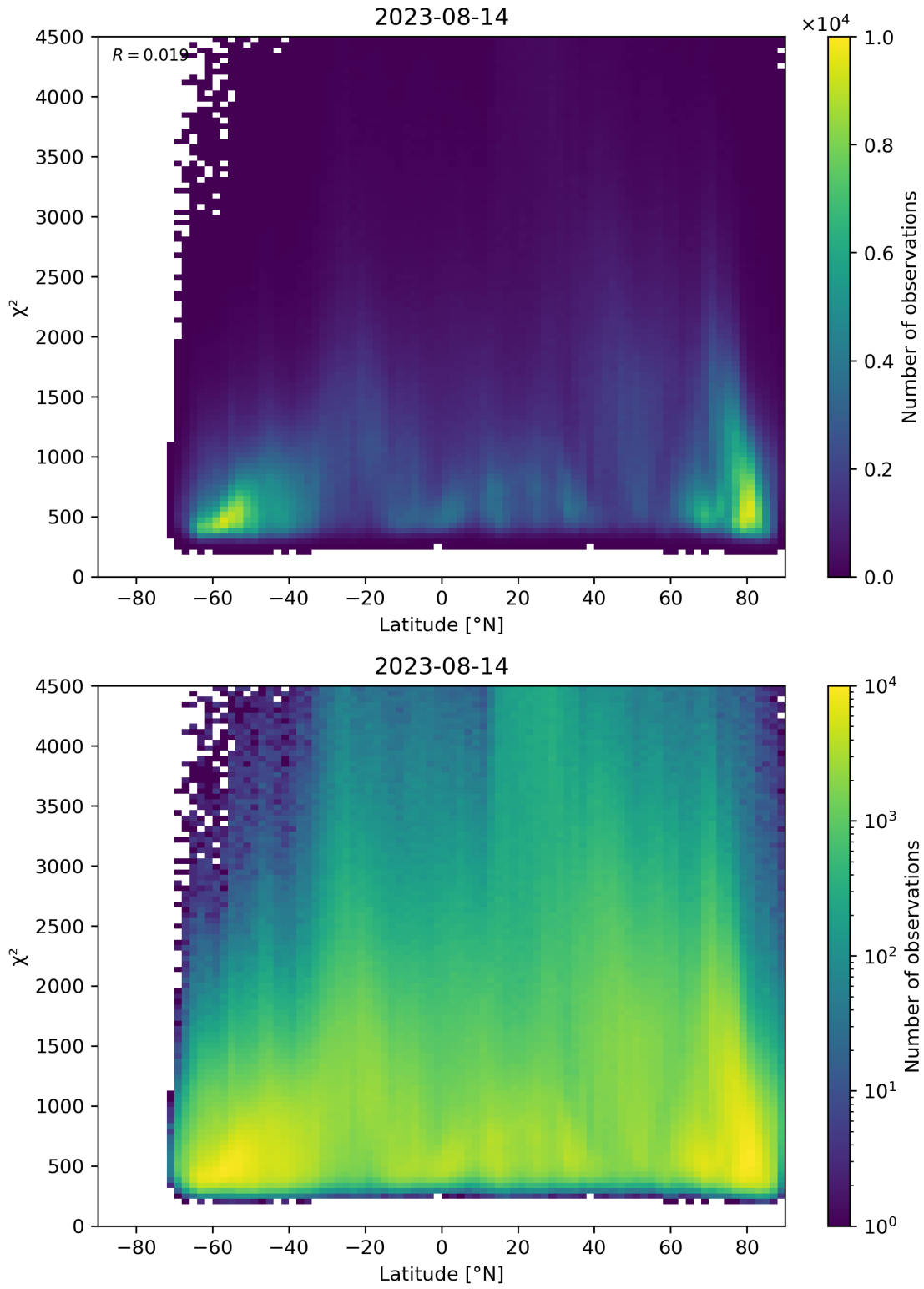
Figure 54: Scatter density plot of “Latitude” against “ \chi^2 ” for 2023-08-14 to 2023-08-15.
