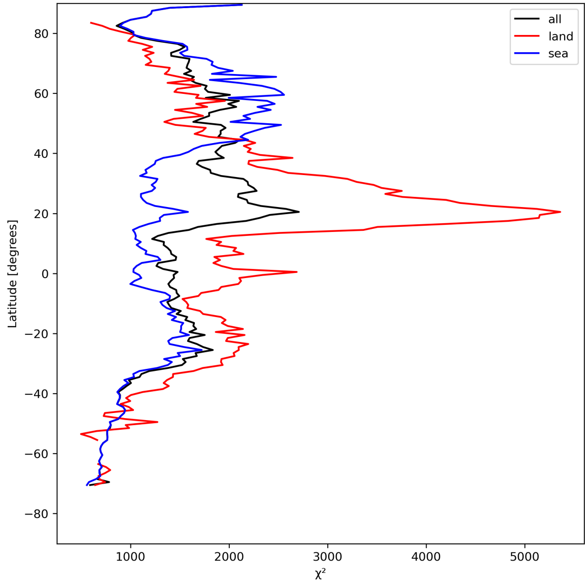
Figure 14: Zonal average of “ \chi^2 ” for 2023-08-14 to 2023-08-15.
