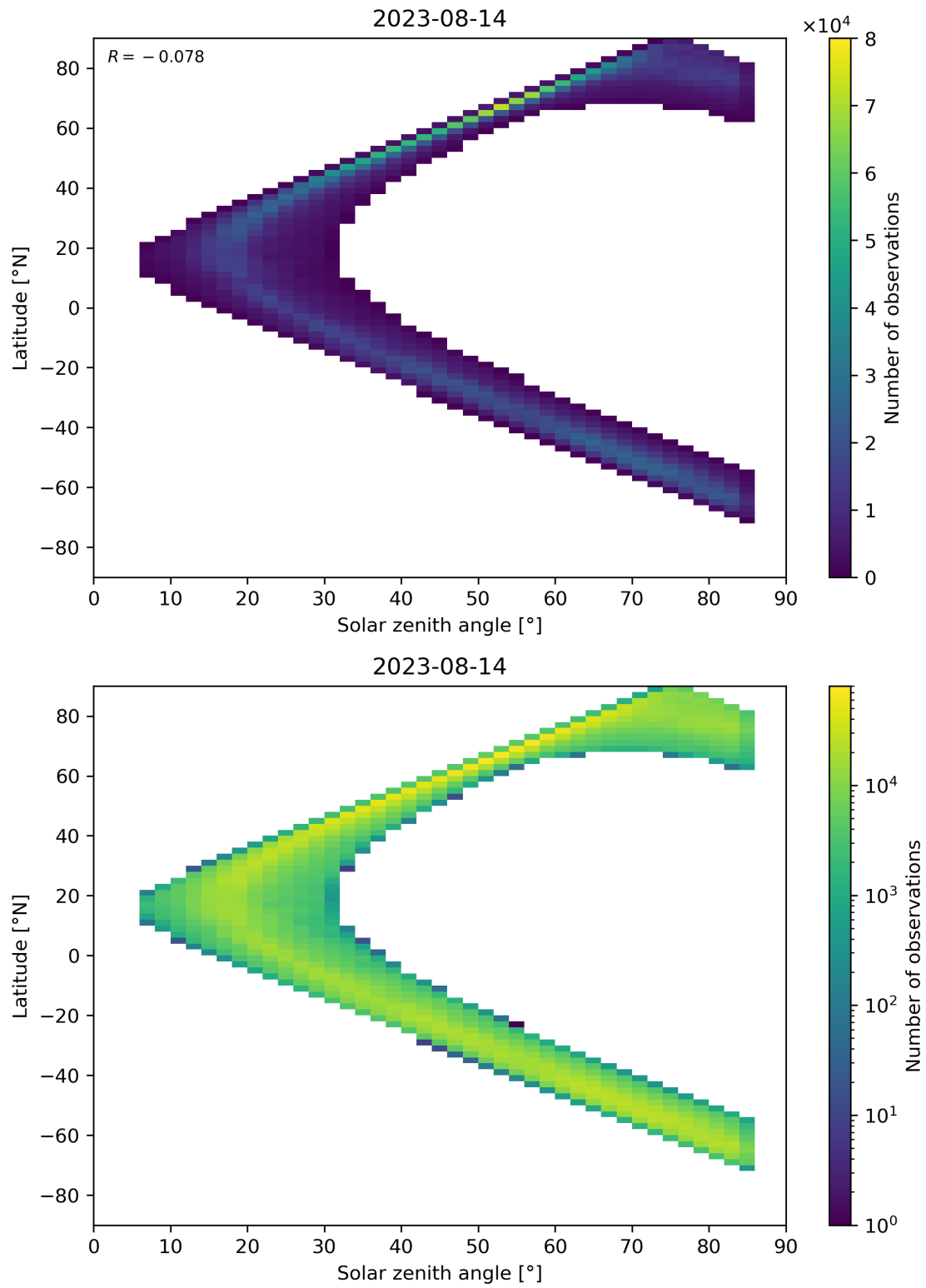
Figure 66: Scatter density plot of “Solar zenith angle” against “Latitude” for 2023-08-14 to 2023-08-15.
