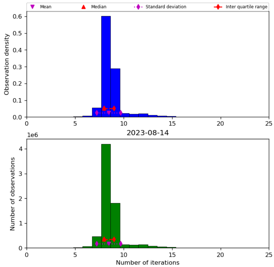
Figure 24: Histogram of “Number of iterations” for 2023-08-14 to 2023-08-15
