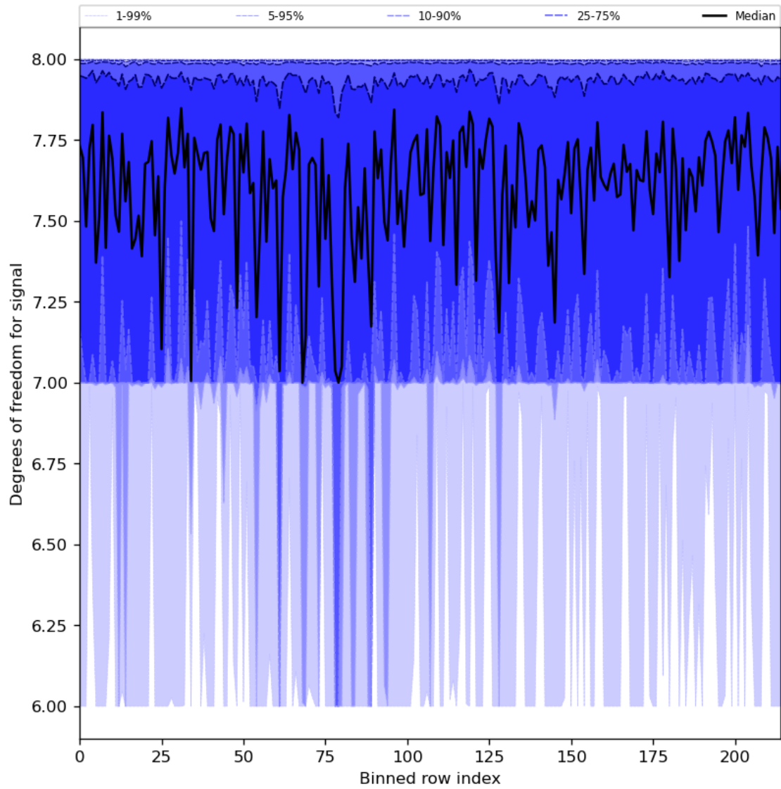
Figure 31: Along track statistics of “Degrees of freedom for signal” for 2023-08-14 to 2023-08-15
