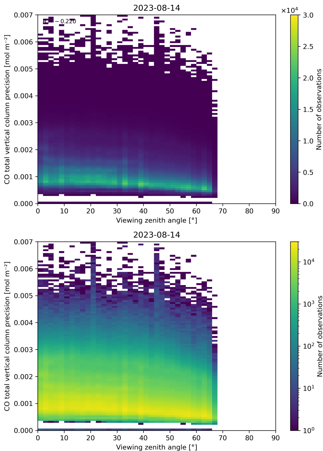
Figure 71: Scatter density plot of “Viewing zenith angle” against “CO total vertical column precision” for 2023-08-14 to 2023-08-15.
