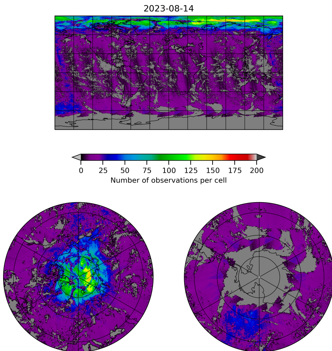
Figure 8: Map of the number of observations for 2023-08-14 to 2023-08-15
