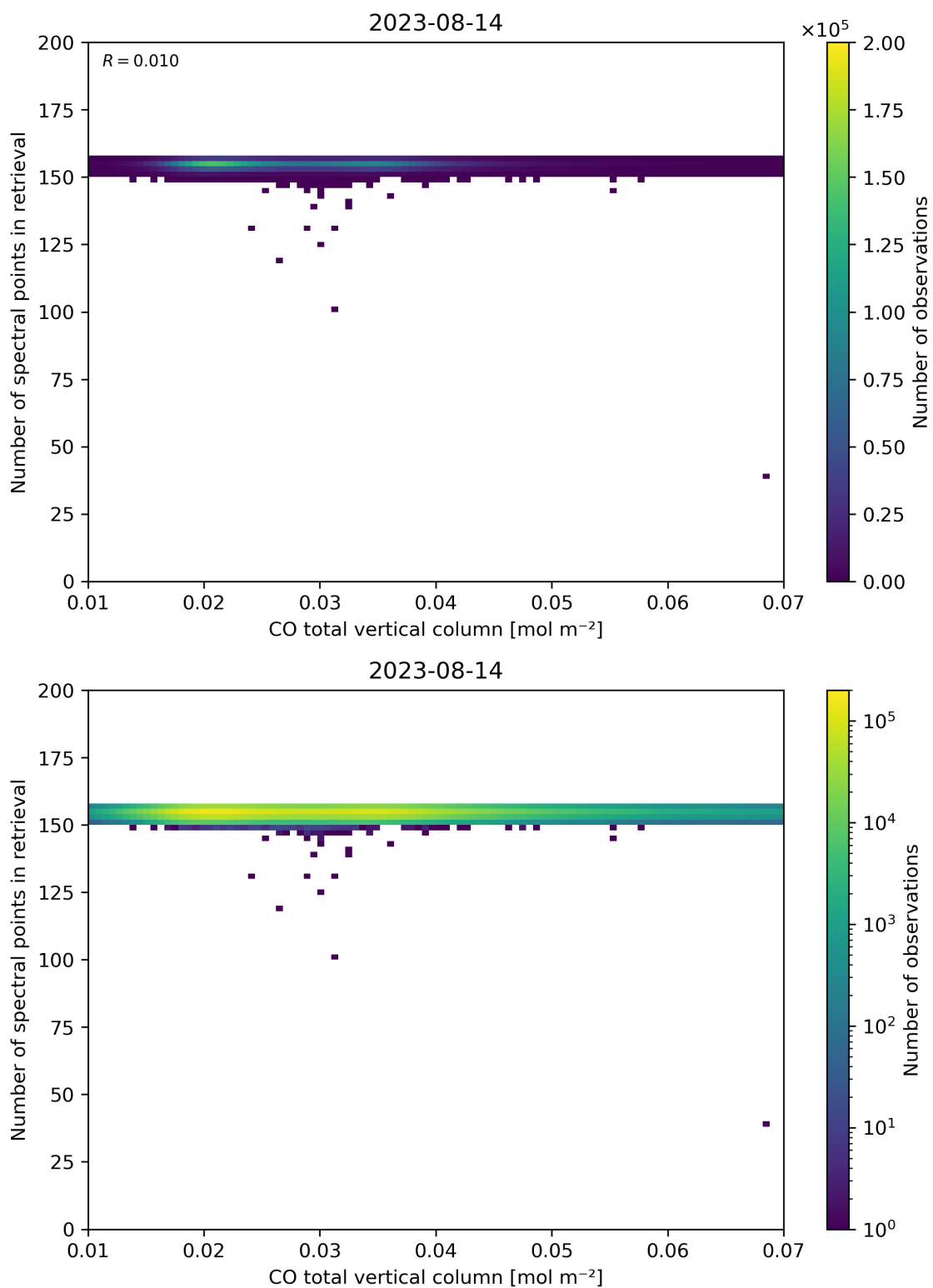
Figure 43: Scatter density plot of “CO total vertical column” against “Number of spectral points in retrieval” for 2023-08-14 to 2023-08-15.
