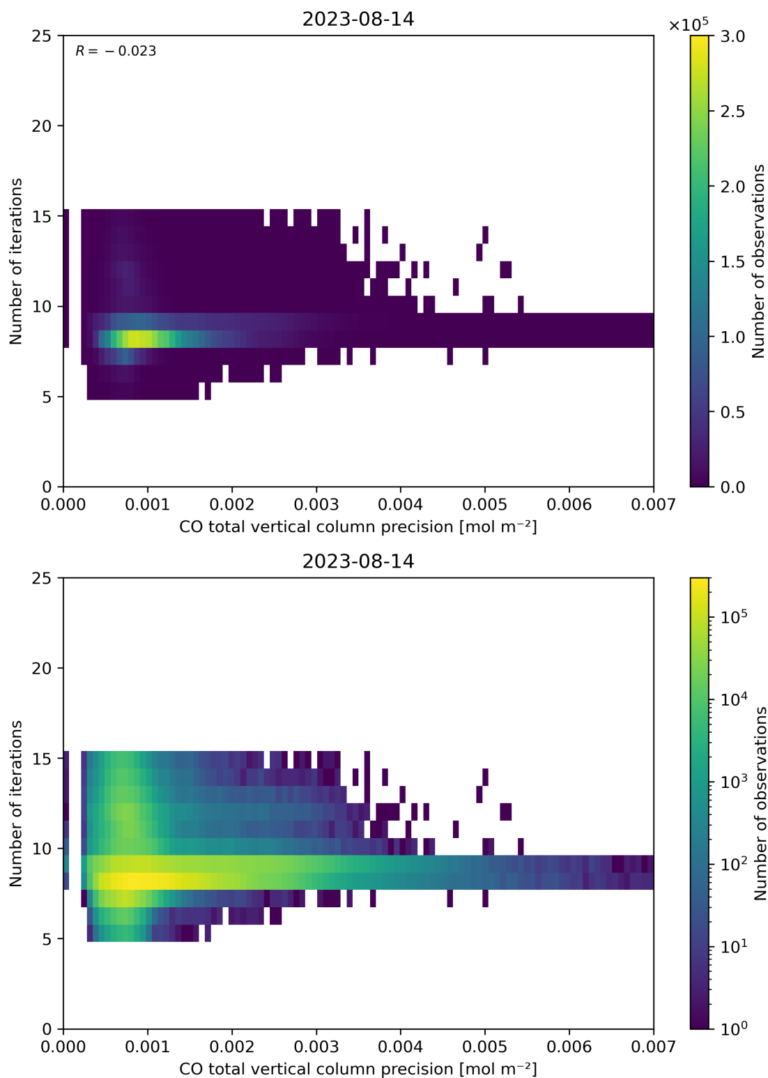
Figure 46: Scatter density plot of “CO total vertical column precision” against “Number of iterations” for 2023-08-14 to 2023-08-15.
