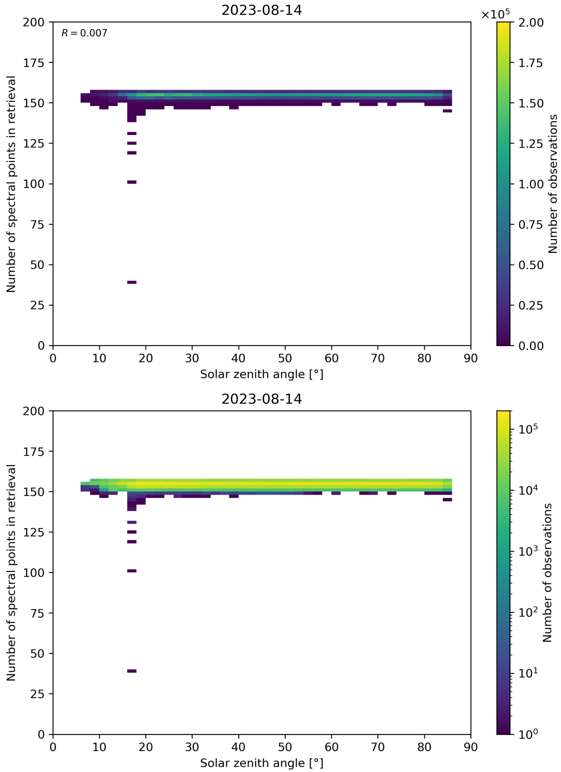
Figure 68: Scatter density plot of “Solar zenith angle” against “Number of spectral points in retrieval” for 2023-08-14 to 2023-08-15.
