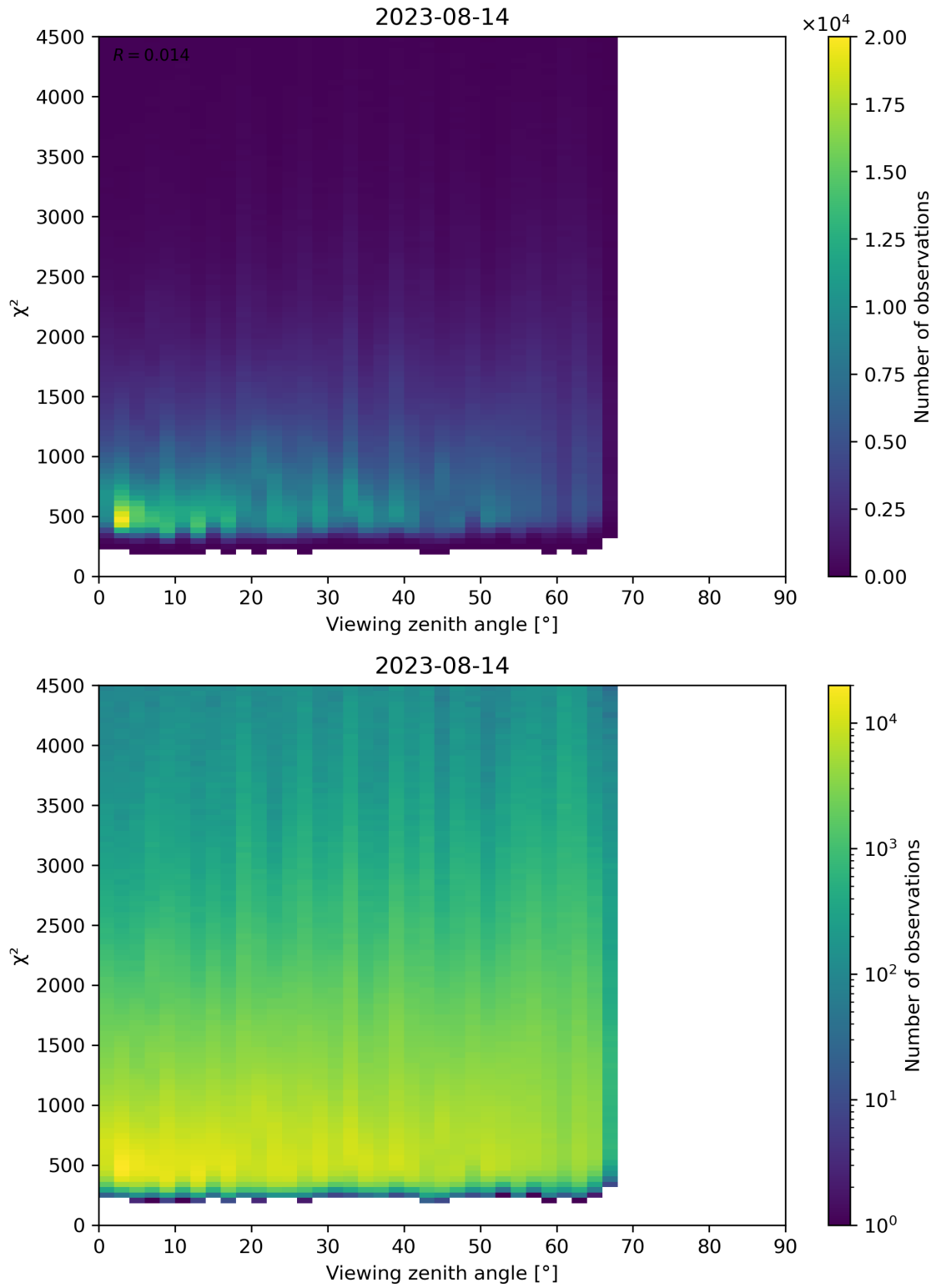
Figure 72: Scatter density plot of “Viewing zenith angle” against “ \chi^2 ” for 2023-08-14 to 2023-08-15.
