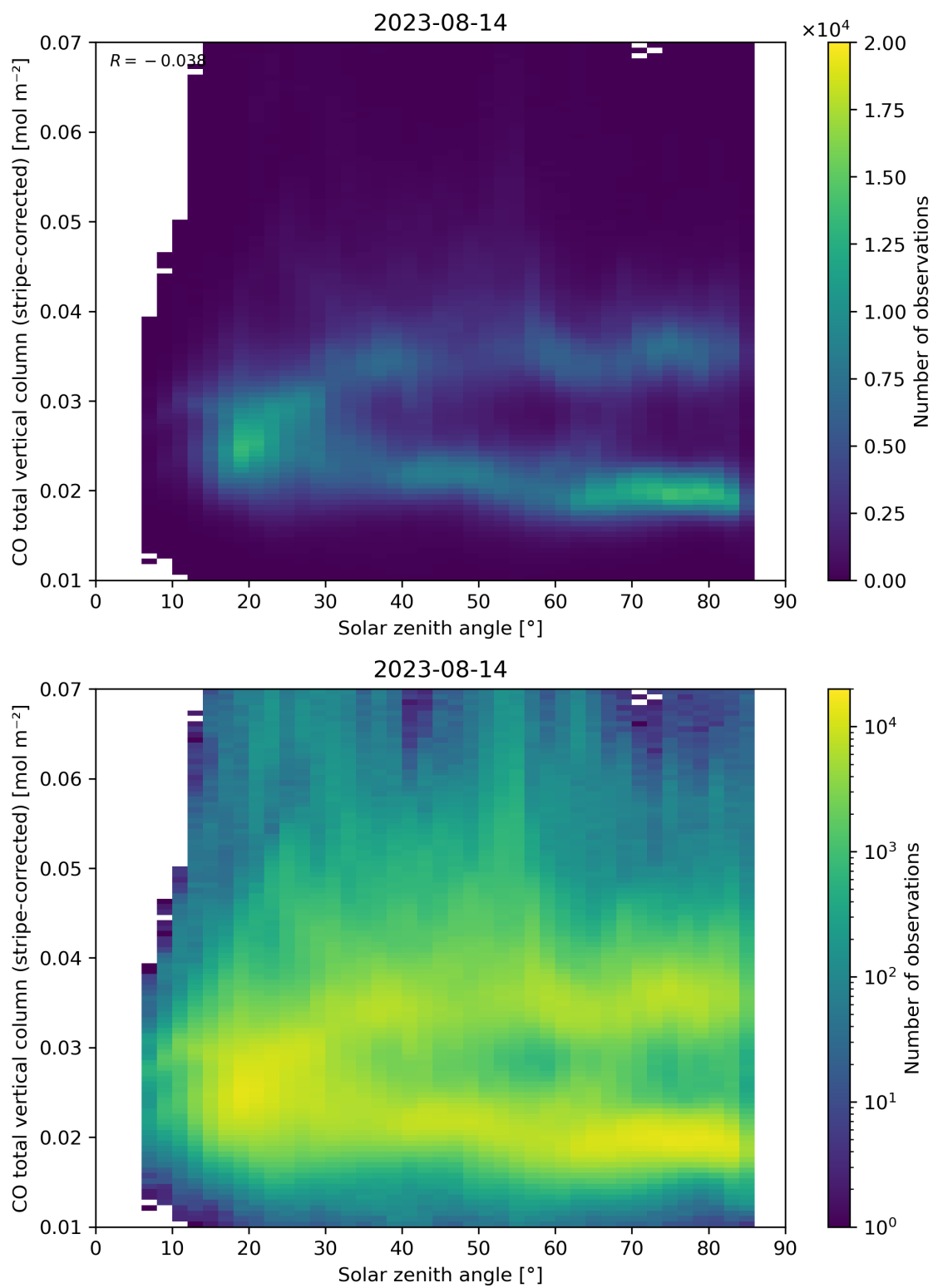
Figure 62: Scatter density plot of “Solar zenith angle” against “CO total vertical column (stripe-corrected)” for 2023-08-14 to 2023-08-15.
