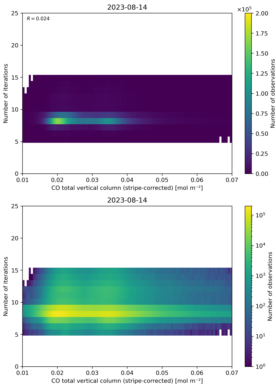
Figure 39: Scatter density plot of “CO total vertical column (stripe-corrected)” against “Number of iterations” for 2023-08-14 to 2023-08-15.
