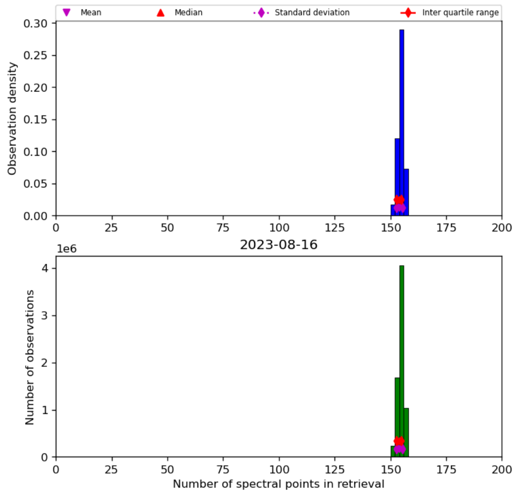
Figure 21: Histogram of “Number of spectral points in retrieval” for 2023-08-15 to 2023-08-17
