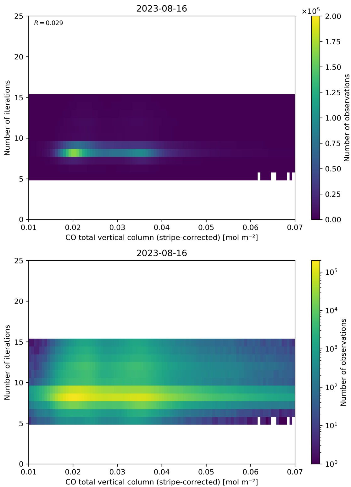
Figure 39: Scatter density plot of “CO total vertical column (stripe-corrected)” against “Number of iterations” for 2023-08-15 to 2023-08-17.
