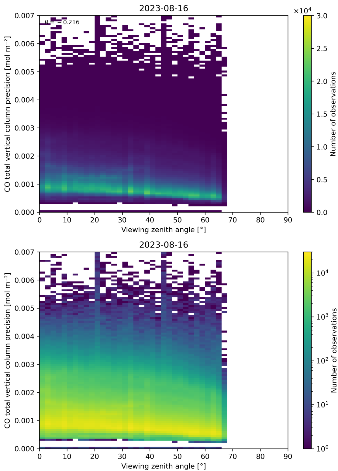
Figure 71: Scatter density plot of “Viewing zenith angle” against “CO total vertical column precision” for 2023-08-15 to 2023-08-17.
