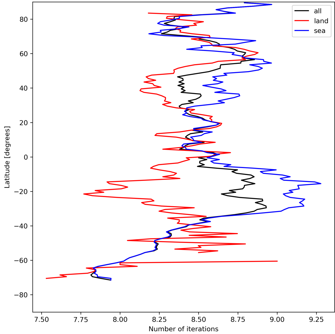
Figure 16: Zonal average of “Number of iterations” for 2023-08-15 to 2023-08-17.
