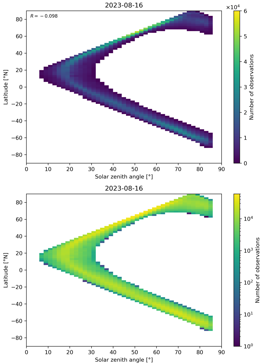
Figure 66: Scatter density plot of “Solar zenith angle” against “Latitude” for 2023-08-15 to 2023-08-17.
