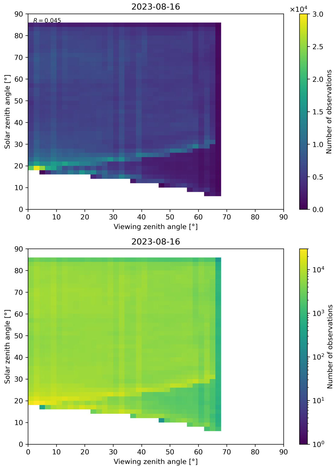
Figure 77: Scatter density plot of “Viewing zenith angle” against “Solar zenith angle” for 2023-08-15 to 2023-08-17.
