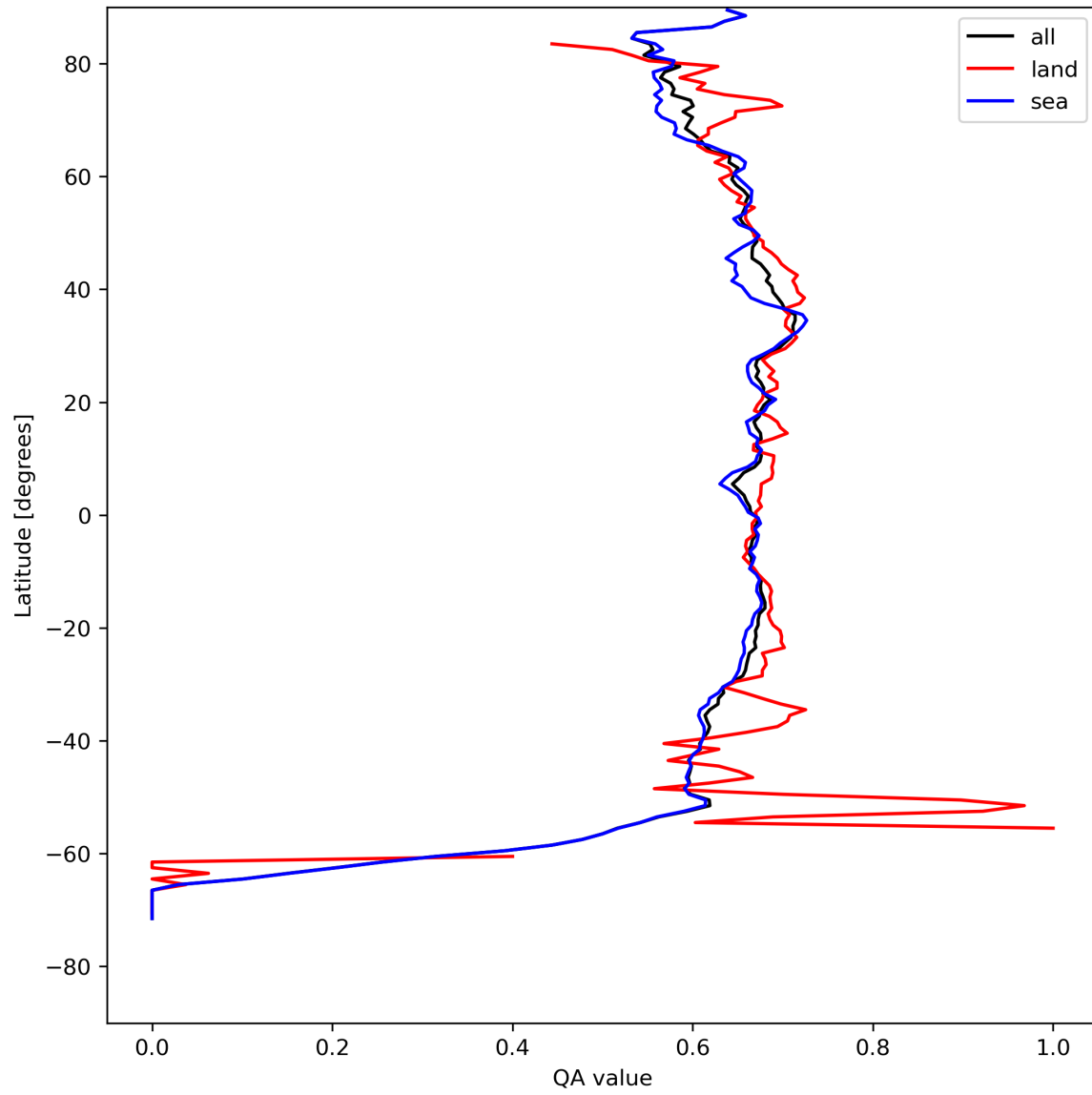
Figure 9: Zonal average of “QA value” for 2023-08-15 to 2023-08-17.
