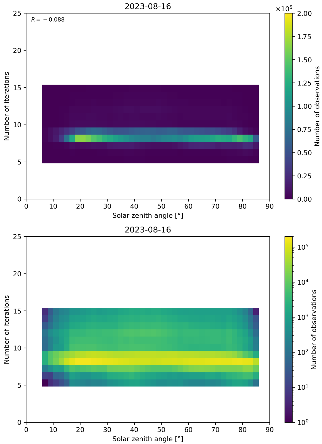
Figure 67: Scatter density plot of “Solar zenith angle” against “Number of iterations” for 2023-08-15 to 2023-08-17.
