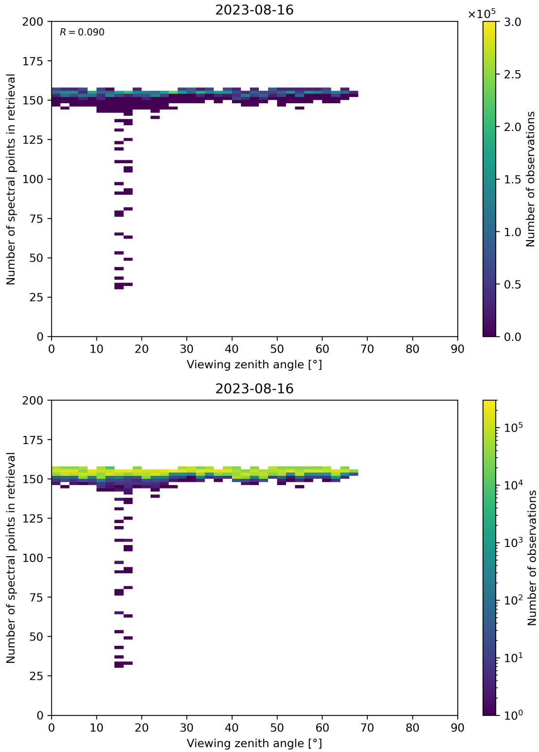
Figure 76: Scatter density plot of “Viewing zenith angle” against “Number of spectral points in retrieval” for 2023-08-15 to 2023-08-17.
