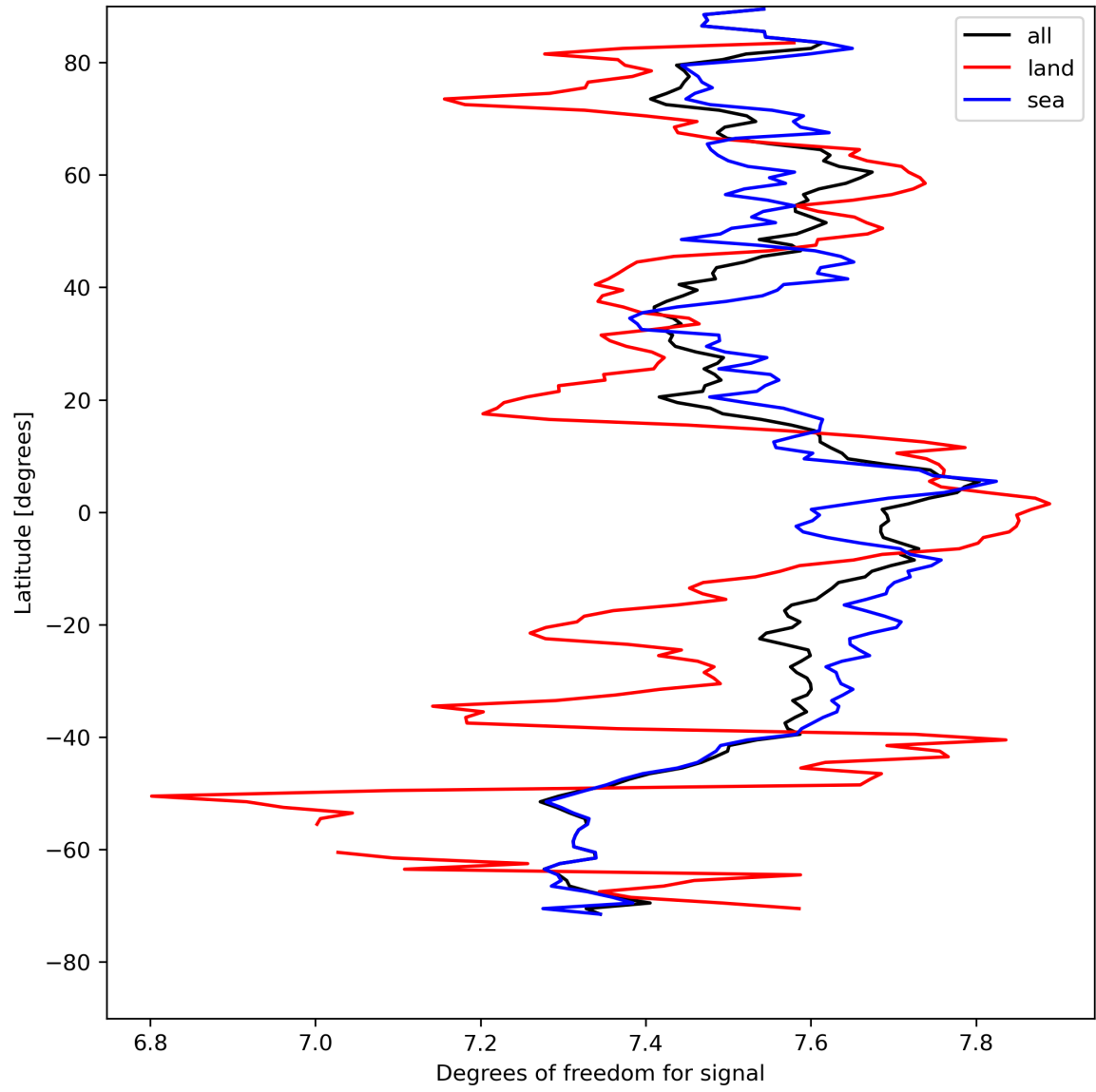
Figure 15: Zonal average of “Degrees of freedom for signal” for 2023-08-15 to 2023-08-17.
