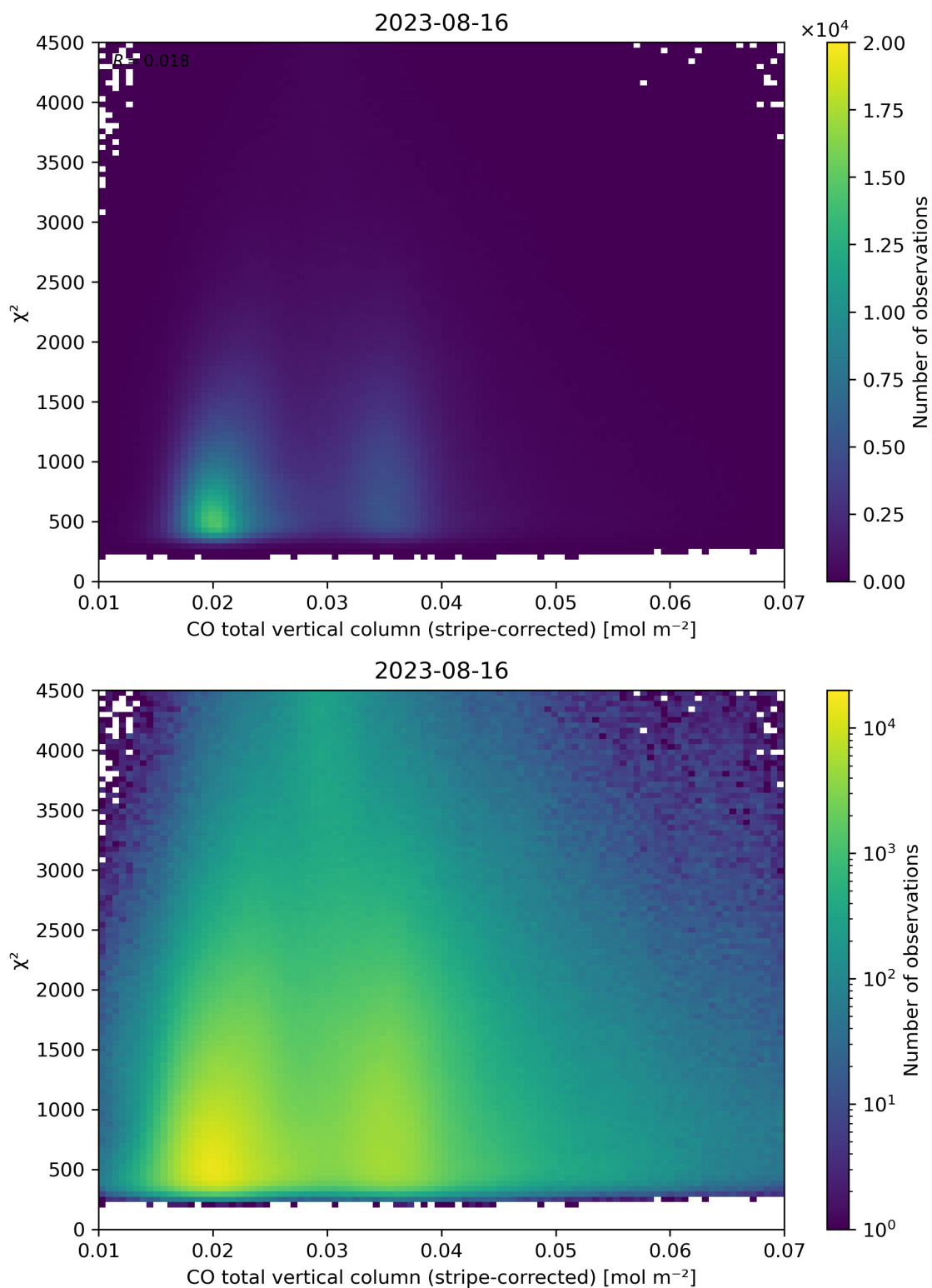
Figure 37: Scatter density plot of “CO total vertical column (stripe-corrected)” against “ \chi^2 ” for 2023-08-15 to 2023-08-17.
