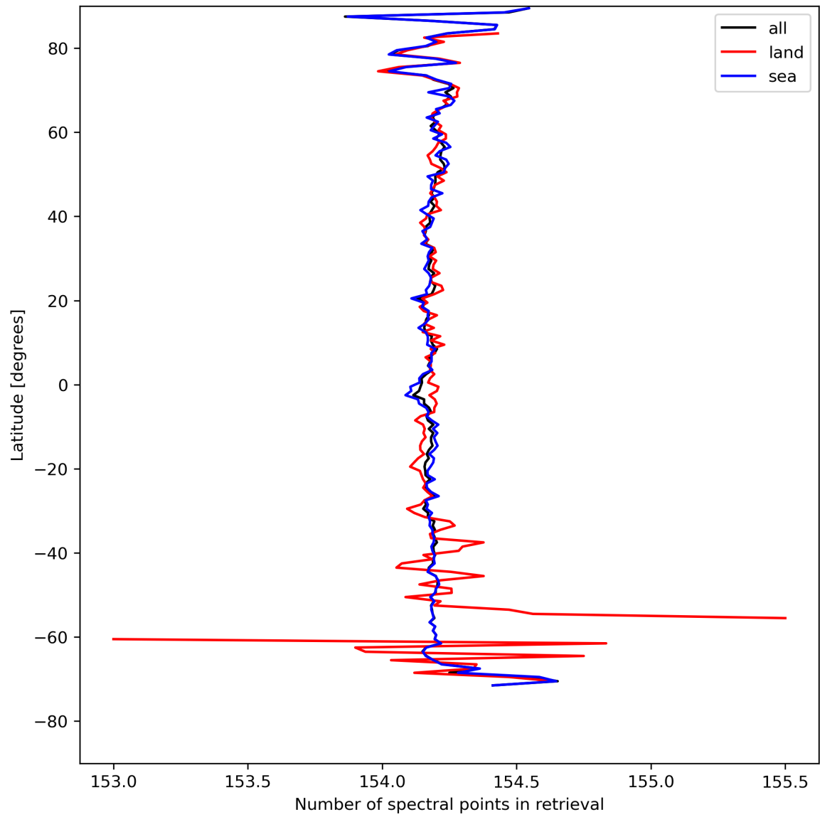
Figure 13: Zonal average of “Number of spectral points in retrieval” for 2023-08-15 to 2023-08-17.
