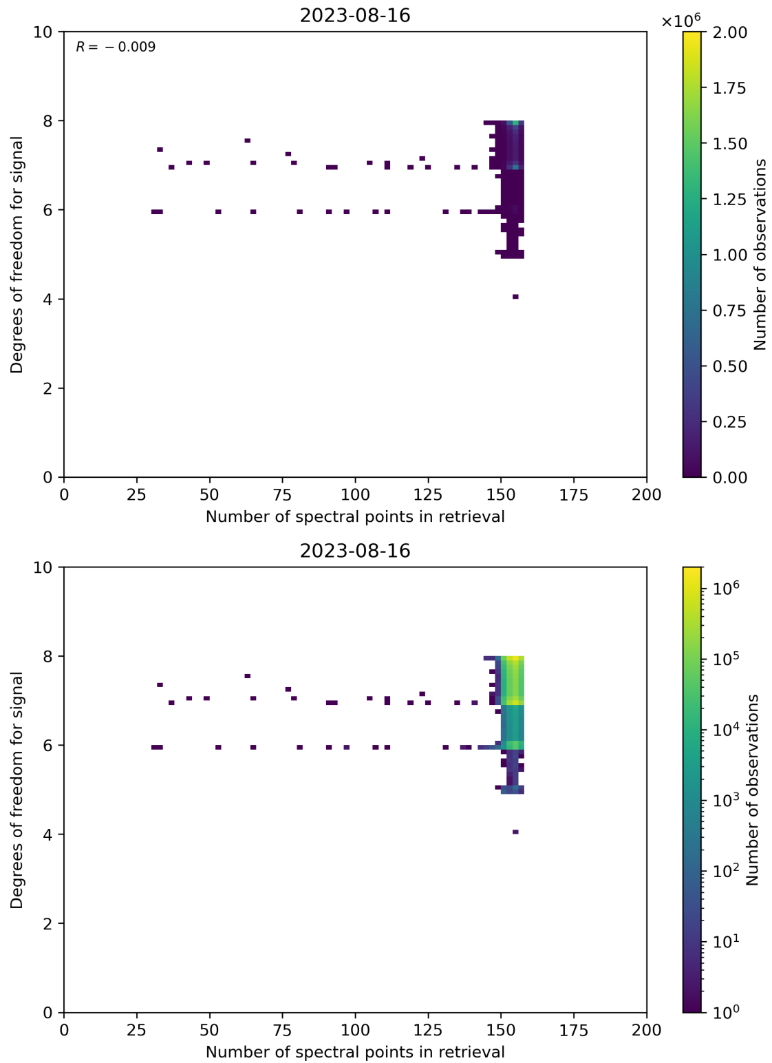
Figure 59: Scatter density plot of “Number of spectral points in retrieval” against “Degrees of freedom for signal” for 2023-08-15 to 2023-08-17.
