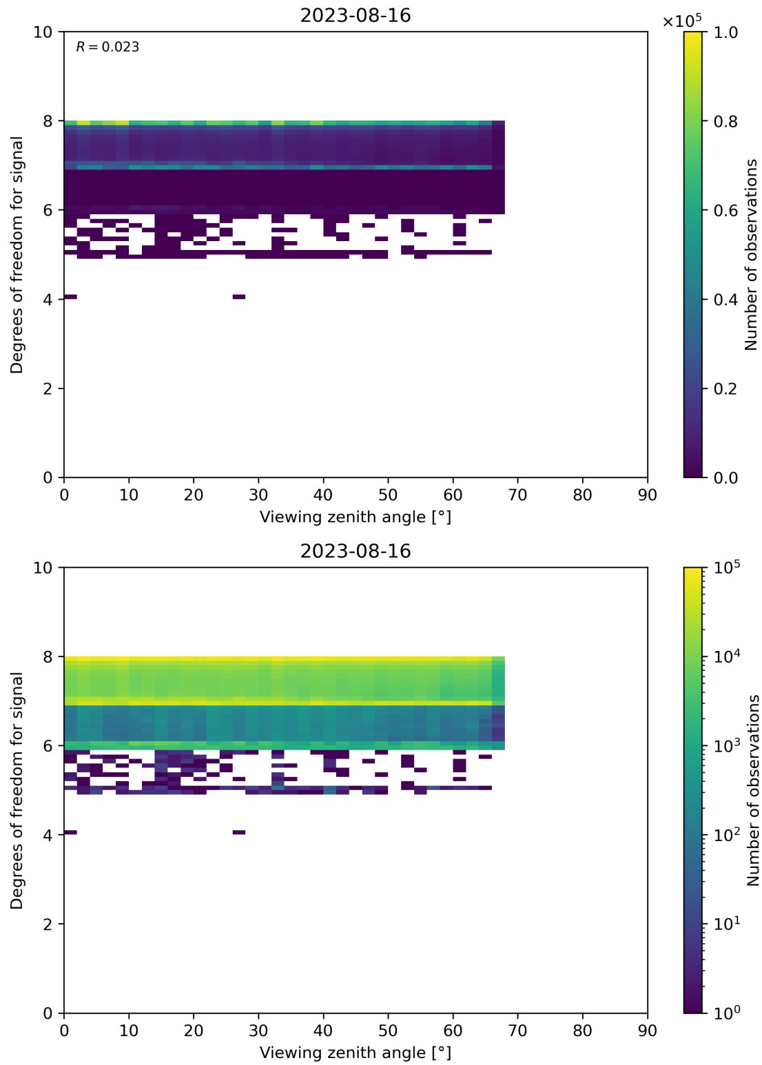
Figure 73: Scatter density plot of “Viewing zenith angle” against “Degrees of freedom for signal” for 2023-08-15 to 2023-08-17.
