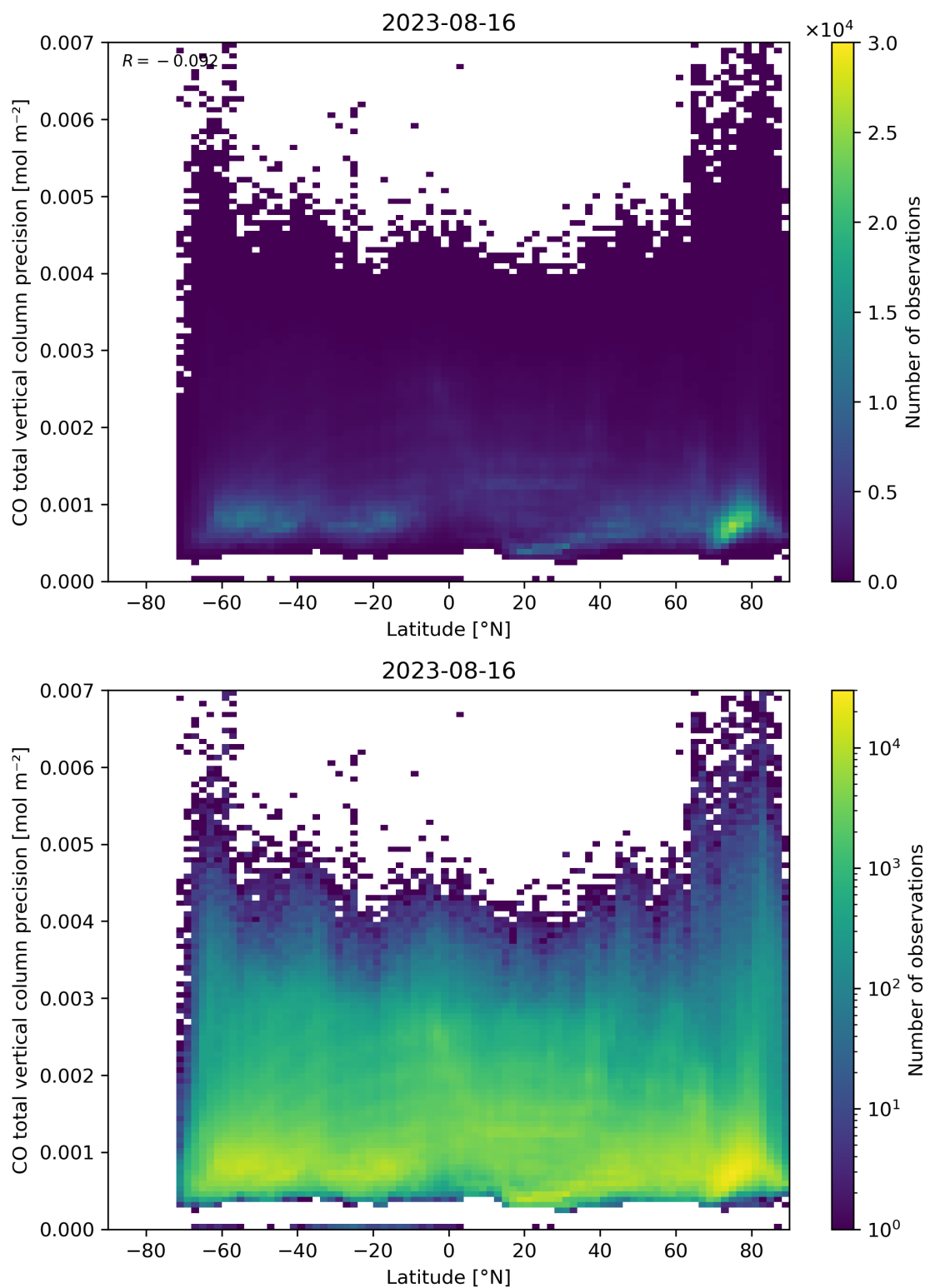
Figure 53: Scatter density plot of “Latitude” against “CO total vertical column precision” for 2023-08-15 to 2023-08-17.
