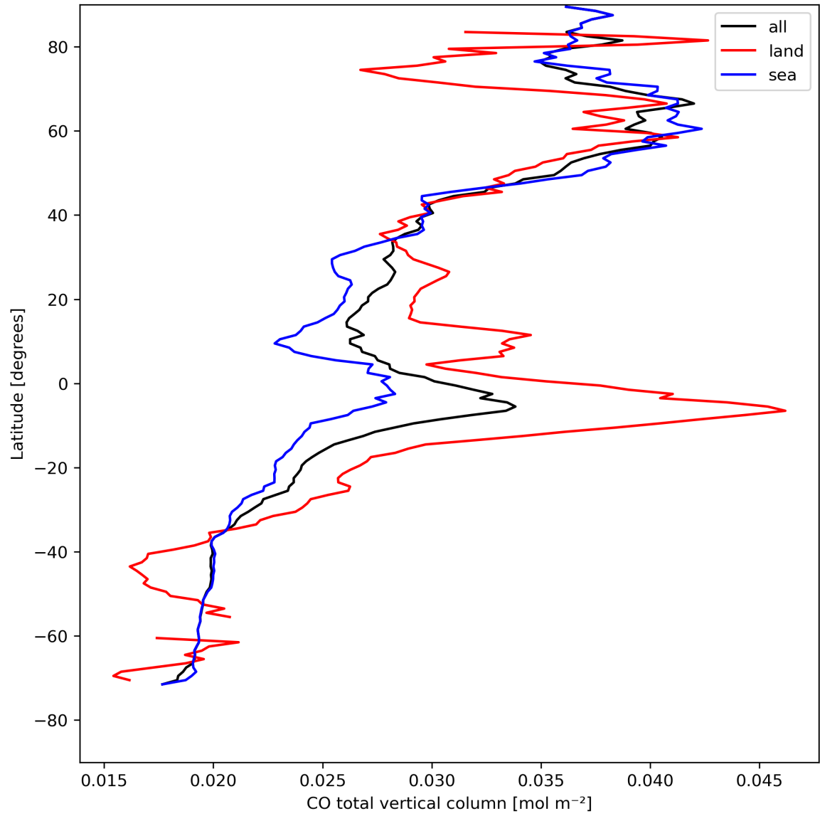
Figure 10: Zonal average of “CO total vertical column” for 2023-08-15 to 2023-08-17.
