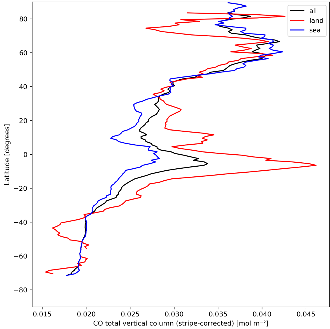
Figure 11: Zonal average of “CO total vertical column (stripe-corrected)” for 2023-08-15 to 2023-08-17.
