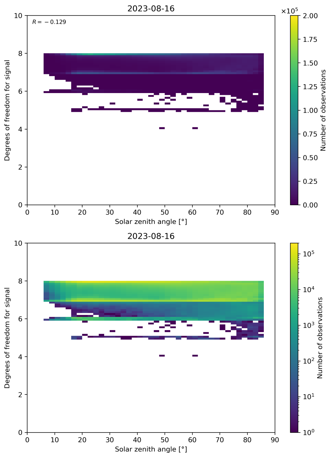
Figure 65: Scatter density plot of “Solar zenith angle” against “Degrees of freedom for signal” for 2023-08-15 to 2023-08-17.
