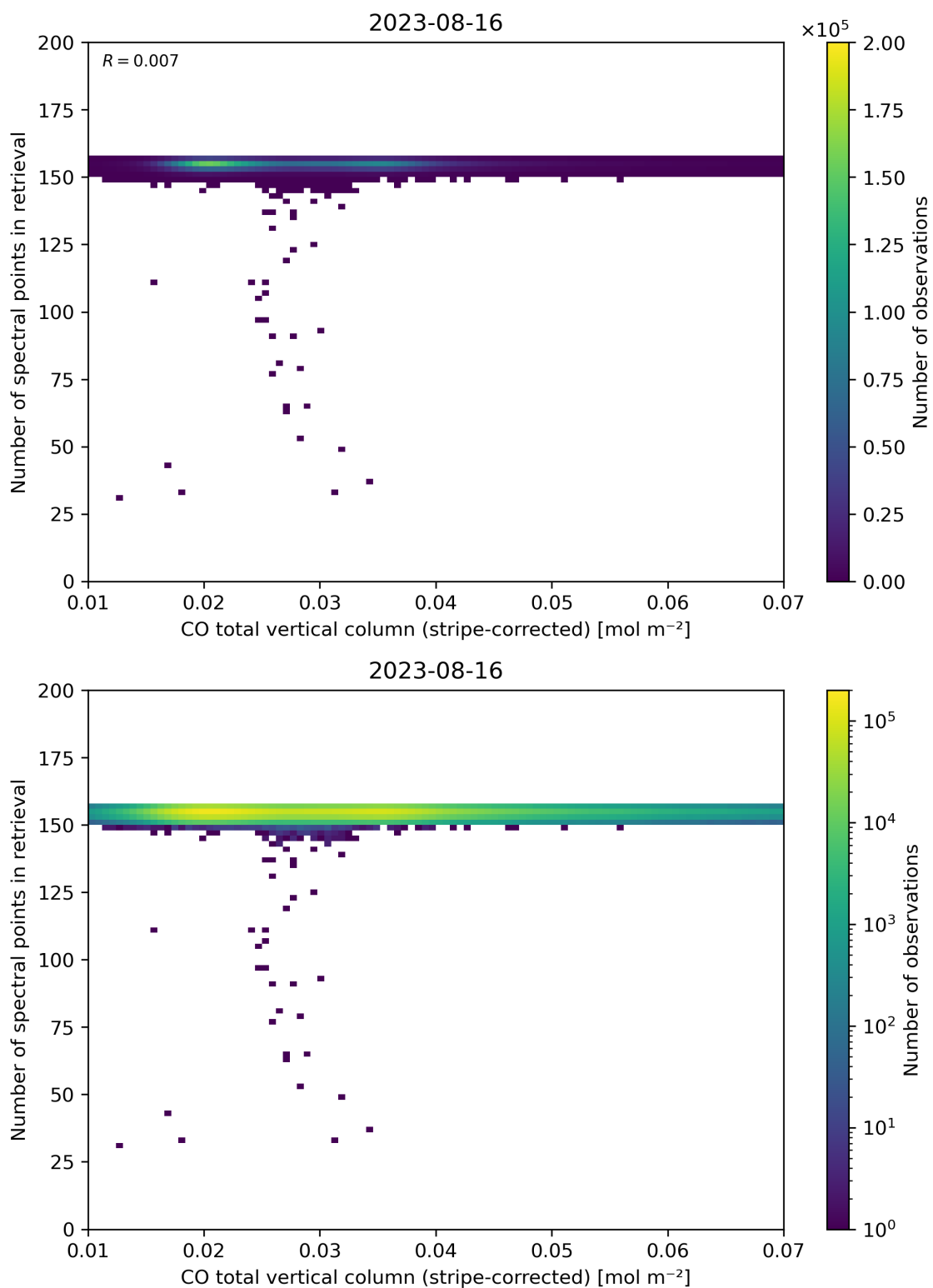
Figure 40: Scatter density plot of “CO total vertical column (stripe-corrected)” against “Number of spectral points in retrieval” for 2023-08-15 to 2023-08-17.
