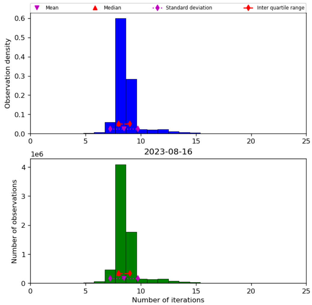
Figure 24: Histogram of “Number of iterations” for 2023-08-15 to 2023-08-17
