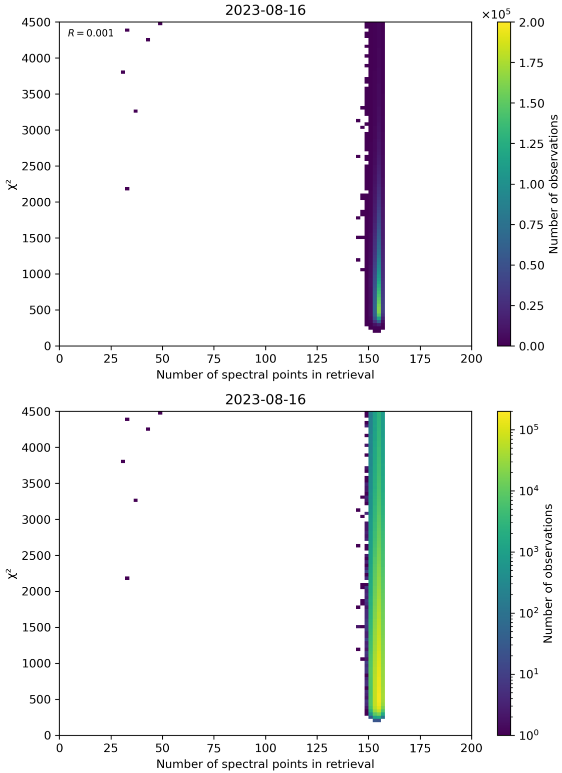
Figure 58: Scatter density plot of “Number of spectral points in retrieval” against “ \chi^2 ” for 2023-08-15 to 2023-08-17.
