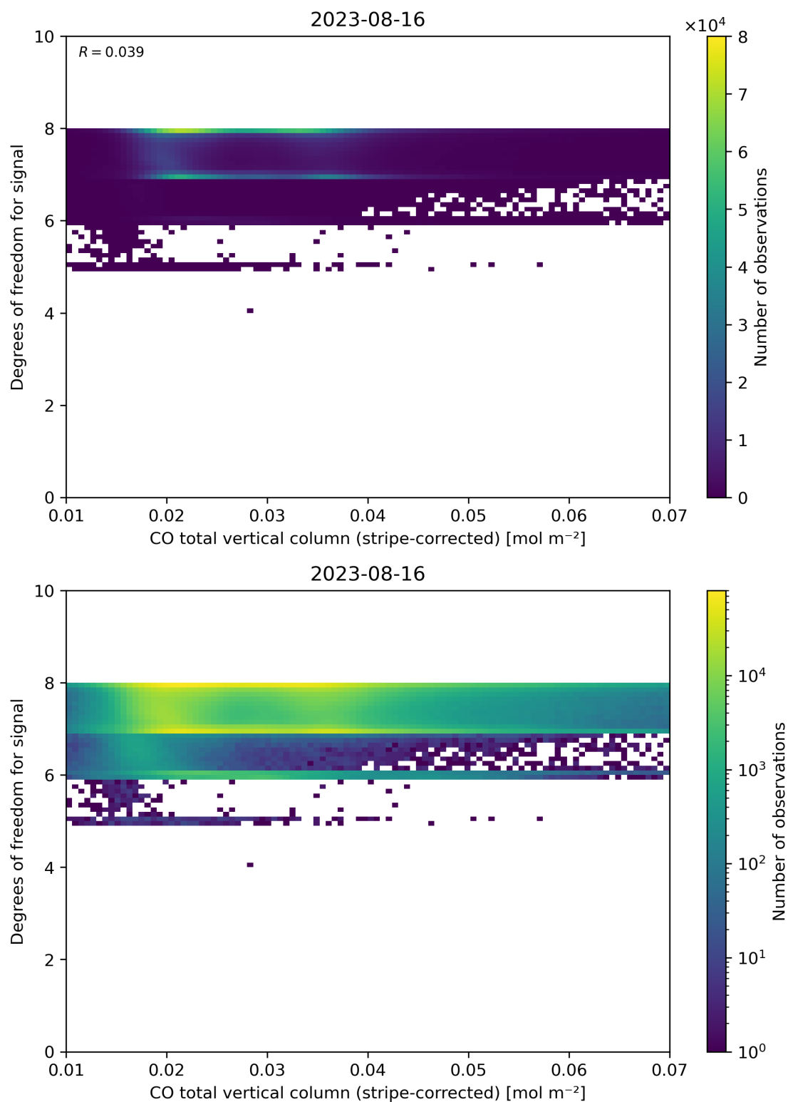
Figure 38: Scatter density plot of “CO total vertical column (stripe-corrected)” against “Degrees of freedom for signal” for 2023-08-15 to 2023-08-17.
