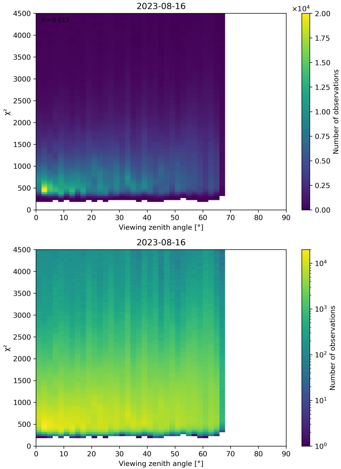
Figure 72: Scatter density plot of “Viewing zenith angle” against “ \chi^2 ” for 2023-08-15 to 2023-08-17.
