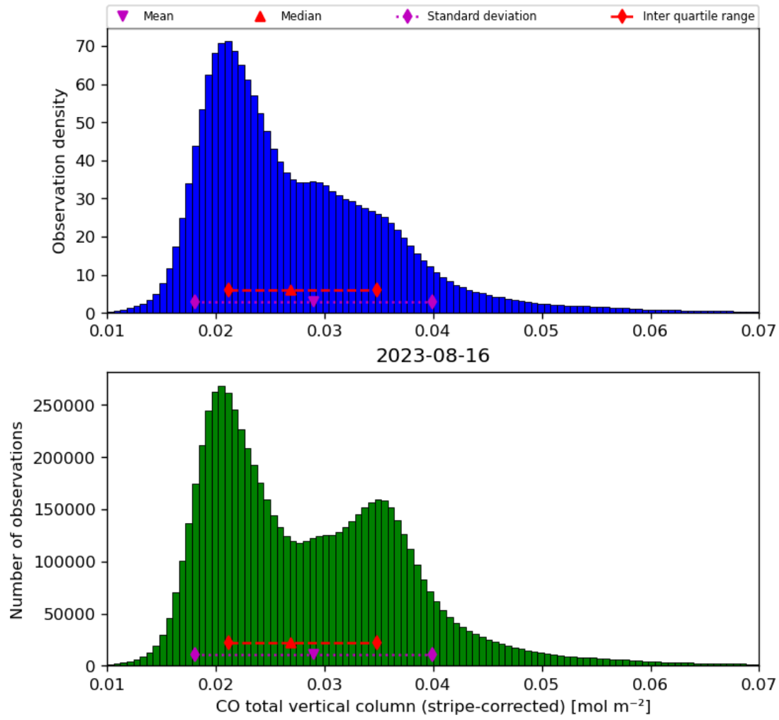
Figure 19: Histogram of “CO total vertical column (stripe-corrected)” for 2023-08-15 to 2023-08-17
