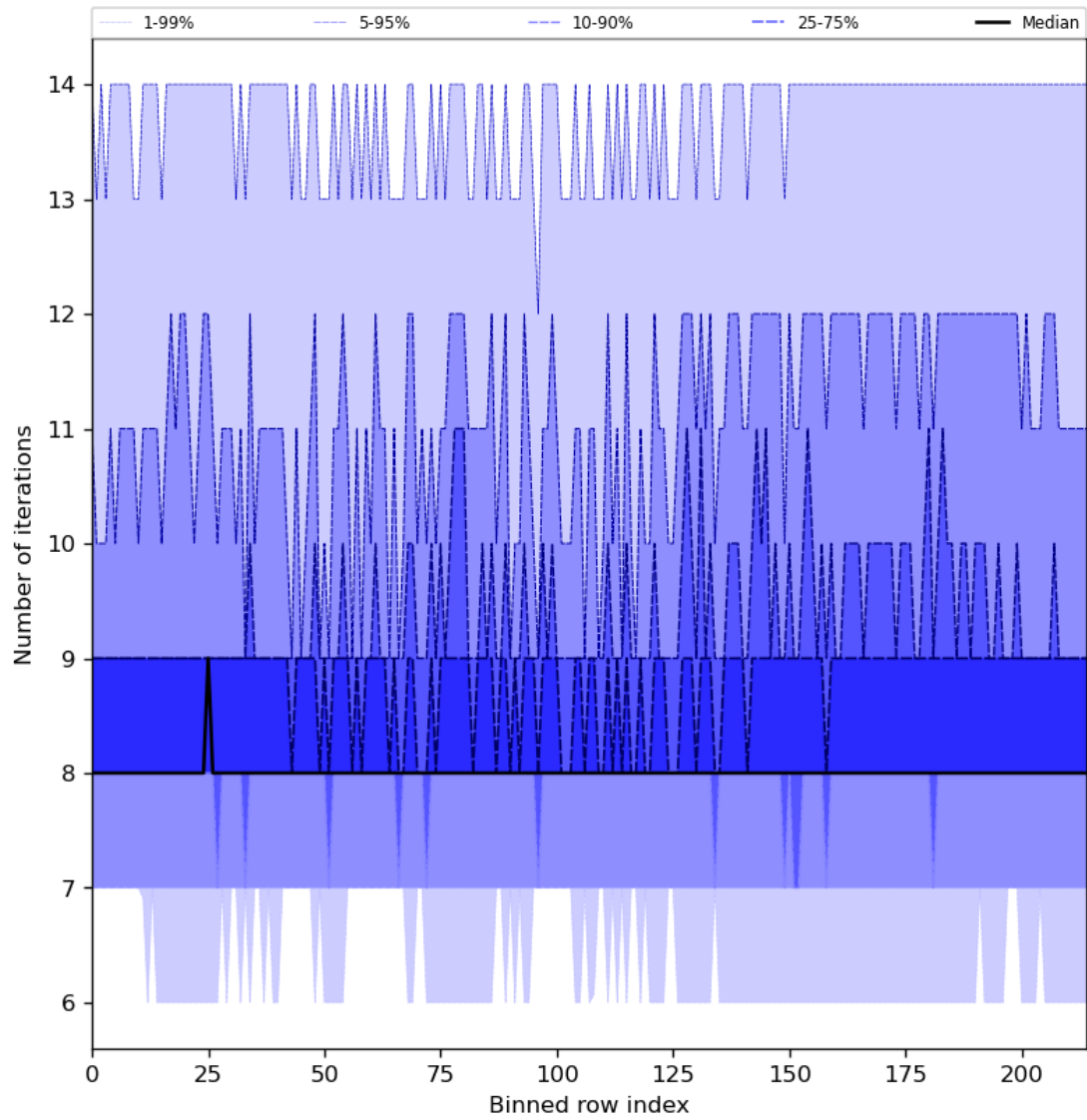
Figure 32: Along track statistics of “Number of iterations” for 2023-08-15 to 2023-08-17
