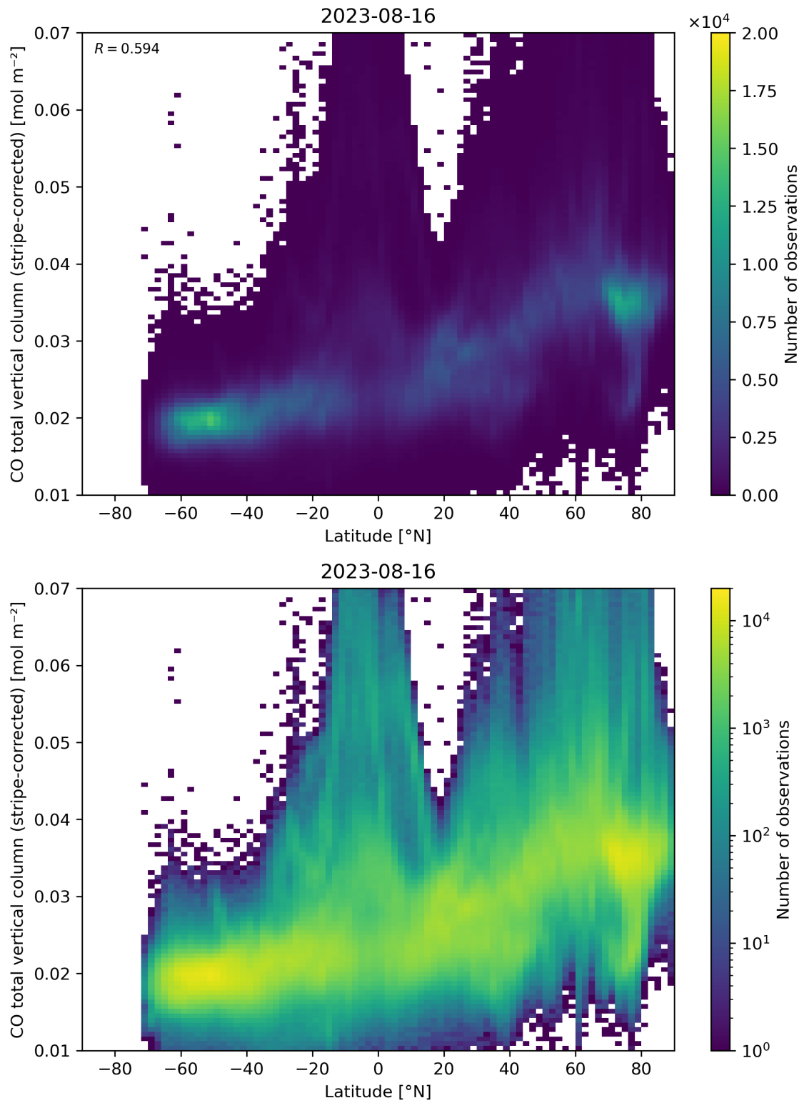
Figure 52: Scatter density plot of “Latitude” against “CO total vertical column (stripe-corrected)” for 2023-08-15 to 2023-08-17.
