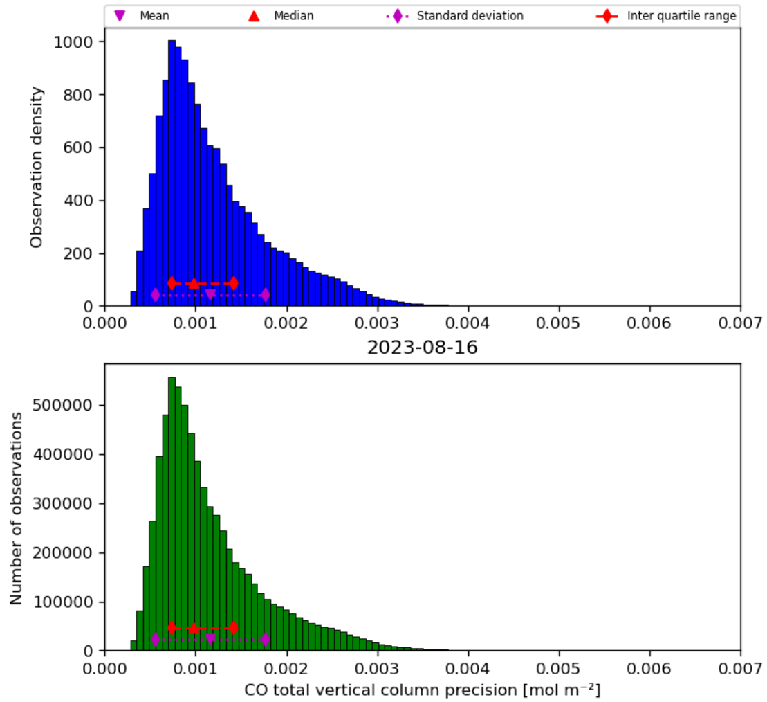
Figure 20: Histogram of “CO total vertical column precision” for 2023-08-15 to 2023-08-17
