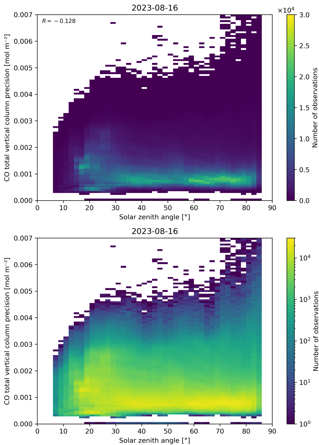
Figure 63: Scatter density plot of “Solar zenith angle” against “CO total vertical column precision” for 2023-08-15 to 2023-08-17.
