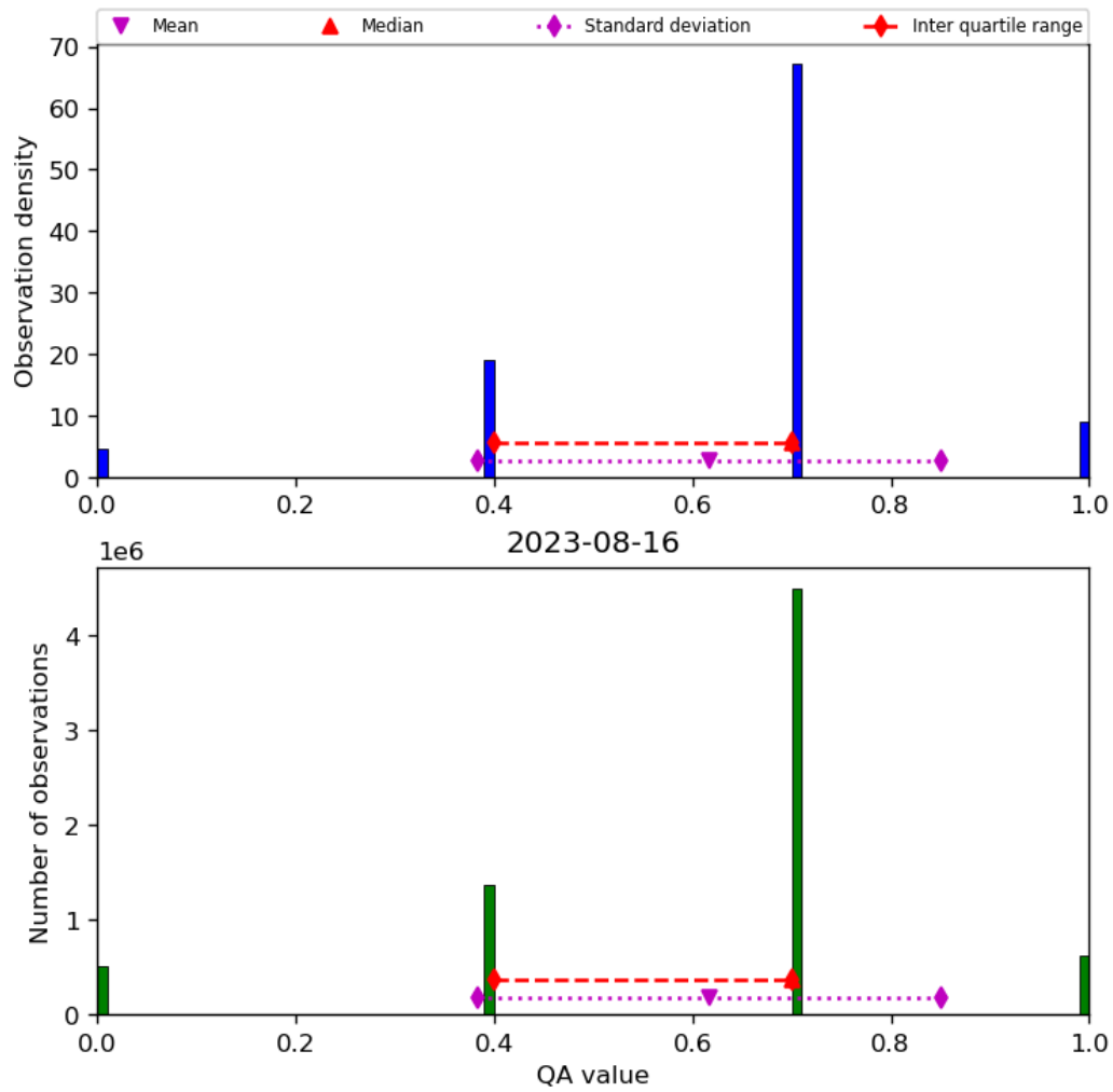
Figure 17: Histogram of “QA value” for 2023-08-15 to 2023-08-17
