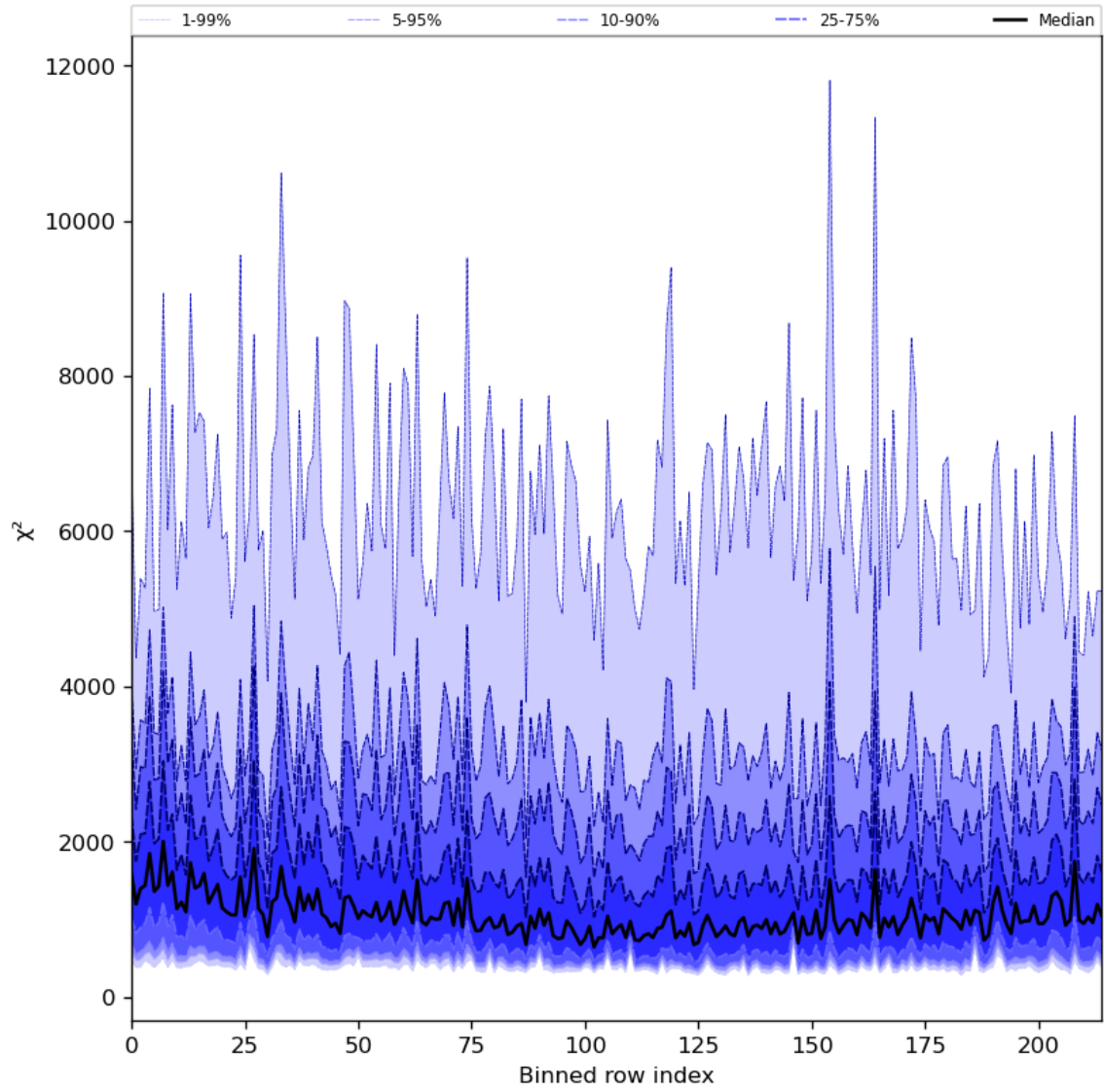
Figure 30: Along track statistics of “ \chi^2 ” for 2023-08-15 to 2023-08-17
