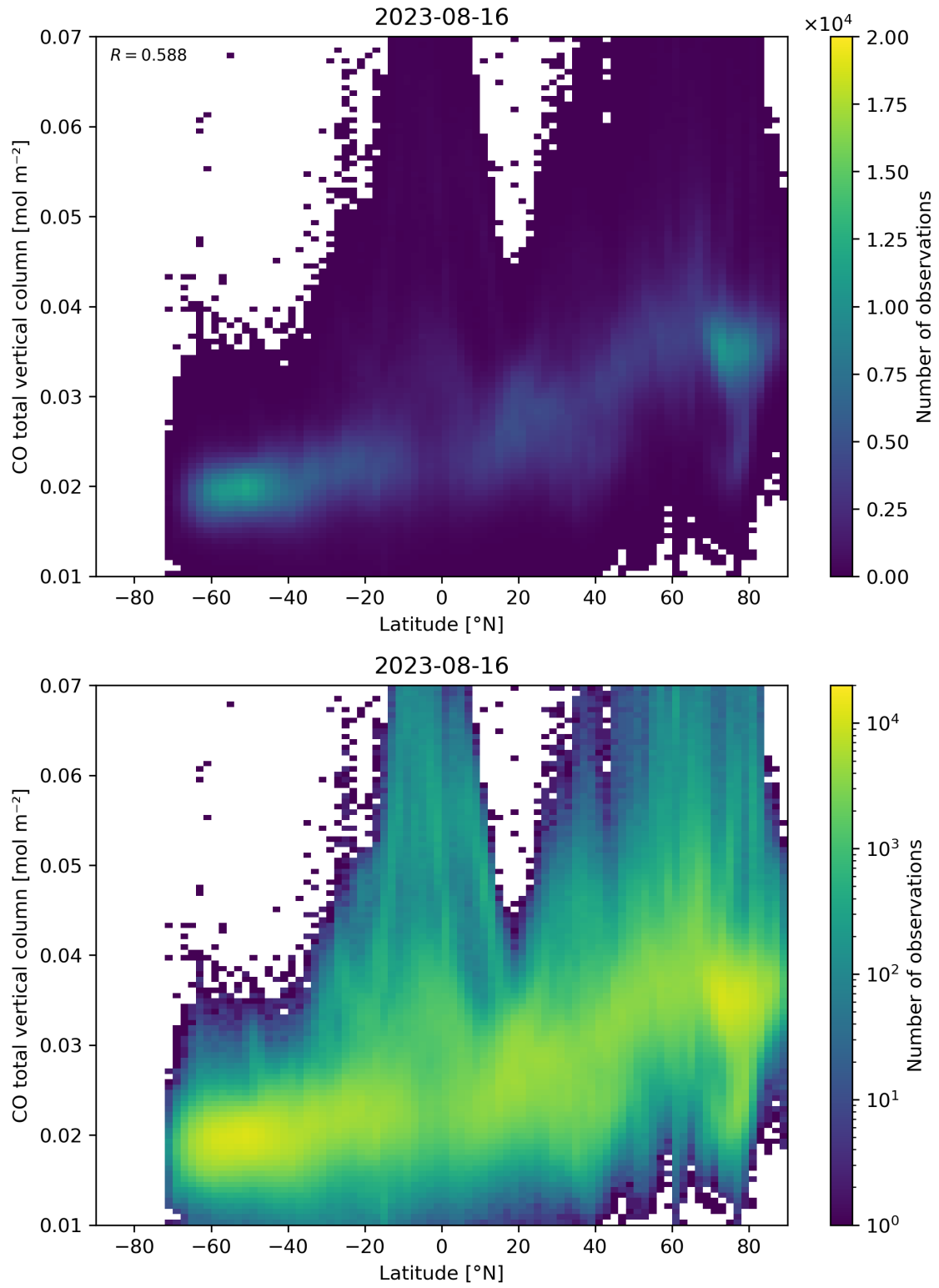
Figure 51: Scatter density plot of “Latitude” against “CO total vertical column” for 2023-08-15 to 2023-08-17.
