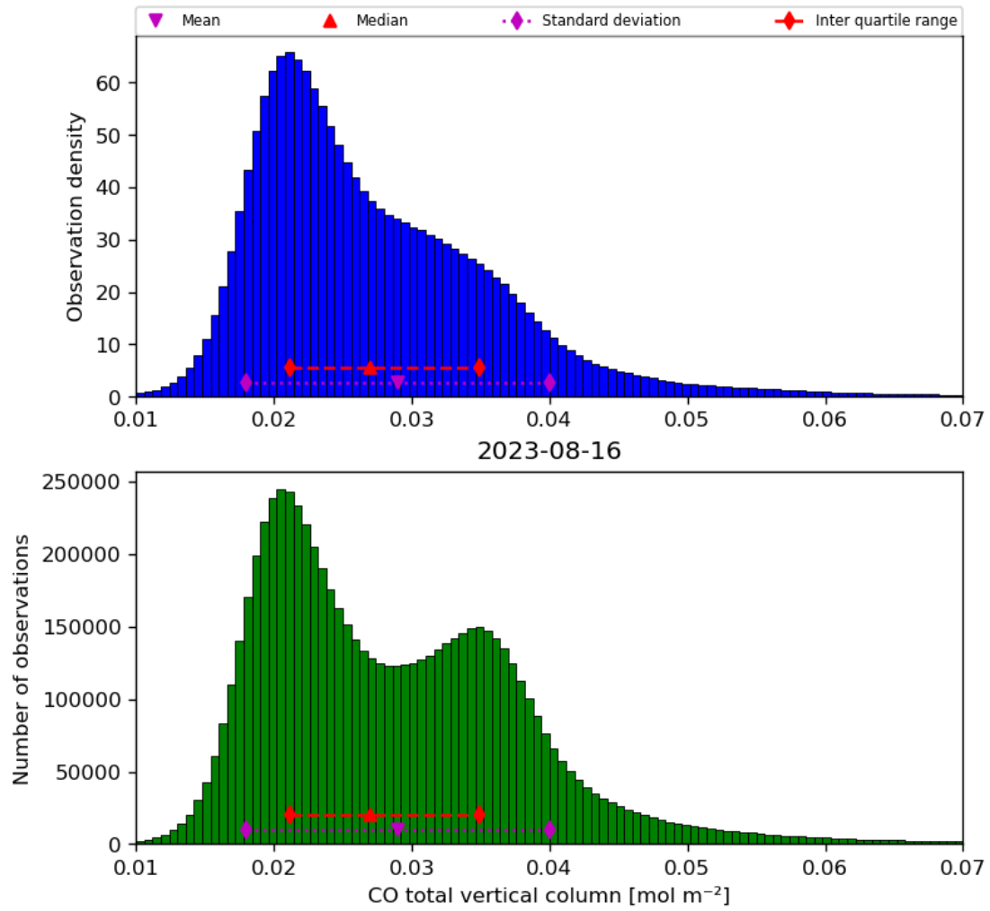
Figure 18: Histogram of “CO total vertical column” for 2023-08-15 to 2023-08-17
