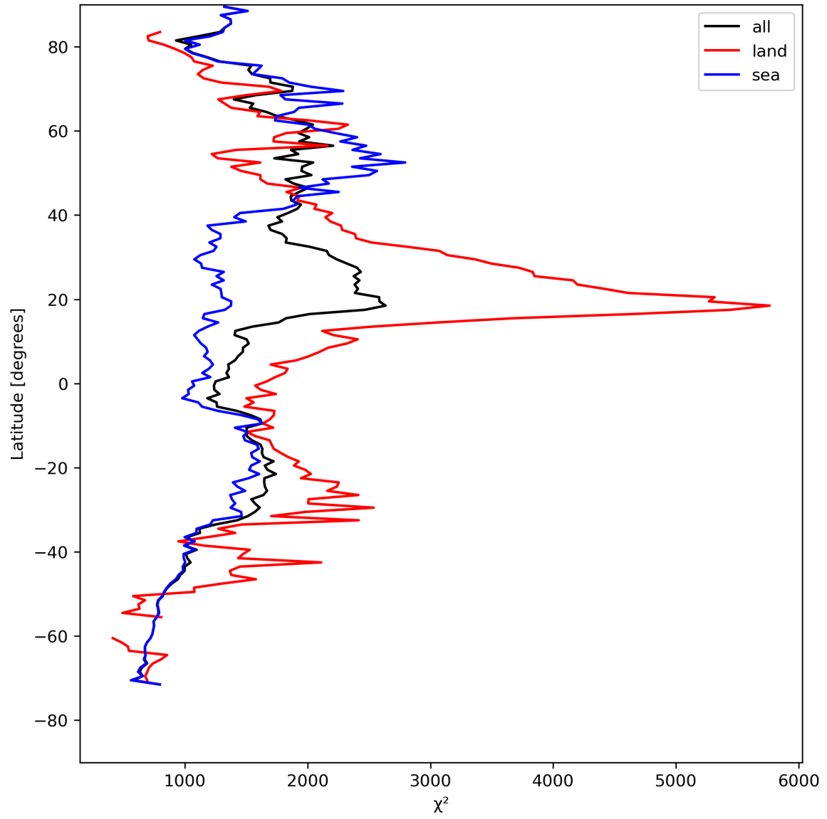
Figure 14: Zonal average of “ \chi^2 ” for 2023-08-15 to 2023-08-17.
