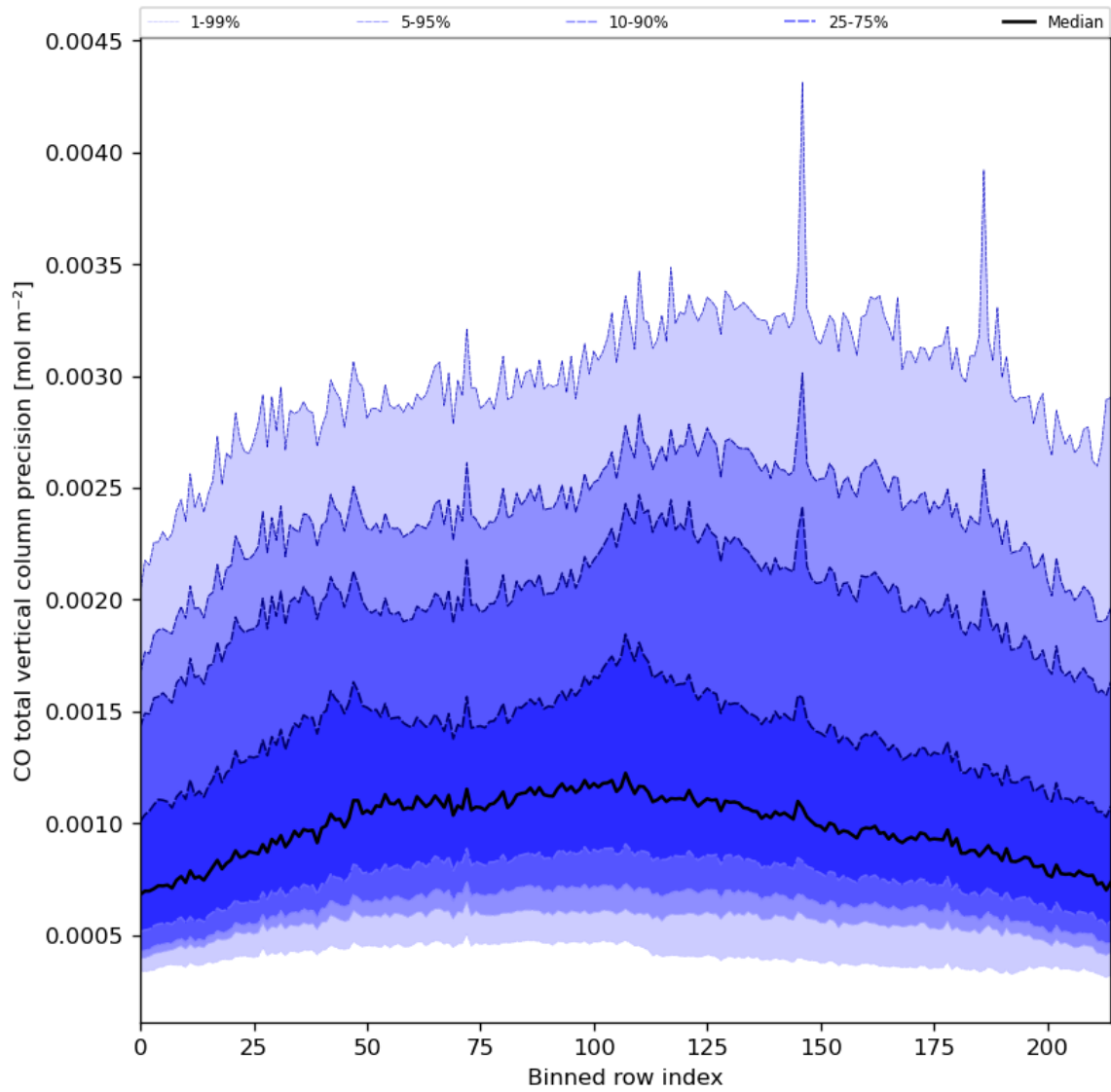
Figure 28: Along track statistics of “CO total vertical column precision” for 2023-08-15 to 2023-08-17
