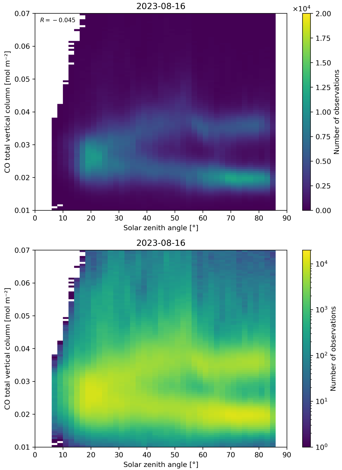
Figure 61: Scatter density plot of “Solar zenith angle” against “CO total vertical column” for 2023-08-15 to 2023-08-17.
