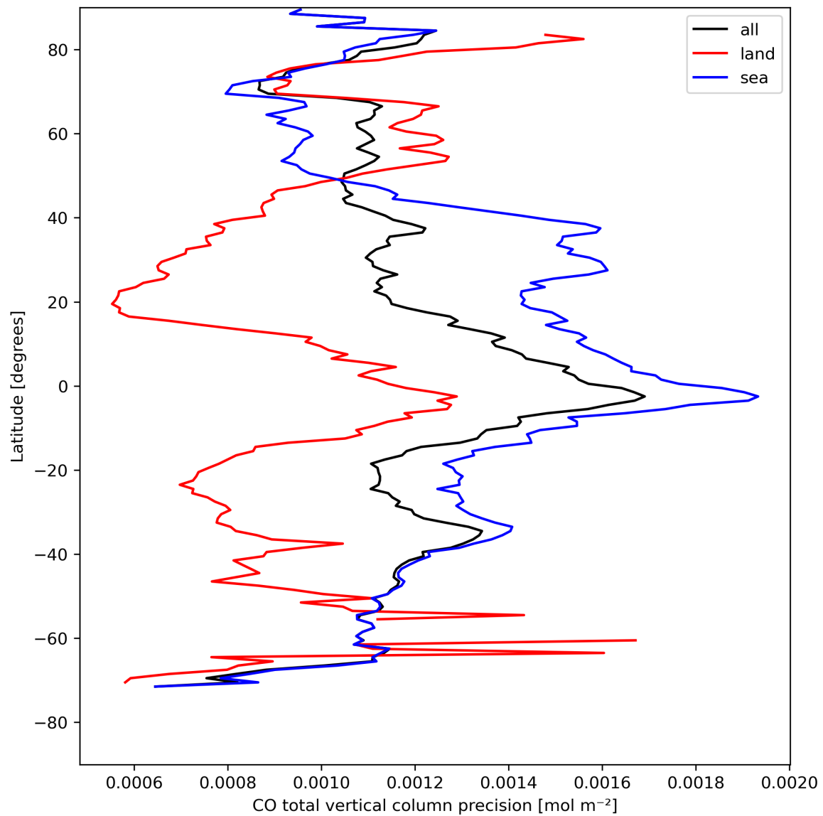
Figure 12: Zonal average of “CO total vertical column precision” for 2023-08-15 to 2023-08-17.
