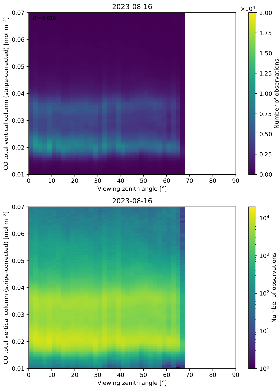
Figure 70: Scatter density plot of “Viewing zenith angle” against “CO total vertical column (stripe-corrected)” for 2023-08-15 to 2023-08-17.
