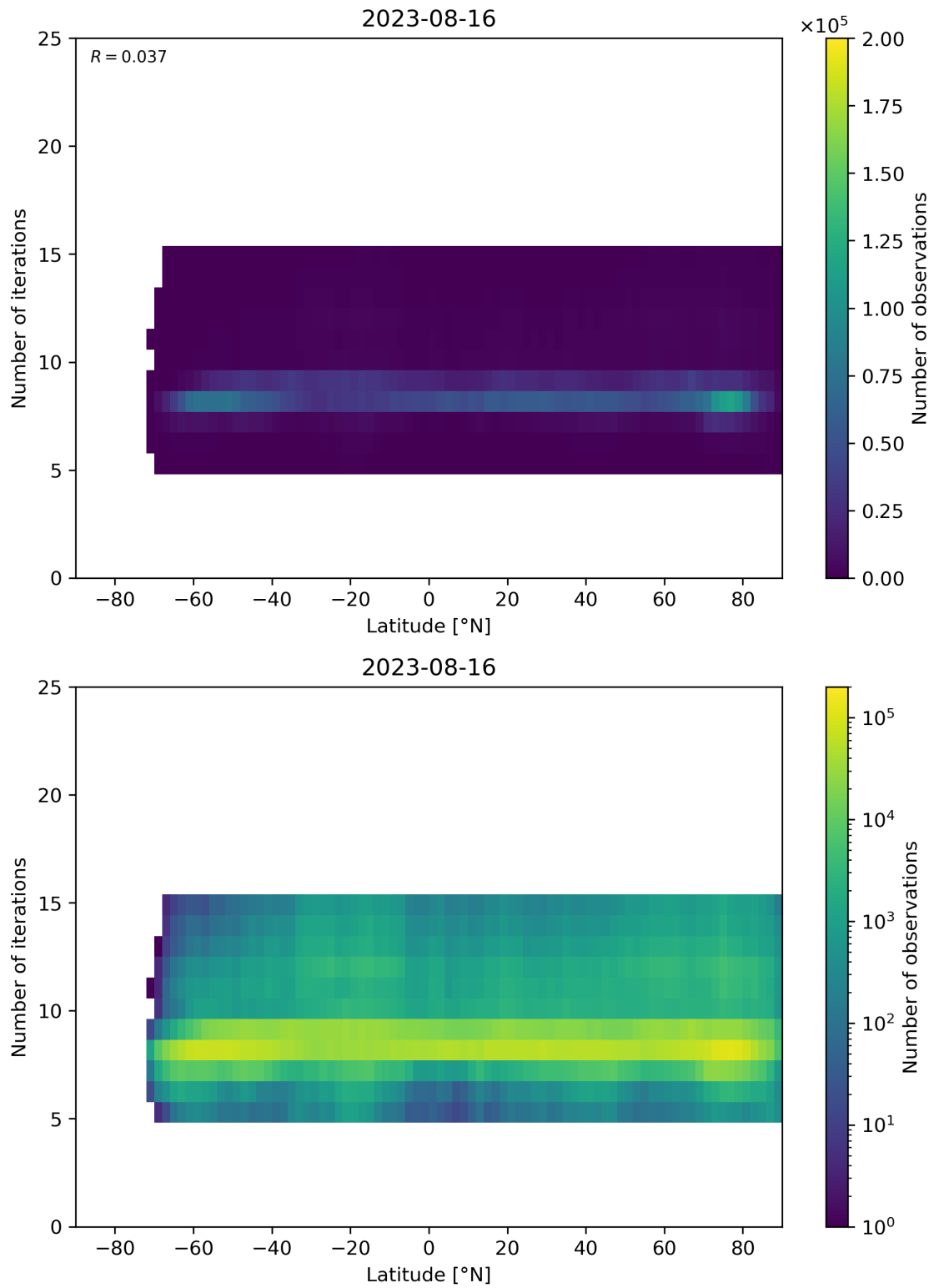
Figure 56: Scatter density plot of “Latitude” against “Number of iterations” for 2023-08-15 to 2023-08-17.
