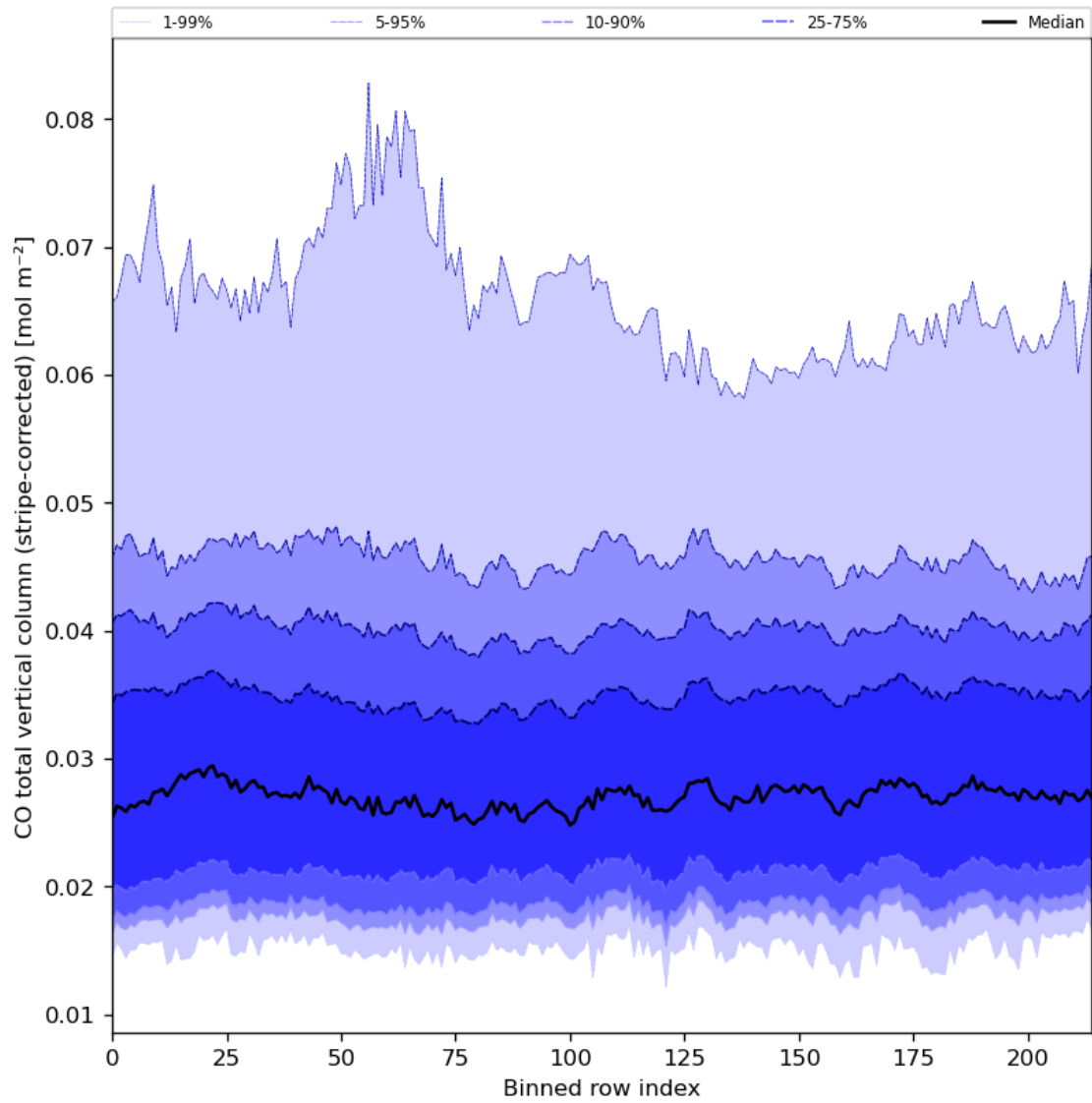
Figure 27: Along track statistics of “CO total vertical column (stripe-corrected)” for 2023-08-15 to 2023-08-17
