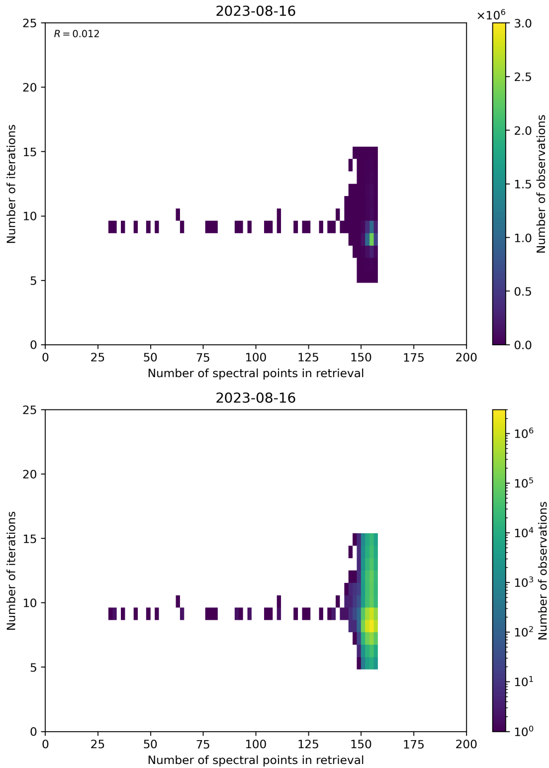
Figure 60: Scatter density plot of “Number of spectral points in retrieval” against “Number of iterations” for 2023-08-15 to 2023-08-17.
