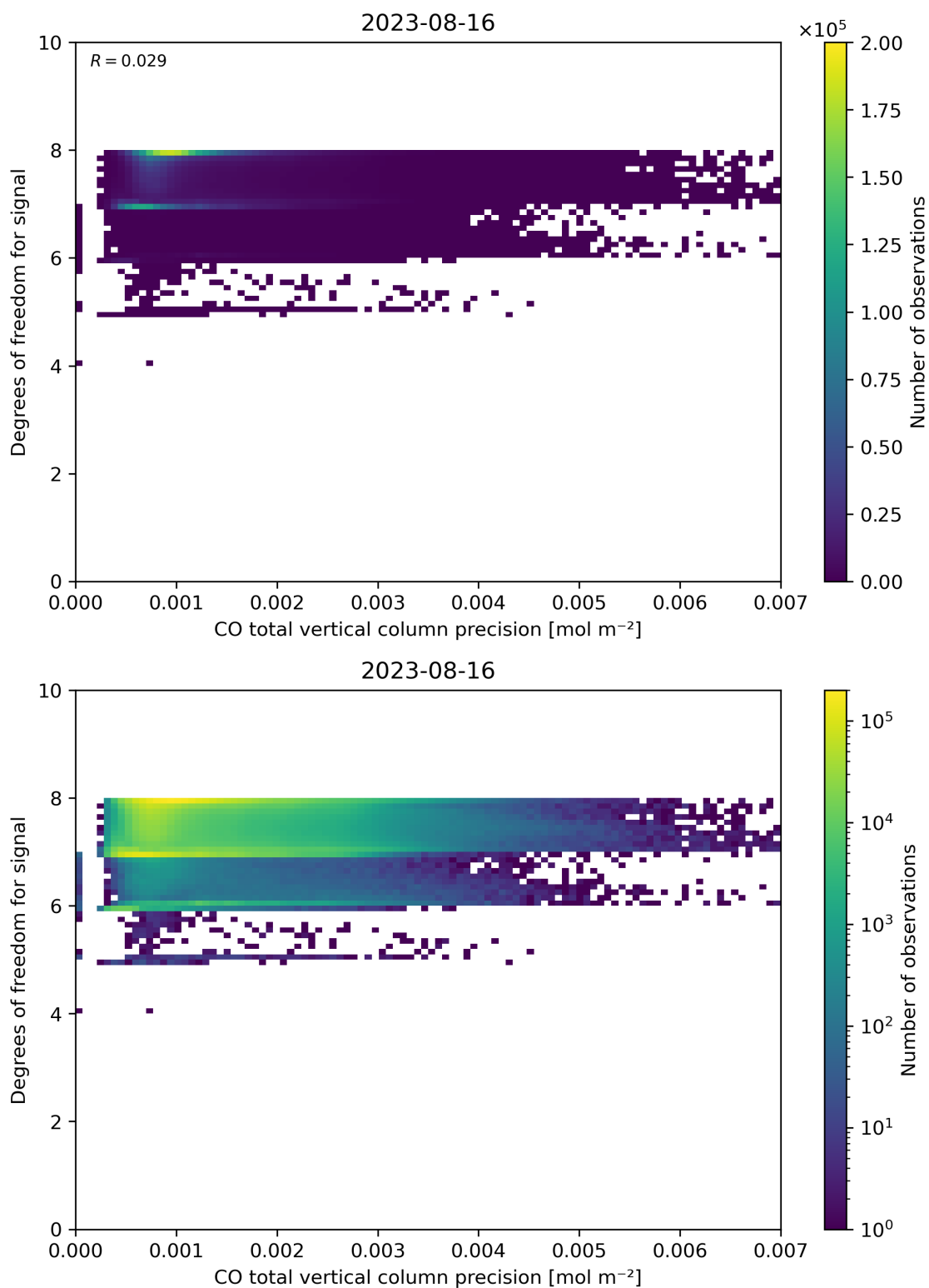
Figure 45: Scatter density plot of “CO total vertical column precision” against “Degrees of freedom for signal” for 2023-08-15 to 2023-08-17.
