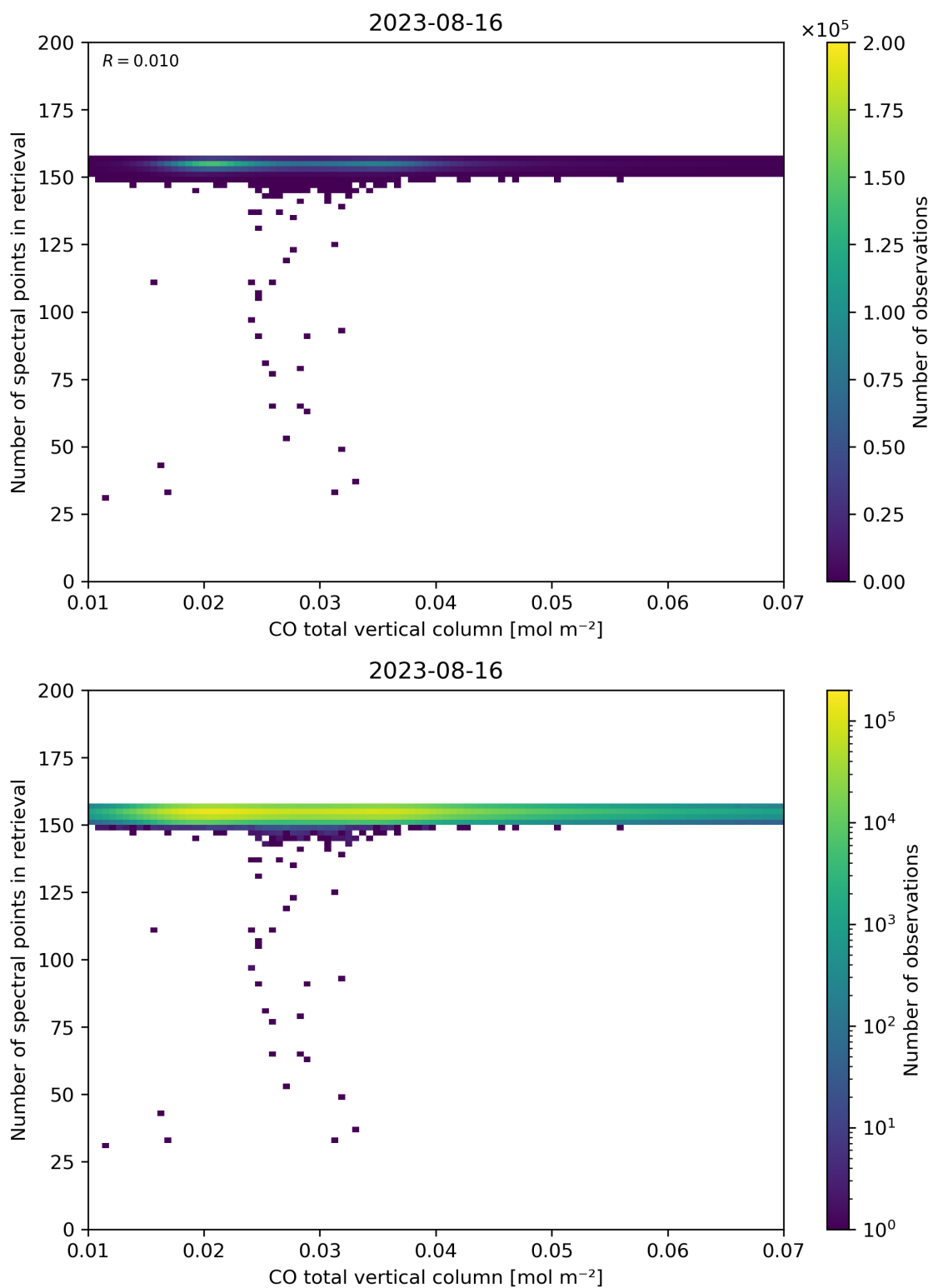
Figure 43: Scatter density plot of “CO total vertical column” against “Number of spectral points in retrieval” for 2023-08-15 to 2023-08-17.
