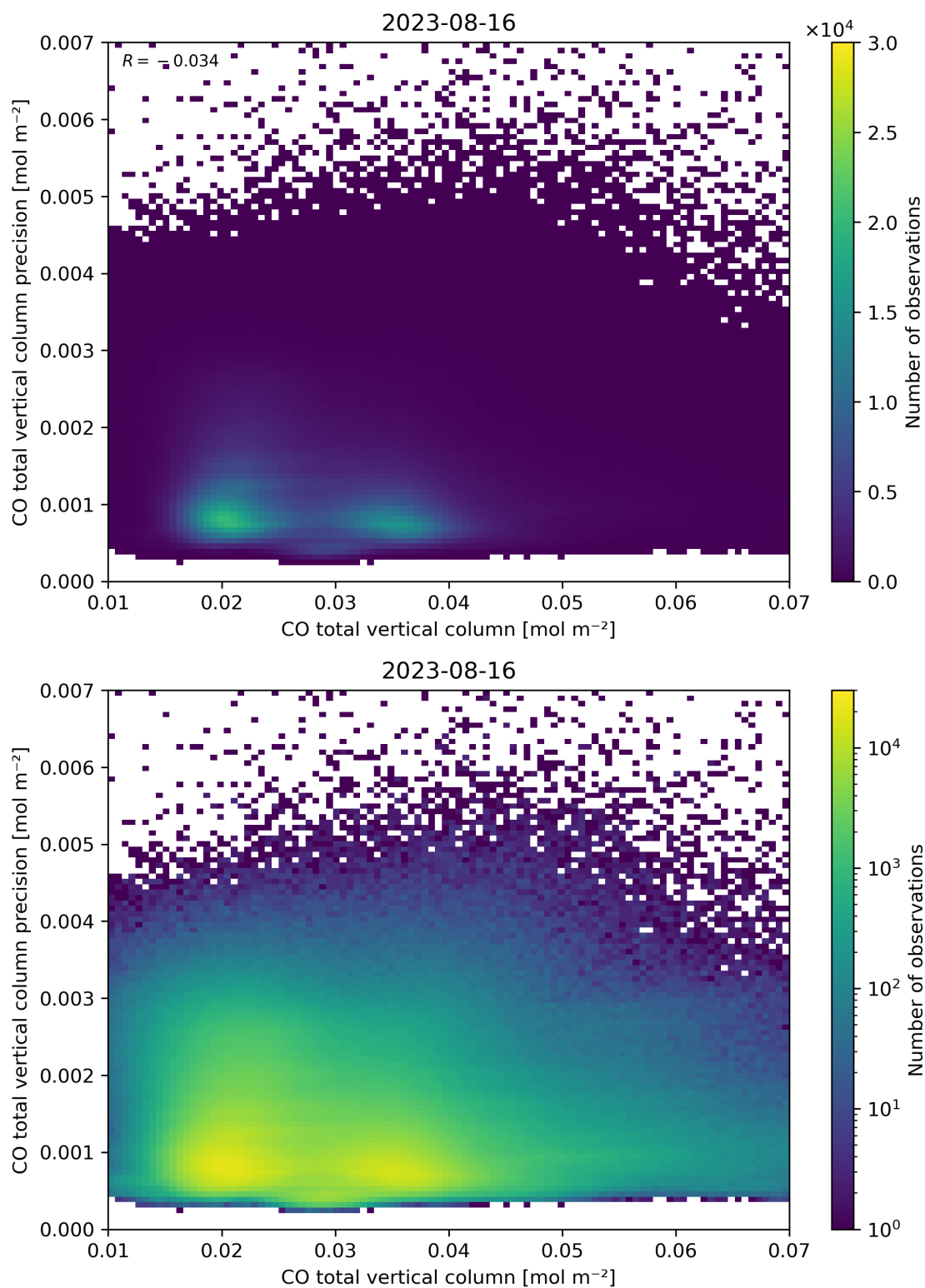
Figure 34: Scatter density plot of “CO total vertical column” against “CO total vertical column precision” for 2023-08-15 to 2023-08-17.
