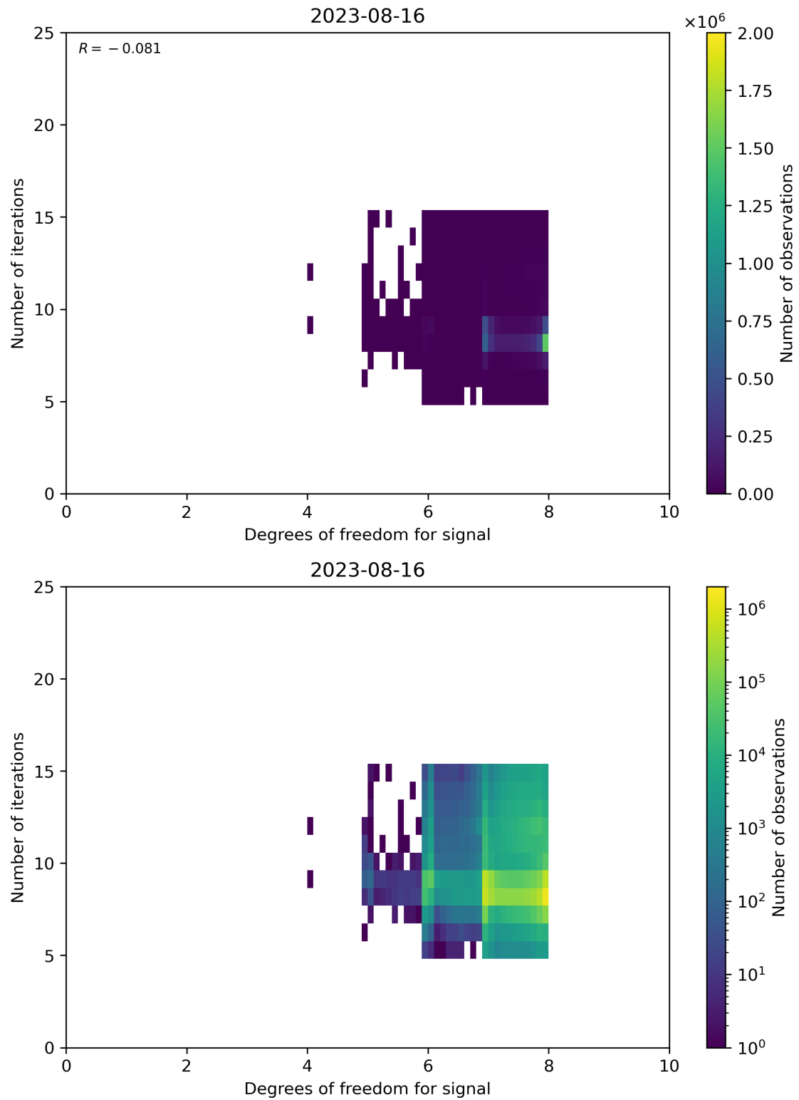
Figure 50: Scatter density plot of “Degrees of freedom for signal” against “Number of iterations” for 2023-08-15 to 2023-08-17.
