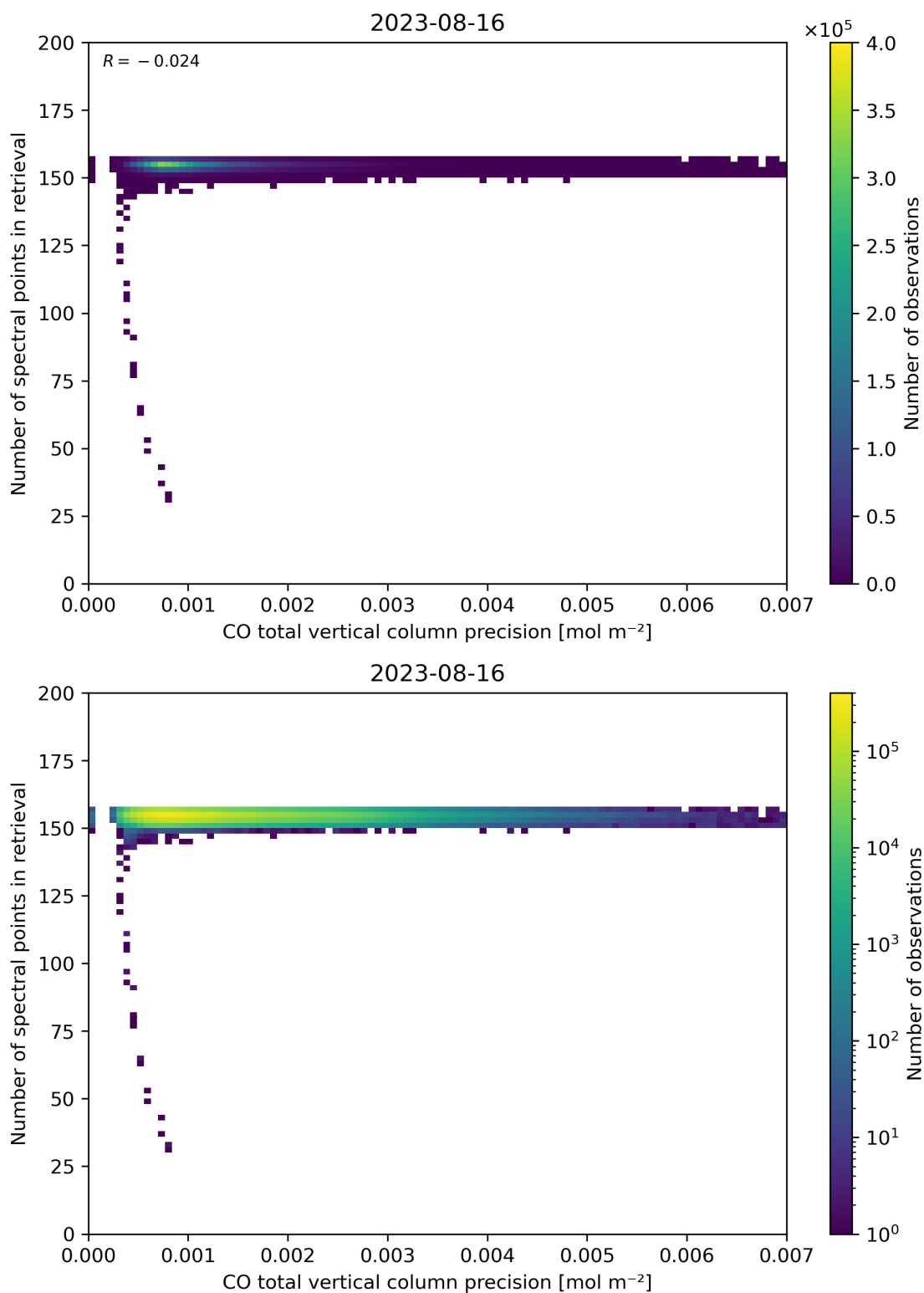
Figure 47: Scatter density plot of “CO total vertical column precision” against “Number of spectral points in retrieval” for 2023-08-15 to 2023-08-17.
