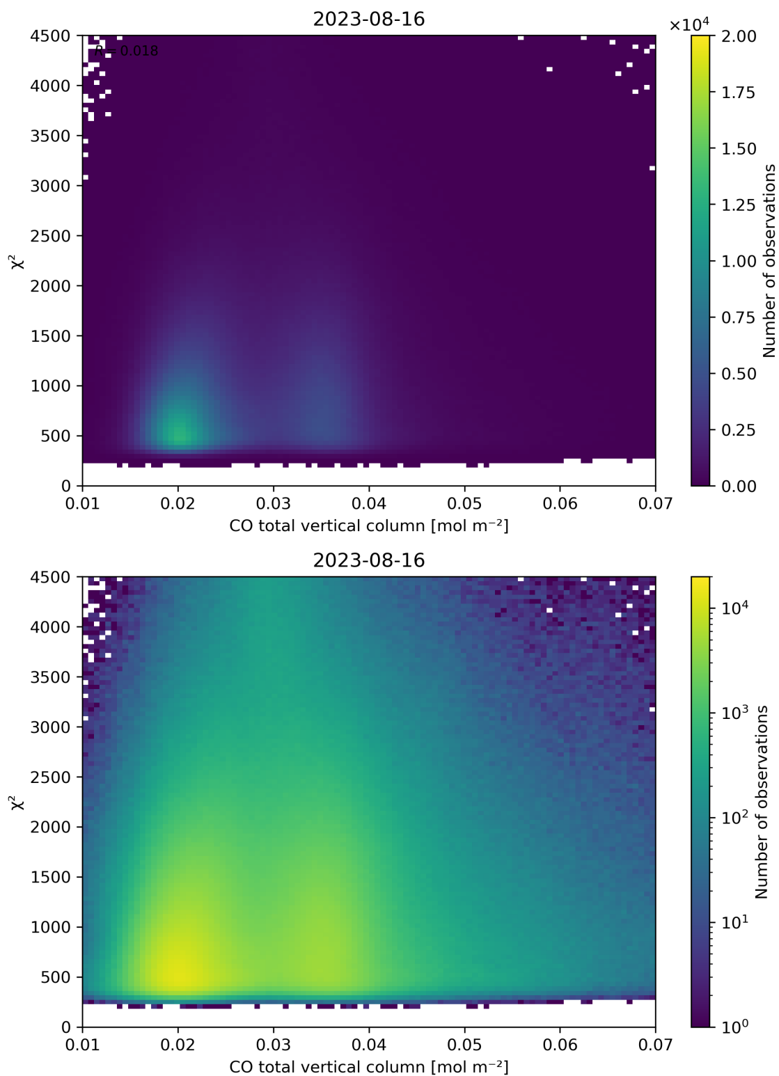
Figure 35: Scatter density plot of “CO total vertical column” against “ \chi^2 ” for 2023-08-15 to 2023-08-17.
