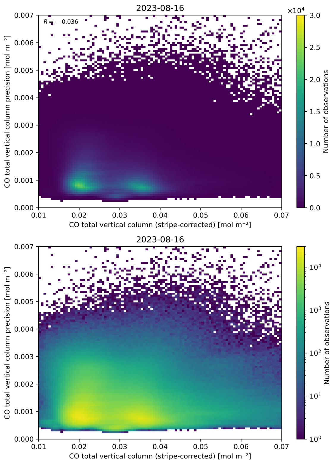
Figure 36: Scatter density plot of “CO total vertical column (stripe-corrected)” against “CO total vertical column precision” for 2023-08-15 to 2023-08-17.
