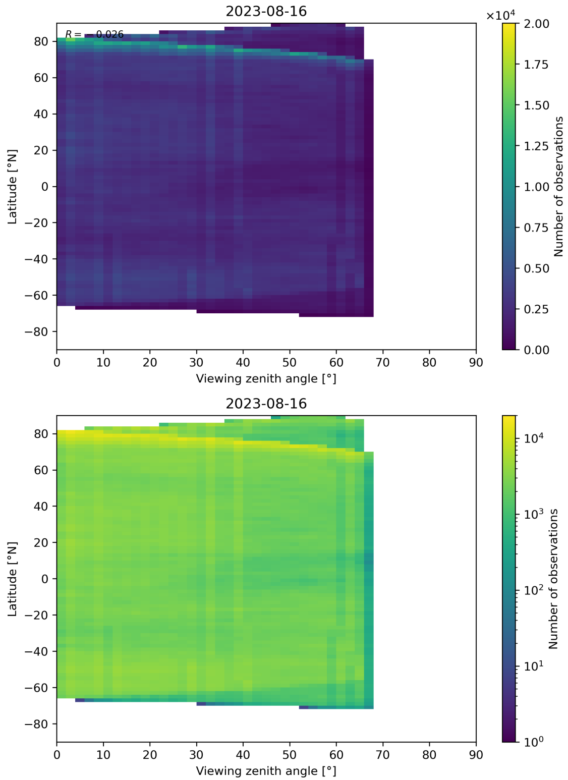
Figure 74: Scatter density plot of “Viewing zenith angle” against “Latitude” for 2023-08-15 to 2023-08-17.
