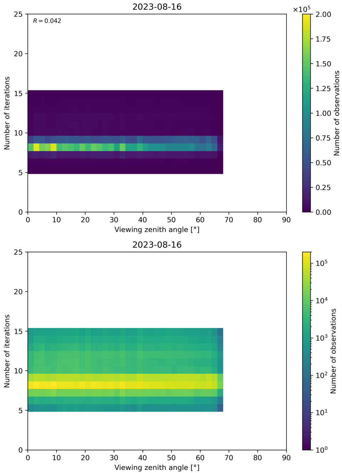
Figure 75: Scatter density plot of “Viewing zenith angle” against “Number of iterations” for 2023-08-15 to 2023-08-17.
