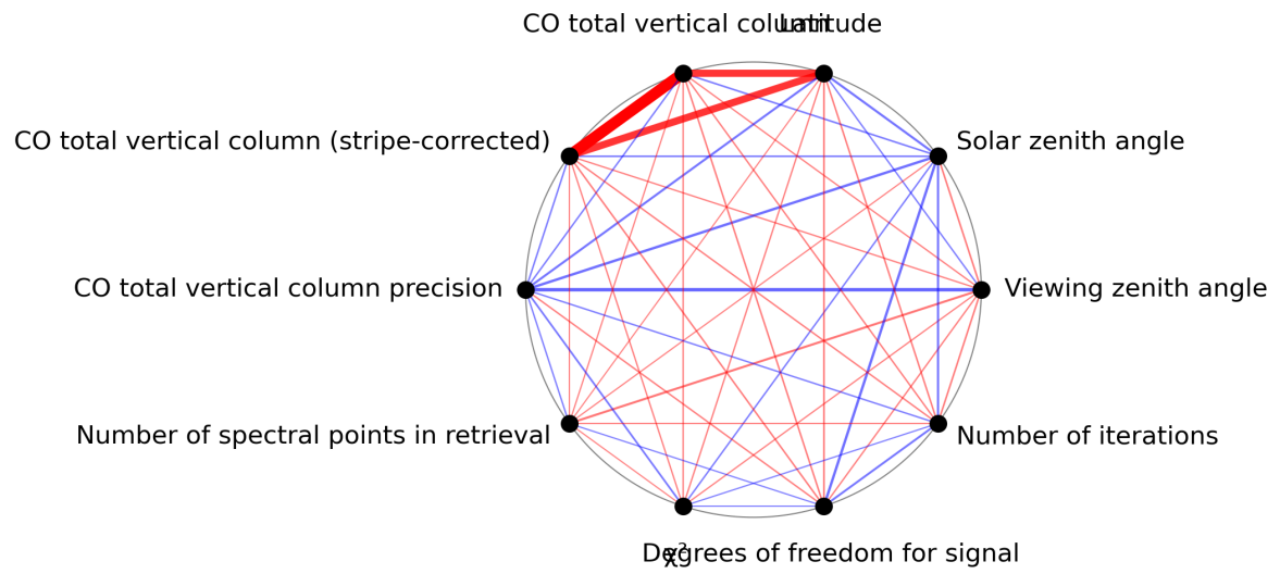
Figure 1: Map of correlation graph for 2023-08-15 to 2023-08-17.
