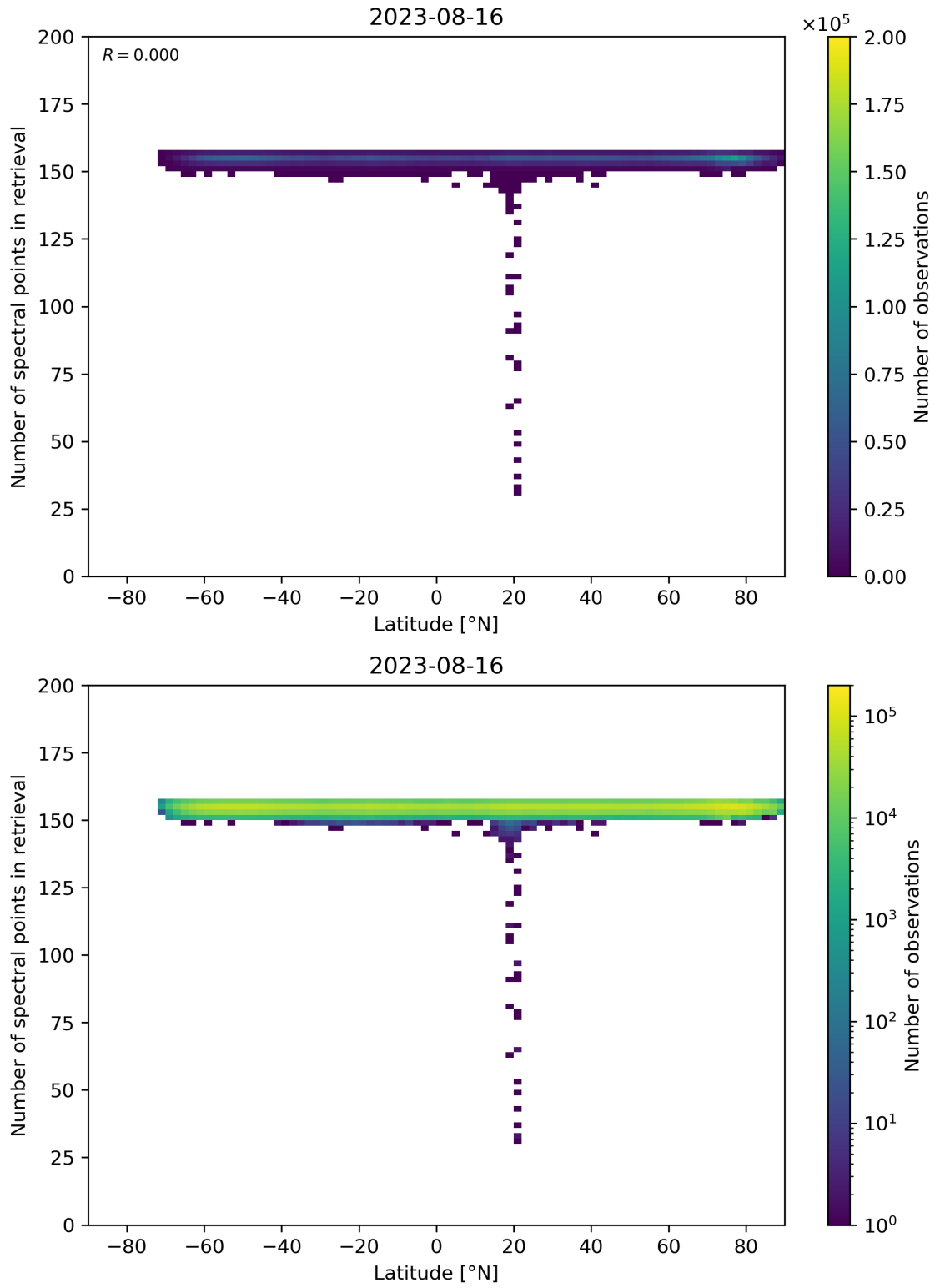
Figure 57: Scatter density plot of “Latitude” against “Number of spectral points in retrieval” for 2023-08-15 to 2023-08-17.
