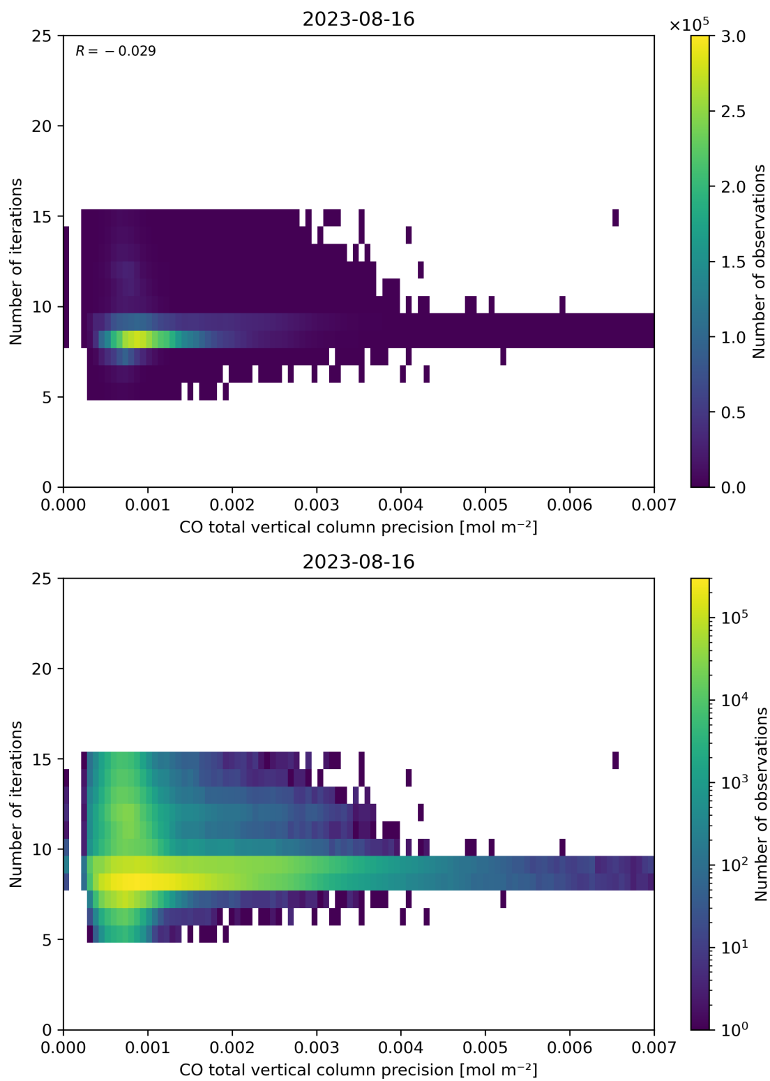
Figure 46: Scatter density plot of “CO total vertical column precision” against “Number of iterations” for 2023-08-15 to 2023-08-17.
