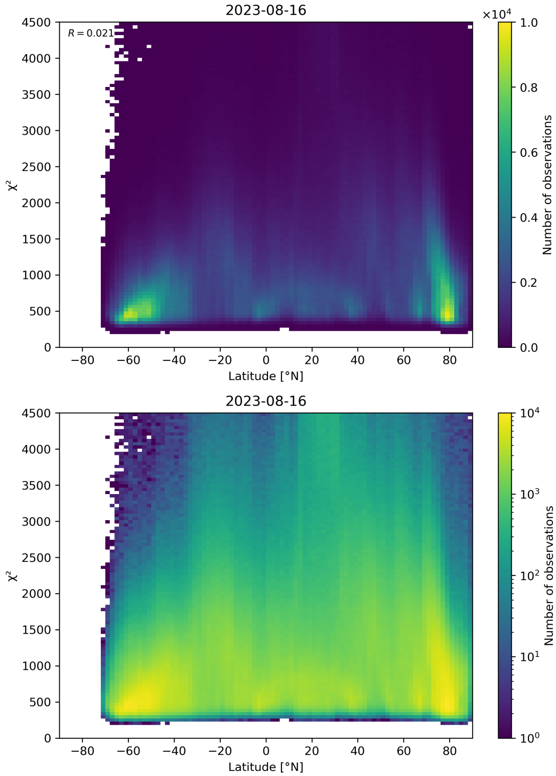
Figure 54: Scatter density plot of “Latitude” against “ \chi^2 ” for 2023-08-15 to 2023-08-17.
