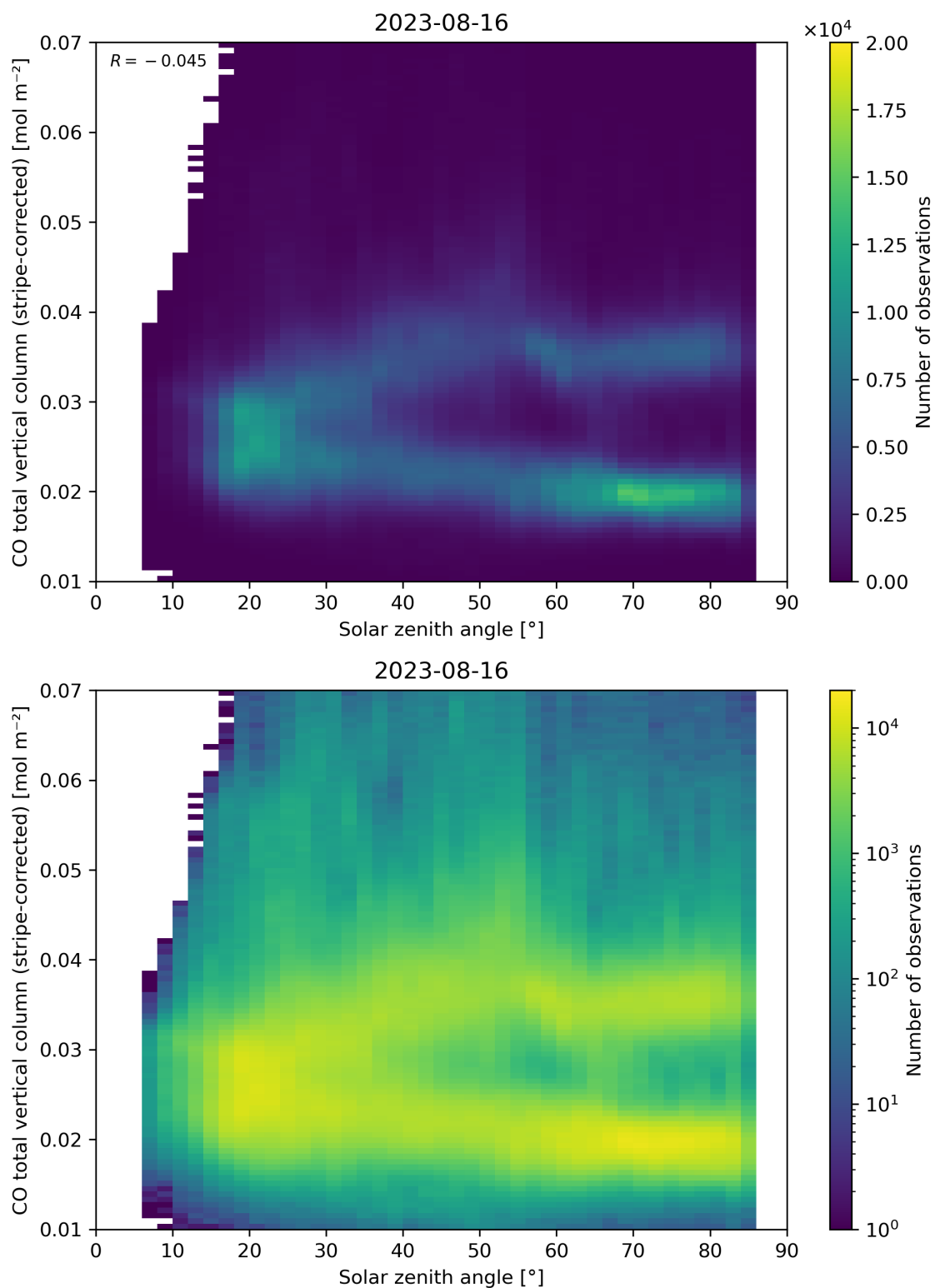
Figure 62: Scatter density plot of “Solar zenith angle” against “CO total vertical column (stripe-corrected)” for 2023-08-15 to 2023-08-17.
