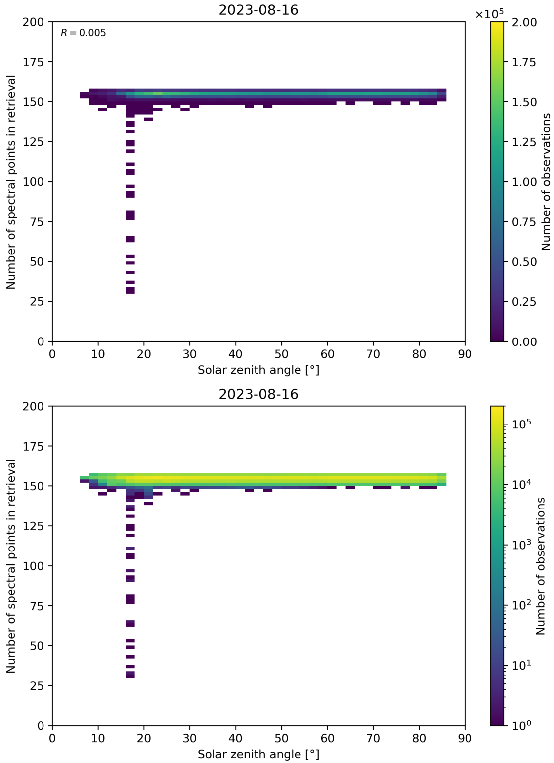
Figure 68: Scatter density plot of “Solar zenith angle” against “Number of spectral points in retrieval” for 2023-08-15 to 2023-08-17.
