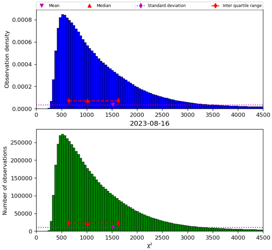
Figure 22: Histogram of “ \chi^2 ” for 2023-08-15 to 2023-08-17
