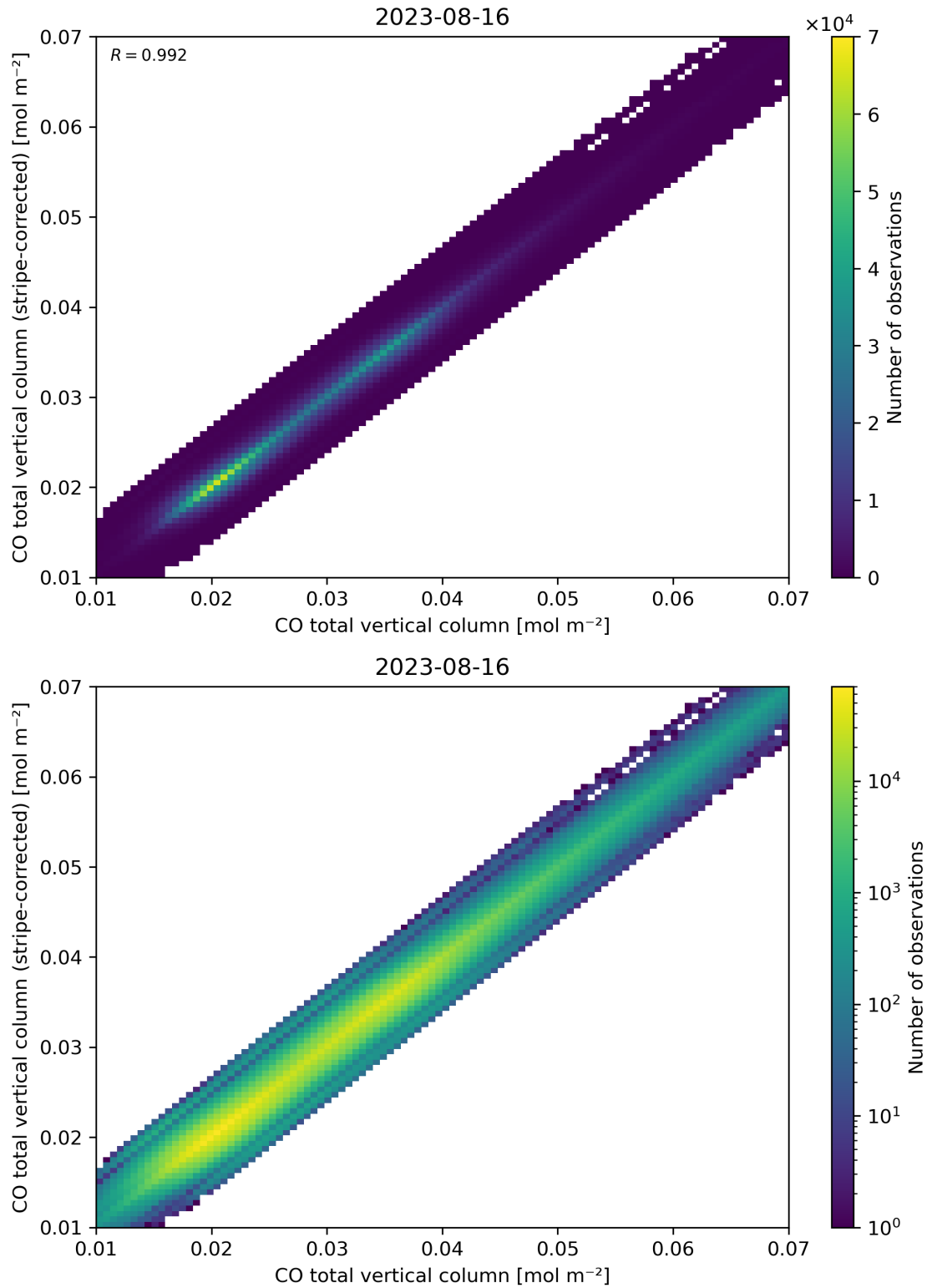
Figure 33: Scatter density plot of “CO total vertical column” against “CO total vertical column (stripe-corrected)” for 2023-08-15 to 2023-08-17.
