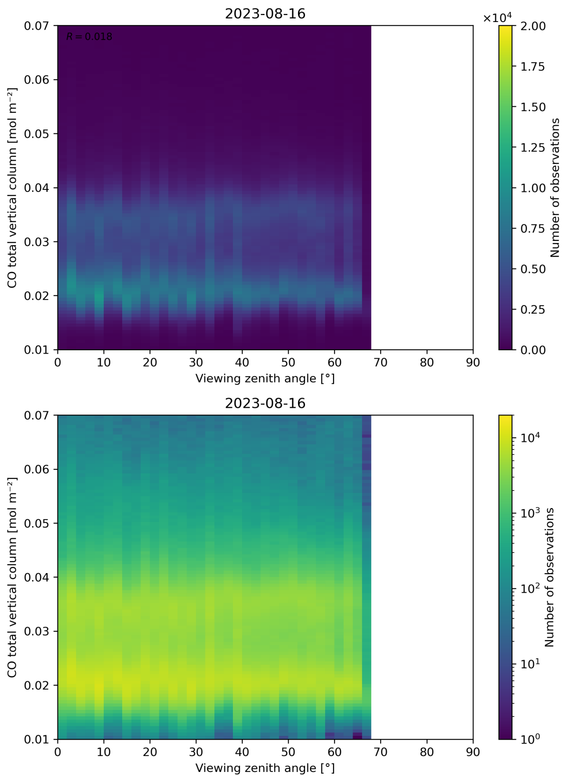
Figure 69: Scatter density plot of “Viewing zenith angle” against “CO total vertical column” for 2023-08-15 to 2023-08-17.
