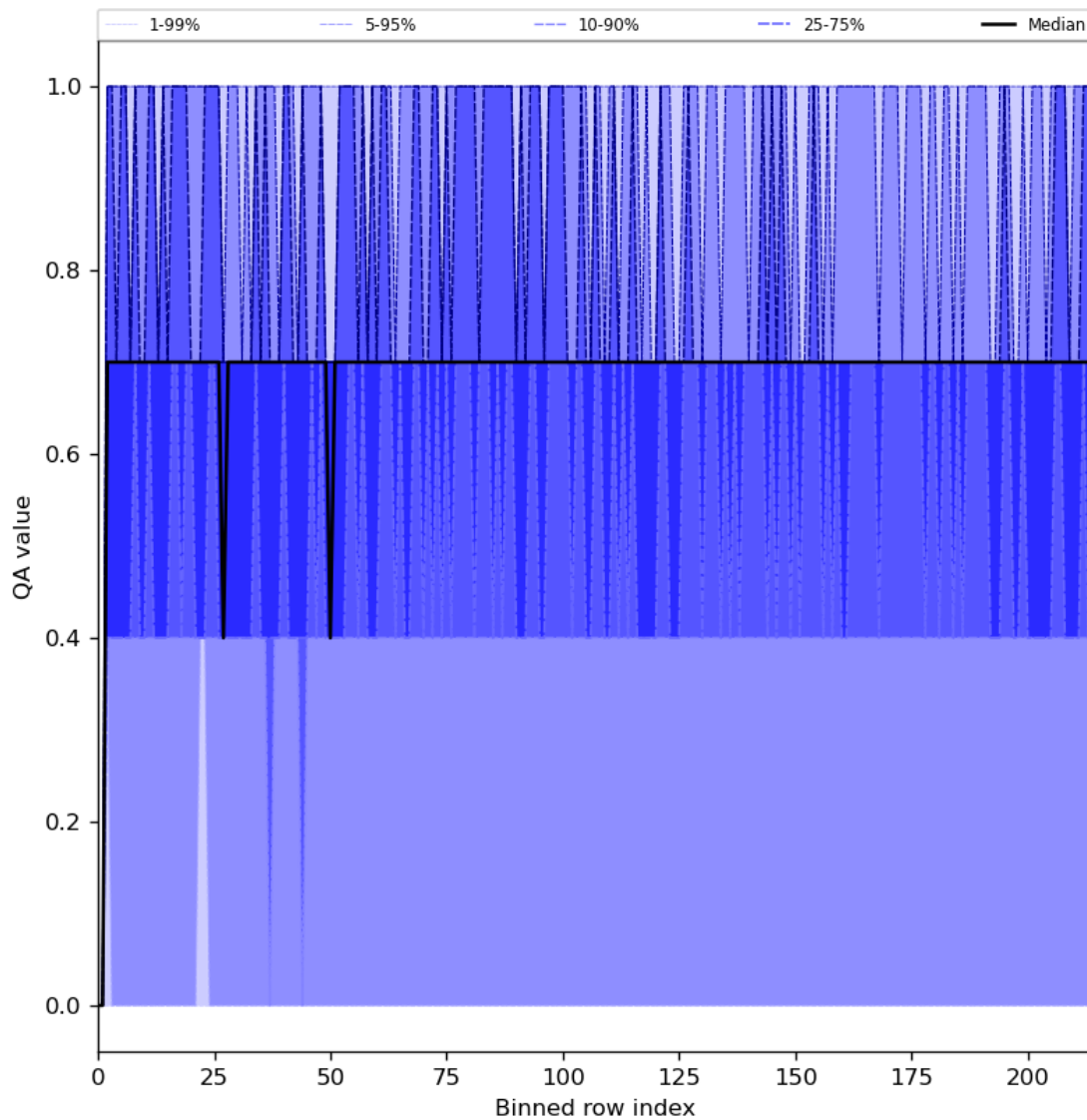
Figure 25: Along track statistics of “QA value” for 2023-08-15 to 2023-08-17
