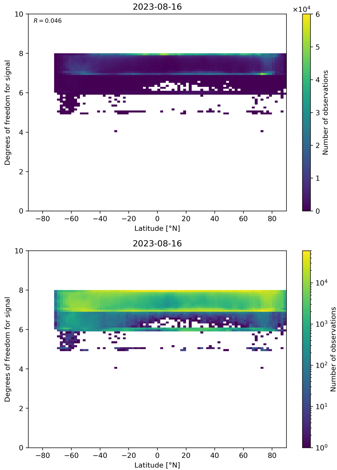
Figure 55: Scatter density plot of “Latitude” against “Degrees of freedom for signal” for 2023-08-15 to 2023-08-17.
