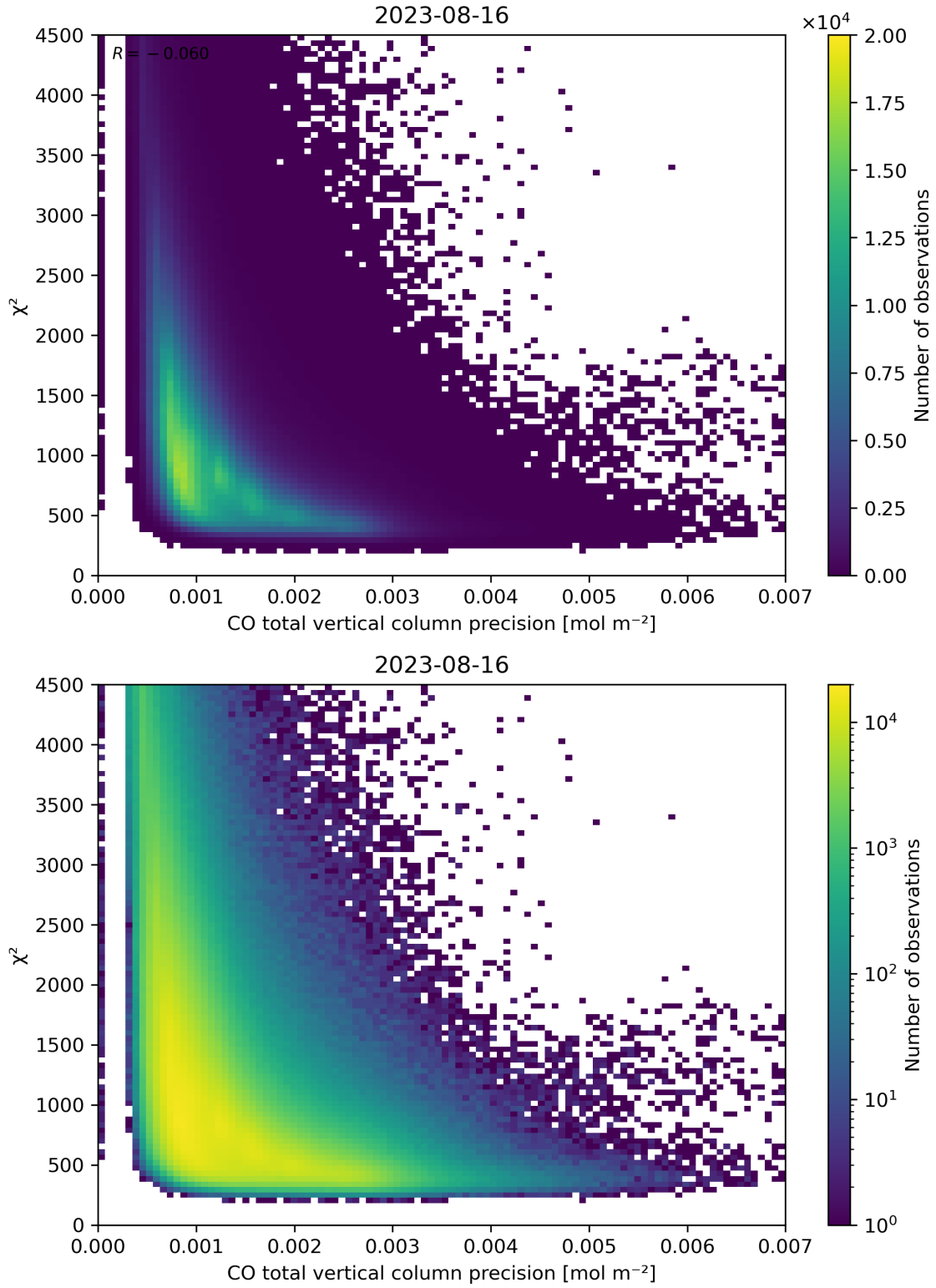
Figure 44: Scatter density plot of “CO total vertical column precision” against “ \chi^2 ” for 2023-08-15 to 2023-08-17.
