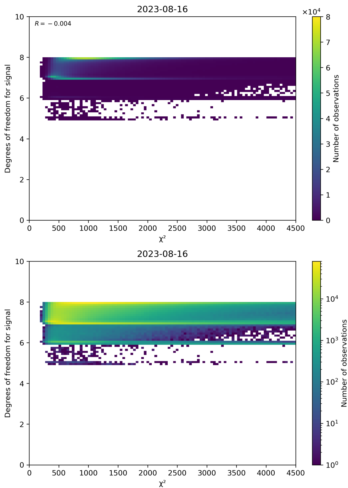
Figure 48: Scatter density plot of “ \chi^2 ” against “Degrees of freedom for signal” for 2023-08-15 to 2023-08-17.
