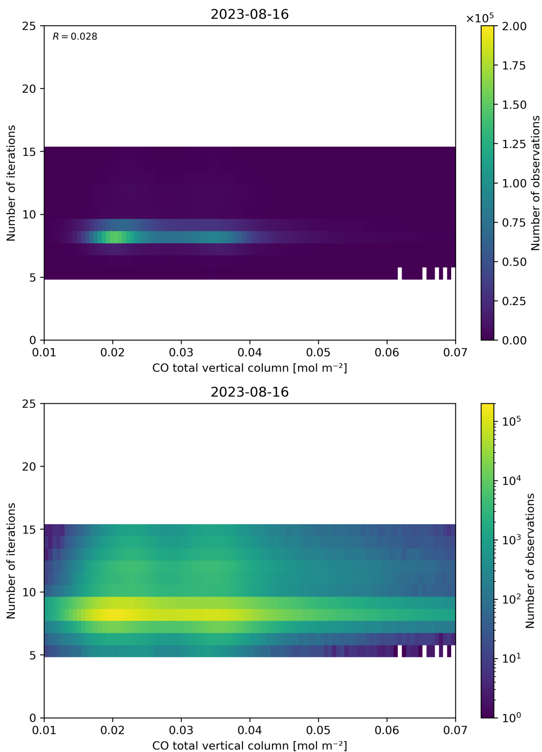
Figure 42: Scatter density plot of “CO total vertical column” against “Number of iterations” for 2023-08-15 to 2023-08-17.
