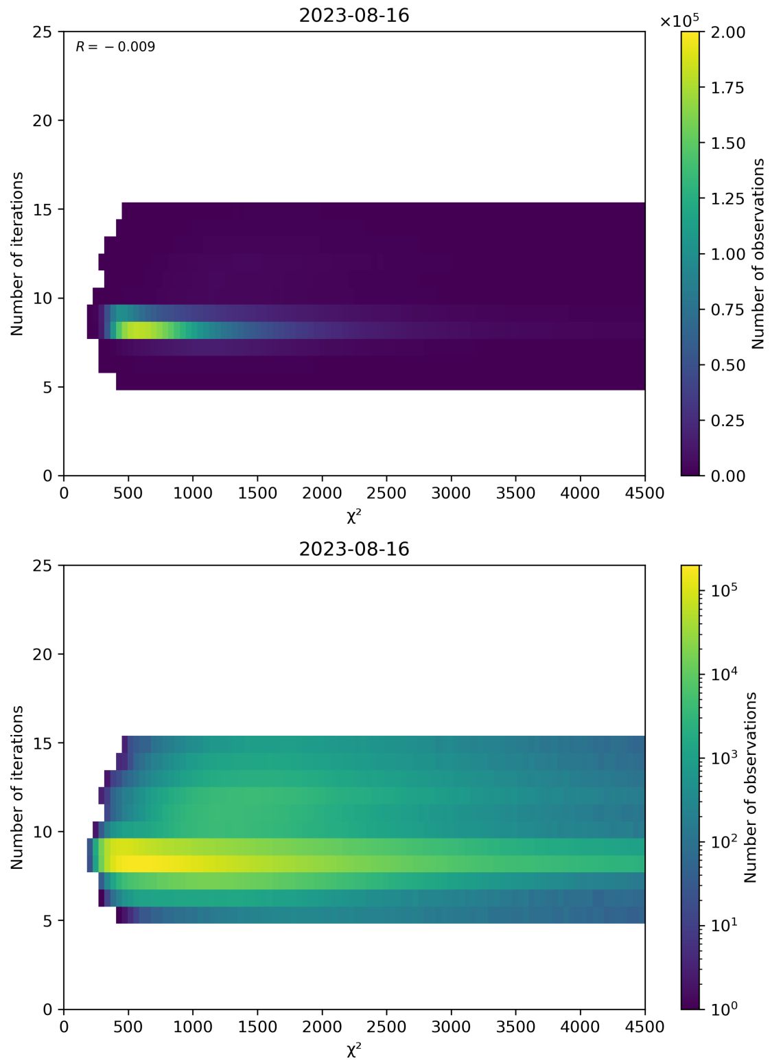
Figure 49: Scatter density plot of “ \chi^2 ” against “Number of iterations” for 2023-08-15 to 2023-08-17.
