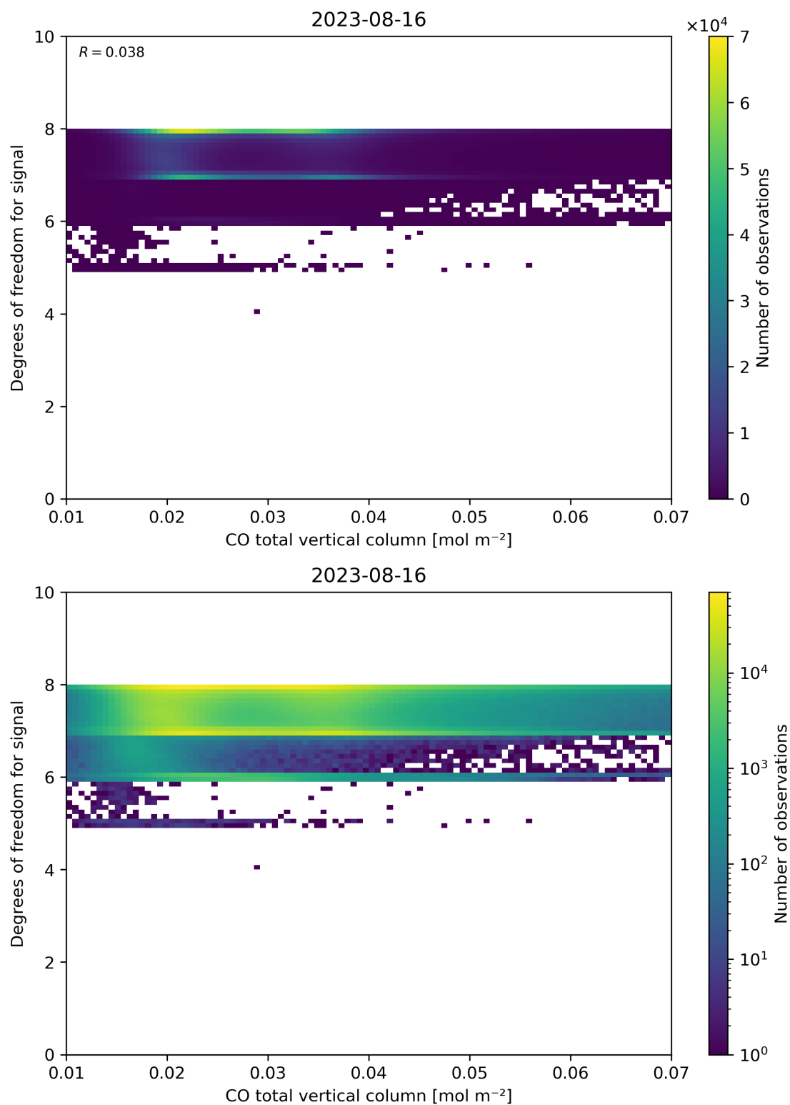
Figure 41: Scatter density plot of “CO total vertical column” against “Degrees of freedom for signal” for 2023-08-15 to 2023-08-17.
