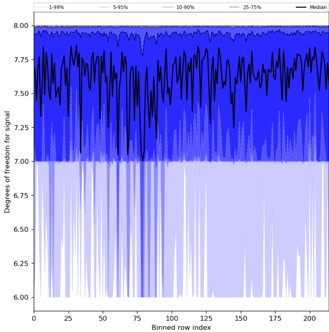
Figure 31: Along track statistics of “Degrees of freedom for signal” for 2023-08-15 to 2023-08-17
