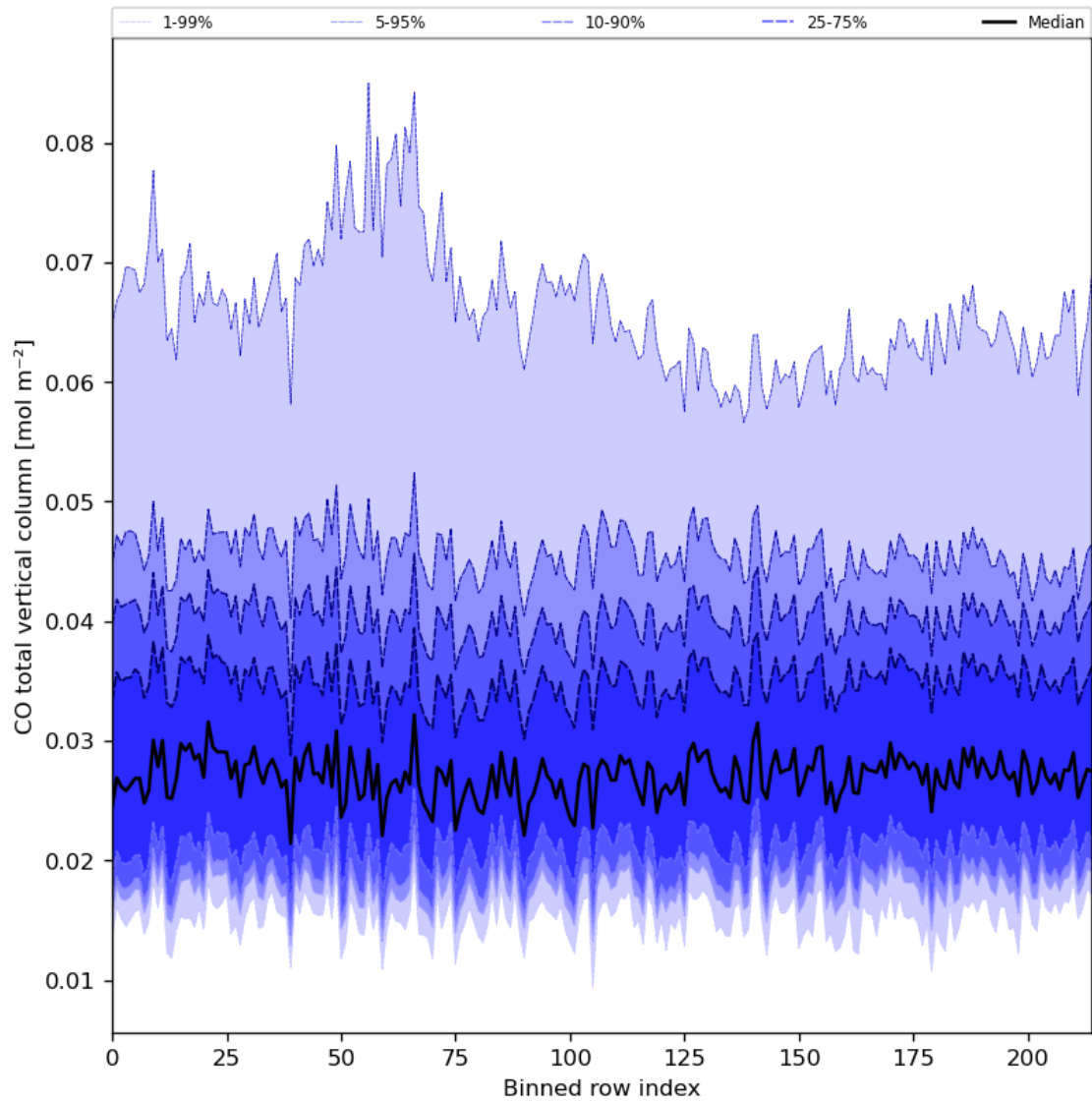
Figure 26: Along track statistics of “CO total vertical column” for 2023-08-15 to 2023-08-17
