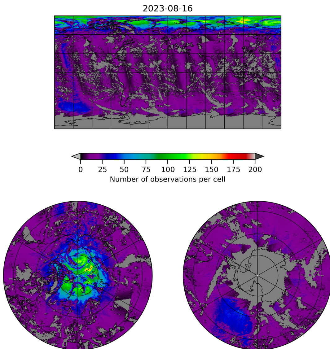
Figure 8: Map of the number of observations for 2023-08-15 to 2023-08-17
