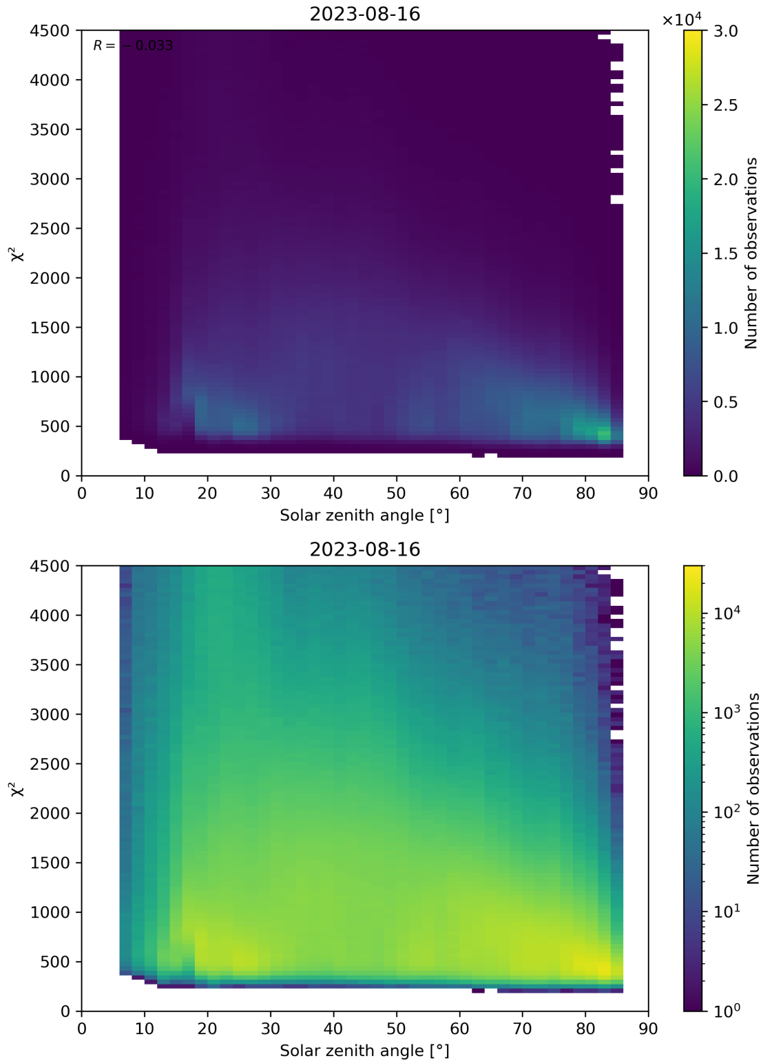
Figure 64: Scatter density plot of “Solar zenith angle” against “ \chi^2 ” for 2023-08-15 to 2023-08-17.
