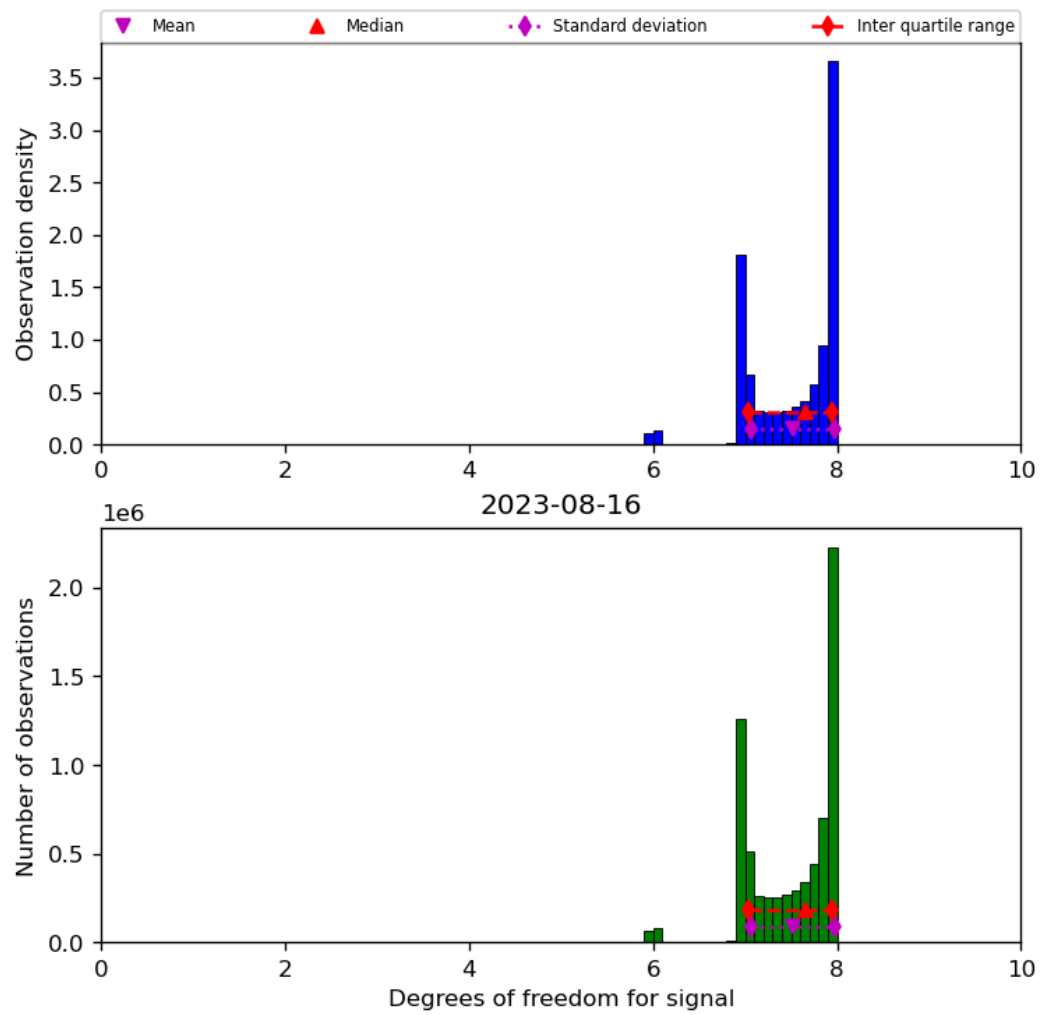
Figure 23: Histogram of “Degrees of freedom for signal” for 2023-08-15 to 2023-08-17
