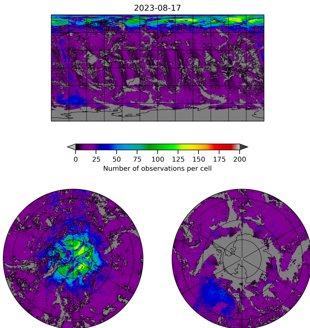
Figure 8: Map of the number of observations for 2023-08-16 to 2023-08-18
