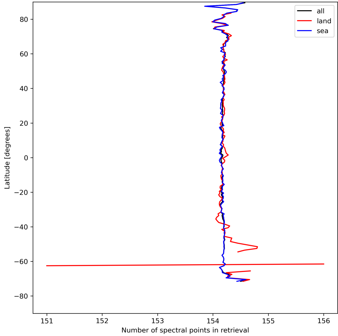
Figure 13: Zonal average of “Number of spectral points in retrieval” for 2023-08-17 to 2023-08-19.
