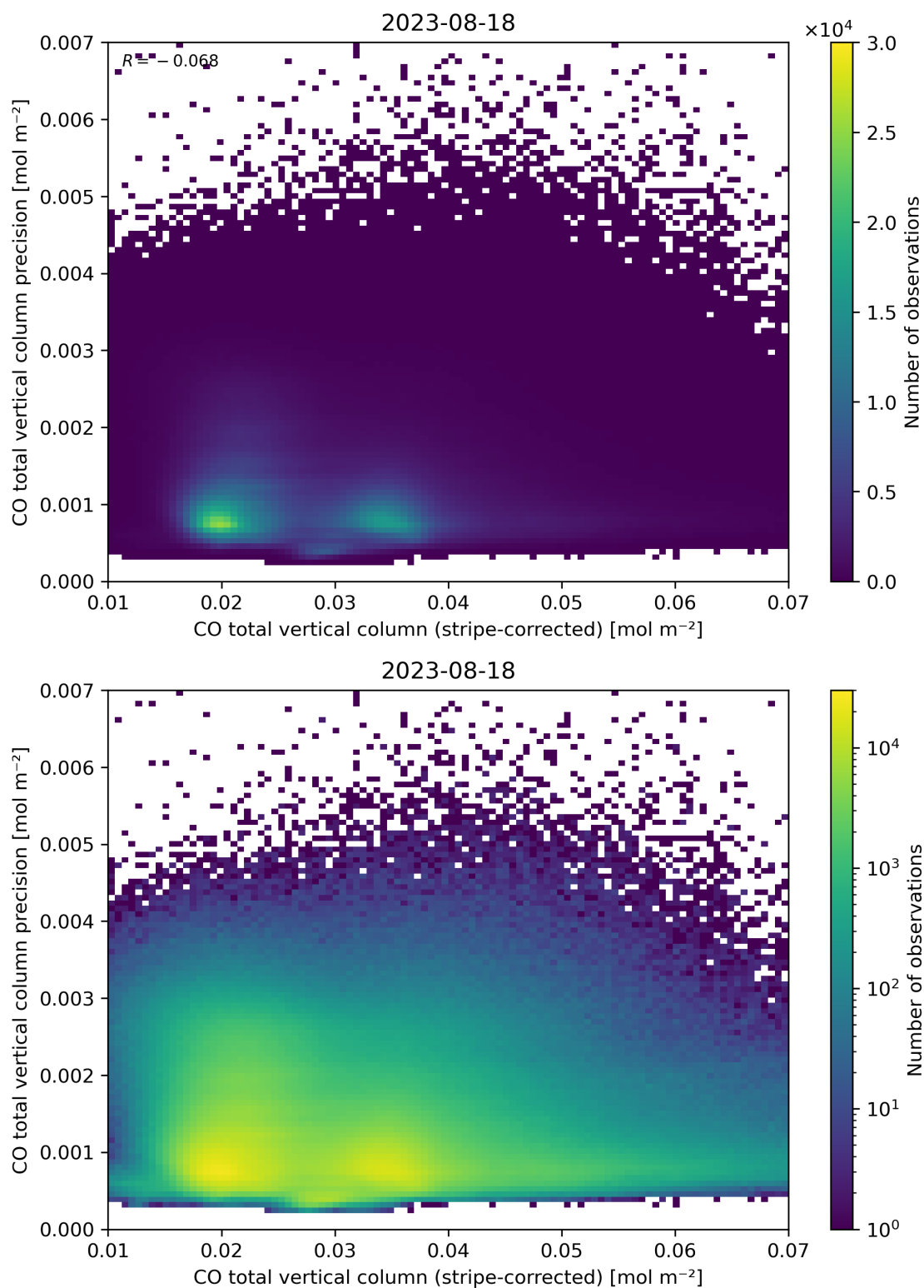
Figure 36: Scatter density plot of “CO total vertical column (stripe-corrected)” against “CO total vertical column precision” for 2023-08-17 to 2023-08-19.
