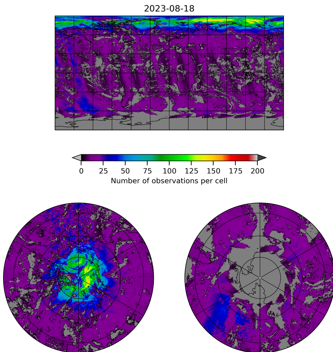
Figure 8: Map of the number of observations for 2023-08-17 to 2023-08-19
