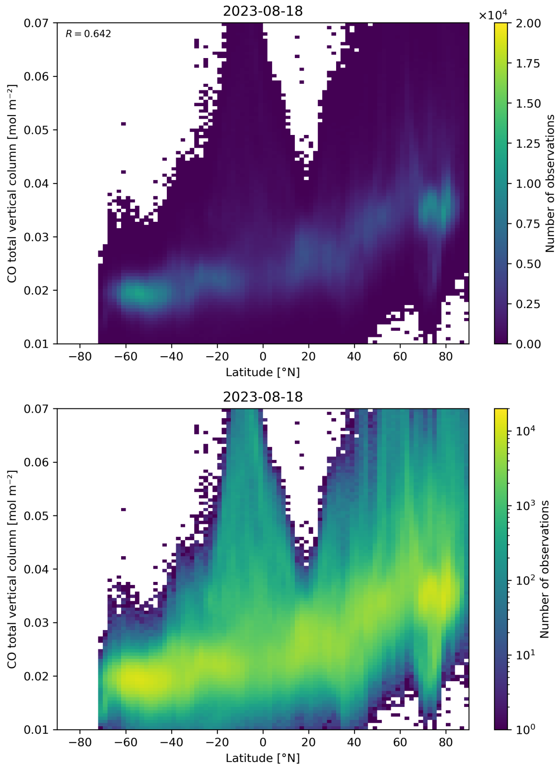
Figure 51: Scatter density plot of “Latitude” against “CO total vertical column” for 2023-08-17 to 2023-08-19.
