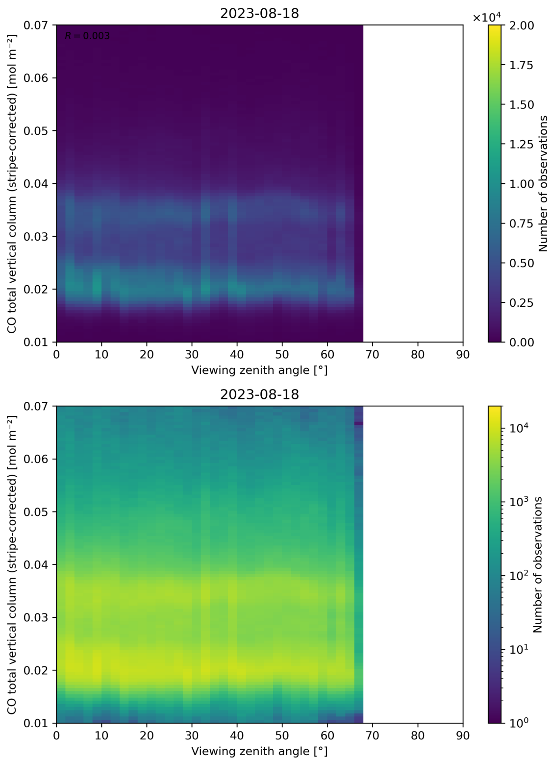
Figure 70: Scatter density plot of “Viewing zenith angle” against “CO total vertical column (stripe-corrected)” for 2023-08-17 to 2023-08-19.
