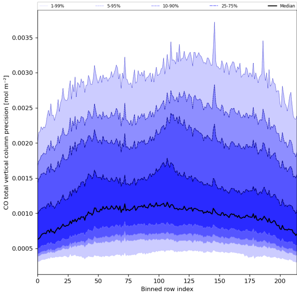
Figure 28: Along track statistics of “CO total vertical column precision” for 2023-08-17 to 2023-08-19
