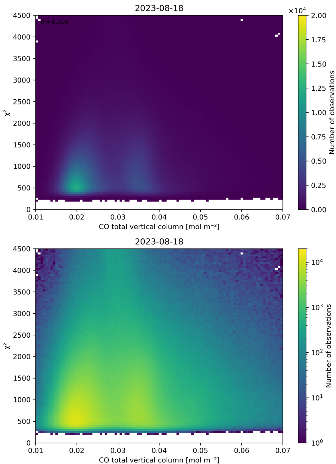
Figure 35: Scatter density plot of “CO total vertical column” against “ \chi^2 ” for 2023-08-17 to 2023-08-19.
