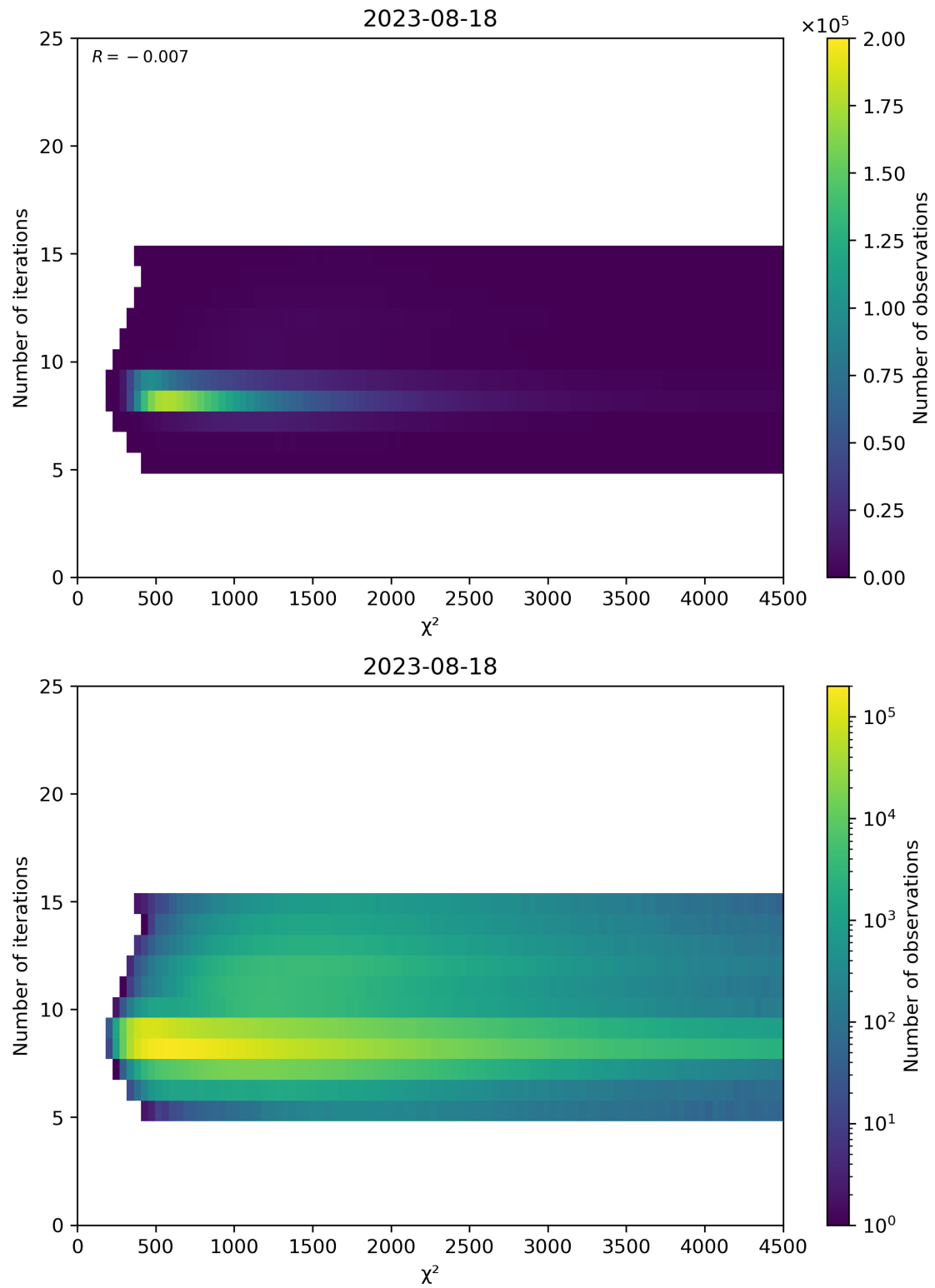
Figure 49: Scatter density plot of “ \chi^2 ” against “Number of iterations” for 2023-08-17 to 2023-08-19.
