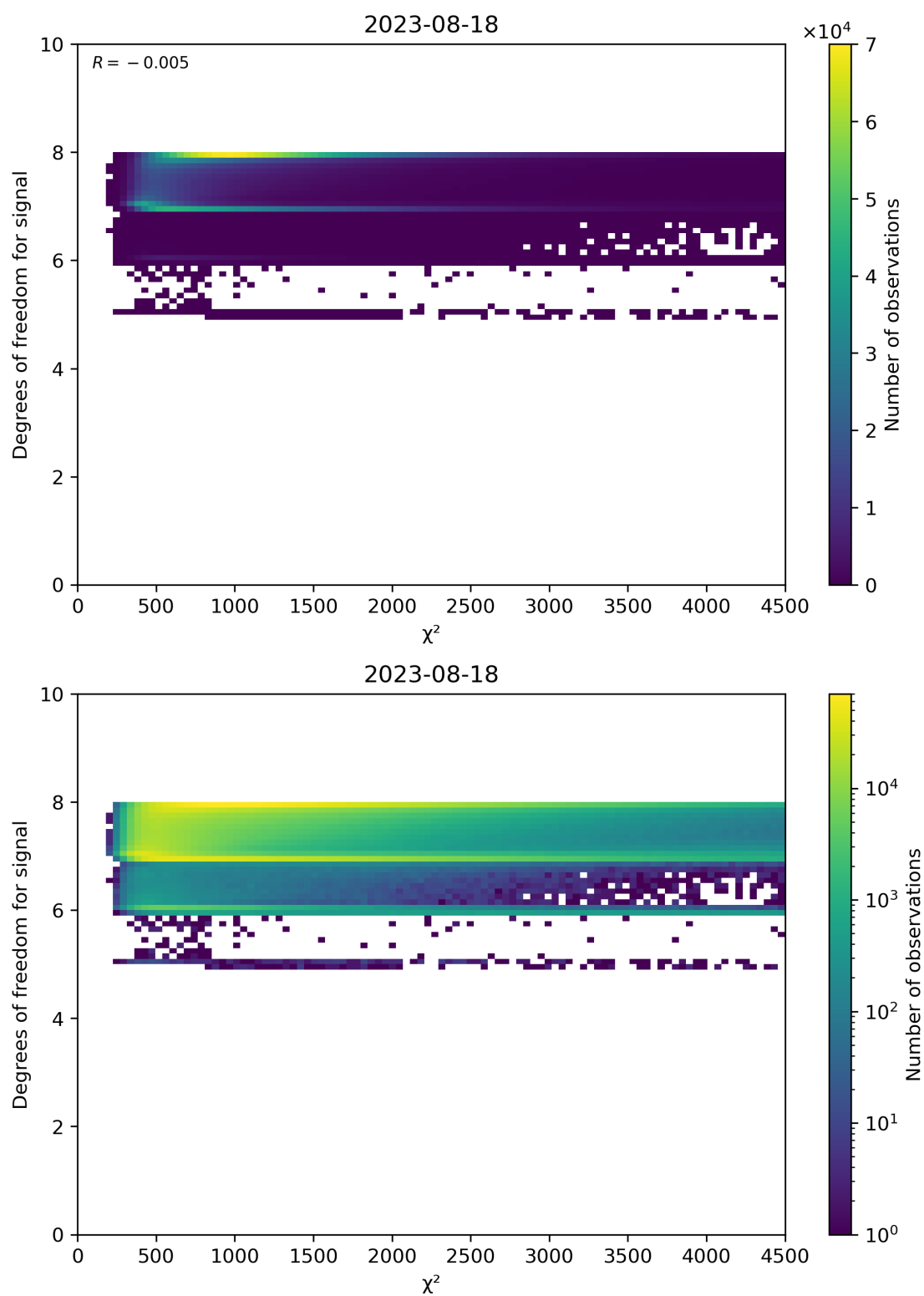
Figure 48: Scatter density plot of " \chi^2 " against "Degrees of freedom for signal" for 2023-08-17 to 2023-08-19.
