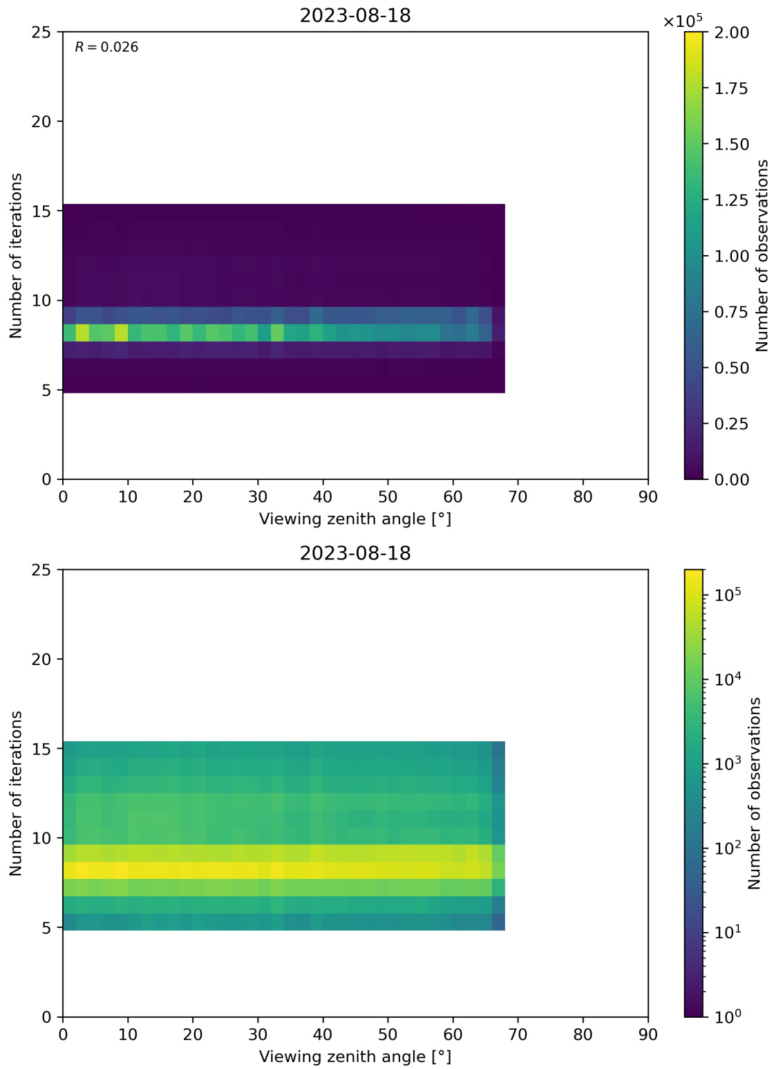
Figure 75: Scatter density plot of “Viewing zenith angle” against “Number of iterations” for 2023-08-17 to 2023-08-19.
