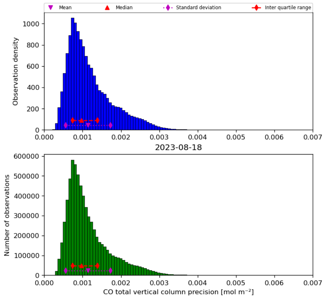
Figure 20: Histogram of “CO total vertical column precision” for 2023-08-17 to 2023-08-19
