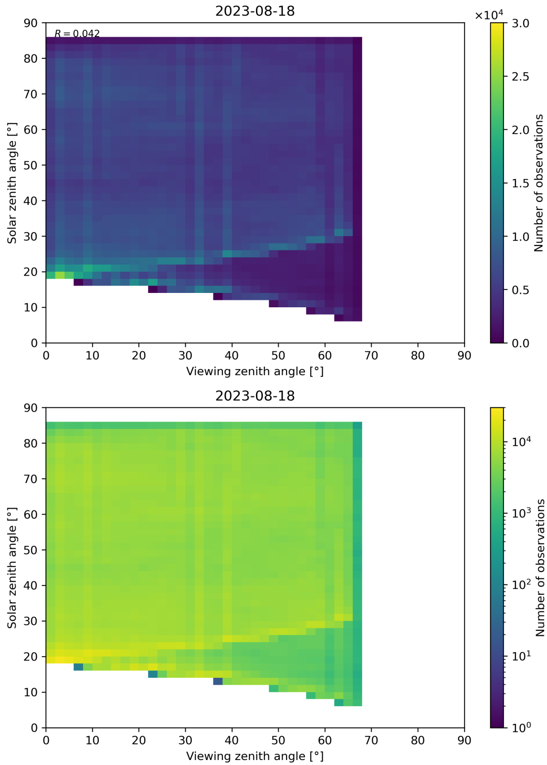
Figure 77: Scatter density plot of “Viewing zenith angle” against “Solar zenith angle” for 2023-08-17 to 2023-08-19.
