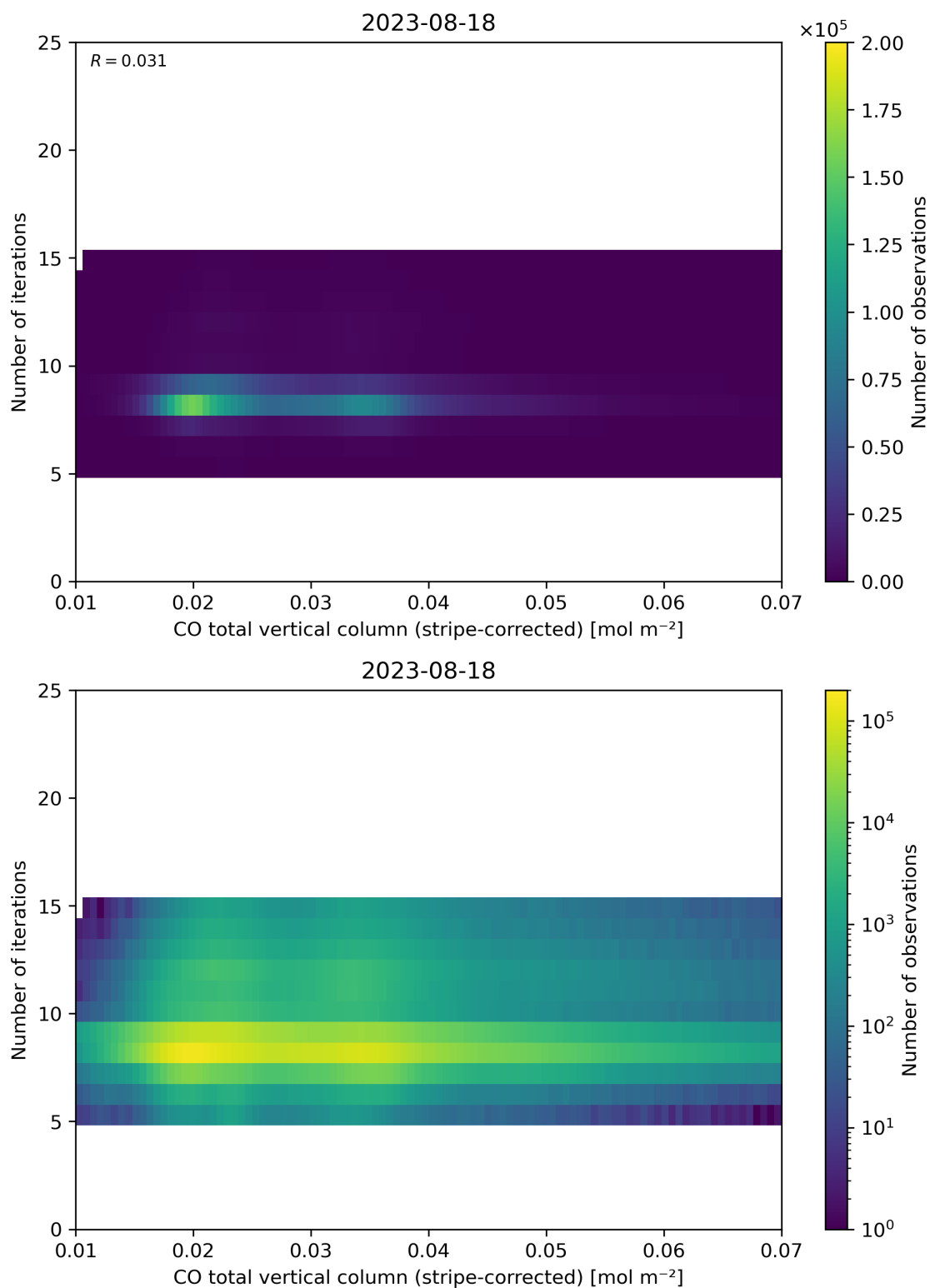
Figure 39: Scatter density plot of “CO total vertical column (stripe-corrected)” against “Number of iterations” for 2023-08-17 to 2023-08-19.
