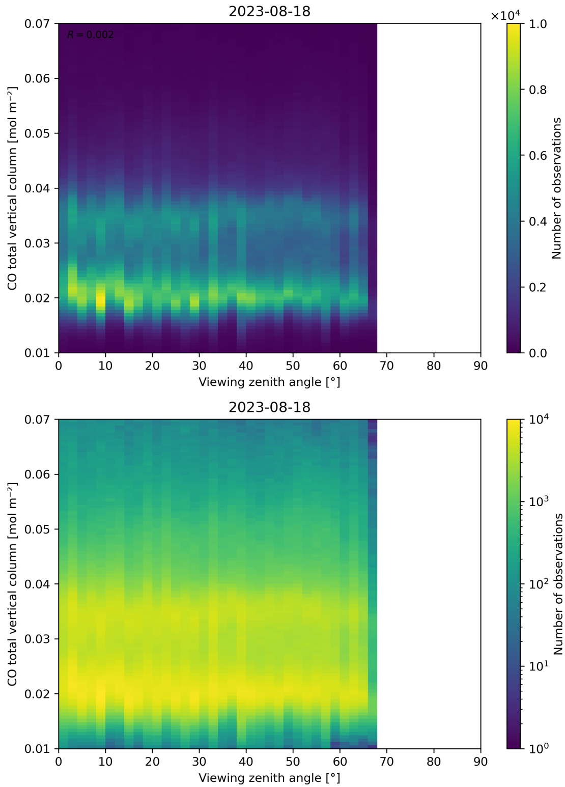
Figure 69: Scatter density plot of “Viewing zenith angle” against “CO total vertical column” for 2023-08-17 to 2023-08-19.
