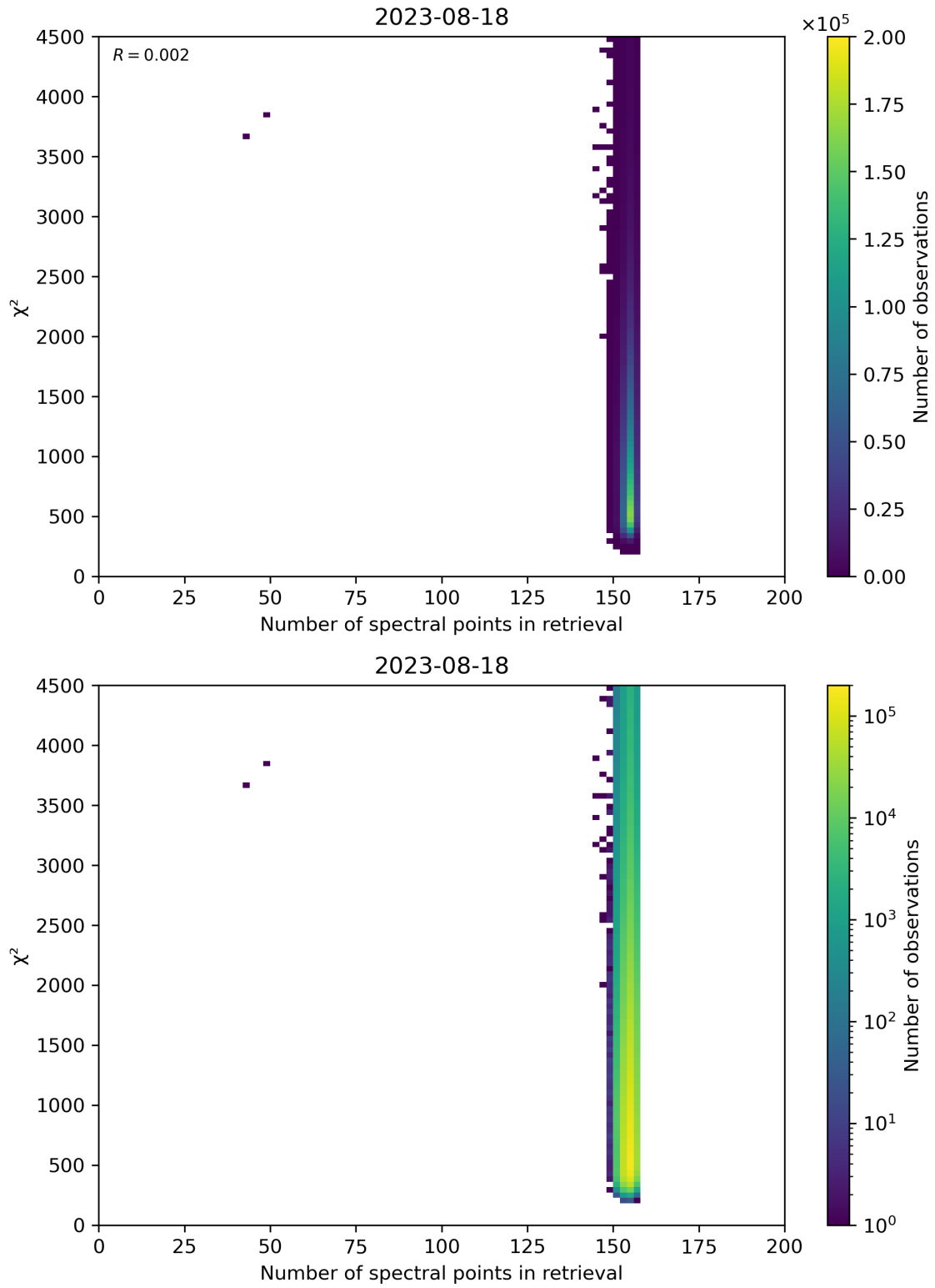
Figure 58: Scatter density plot of “Number of spectral points in retrieval” against “ \chi^2 ” for 2023-08-17 to 2023-08-19.
