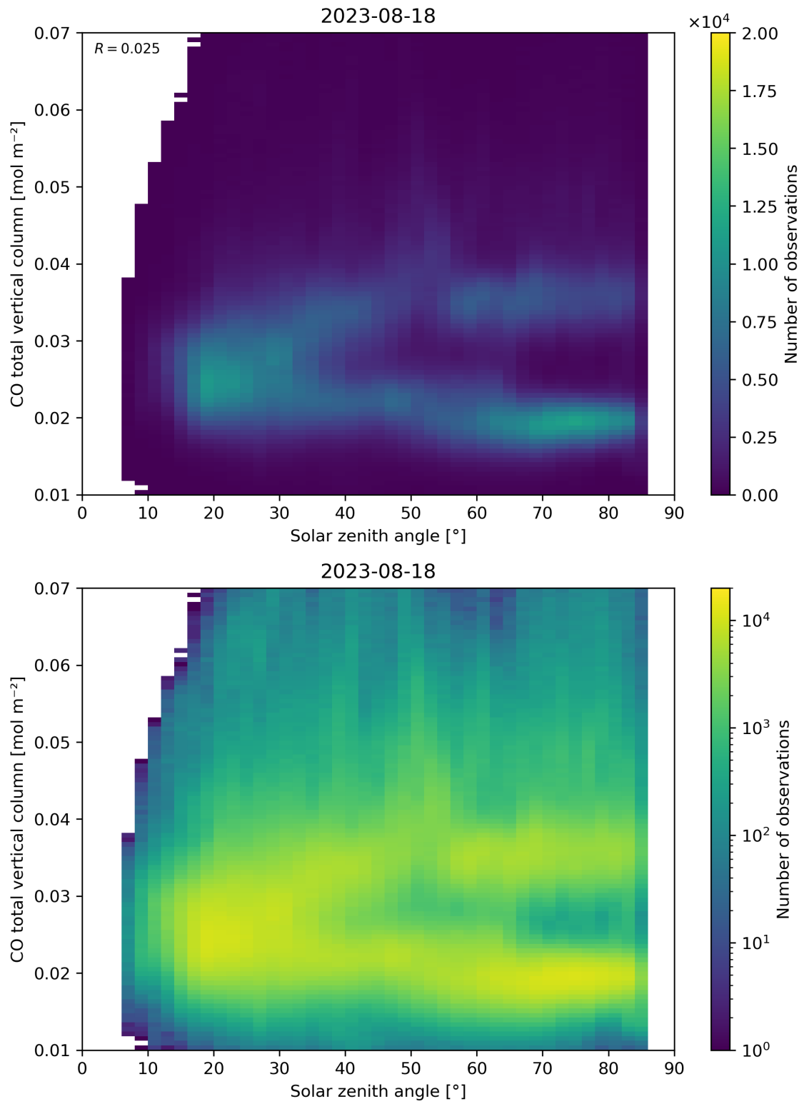
Figure 61: Scatter density plot of “Solar zenith angle” against “CO total vertical column” for 2023-08-17 to 2023-08-19.
