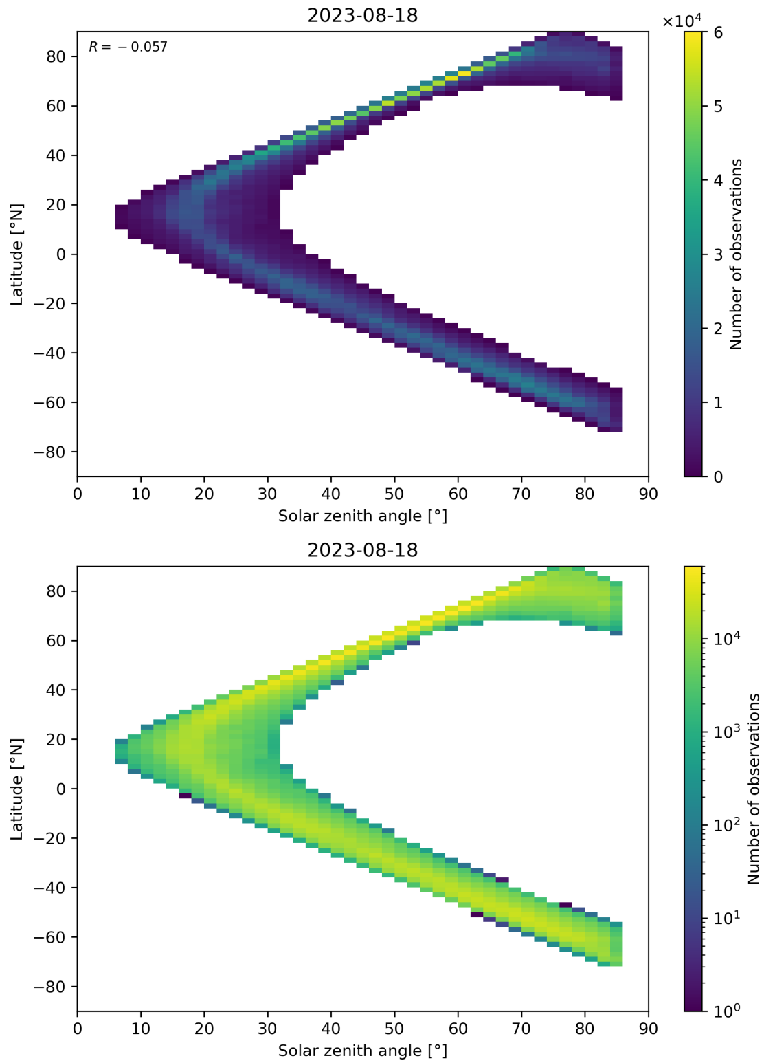
Figure 66: Scatter density plot of “Solar zenith angle” against “Latitude” for 2023-08-17 to 2023-08-19.
