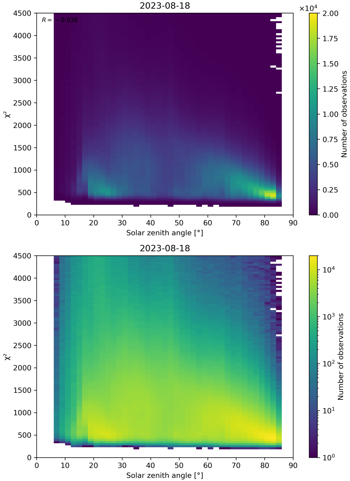
Figure 64: Scatter density plot of “Solar zenith angle” against “ \chi^2 ” for 2023-08-17 to 2023-08-19.
