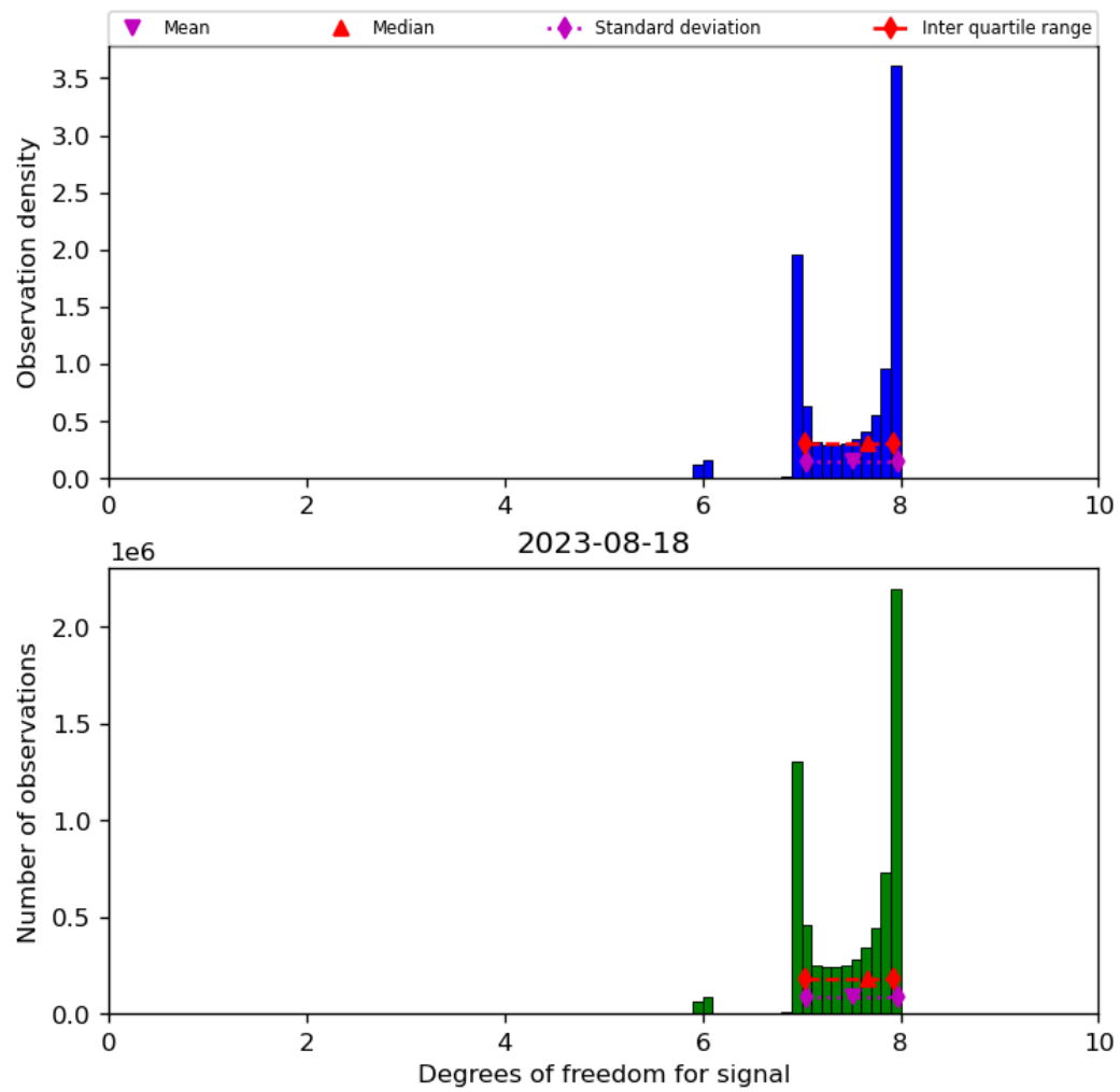
Figure 23: Histogram of “Degrees of freedom for signal” for 2023-08-17 to 2023-08-19
