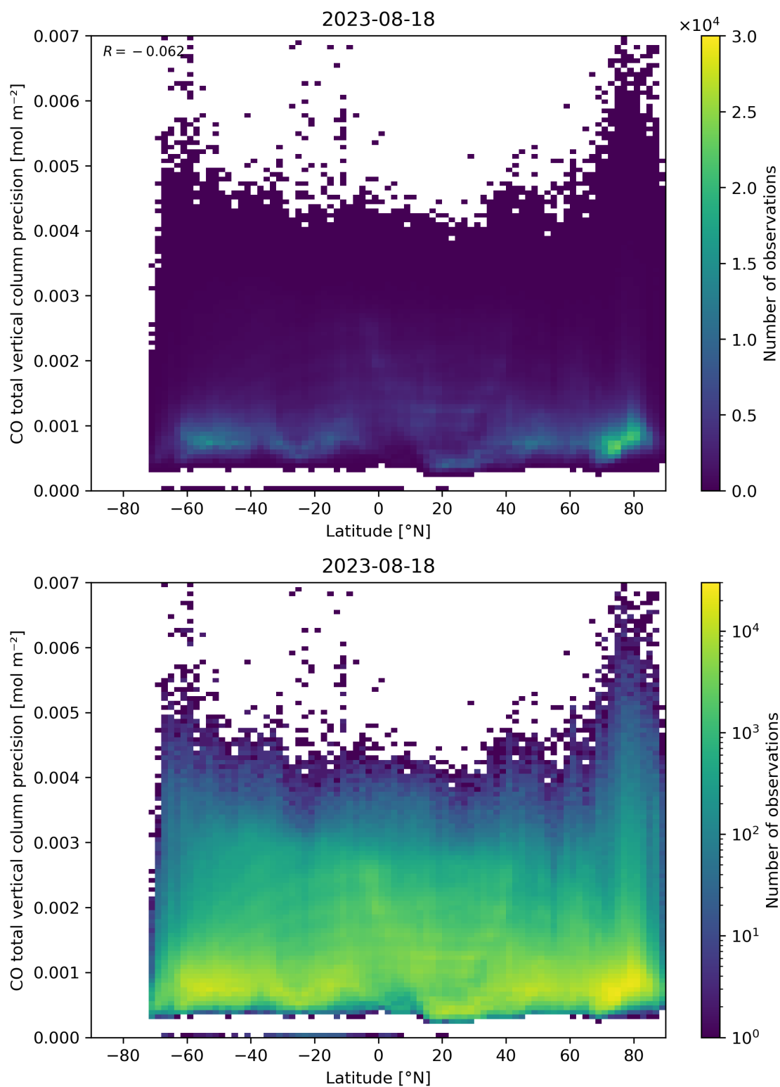
Figure 53: Scatter density plot of “Latitude” against “CO total vertical column precision” for 2023-08-17 to 2023-08-19.
