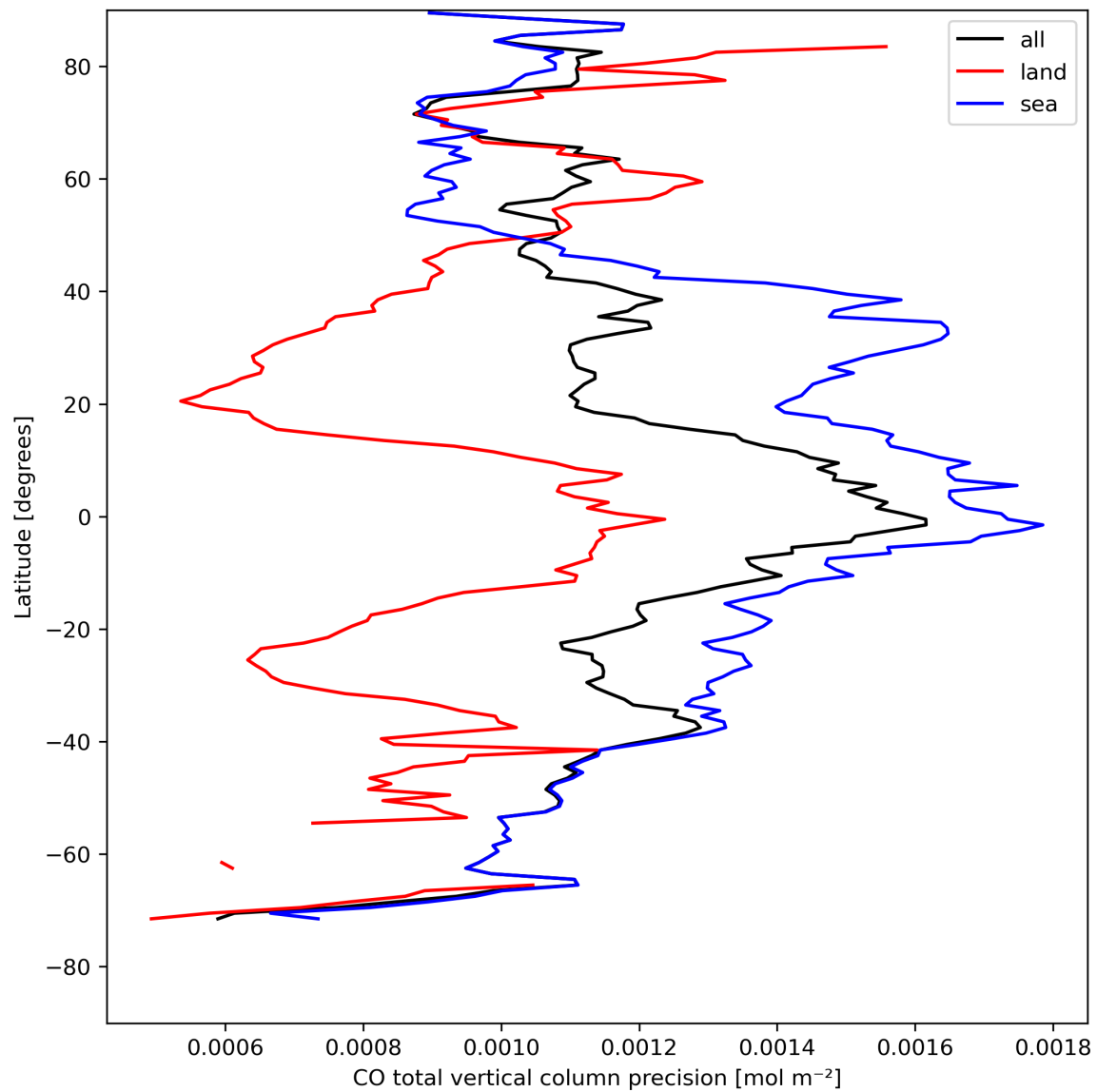
Figure 12: Zonal average of “CO total vertical column precision” for 2023-08-17 to 2023-08-19.
