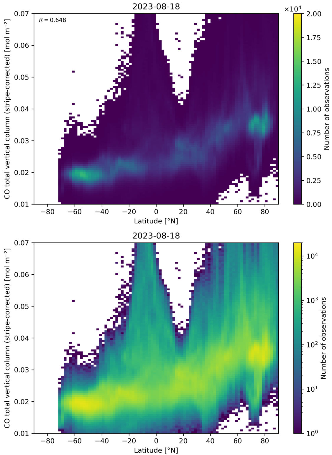
Figure 52: Scatter density plot of “Latitude” against “CO total vertical column (stripe-corrected)” for 2023-08-17 to 2023-08-19.
