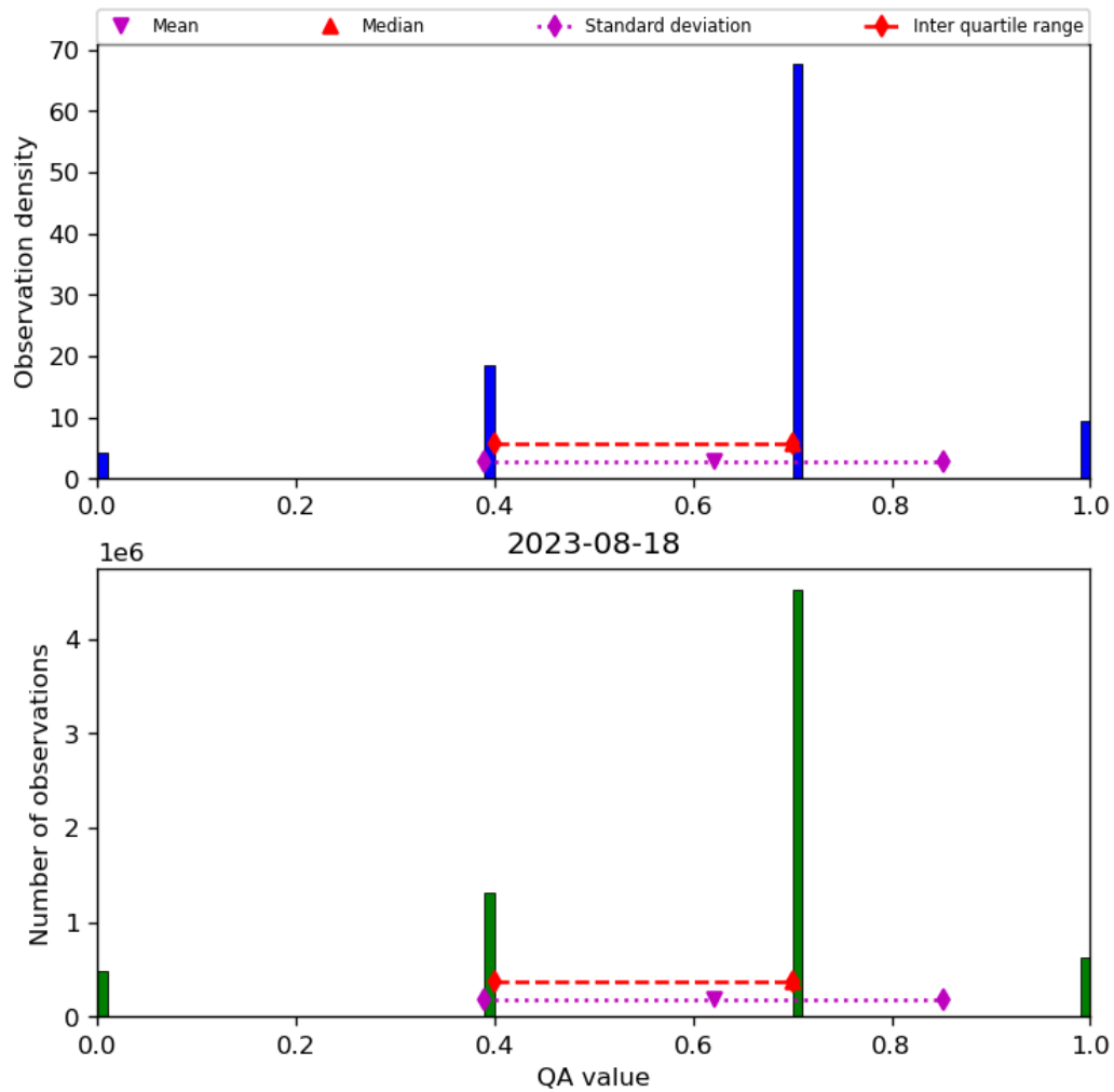
Figure 17: Histogram of “QA value” for 2023-08-17 to 2023-08-19
