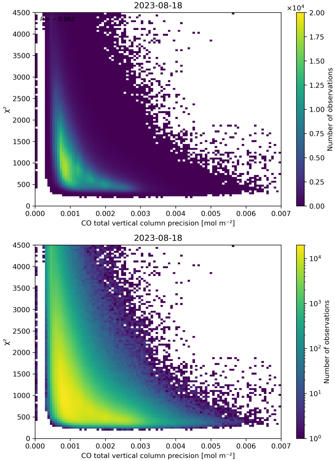
Figure 44: Scatter density plot of “CO total vertical column precision” against “ \chi^2 ” for 2023-08-17 to 2023-08-19.
