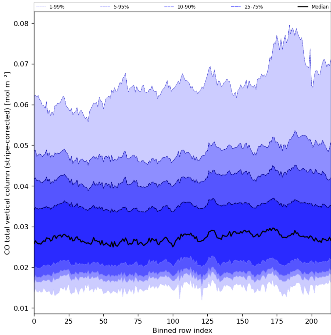
Figure 27: Along track statistics of “CO total vertical column (stripe-corrected)” for 2023-08-17 to 2023-08-19
