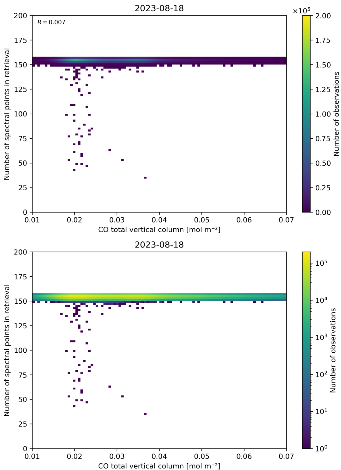
Figure 43: Scatter density plot of “CO total vertical column” against “Number of spectral points in retrieval” for 2023-08-17 to 2023-08-19.
