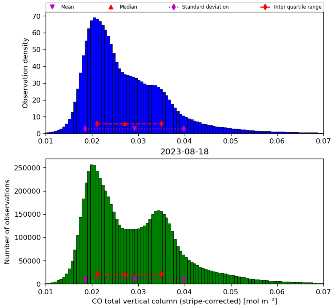
Figure 19: Histogram of “CO total vertical column (stripe-corrected)” for 2023-08-17 to 2023-08-19
