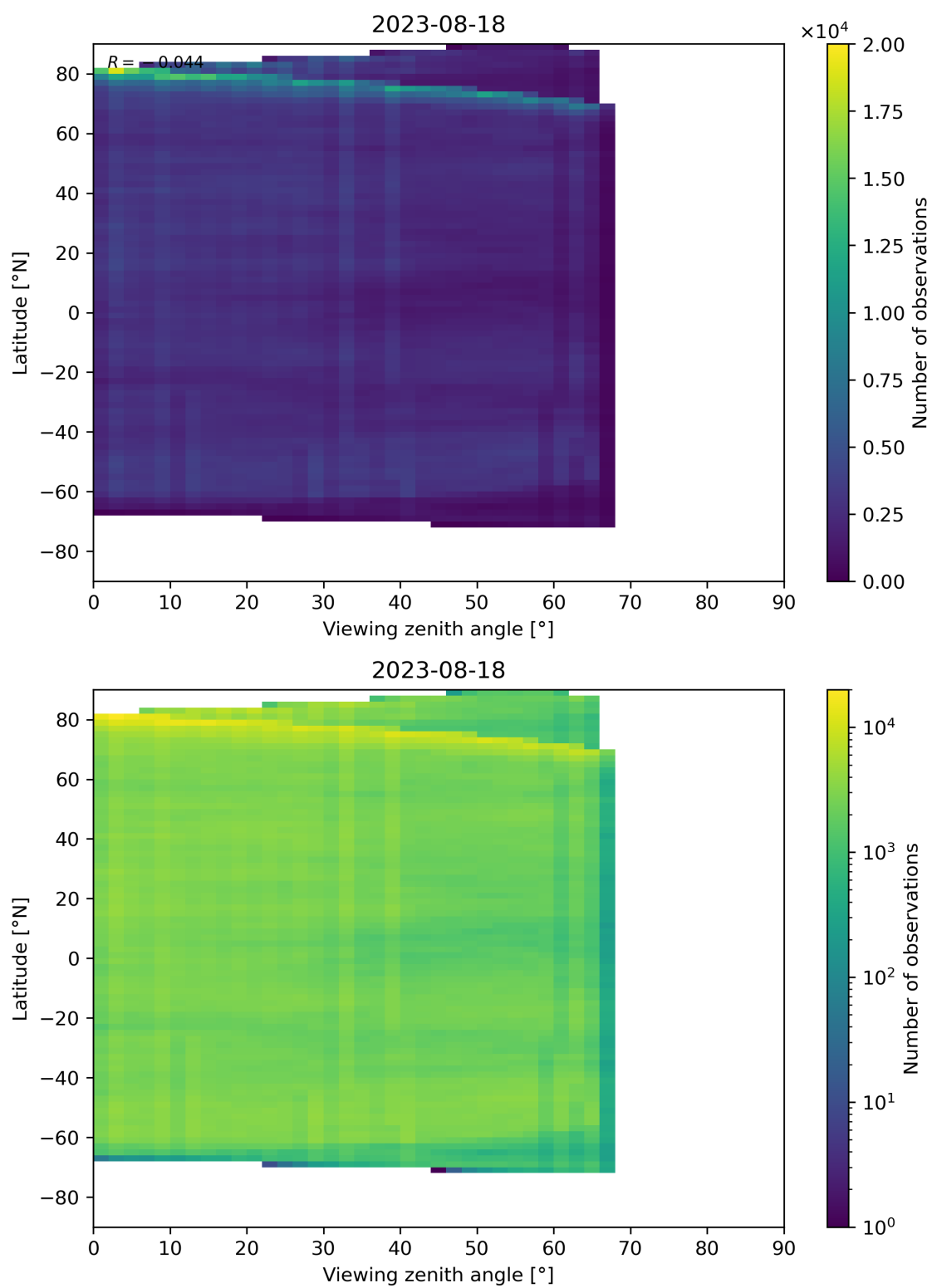
Figure 74: Scatter density plot of “Viewing zenith angle” against “Latitude” for 2023-08-17 to 2023-08-19.
