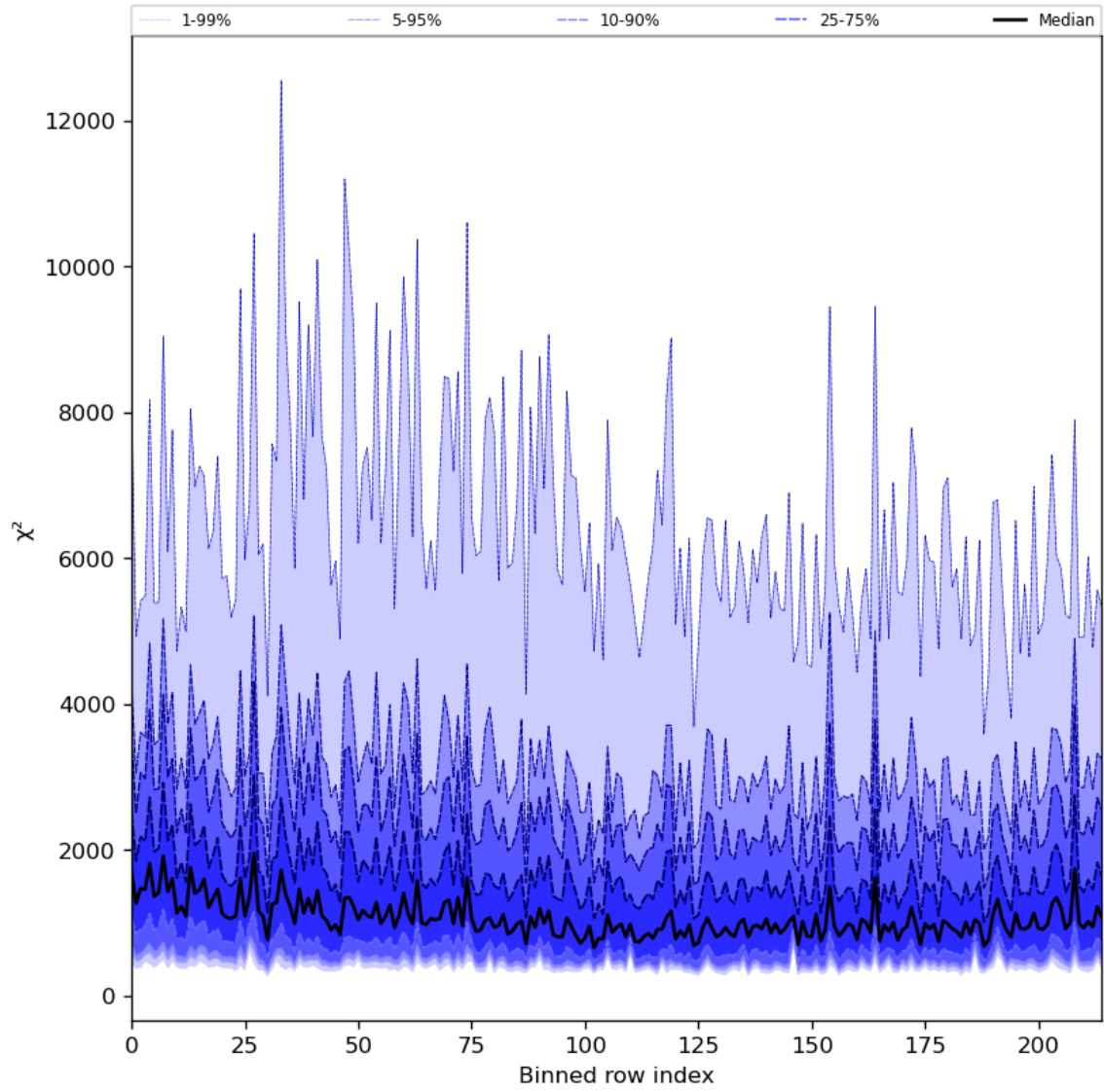
Figure 30: Along track statistics of “ \chi^2 ” for 2023-08-17 to 2023-08-19
