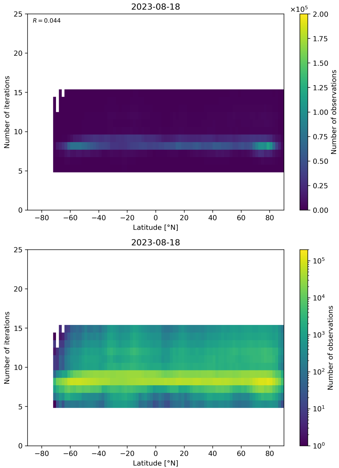
Figure 56: Scatter density plot of “Latitude” against “Number of iterations” for 2023-08-17 to 2023-08-19.
