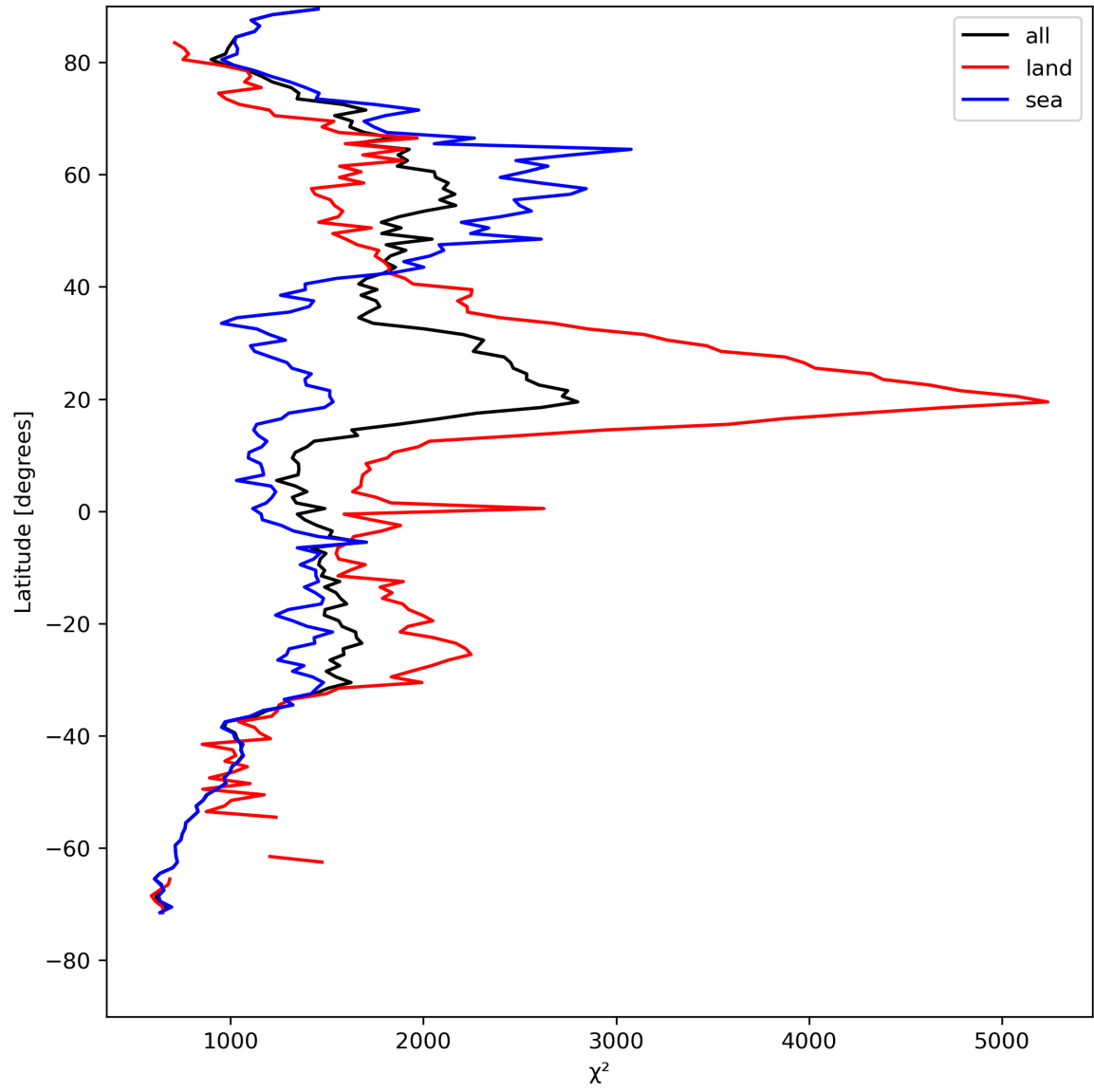
Figure 14: Zonal average of “ \chi^2 ” for 2023-08-17 to 2023-08-19.
