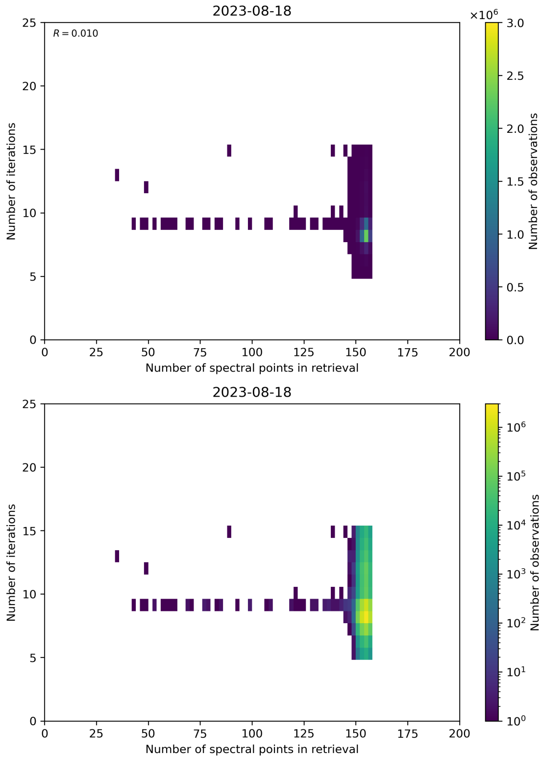
Figure 60: Scatter density plot of “Number of spectral points in retrieval” against “Number of iterations” for 2023-08-17 to 2023-08-19.
