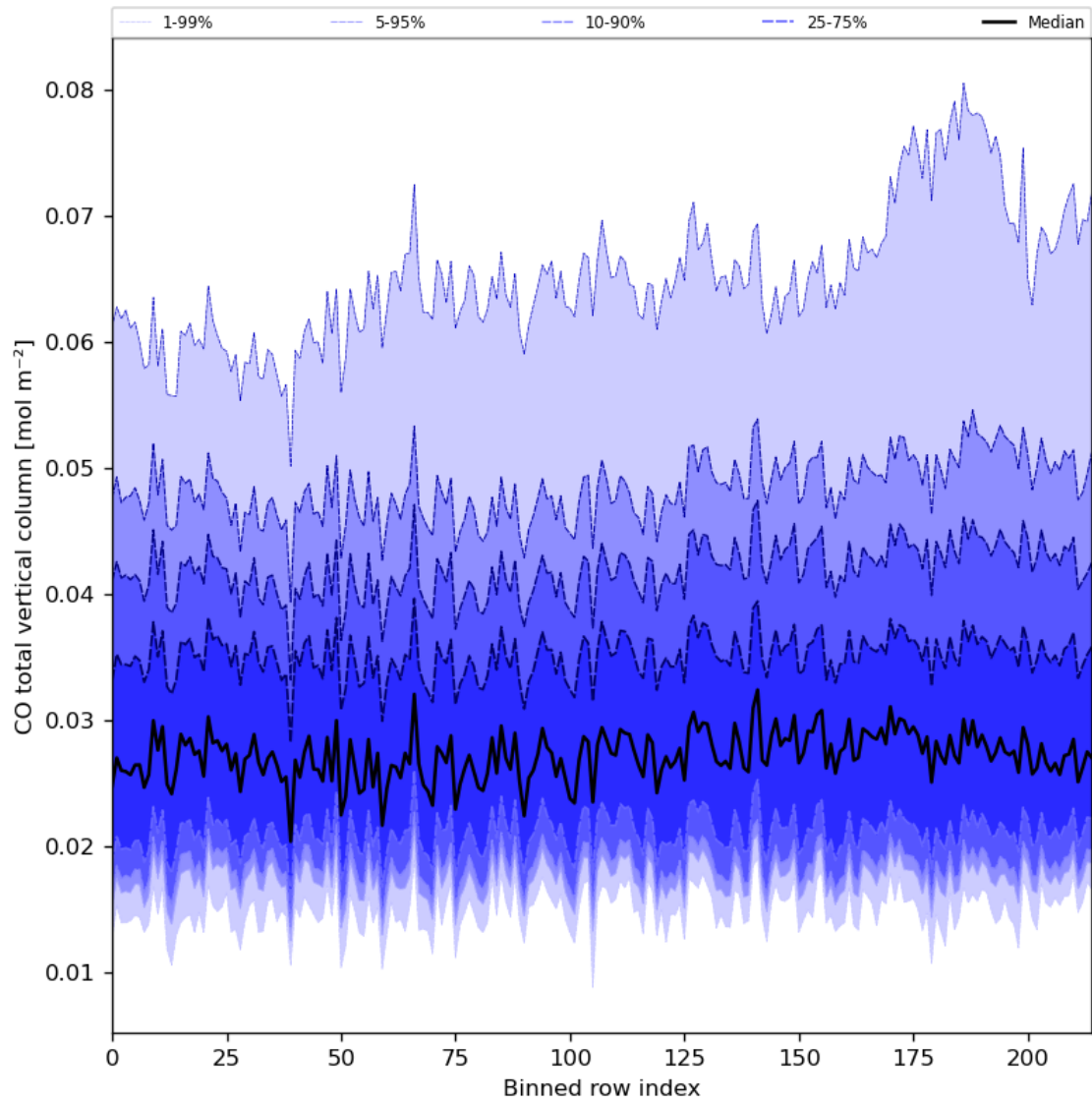
Figure 26: Along track statistics of “CO total vertical column” for 2023-08-17 to 2023-08-19
