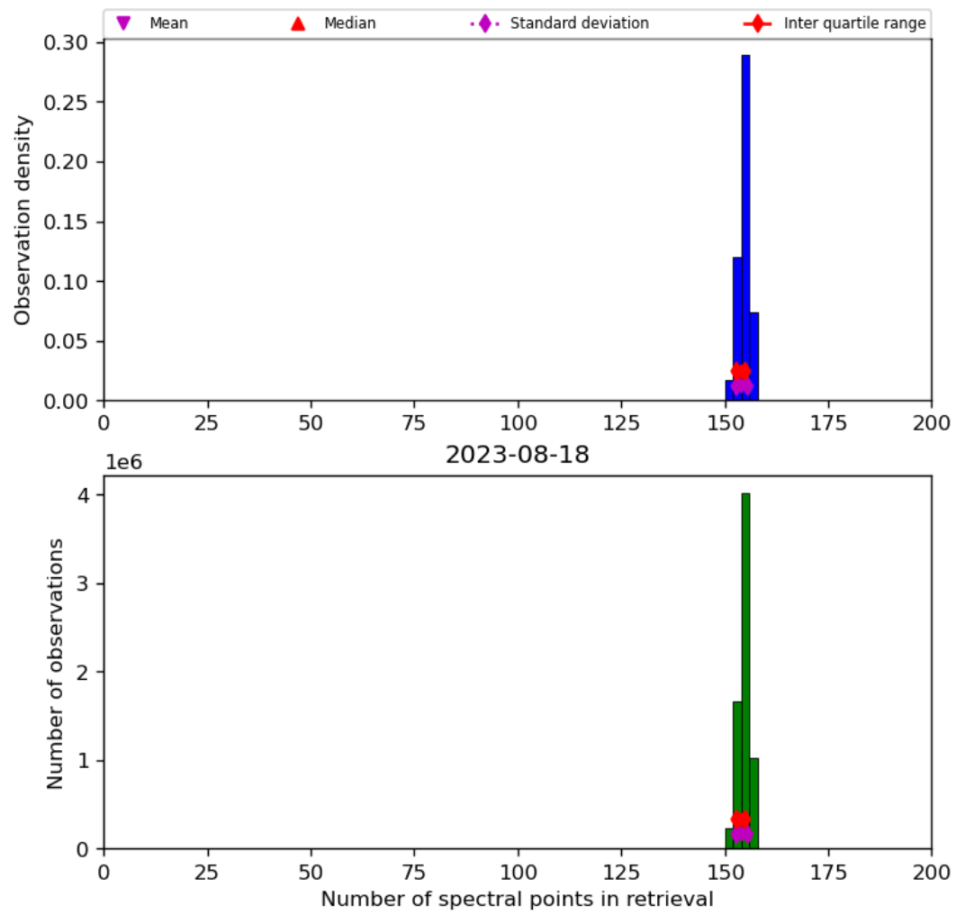
Figure 21: Histogram of “Number of spectral points in retrieval” for 2023-08-17 to 2023-08-19
