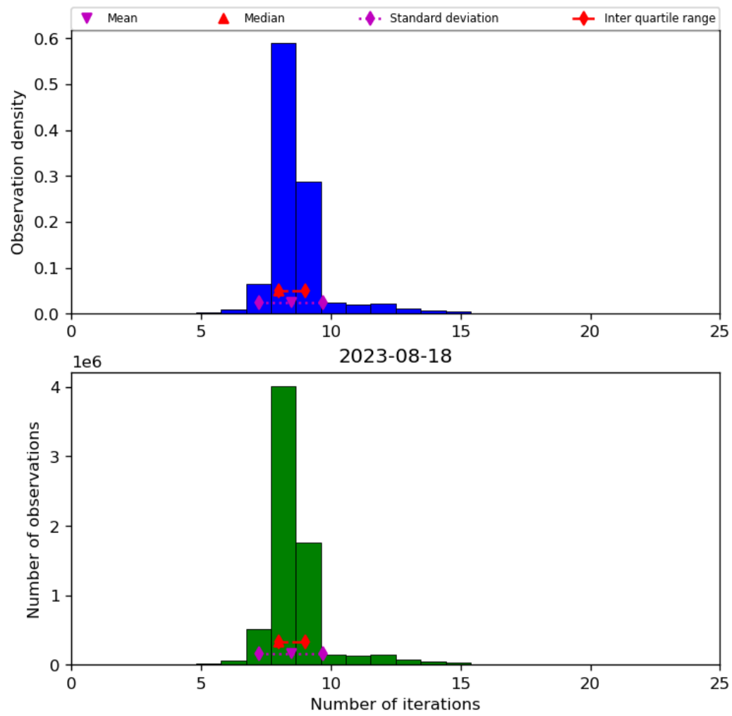
Figure 24: Histogram of “Number of iterations” for 2023-08-17 to 2023-08-19
