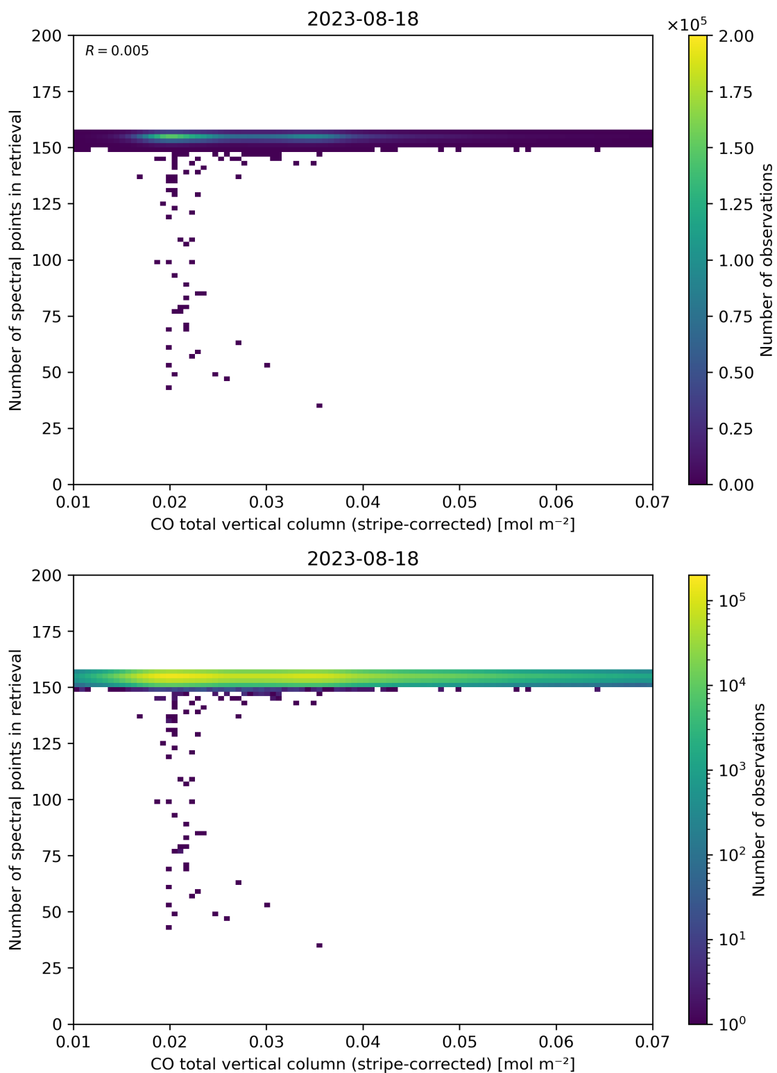
Figure 40: Scatter density plot of “CO total vertical column (stripe-corrected)” against “Number of spectral points in retrieval” for 2023-08-17 to 2023-08-19.
