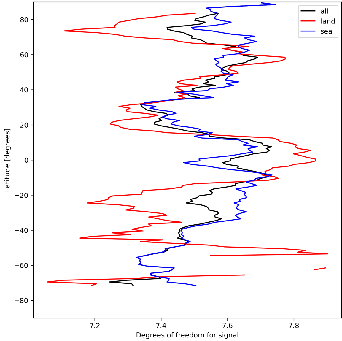
Figure 15: Zonal average of “Degrees of freedom for signal” for 2023-08-17 to 2023-08-19.
