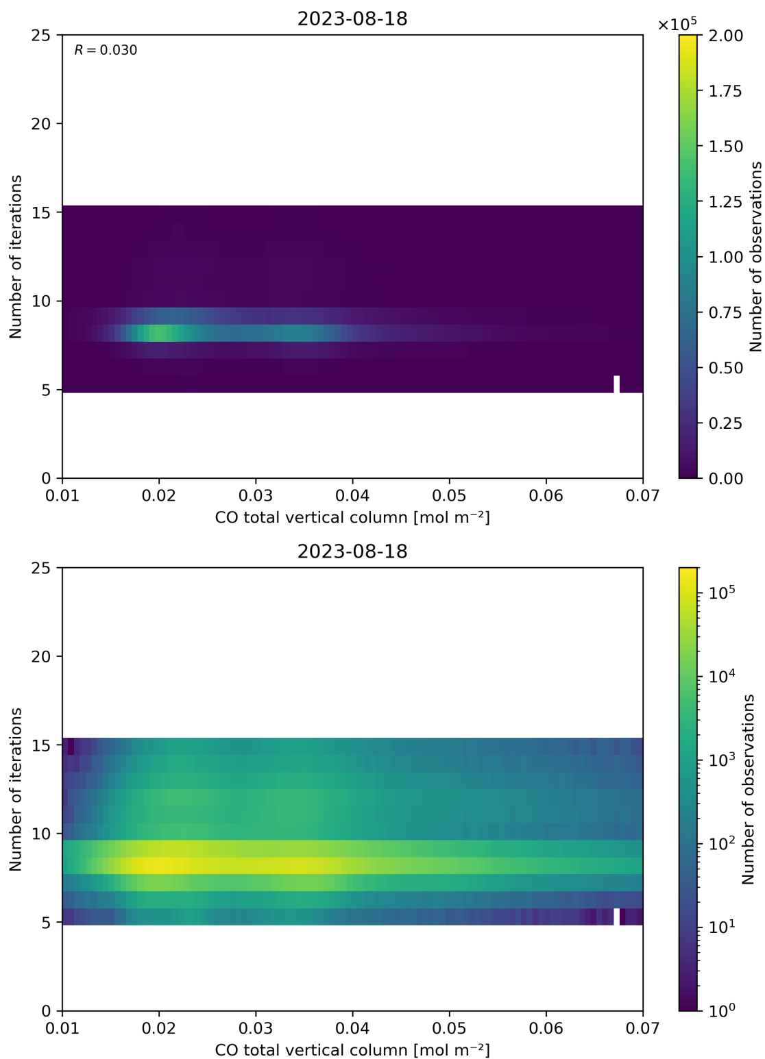
Figure 42: Scatter density plot of “CO total vertical column” against “Number of iterations” for 2023-08-17 to 2023-08-19.
