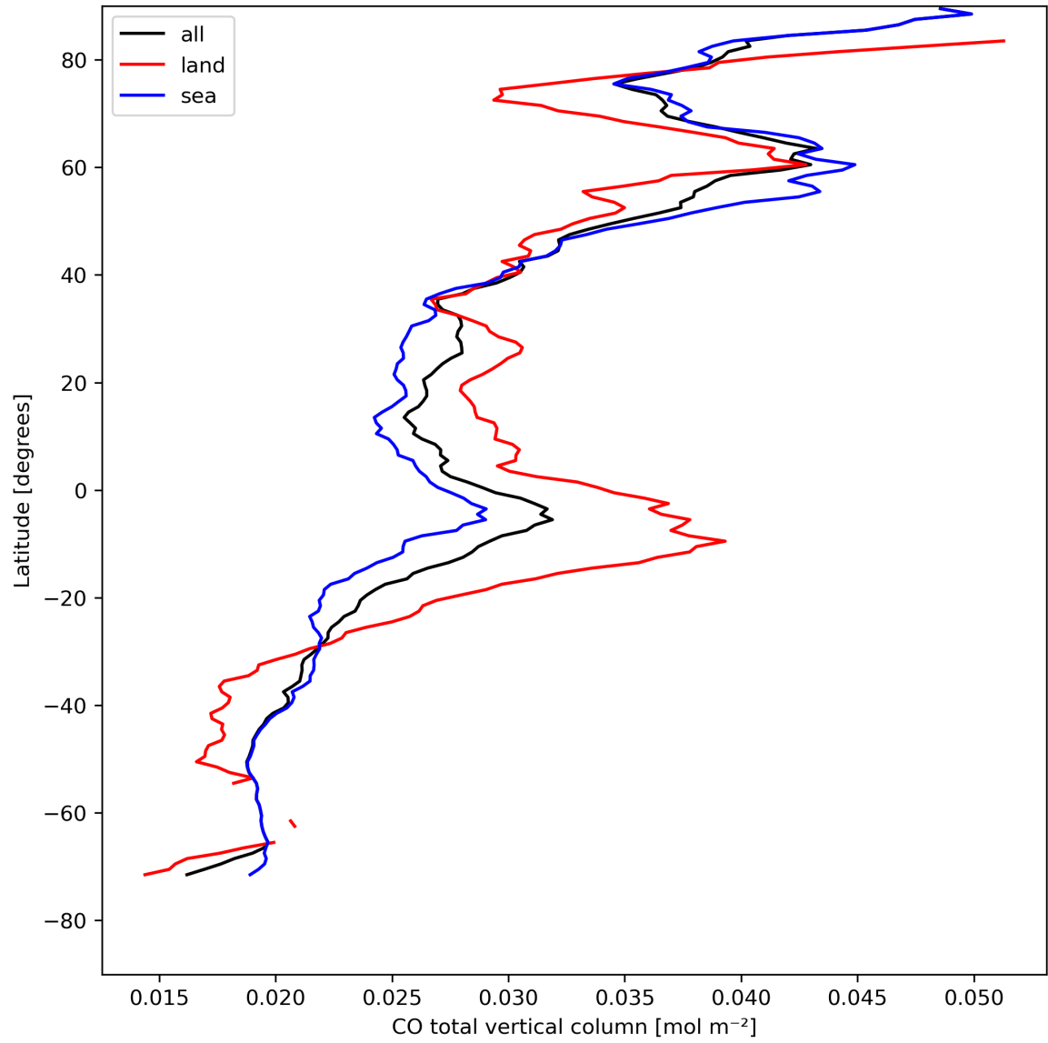
Figure 10: Zonal average of “CO total vertical column” for 2023-08-17 to 2023-08-19.
