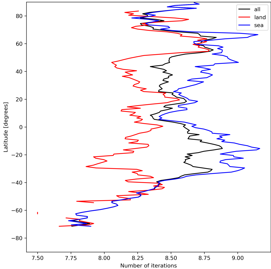
Figure 16: Zonal average of “Number of iterations” for 2023-08-17 to 2023-08-19.
