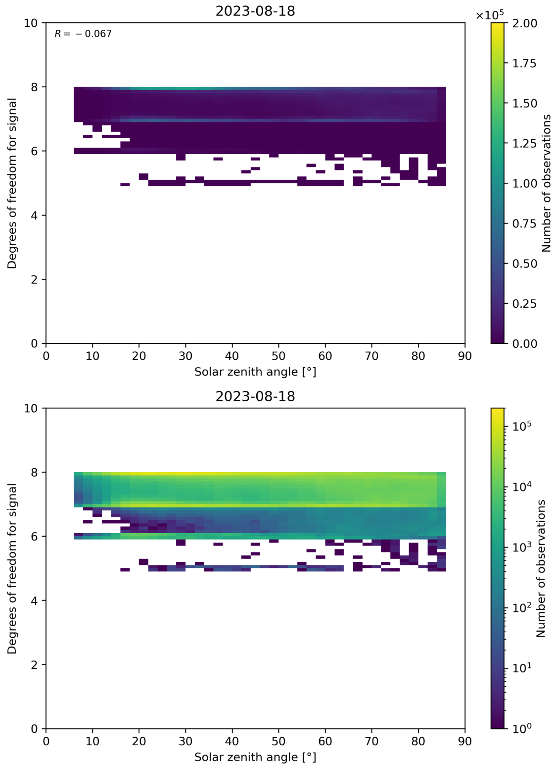
Figure 65: Scatter density plot of “Solar zenith angle” against “Degrees of freedom for signal” for 2023-08-17 to 2023-08-19.
