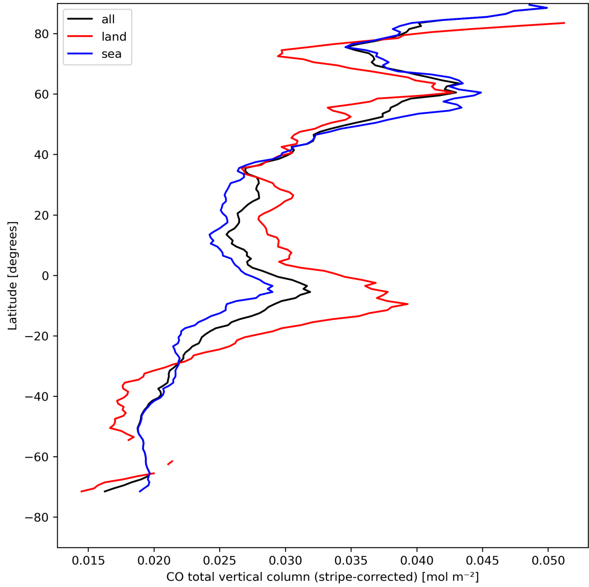
Figure 11: Zonal average of “CO total vertical column (stripe-corrected)” for 2023-08-17 to 2023-08-19.
