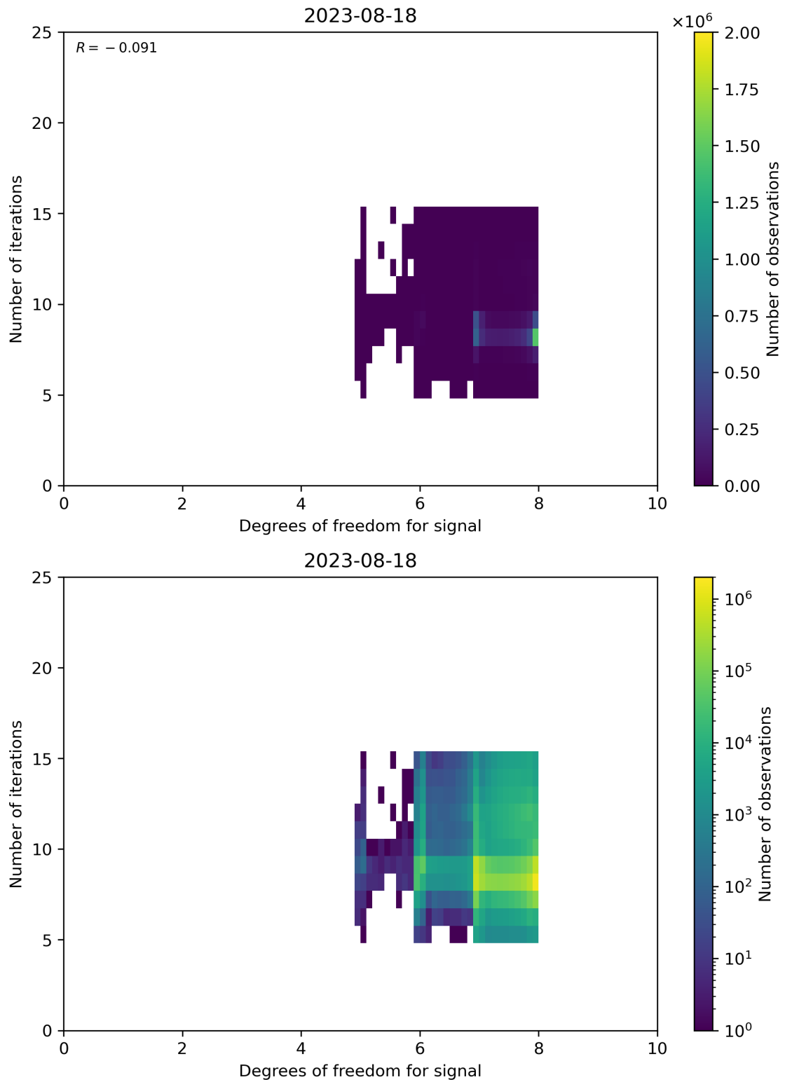
Figure 50: Scatter density plot of “Degrees of freedom for signal” against “Number of iterations” for 2023-08-17 to 2023-08-19.
