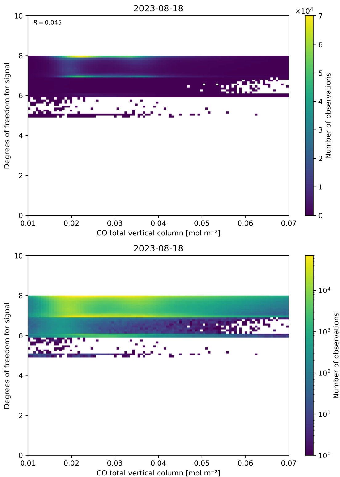
Figure 41: Scatter density plot of “CO total vertical column” against “Degrees of freedom for signal” for 2023-08-17 to 2023-08-19.
