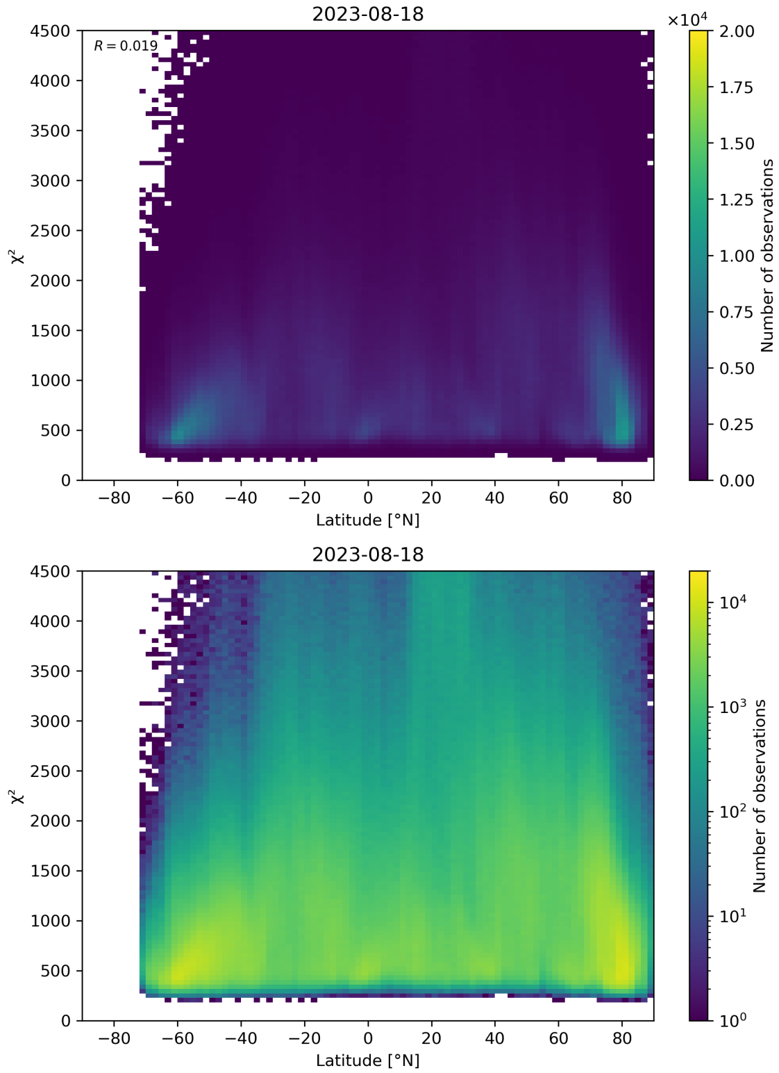
Figure 54: Scatter density plot of “Latitude” against “ \chi^2 ” for 2023-08-17 to 2023-08-19.
