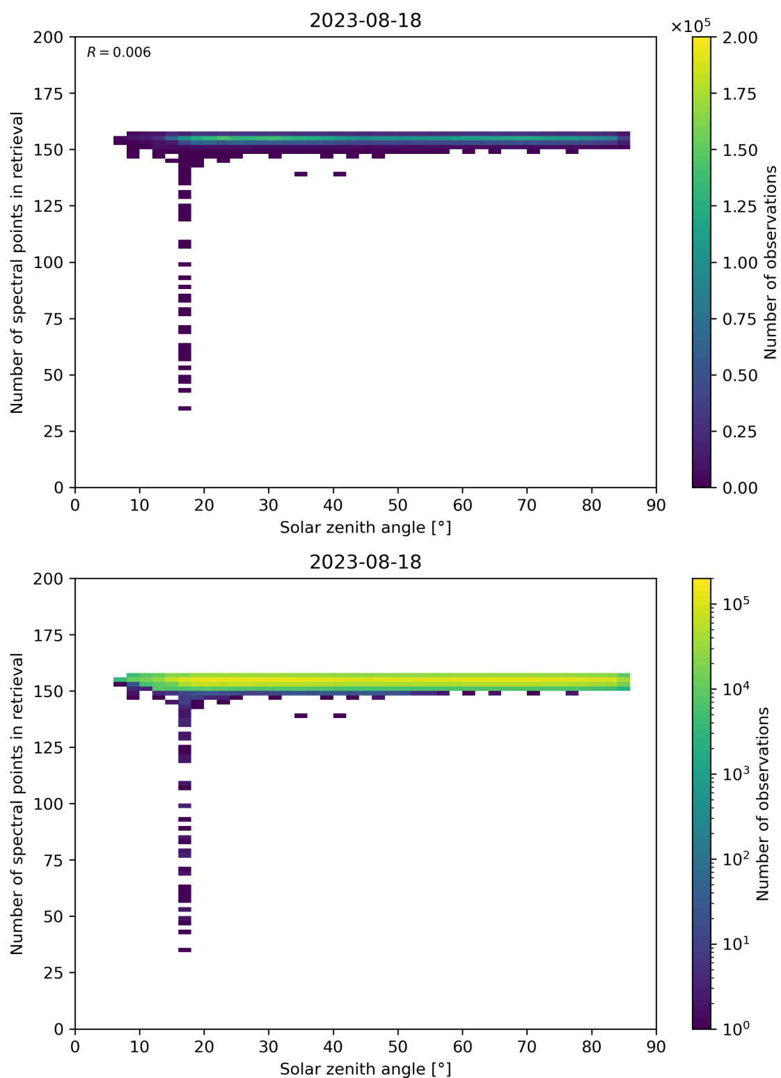
Figure 68: Scatter density plot of “Solar zenith angle” against “Number of spectral points in retrieval” for 2023-08-17 to 2023-08-19.
