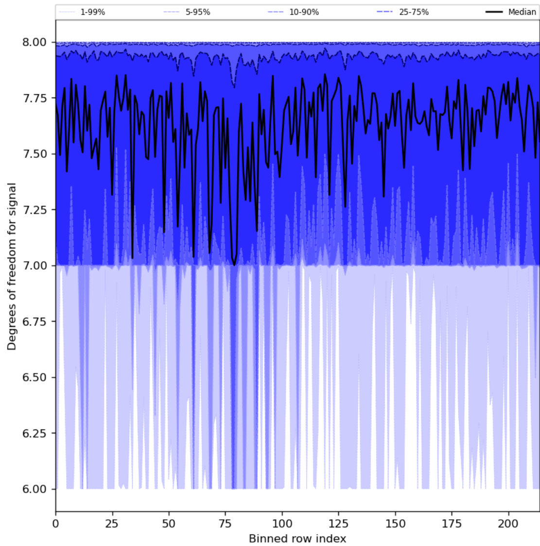
Figure 31: Along track statistics of “Degrees of freedom for signal” for 2023-08-17 to 2023-08-19
