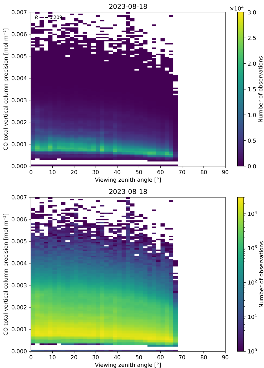
Figure 71: Scatter density plot of “Viewing zenith angle” against “CO total vertical column precision” for 2023-08-17 to 2023-08-19.
