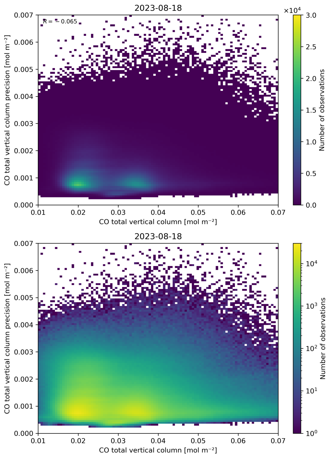
Figure 34: Scatter density plot of “CO total vertical column” against “CO total vertical column precision” for 2023-08-17 to 2023-08-19.
