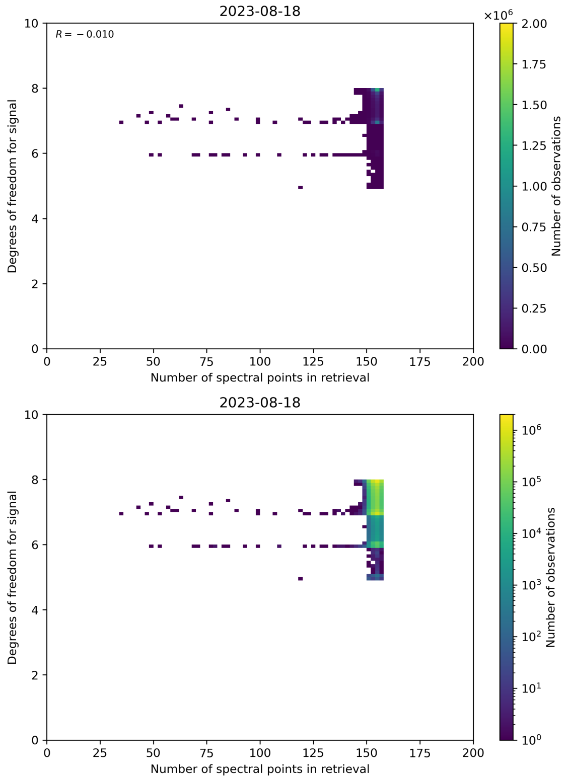
Figure 59: Scatter density plot of “Number of spectral points in retrieval” against “Degrees of freedom for signal” for 2023-08-17 to 2023-08-19.
