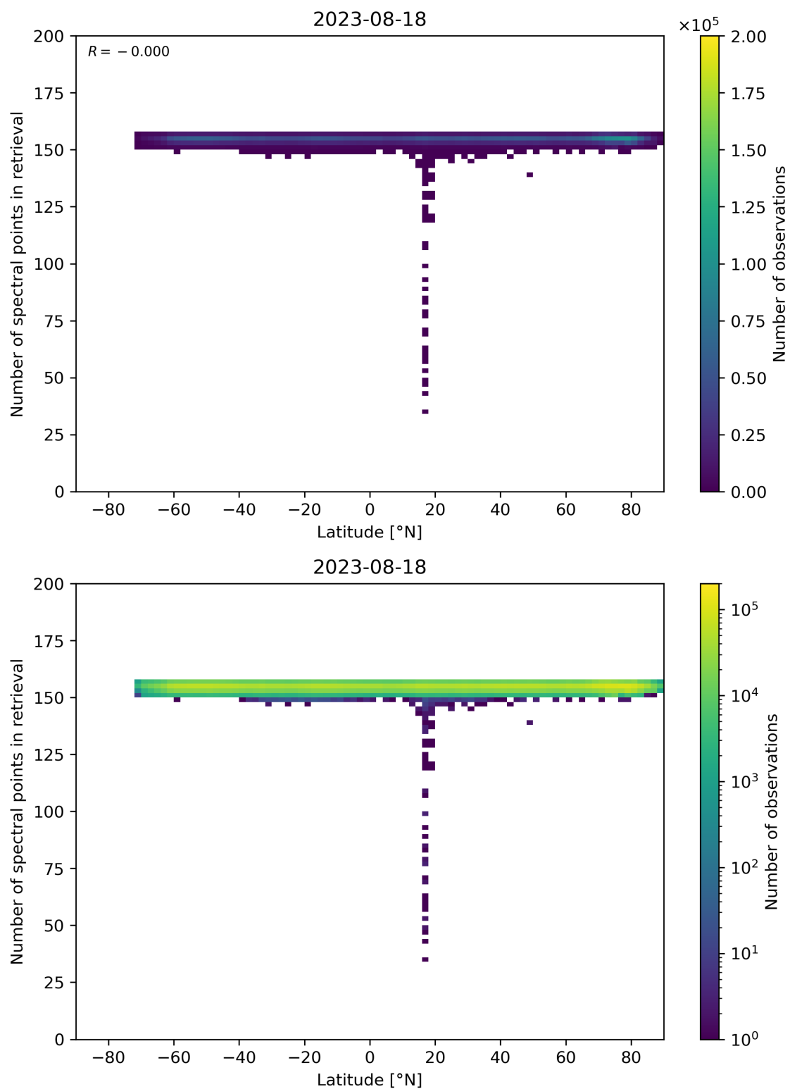
Figure 57: Scatter density plot of “Latitude” against “Number of spectral points in retrieval” for 2023-08-17 to 2023-08-19.
