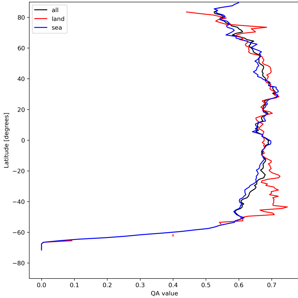
Figure 9: Zonal average of “QA value” for 2023-08-17 to 2023-08-19.
