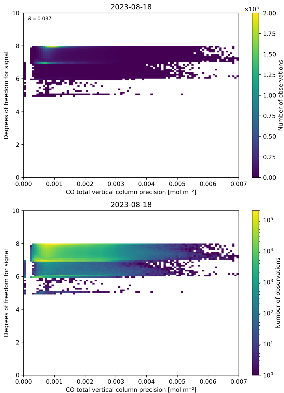
Figure 45: Scatter density plot of “CO total vertical column precision” against “Degrees of freedom for signal” for 2023-08-17 to 2023-08-19.
