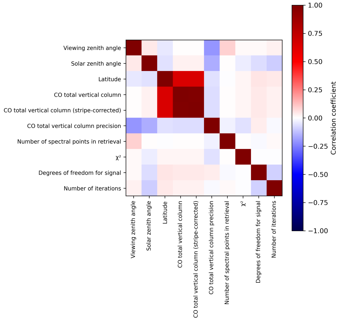
Figure 2: Map of correlation matrix for 2023-08-17 to 2023-08-19.
