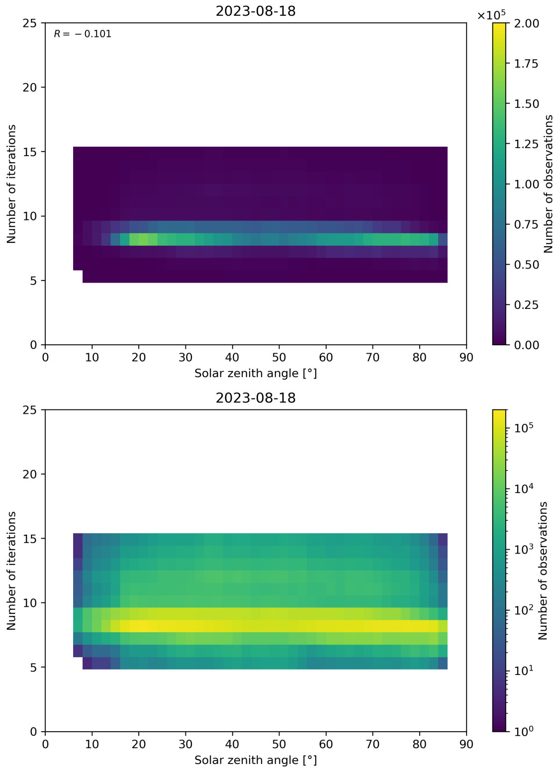
Figure 67: Scatter density plot of “Solar zenith angle” against “Number of iterations” for 2023-08-17 to 2023-08-19.
