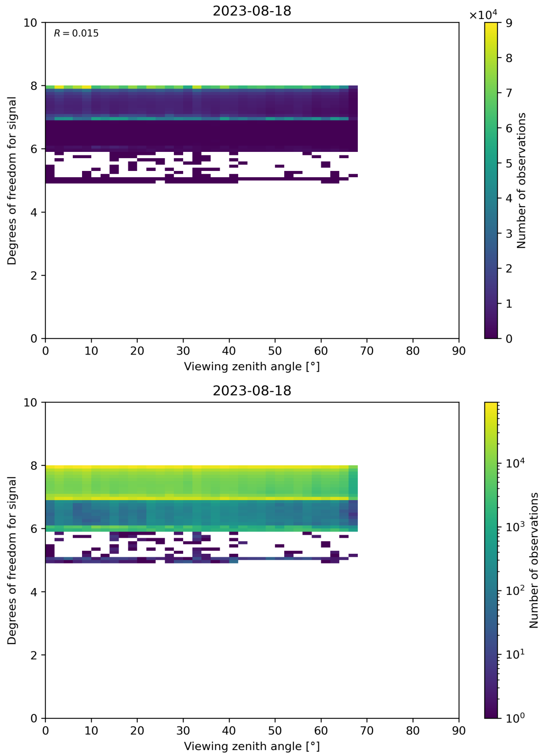
Figure 73: Scatter density plot of “Viewing zenith angle” against “Degrees of freedom for signal” for 2023-08-17 to 2023-08-19.
