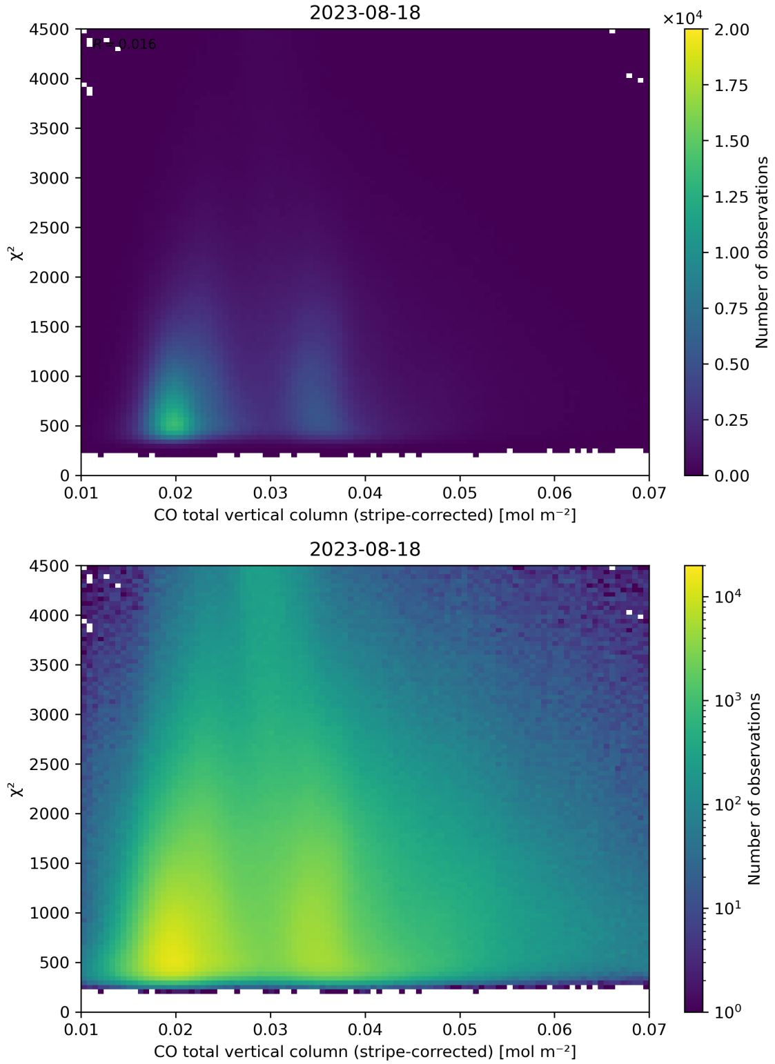
Figure 37: Scatter density plot of “CO total vertical column (stripe-corrected)” against “ \chi^2 ” for 2023-08-17 to 2023-08-19.
