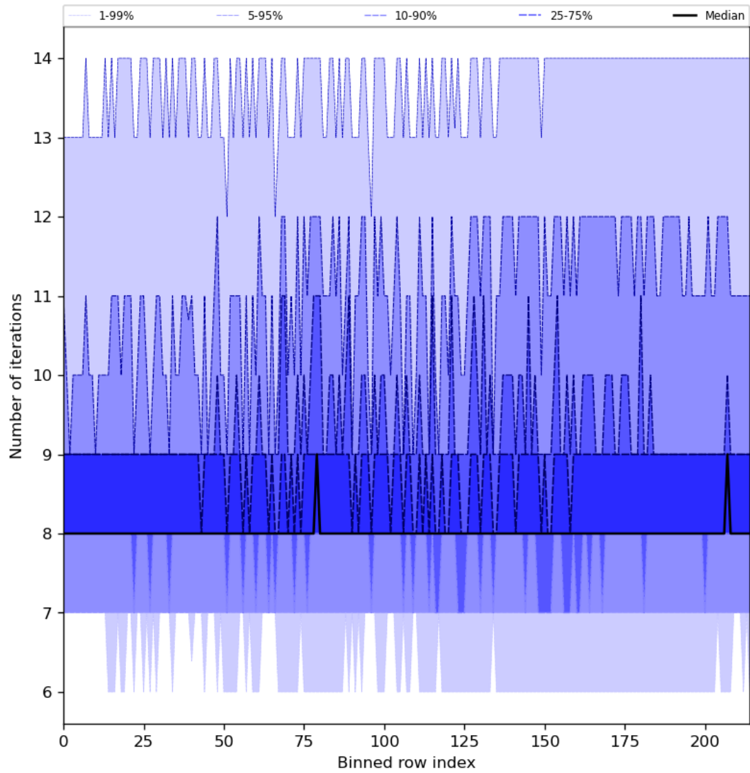
Figure 32: Along track statistics of “Number of iterations” for 2023-08-17 to 2023-08-19
