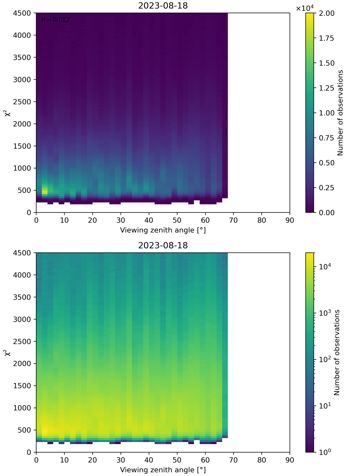
Figure 72: Scatter density plot of “Viewing zenith angle” against “ \chi^2 ” for 2023-08-17 to 2023-08-19.
