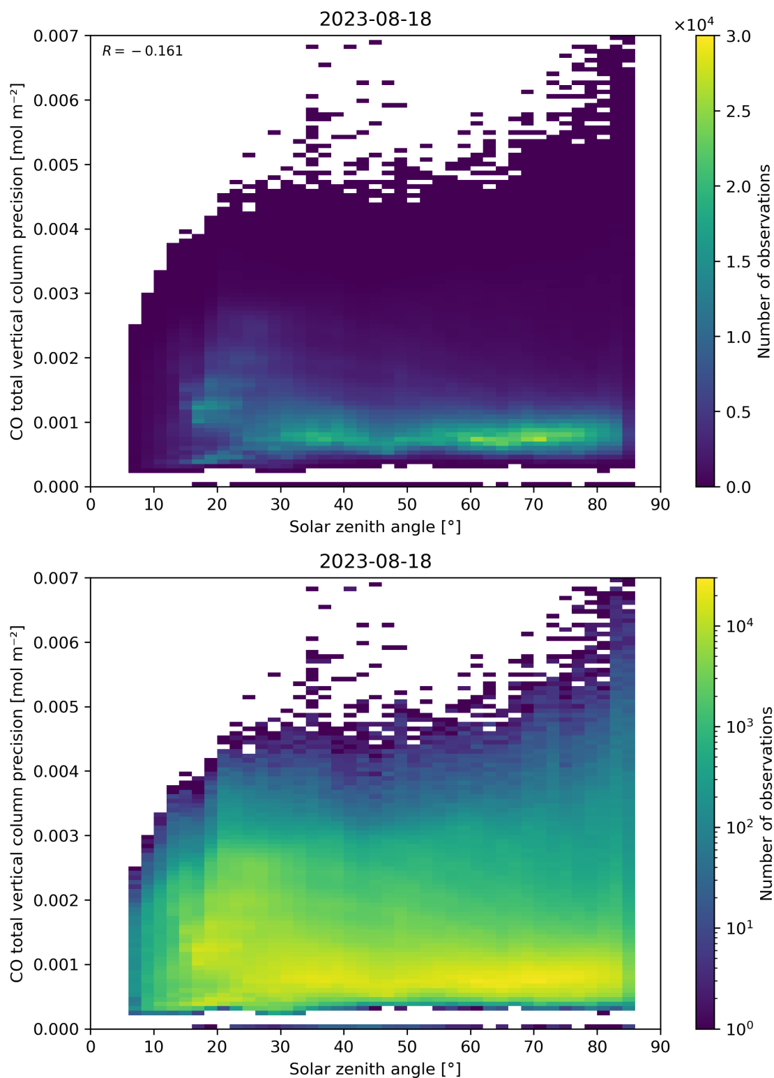
Figure 63: Scatter density plot of “Solar zenith angle” against “CO total vertical column precision” for 2023-08-17 to 2023-08-19.
