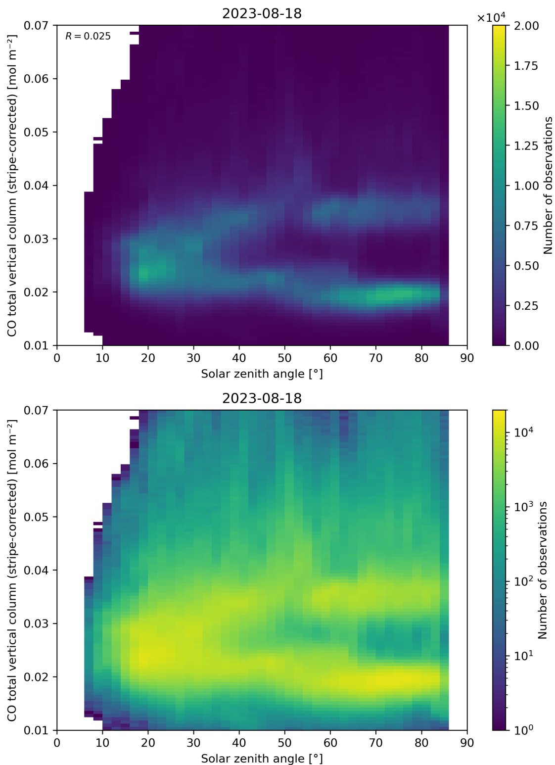
Figure 62: Scatter density plot of “Solar zenith angle” against “CO total vertical column (stripe-corrected)” for 2023-08-17 to 2023-08-19.
