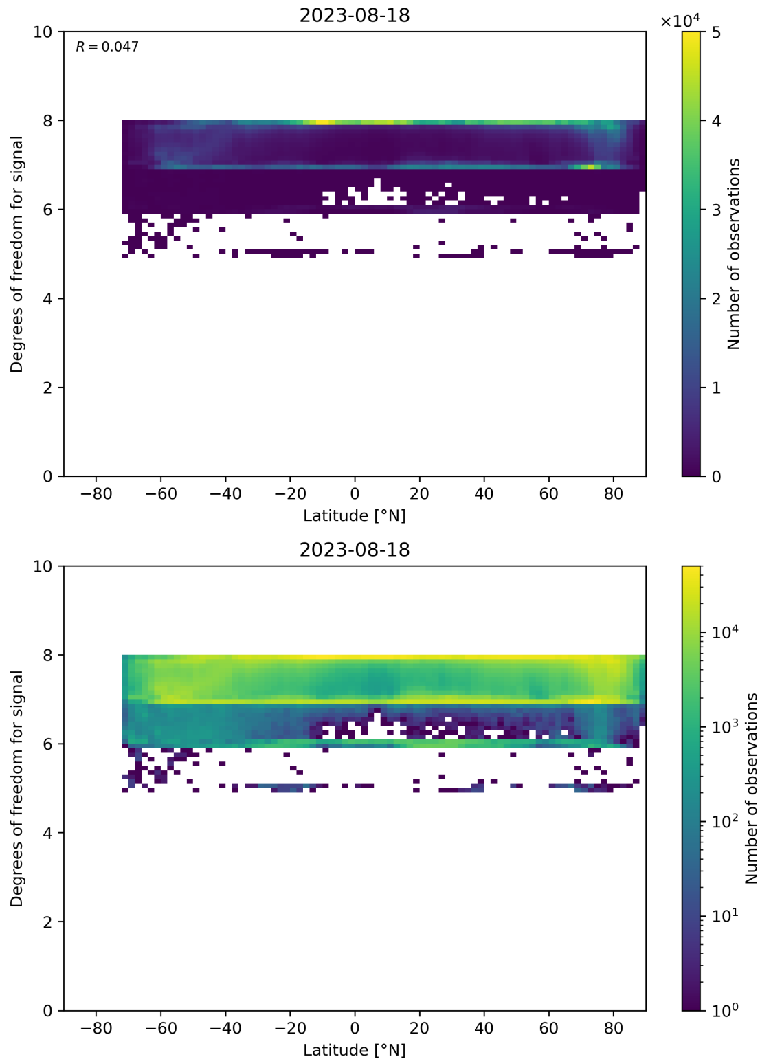
Figure 55: Scatter density plot of “Latitude” against “Degrees of freedom for signal” for 2023-08-17 to 2023-08-19.
