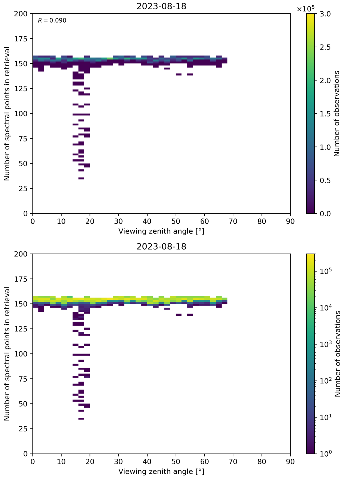
Figure 76: Scatter density plot of “Viewing zenith angle” against “Number of spectral points in retrieval” for 2023-08-17 to 2023-08-19.
