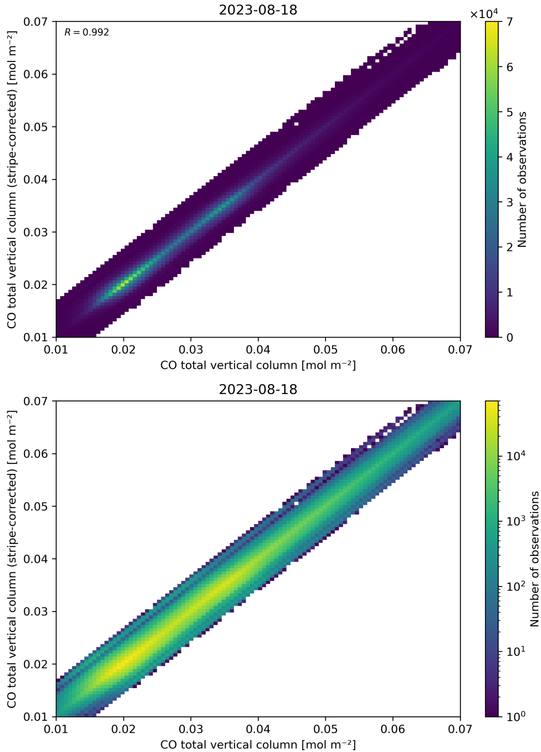
Figure 33: Scatter density plot of “CO total vertical column” against “CO total vertical column (stripe-corrected)” for 2023-08-17 to 2023-08-19.
