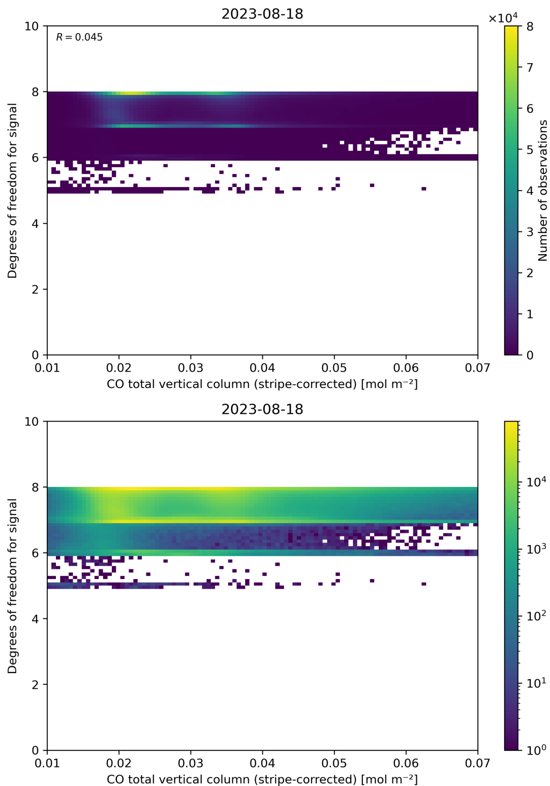
Figure 38: Scatter density plot of “CO total vertical column (stripe-corrected)” against “Degrees of freedom for signal” for 2023-08-17 to 2023-08-19.
