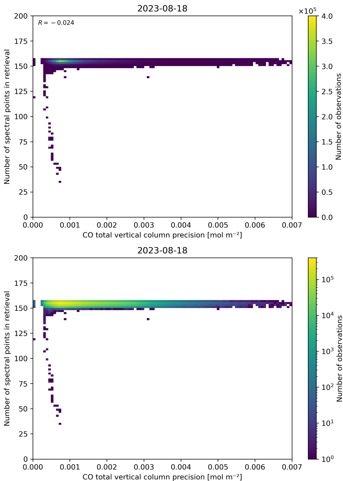
Figure 47: Scatter density plot of “CO total vertical column precision” against “Number of spectral points in retrieval” for 2023-08-17 to 2023-08-19.
