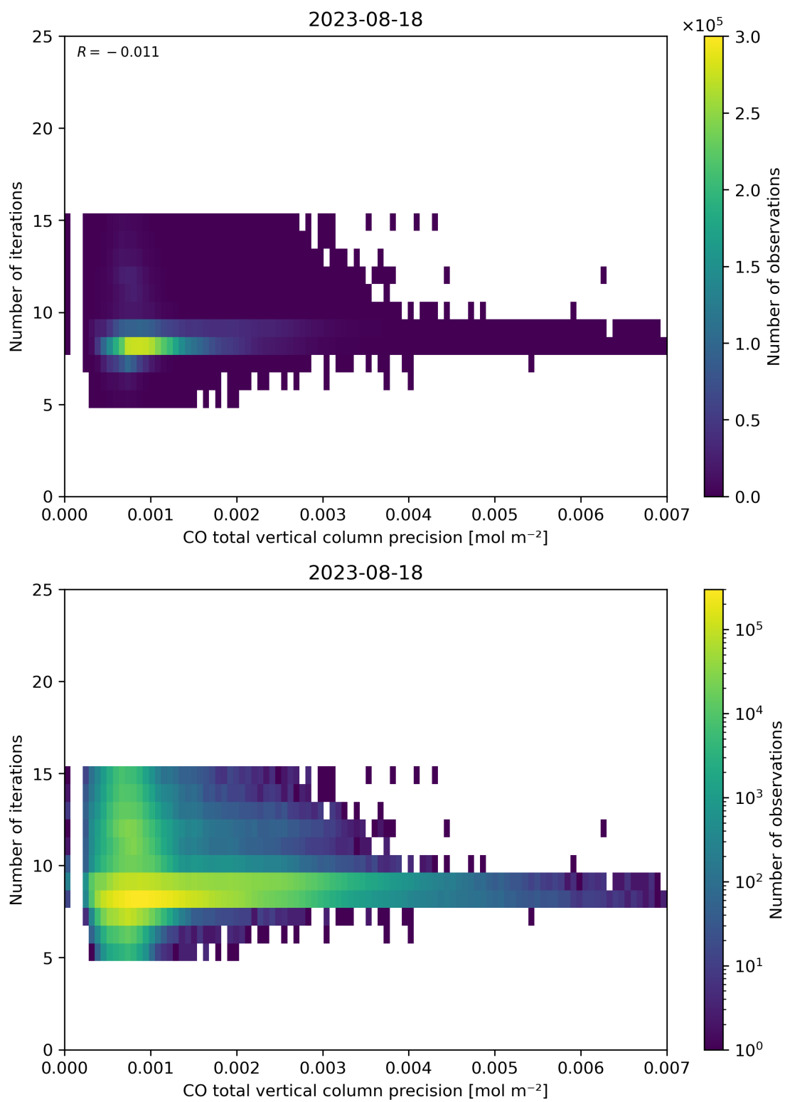
Figure 46: Scatter density plot of “CO total vertical column precision” against “Number of iterations” for 2023-08-17 to 2023-08-19.
