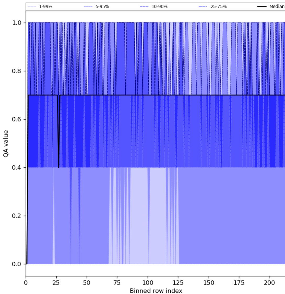
Figure 25: Along track statistics of “QA value” for 2023-08-17 to 2023-08-19
