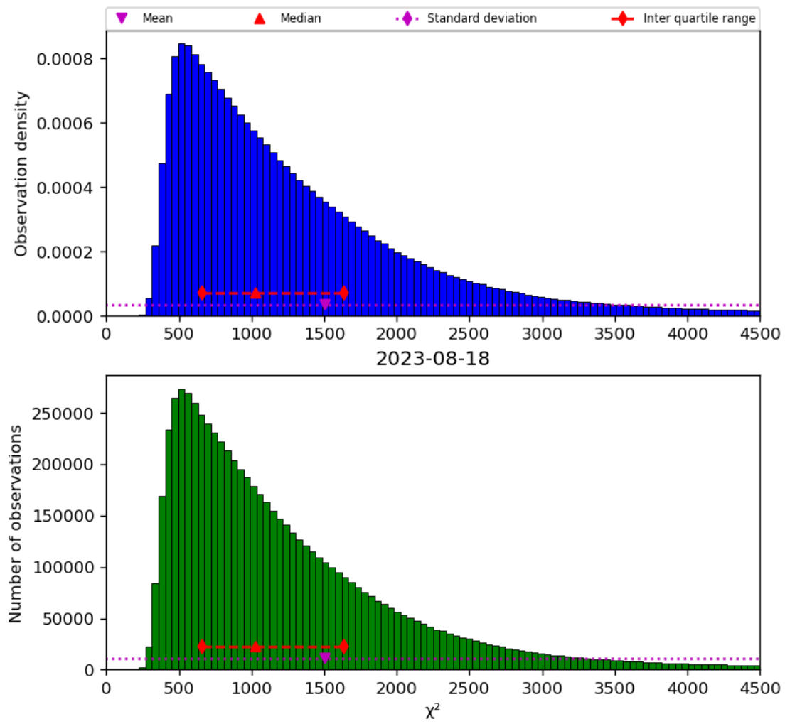
Figure 22: Histogram of “ \chi^2 ” for 2023-08-17 to 2023-08-19
