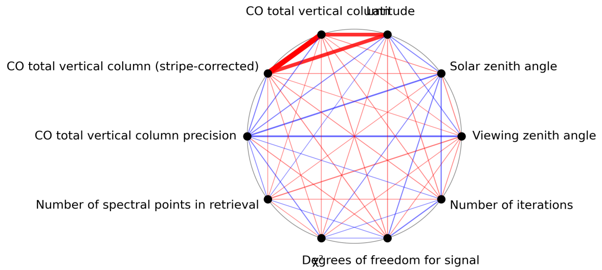
Figure 1: Map of correlation graph for 2023-08-17 to 2023-08-19.
