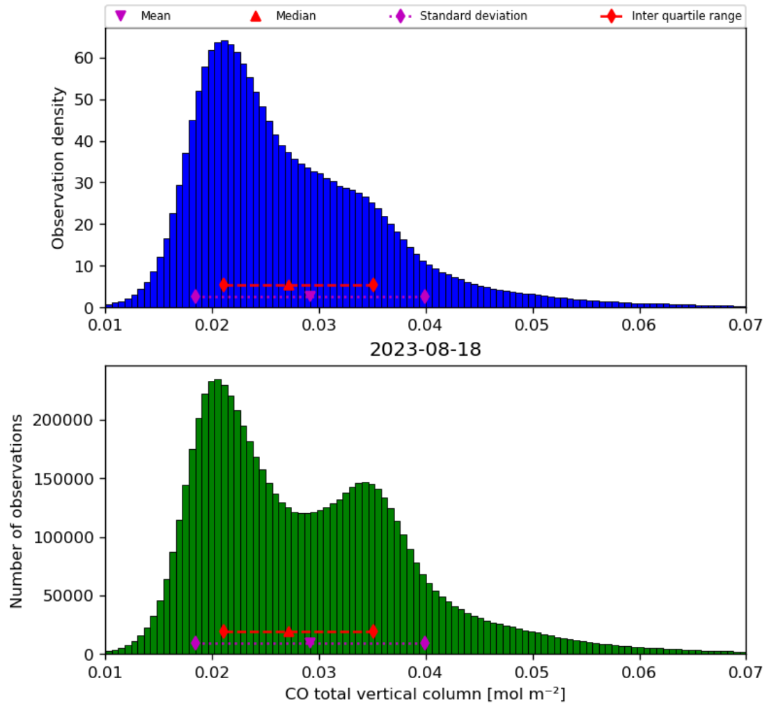
Figure 18: Histogram of “CO total vertical column” for 2023-08-17 to 2023-08-19
