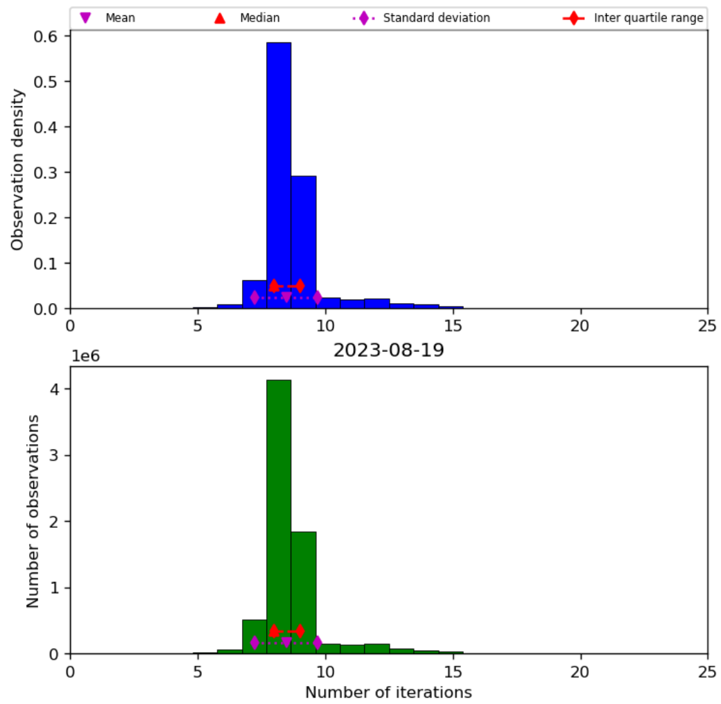
Figure 24: Histogram of “Number of iterations” for 2023-08-18 to 2023-08-20
