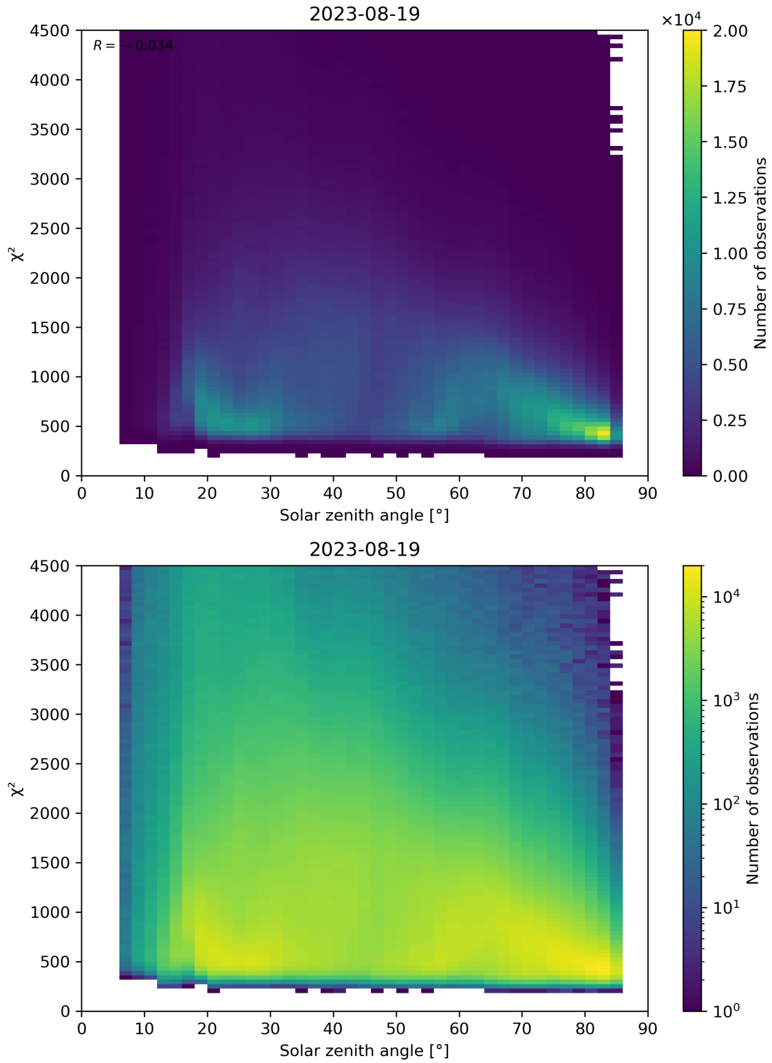
Figure 64: Scatter density plot of “Solar zenith angle” against “ \chi^2 ” for 2023-08-18 to 2023-08-20.
