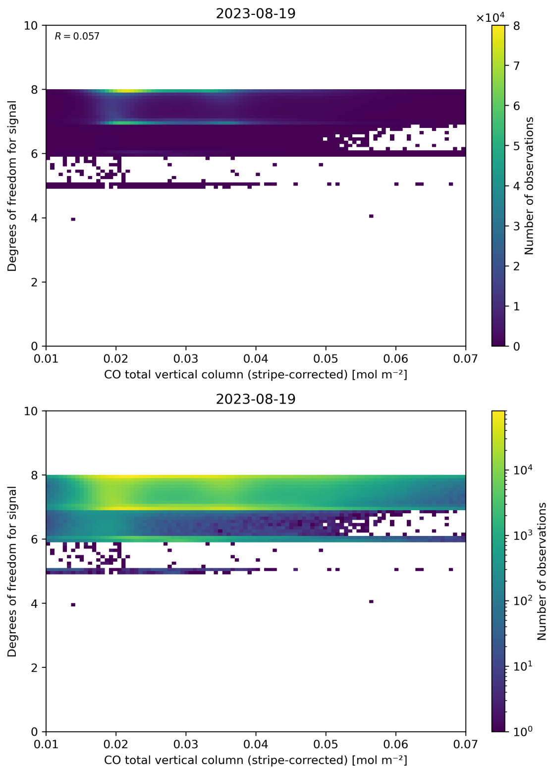
Figure 38: Scatter density plot of “CO total vertical column (stripe-corrected)” against “Degrees of freedom for signal” for 2023-08-18 to 2023-08-20.
