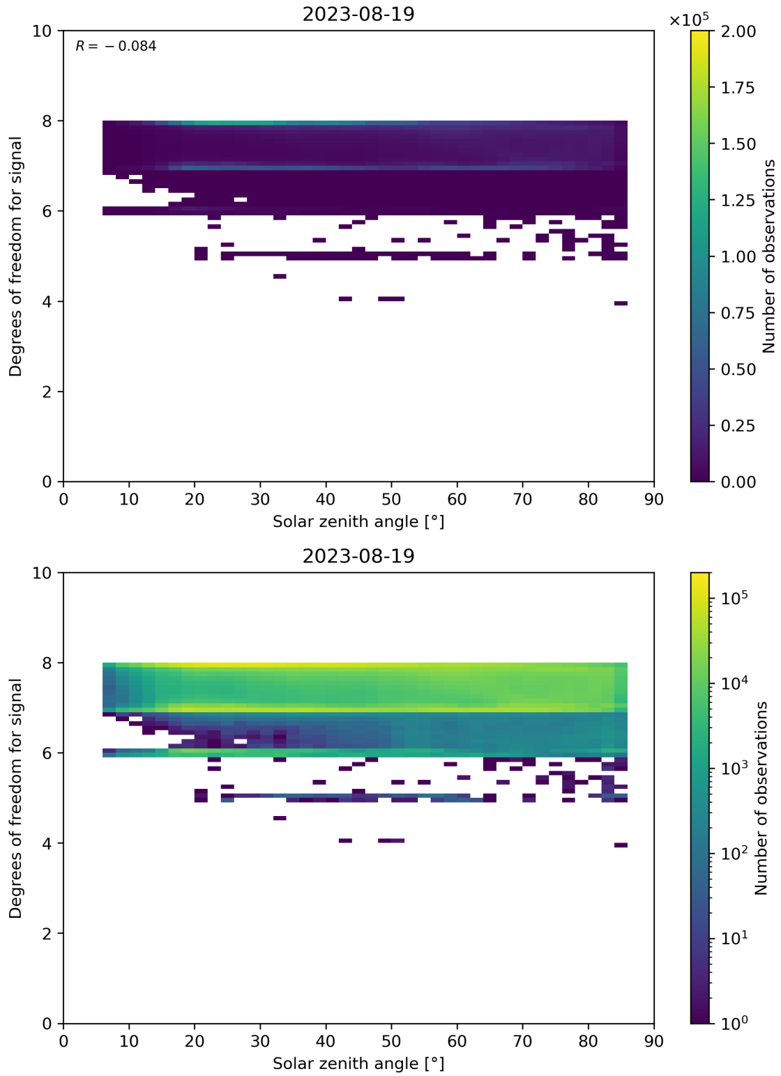
Figure 65: Scatter density plot of “Solar zenith angle” against “Degrees of freedom for signal” for 2023-08-18 to 2023-08-20.
