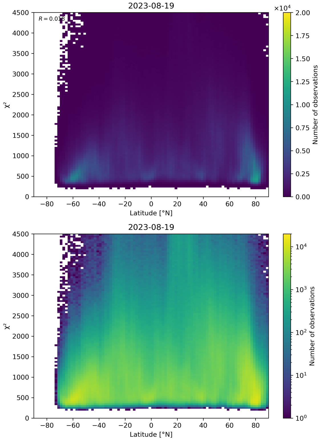
Figure 54: Scatter density plot of “Latitude” against “ \chi^2 ” for 2023-08-18 to 2023-08-20.
