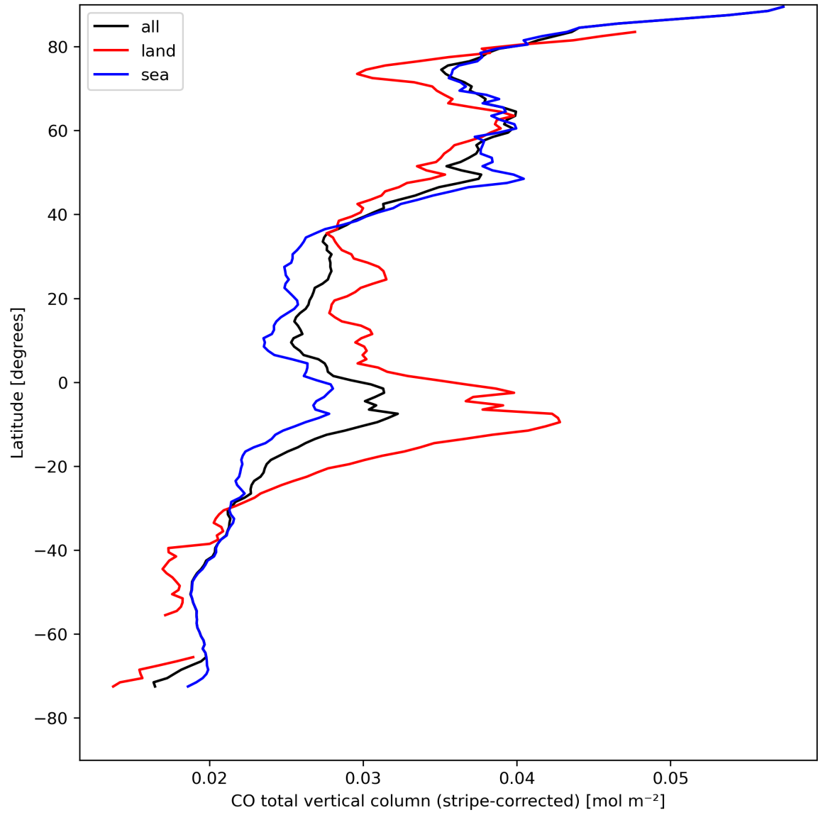
Figure 11: Zonal average of “CO total vertical column (stripe-corrected)” for 2023-08-18 to 2023-08-20.
