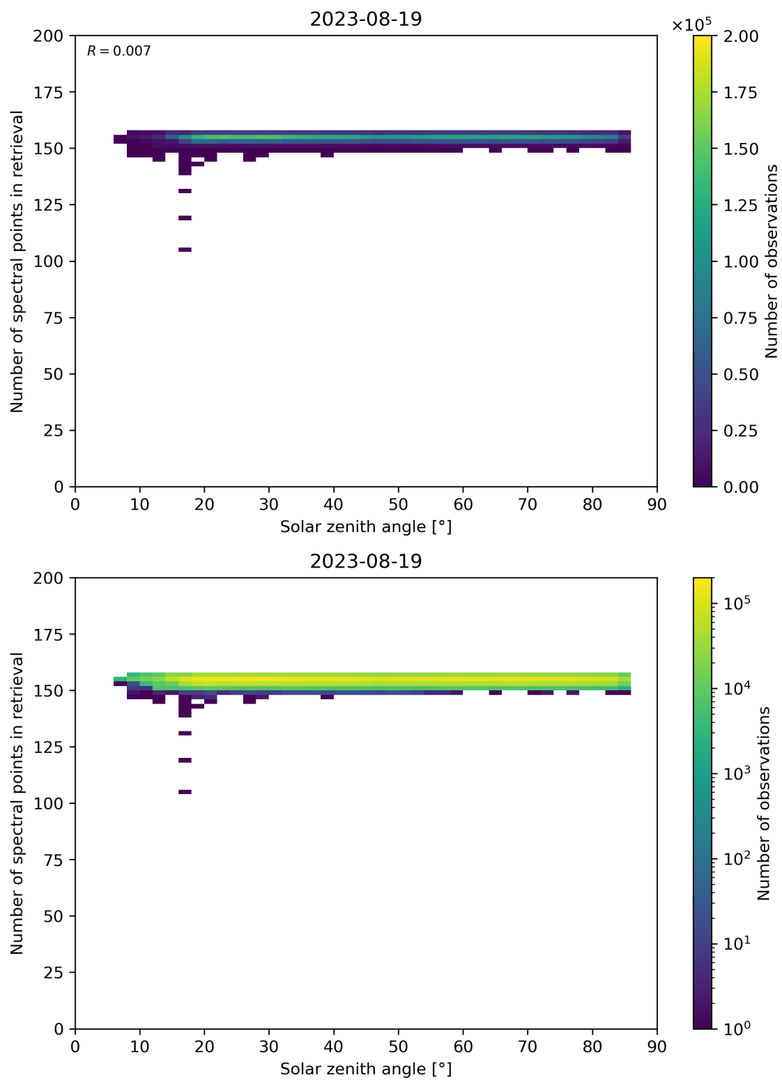
Figure 68: Scatter density plot of “Solar zenith angle” against “Number of spectral points in retrieval” for 2023-08-18 to 2023-08-20.
