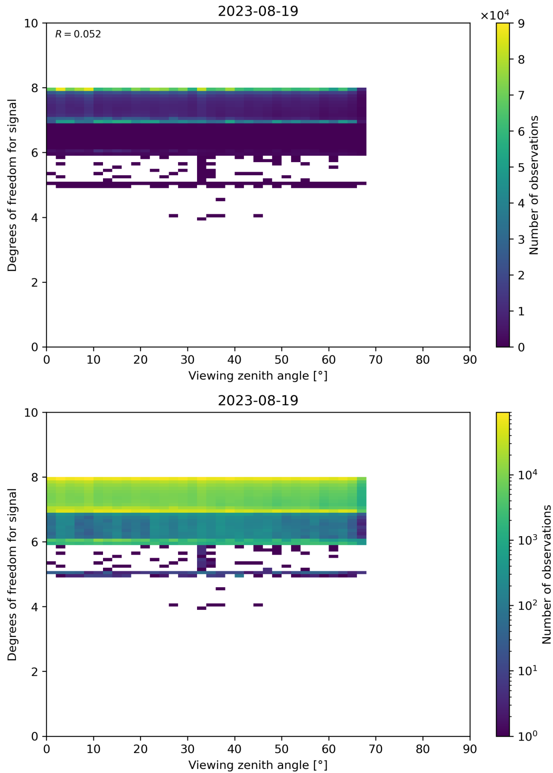
Figure 73: Scatter density plot of “Viewing zenith angle” against “Degrees of freedom for signal” for 2023-08-18 to 2023-08-20.
