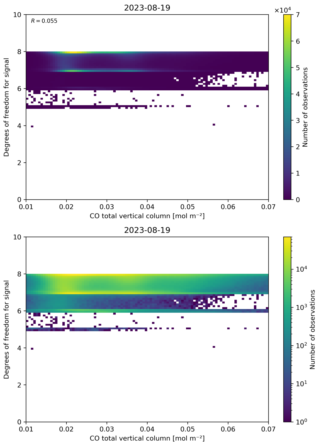
Figure 41: Scatter density plot of “CO total vertical column” against “Degrees of freedom for signal” for 2023-08-18 to 2023-08-20.
