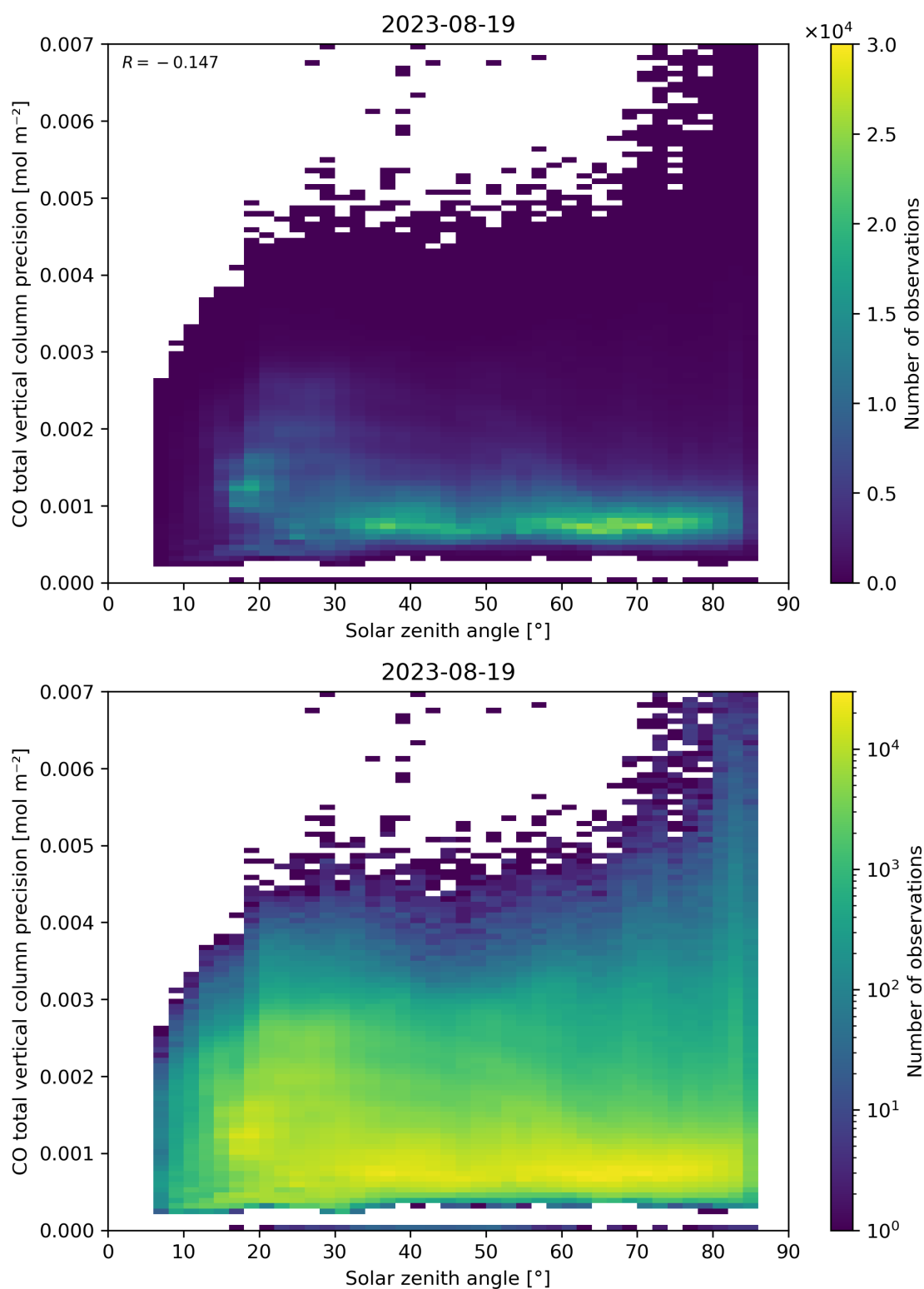
Figure 63: Scatter density plot of “Solar zenith angle” against “CO total vertical column precision” for 2023-08-18 to 2023-08-20.
