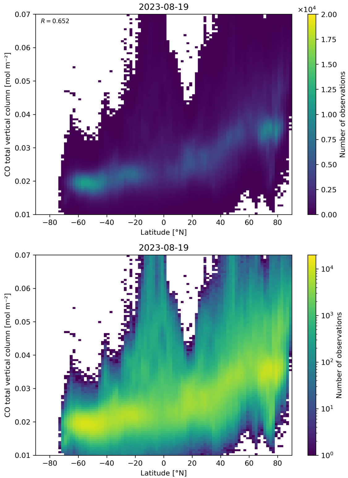
Figure 51: Scatter density plot of “Latitude” against “CO total vertical column” for 2023-08-18 to 2023-08-20.
