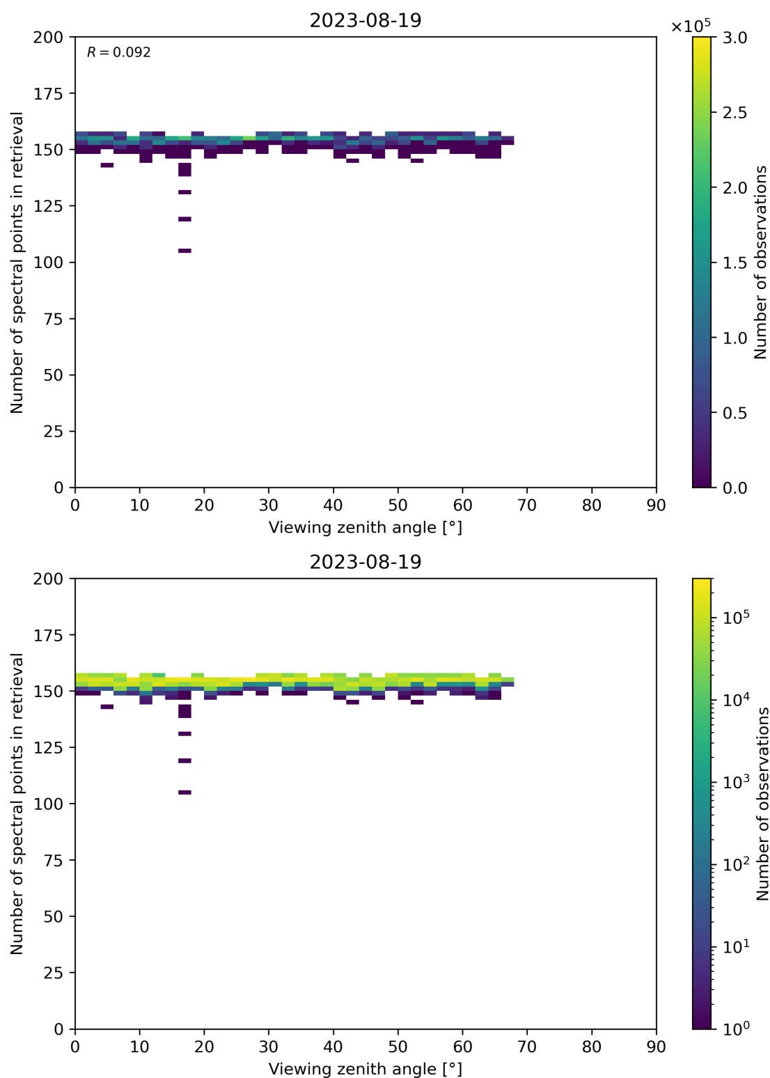
Figure 76: Scatter density plot of “Viewing zenith angle” against “Number of spectral points in retrieval” for 2023-08-18 to 2023-08-20.
