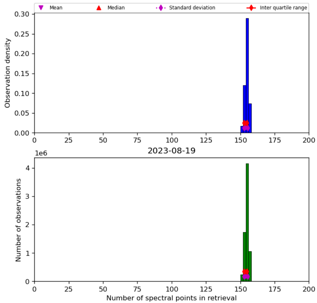
Figure 21: Histogram of “Number of spectral points in retrieval” for 2023-08-18 to 2023-08-20
