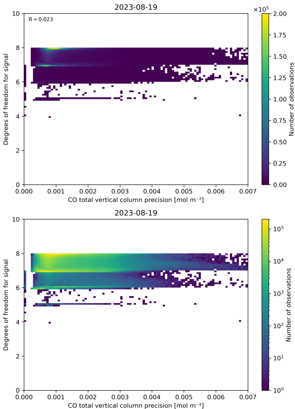
Figure 45: Scatter density plot of “CO total vertical column precision” against “Degrees of freedom for signal” for 2023-08-18 to 2023-08-20.
