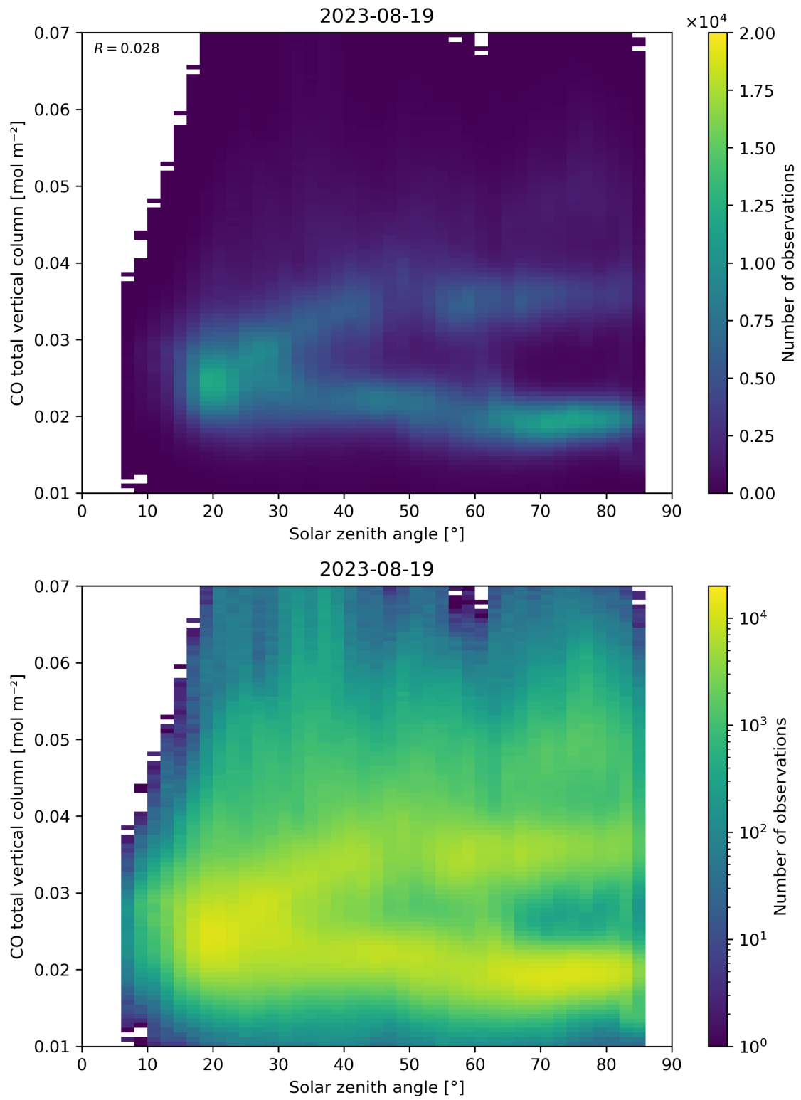
Figure 61: Scatter density plot of “Solar zenith angle” against “CO total vertical column” for 2023-08-18 to 2023-08-20.
