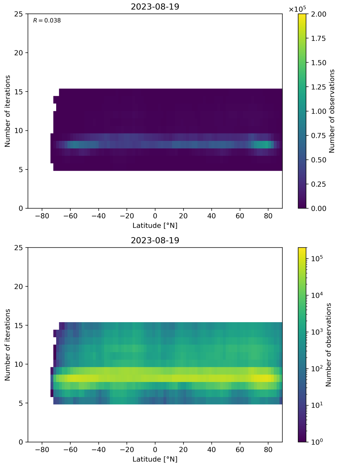
Figure 56: Scatter density plot of “Latitude” against “Number of iterations” for 2023-08-18 to 2023-08-20.
