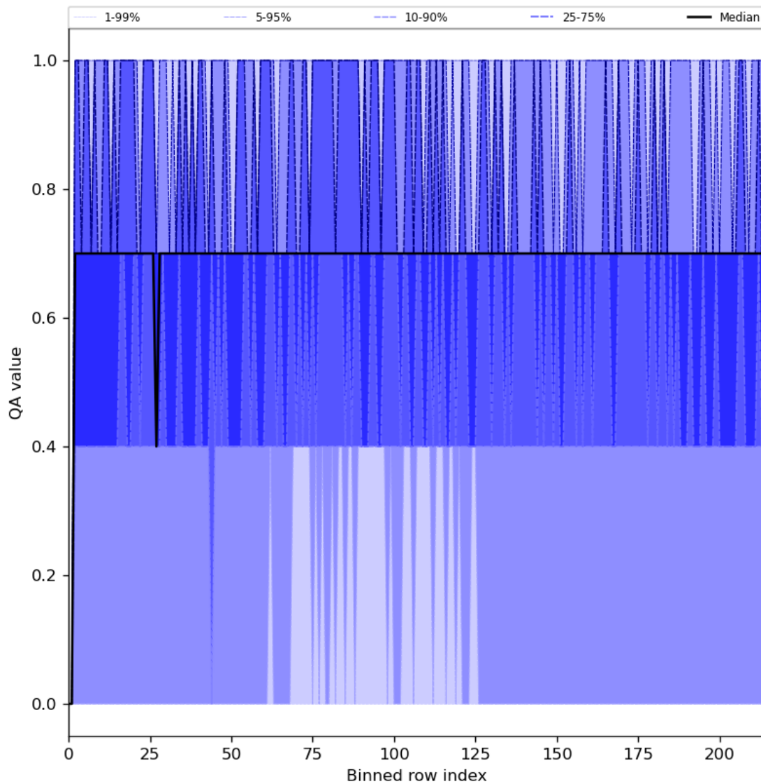
Figure 25: Along track statistics of “QA value” for 2023-08-18 to 2023-08-20
