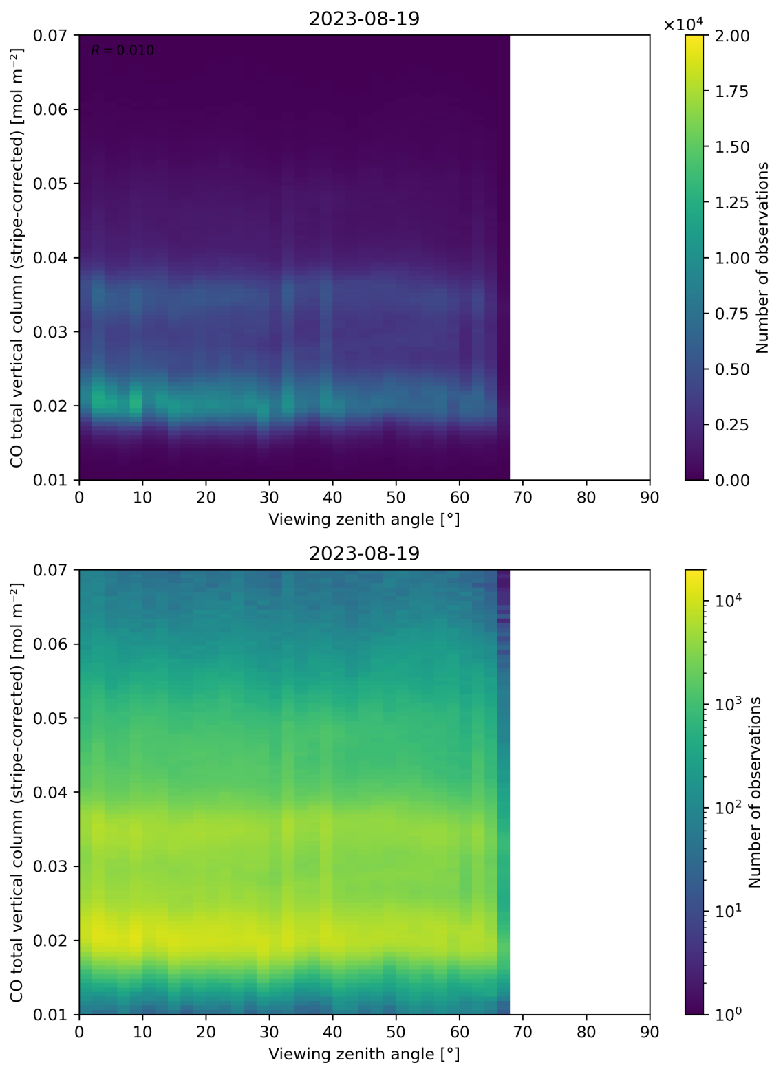
Figure 70: Scatter density plot of “Viewing zenith angle” against “CO total vertical column (stripe-corrected)” for 2023-08-18 to 2023-08-20.
