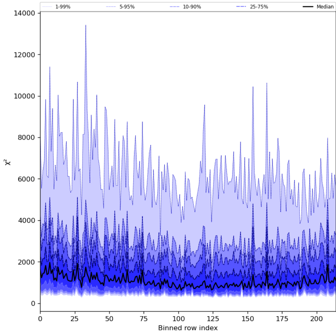
Figure 30: Along track statistics of “ \chi^2 ” for 2023-08-18 to 2023-08-20
