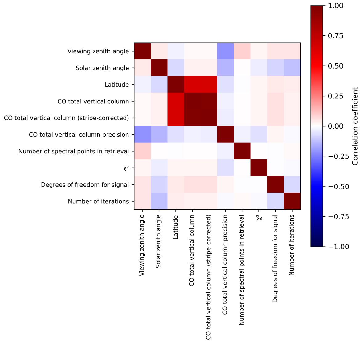
Figure 2: Map of correlation matrix for 2023-08-18 to 2023-08-20.
