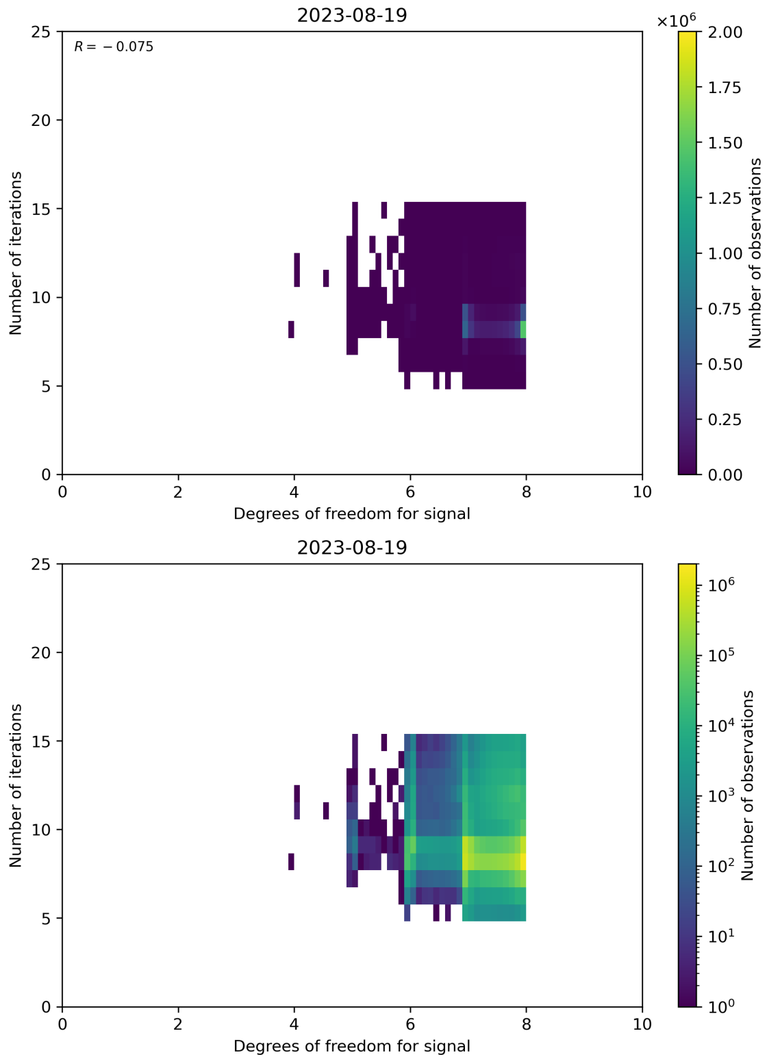
Figure 50: Scatter density plot of “Degrees of freedom for signal” against “Number of iterations” for 2023-08-18 to 2023-08-20.
