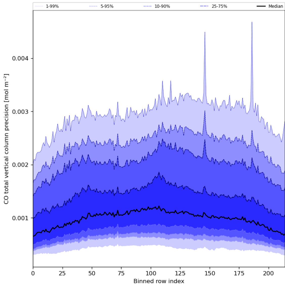
Figure 28: Along track statistics of “CO total vertical column precision” for 2023-08-18 to 2023-08-20
