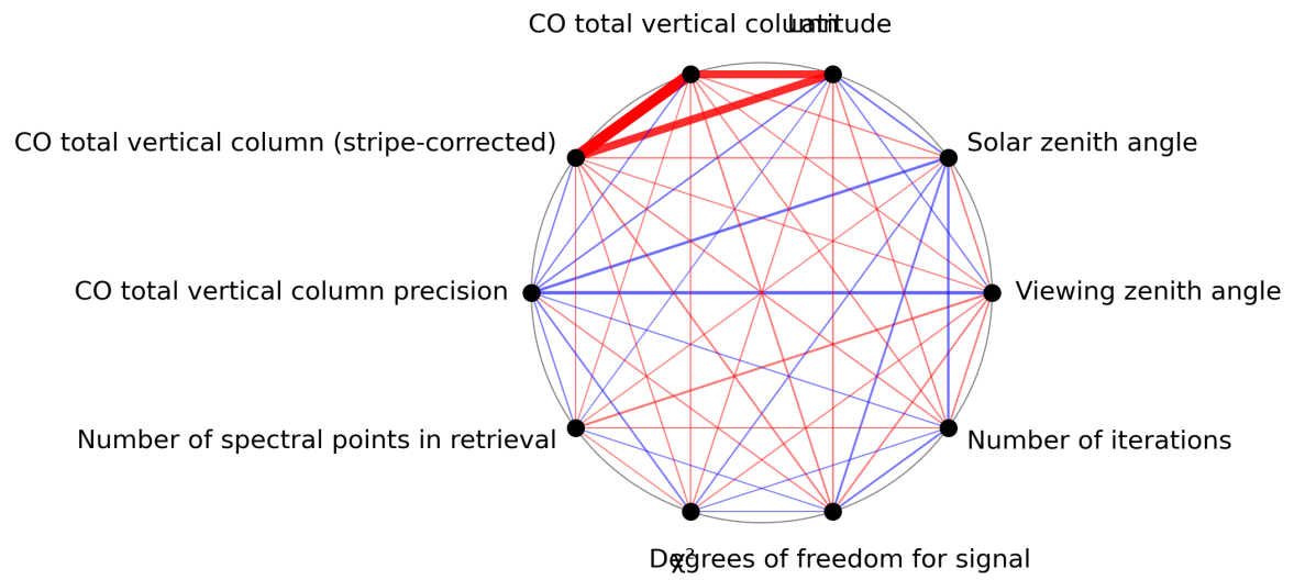
Figure 1: Map of correlation graph for 2023-08-18 to 2023-08-20.
