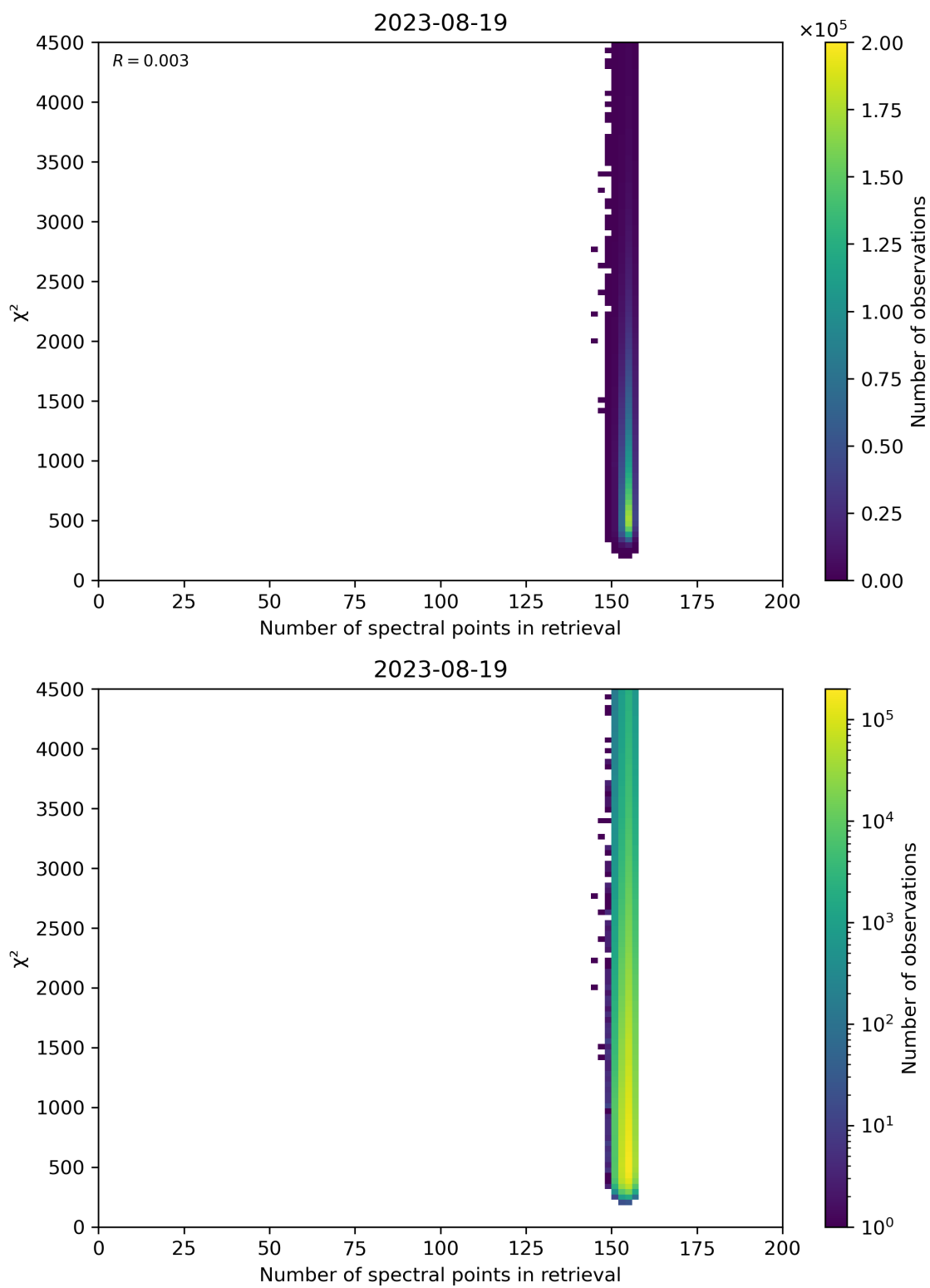
Figure 58: Scatter density plot of “Number of spectral points in retrieval” against “ \chi^2 ” for 2023-08-18 to 2023-08-20.
