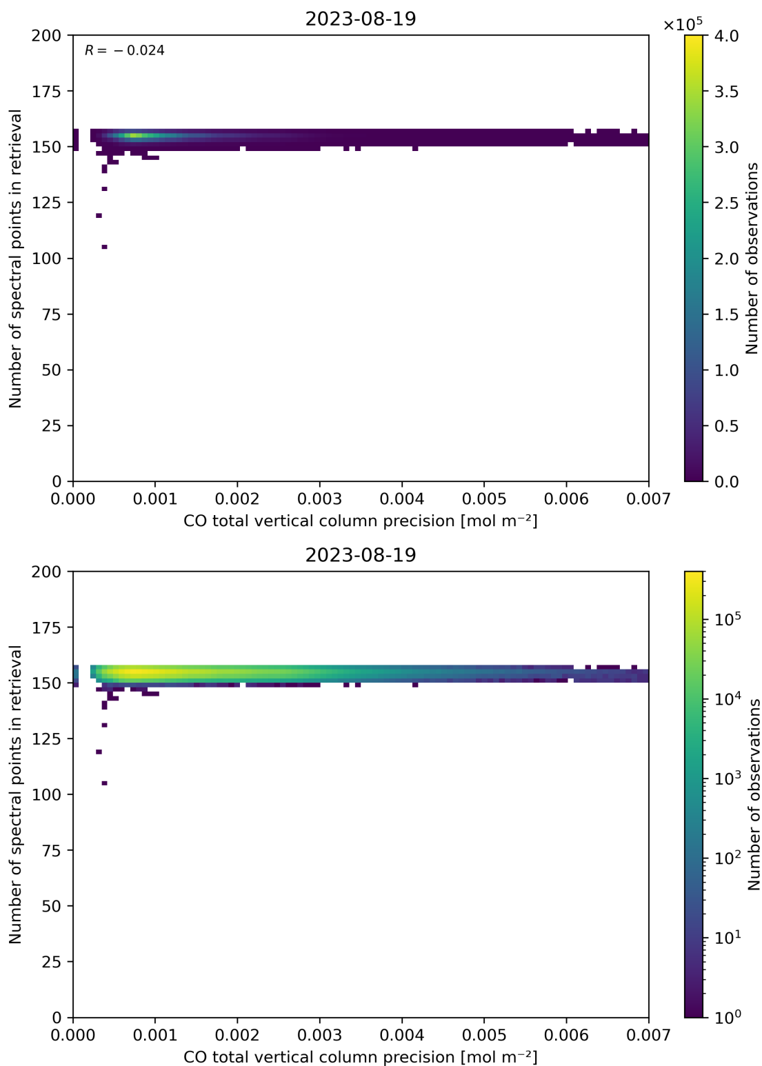
Figure 47: Scatter density plot of “CO total vertical column precision” against “Number of spectral points in retrieval” for 2023-08-18 to 2023-08-20.
