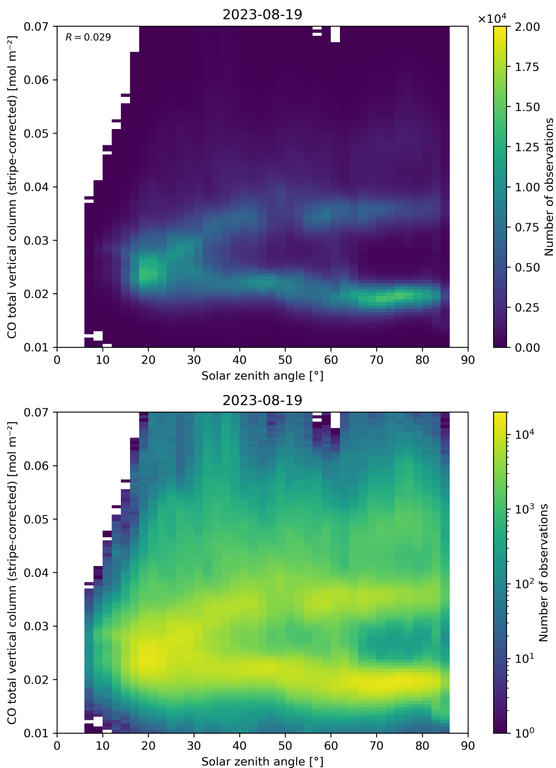
Figure 62: Scatter density plot of “Solar zenith angle” against “CO total vertical column (stripe-corrected)” for 2023-08-18 to 2023-08-20.
