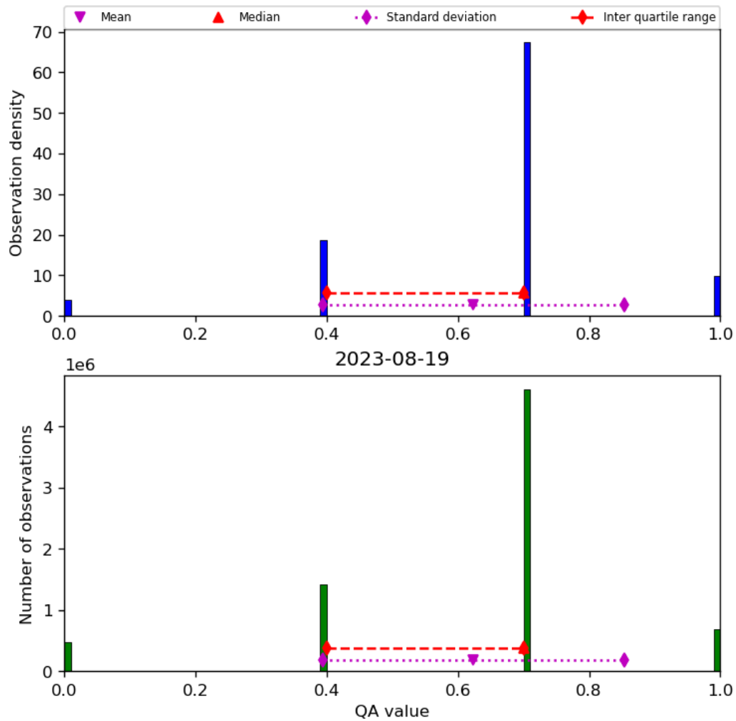
Figure 17: Histogram of “QA value” for 2023-08-18 to 2023-08-20
