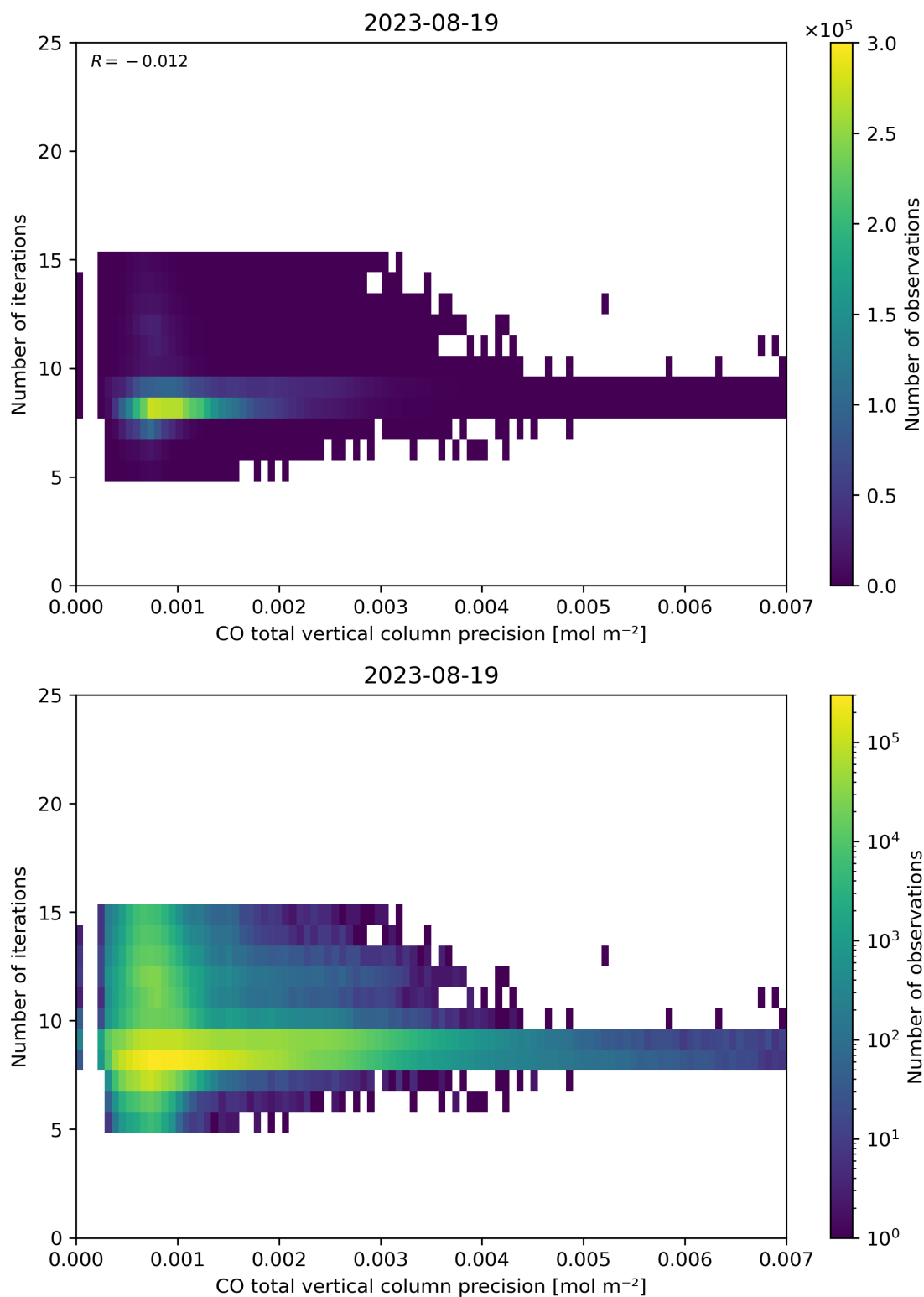
Figure 46: Scatter density plot of “CO total vertical column precision” against “Number of iterations” for 2023-08-18 to 2023-08-20.
