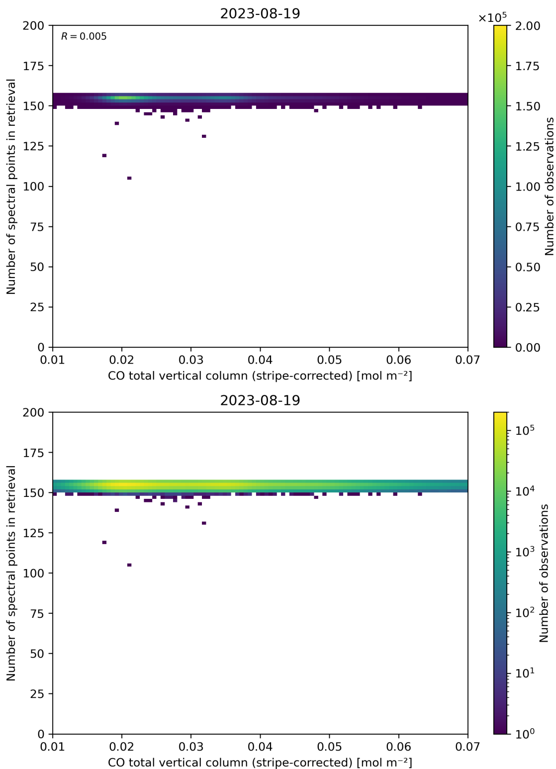
Figure 40: Scatter density plot of “CO total vertical column (stripe-corrected)” against “Number of spectral points in retrieval” for 2023-08-18 to 2023-08-20.
