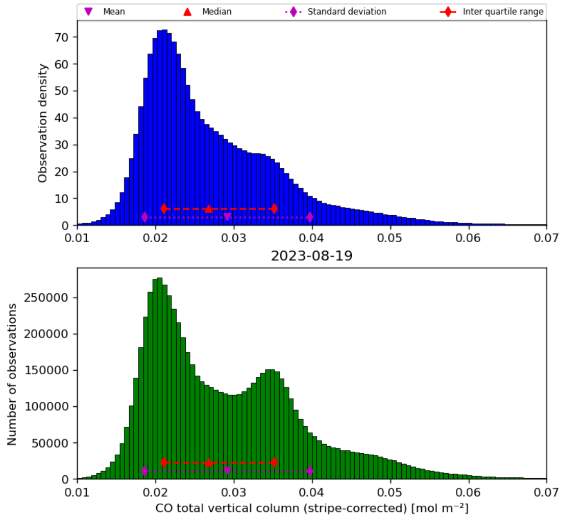
Figure 19: Histogram of “CO total vertical column (stripe-corrected)” for 2023-08-18 to 2023-08-20
