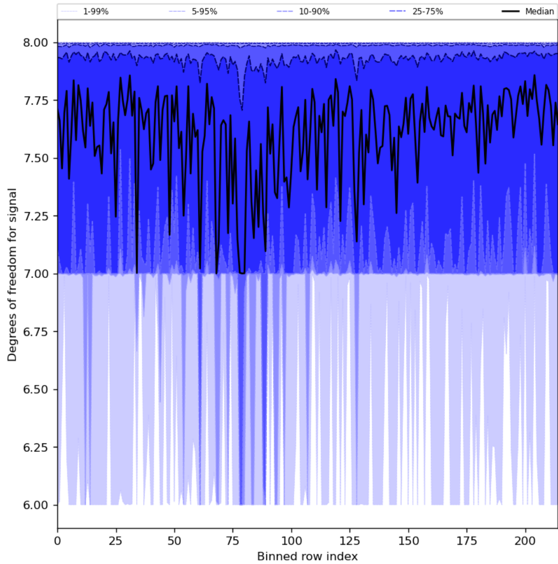
Figure 31: Along track statistics of “Degrees of freedom for signal” for 2023-08-18 to 2023-08-20
