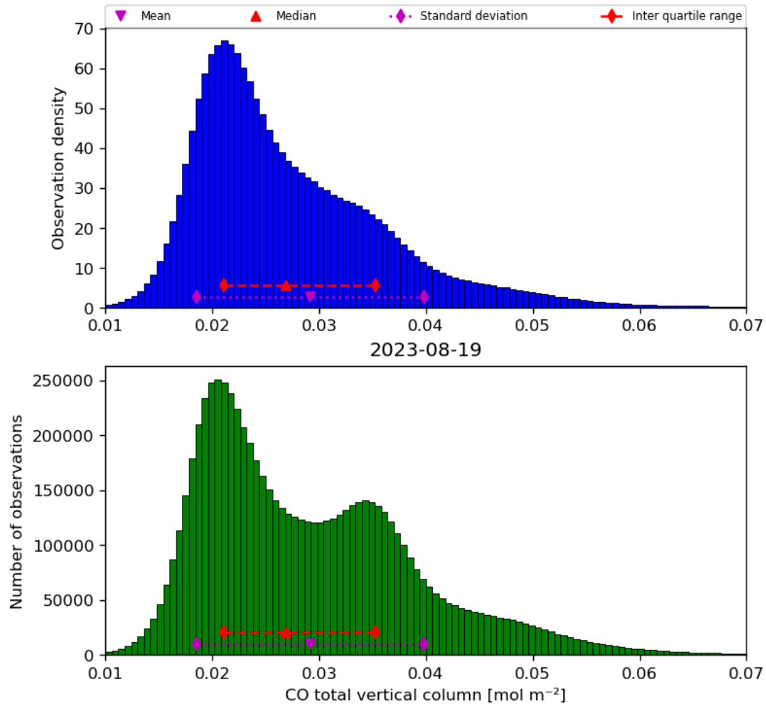
Figure 18: Histogram of “CO total vertical column” for 2023-08-18 to 2023-08-20
