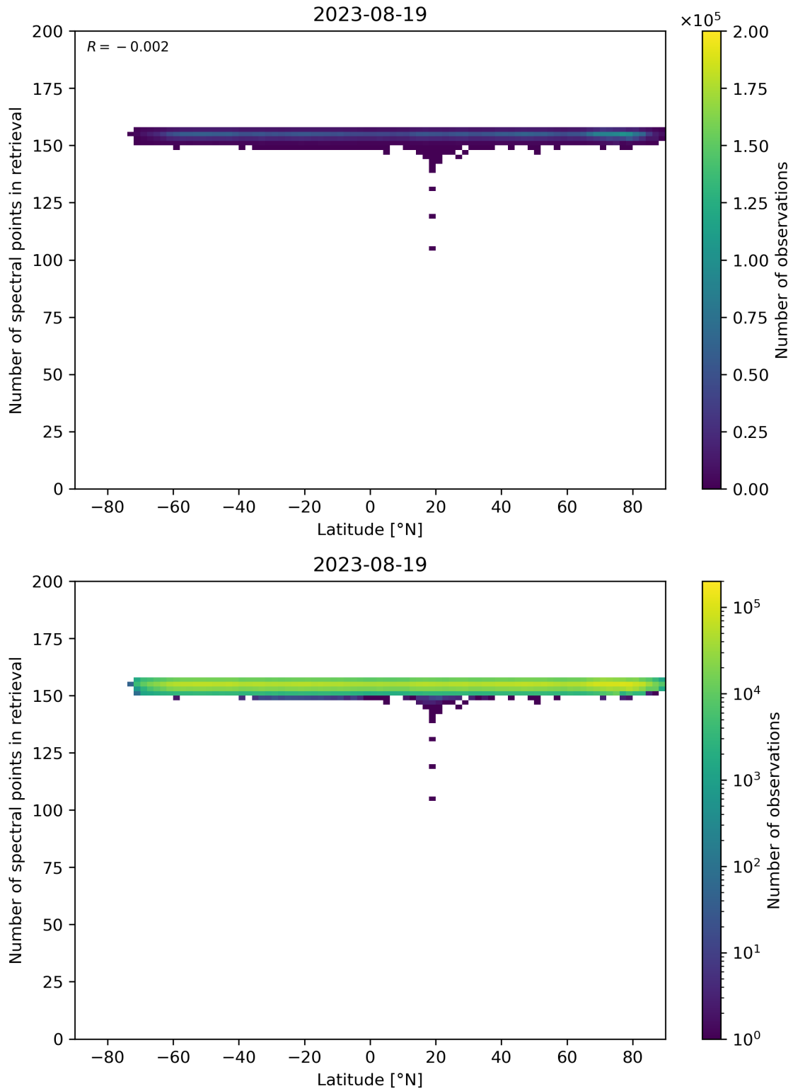
Figure 57: Scatter density plot of “Latitude” against “Number of spectral points in retrieval” for 2023-08-18 to 2023-08-20.
