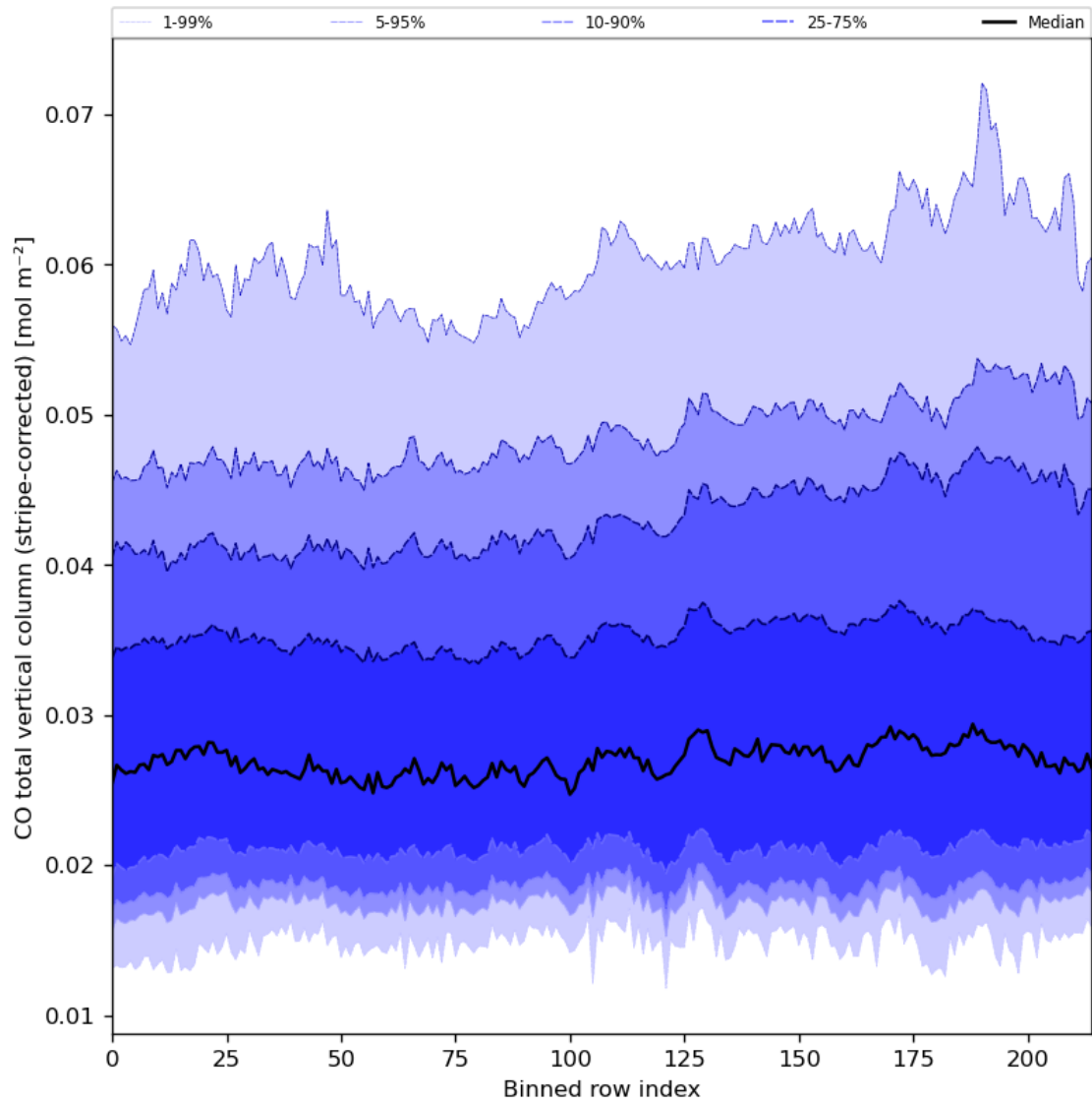
Figure 27: Along track statistics of “CO total vertical column (stripe-corrected)” for 2023-08-18 to 2023-08-20
