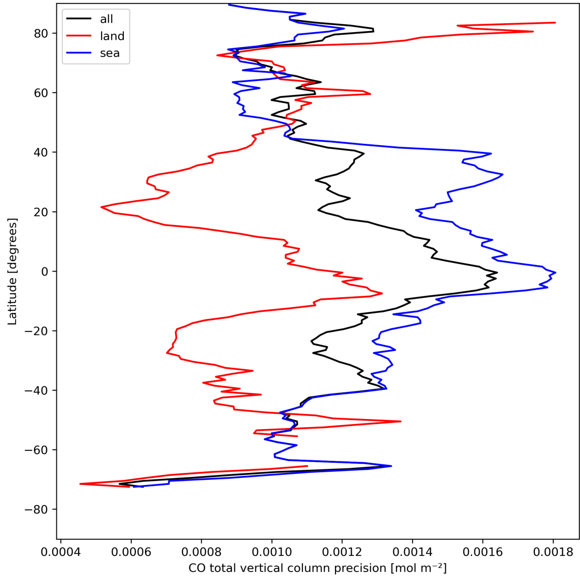
Figure 12: Zonal average of “CO total vertical column precision” for 2023-08-18 to 2023-08-20.
