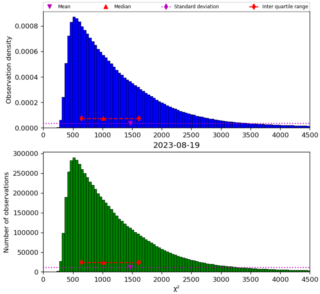
Figure 22: Histogram of “ \chi^2 ” for 2023-08-18 to 2023-08-20
