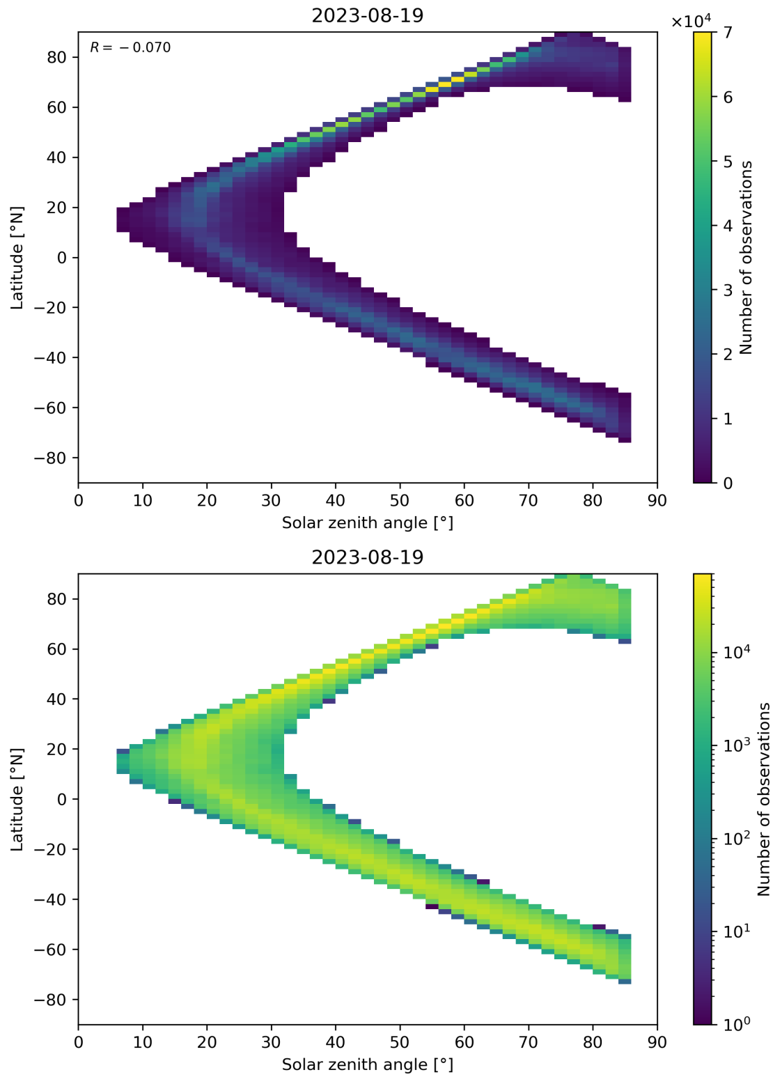
Figure 66: Scatter density plot of “Solar zenith angle” against “Latitude” for 2023-08-18 to 2023-08-20.
