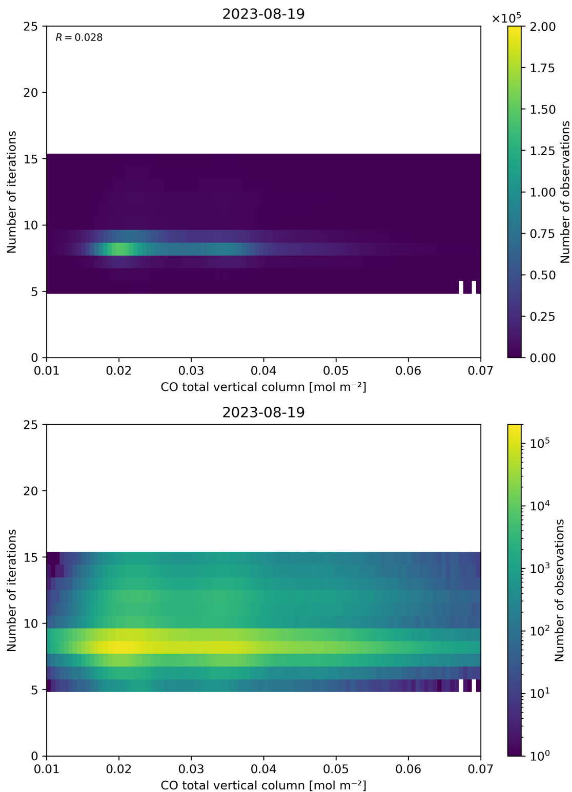
Figure 42: Scatter density plot of “CO total vertical column” against “Number of iterations” for 2023-08-18 to 2023-08-20.
