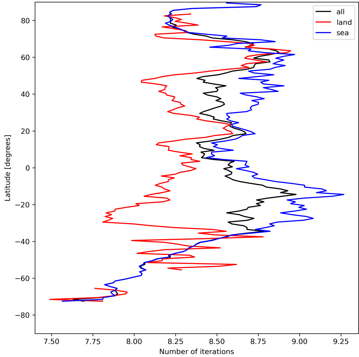
Figure 16: Zonal average of “Number of iterations” for 2023-08-18 to 2023-08-20.
