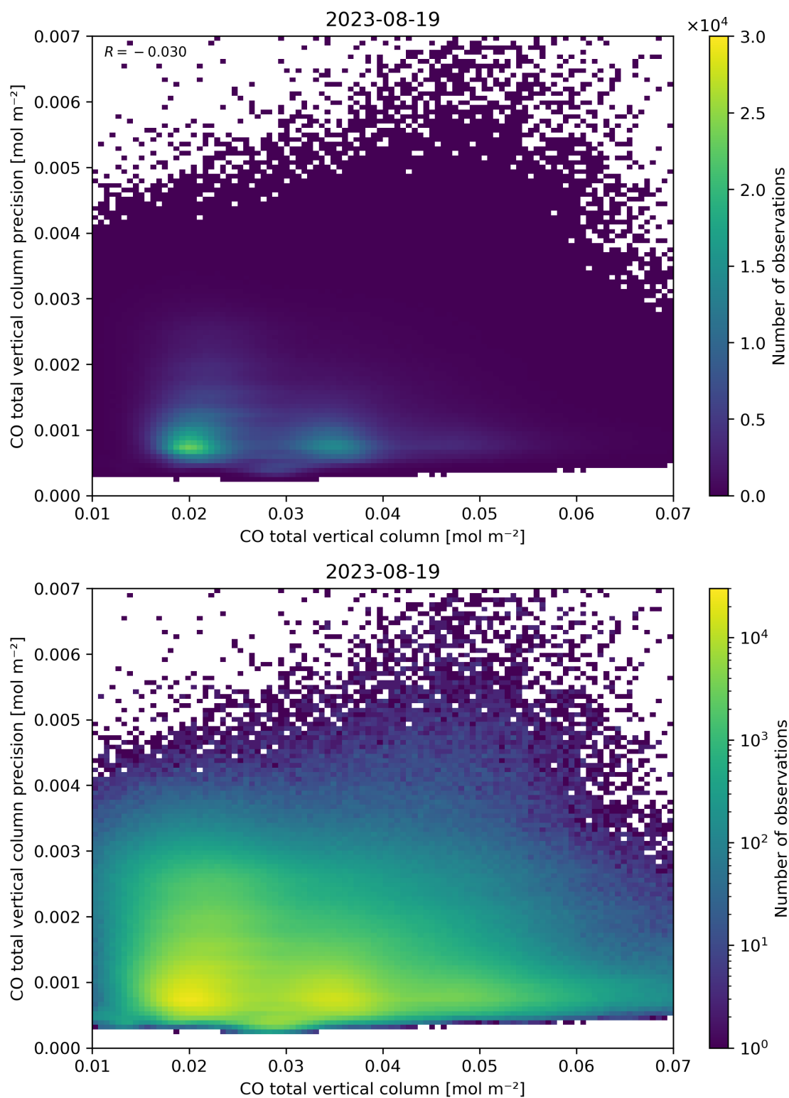
Figure 34: Scatter density plot of “CO total vertical column” against “CO total vertical column precision” for 2023-08-18 to 2023-08-20.
