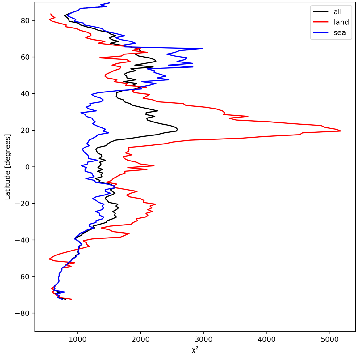
Figure 14: Zonal average of “ \chi^2 ” for 2023-08-18 to 2023-08-20.
