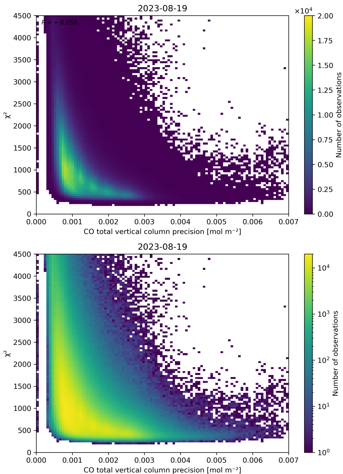
Figure 44: Scatter density plot of “CO total vertical column precision” against “ \chi^2 ” for 2023-08-18 to 2023-08-20.
