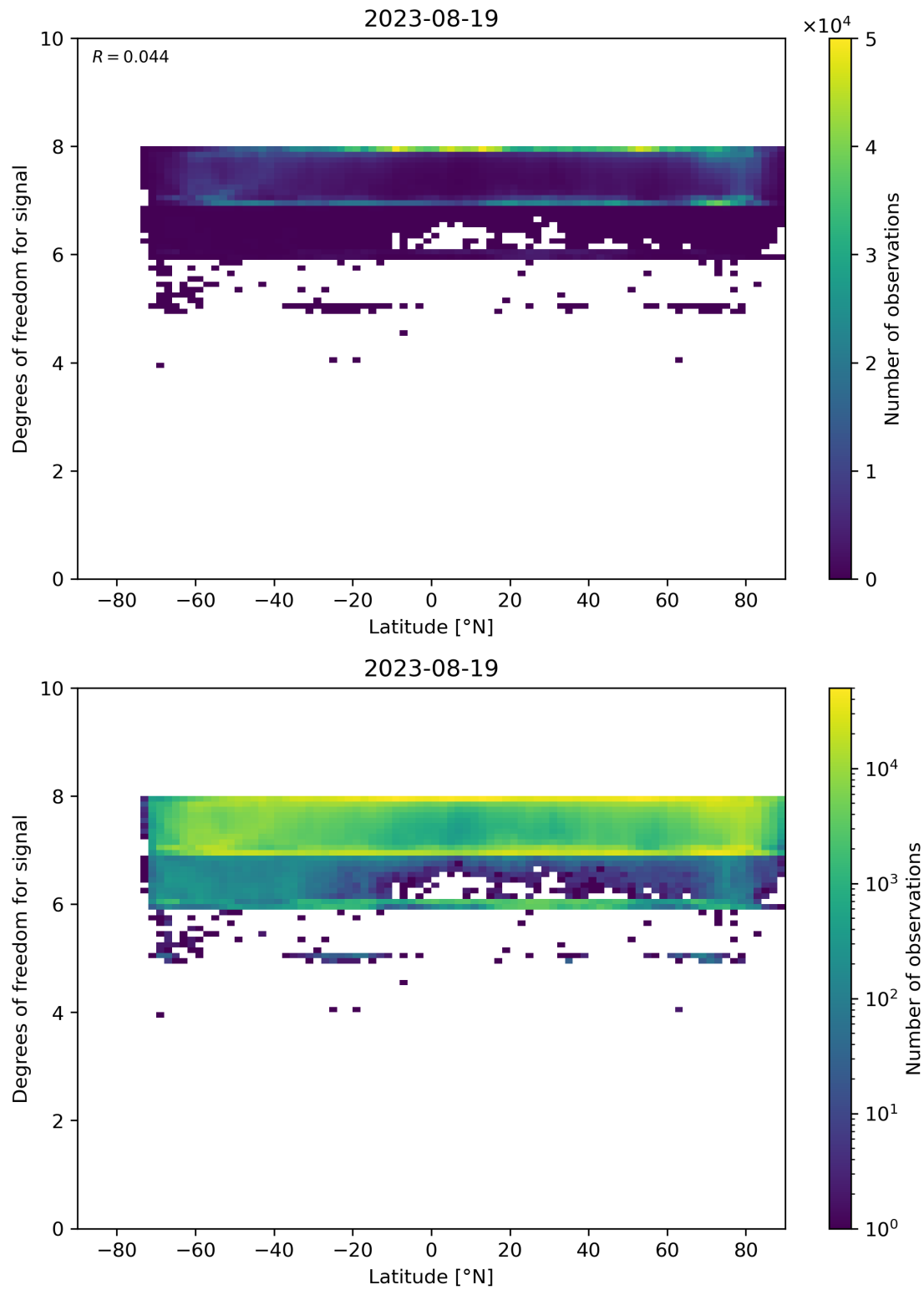
Figure 55: Scatter density plot of “Latitude” against “Degrees of freedom for signal” for 2023-08-18 to 2023-08-20.
