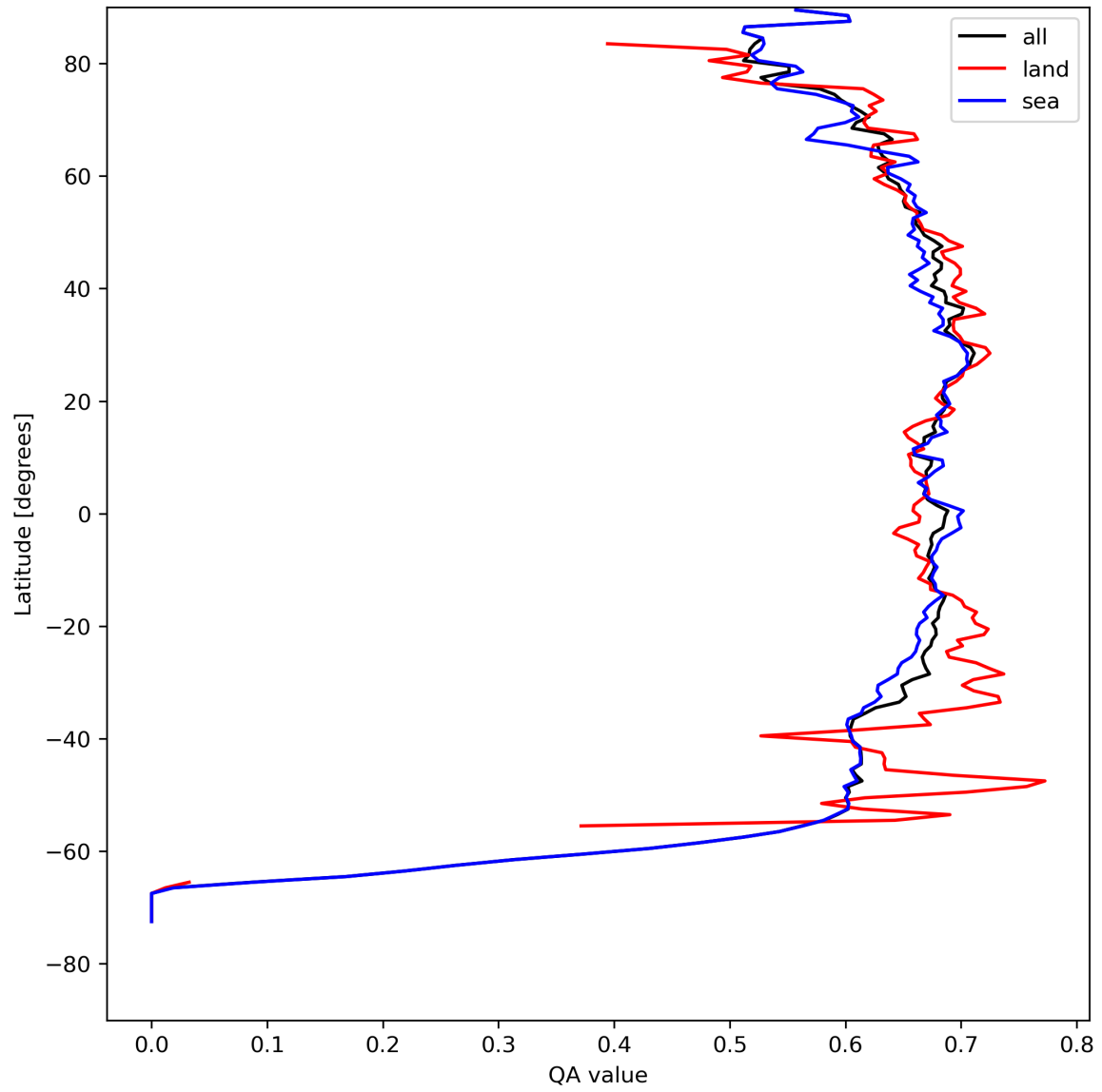
Figure 9: Zonal average of “QA value” for 2023-08-18 to 2023-08-20.
