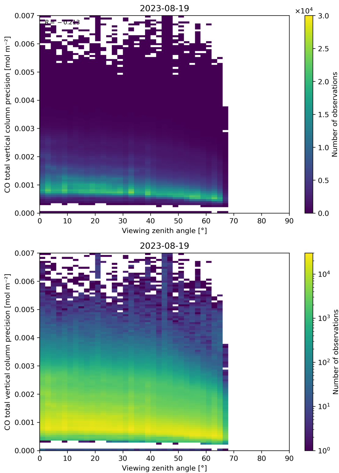
Figure 71: Scatter density plot of “Viewing zenith angle” against “CO total vertical column precision” for 2023-08-18 to 2023-08-20.
