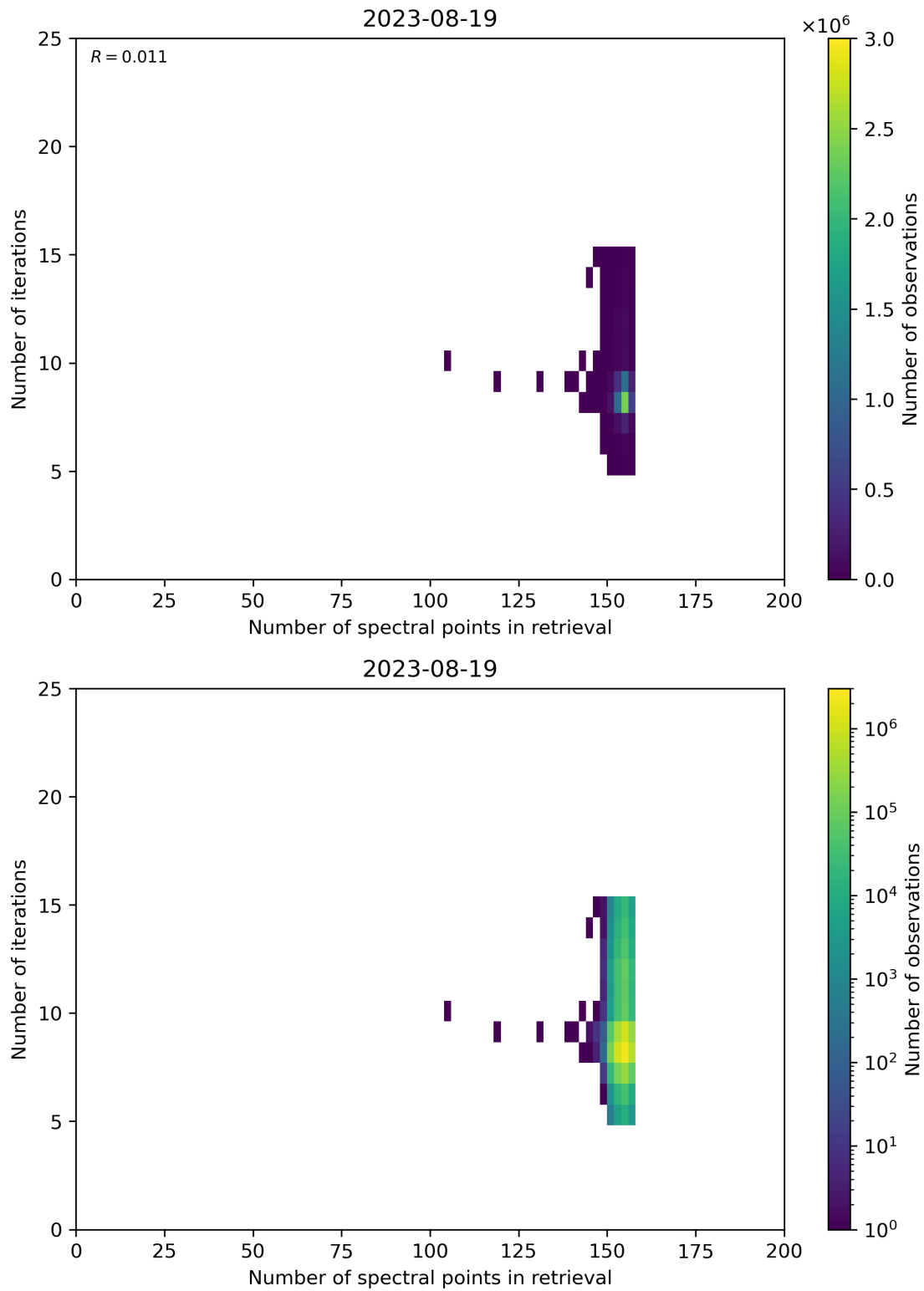
Figure 60: Scatter density plot of “Number of spectral points in retrieval” against “Number of iterations” for 2023-08-18 to 2023-08-20.
