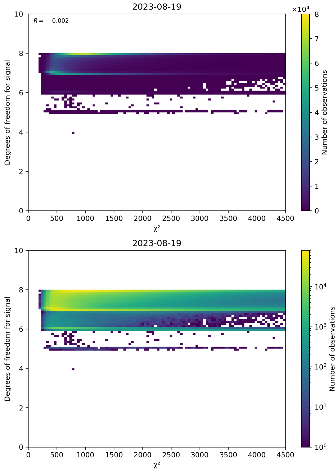
Figure 48: Scatter density plot of “ \chi^2 ” against “Degrees of freedom for signal” for 2023-08-18 to 2023-08-20.
