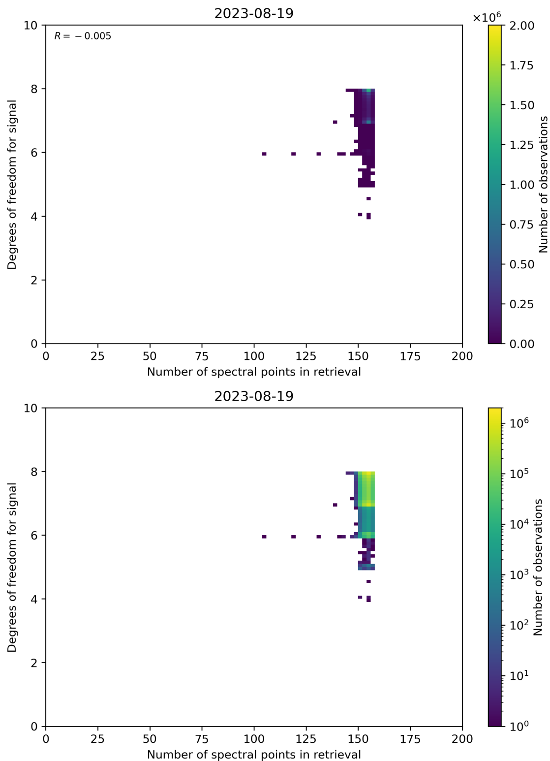
Figure 59: Scatter density plot of “Number of spectral points in retrieval” against “Degrees of freedom for signal” for 2023-08-18 to 2023-08-20.
