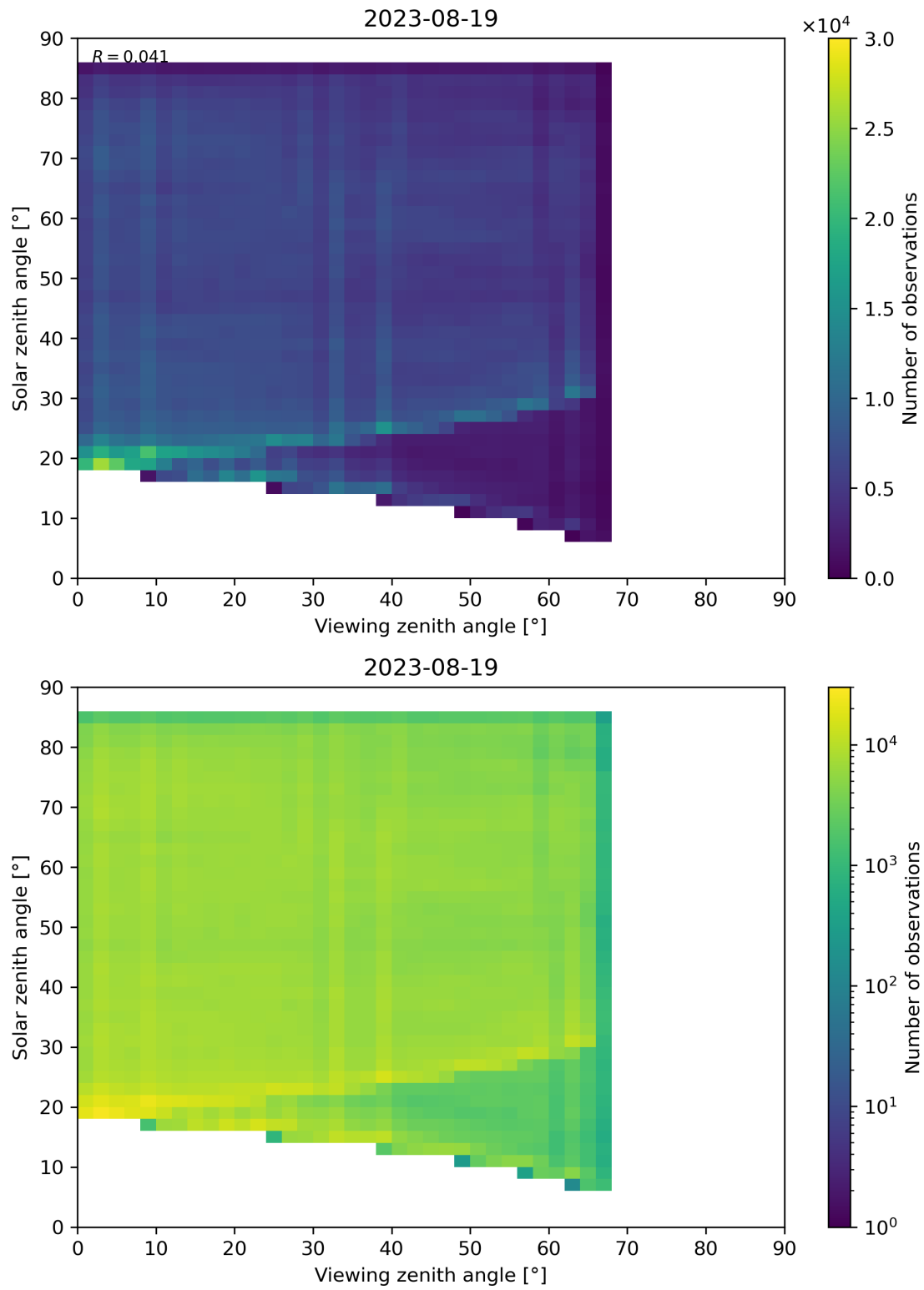
Figure 77: Scatter density plot of “Viewing zenith angle” against “Solar zenith angle” for 2023-08-18 to 2023-08-20.
