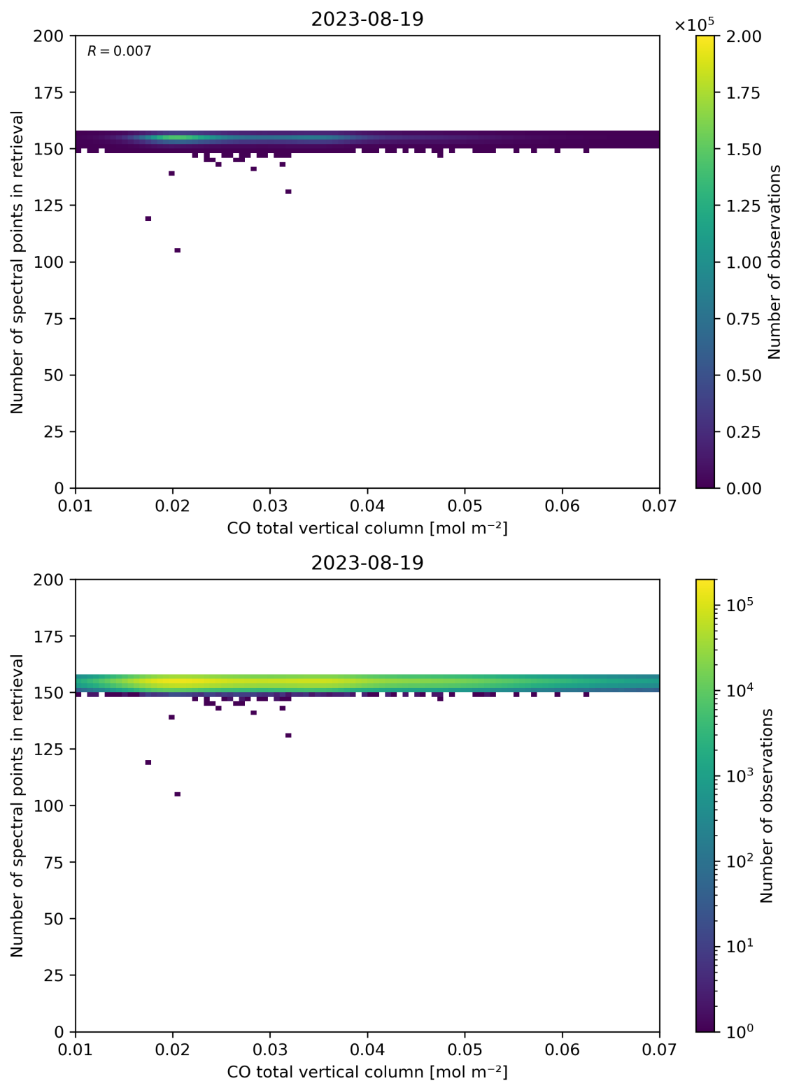
Figure 43: Scatter density plot of “CO total vertical column” against “Number of spectral points in retrieval” for 2023-08-18 to 2023-08-20.
