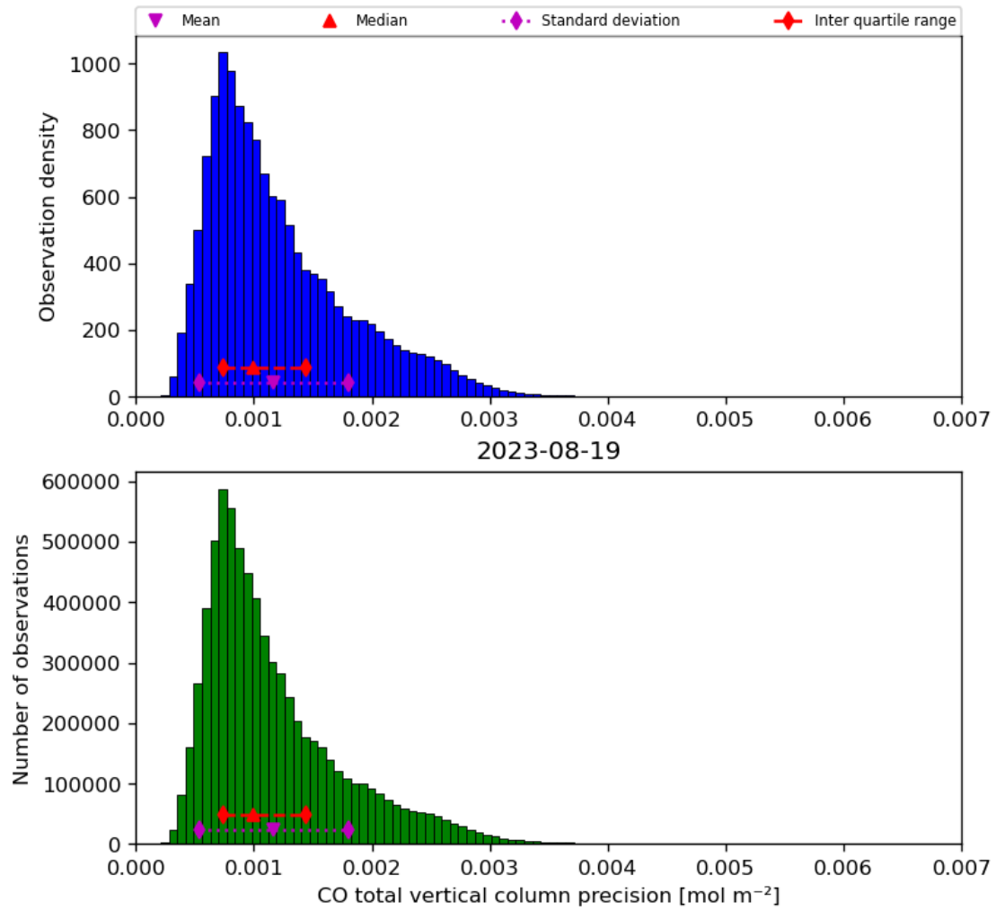
Figure 20: Histogram of “CO total vertical column precision” for 2023-08-18 to 2023-08-20
