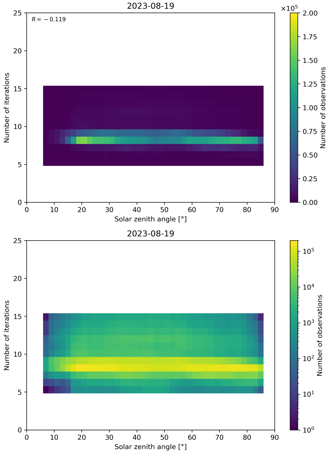
Figure 67: Scatter density plot of “Solar zenith angle” against “Number of iterations” for 2023-08-18 to 2023-08-20.
