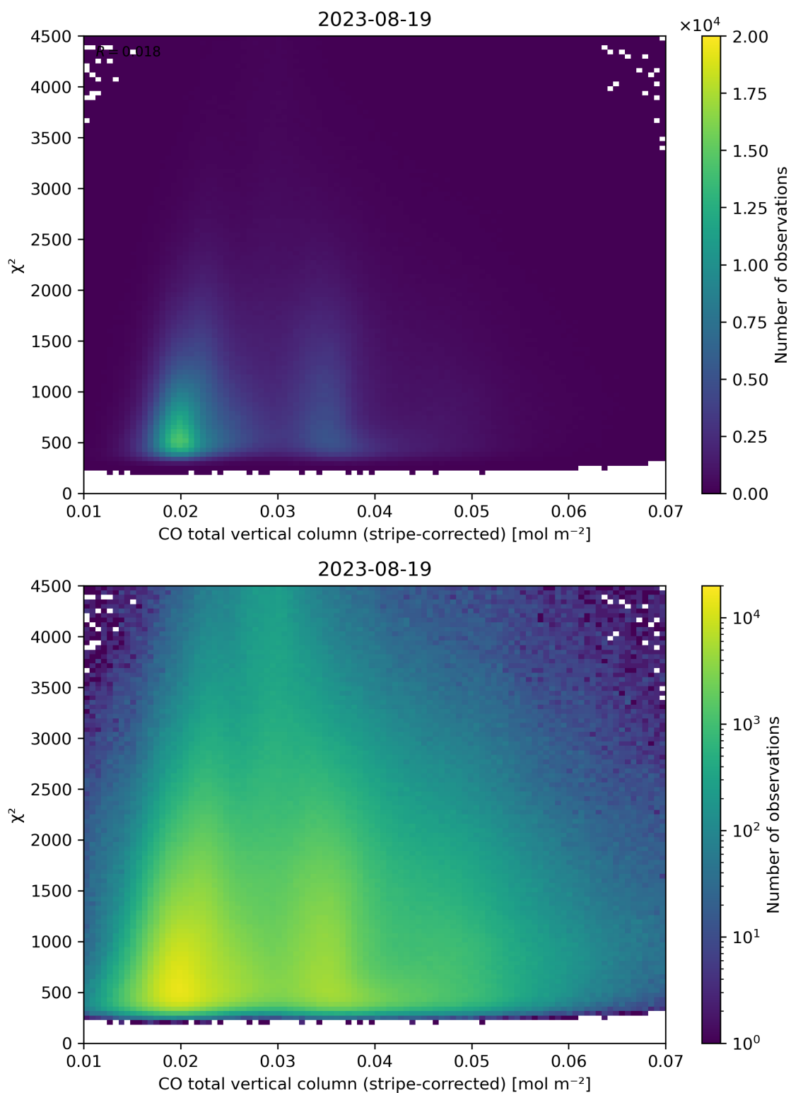
Figure 37: Scatter density plot of “CO total vertical column (stripe-corrected)” against “ \chi^2 ” for 2023-08-18 to 2023-08-20.
