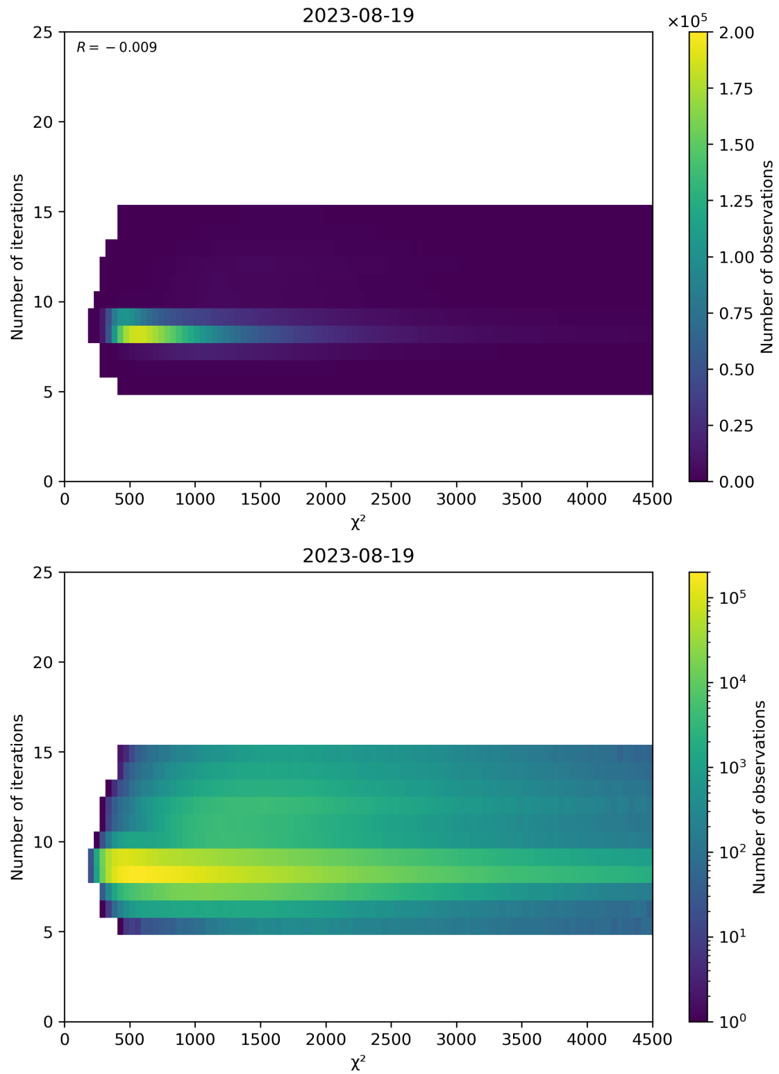
Figure 49: Scatter density plot of “ \chi^2 ” against “Number of iterations” for 2023-08-18 to 2023-08-20.
