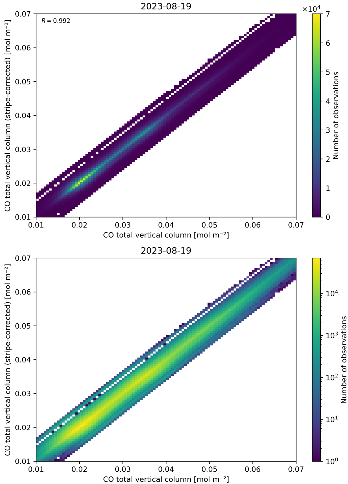
Figure 33: Scatter density plot of “CO total vertical column” against “CO total vertical column (stripe-corrected)” for 2023-08-18 to 2023-08-20.
