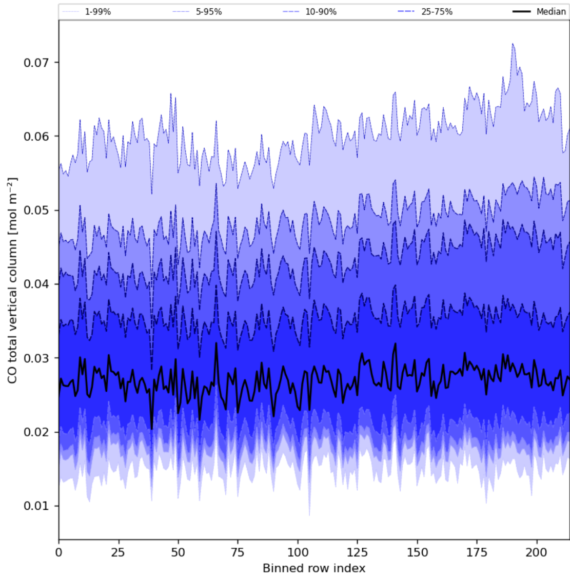
Figure 26: Along track statistics of “CO total vertical column” for 2023-08-18 to 2023-08-20
