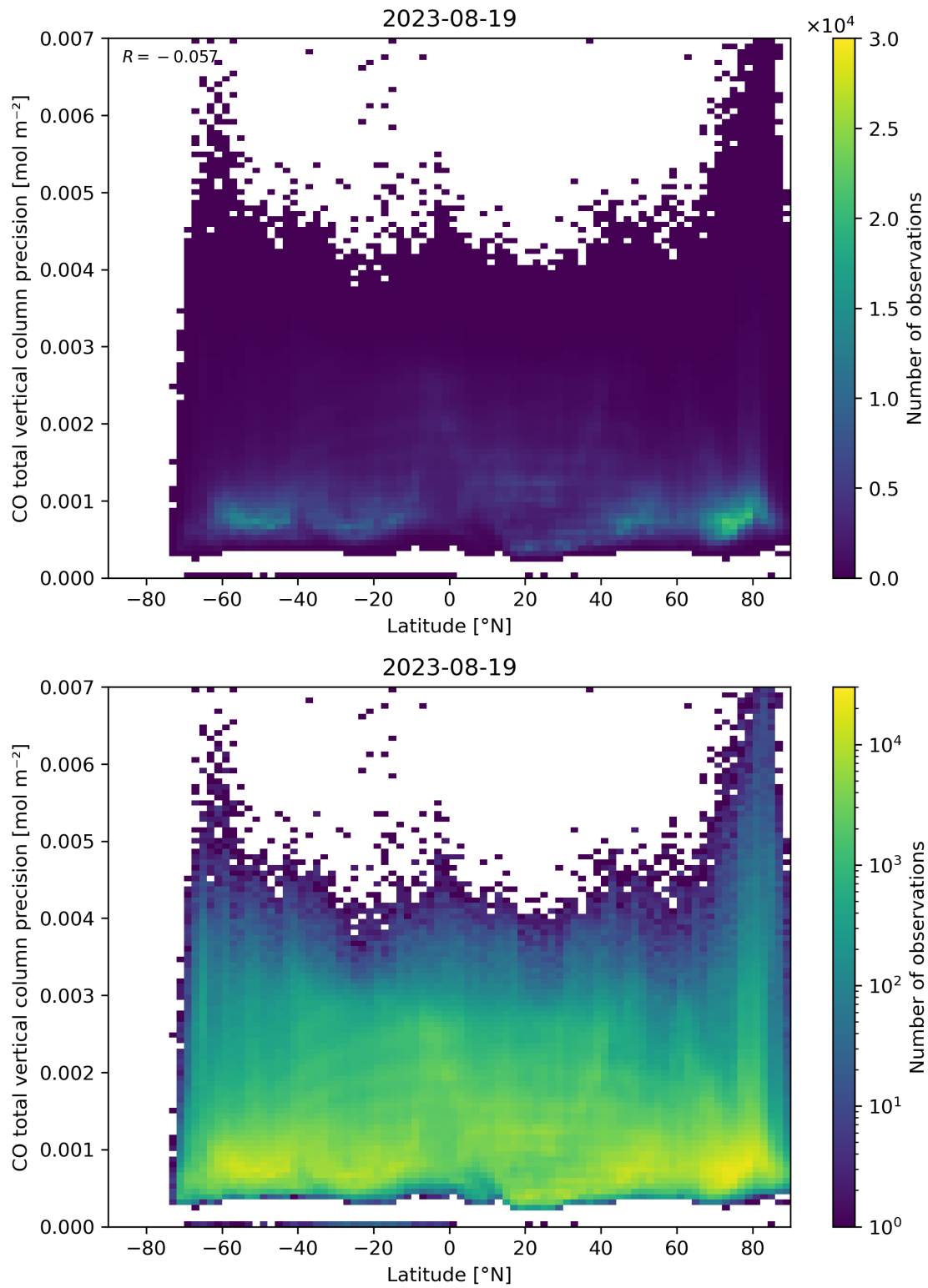
Figure 53: Scatter density plot of “Latitude” against “CO total vertical column precision” for 2023-08-18 to 2023-08-20.
