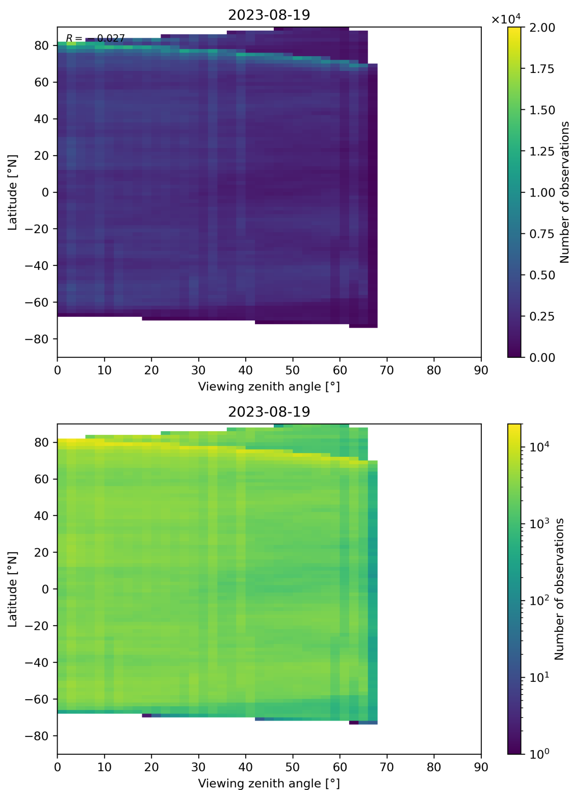
Figure 74: Scatter density plot of “Viewing zenith angle” against “Latitude” for 2023-08-18 to 2023-08-20.
