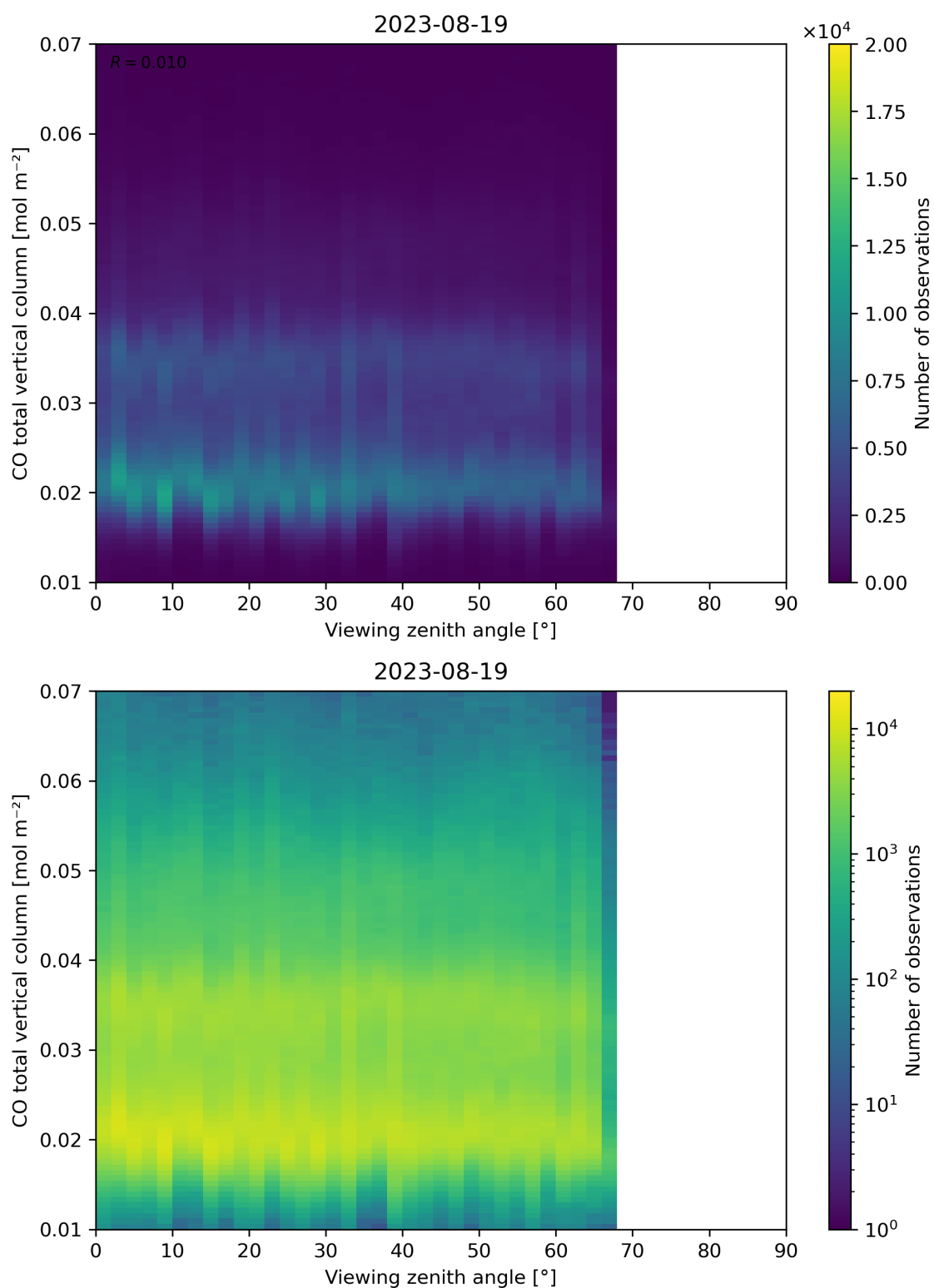
Figure 69: Scatter density plot of “Viewing zenith angle” against “CO total vertical column” for 2023-08-18 to 2023-08-20.
