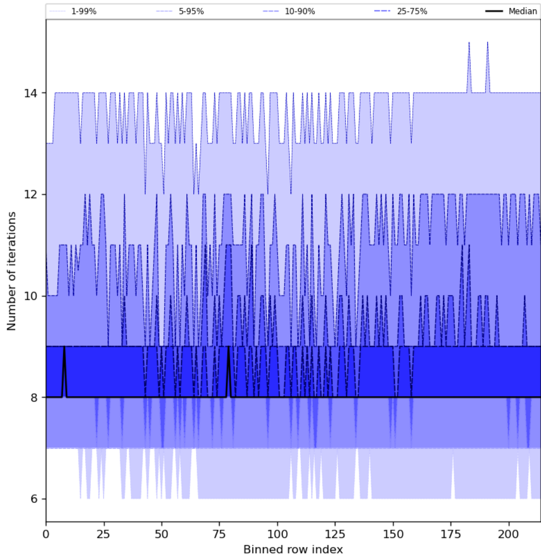
Figure 32: Along track statistics of “Number of iterations” for 2023-08-18 to 2023-08-20
