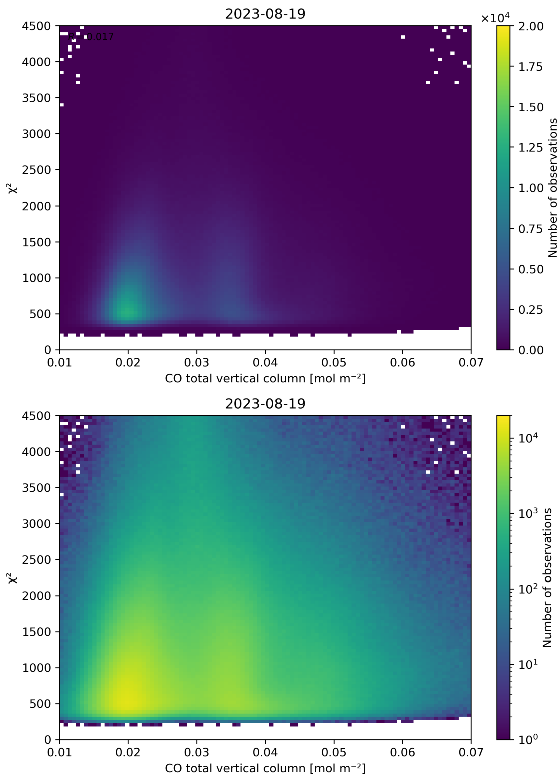
Figure 35: Scatter density plot of “CO total vertical column” against “ \chi^2 ” for 2023-08-18 to 2023-08-20.
