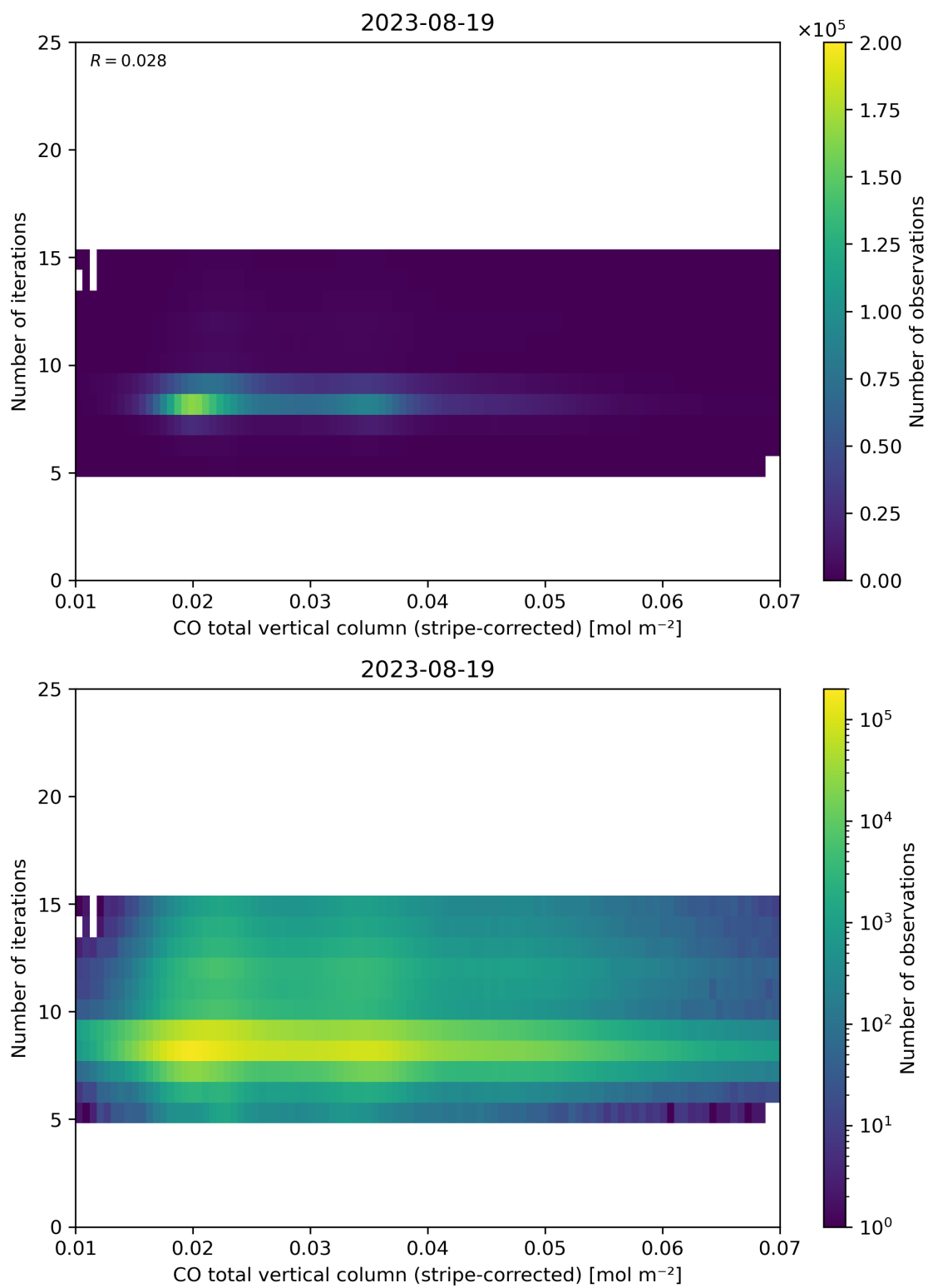
Figure 39: Scatter density plot of “CO total vertical column (stripe-corrected)” against “Number of iterations” for 2023-08-18 to 2023-08-20.
