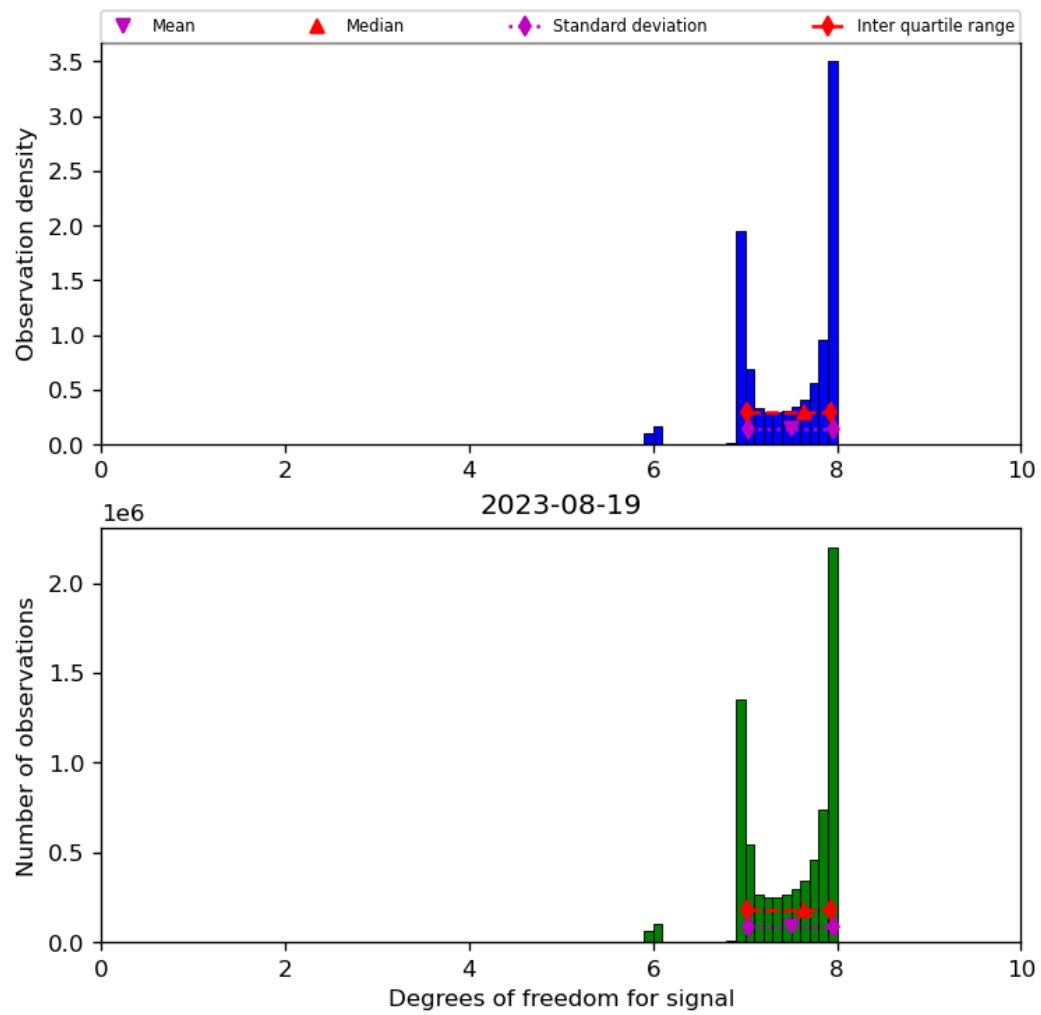
Figure 23: Histogram of “Degrees of freedom for signal” for 2023-08-18 to 2023-08-20
