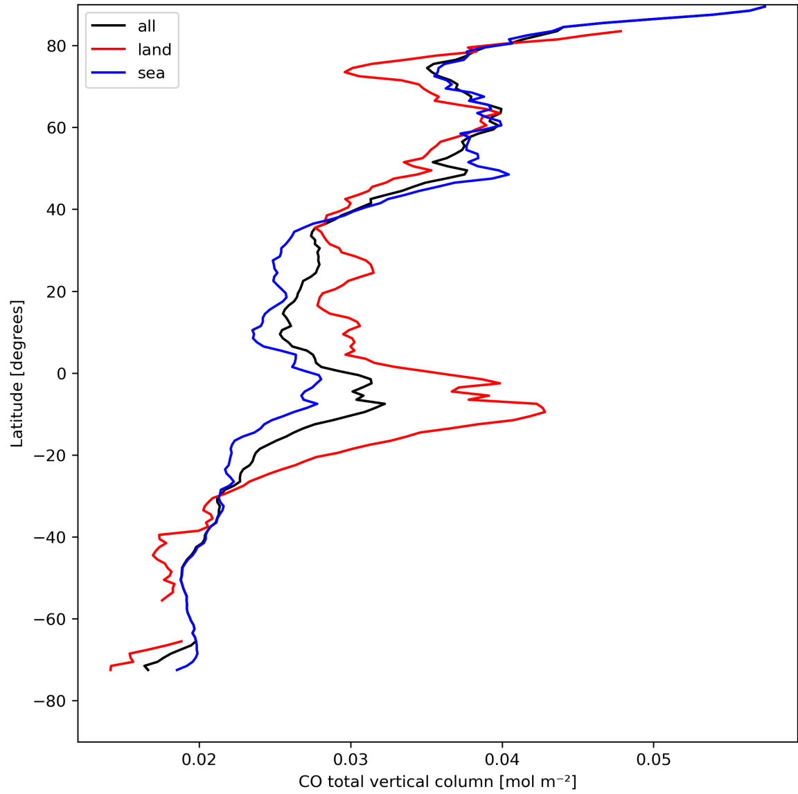
Figure 10: Zonal average of “CO total vertical column” for 2023-08-18 to 2023-08-20.
