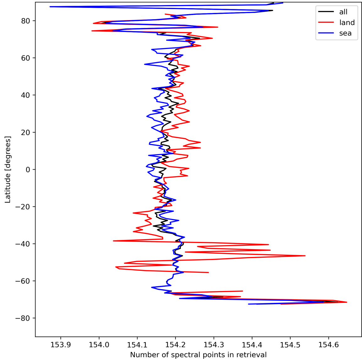
Figure 13: Zonal average of “Number of spectral points in retrieval” for 2023-08-18 to 2023-08-20.
