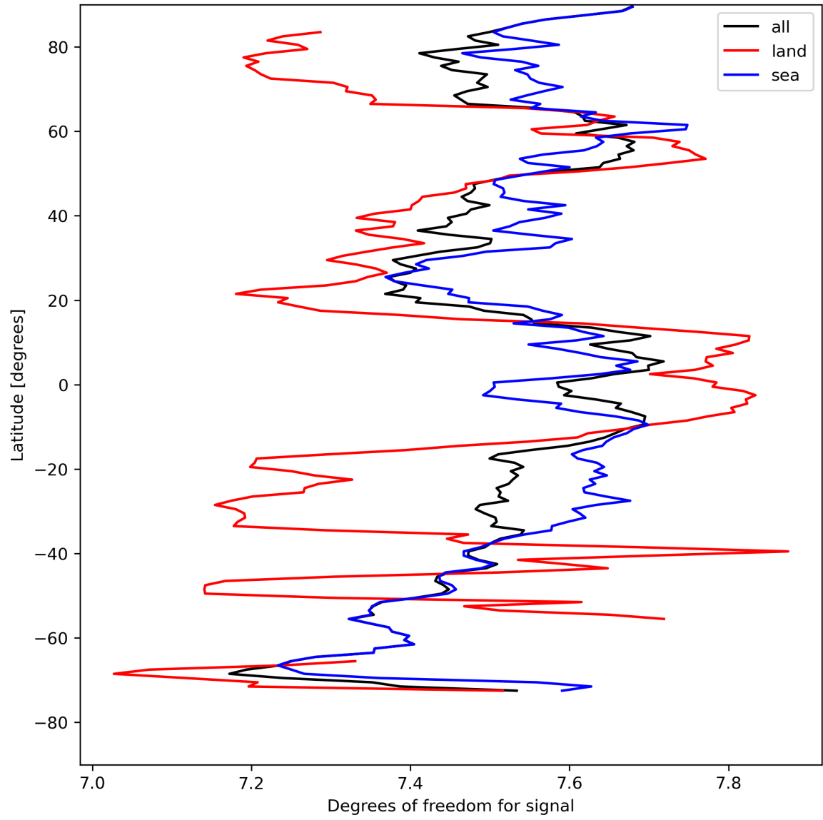
Figure 15: Zonal average of “Degrees of freedom for signal” for 2023-08-18 to 2023-08-20.
