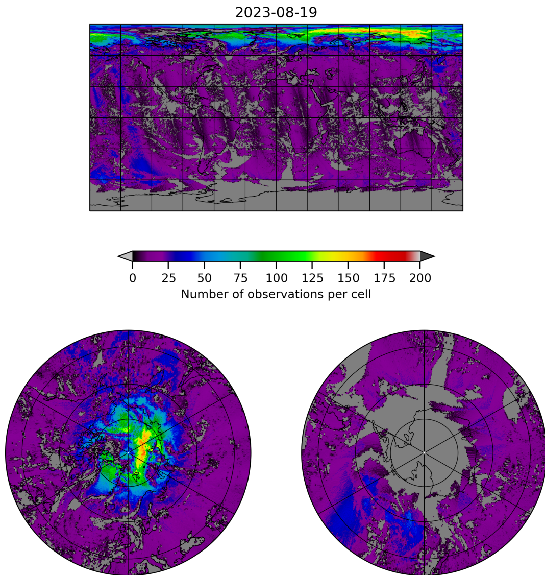
Figure 8: Map of the number of observations for 2023-08-18 to 2023-08-20
