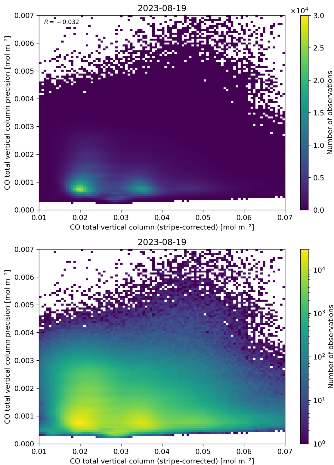
Figure 36: Scatter density plot of “CO total vertical column (stripe-corrected)” against “CO total vertical column precision” for 2023-08-18 to 2023-08-20.
