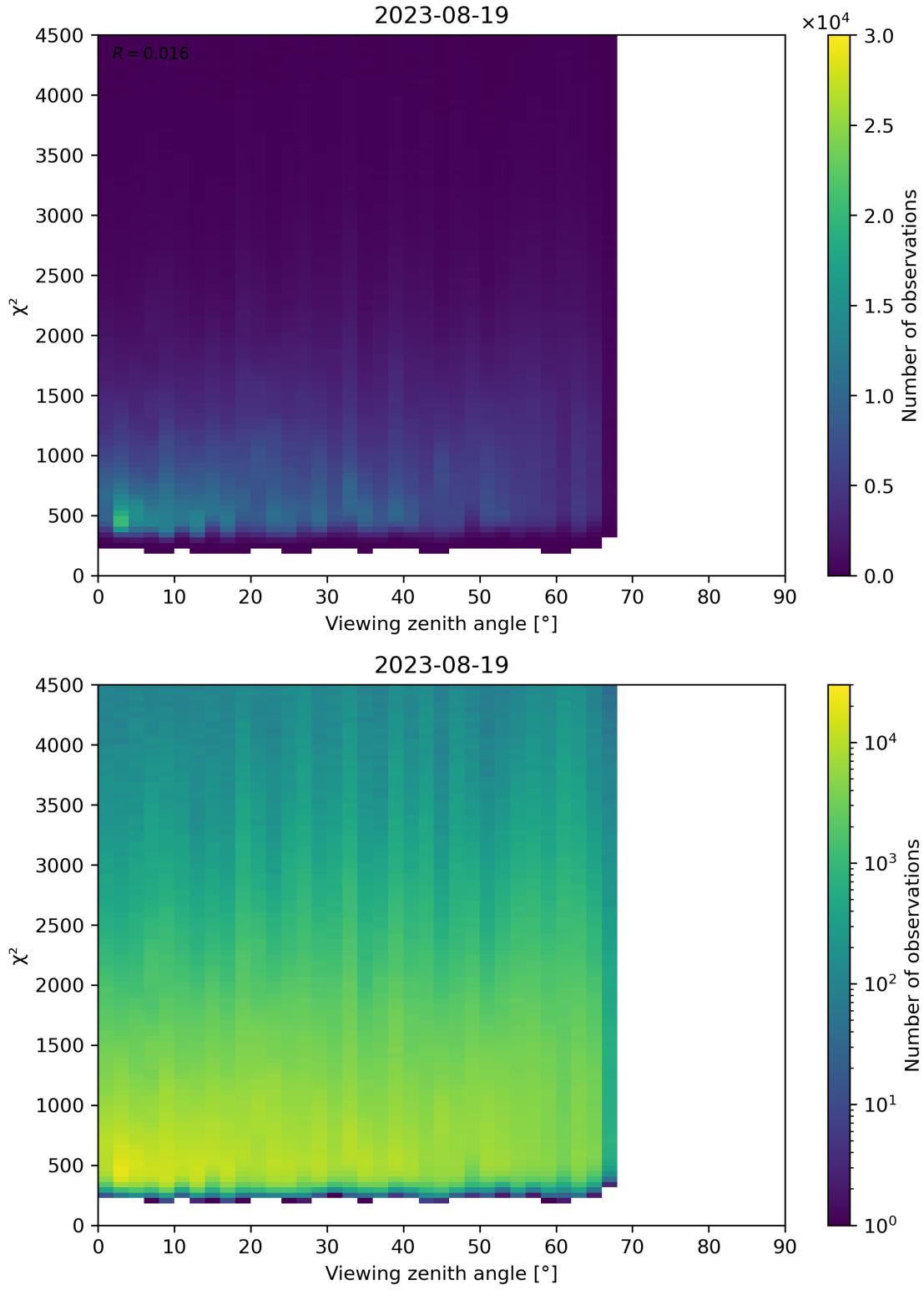
Figure 72: Scatter density plot of “Viewing zenith angle” against “ \chi^2 ” for 2023-08-18 to 2023-08-20.
