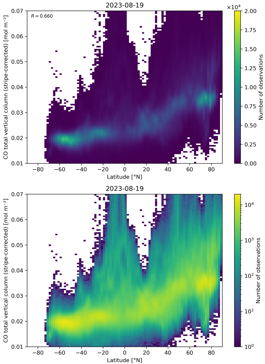
Figure 52: Scatter density plot of “Latitude” against “CO total vertical column (stripe-corrected)” for 2023-08-18 to 2023-08-20.
