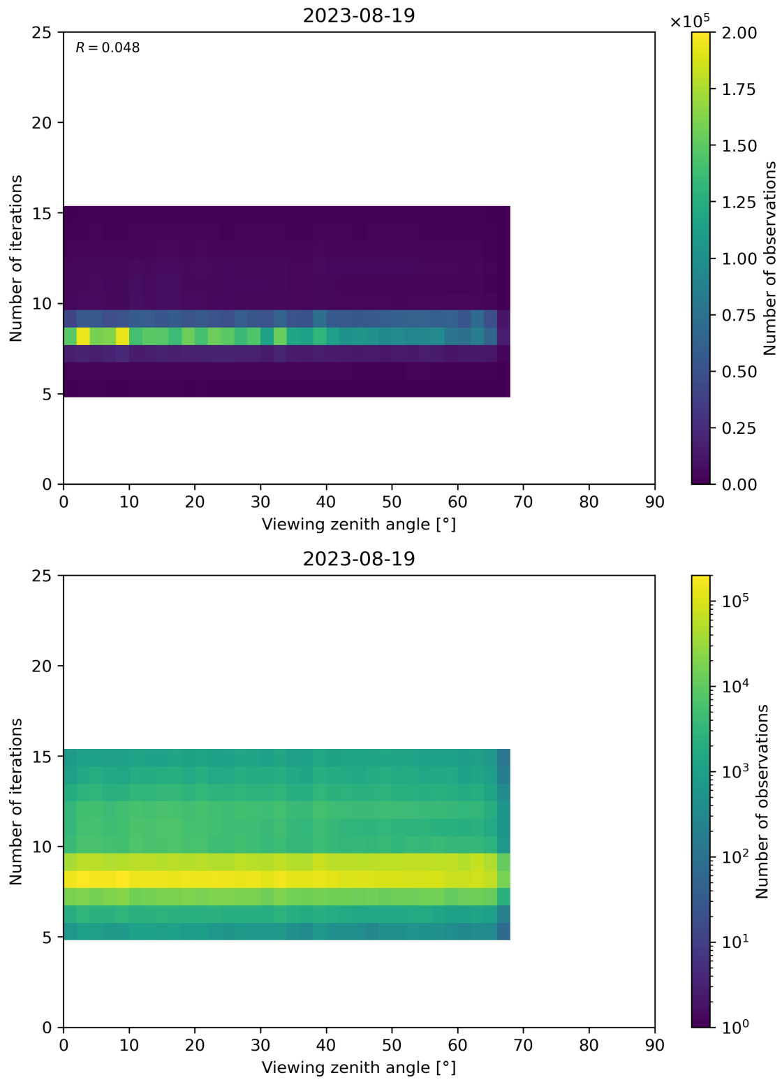
Figure 75: Scatter density plot of “Viewing zenith angle” against “Number of iterations” for 2023-08-18 to 2023-08-20.
