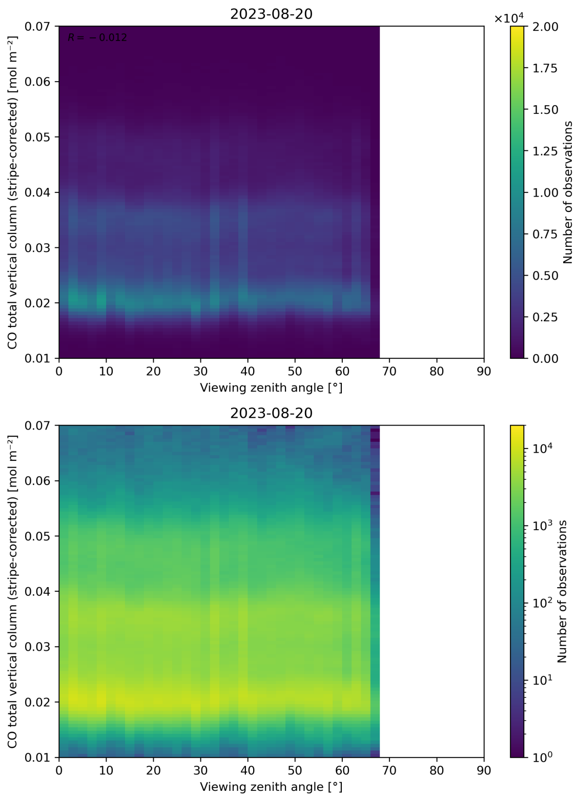
Figure 70: Scatter density plot of “Viewing zenith angle” against “CO total vertical column (stripe-corrected)” for 2023-08-20 to 2023-08-21.
