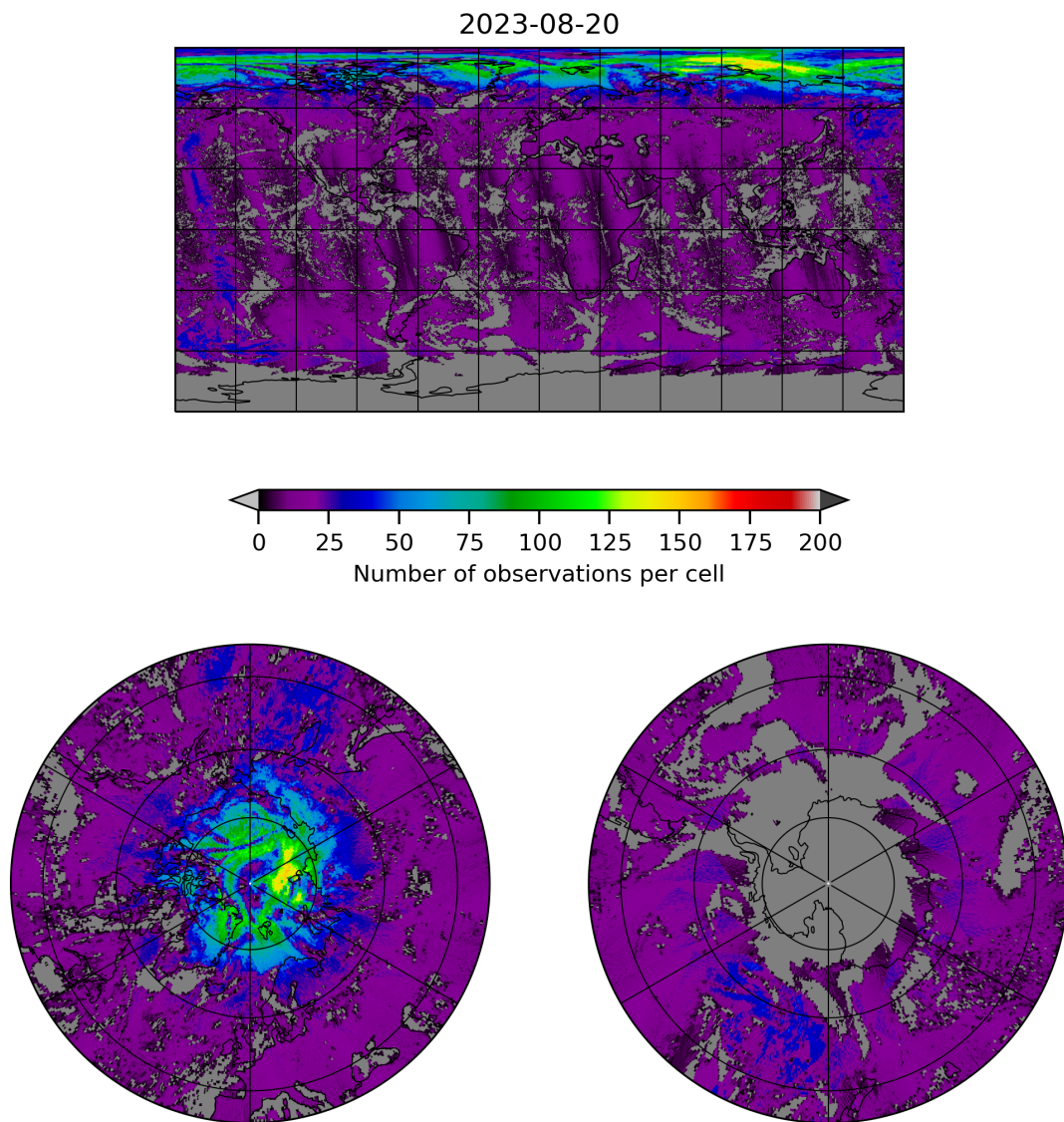
Figure 8: Map of the number of observations for 2023-08-20 to 2023-08-21
