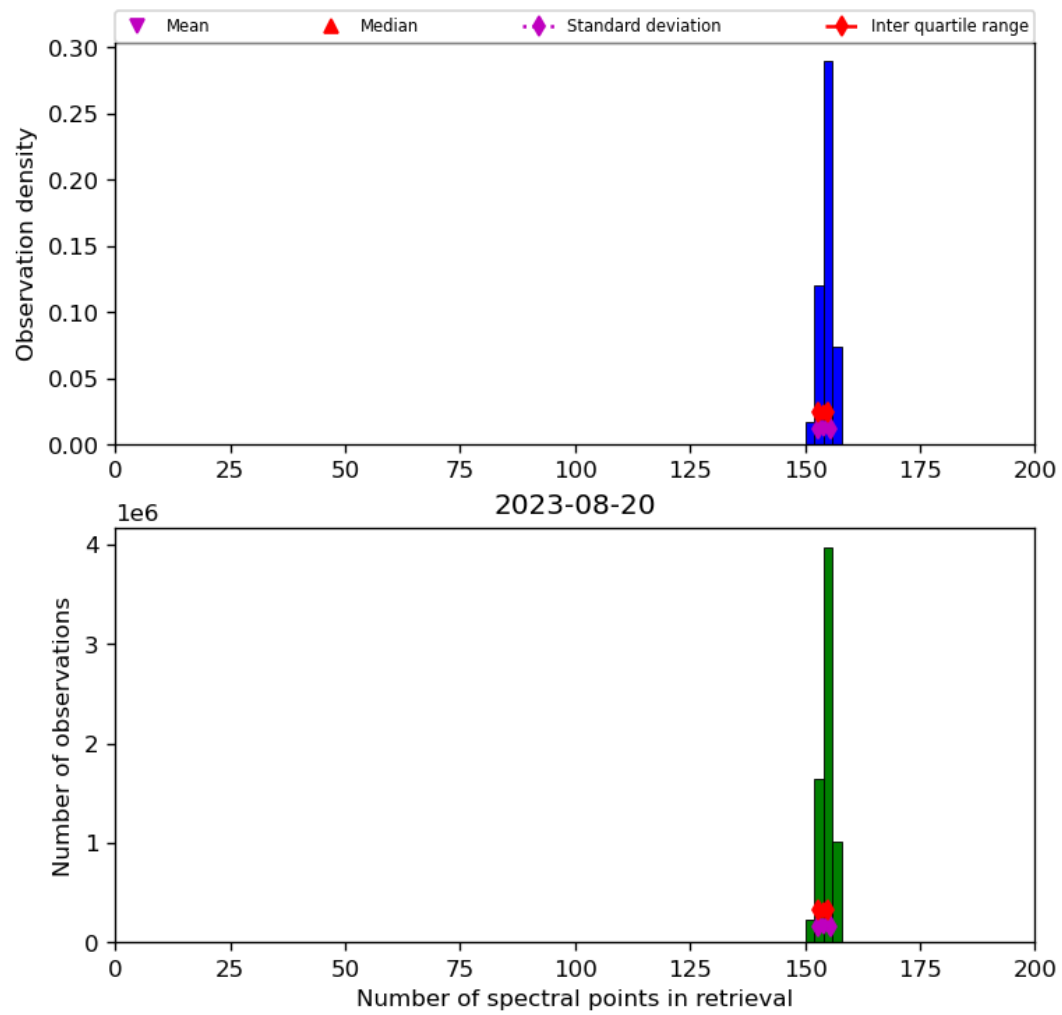
Figure 21: Histogram of “Number of spectral points in retrieval” for 2023-08-20 to 2023-08-21
