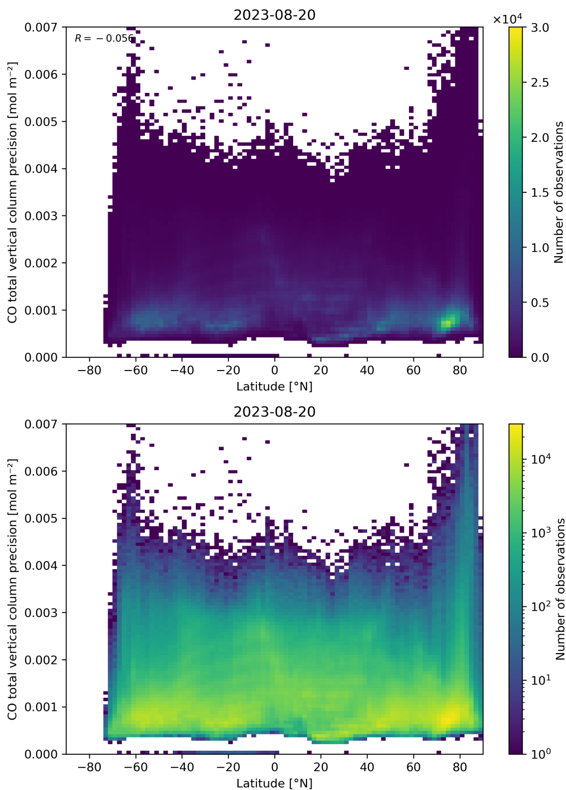
Figure 53: Scatter density plot of “Latitude” against “CO total vertical column precision” for 2023-08-20 to 2023-08-21.
