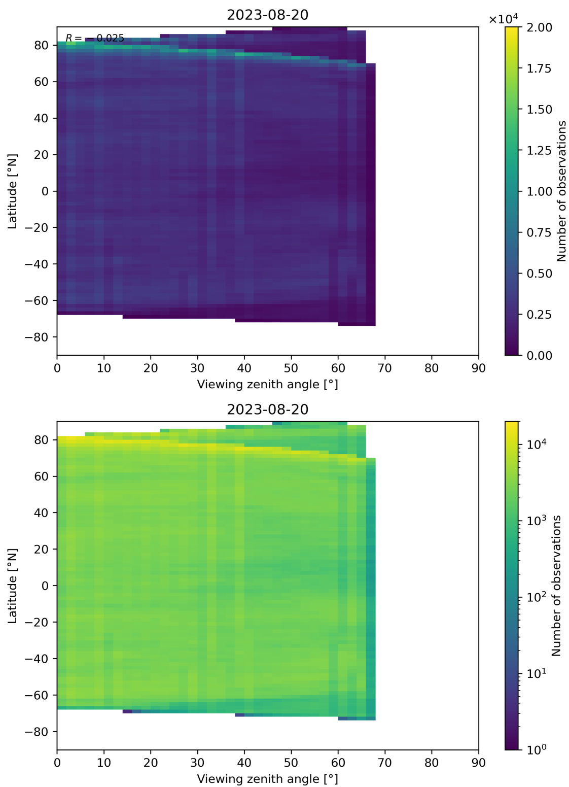
Figure 74: Scatter density plot of “Viewing zenith angle” against “Latitude” for 2023-08-20 to 2023-08-21.
