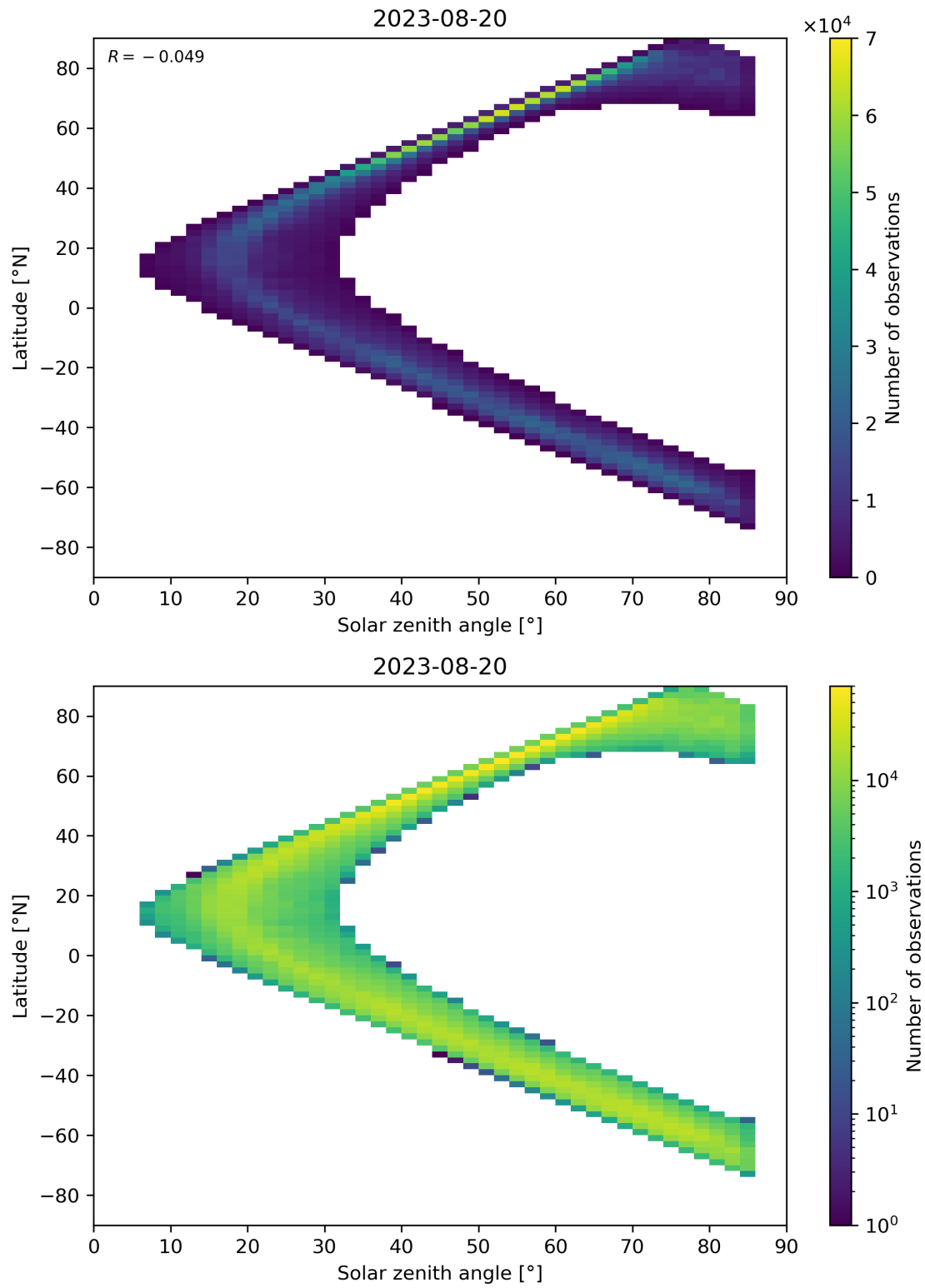
Figure 66: Scatter density plot of “Solar zenith angle” against “Latitude” for 2023-08-20 to 2023-08-21.
