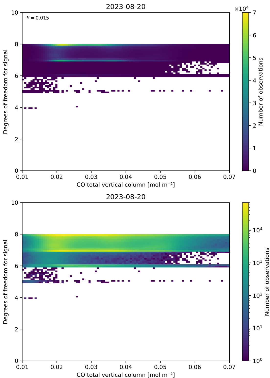
Figure 41: Scatter density plot of “CO total vertical column” against “Degrees of freedom for signal” for 2023-08-20 to 2023-08-21.
