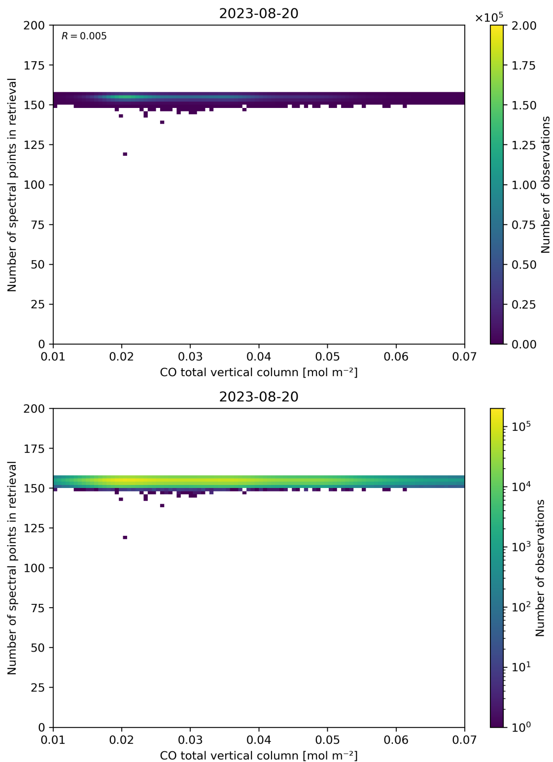
Figure 43: Scatter density plot of “CO total vertical column” against “Number of spectral points in retrieval” for 2023-08-20 to 2023-08-21.
