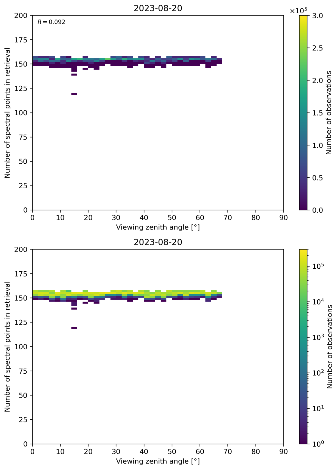
Figure 76: Scatter density plot of “Viewing zenith angle” against “Number of spectral points in retrieval” for 2023-08-20 to 2023-08-21.
