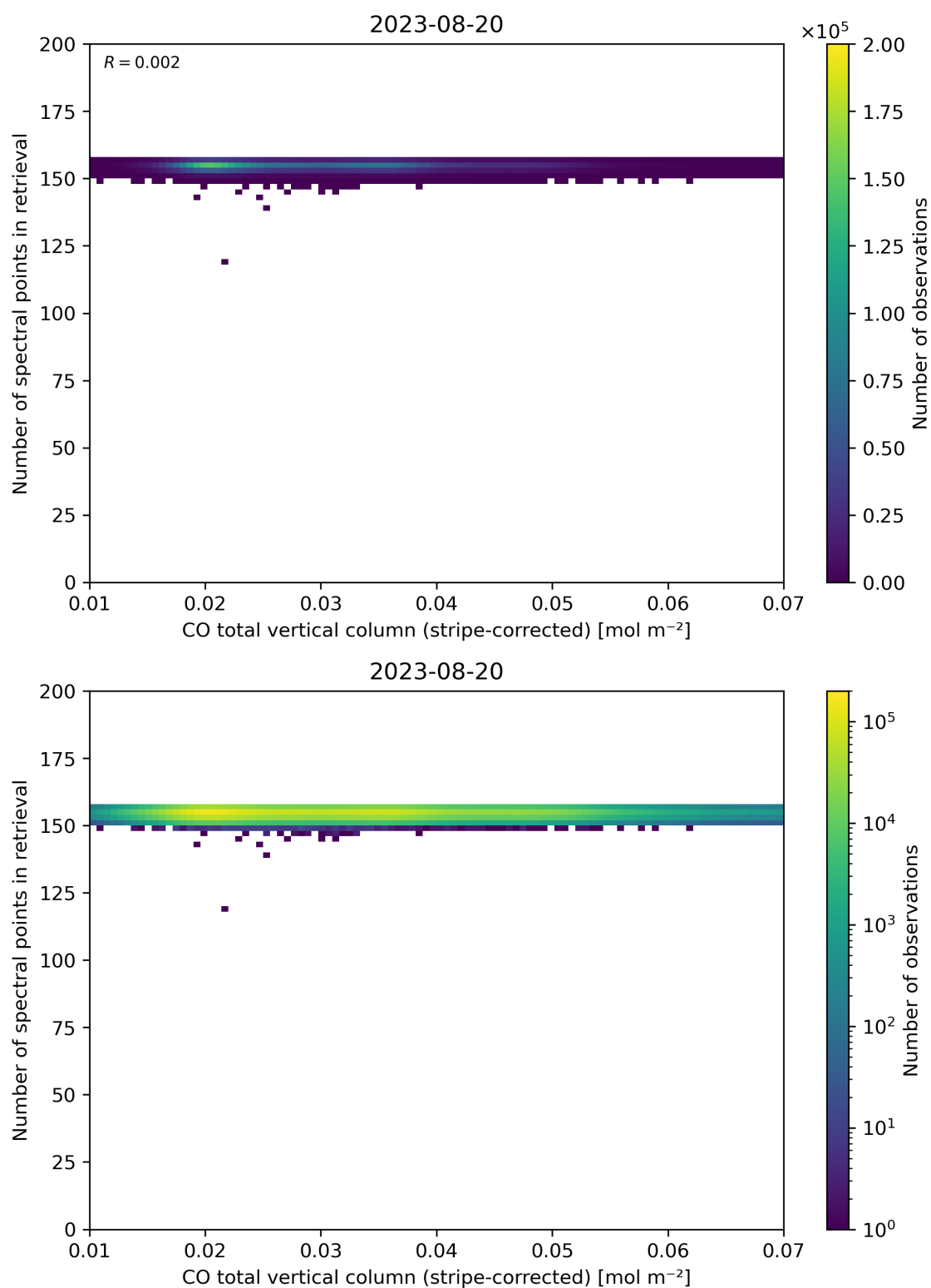
Figure 40: Scatter density plot of “CO total vertical column (stripe-corrected)” against “Number of spectral points in retrieval” for 2023-08-20 to 2023-08-21.
