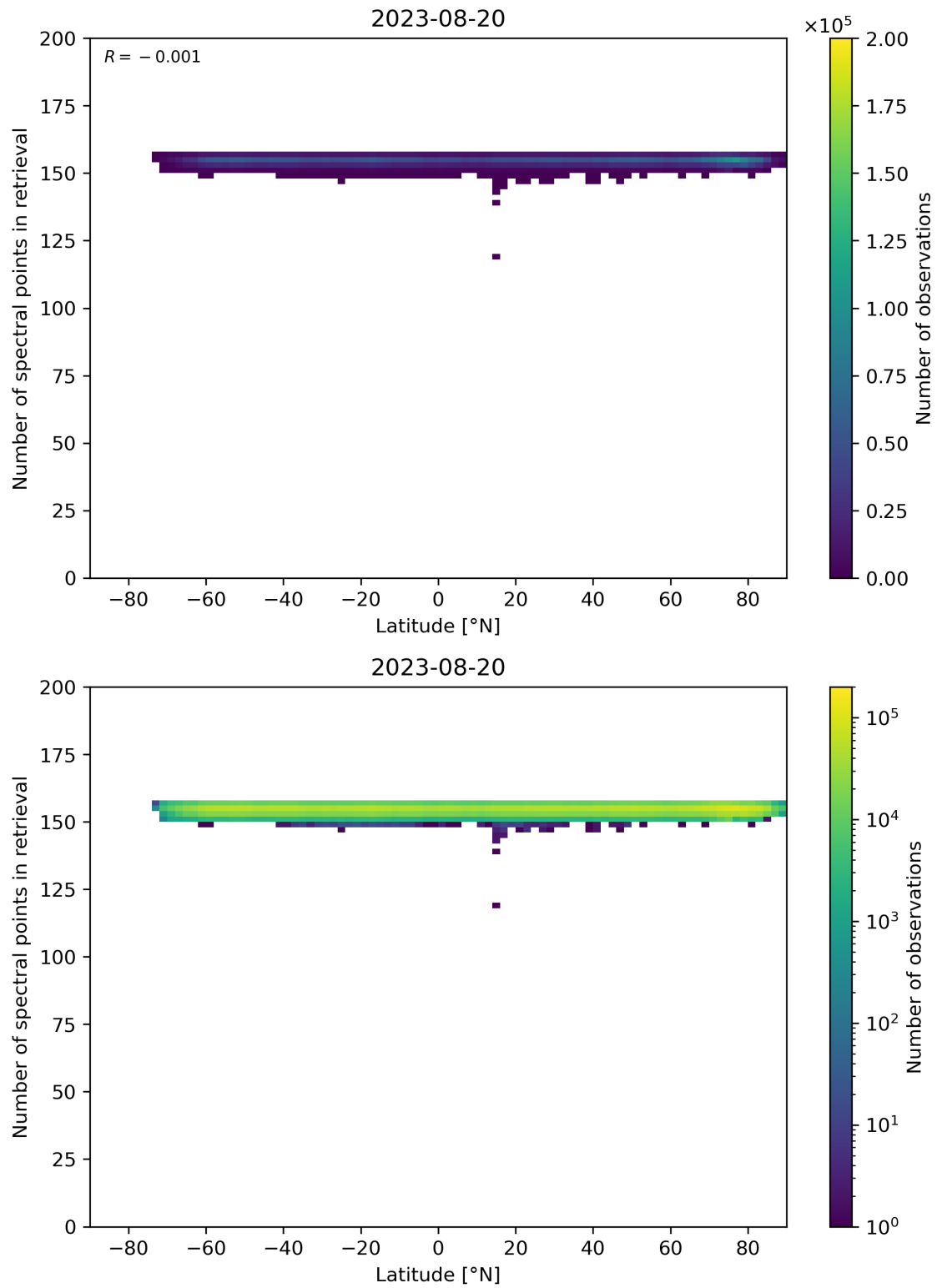
Figure 57: Scatter density plot of “Latitude” against “Number of spectral points in retrieval” for 2023-08-20 to 2023-08-21.
