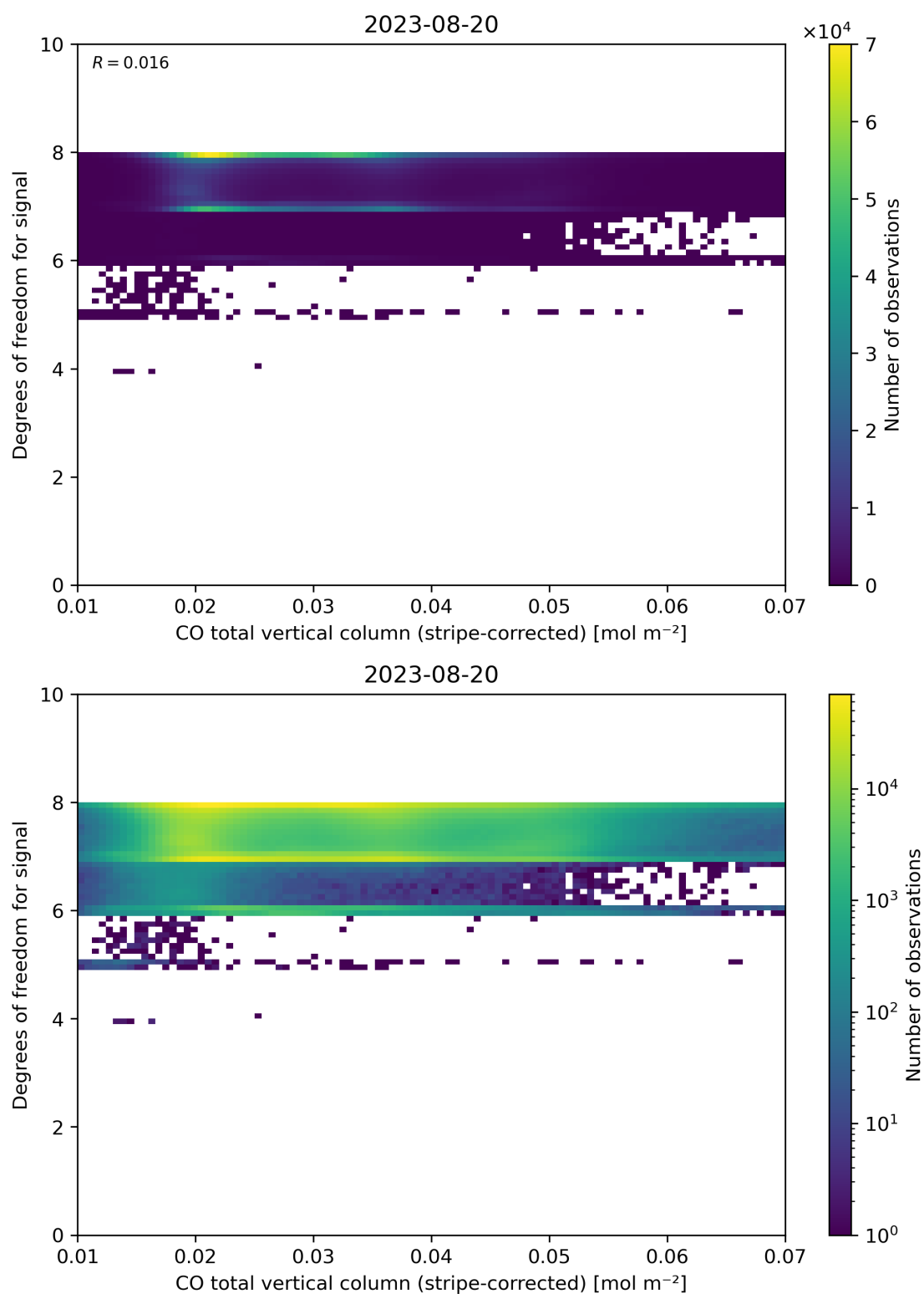
Figure 38: Scatter density plot of “CO total vertical column (stripe-corrected)” against “Degrees of freedom for signal” for 2023-08-20 to 2023-08-21.
