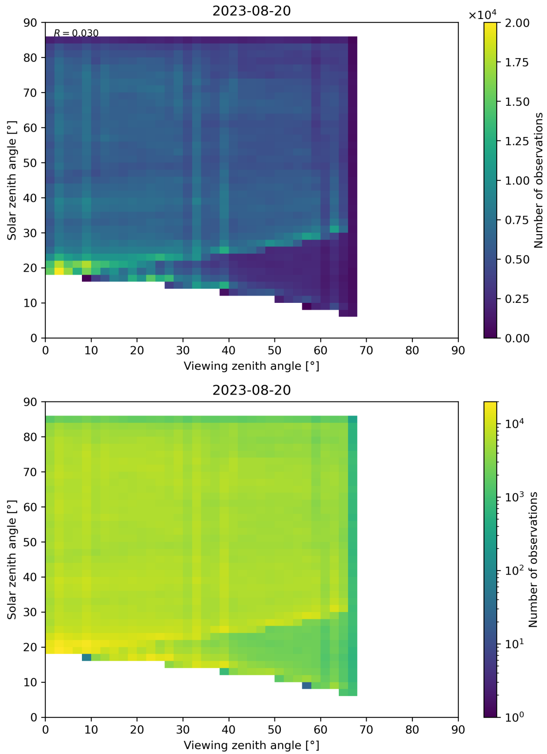
Figure 77: Scatter density plot of “Viewing zenith angle” against “Solar zenith angle” for 2023-08-20 to 2023-08-21.
