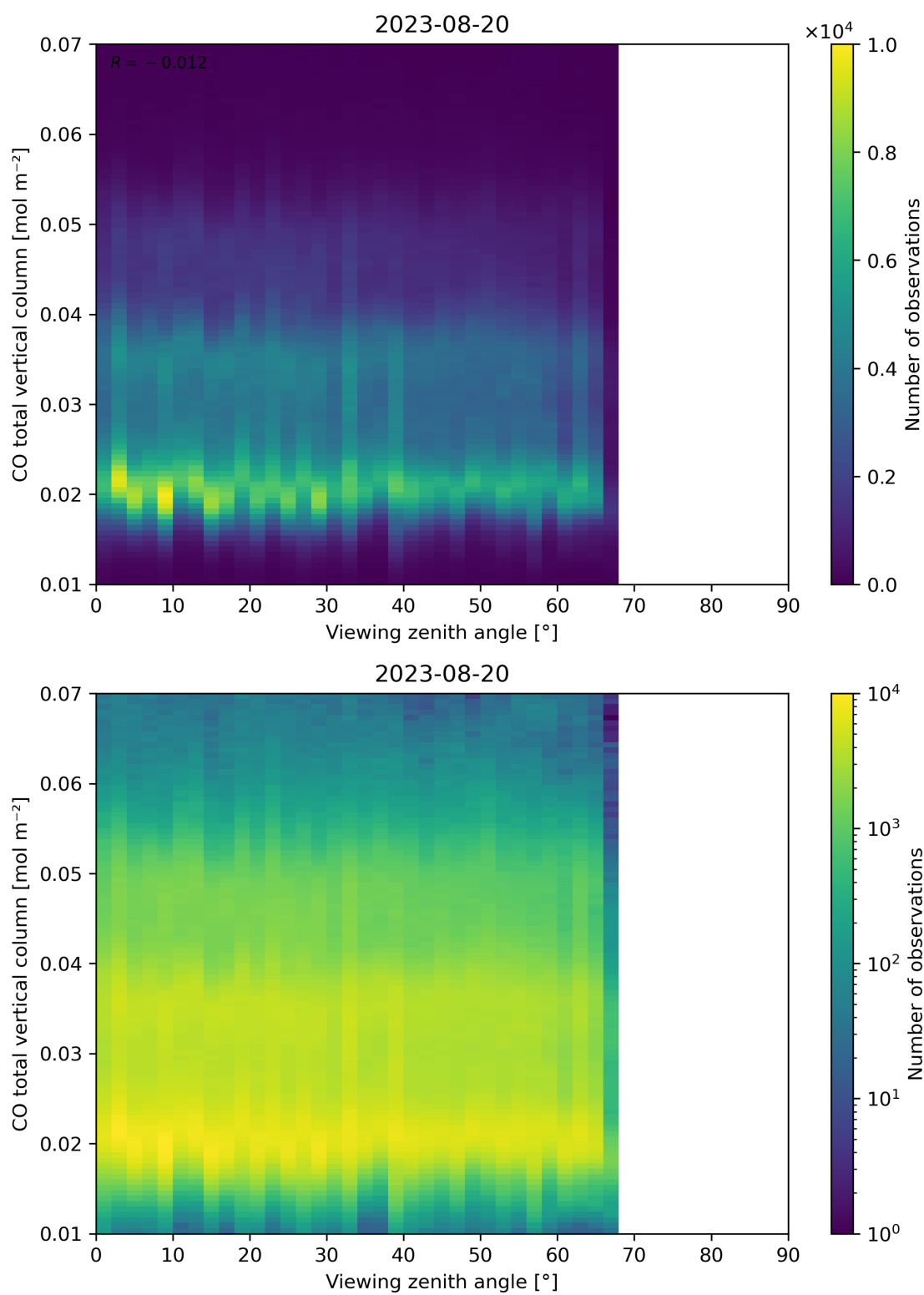
Figure 69: Scatter density plot of “Viewing zenith angle” against “CO total vertical column” for 2023-08-20 to 2023-08-21.
