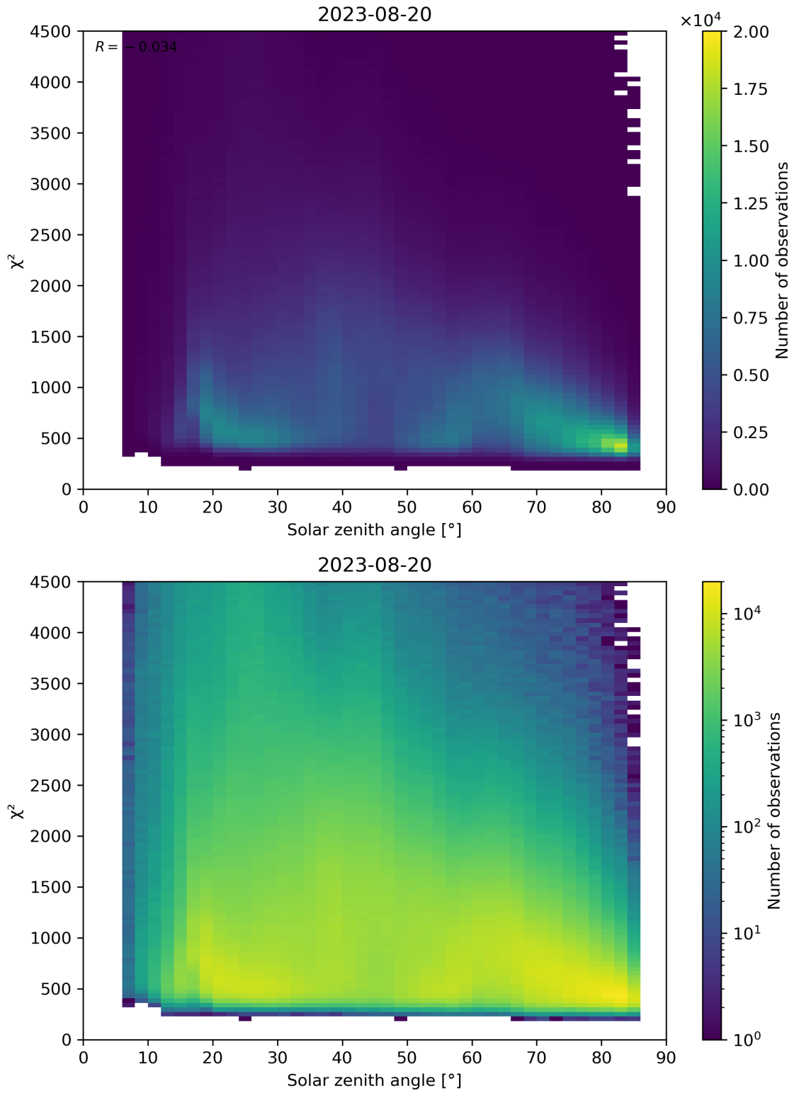
Figure 64: Scatter density plot of “Solar zenith angle” against “ \chi^2 ” for 2023-08-20 to 2023-08-21.
