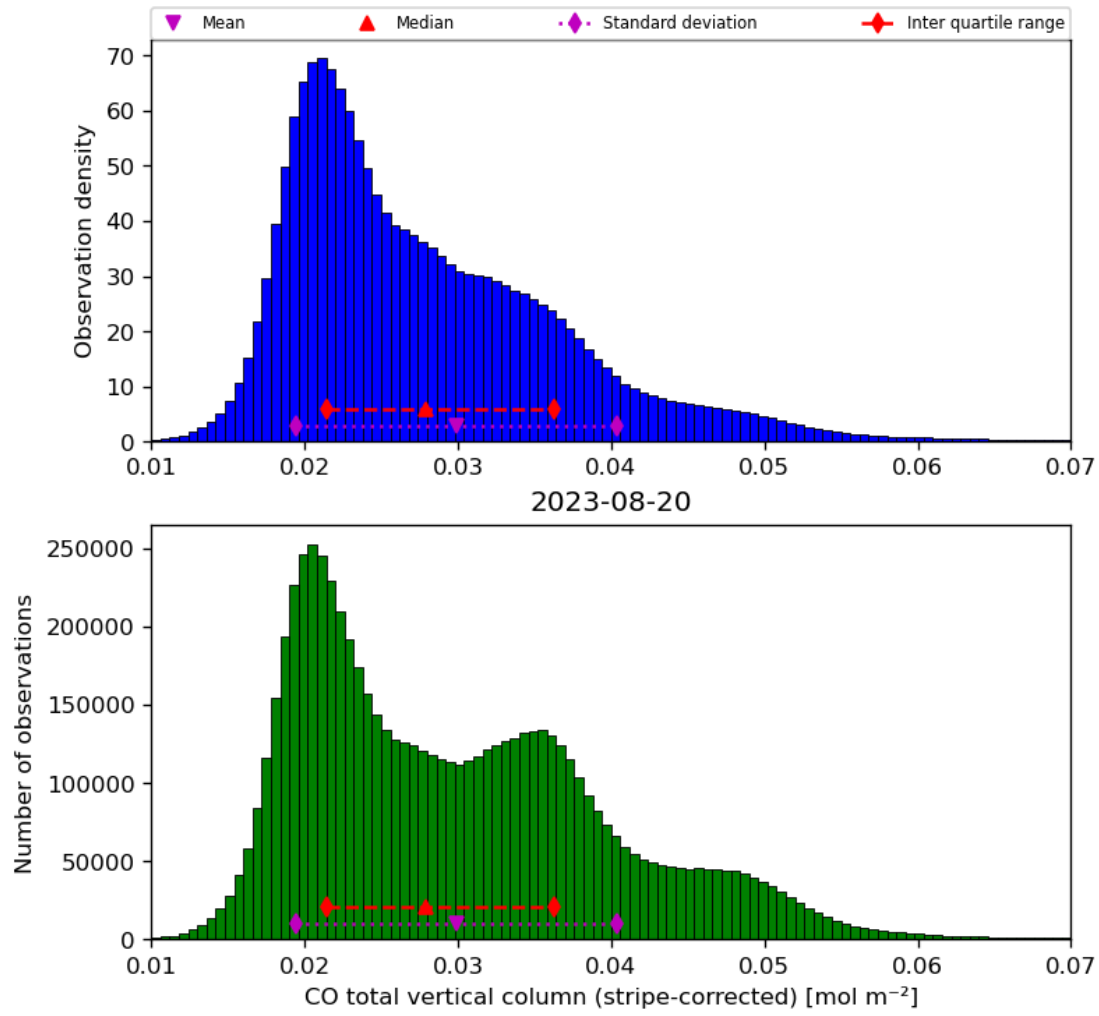
Figure 19: Histogram of “CO total vertical column (stripe-corrected)” for 2023-08-20 to 2023-08-21
