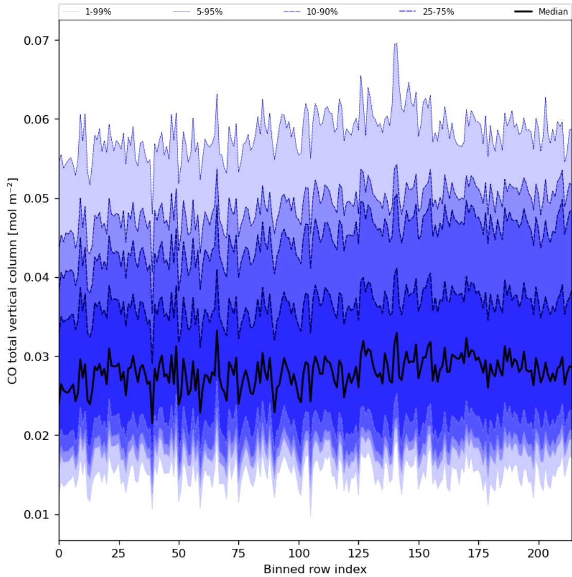
Figure 26: Along track statistics of “CO total vertical column” for 2023-08-20 to 2023-08-21
