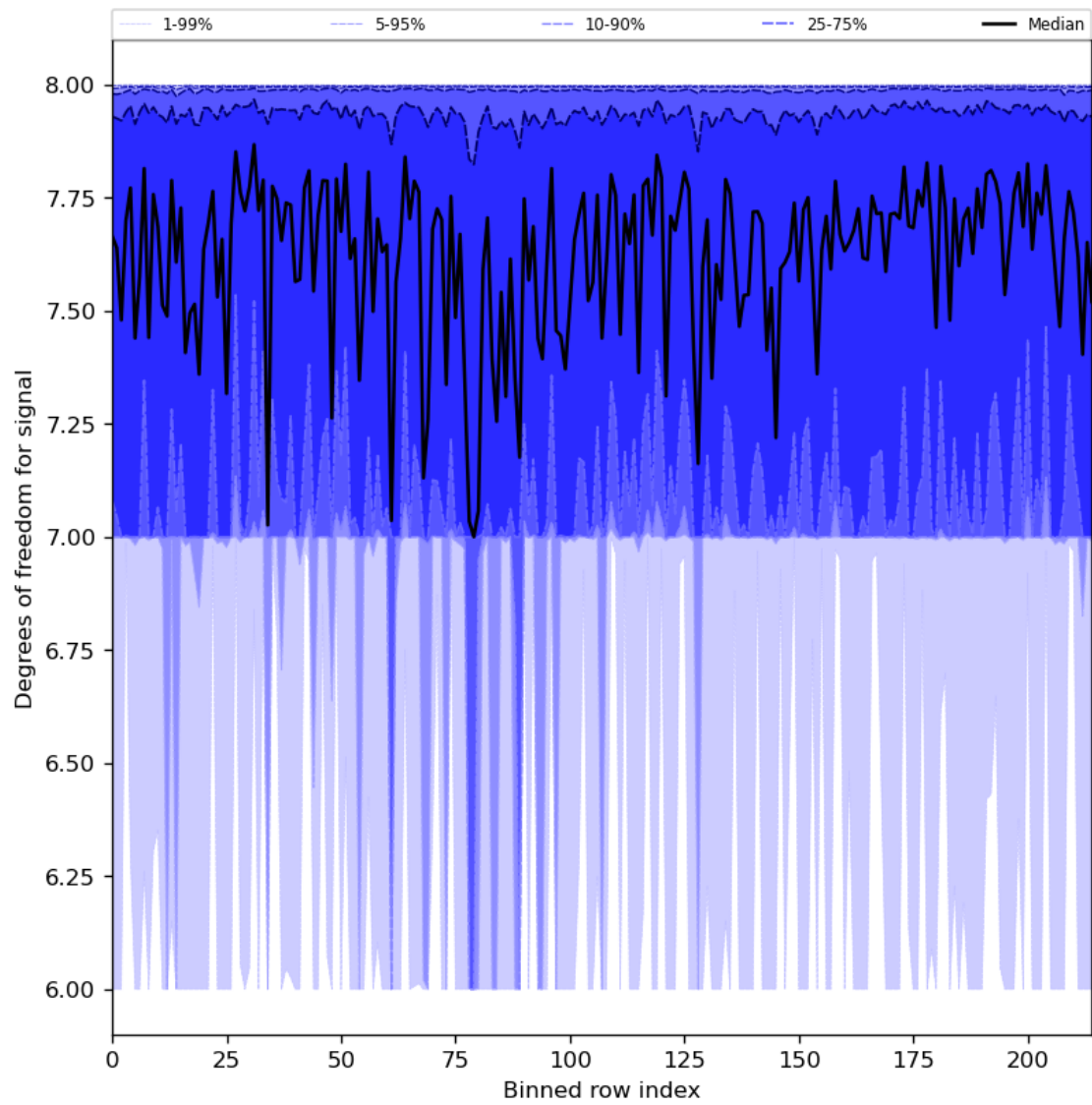
Figure 31: Along track statistics of “Degrees of freedom for signal” for 2023-08-20 to 2023-08-21
