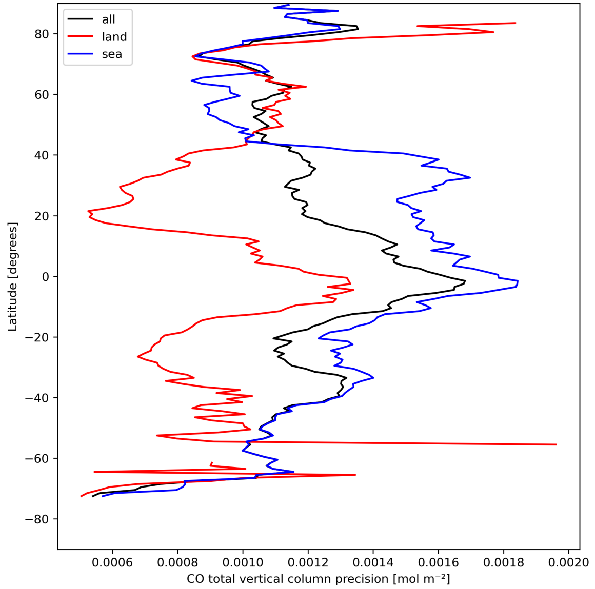
Figure 12: Zonal average of “CO total vertical column precision” for 2023-08-20 to 2023-08-21.
