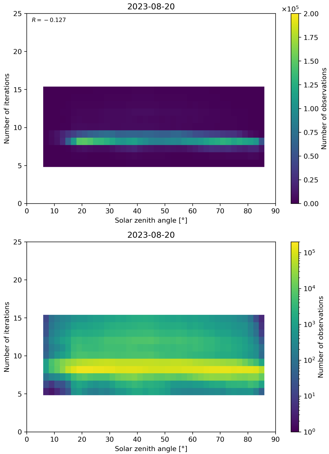
Figure 67: Scatter density plot of “Solar zenith angle” against “Number of iterations” for 2023-08-20 to 2023-08-21.
