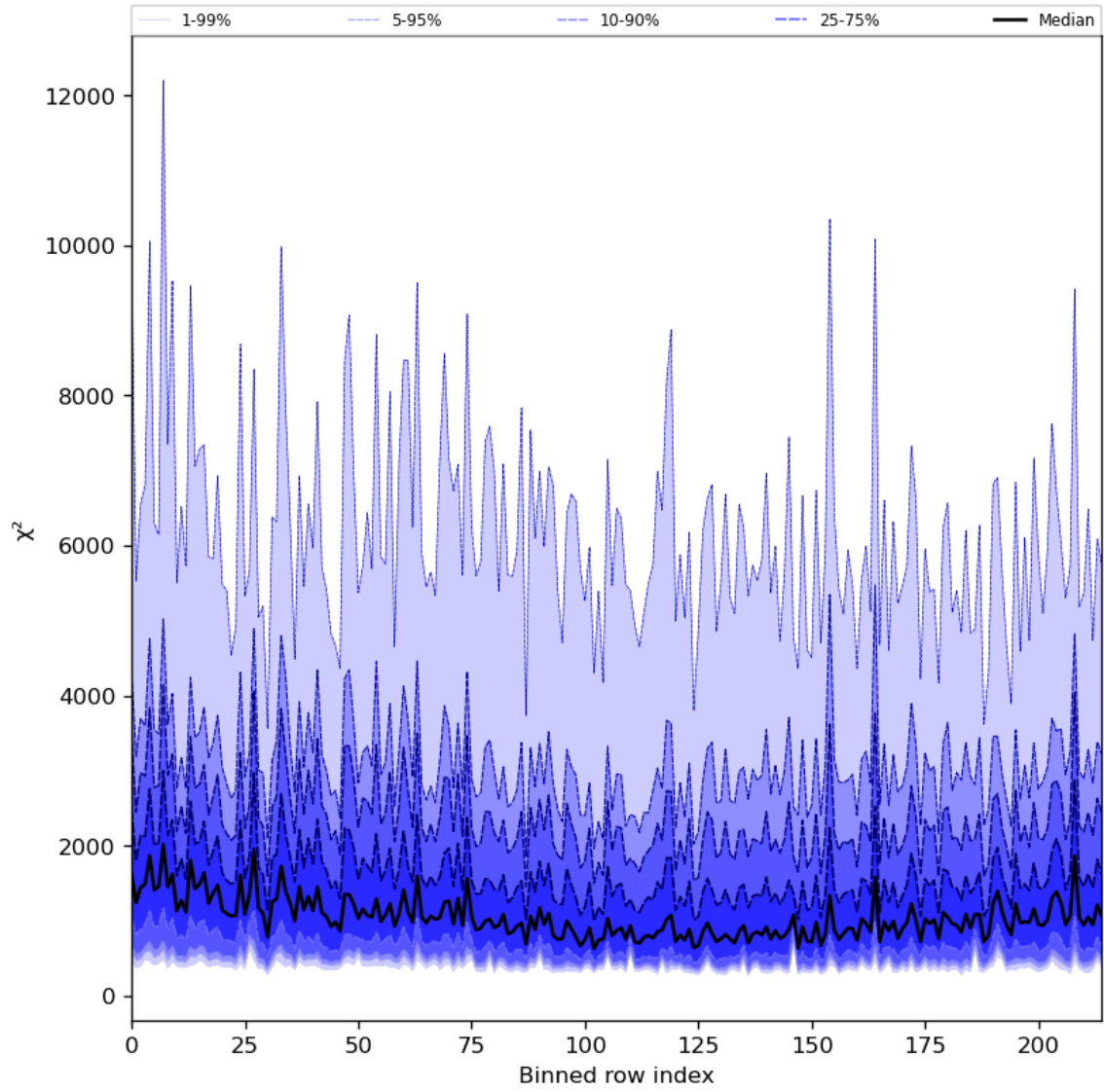
Figure 30: Along track statistics of “ \chi^2 ” for 2023-08-20 to 2023-08-21
