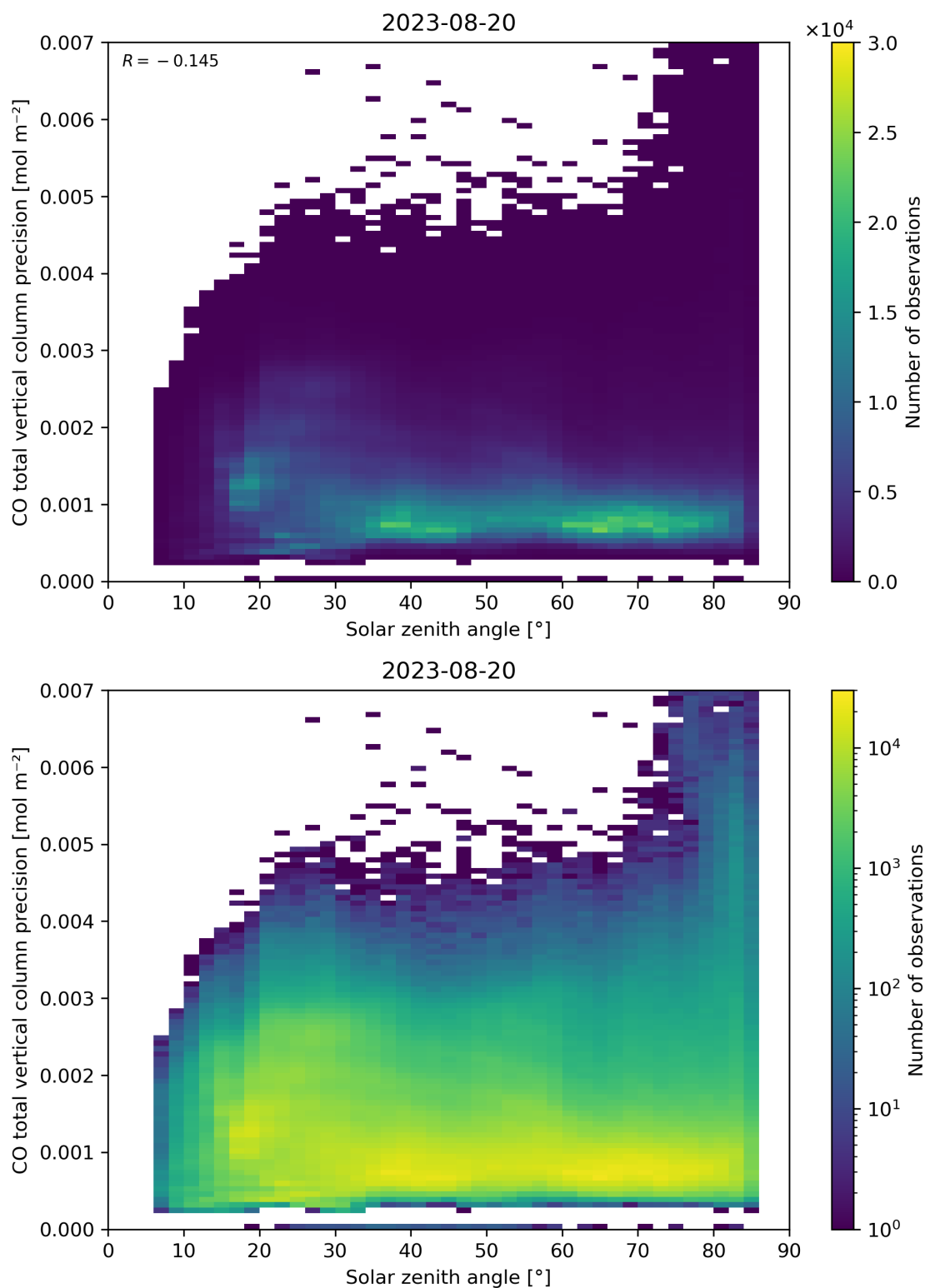
Figure 63: Scatter density plot of “Solar zenith angle” against “CO total vertical column precision” for 2023-08-20 to 2023-08-21.
