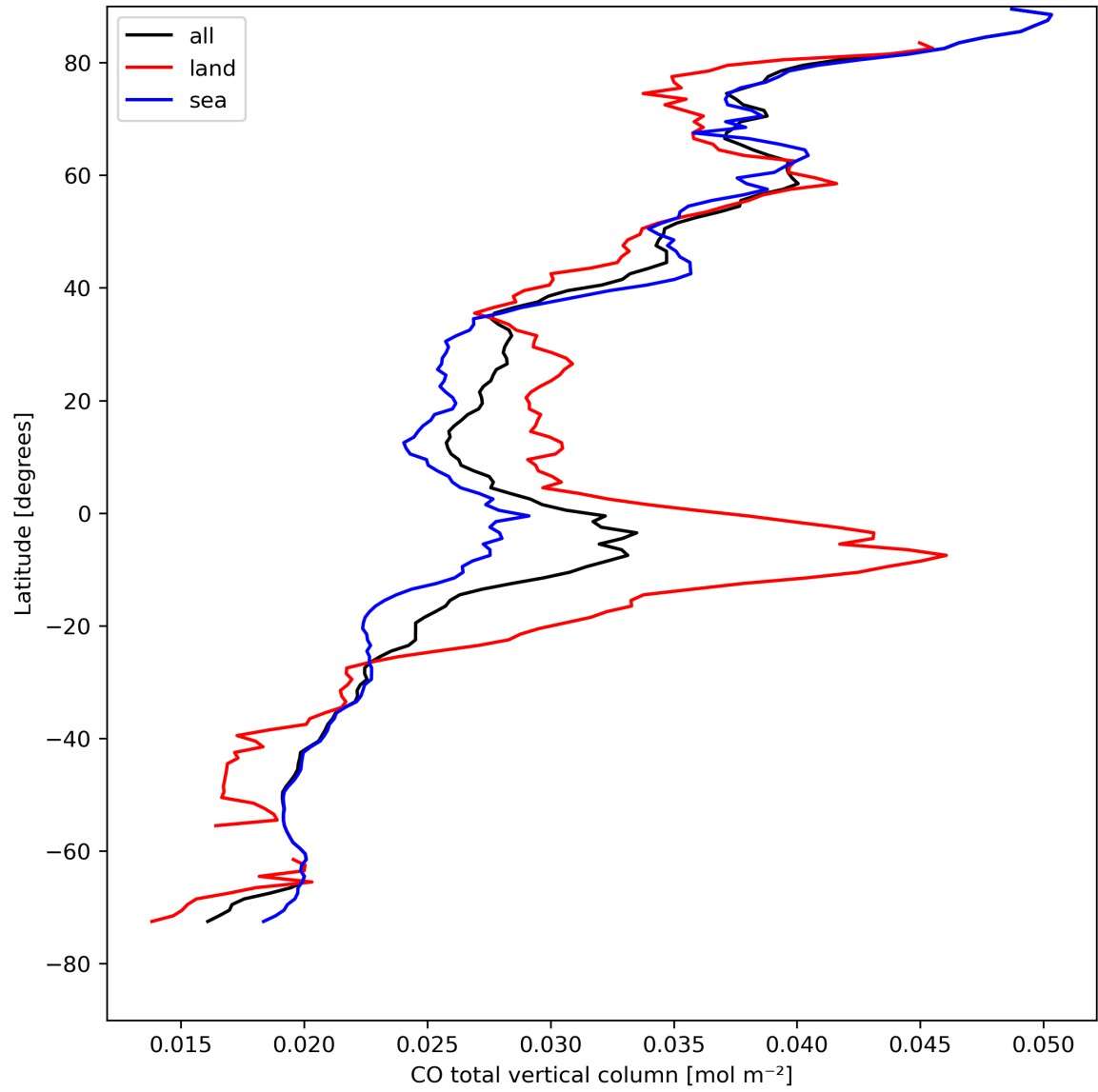
Figure 10: Zonal average of “CO total vertical column” for 2023-08-20 to 2023-08-21.
