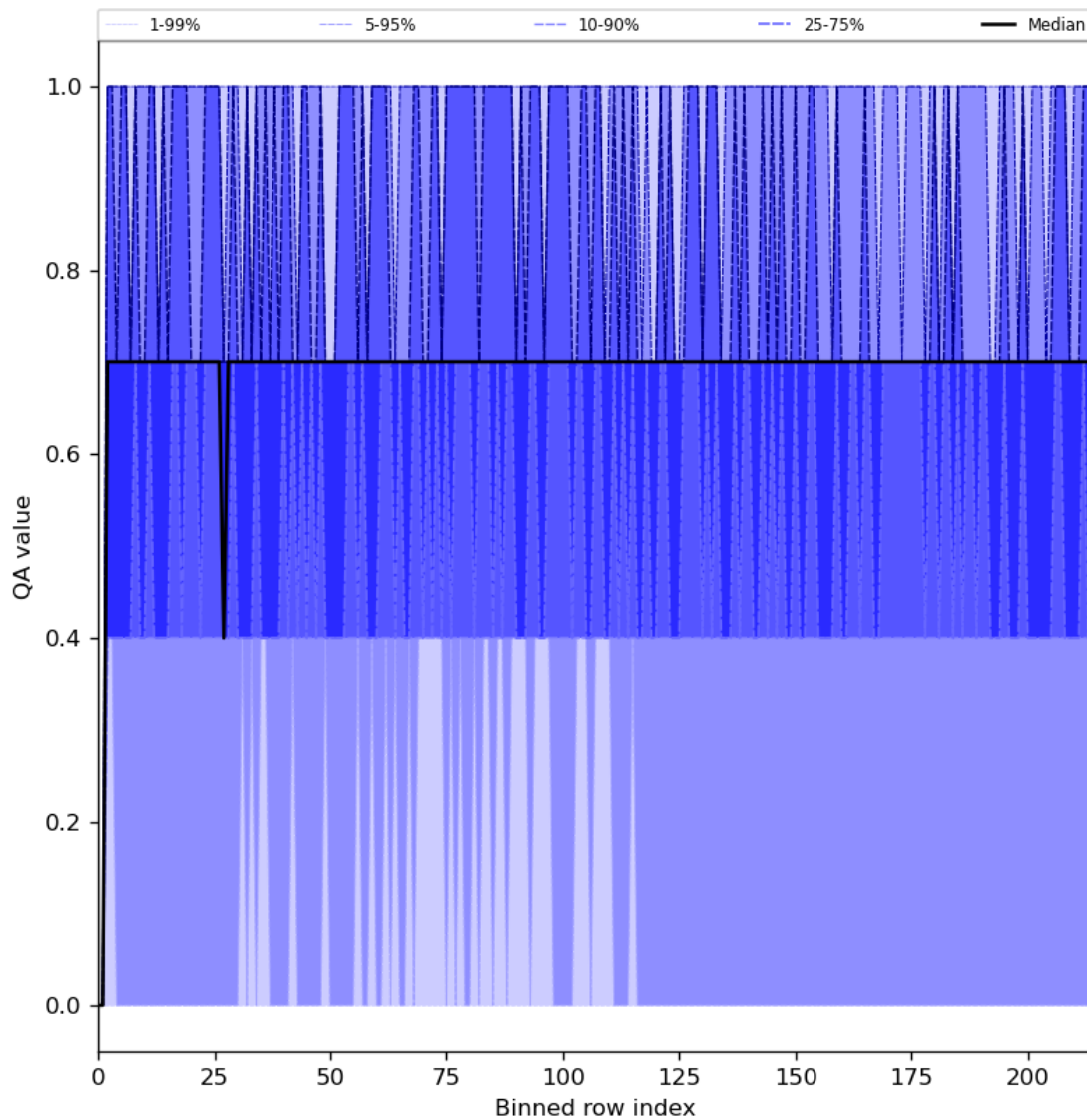
Figure 25: Along track statistics of “QA value” for 2023-08-20 to 2023-08-21
