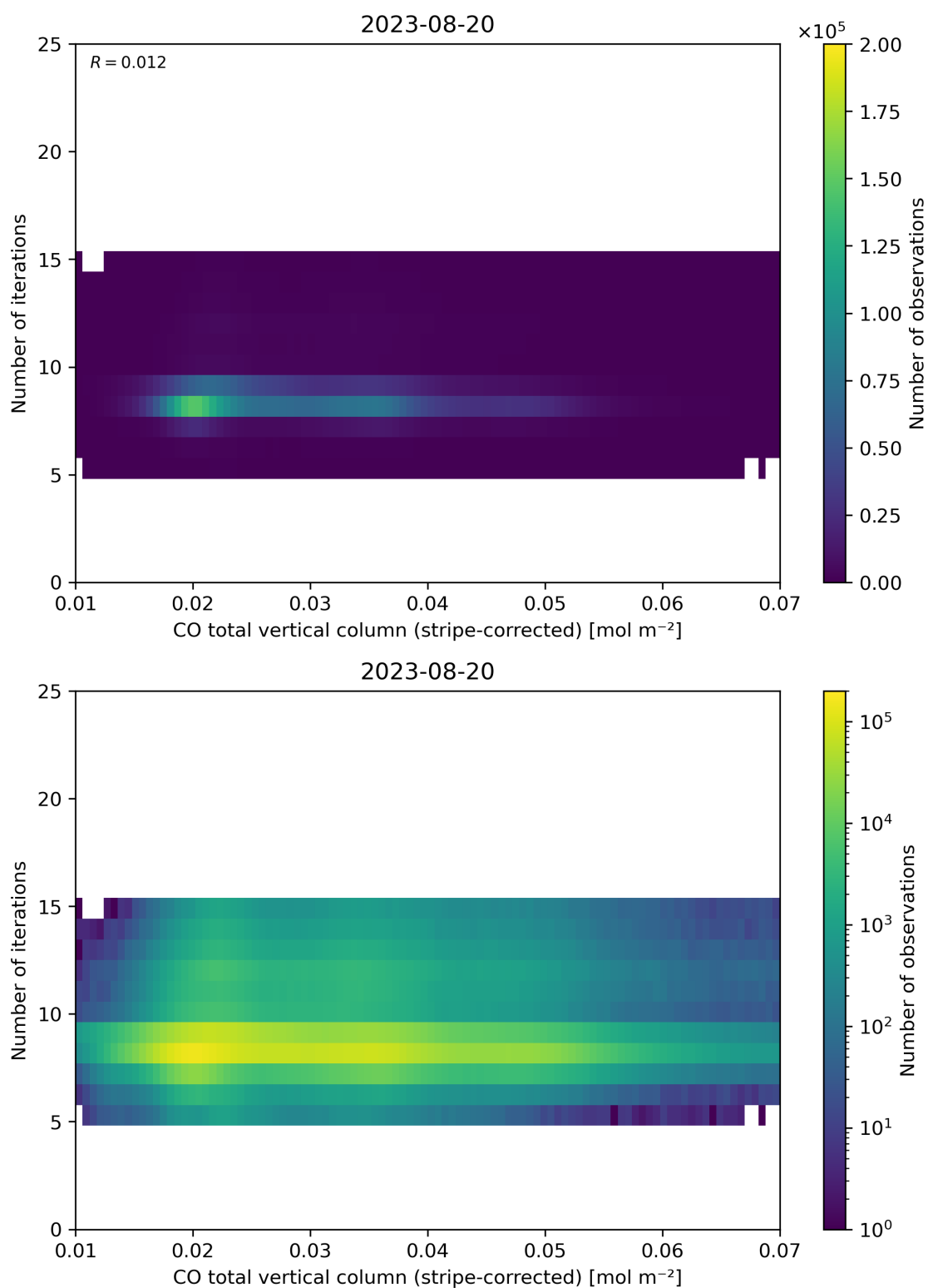
Figure 39: Scatter density plot of “CO total vertical column (stripe-corrected)” against “Number of iterations” for 2023-08-20 to 2023-08-21.
