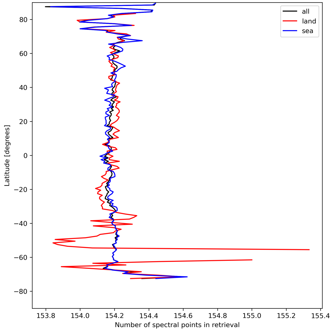
Figure 13: Zonal average of “Number of spectral points in retrieval” for 2023-08-20 to 2023-08-21.
