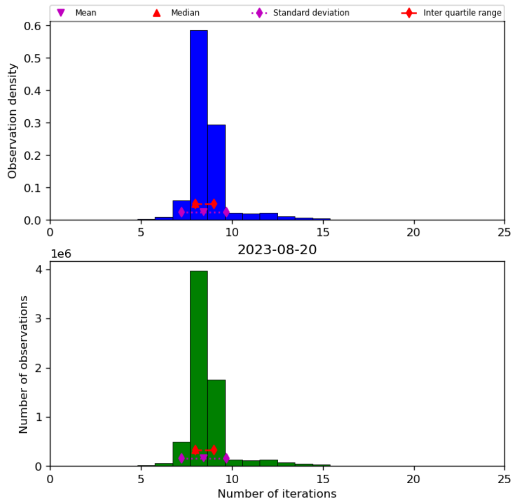
Figure 24: Histogram of “Number of iterations” for 2023-08-20 to 2023-08-21
