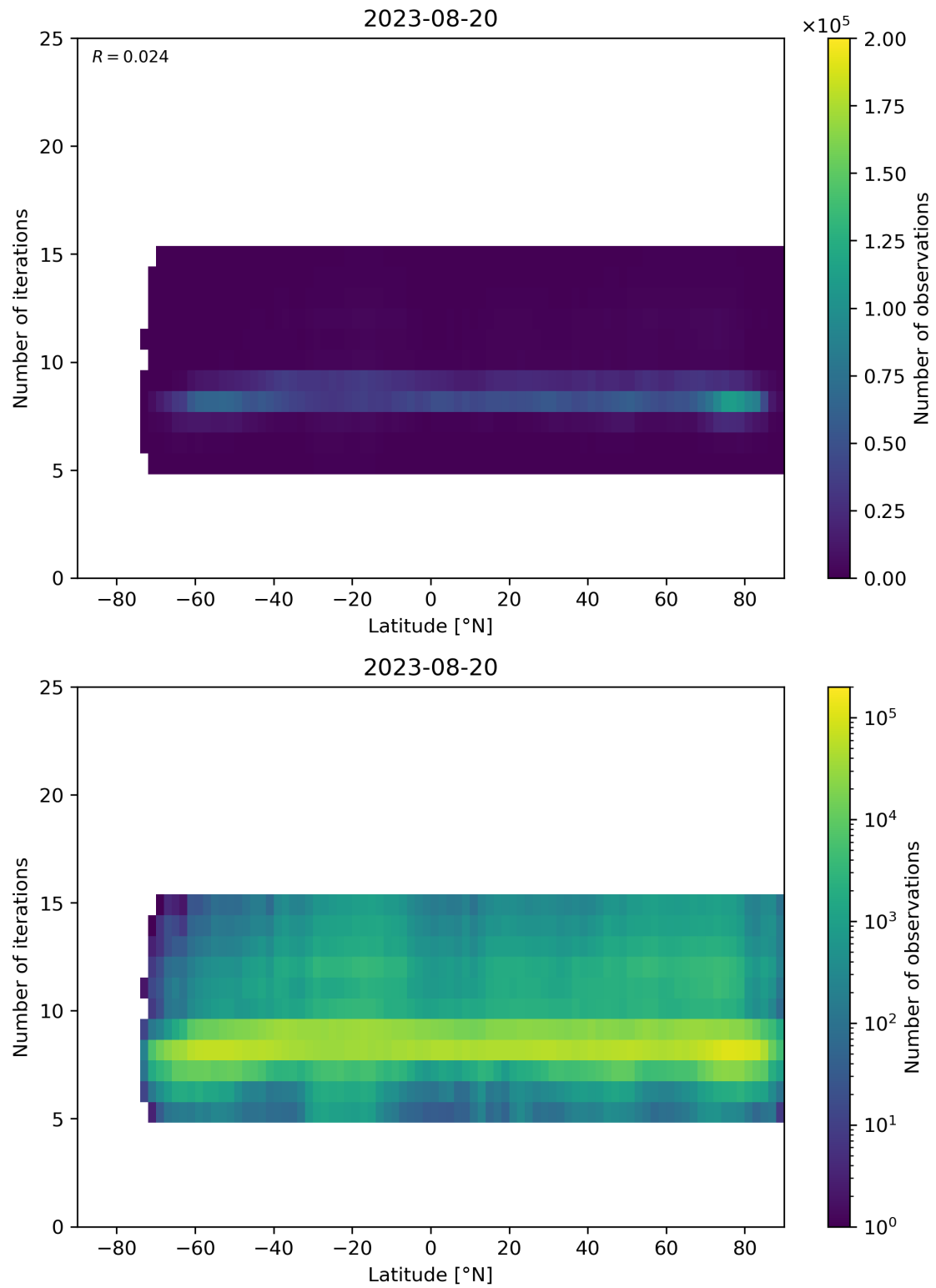
Figure 56: Scatter density plot of “Latitude” against “Number of iterations” for 2023-08-20 to 2023-08-21.
