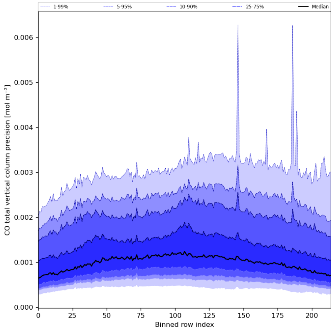
Figure 28: Along track statistics of “CO total vertical column precision” for 2023-08-20 to 2023-08-21
