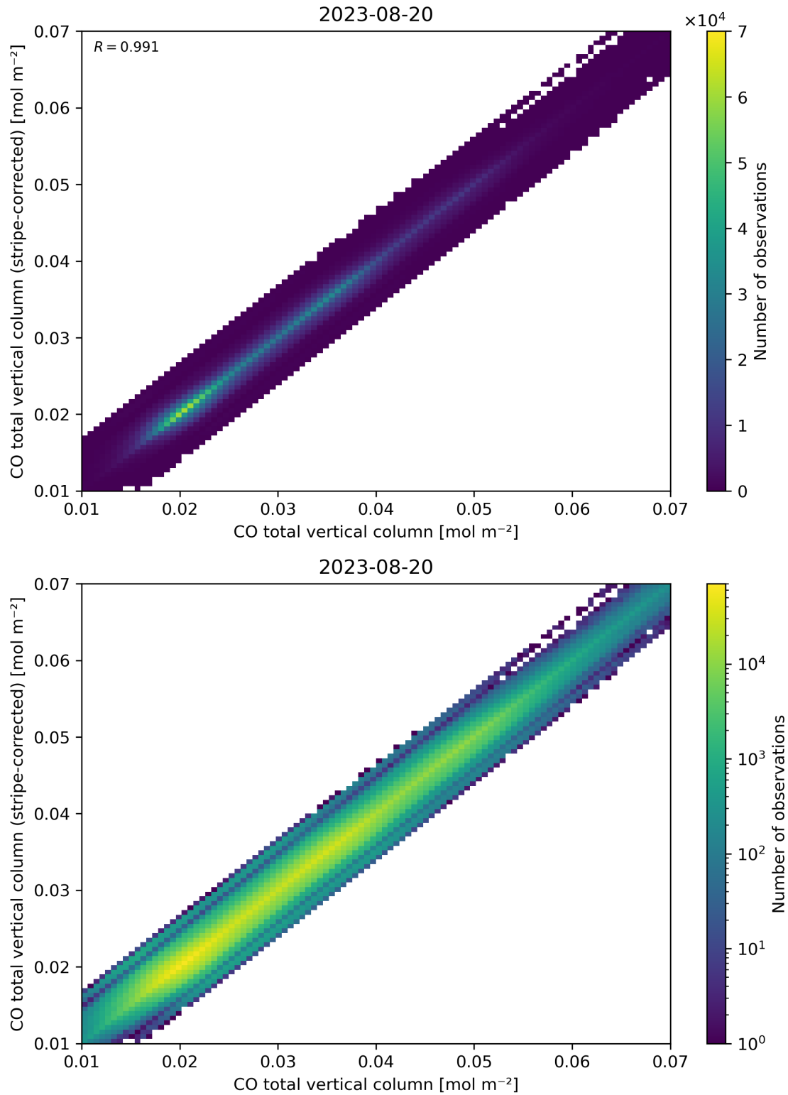
Figure 33: Scatter density plot of “CO total vertical column” against “CO total vertical column (stripe-corrected)” for 2023-08-20 to 2023-08-21.
