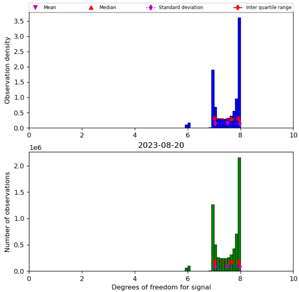
Figure 23: Histogram of “Degrees of freedom for signal” for 2023-08-20 to 2023-08-21
