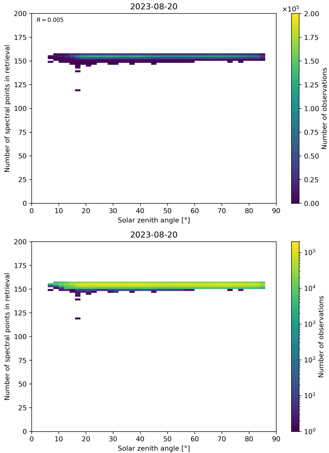
Figure 68: Scatter density plot of “Solar zenith angle” against “Number of spectral points in retrieval” for 2023-08-20 to 2023-08-21.
