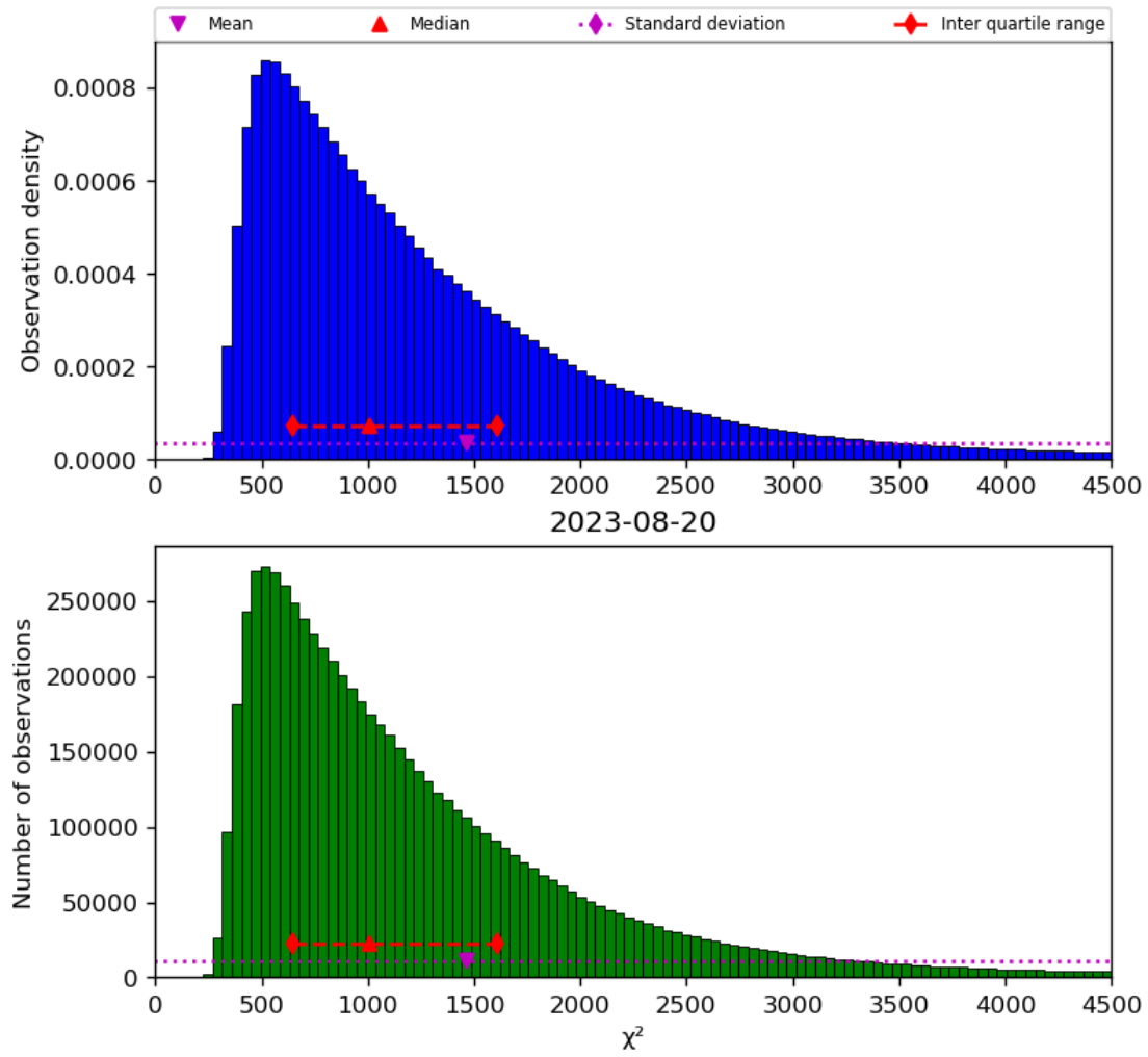
Figure 22: Histogram of “ \chi^2 ” for 2023-08-20 to 2023-08-21
