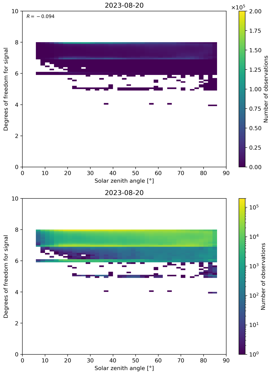
Figure 65: Scatter density plot of “Solar zenith angle” against “Degrees of freedom for signal” for 2023-08-20 to 2023-08-21.
