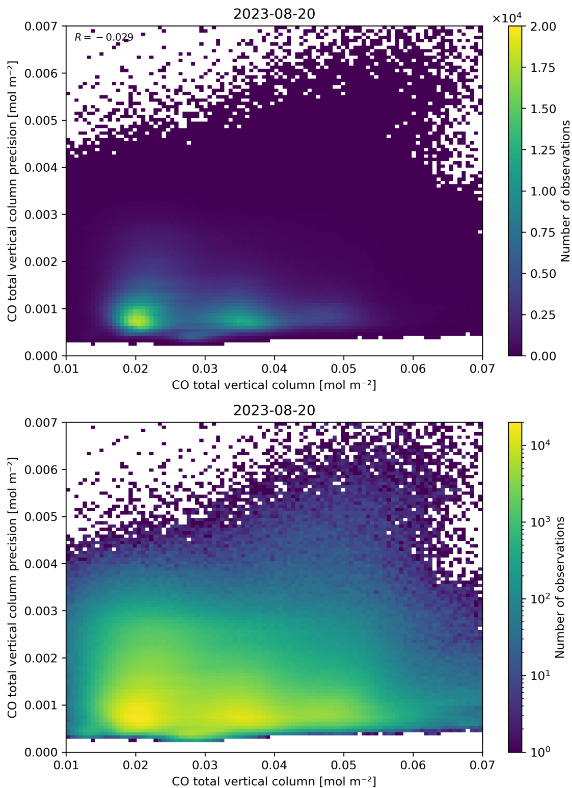
Figure 34: Scatter density plot of “CO total vertical column” against “CO total vertical column precision” for 2023-08-20 to 2023-08-21.
