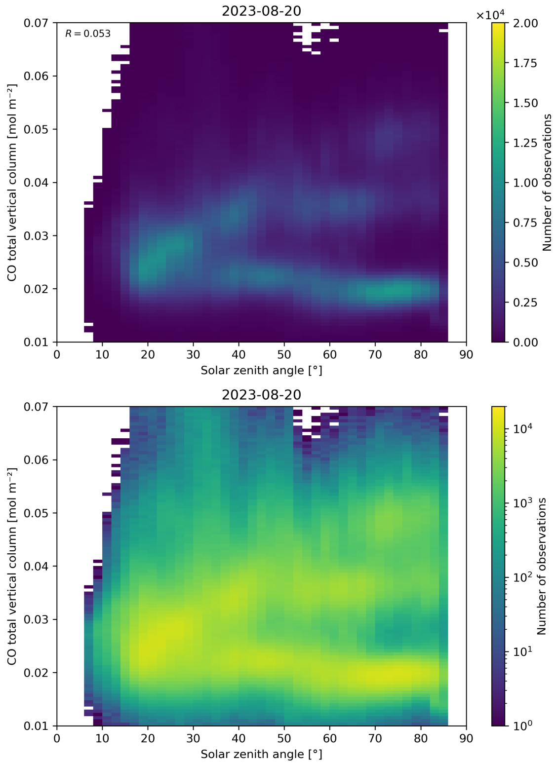
Figure 61: Scatter density plot of “Solar zenith angle” against “CO total vertical column” for 2023-08-20 to 2023-08-21.
