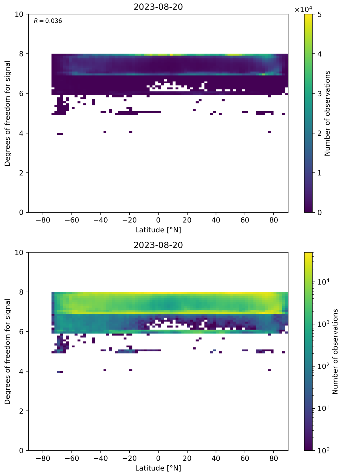
Figure 55: Scatter density plot of “Latitude” against “Degrees of freedom for signal” for 2023-08-20 to 2023-08-21.
