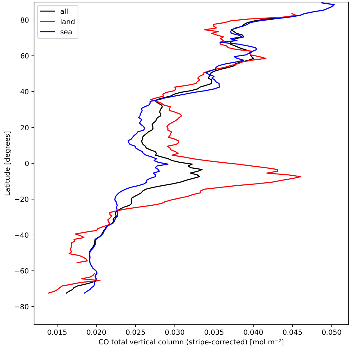
Figure 11: Zonal average of “CO total vertical column (stripe-corrected)” for 2023-08-20 to 2023-08-21.
