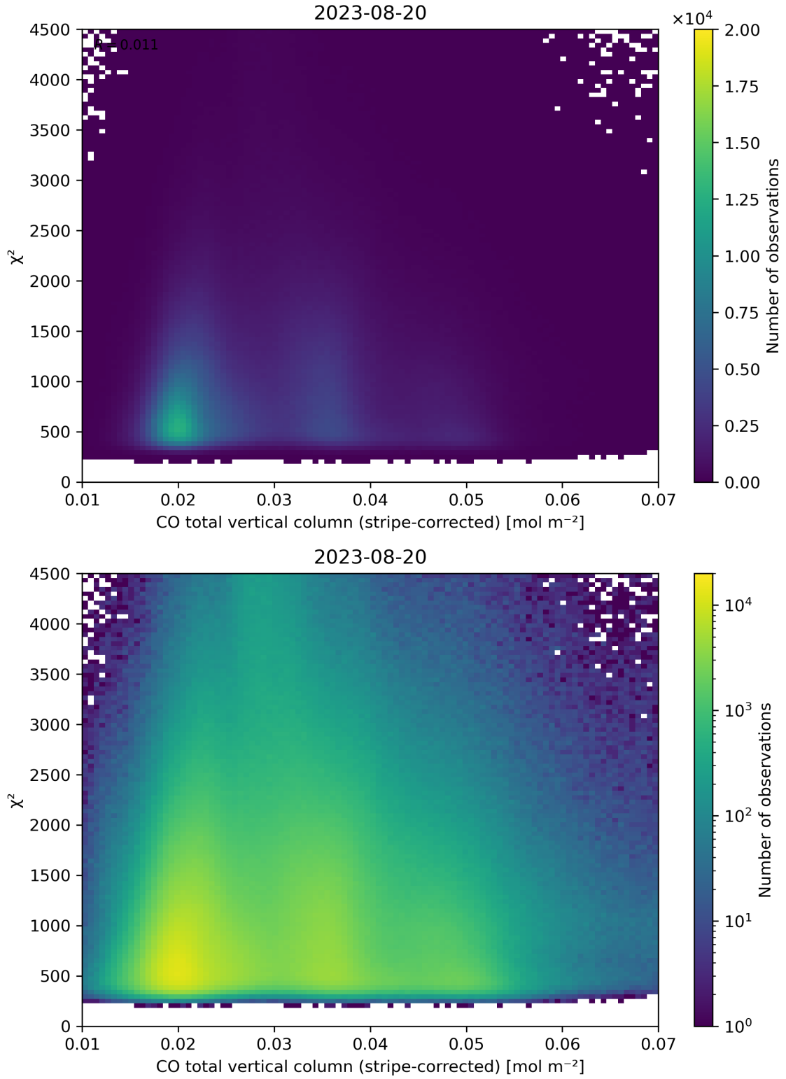
Figure 37: Scatter density plot of “CO total vertical column (stripe-corrected)” against “ \chi^2 ” for 2023-08-20 to 2023-08-21.
