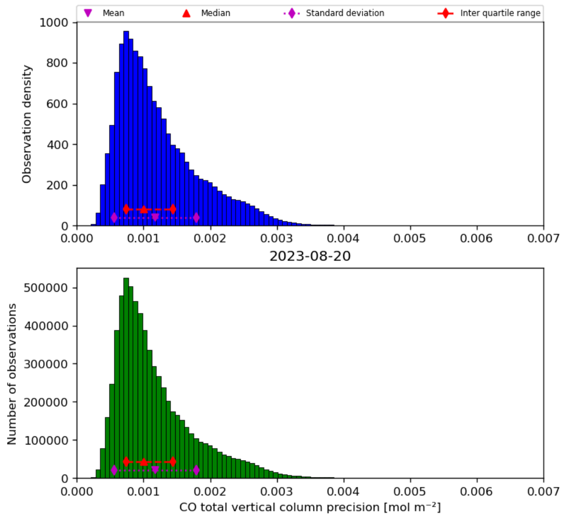
Figure 20: Histogram of “CO total vertical column precision” for 2023-08-20 to 2023-08-21
