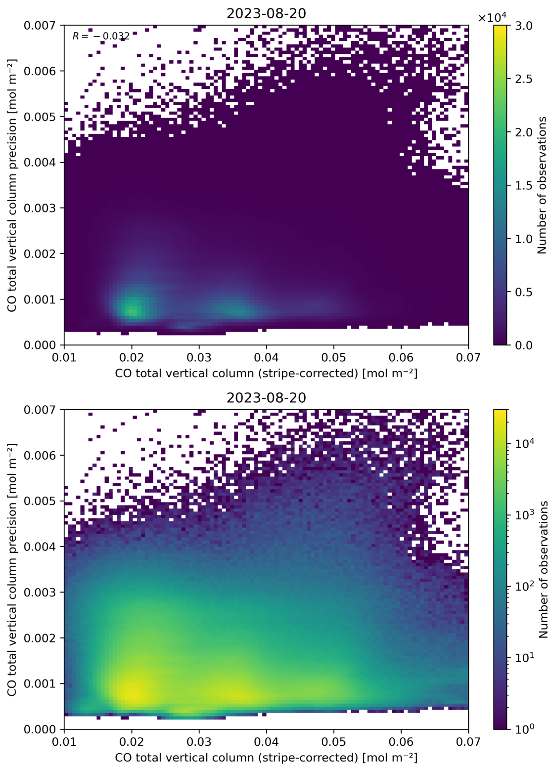
Figure 36: Scatter density plot of “CO total vertical column (stripe-corrected)” against “CO total vertical column precision” for 2023-08-20 to 2023-08-21.
