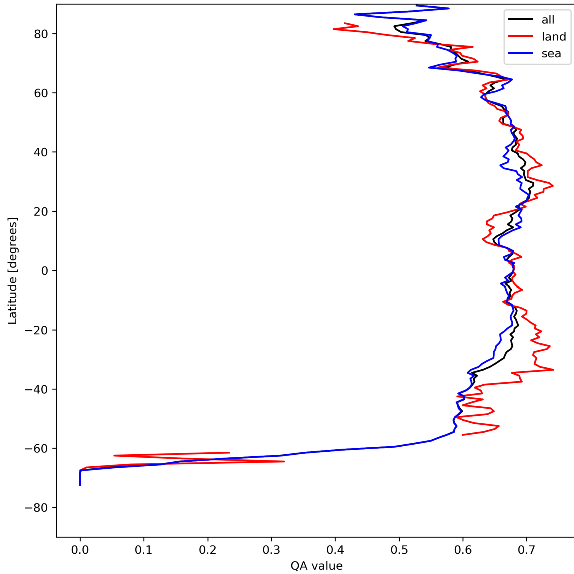
Figure 9: Zonal average of “QA value” for 2023-08-20 to 2023-08-21.
