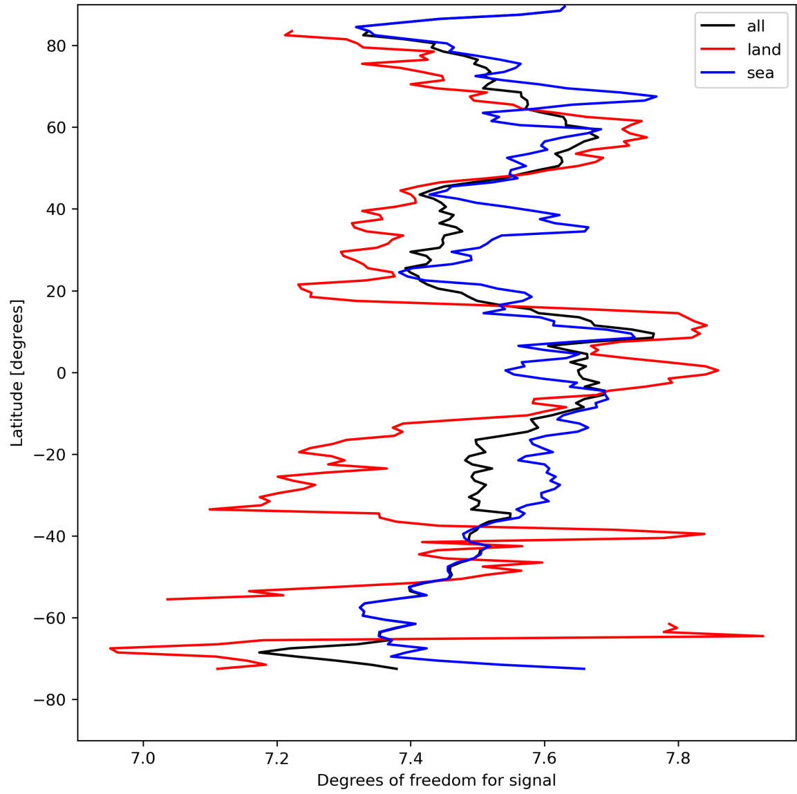
Figure 15: Zonal average of “Degrees of freedom for signal” for 2023-08-20 to 2023-08-21.
