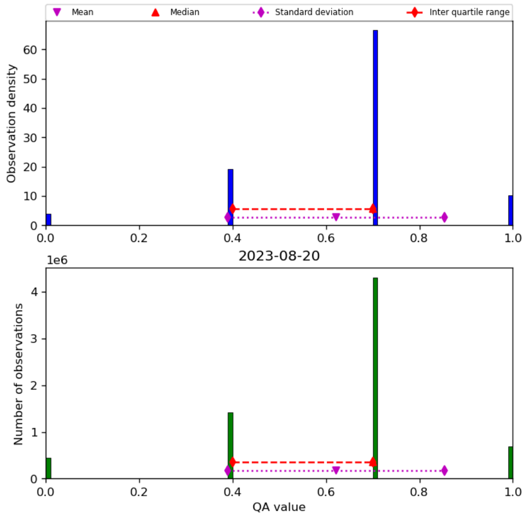
Figure 17: Histogram of “QA value” for 2023-08-20 to 2023-08-21
