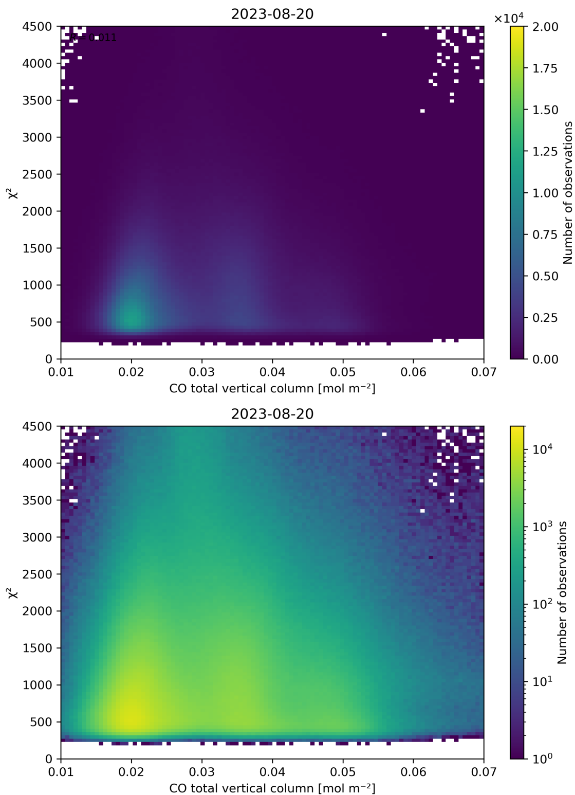
Figure 35: Scatter density plot of “CO total vertical column” against “ \chi^2 ” for 2023-08-20 to 2023-08-21.
