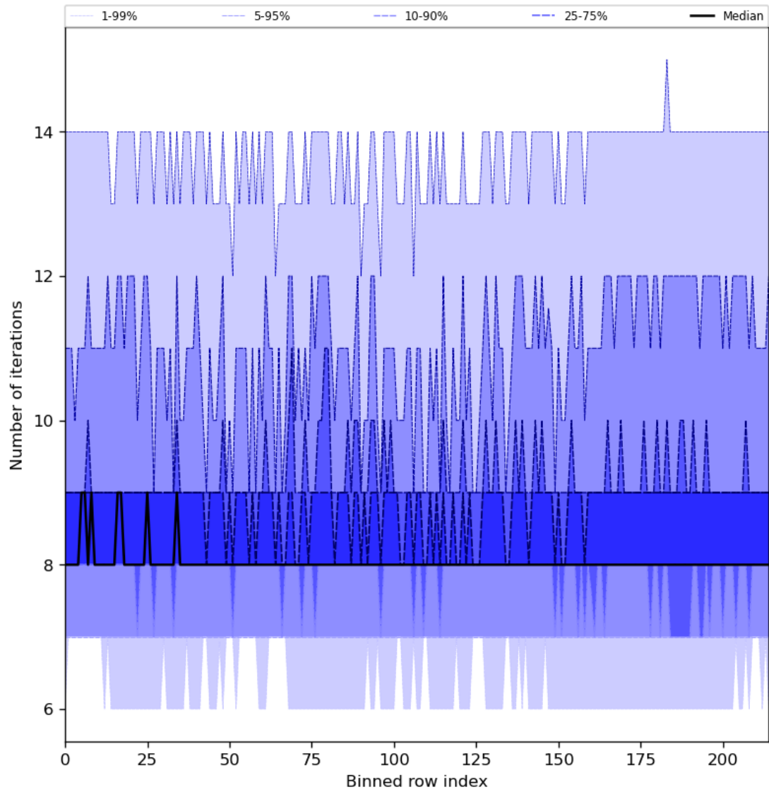
Figure 32: Along track statistics of “Number of iterations” for 2023-08-20 to 2023-08-21
