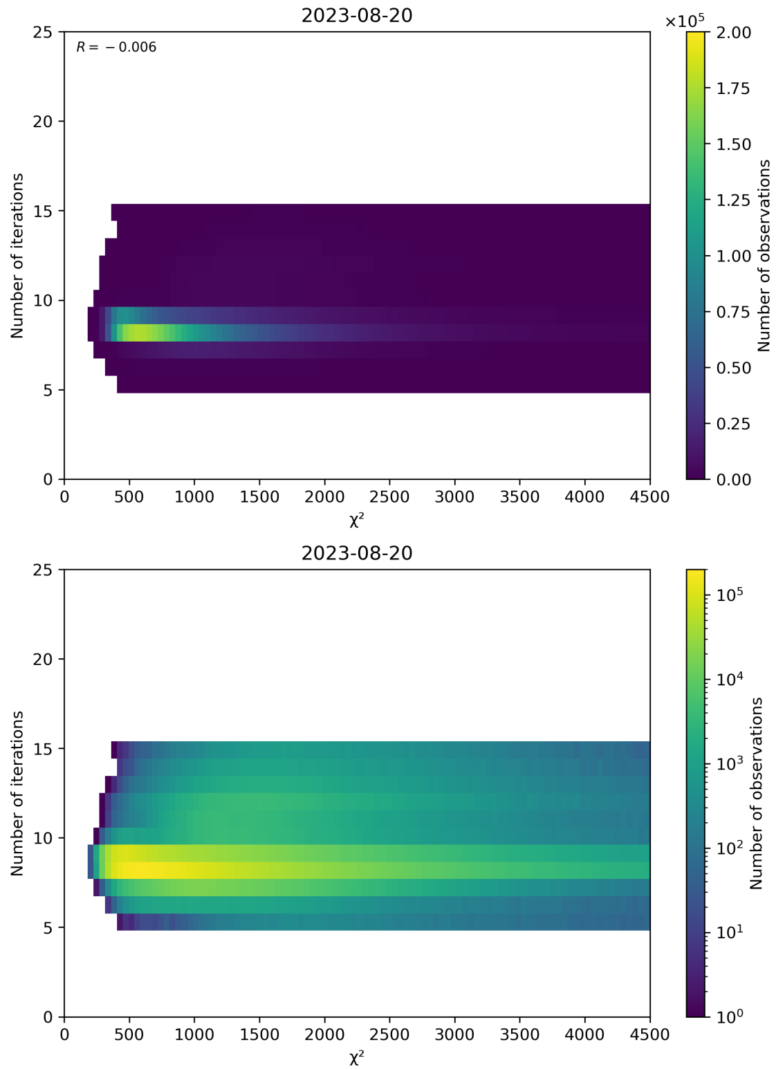
Figure 49: Scatter density plot of “ \chi^2 ” against “Number of iterations” for 2023-08-20 to 2023-08-21.
