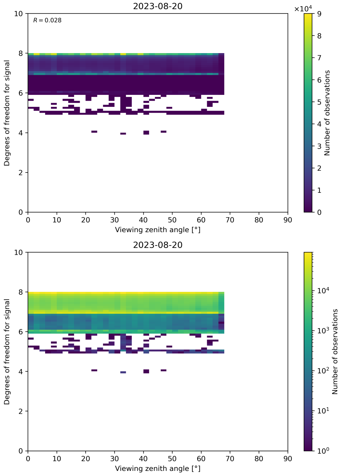
Figure 73: Scatter density plot of “Viewing zenith angle” against “Degrees of freedom for signal” for 2023-08-20 to 2023-08-21.
