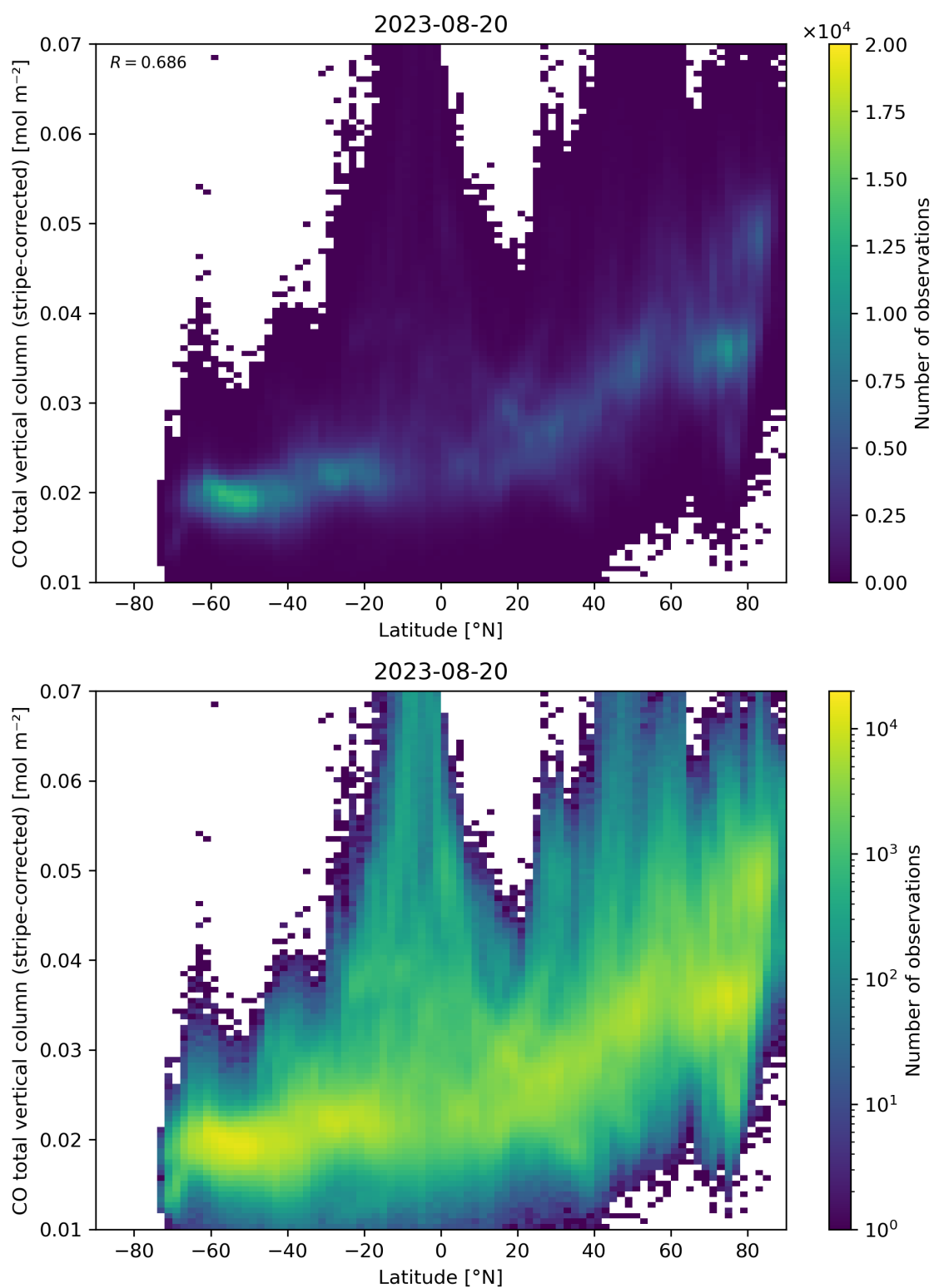
Figure 52: Scatter density plot of “Latitude” against “CO total vertical column (stripe-corrected)” for 2023-08-20 to 2023-08-21.
