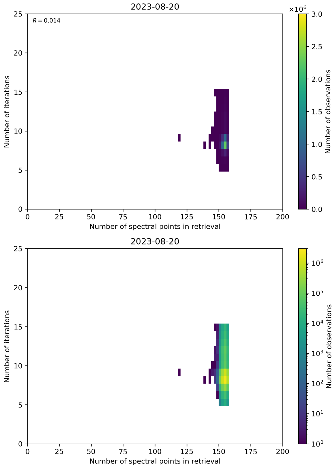
Figure 60: Scatter density plot of “Number of spectral points in retrieval” against “Number of iterations” for 2023-08-20 to 2023-08-21.
