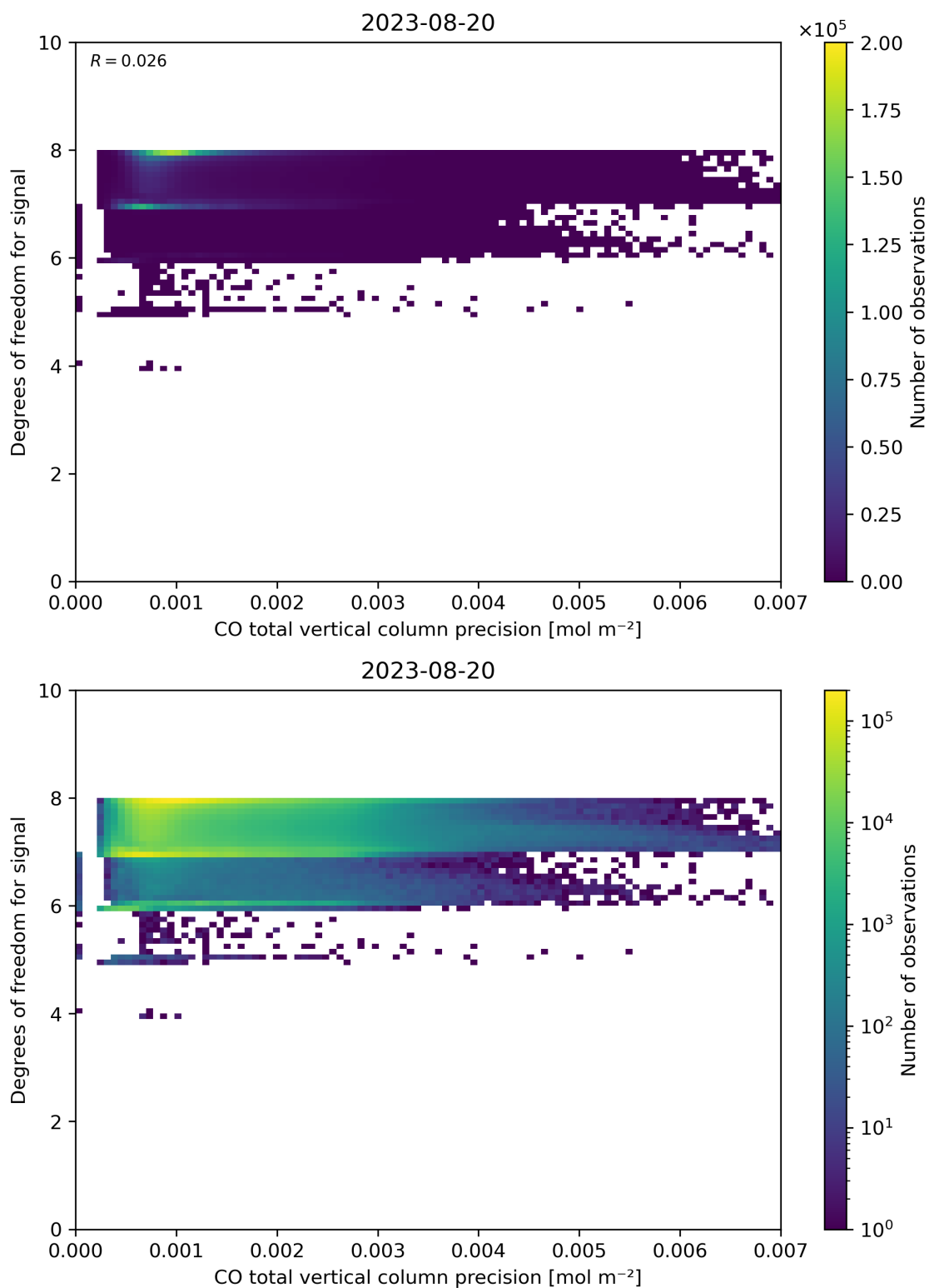
Figure 45: Scatter density plot of “CO total vertical column precision” against “Degrees of freedom for signal” for 2023-08-20 to 2023-08-21.
