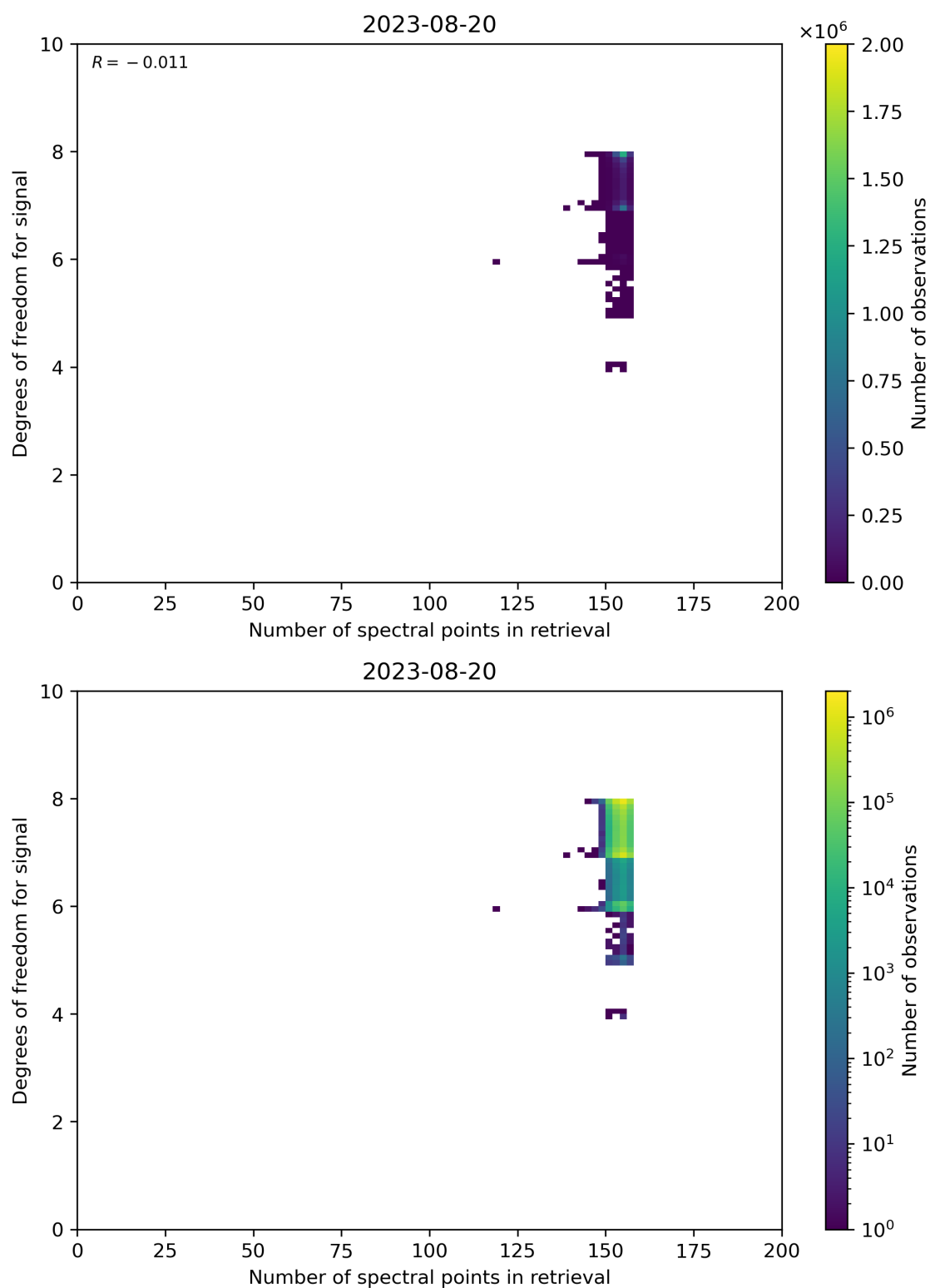
Figure 59: Scatter density plot of “Number of spectral points in retrieval” against “Degrees of freedom for signal” for 2023-08-20 to 2023-08-21.
