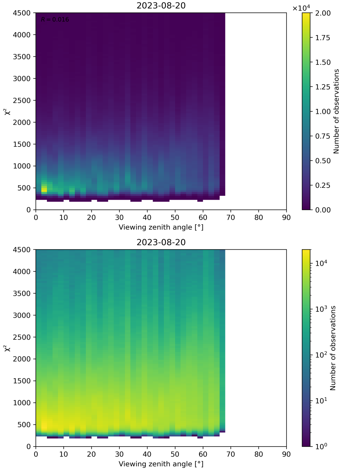
Figure 72: Scatter density plot of “Viewing zenith angle” against “ \chi^2 ” for 2023-08-20 to 2023-08-21.
