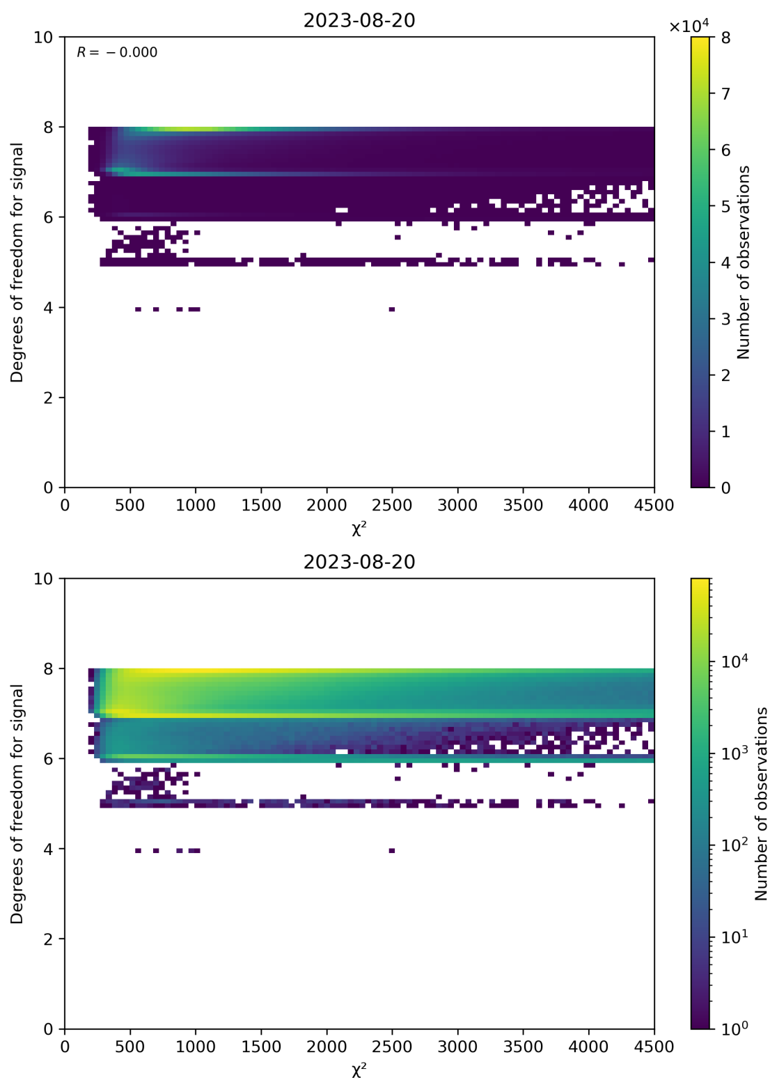
Figure 48: Scatter density plot of “ \chi^2 ” against “Degrees of freedom for signal” for 2023-08-20 to 2023-08-21.
