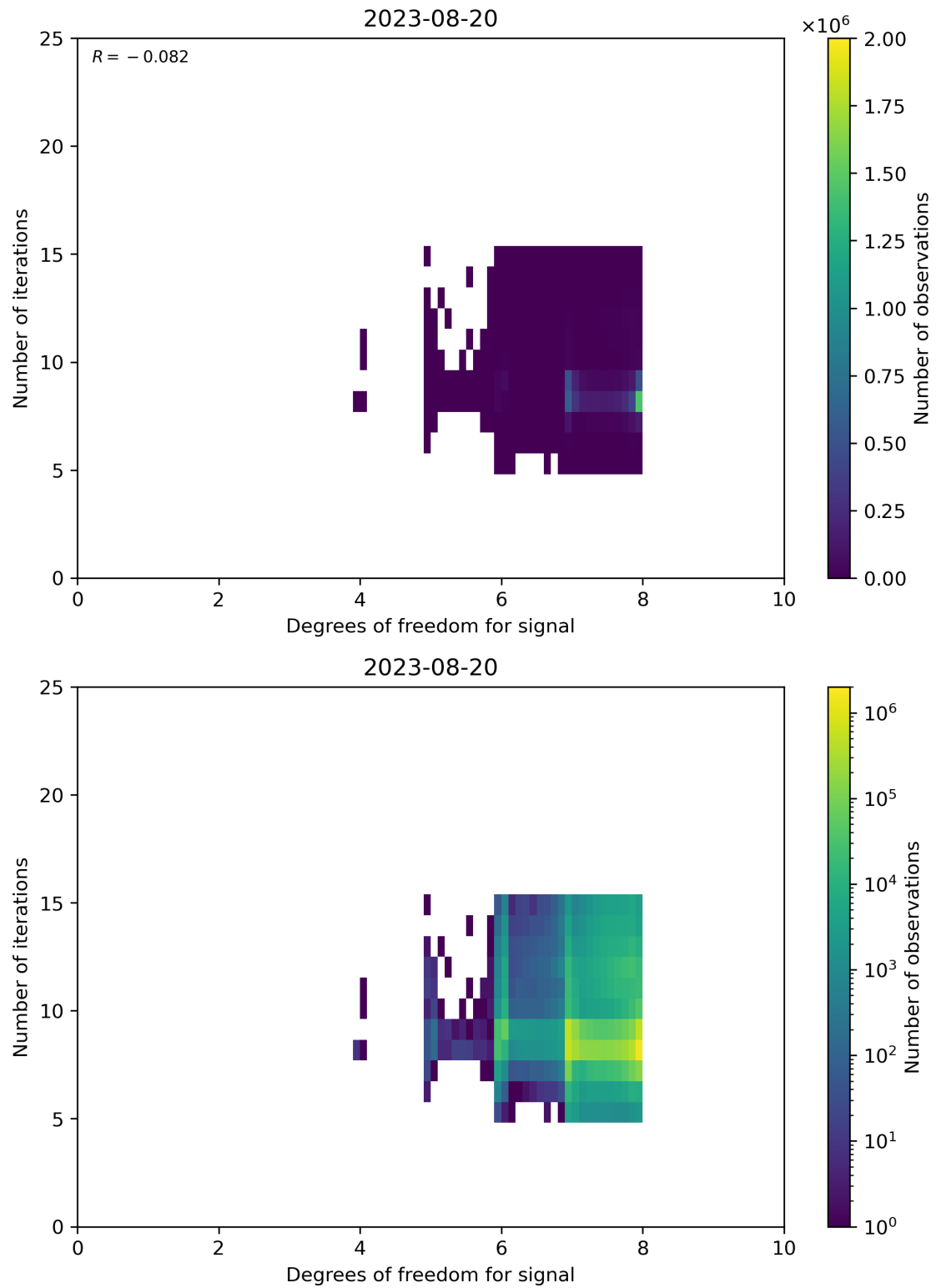
Figure 50: Scatter density plot of “Degrees of freedom for signal” against “Number of iterations” for 2023-08-20 to 2023-08-21.
