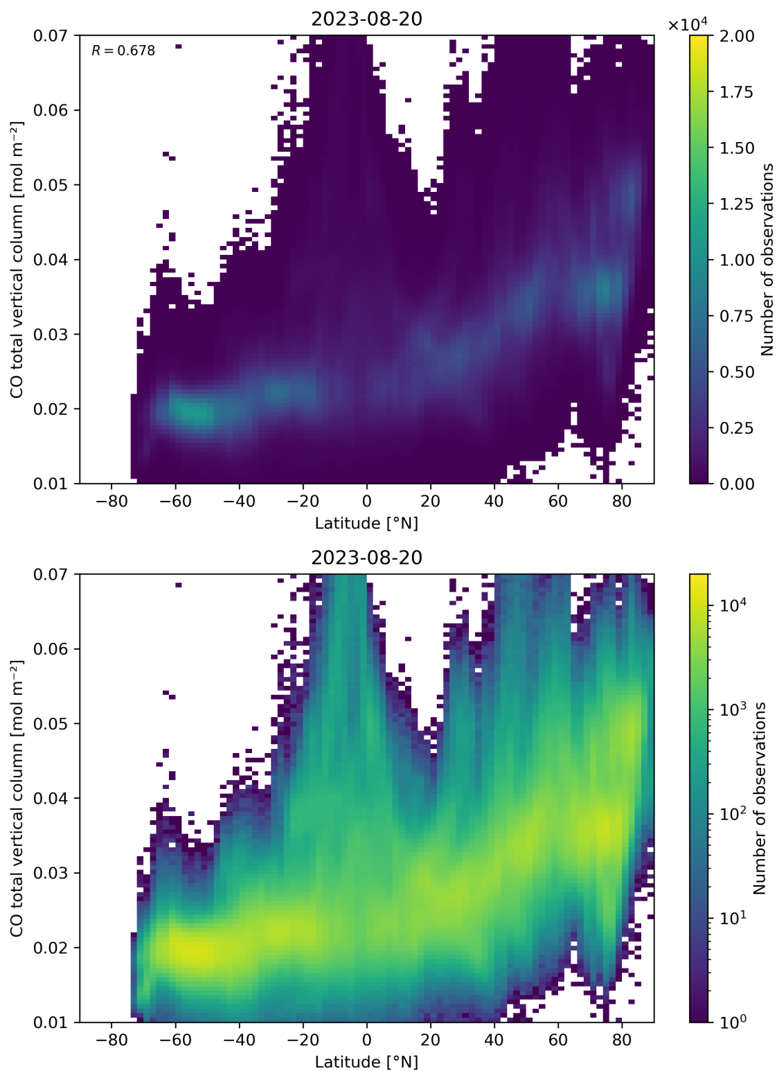
Figure 51: Scatter density plot of “Latitude” against “CO total vertical column” for 2023-08-20 to 2023-08-21.
