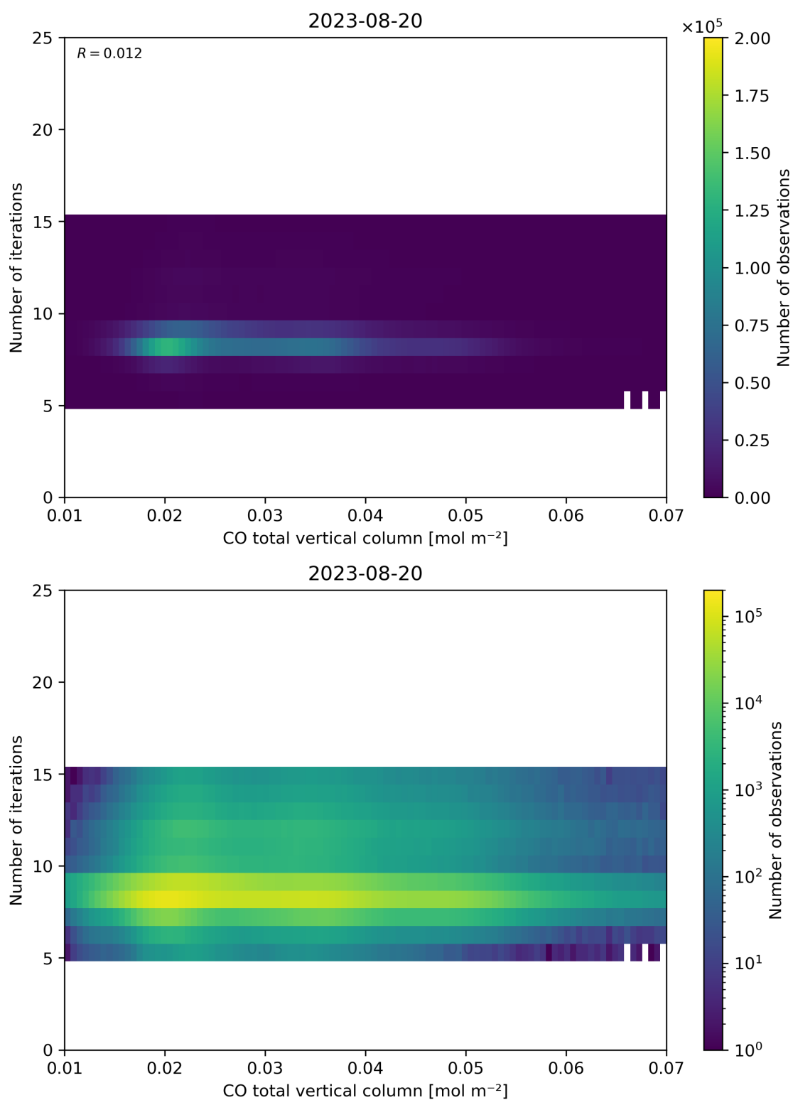
Figure 42: Scatter density plot of “CO total vertical column” against “Number of iterations” for 2023-08-20 to 2023-08-21.
