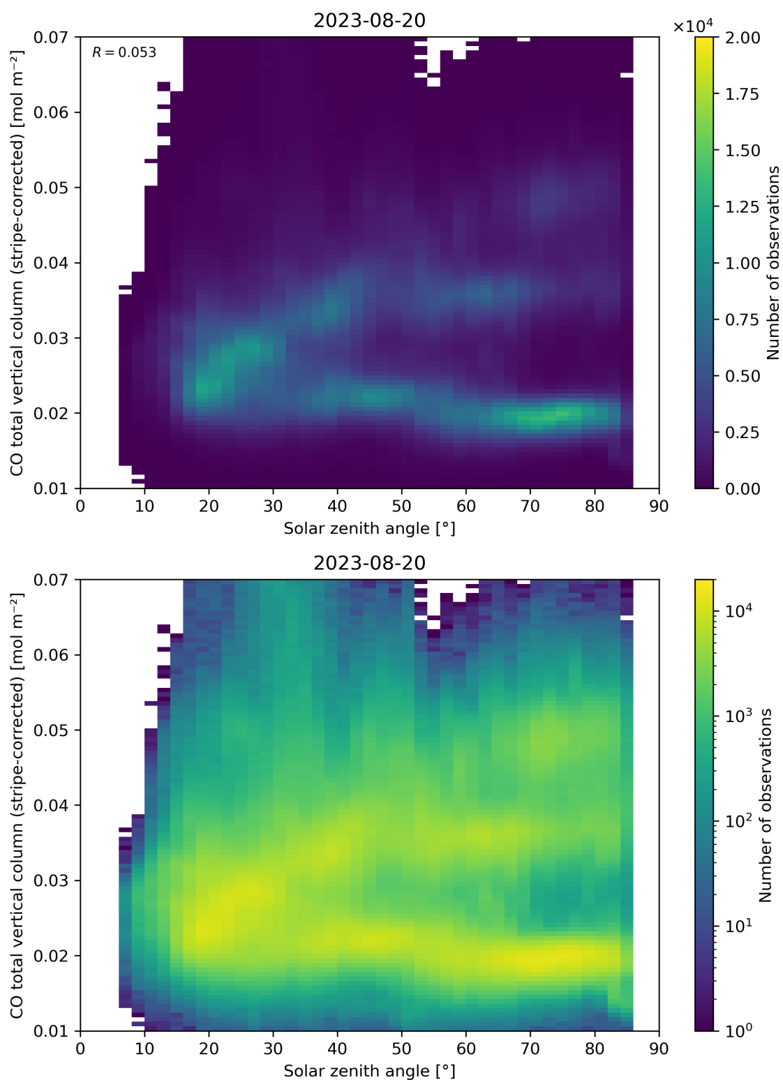
Figure 62: Scatter density plot of “Solar zenith angle” against “CO total vertical column (stripe-corrected)” for 2023-08-20 to 2023-08-21.
