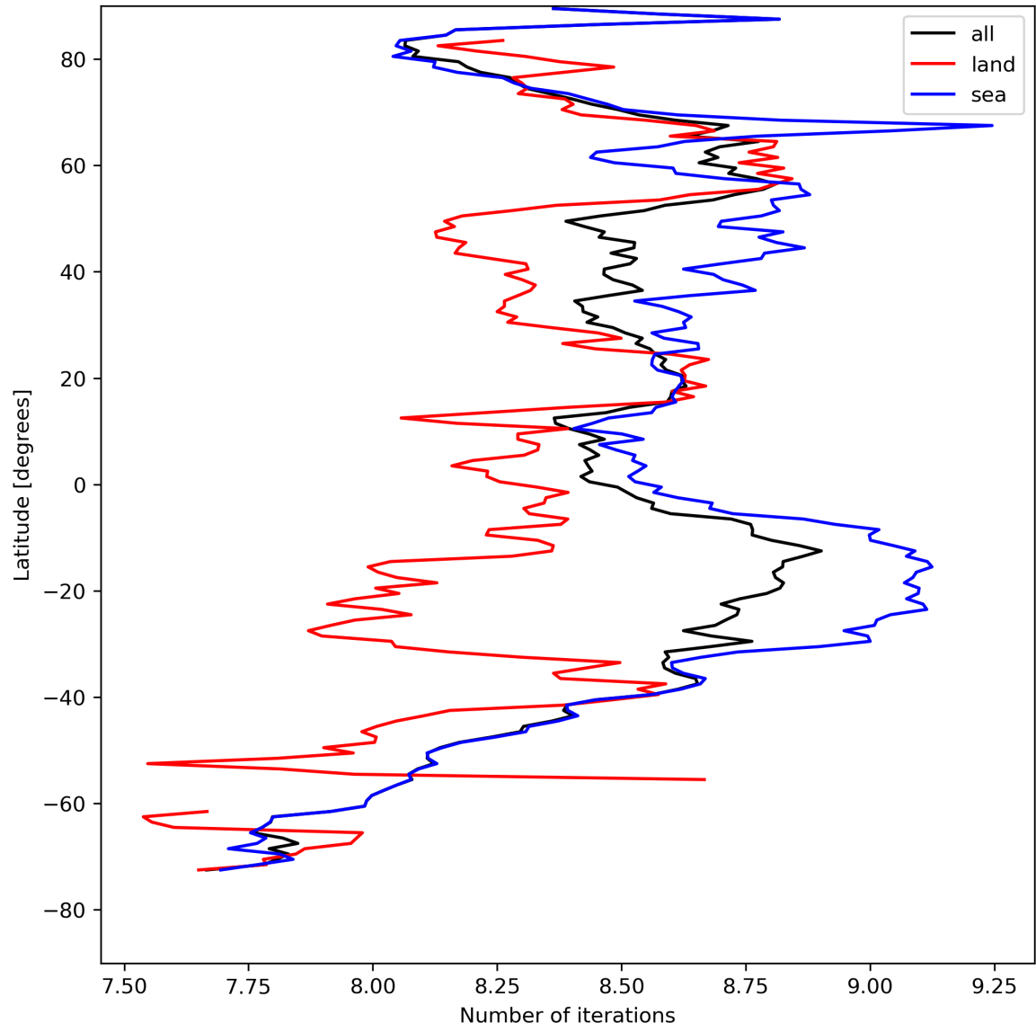
Figure 16: Zonal average of “Number of iterations” for 2023-08-20 to 2023-08-21.
