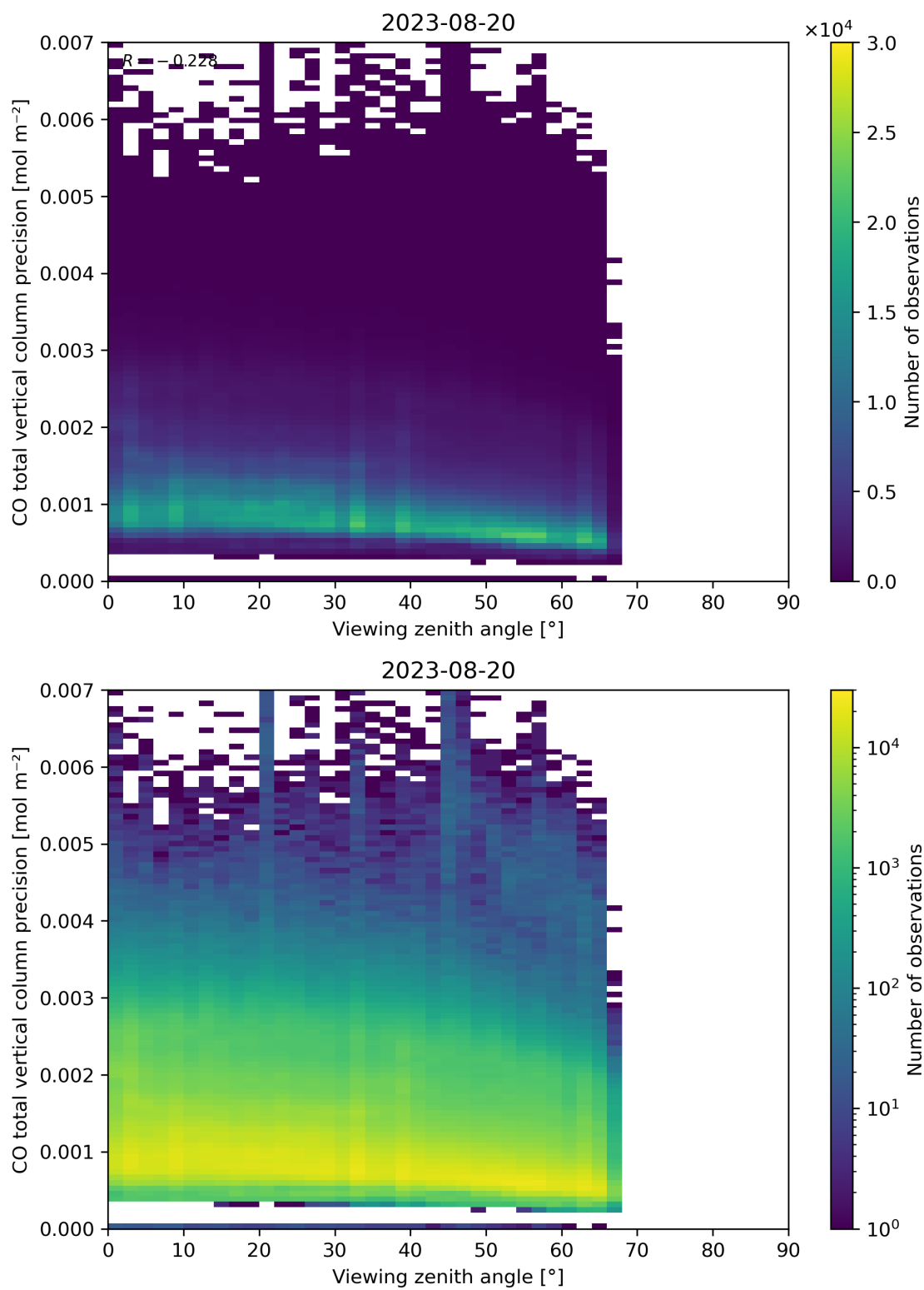
Figure 71: Scatter density plot of “Viewing zenith angle” against “CO total vertical column precision” for 2023-08-20 to 2023-08-21.
