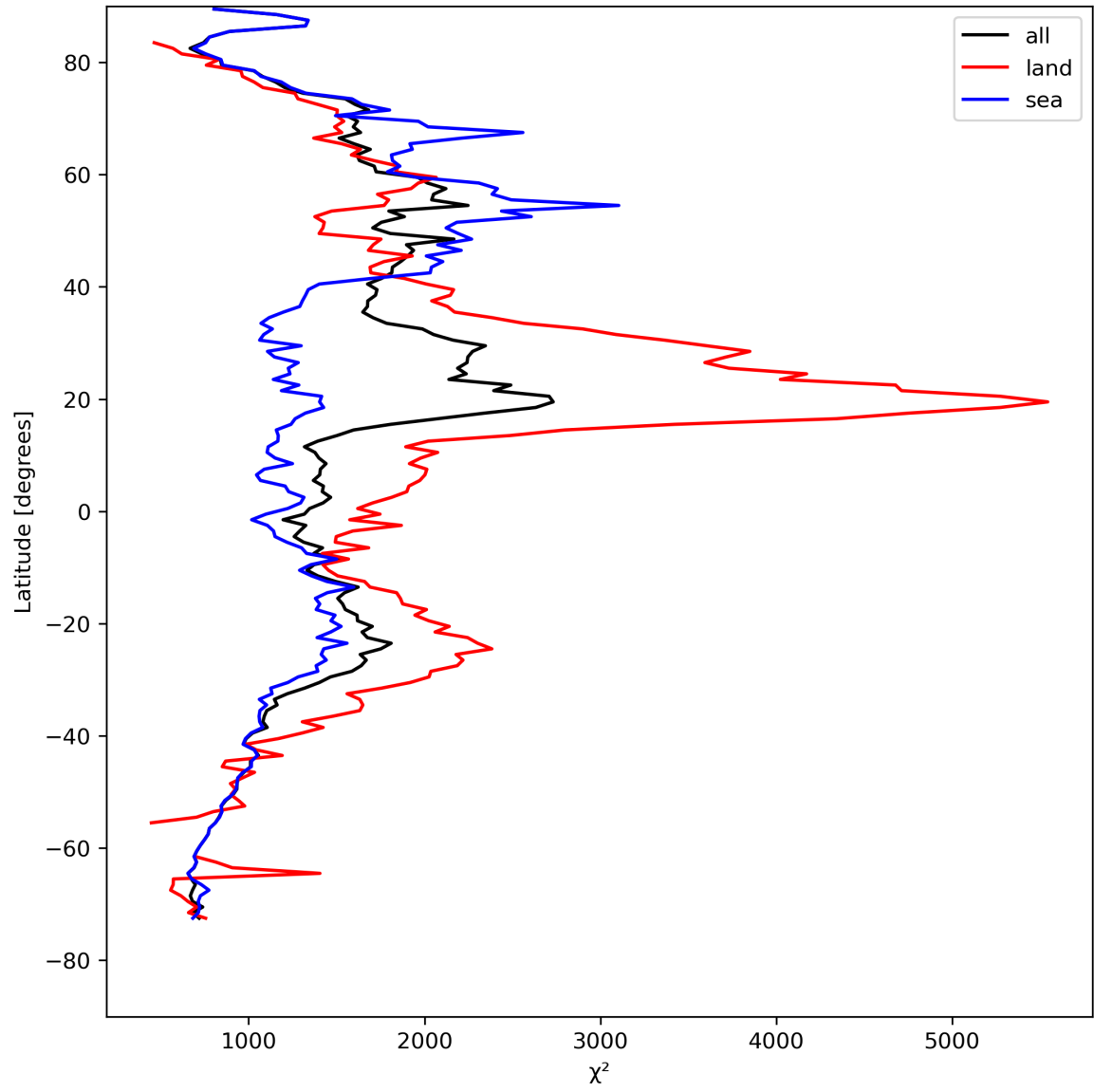
Figure 14: Zonal average of “ \chi^2 ” for 2023-08-20 to 2023-08-21.
