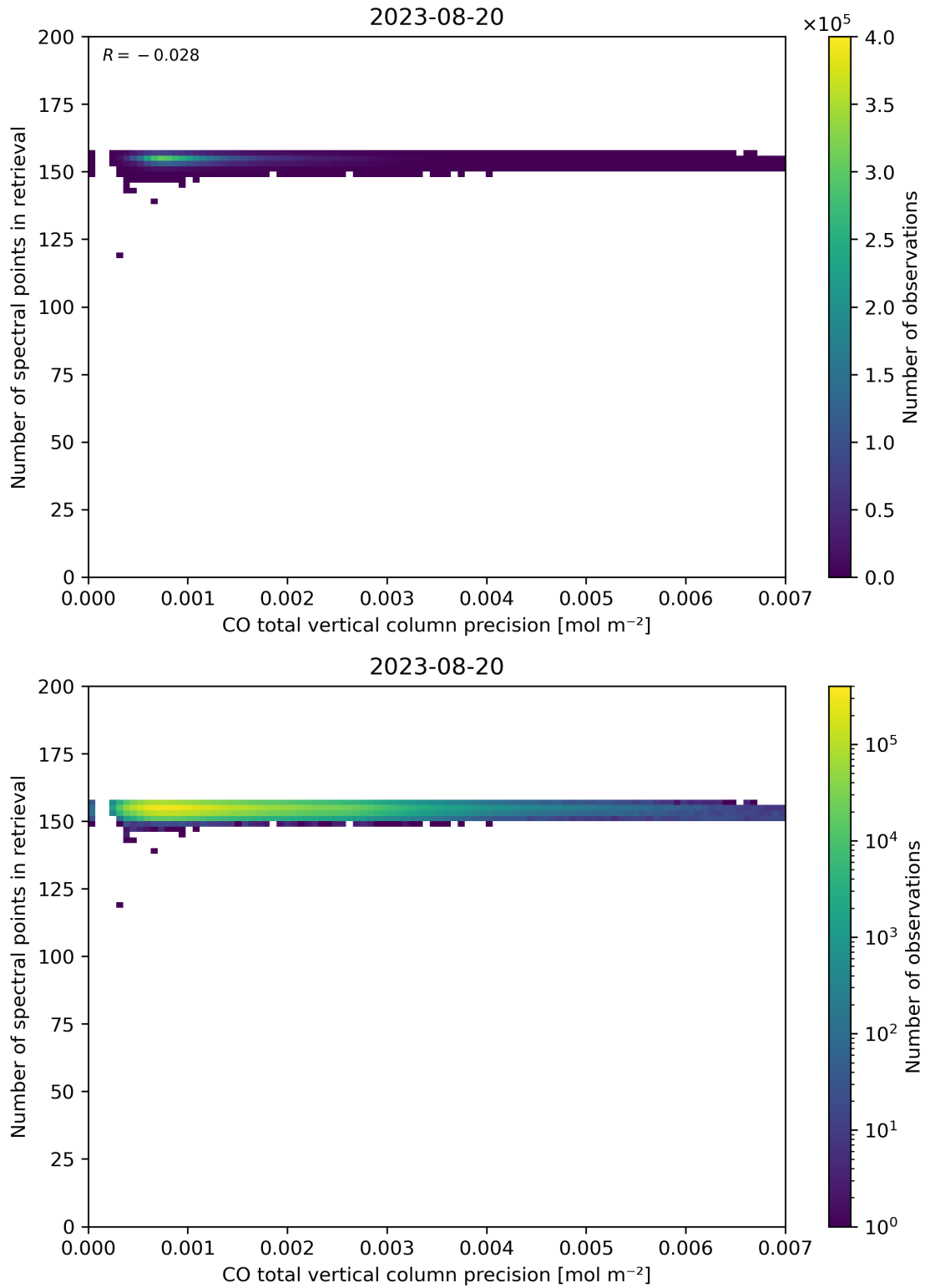
Figure 47: Scatter density plot of “CO total vertical column precision” against “Number of spectral points in retrieval” for 2023-08-20 to 2023-08-21.
