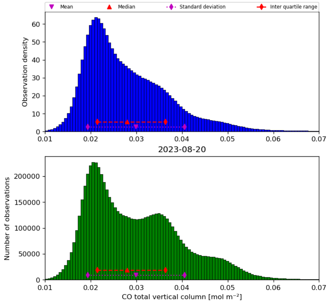
Figure 18: Histogram of “CO total vertical column” for 2023-08-20 to 2023-08-21
