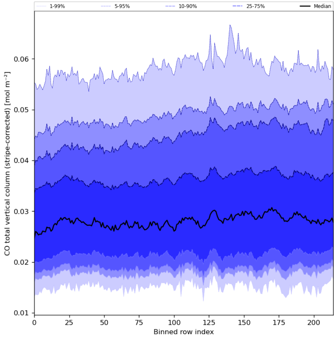
Figure 27: Along track statistics of “CO total vertical column (stripe-corrected)” for 2023-08-20 to 2023-08-21
