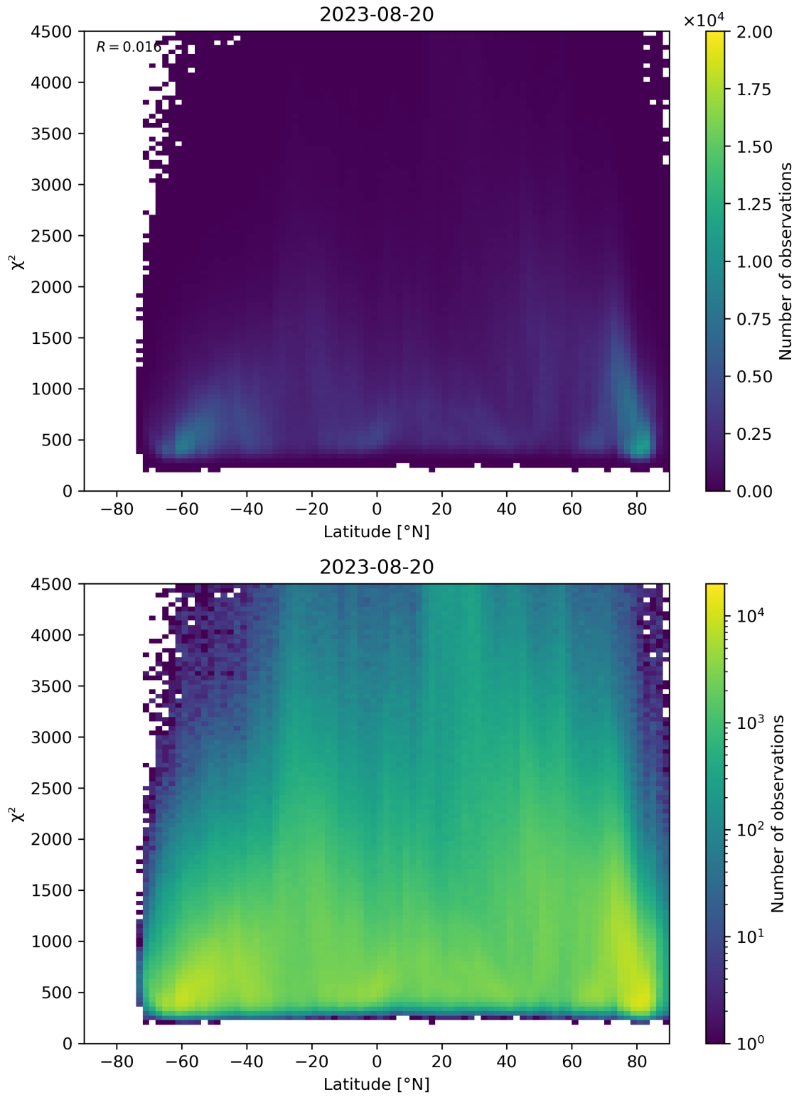
Figure 54: Scatter density plot of “Latitude” against “ \chi^2 ” for 2023-08-20 to 2023-08-21.
