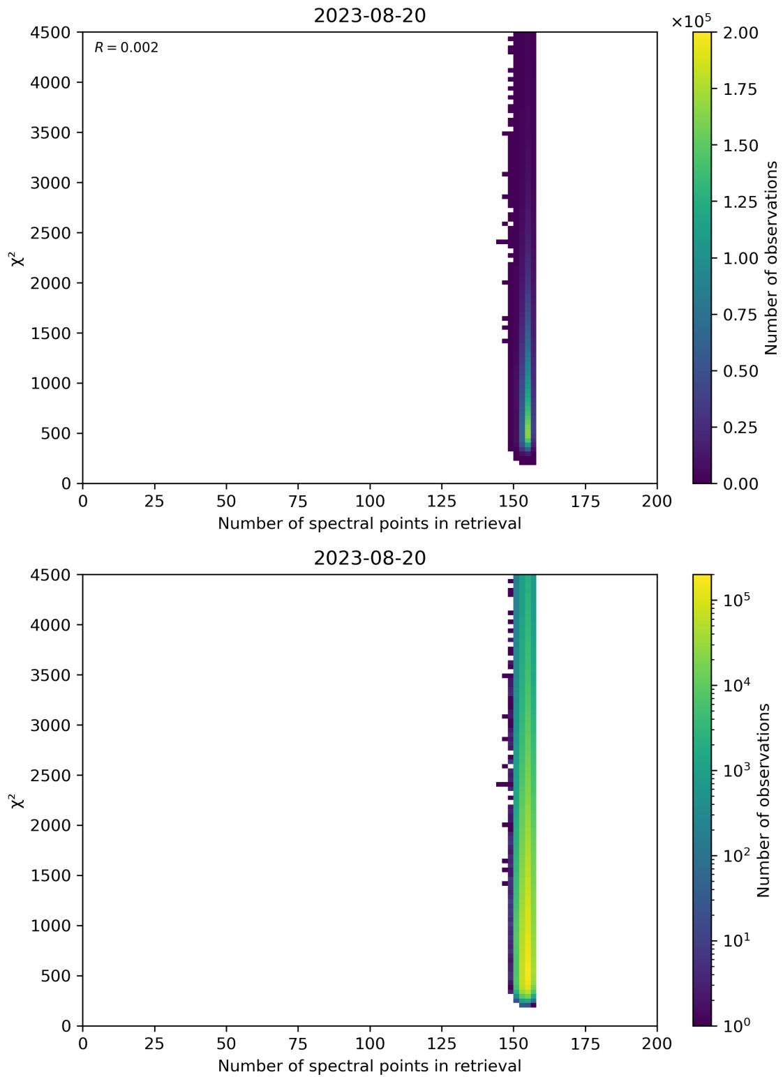
Figure 58: Scatter density plot of “Number of spectral points in retrieval” against “ \chi^2 ” for 2023-08-20 to 2023-08-21.
