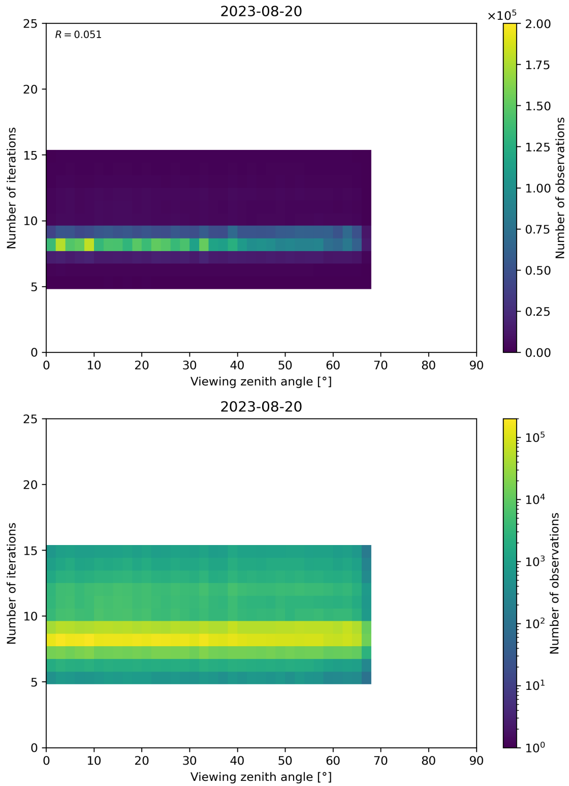
Figure 75: Scatter density plot of “Viewing zenith angle” against “Number of iterations” for 2023-08-20 to 2023-08-21.
