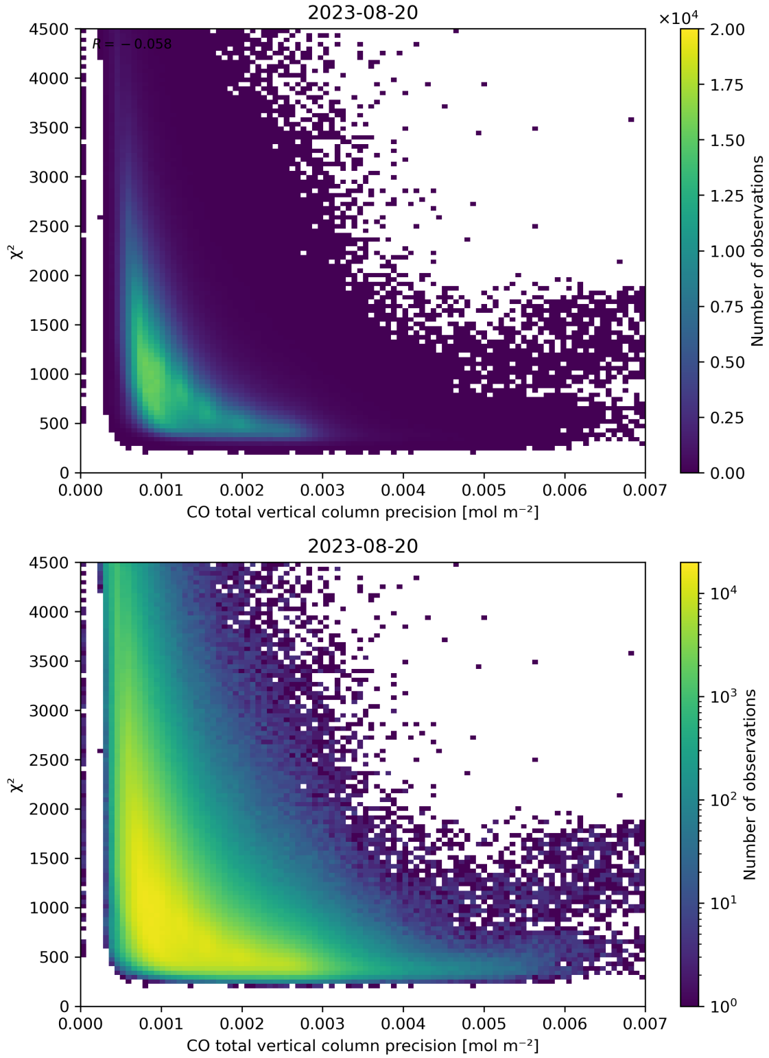
Figure 44: Scatter density plot of “CO total vertical column precision” against “ \chi^2 ” for 2023-08-20 to 2023-08-21.
