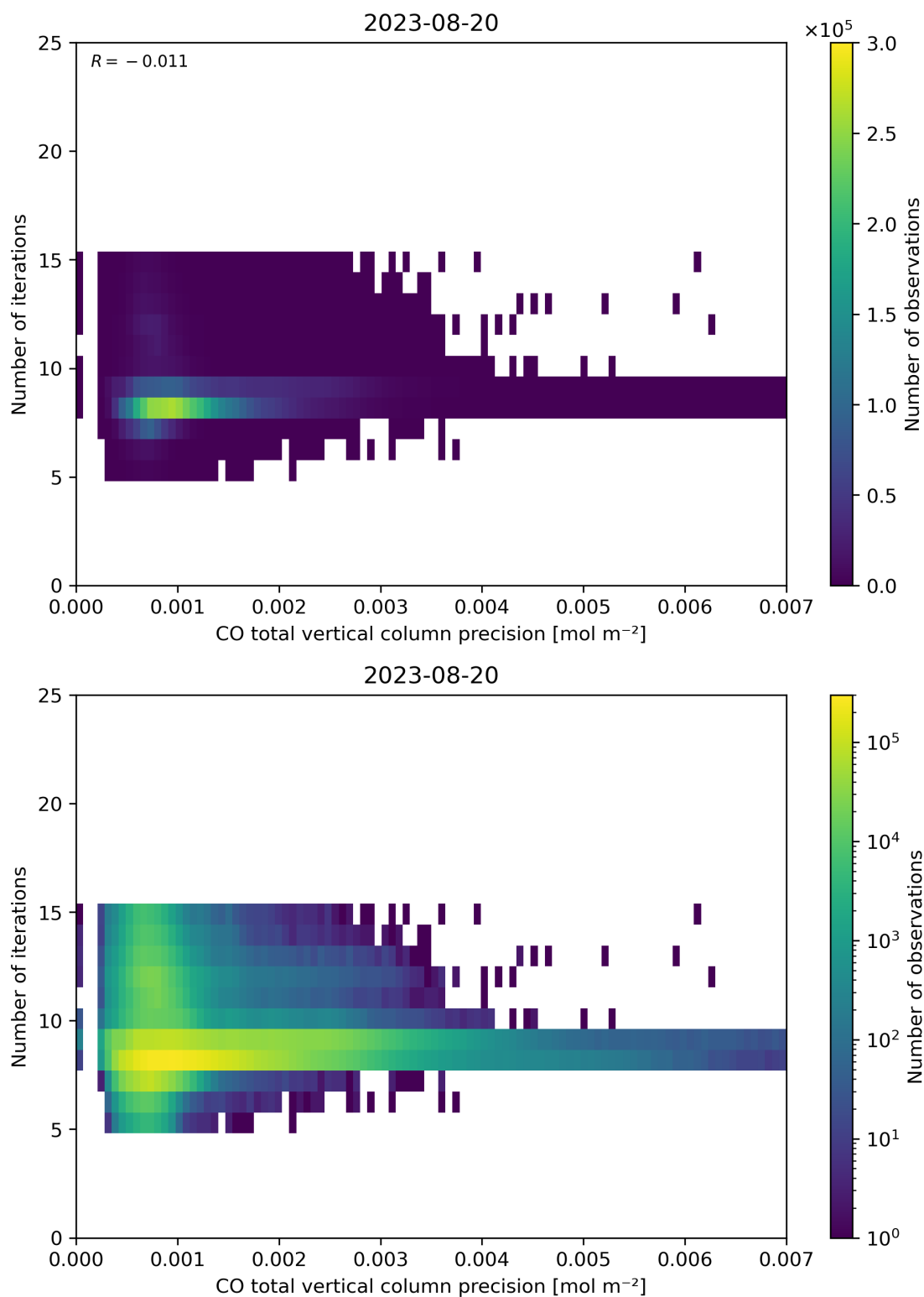
Figure 46: Scatter density plot of “CO total vertical column precision” against “Number of iterations” for 2023-08-20 to 2023-08-21.
