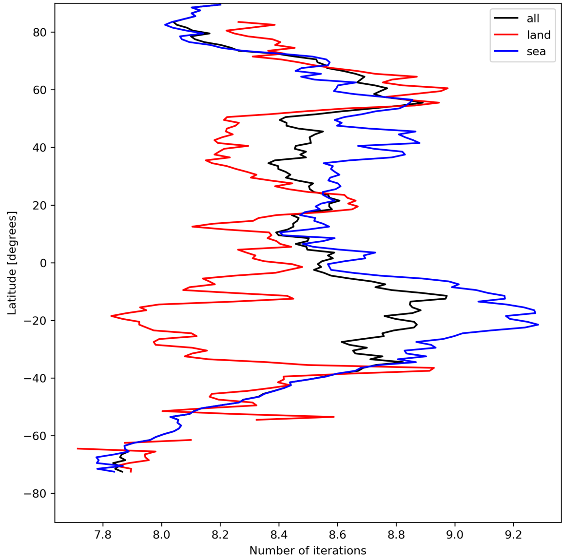
Figure 16: Zonal average of “Number of iterations” for 2023-08-20 to 2023-08-22.
