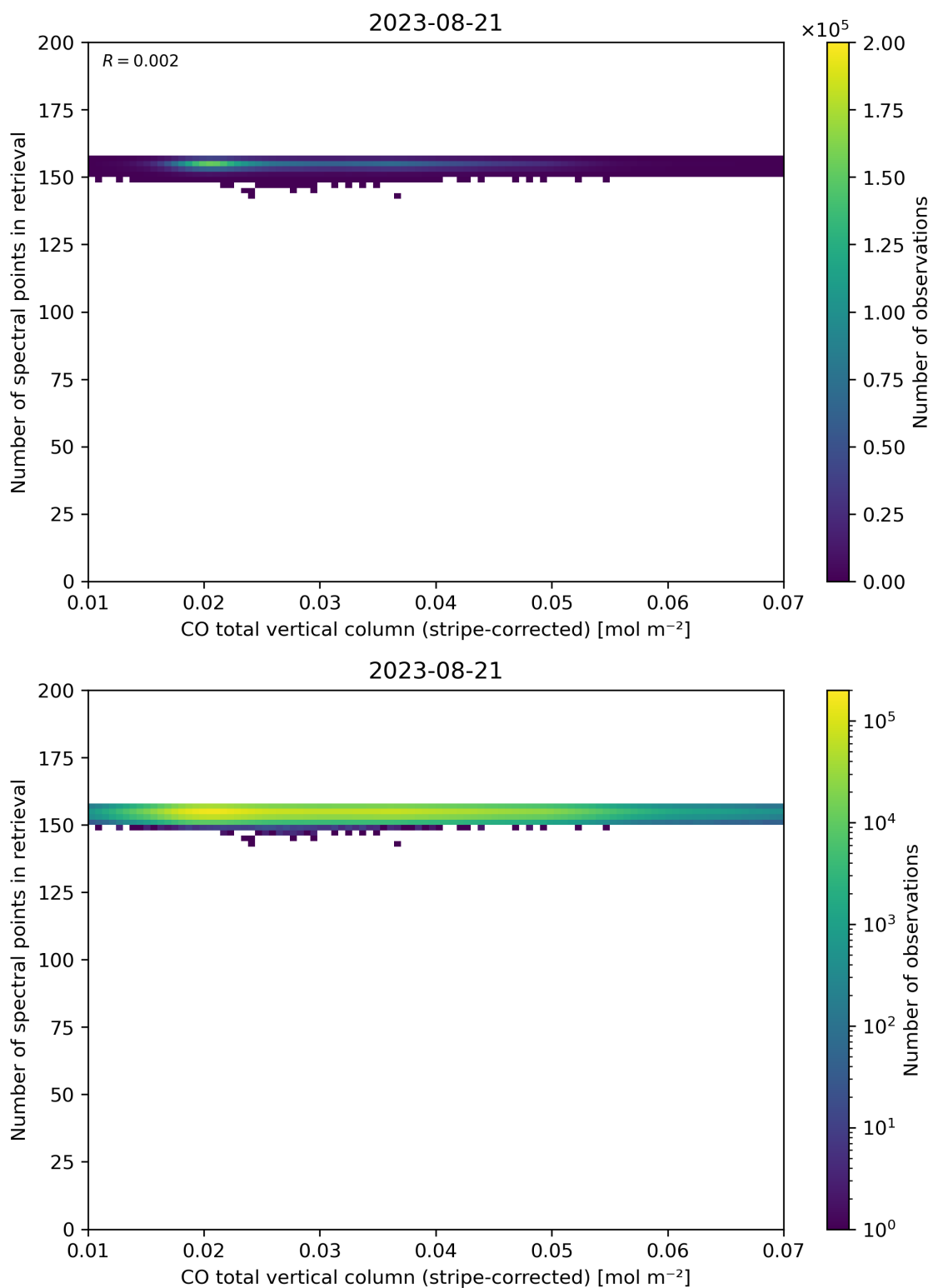
Figure 40: Scatter density plot of “CO total vertical column (stripe-corrected)” against “Number of spectral points in retrieval” for 2023-08-20 to 2023-08-22.
