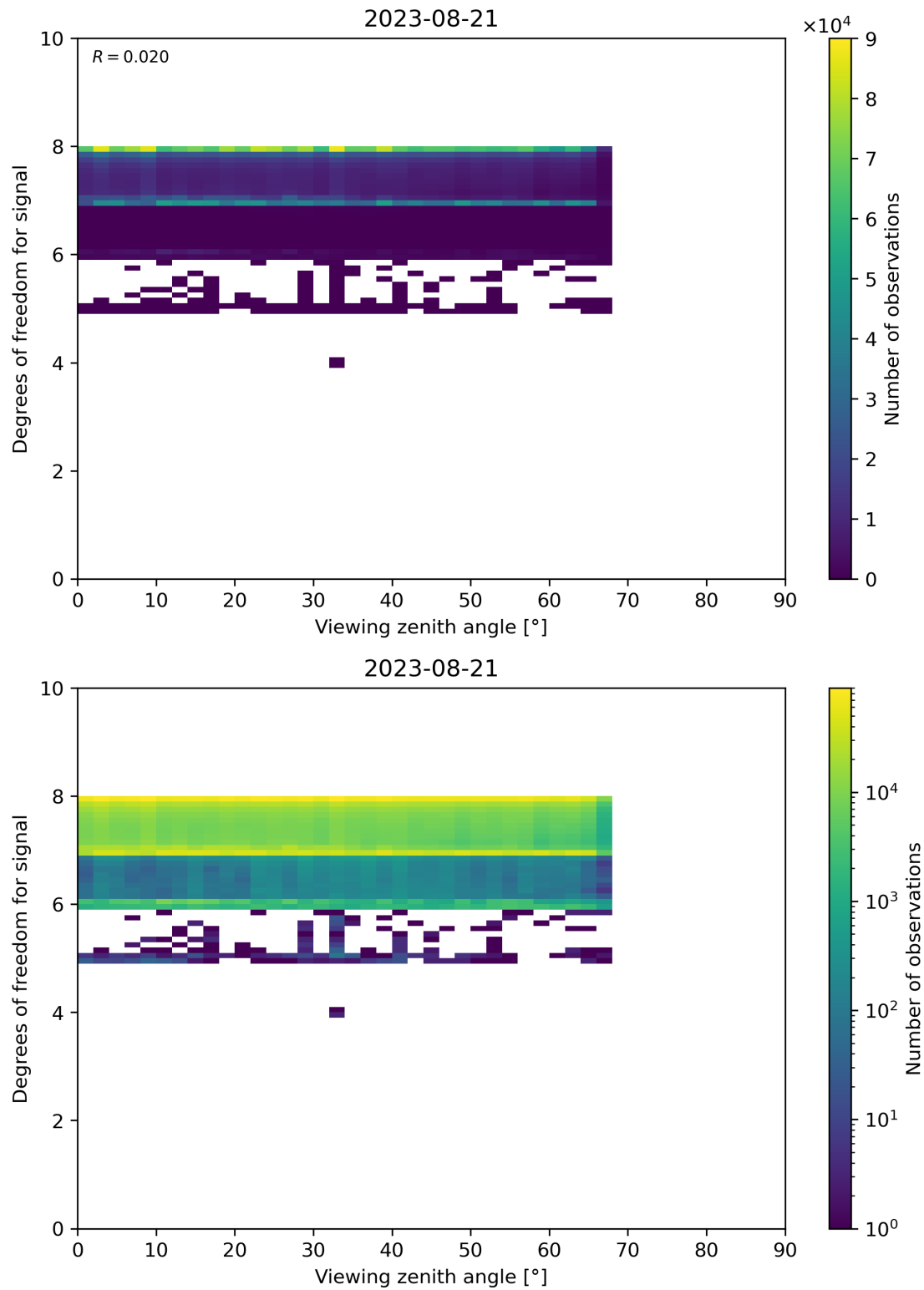
Figure 73: Scatter density plot of “Viewing zenith angle” against “Degrees of freedom for signal” for 2023-08-20 to 2023-08-22.
