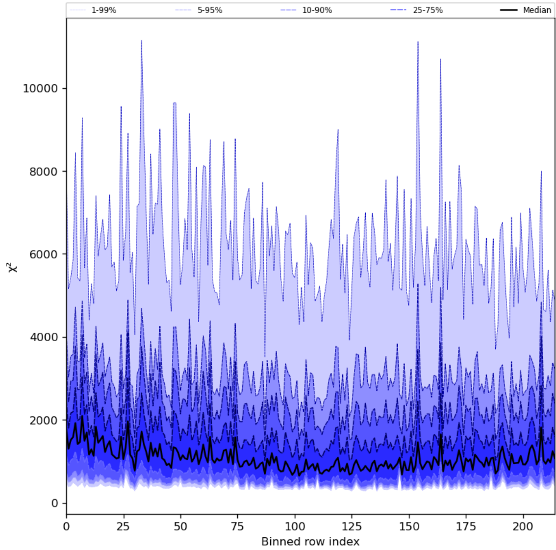
Figure 30: Along track statistics of “ \chi^2 ” for 2023-08-20 to 2023-08-22
