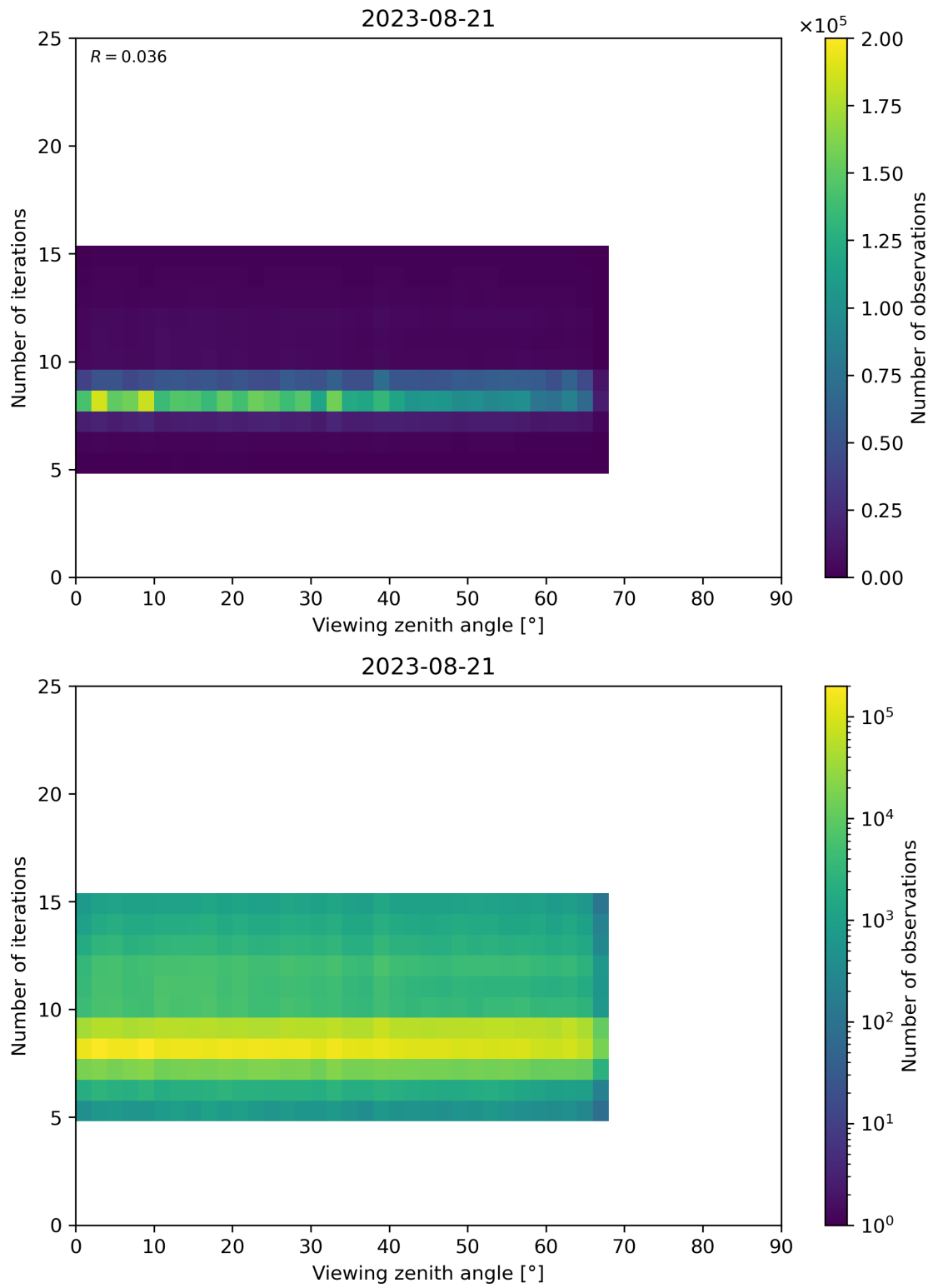
Figure 75: Scatter density plot of “Viewing zenith angle” against “Number of iterations” for 2023-08-20 to 2023-08-22.
