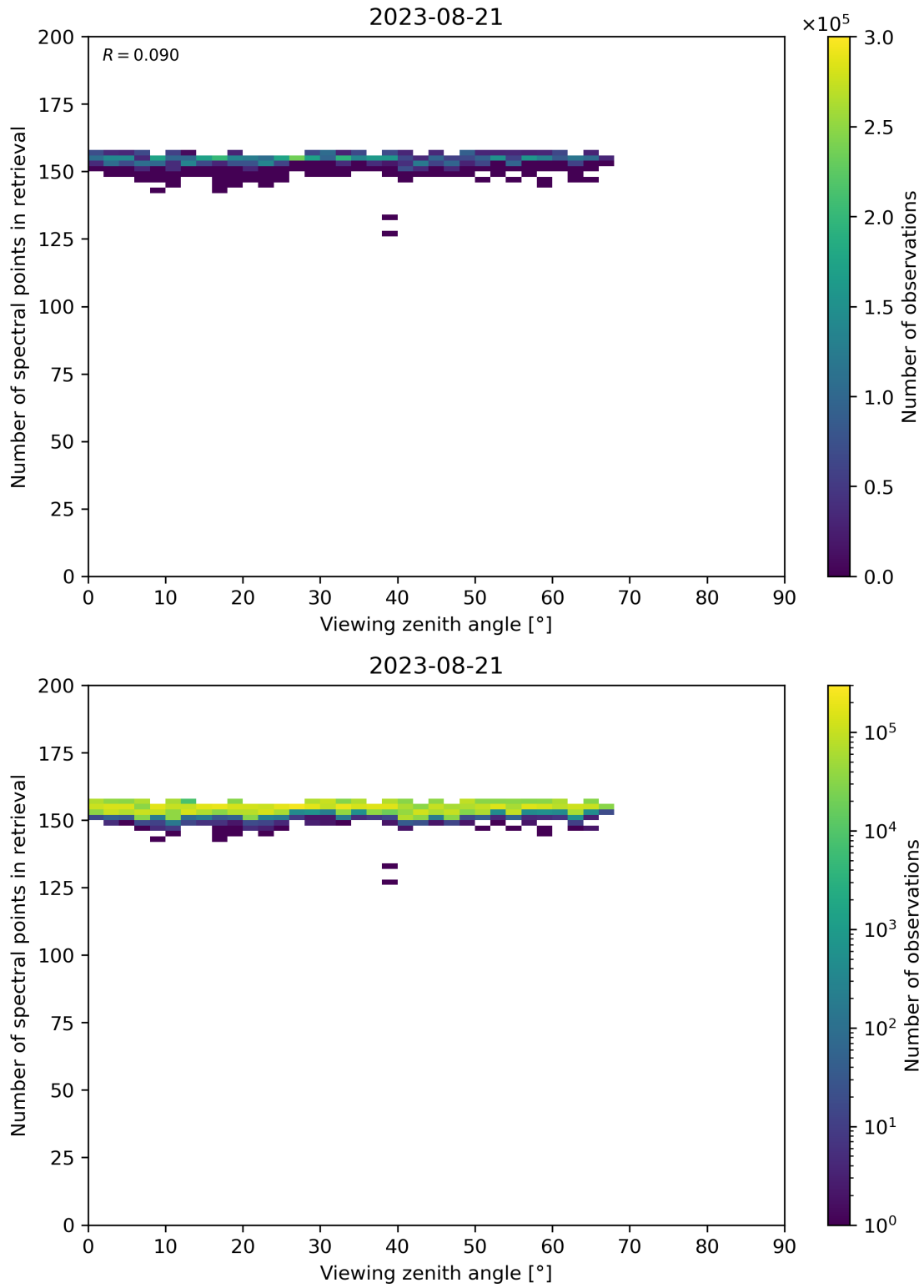
Figure 76: Scatter density plot of “Viewing zenith angle” against “Number of spectral points in retrieval” for 2023-08-20 to 2023-08-22.
