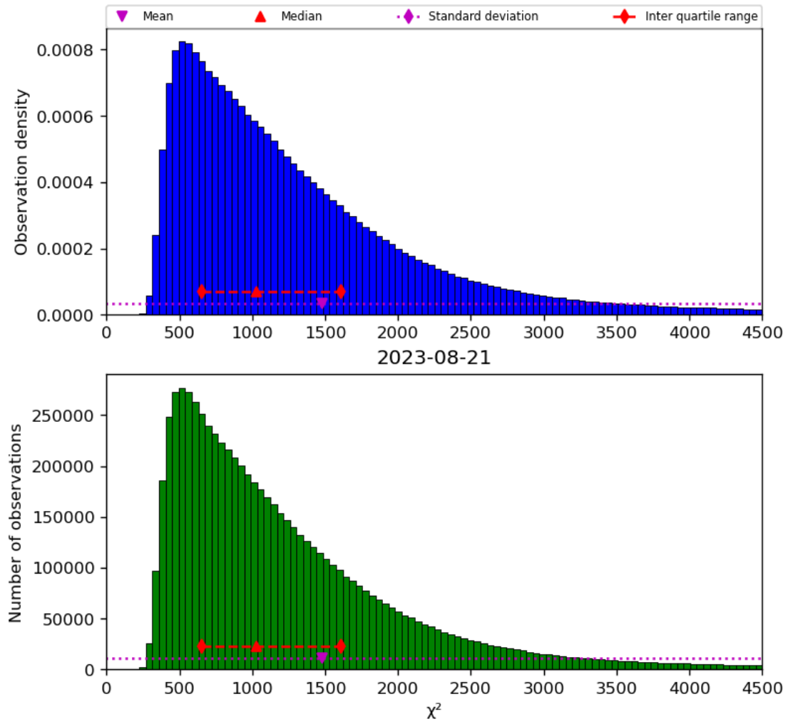
Figure 22: Histogram of “ \chi^2 ” for 2023-08-20 to 2023-08-22
