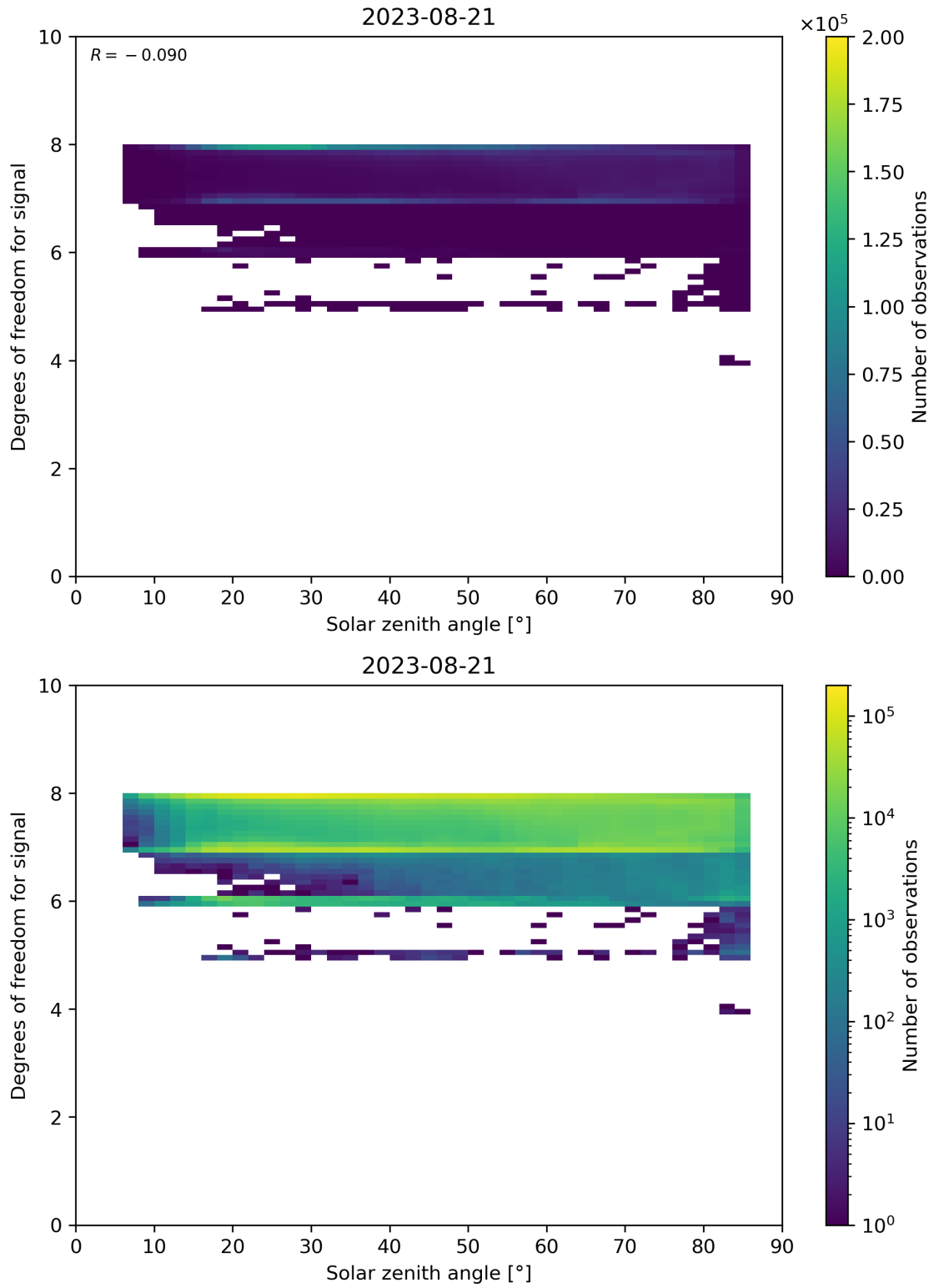
Figure 65: Scatter density plot of “Solar zenith angle” against “Degrees of freedom for signal” for 2023-08-20 to 2023-08-22.
