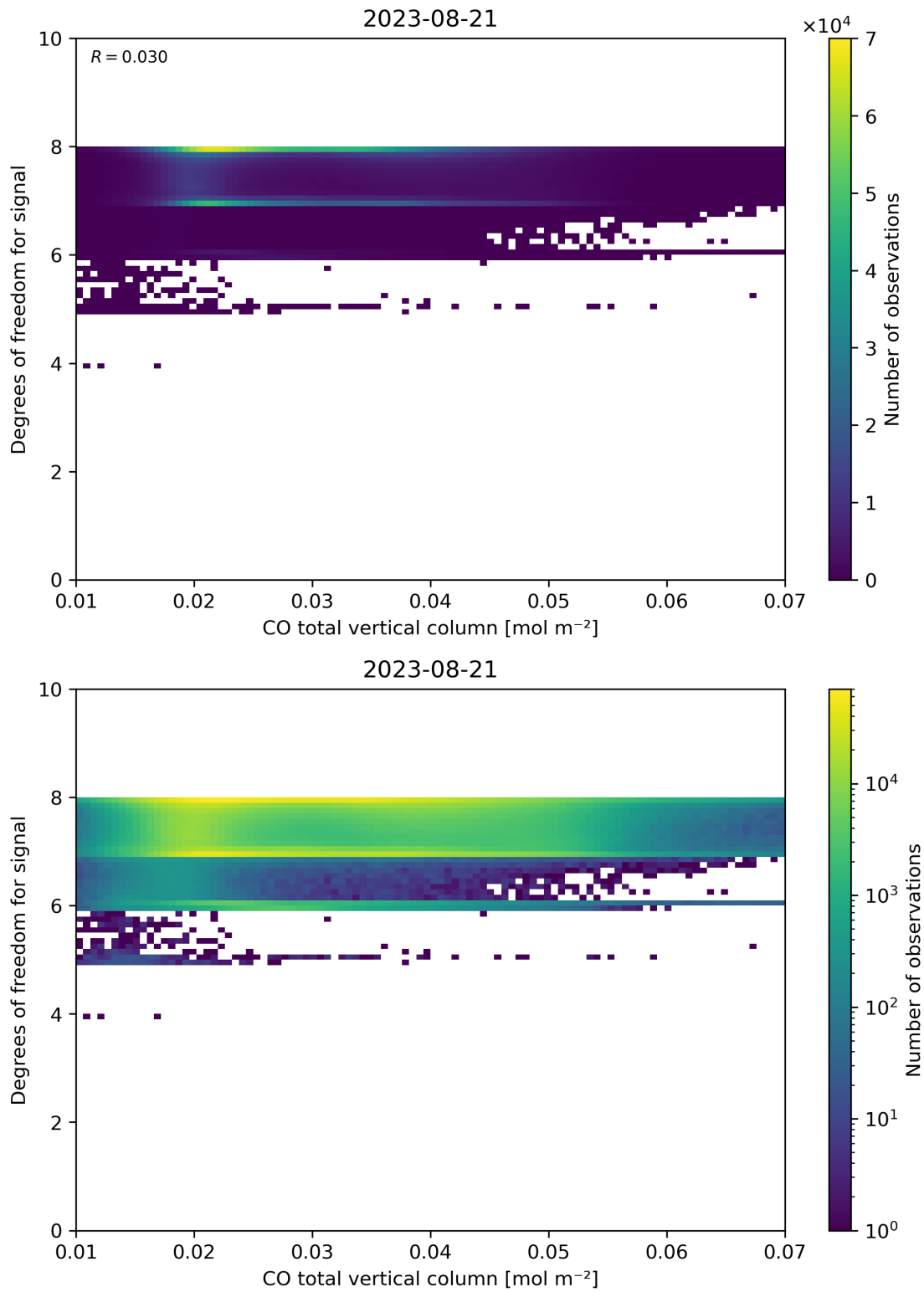
Figure 41: Scatter density plot of “CO total vertical column” against “Degrees of freedom for signal” for 2023-08-20 to 2023-08-22.
