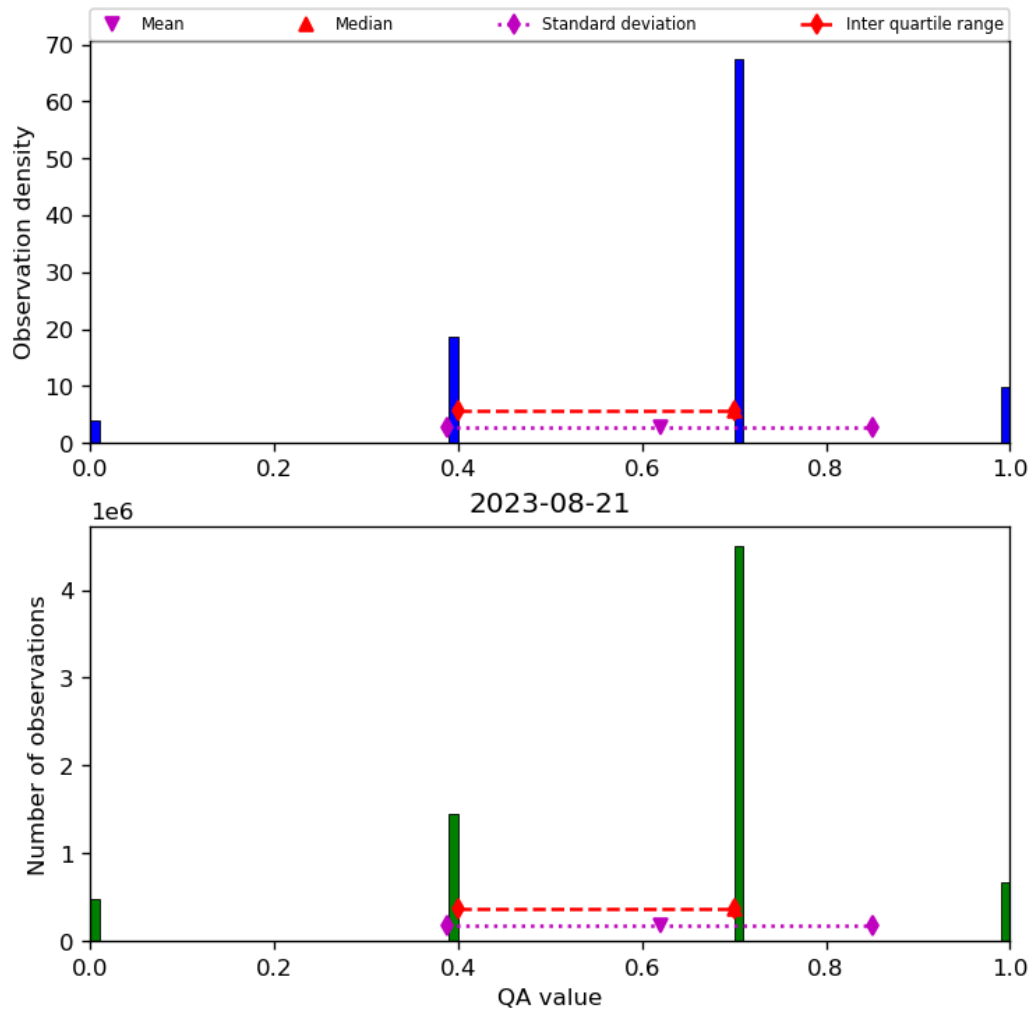
Figure 17: Histogram of "QA value" for 2023-08-20 to 2023-08-22
