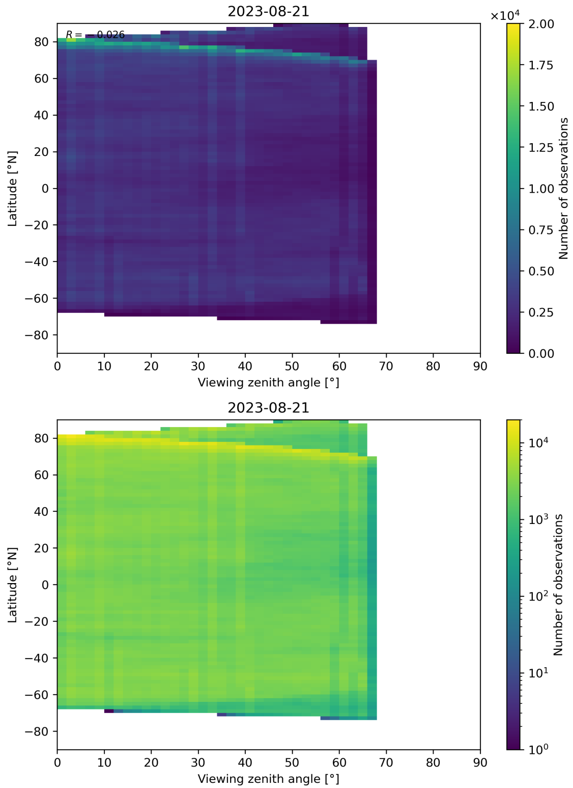
Figure 74: Scatter density plot of “Viewing zenith angle” against “Latitude” for 2023-08-20 to 2023-08-22.
