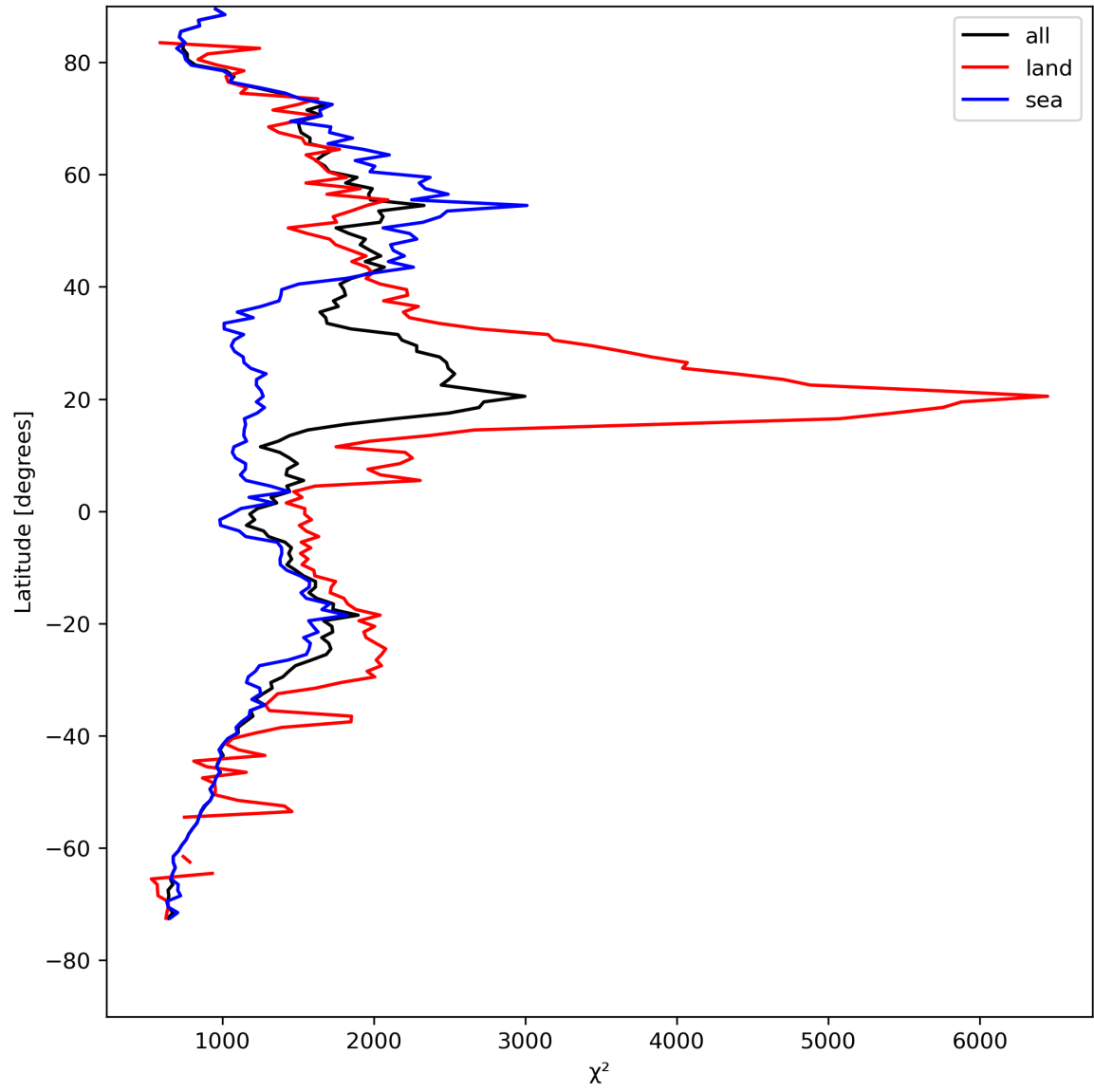
Figure 14: Zonal average of “ \chi^2 ” for 2023-08-20 to 2023-08-22.
