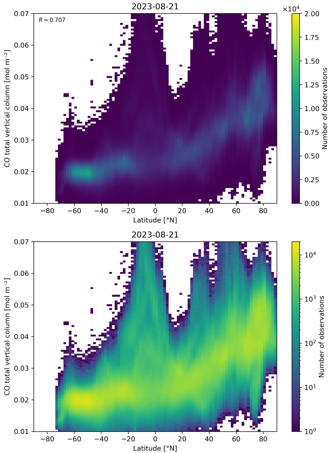
Figure 51: Scatter density plot of “Latitude” against “CO total vertical column” for 2023-08-20 to 2023-08-22.
