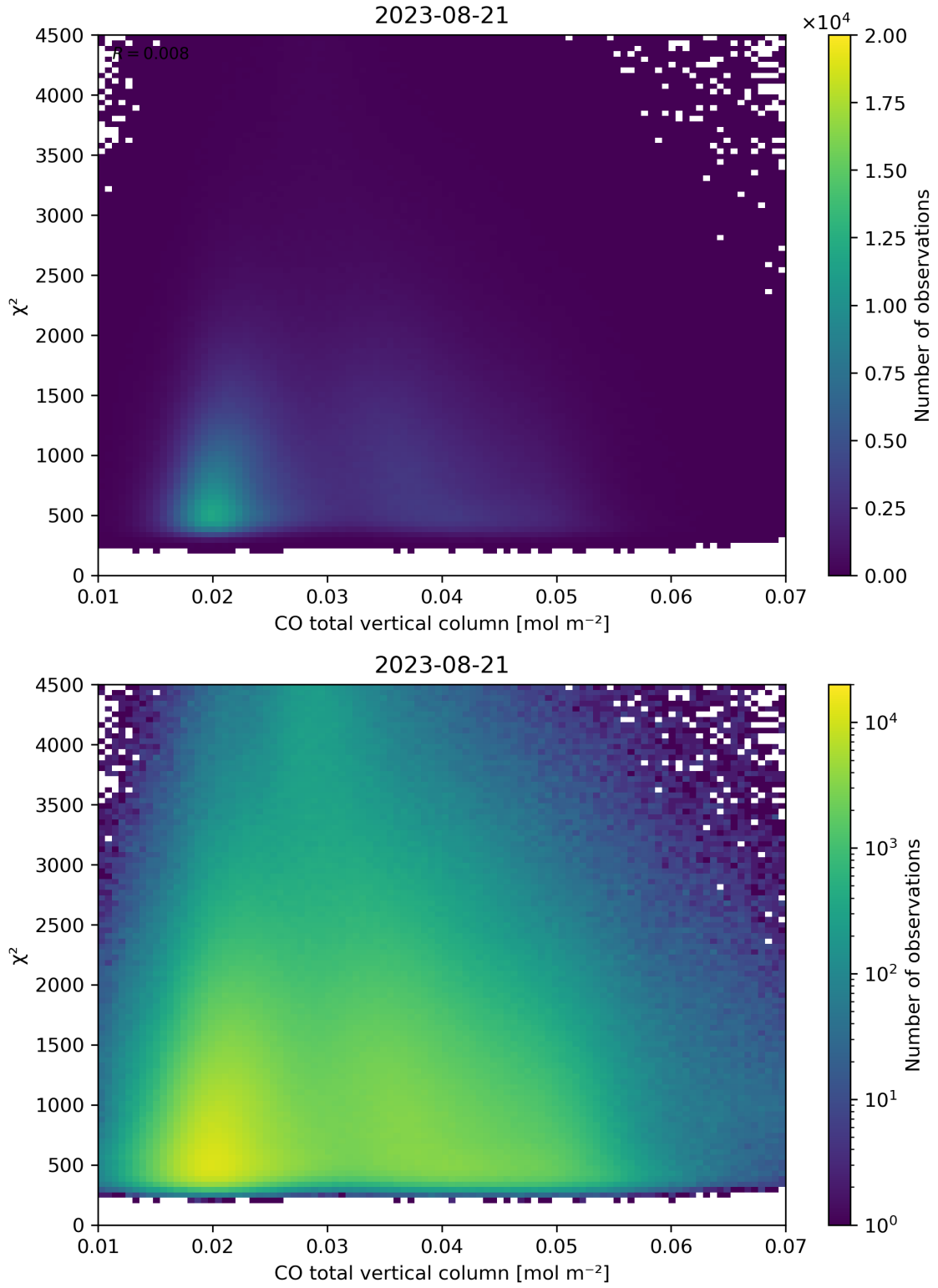
Figure 35: Scatter density plot of “CO total vertical column” against “ \chi^2 ” for 2023-08-20 to 2023-08-22.
