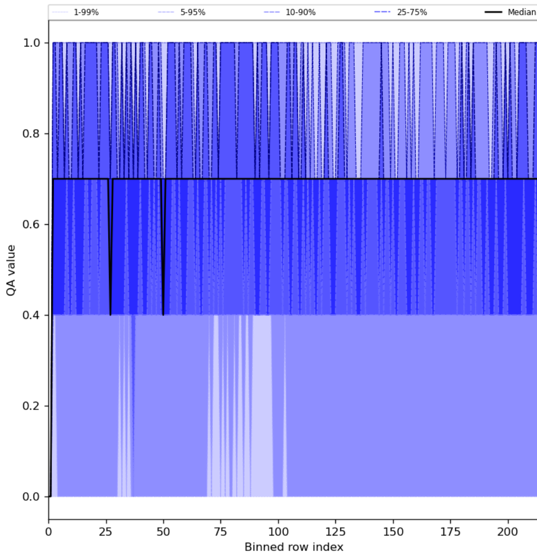
Figure 25: Along track statistics of “QA value” for 2023-08-20 to 2023-08-22
