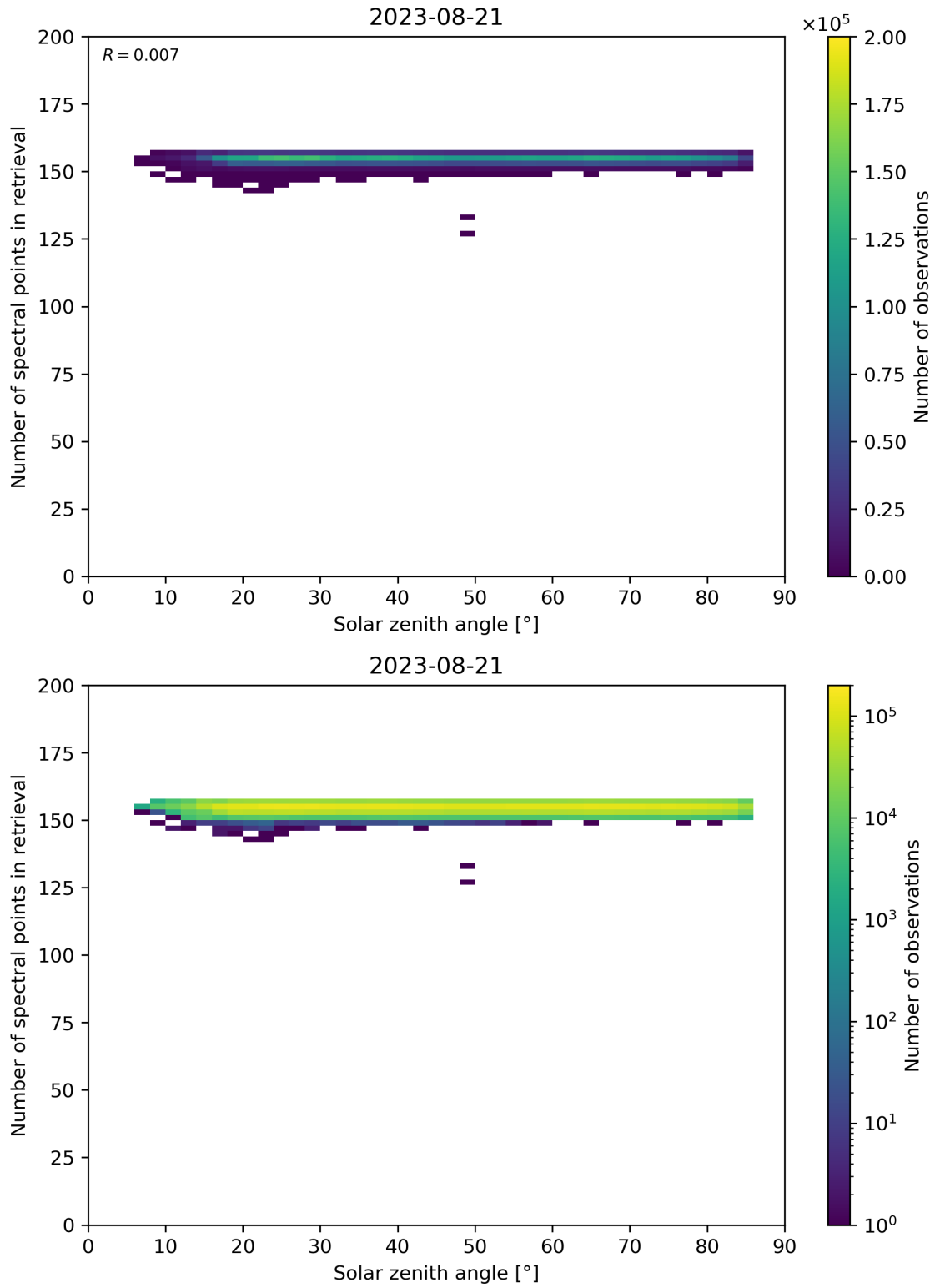
Figure 68: Scatter density plot of “Solar zenith angle” against “Number of spectral points in retrieval” for 2023-08-20 to 2023-08-22.
