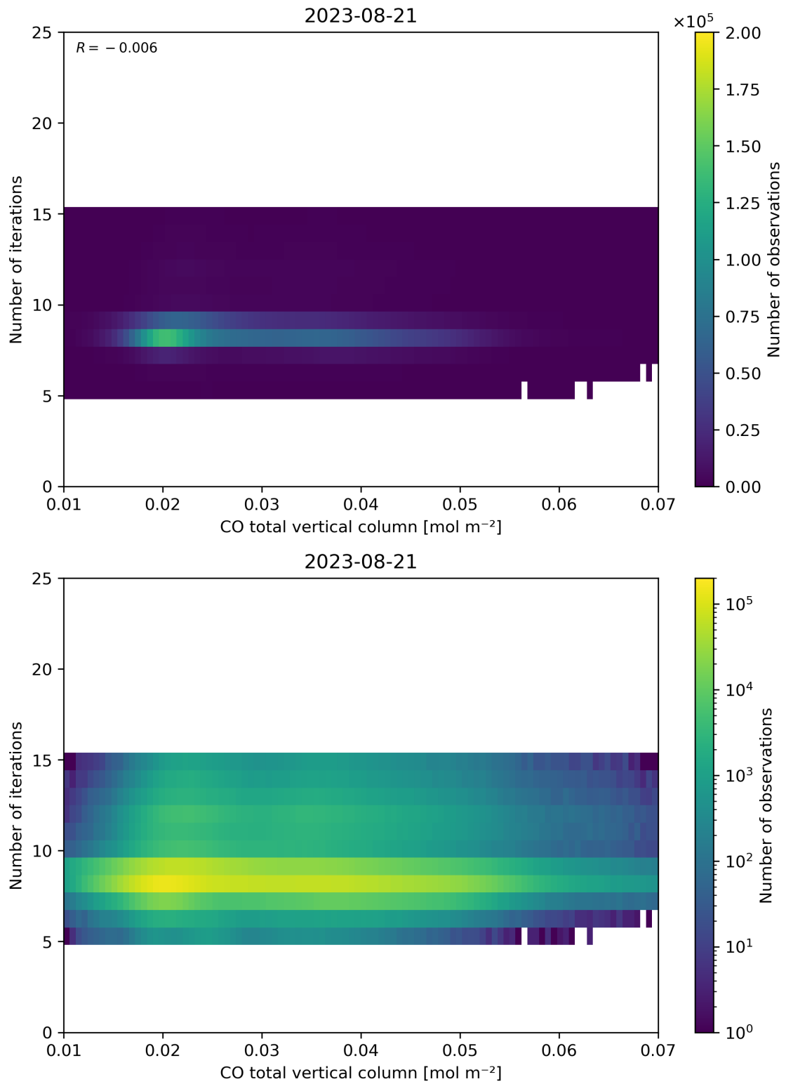
Figure 42: Scatter density plot of “CO total vertical column” against “Number of iterations” for 2023-08-20 to 2023-08-22.
