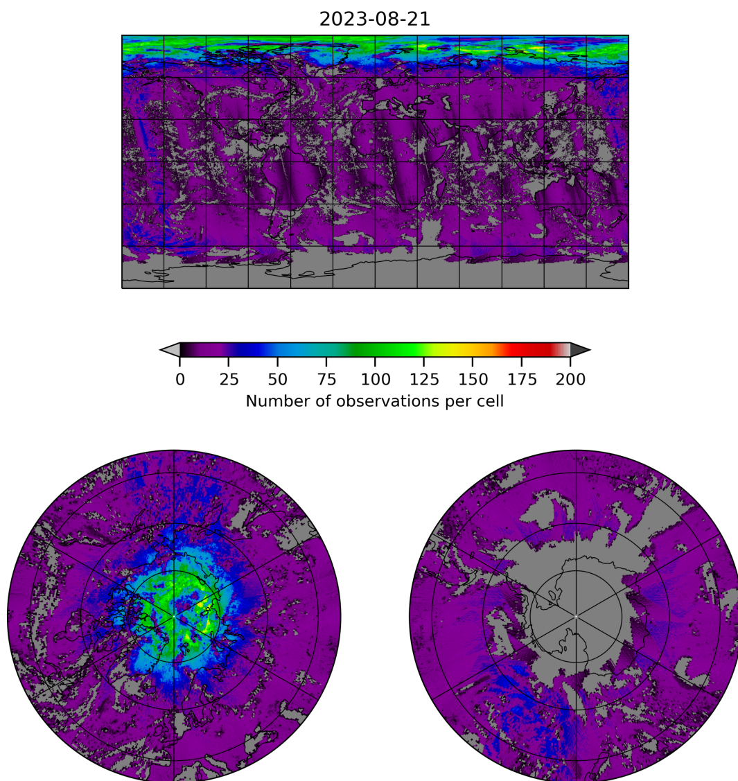
Figure 8: Map of the number of observations for 2023-08-20 to 2023-08-22
