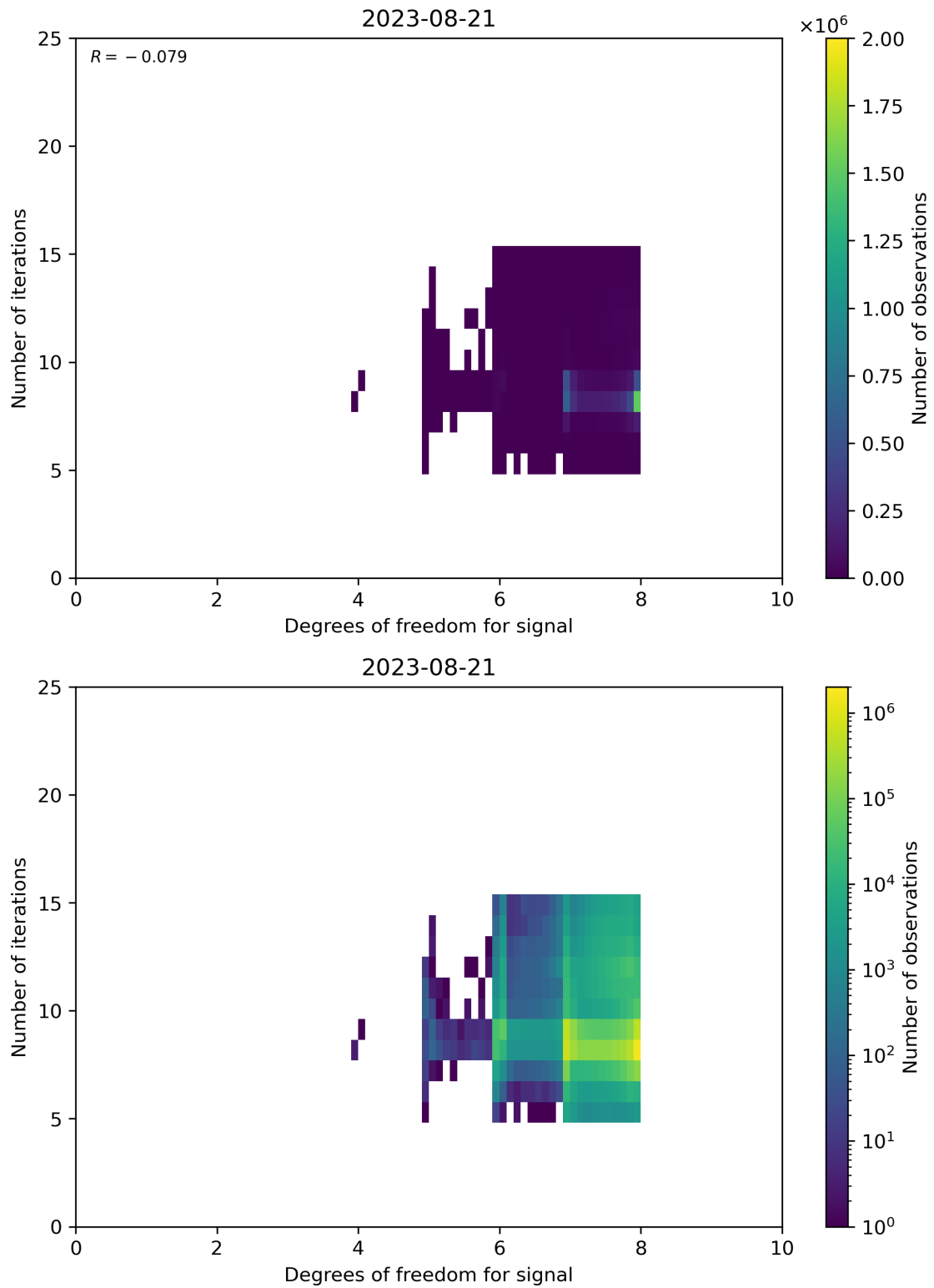
Figure 50: Scatter density plot of “Degrees of freedom for signal” against “Number of iterations” for 2023-08-20 to 2023-08-22.
