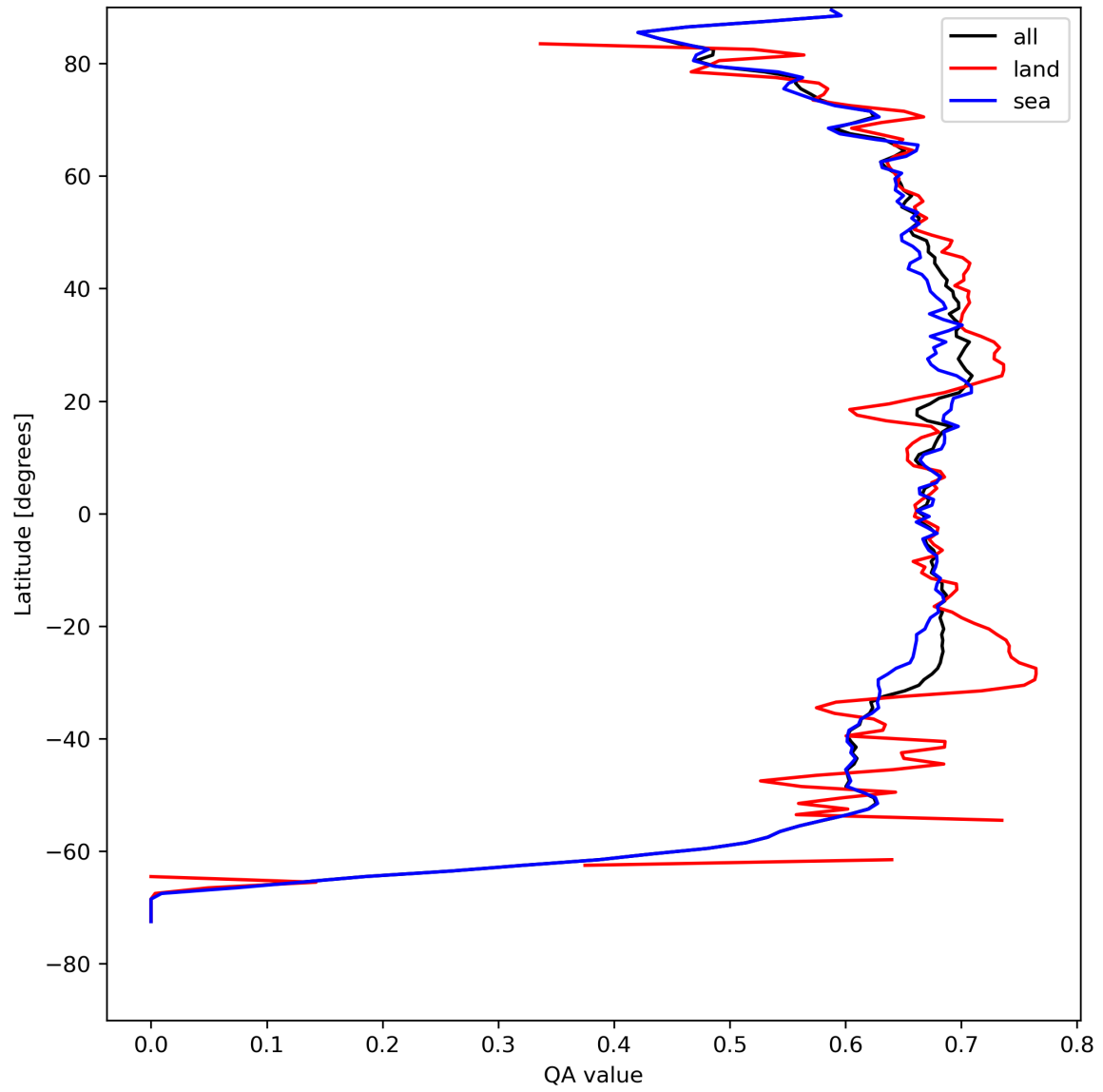
Figure 9: Zonal average of “QA value” for 2023-08-20 to 2023-08-22.
