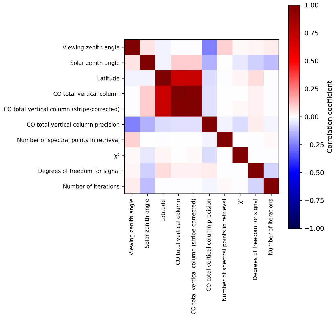
Figure 2: Map of correlation matrix for 2023-08-20 to 2023-08-22.
