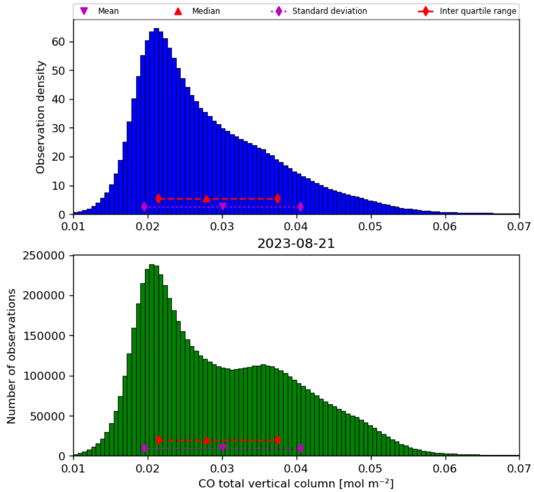
Figure 18: Histogram of “CO total vertical column” for 2023-08-20 to 2023-08-22
