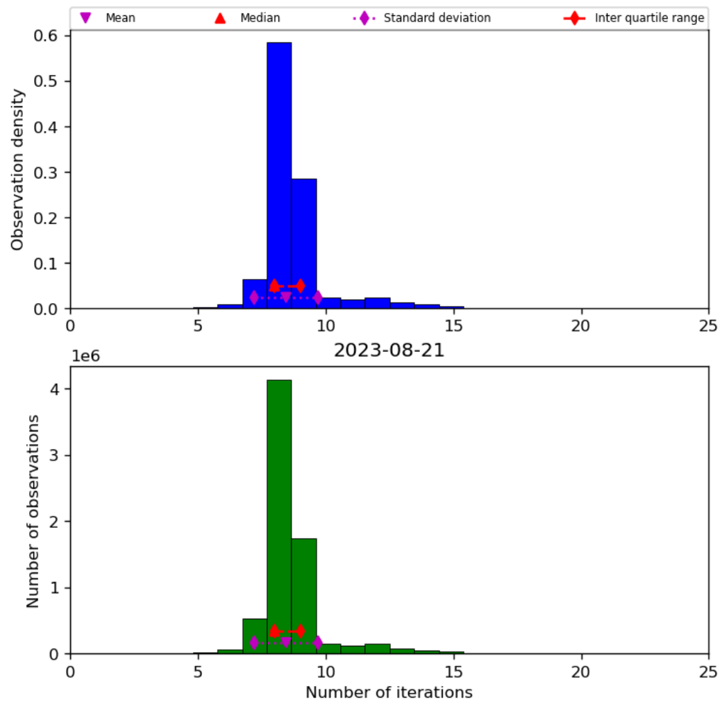
Figure 24: Histogram of “Number of iterations” for 2023-08-20 to 2023-08-22
