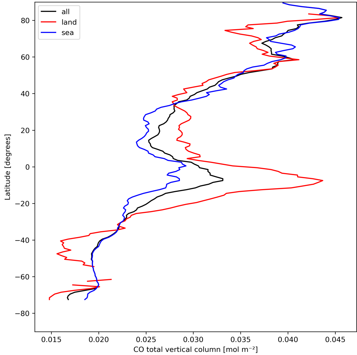
Figure 10: Zonal average of “CO total vertical column” for 2023-08-20 to 2023-08-22.
