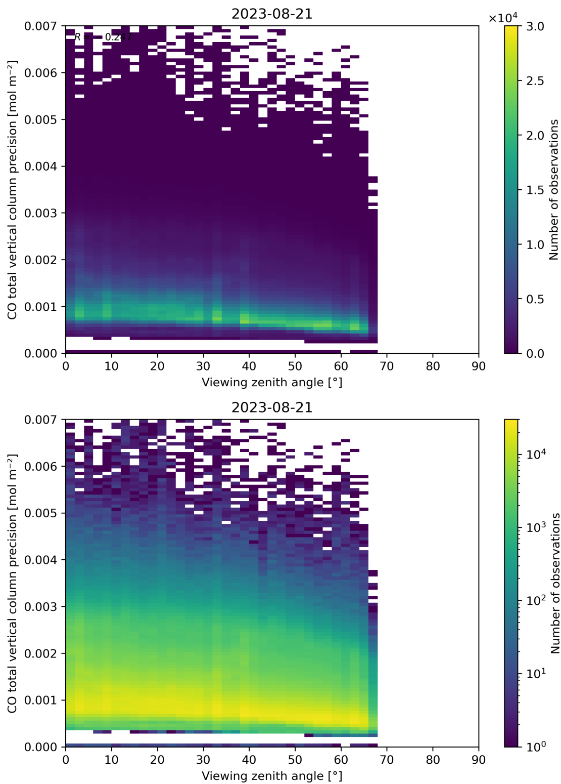
Figure 71: Scatter density plot of “Viewing zenith angle” against “CO total vertical column precision” for 2023-08-20 to 2023-08-22.
