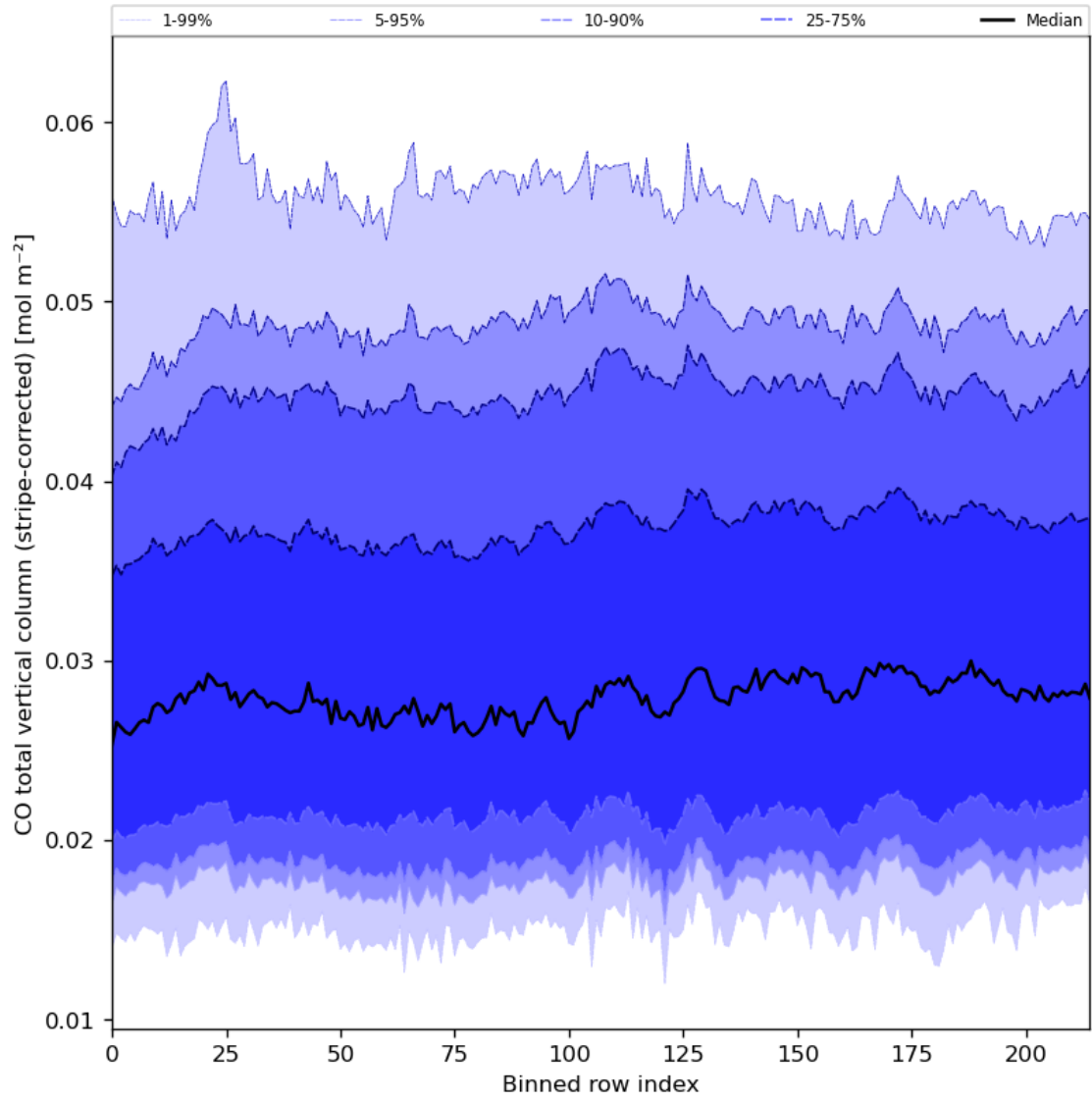
Figure 27: Along track statistics of “CO total vertical column (stripe-corrected)” for 2023-08-20 to 2023-08-22
