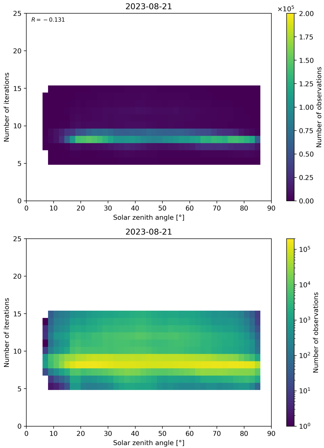
Figure 67: Scatter density plot of “Solar zenith angle” against “Number of iterations” for 2023-08-20 to 2023-08-22.
