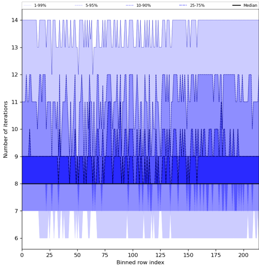
Figure 32: Along track statistics of “Number of iterations” for 2023-08-20 to 2023-08-22
