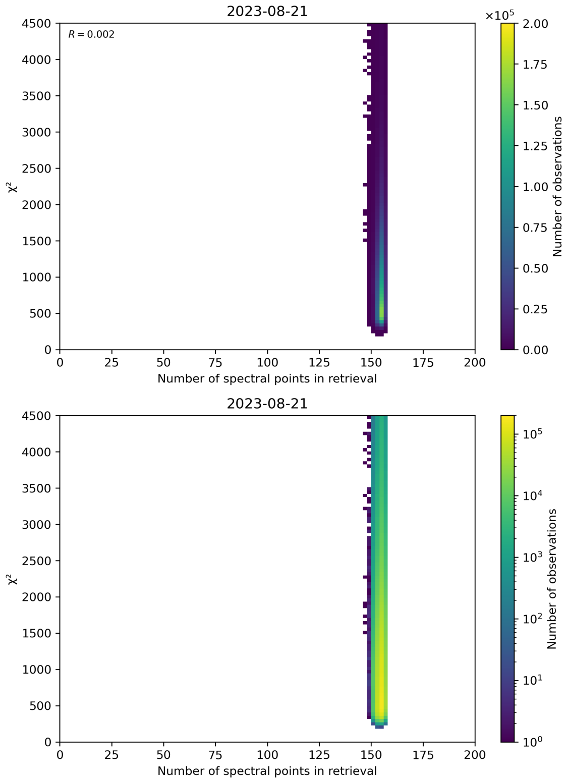
Figure 58: Scatter density plot of “Number of spectral points in retrieval” against “ \chi^2 ” for 2023-08-20 to 2023-08-22.
