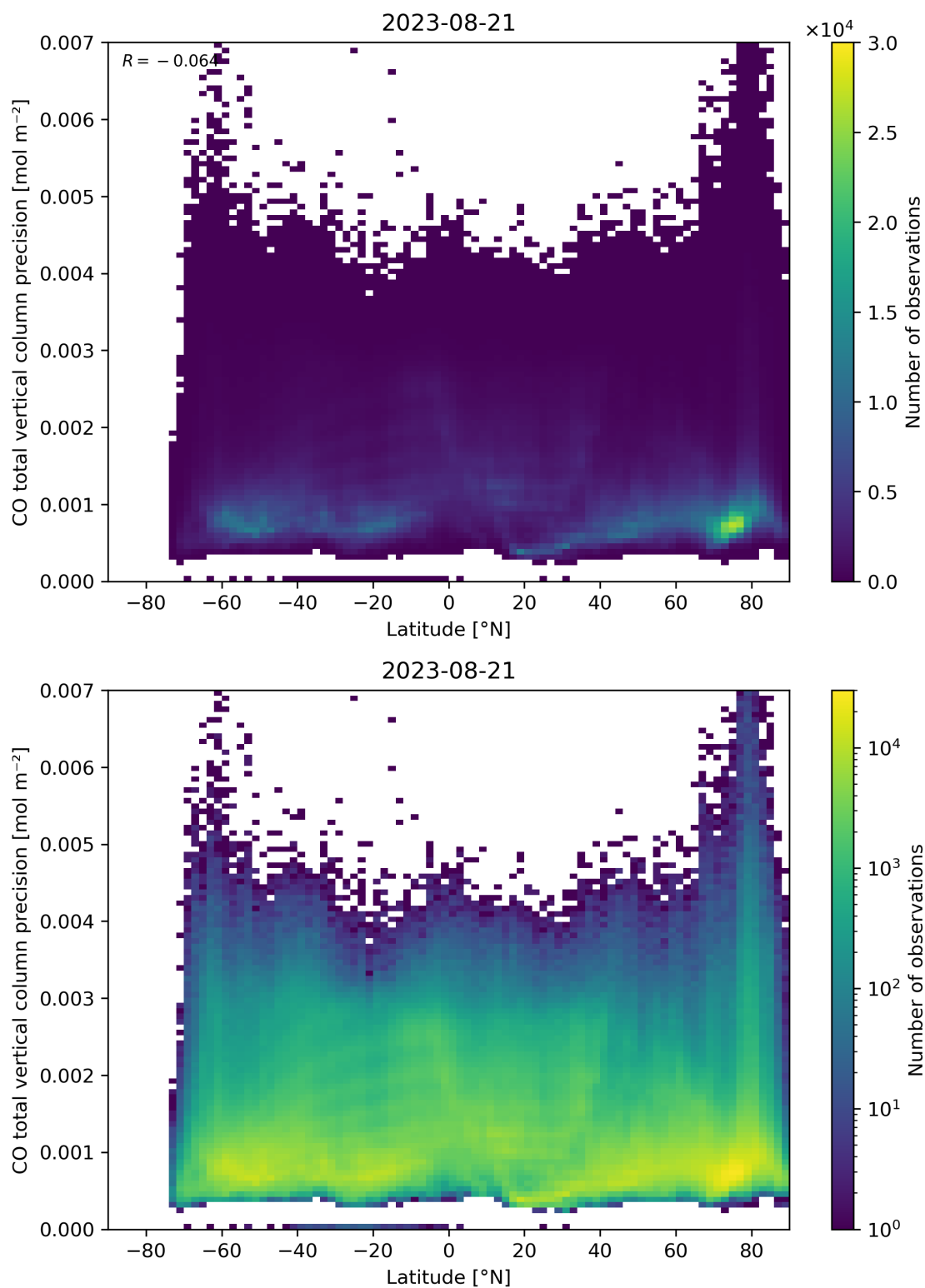
Figure 53: Scatter density plot of “Latitude” against “CO total vertical column precision” for 2023-08-20 to 2023-08-22.
