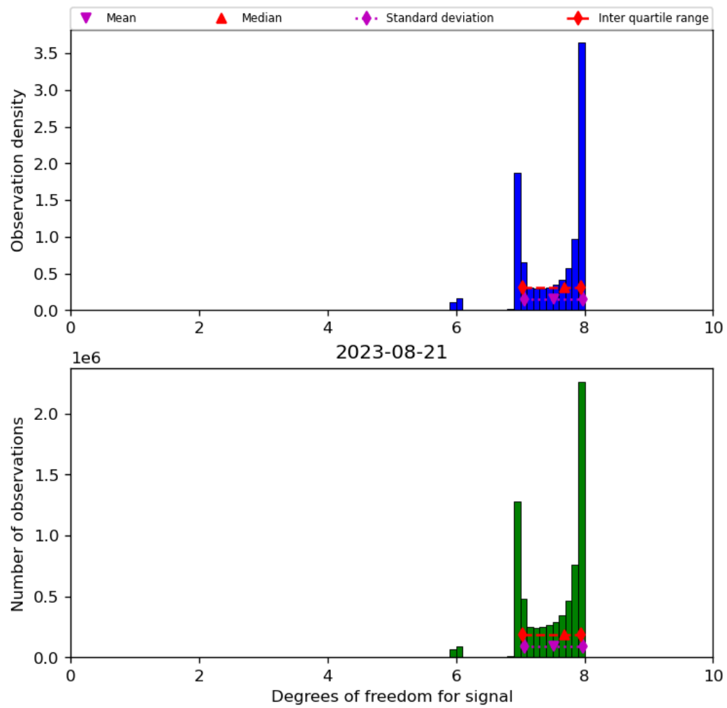
Figure 23: Histogram of “Degrees of freedom for signal” for 2023-08-20 to 2023-08-22
