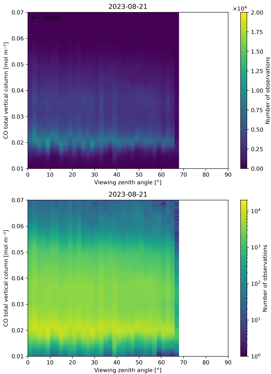
Figure 69: Scatter density plot of “Viewing zenith angle” against “CO total vertical column” for 2023-08-20 to 2023-08-22.
