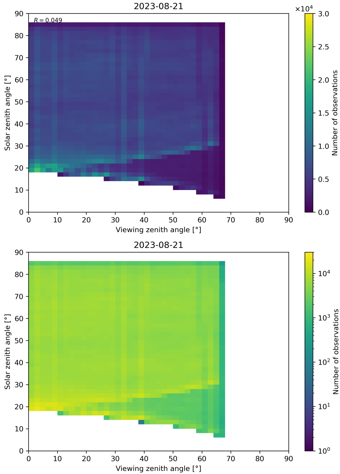
Figure 77: Scatter density plot of “Viewing zenith angle” against “Solar zenith angle” for 2023-08-20 to 2023-08-22.
