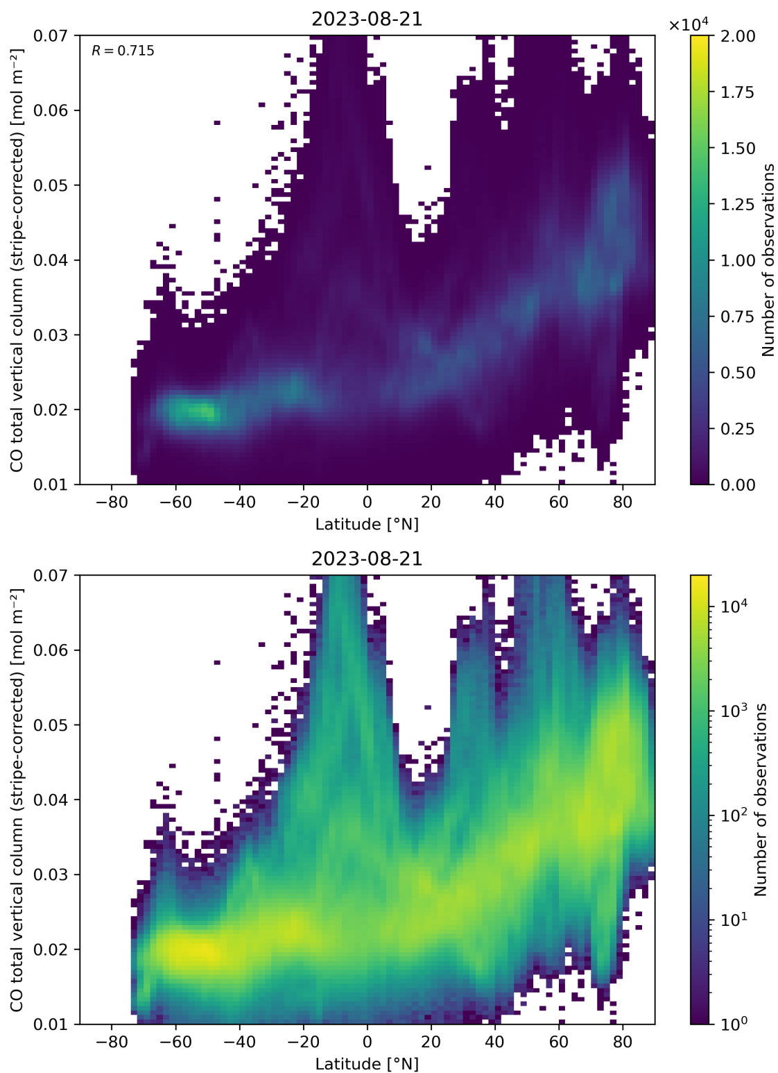
Figure 52: Scatter density plot of “Latitude” against “CO total vertical column (stripe-corrected)” for 2023-08-20 to 2023-08-22.
