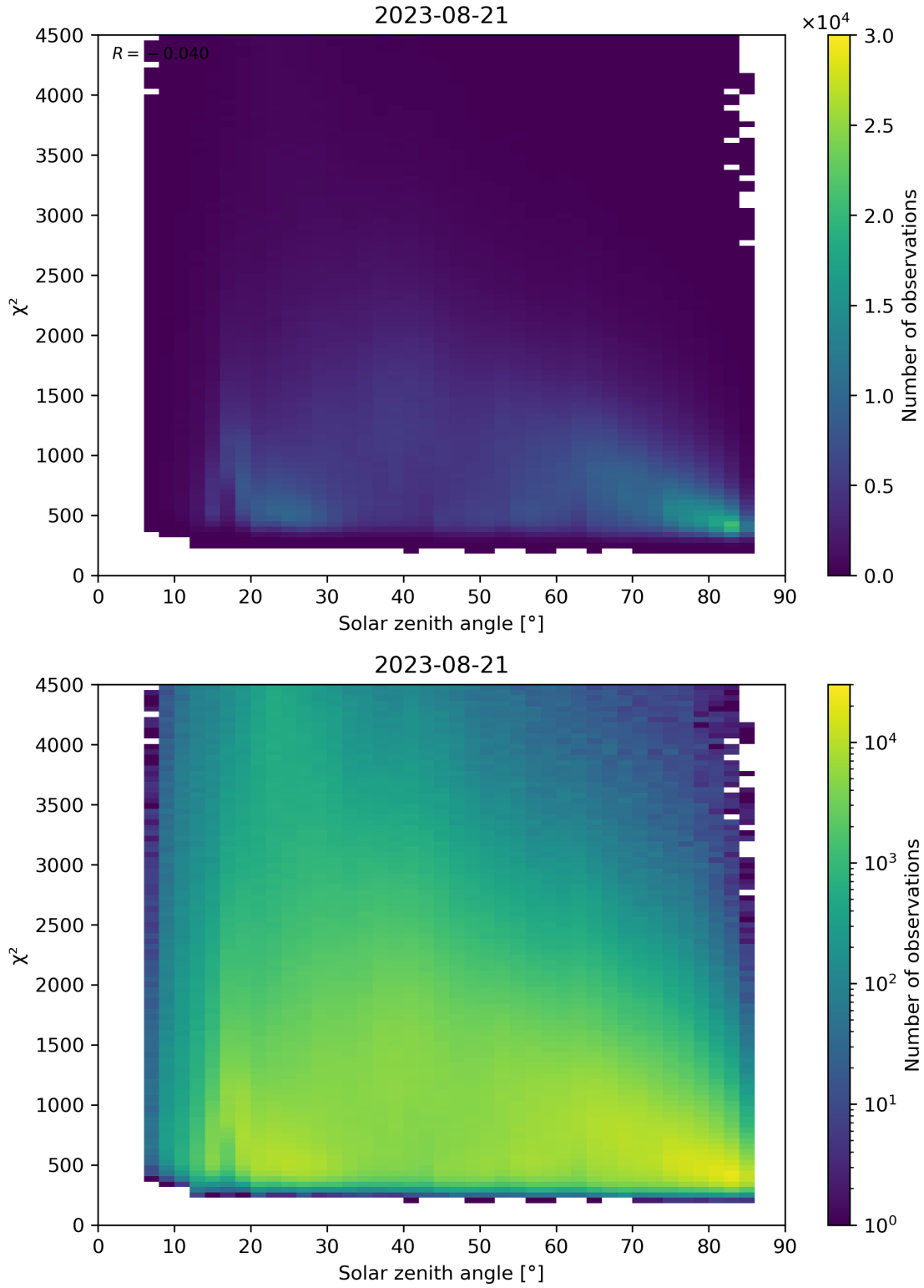
Figure 64: Scatter density plot of “Solar zenith angle” against “ \chi^2 ” for 2023-08-20 to 2023-08-22.
