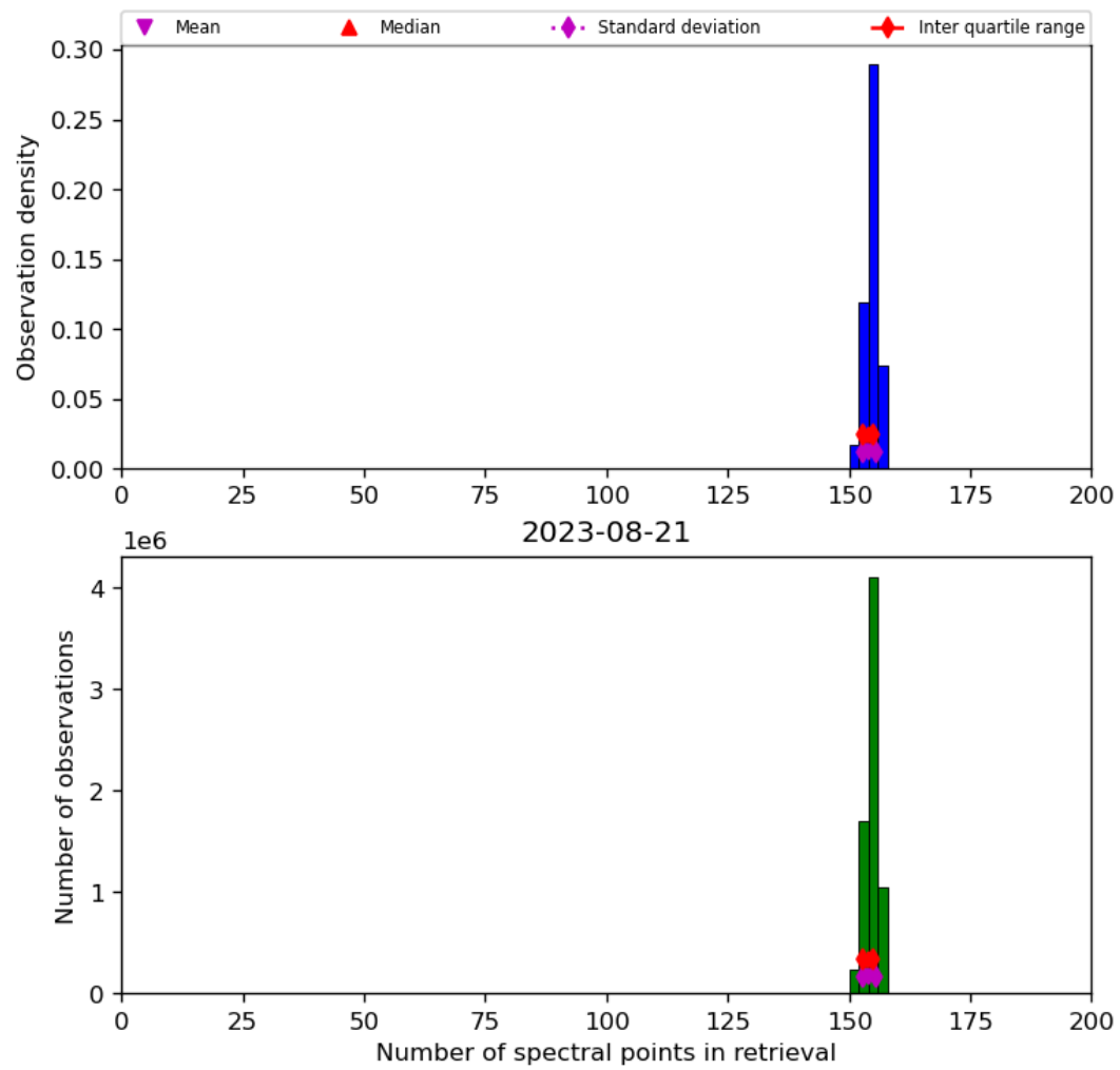
Figure 21: Histogram of “Number of spectral points in retrieval” for 2023-08-20 to 2023-08-22
