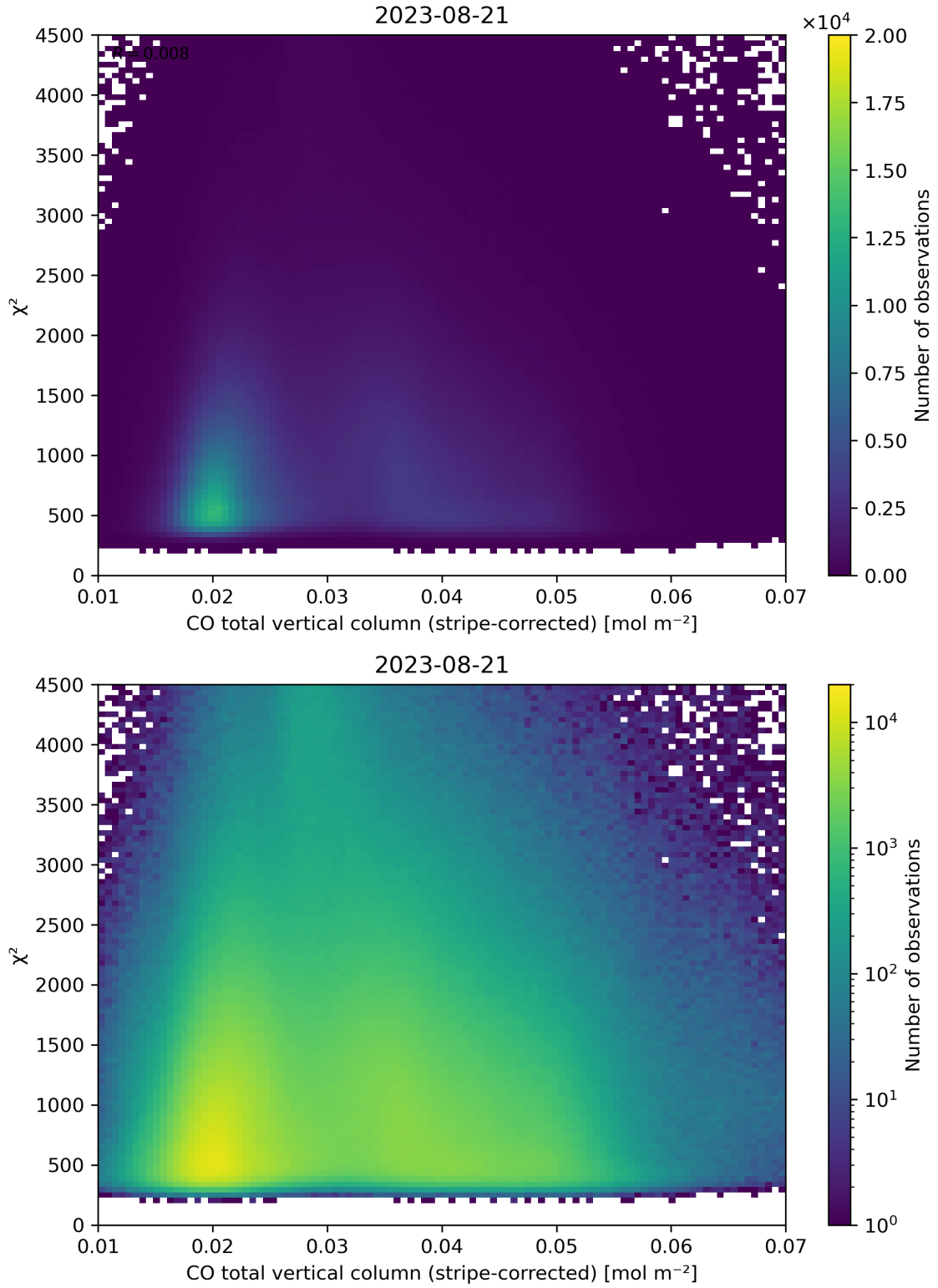
Figure 37: Scatter density plot of “CO total vertical column (stripe-corrected)” against “ \chi^2 ” for 2023-08-20 to 2023-08-22.
