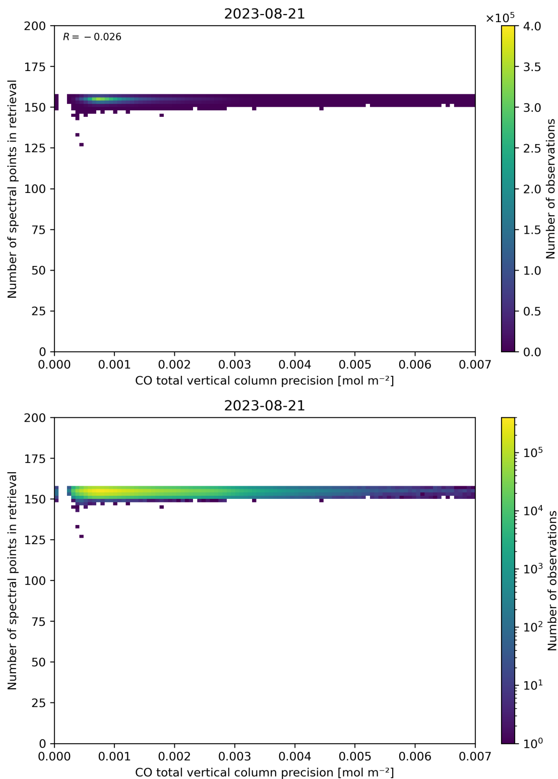
Figure 47: Scatter density plot of “CO total vertical column precision” against “Number of spectral points in retrieval” for 2023-08-20 to 2023-08-22.
