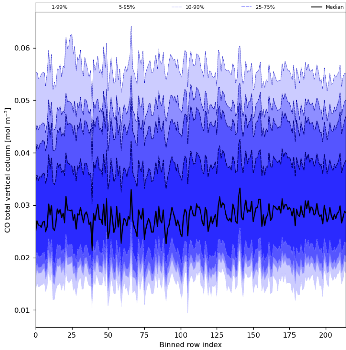
Figure 26: Along track statistics of “CO total vertical column” for 2023-08-20 to 2023-08-22
