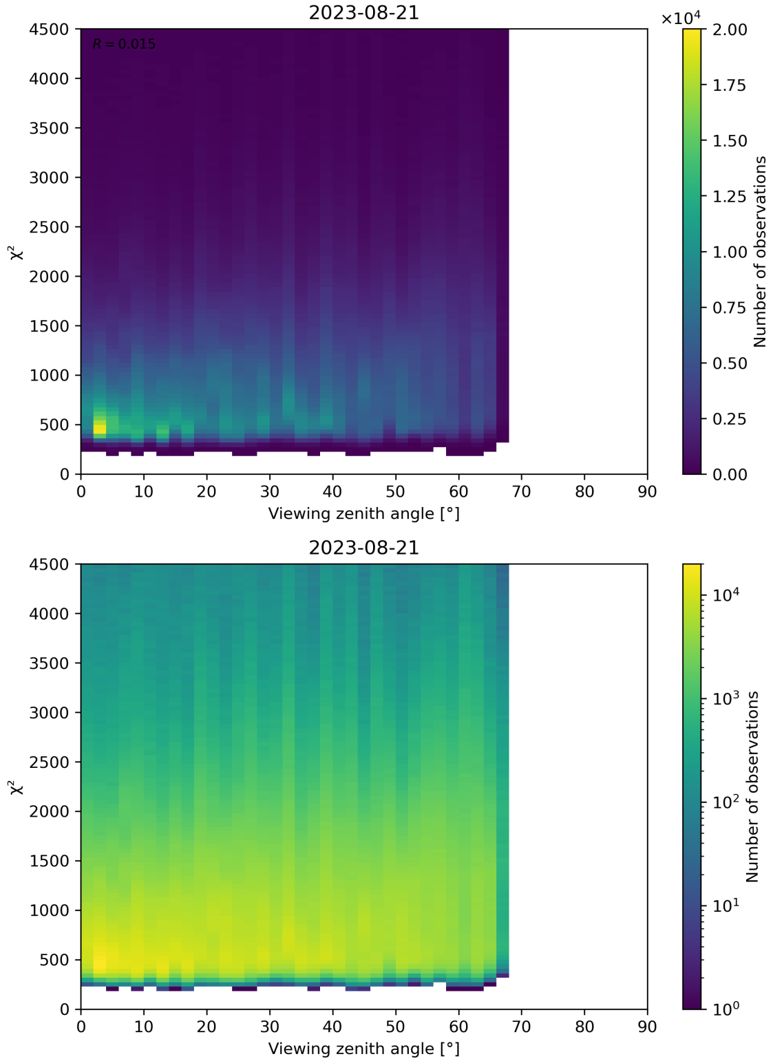
Figure 72: Scatter density plot of “Viewing zenith angle” against “ \chi^2 ” for 2023-08-20 to 2023-08-22.
