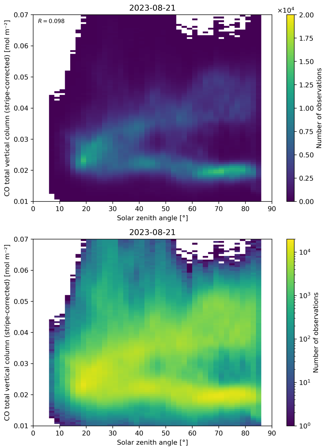
Figure 62: Scatter density plot of “Solar zenith angle” against “CO total vertical column (stripe-corrected)” for 2023-08-20 to 2023-08-22.
