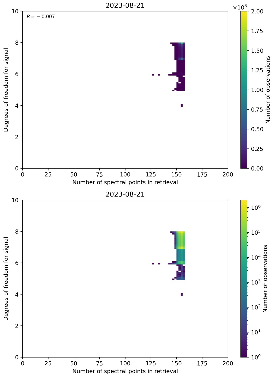
Figure 59: Scatter density plot of “Number of spectral points in retrieval” against “Degrees of freedom for signal” for 2023-08-20 to 2023-08-22.
