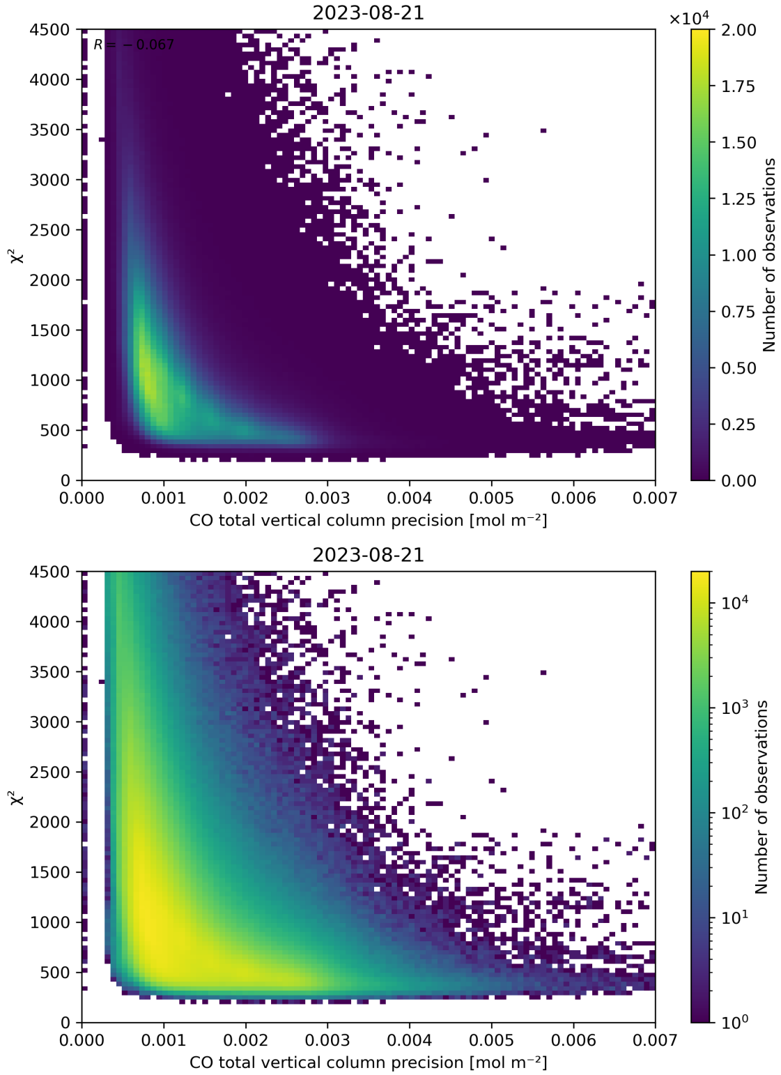
Figure 44: Scatter density plot of “CO total vertical column precision” against “ \chi^2 ” for 2023-08-20 to 2023-08-22.
