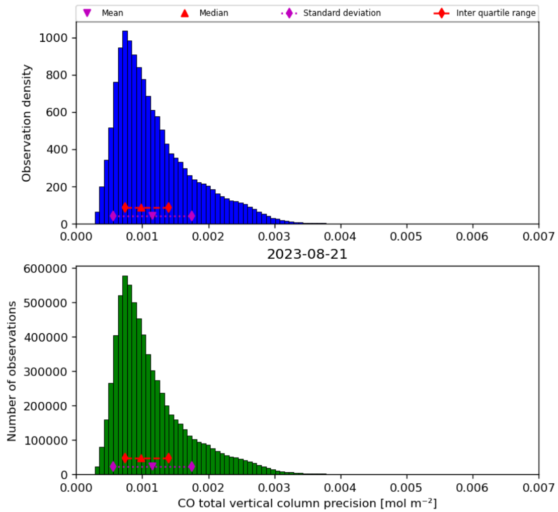
Figure 20: Histogram of “CO total vertical column precision” for 2023-08-20 to 2023-08-22
