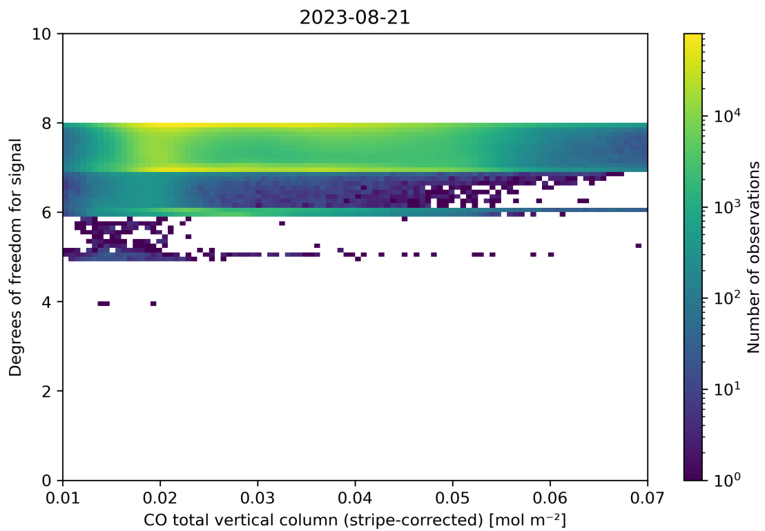
Figure 38: Scatter density plot of “CO total vertical column (stripe-corrected)” against “Degrees of freedom for signal” for 2023-08-20 to 2023-08-22.
