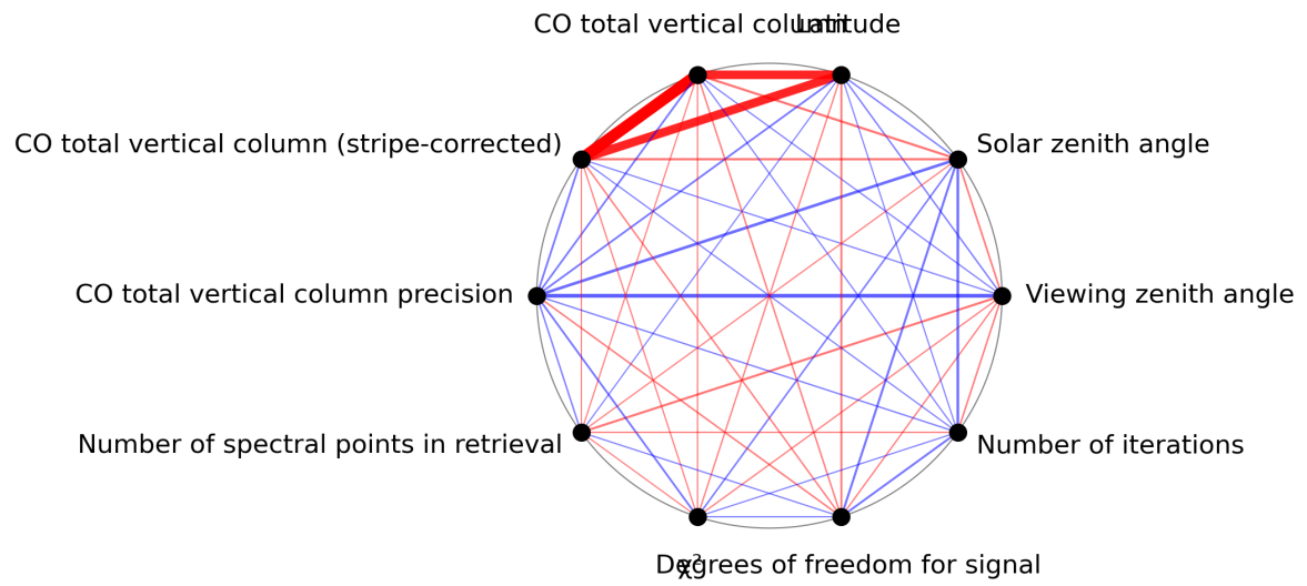
Figure 1: Map of correlation graph for 2023-08-20 to 2023-08-22.
