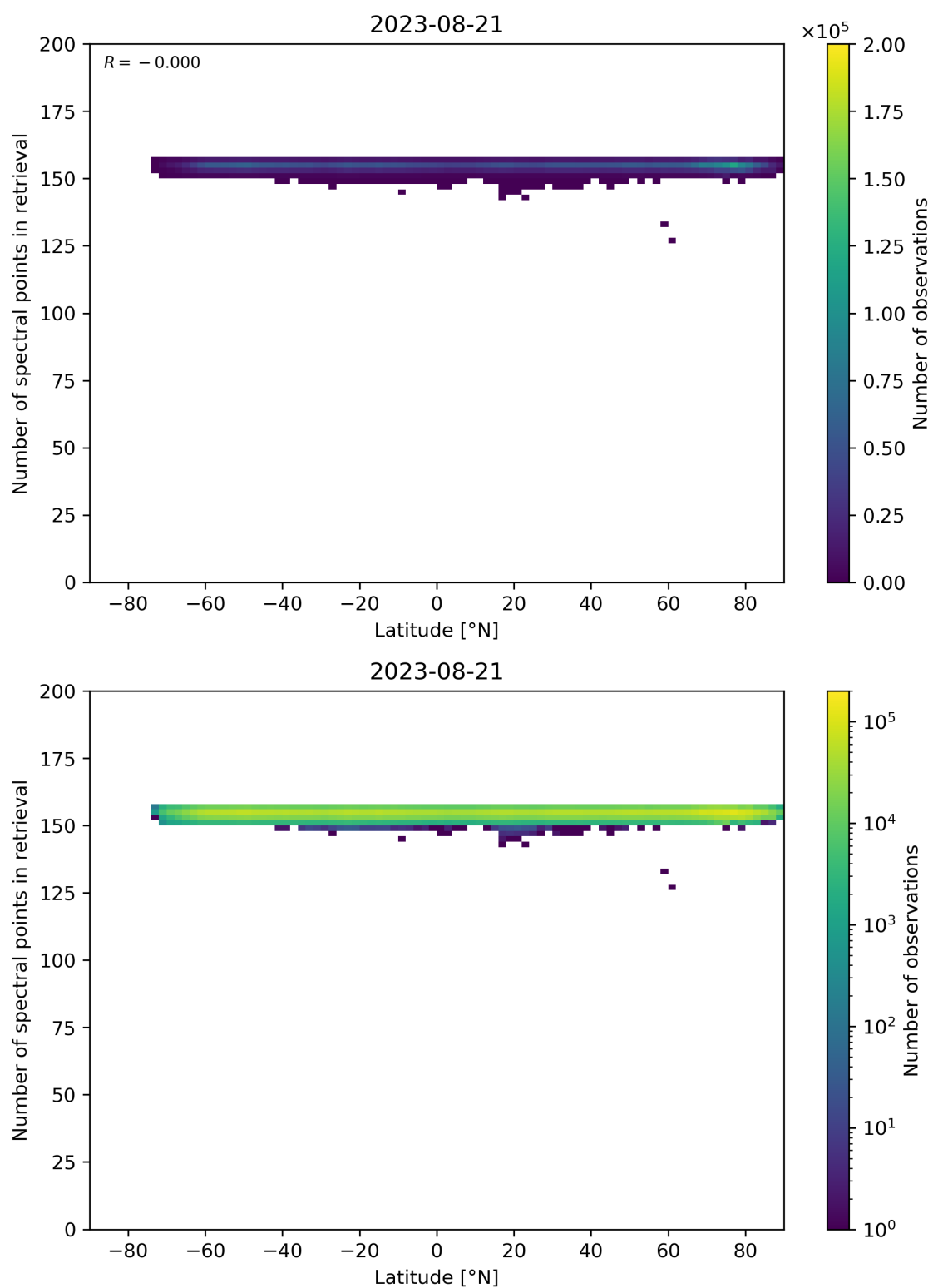
Figure 57: Scatter density plot of “Latitude” against “Number of spectral points in retrieval” for 2023-08-20 to 2023-08-22.
