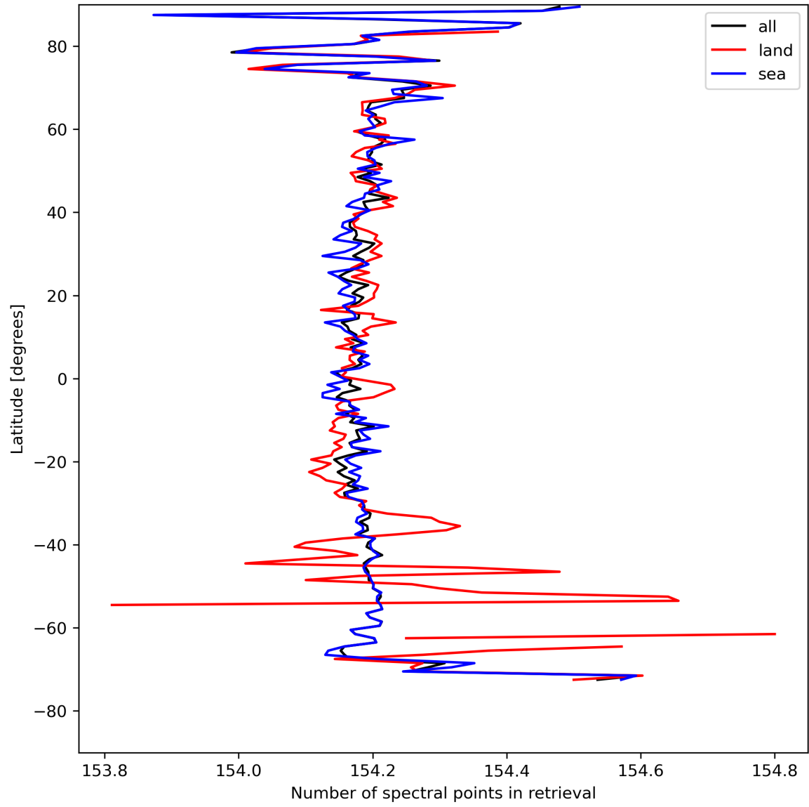
Figure 13: Zonal average of “Number of spectral points in retrieval” for 2023-08-20 to 2023-08-22.
