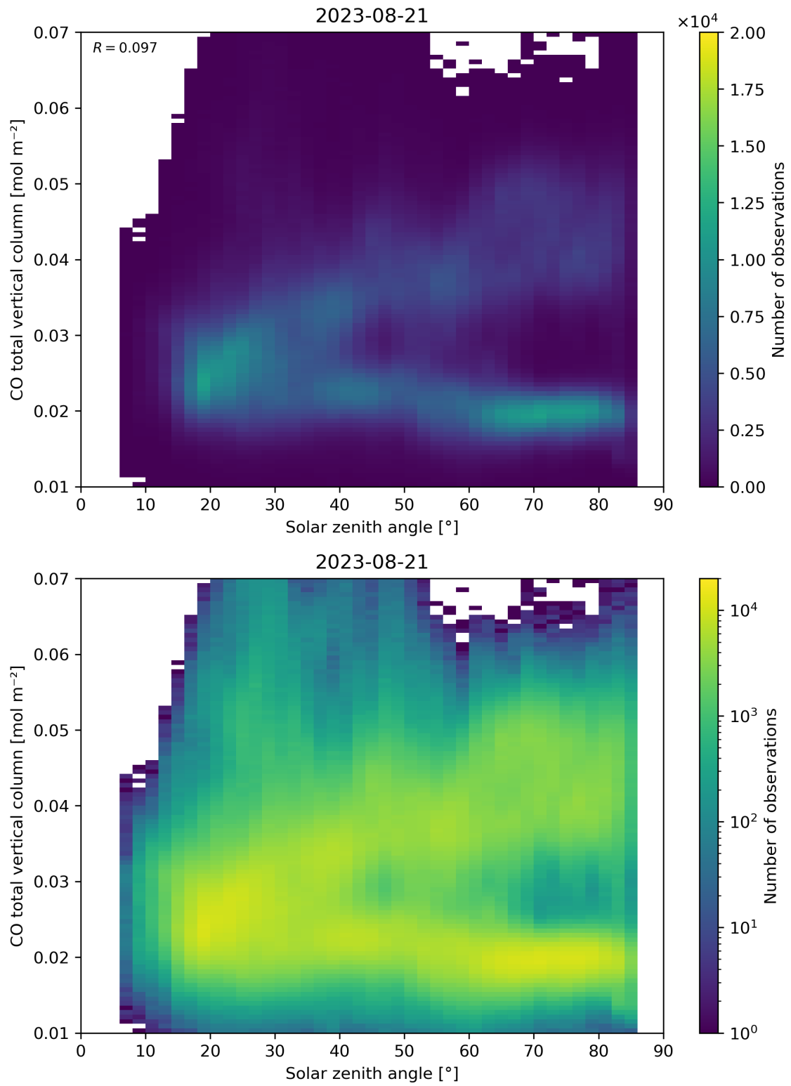
Figure 61: Scatter density plot of “Solar zenith angle” against “CO total vertical column” for 2023-08-20 to 2023-08-22.
