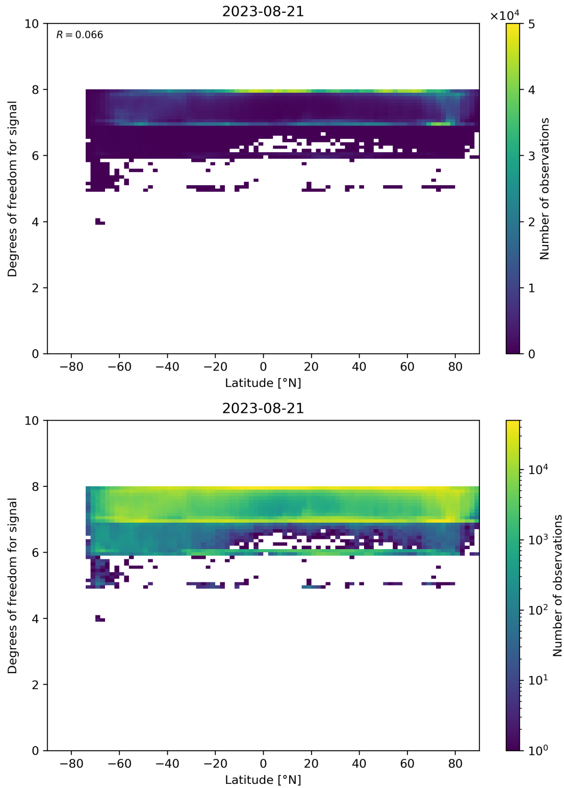
Figure 55: Scatter density plot of “Latitude” against “Degrees of freedom for signal” for 2023-08-20 to 2023-08-22.
