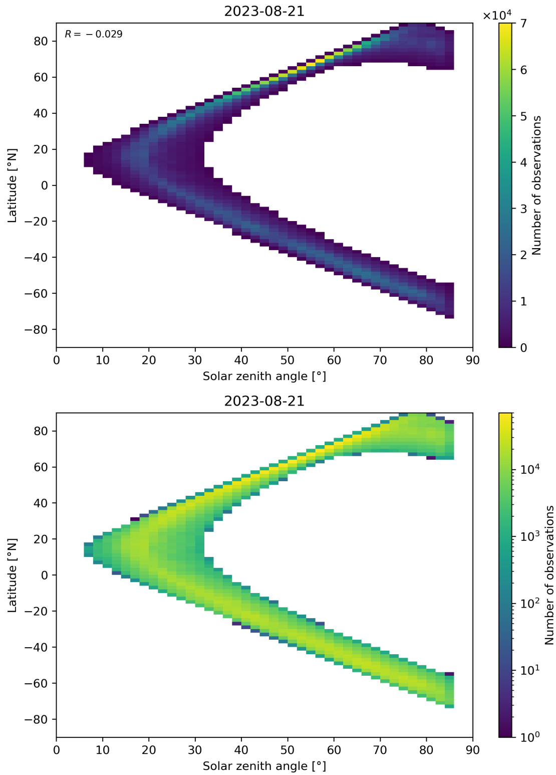
Figure 66: Scatter density plot of “Solar zenith angle” against “Latitude” for 2023-08-20 to 2023-08-22.
