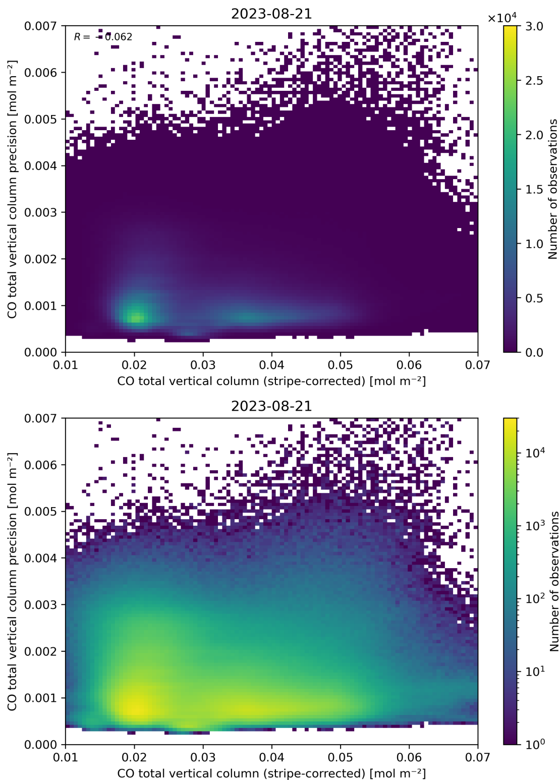
Figure 36: Scatter density plot of “CO total vertical column (stripe-corrected)” against “CO total vertical column precision” for 2023-08-20 to 2023-08-22.
