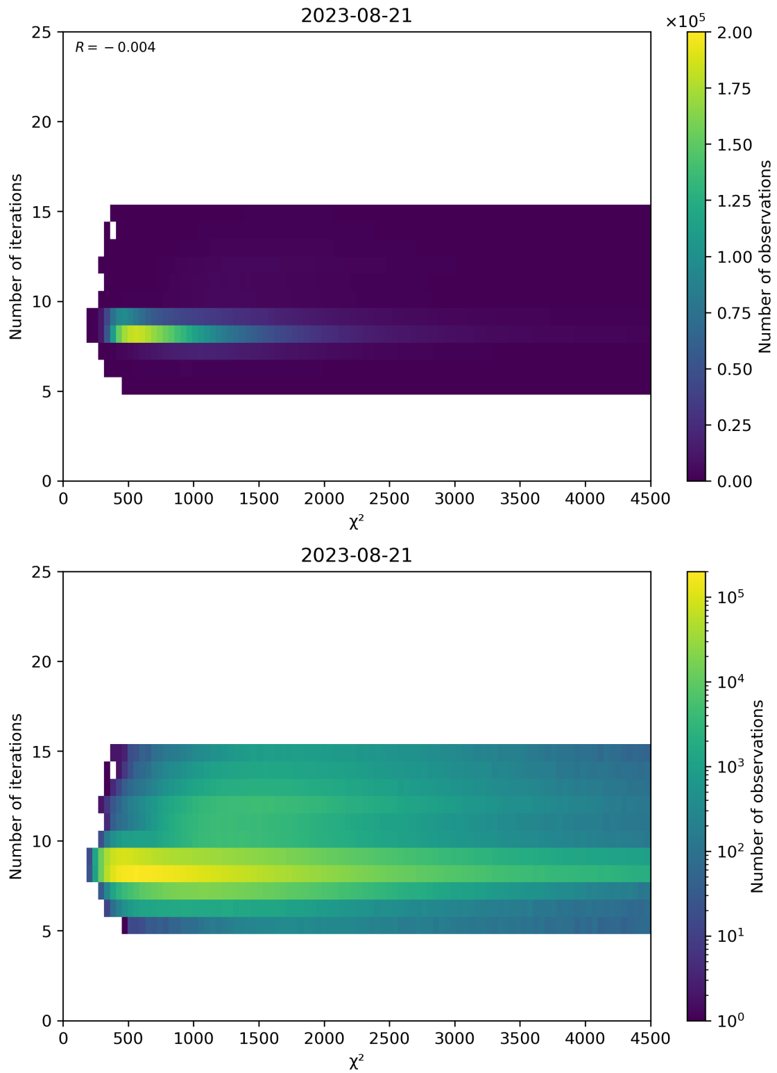
Figure 49: Scatter density plot of “ \chi^2 ” against “Number of iterations” for 2023-08-20 to 2023-08-22.
