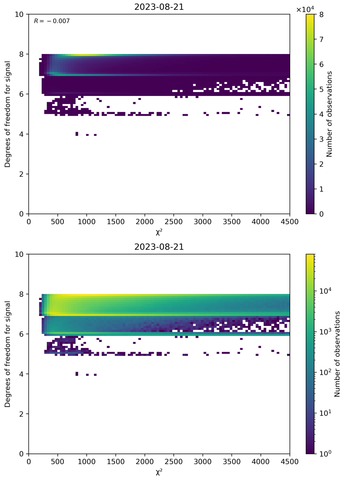
Figure 48: Scatter density plot of “ \chi^2 ” against “Degrees of freedom for signal” for 2023-08-20 to 2023-08-22.
