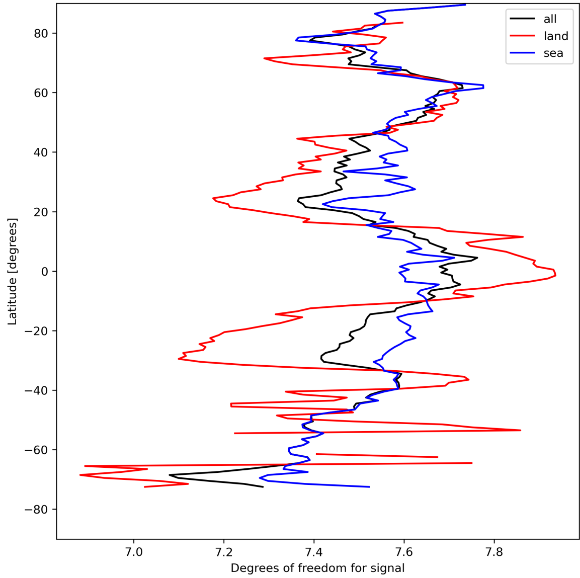
Figure 15: Zonal average of “Degrees of freedom for signal” for 2023-08-20 to 2023-08-22.
