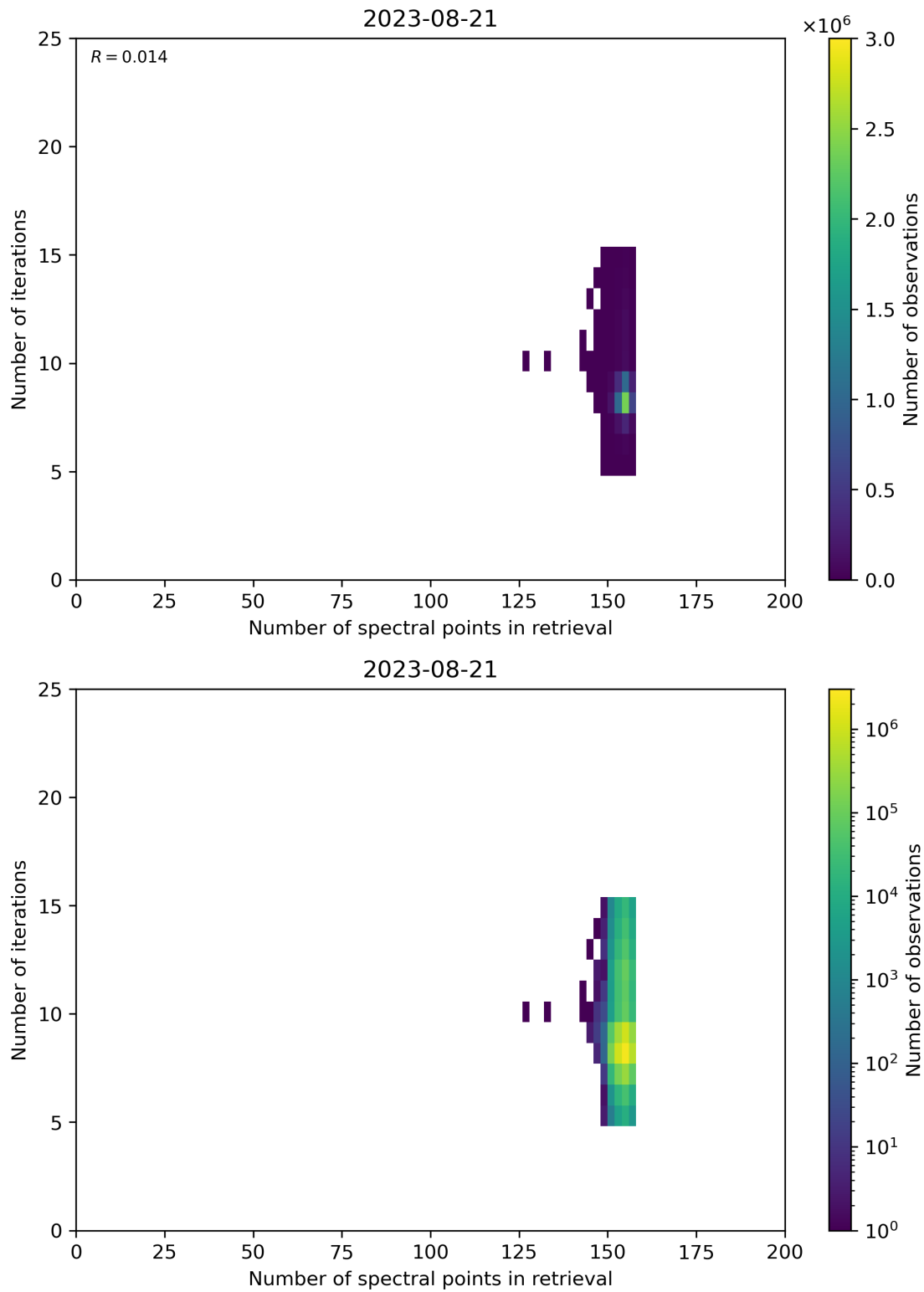
Figure 60: Scatter density plot of “Number of spectral points in retrieval” against “Number of iterations” for 2023-08-20 to 2023-08-22.
