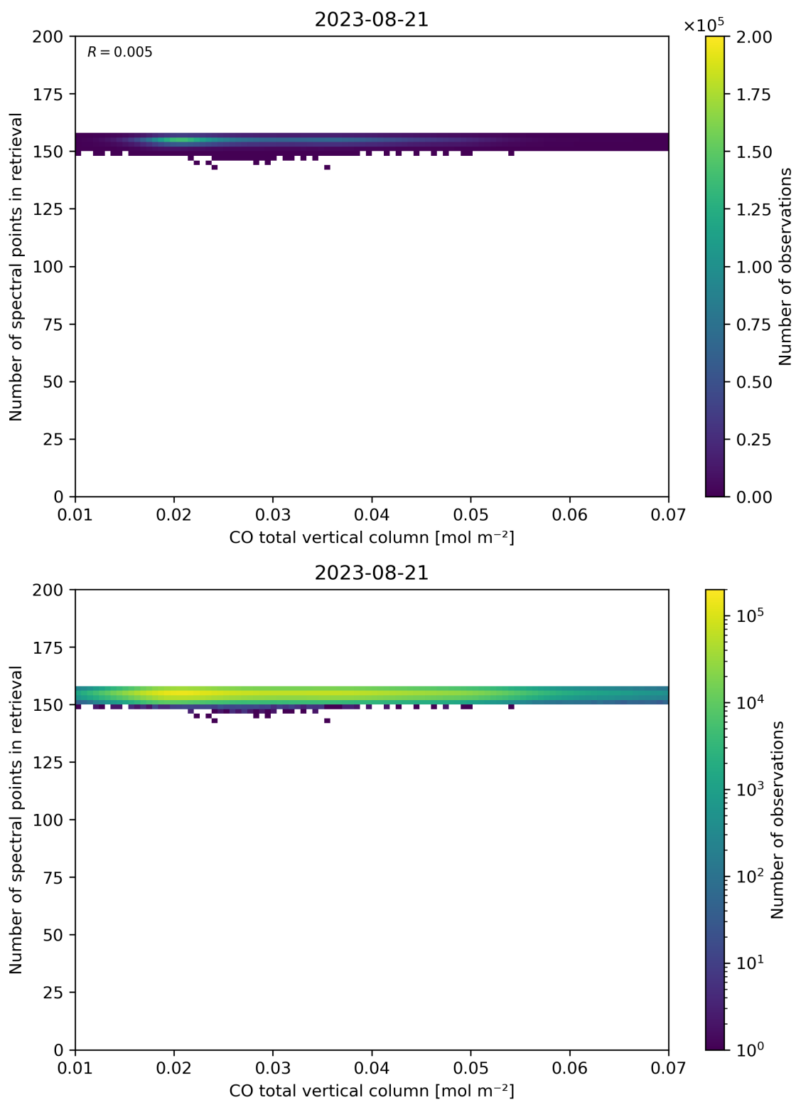
Figure 43: Scatter density plot of “CO total vertical column” against “Number of spectral points in retrieval” for 2023-08-20 to 2023-08-22.
