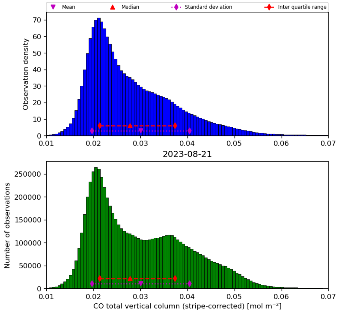
Figure 19: Histogram of “CO total vertical column (stripe-corrected)” for 2023-08-20 to 2023-08-22
