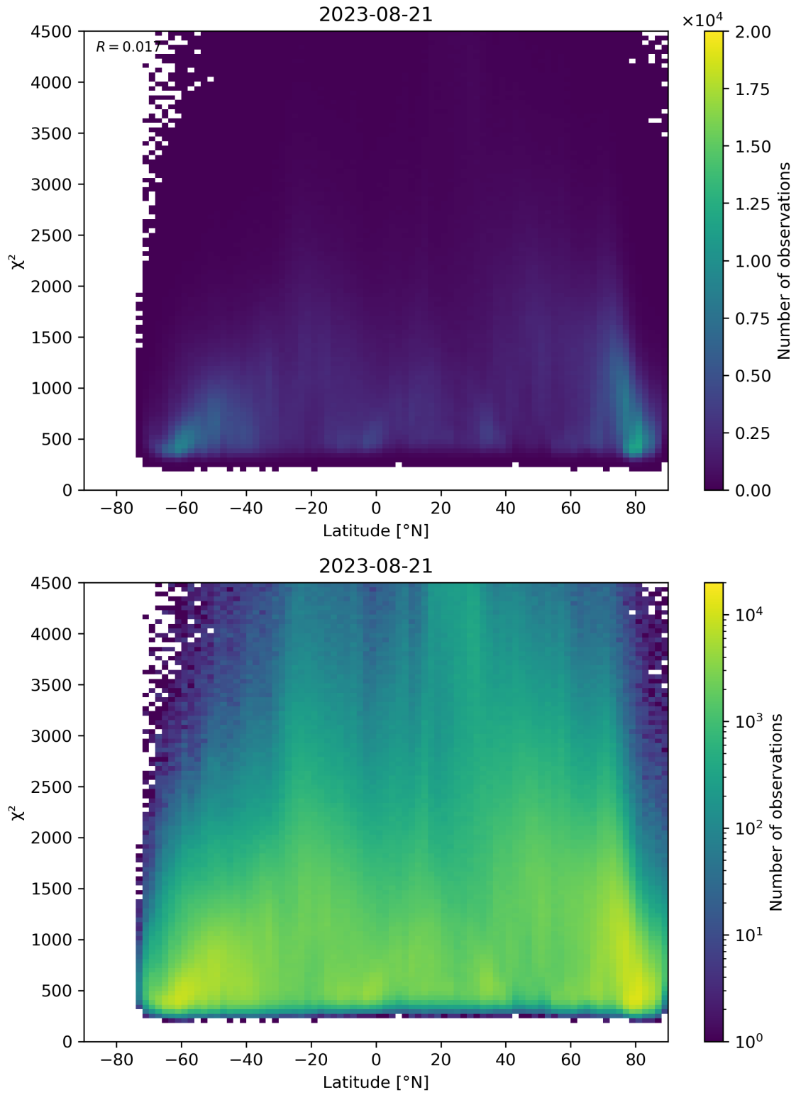
Figure 54: Scatter density plot of “Latitude” against “ \chi^2 ” for 2023-08-20 to 2023-08-22.
