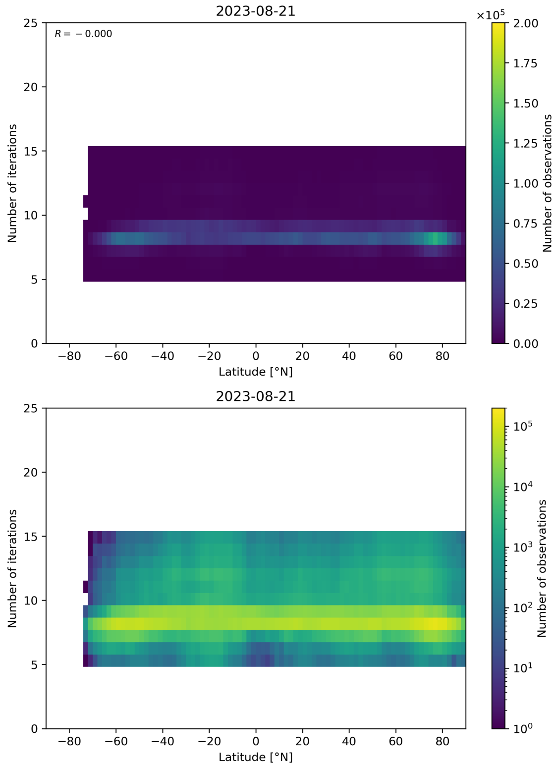
Figure 56: Scatter density plot of “Latitude” against “Number of iterations” for 2023-08-20 to 2023-08-22.
