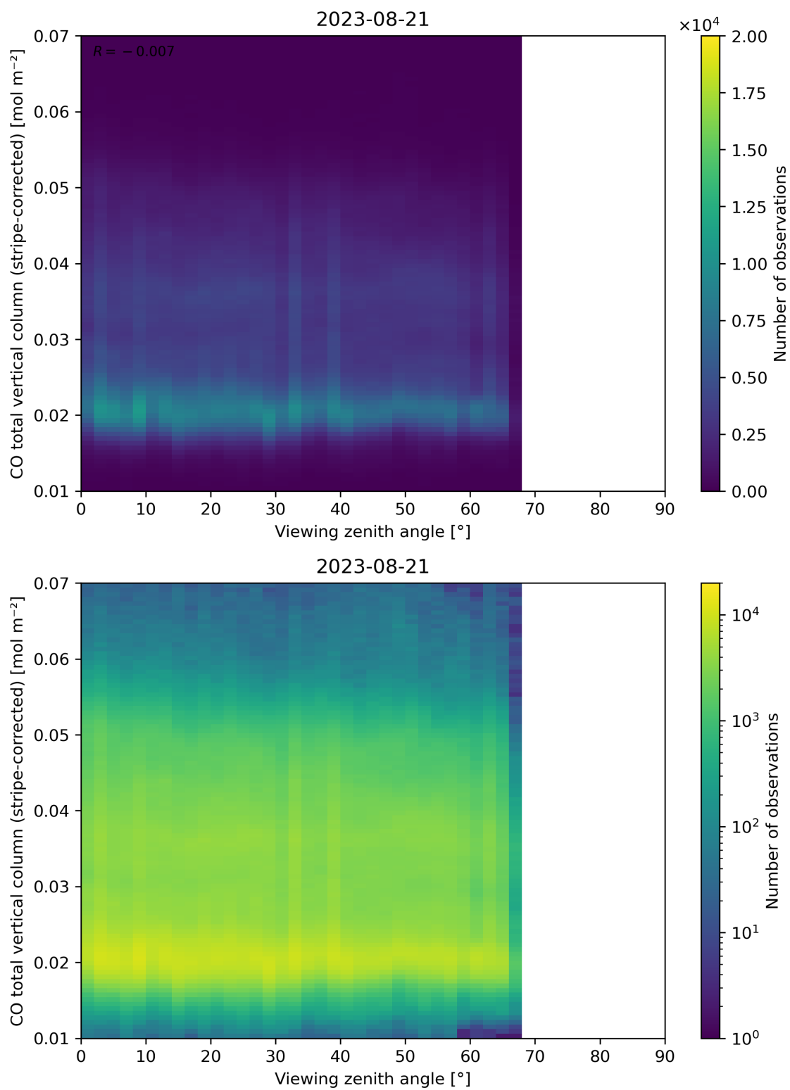
Figure 70: Scatter density plot of “Viewing zenith angle” against “CO total vertical column (stripe-corrected)” for 2023-08-20 to 2023-08-22.
