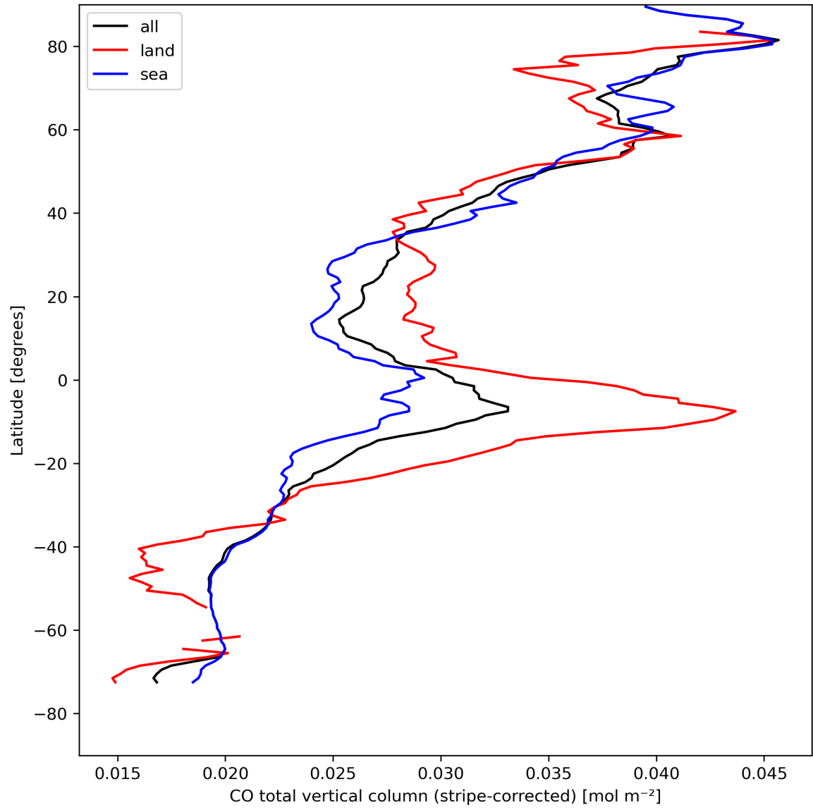
Figure 11: Zonal average of “CO total vertical column (stripe-corrected)” for 2023-08-20 to 2023-08-22.
