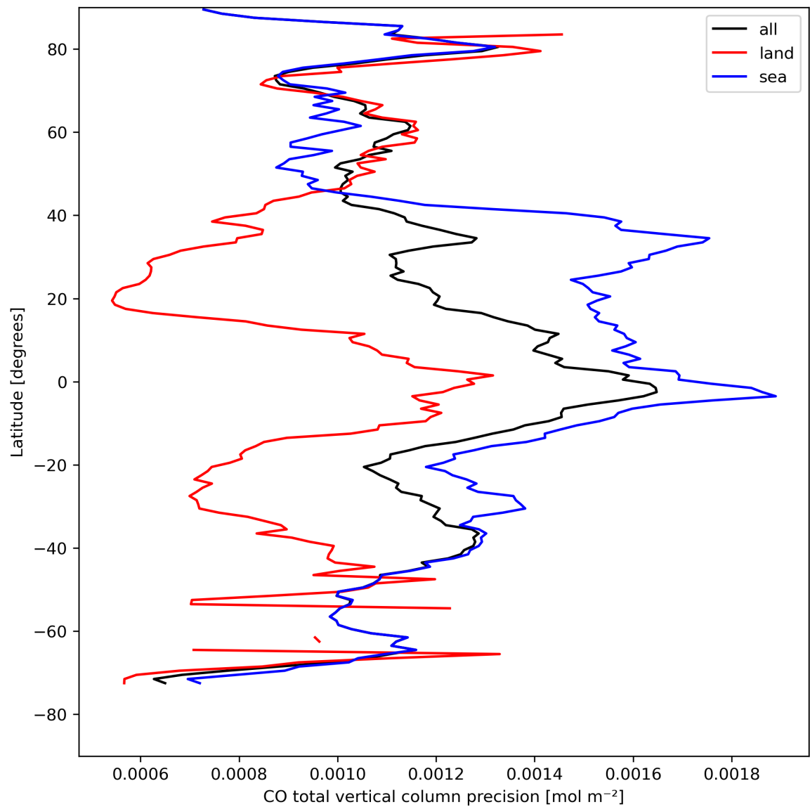
Figure 12: Zonal average of “CO total vertical column precision” for 2023-08-20 to 2023-08-22.
