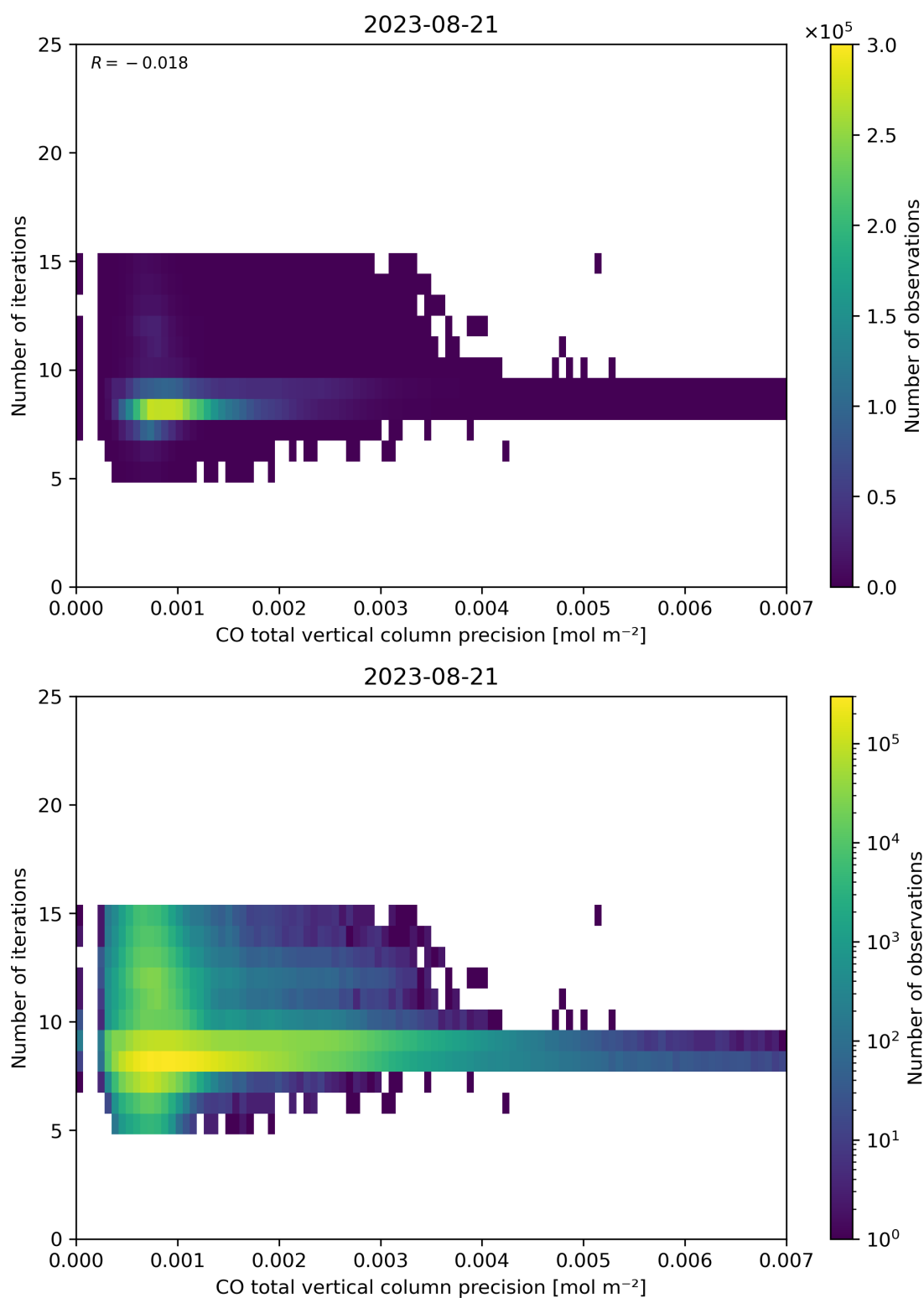
Figure 46: Scatter density plot of “CO total vertical column precision” against “Number of iterations” for 2023-08-20 to 2023-08-22.
