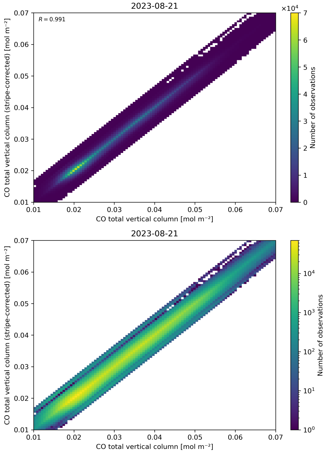
Figure 33: Scatter density plot of “CO total vertical column” against “CO total vertical column (stripe-corrected)” for 2023-08-20 to 2023-08-22.
