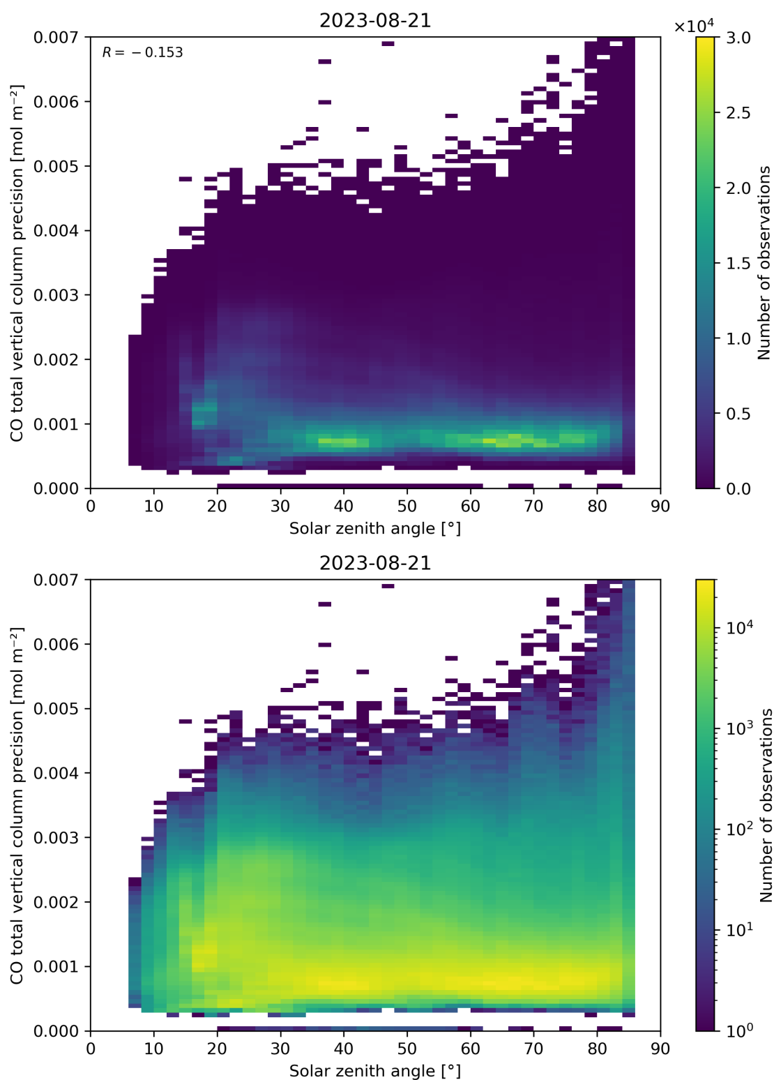
Figure 63: Scatter density plot of “Solar zenith angle” against “CO total vertical column precision” for 2023-08-20 to 2023-08-22.
