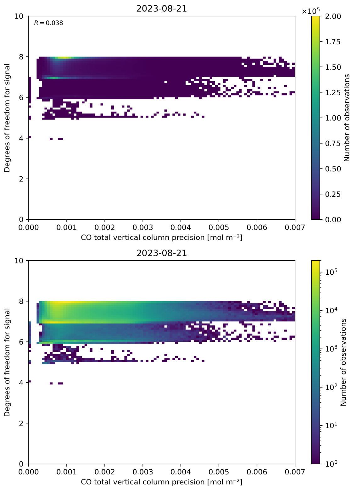
Figure 45: Scatter density plot of “CO total vertical column precision” against “Degrees of freedom for signal” for 2023-08-20 to 2023-08-22.
