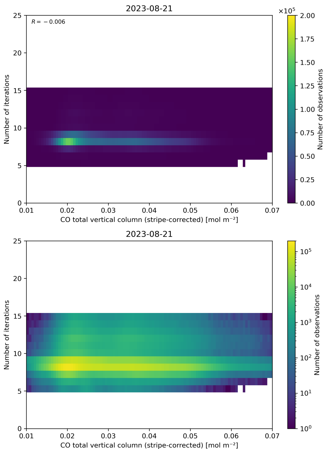
Figure 39: Scatter density plot of “CO total vertical column (stripe-corrected)” against “Number of iterations” for 2023-08-20 to 2023-08-22.
