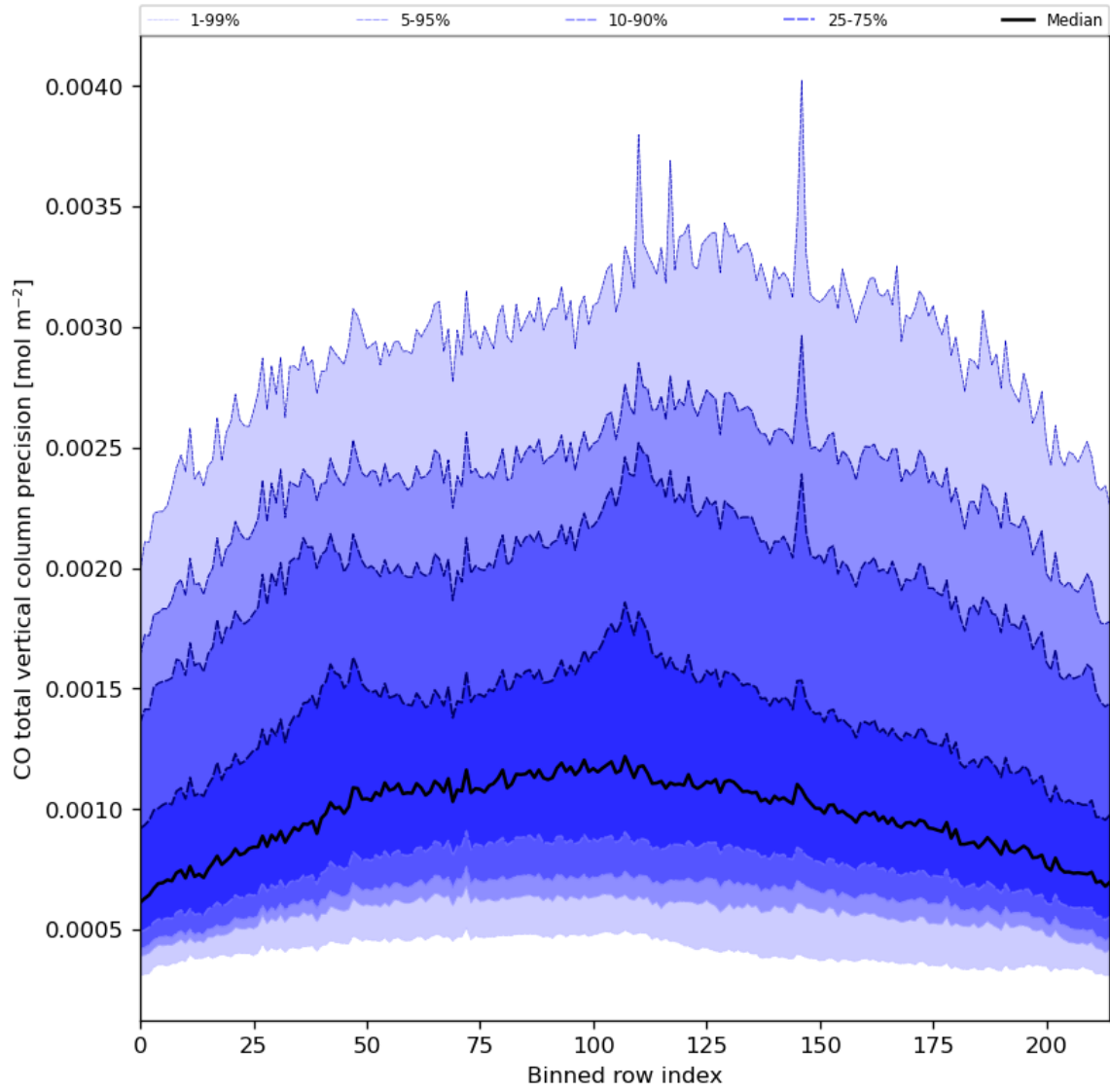
Figure 28: Along track statistics of “CO total vertical column precision” for 2023-08-20 to 2023-08-22
