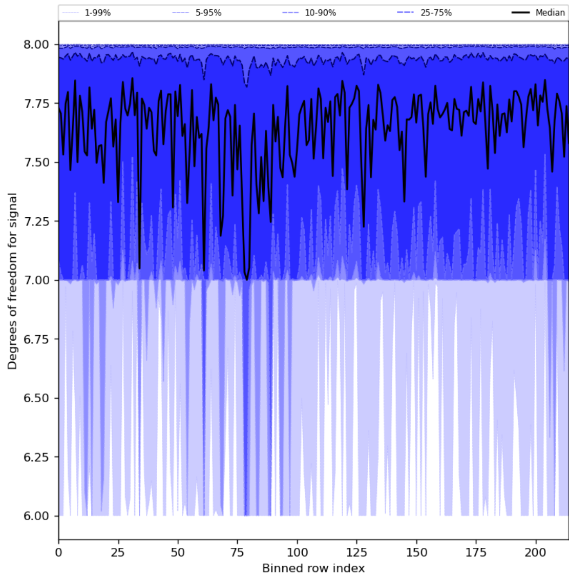
Figure 31: Along track statistics of “Degrees of freedom for signal” for 2023-08-20 to 2023-08-22
