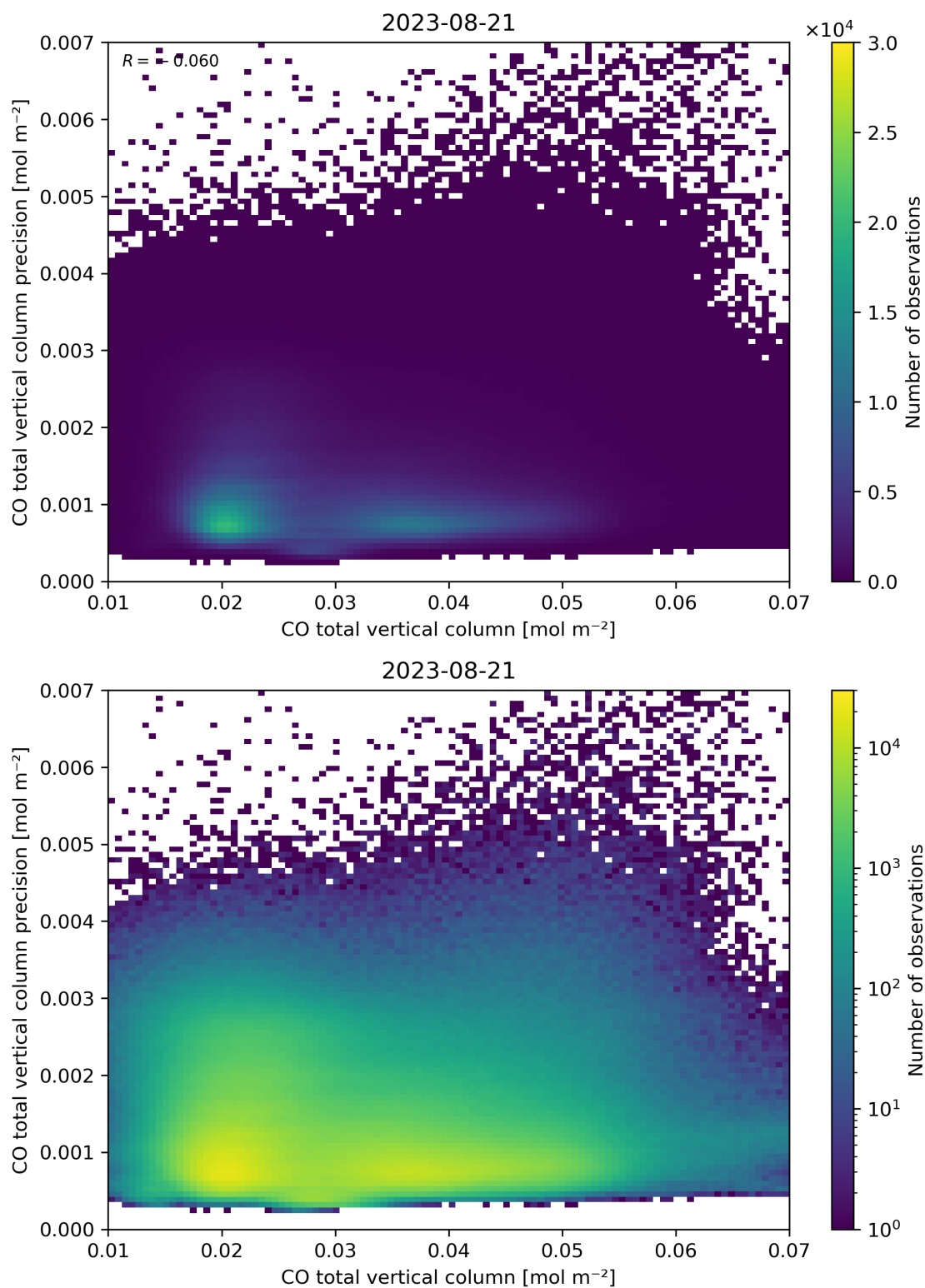
Figure 34: Scatter density plot of “CO total vertical column” against “CO total vertical column precision” for 2023-08-20 to 2023-08-22.
