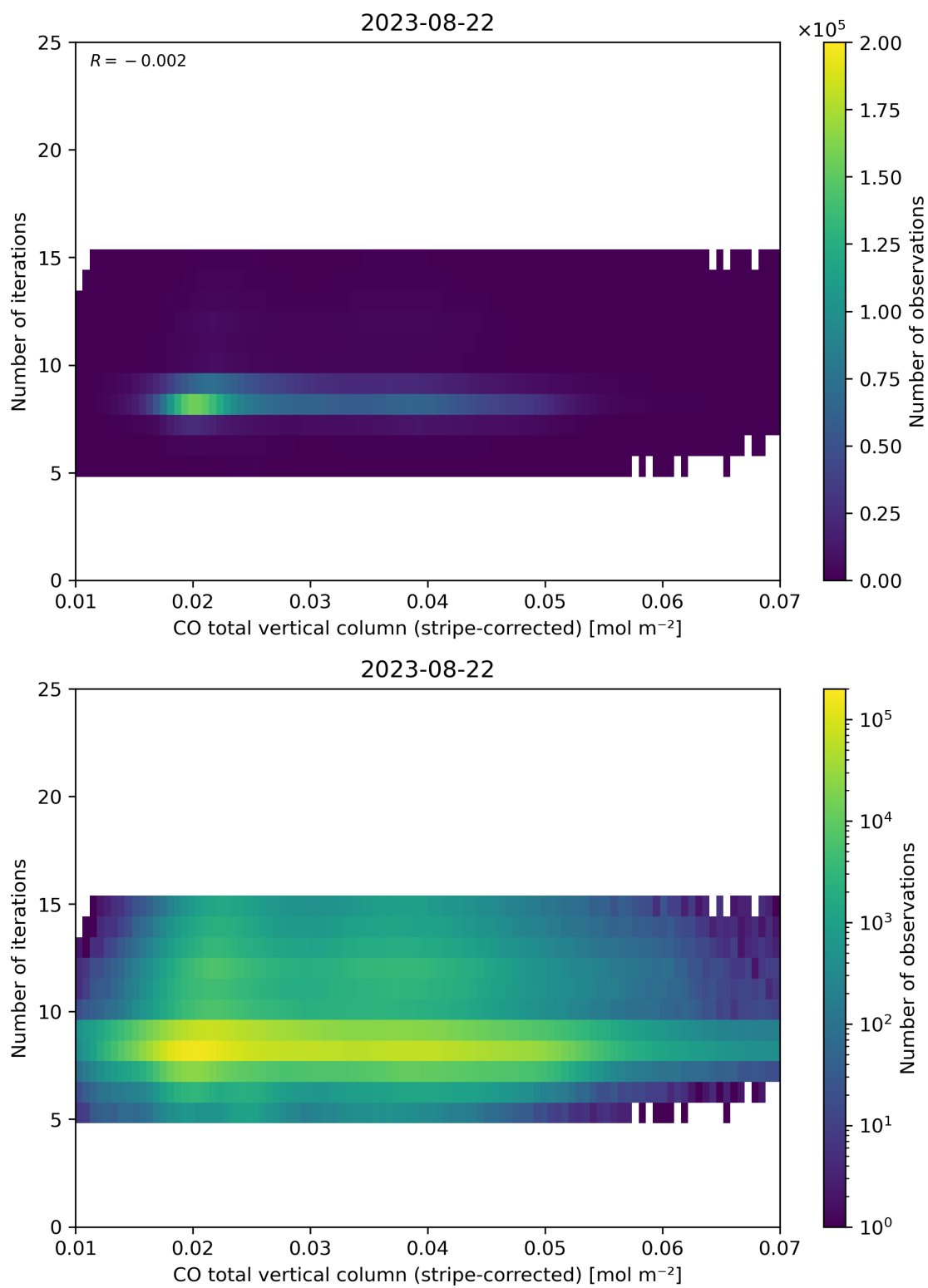
Figure 39: Scatter density plot of “CO total vertical column (stripe-corrected)” against “Number of iterations” for 2023-08-21 to 2023-08-23.
