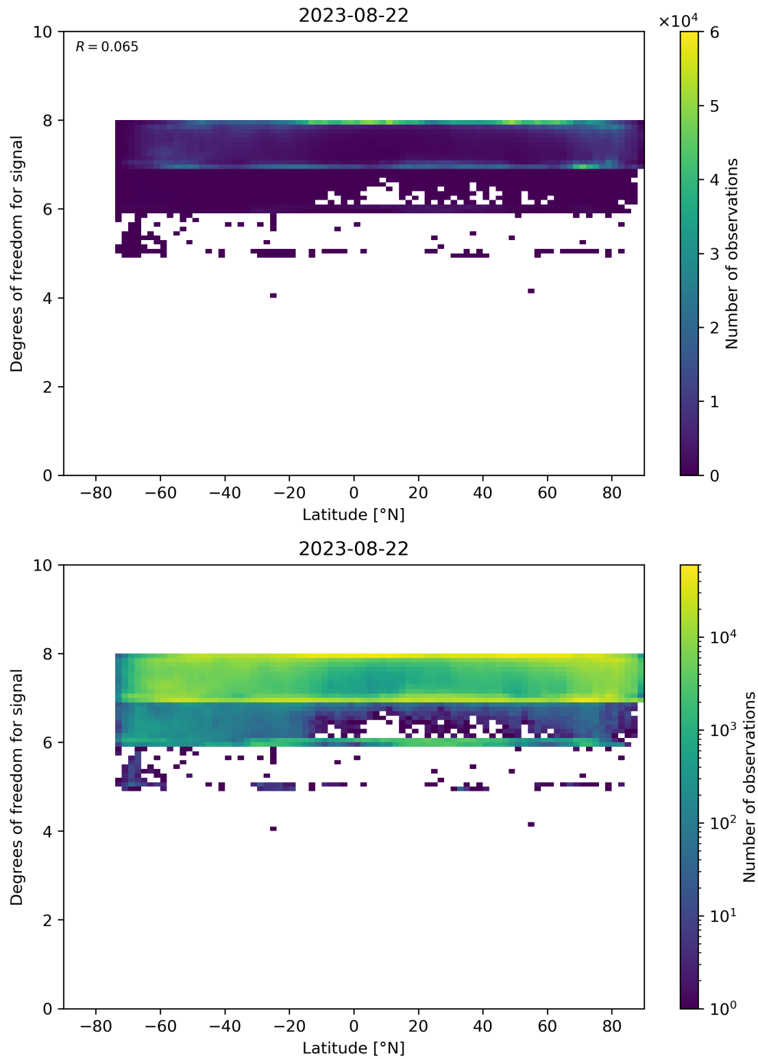
Figure 55: Scatter density plot of “Latitude” against “Degrees of freedom for signal” for 2023-08-21 to 2023-08-23.
