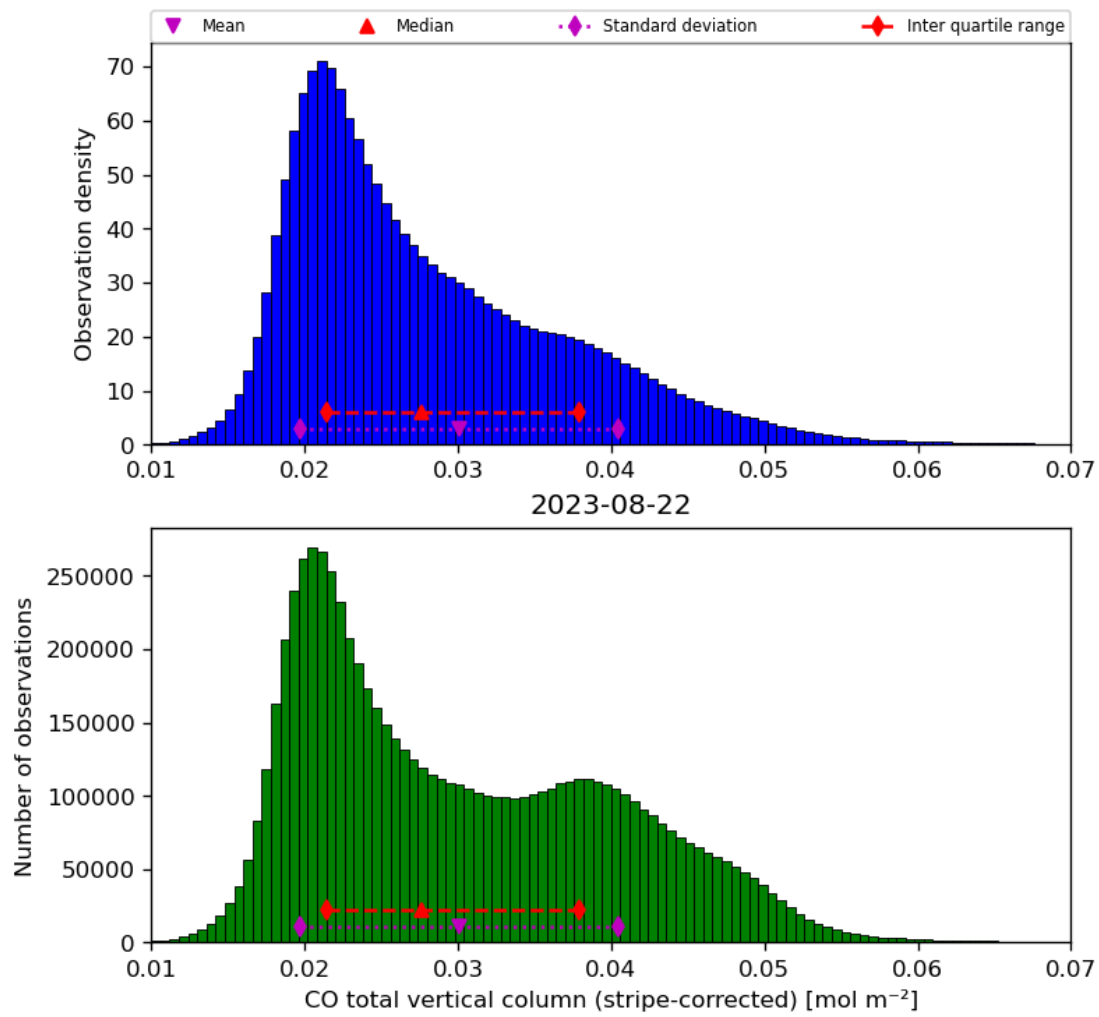
Figure 19: Histogram of “CO total vertical column (stripe-corrected)” for 2023-08-21 to 2023-08-23
