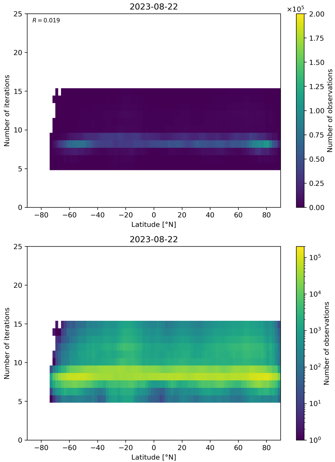
Figure 56: Scatter density plot of “Latitude” against “Number of iterations” for 2023-08-21 to 2023-08-23.
