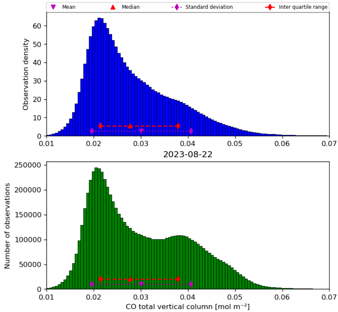
Figure 18: Histogram of “CO total vertical column” for 2023-08-21 to 2023-08-23
