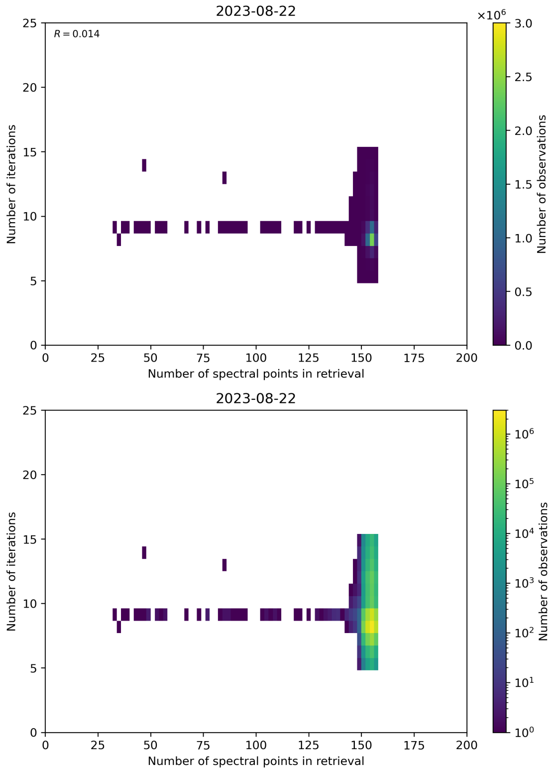
Figure 60: Scatter density plot of “Number of spectral points in retrieval” against “Number of iterations” for 2023-08-21 to 2023-08-23.
