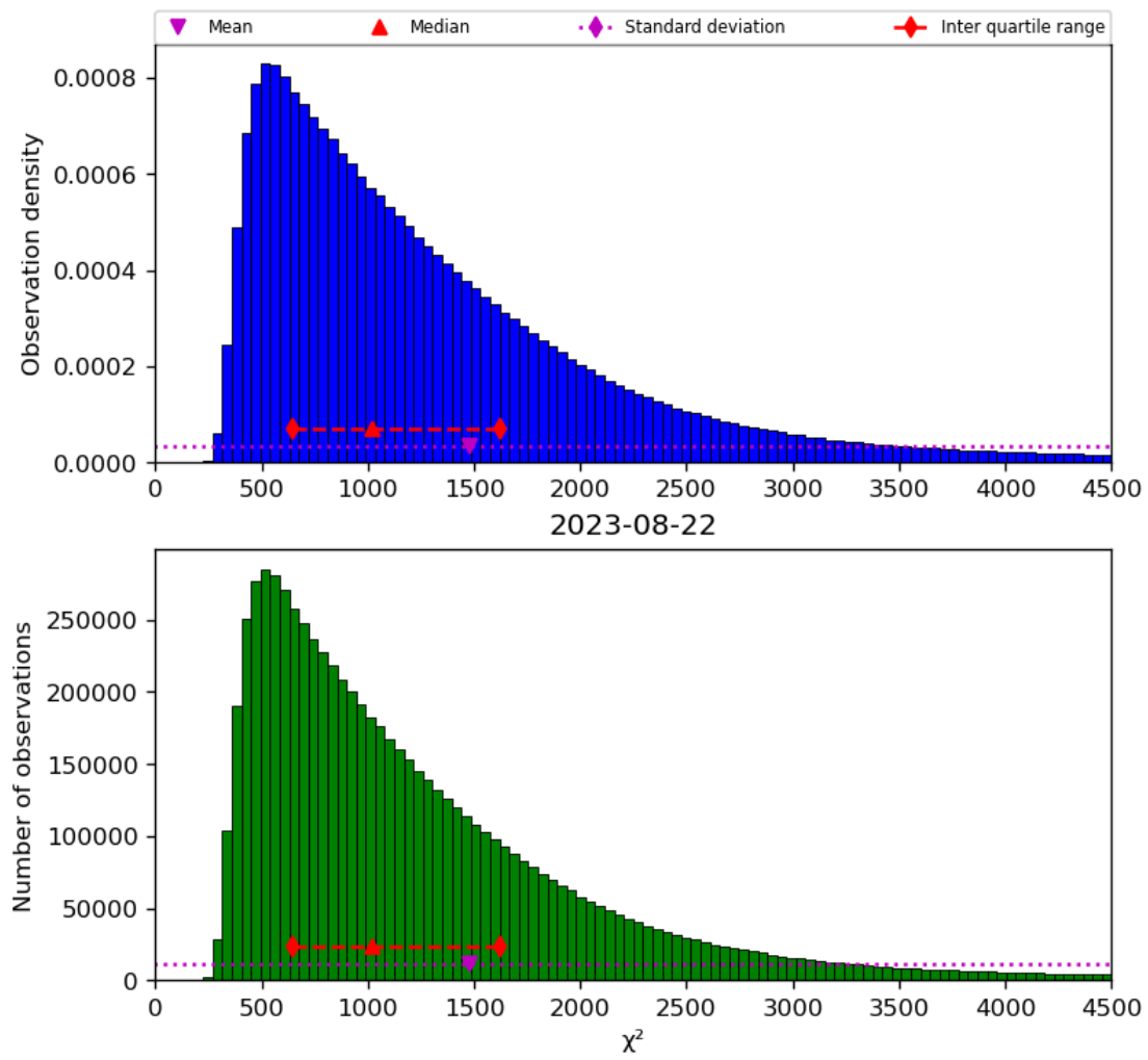
Figure 22: Histogram of “ \chi^2 ” for 2023-08-21 to 2023-08-23
