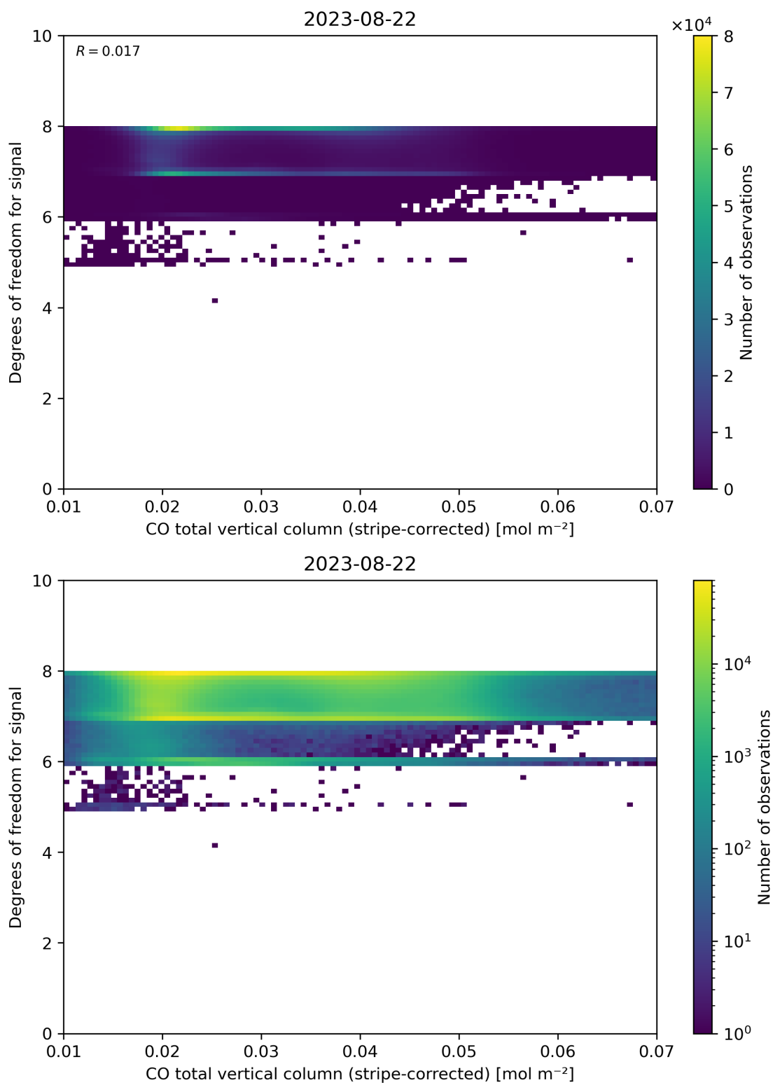
Figure 38: Scatter density plot of “CO total vertical column (stripe-corrected)” against “Degrees of freedom for signal” for 2023-08-21 to 2023-08-23.
