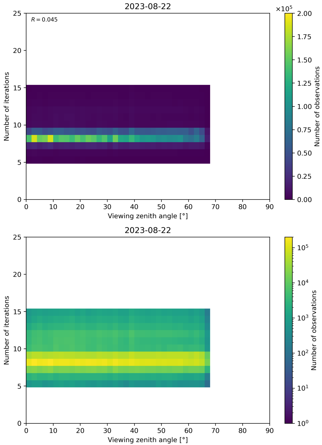
Figure 75: Scatter density plot of “Viewing zenith angle” against “Number of iterations” for 2023-08-21 to 2023-08-23.
