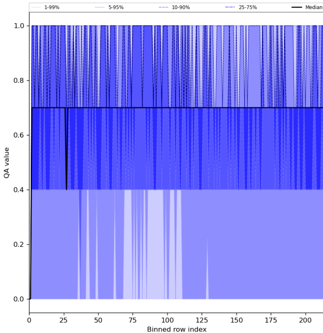
Figure 25: Along track statistics of “QA value” for 2023-08-21 to 2023-08-23
