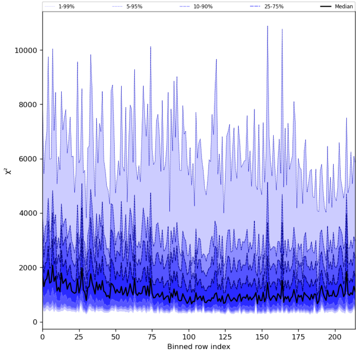
Figure 30: Along track statistics of “ \chi^2 ” for 2023-08-21 to 2023-08-23
