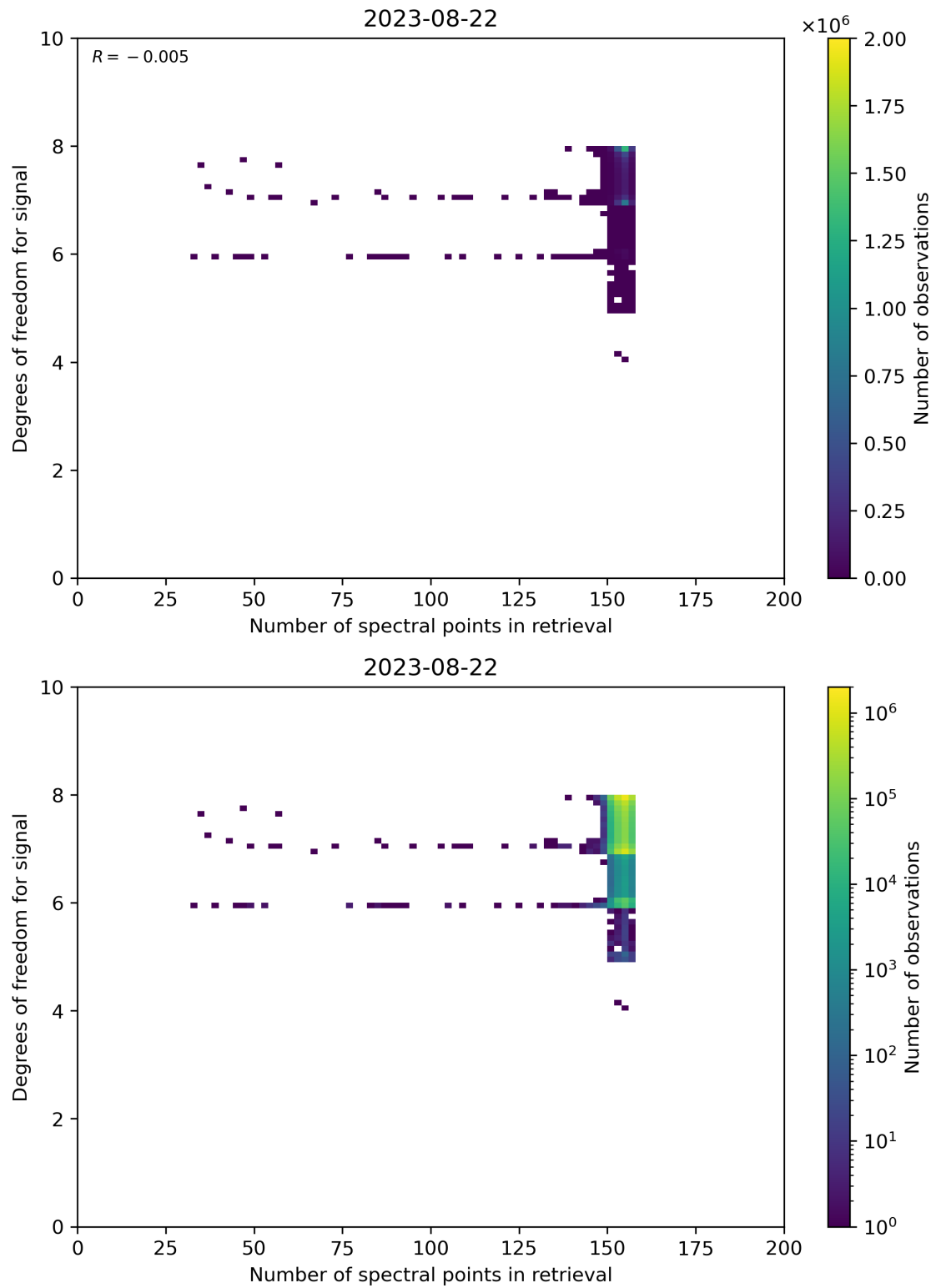
Figure 59: Scatter density plot of “Number of spectral points in retrieval” against “Degrees of freedom for signal” for 2023-08-21 to 2023-08-23.
