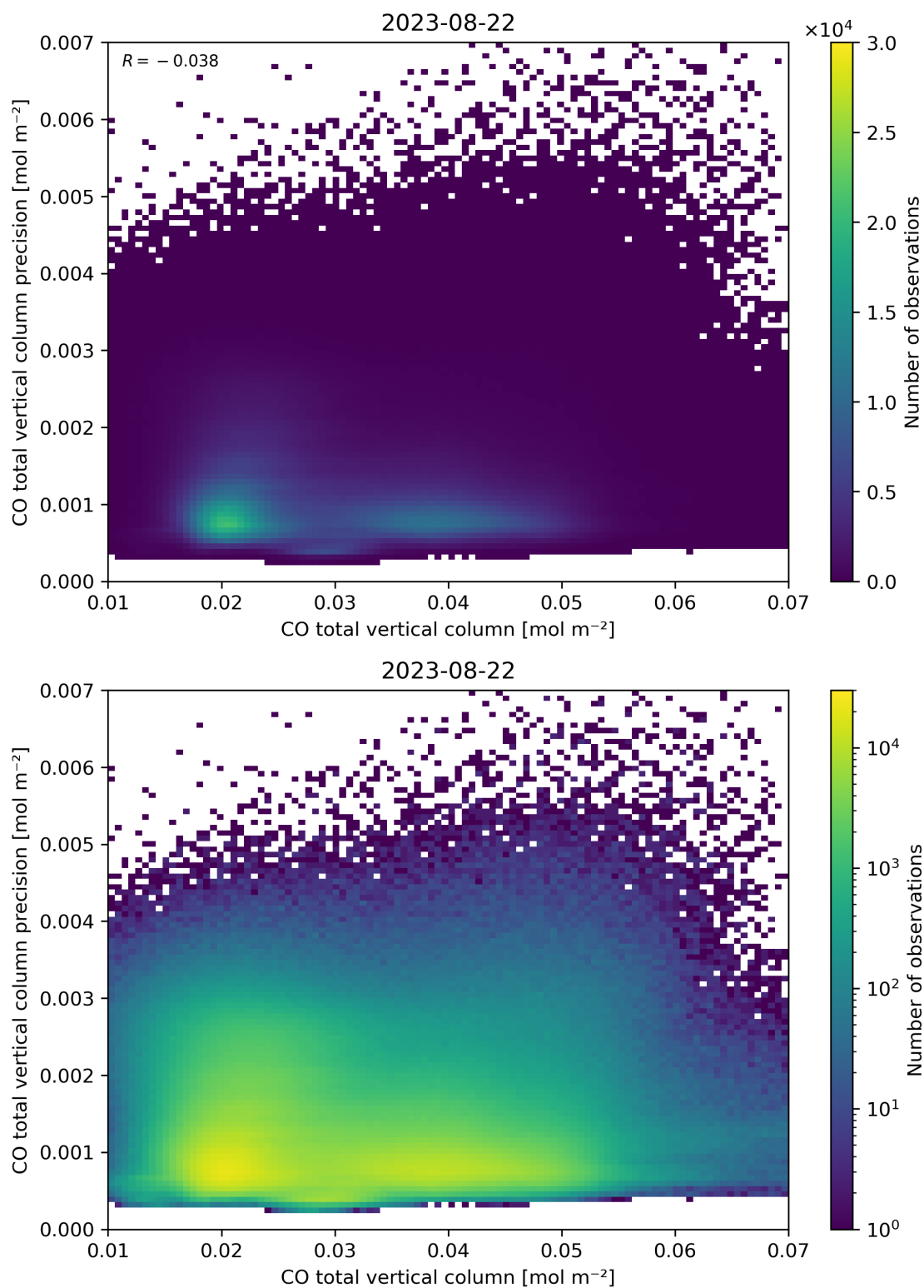
Figure 34: Scatter density plot of “CO total vertical column” against “CO total vertical column precision” for 2023-08-21 to 2023-08-23.
