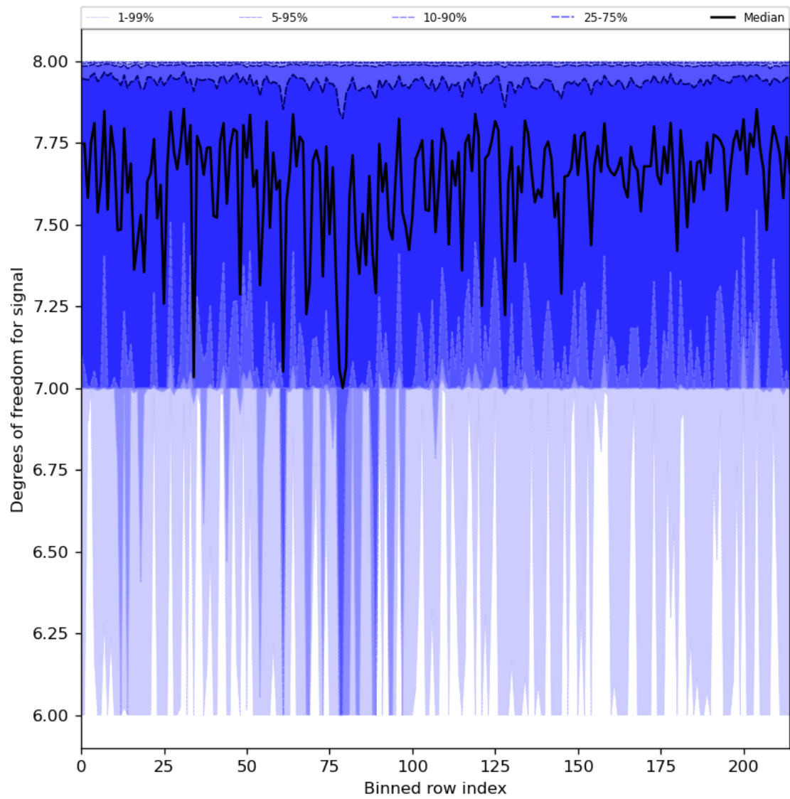
Figure 31: Along track statistics of “Degrees of freedom for signal” for 2023-08-21 to 2023-08-23
