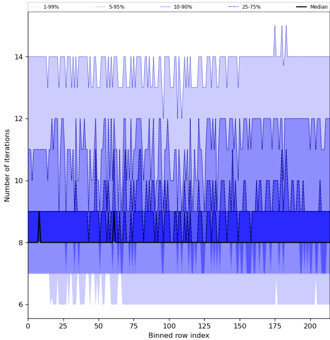
Figure 32: Along track statistics of “Number of iterations” for 2023-08-21 to 2023-08-23
