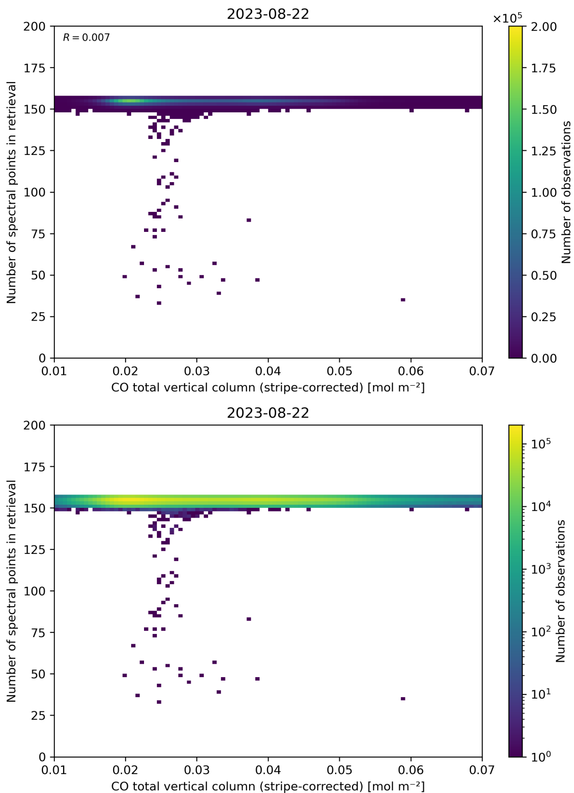
Figure 40: Scatter density plot of “CO total vertical column (stripe-corrected)” against “Number of spectral points in retrieval” for 2023-08-21 to 2023-08-23.
