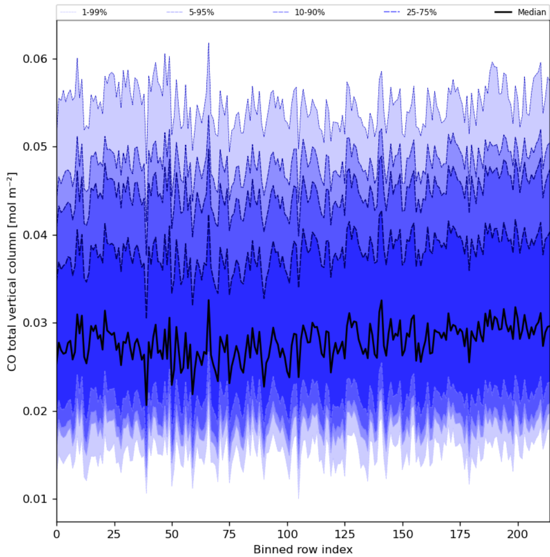
Figure 26: Along track statistics of “CO total vertical column” for 2023-08-21 to 2023-08-23
