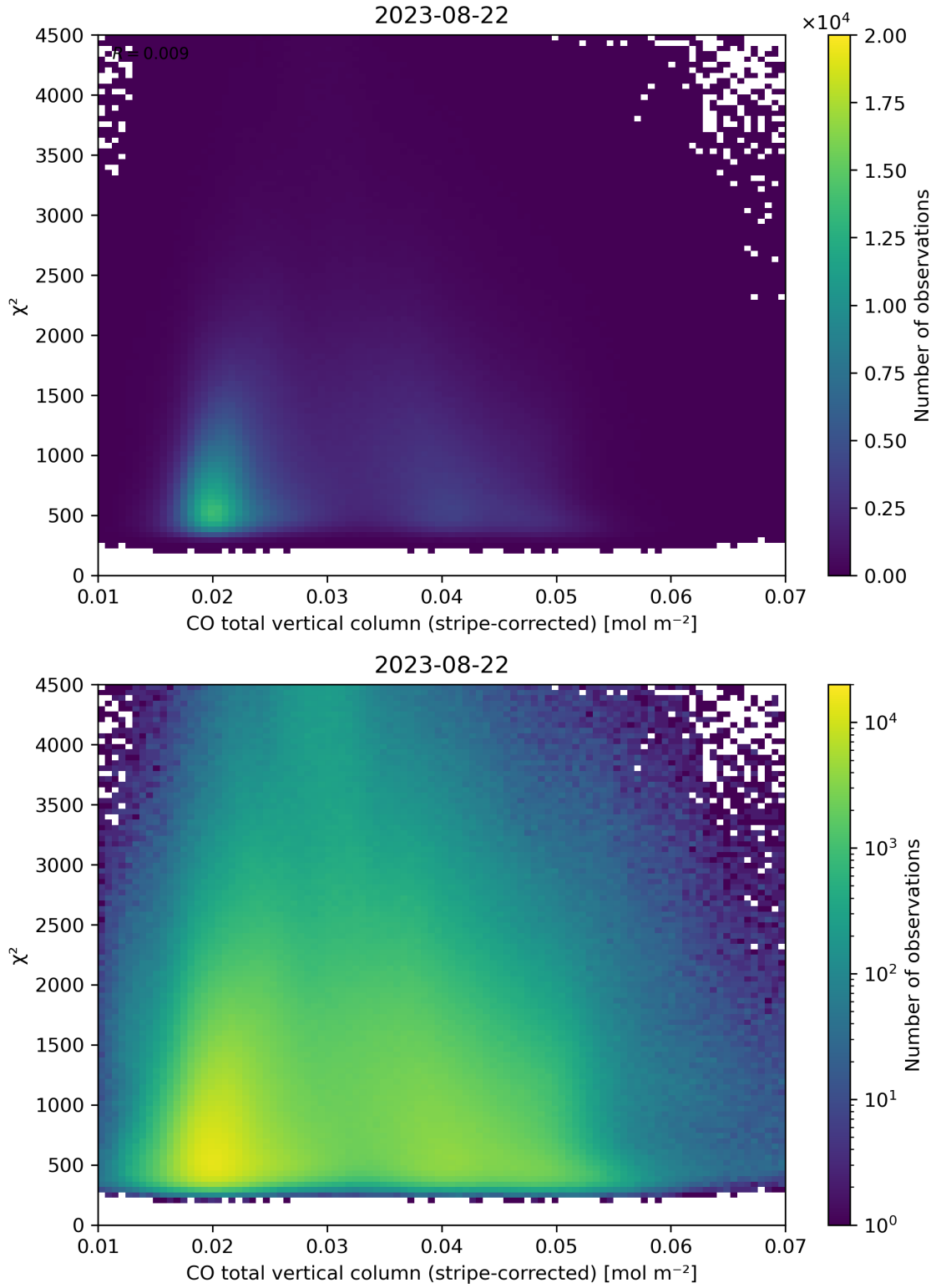
Figure 37: Scatter density plot of “CO total vertical column (stripe-corrected)” against “ \chi^2 ” for 2023-08-21 to 2023-08-23.
