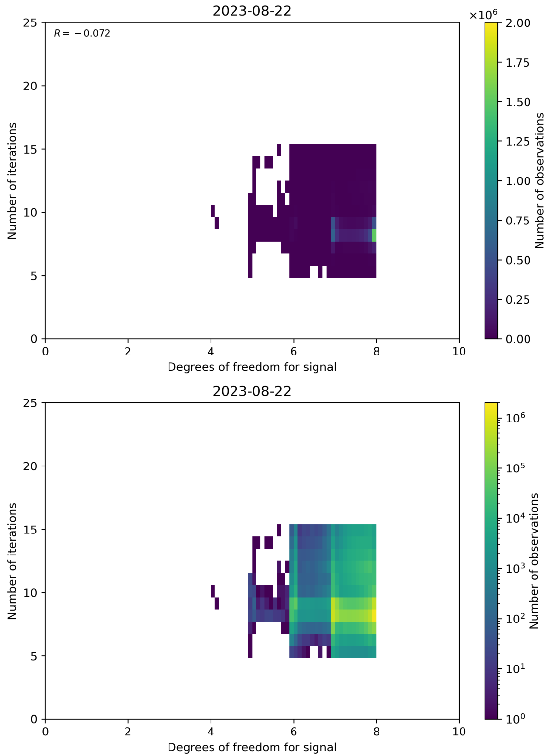
Figure 50: Scatter density plot of “Degrees of freedom for signal” against “Number of iterations” for 2023-08-21 to 2023-08-23.
