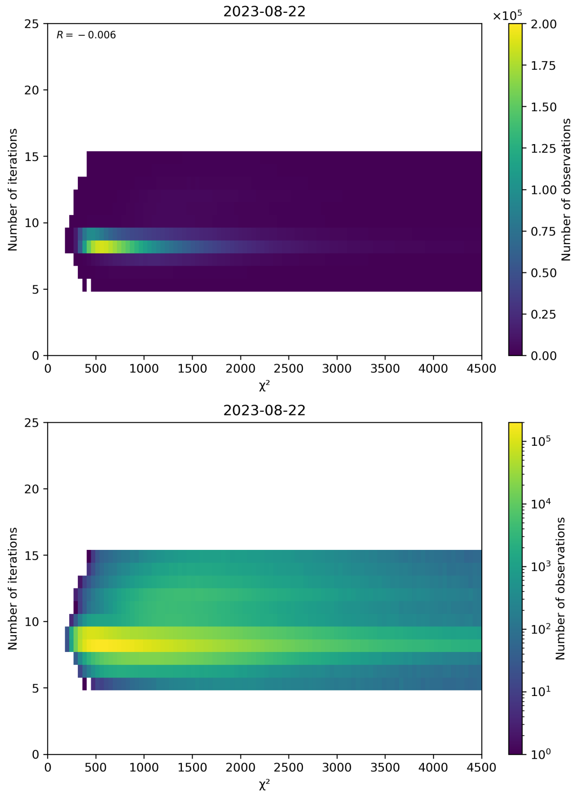
Figure 49: Scatter density plot of “ \chi^2 ” against “Number of iterations” for 2023-08-21 to 2023-08-23.
