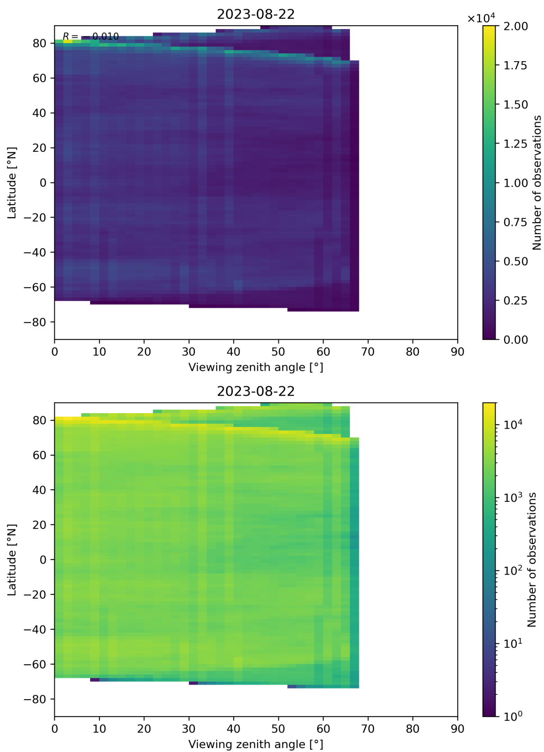
Figure 74: Scatter density plot of “Viewing zenith angle” against “Latitude” for 2023-08-21 to 2023-08-23.
