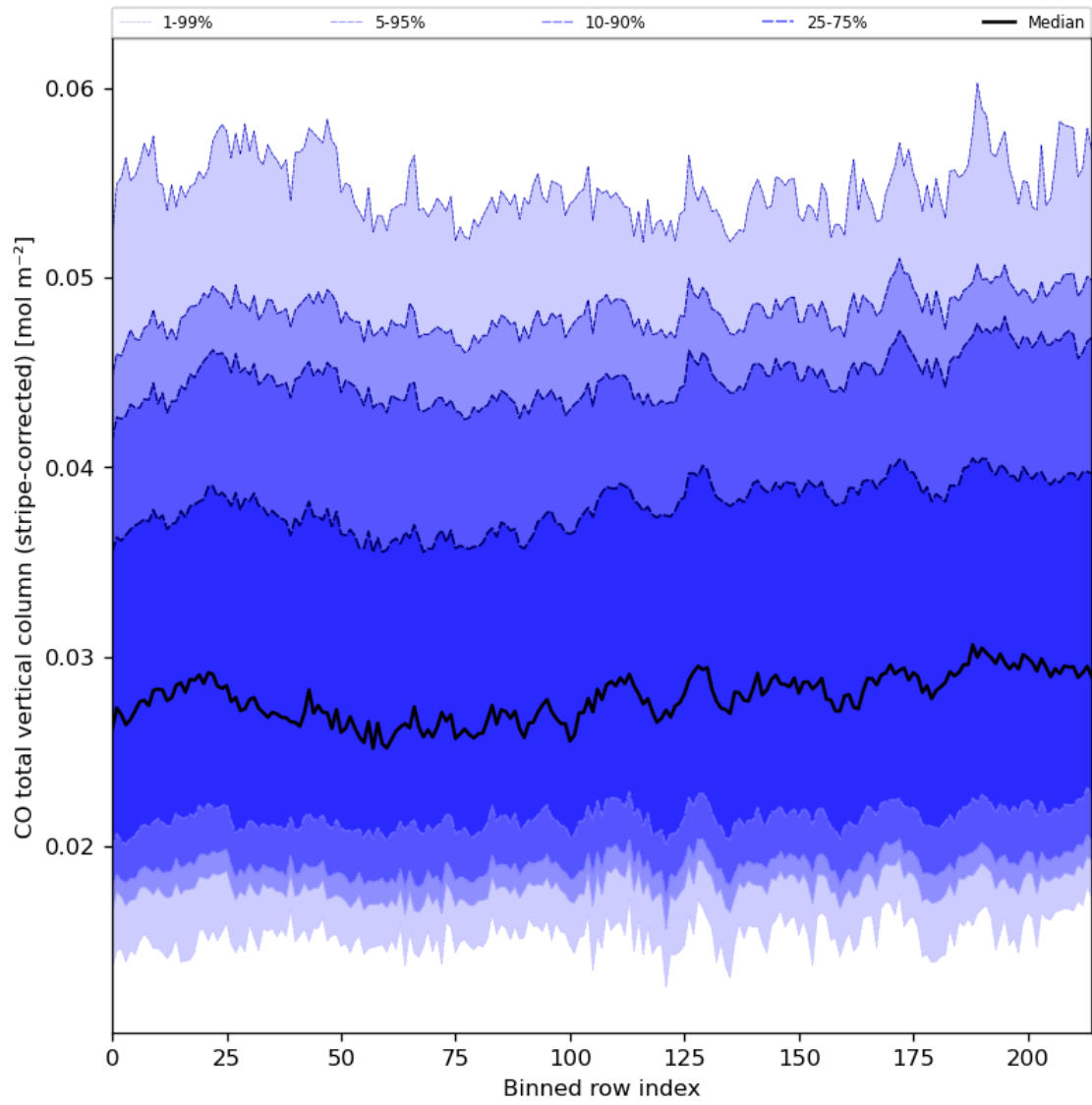
Figure 27: Along track statistics of “CO total vertical column (stripe-corrected)” for 2023-08-21 to 2023-08-23
