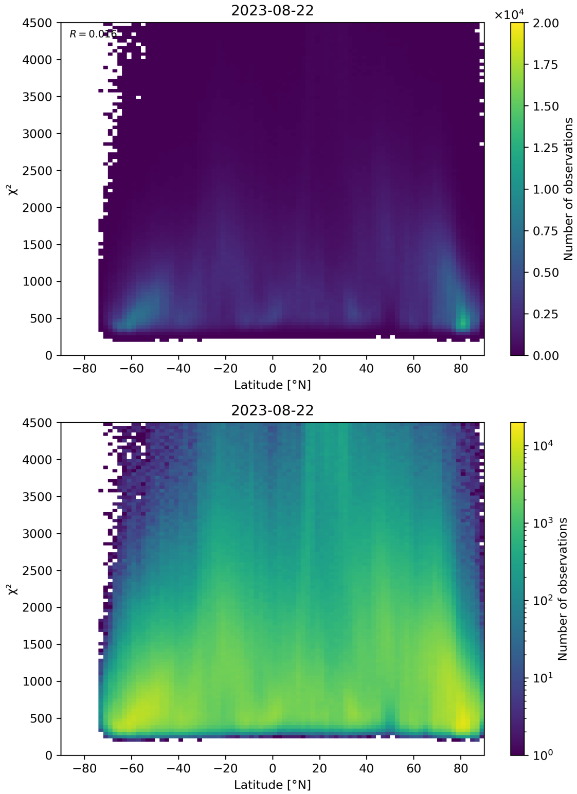
Figure 54: Scatter density plot of “Latitude” against “ \chi^2 ” for 2023-08-21 to 2023-08-23.
