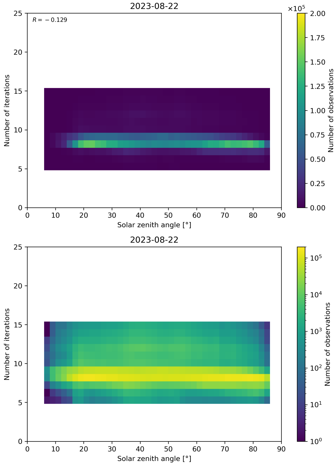
Figure 67: Scatter density plot of “Solar zenith angle” against “Number of iterations” for 2023-08-21 to 2023-08-23.
