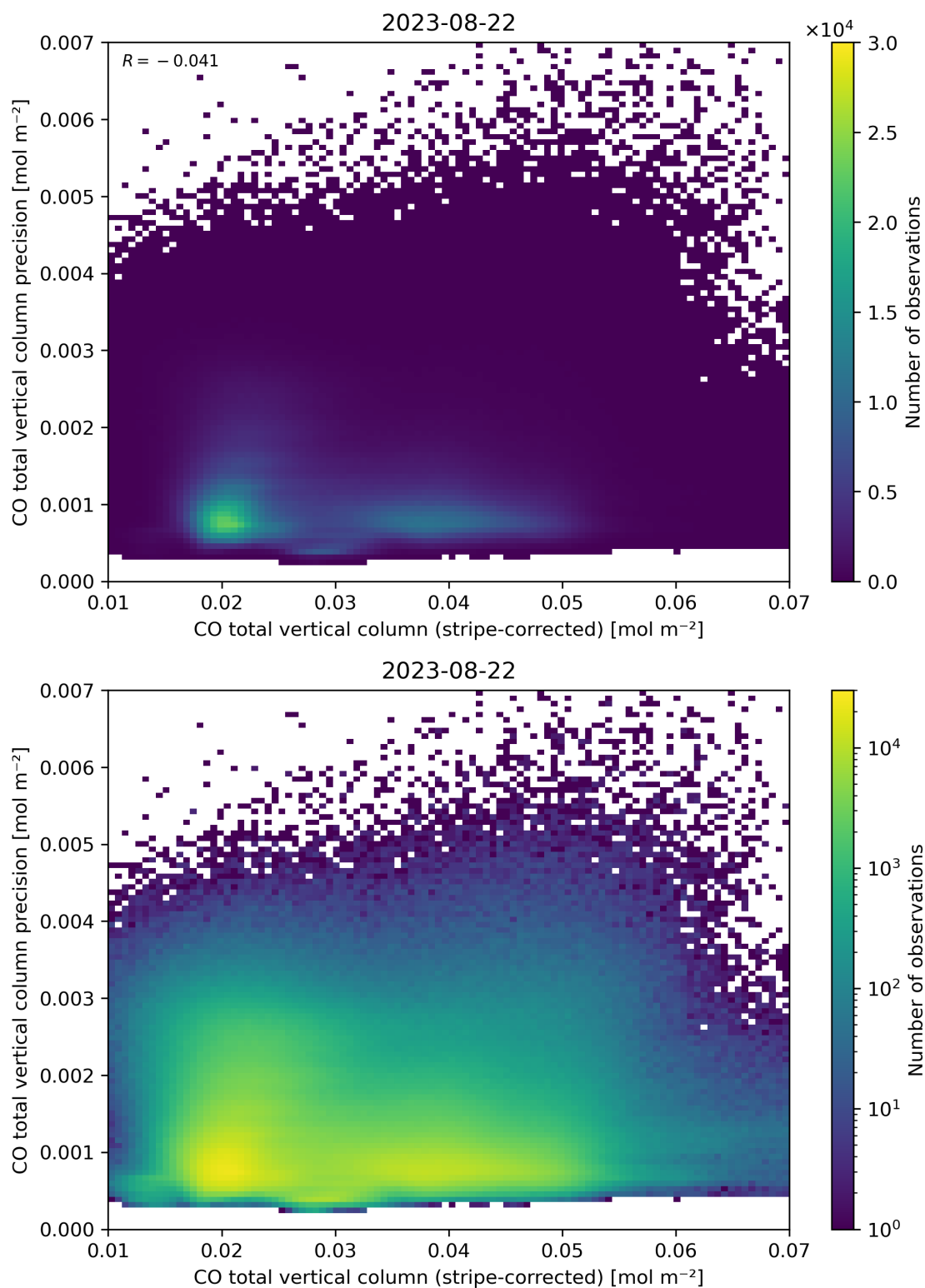
Figure 36: Scatter density plot of “CO total vertical column (stripe-corrected)” against “CO total vertical column precision” for 2023-08-21 to 2023-08-23.
