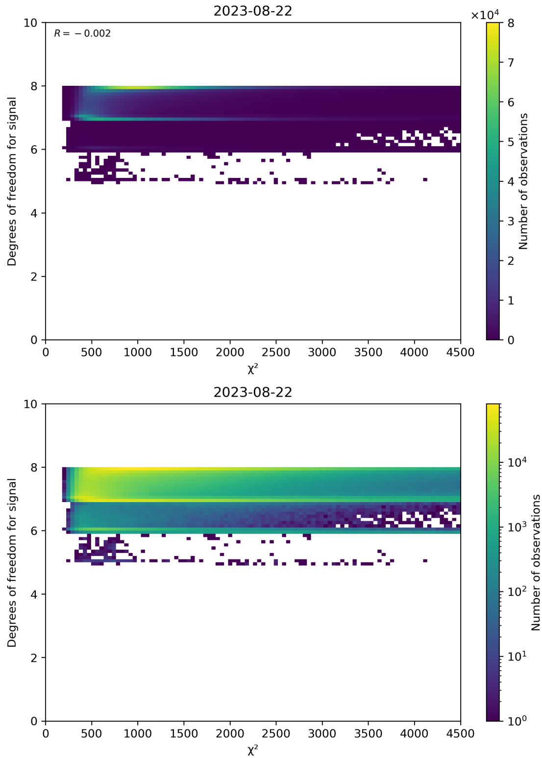
Figure 48: Scatter density plot of “ \chi^2 ” against “Degrees of freedom for signal” for 2023-08-21 to 2023-08-23.
