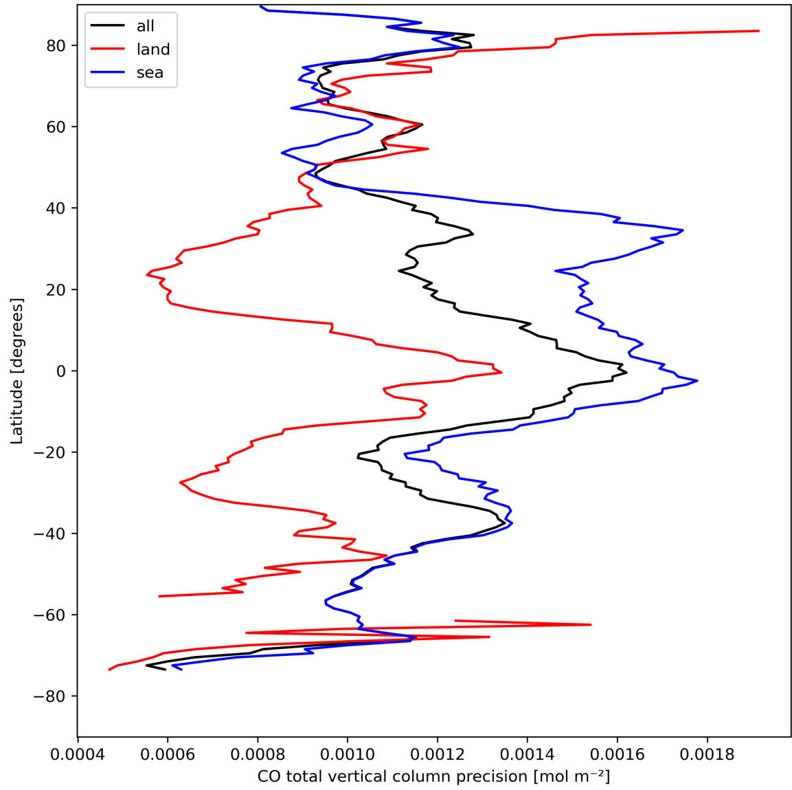
Figure 12: Zonal average of “CO total vertical column precision” for 2023-08-21 to 2023-08-23.
