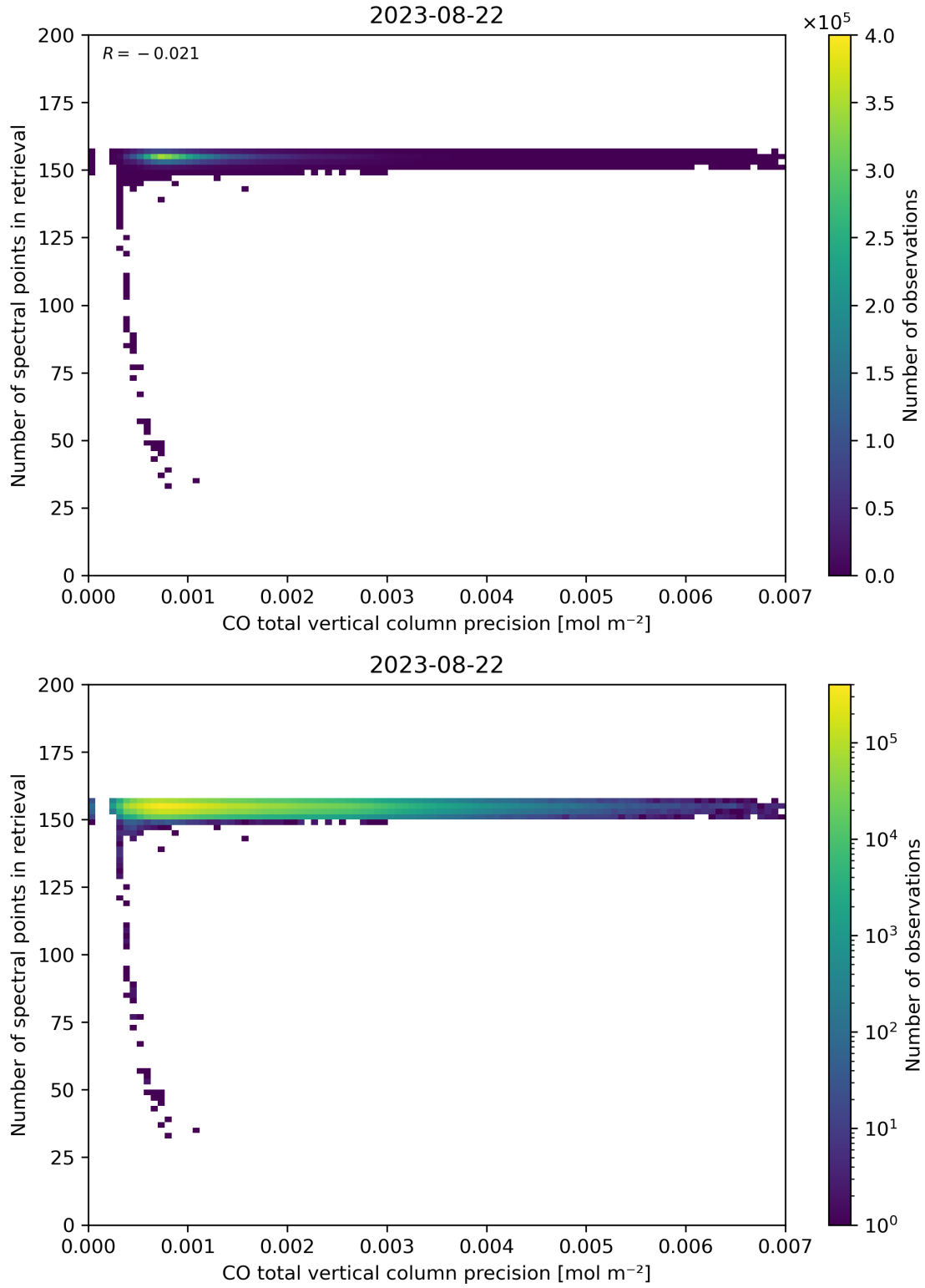
Figure 47: Scatter density plot of “CO total vertical column precision” against “Number of spectral points in retrieval” for 2023-08-21 to 2023-08-23.
