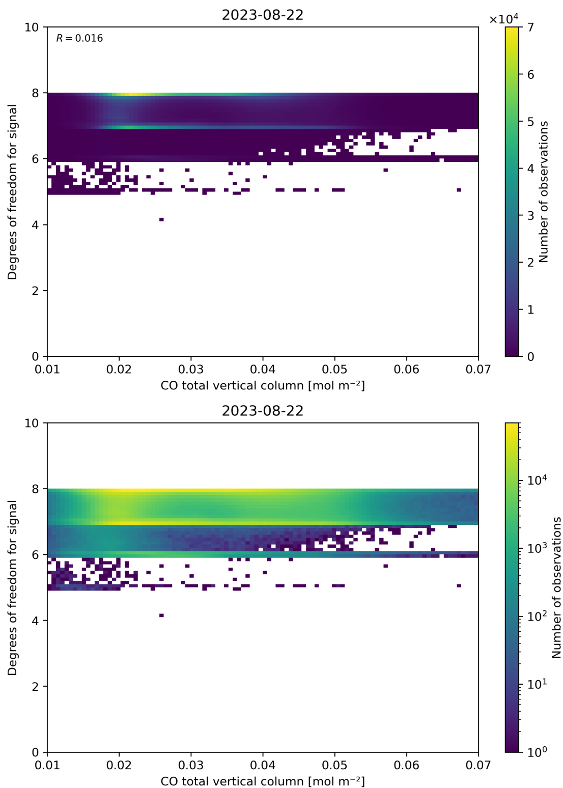
Figure 41: Scatter density plot of “CO total vertical column” against “Degrees of freedom for signal” for 2023-08-21 to 2023-08-23.
