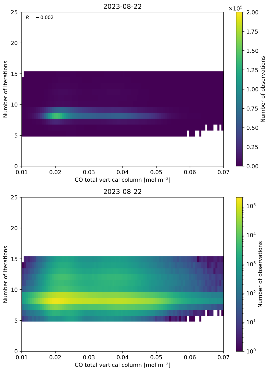
Figure 42: Scatter density plot of “CO total vertical column” against “Number of iterations” for 2023-08-21 to 2023-08-23.
