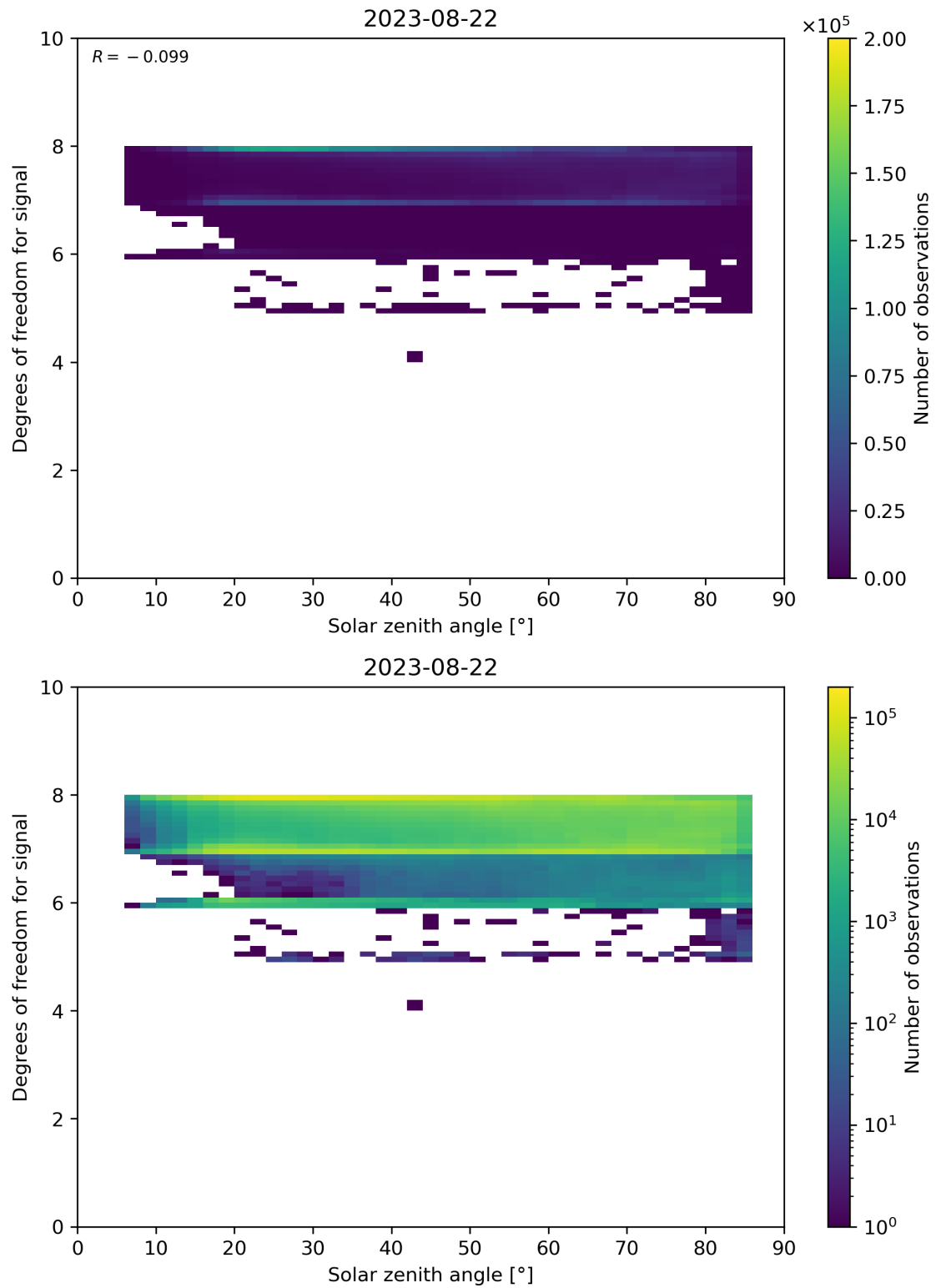
Figure 65: Scatter density plot of “Solar zenith angle” against “Degrees of freedom for signal” for 2023-08-21 to 2023-08-23.
