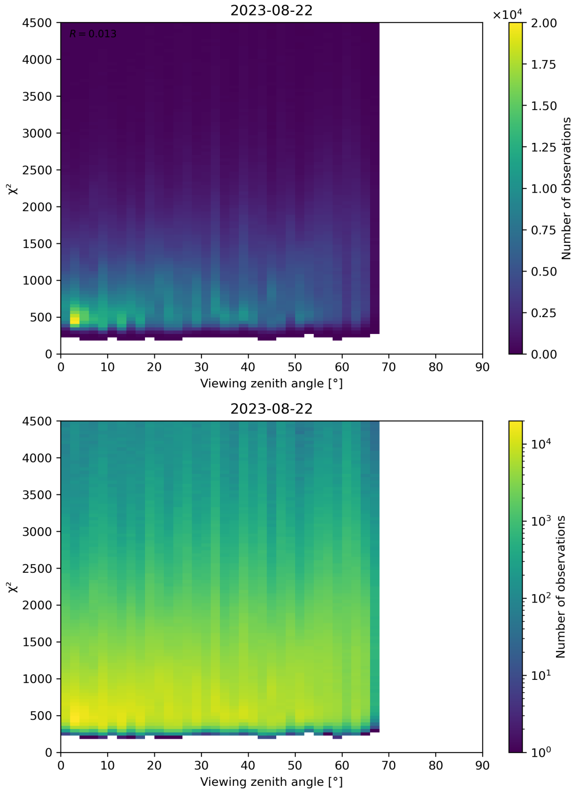
Figure 72: Scatter density plot of “Viewing zenith angle” against “ \chi^2 ” for 2023-08-21 to 2023-08-23.
