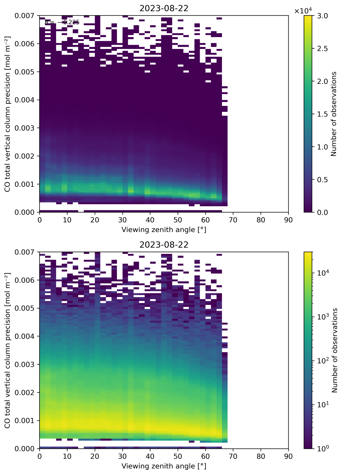
Figure 71: Scatter density plot of “Viewing zenith angle” against “CO total vertical column precision” for 2023-08-21 to 2023-08-23.
