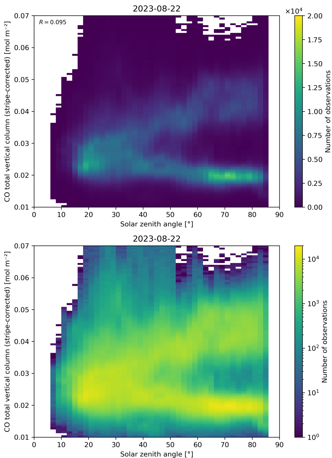
Figure 62: Scatter density plot of “Solar zenith angle” against “CO total vertical column (stripe-corrected)” for 2023-08-21 to 2023-08-23.
