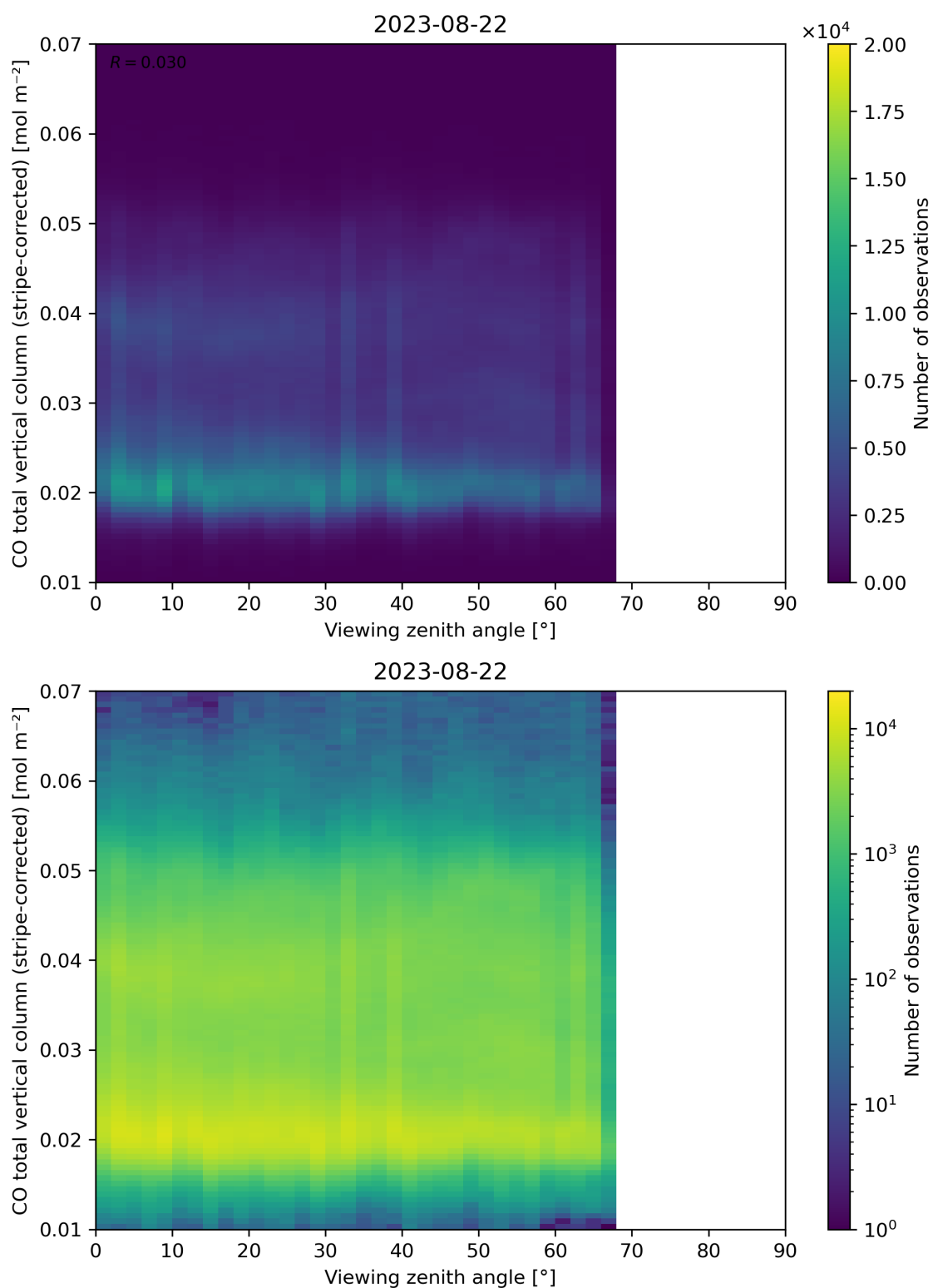
Figure 70: Scatter density plot of “Viewing zenith angle” against “CO total vertical column (stripe-corrected)” for 2023-08-21 to 2023-08-23.
