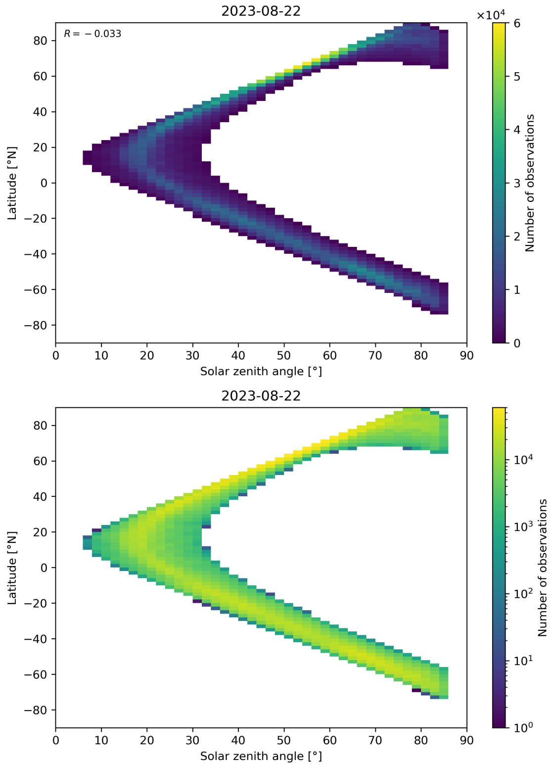
Figure 66: Scatter density plot of “Solar zenith angle” against “Latitude” for 2023-08-21 to 2023-08-23.
