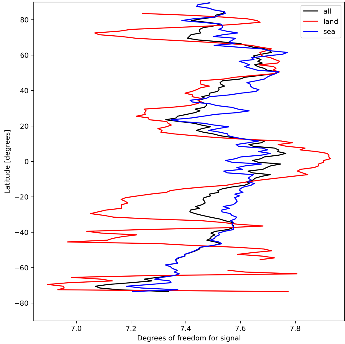
Figure 15: Zonal average of “Degrees of freedom for signal” for 2023-08-21 to 2023-08-23.
