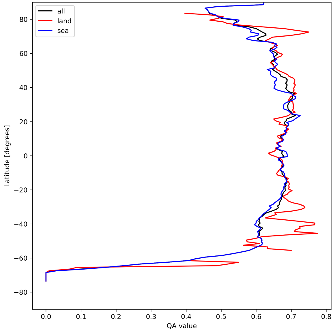
Figure 9: Zonal average of “QA value” for 2023-08-21 to 2023-08-23.
