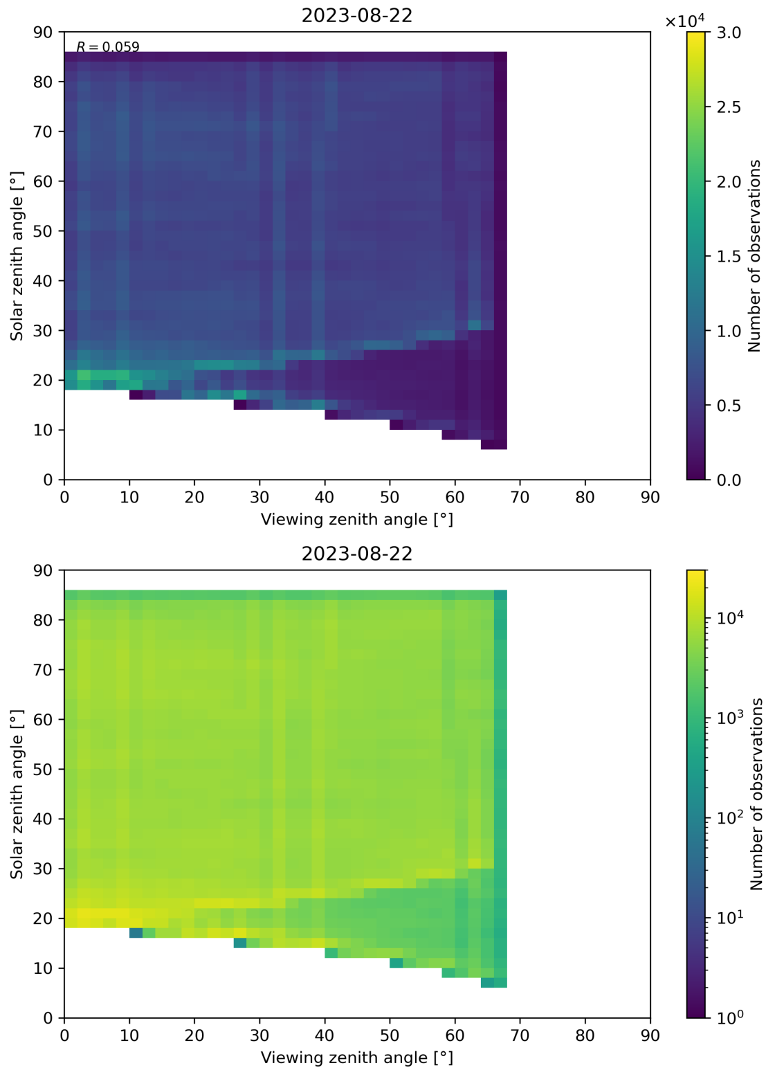
Figure 77: Scatter density plot of “Viewing zenith angle” against “Solar zenith angle” for 2023-08-21 to 2023-08-23.
