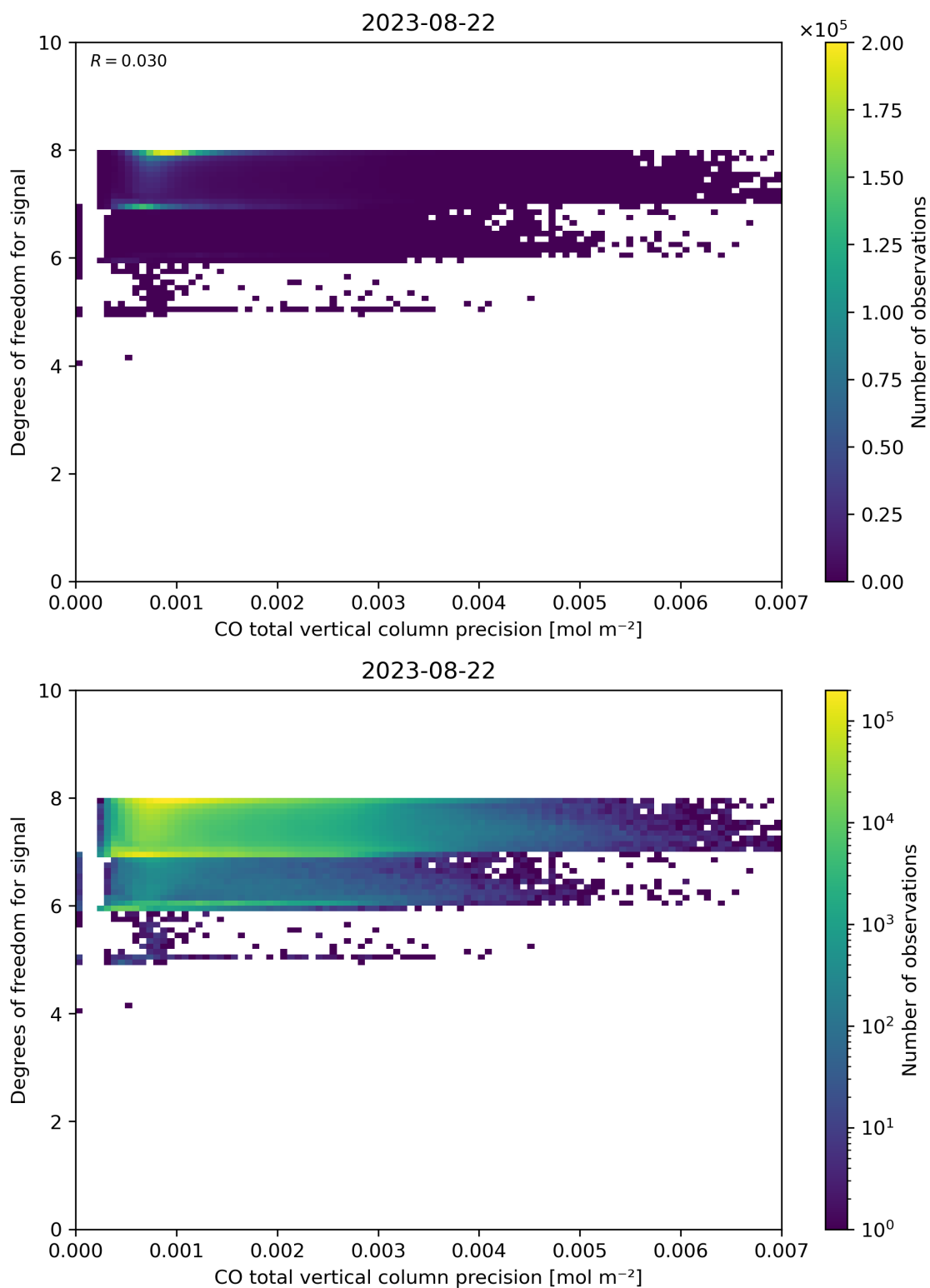
Figure 45: Scatter density plot of “CO total vertical column precision” against “Degrees of freedom for signal” for 2023-08-21 to 2023-08-23.
