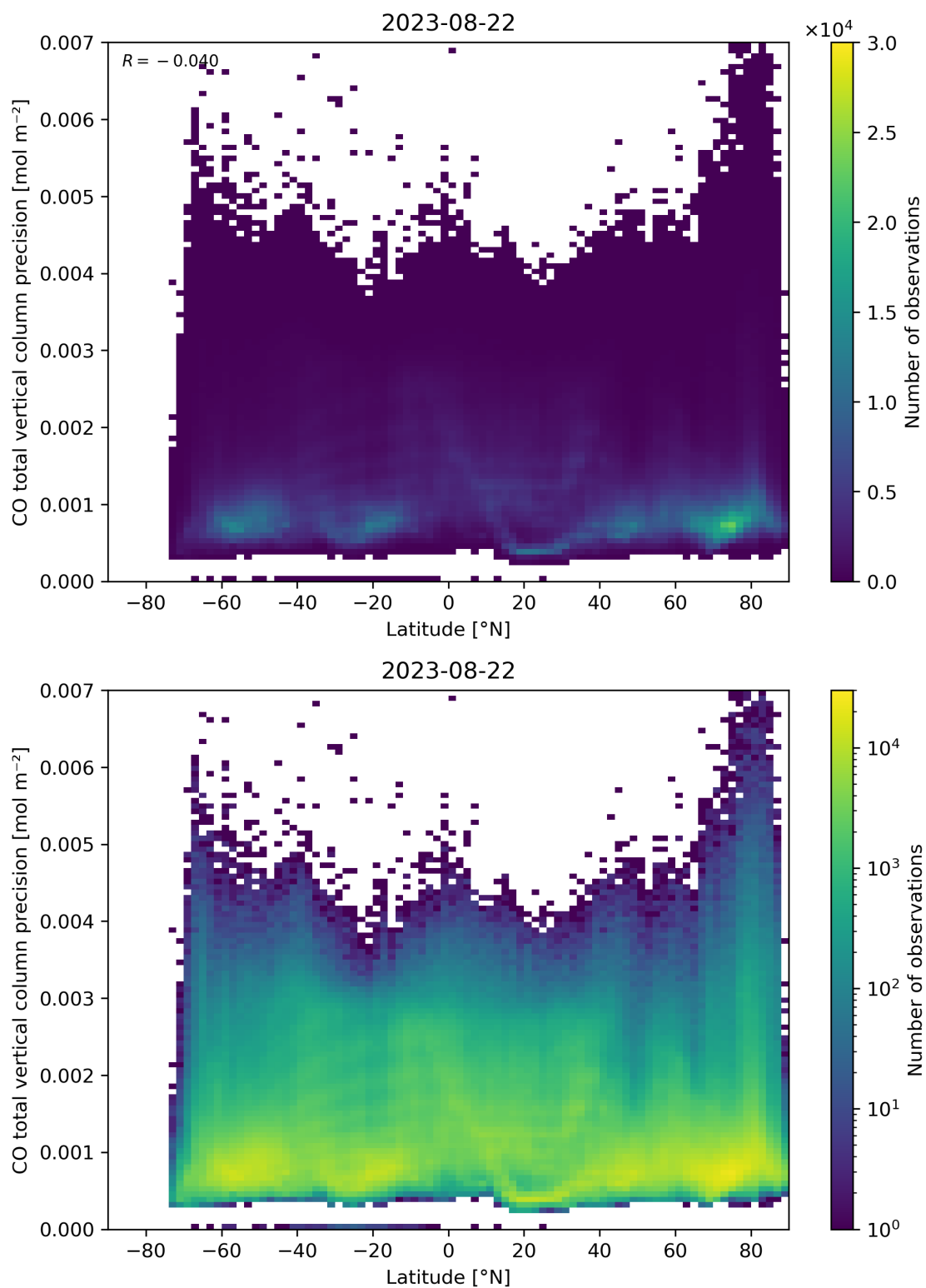
Figure 53: Scatter density plot of “Latitude” against “CO total vertical column precision” for 2023-08-21 to 2023-08-23.
