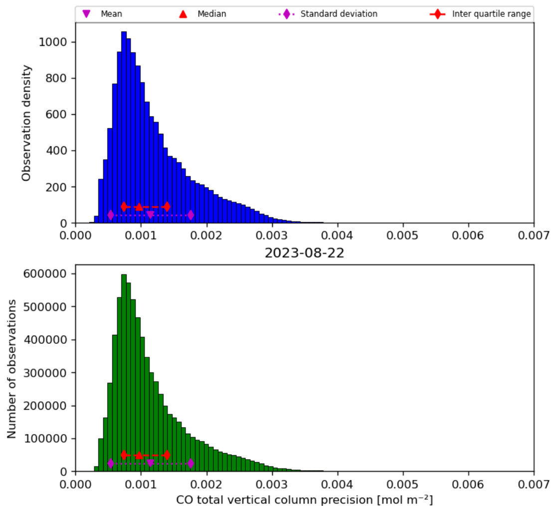
Figure 20: Histogram of “CO total vertical column precision” for 2023-08-21 to 2023-08-23
