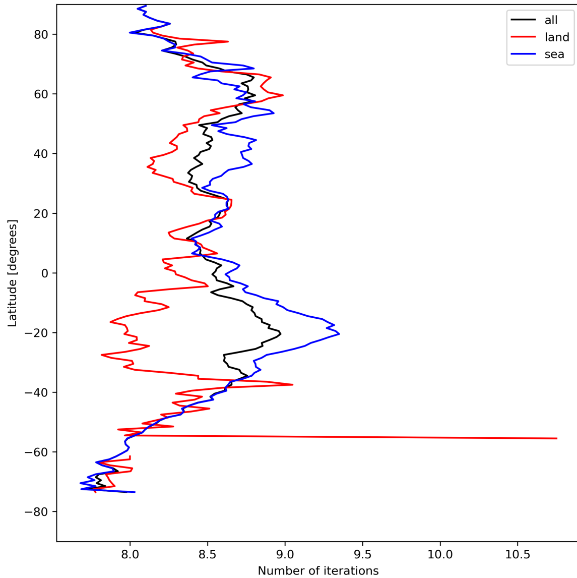
Figure 16: Zonal average of “Number of iterations” for 2023-08-21 to 2023-08-23.
