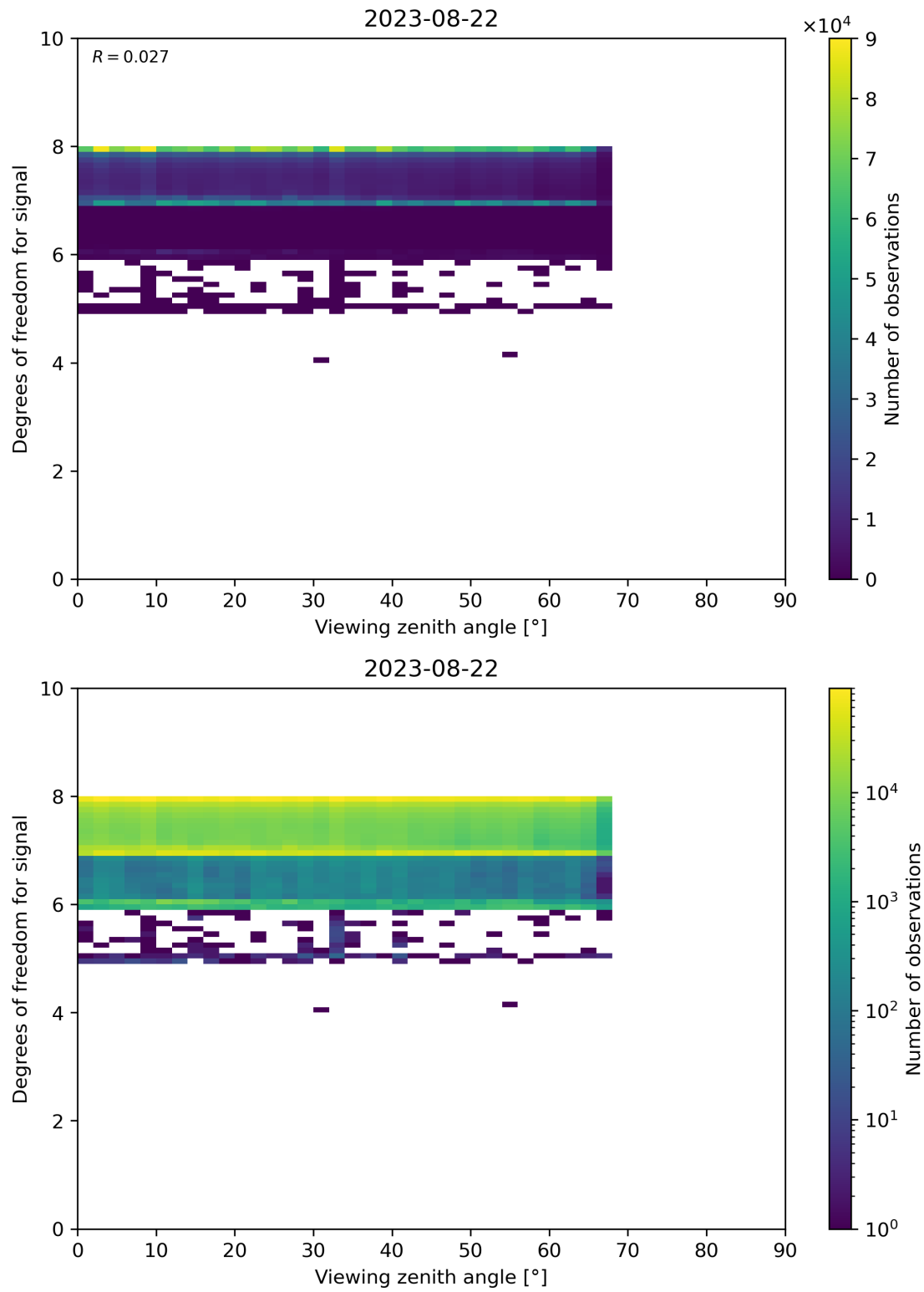
Figure 73: Scatter density plot of “Viewing zenith angle” against “Degrees of freedom for signal” for 2023-08-21 to 2023-08-23.
