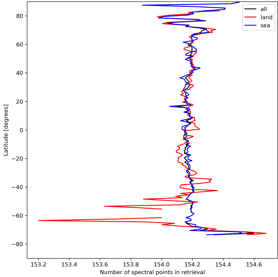
Figure 13: Zonal average of “Number of spectral points in retrieval” for 2023-08-21 to 2023-08-23.
