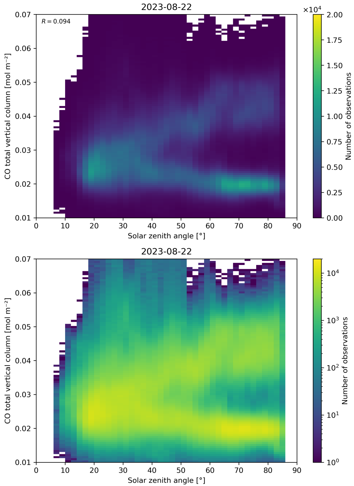
Figure 61: Scatter density plot of “Solar zenith angle” against “CO total vertical column” for 2023-08-21 to 2023-08-23.
