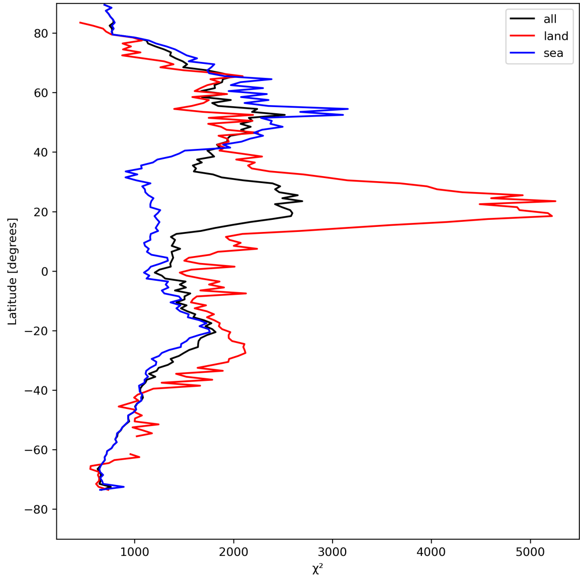
Figure 14: Zonal average of “ \chi^2 ” for 2023-08-21 to 2023-08-23.
