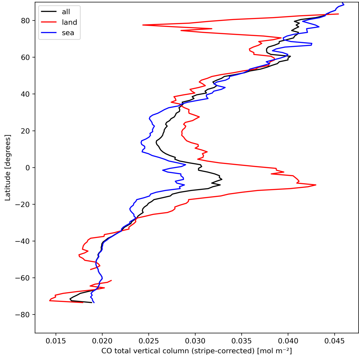
Figure 11: Zonal average of “CO total vertical column (stripe-corrected)” for 2023-08-21 to 2023-08-23.
