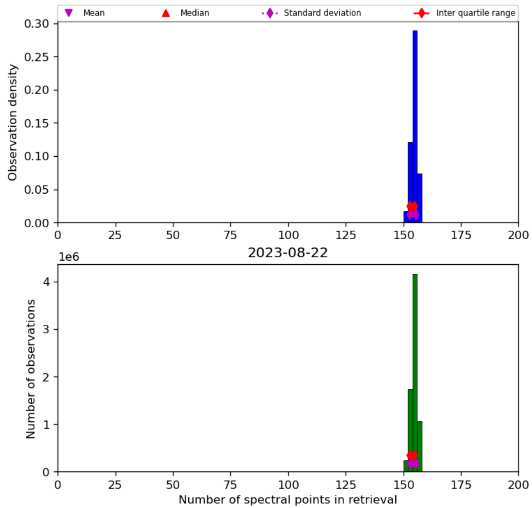
Figure 21: Histogram of “Number of spectral points in retrieval” for 2023-08-21 to 2023-08-23
