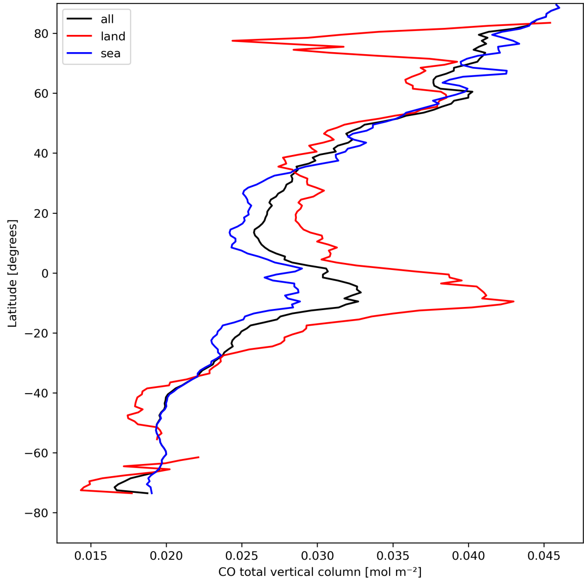
Figure 10: Zonal average of “CO total vertical column” for 2023-08-21 to 2023-08-23.
