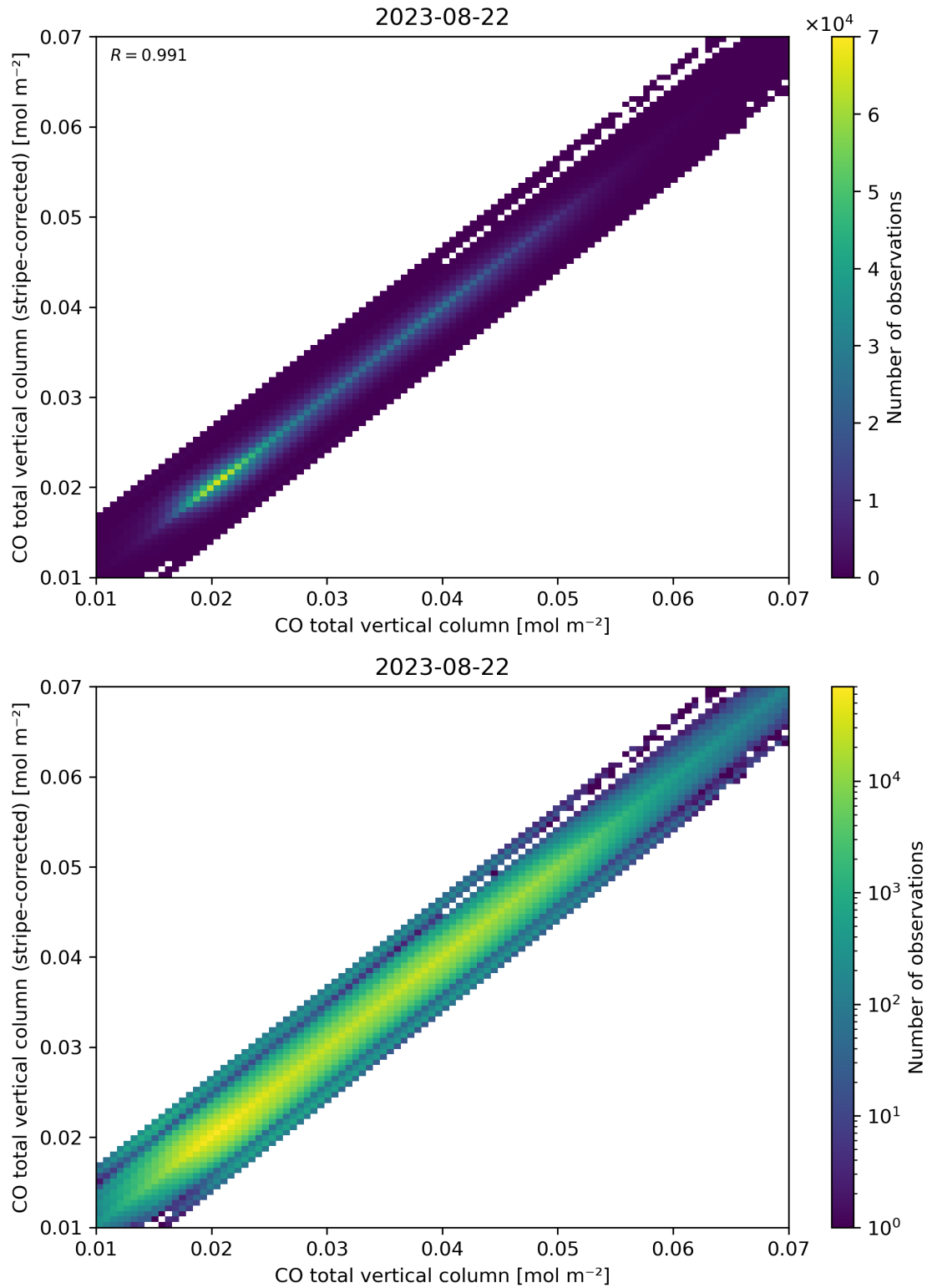
Figure 33: Scatter density plot of “CO total vertical column” against “CO total vertical column (stripe-corrected)” for 2023-08-21 to 2023-08-23.
