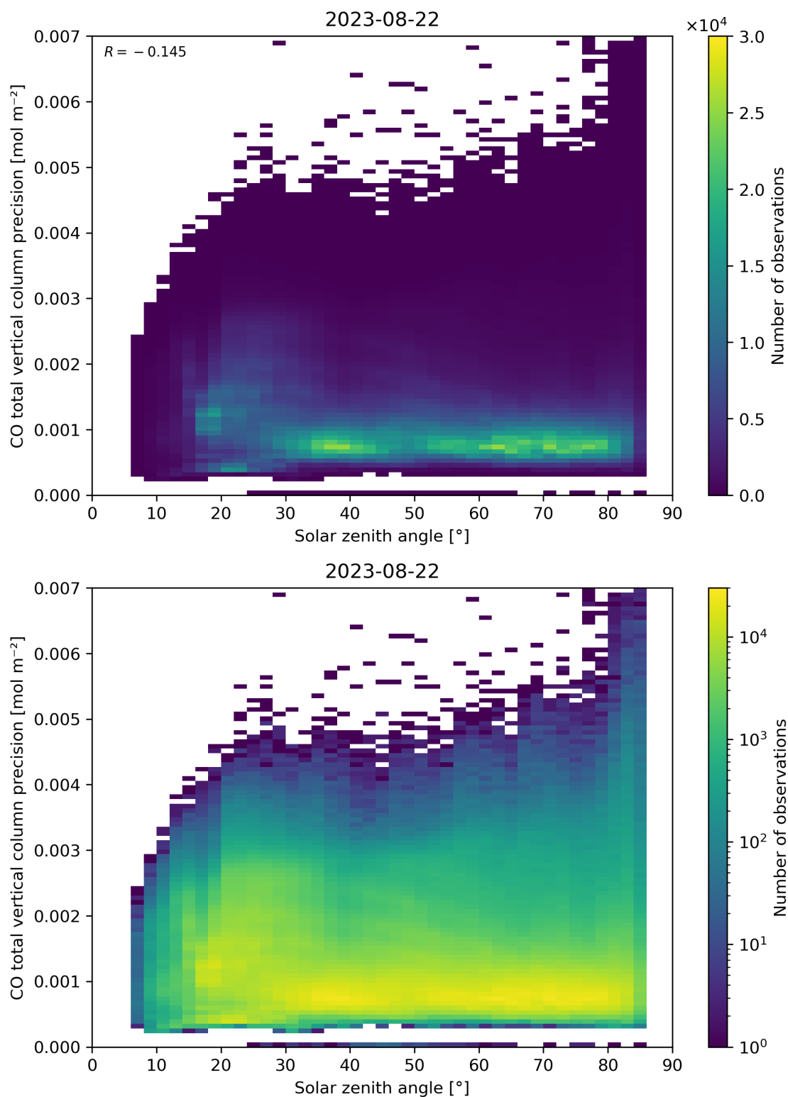
Figure 63: Scatter density plot of “Solar zenith angle” against “CO total vertical column precision” for 2023-08-21 to 2023-08-23.
