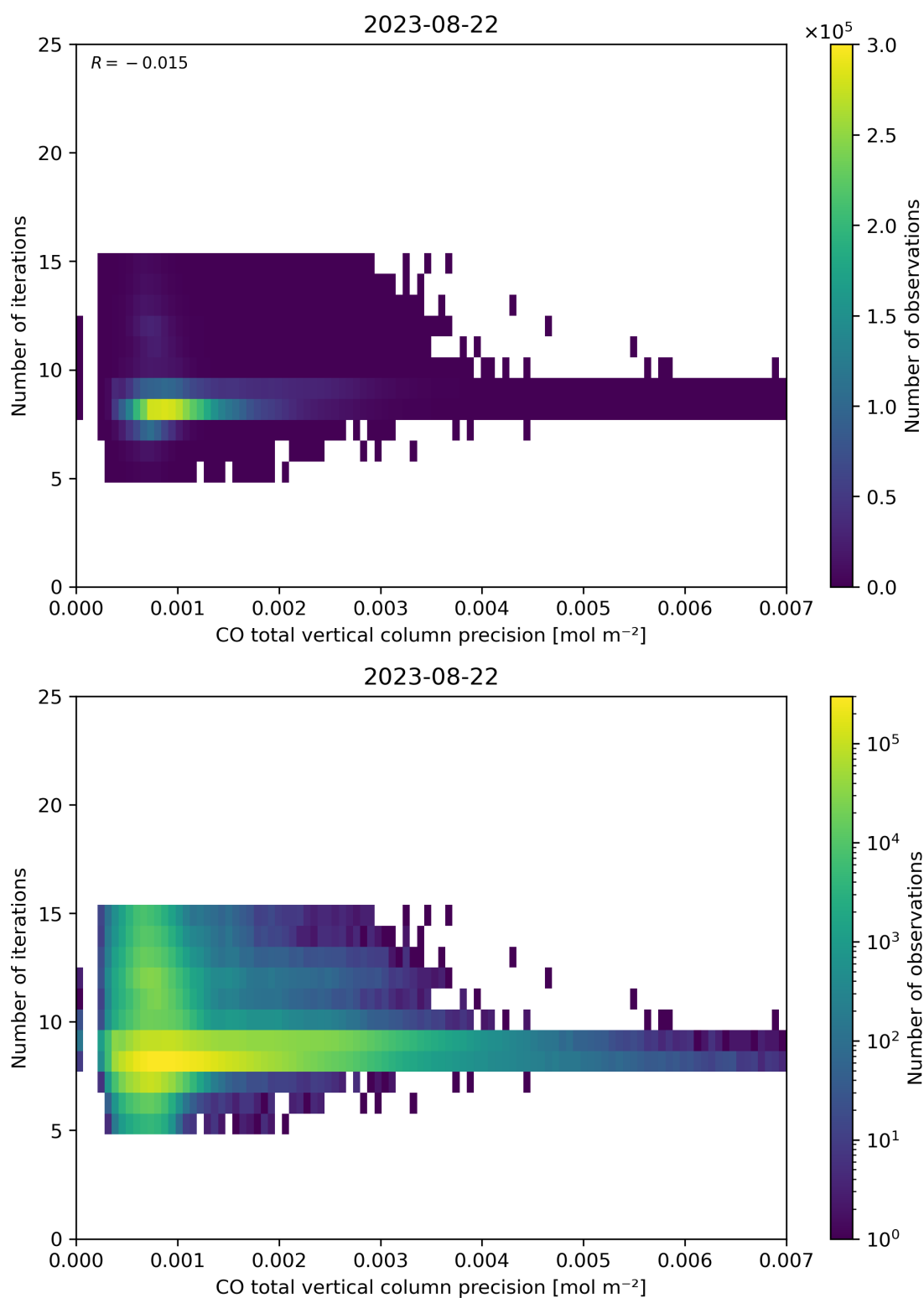
Figure 46: Scatter density plot of “CO total vertical column precision” against “Number of iterations” for 2023-08-21 to 2023-08-23.
