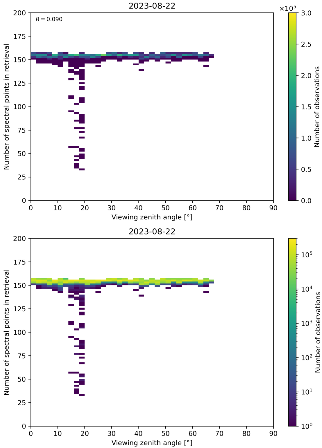
Figure 76: Scatter density plot of “Viewing zenith angle” against “Number of spectral points in retrieval” for 2023-08-21 to 2023-08-23.
