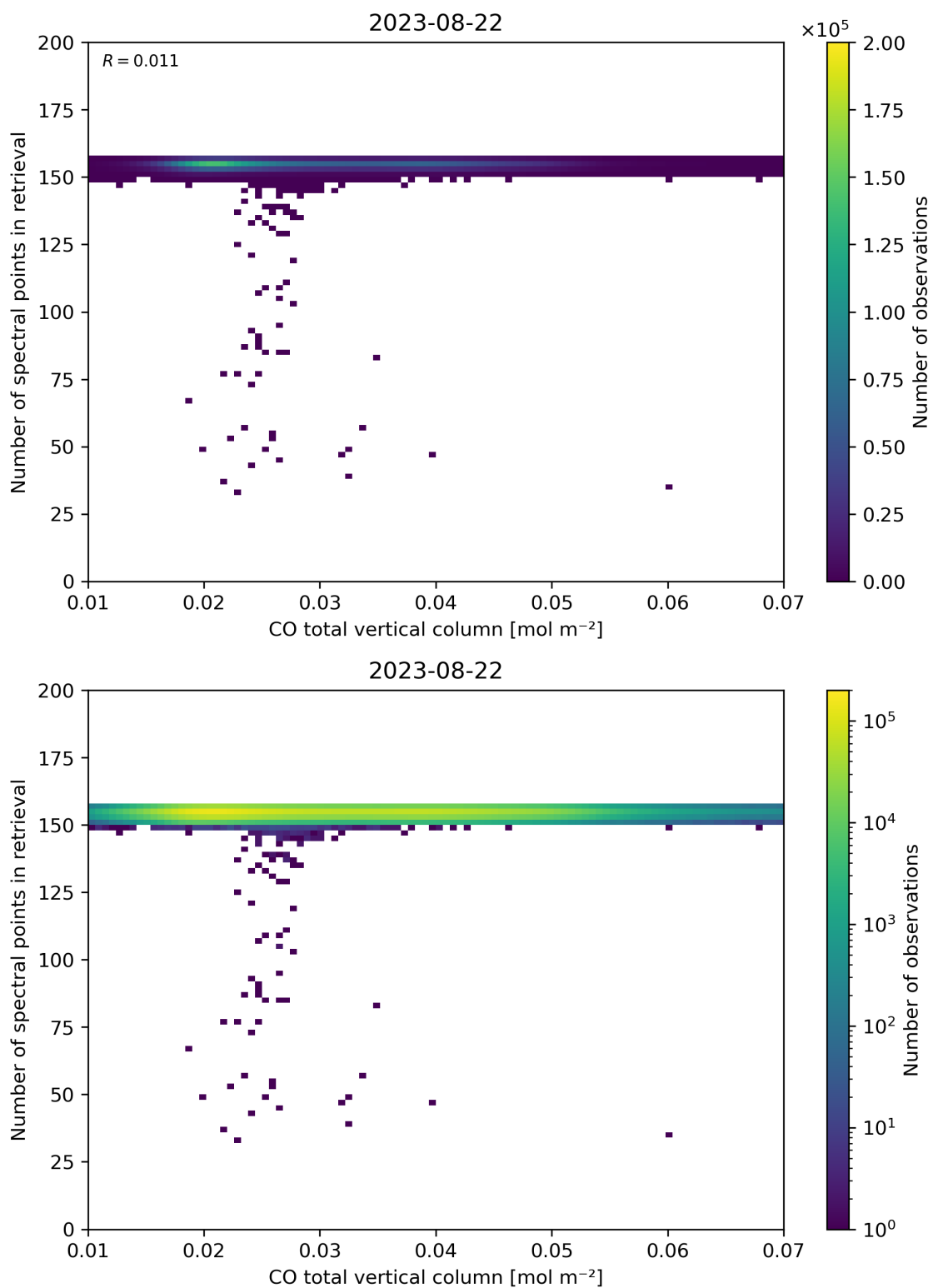
Figure 43: Scatter density plot of “CO total vertical column” against “Number of spectral points in retrieval” for 2023-08-21 to 2023-08-23.
