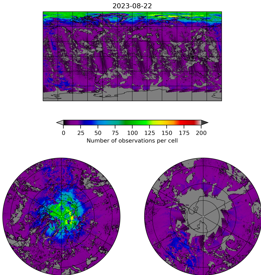
Figure 8: Map of the number of observations for 2023-08-21 to 2023-08-23
