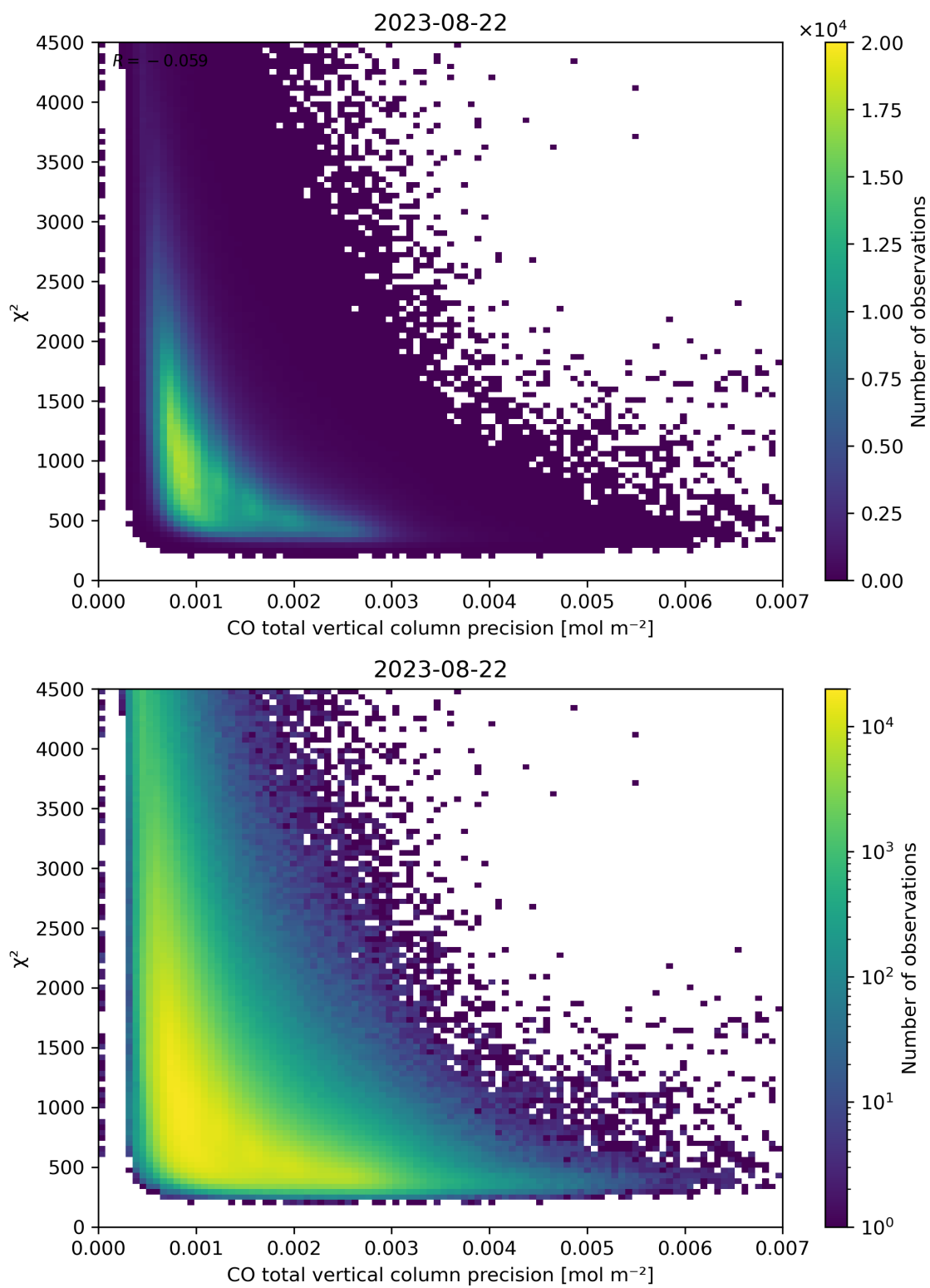
Figure 44: Scatter density plot of “CO total vertical column precision” against “ \chi^2 ” for 2023-08-21 to 2023-08-23.
