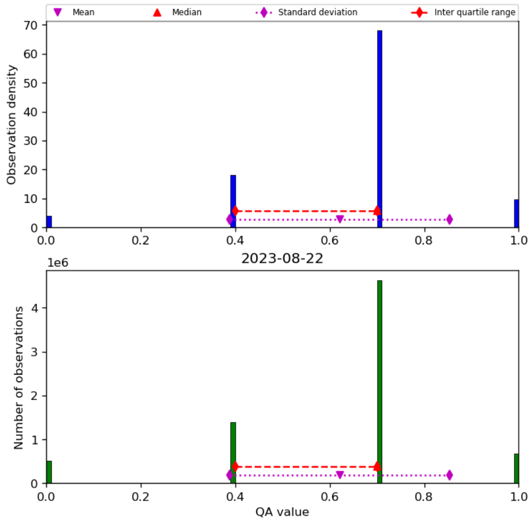
Figure 17: Histogram of “QA value” for 2023-08-21 to 2023-08-23
