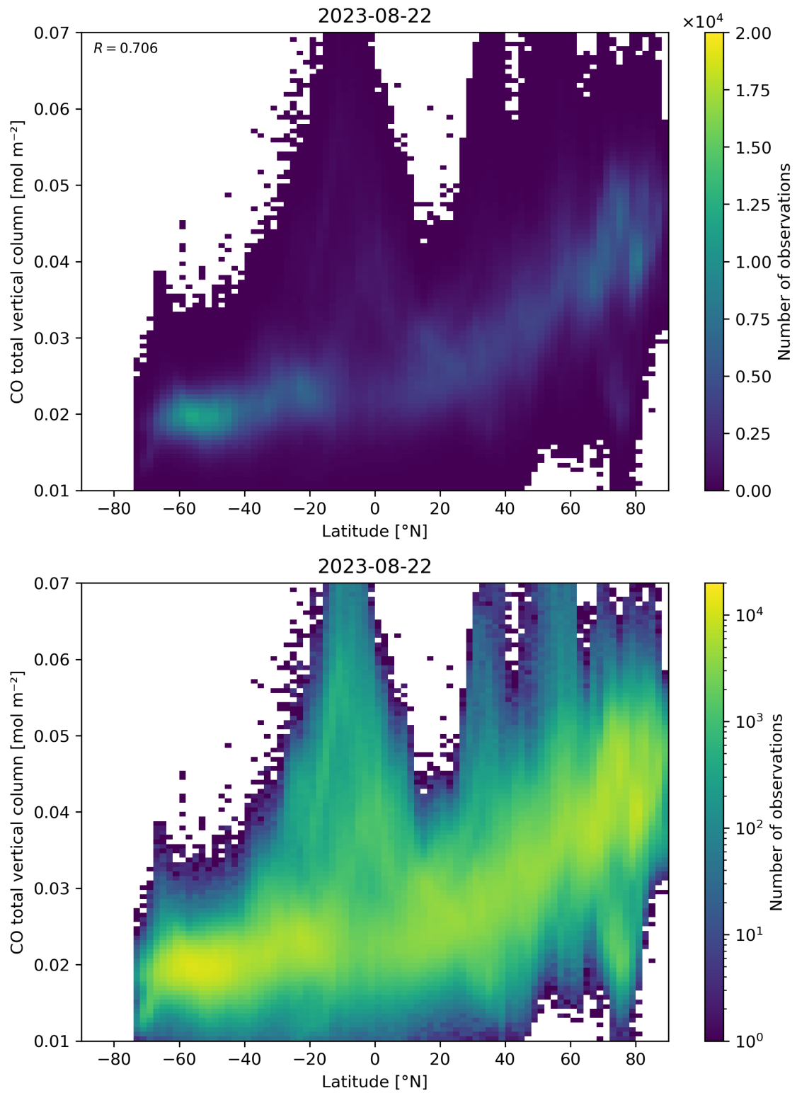
Figure 51: Scatter density plot of “Latitude” against “CO total vertical column” for 2023-08-21 to 2023-08-23.
