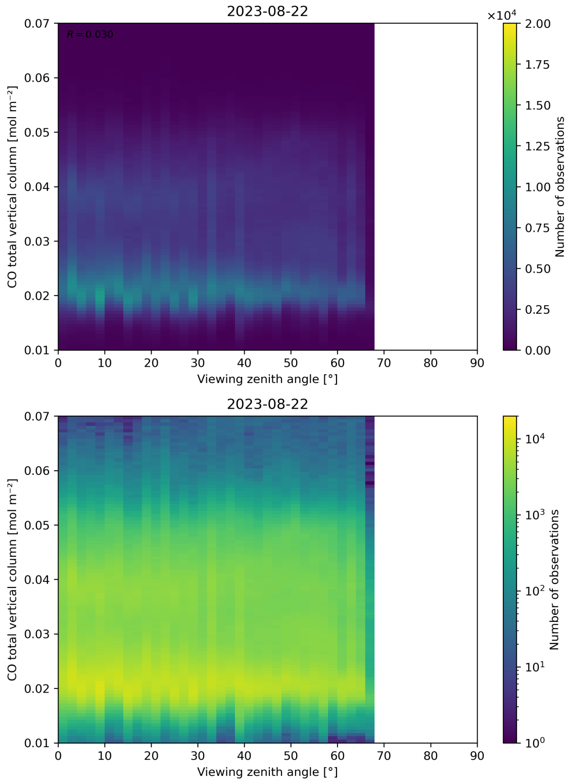
Figure 69: Scatter density plot of “Viewing zenith angle” against “CO total vertical column” for 2023-08-21 to 2023-08-23.
