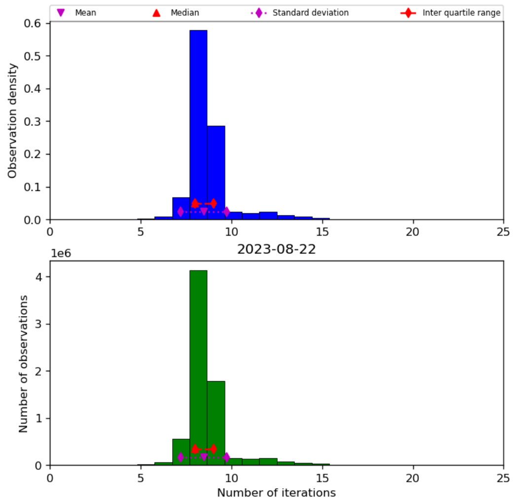
Figure 24: Histogram of “Number of iterations” for 2023-08-21 to 2023-08-23
