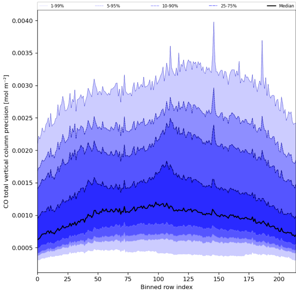
Figure 28: Along track statistics of “CO total vertical column precision” for 2023-08-21 to 2023-08-23
