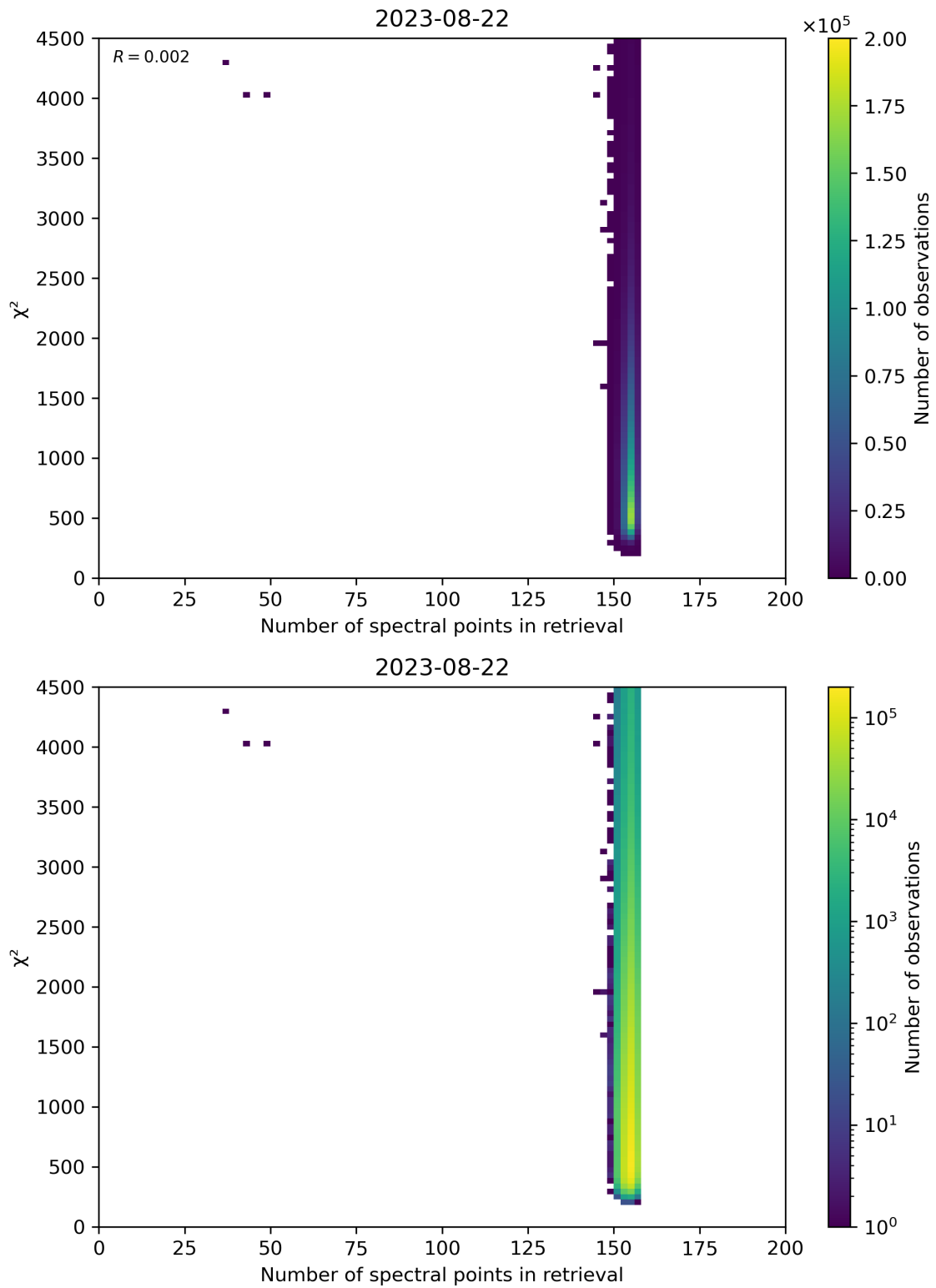
Figure 58: Scatter density plot of “Number of spectral points in retrieval” against “ \chi^2 ” for 2023-08-21 to 2023-08-23.
