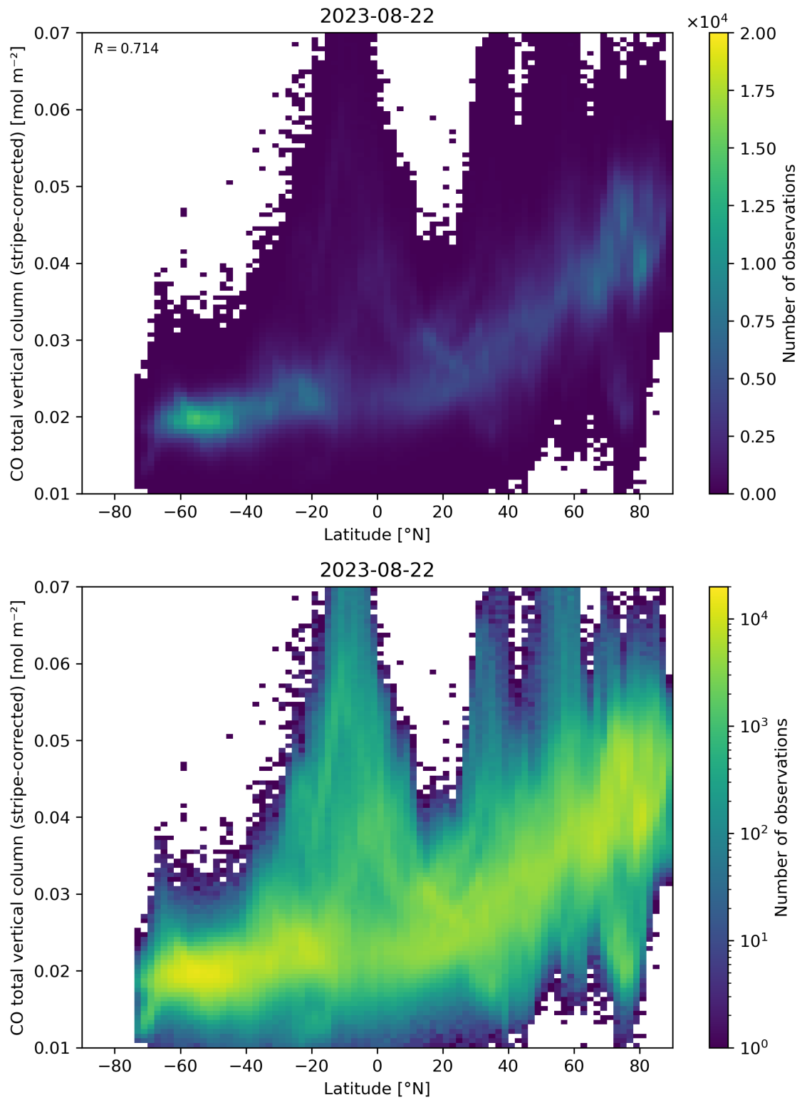
Figure 52: Scatter density plot of “Latitude” against “CO total vertical column (stripe-corrected)” for 2023-08-21 to 2023-08-23.
