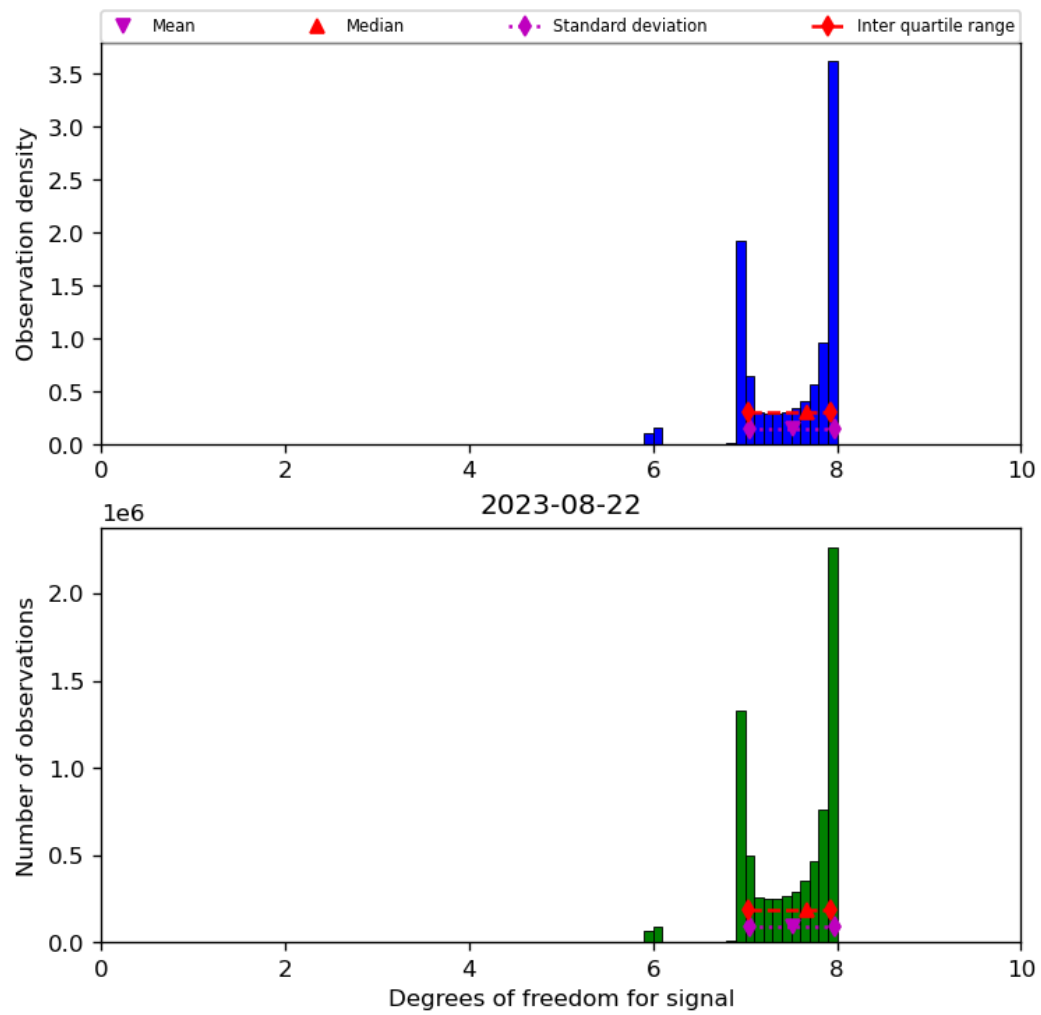
Figure 23: Histogram of “Degrees of freedom for signal” for 2023-08-21 to 2023-08-23
