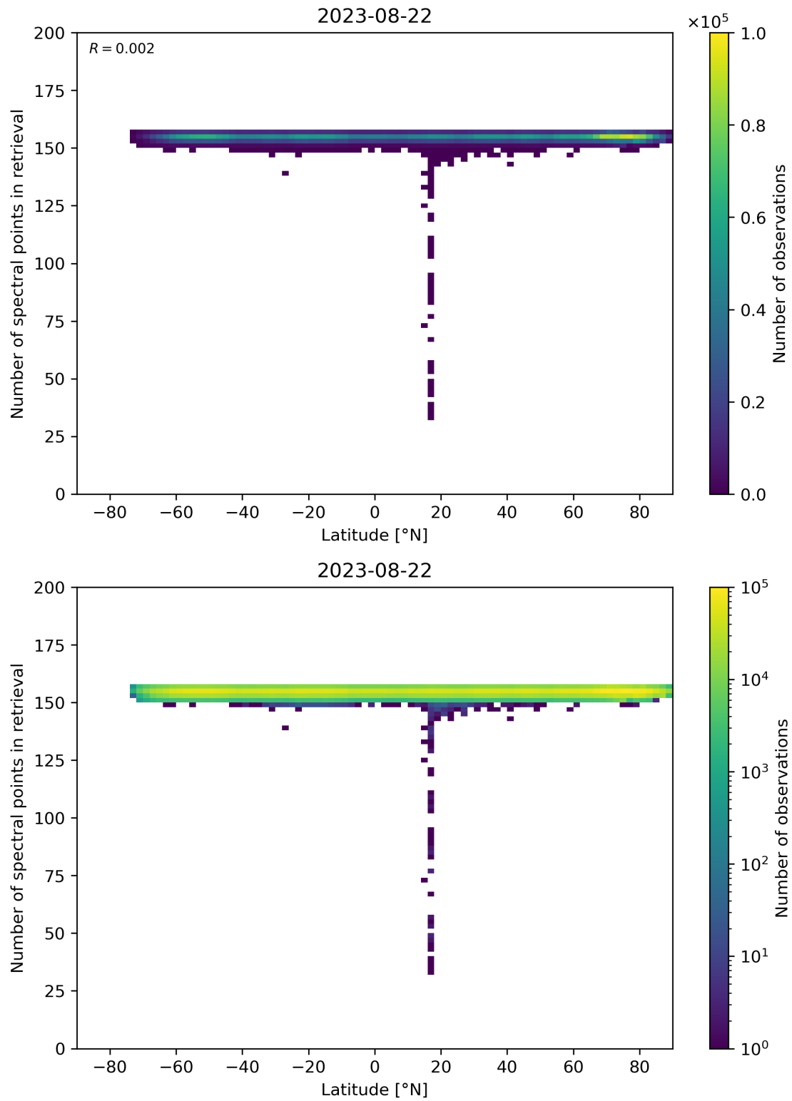
Figure 57: Scatter density plot of “Latitude” against “Number of spectral points in retrieval” for 2023-08-21 to 2023-08-23.
