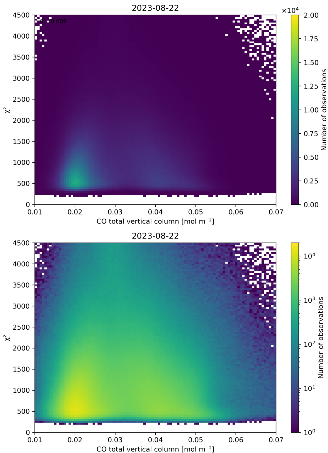
Figure 35: Scatter density plot of “CO total vertical column” against “ \chi^2 ” for 2023-08-21 to 2023-08-23.
