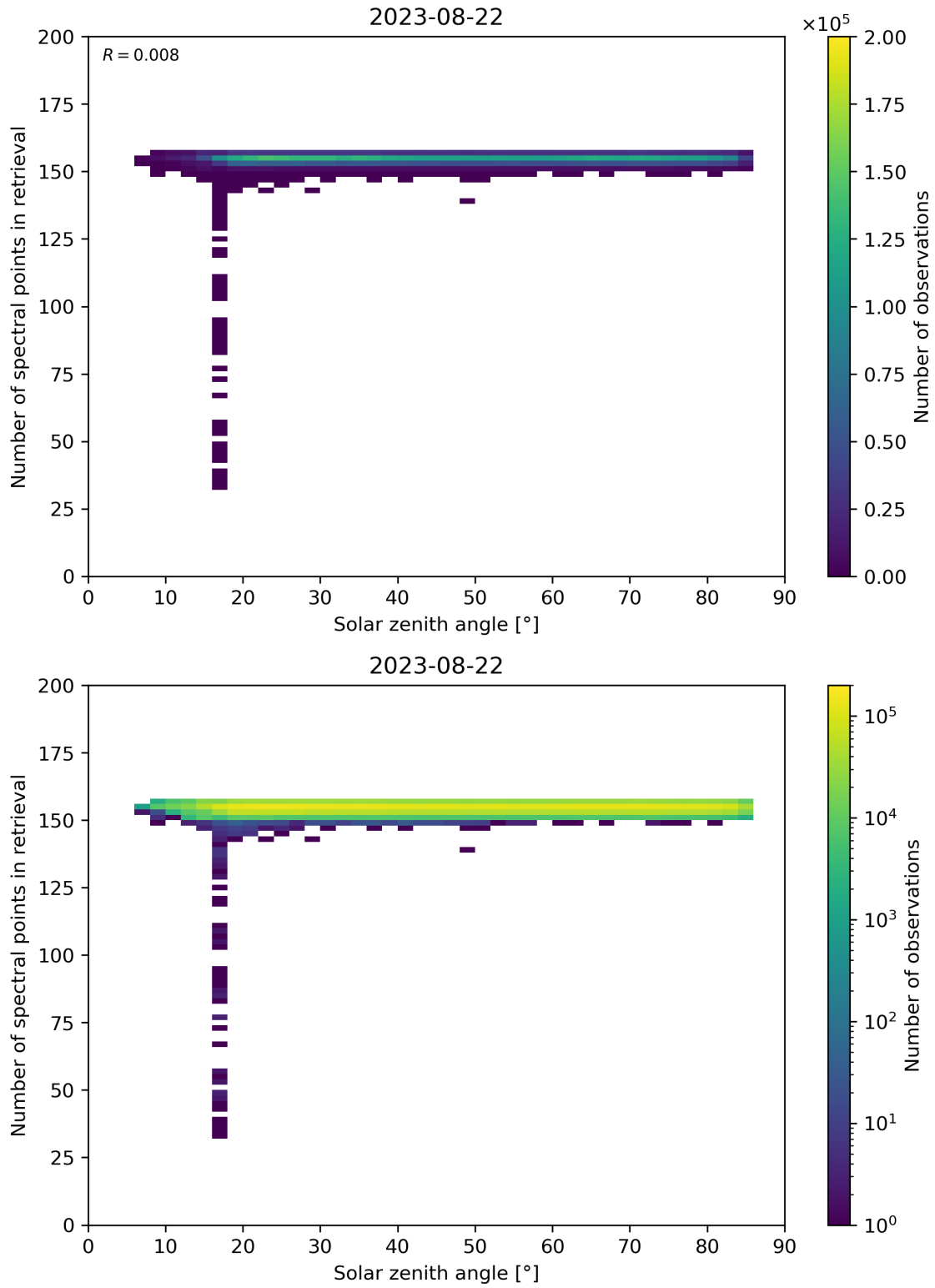
Figure 68: Scatter density plot of “Solar zenith angle” against “Number of spectral points in retrieval” for 2023-08-21 to 2023-08-23.
