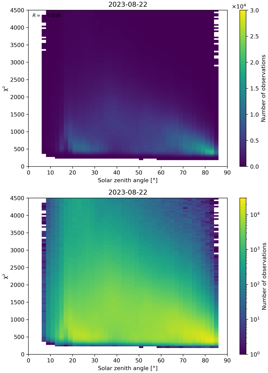
Figure 64: Scatter density plot of “Solar zenith angle” against “ \chi^2 ” for 2023-08-21 to 2023-08-23.
