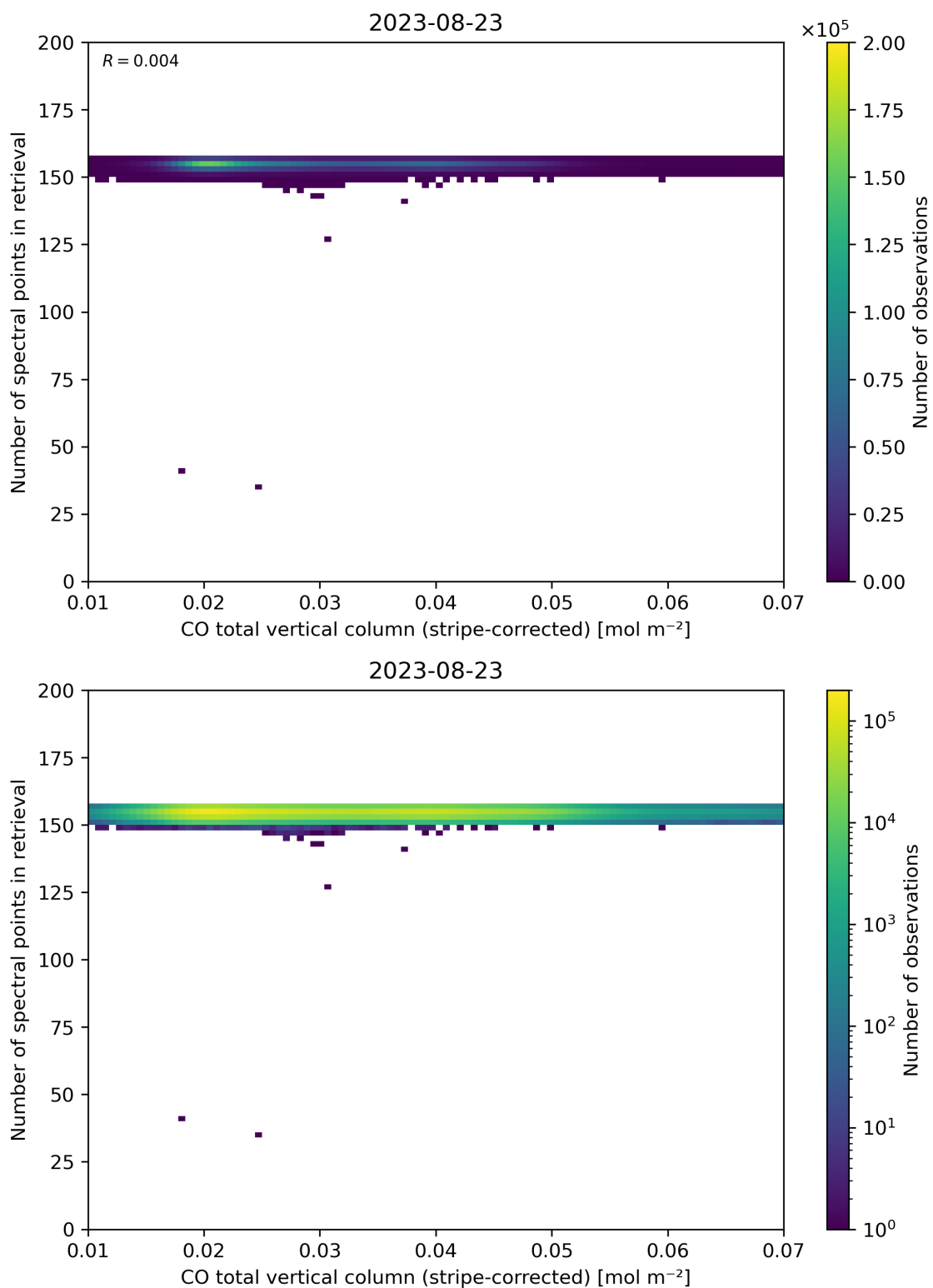
Figure 40: Scatter density plot of “CO total vertical column (stripe-corrected)” against “Number of spectral points in retrieval” for 2023-08-22 to 2023-08-24.
