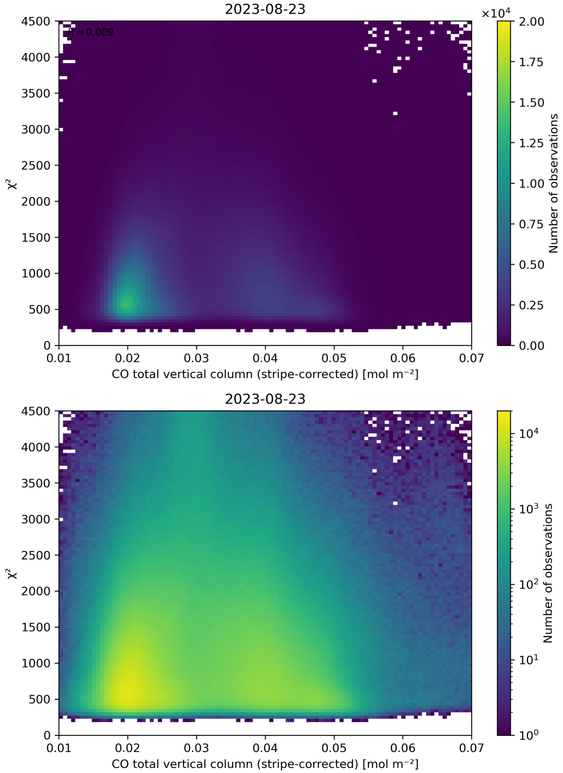
Figure 37: Scatter density plot of “CO total vertical column (stripe-corrected)” against “ \chi^2 ” for 2023-08-22 to 2023-08-24.
