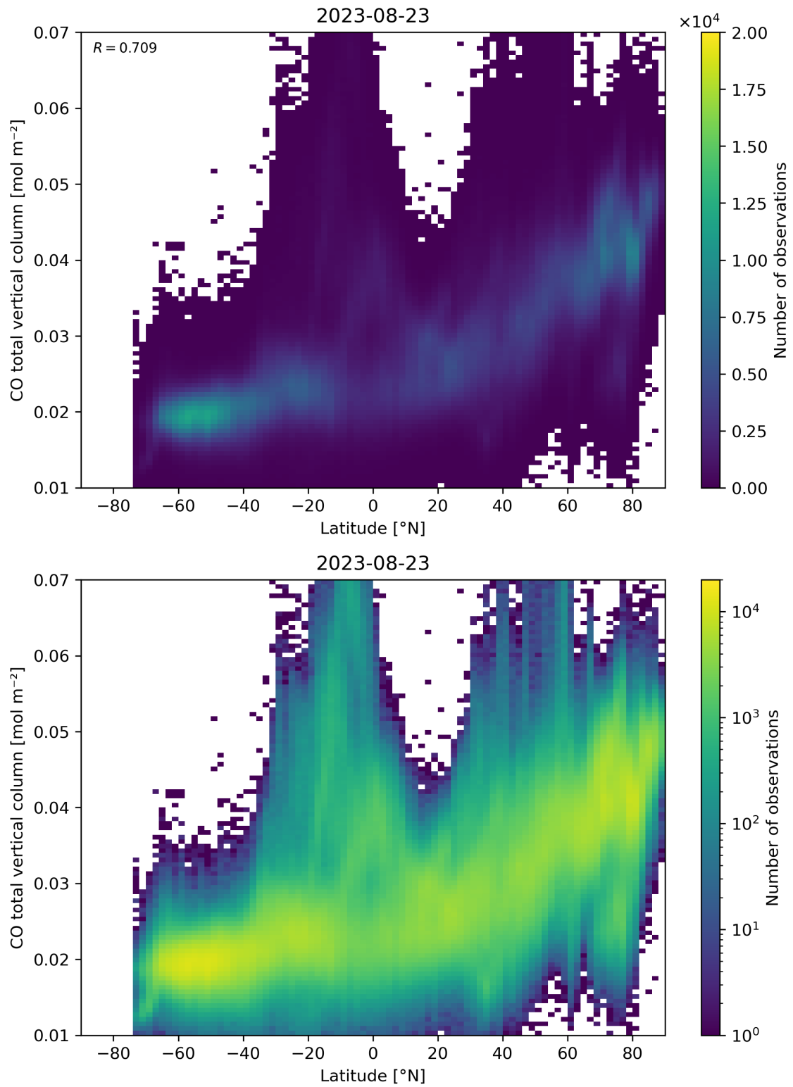
Figure 51: Scatter density plot of “Latitude” against “CO total vertical column” for 2023-08-22 to 2023-08-24.
