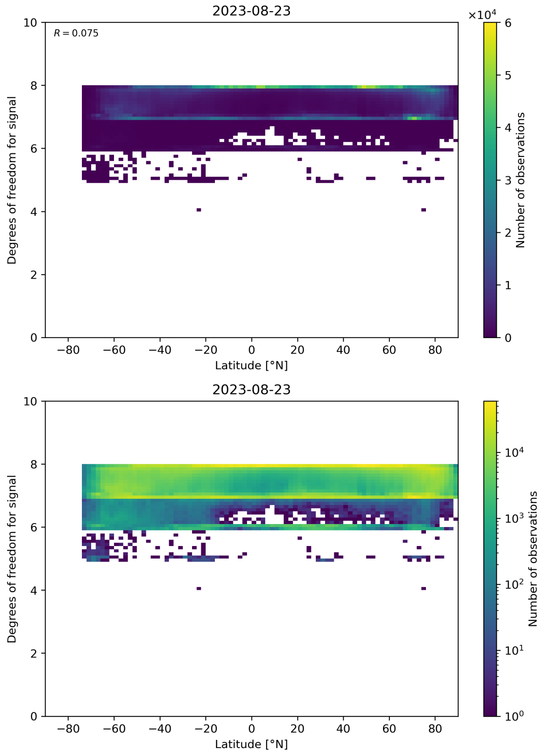
Figure 55: Scatter density plot of “Latitude” against “Degrees of freedom for signal” for 2023-08-22 to 2023-08-24.
