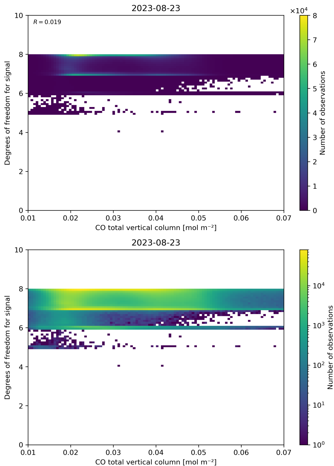
Figure 41: Scatter density plot of “CO total vertical column” against “Degrees of freedom for signal” for 2023-08-22 to 2023-08-24.
