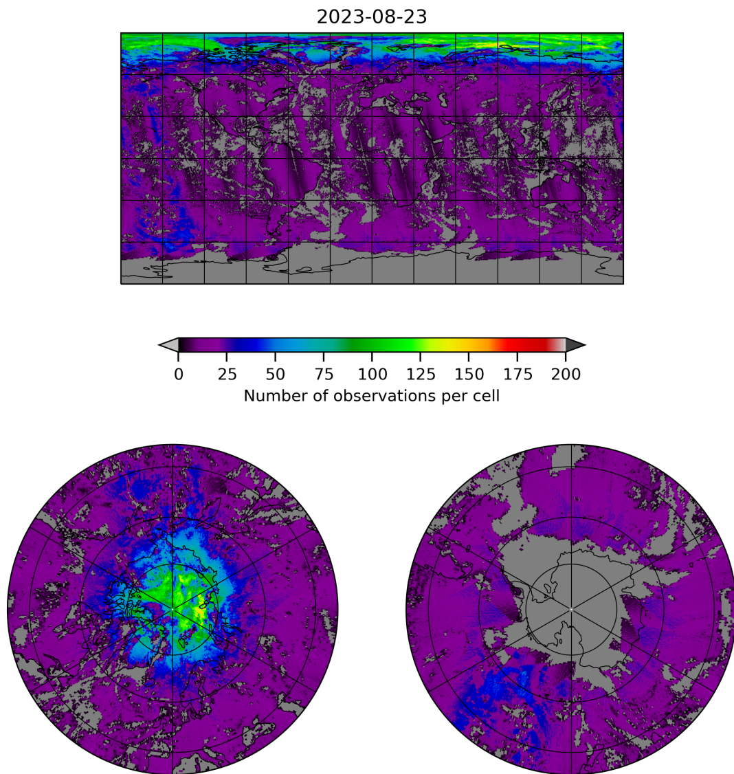
Figure 8: Map of the number of observations for 2023-08-22 to 2023-08-24
