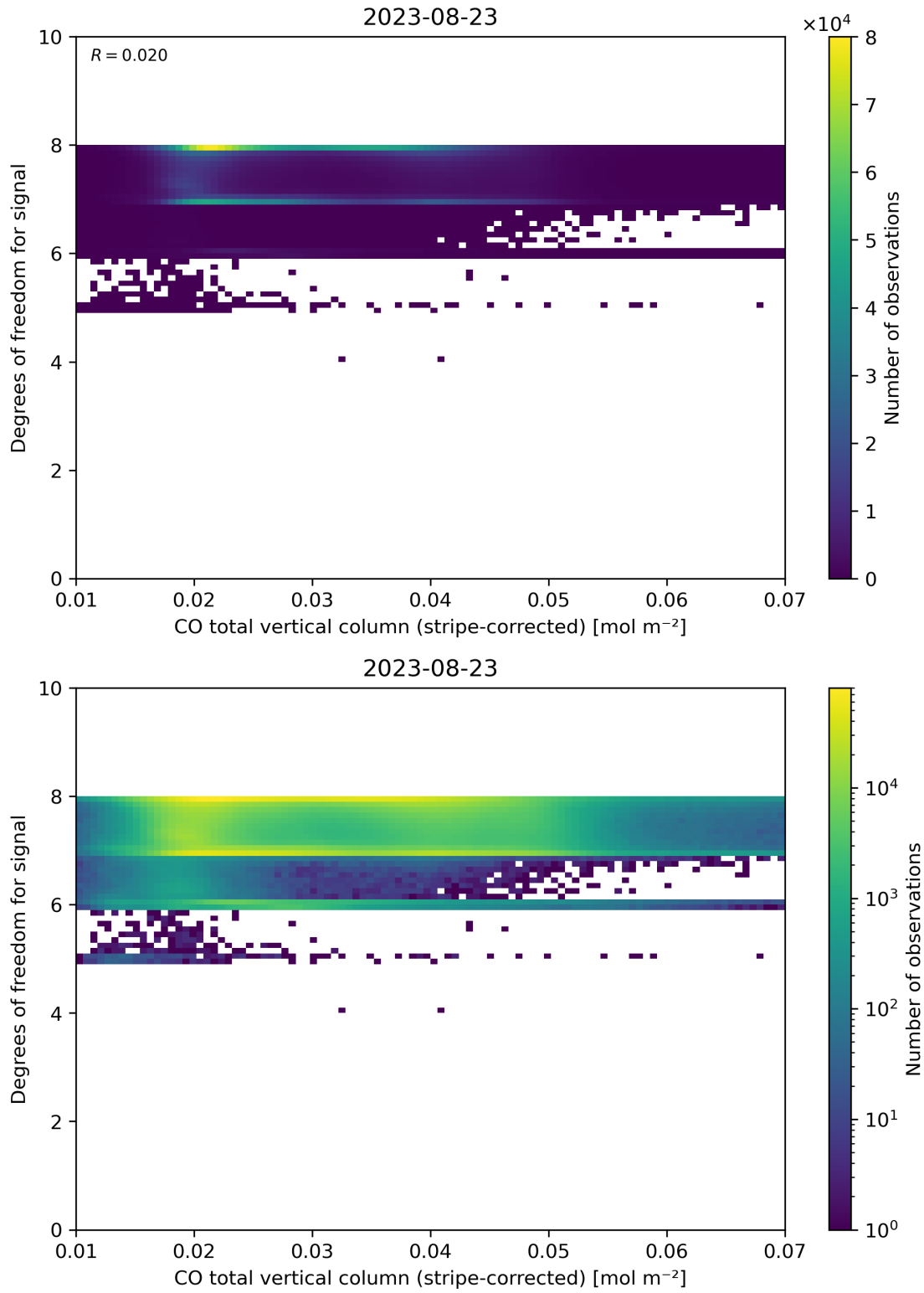
Figure 38: Scatter density plot of “CO total vertical column (stripe-corrected)” against “Degrees of freedom for signal” for 2023-08-22 to 2023-08-24.
