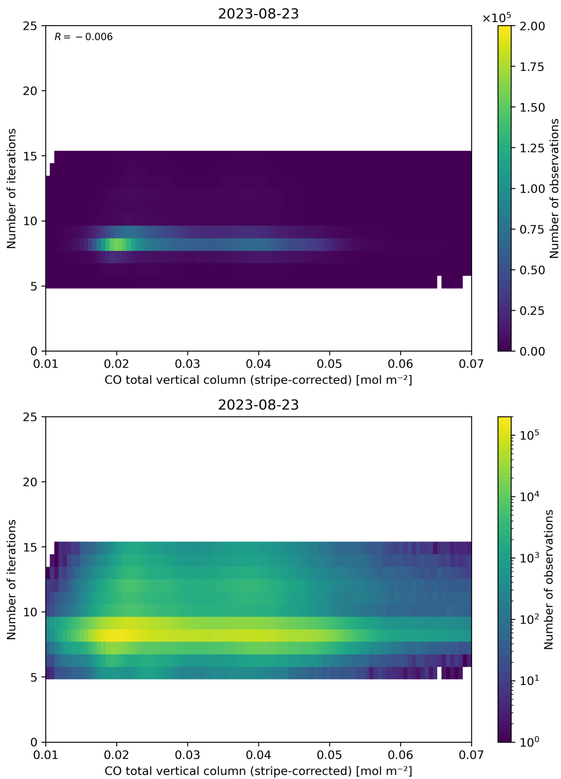
Figure 39: Scatter density plot of “CO total vertical column (stripe-corrected)” against “Number of iterations” for 2023-08-22 to 2023-08-24.
