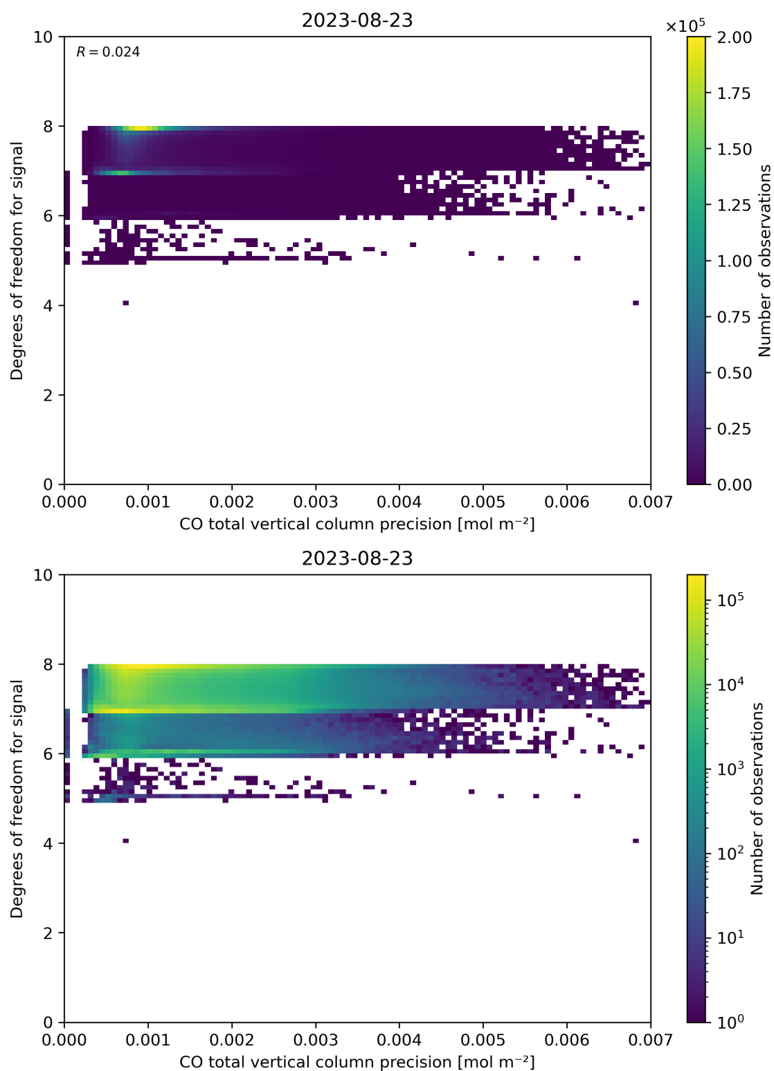
Figure 45: Scatter density plot of “CO total vertical column precision” against “Degrees of freedom for signal” for 2023-08-22 to 2023-08-24.
