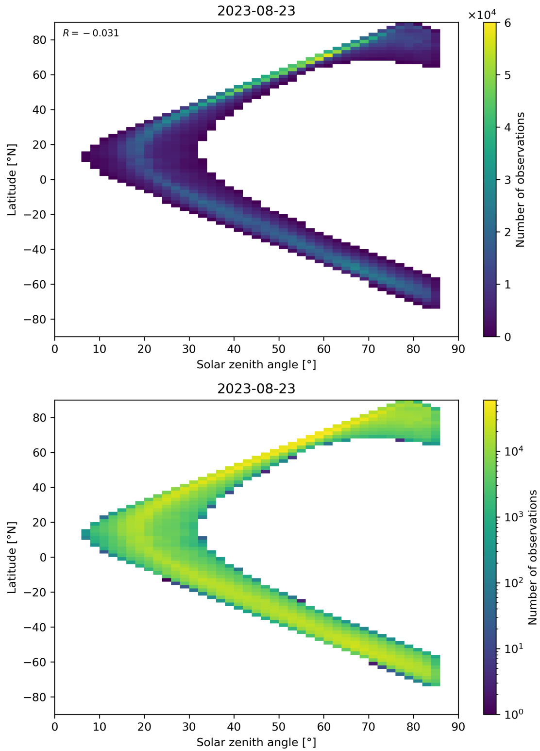
Figure 66: Scatter density plot of “Solar zenith angle” against “Latitude” for 2023-08-22 to 2023-08-24.
