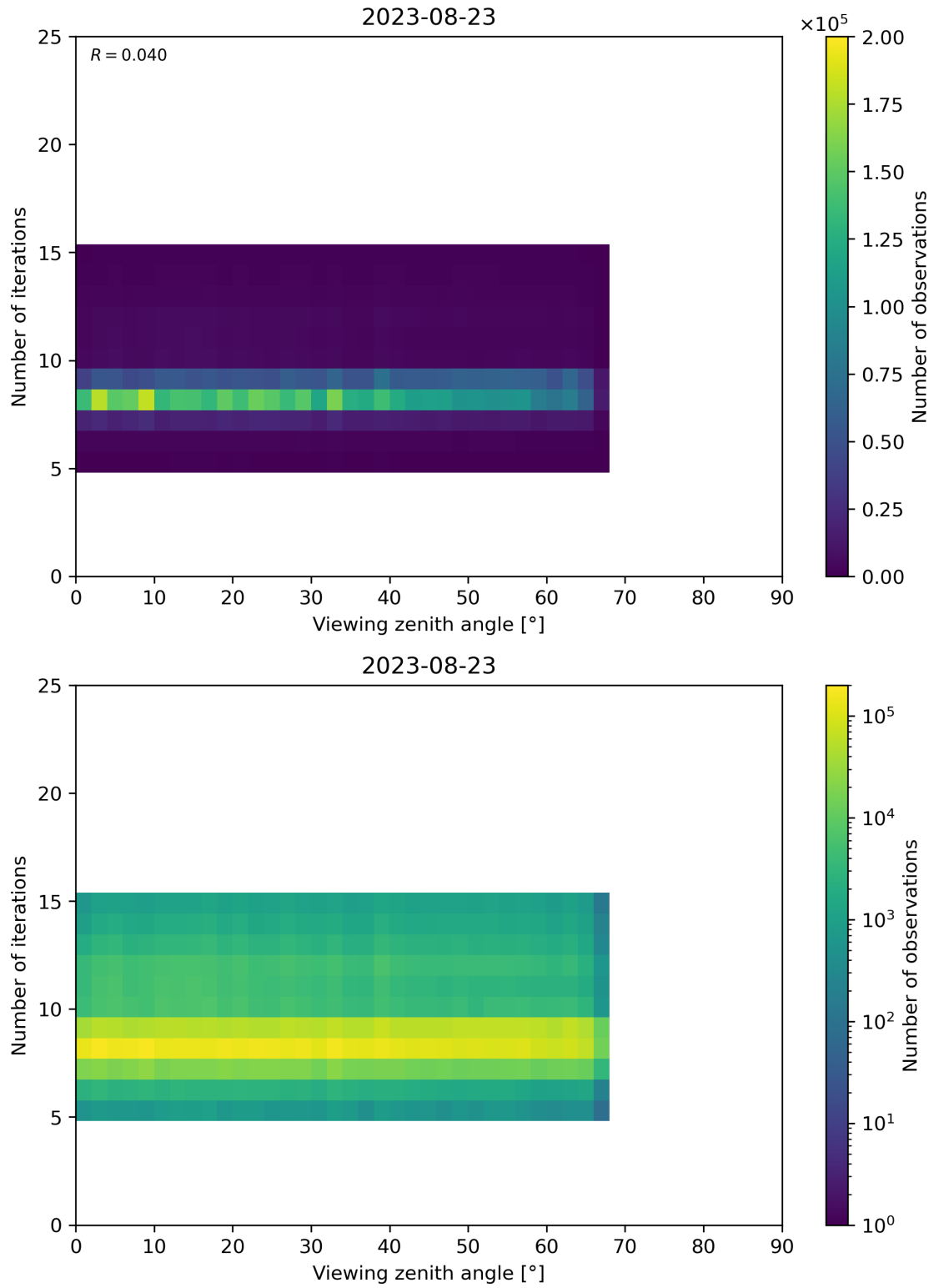
Figure 75: Scatter density plot of “Viewing zenith angle” against “Number of iterations” for 2023-08-22 to 2023-08-24.
