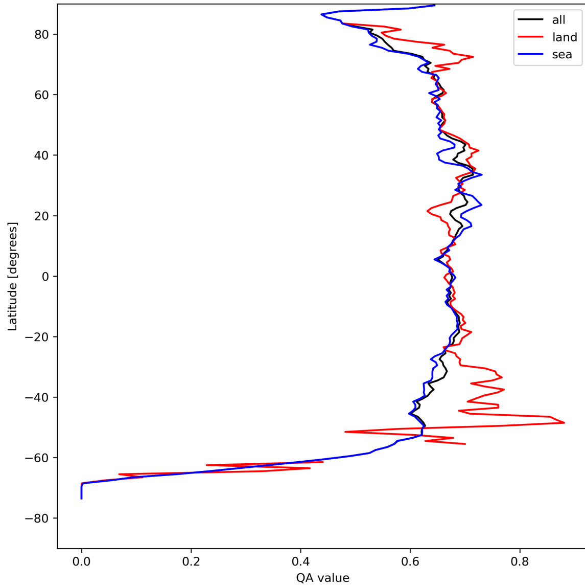
Figure 9: Zonal average of “QA value” for 2023-08-22 to 2023-08-24.
