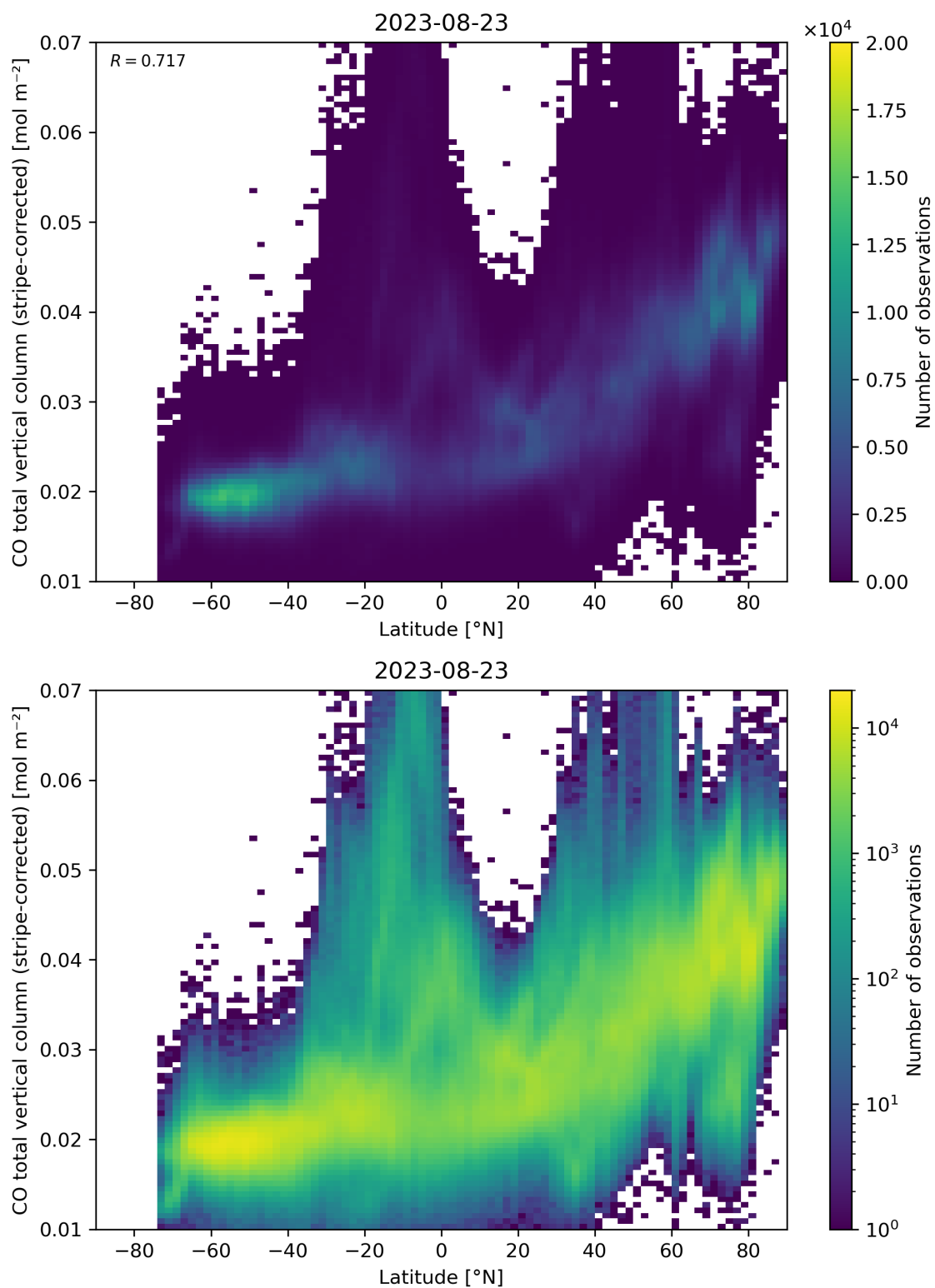
Figure 52: Scatter density plot of “Latitude” against “CO total vertical column (stripe-corrected)” for 2023-08-22 to 2023-08-24.
