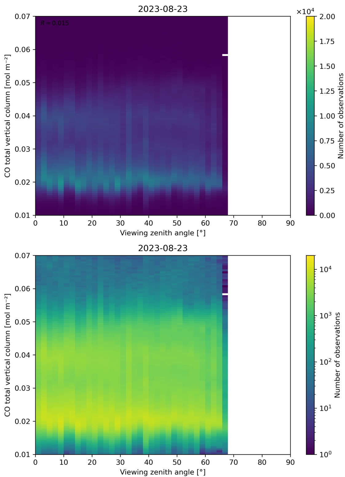
Figure 69: Scatter density plot of “Viewing zenith angle” against “CO total vertical column” for 2023-08-22 to 2023-08-24.
