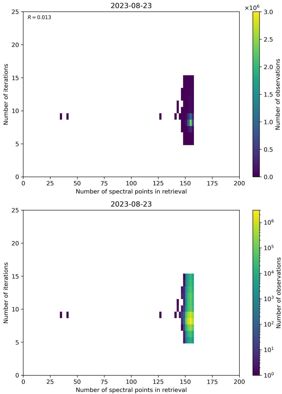
Figure 60: Scatter density plot of “Number of spectral points in retrieval” against “Number of iterations” for 2023-08-22 to 2023-08-24.
