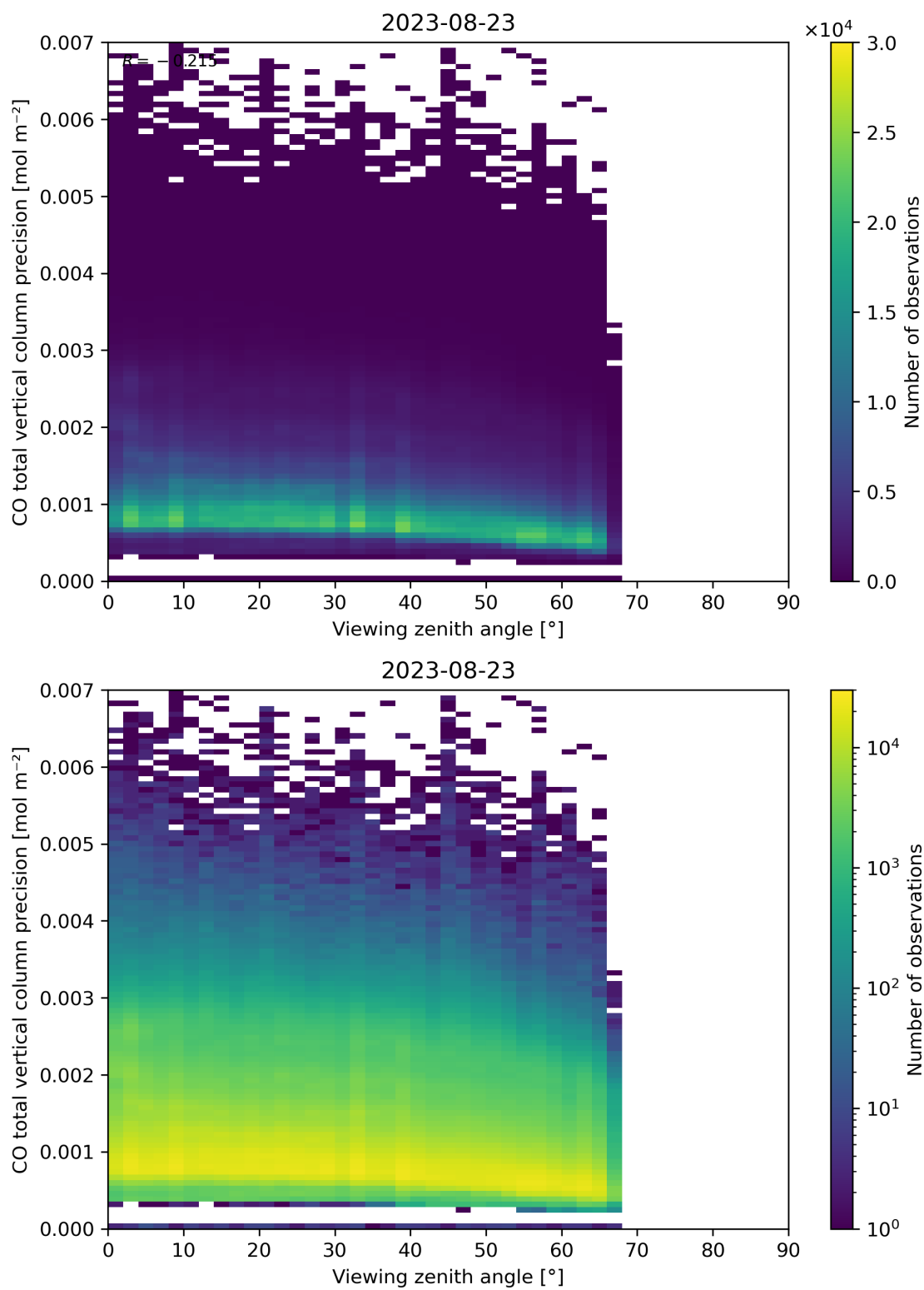
Figure 71: Scatter density plot of “Viewing zenith angle” against “CO total vertical column precision” for 2023-08-22 to 2023-08-24.
