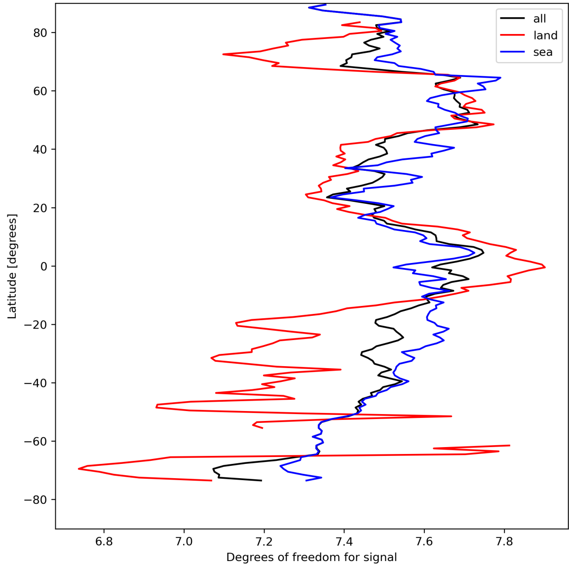
Figure 15: Zonal average of “Degrees of freedom for signal” for 2023-08-22 to 2023-08-24.
