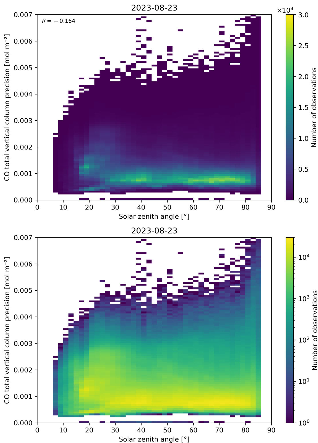
Figure 63: Scatter density plot of “Solar zenith angle” against “CO total vertical column precision” for 2023-08-22 to 2023-08-24.
