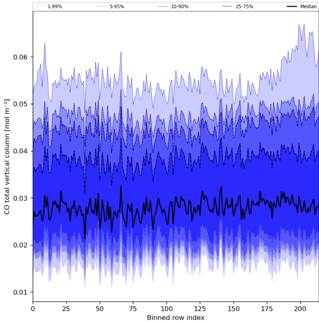
Figure 26: Along track statistics of “CO total vertical column” for 2023-08-22 to 2023-08-24
