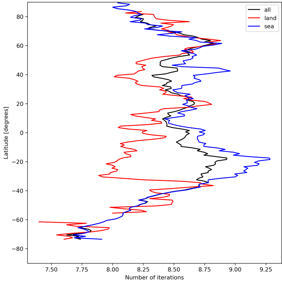
Figure 16: Zonal average of “Number of iterations” for 2023-08-22 to 2023-08-24.
