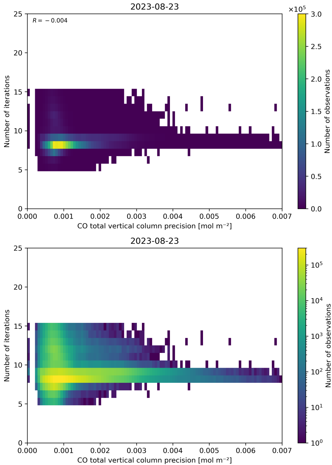
Figure 46: Scatter density plot of “CO total vertical column precision” against “Number of iterations” for 2023-08-22 to 2023-08-24.
