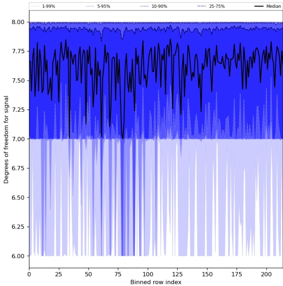
Figure 31: Along track statistics of “Degrees of freedom for signal” for 2023-08-22 to 2023-08-24
