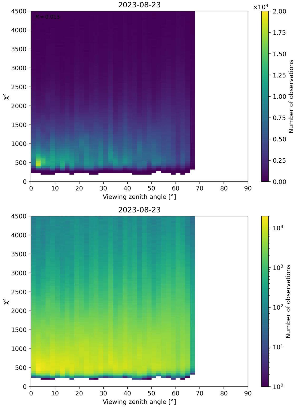
Figure 72: Scatter density plot of “Viewing zenith angle” against “ \chi^2 ” for 2023-08-22 to 2023-08-24.
