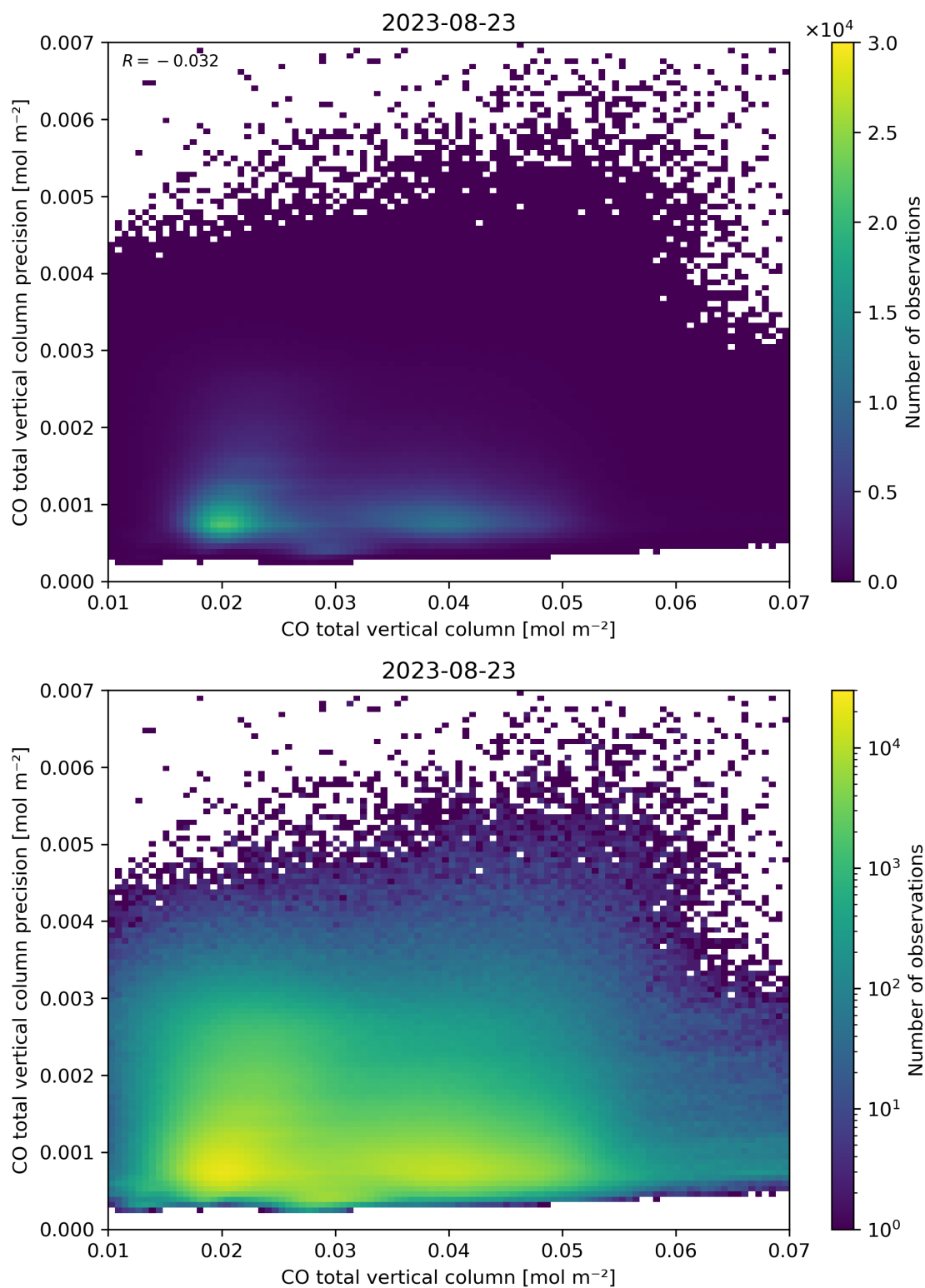
Figure 34: Scatter density plot of “CO total vertical column” against “CO total vertical column precision” for 2023-08-22 to 2023-08-24.
