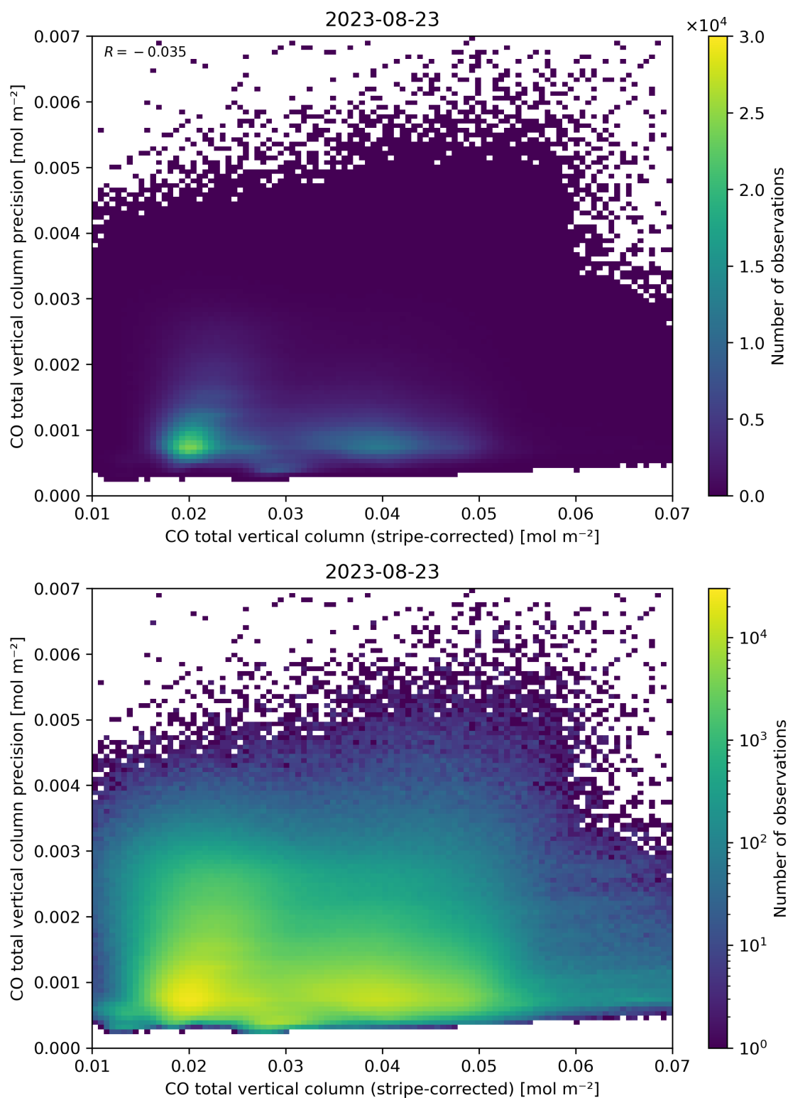
Figure 36: Scatter density plot of “CO total vertical column (stripe-corrected)” against “CO total vertical column precision” for 2023-08-22 to 2023-08-24.
