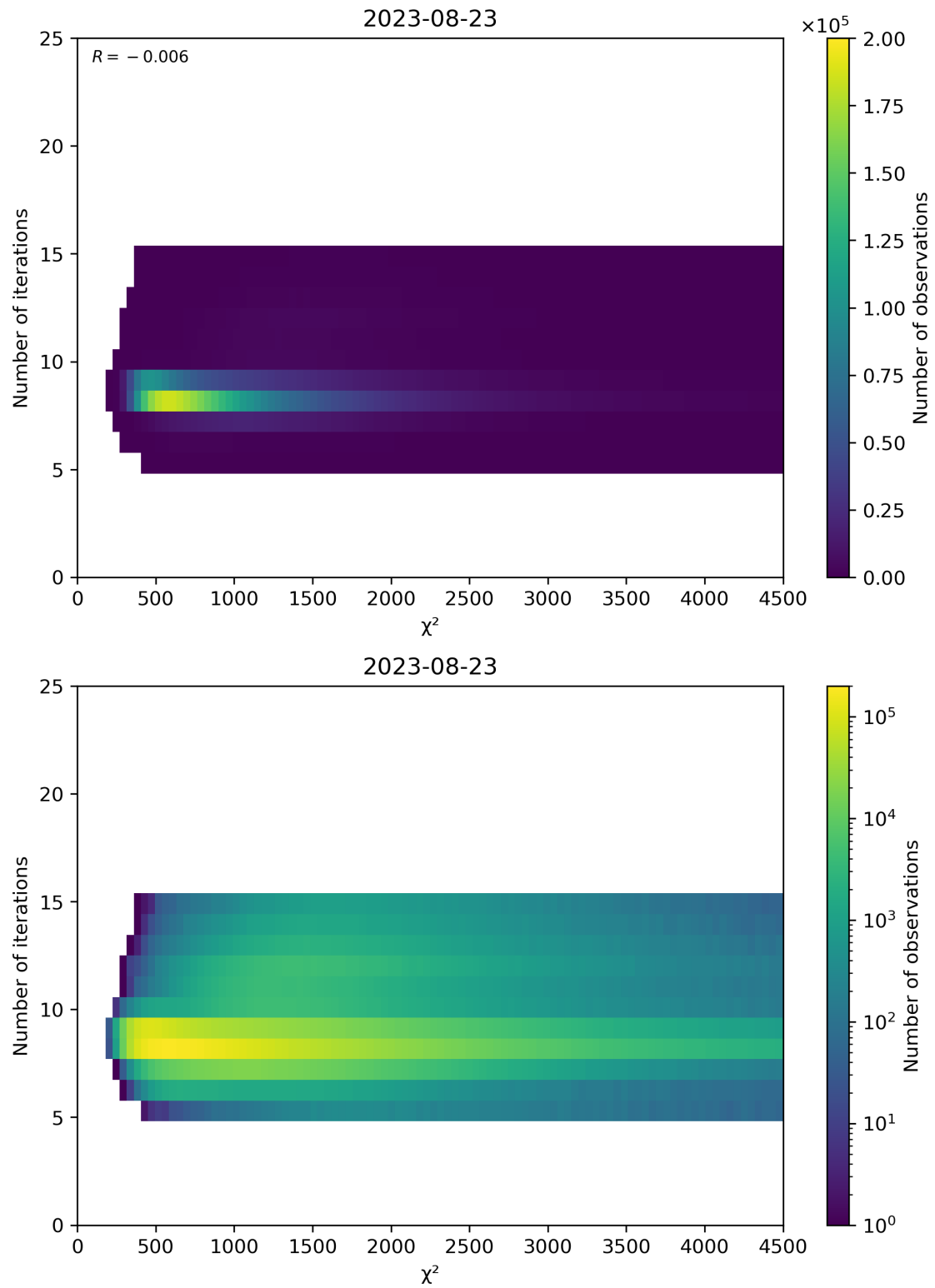
Figure 49: Scatter density plot of “ \chi^2 ” against “Number of iterations” for 2023-08-22 to 2023-08-24.
