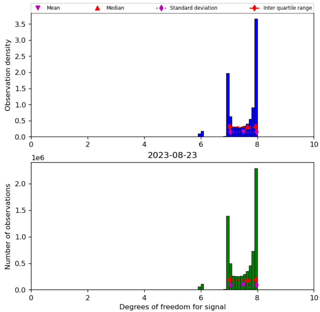
Figure 23: Histogram of “Degrees of freedom for signal” for 2023-08-22 to 2023-08-24
