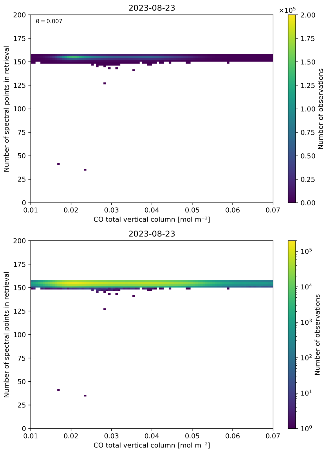
Figure 43: Scatter density plot of “CO total vertical column” against “Number of spectral points in retrieval” for 2023-08-22 to 2023-08-24.
