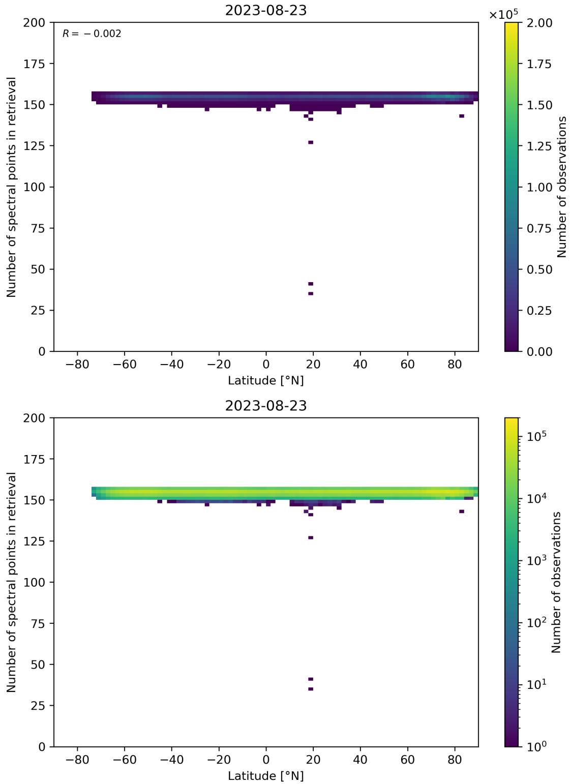
Figure 57: Scatter density plot of “Latitude” against “Number of spectral points in retrieval” for 2023-08-22 to 2023-08-24.
