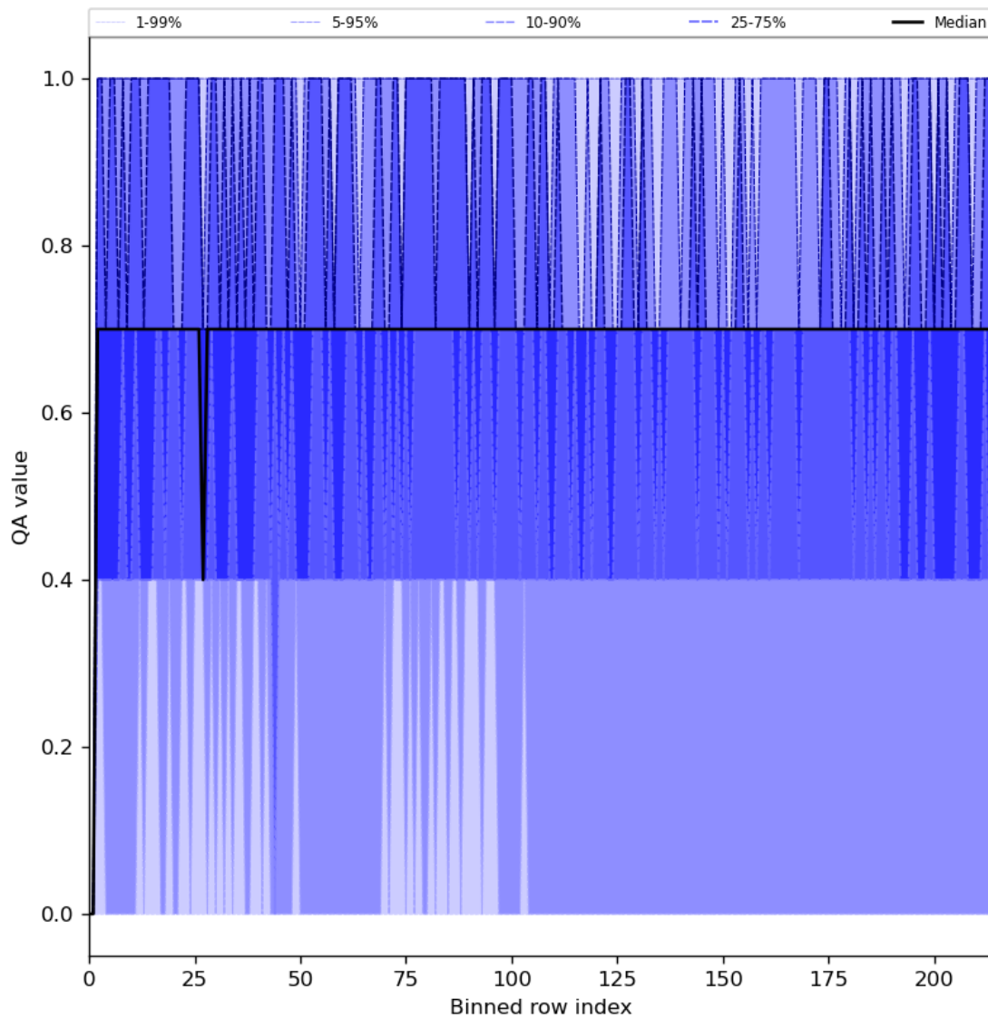
Figure 25: Along track statistics of “QA value” for 2023-08-22 to 2023-08-24
