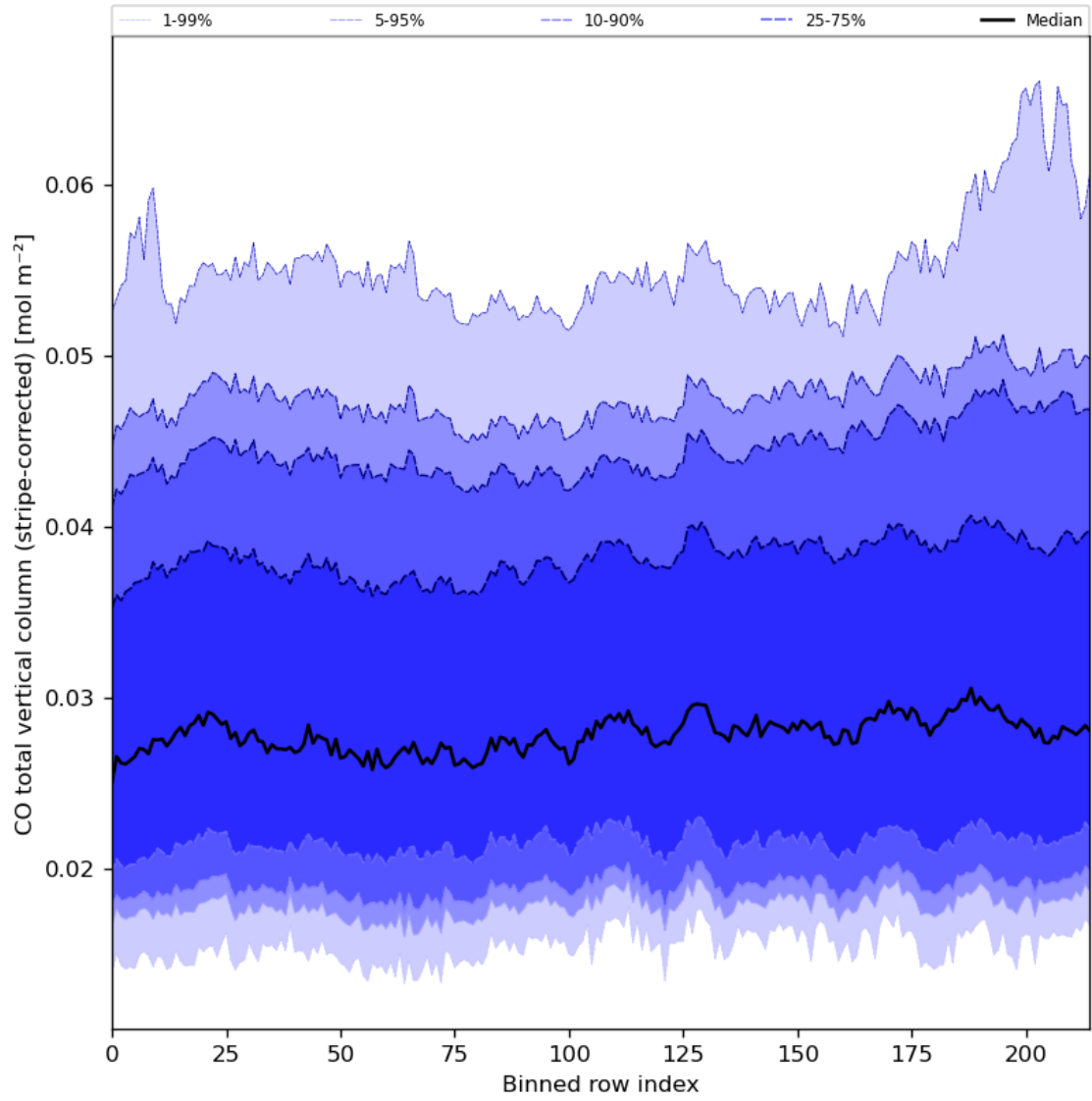
Figure 27: Along track statistics of “CO total vertical column (stripe-corrected)” for 2023-08-22 to 2023-08-24
