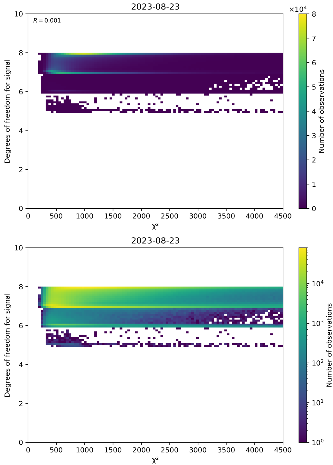
Figure 48: Scatter density plot of “ \chi^2 ” against “Degrees of freedom for signal” for 2023-08-22 to 2023-08-24.
