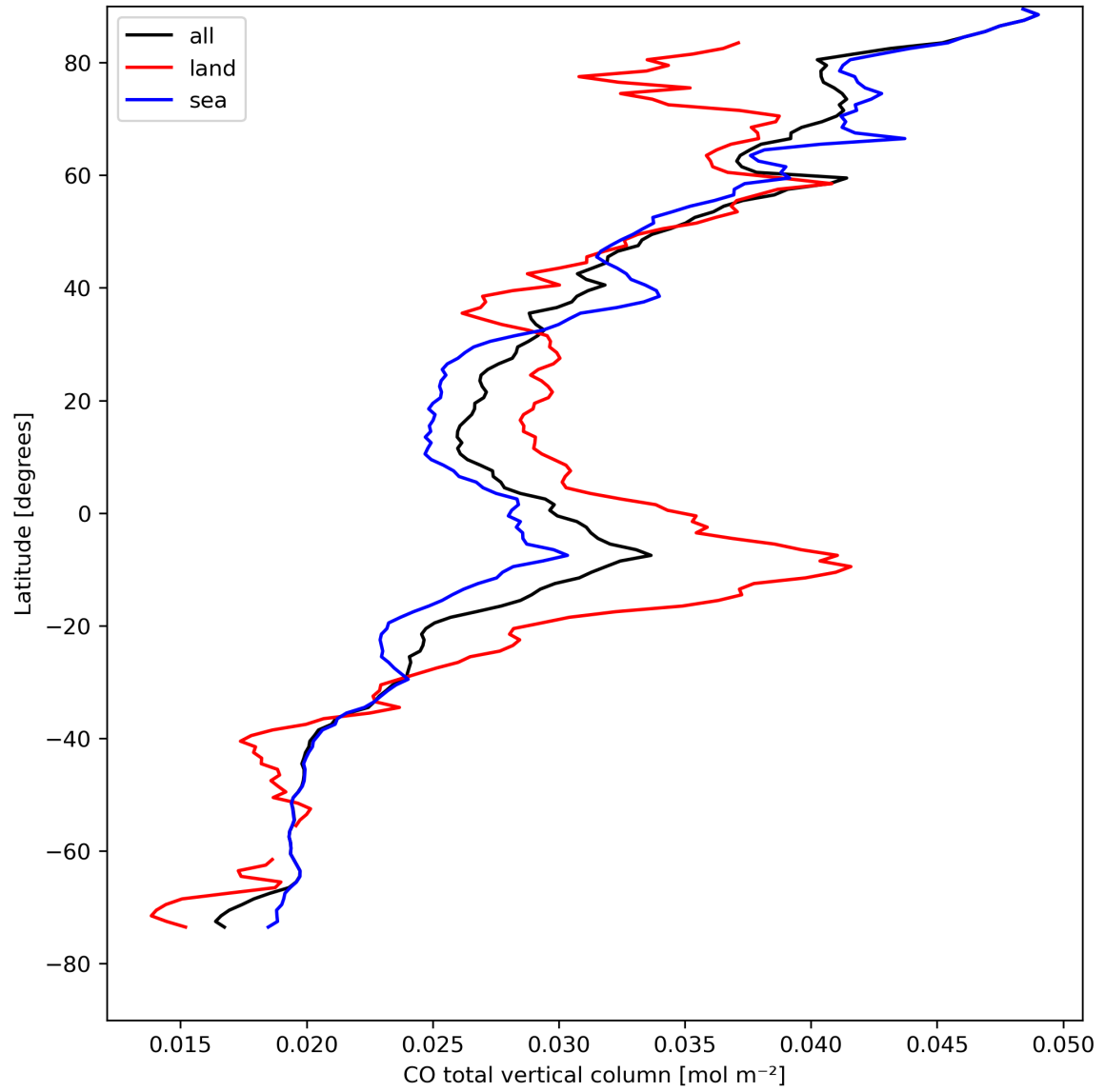
Figure 10: Zonal average of “CO total vertical column” for 2023-08-22 to 2023-08-24.
