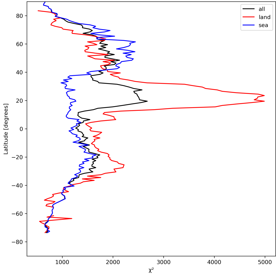
Figure 14: Zonal average of “ \chi^2 ” for 2023-08-22 to 2023-08-24.
