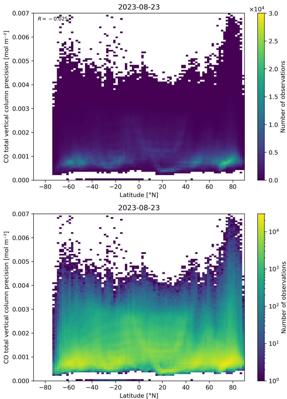
Figure 53: Scatter density plot of “Latitude” against “CO total vertical column precision” for 2023-08-22 to 2023-08-24.
