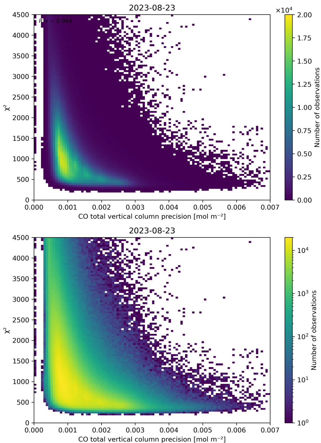
Figure 44: Scatter density plot of “CO total vertical column precision” against “ \chi^2 ” for 2023-08-22 to 2023-08-24.
