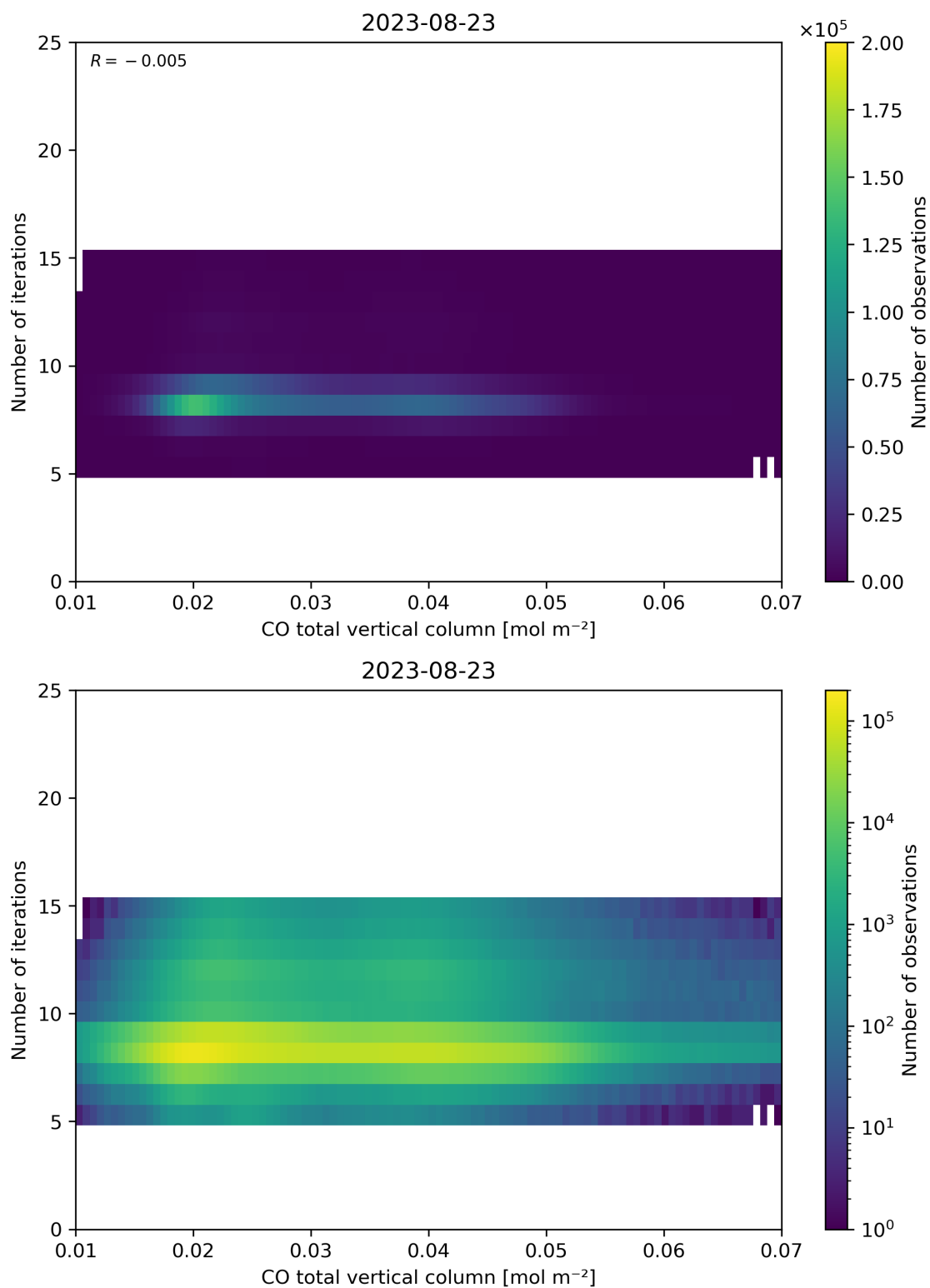
Figure 42: Scatter density plot of “CO total vertical column” against “Number of iterations” for 2023-08-22 to 2023-08-24.
