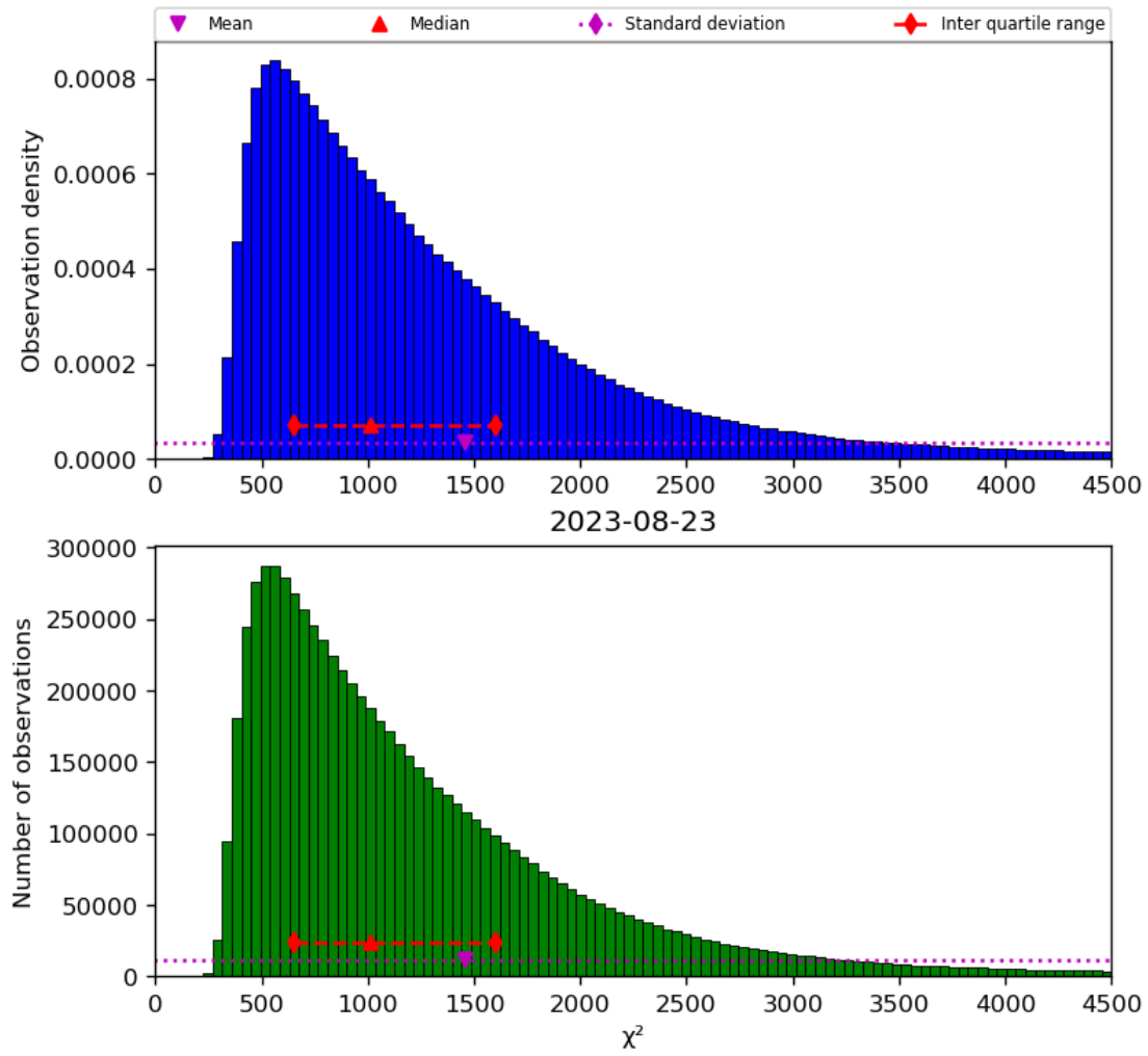
Figure 22: Histogram of “ \chi^2 ” for 2023-08-22 to 2023-08-24
