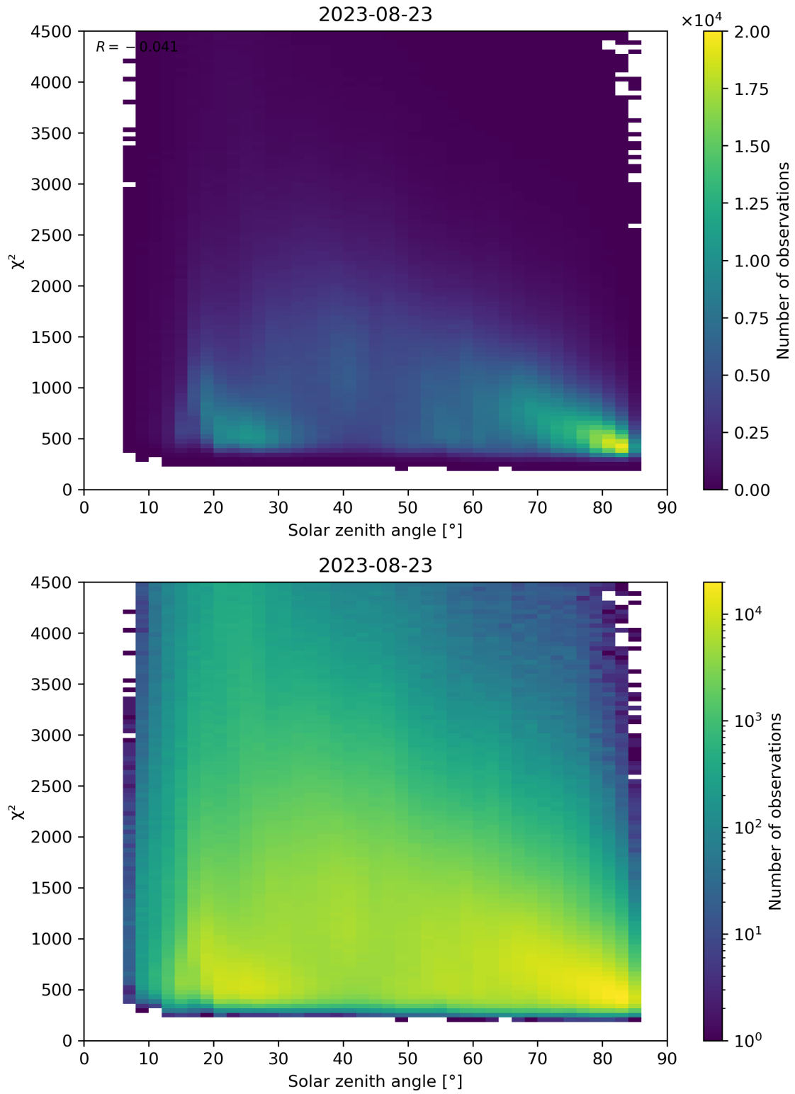
Figure 64: Scatter density plot of “Solar zenith angle” against “ \chi^2 ” for 2023-08-22 to 2023-08-24.
