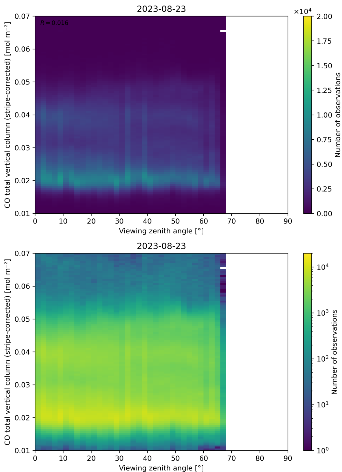
Figure 70: Scatter density plot of “Viewing zenith angle” against “CO total vertical column (stripe-corrected)” for 2023-08-22 to 2023-08-24.
