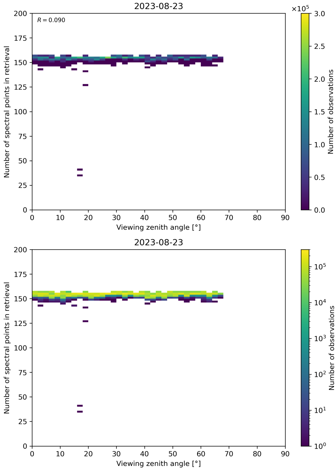
Figure 76: Scatter density plot of “Viewing zenith angle” against “Number of spectral points in retrieval” for 2023-08-22 to 2023-08-24.
