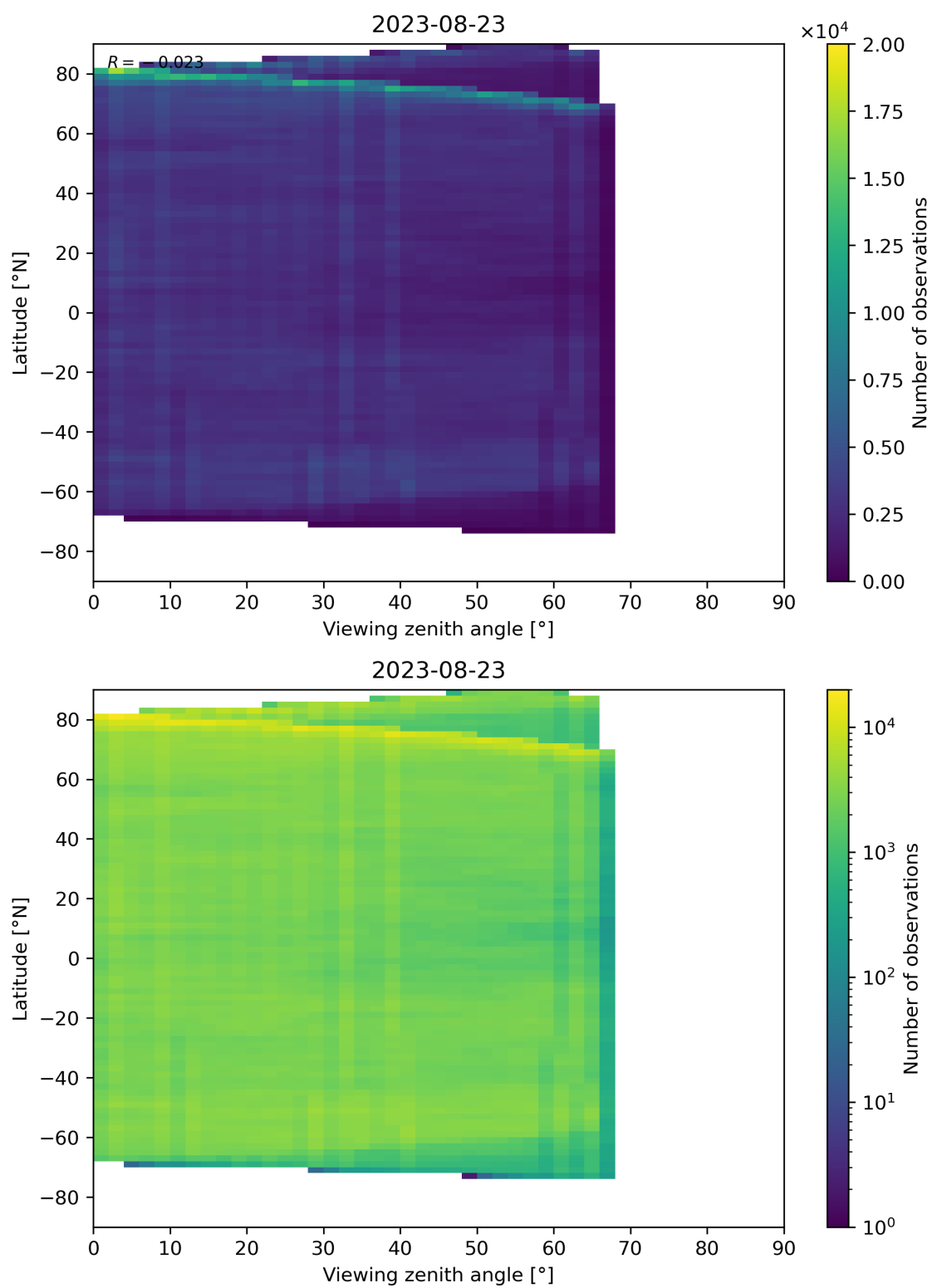
Figure 74: Scatter density plot of “Viewing zenith angle” against “Latitude” for 2023-08-22 to 2023-08-24.
