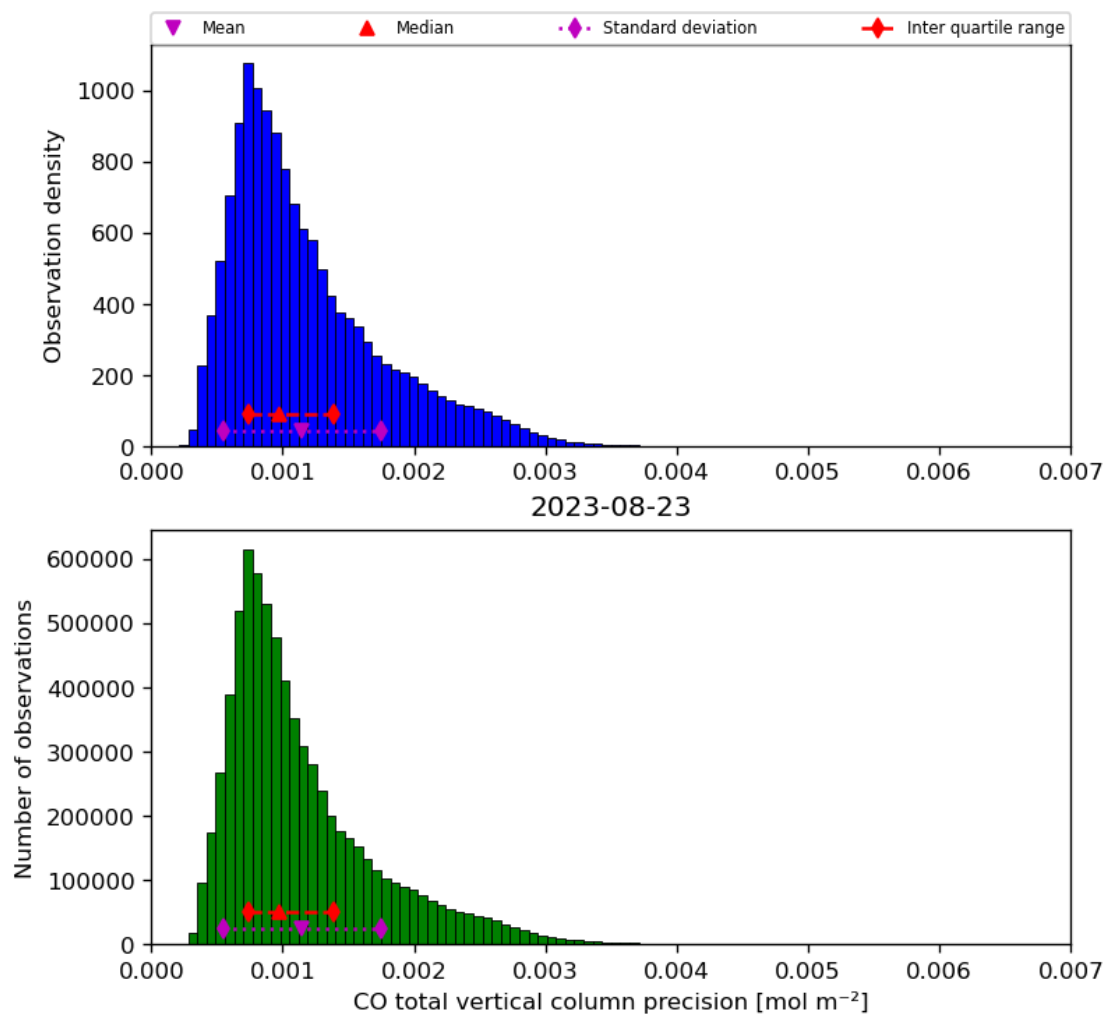
Figure 20: Histogram of “CO total vertical column precision” for 2023-08-22 to 2023-08-24
