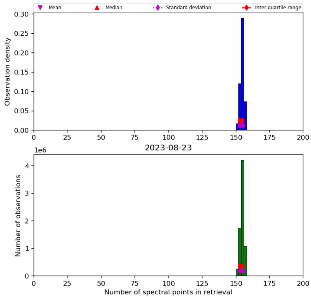
Figure 21: Histogram of “Number of spectral points in retrieval” for 2023-08-22 to 2023-08-24
