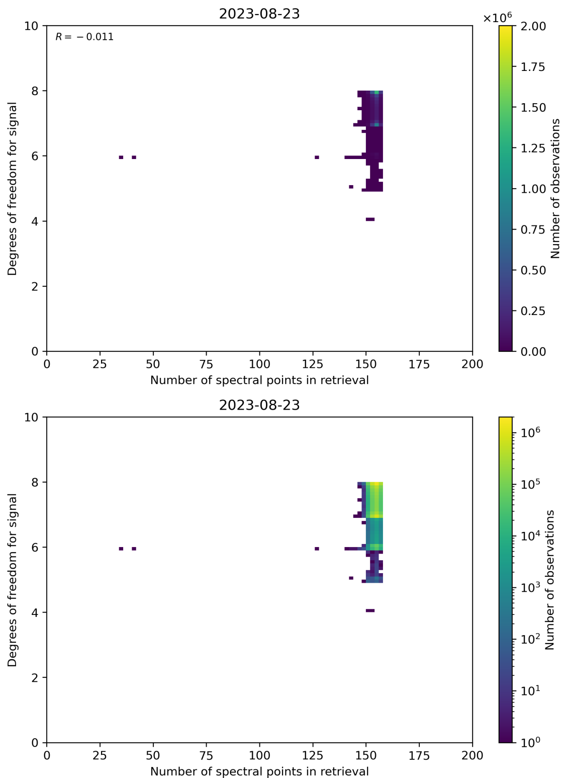
Figure 59: Scatter density plot of “Number of spectral points in retrieval” against “Degrees of freedom for signal” for 2023-08-22 to 2023-08-24.
