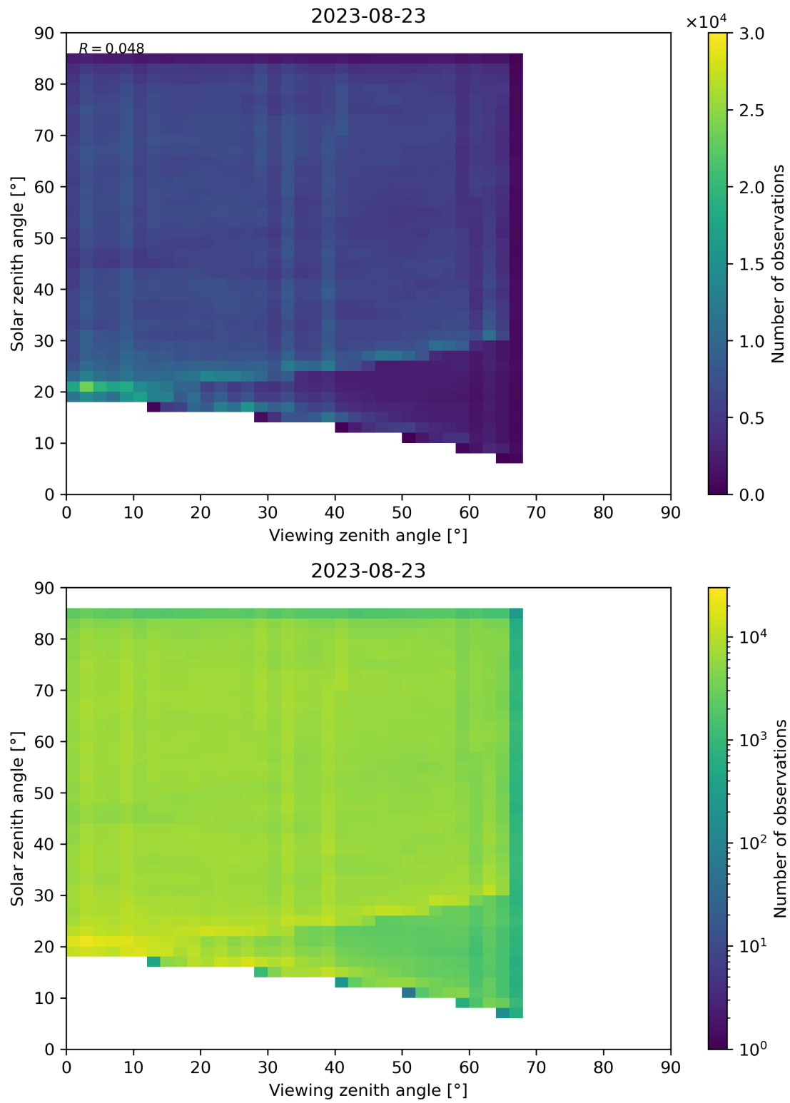
Figure 77: Scatter density plot of “Viewing zenith angle” against “Solar zenith angle” for 2023-08-22 to 2023-08-24.
