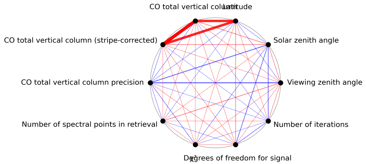
Figure 1: Map of correlation graph for 2023-08-22 to 2023-08-24.
