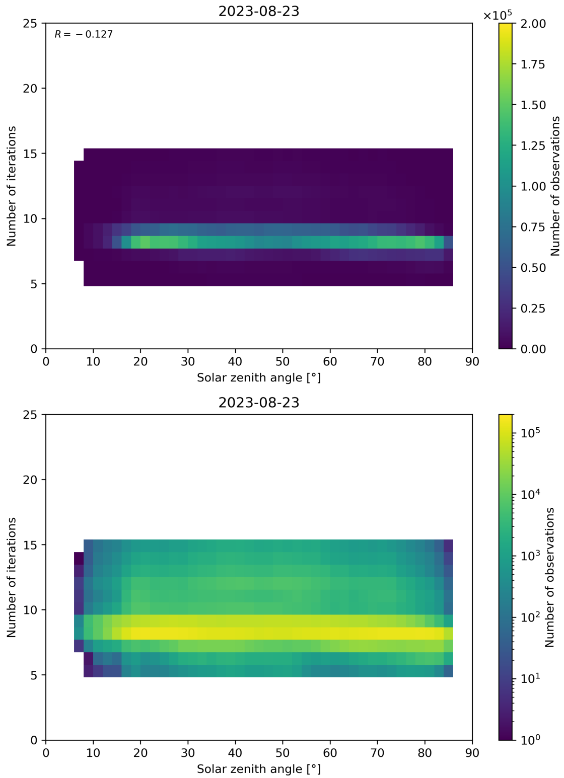
Figure 67: Scatter density plot of “Solar zenith angle” against “Number of iterations” for 2023-08-22 to 2023-08-24.
