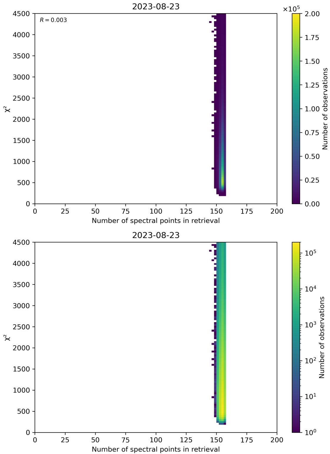
Figure 58: Scatter density plot of “Number of spectral points in retrieval” against “ \chi^2 ” for 2023-08-22 to 2023-08-24.
