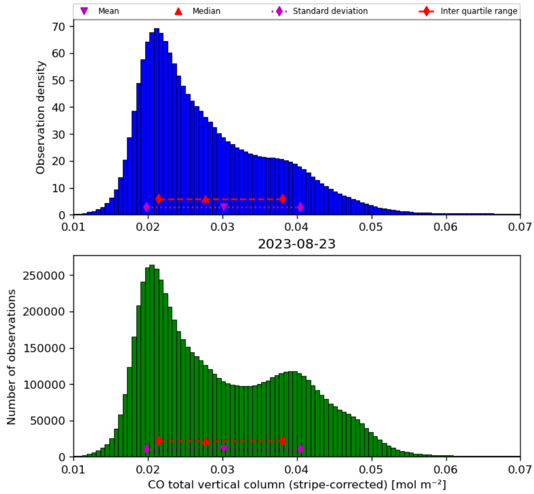
Figure 19: Histogram of “CO total vertical column (stripe-corrected)” for 2023-08-22 to 2023-08-24
