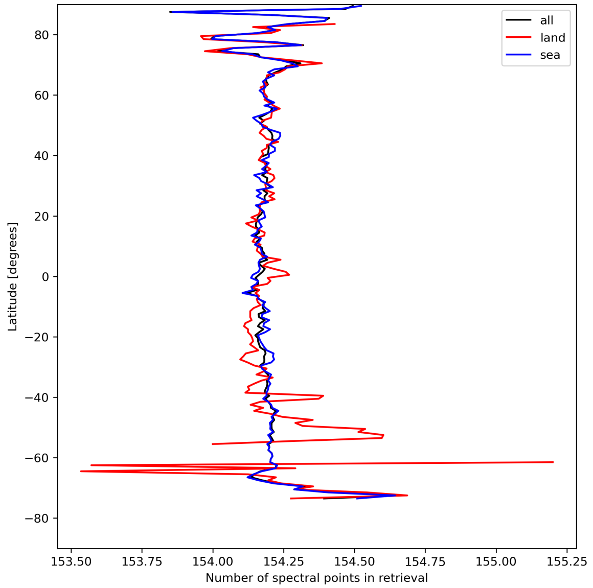
Figure 13: Zonal average of “Number of spectral points in retrieval” for 2023-08-22 to 2023-08-24.
