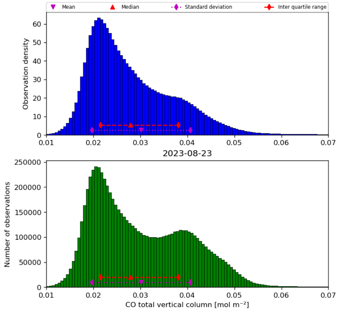
Figure 18: Histogram of “CO total vertical column” for 2023-08-22 to 2023-08-24
