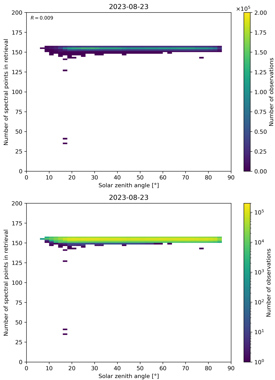
Figure 68: Scatter density plot of “Solar zenith angle” against “Number of spectral points in retrieval” for 2023-08-22 to 2023-08-24.
