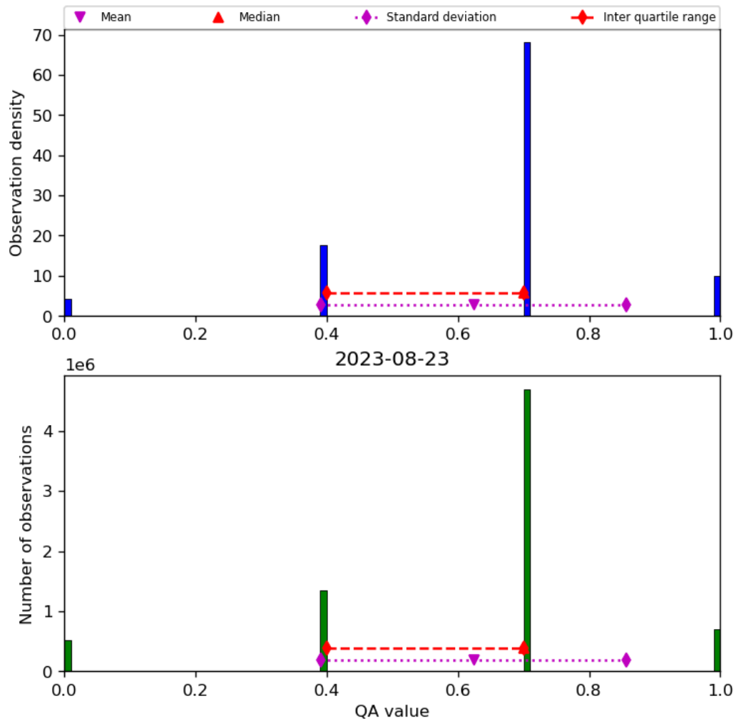
Figure 17: Histogram of “QA value” for 2023-08-22 to 2023-08-24
