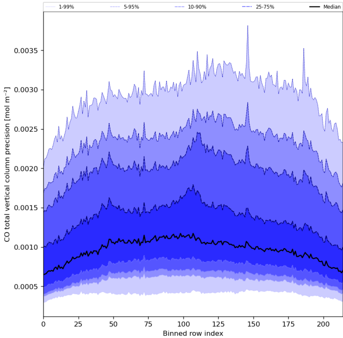
Figure 28: Along track statistics of “CO total vertical column precision” for 2023-08-22 to 2023-08-24
