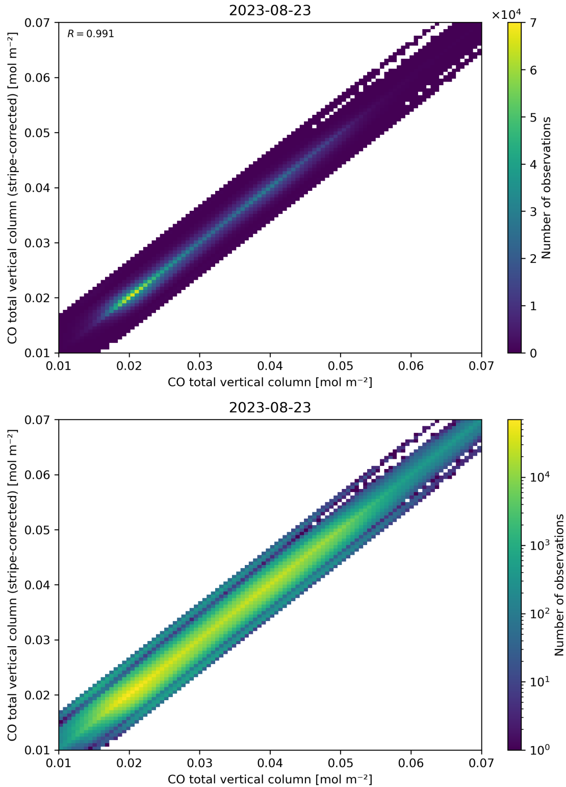
Figure 33: Scatter density plot of “CO total vertical column” against “CO total vertical column (stripe-corrected)” for 2023-08-22 to 2023-08-24.
