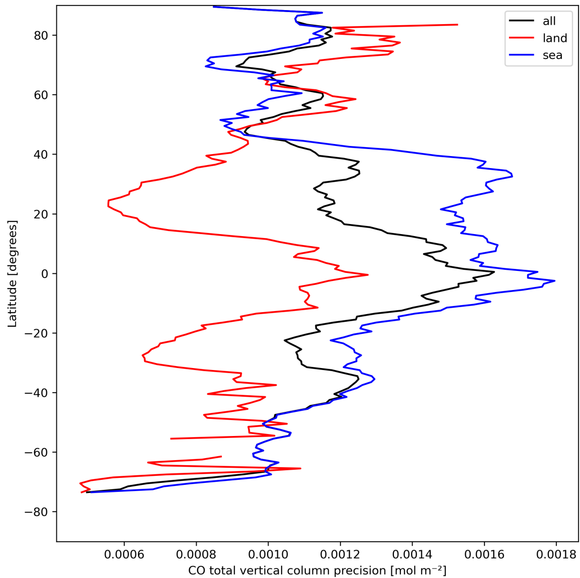
Figure 12: Zonal average of “CO total vertical column precision” for 2023-08-22 to 2023-08-24.
