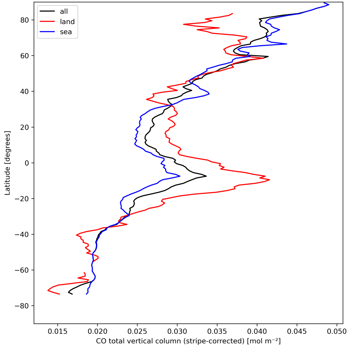
Figure 11: Zonal average of “CO total vertical column (stripe-corrected)” for 2023-08-22 to 2023-08-24.
