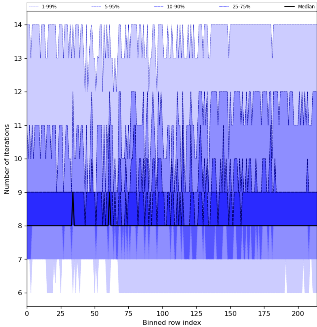
Figure 32: Along track statistics of “Number of iterations” for 2023-08-22 to 2023-08-24
