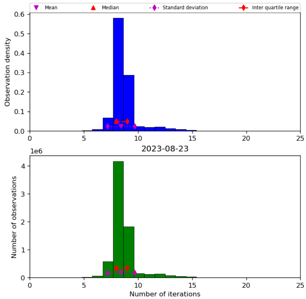
Figure 24: Histogram of “Number of iterations” for 2023-08-22 to 2023-08-24
