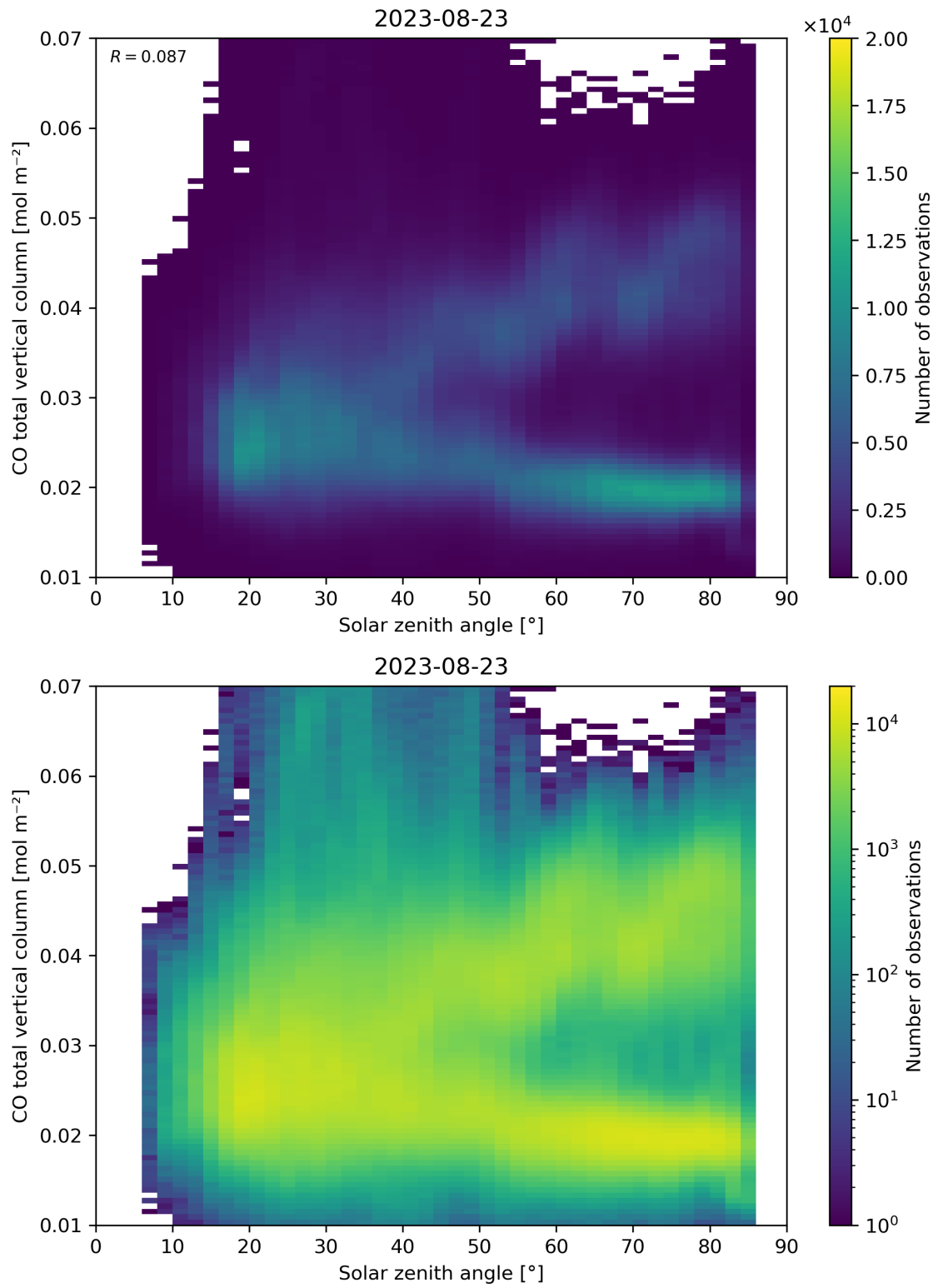
Figure 61: Scatter density plot of “Solar zenith angle” against “CO total vertical column” for 2023-08-22 to 2023-08-24.
