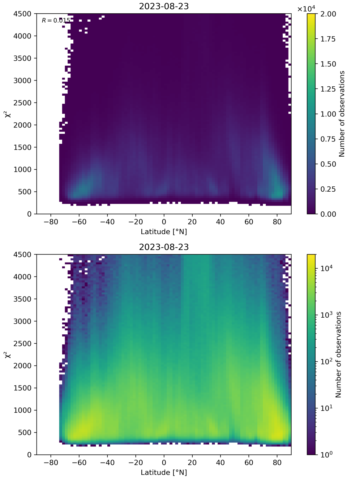
Figure 54: Scatter density plot of “Latitude” against “ \chi^2 ” for 2023-08-22 to 2023-08-24.
