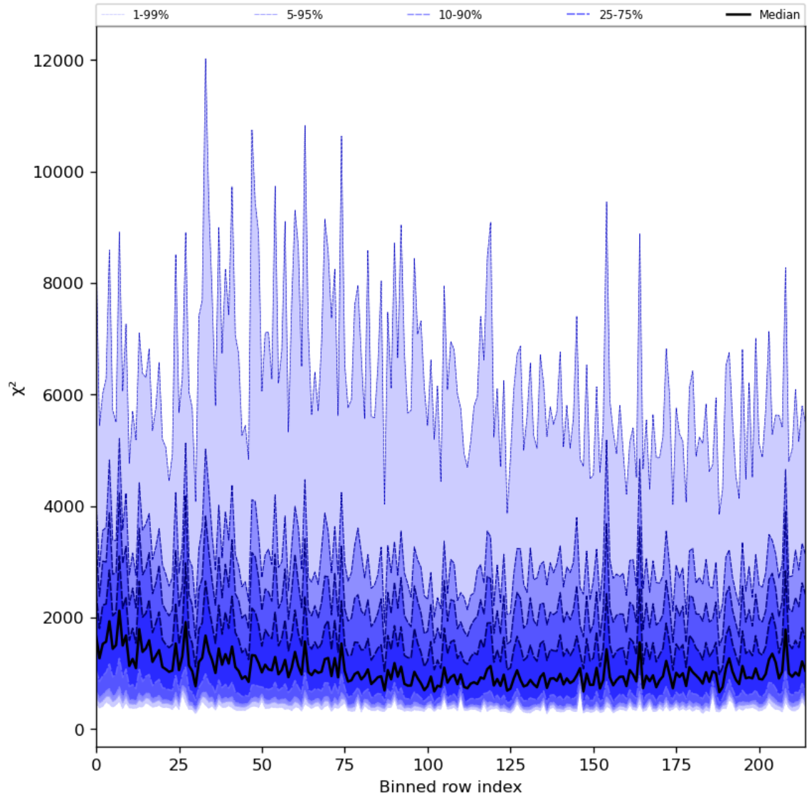
Figure 30: Along track statistics of “ \chi^2 ” for 2023-08-22 to 2023-08-24
