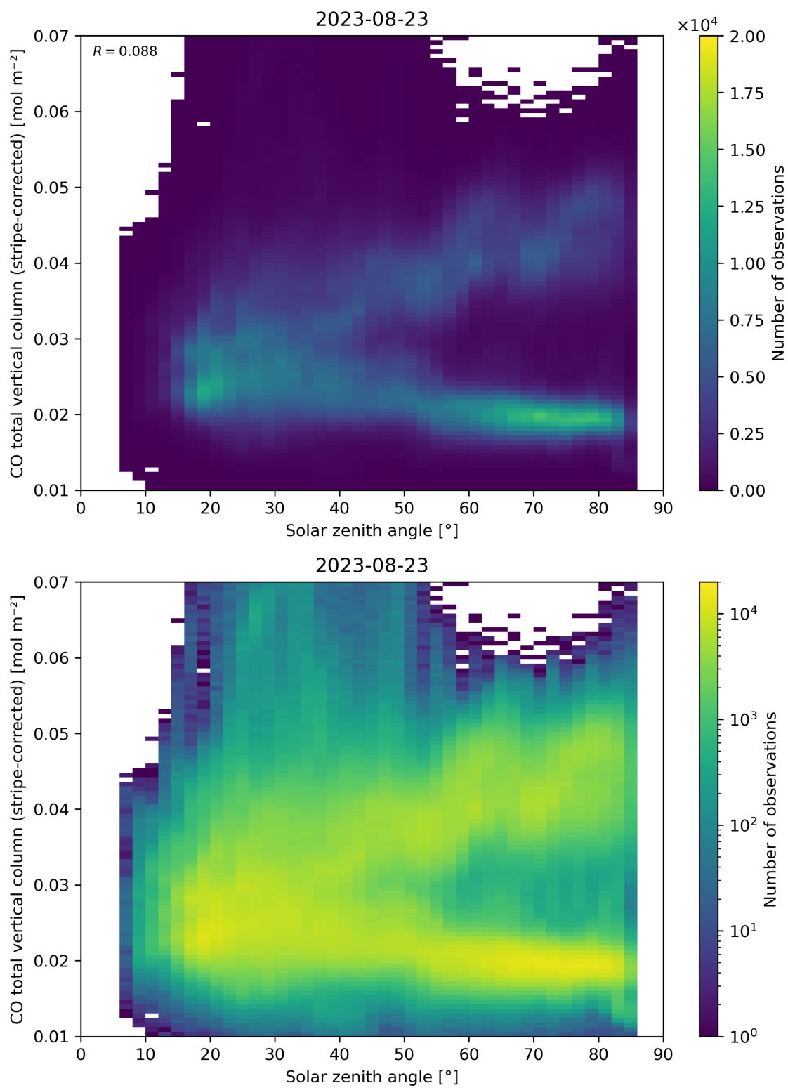
Figure 62: Scatter density plot of “Solar zenith angle” against “CO total vertical column (stripe-corrected)” for 2023-08-22 to 2023-08-24.
