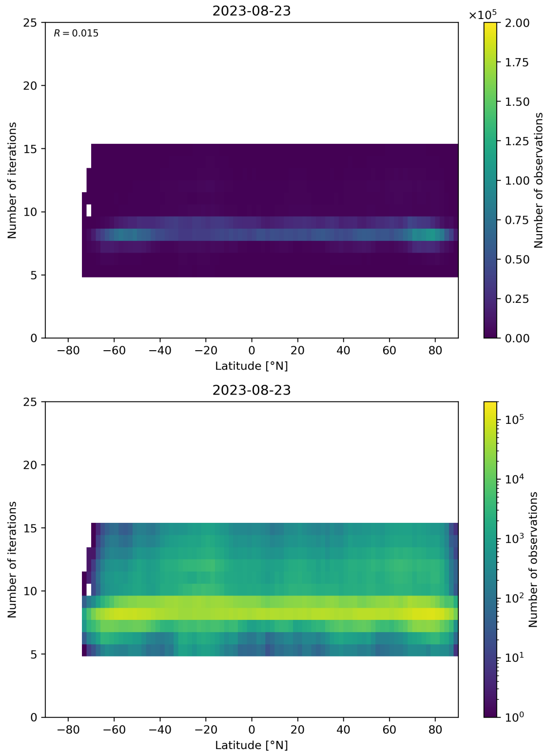
Figure 56: Scatter density plot of “Latitude” against “Number of iterations” for 2023-08-22 to 2023-08-24.
