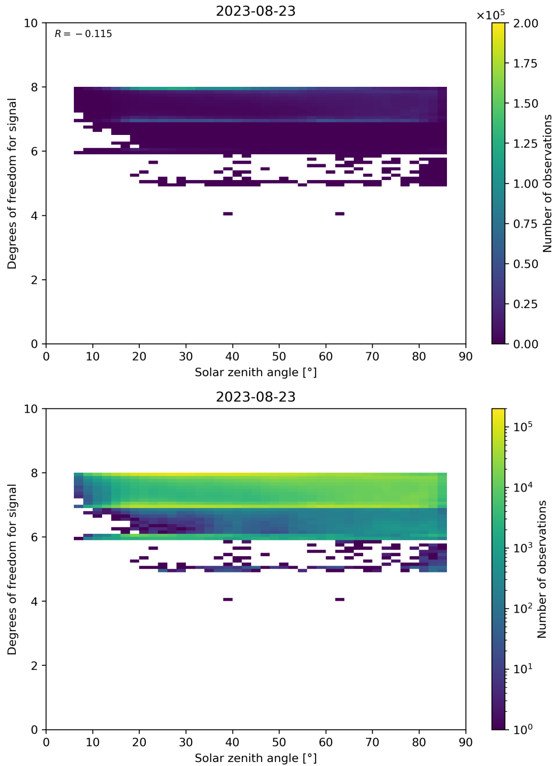
Figure 65: Scatter density plot of “Solar zenith angle” against “Degrees of freedom for signal” for 2023-08-22 to 2023-08-24.
