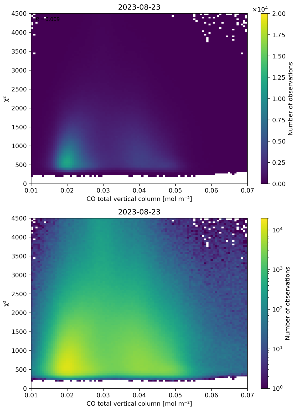
Figure 35: Scatter density plot of “CO total vertical column” against “ \chi^2 ” for 2023-08-22 to 2023-08-24.
