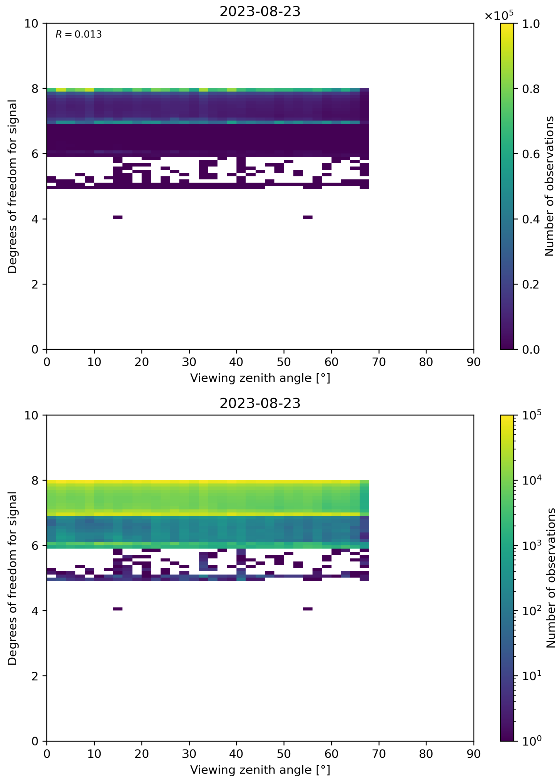
Figure 73: Scatter density plot of “Viewing zenith angle” against “Degrees of freedom for signal” for 2023-08-22 to 2023-08-24.
