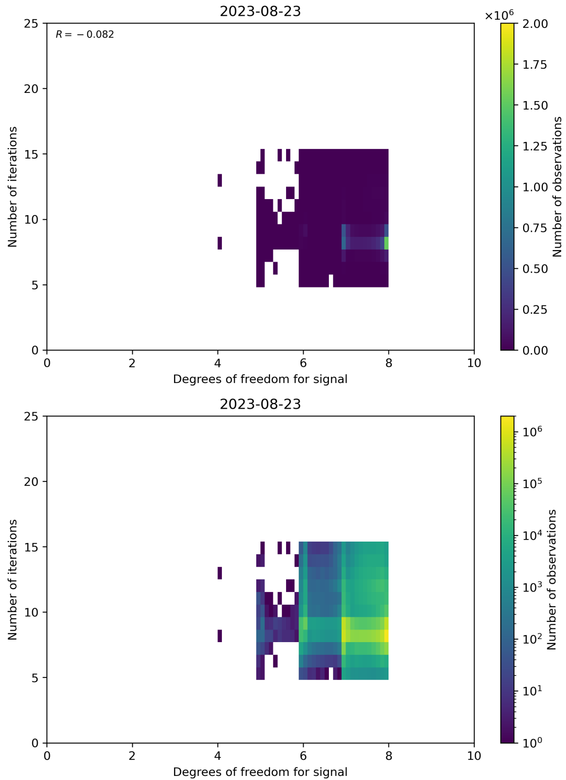
Figure 50: Scatter density plot of “Degrees of freedom for signal” against “Number of iterations” for 2023-08-22 to 2023-08-24.
