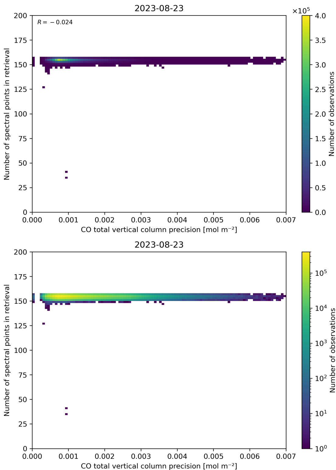
Figure 47: Scatter density plot of “CO total vertical column precision” against “Number of spectral points in retrieval” for 2023-08-22 to 2023-08-24.
