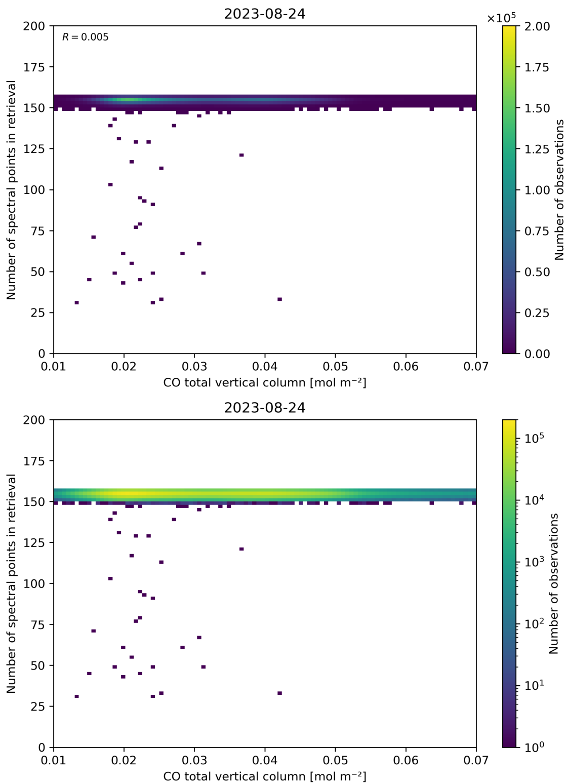
Figure 43: Scatter density plot of “CO total vertical column” against “Number of spectral points in retrieval” for 2023-08-23 to 2023-08-25.
