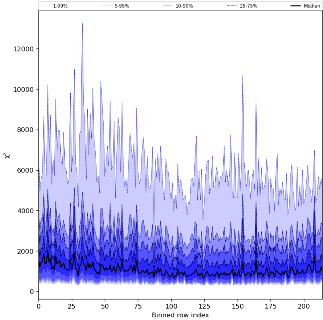
Figure 30: Along track statistics of “ \chi^2 ” for 2023-08-23 to 2023-08-25
