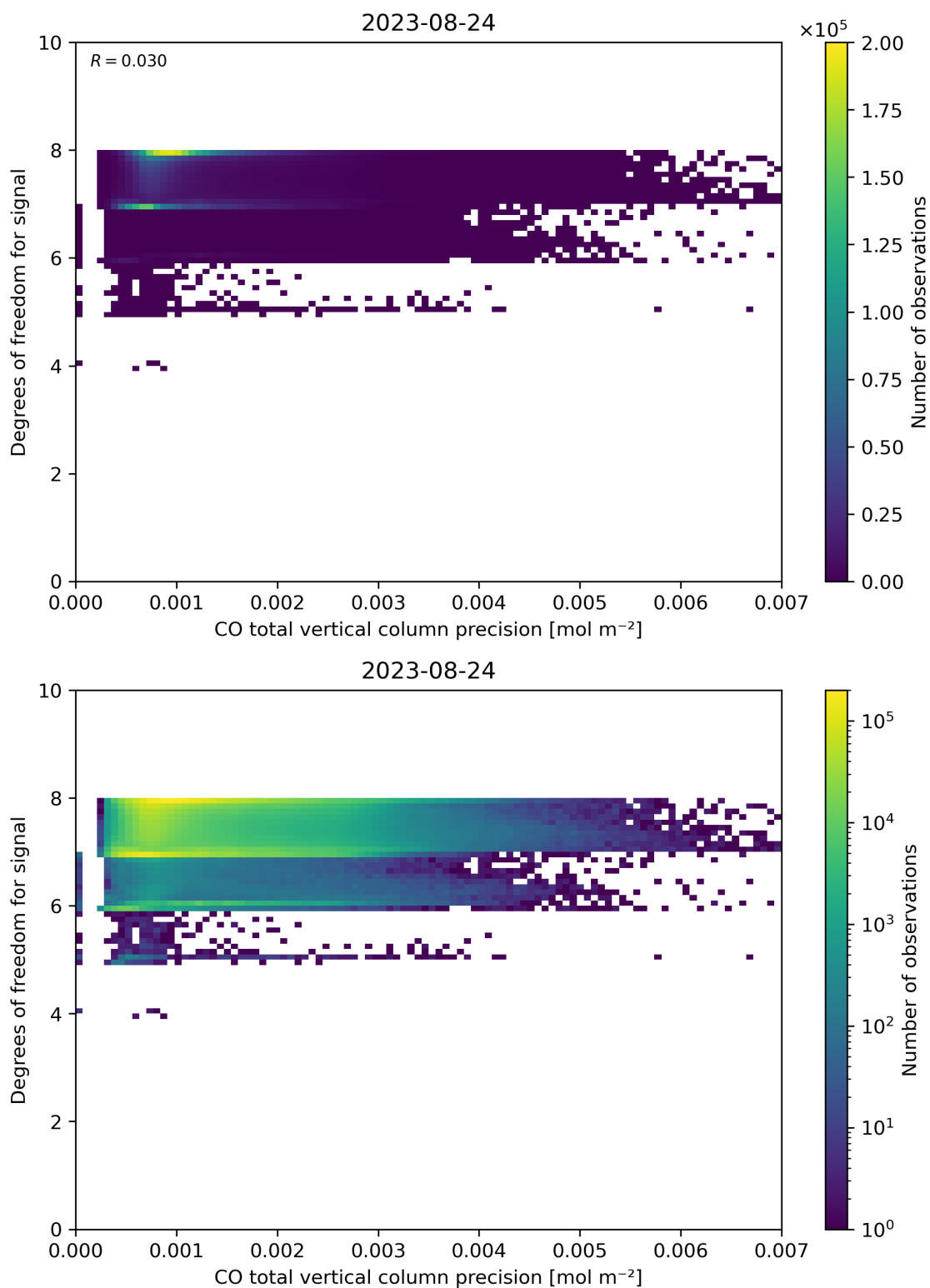
Figure 45: Scatter density plot of “CO total vertical column precision” against “Degrees of freedom for signal” for 2023-08-23 to 2023-08-25.
