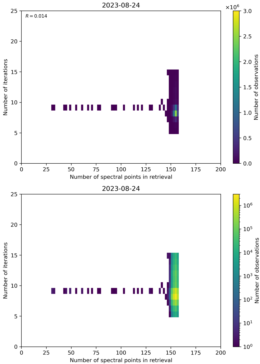
Figure 60: Scatter density plot of “Number of spectral points in retrieval” against “Number of iterations” for 2023-08-23 to 2023-08-25.
