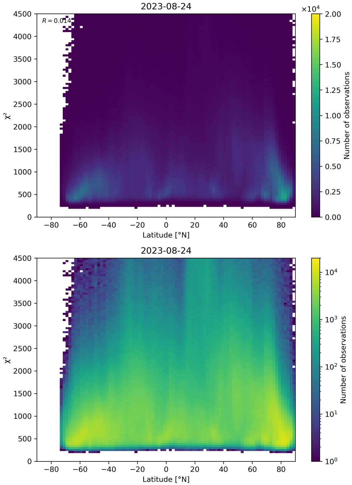
Figure 54: Scatter density plot of “Latitude” against “ \chi^2 ” for 2023-08-23 to 2023-08-25.
