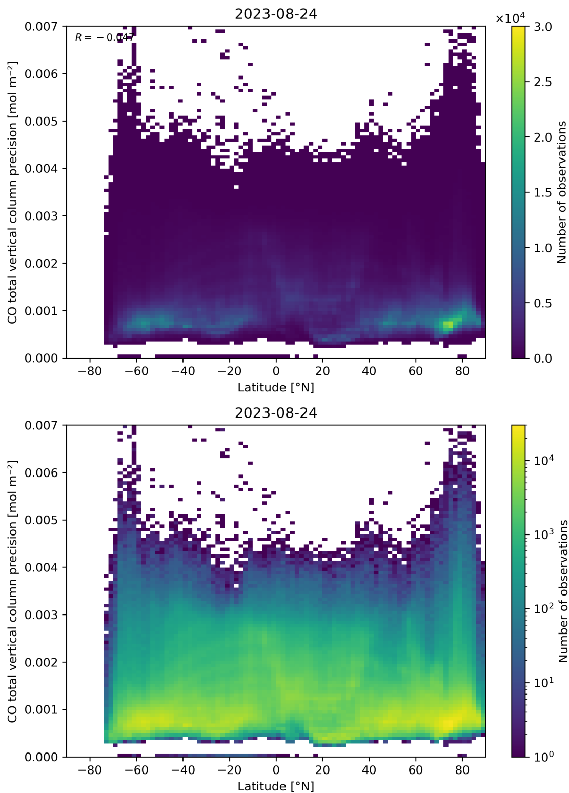
Figure 53: Scatter density plot of “Latitude” against “CO total vertical column precision” for 2023-08-23 to 2023-08-25.
