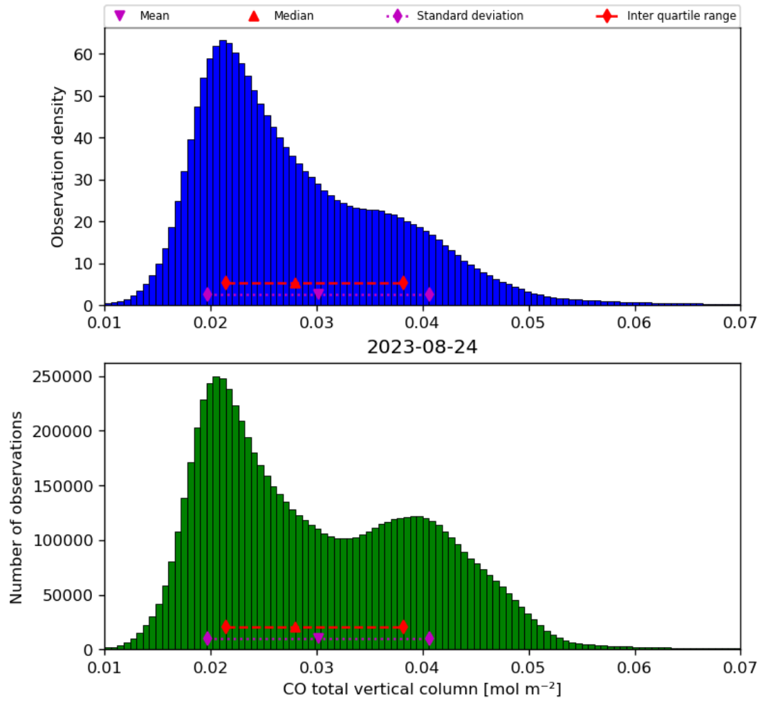
Figure 18: Histogram of “CO total vertical column” for 2023-08-23 to 2023-08-25
