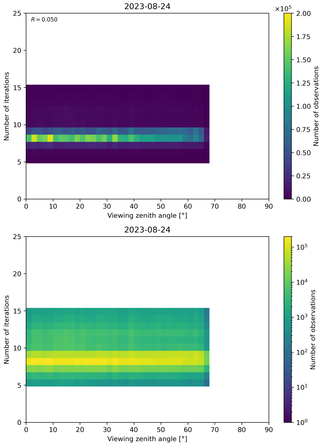
Figure 75: Scatter density plot of “Viewing zenith angle” against “Number of iterations” for 2023-08-23 to 2023-08-25.
