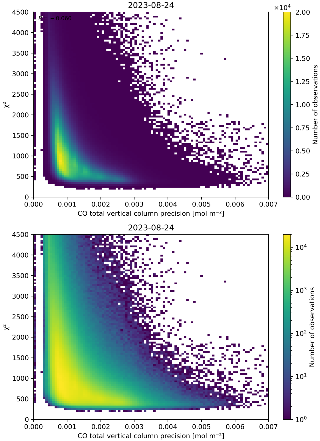
Figure 44: Scatter density plot of “CO total vertical column precision” against “ \chi^2 ” for 2023-08-23 to 2023-08-25.
