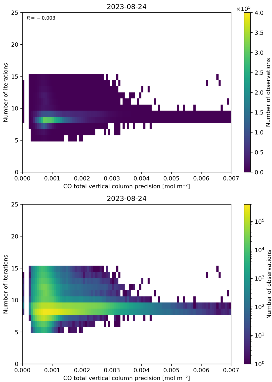
Figure 46: Scatter density plot of “CO total vertical column precision” against “Number of iterations” for 2023-08-23 to 2023-08-25.
