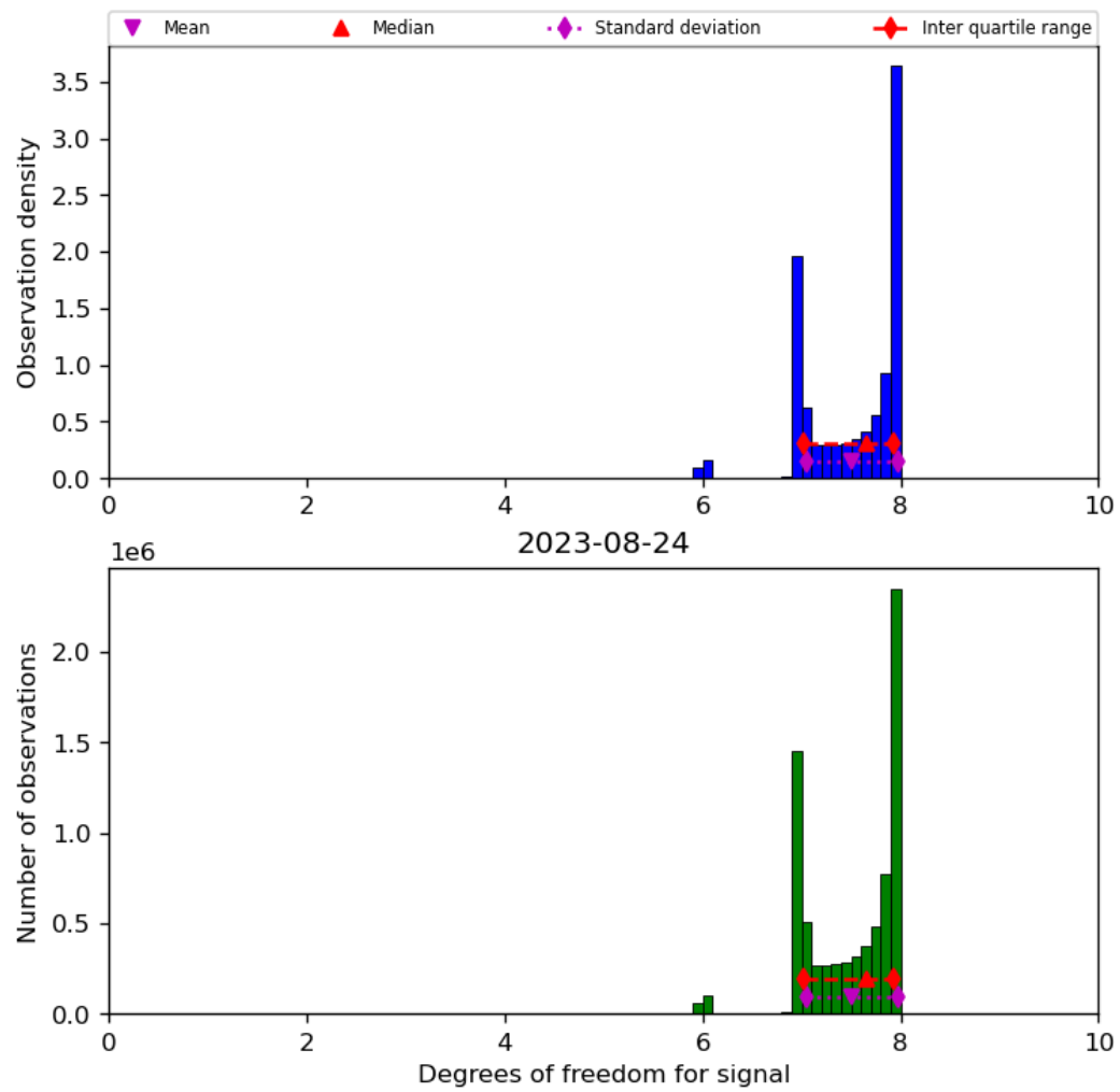
Figure 23: Histogram of “Degrees of freedom for signal” for 2023-08-23 to 2023-08-25
