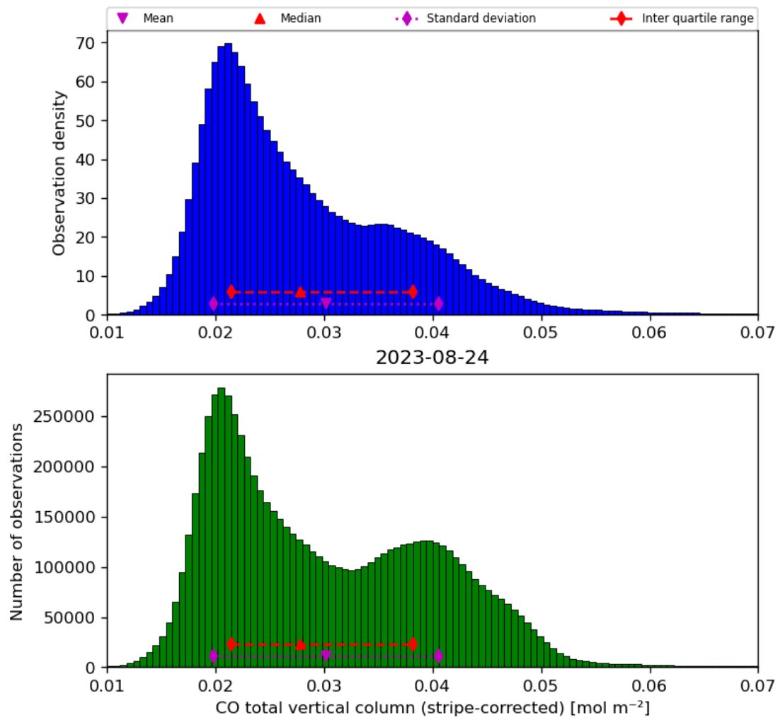
Figure 19: Histogram of “CO total vertical column (stripe-corrected)” for 2023-08-23 to 2023-08-25
