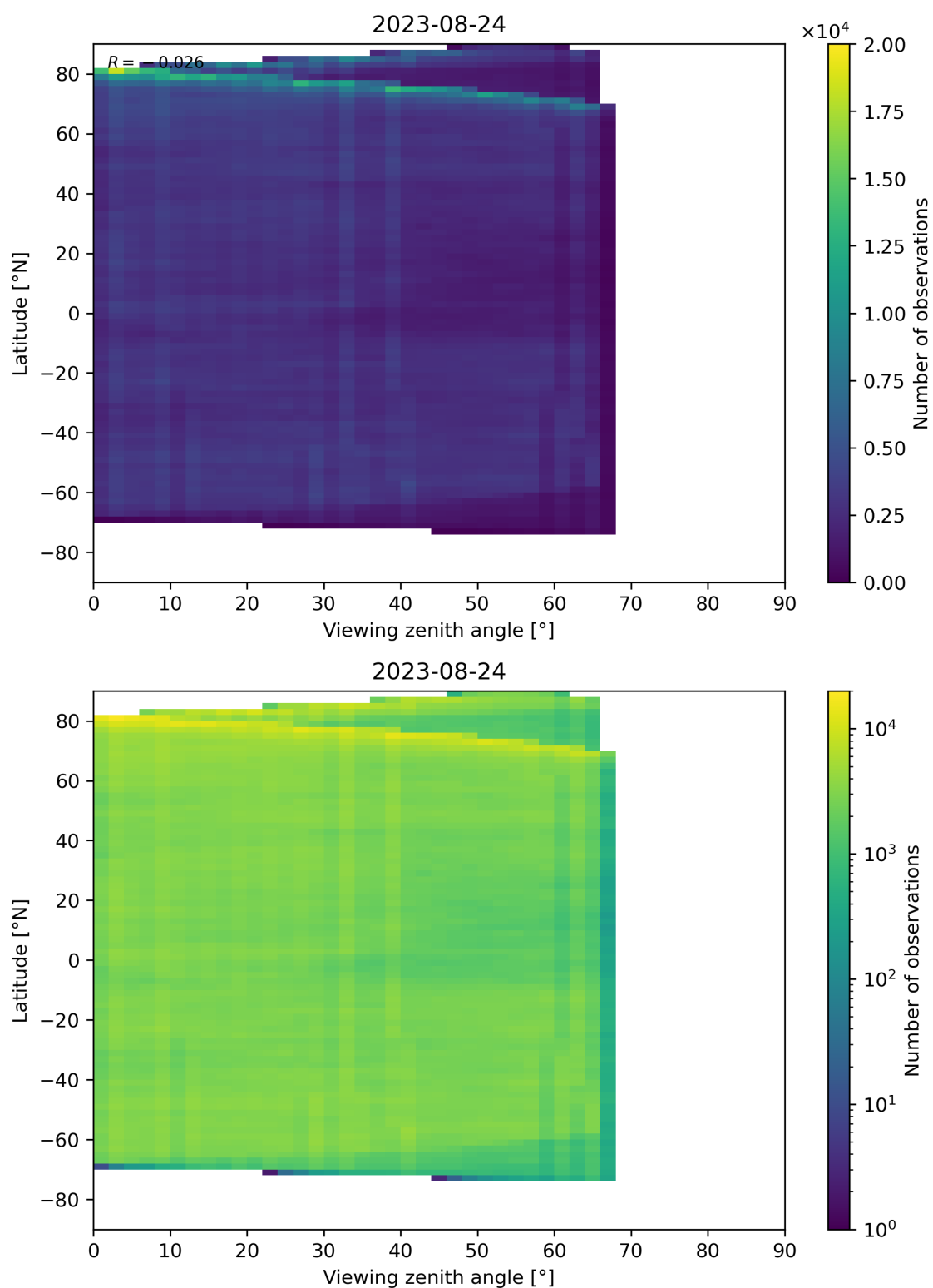
Figure 74: Scatter density plot of “Viewing zenith angle” against “Latitude” for 2023-08-23 to 2023-08-25.
