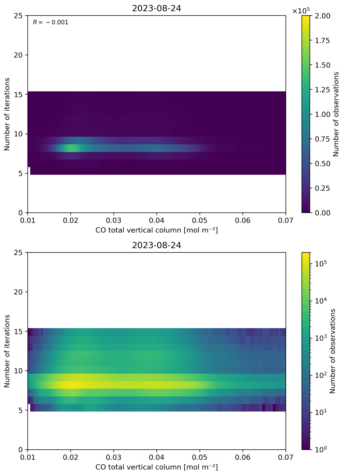
Figure 42: Scatter density plot of “CO total vertical column” against “Number of iterations” for 2023-08-23 to 2023-08-25.
