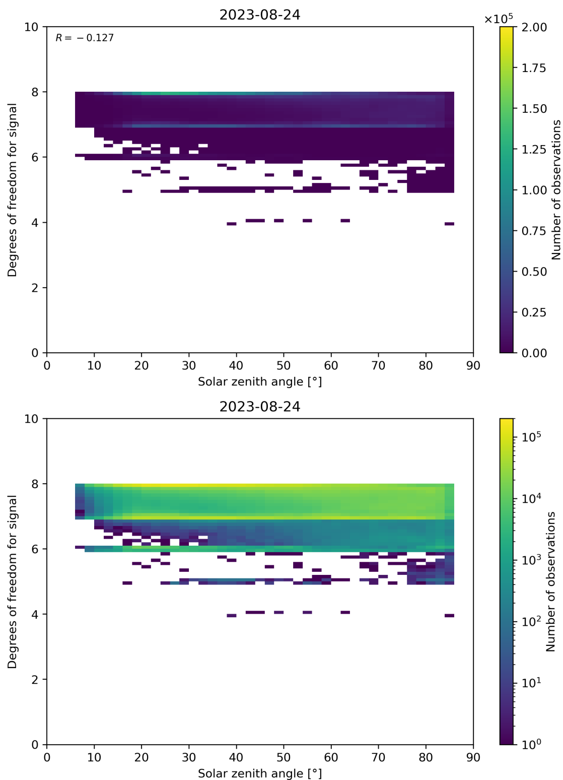
Figure 65: Scatter density plot of “Solar zenith angle” against “Degrees of freedom for signal” for 2023-08-23 to 2023-08-25.
