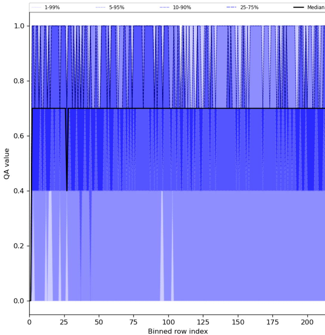
Figure 25: Along track statistics of “QA value” for 2023-08-23 to 2023-08-25
