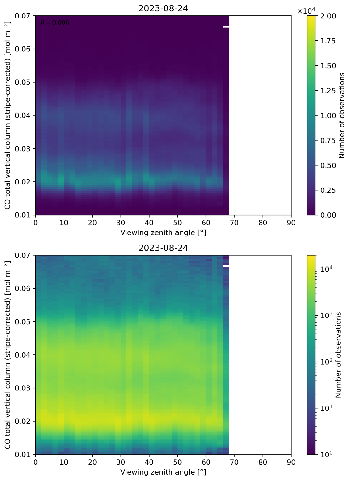
Figure 70: Scatter density plot of “Viewing zenith angle” against “CO total vertical column (stripe-corrected)” for 2023-08-23 to 2023-08-25.
