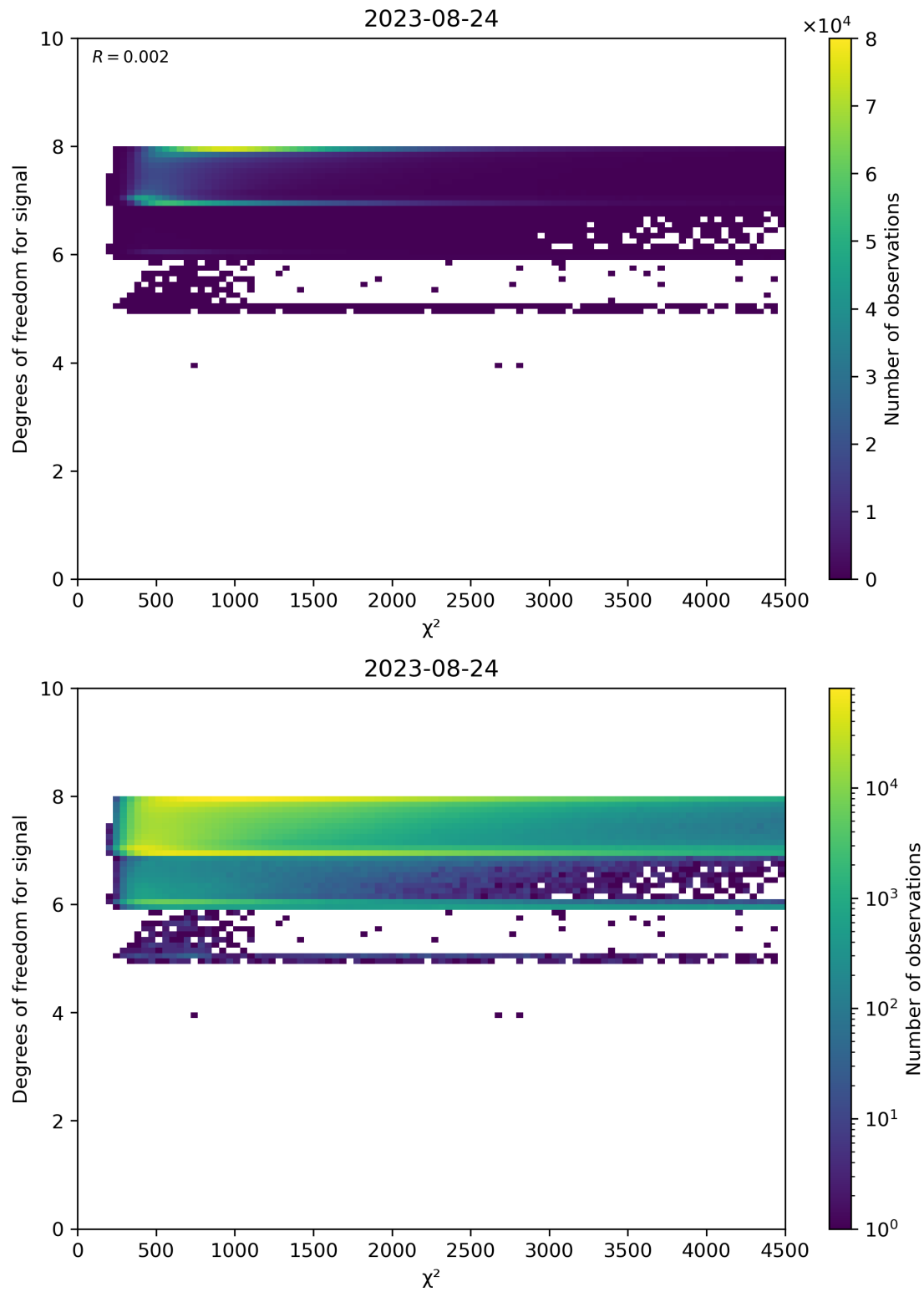
Figure 48: Scatter density plot of “ \chi^2 ” against “Degrees of freedom for signal” for 2023-08-23 to 2023-08-25.
