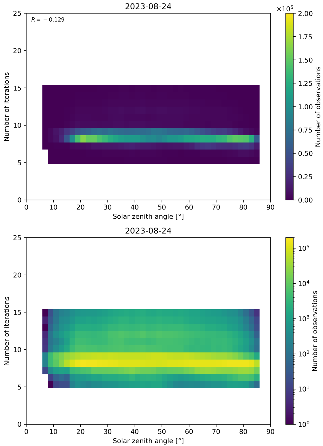
Figure 67: Scatter density plot of “Solar zenith angle” against “Number of iterations” for 2023-08-23 to 2023-08-25.
