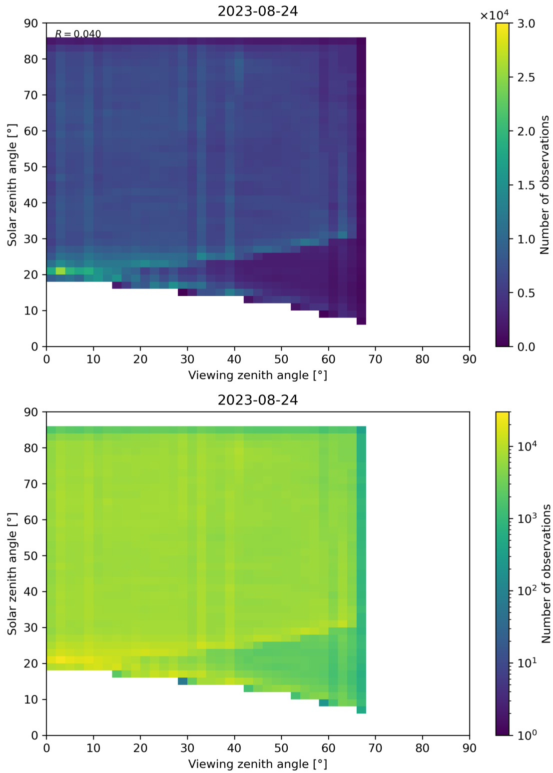
Figure 77: Scatter density plot of “Viewing zenith angle” against “Solar zenith angle” for 2023-08-23 to 2023-08-25.
