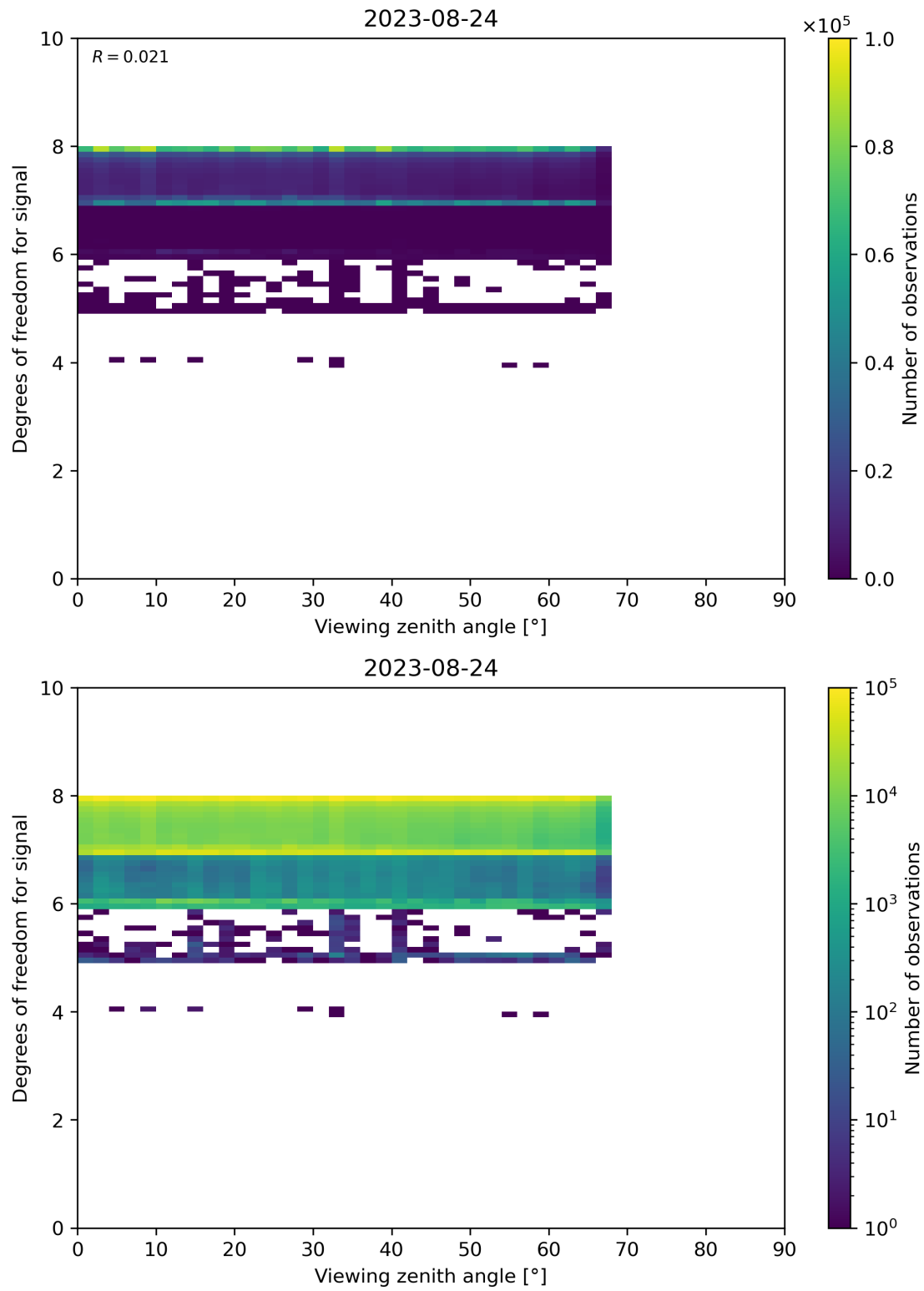
Figure 73: Scatter density plot of “Viewing zenith angle” against “Degrees of freedom for signal” for 2023-08-23 to 2023-08-25.
