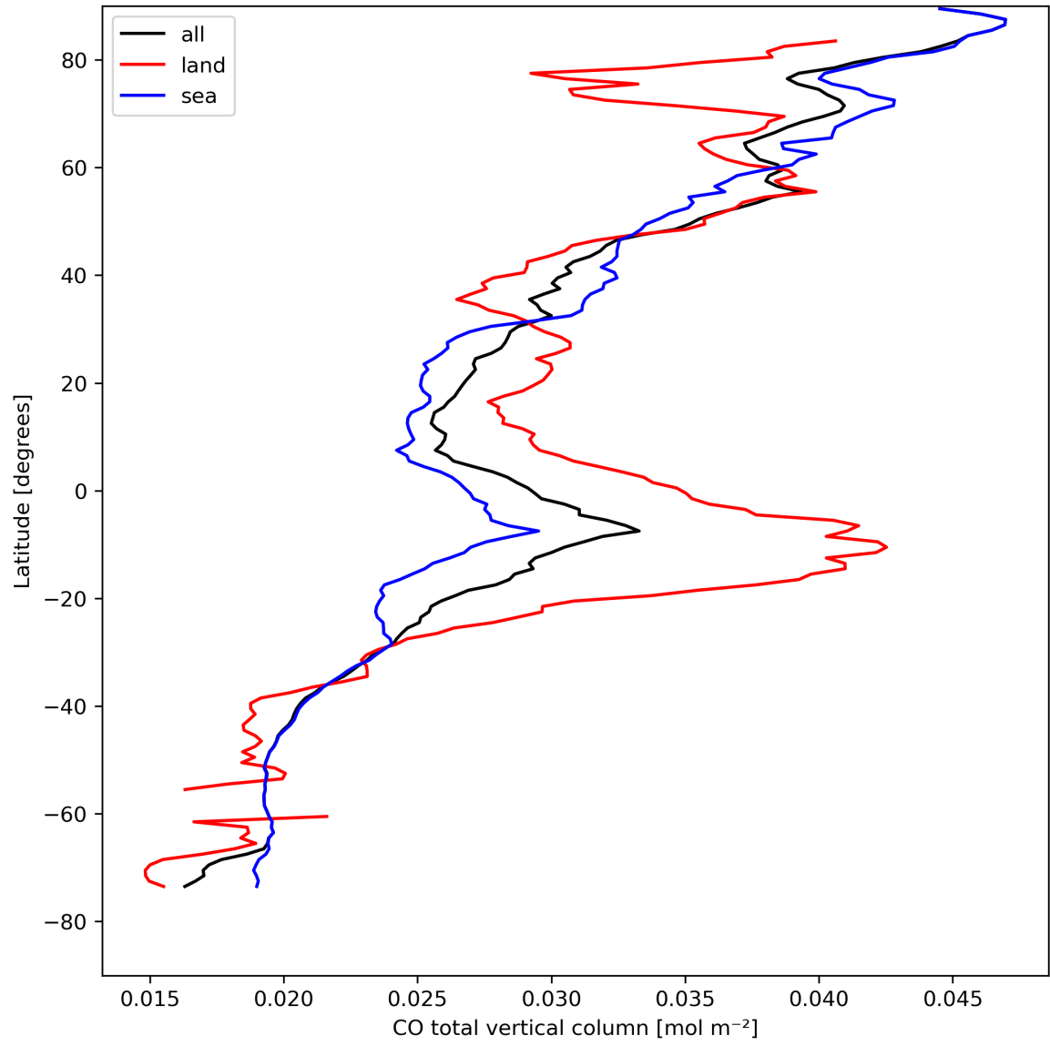
Figure 10: Zonal average of “CO total vertical column” for 2023-08-23 to 2023-08-25.
