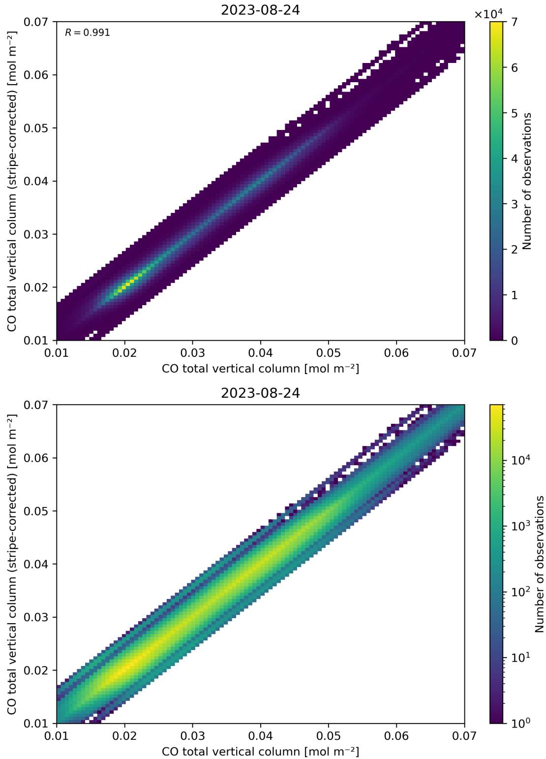
Figure 33: Scatter density plot of “CO total vertical column” against “CO total vertical column (stripe-corrected)” for 2023-08-23 to 2023-08-25.
