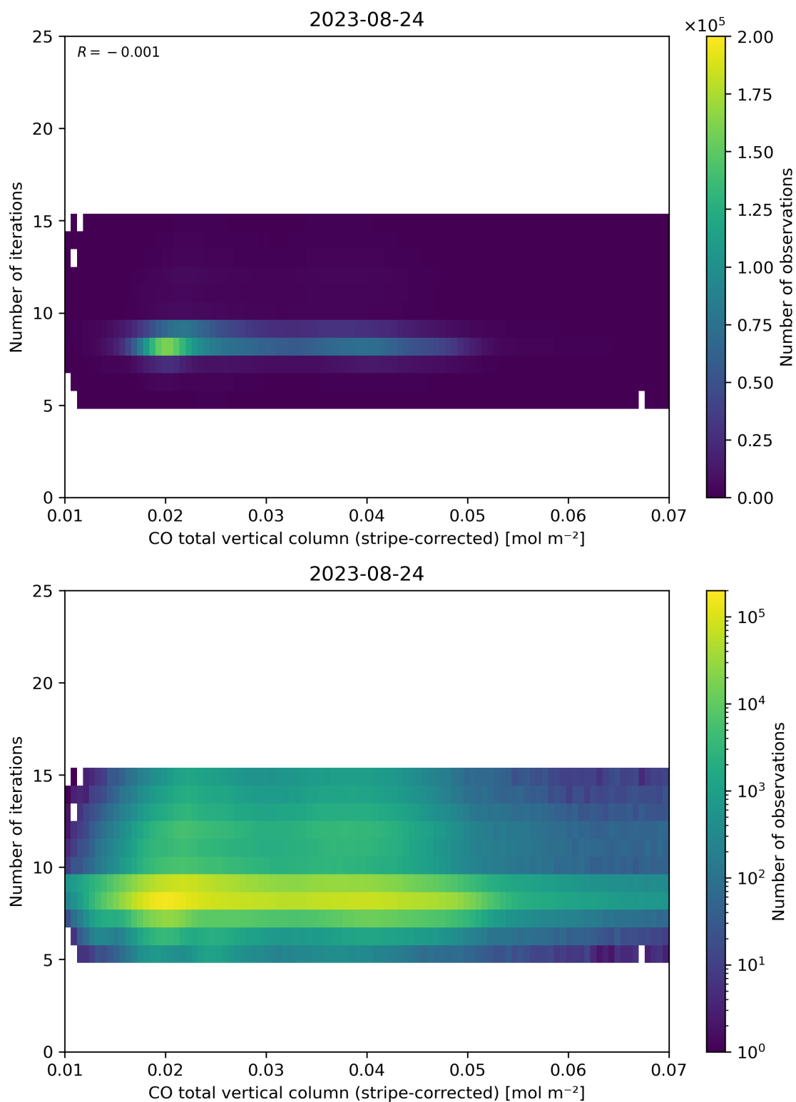
Figure 39: Scatter density plot of “CO total vertical column (stripe-corrected)” against “Number of iterations” for 2023-08-23 to 2023-08-25.
