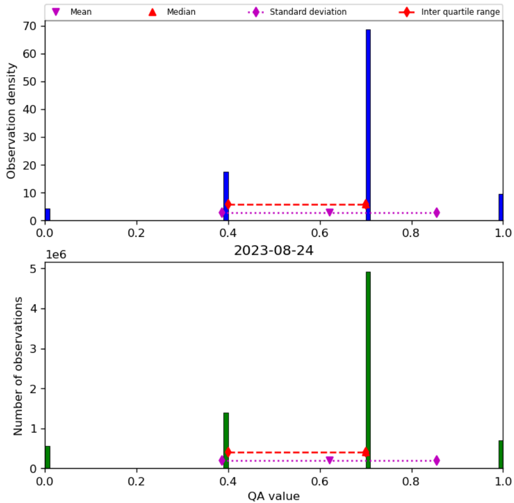
Figure 17: Histogram of “QA value” for 2023-08-23 to 2023-08-25
