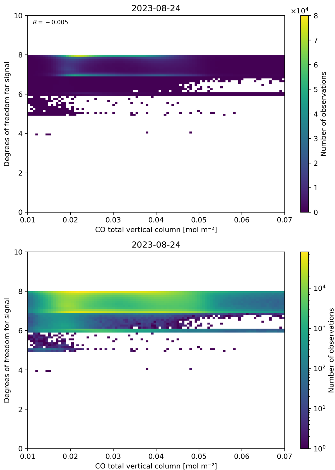
Figure 41: Scatter density plot of “CO total vertical column” against “Degrees of freedom for signal” for 2023-08-23 to 2023-08-25.
