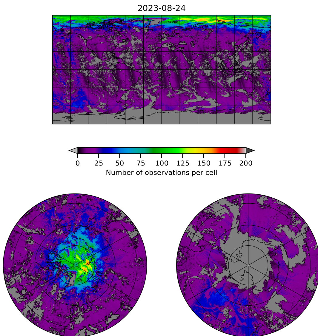
Figure 8: Map of the number of observations for 2023-08-23 to 2023-08-25
