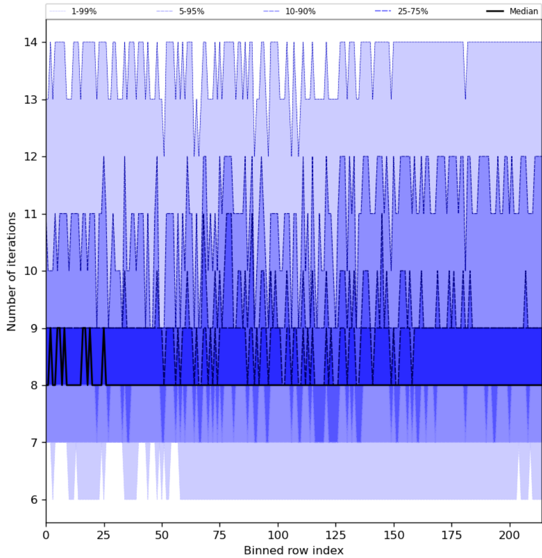
Figure 32: Along track statistics of “Number of iterations” for 2023-08-23 to 2023-08-25
