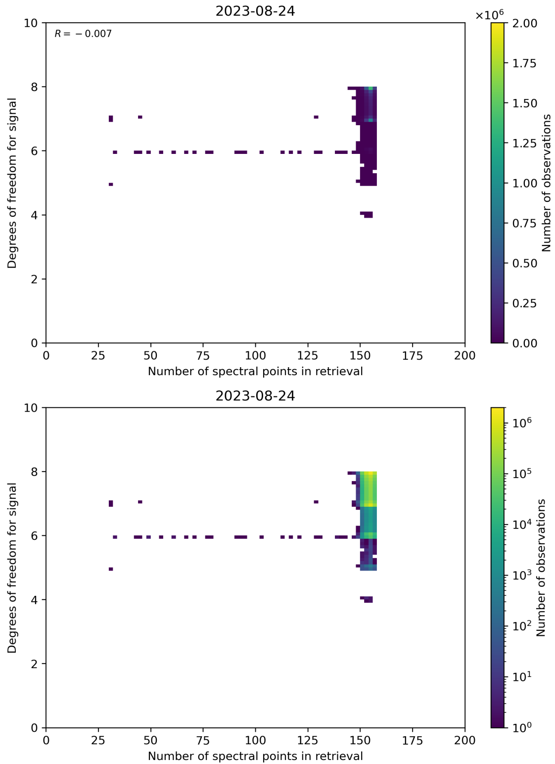
Figure 59: Scatter density plot of “Number of spectral points in retrieval” against “Degrees of freedom for signal” for 2023-08-23 to 2023-08-25.
