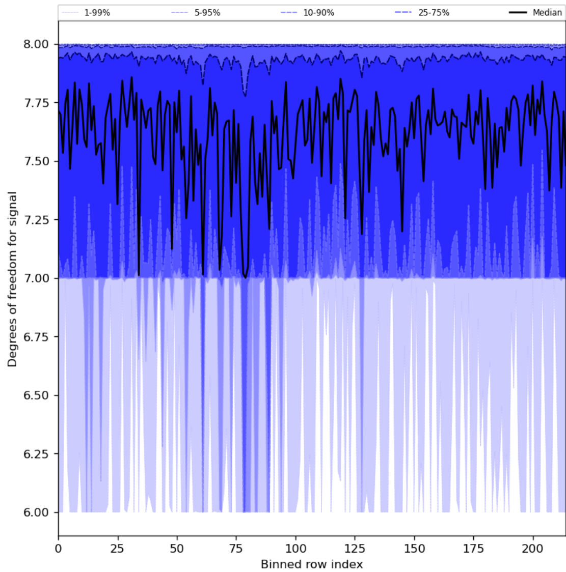
Figure 31: Along track statistics of “Degrees of freedom for signal” for 2023-08-23 to 2023-08-25
