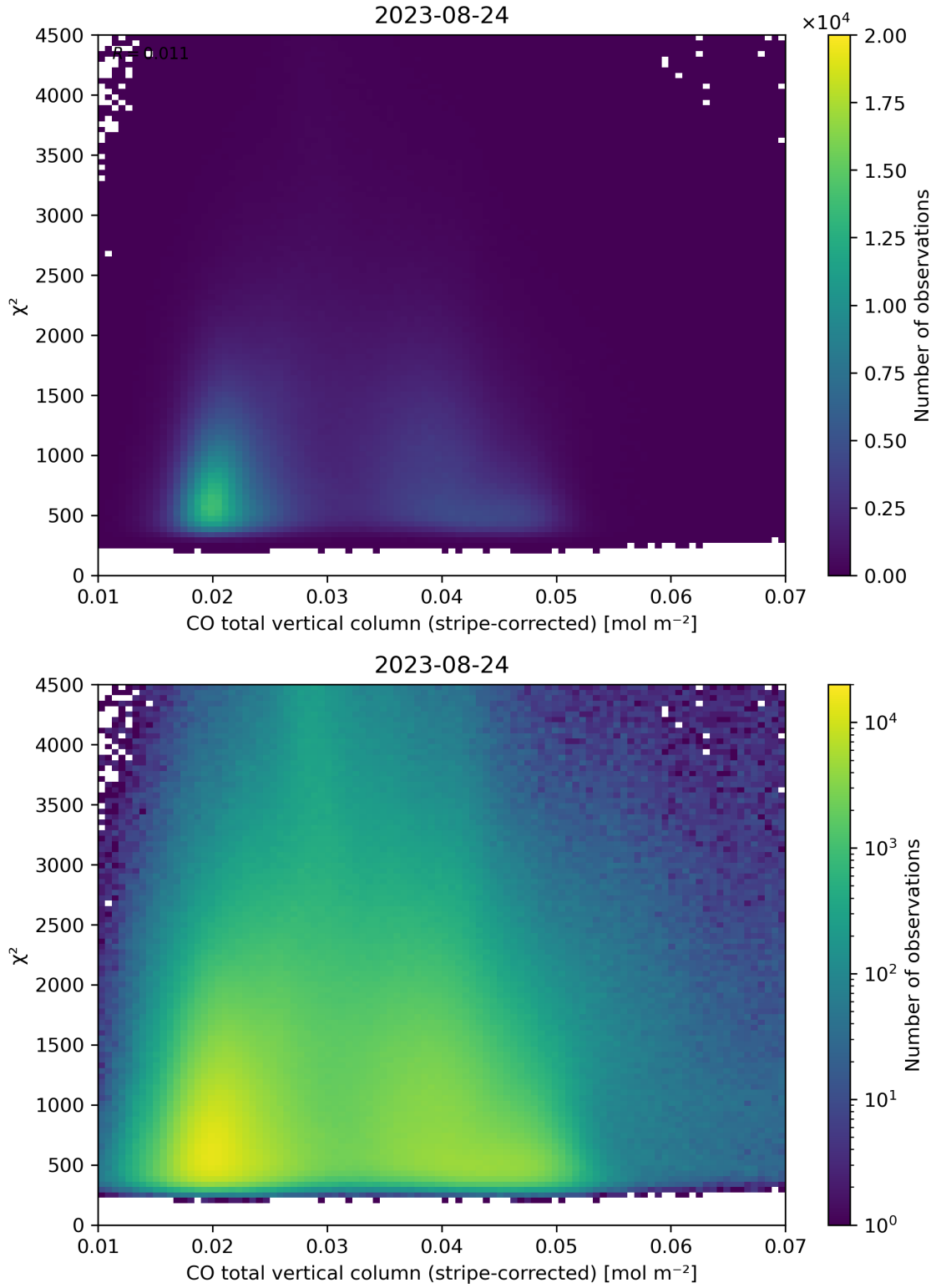
Figure 37: Scatter density plot of “CO total vertical column (stripe-corrected)” against “ \chi^2 ” for 2023-08-23 to 2023-08-25.
