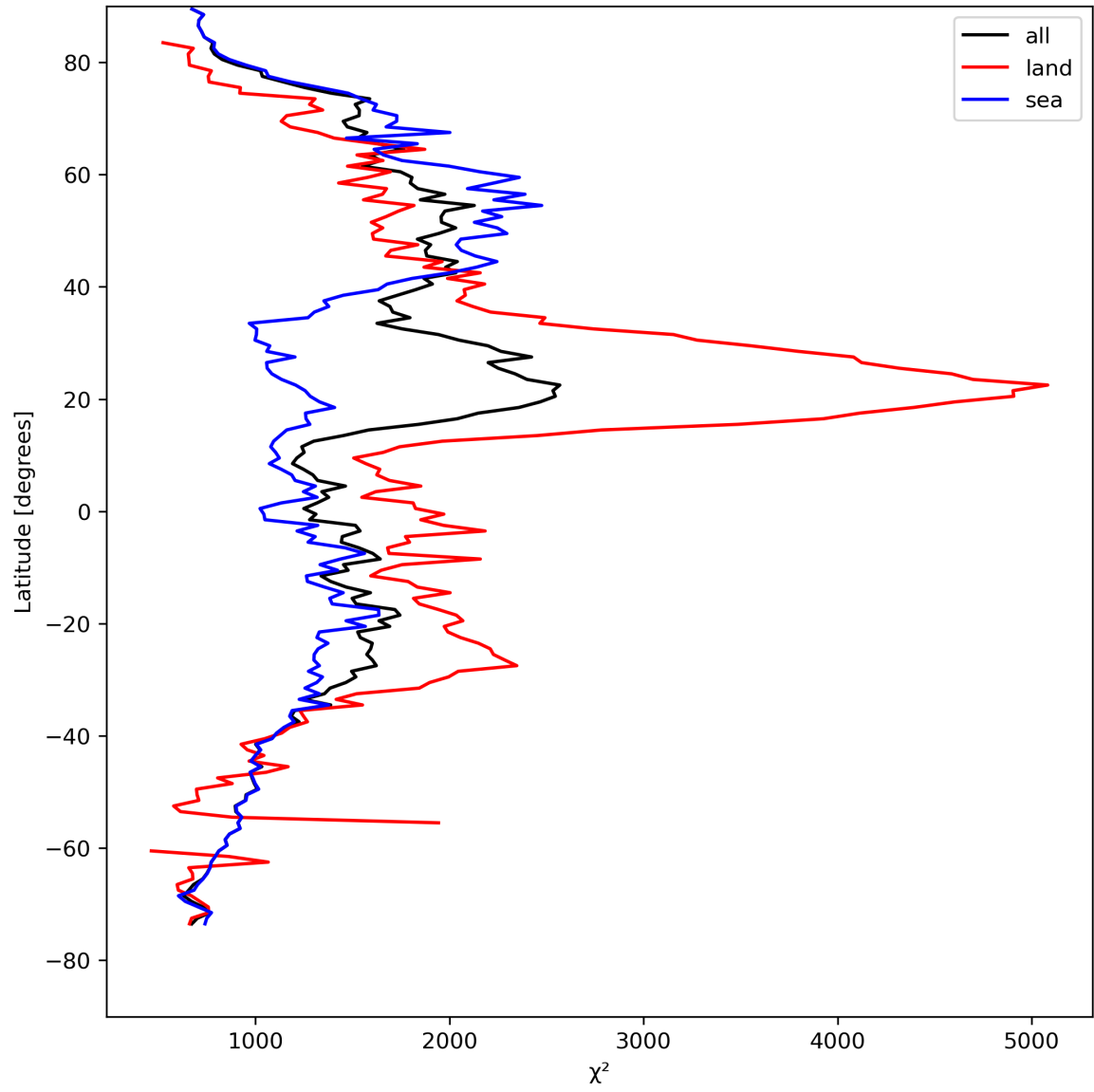
Figure 14: Zonal average of “ \chi^2 ” for 2023-08-23 to 2023-08-25.
