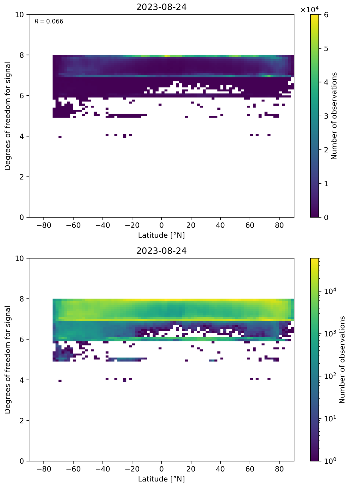
Figure 55: Scatter density plot of “Latitude” against “Degrees of freedom for signal” for 2023-08-23 to 2023-08-25.
