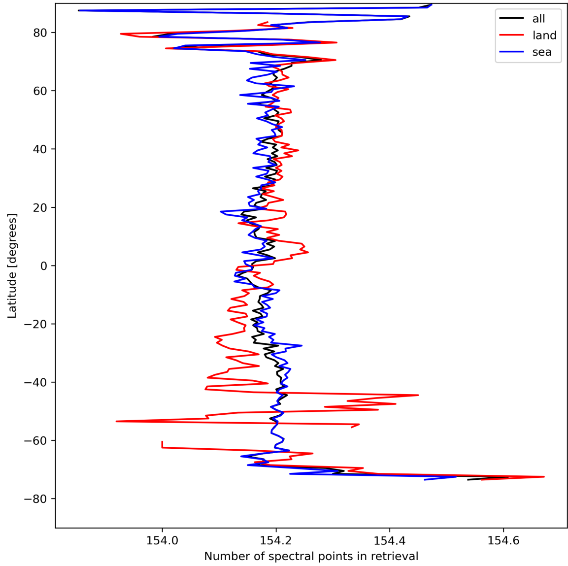
Figure 13: Zonal average of “Number of spectral points in retrieval” for 2023-08-23 to 2023-08-25.
