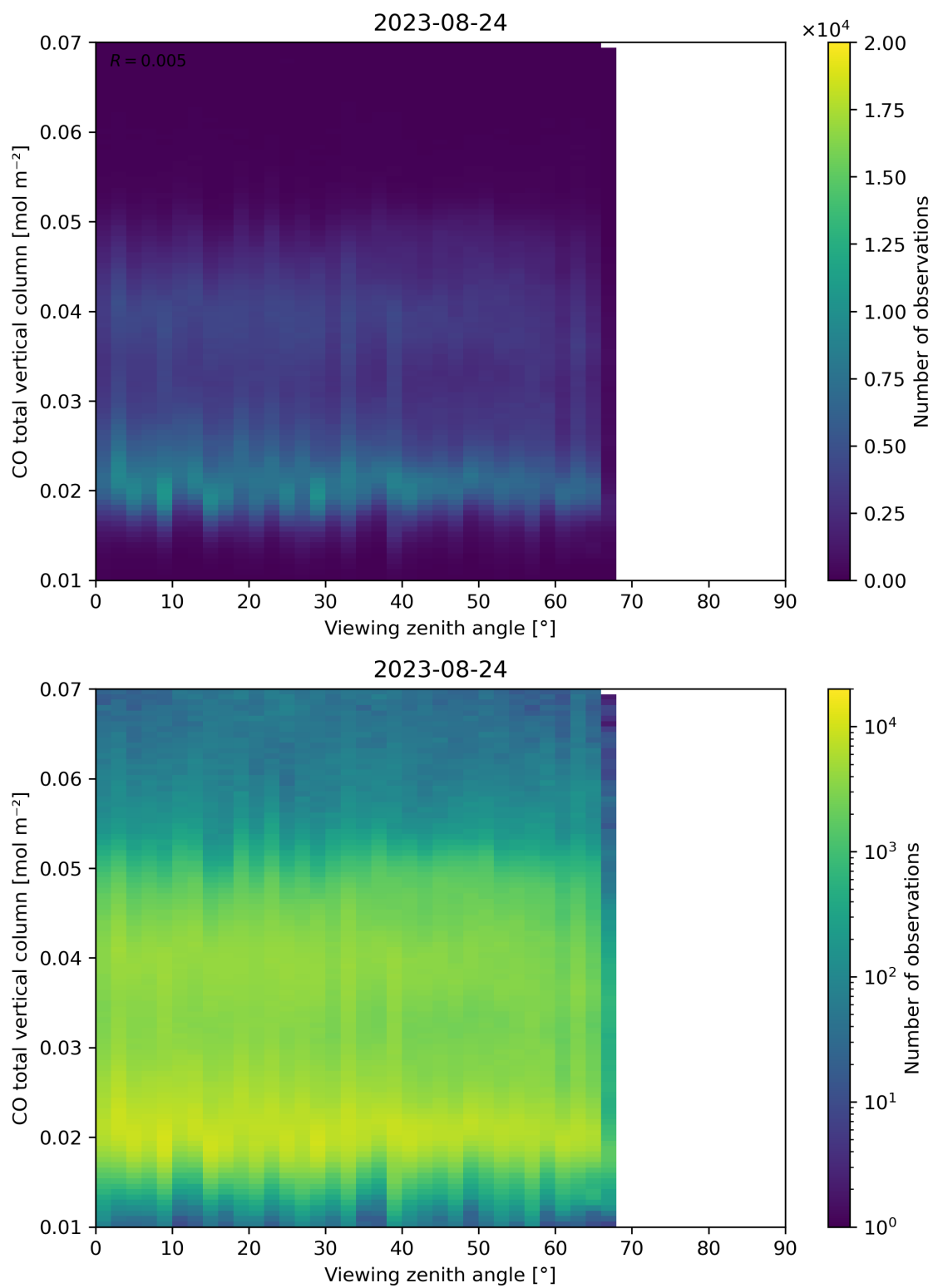
Figure 69: Scatter density plot of “Viewing zenith angle” against “CO total vertical column” for 2023-08-23 to 2023-08-25.
