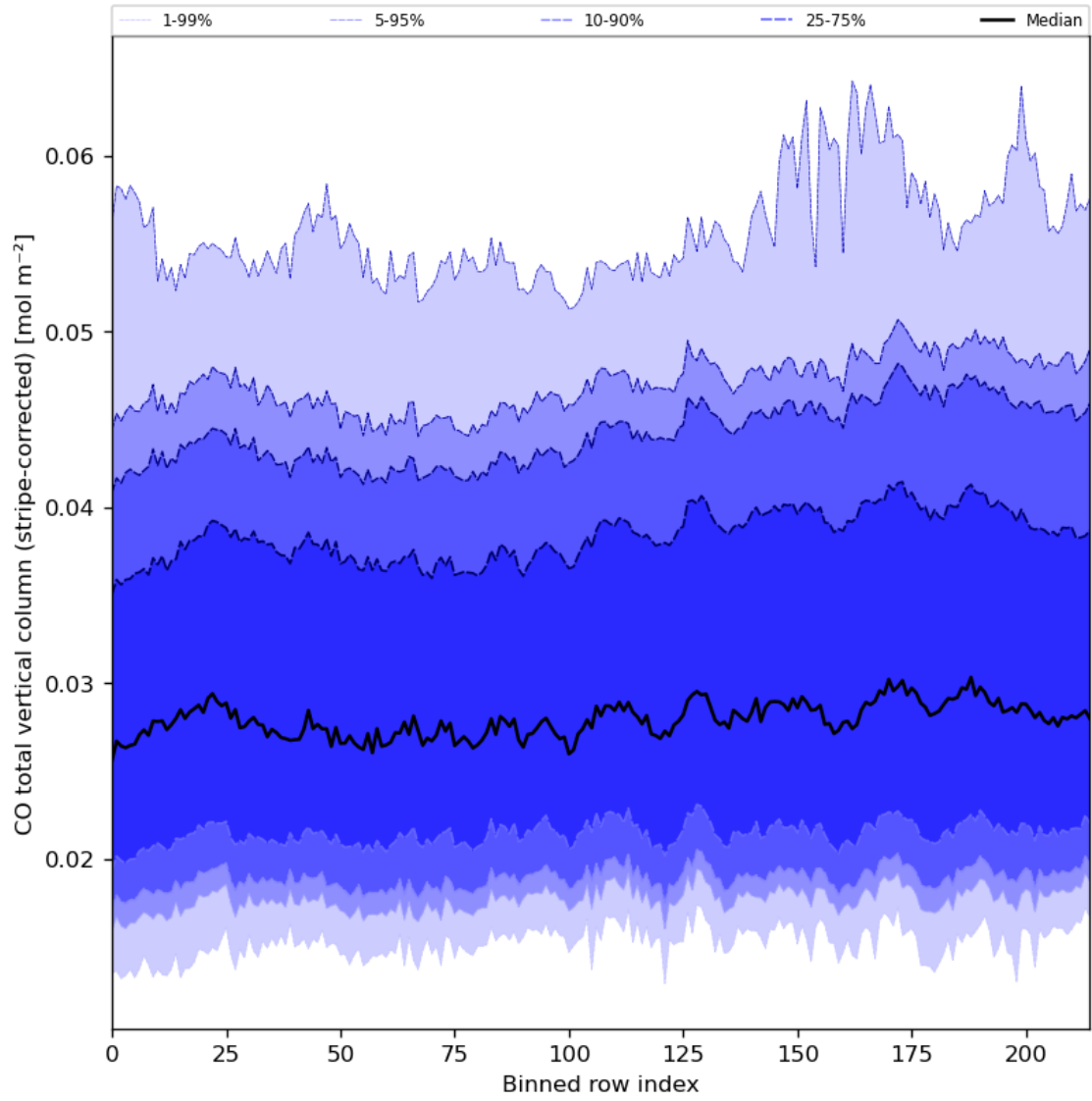
Figure 27: Along track statistics of “CO total vertical column (stripe-corrected)” for 2023-08-23 to 2023-08-25
