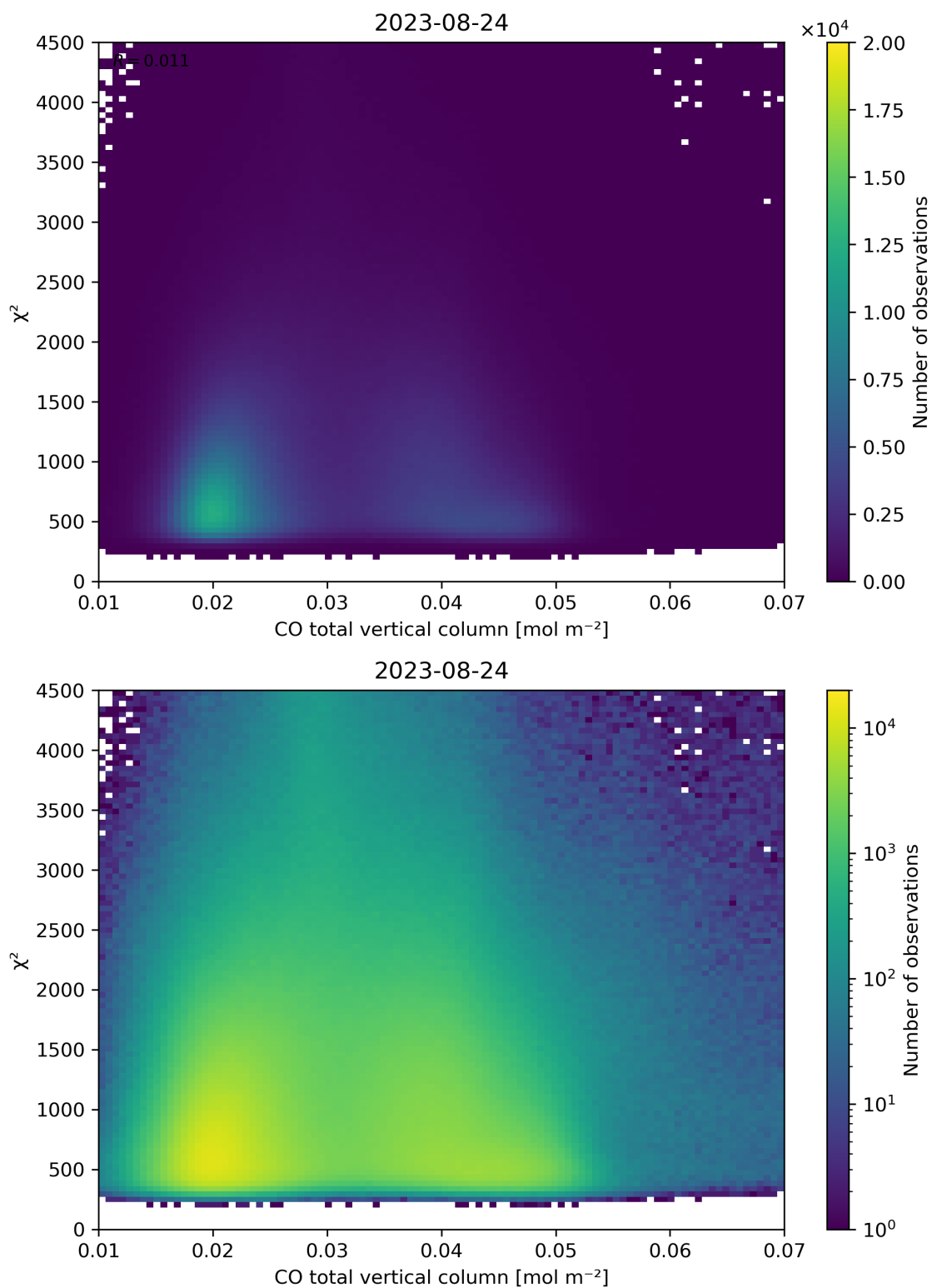
Figure 35: Scatter density plot of “CO total vertical column” against “ \chi^2 ” for 2023-08-23 to 2023-08-25.
