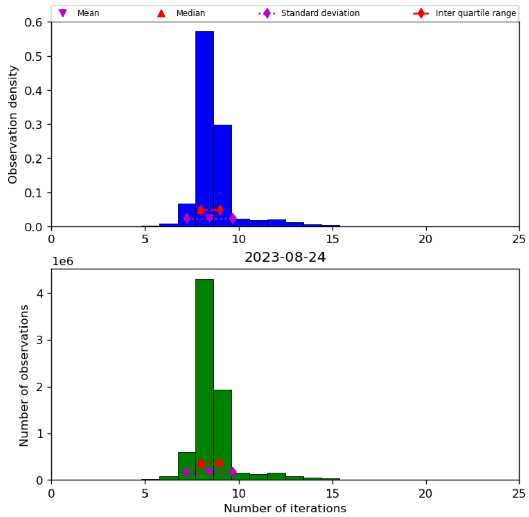
Figure 24: Histogram of “Number of iterations” for 2023-08-23 to 2023-08-25
