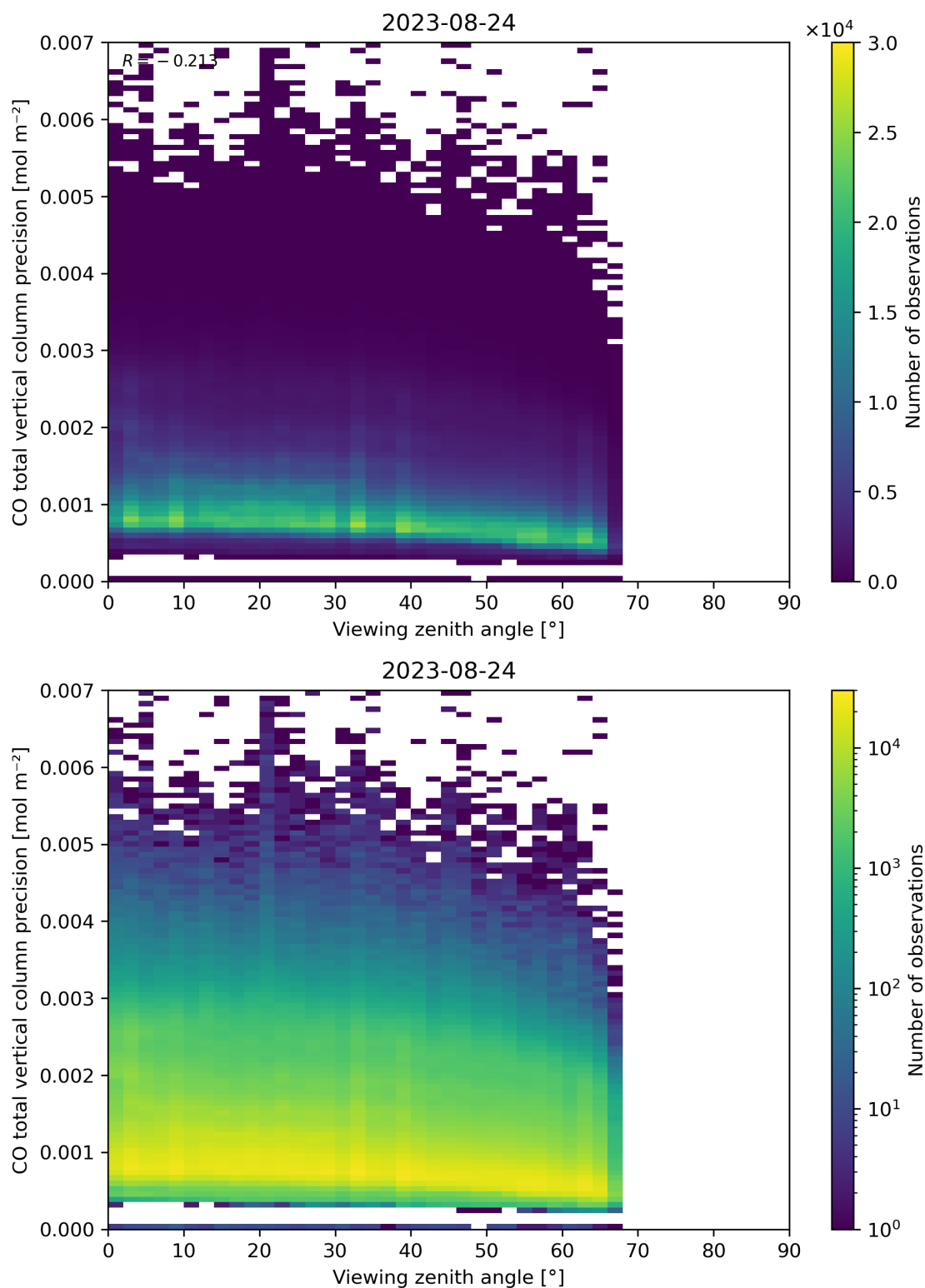
Figure 71: Scatter density plot of “Viewing zenith angle” against “CO total vertical column precision” for 2023-08-23 to 2023-08-25.
