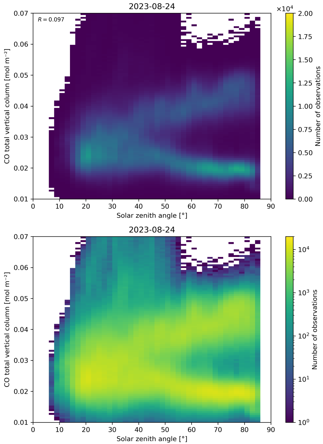
Figure 61: Scatter density plot of “Solar zenith angle” against “CO total vertical column” for 2023-08-23 to 2023-08-25.
