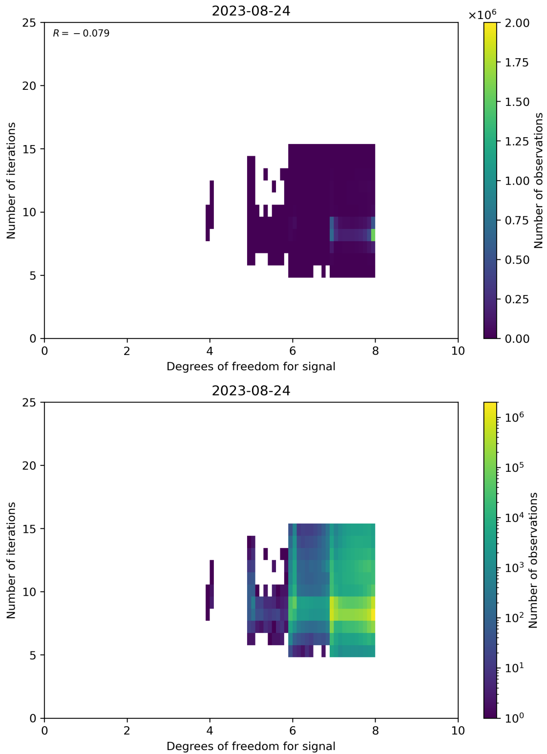
Figure 50: Scatter density plot of “Degrees of freedom for signal” against “Number of iterations” for 2023-08-23 to 2023-08-25.
