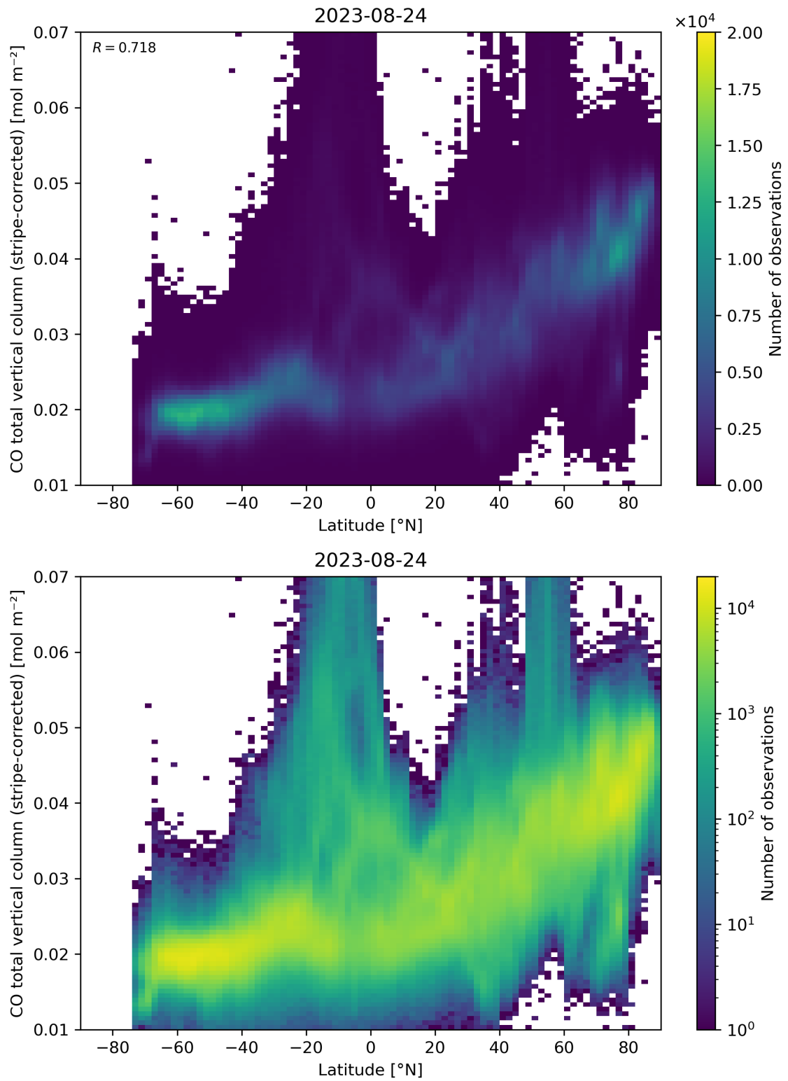
Figure 52: Scatter density plot of “Latitude” against “CO total vertical column (stripe-corrected)” for 2023-08-23 to 2023-08-25.
