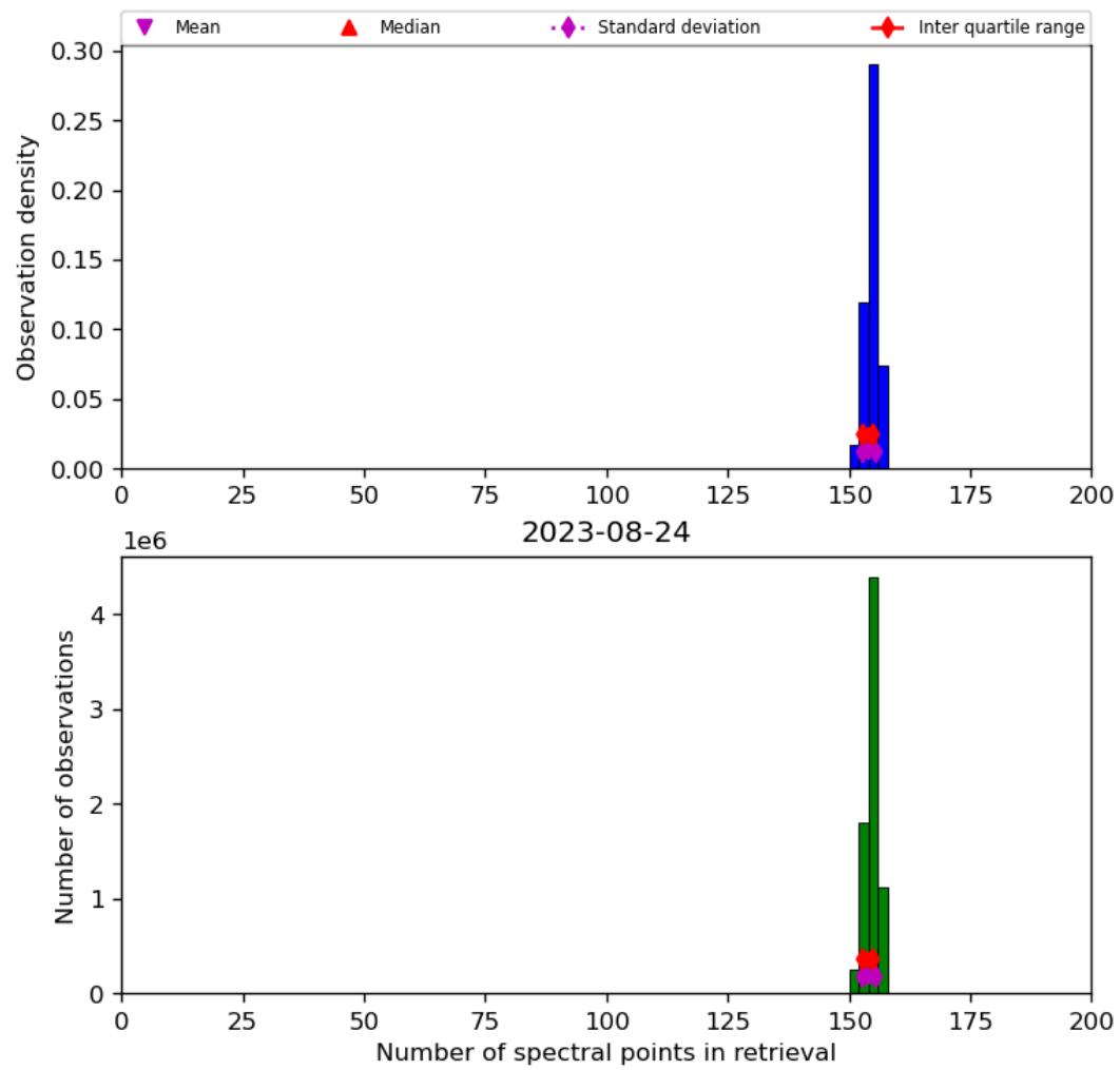
Figure 21: Histogram of “Number of spectral points in retrieval” for 2023-08-23 to 2023-08-25
