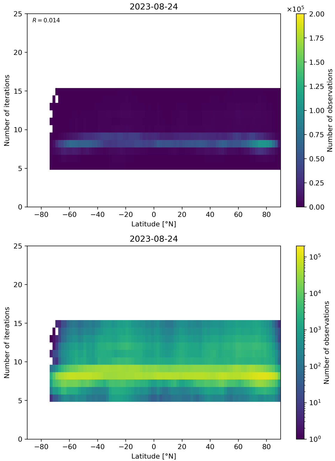
Figure 56: Scatter density plot of “Latitude” against “Number of iterations” for 2023-08-23 to 2023-08-25.
