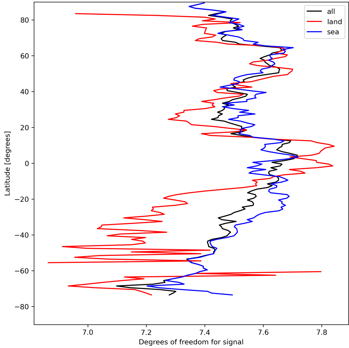
Figure 15: Zonal average of “Degrees of freedom for signal” for 2023-08-23 to 2023-08-25.
