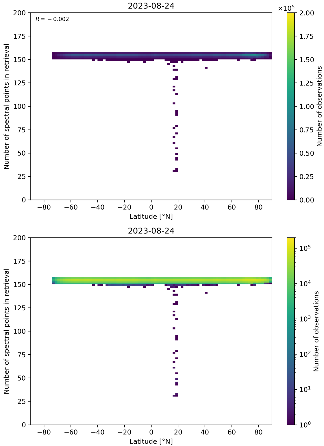
Figure 57: Scatter density plot of “Latitude” against “Number of spectral points in retrieval” for 2023-08-23 to 2023-08-25.
