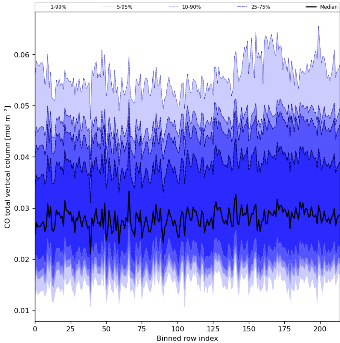
Figure 26: Along track statistics of “CO total vertical column” for 2023-08-23 to 2023-08-25
