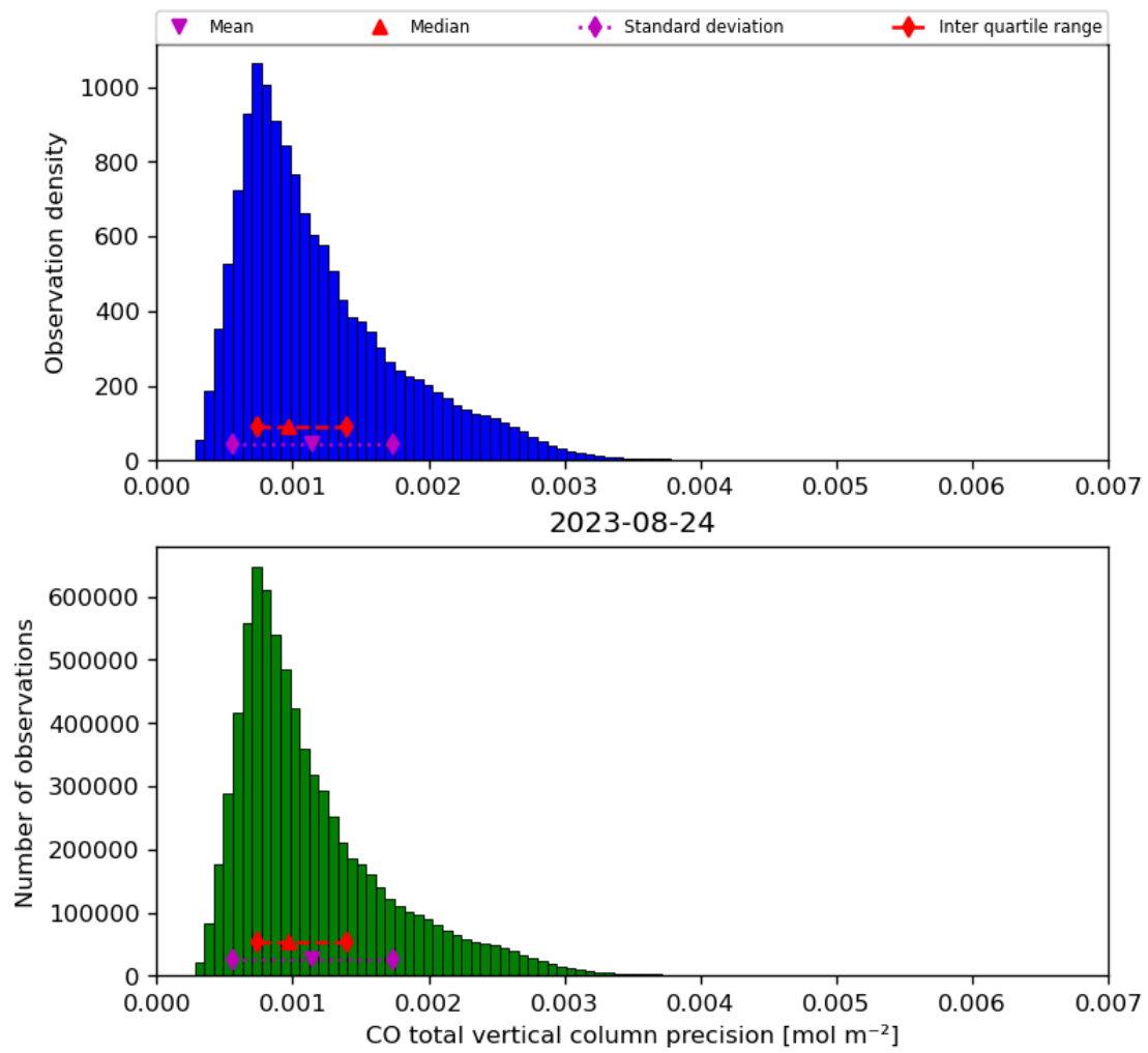
Figure 20: Histogram of “CO total vertical column precision” for 2023-08-23 to 2023-08-25
