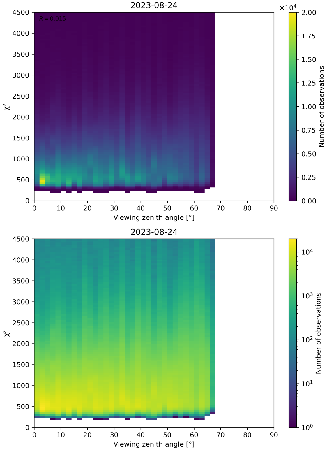
Figure 72: Scatter density plot of “Viewing zenith angle” against “ \chi^2 ” for 2023-08-23 to 2023-08-25.
