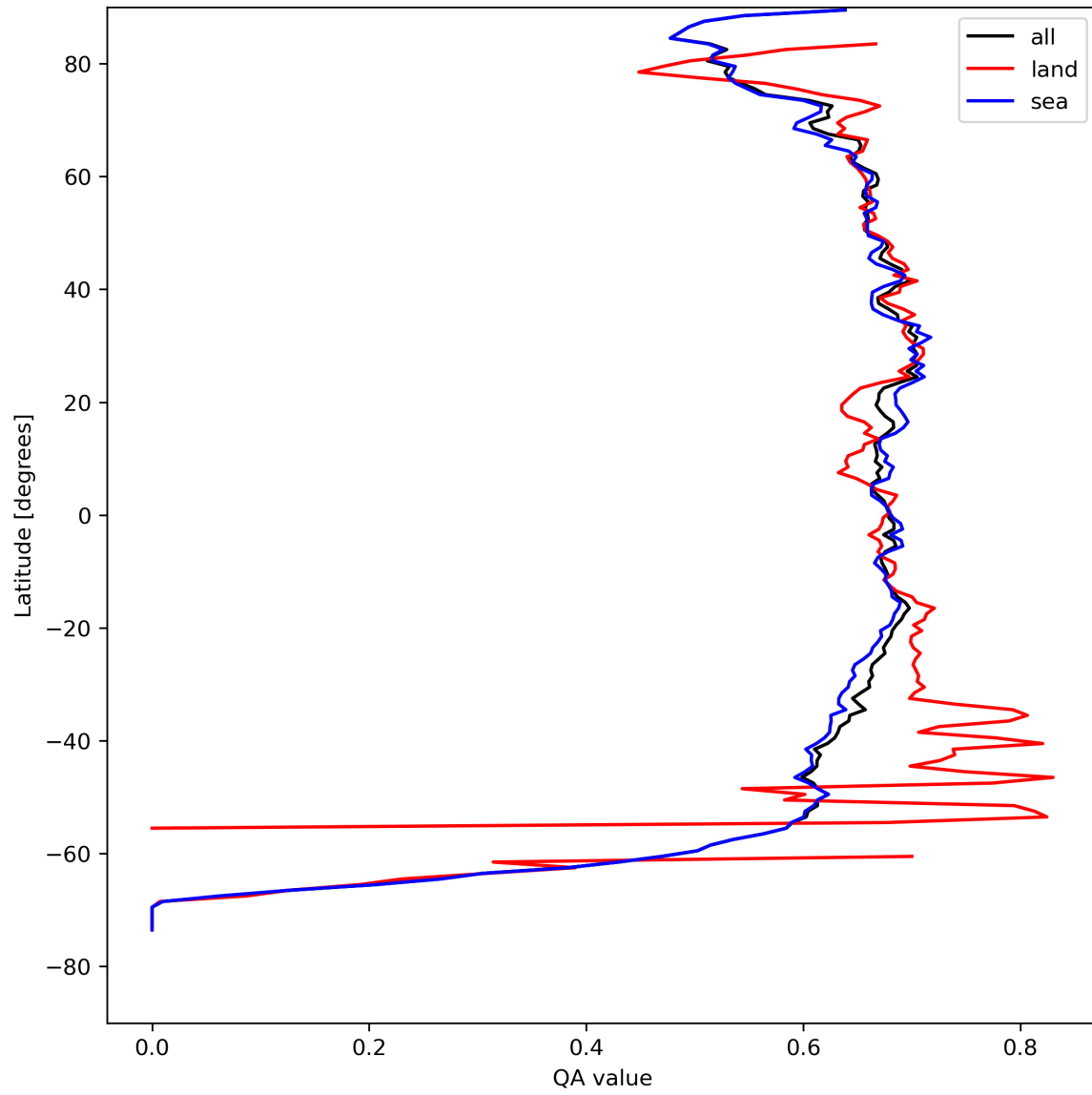
Figure 9: Zonal average of “QA value” for 2023-08-23 to 2023-08-25.
