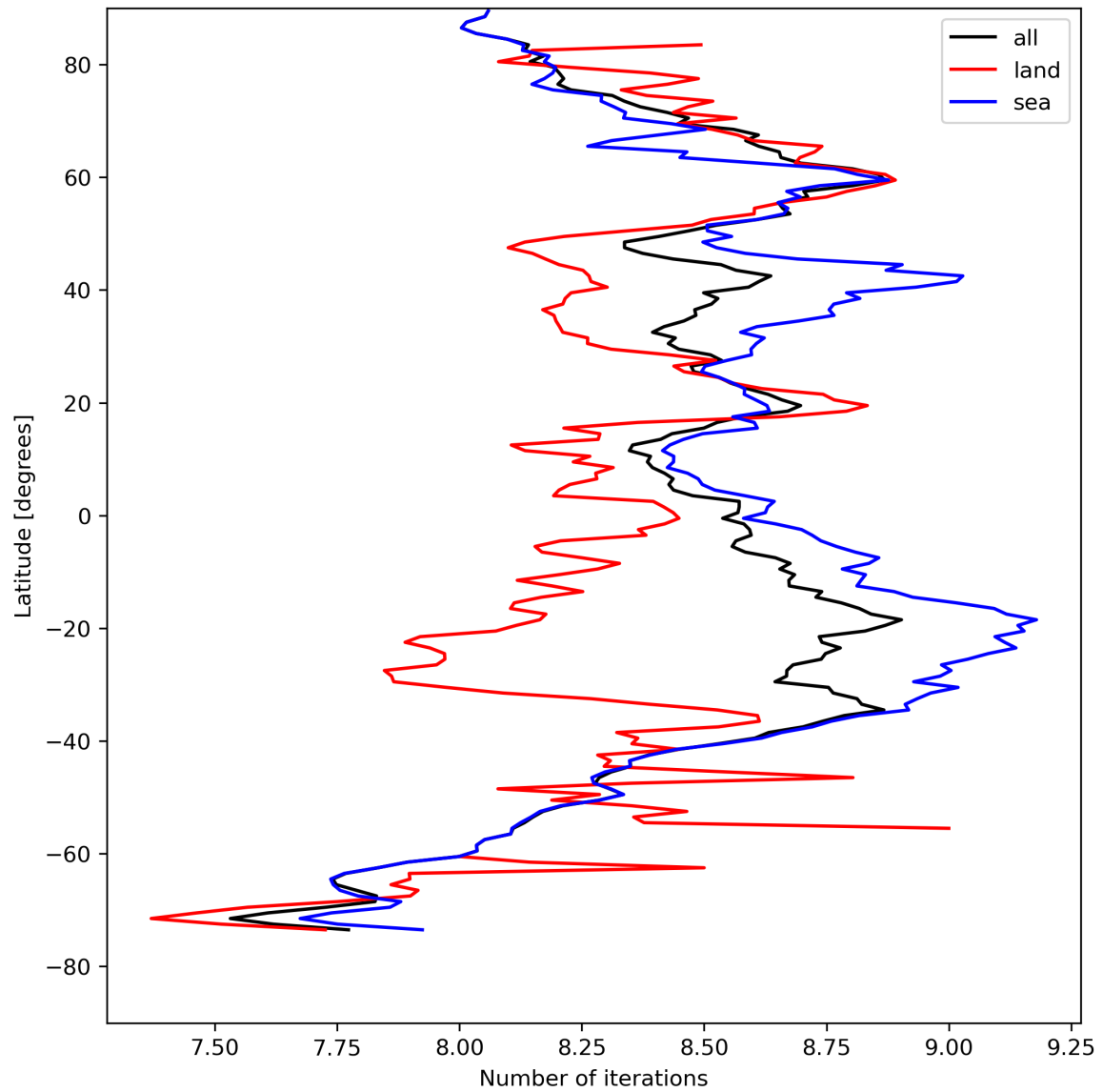
Figure 16: Zonal average of “Number of iterations” for 2023-08-23 to 2023-08-25.
