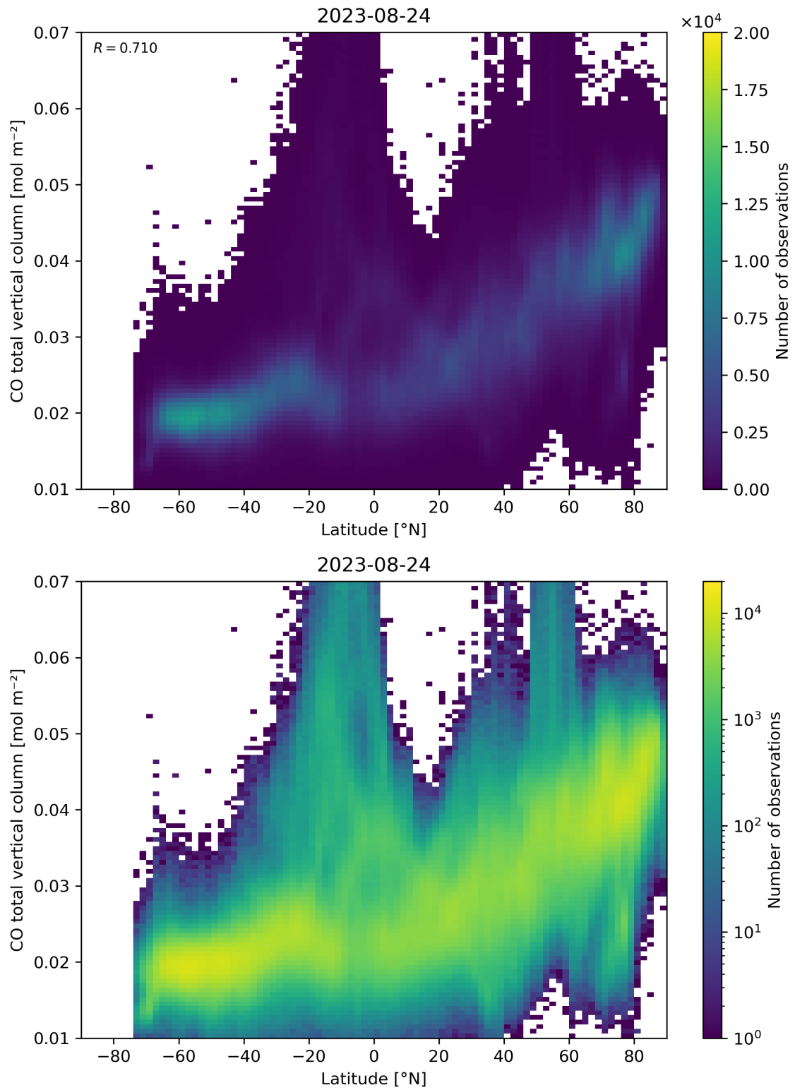
Figure 51: Scatter density plot of “Latitude” against “CO total vertical column” for 2023-08-23 to 2023-08-25.
