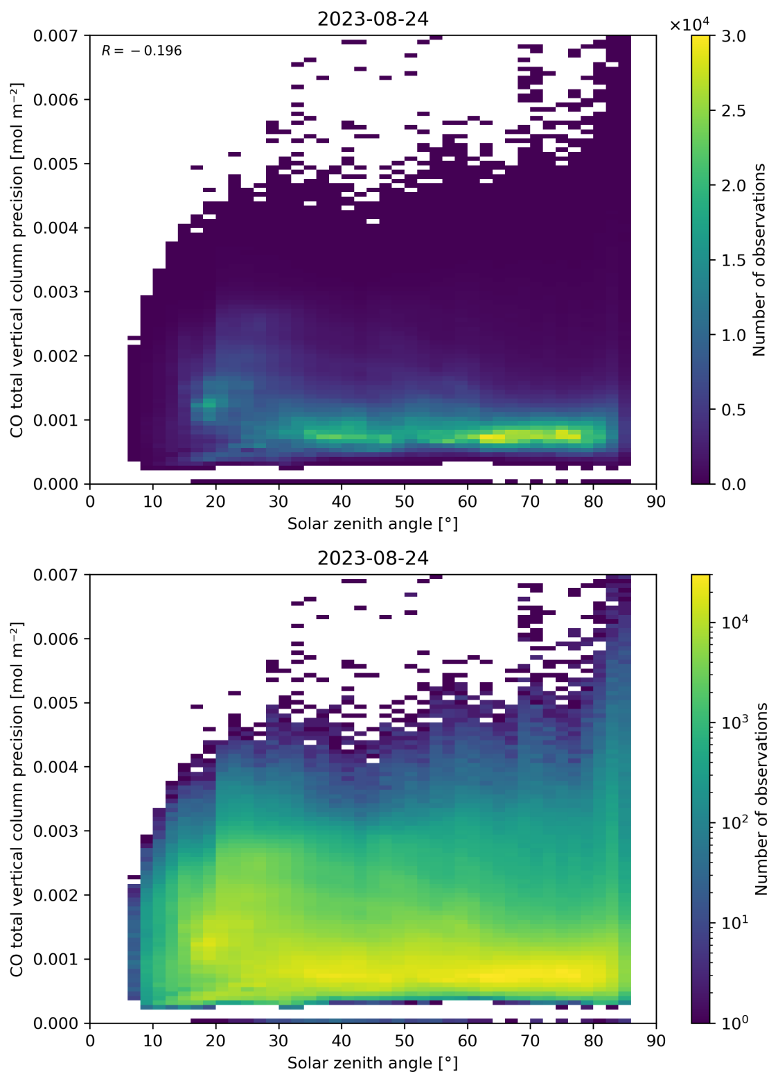
Figure 63: Scatter density plot of “Solar zenith angle” against “CO total vertical column precision” for 2023-08-23 to 2023-08-25.
