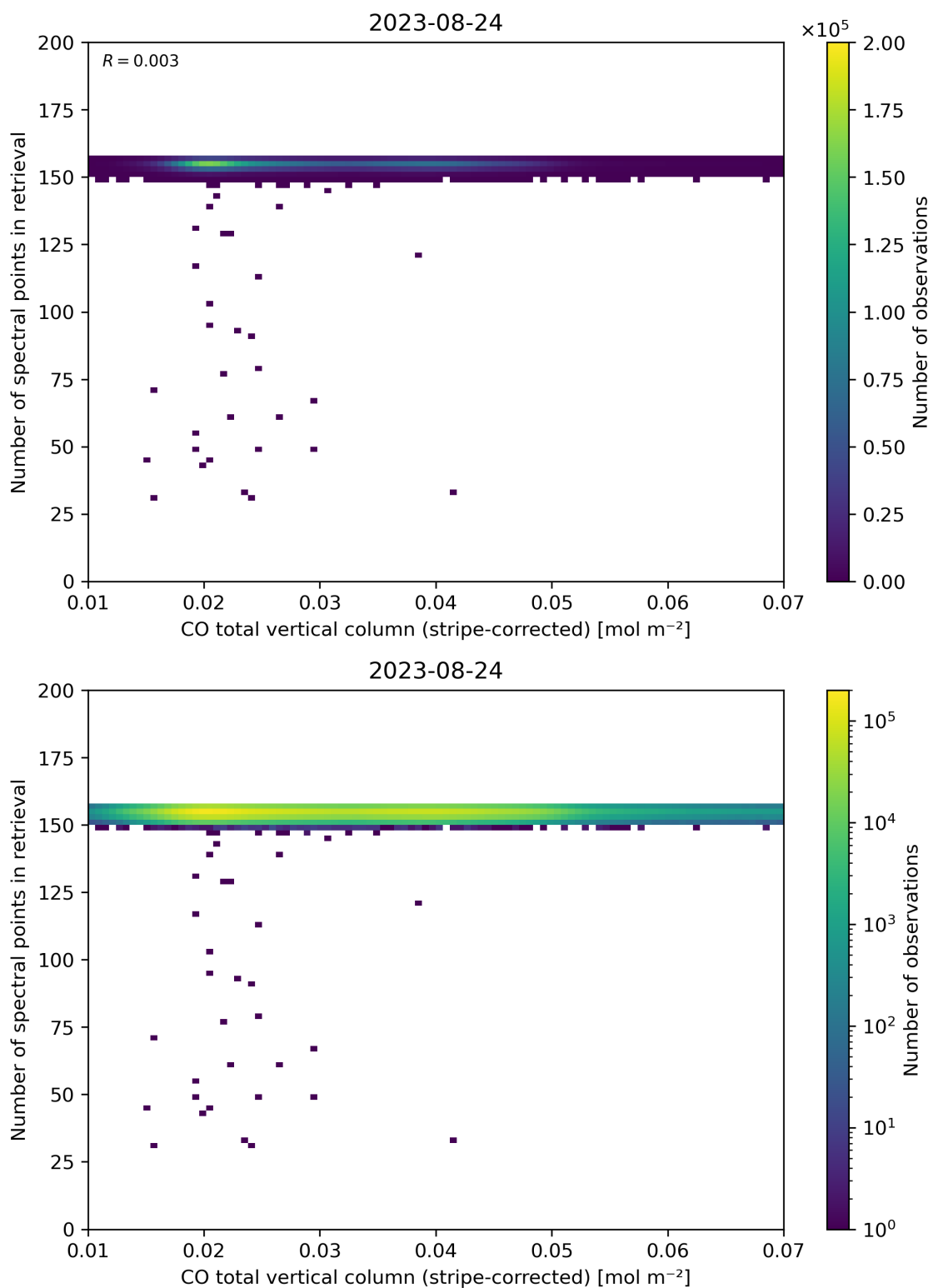
Figure 40: Scatter density plot of “CO total vertical column (stripe-corrected)” against “Number of spectral points in retrieval” for 2023-08-23 to 2023-08-25.
