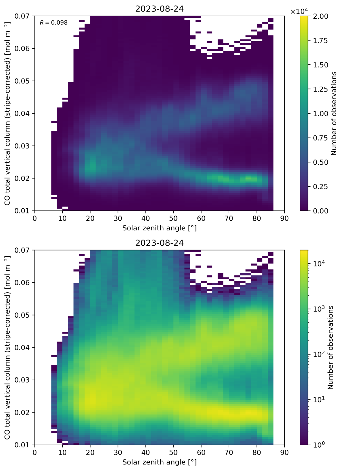
Figure 62: Scatter density plot of “Solar zenith angle” against “CO total vertical column (stripe-corrected)” for 2023-08-23 to 2023-08-25.
