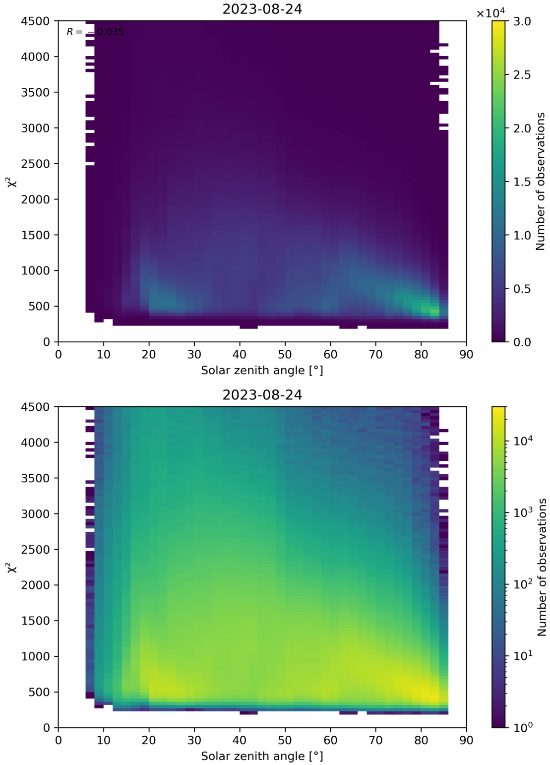
Figure 64: Scatter density plot of “Solar zenith angle” against “ \chi^2 ” for 2023-08-23 to 2023-08-25.
