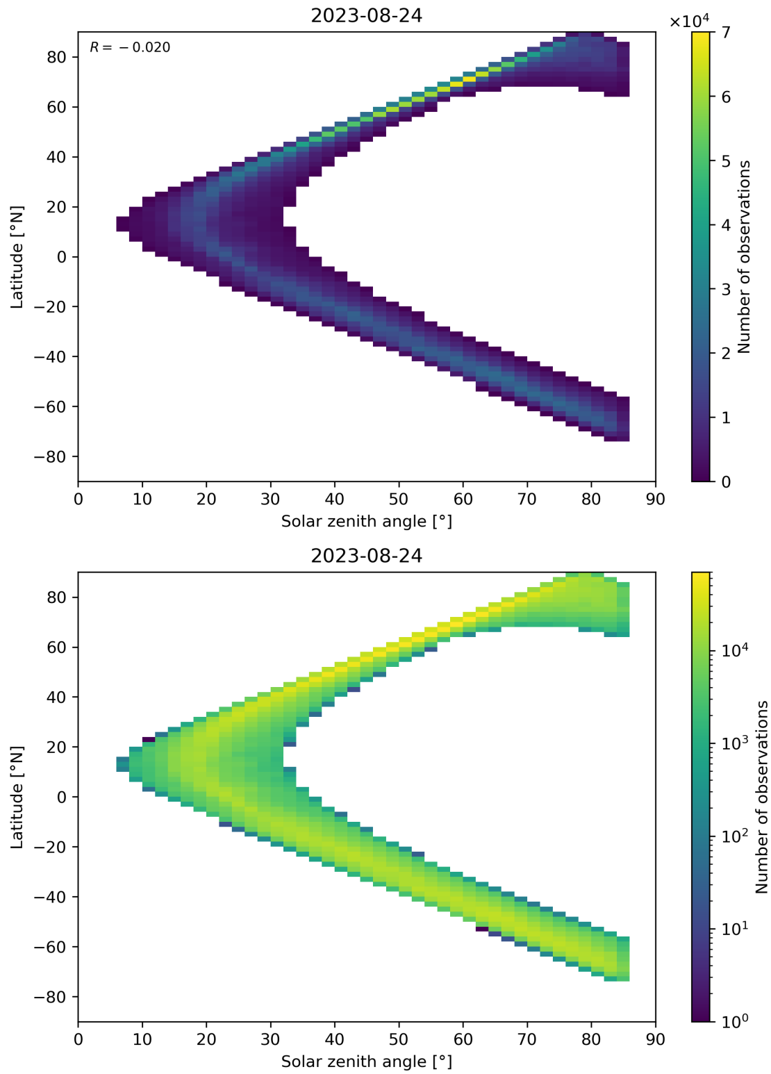
Figure 66: Scatter density plot of “Solar zenith angle” against “Latitude” for 2023-08-23 to 2023-08-25.
