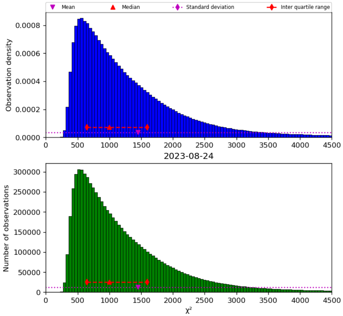
Figure 22: Histogram of “ \chi^2 ” for 2023-08-23 to 2023-08-25
