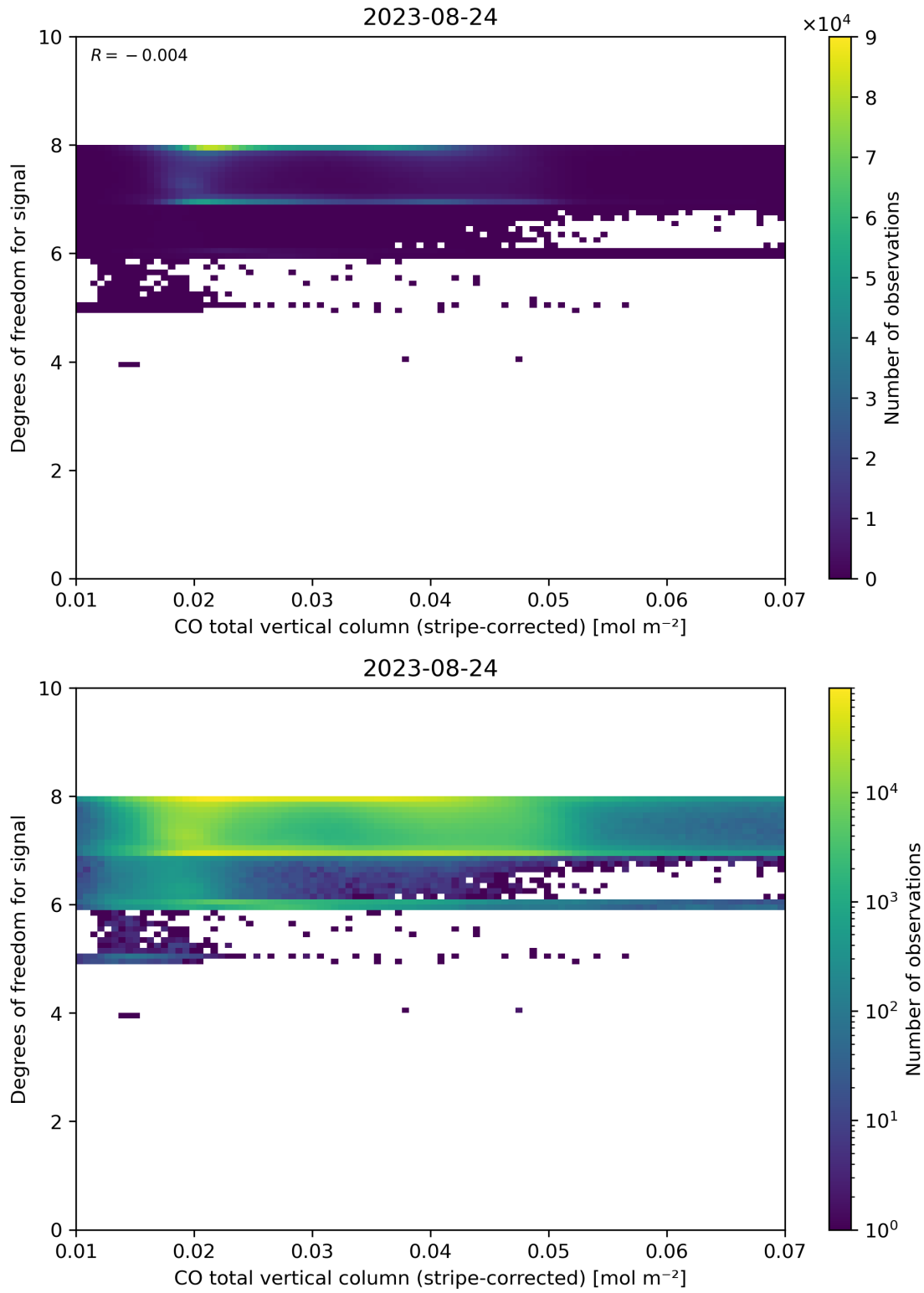
Figure 38: Scatter density plot of “CO total vertical column (stripe-corrected)” against “Degrees of freedom for signal” for 2023-08-23 to 2023-08-25.
