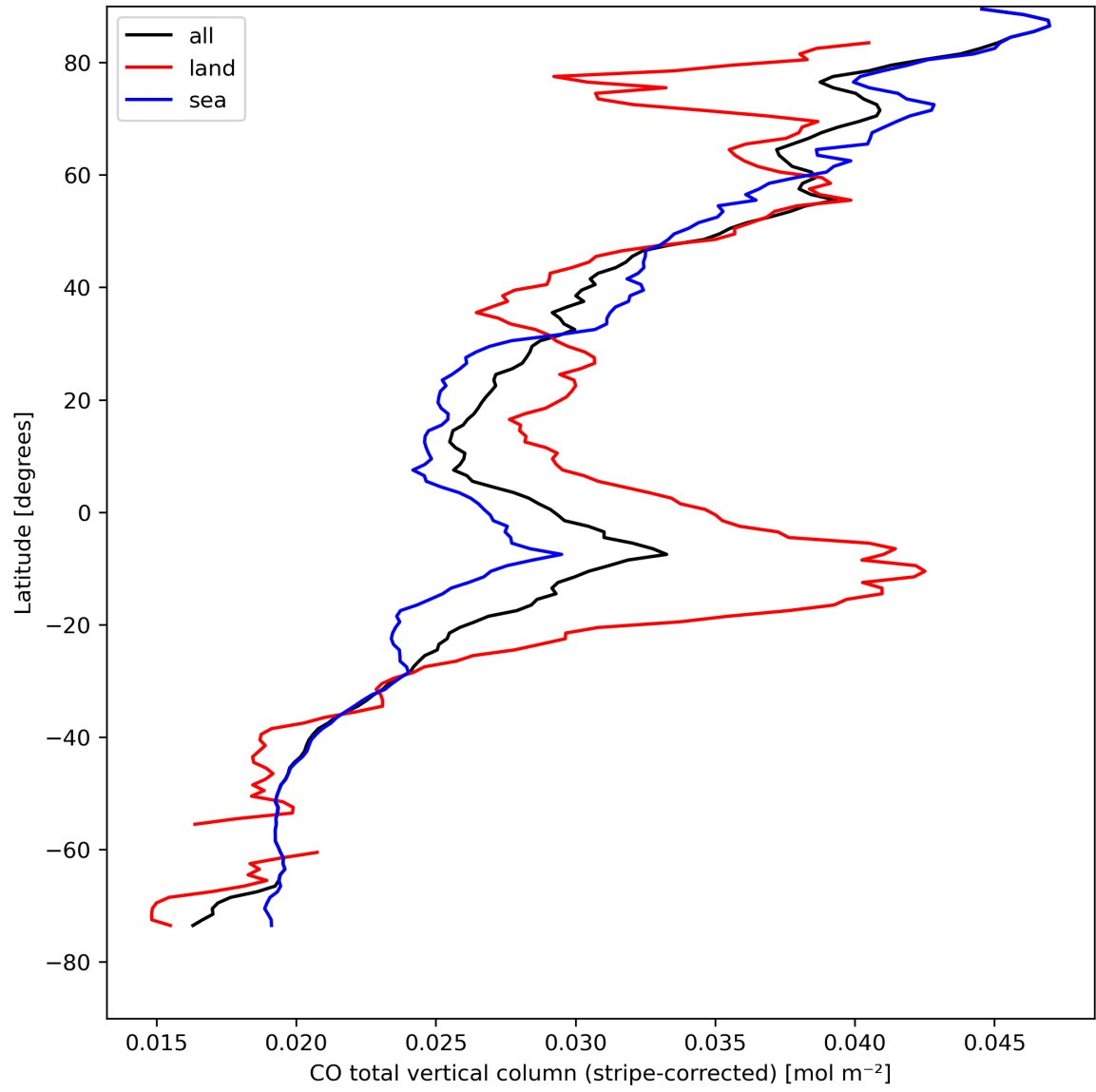
Figure 11: Zonal average of “CO total vertical column (stripe-corrected)” for 2023-08-23 to 2023-08-25.
