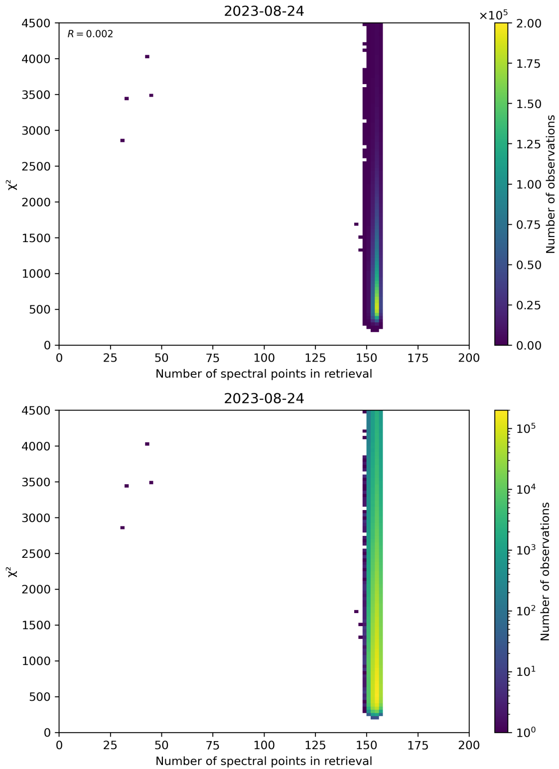
Figure 58: Scatter density plot of “Number of spectral points in retrieval” against “ \chi^2 ” for 2023-08-23 to 2023-08-25.
