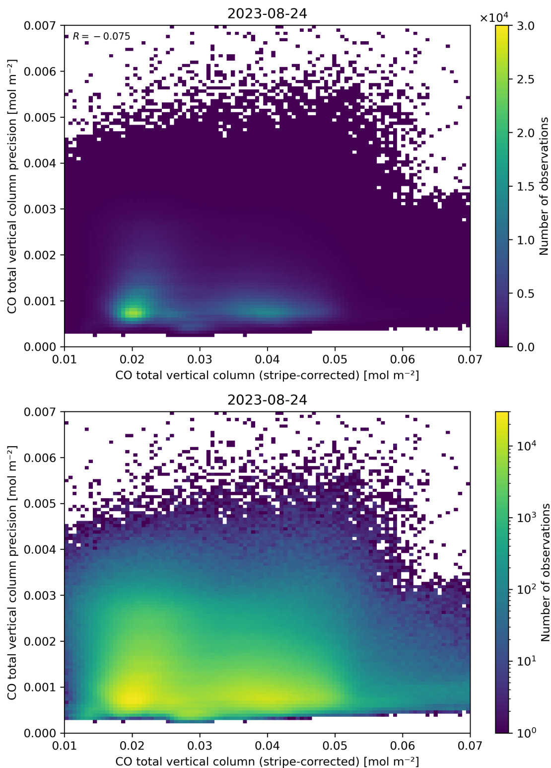
Figure 36: Scatter density plot of “CO total vertical column (stripe-corrected)” against “CO total vertical column precision” for 2023-08-23 to 2023-08-25.
