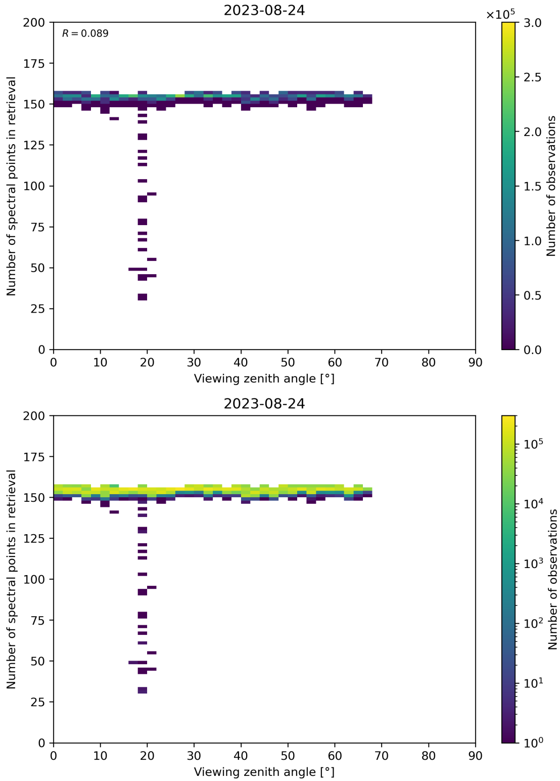
Figure 76: Scatter density plot of “Viewing zenith angle” against “Number of spectral points in retrieval” for 2023-08-23 to 2023-08-25.
