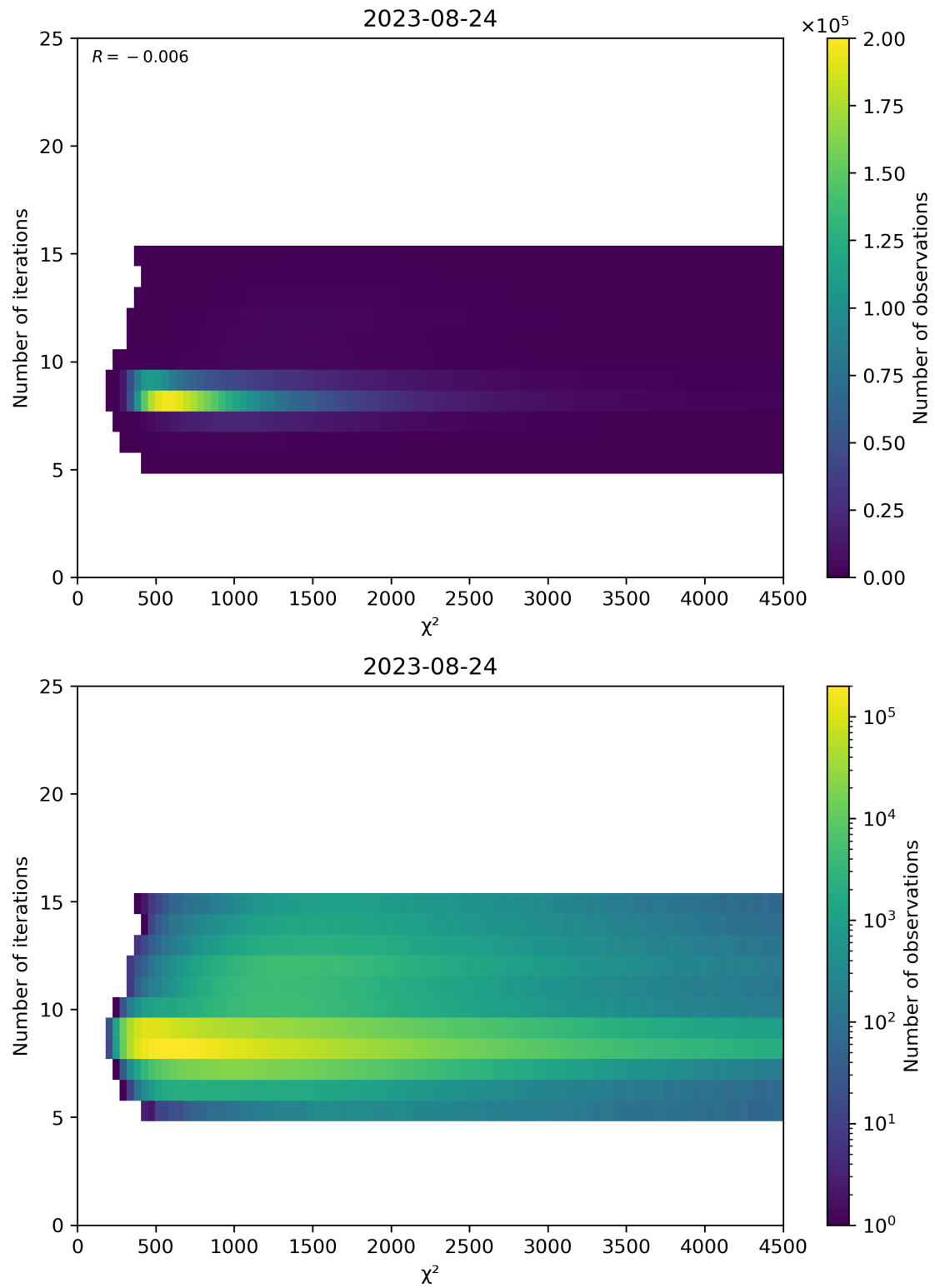
Figure 49: Scatter density plot of “ \chi^2 ” against “Number of iterations” for 2023-08-23 to 2023-08-25.
