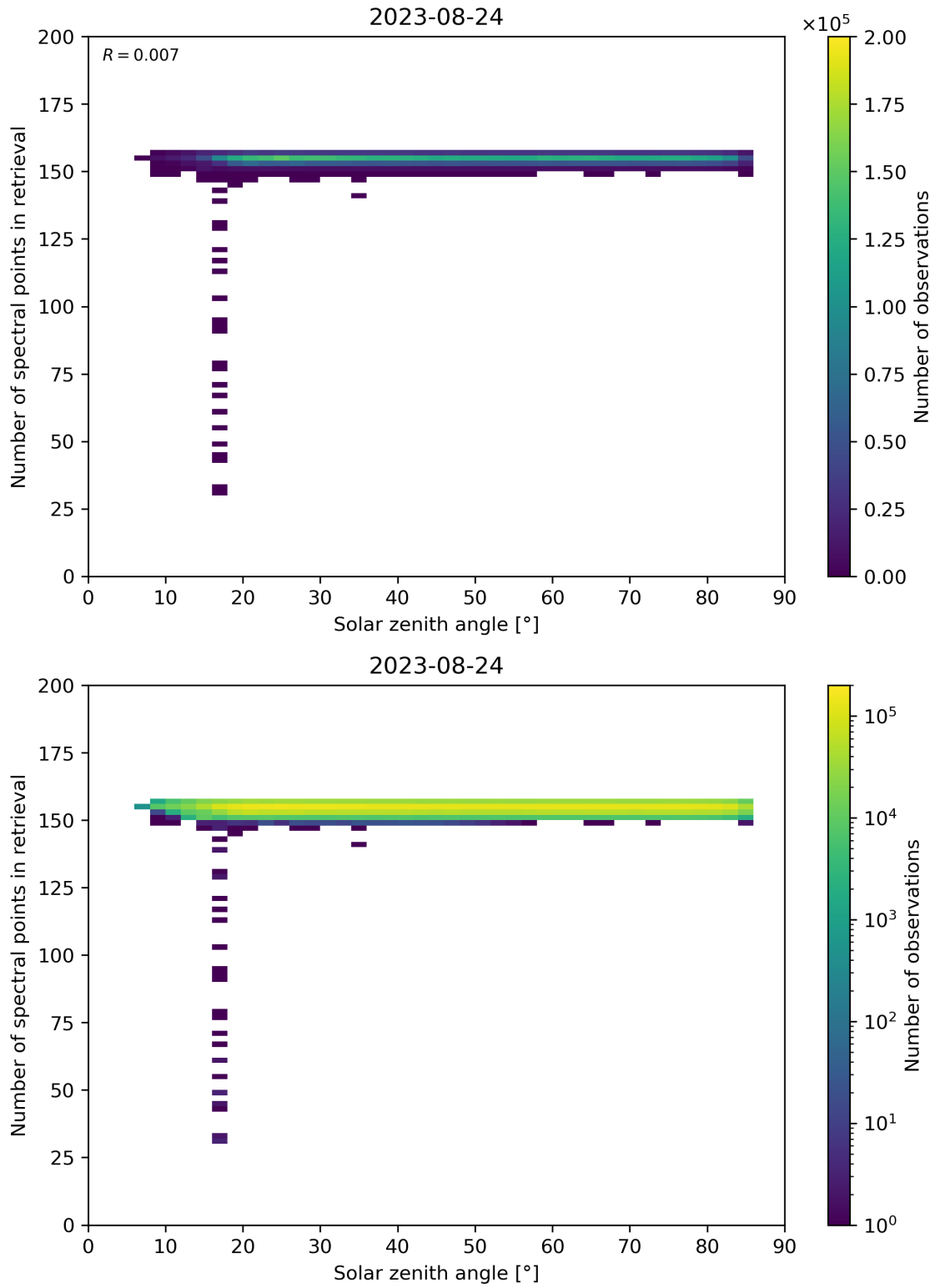
Figure 68: Scatter density plot of “Solar zenith angle” against “Number of spectral points in retrieval” for 2023-08-23 to 2023-08-25.
