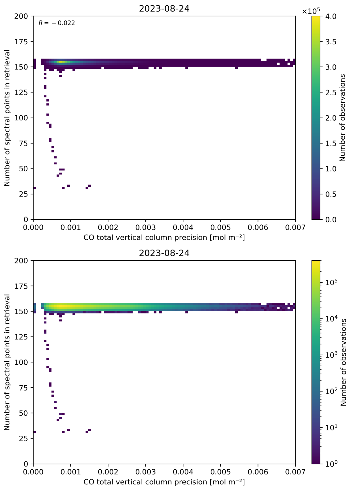
Figure 47: Scatter density plot of “CO total vertical column precision” against “Number of spectral points in retrieval” for 2023-08-23 to 2023-08-25.
