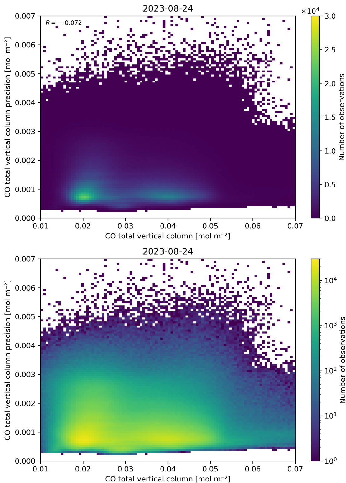
Figure 34: Scatter density plot of “CO total vertical column” against “CO total vertical column precision” for 2023-08-23 to 2023-08-25.
