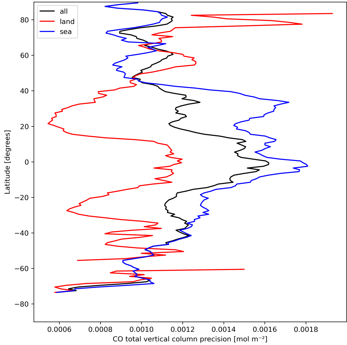
Figure 12: Zonal average of “CO total vertical column precision” for 2023-08-23 to 2023-08-25.
