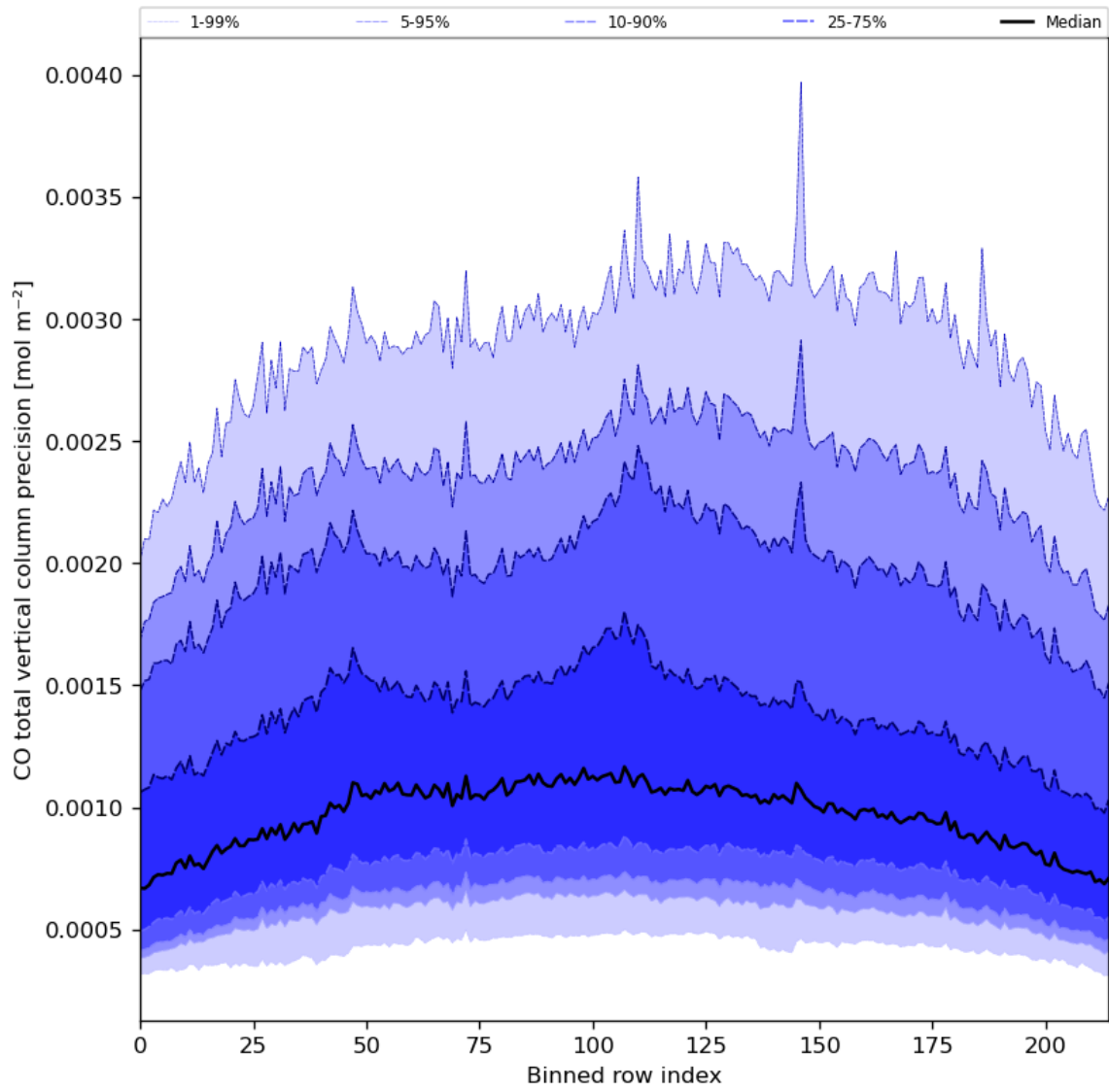
Figure 28: Along track statistics of “CO total vertical column precision” for 2023-08-23 to 2023-08-25
