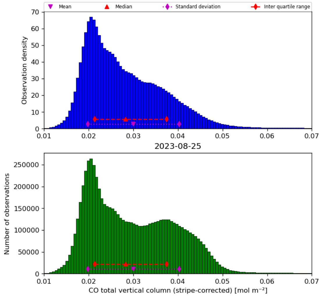
Figure 19: Histogram of “CO total vertical column (stripe-corrected)” for 2023-08-25 to 2023-08-26
