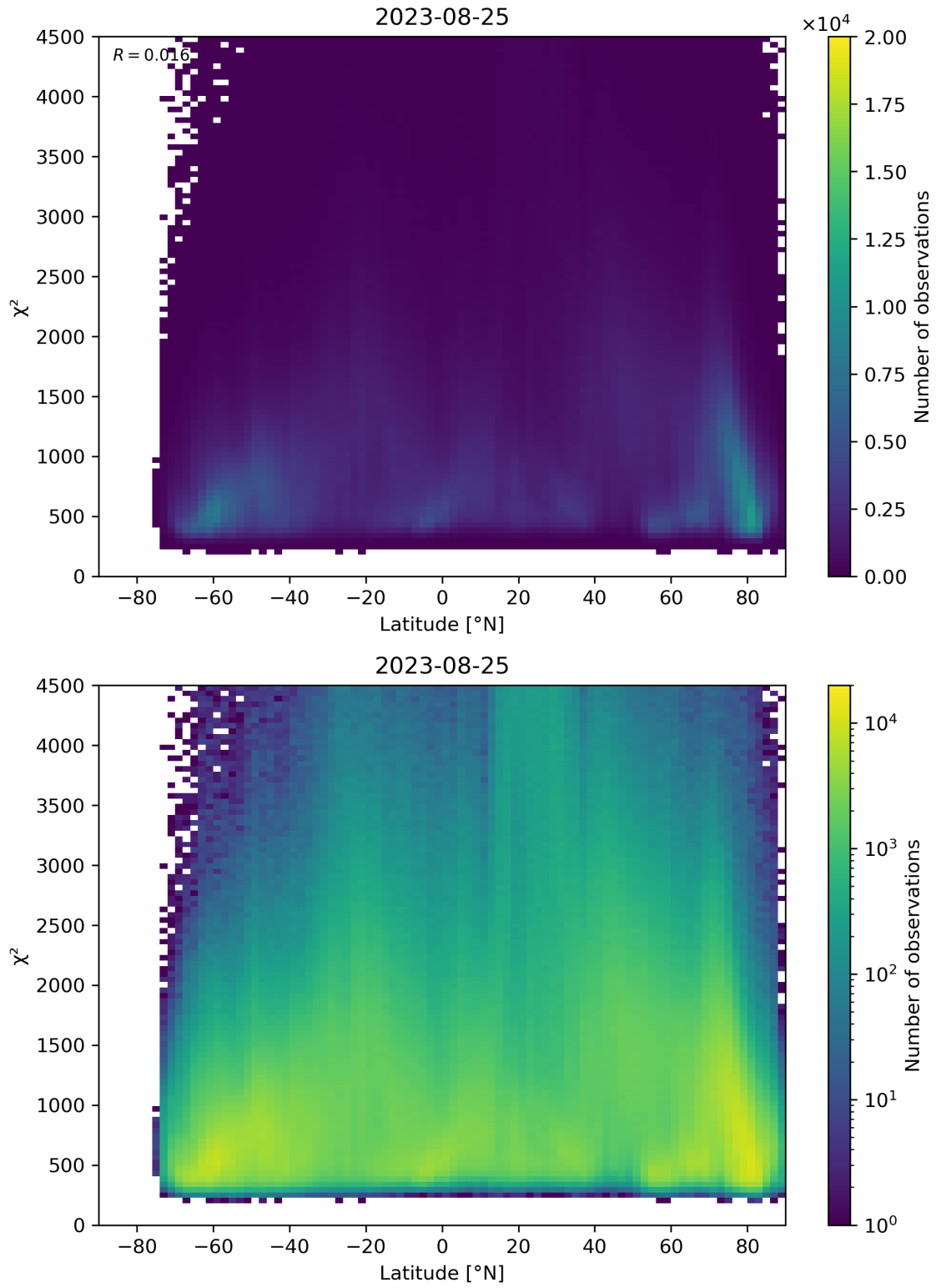
Figure 54: Scatter density plot of “Latitude” against “ \chi^2 ” for 2023-08-25 to 2023-08-26.
