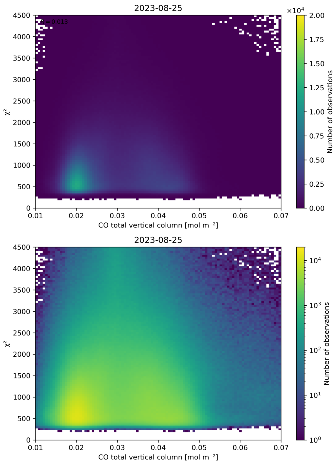
Figure 35: Scatter density plot of “CO total vertical column” against “ \chi^2 ” for 2023-08-25 to 2023-08-26.
