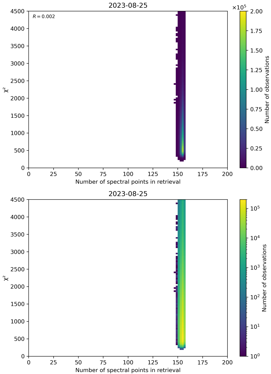
Figure 58: Scatter density plot of “Number of spectral points in retrieval” against “ \chi^2 ” for 2023-08-25 to 2023-08-26.
