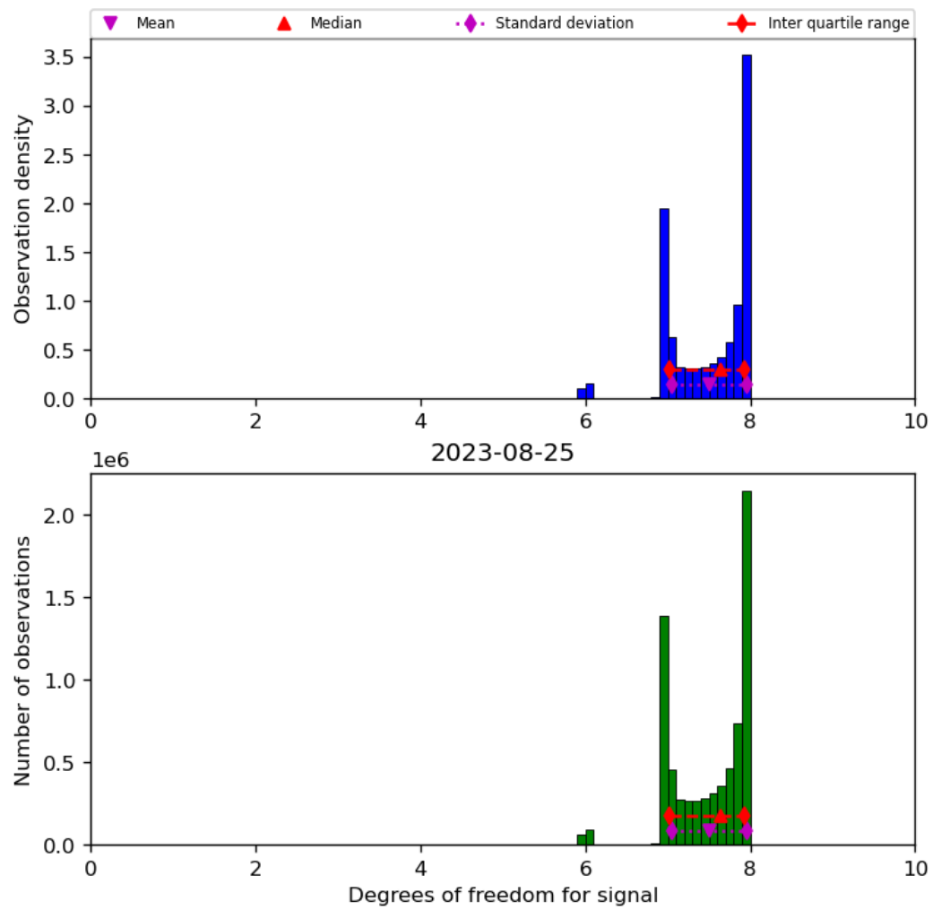
Figure 23: Histogram of “Degrees of freedom for signal” for 2023-08-25 to 2023-08-26
