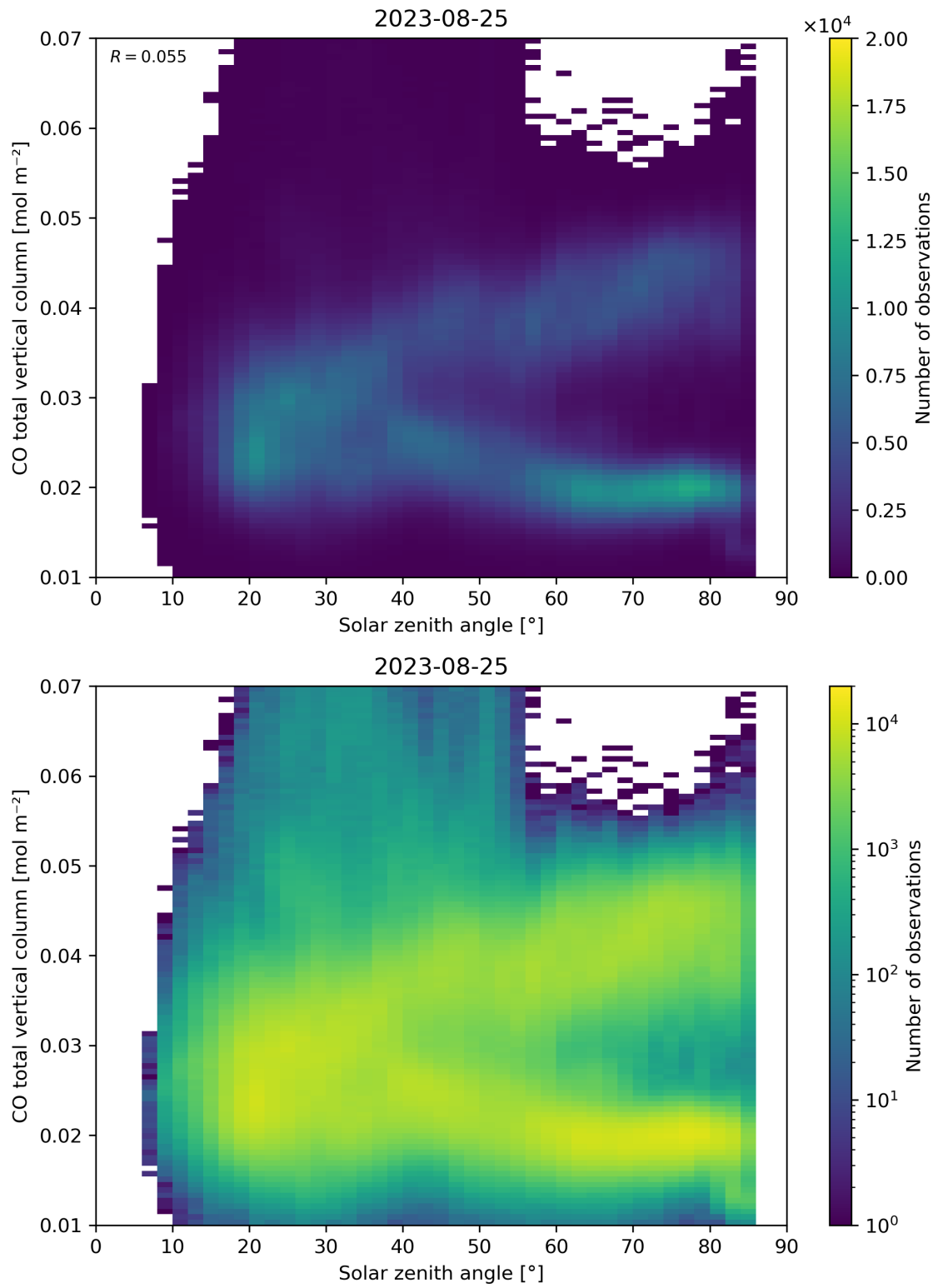
Figure 61: Scatter density plot of “Solar zenith angle” against “CO total vertical column” for 2023-08-25 to 2023-08-26.
