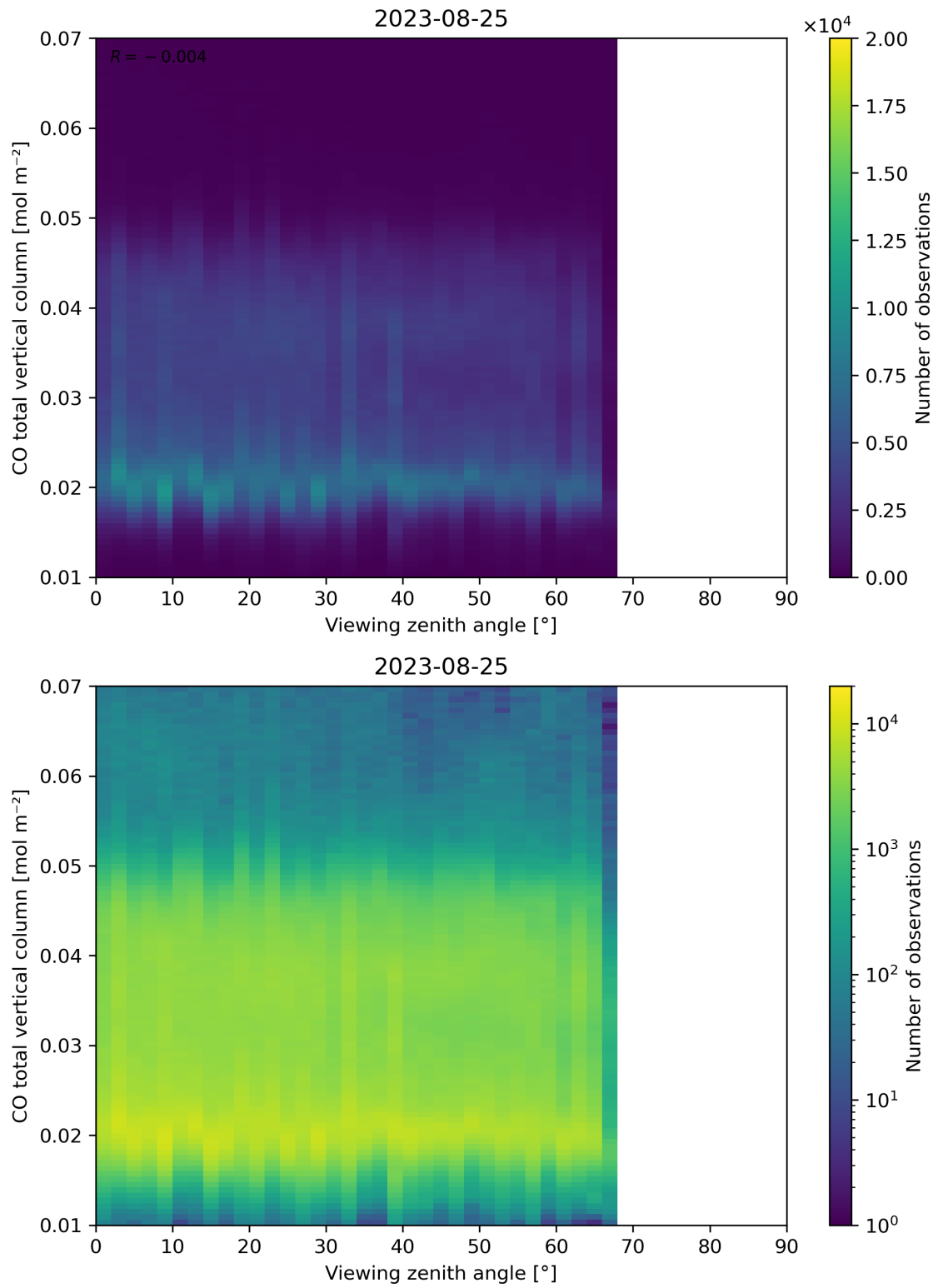
Figure 69: Scatter density plot of “Viewing zenith angle” against “CO total vertical column” for 2023-08-25 to 2023-08-26.
