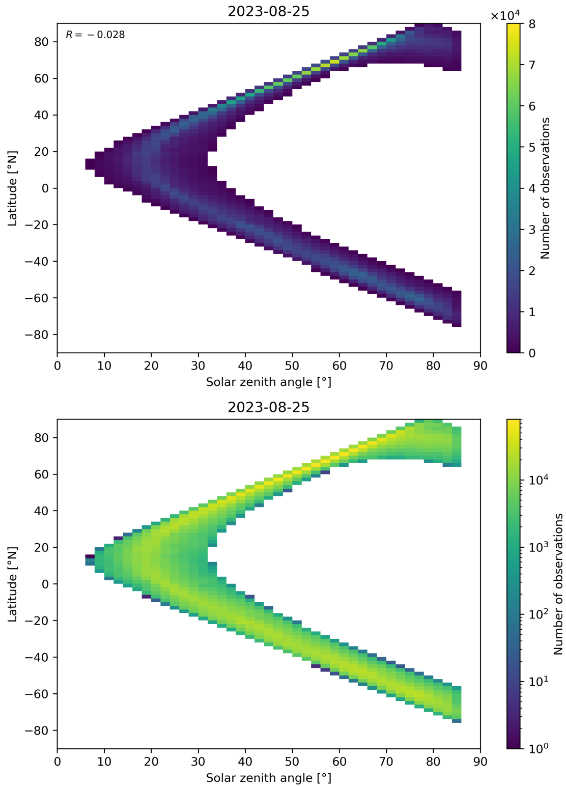
Figure 66: Scatter density plot of “Solar zenith angle” against “Latitude” for 2023-08-25 to 2023-08-26.
