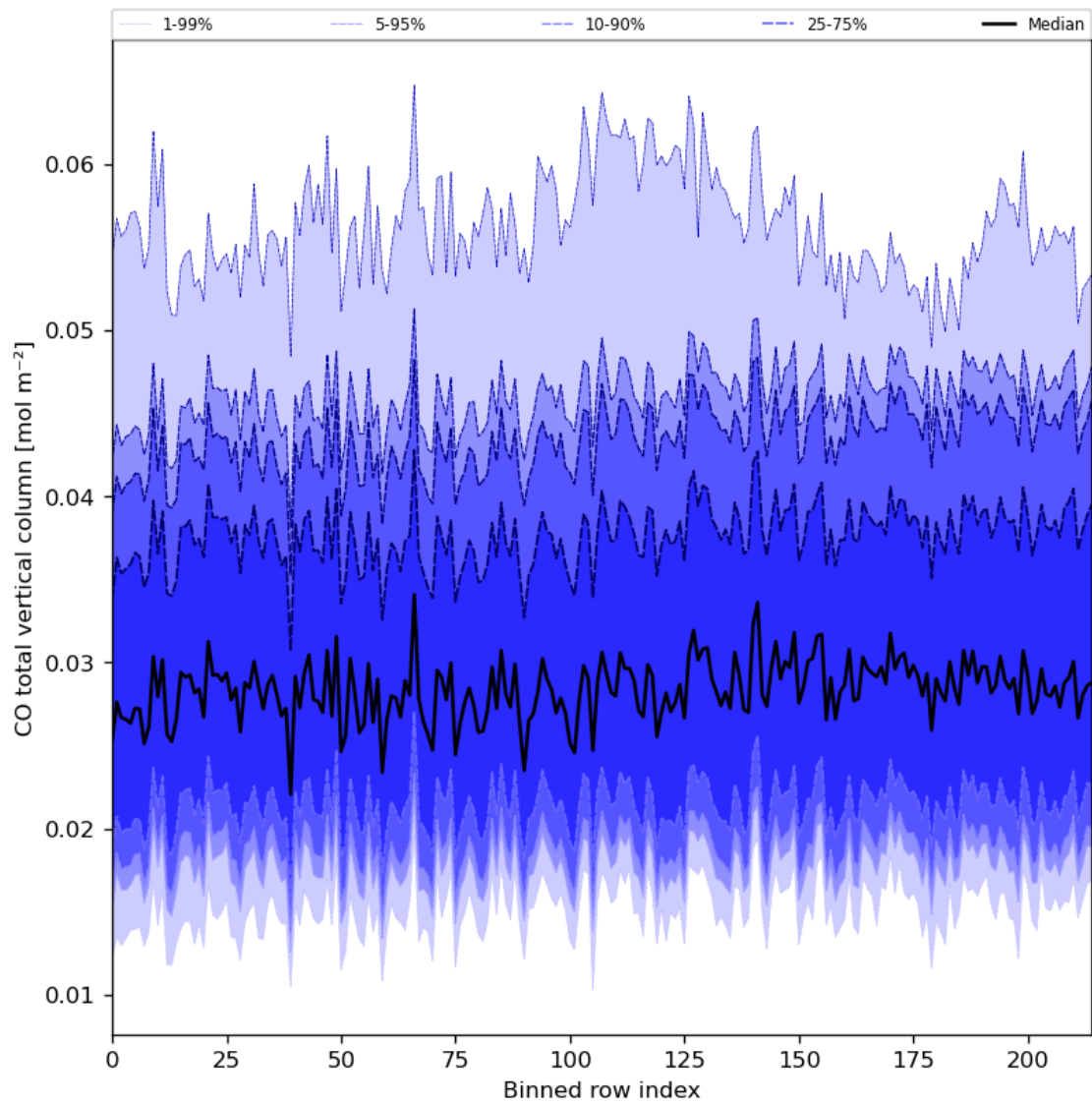
Figure 26: Along track statistics of “CO total vertical column” for 2023-08-25 to 2023-08-26
