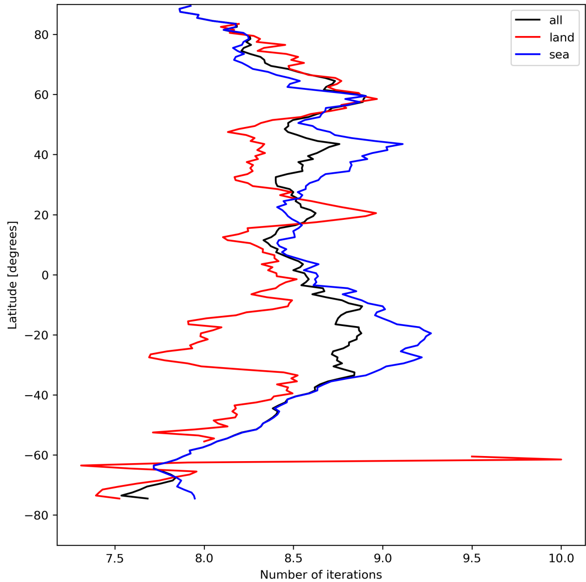
Figure 16: Zonal average of “Number of iterations” for 2023-08-25 to 2023-08-26.
