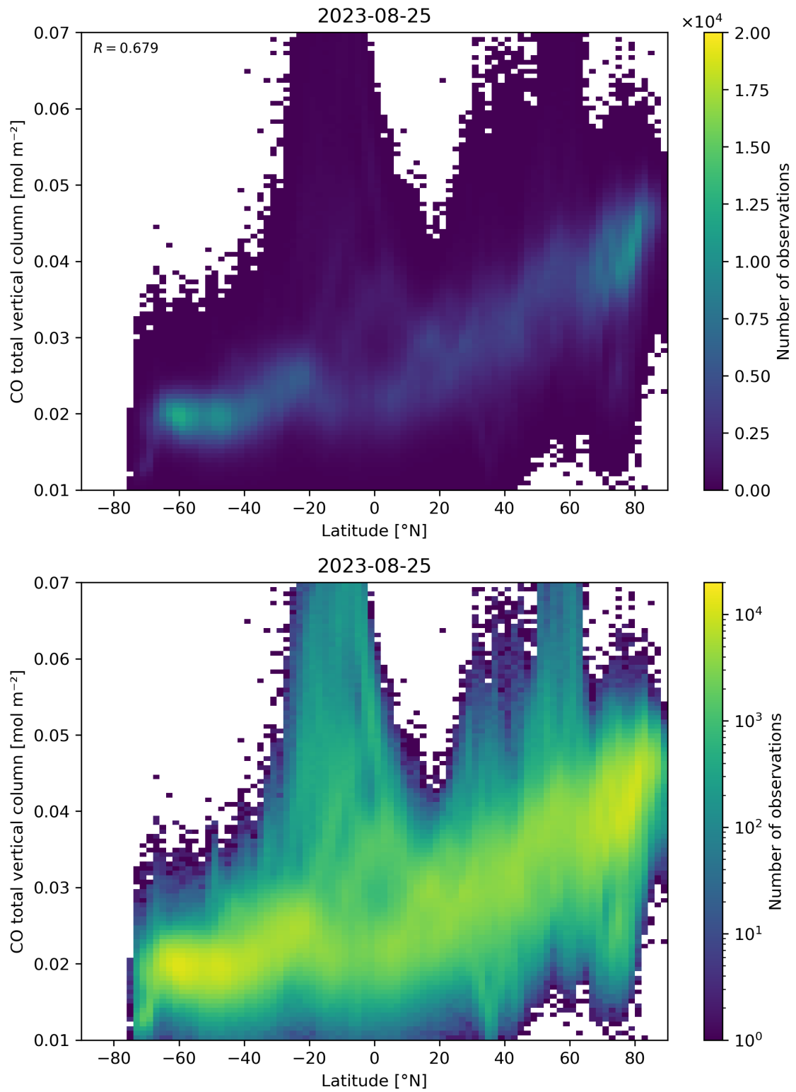
Figure 51: Scatter density plot of “Latitude” against “CO total vertical column” for 2023-08-25 to 2023-08-26.
