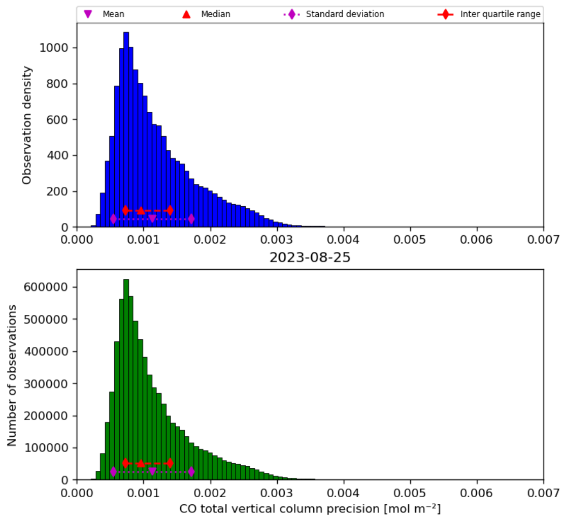
Figure 20: Histogram of “CO total vertical column precision” for 2023-08-25 to 2023-08-26
