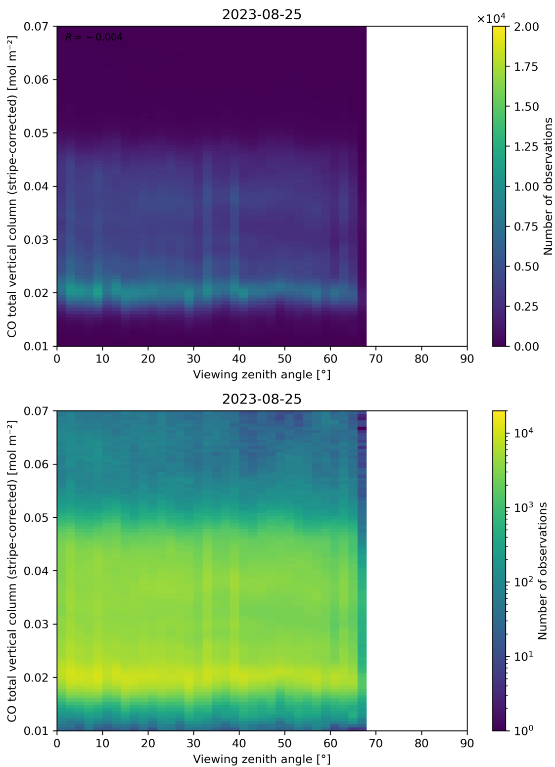
Figure 70: Scatter density plot of “Viewing zenith angle” against “CO total vertical column (stripe-corrected)” for 2023-08-25 to 2023-08-26.
