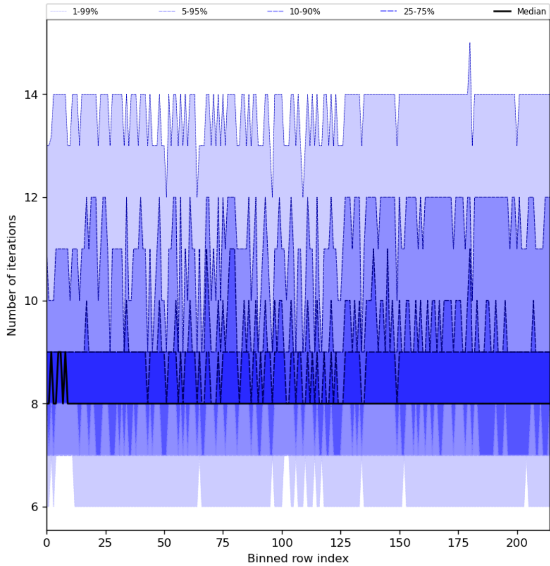
Figure 32: Along track statistics of “Number of iterations” for 2023-08-25 to 2023-08-26
