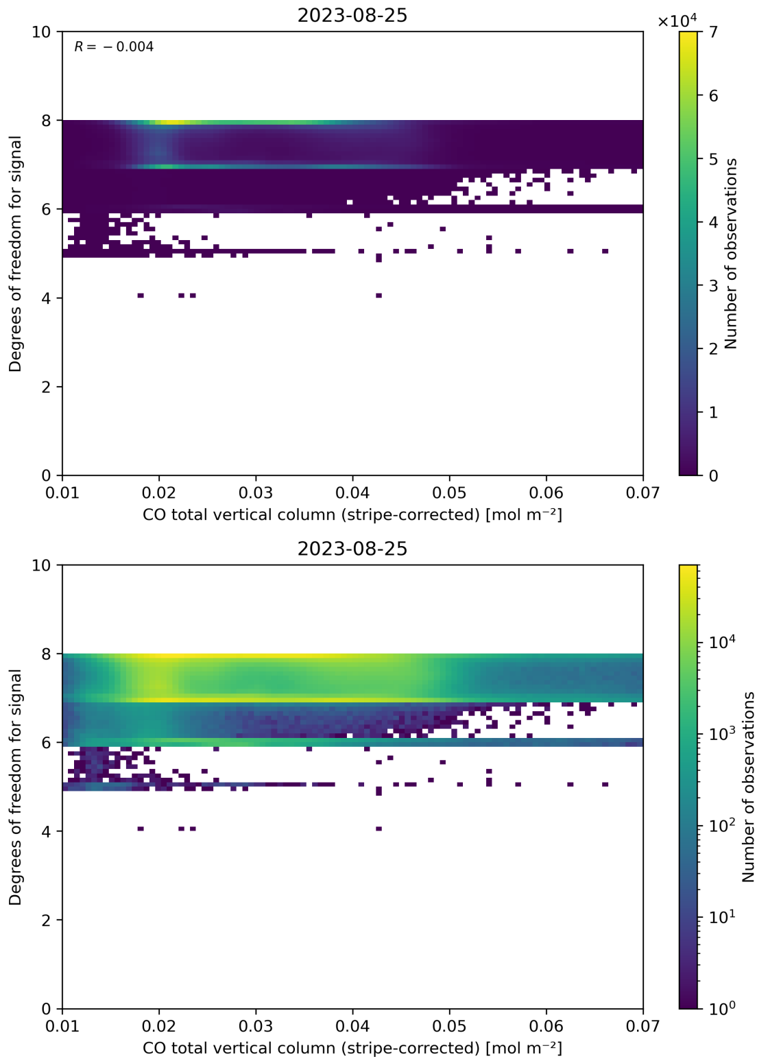
Figure 38: Scatter density plot of “CO total vertical column (stripe-corrected)” against “Degrees of freedom for signal” for 2023-08-25 to 2023-08-26.
