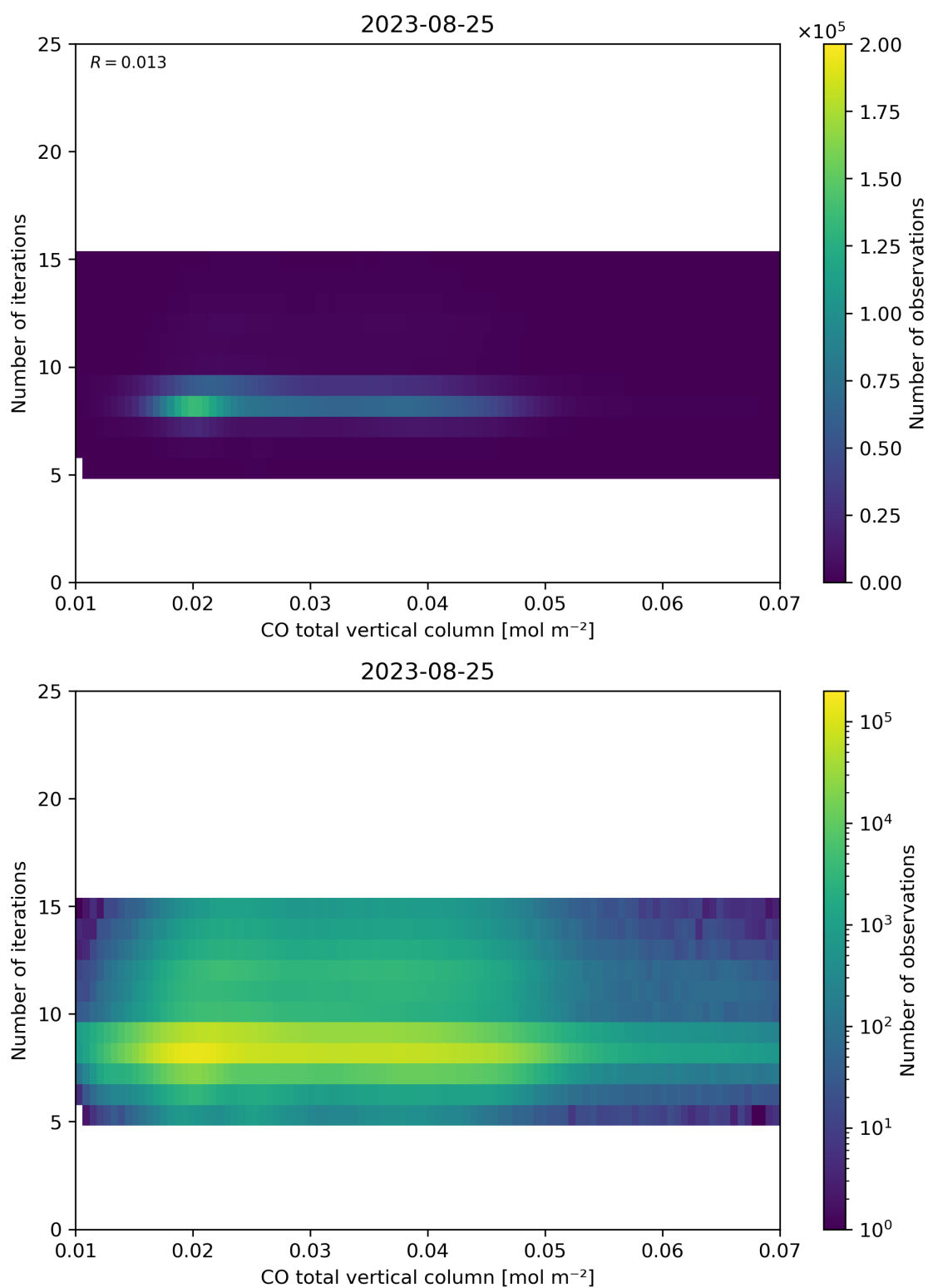
Figure 42: Scatter density plot of “CO total vertical column” against “Number of iterations” for 2023-08-25 to 2023-08-26.
