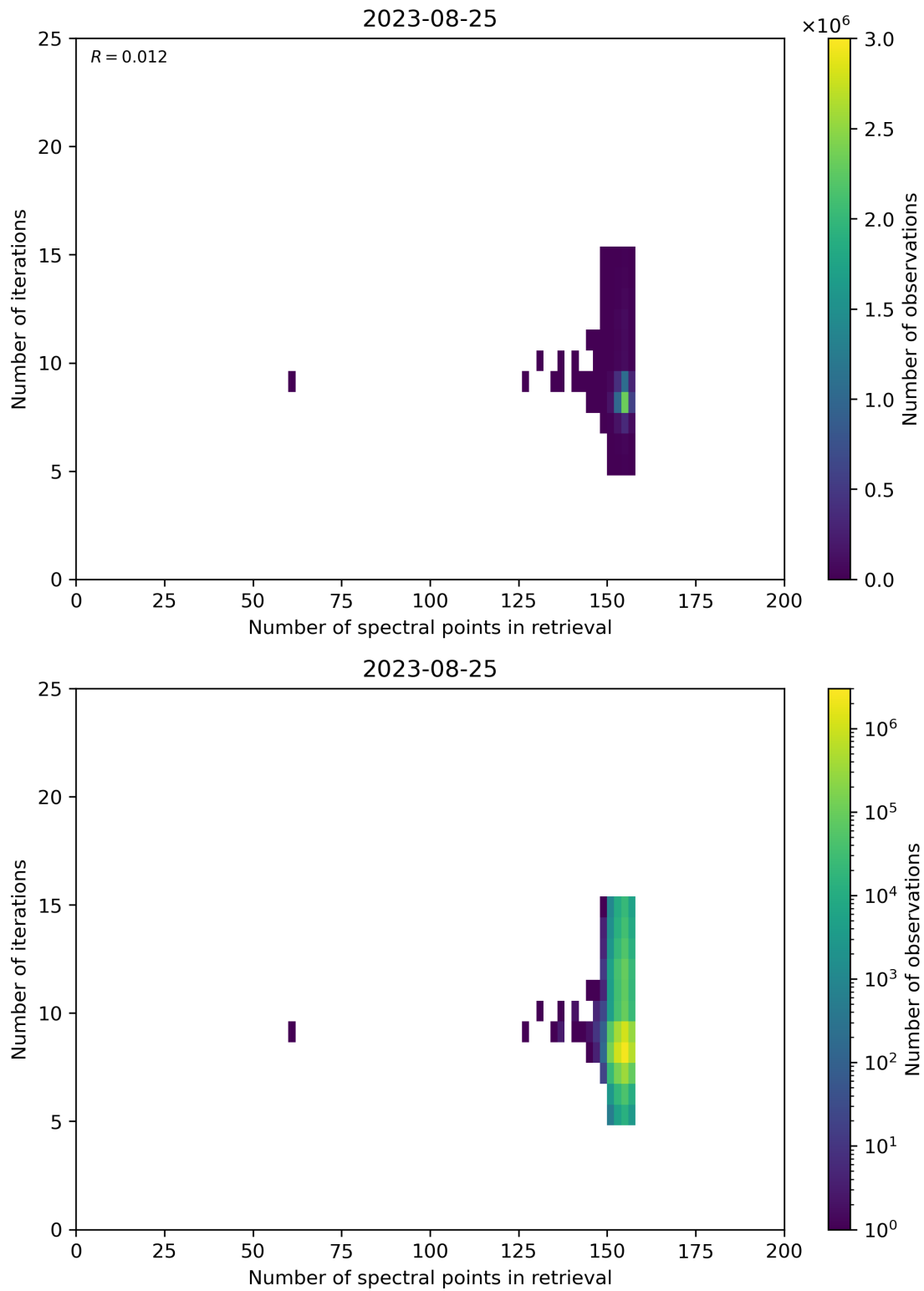
Figure 60: Scatter density plot of “Number of spectral points in retrieval” against “Number of iterations” for 2023-08-25 to 2023-08-26.
