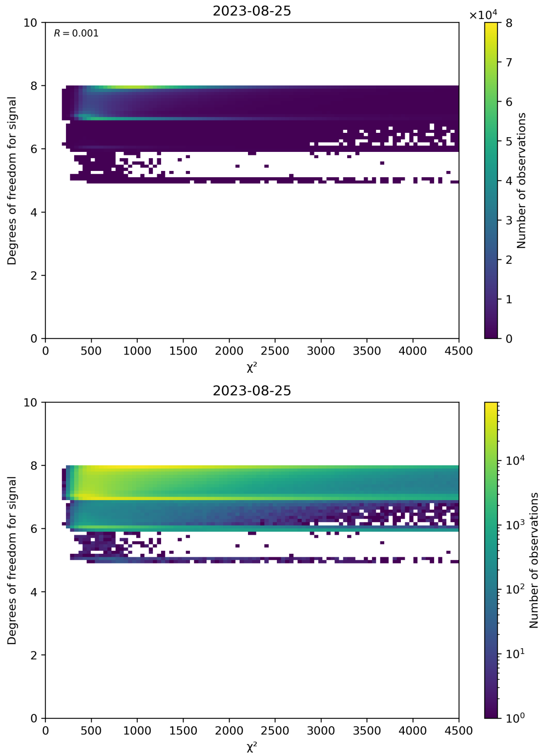
Figure 48: Scatter density plot of “ \chi^2 ” against “Degrees of freedom for signal” for 2023-08-25 to 2023-08-26.
