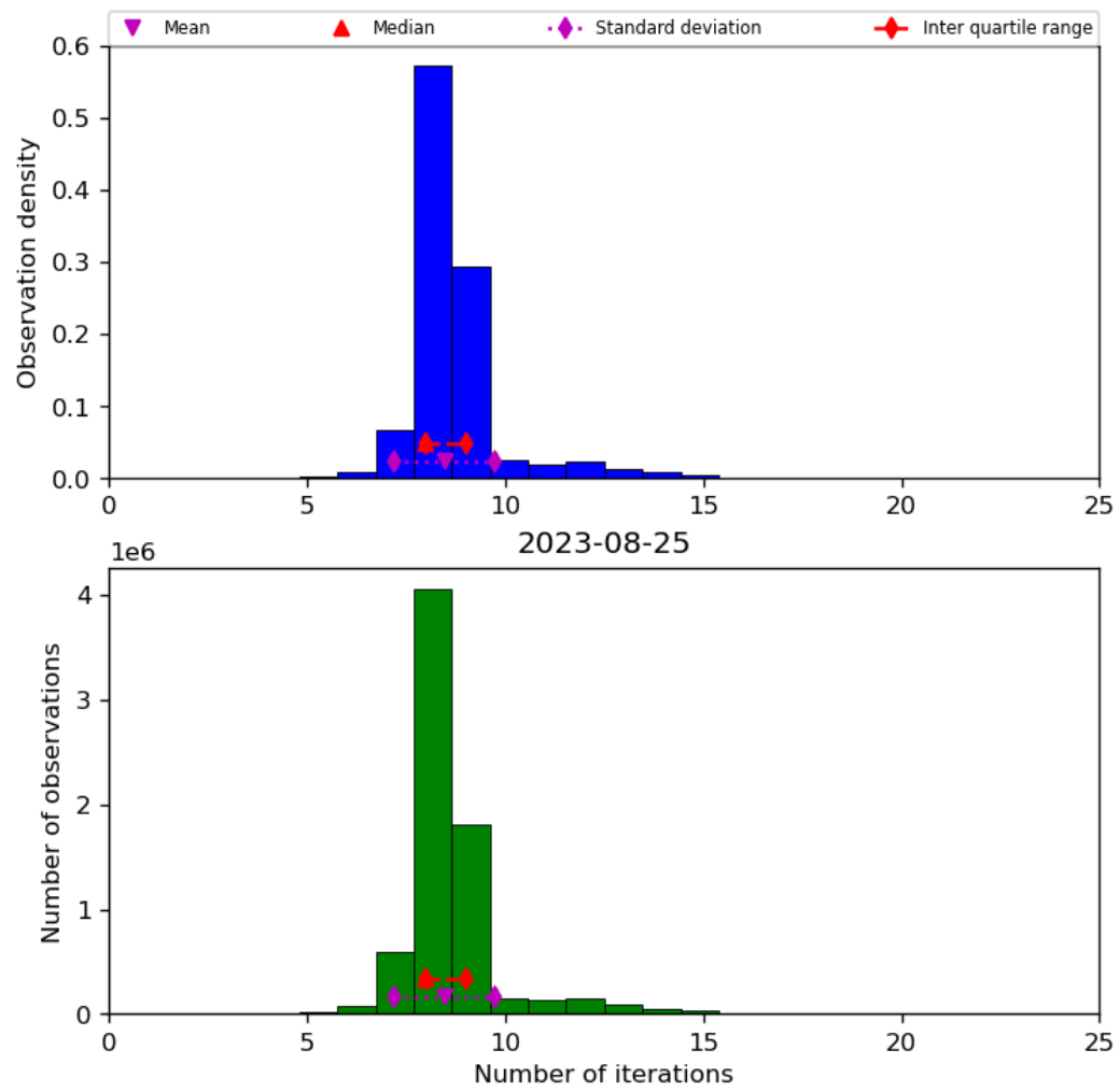
Figure 24: Histogram of “Number of iterations” for 2023-08-25 to 2023-08-26
