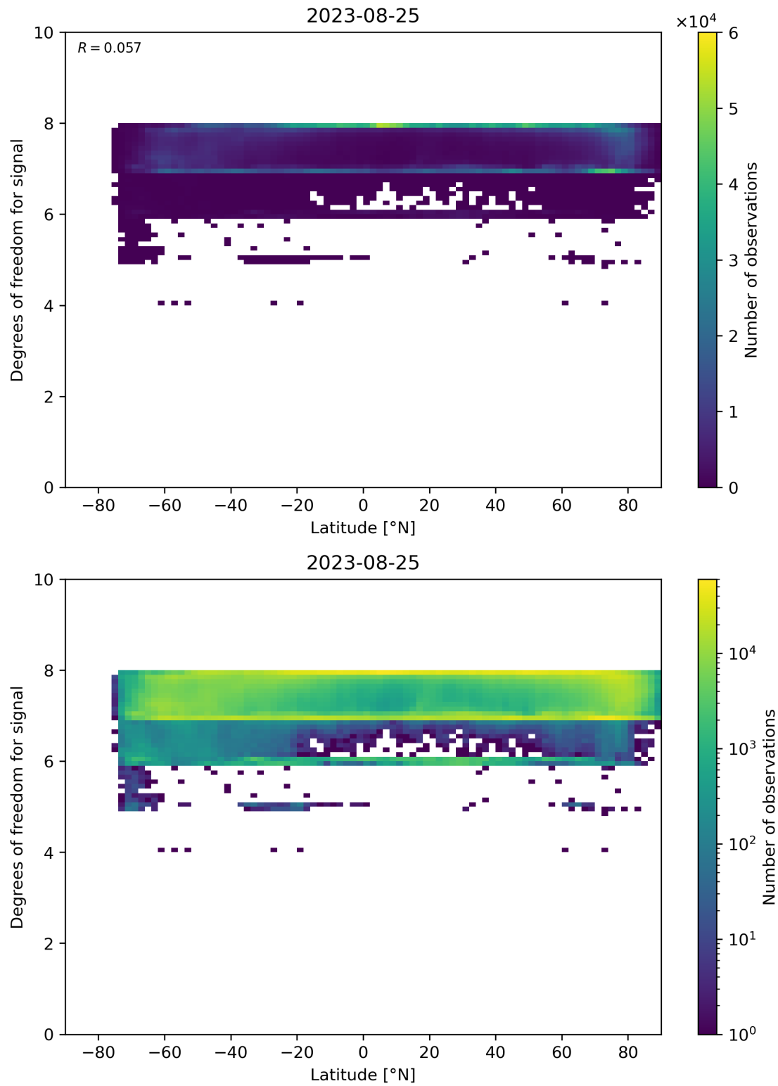
Figure 55: Scatter density plot of “Latitude” against “Degrees of freedom for signal” for 2023-08-25 to 2023-08-26.
