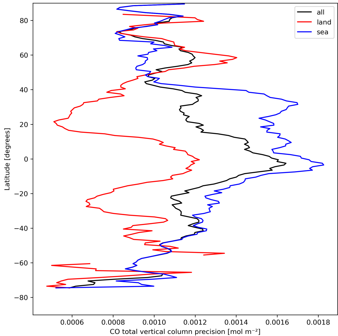
Figure 12: Zonal average of “CO total vertical column precision” for 2023-08-25 to 2023-08-26.
