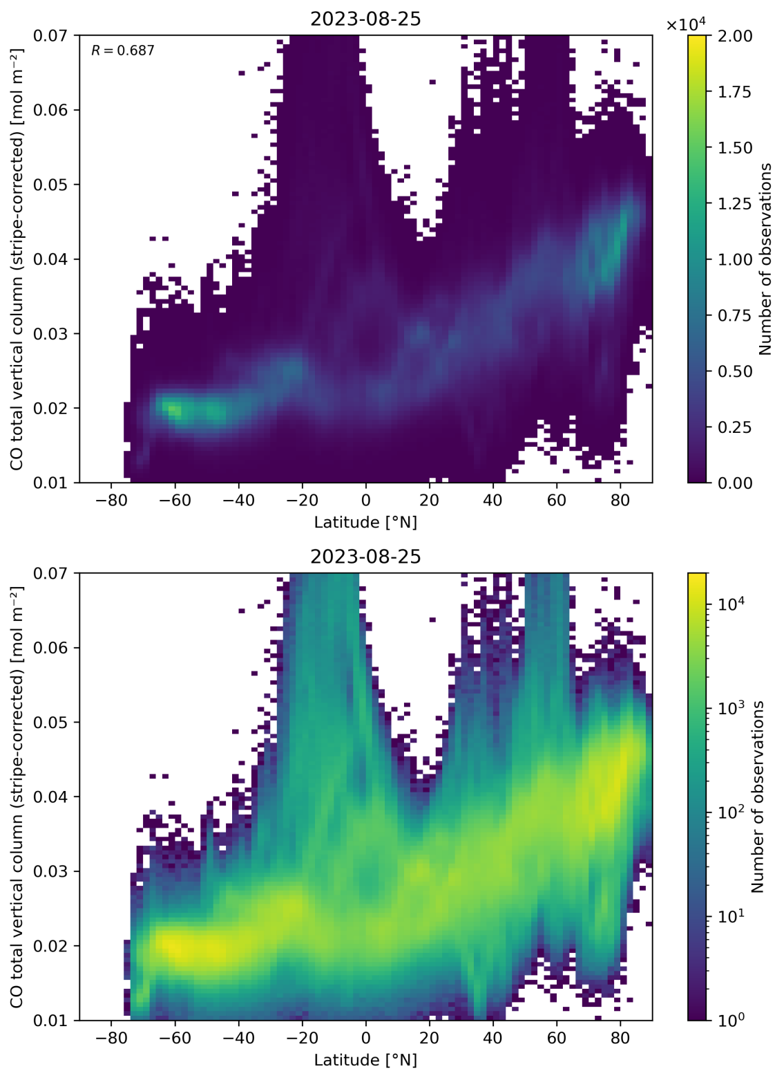
Figure 52: Scatter density plot of “Latitude” against “CO total vertical column (stripe-corrected)” for 2023-08-25 to 2023-08-26.
