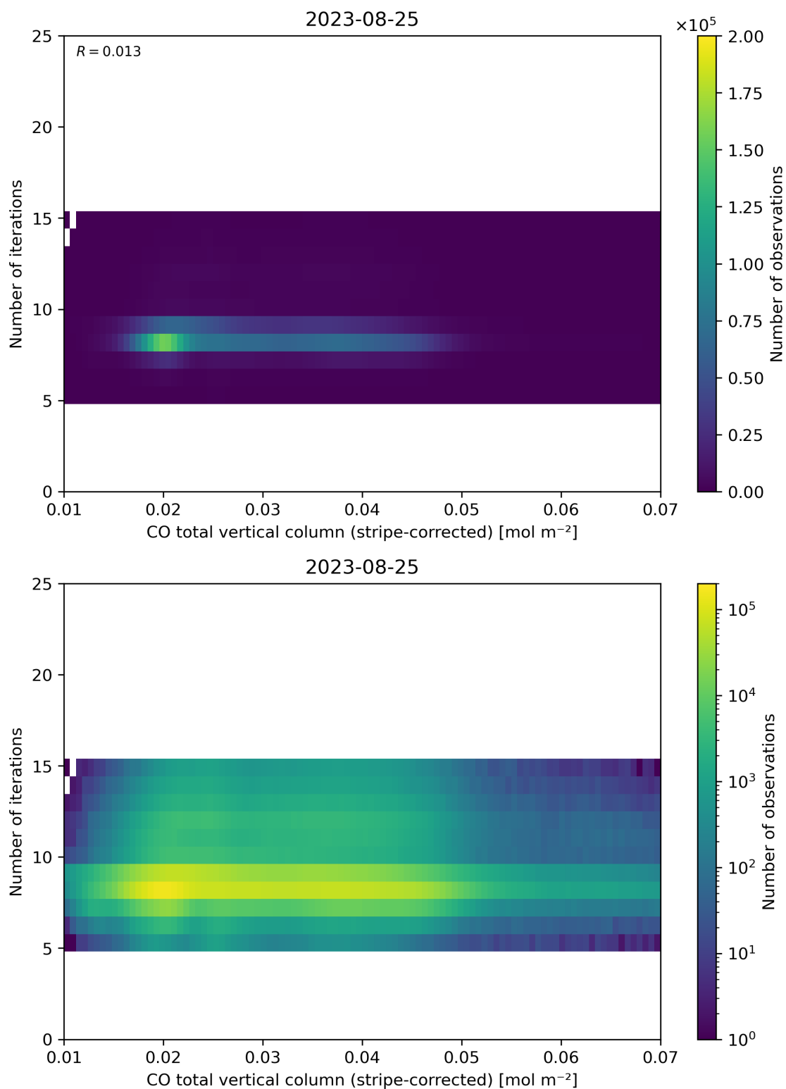
Figure 39: Scatter density plot of “CO total vertical column (stripe-corrected)” against “Number of iterations” for 2023-08-25 to 2023-08-26.
