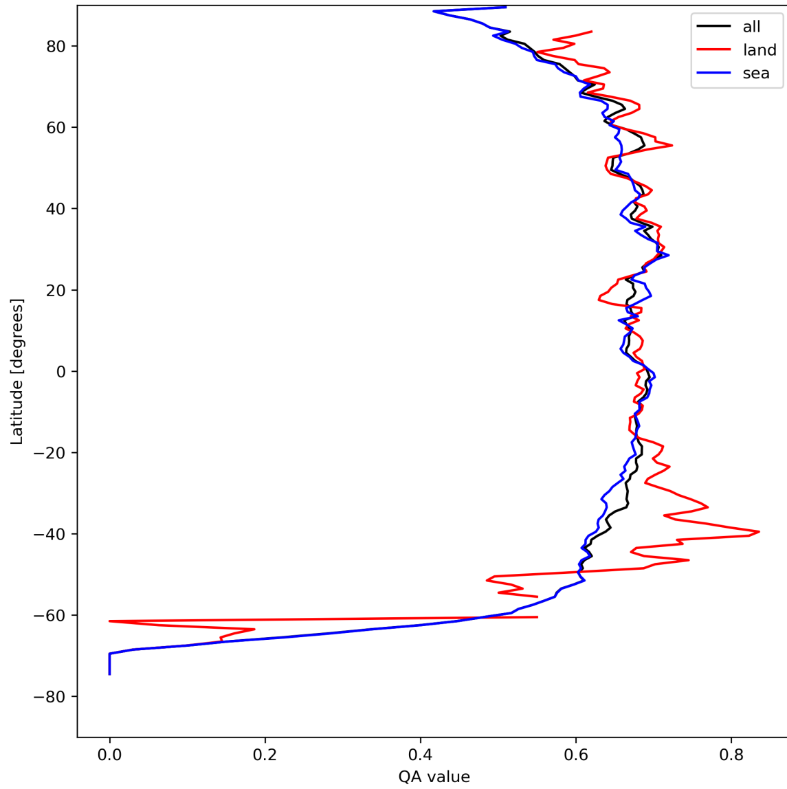
Figure 9: Zonal average of “QA value” for 2023-08-25 to 2023-08-26.
