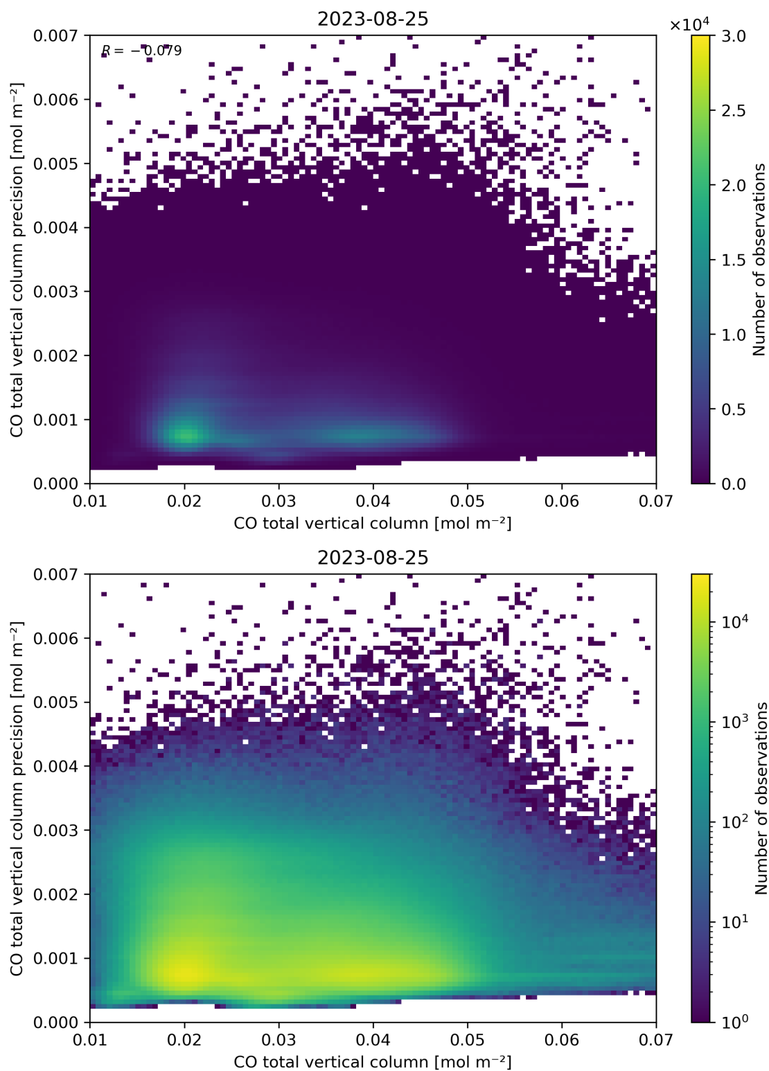
Figure 34: Scatter density plot of “CO total vertical column” against “CO total vertical column precision” for 2023-08-25 to 2023-08-26.
