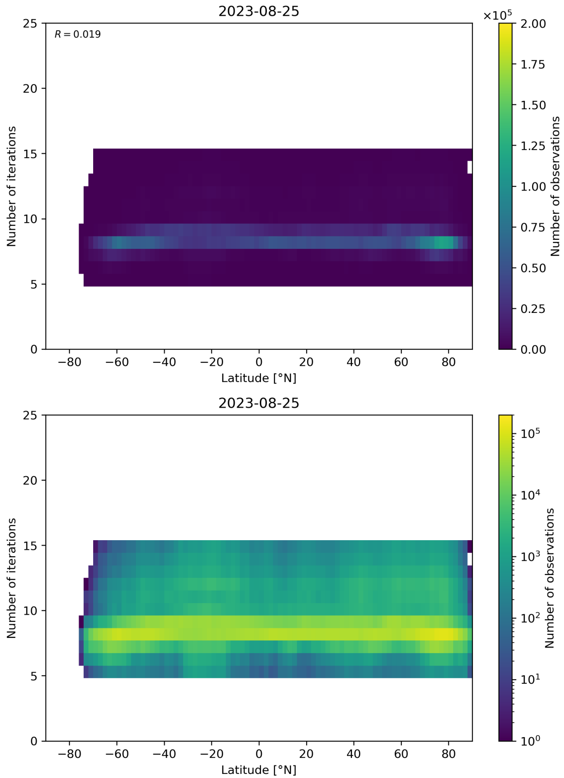
Figure 56: Scatter density plot of “Latitude” against “Number of iterations” for 2023-08-25 to 2023-08-26.
