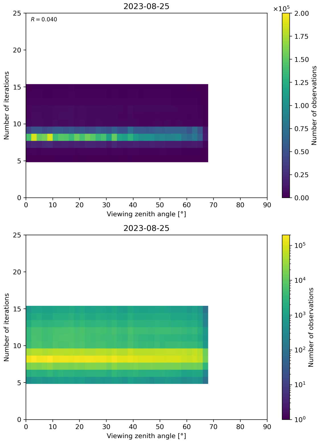
Figure 75: Scatter density plot of “Viewing zenith angle” against “Number of iterations” for 2023-08-25 to 2023-08-26.
