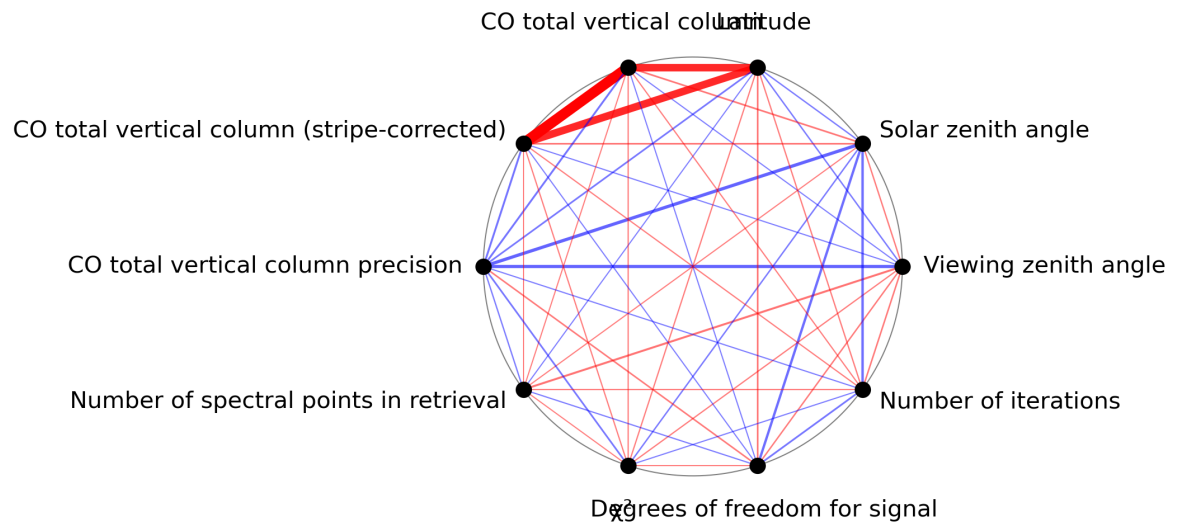
Figure 1: Map of correlation graph for 2023-08-25 to 2023-08-26.
