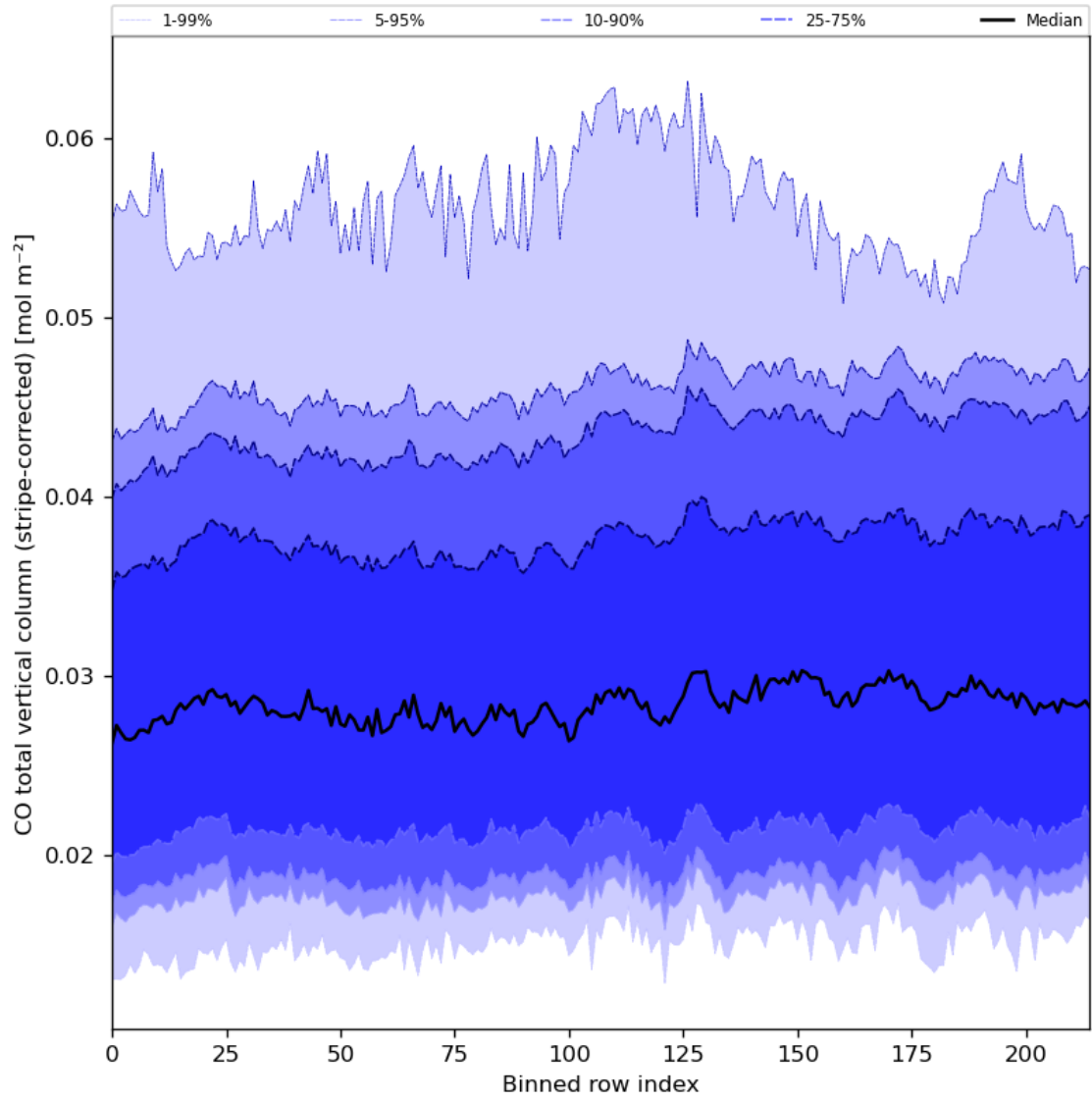
Figure 27: Along track statistics of “CO total vertical column (stripe-corrected)” for 2023-08-25 to 2023-08-26
