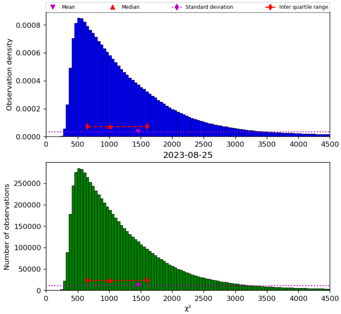
Figure 22: Histogram of “ \chi^2 ” for 2023-08-25 to 2023-08-26
