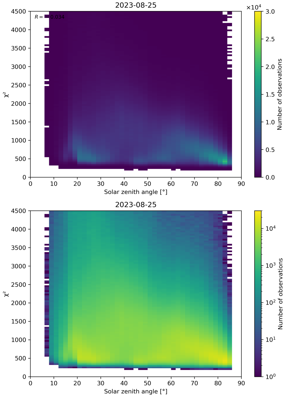
Figure 64: Scatter density plot of “Solar zenith angle” against “ \chi^2 ” for 2023-08-25 to 2023-08-26.
