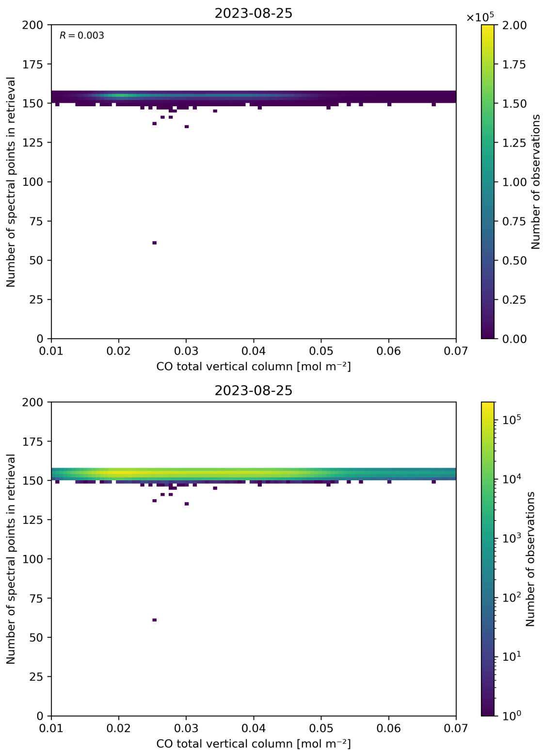
Figure 43: Scatter density plot of “CO total vertical column” against “Number of spectral points in retrieval” for 2023-08-25 to 2023-08-26.
