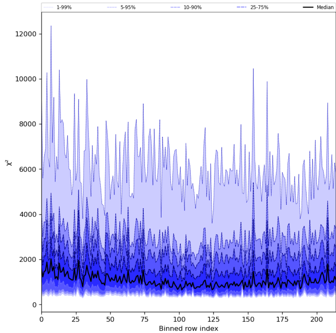
Figure 30: Along track statistics of “ \chi^2 ” for 2023-08-25 to 2023-08-26
