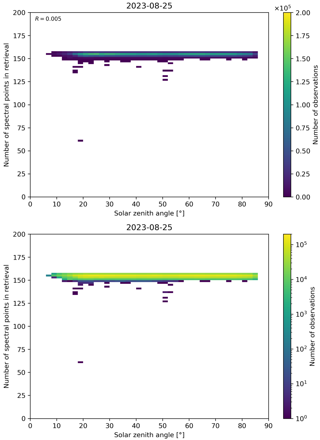
Figure 68: Scatter density plot of “Solar zenith angle” against “Number of spectral points in retrieval” for 2023-08-25 to 2023-08-26.
