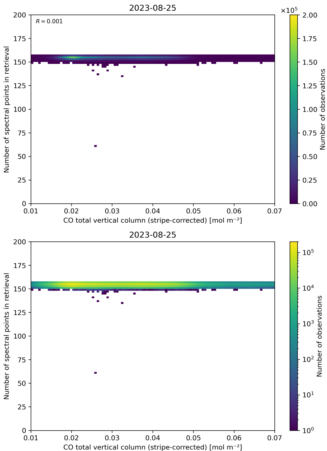
Figure 40: Scatter density plot of “CO total vertical column (stripe-corrected)” against “Number of spectral points in retrieval” for 2023-08-25 to 2023-08-26.
