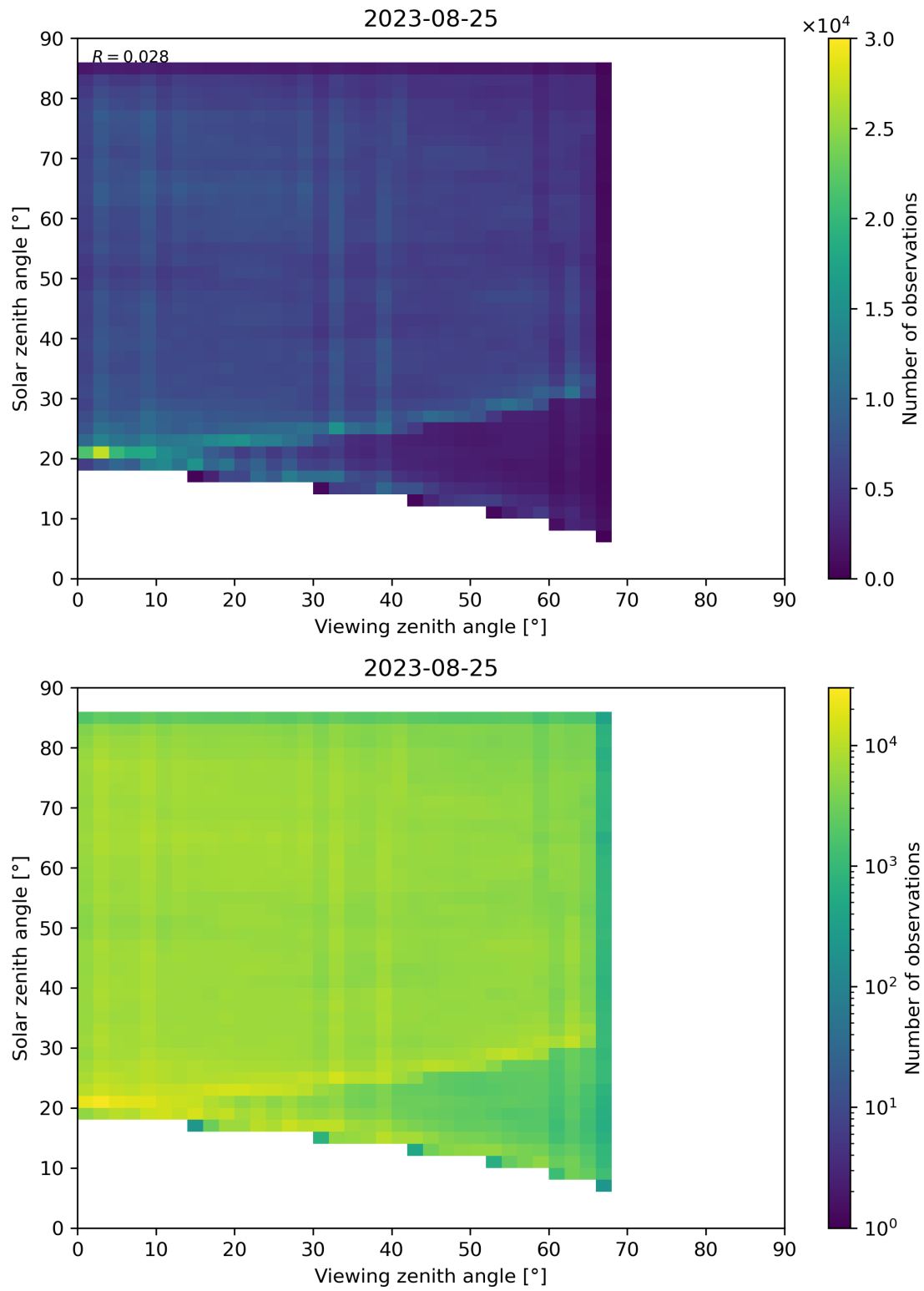
Figure 77: Scatter density plot of “Viewing zenith angle” against “Solar zenith angle” for 2023-08-25 to 2023-08-26.
