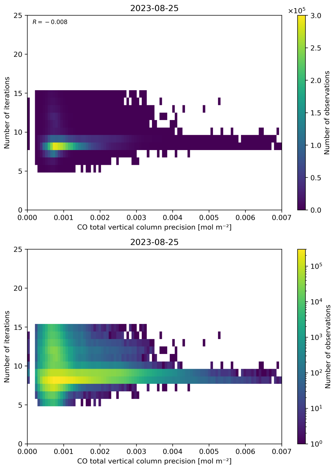
Figure 46: Scatter density plot of “CO total vertical column precision” against “Number of iterations” for 2023-08-25 to 2023-08-26.
