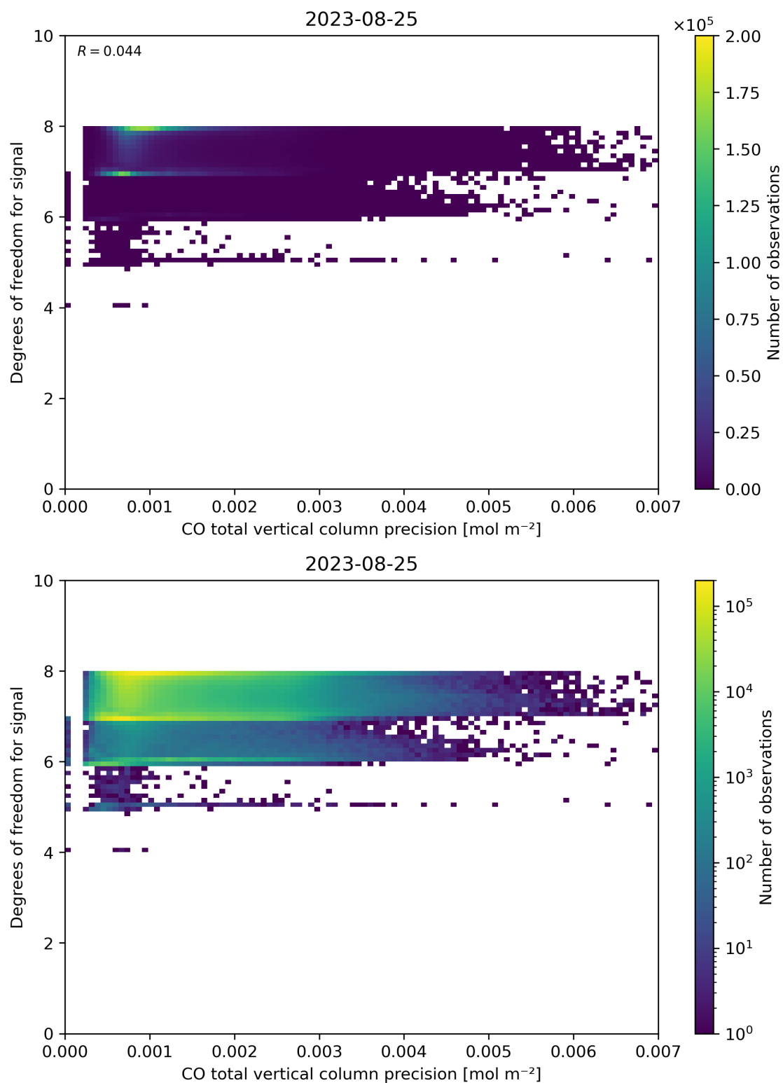
Figure 45: Scatter density plot of “CO total vertical column precision” against “Degrees of freedom for signal” for 2023-08-25 to 2023-08-26.
