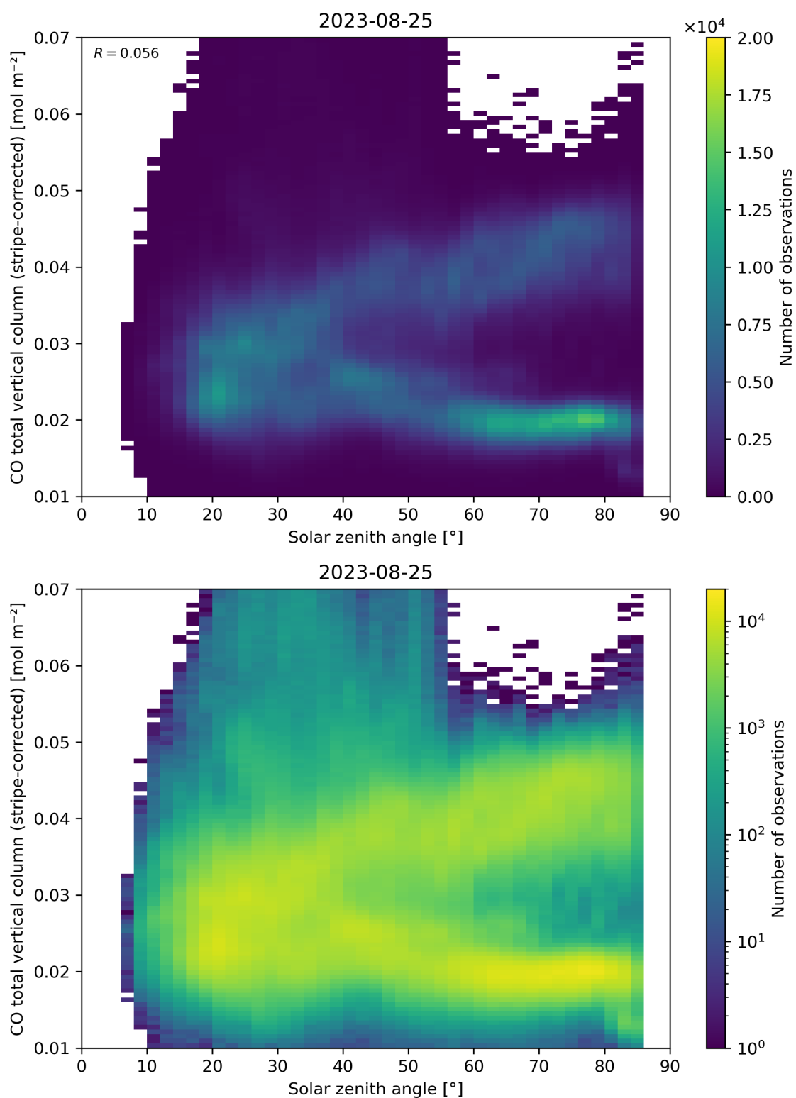
Figure 62: Scatter density plot of “Solar zenith angle” against “CO total vertical column (stripe-corrected)” for 2023-08-25 to 2023-08-26.
