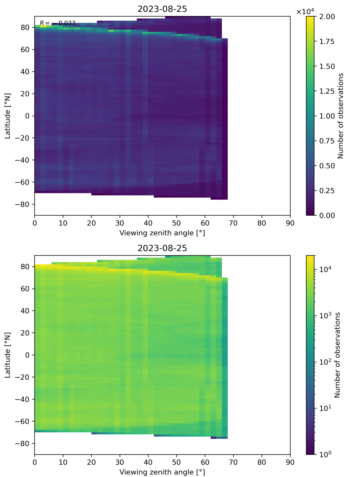
Figure 74: Scatter density plot of “Viewing zenith angle” against “Latitude” for 2023-08-25 to 2023-08-26.
