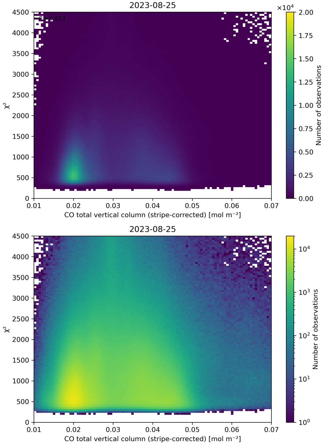
Figure 37: Scatter density plot of “CO total vertical column (stripe-corrected)” against “ \chi^2 ” for 2023-08-25 to 2023-08-26.
