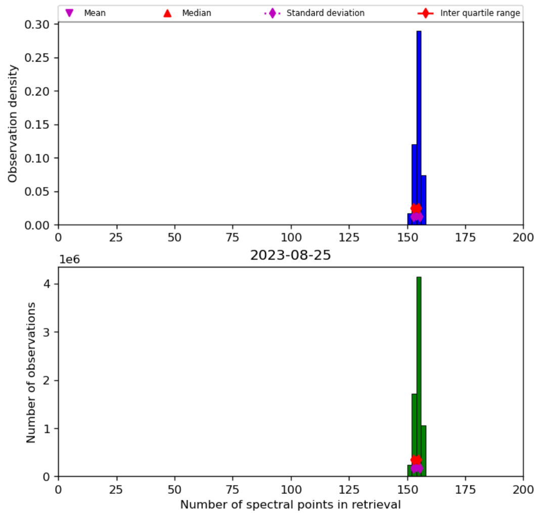
Figure 21: Histogram of “Number of spectral points in retrieval” for 2023-08-25 to 2023-08-26
