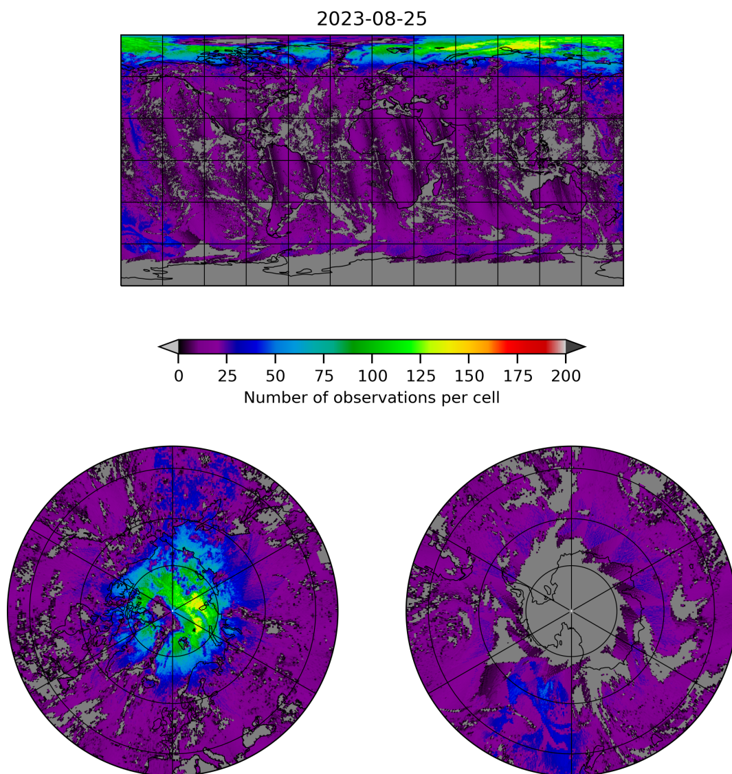
Figure 8: Map of the number of observations for 2023-08-25 to 2023-08-26
