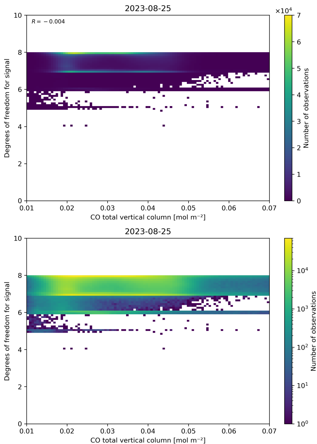
Figure 41: Scatter density plot of “CO total vertical column” against “Degrees of freedom for signal” for 2023-08-25 to 2023-08-26.
