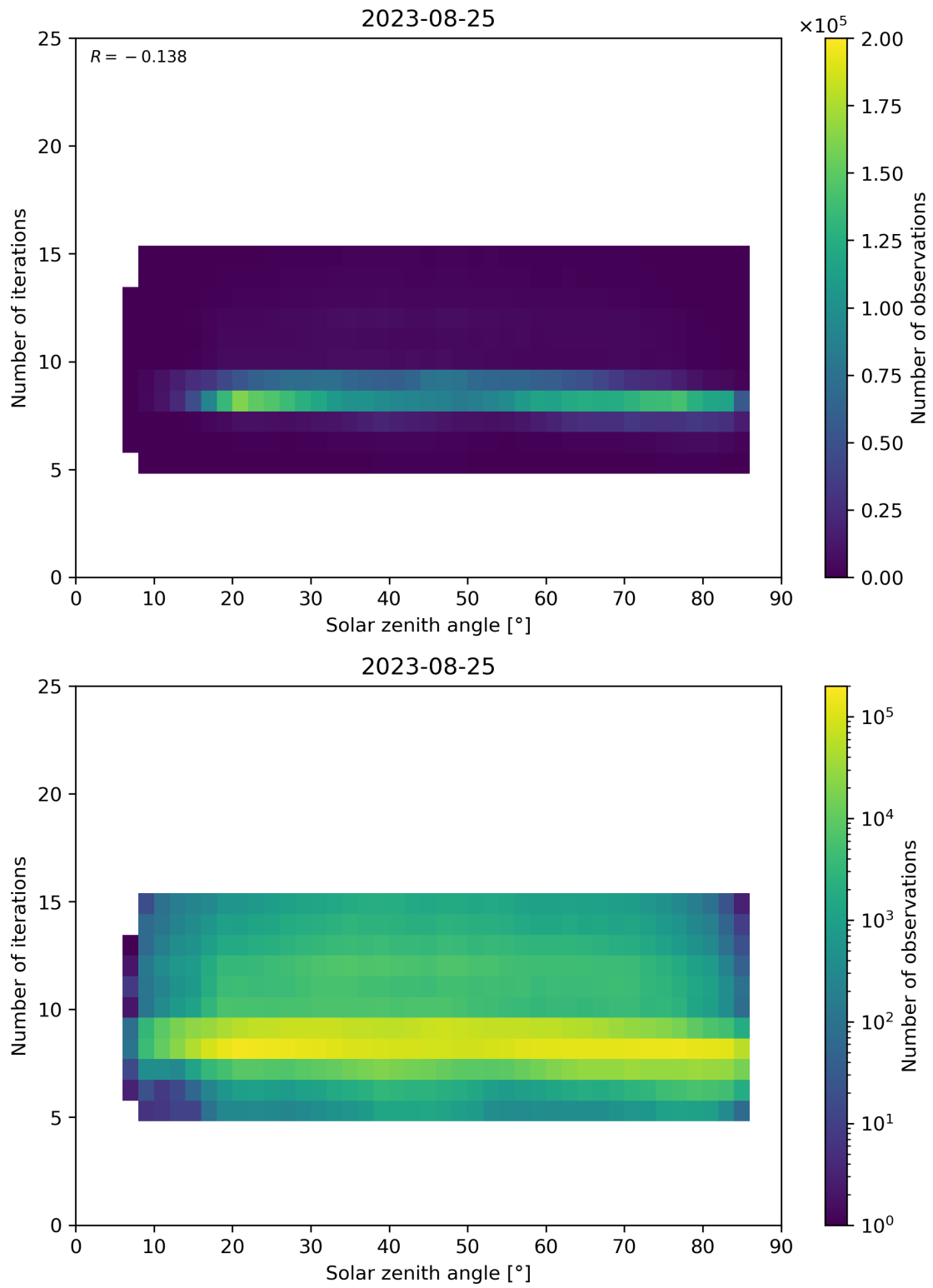
Figure 67: Scatter density plot of “Solar zenith angle” against “Number of iterations” for 2023-08-25 to 2023-08-26.
