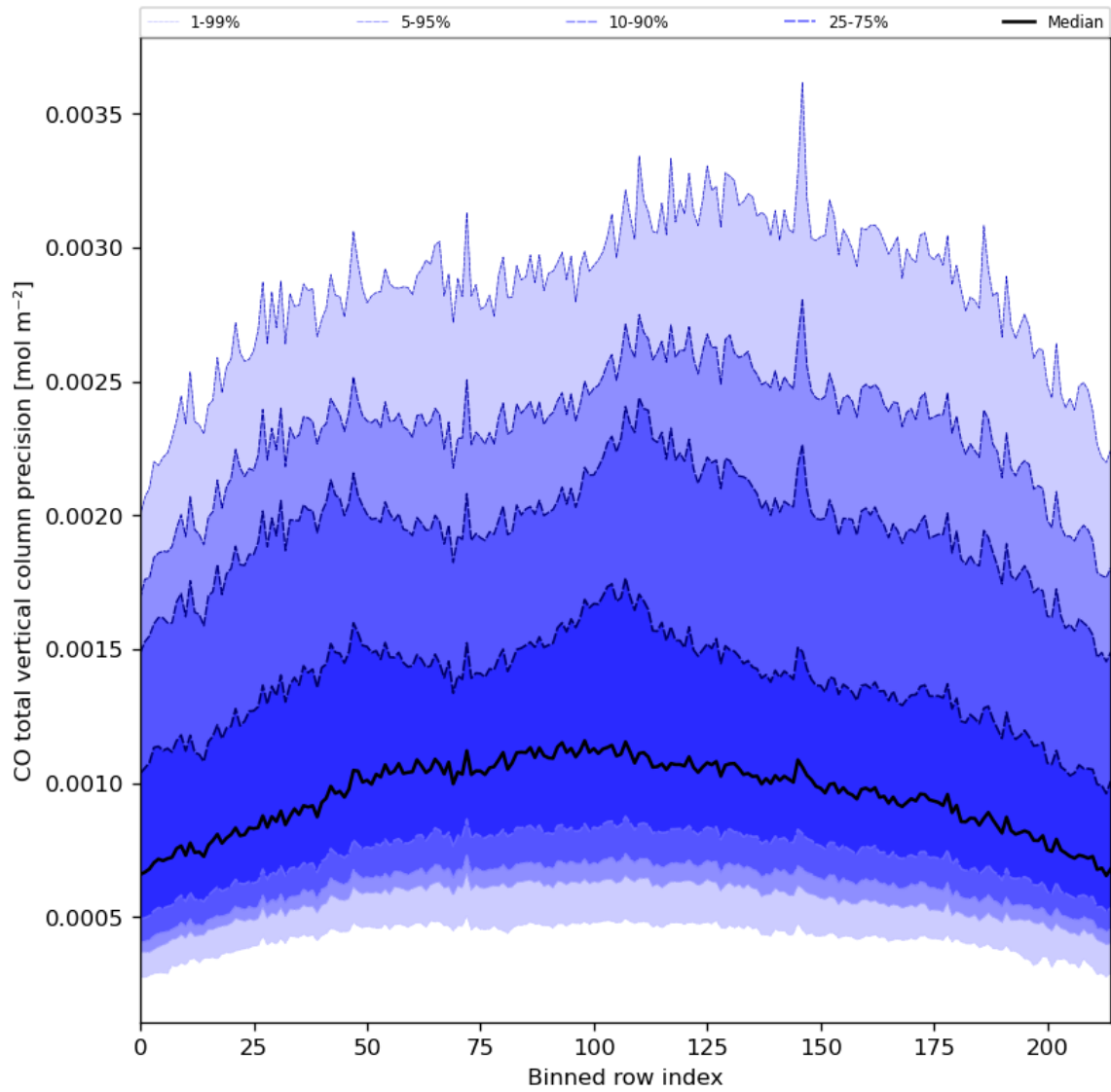
Figure 28: Along track statistics of “CO total vertical column precision” for 2023-08-25 to 2023-08-26
