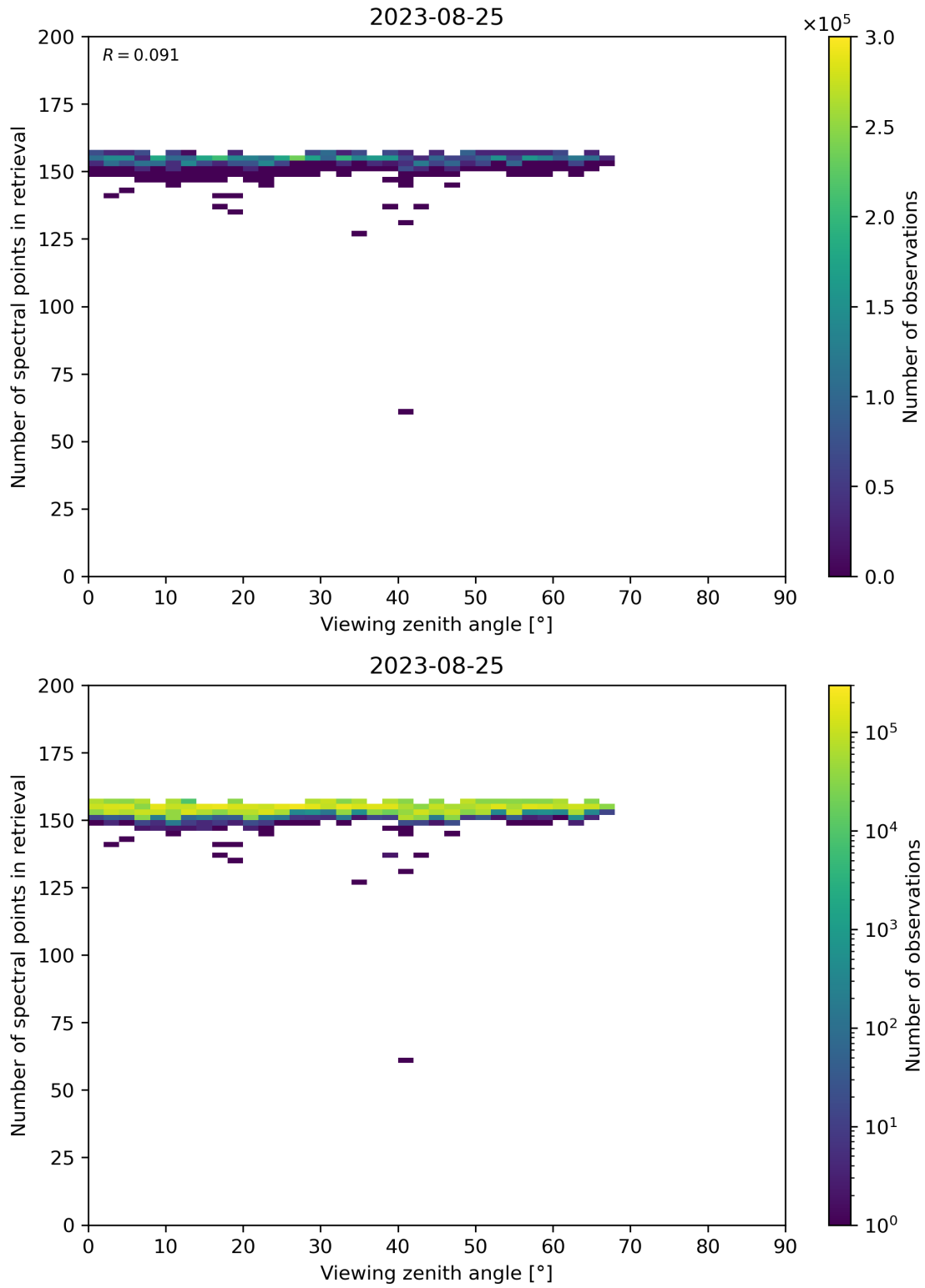
Figure 76: Scatter density plot of “Viewing zenith angle” against “Number of spectral points in retrieval” for 2023-08-25 to 2023-08-26.
