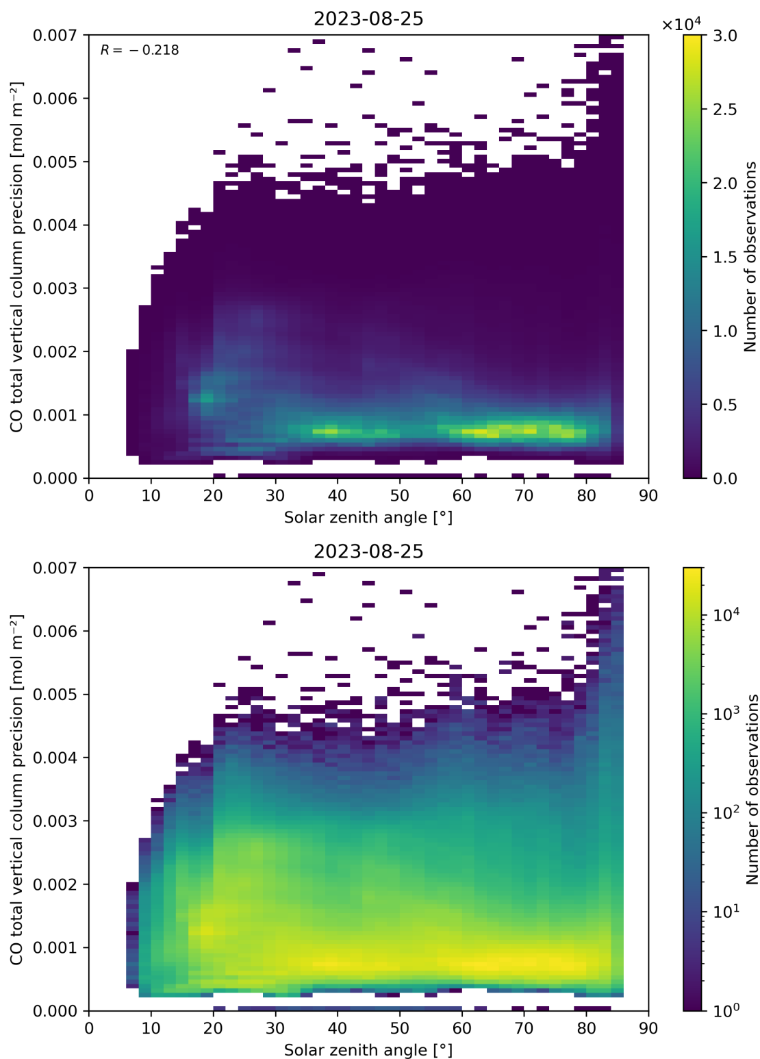
Figure 63: Scatter density plot of “Solar zenith angle” against “CO total vertical column precision” for 2023-08-25 to 2023-08-26.
