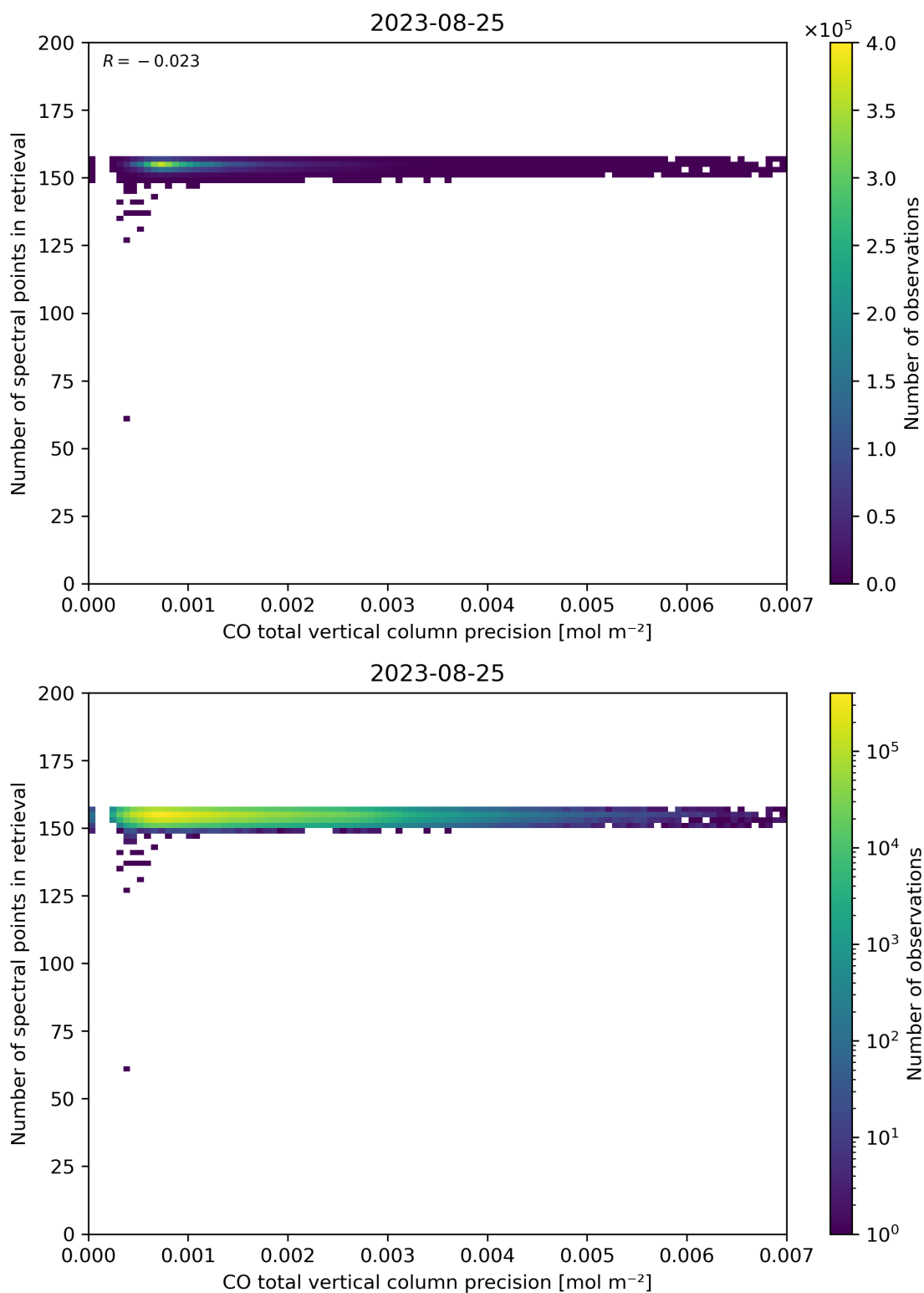
Figure 47: Scatter density plot of “CO total vertical column precision” against “Number of spectral points in retrieval” for 2023-08-25 to 2023-08-26.
