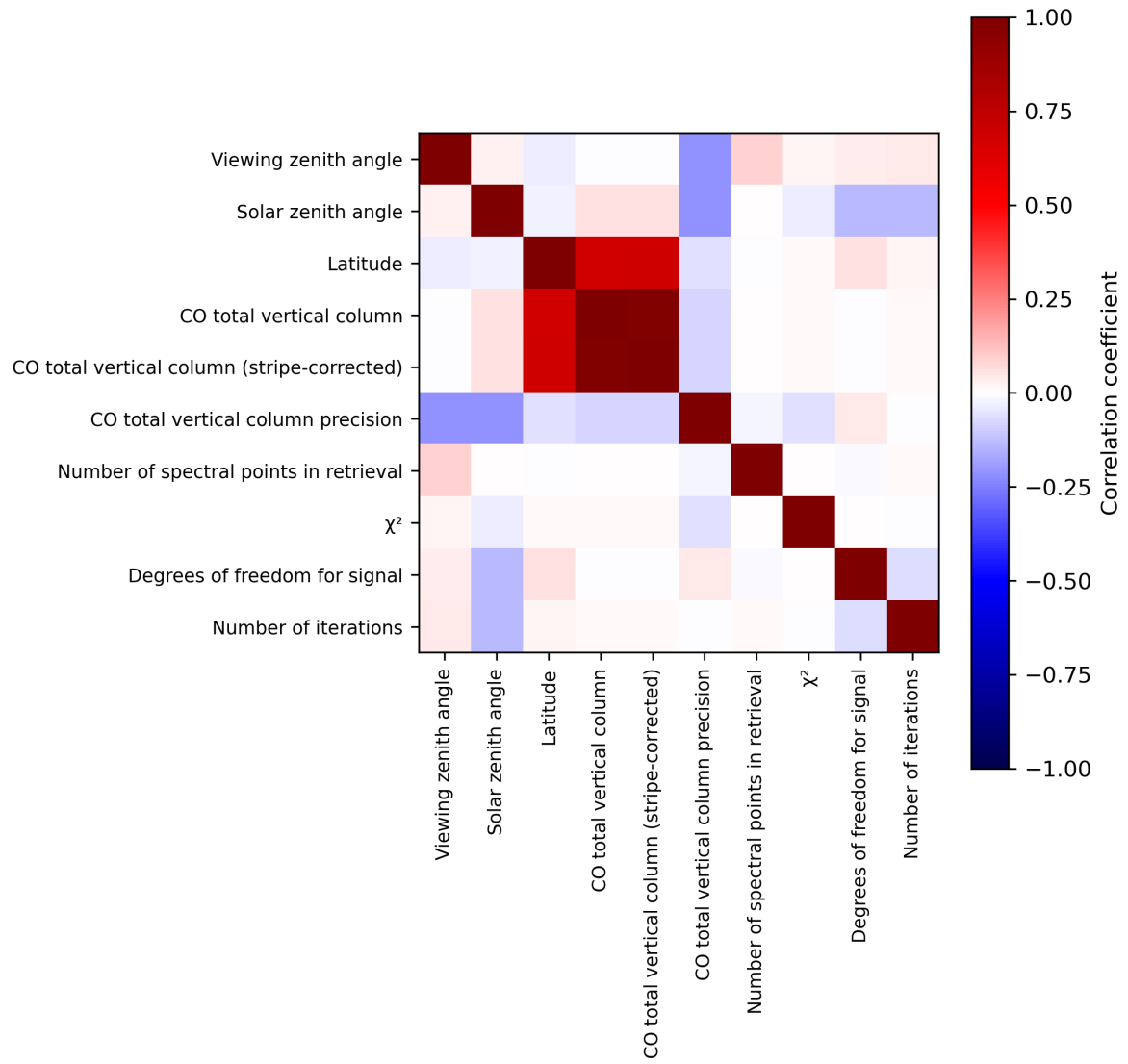
Figure 2: Map of correlation matrix for 2023-08-25 to 2023-08-26.
