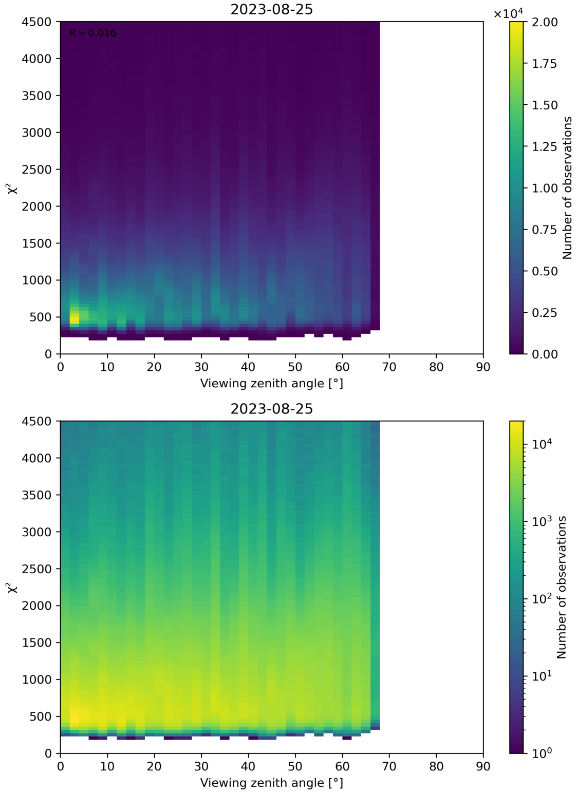
Figure 72: Scatter density plot of “Viewing zenith angle” against “ \chi^2 ” for 2023-08-25 to 2023-08-26.
