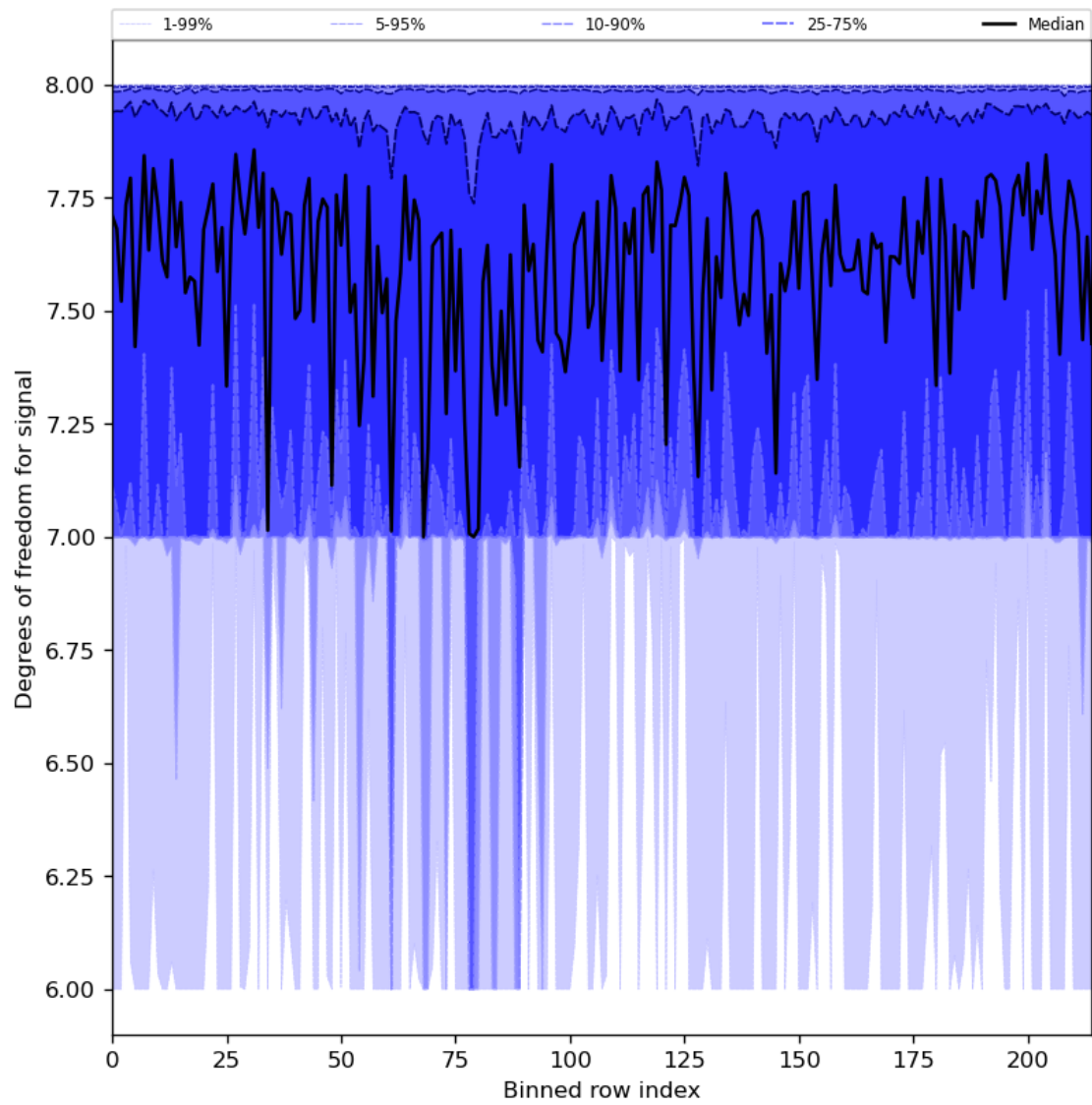
Figure 31: Along track statistics of “Degrees of freedom for signal” for 2023-08-25 to 2023-08-26
