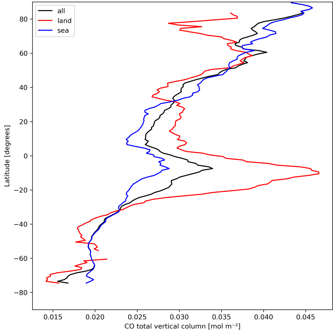
Figure 10: Zonal average of “CO total vertical column” for 2023-08-25 to 2023-08-26.
