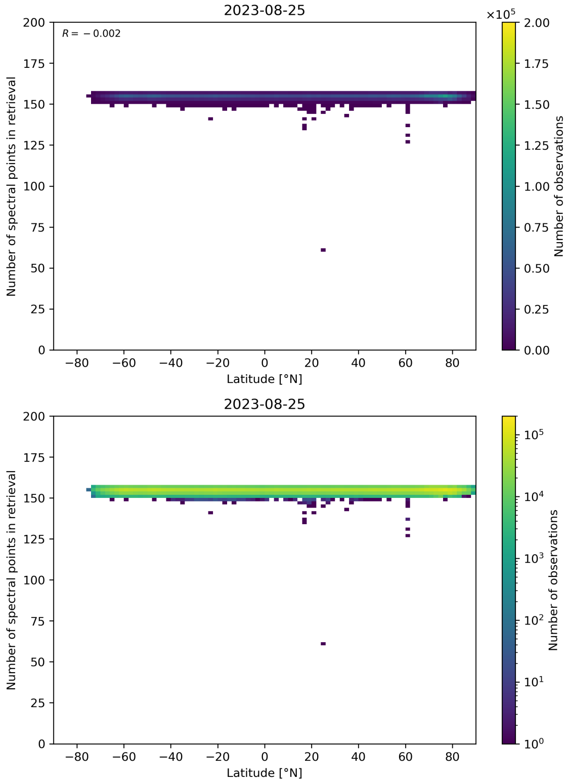
Figure 57: Scatter density plot of “Latitude” against “Number of spectral points in retrieval” for 2023-08-25 to 2023-08-26.
