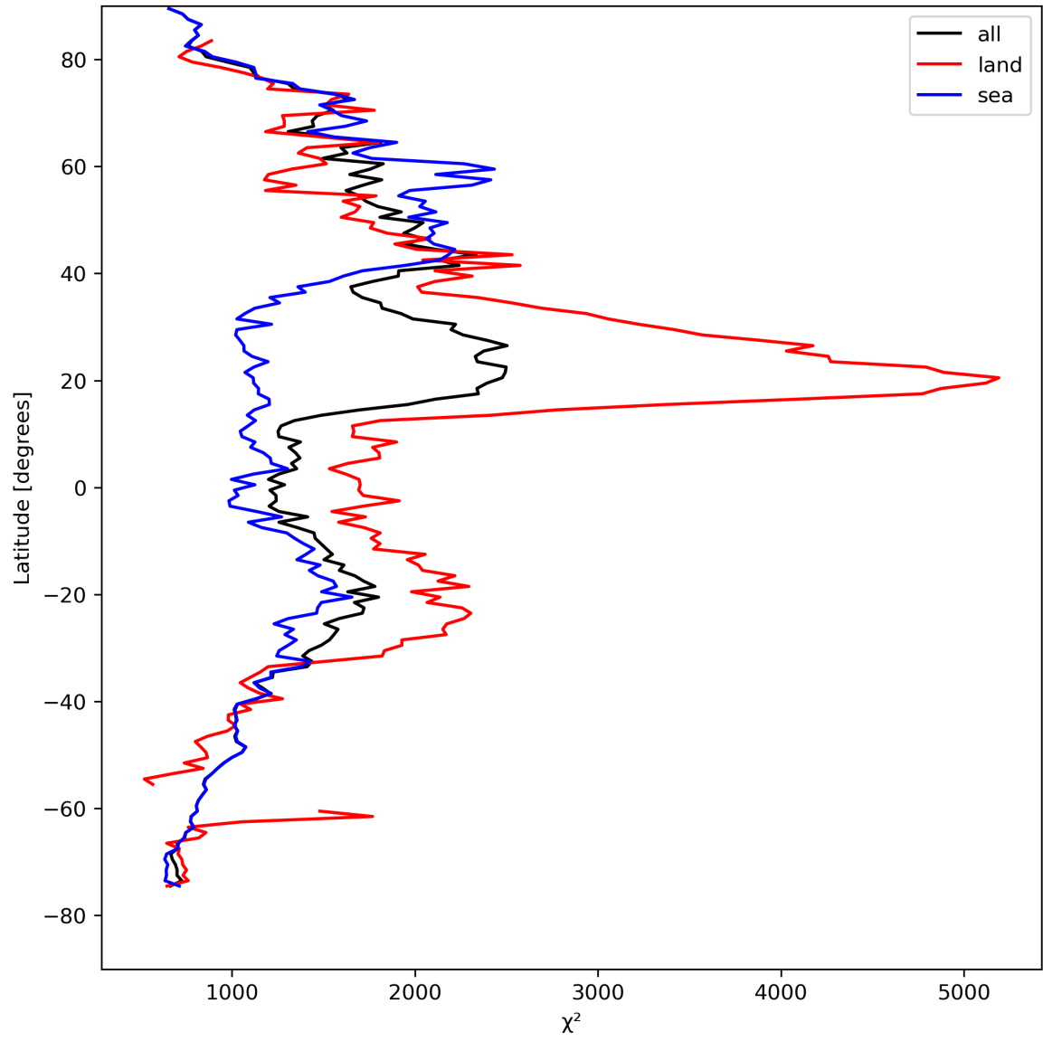
Figure 14: Zonal average of “ \chi^2 ” for 2023-08-25 to 2023-08-26.
