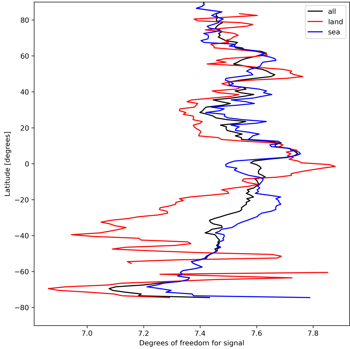
Figure 15: Zonal average of “Degrees of freedom for signal” for 2023-08-25 to 2023-08-26.
