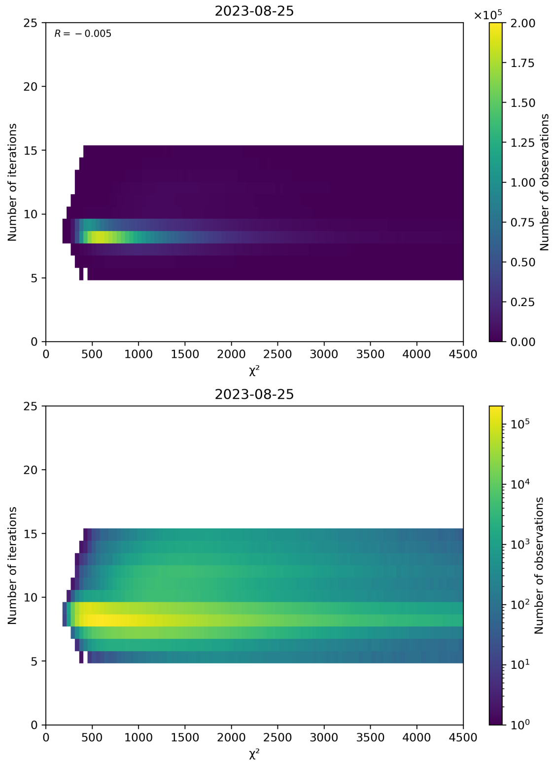
Figure 49: Scatter density plot of “ \chi^2 ” against “Number of iterations” for 2023-08-25 to 2023-08-26.
