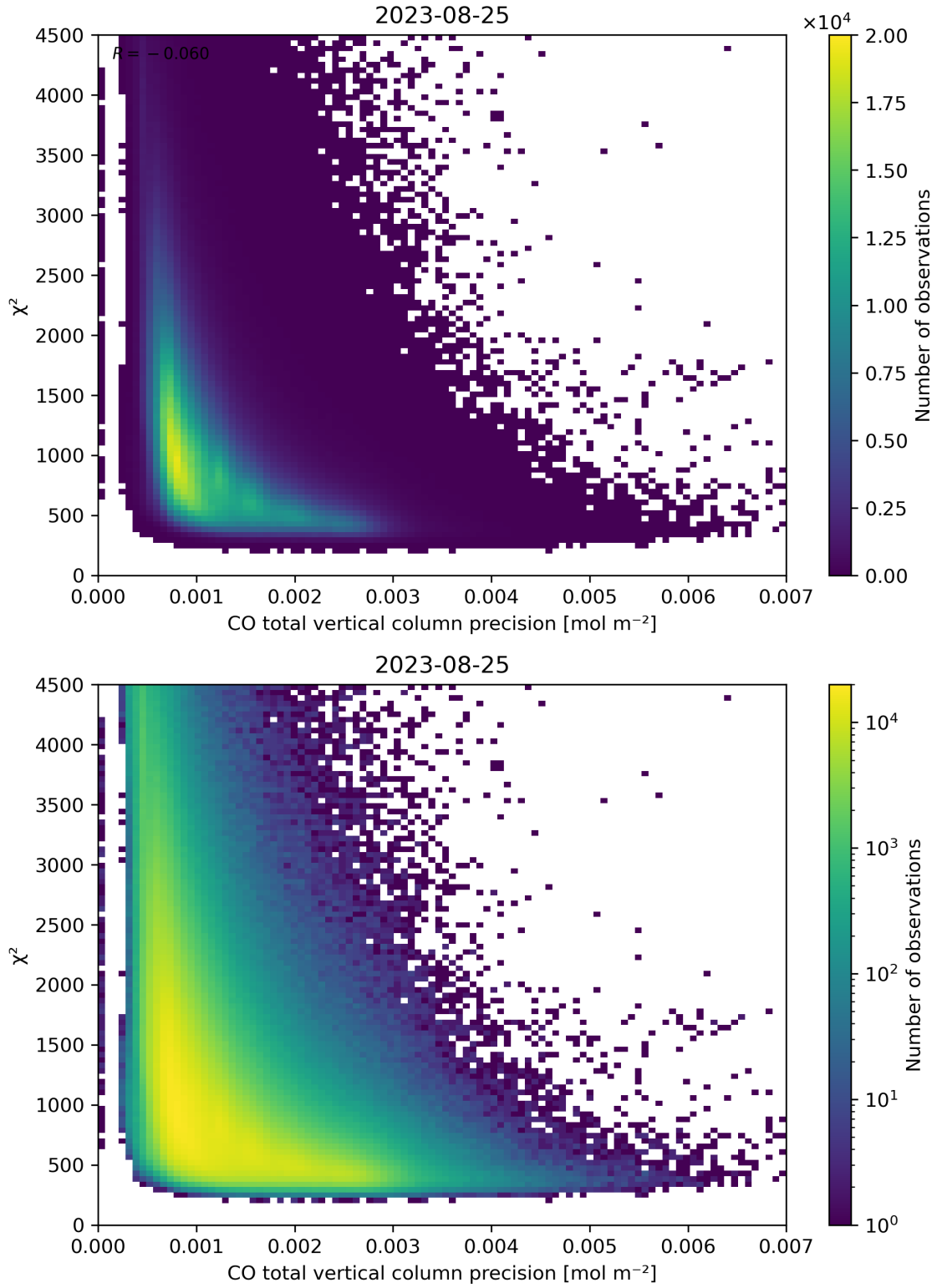
Figure 44: Scatter density plot of “CO total vertical column precision” against “ \chi^2 ” for 2023-08-25 to 2023-08-26.
