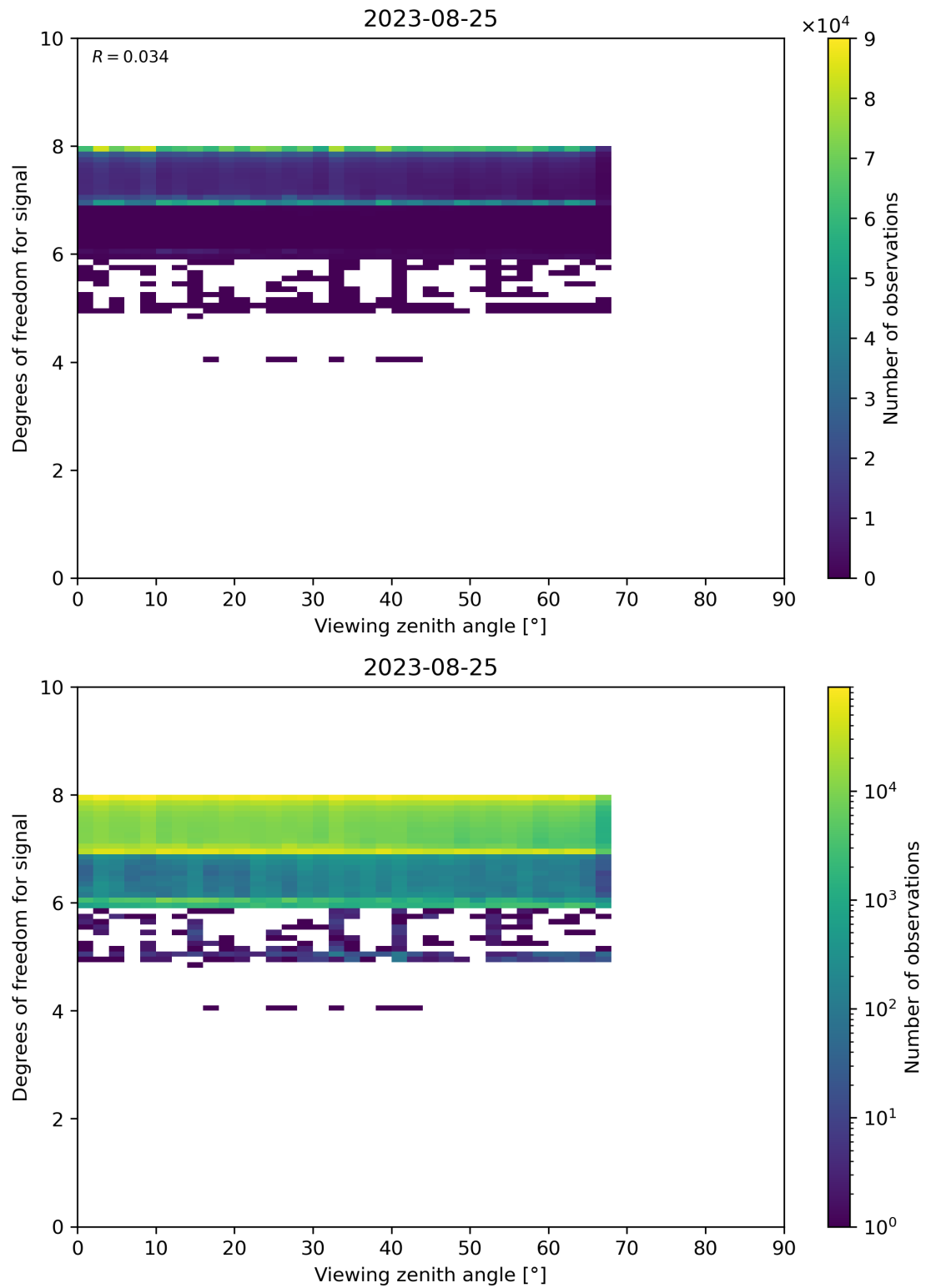
Figure 73: Scatter density plot of “Viewing zenith angle” against “Degrees of freedom for signal” for 2023-08-25 to 2023-08-26.
