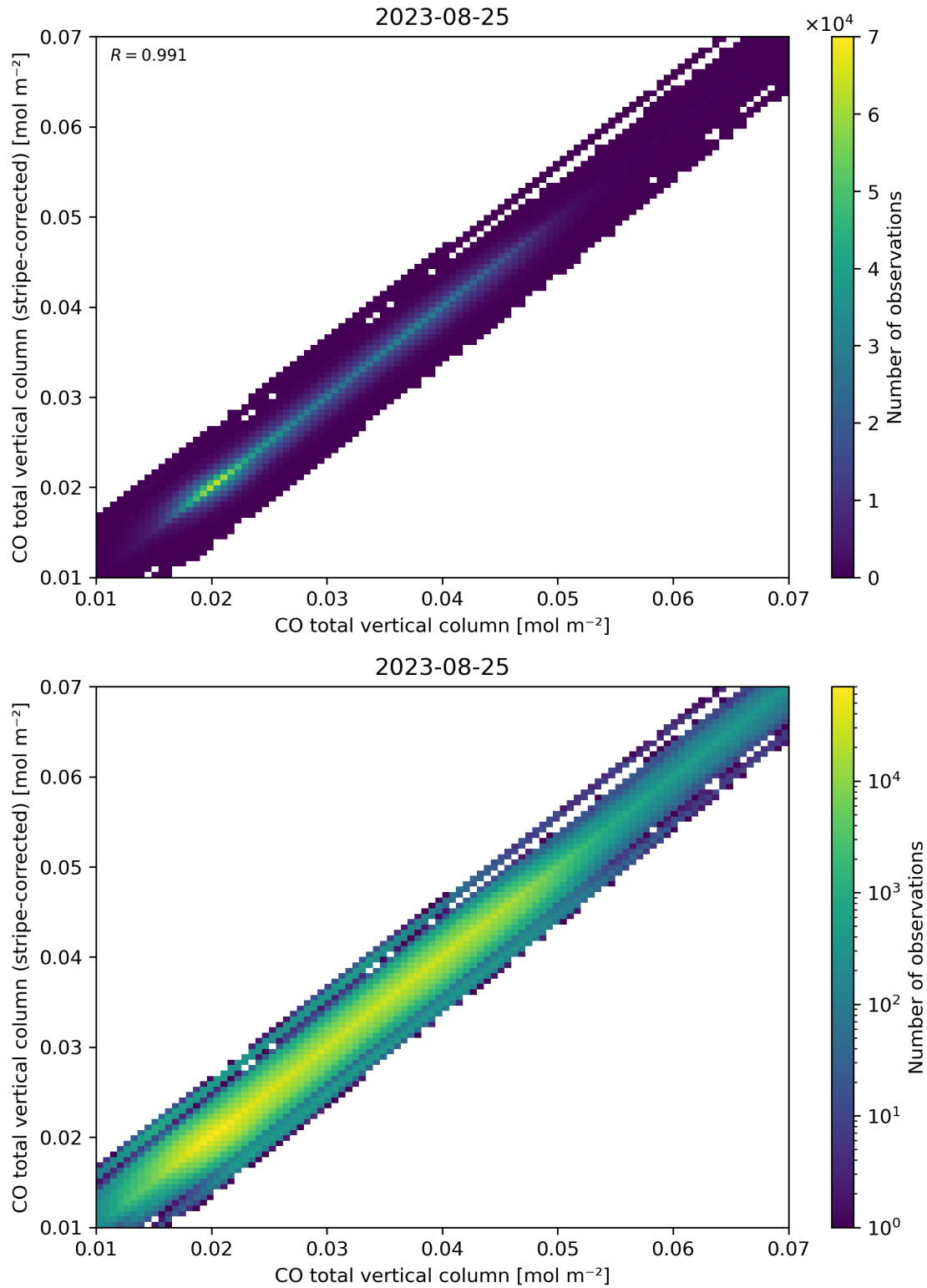
Figure 33: Scatter density plot of “CO total vertical column” against “CO total vertical column (stripe-corrected)” for 2023-08-25 to 2023-08-26.
