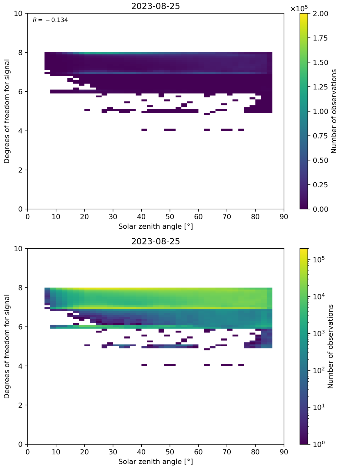
Figure 65: Scatter density plot of “Solar zenith angle” against “Degrees of freedom for signal” for 2023-08-25 to 2023-08-26.
