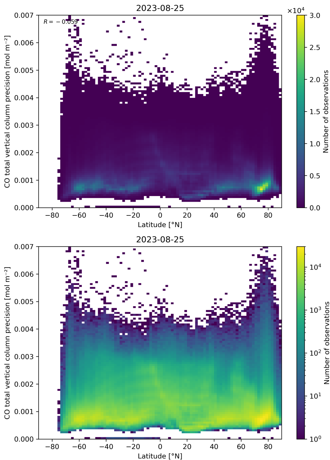
Figure 53: Scatter density plot of “Latitude” against “CO total vertical column precision” for 2023-08-25 to 2023-08-26.
