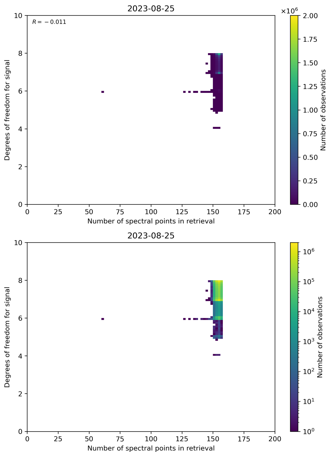
Figure 59: Scatter density plot of “Number of spectral points in retrieval” against “Degrees of freedom for signal” for 2023-08-25 to 2023-08-26.
