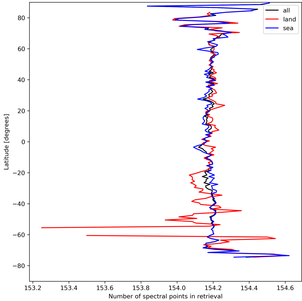
Figure 13: Zonal average of “Number of spectral points in retrieval” for 2023-08-25 to 2023-08-26.
