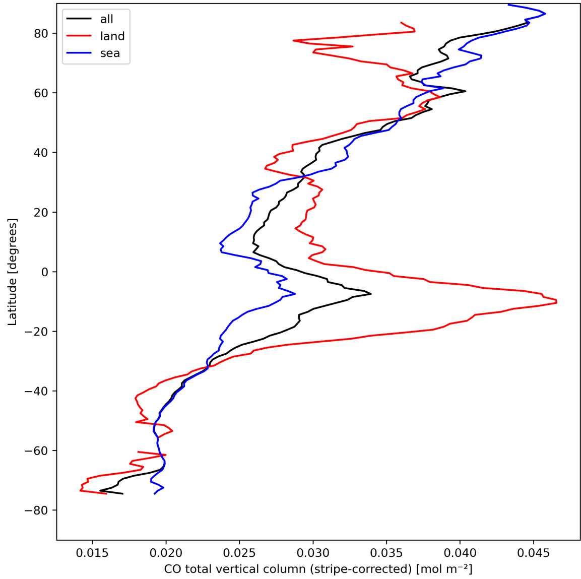
Figure 11: Zonal average of “CO total vertical column (stripe-corrected)” for 2023-08-25 to 2023-08-26.
