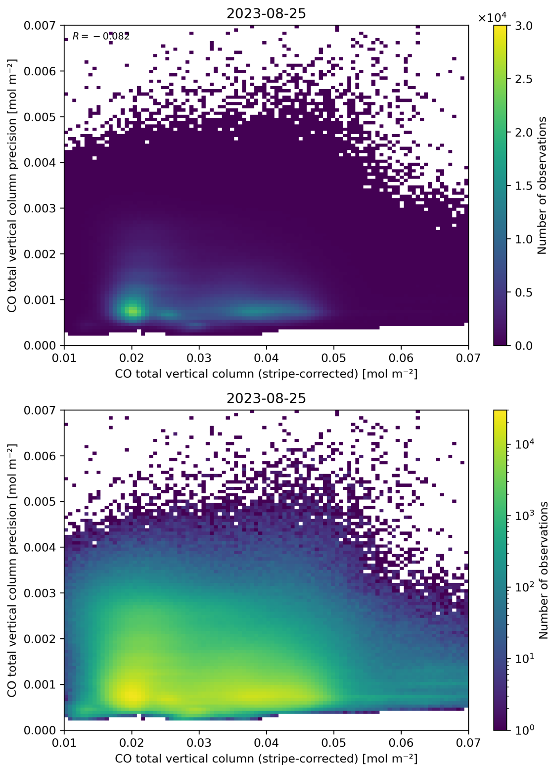
Figure 36: Scatter density plot of “CO total vertical column (stripe-corrected)” against “CO total vertical column precision” for 2023-08-25 to 2023-08-26.
