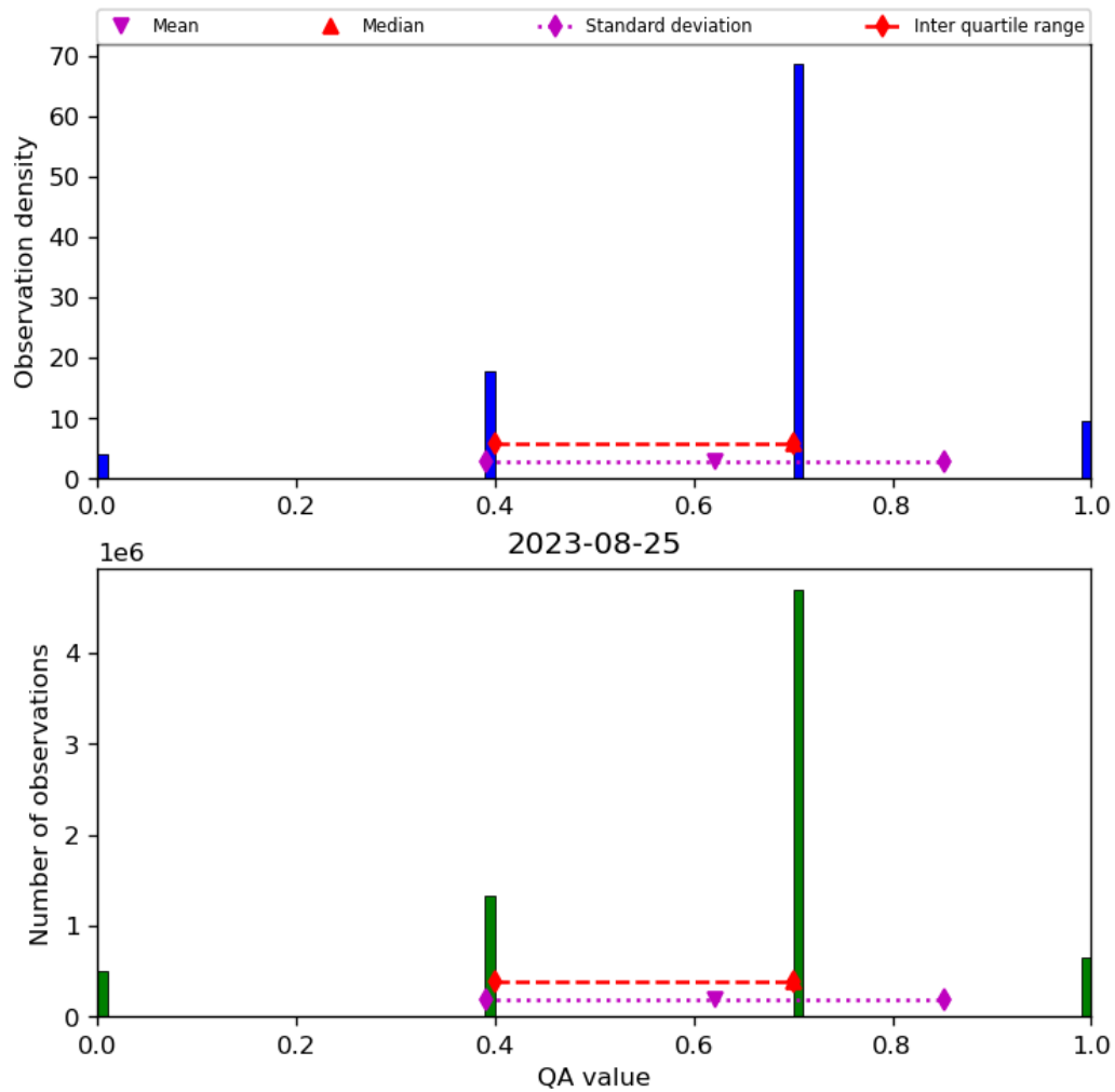
Figure 17: Histogram of “QA value” for 2023-08-25 to 2023-08-26
