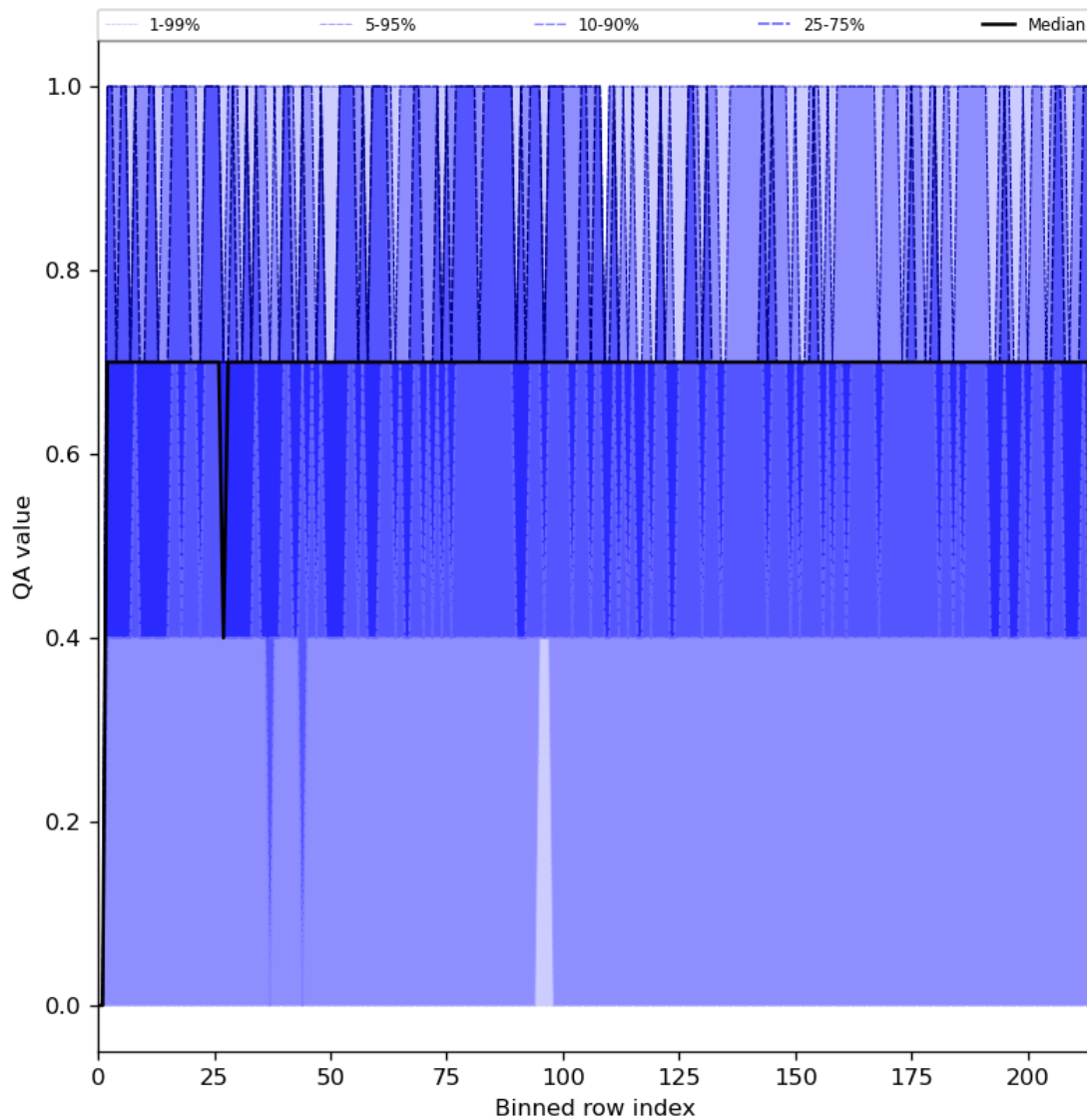
Figure 25: Along track statistics of “QA value” for 2023-08-25 to 2023-08-26
