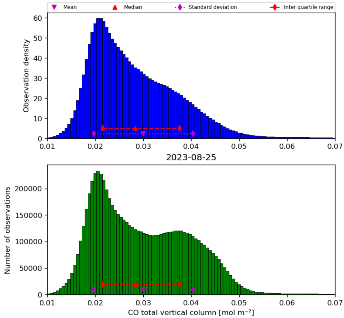
Figure 18: Histogram of “CO total vertical column” for 2023-08-25 to 2023-08-26
