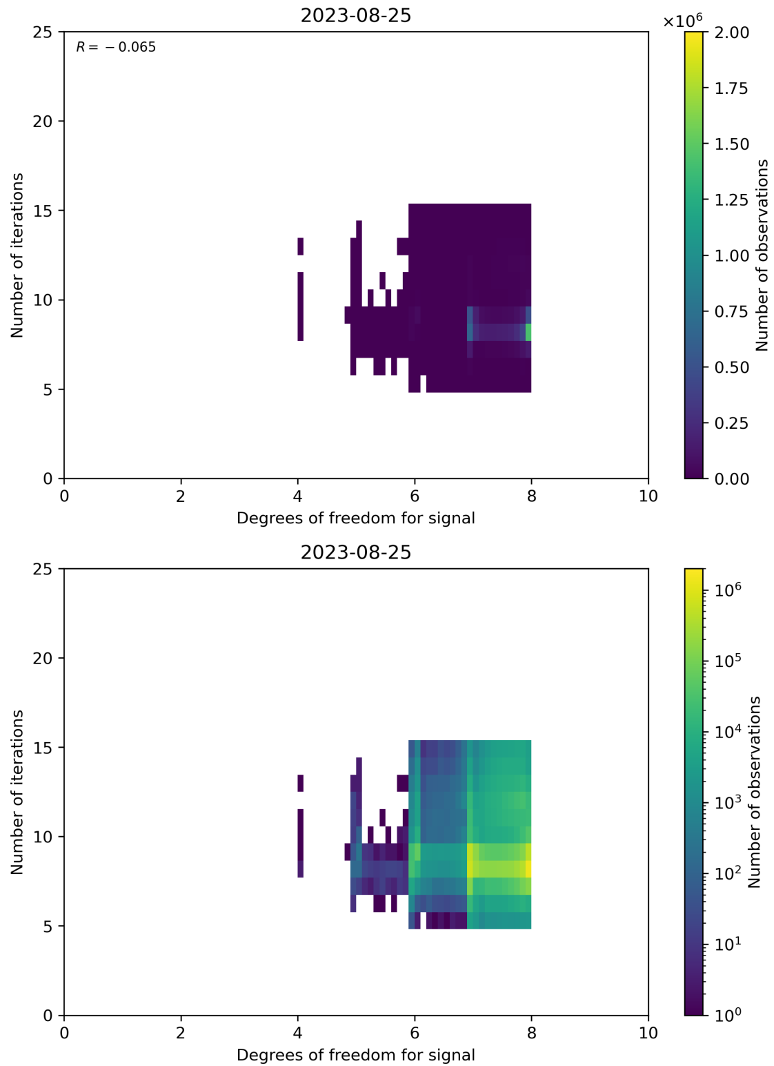
Figure 50: Scatter density plot of “Degrees of freedom for signal” against “Number of iterations” for 2023-08-25 to 2023-08-26.
