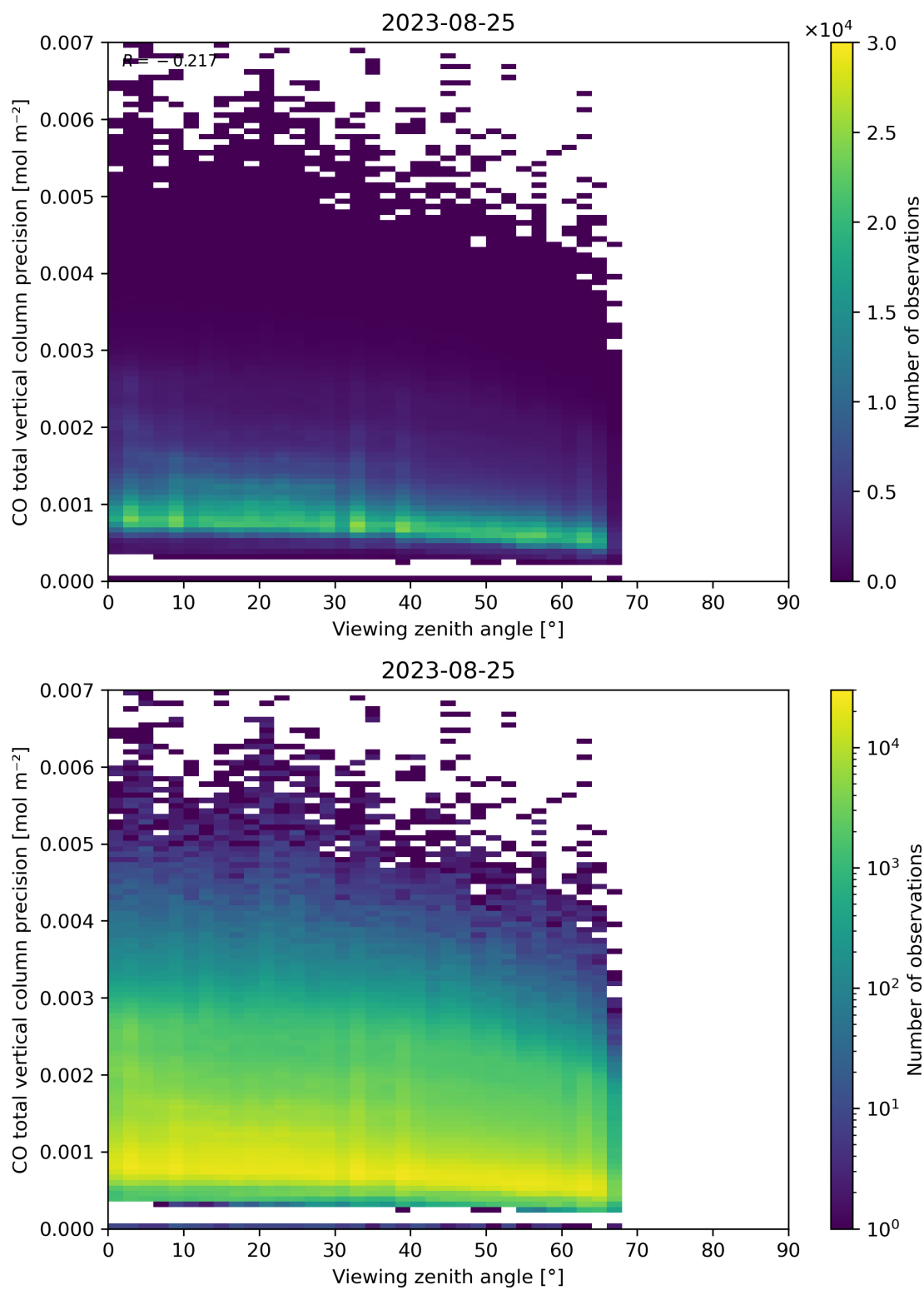
Figure 71: Scatter density plot of “Viewing zenith angle” against “CO total vertical column precision” for 2023-08-25 to 2023-08-26.
