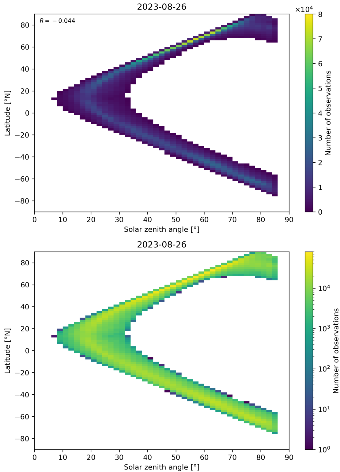
Figure 66: Scatter density plot of “Solar zenith angle” against “Latitude” for 2023-08-25 to 2023-08-27.
