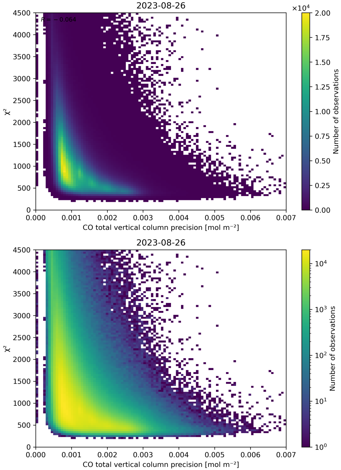
Figure 44: Scatter density plot of “CO total vertical column precision” against “ \chi^2 ” for 2023-08-25 to 2023-08-27.
