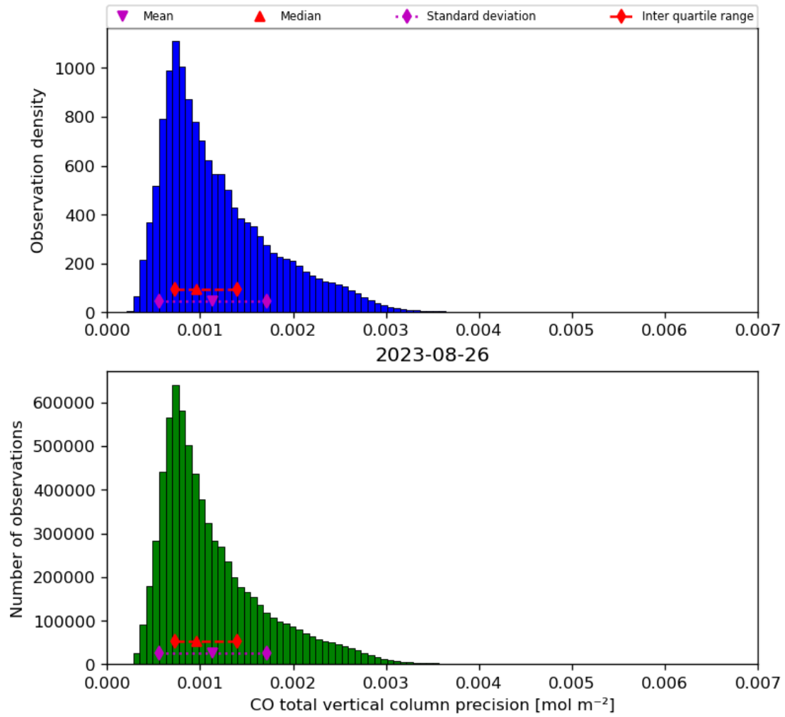
Figure 20: Histogram of “CO total vertical column precision” for 2023-08-25 to 2023-08-27
