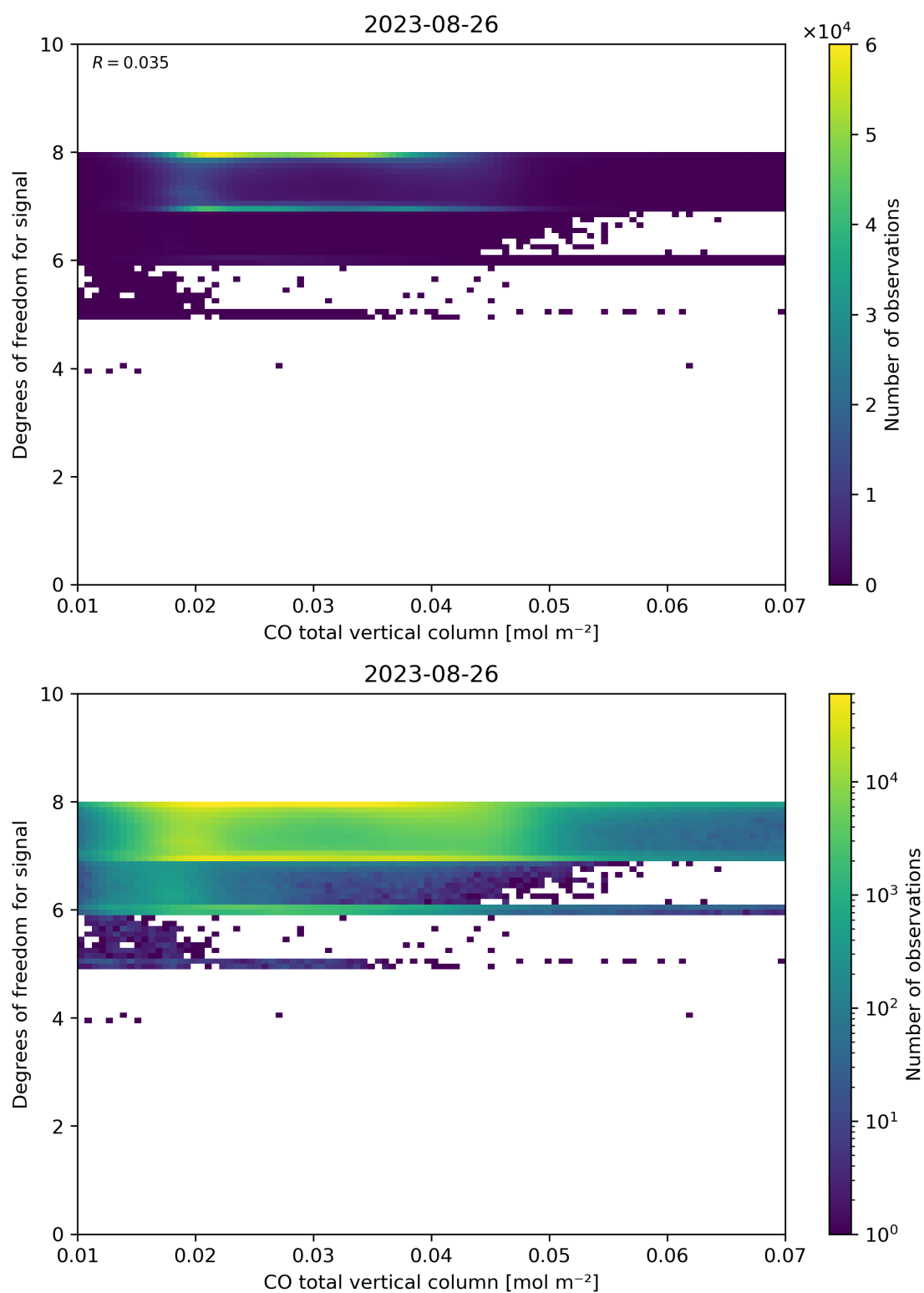
Figure 41: Scatter density plot of “CO total vertical column” against “Degrees of freedom for signal” for 2023-08-25 to 2023-08-27.
