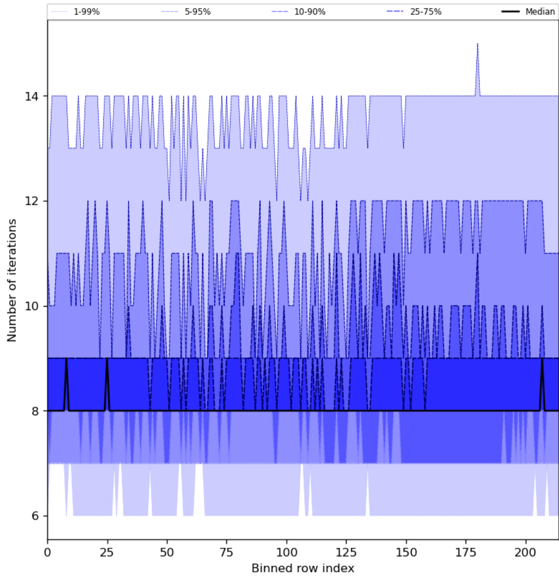
Figure 32: Along track statistics of “Number of iterations” for 2023-08-25 to 2023-08-27
