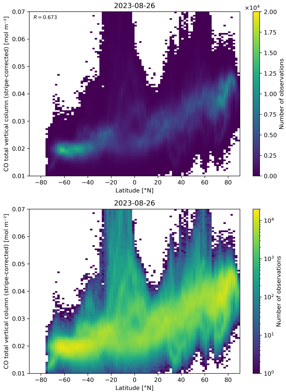
Figure 52: Scatter density plot of “Latitude” against “CO total vertical column (stripe-corrected)” for 2023-08-25 to 2023-08-27.
