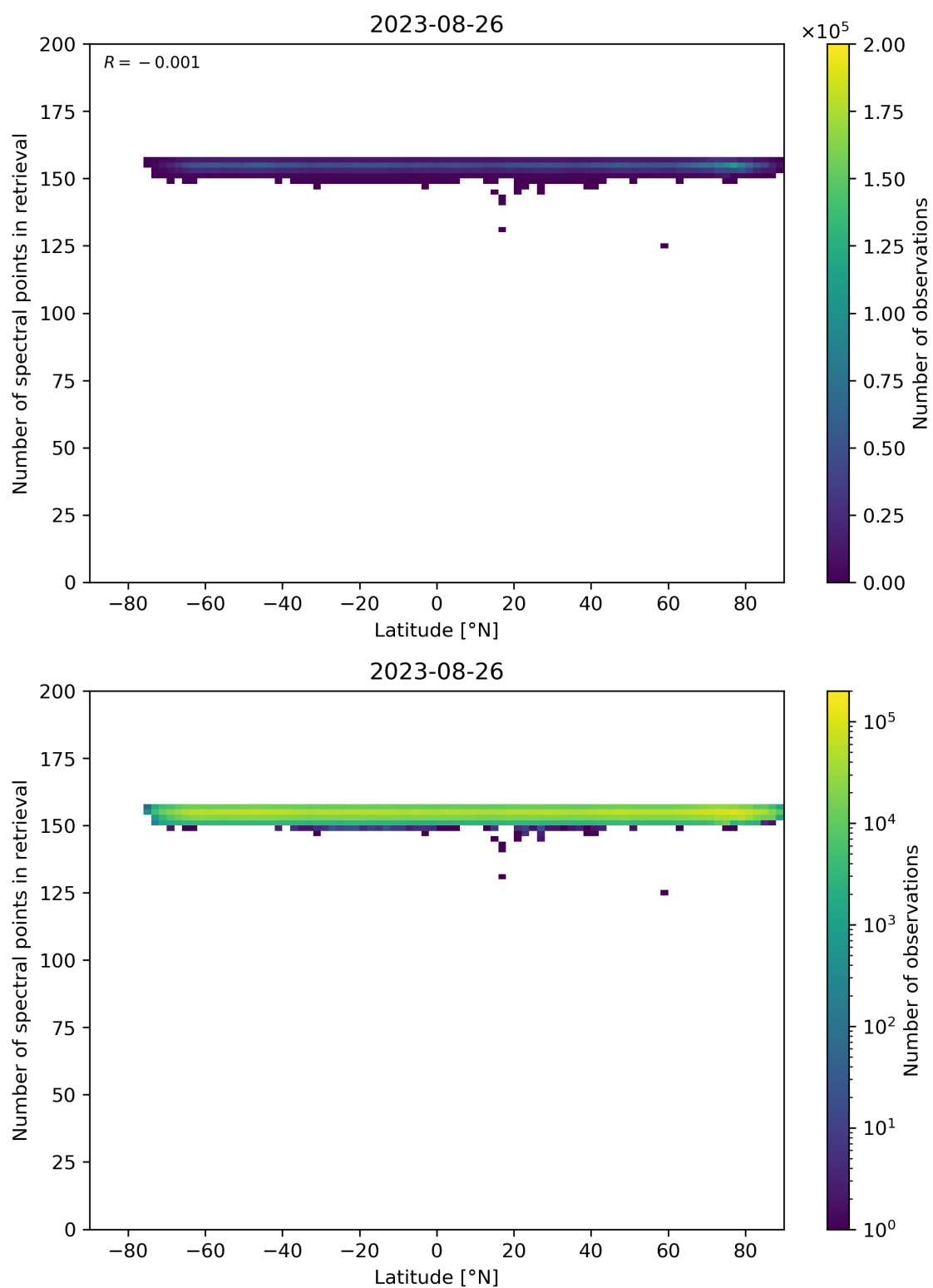
Figure 57: Scatter density plot of “Latitude” against “Number of spectral points in retrieval” for 2023-08-25 to 2023-08-27.
