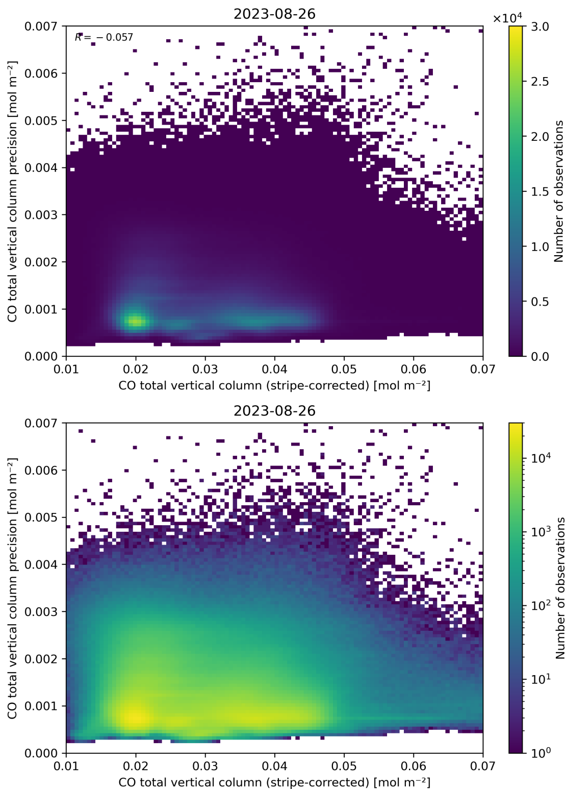
Figure 36: Scatter density plot of “CO total vertical column (stripe-corrected)” against “CO total vertical column precision” for 2023-08-25 to 2023-08-27.
