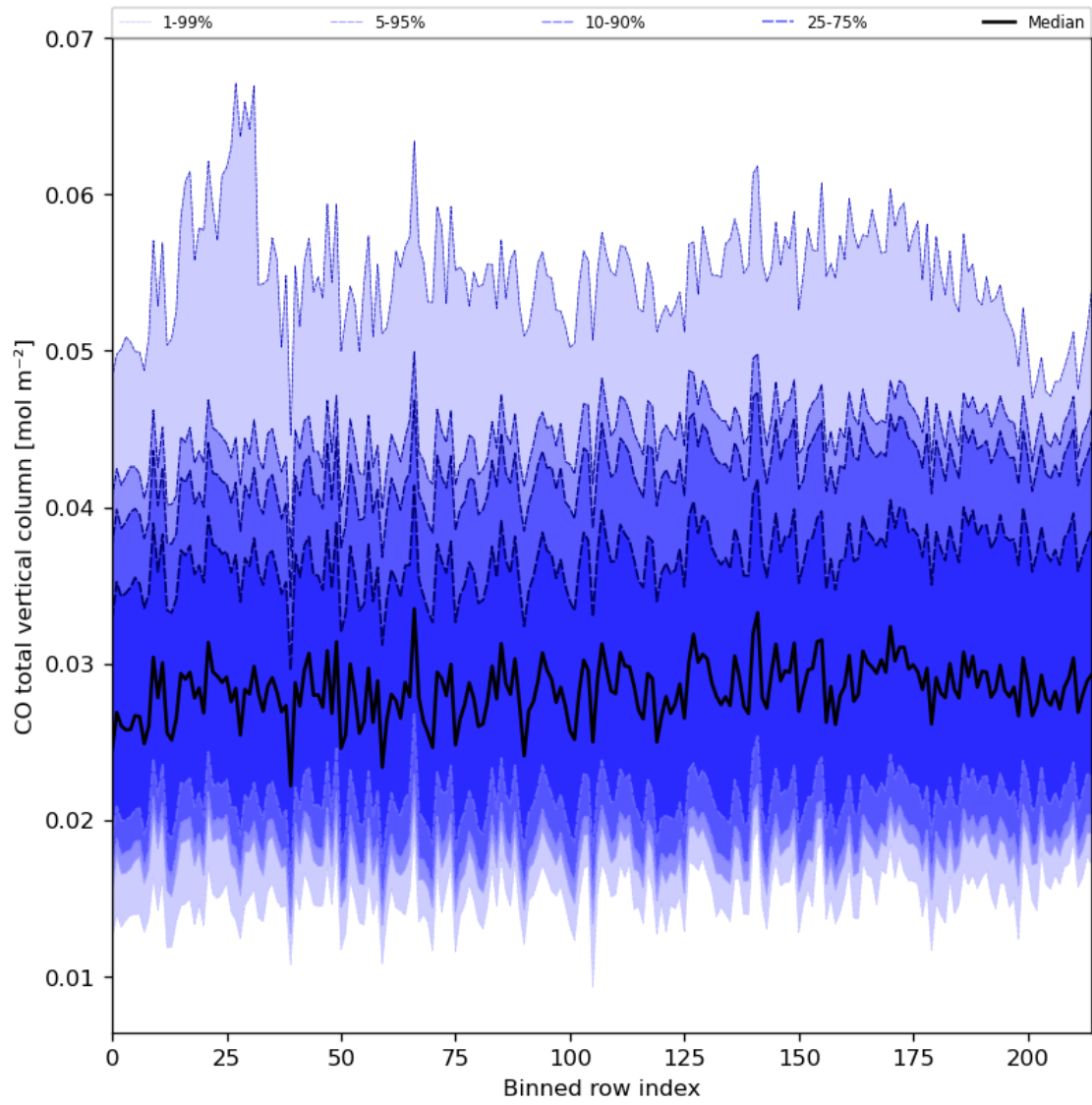
Figure 26: Along track statistics of “CO total vertical column” for 2023-08-25 to 2023-08-27
