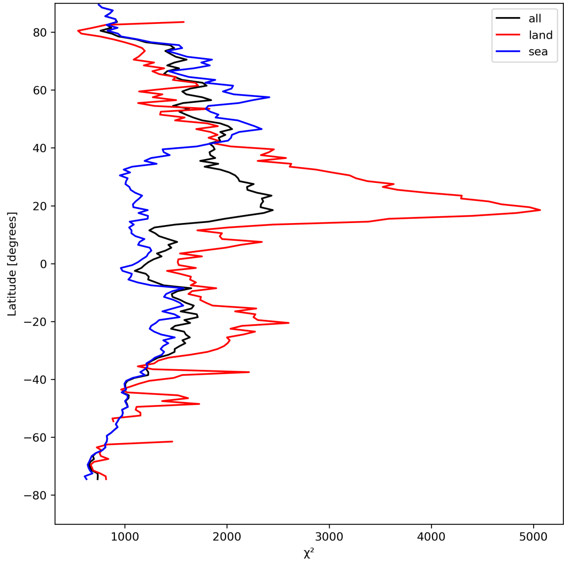
Figure 14: Zonal average of “ \chi^2 ” for 2023-08-25 to 2023-08-27.
