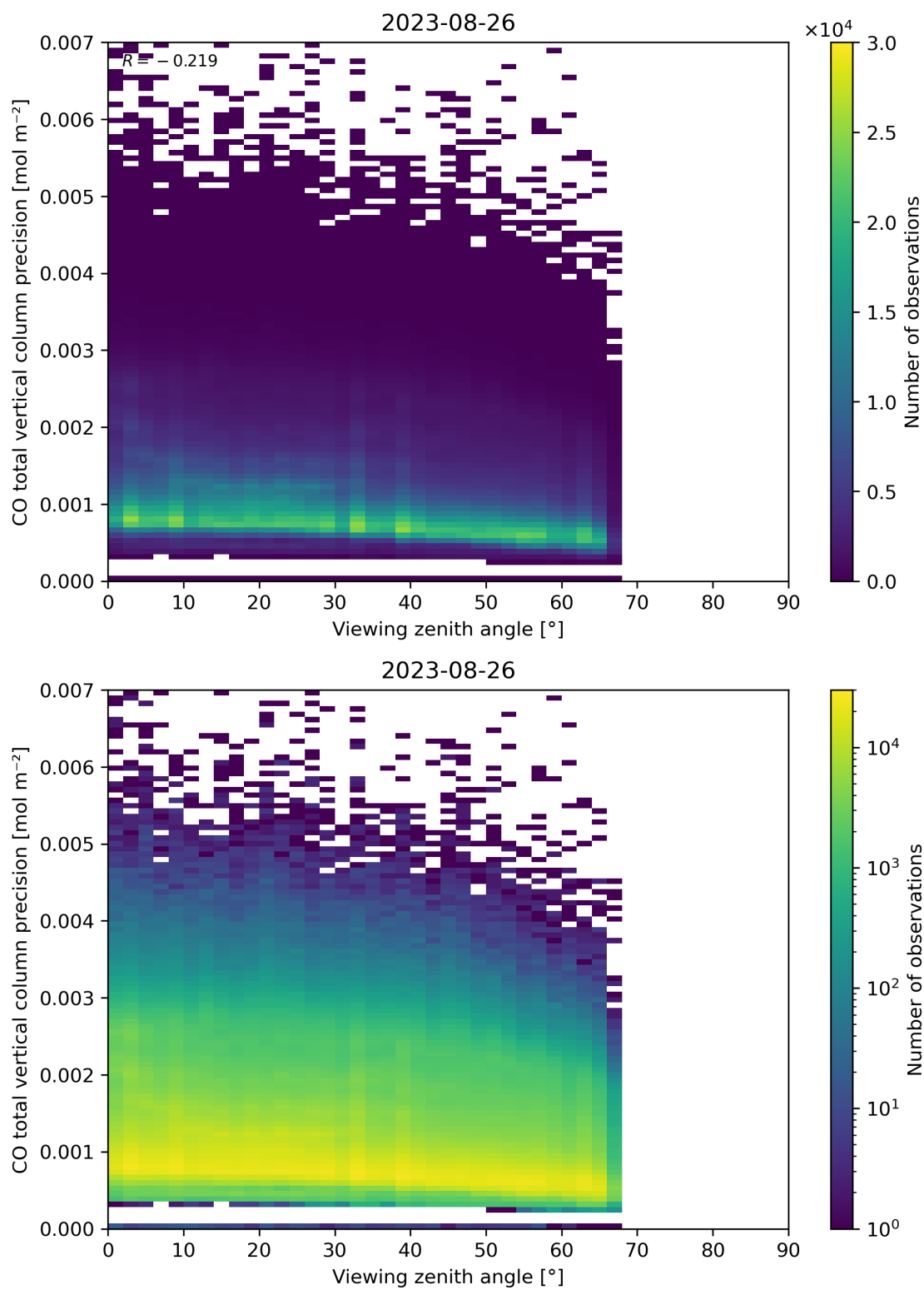
Figure 71: Scatter density plot of “Viewing zenith angle” against “CO total vertical column precision” for 2023-08-25 to 2023-08-27.
