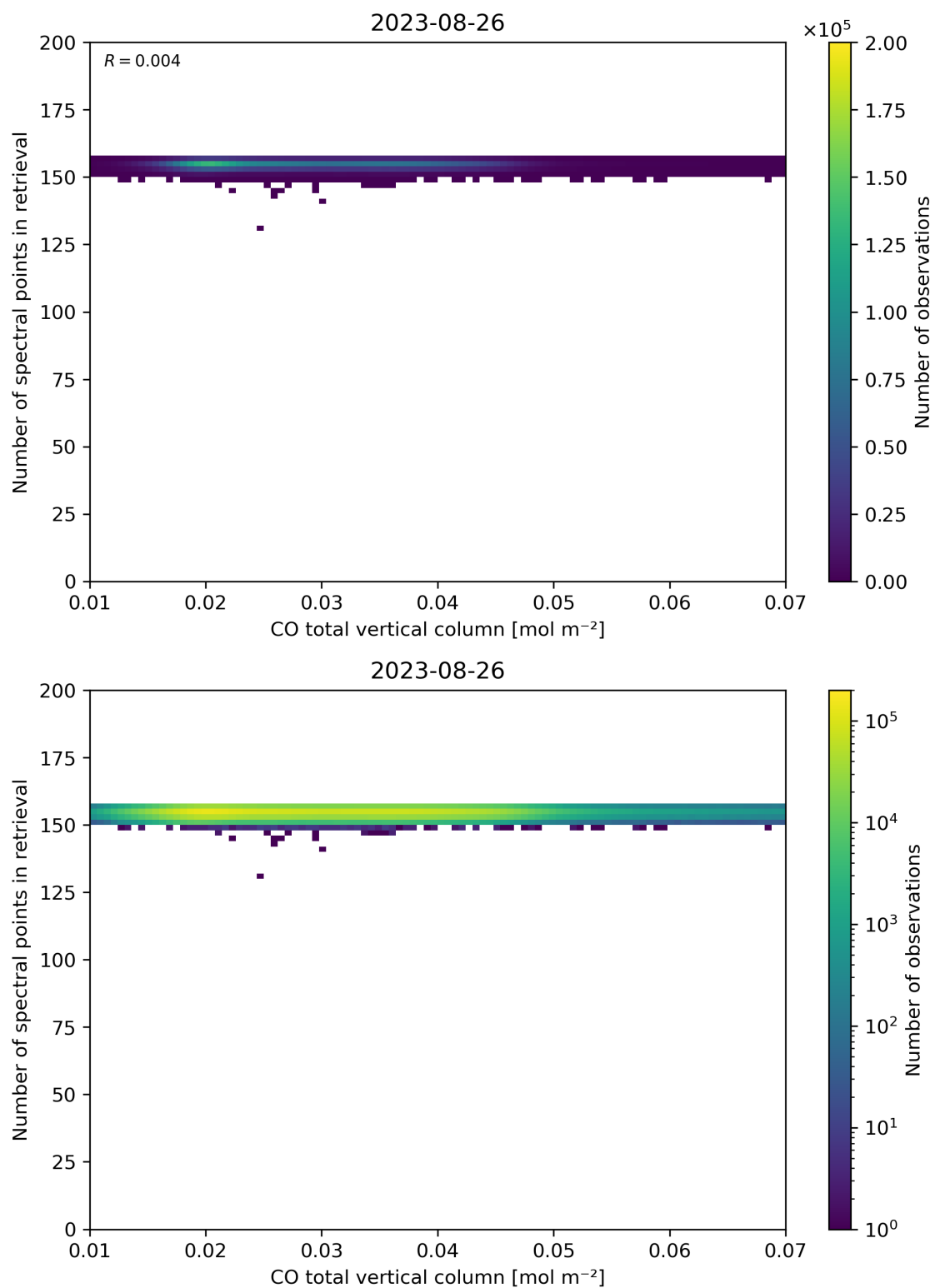
Figure 43: Scatter density plot of “CO total vertical column” against “Number of spectral points in retrieval” for 2023-08-25 to 2023-08-27.
