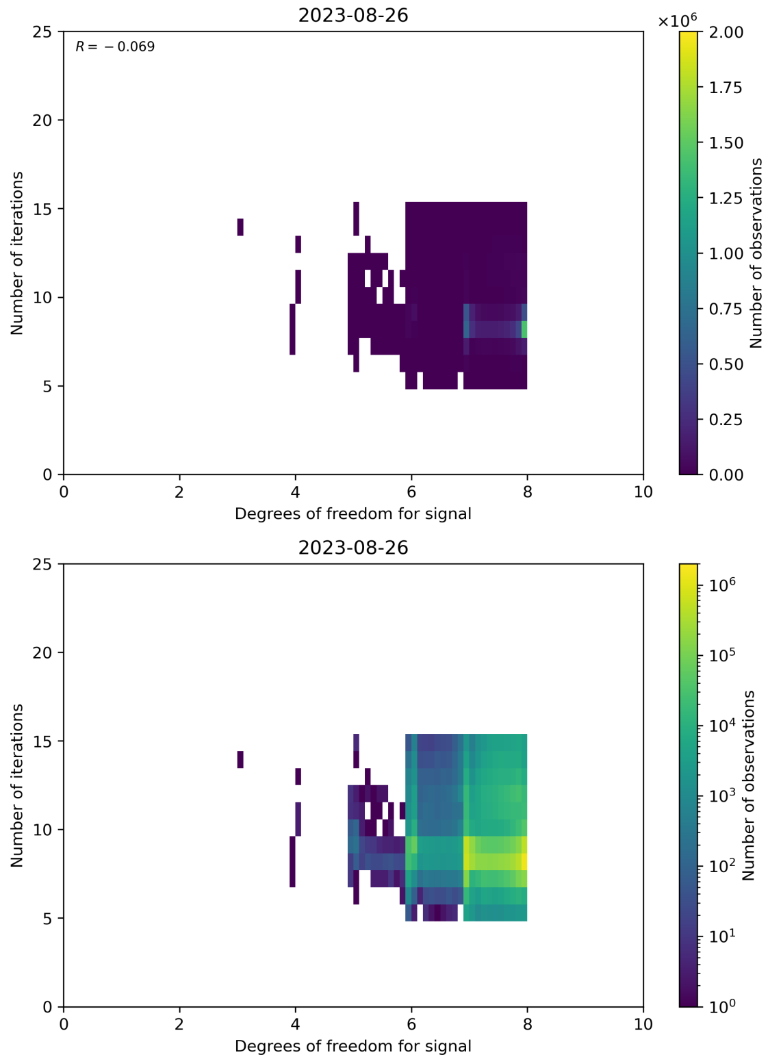
Figure 50: Scatter density plot of “Degrees of freedom for signal” against “Number of iterations” for 2023-08-25 to 2023-08-27.
