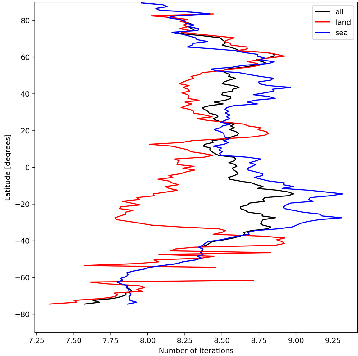
Figure 16: Zonal average of “Number of iterations” for 2023-08-25 to 2023-08-27.
