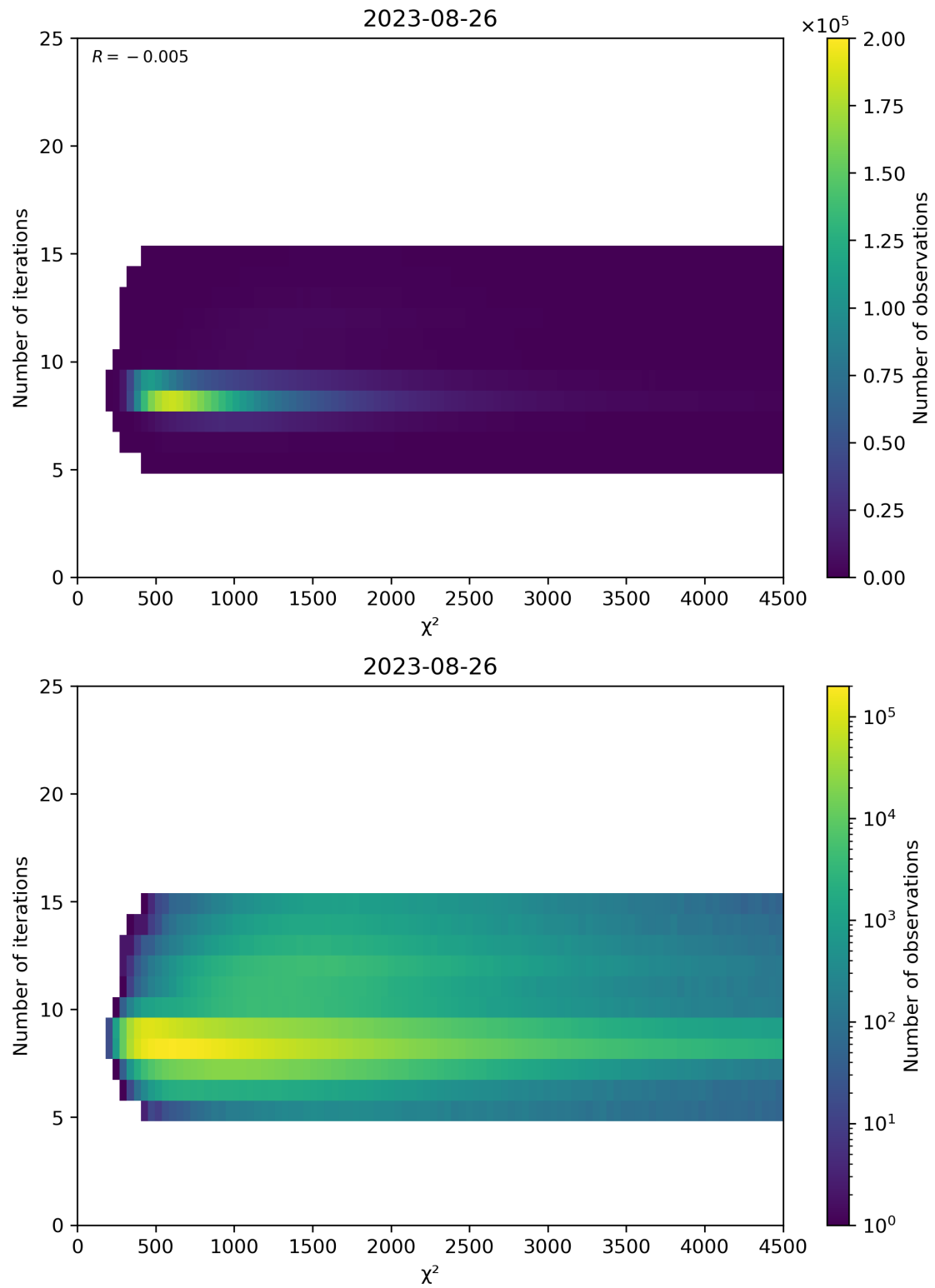
Figure 49: Scatter density plot of “ \chi^2 ” against “Number of iterations” for 2023-08-25 to 2023-08-27.
