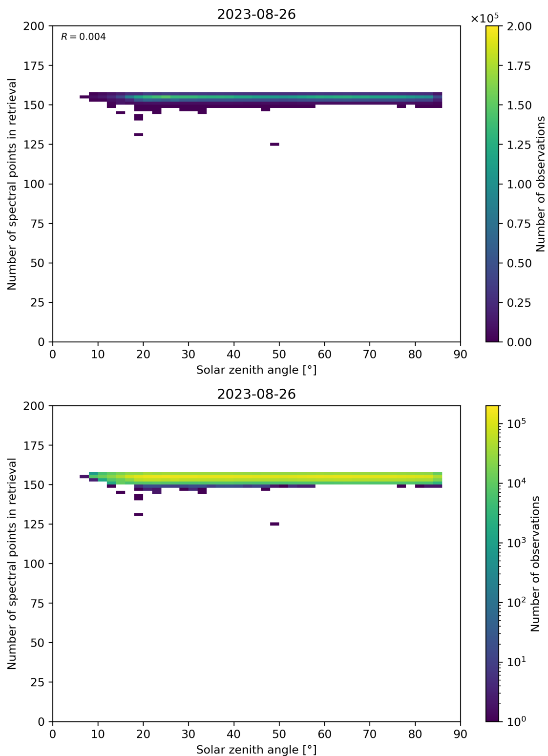
Figure 68: Scatter density plot of “Solar zenith angle” against “Number of spectral points in retrieval” for 2023-08-25 to 2023-08-27.
