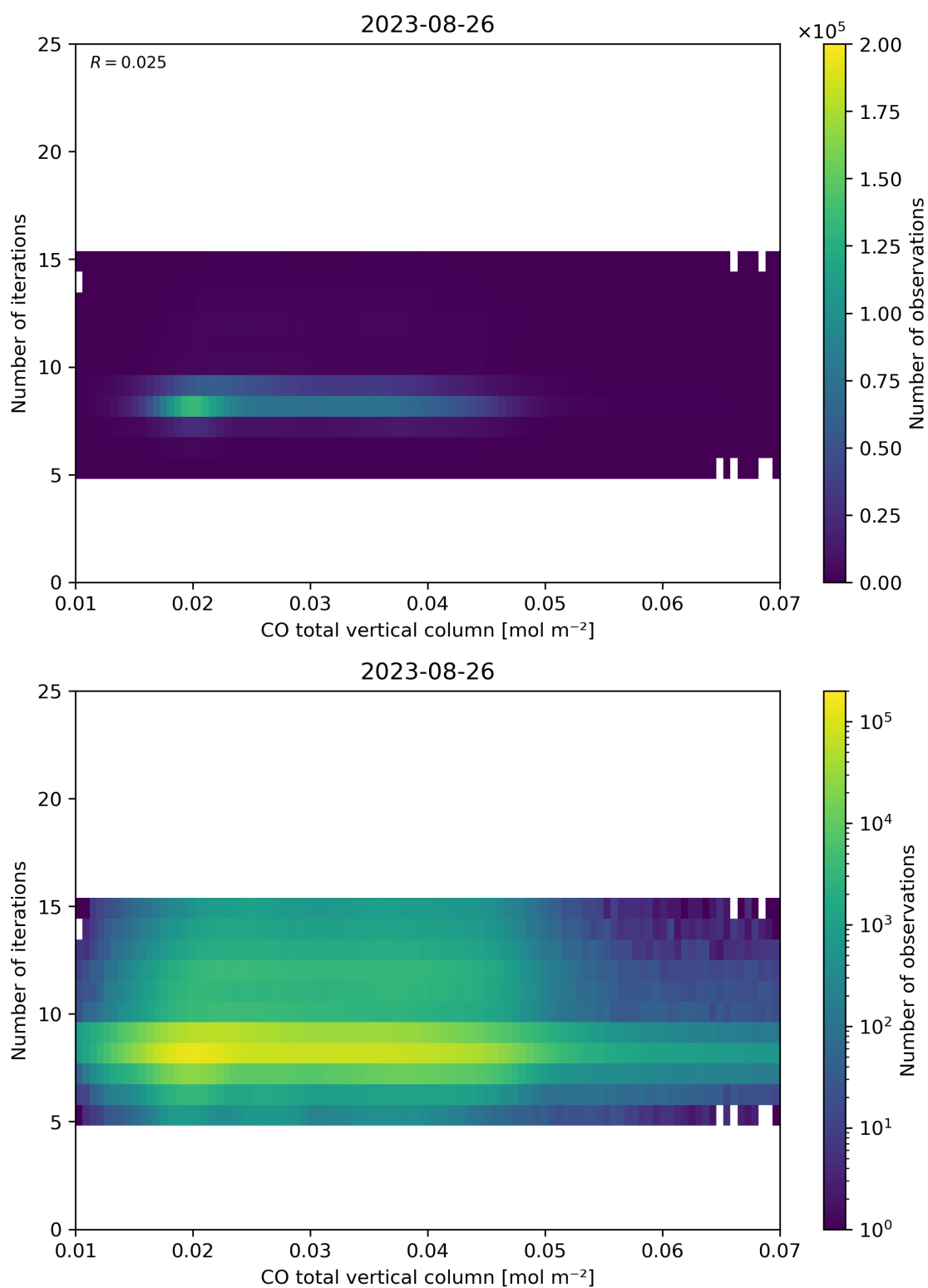
Figure 42: Scatter density plot of “CO total vertical column” against “Number of iterations” for 2023-08-25 to 2023-08-27.
