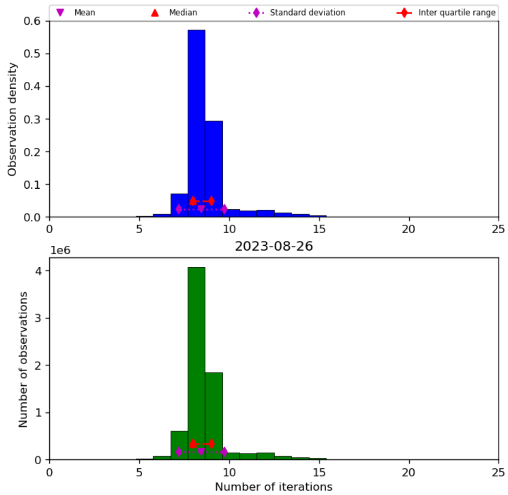
Figure 24: Histogram of “Number of iterations” for 2023-08-25 to 2023-08-27
