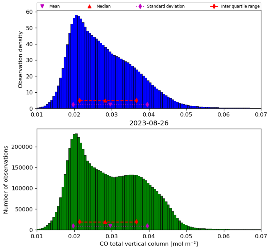
Figure 18: Histogram of “CO total vertical column” for 2023-08-25 to 2023-08-27
