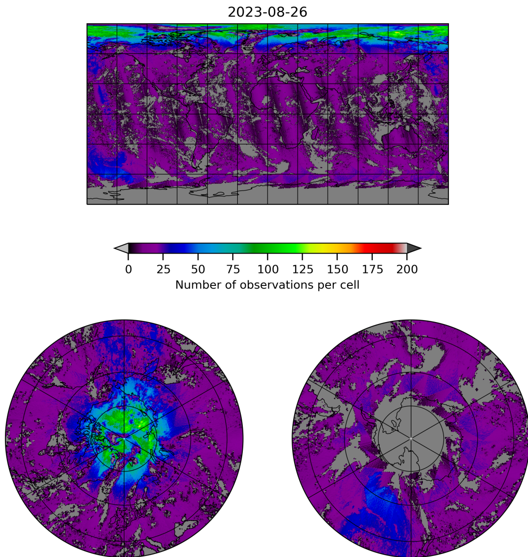
Figure 8: Map of the number of observations for 2023-08-25 to 2023-08-27
