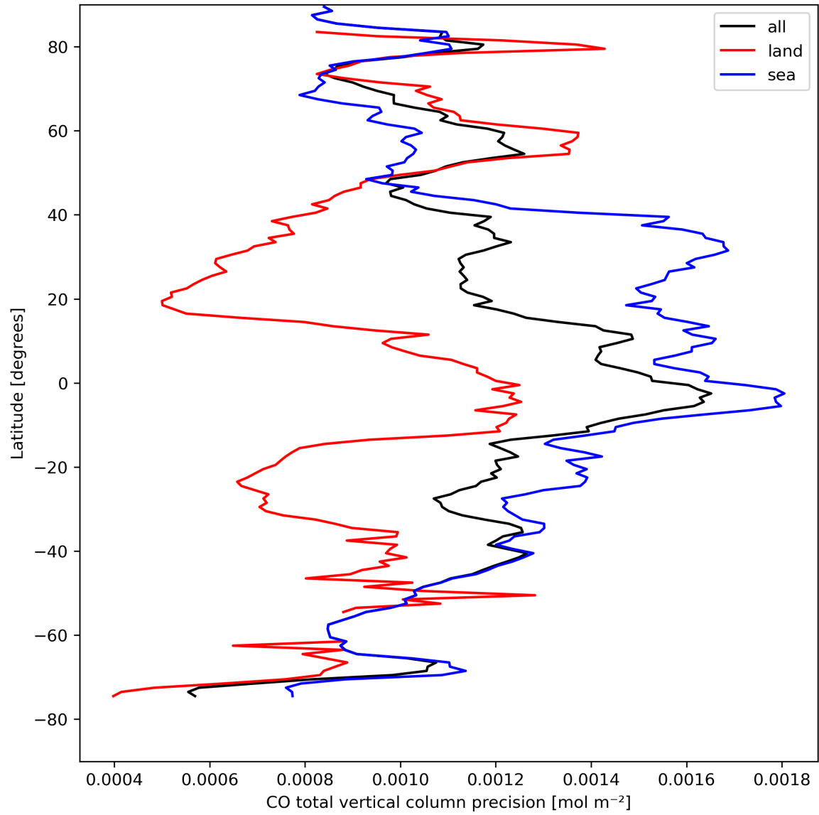
Figure 12: Zonal average of “CO total vertical column precision” for 2023-08-25 to 2023-08-27.
