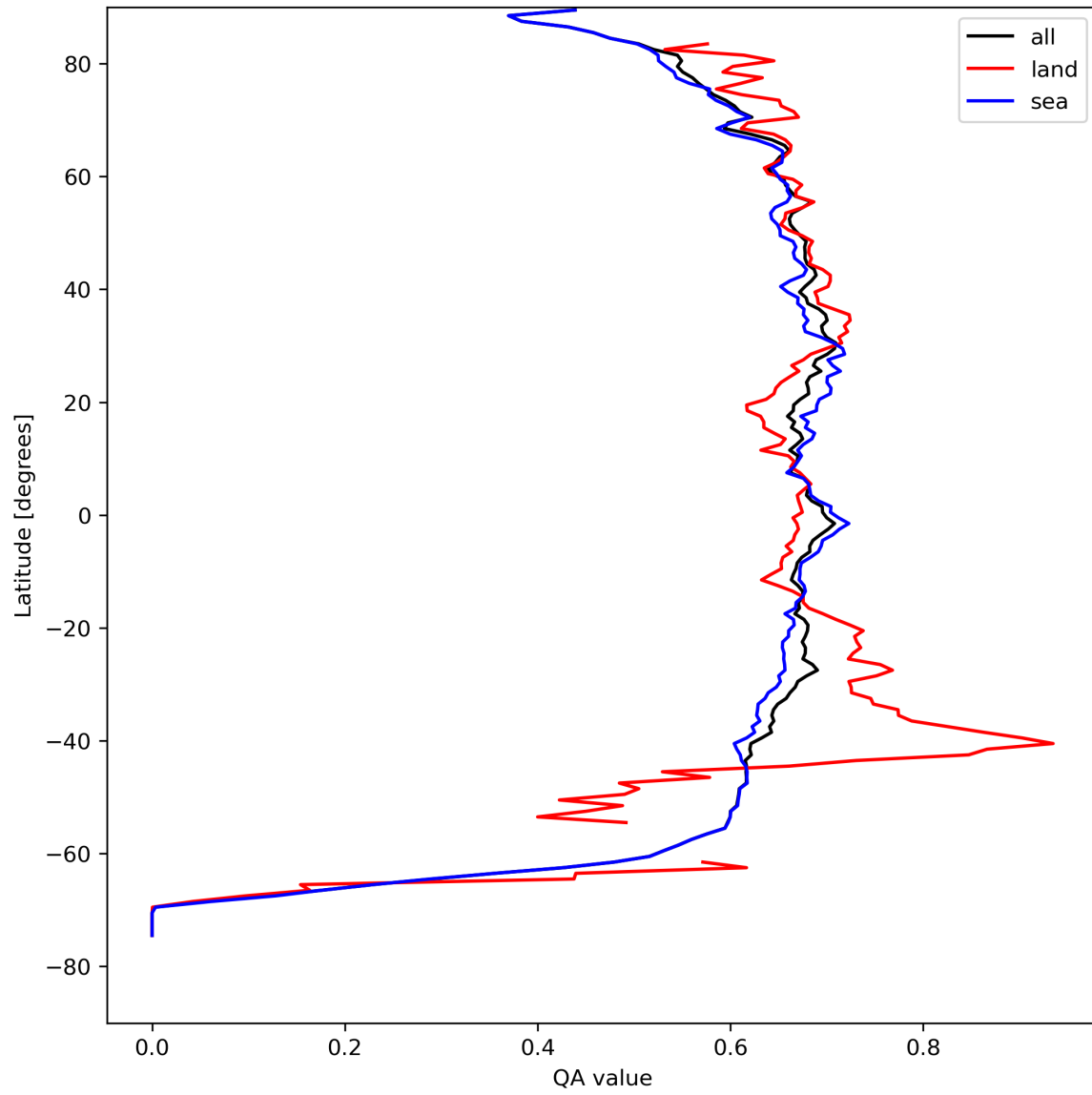
Figure 9: Zonal average of “QA value” for 2023-08-25 to 2023-08-27.
