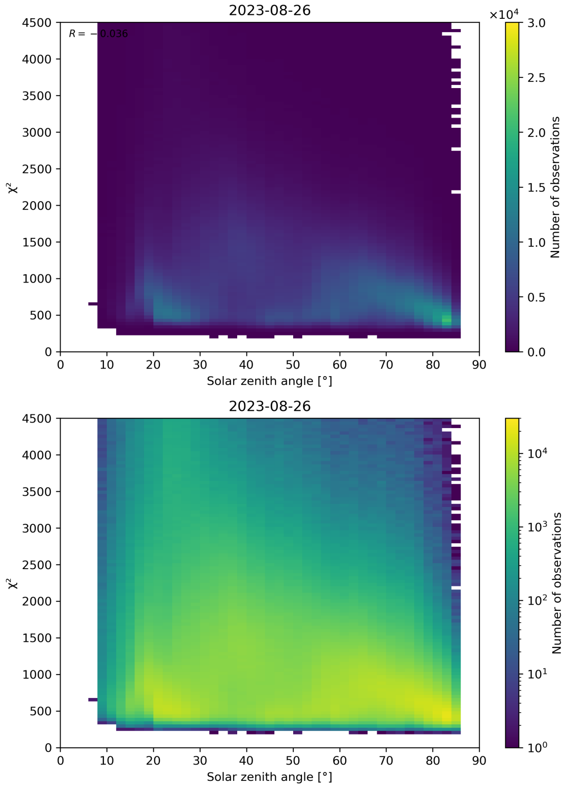
Figure 64: Scatter density plot of “Solar zenith angle” against “ \chi^2 ” for 2023-08-25 to 2023-08-27.
