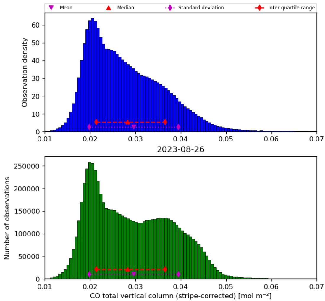
Figure 19: Histogram of “CO total vertical column (stripe-corrected)” for 2023-08-25 to 2023-08-27
