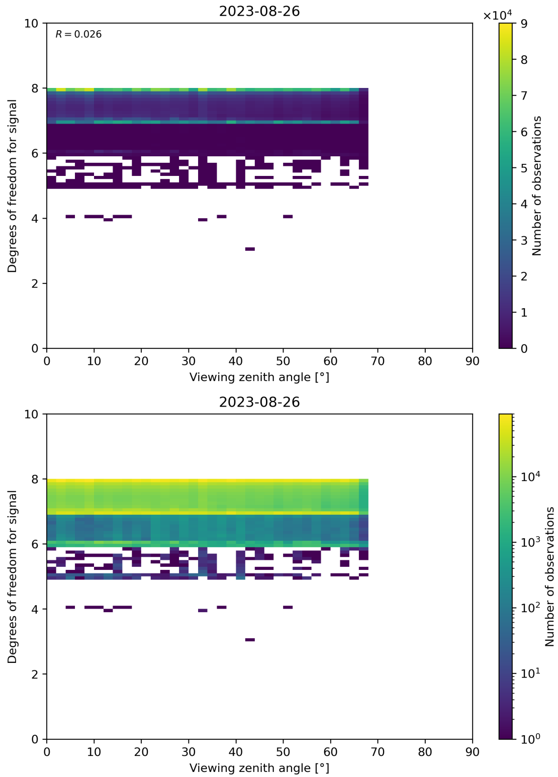
Figure 73: Scatter density plot of “Viewing zenith angle” against “Degrees of freedom for signal” for 2023-08-25 to 2023-08-27.
