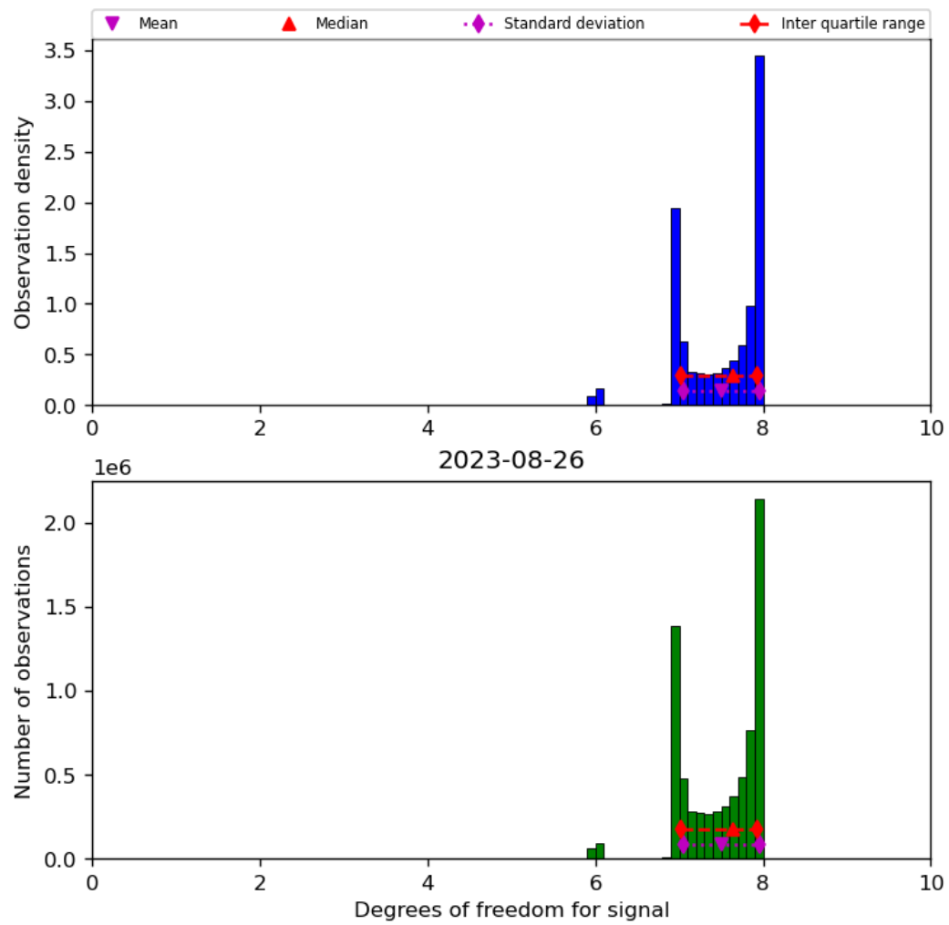
Figure 23: Histogram of “Degrees of freedom for signal” for 2023-08-25 to 2023-08-27
