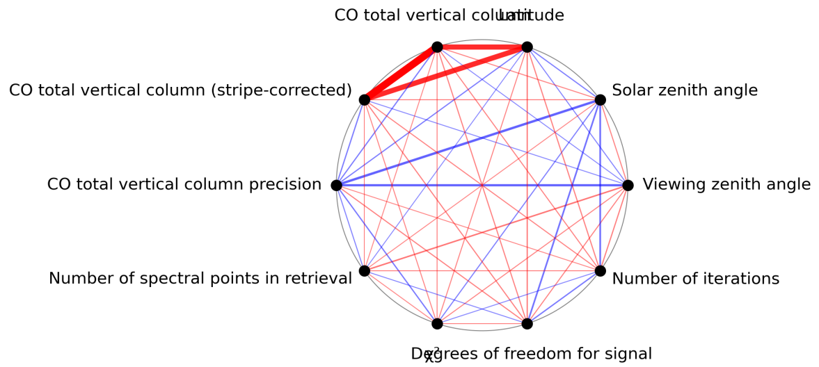
Figure 1: Map of correlation graph for 2023-08-25 to 2023-08-27.
