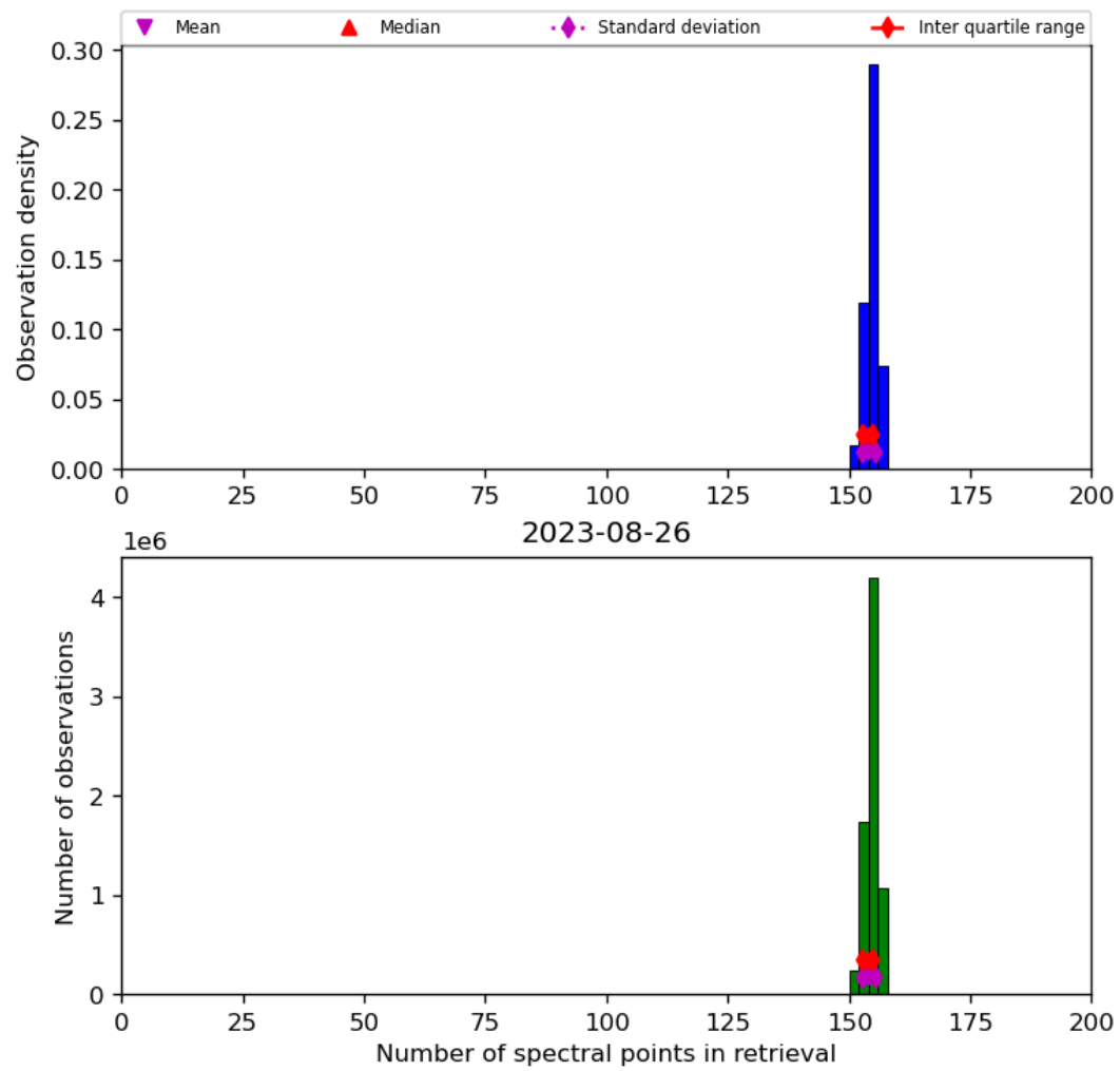
Figure 21: Histogram of “Number of spectral points in retrieval” for 2023-08-25 to 2023-08-27
