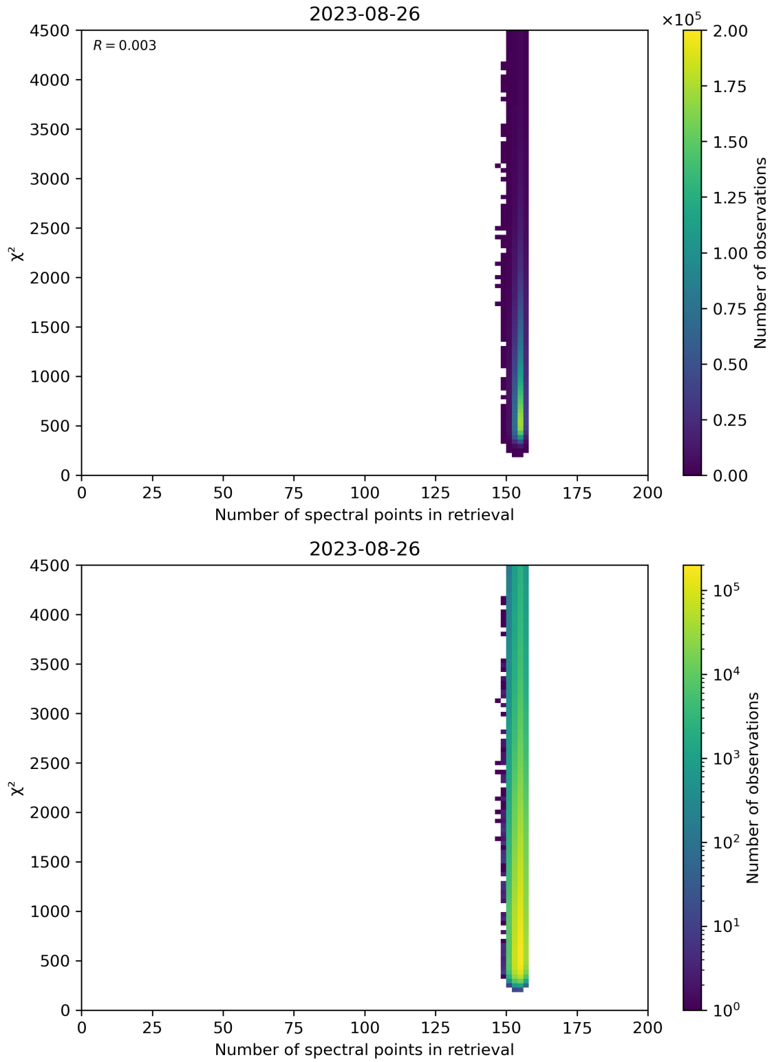
Figure 58: Scatter density plot of “Number of spectral points in retrieval” against “ \chi^2 ” for 2023-08-25 to 2023-08-27.
