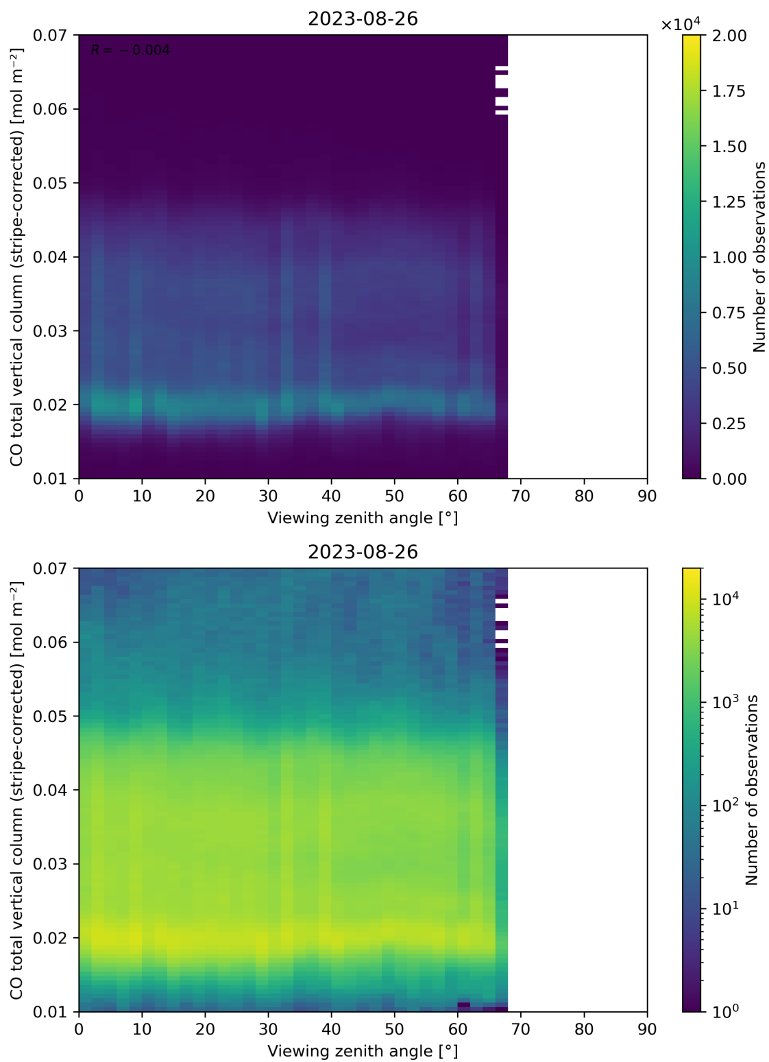
Figure 70: Scatter density plot of “Viewing zenith angle” against “CO total vertical column (stripe-corrected)” for 2023-08-25 to 2023-08-27.
