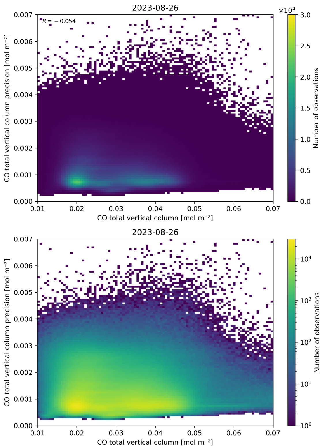
Figure 34: Scatter density plot of “CO total vertical column” against “CO total vertical column precision” for 2023-08-25 to 2023-08-27.
