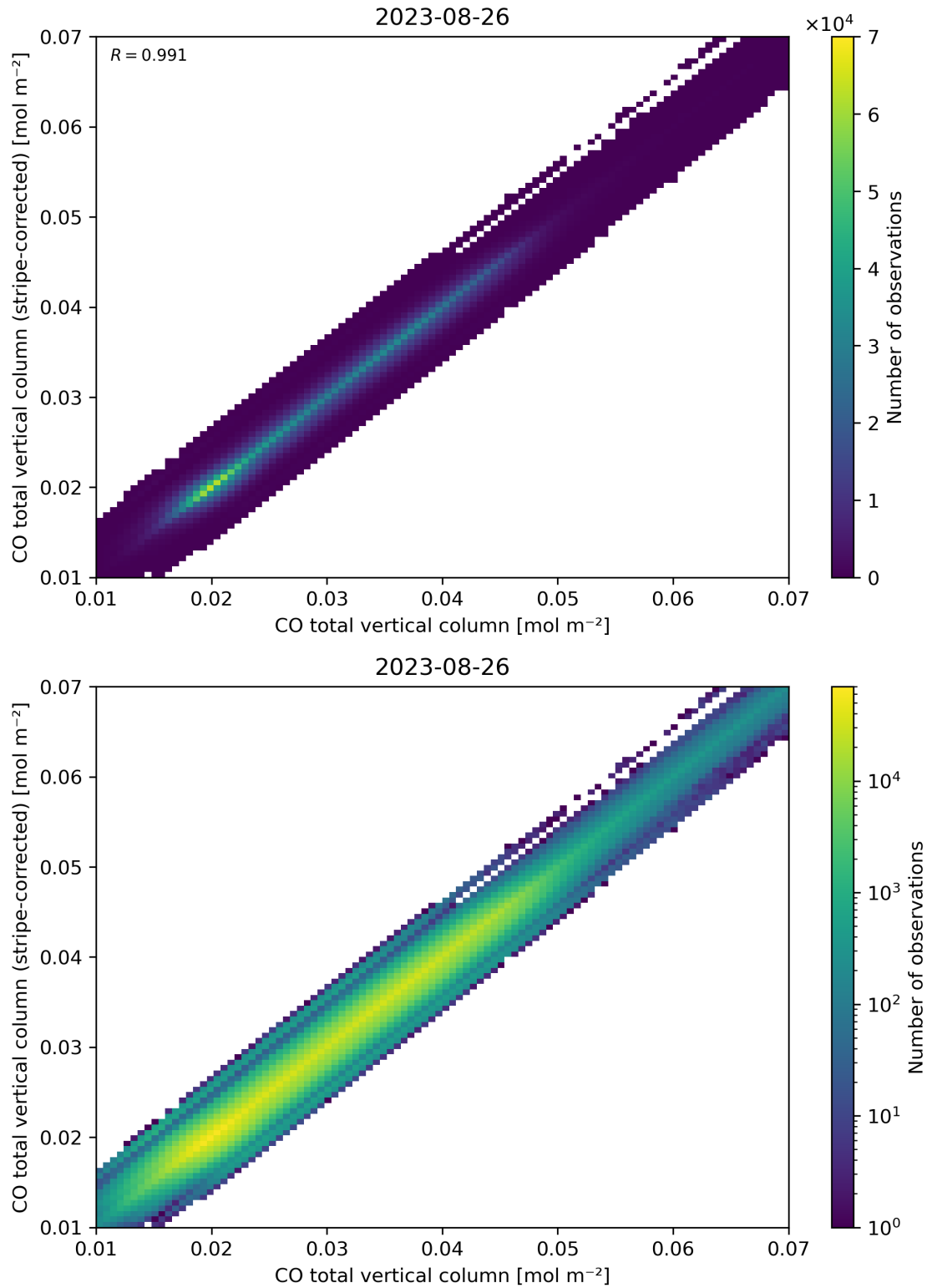
Figure 33: Scatter density plot of “CO total vertical column” against “CO total vertical column (stripe-corrected)” for 2023-08-25 to 2023-08-27.
