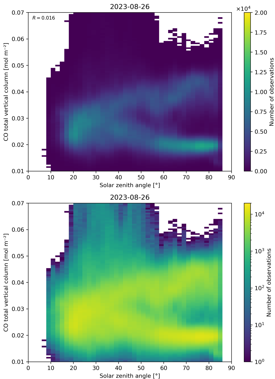
Figure 61: Scatter density plot of “Solar zenith angle” against “CO total vertical column” for 2023-08-25 to 2023-08-27.
