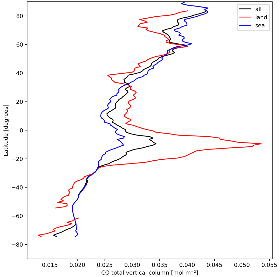
Figure 10: Zonal average of “CO total vertical column” for 2023-08-25 to 2023-08-27.
