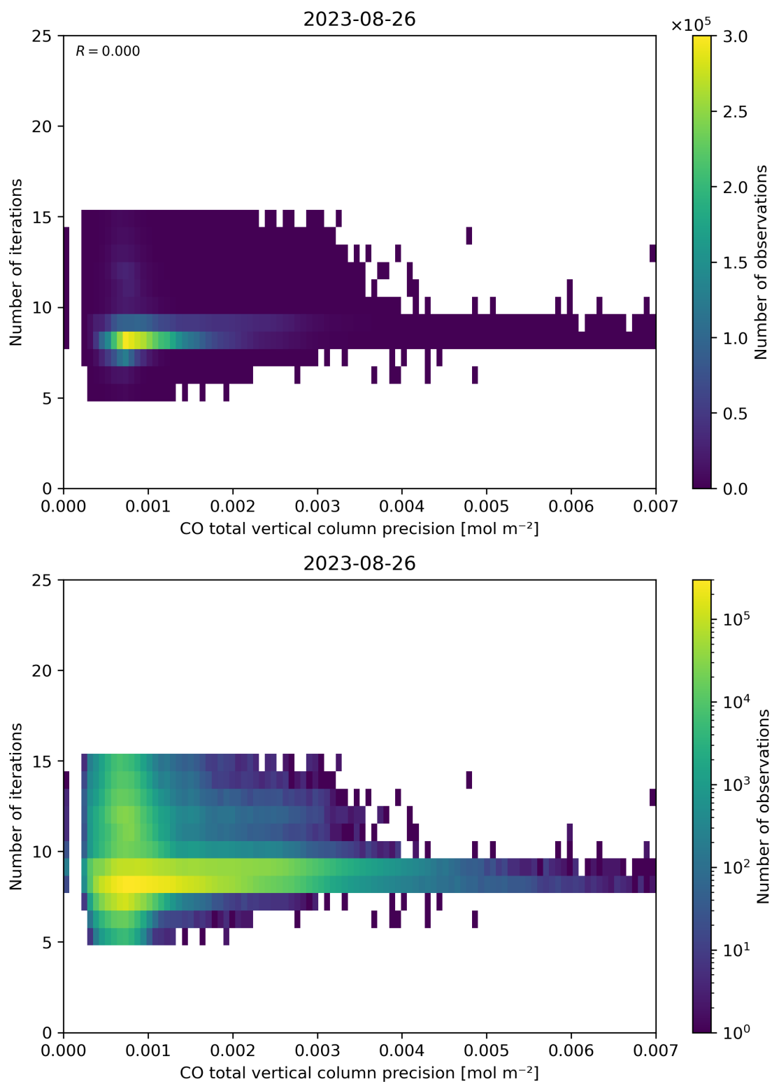
Figure 46: Scatter density plot of “CO total vertical column precision” against “Number of iterations” for 2023-08-25 to 2023-08-27.
