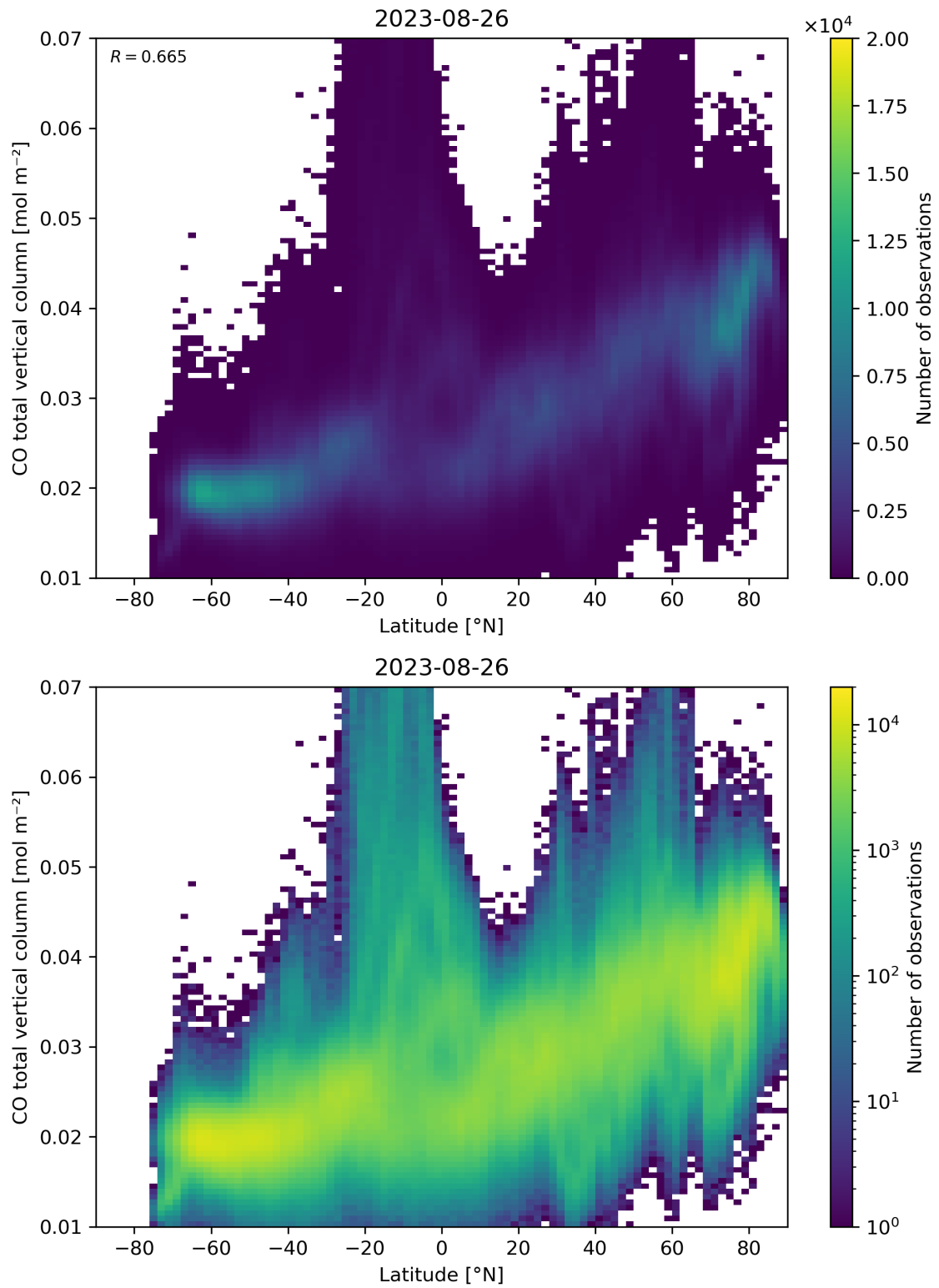
Figure 51: Scatter density plot of “Latitude” against “CO total vertical column” for 2023-08-25 to 2023-08-27.
