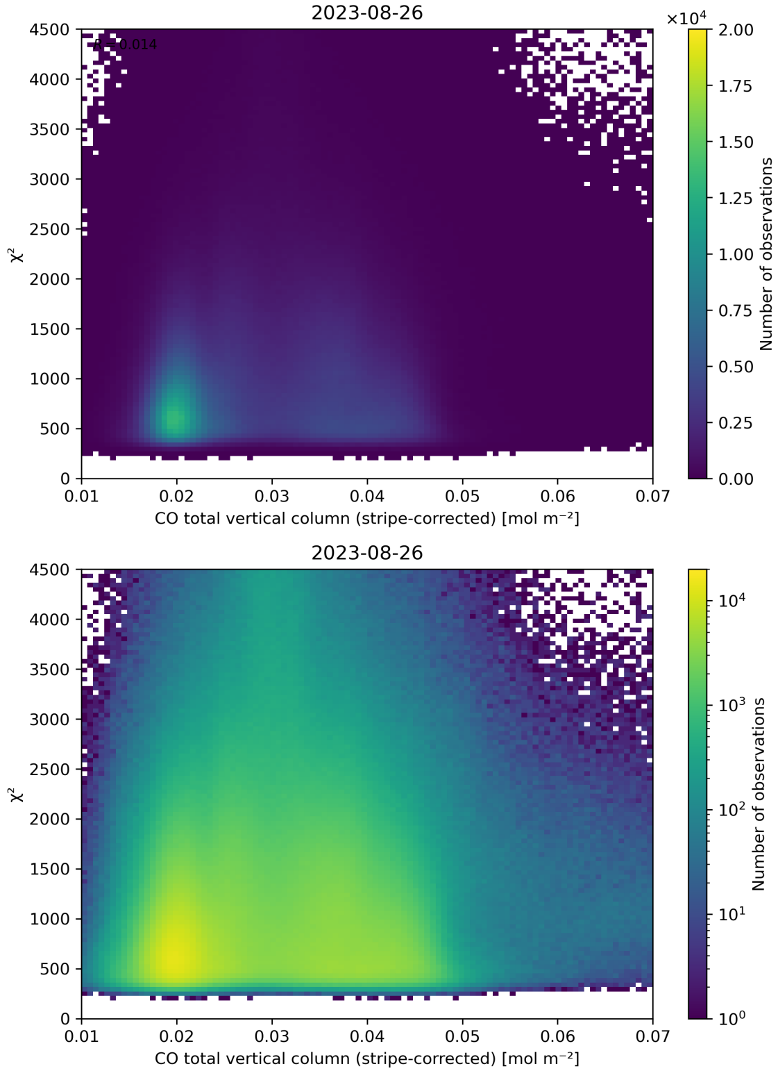
Figure 37: Scatter density plot of “CO total vertical column (stripe-corrected)” against “ \chi^2 ” for 2023-08-25 to 2023-08-27.
