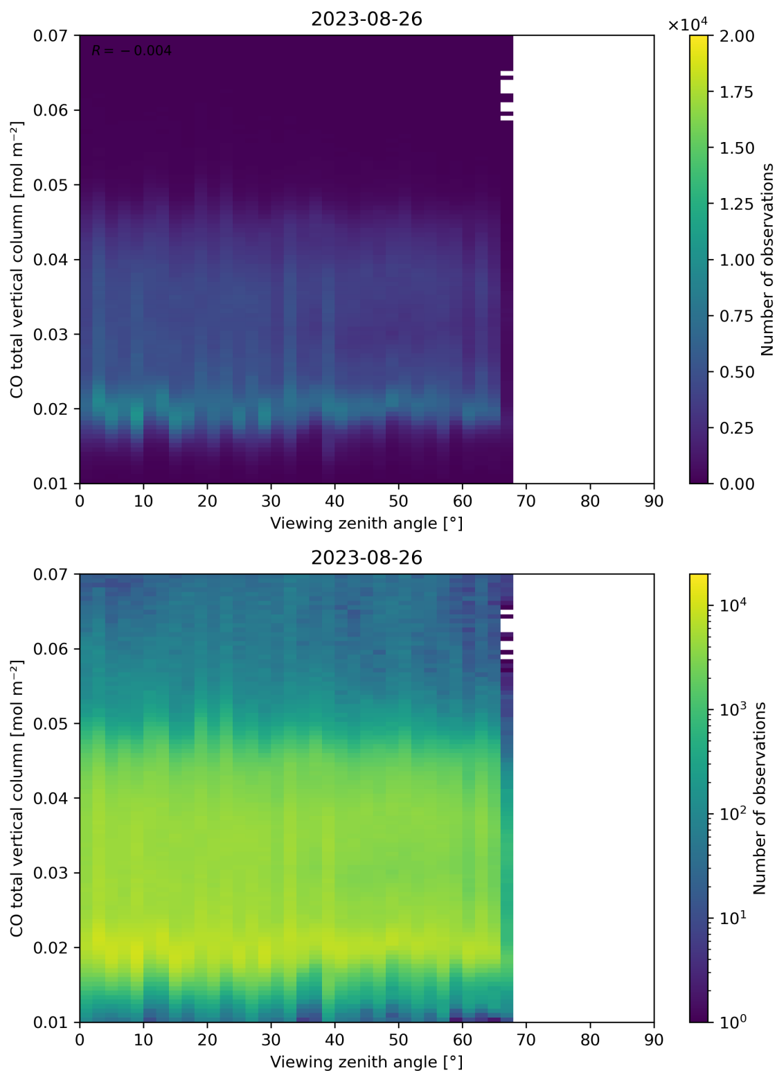
Figure 69: Scatter density plot of “Viewing zenith angle” against “CO total vertical column” for 2023-08-25 to 2023-08-27.
