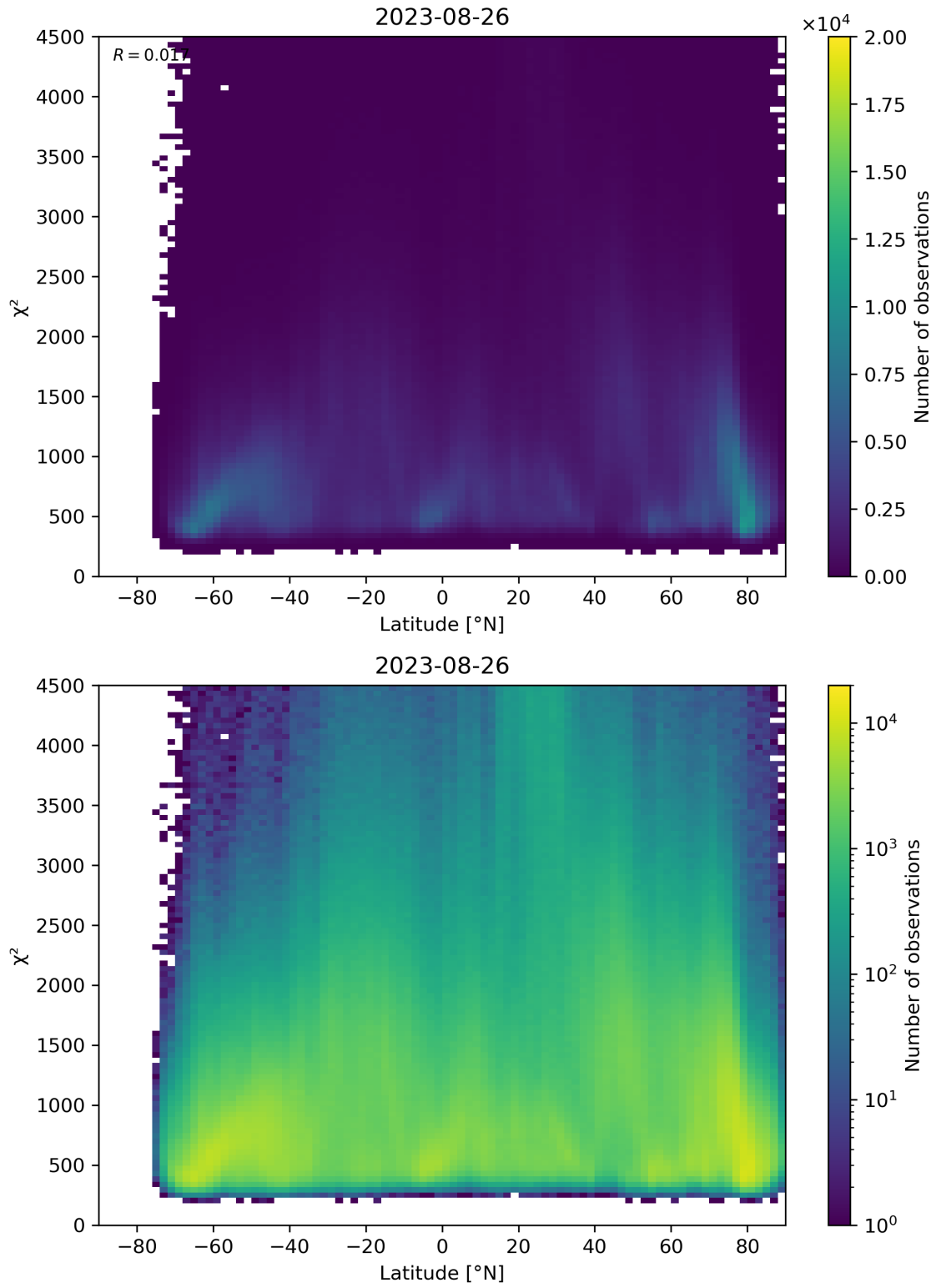
Figure 54: Scatter density plot of “Latitude” against “ \chi^2 ” for 2023-08-25 to 2023-08-27.
