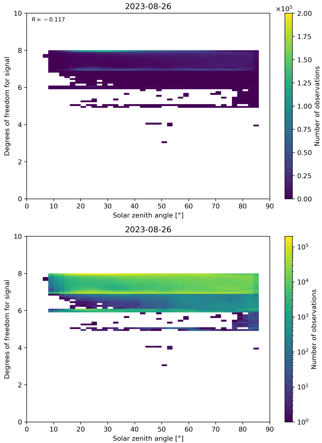
Figure 65: Scatter density plot of “Solar zenith angle” against “Degrees of freedom for signal” for 2023-08-25 to 2023-08-27.
