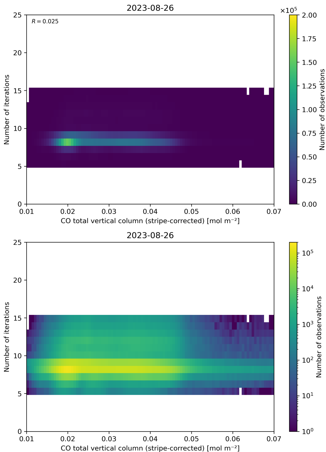
Figure 39: Scatter density plot of “CO total vertical column (stripe-corrected)” against “Number of iterations” for 2023-08-25 to 2023-08-27.
