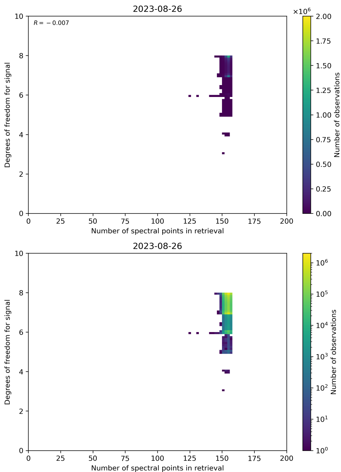
Figure 59: Scatter density plot of “Number of spectral points in retrieval” against “Degrees of freedom for signal” for 2023-08-25 to 2023-08-27.
