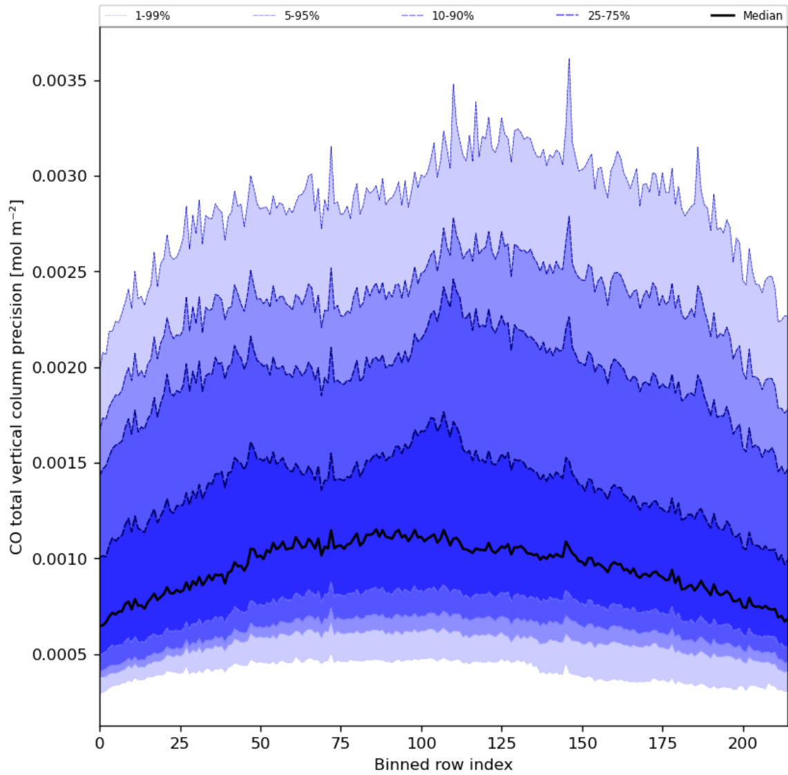
Figure 28: Along track statistics of “CO total vertical column precision” for 2023-08-25 to 2023-08-27
