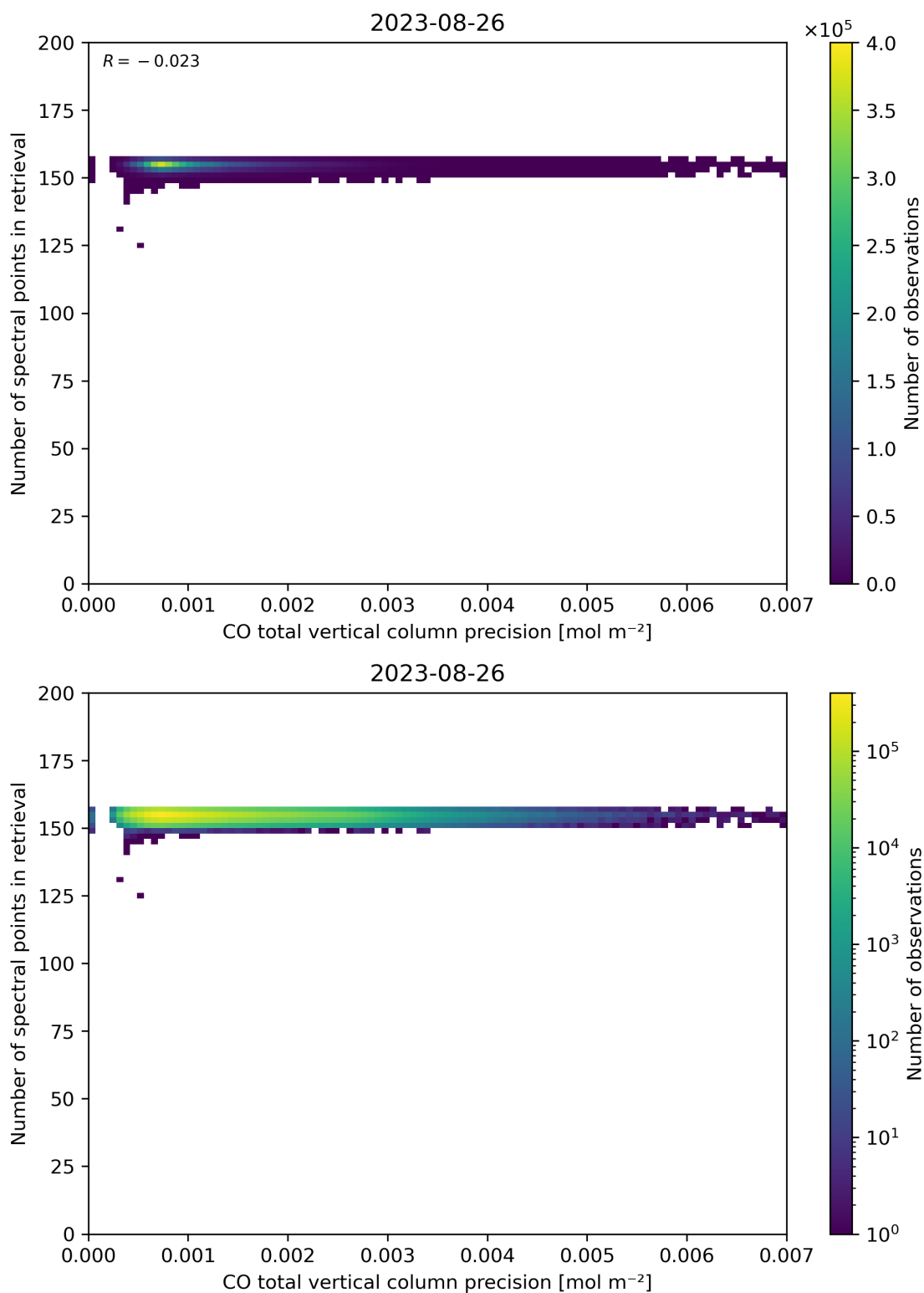
Figure 47: Scatter density plot of “CO total vertical column precision” against “Number of spectral points in retrieval” for 2023-08-25 to 2023-08-27.
