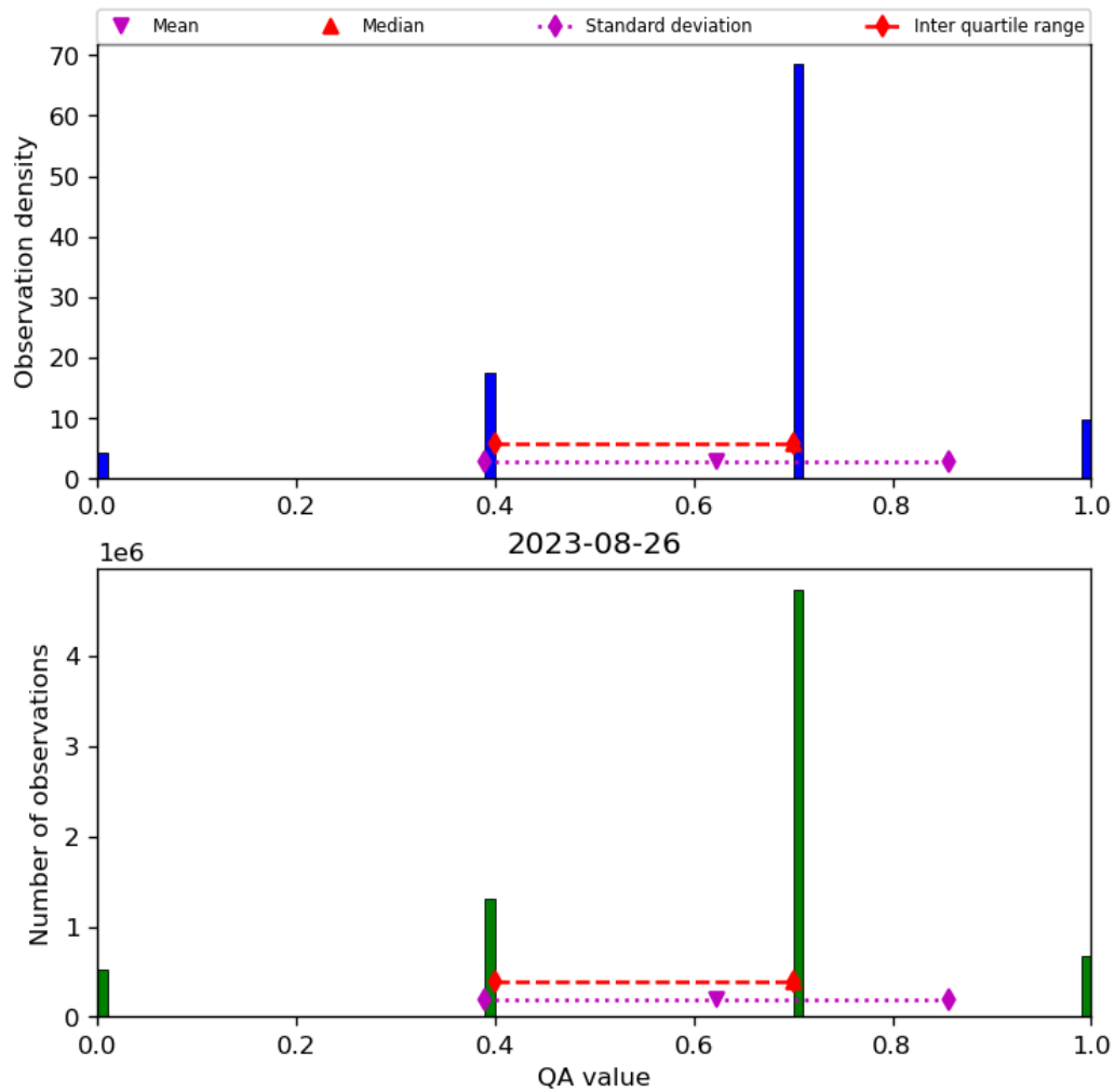
Figure 17: Histogram of “QA value” for 2023-08-25 to 2023-08-27
