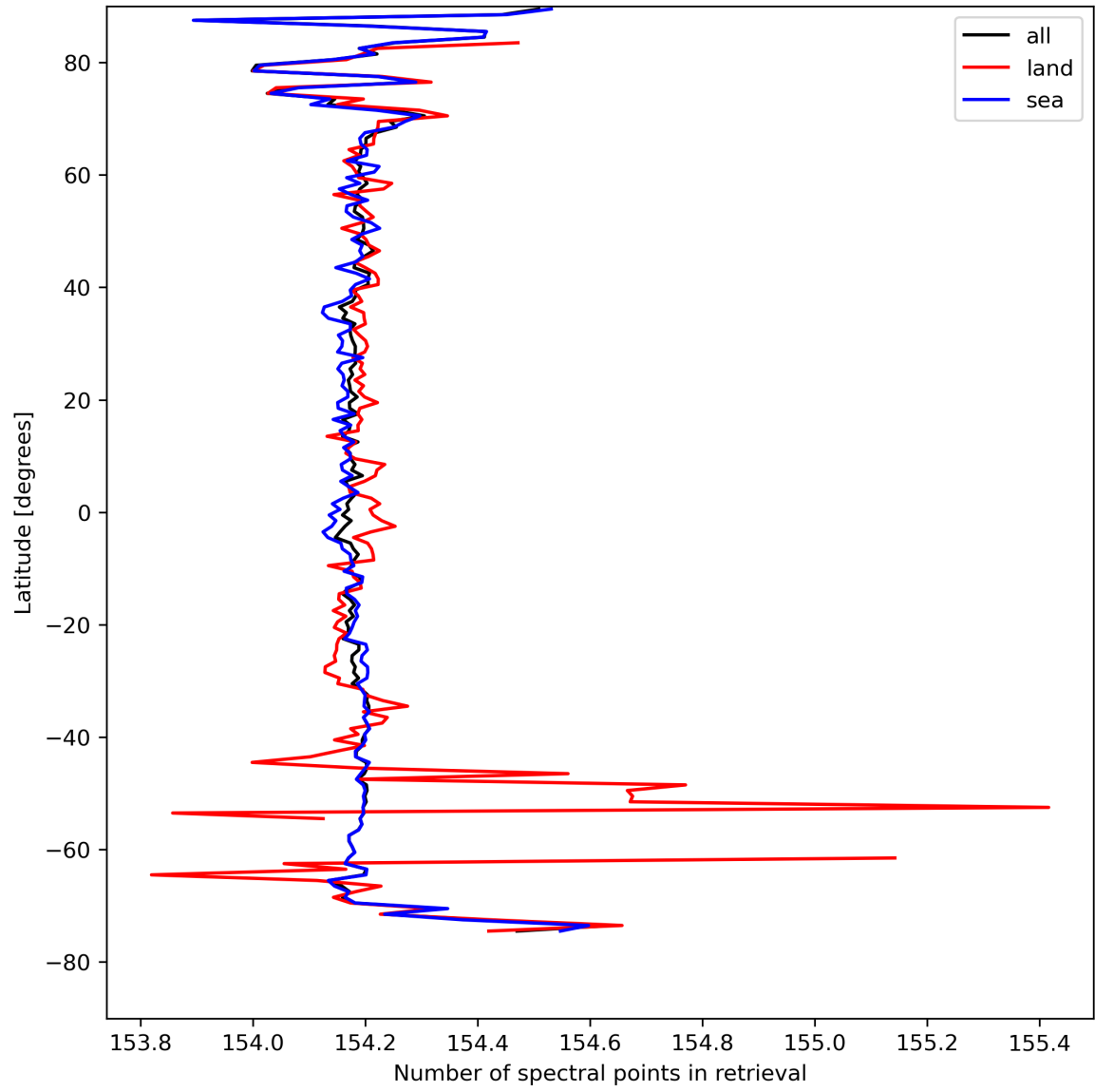
Figure 13: Zonal average of “Number of spectral points in retrieval” for 2023-08-25 to 2023-08-27.
