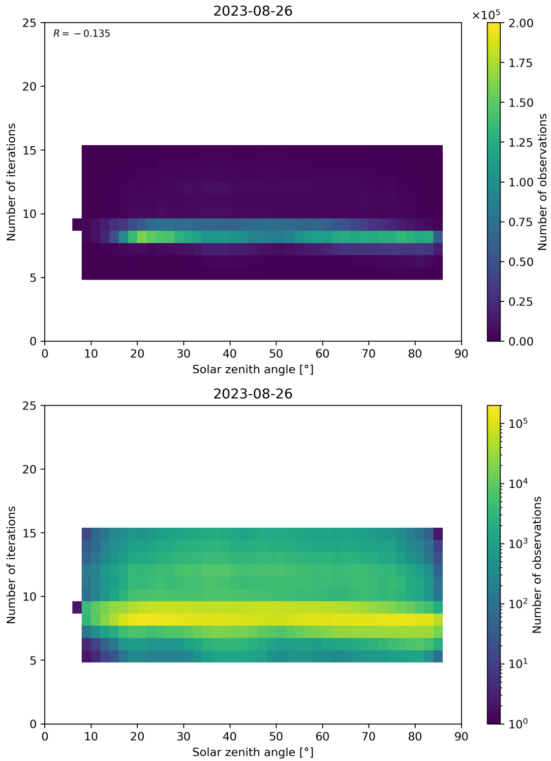
Figure 67: Scatter density plot of “Solar zenith angle” against “Number of iterations” for 2023-08-25 to 2023-08-27.
