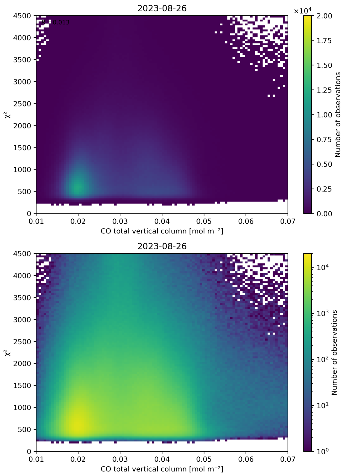
Figure 35: Scatter density plot of “CO total vertical column” against “ \chi^2 ” for 2023-08-25 to 2023-08-27.
