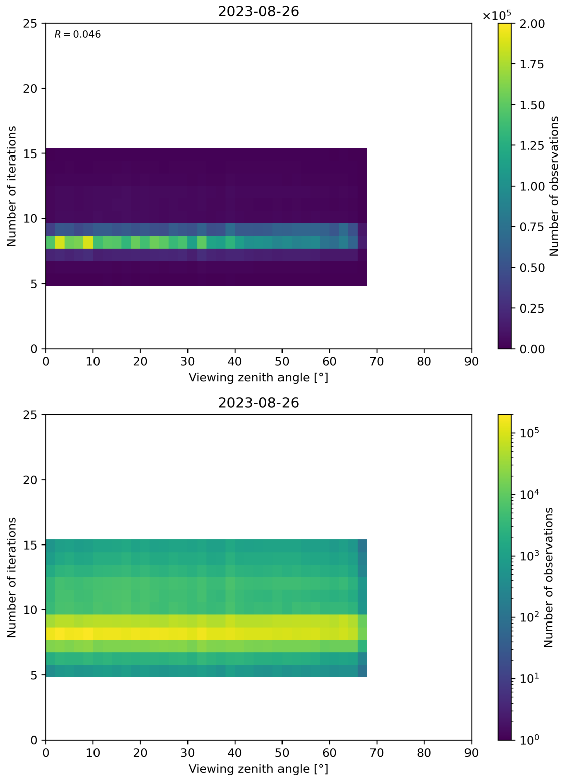
Figure 75: Scatter density plot of “Viewing zenith angle” against “Number of iterations” for 2023-08-25 to 2023-08-27.
