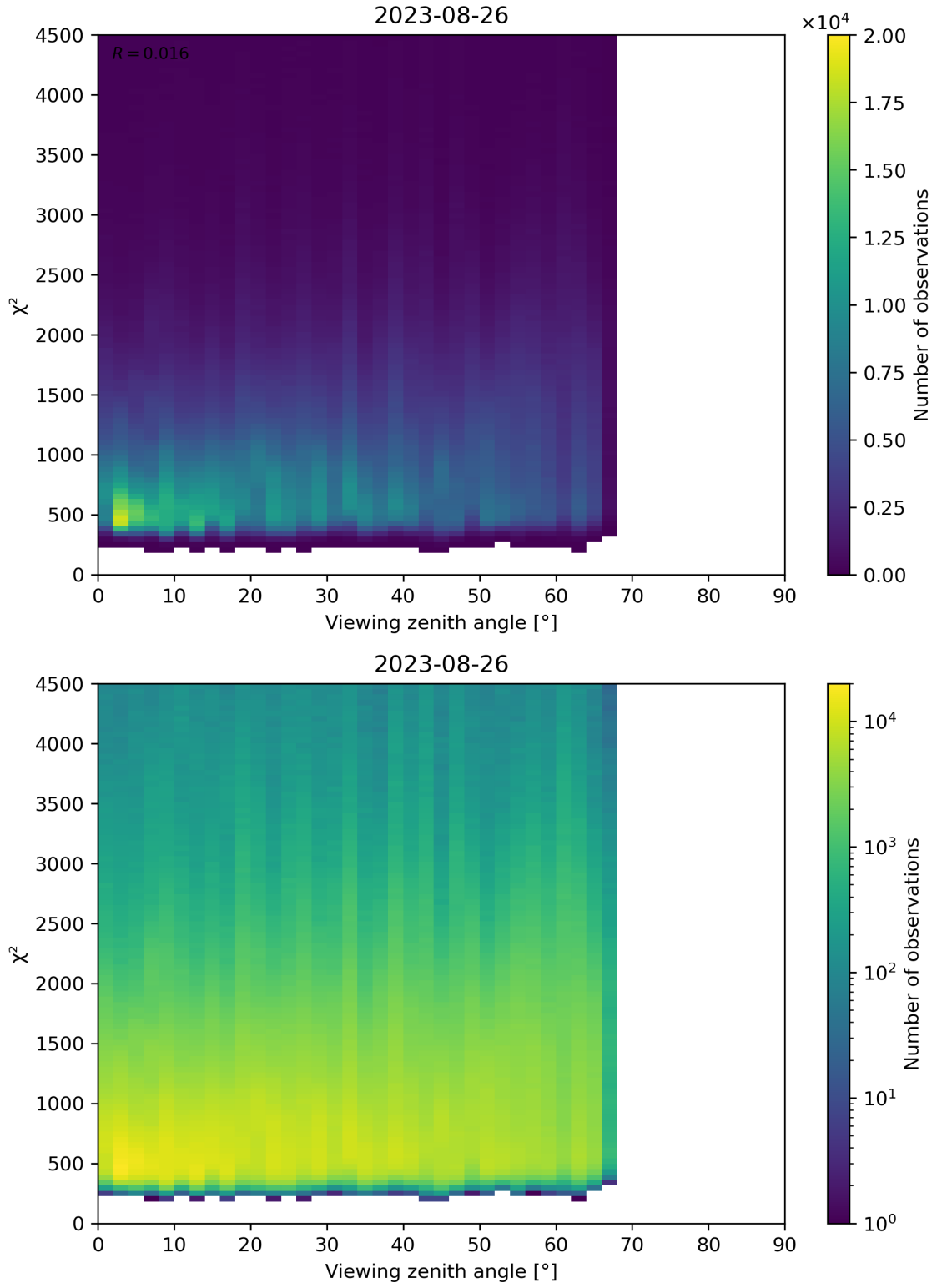
Figure 72: Scatter density plot of “Viewing zenith angle” against “ \chi^2 ” for 2023-08-25 to 2023-08-27.
