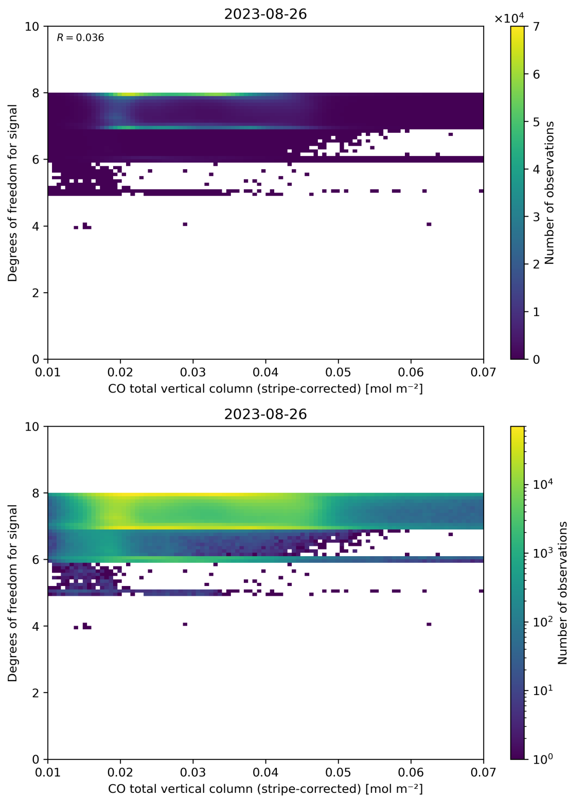
Figure 38: Scatter density plot of “CO total vertical column (stripe-corrected)” against “Degrees of freedom for signal” for 2023-08-25 to 2023-08-27.
