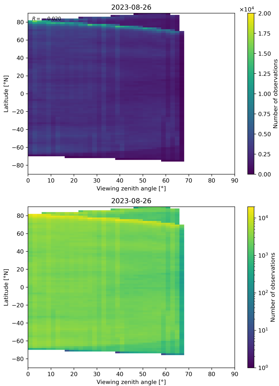
Figure 74: Scatter density plot of “Viewing zenith angle” against “Latitude” for 2023-08-25 to 2023-08-27.
