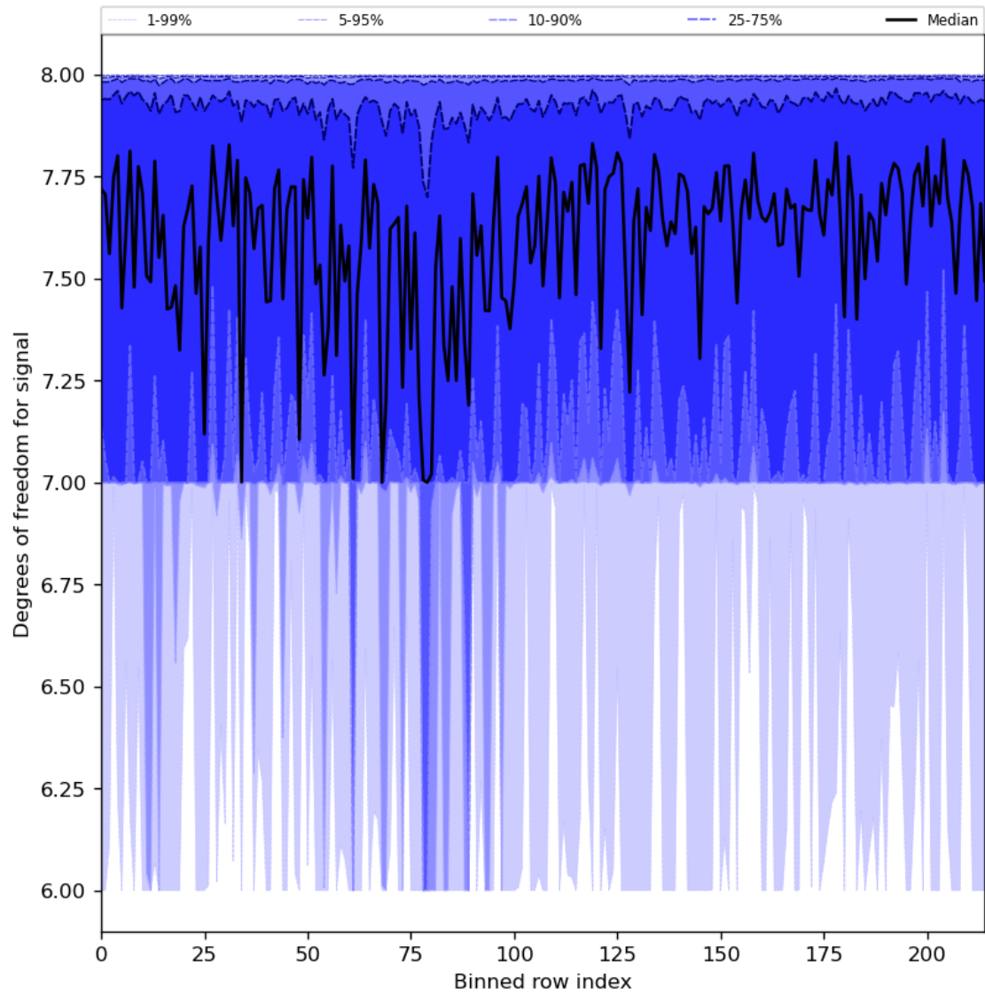
Figure 31: Along track statistics of “Degrees of freedom for signal” for 2023-08-25 to 2023-08-27
