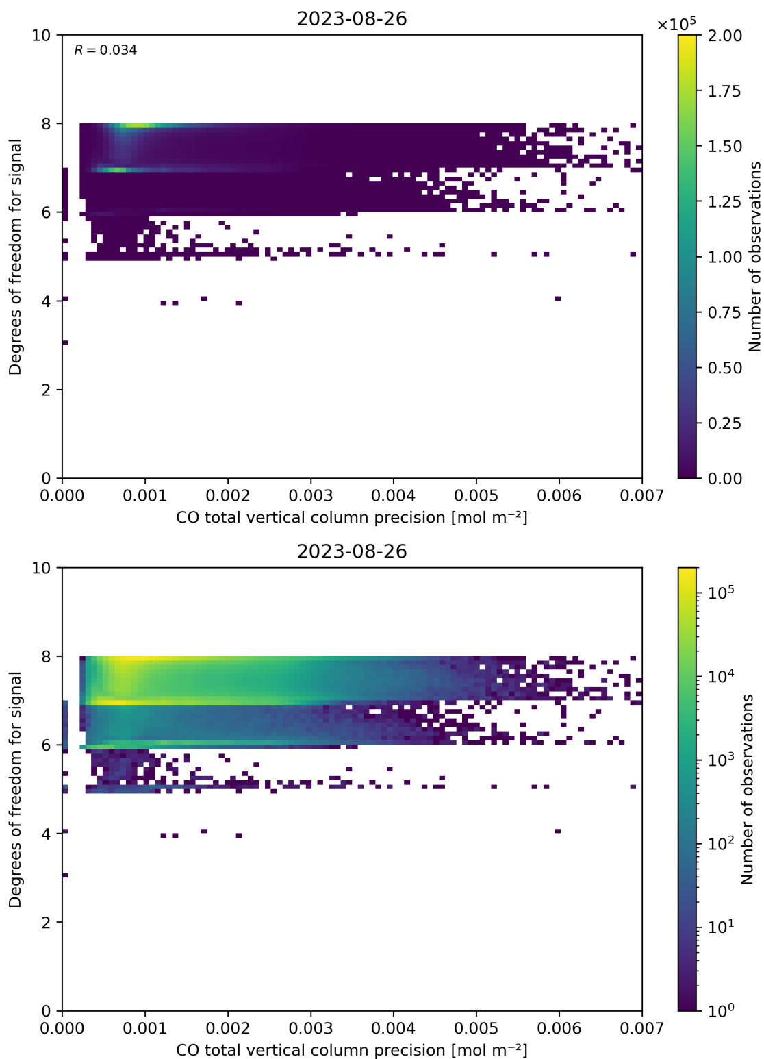
Figure 45: Scatter density plot of “CO total vertical column precision” against “Degrees of freedom for signal” for 2023-08-25 to 2023-08-27.
