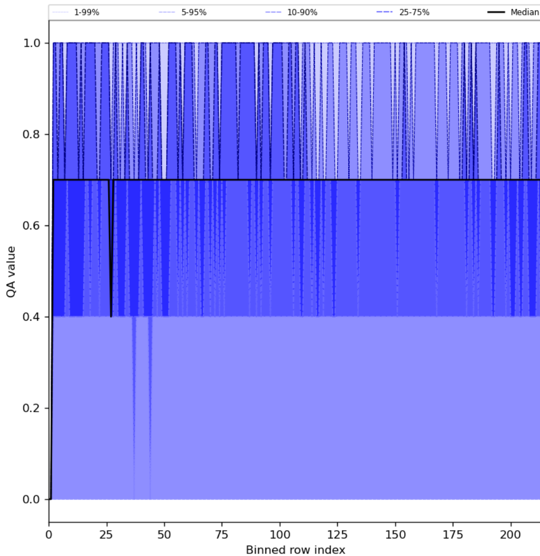
Figure 25: Along track statistics of “QA value” for 2023-08-25 to 2023-08-27
