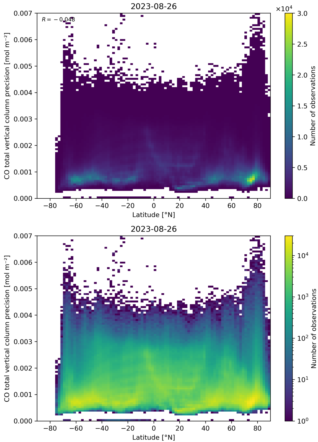
Figure 53: Scatter density plot of “Latitude” against “CO total vertical column precision” for 2023-08-25 to 2023-08-27.
