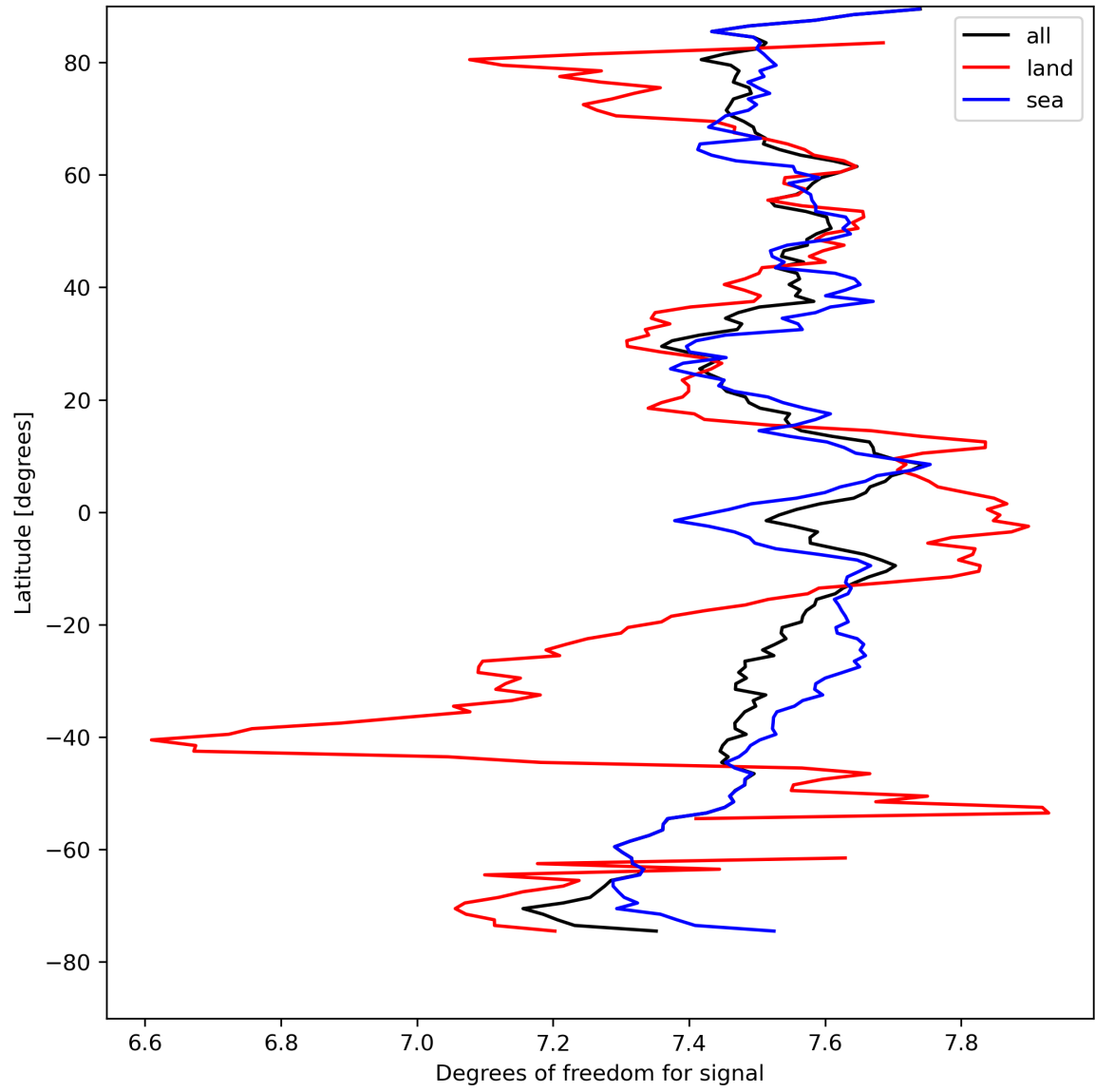
Figure 15: Zonal average of “Degrees of freedom for signal” for 2023-08-25 to 2023-08-27.
