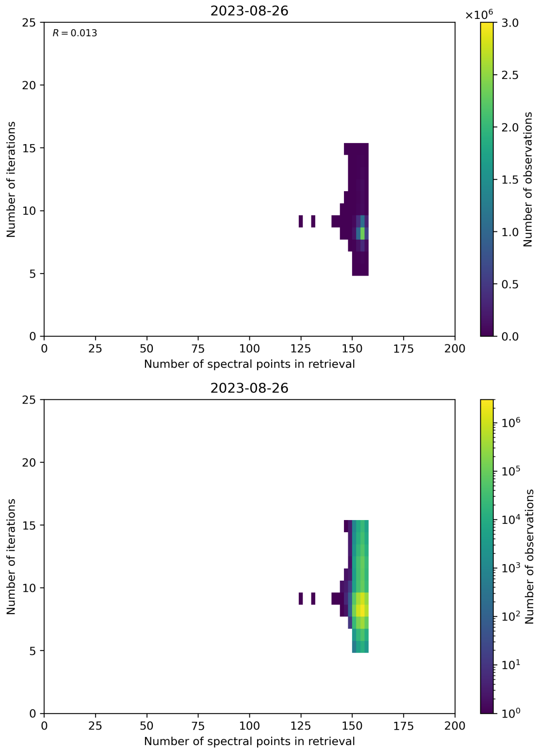
Figure 60: Scatter density plot of “Number of spectral points in retrieval” against “Number of iterations” for 2023-08-25 to 2023-08-27.
