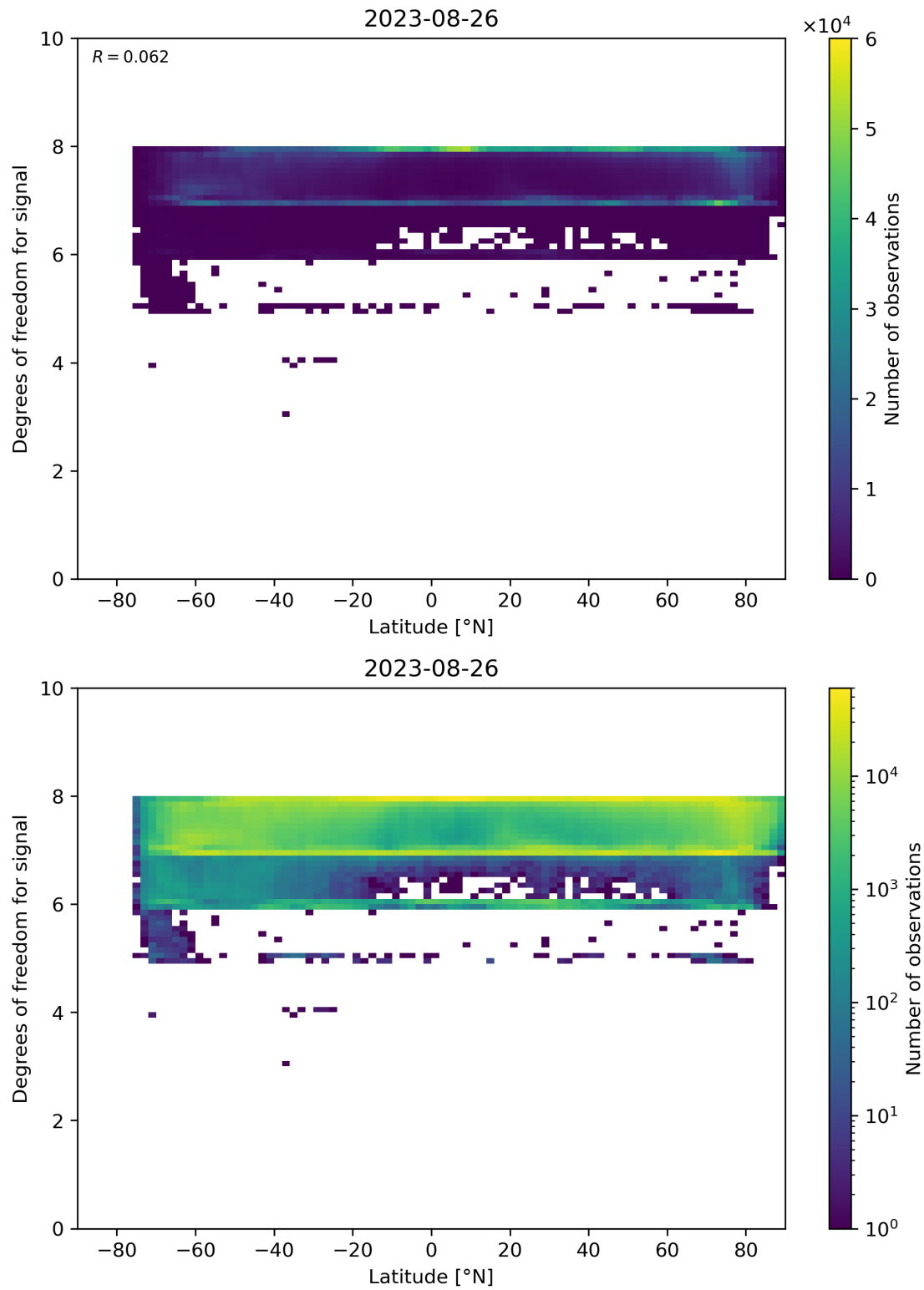
Figure 55: Scatter density plot of “Latitude” against “Degrees of freedom for signal” for 2023-08-25 to 2023-08-27.
