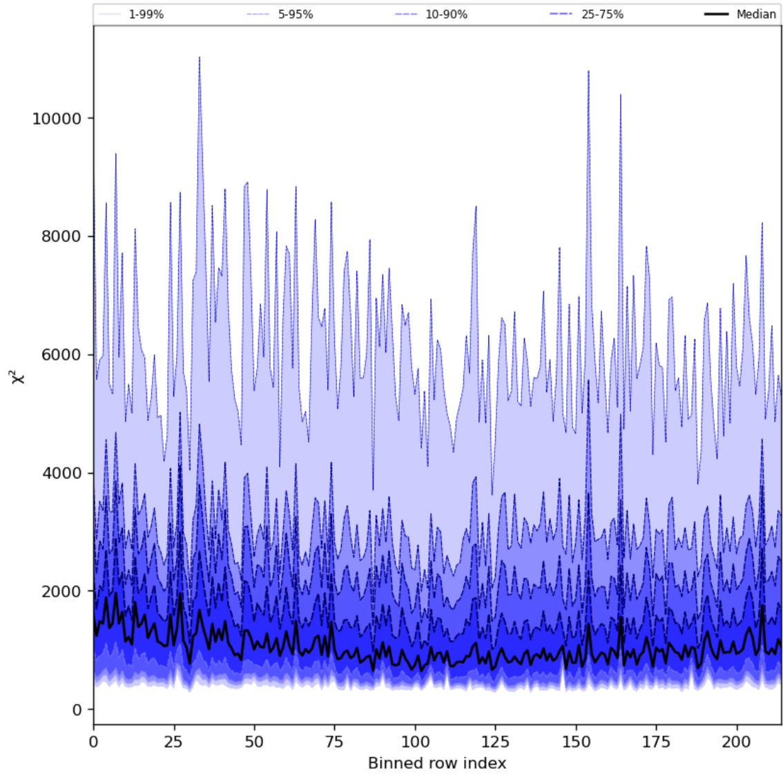
Figure 30: Along track statistics of “ \chi^2 ” for 2023-08-25 to 2023-08-27
