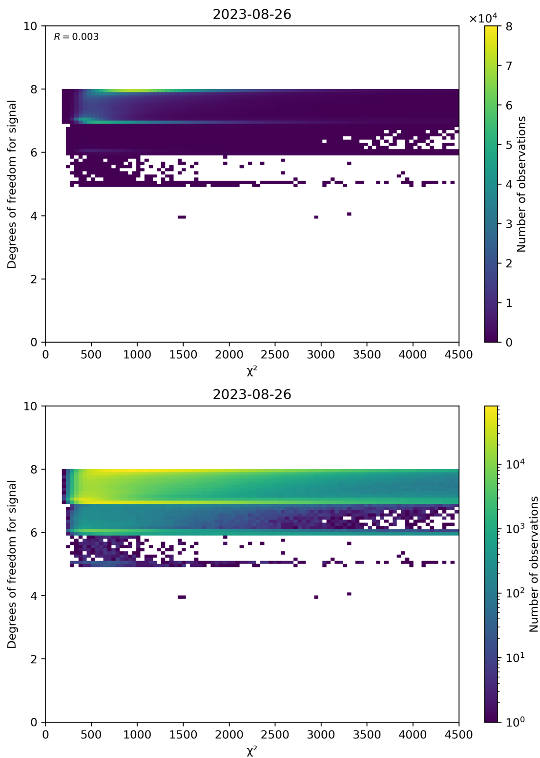
Figure 48: Scatter density plot of “ \chi^2 ” against “Degrees of freedom for signal” for 2023-08-25 to 2023-08-27.
