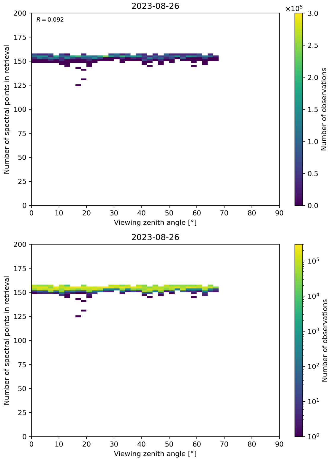
Figure 76: Scatter density plot of “Viewing zenith angle” against “Number of spectral points in retrieval” for 2023-08-25 to 2023-08-27.
