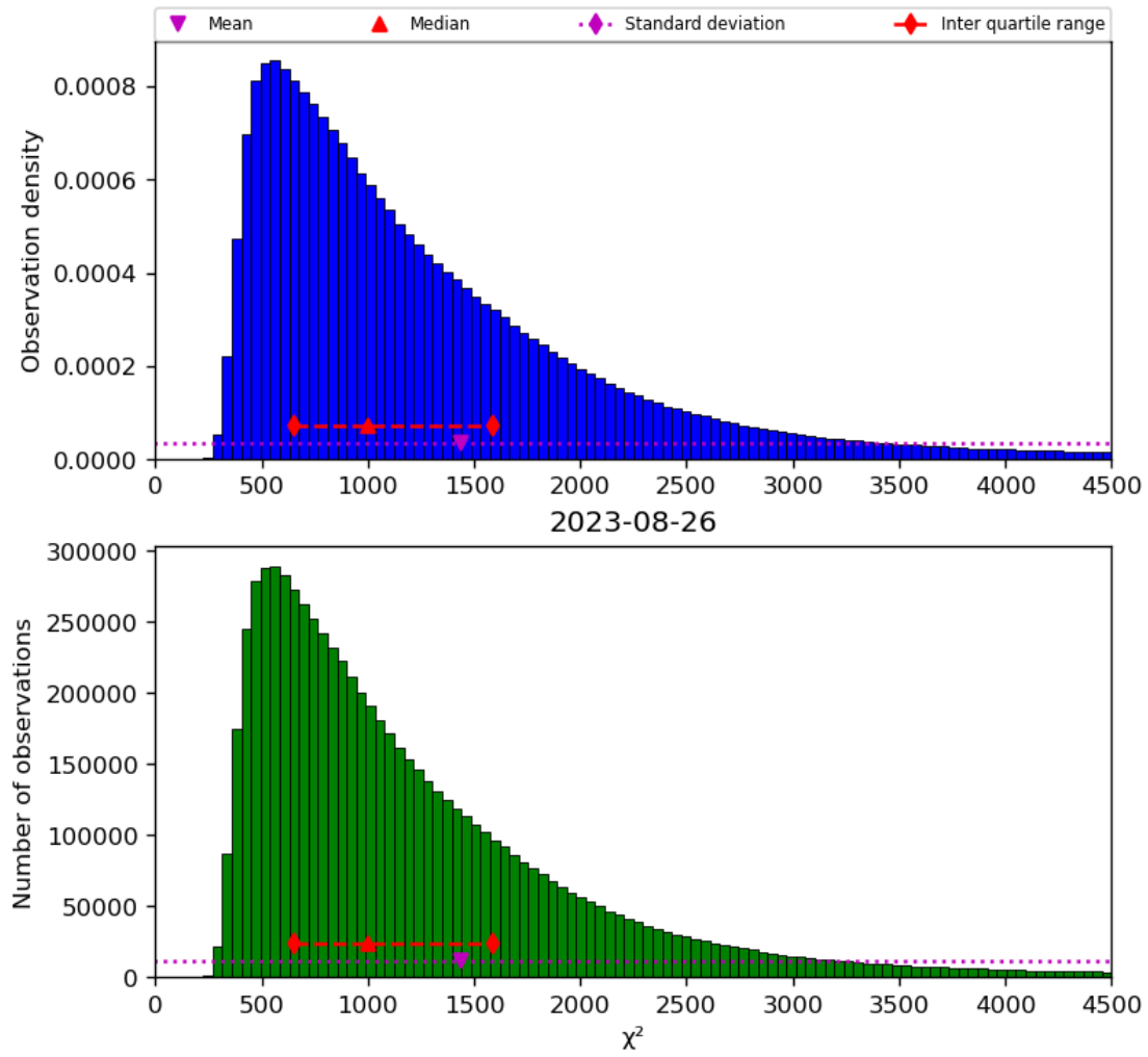
Figure 22: Histogram of " \chi^2 " for 2023-08-25 to 2023-08-27
