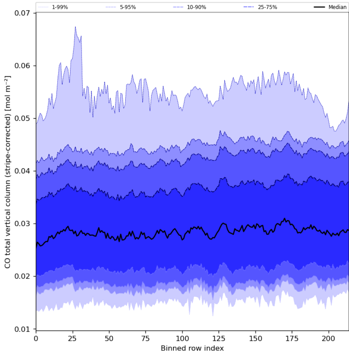
Figure 27: Along track statistics of “CO total vertical column (stripe-corrected)” for 2023-08-25 to 2023-08-27
