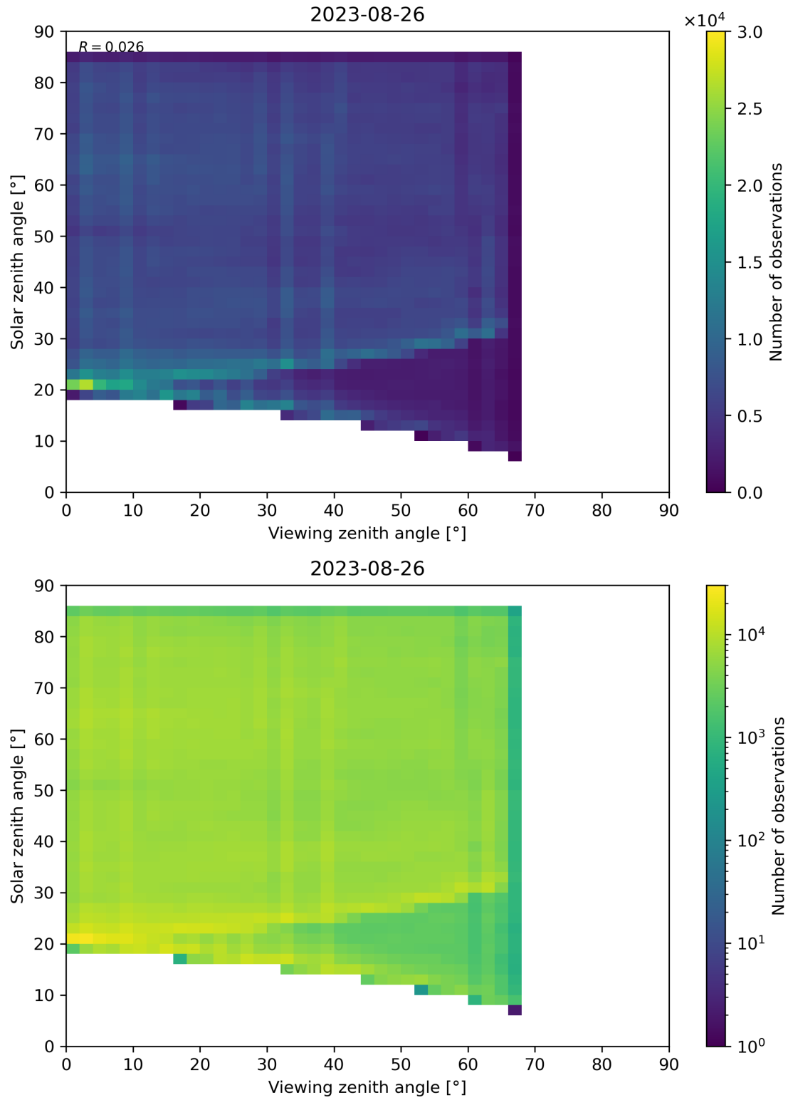
Figure 77: Scatter density plot of “Viewing zenith angle” against “Solar zenith angle” for 2023-08-25 to 2023-08-27.
