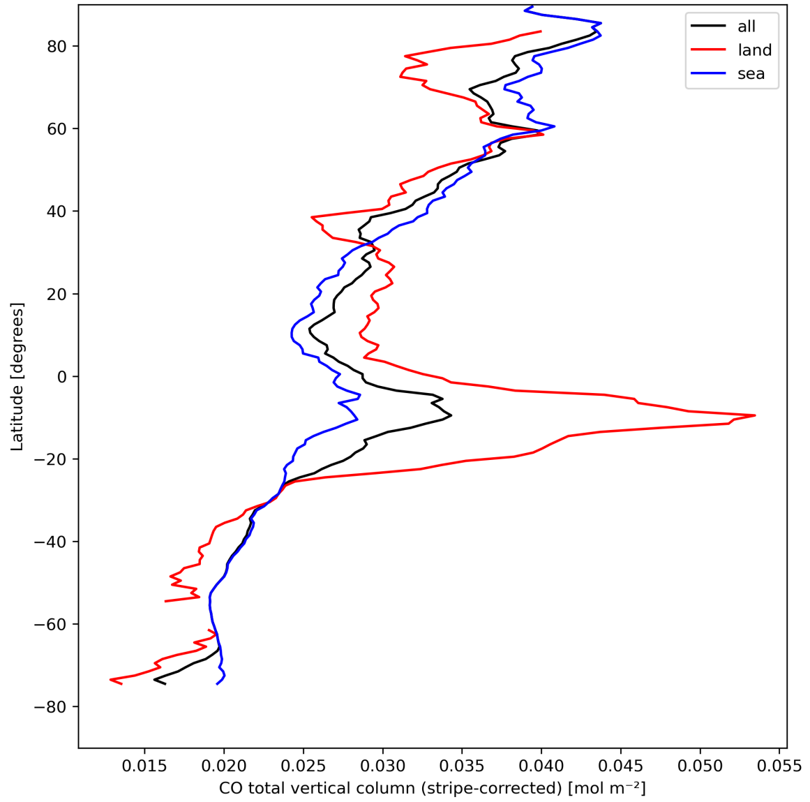
Figure 11: Zonal average of “CO total vertical column (stripe-corrected)” for 2023-08-25 to 2023-08-27.
