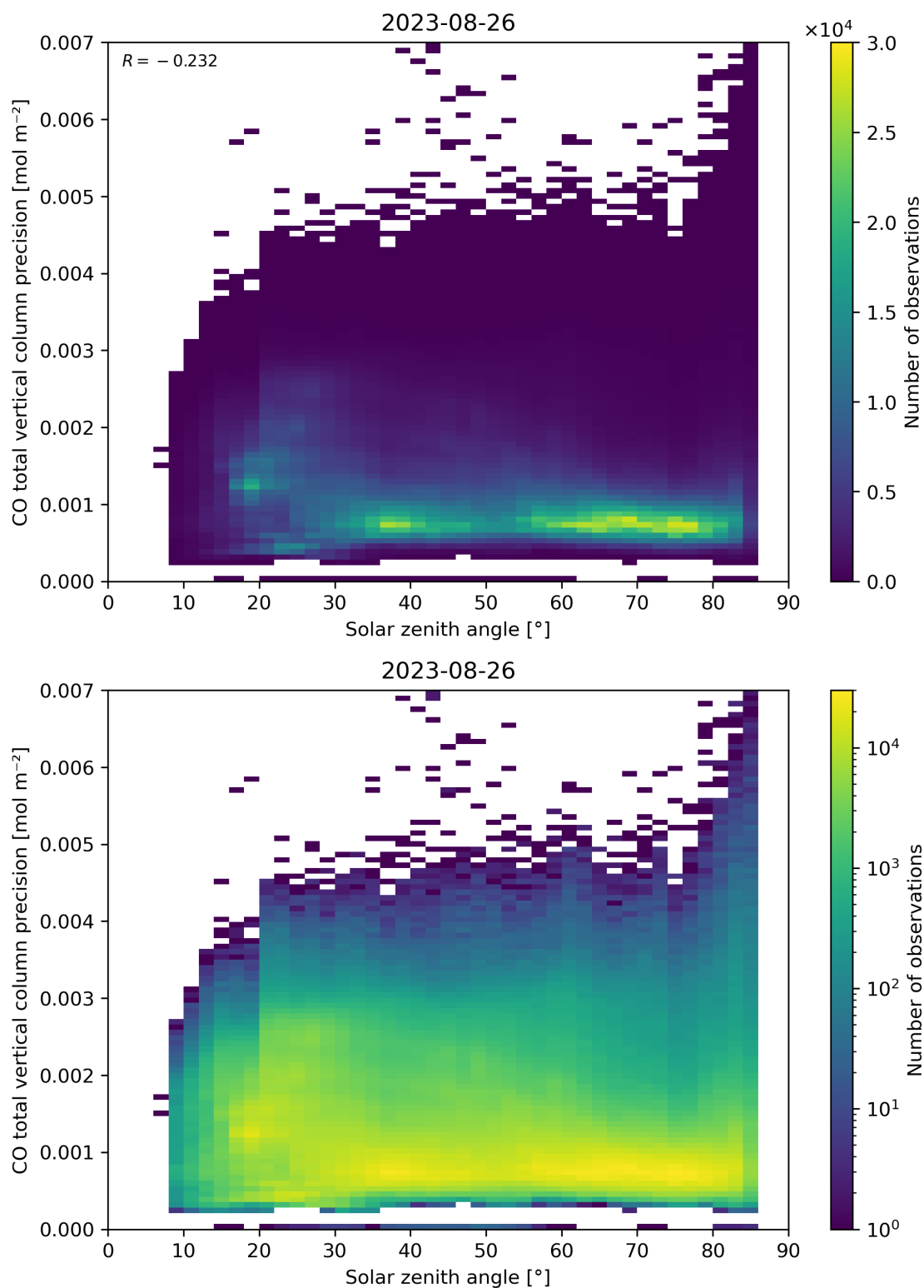
Figure 63: Scatter density plot of “Solar zenith angle” against “CO total vertical column precision” for 2023-08-25 to 2023-08-27.
