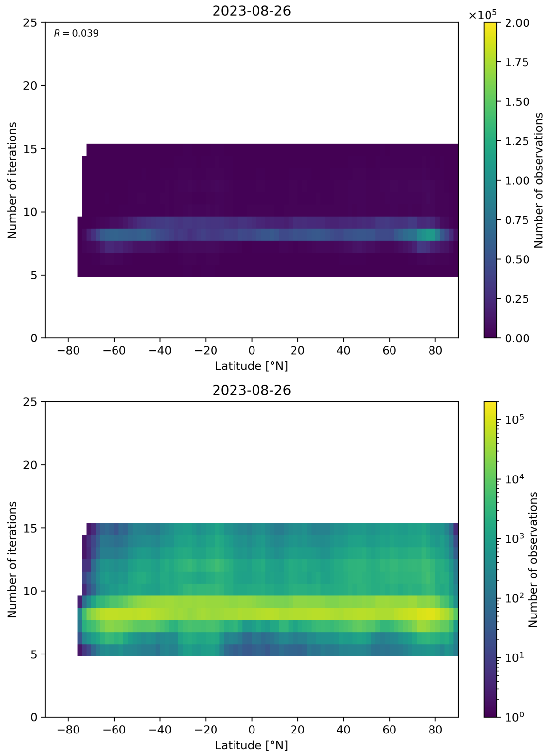
Figure 56: Scatter density plot of “Latitude” against “Number of iterations” for 2023-08-25 to 2023-08-27.
