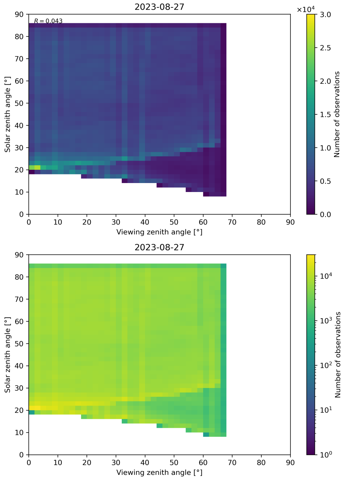
Figure 77: Scatter density plot of “Viewing zenith angle” against “Solar zenith angle” for 2023-08-26 to 2023-08-28.
