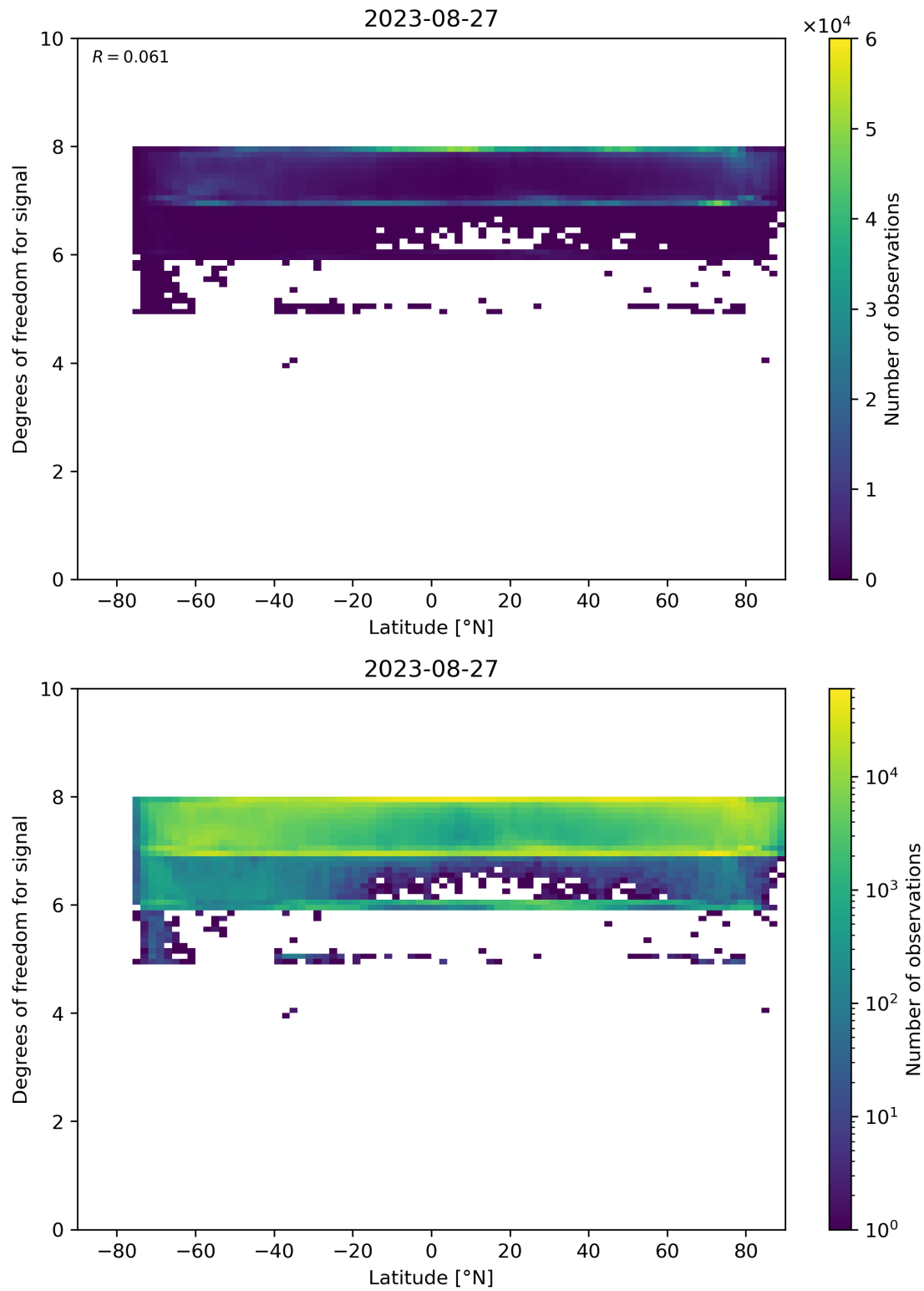
Figure 55: Scatter density plot of “Latitude” against “Degrees of freedom for signal” for 2023-08-26 to 2023-08-28.
