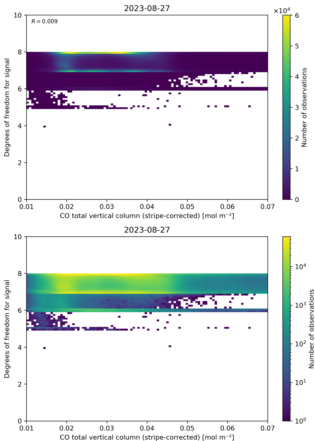
Figure 38: Scatter density plot of “CO total vertical column (stripe-corrected)” against “Degrees of freedom for signal” for 2023-08-26 to 2023-08-28.
