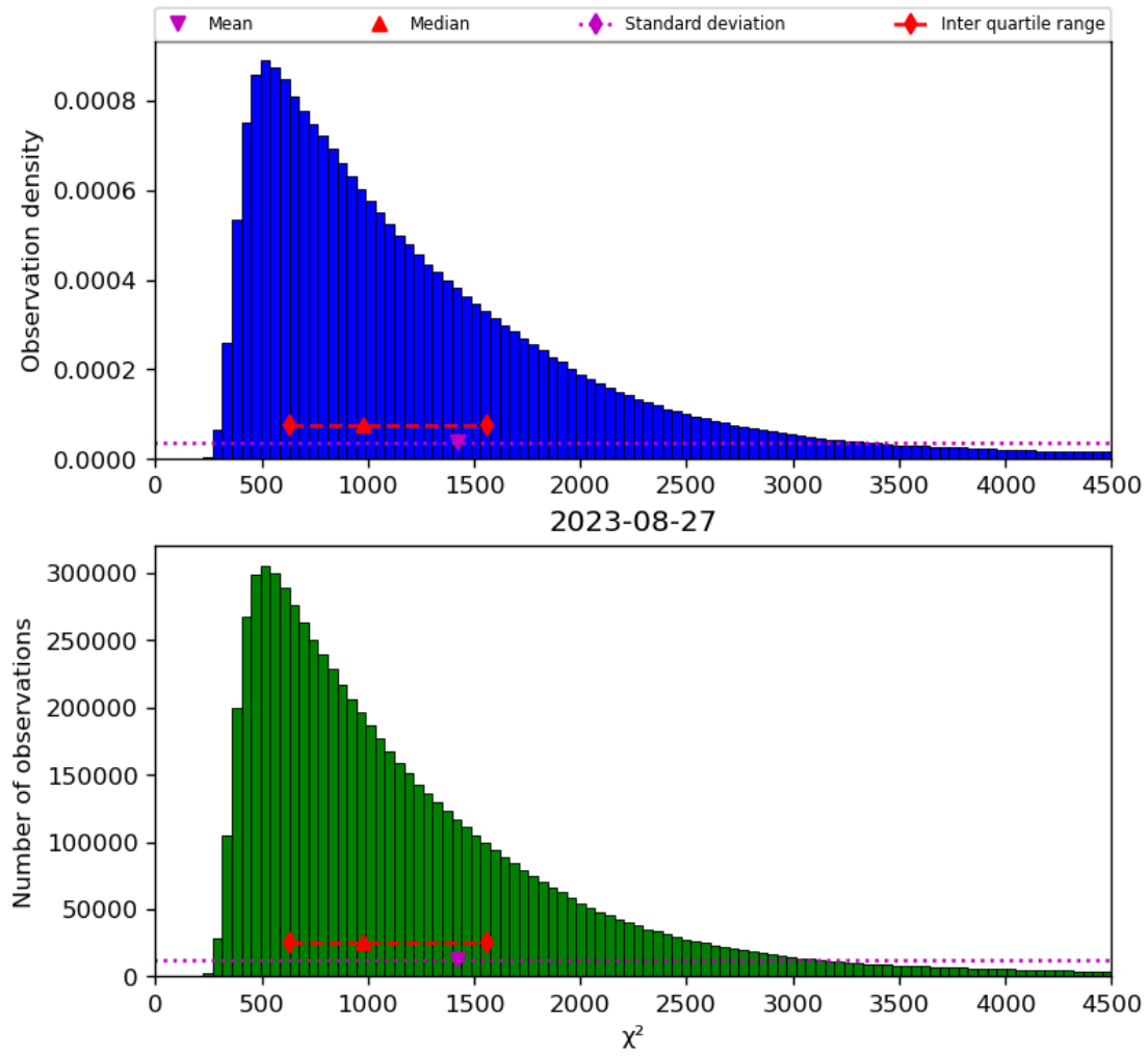
Figure 22: Histogram of “ \chi^2 ” for 2023-08-26 to 2023-08-28
