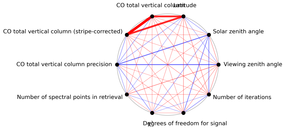
Figure 1: Map of correlation graph for 2023-08-26 to 2023-08-28.
