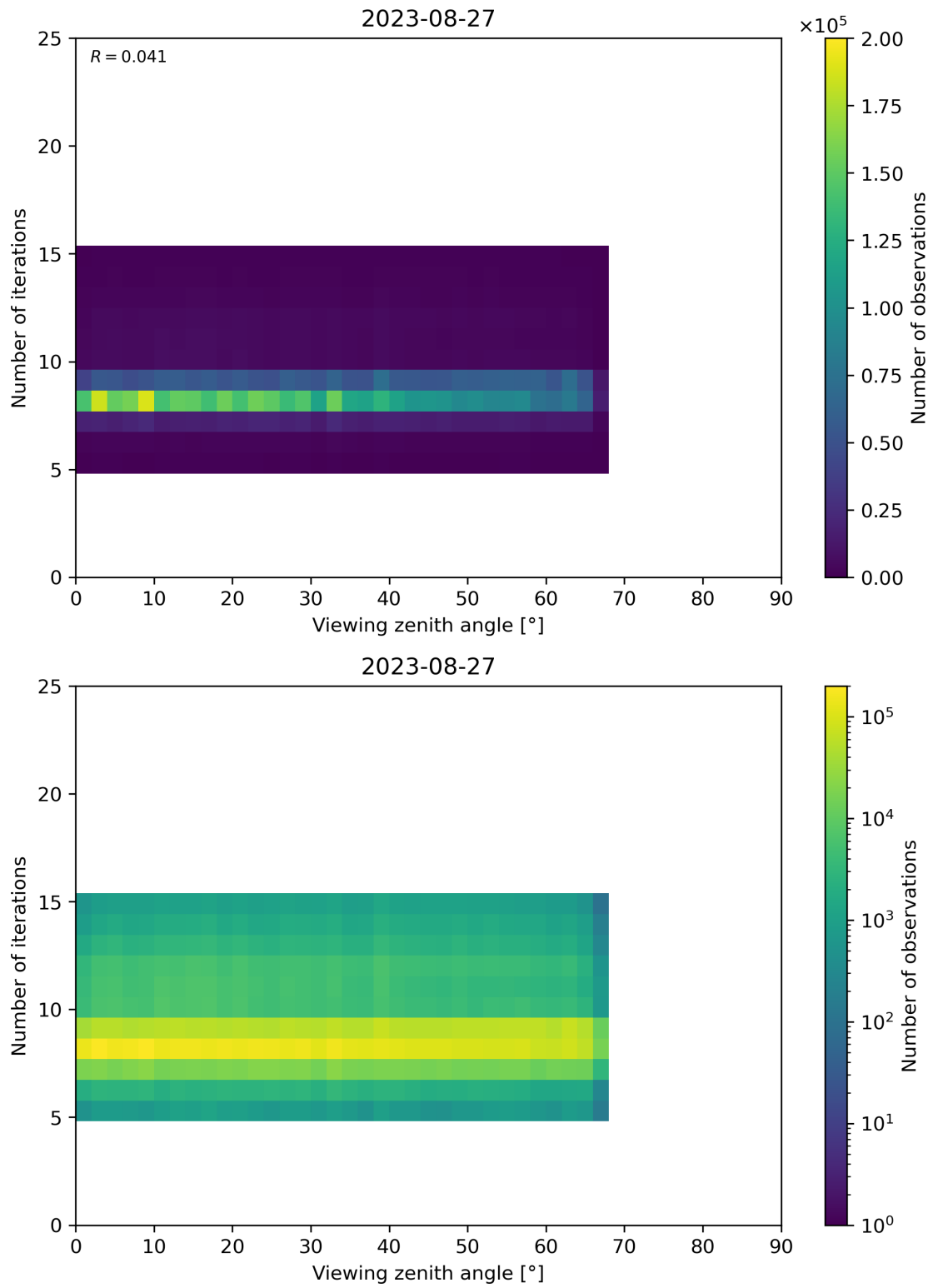
Figure 75: Scatter density plot of “Viewing zenith angle” against “Number of iterations” for 2023-08-26 to 2023-08-28.
