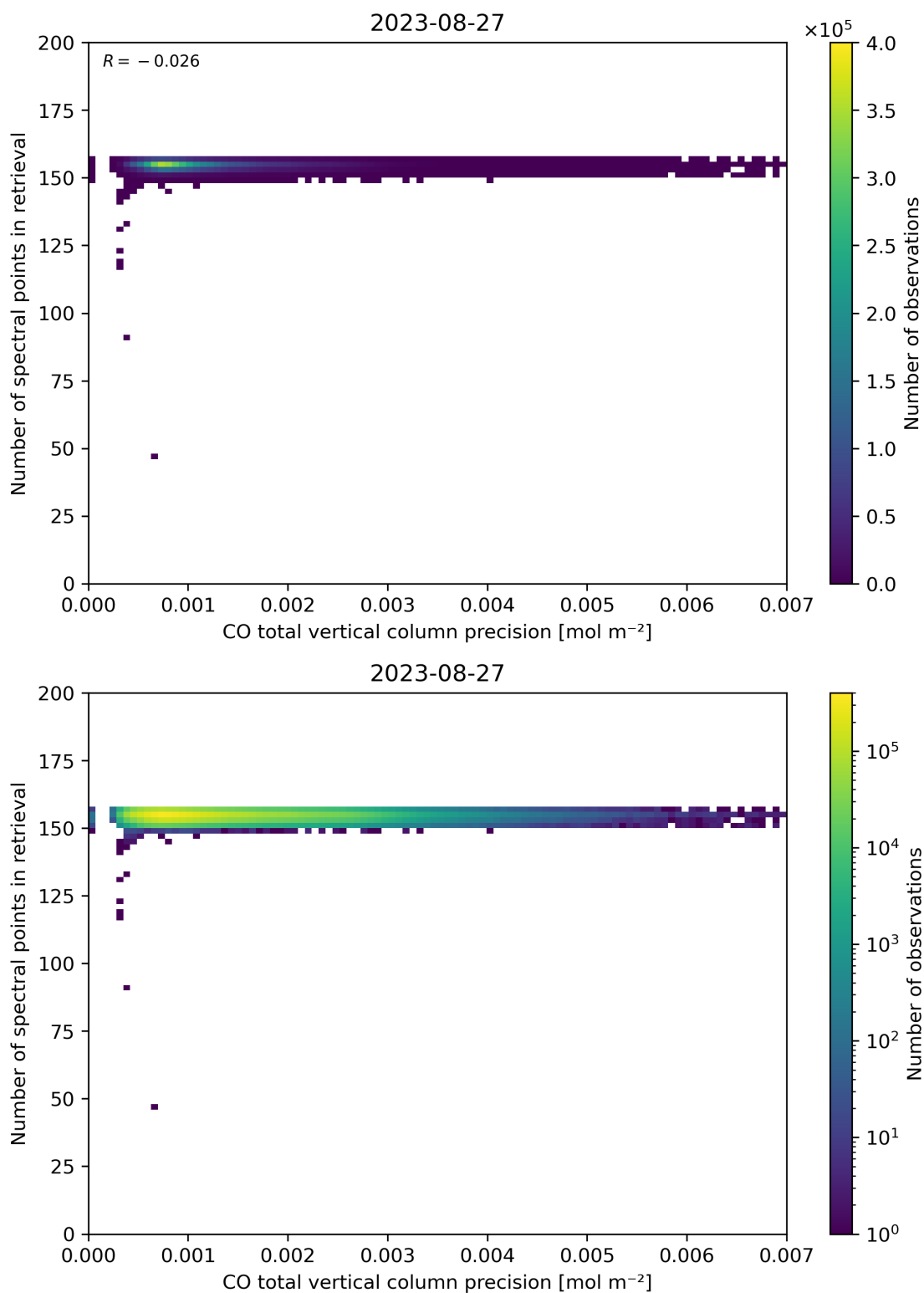
Figure 47: Scatter density plot of “CO total vertical column precision” against “Number of spectral points in retrieval” for 2023-08-26 to 2023-08-28.
