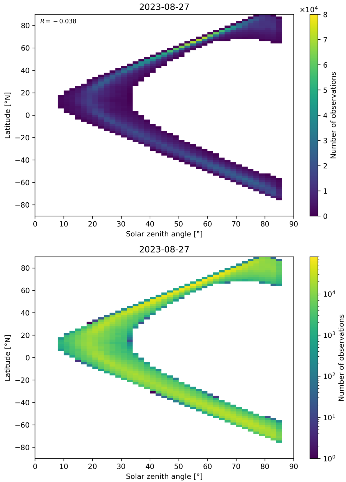
Figure 66: Scatter density plot of “Solar zenith angle” against “Latitude” for 2023-08-26 to 2023-08-28.
