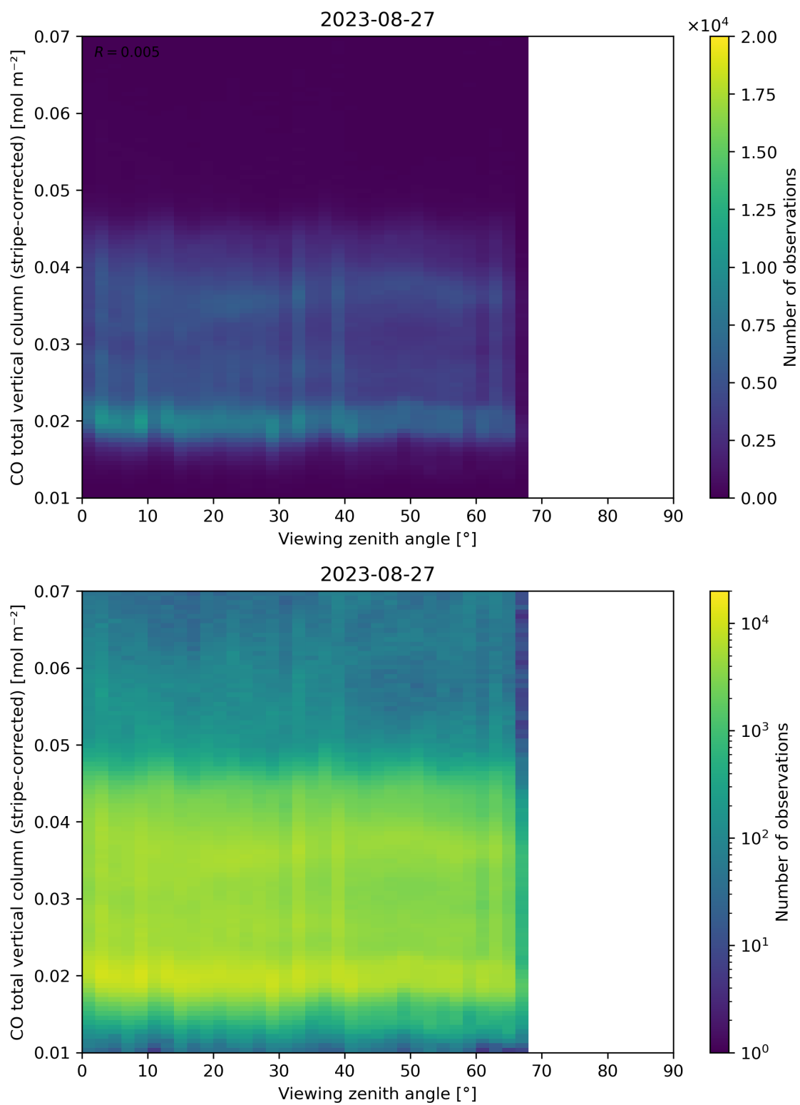
Figure 70: Scatter density plot of “Viewing zenith angle” against “CO total vertical column (stripe-corrected)” for 2023-08-26 to 2023-08-28.
