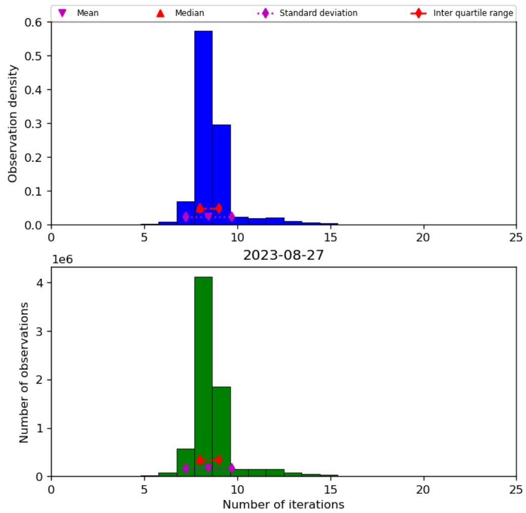
Figure 24: Histogram of “Number of iterations” for 2023-08-26 to 2023-08-28
