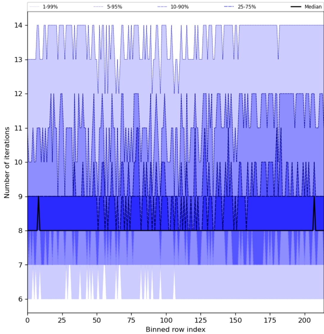
Figure 32: Along track statistics of “Number of iterations” for 2023-08-26 to 2023-08-28
