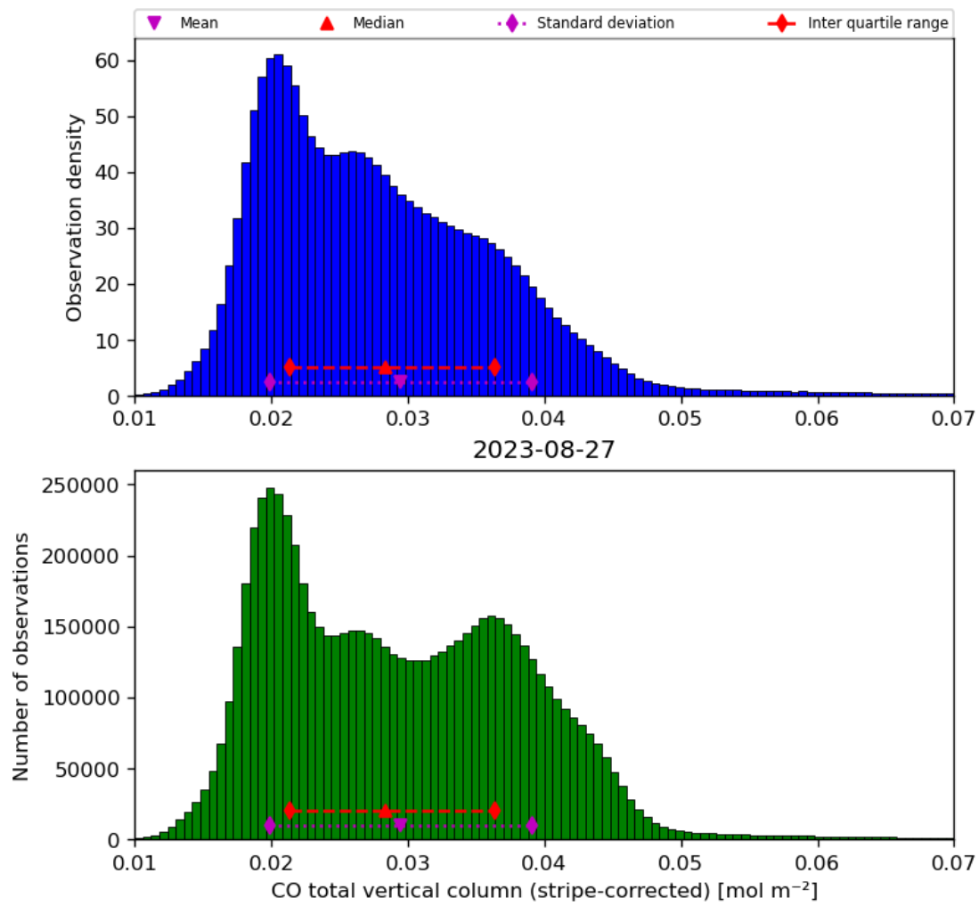
Figure 19: Histogram of “CO total vertical column (stripe-corrected)” for 2023-08-26 to 2023-08-28
