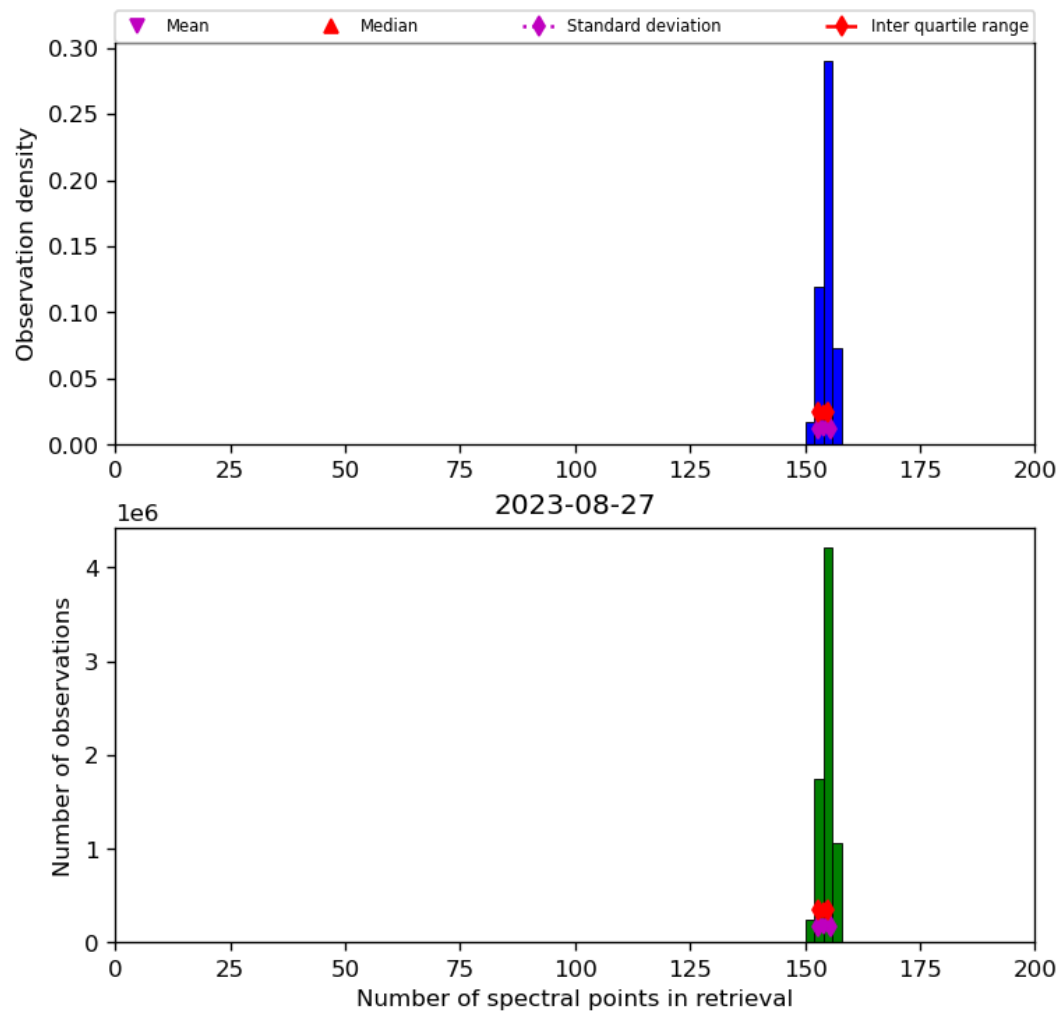
Figure 21: Histogram of “Number of spectral points in retrieval” for 2023-08-26 to 2023-08-28
