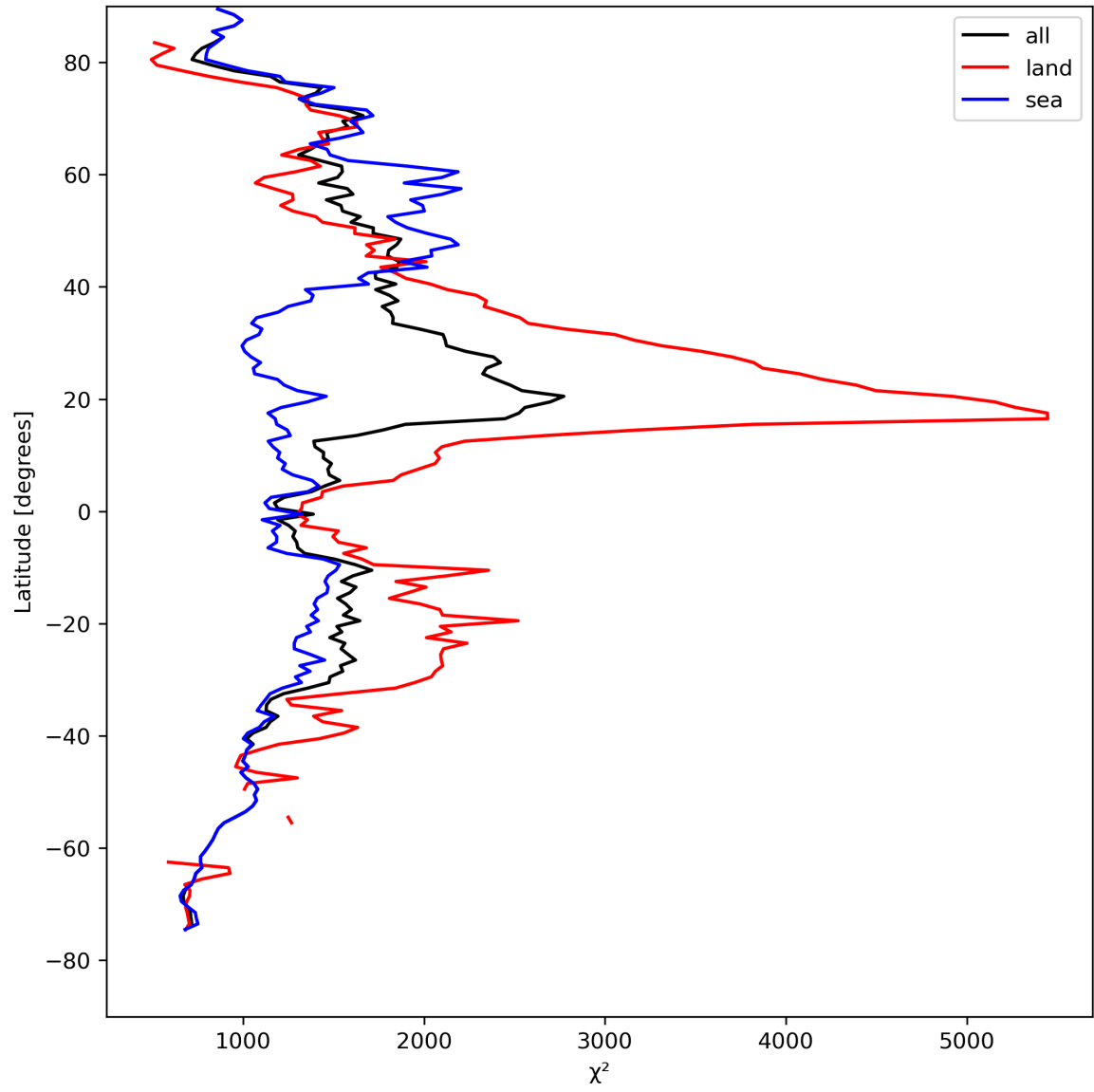
Figure 14: Zonal average of “ \chi^2 ” for 2023-08-26 to 2023-08-28.
