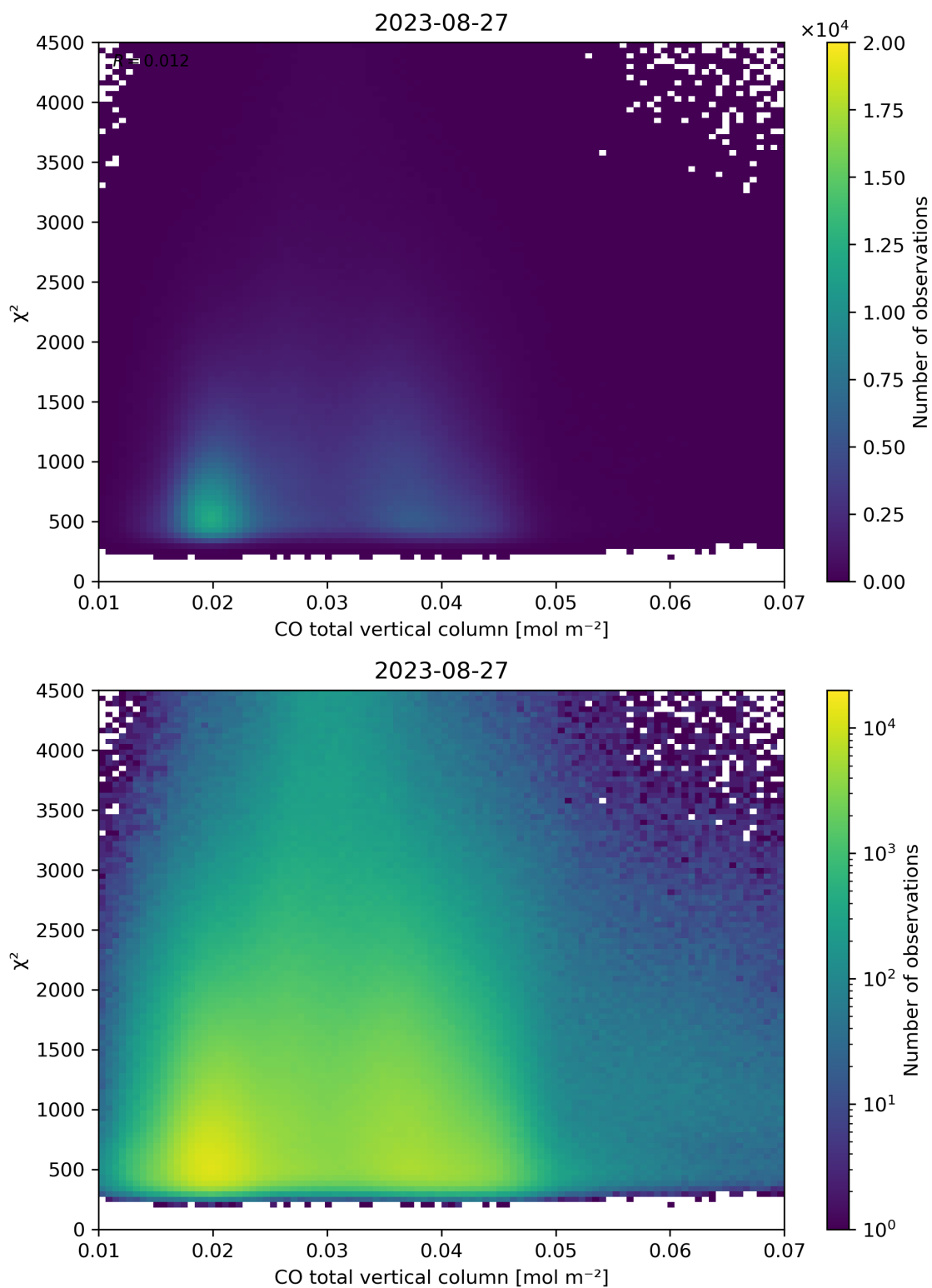
Figure 35: Scatter density plot of “CO total vertical column” against “ \chi^2 ” for 2023-08-26 to 2023-08-28.
