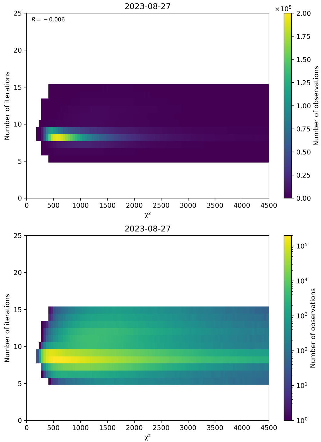
Figure 49: Scatter density plot of “ \chi^2 ” against “Number of iterations” for 2023-08-26 to 2023-08-28.
