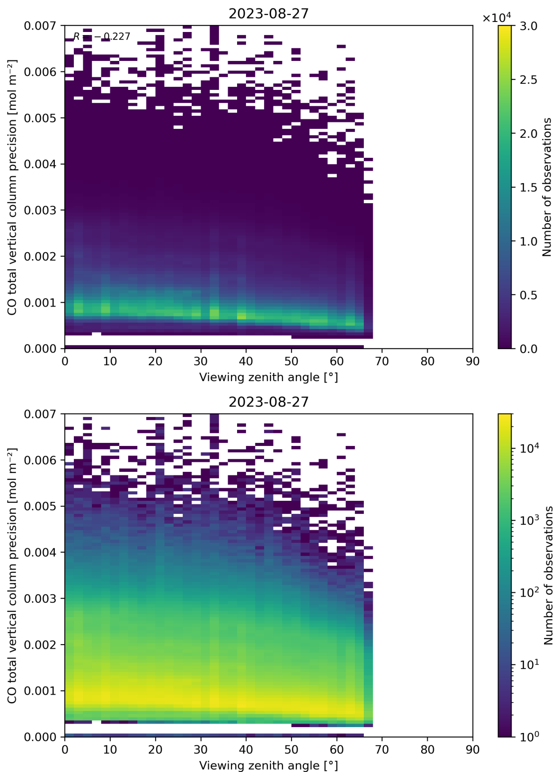
Figure 71: Scatter density plot of “Viewing zenith angle” against “CO total vertical column precision” for 2023-08-26 to 2023-08-28.
