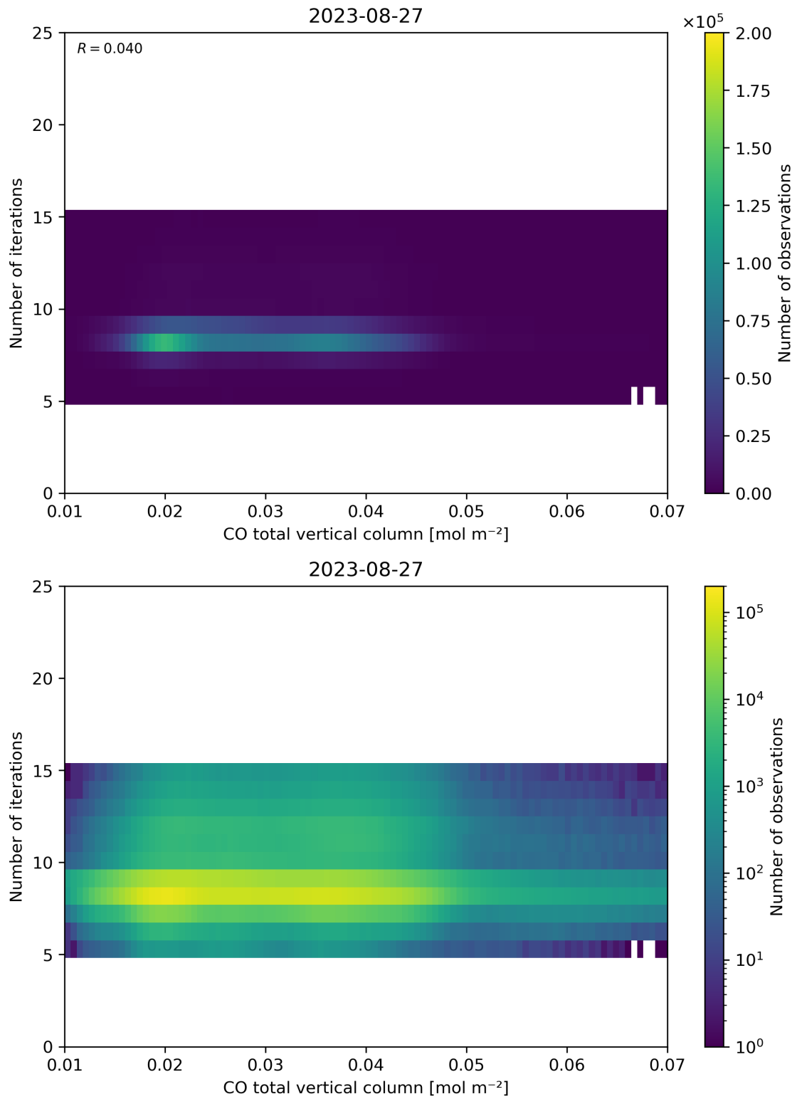
Figure 42: Scatter density plot of “CO total vertical column” against “Number of iterations” for 2023-08-26 to 2023-08-28.
