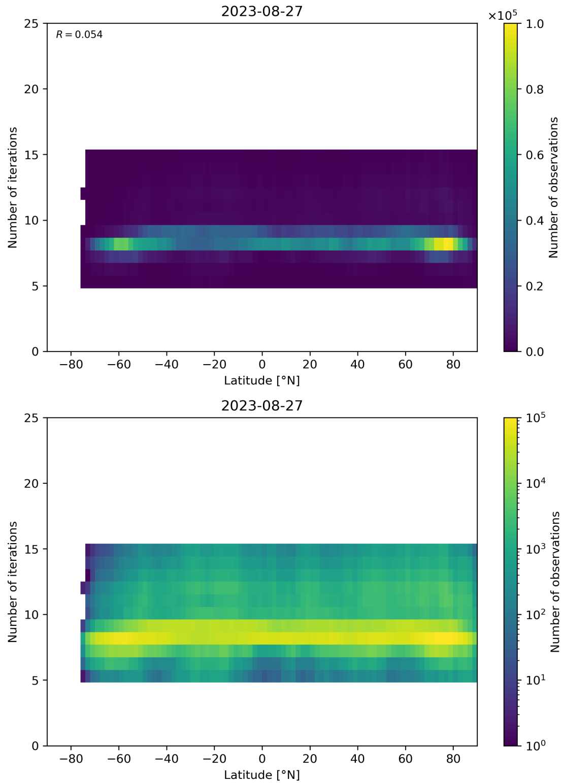
Figure 56: Scatter density plot of “Latitude” against “Number of iterations” for 2023-08-26 to 2023-08-28.
