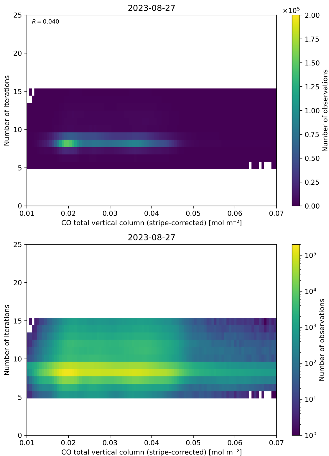
Figure 39: Scatter density plot of “CO total vertical column (stripe-corrected)” against “Number of iterations” for 2023-08-26 to 2023-08-28.
