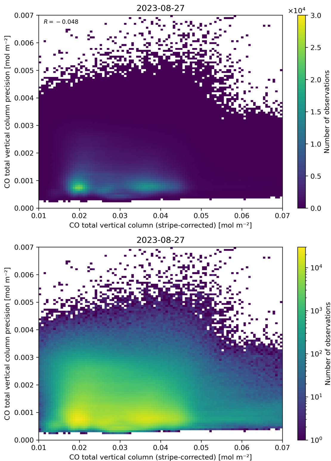
Figure 36: Scatter density plot of “CO total vertical column (stripe-corrected)” against “CO total vertical column precision” for 2023-08-26 to 2023-08-28.
