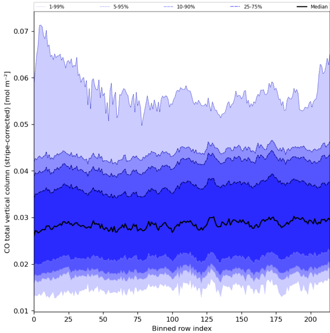
Figure 27: Along track statistics of “CO total vertical column (stripe-corrected)” for 2023-08-26 to 2023-08-28
