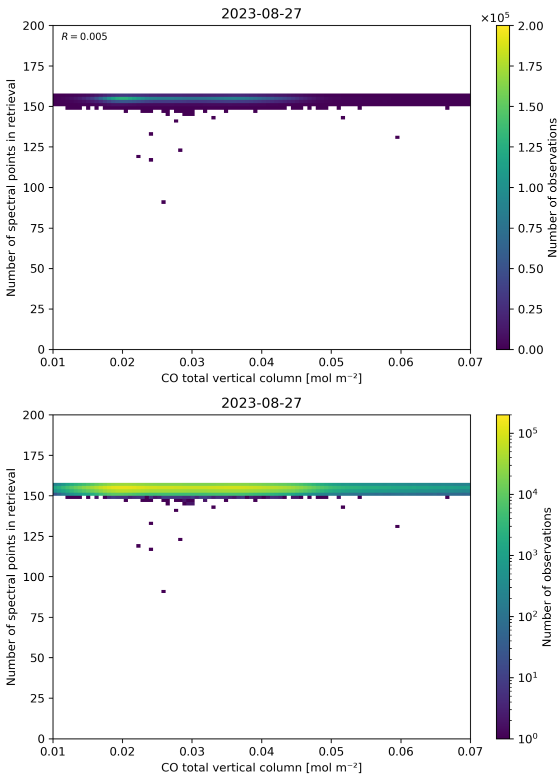
Figure 43: Scatter density plot of “CO total vertical column” against “Number of spectral points in retrieval” for 2023-08-26 to 2023-08-28.
