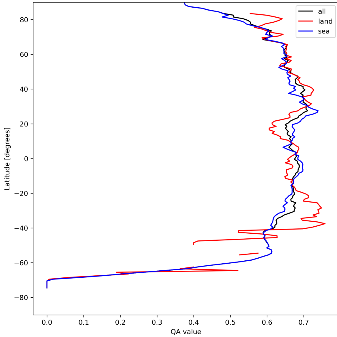
Figure 9: Zonal average of “QA value” for 2023-08-26 to 2023-08-28.
