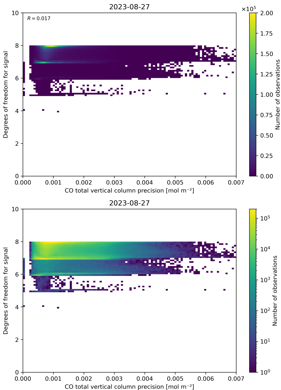
Figure 45: Scatter density plot of “CO total vertical column precision” against “Degrees of freedom for signal” for 2023-08-26 to 2023-08-28.
