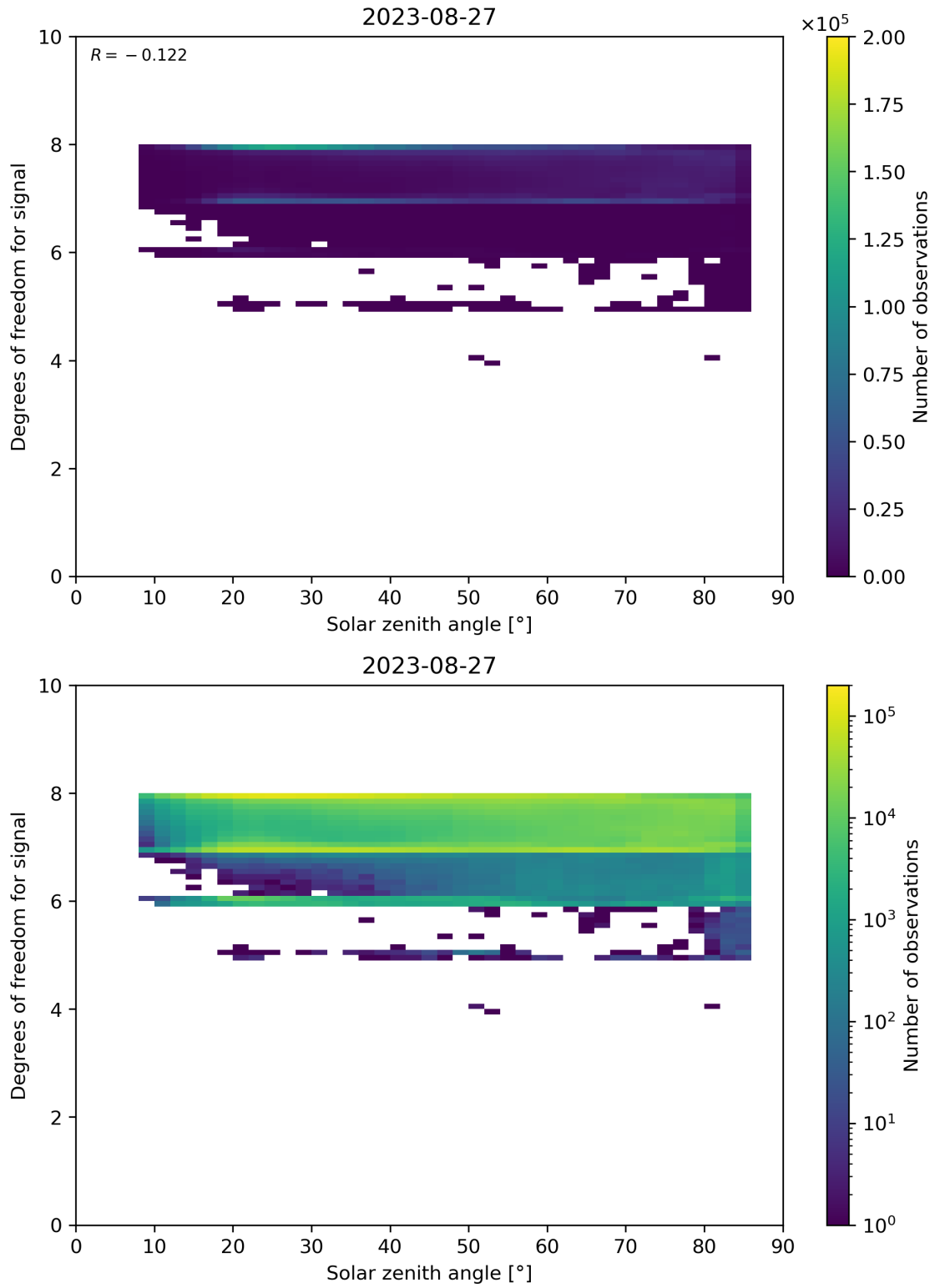
Figure 65: Scatter density plot of “Solar zenith angle” against “Degrees of freedom for signal” for 2023-08-26 to 2023-08-28.
