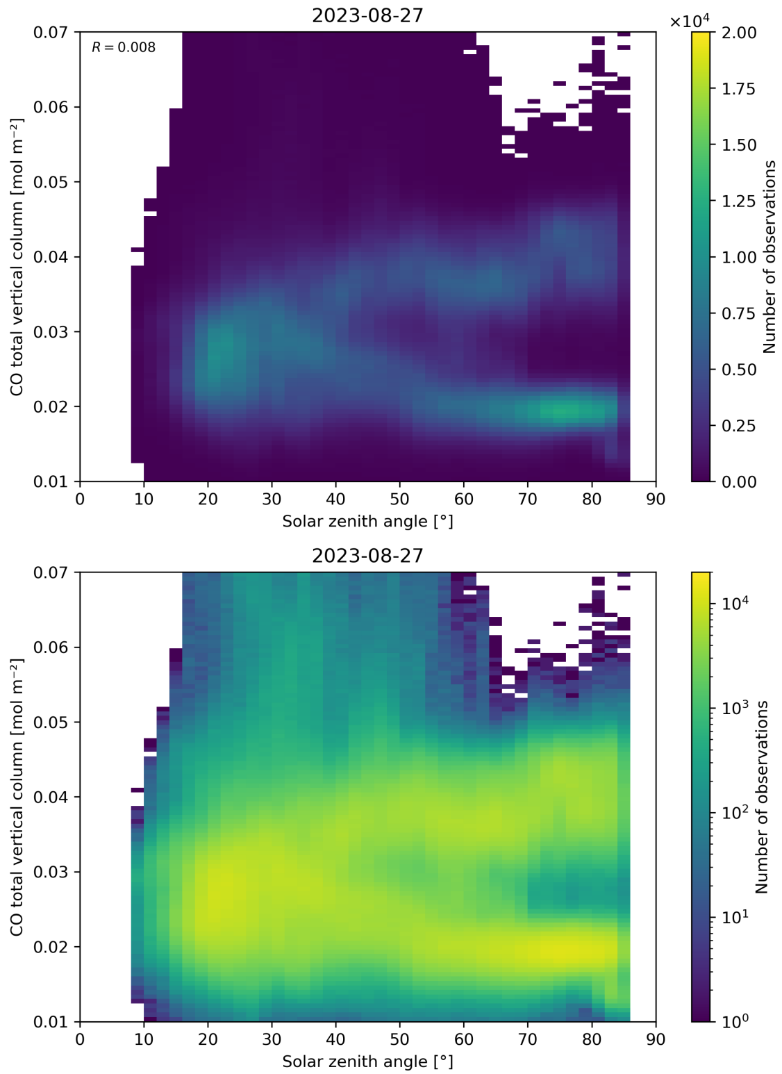
Figure 61: Scatter density plot of “Solar zenith angle” against “CO total vertical column” for 2023-08-26 to 2023-08-28.
