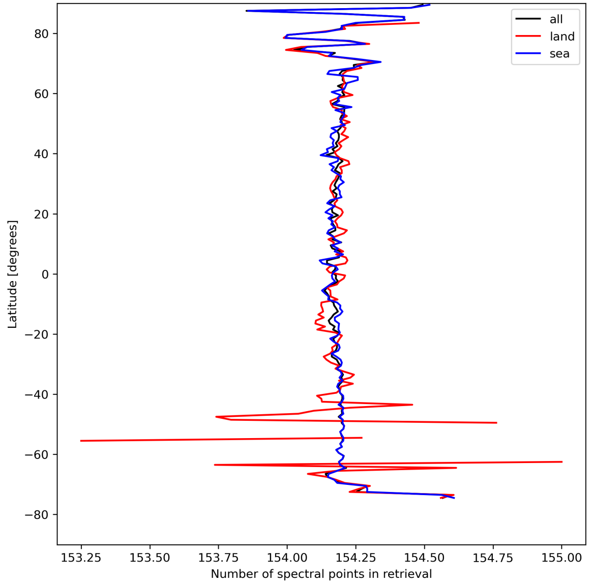
Figure 13: Zonal average of “Number of spectral points in retrieval” for 2023-08-26 to 2023-08-28.
