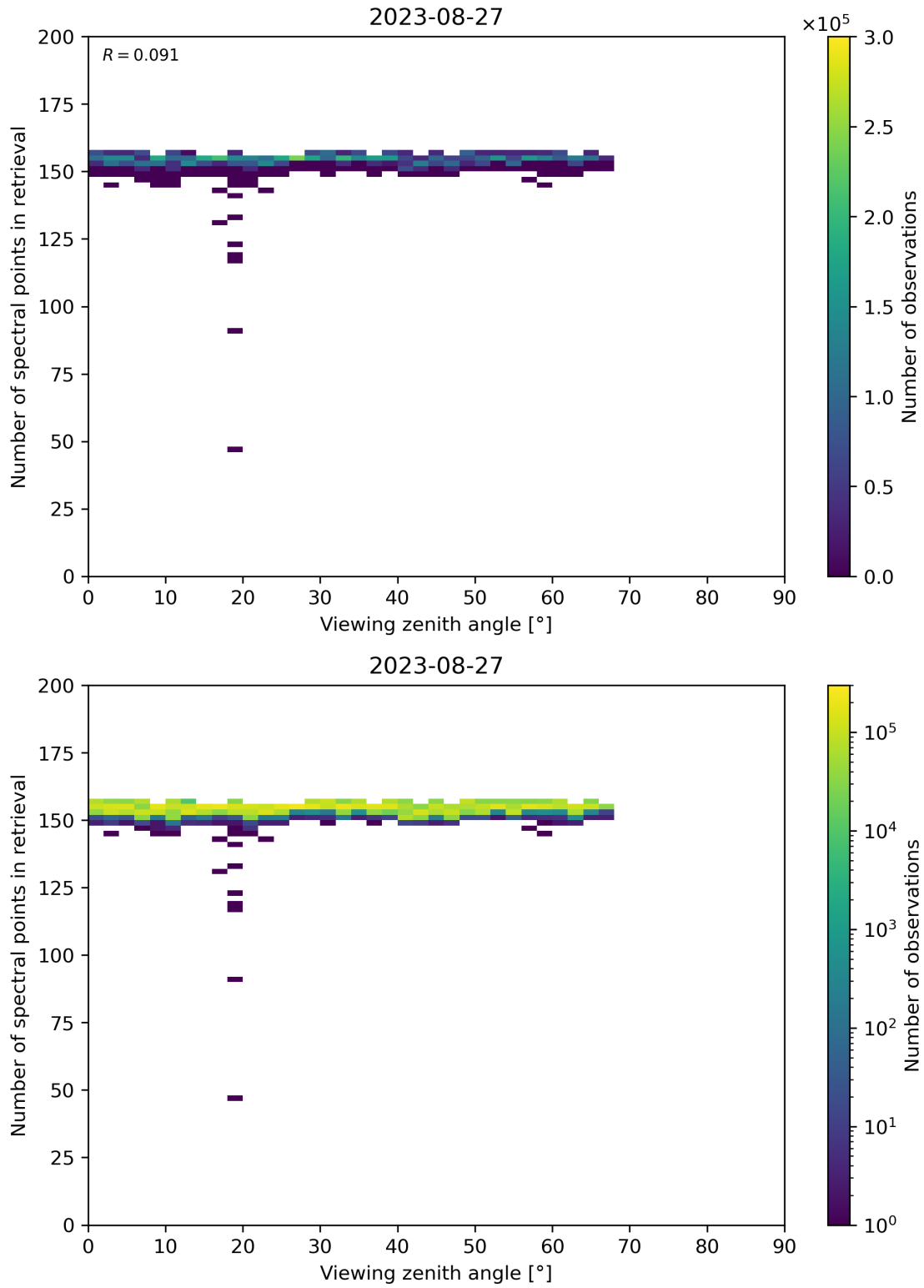
Figure 76: Scatter density plot of “Viewing zenith angle” against “Number of spectral points in retrieval” for 2023-08-26 to 2023-08-28.
