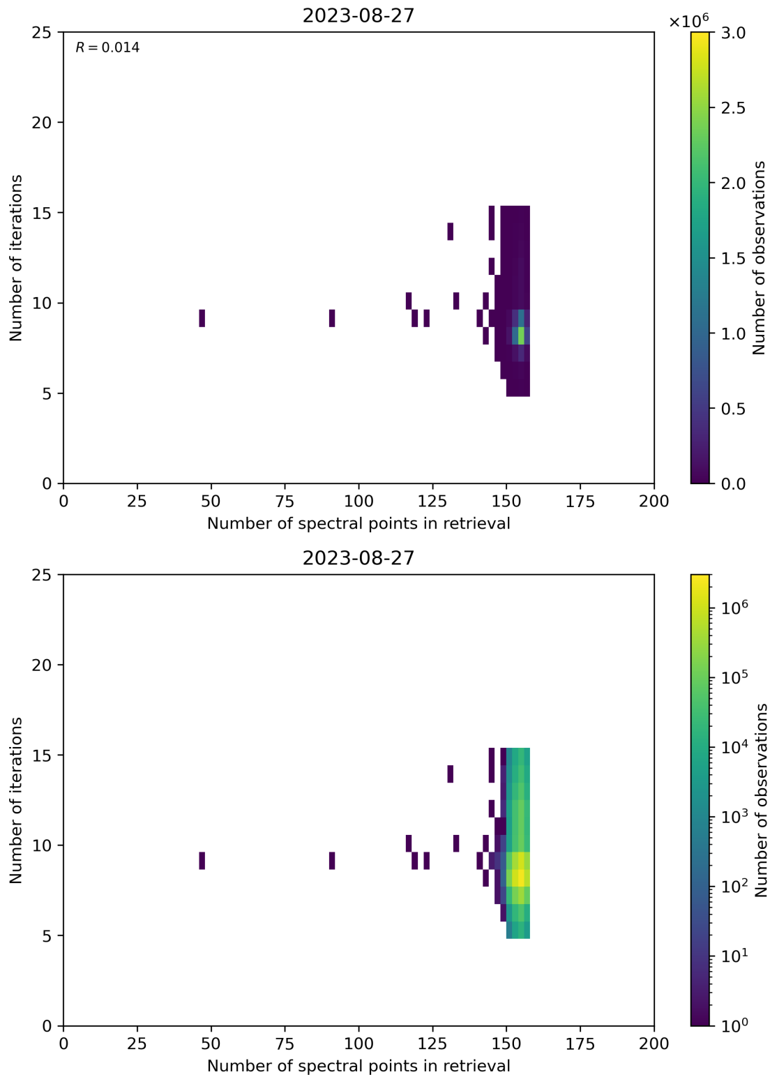
Figure 60: Scatter density plot of “Number of spectral points in retrieval” against “Number of iterations” for 2023-08-26 to 2023-08-28.
