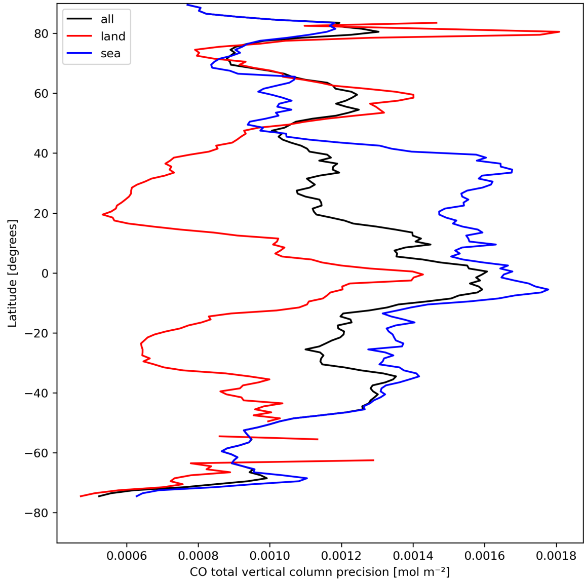
Figure 12: Zonal average of “CO total vertical column precision” for 2023-08-26 to 2023-08-28.
