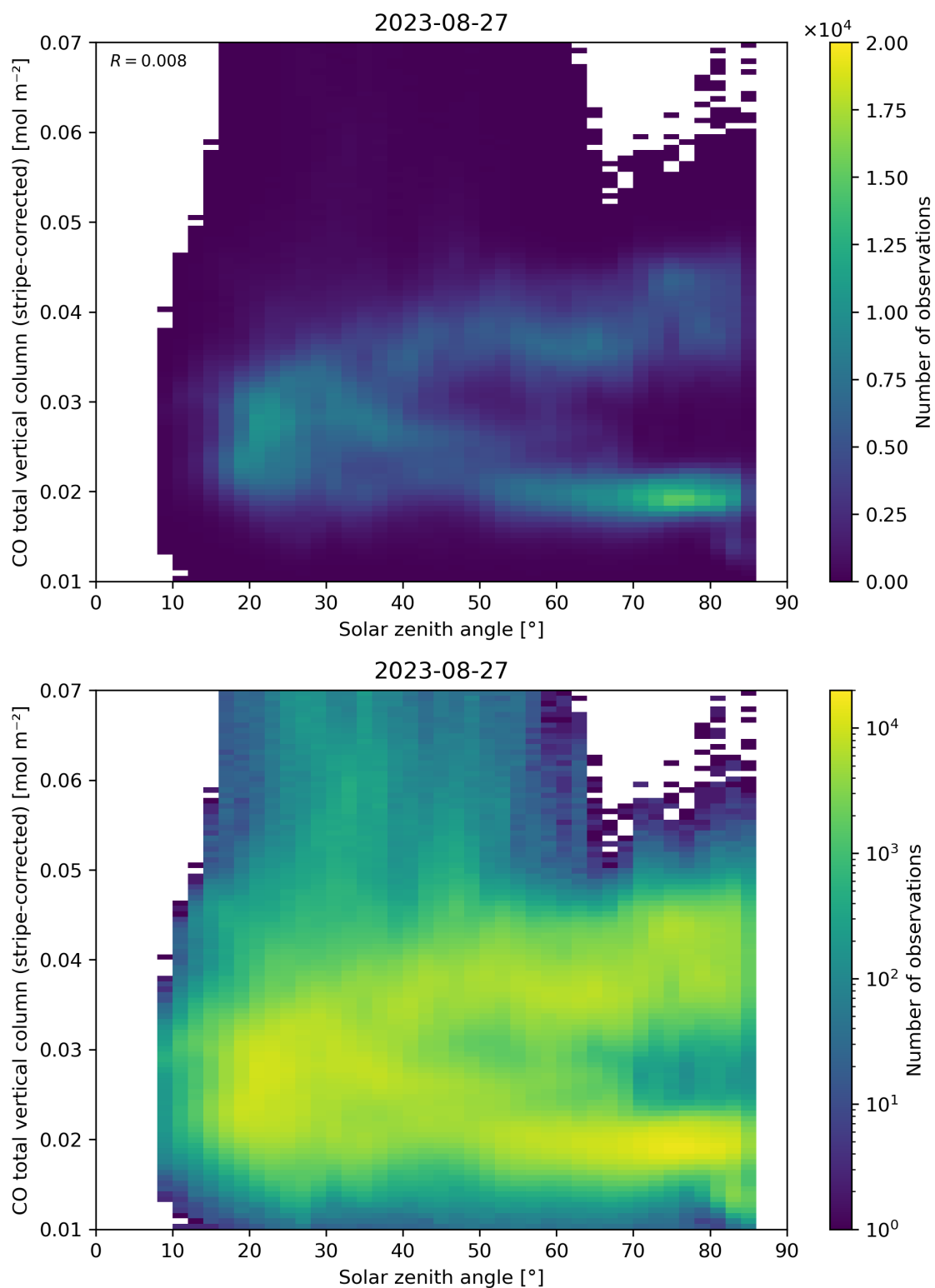
Figure 62: Scatter density plot of “Solar zenith angle” against “CO total vertical column (stripe-corrected)” for 2023-08-26 to 2023-08-28.
