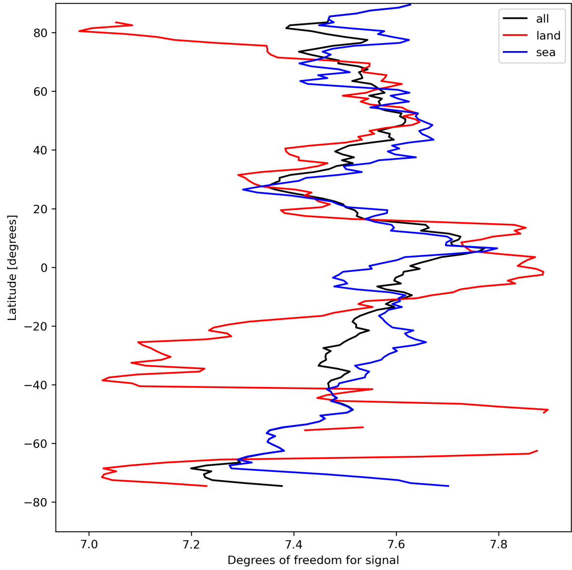
Figure 15: Zonal average of “Degrees of freedom for signal” for 2023-08-26 to 2023-08-28.
