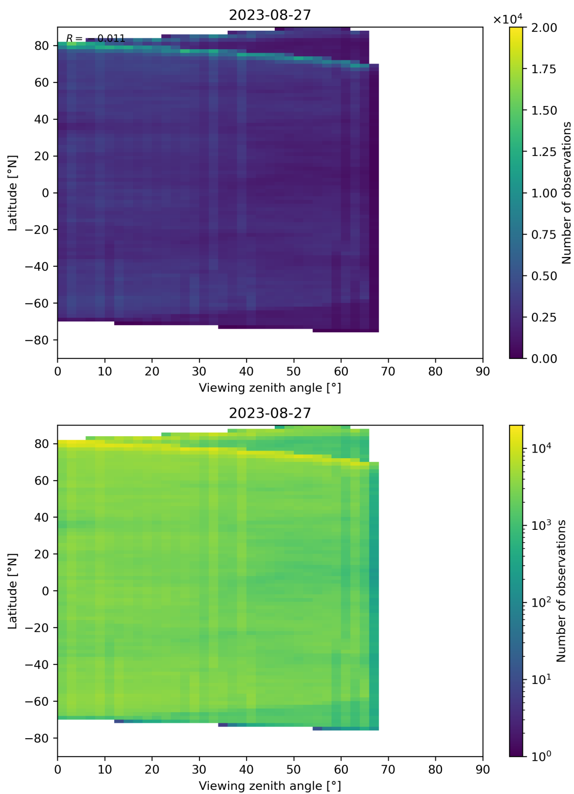
Figure 74: Scatter density plot of “Viewing zenith angle” against “Latitude” for 2023-08-26 to 2023-08-28.
