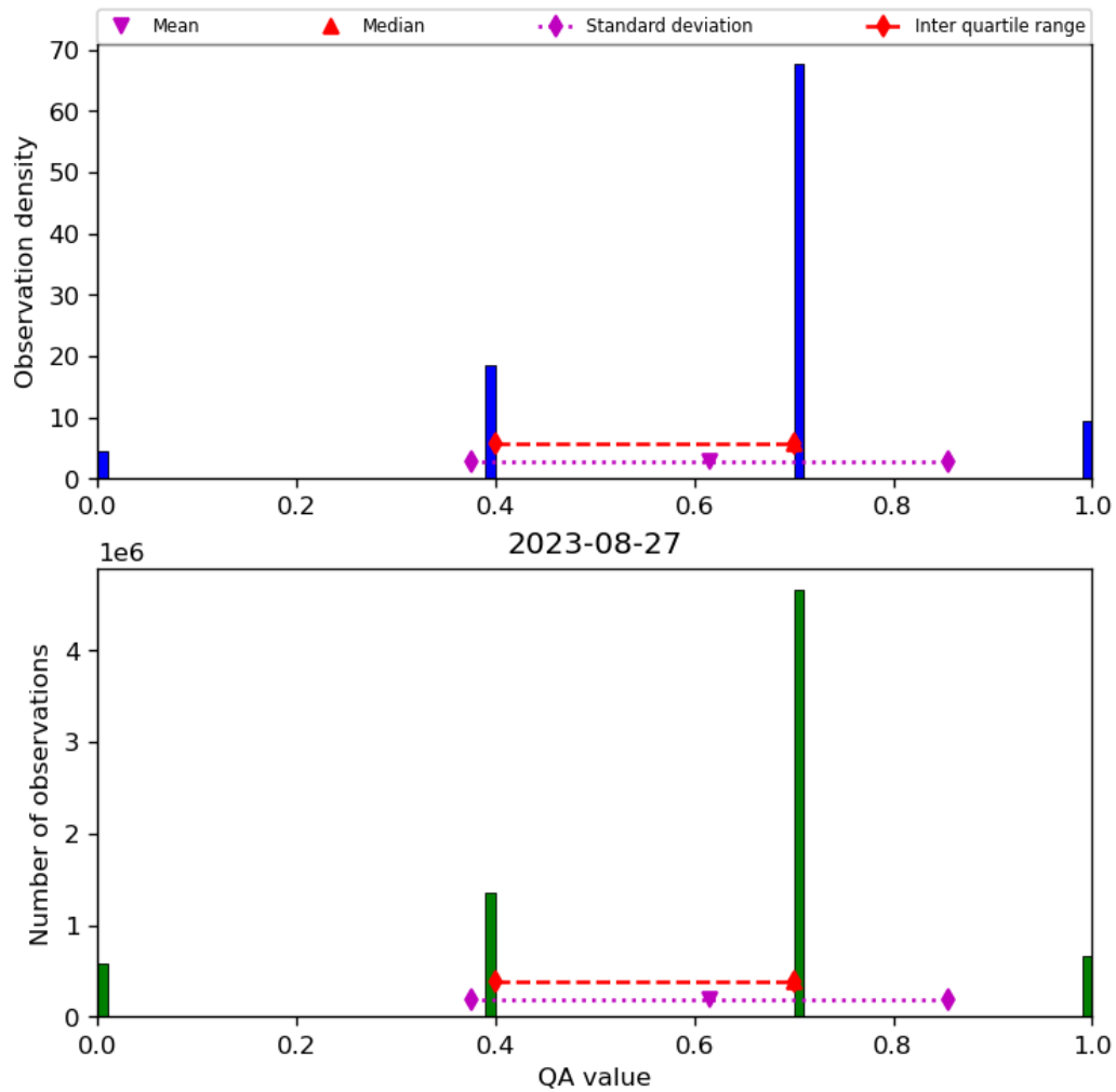
Figure 17: Histogram of “QA value” for 2023-08-26 to 2023-08-28
