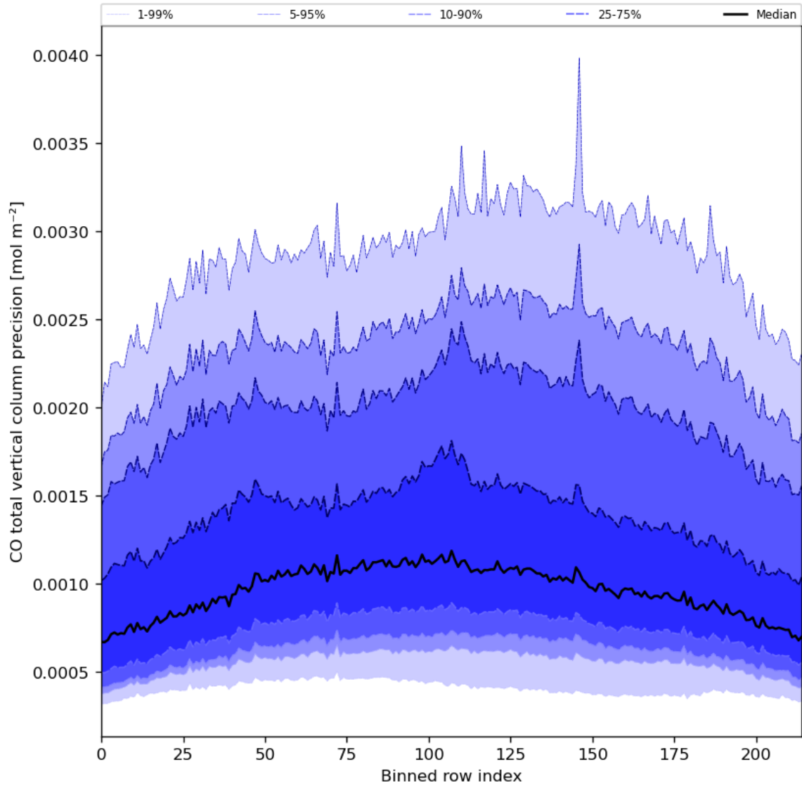
Figure 28: Along track statistics of “CO total vertical column precision” for 2023-08-26 to 2023-08-28
