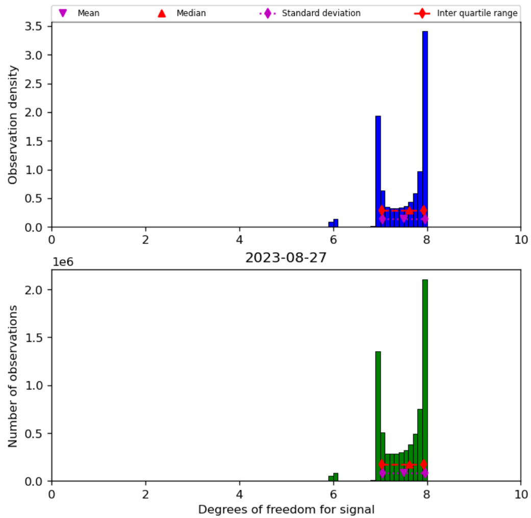
Figure 23: Histogram of “Degrees of freedom for signal” for 2023-08-26 to 2023-08-28
