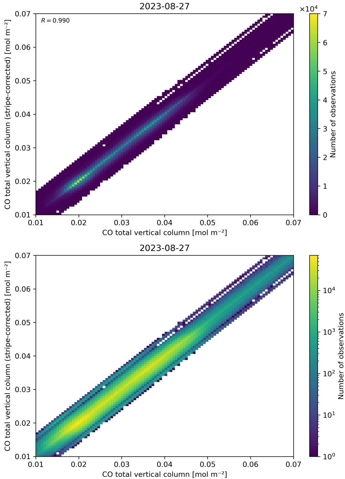
Figure 33: Scatter density plot of “CO total vertical column” against “CO total vertical column (stripe-corrected)” for 2023-08-26 to 2023-08-28.
