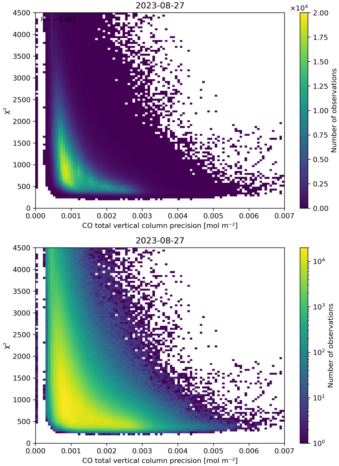
Figure 44: Scatter density plot of “CO total vertical column precision” against “ \chi^2 ” for 2023-08-26 to 2023-08-28.
