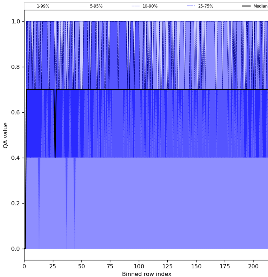
Figure 25: Along track statistics of “QA value” for 2023-08-26 to 2023-08-28
