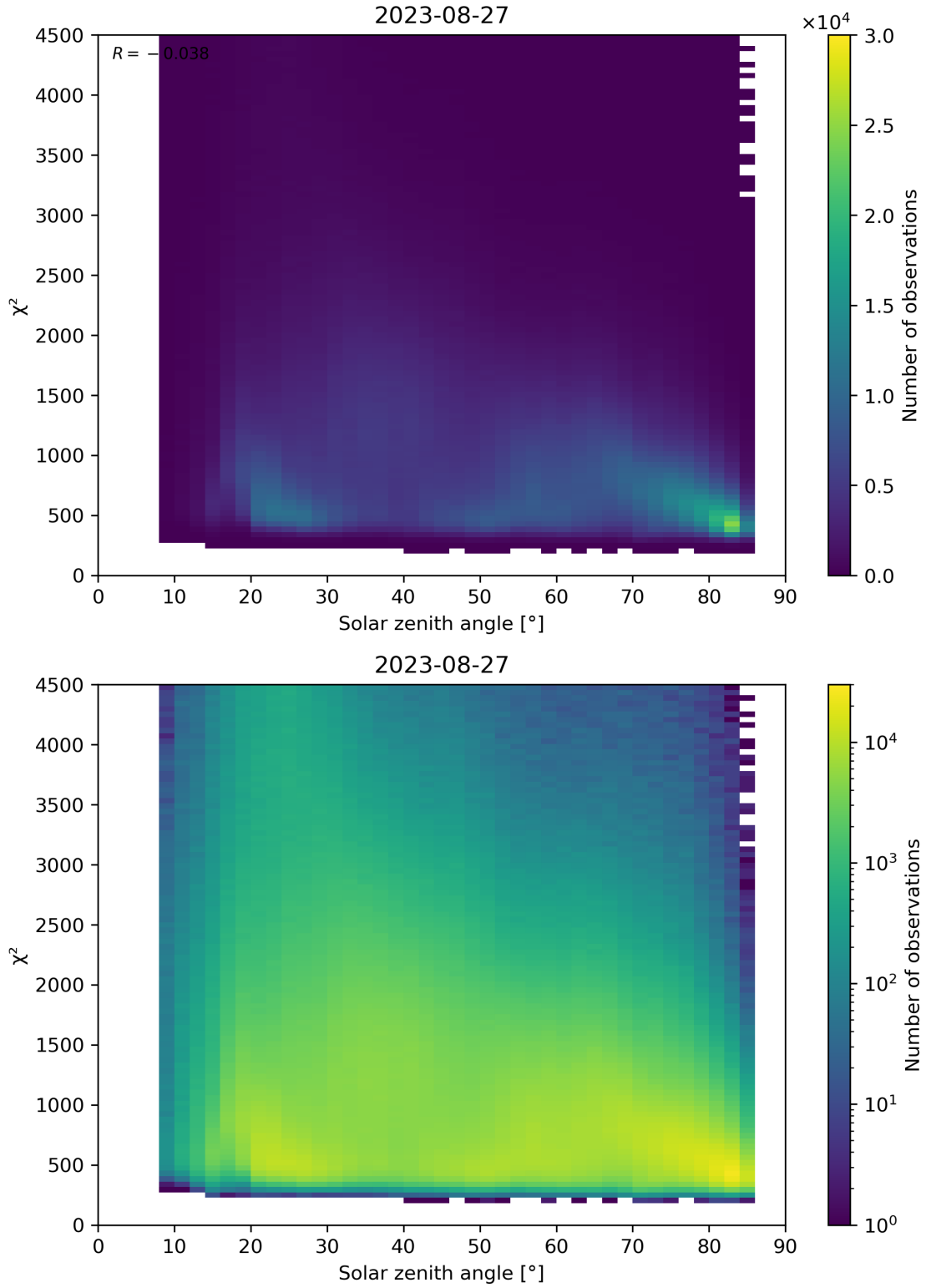
Figure 64: Scatter density plot of “Solar zenith angle” against “ \chi^2 ” for 2023-08-26 to 2023-08-28.
