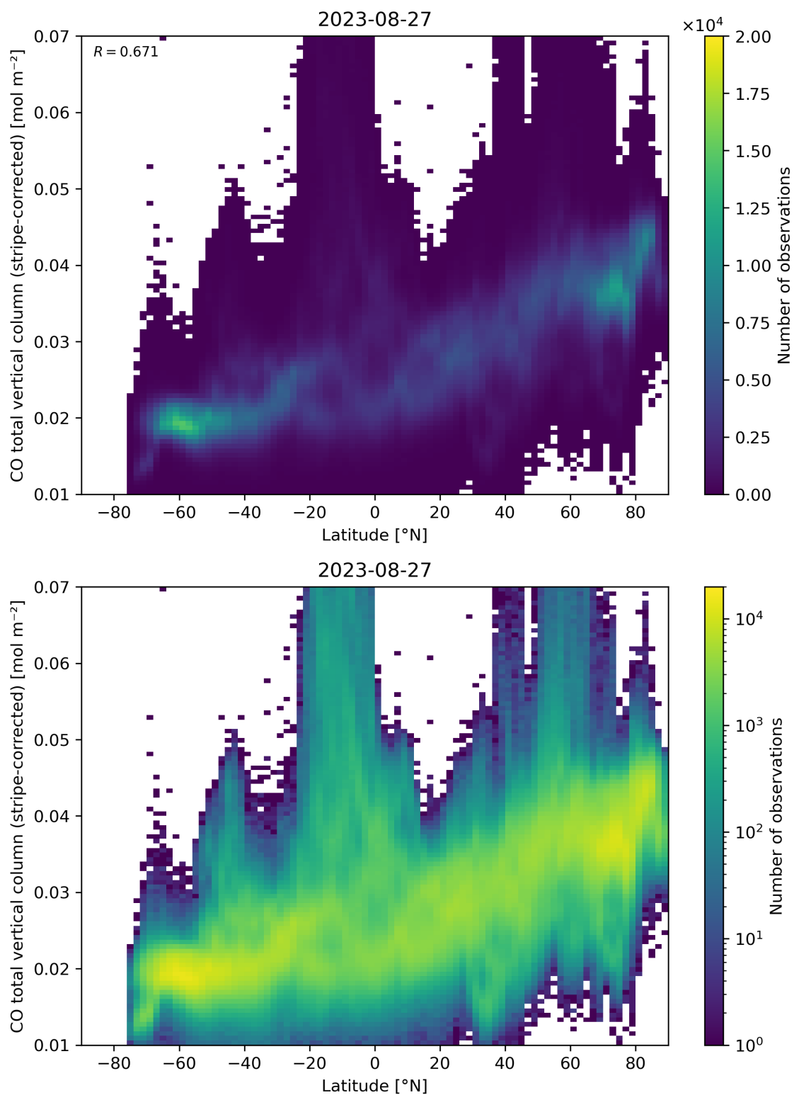
Figure 52: Scatter density plot of “Latitude” against “CO total vertical column (stripe-corrected)” for 2023-08-26 to 2023-08-28.
