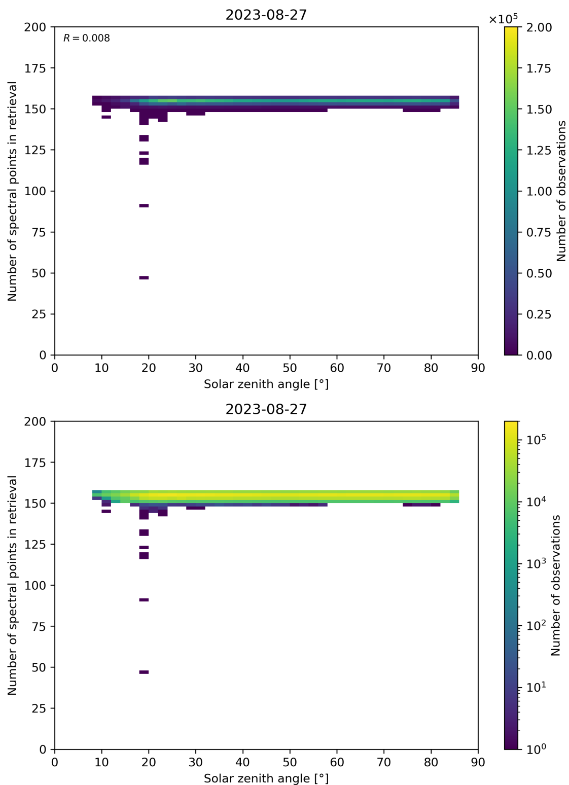
Figure 68: Scatter density plot of “Solar zenith angle” against “Number of spectral points in retrieval” for 2023-08-26 to 2023-08-28.
