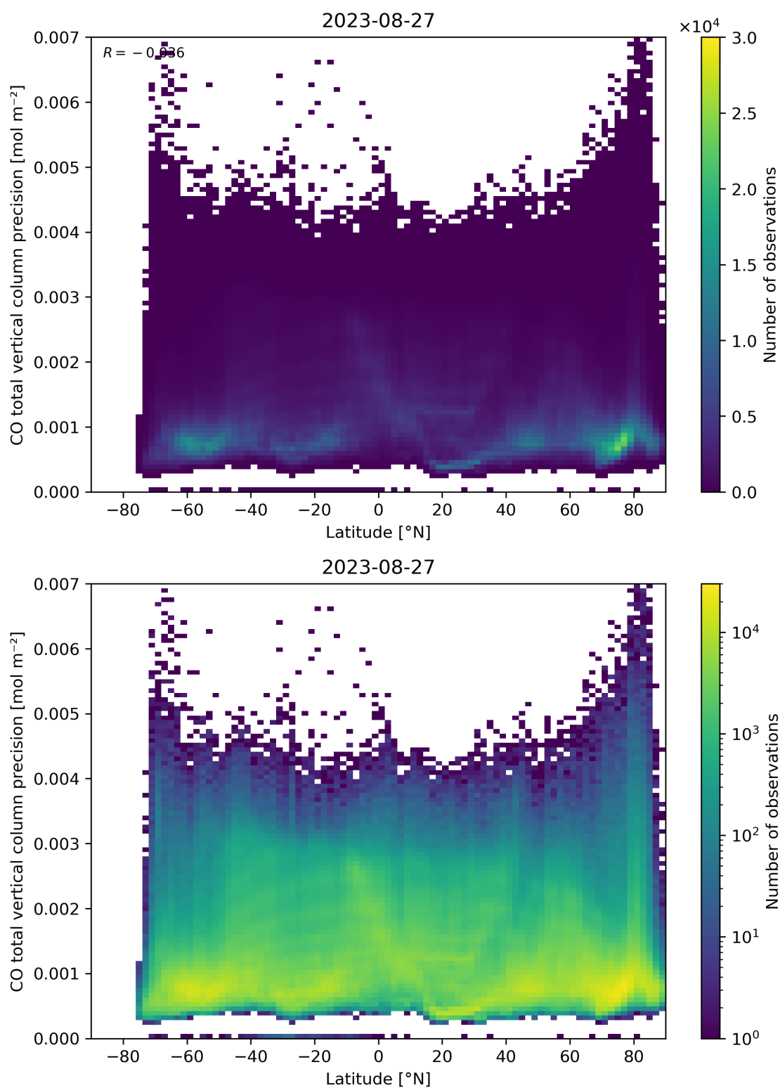
Figure 53: Scatter density plot of “Latitude” against “CO total vertical column precision” for 2023-08-26 to 2023-08-28.
