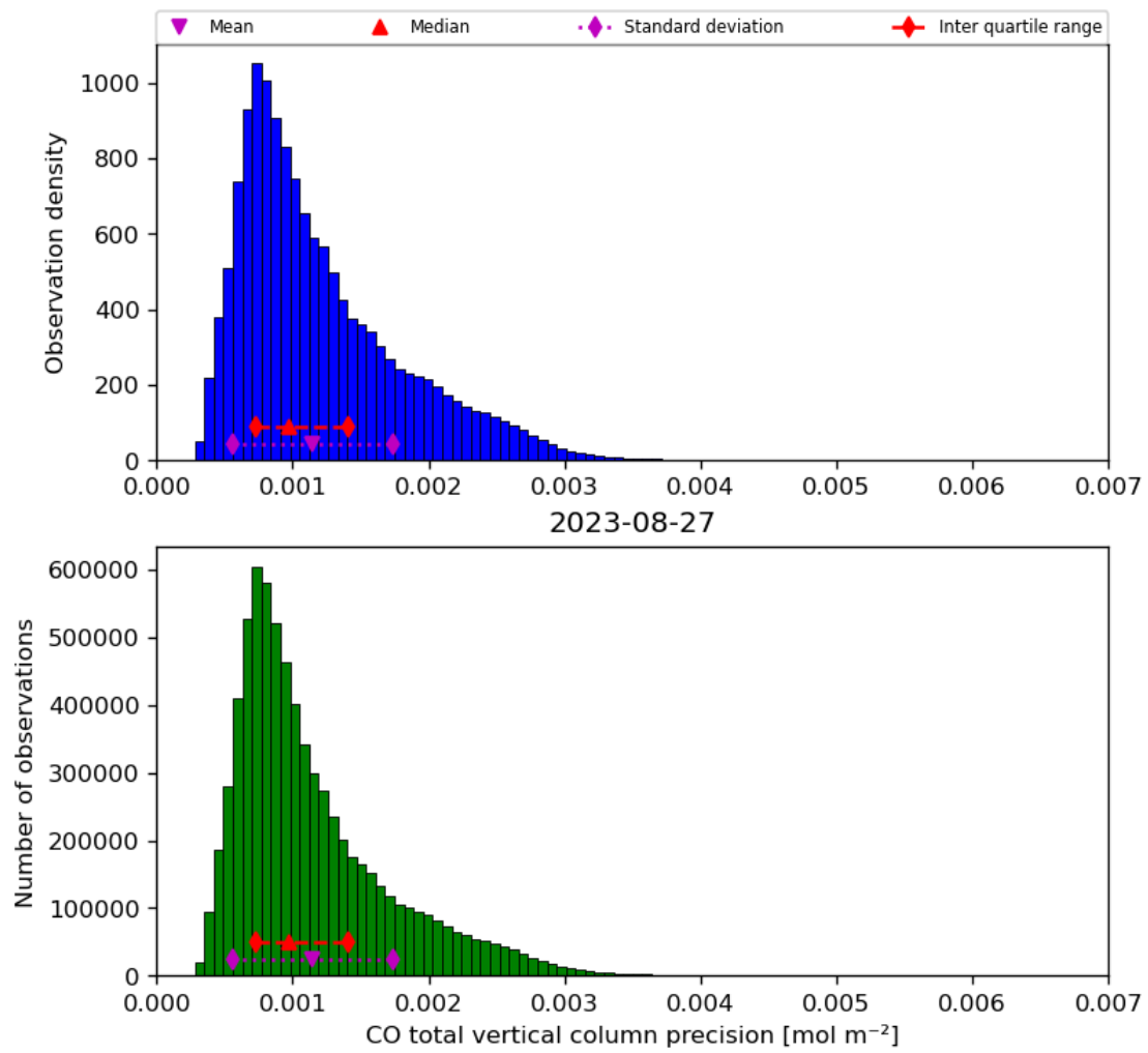
Figure 20: Histogram of “CO total vertical column precision” for 2023-08-26 to 2023-08-28
