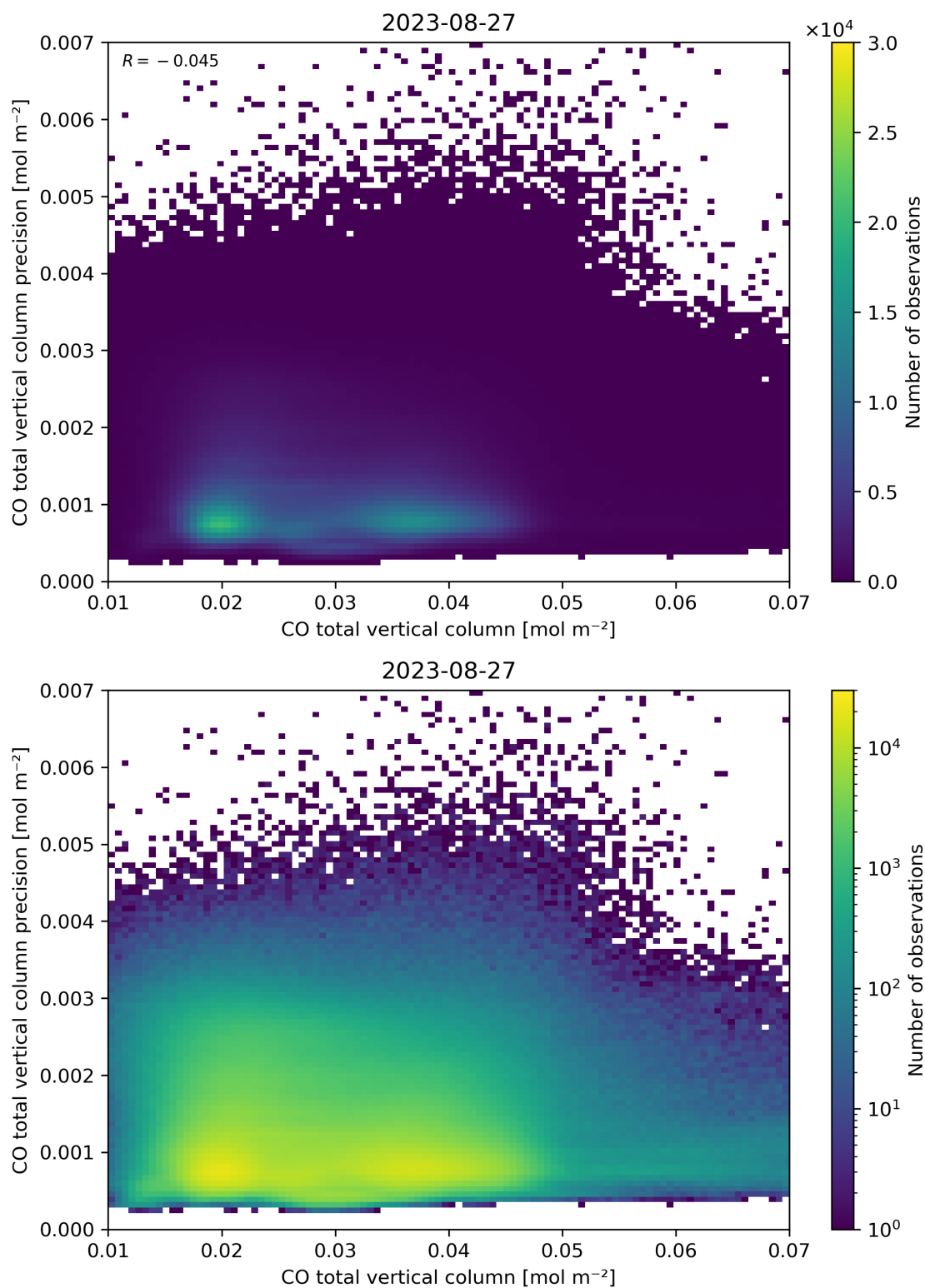
Figure 34: Scatter density plot of “CO total vertical column” against “CO total vertical column precision” for 2023-08-26 to 2023-08-28.
