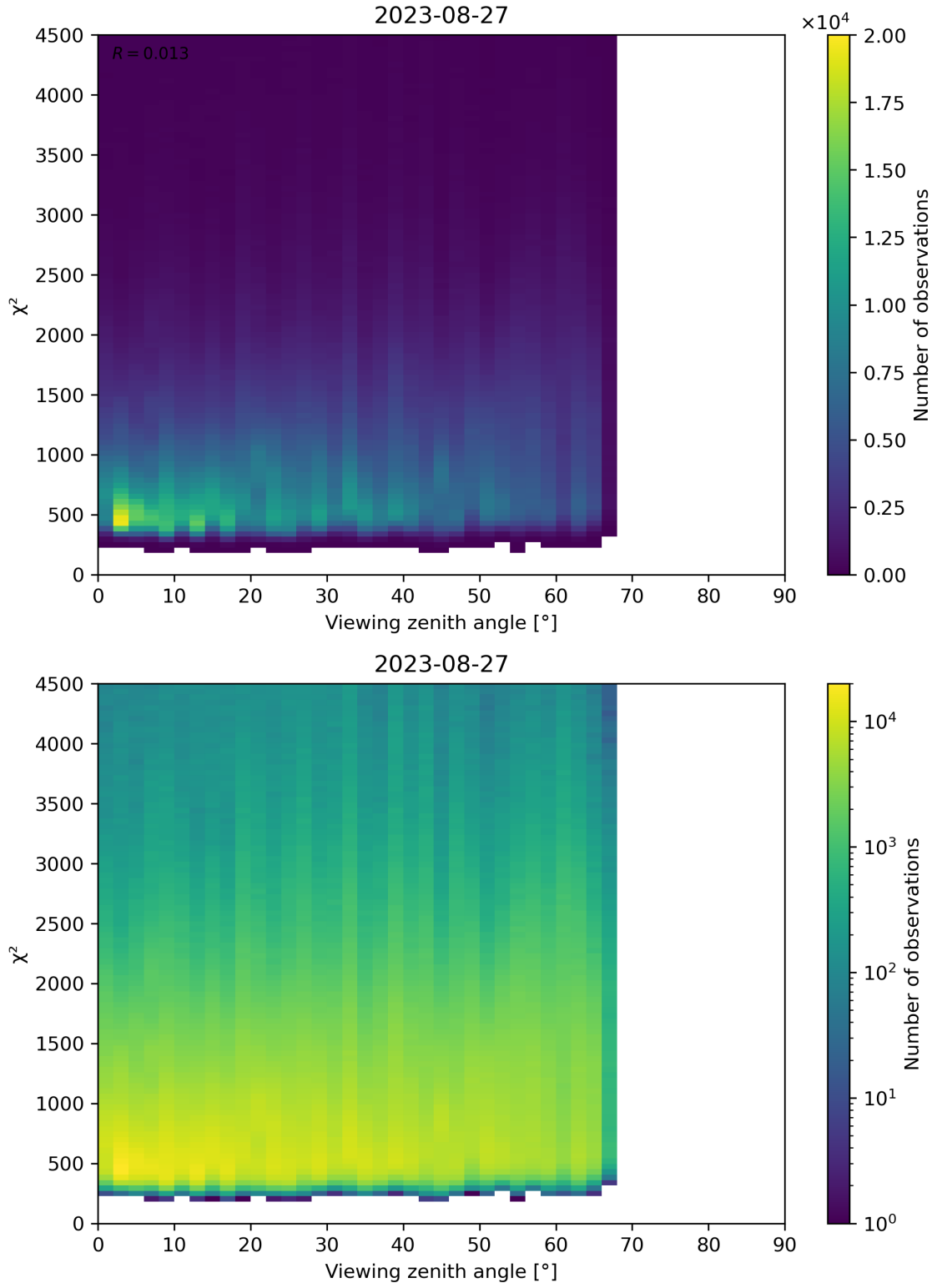
Figure 72: Scatter density plot of “Viewing zenith angle” against “ \chi^2 ” for 2023-08-26 to 2023-08-28.
