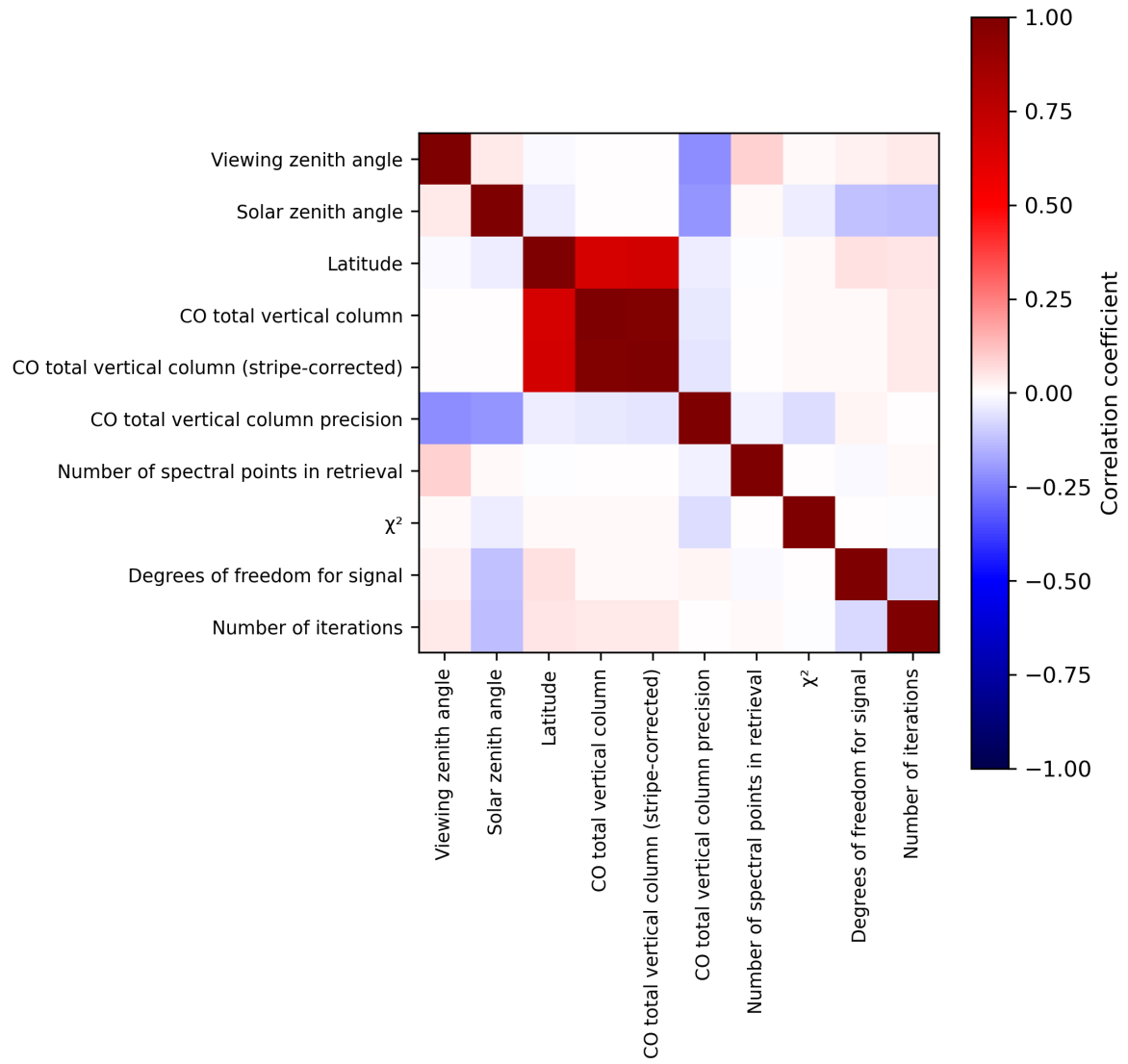
Figure 2: Map of correlation matrix for 2023-08-26 to 2023-08-28.
