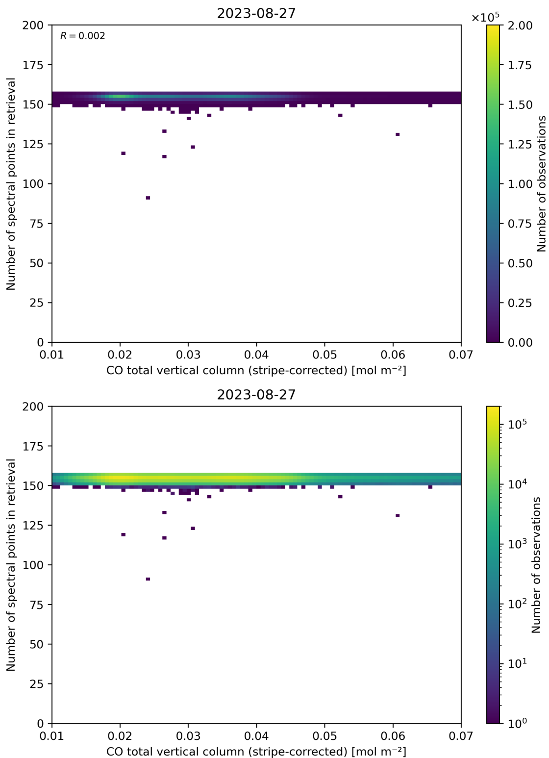
Figure 40: Scatter density plot of “CO total vertical column (stripe-corrected)” against “Number of spectral points in retrieval” for 2023-08-26 to 2023-08-28.
