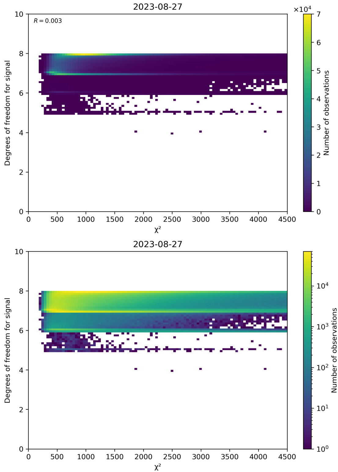
Figure 48: Scatter density plot of “ \chi^2 ” against “Degrees of freedom for signal” for 2023-08-26 to 2023-08-28.
