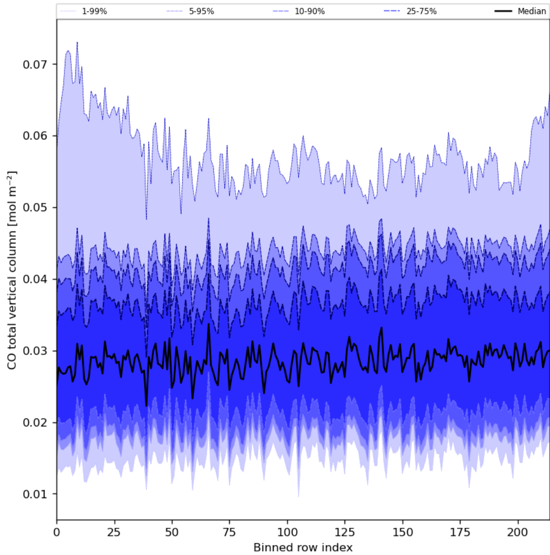
Figure 26: Along track statistics of “CO total vertical column” for 2023-08-26 to 2023-08-28
