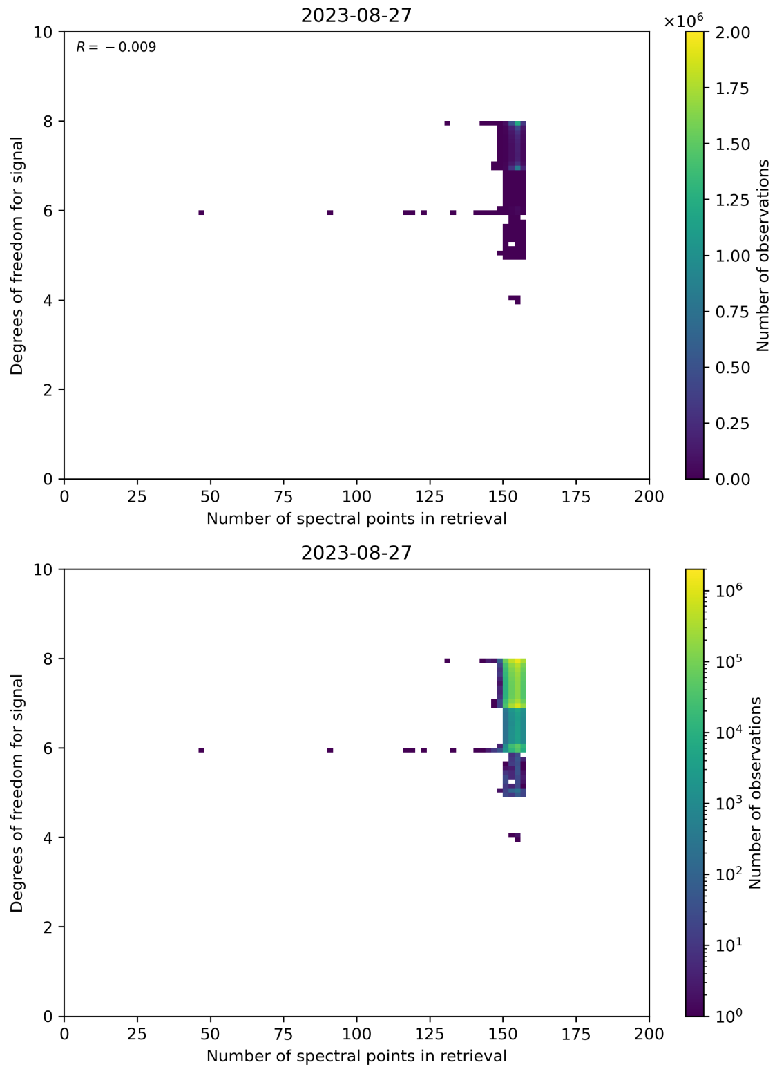
Figure 59: Scatter density plot of “Number of spectral points in retrieval” against “Degrees of freedom for signal” for 2023-08-26 to 2023-08-28.
