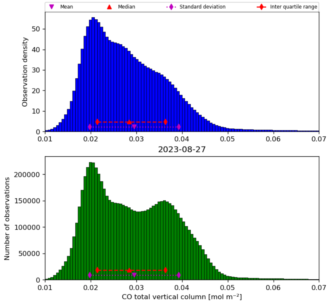
Figure 18: Histogram of “CO total vertical column” for 2023-08-26 to 2023-08-28
