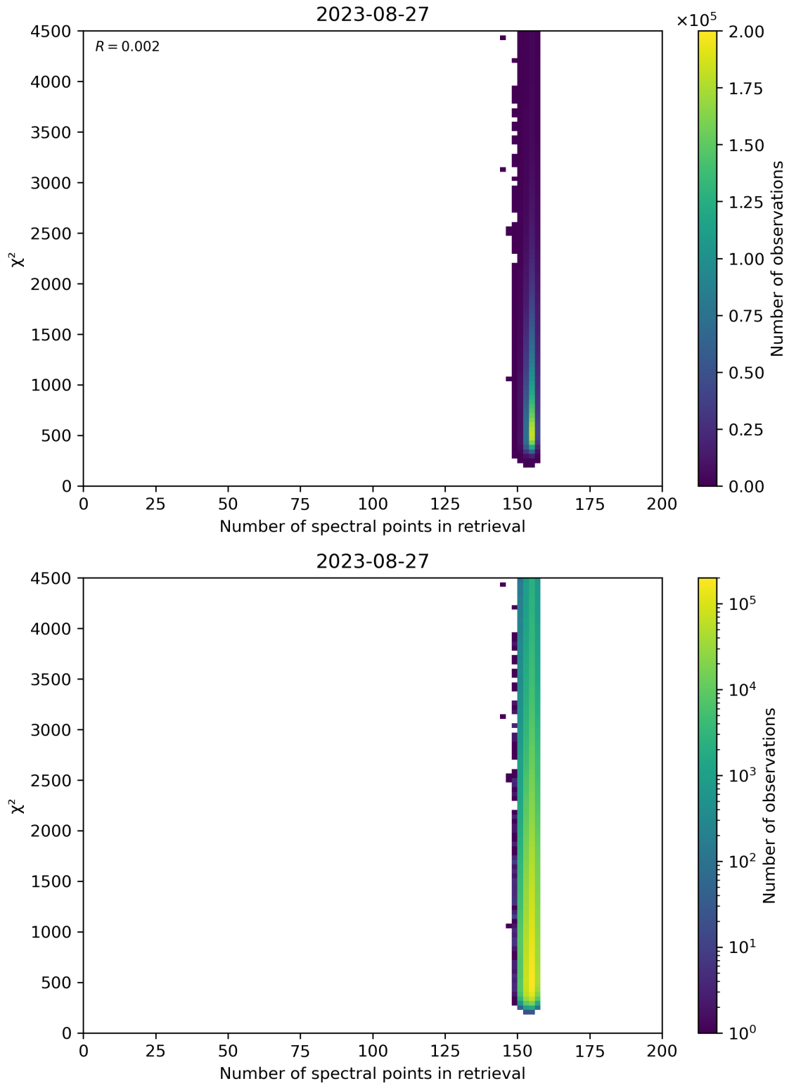
Figure 58: Scatter density plot of “Number of spectral points in retrieval” against “ \chi^2 ” for 2023-08-26 to 2023-08-28.
