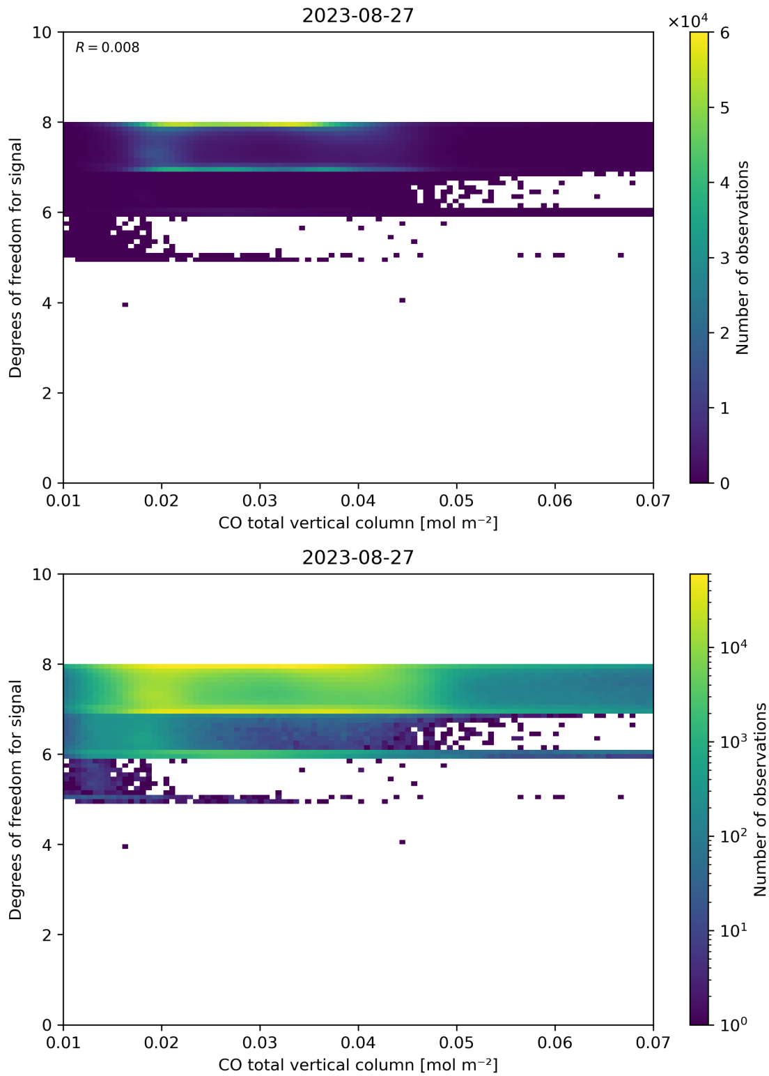
Figure 41: Scatter density plot of “CO total vertical column” against “Degrees of freedom for signal” for 2023-08-26 to 2023-08-28.
