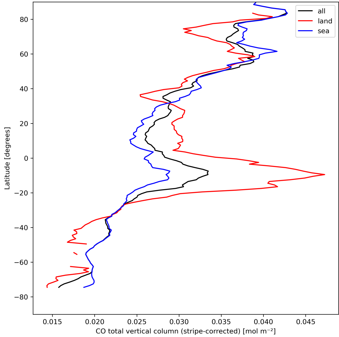
Figure 11: Zonal average of “CO total vertical column (stripe-corrected)” for 2023-08-26 to 2023-08-28.
