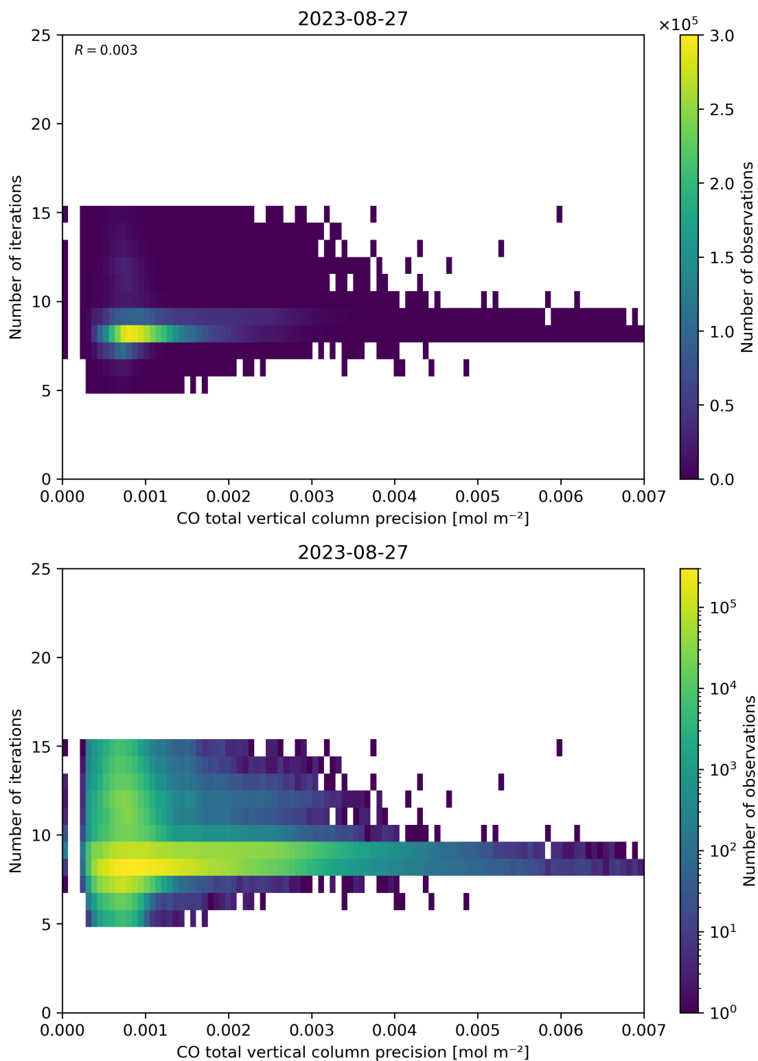
Figure 46: Scatter density plot of “CO total vertical column precision” against “Number of iterations” for 2023-08-26 to 2023-08-28.
