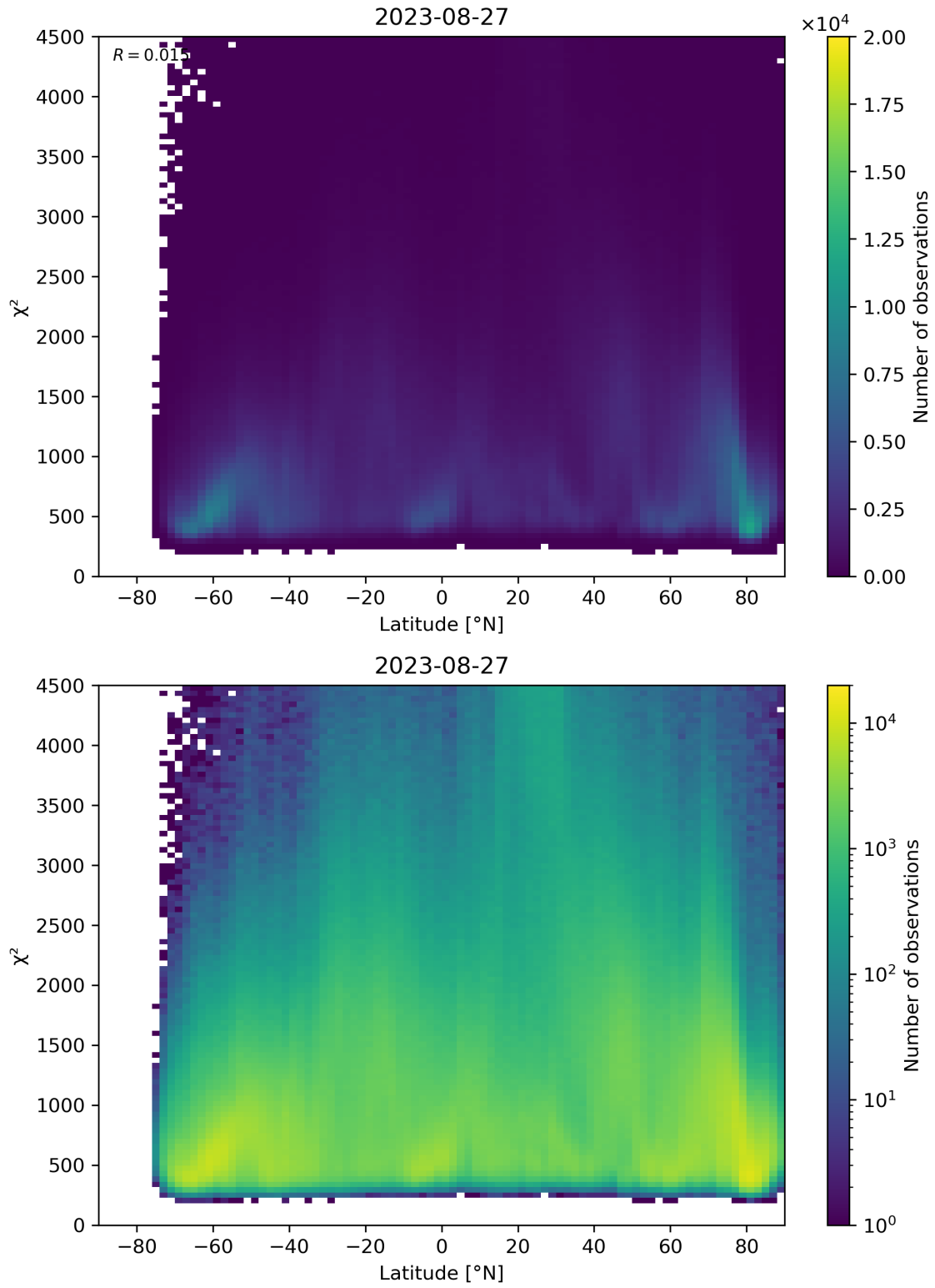
Figure 54: Scatter density plot of “Latitude” against “ \chi^2 ” for 2023-08-26 to 2023-08-28.
