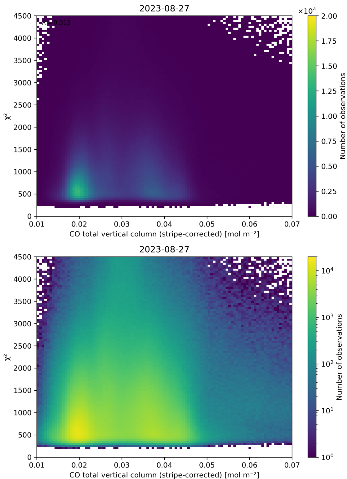
Figure 37: Scatter density plot of “CO total vertical column (stripe-corrected)” against “ \chi^2 ” for 2023-08-26 to 2023-08-28.
