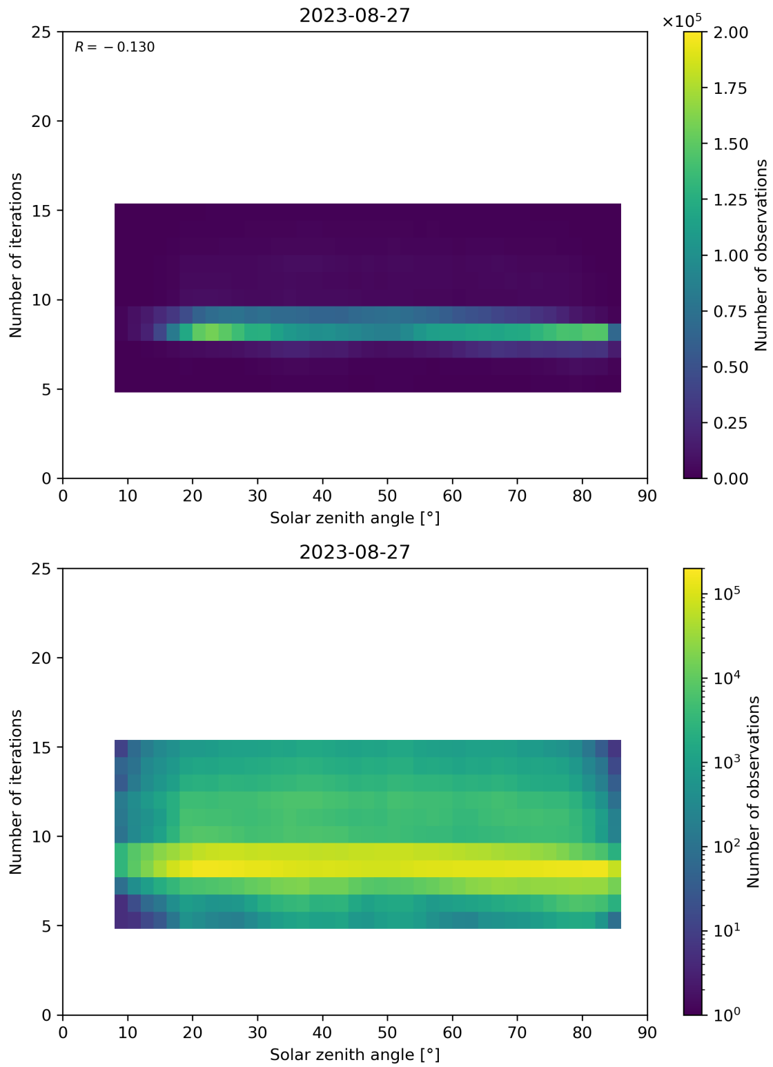
Figure 67: Scatter density plot of “Solar zenith angle” against “Number of iterations” for 2023-08-26 to 2023-08-28.
