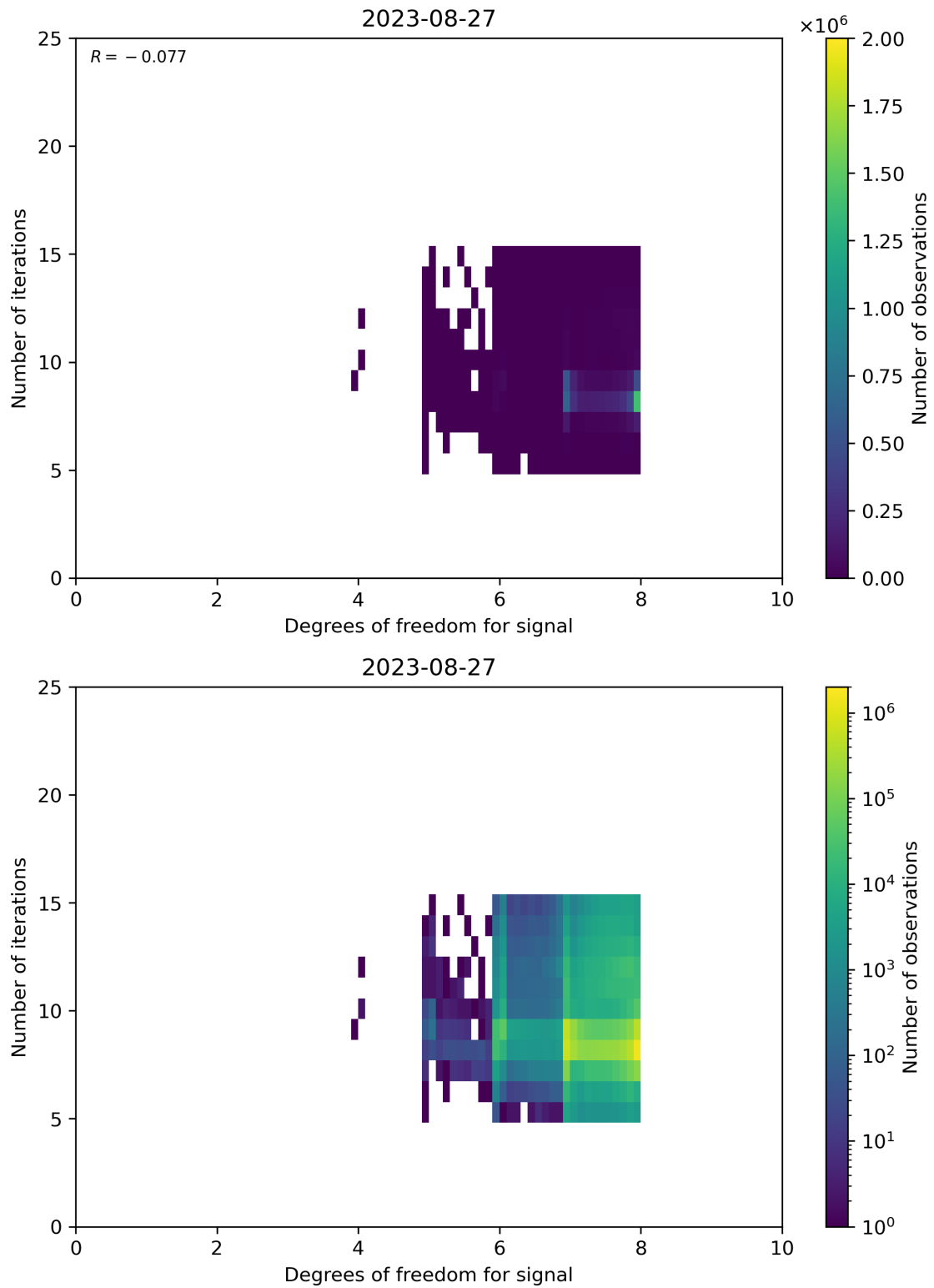
Figure 50: Scatter density plot of “Degrees of freedom for signal” against “Number of iterations” for 2023-08-26 to 2023-08-28.
