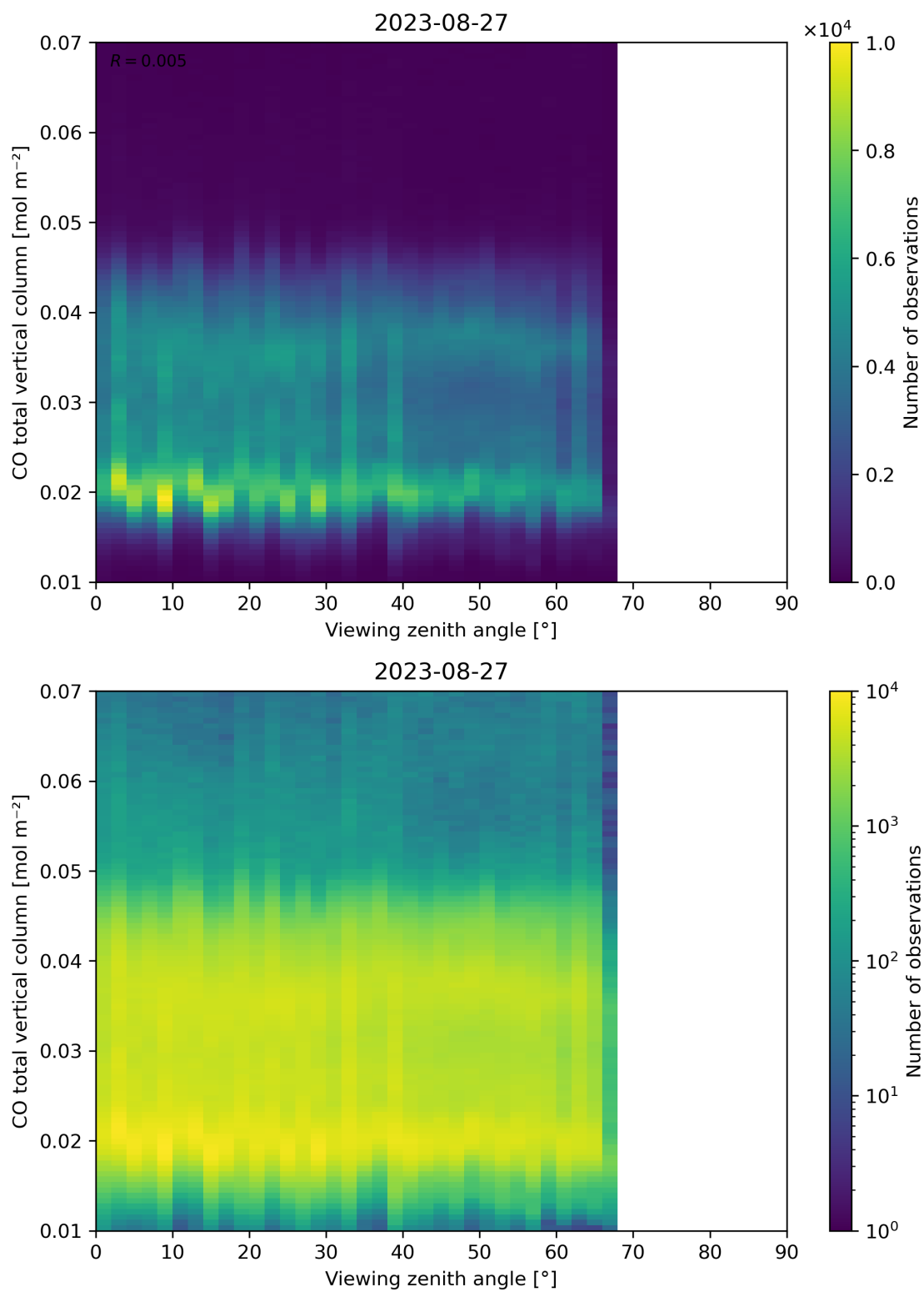
Figure 69: Scatter density plot of “Viewing zenith angle” against “CO total vertical column” for 2023-08-26 to 2023-08-28.
