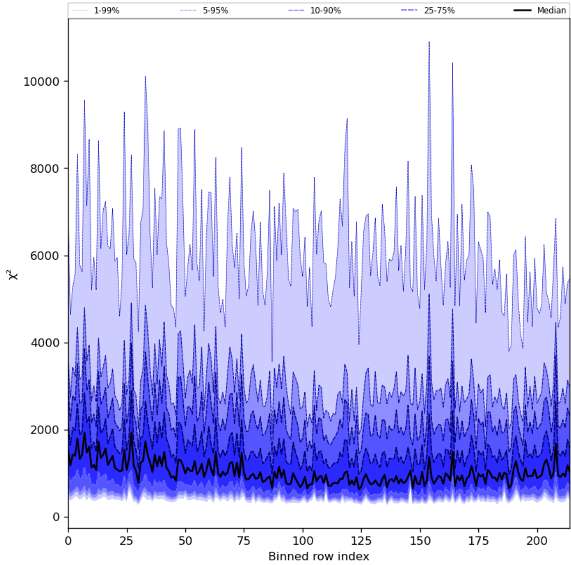
Figure 30: Along track statistics of “ \chi^2 ” for 2023-08-26 to 2023-08-28
