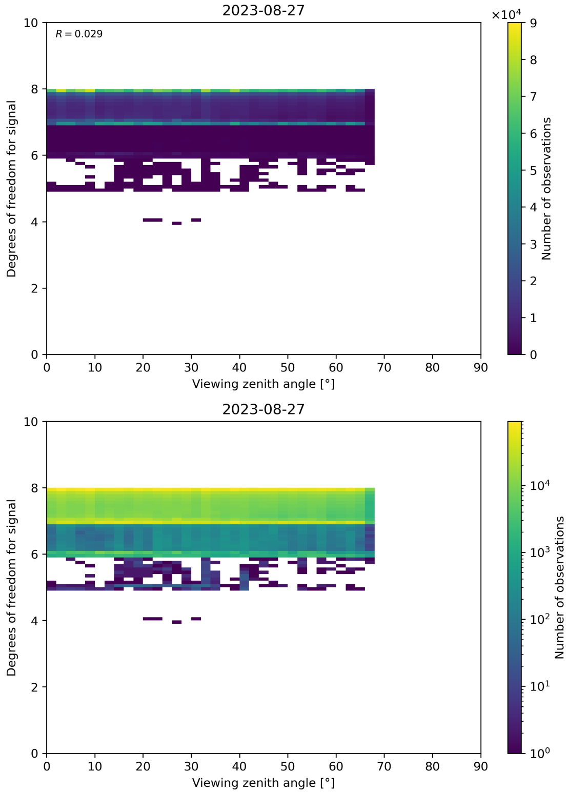
Figure 73: Scatter density plot of “Viewing zenith angle” against “Degrees of freedom for signal” for 2023-08-26 to 2023-08-28.
