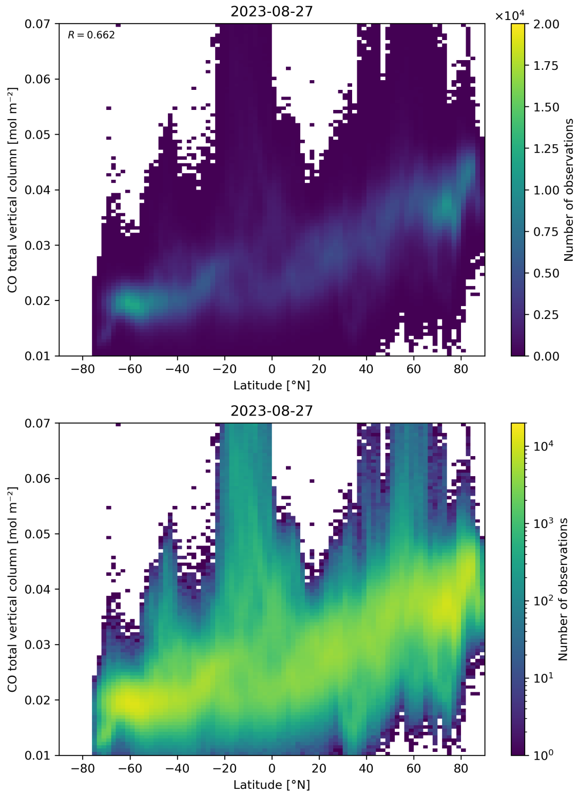
Figure 51: Scatter density plot of “Latitude” against “CO total vertical column” for 2023-08-26 to 2023-08-28.
