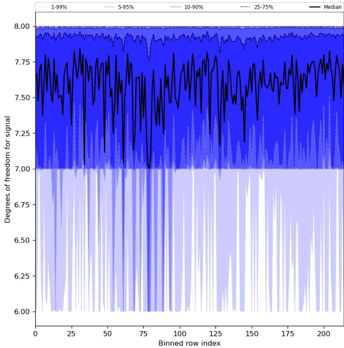
Figure 31: Along track statistics of “Degrees of freedom for signal” for 2023-08-26 to 2023-08-28
