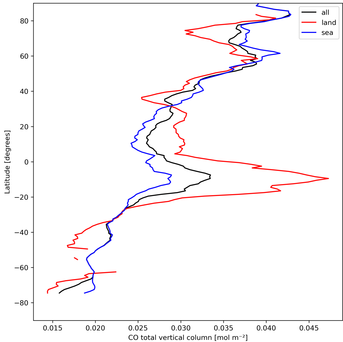
Figure 10: Zonal average of “CO total vertical column” for 2023-08-26 to 2023-08-28.
