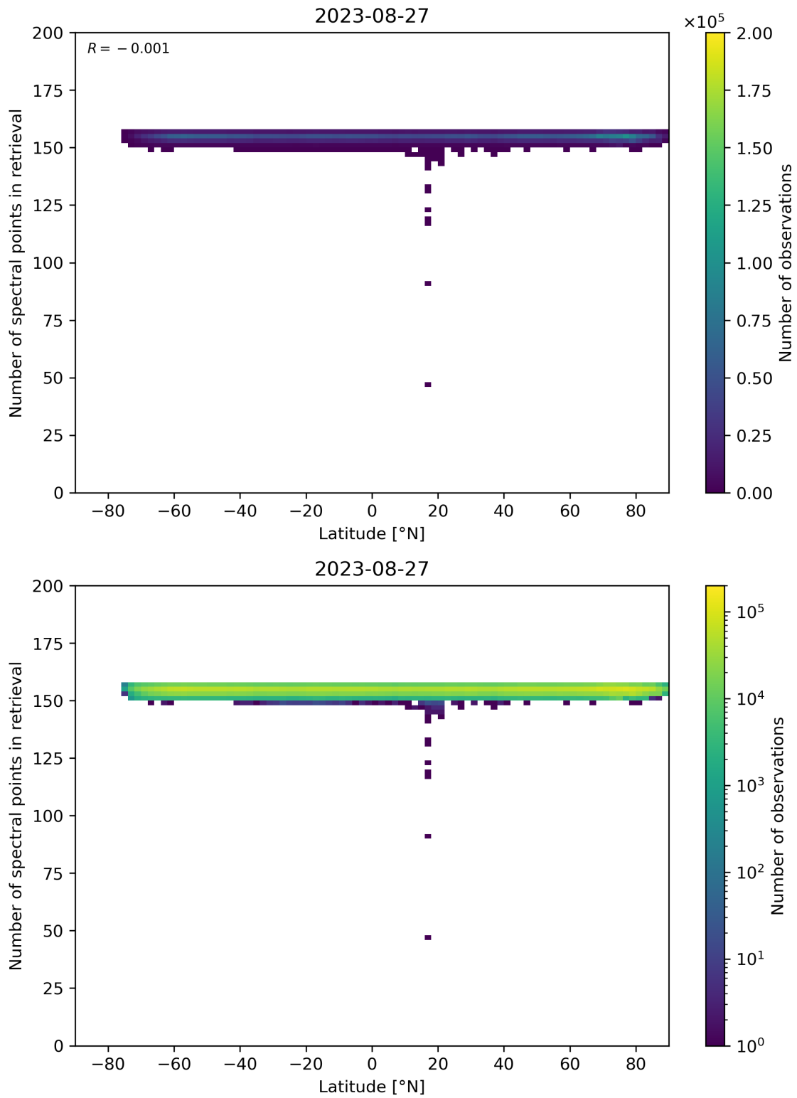
Figure 57: Scatter density plot of “Latitude” against “Number of spectral points in retrieval” for 2023-08-26 to 2023-08-28.
