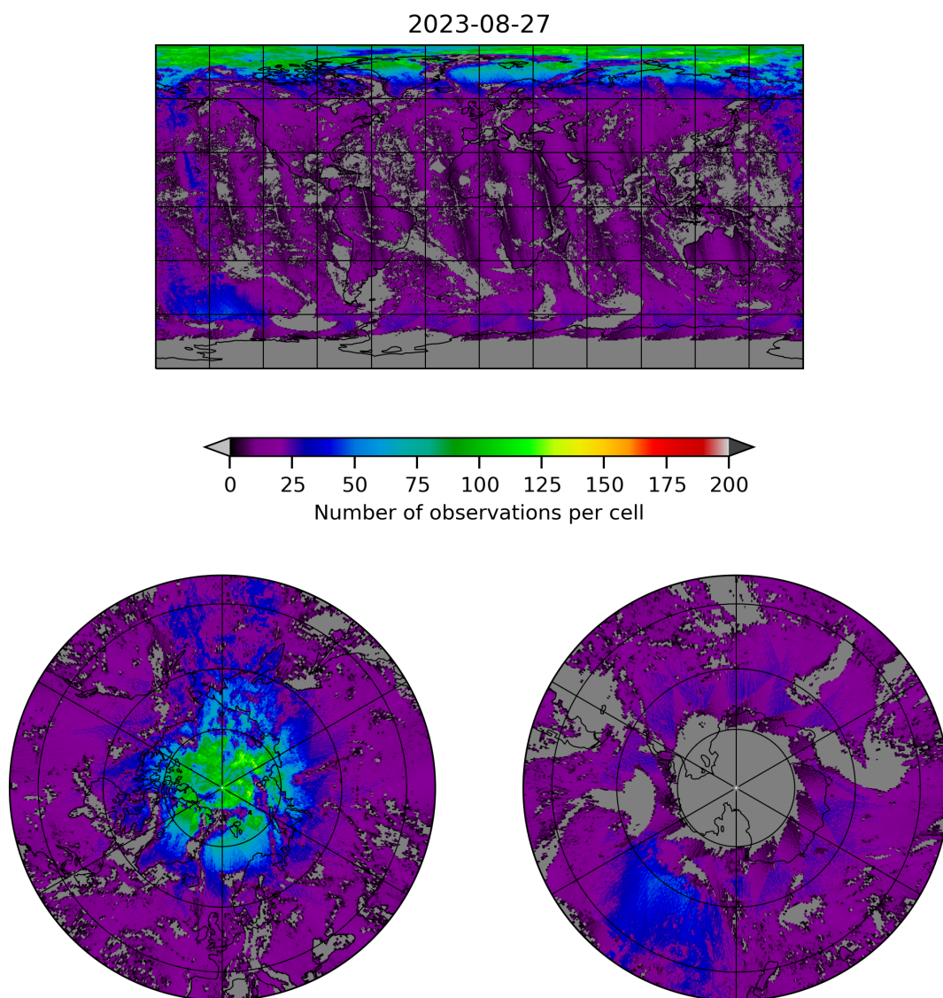
Figure 8: Map of the number of observations for 2023-08-26 to 2023-08-28
