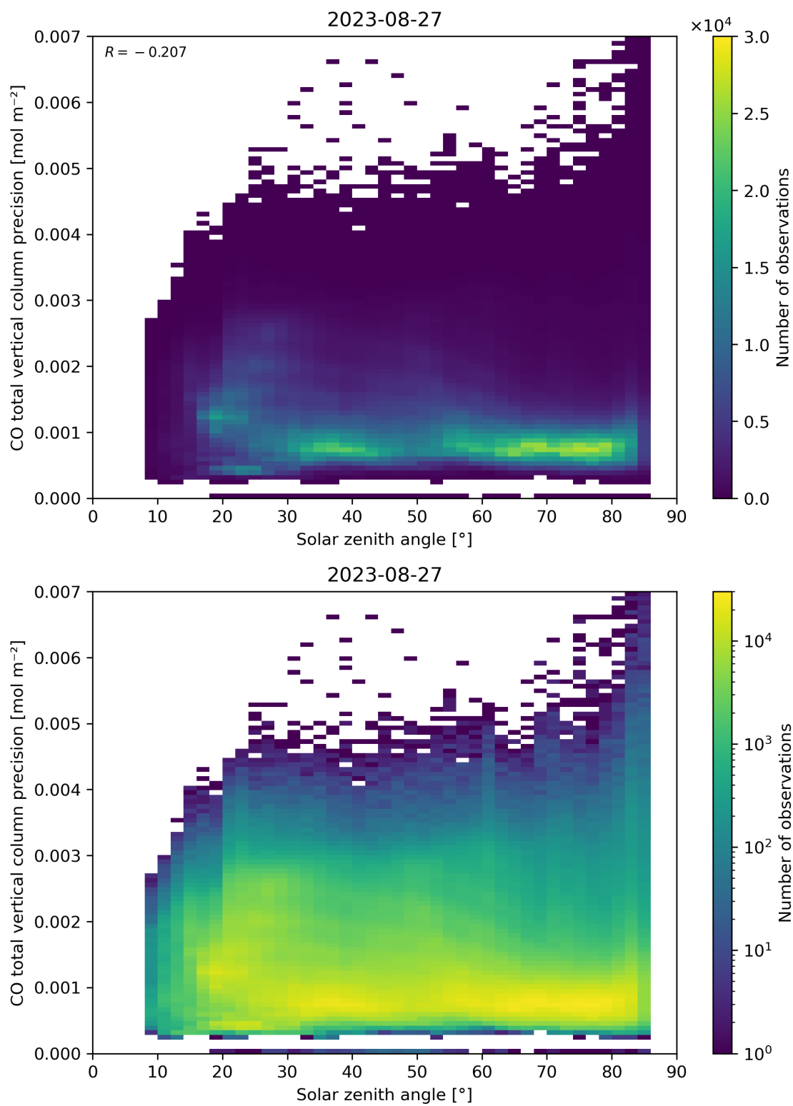
Figure 63: Scatter density plot of “Solar zenith angle” against “CO total vertical column precision” for 2023-08-26 to 2023-08-28.
