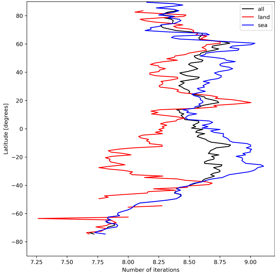
Figure 16: Zonal average of “Number of iterations” for 2023-08-26 to 2023-08-28.
