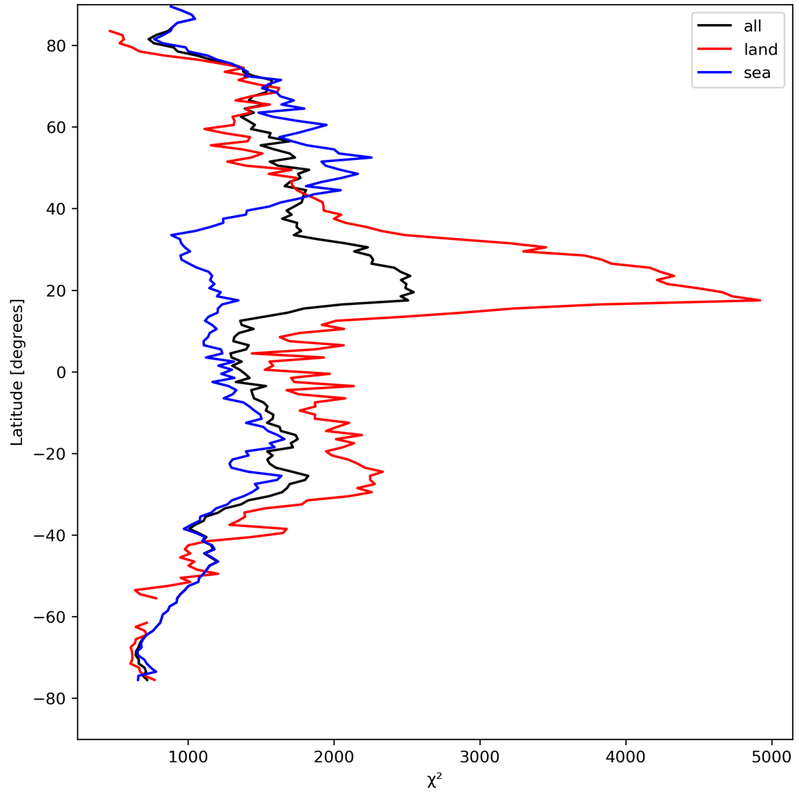
Figure 14: Zonal average of “ \chi^2 ” for 2023-08-27 to 2023-08-29.
