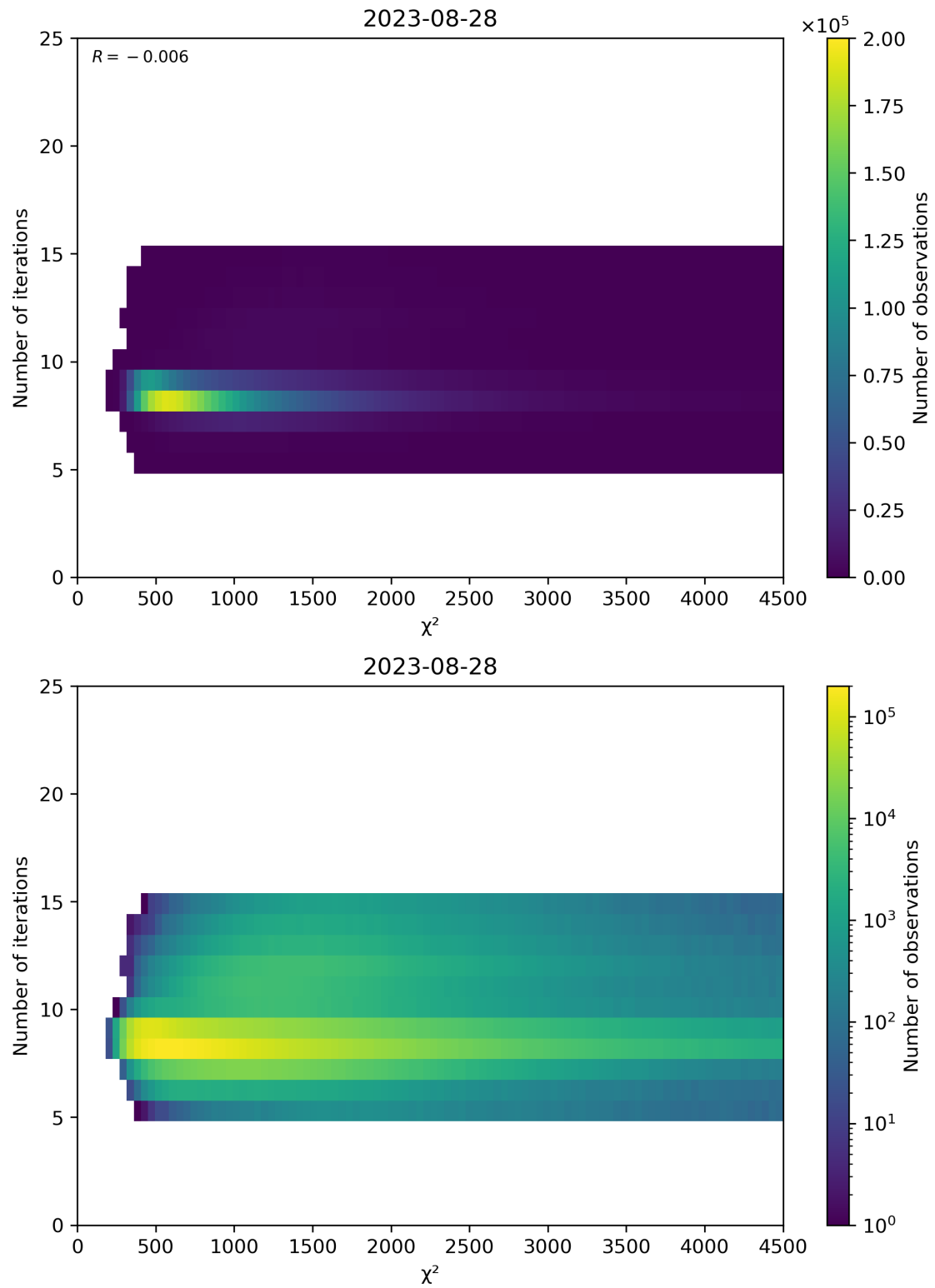
Figure 49: Scatter density plot of “ \chi^2 ” against “Number of iterations” for 2023-08-27 to 2023-08-29.
