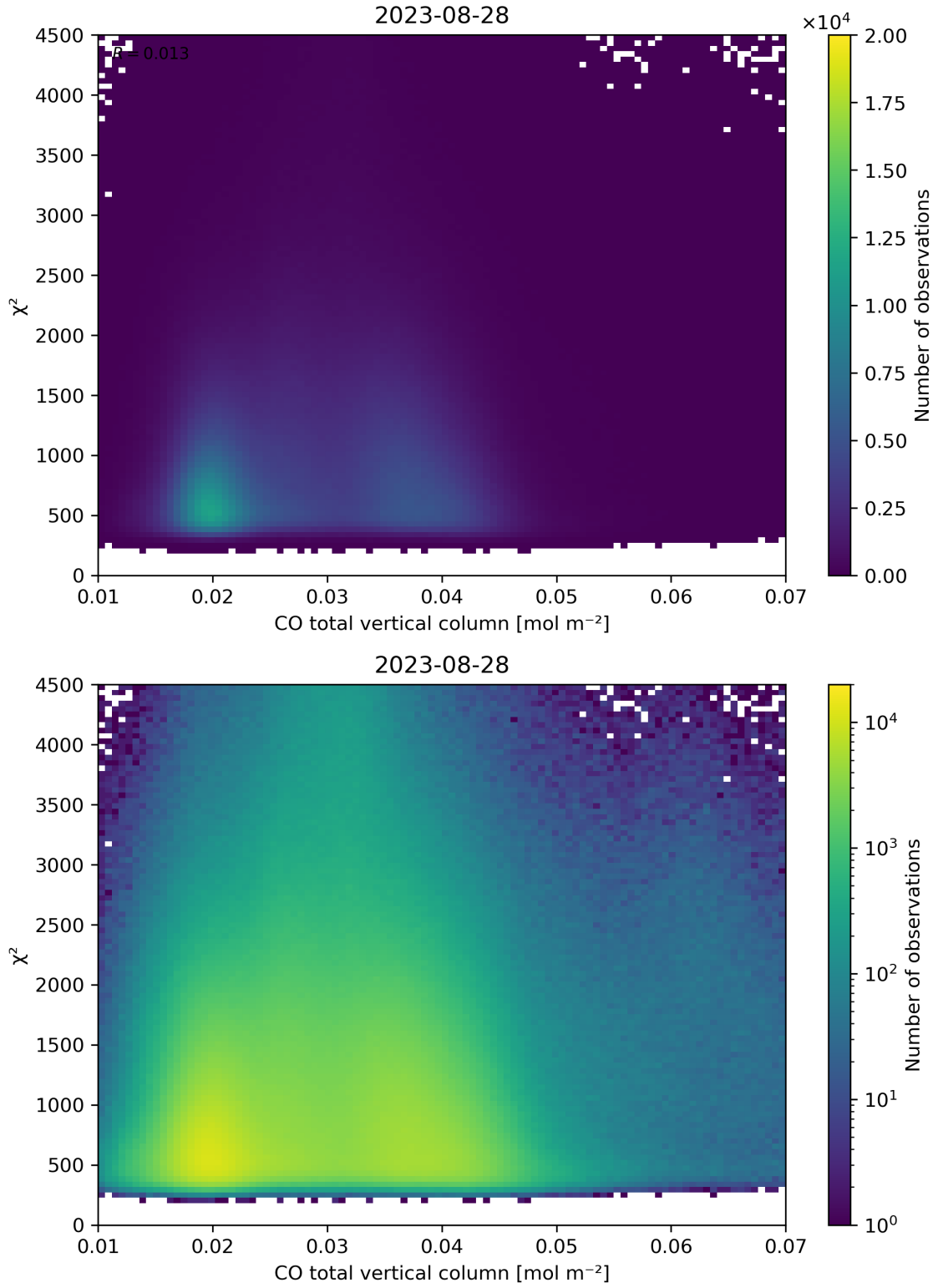
Figure 35: Scatter density plot of “CO total vertical column” against “ \chi^2 ” for 2023-08-27 to 2023-08-29.
