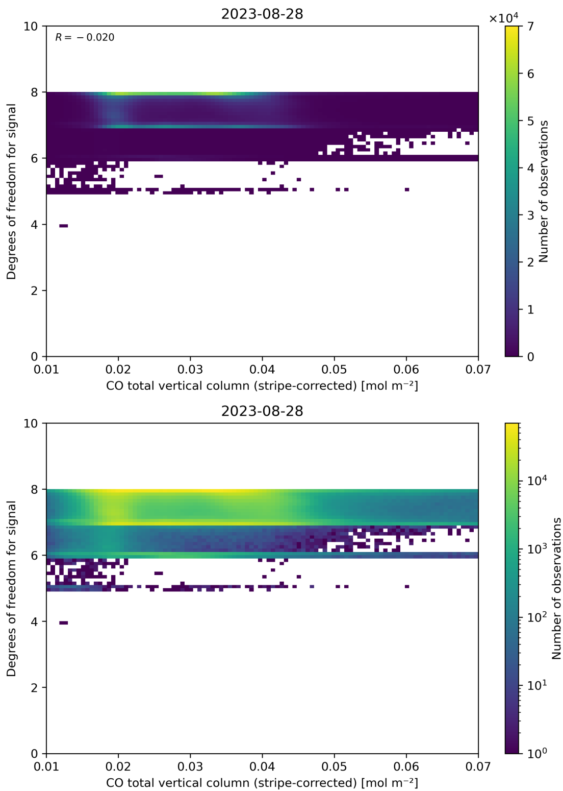
Figure 38: Scatter density plot of “CO total vertical column (stripe-corrected)” against “Degrees of freedom for signal” for 2023-08-27 to 2023-08-29.
