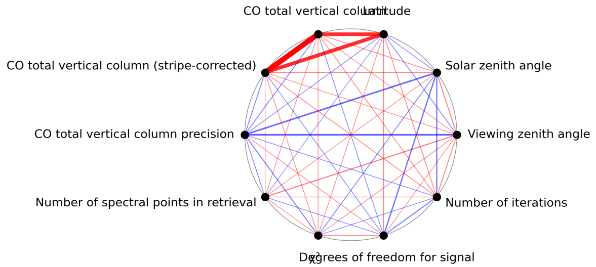
Figure 1: Map of correlation graph for 2023-08-27 to 2023-08-29.
