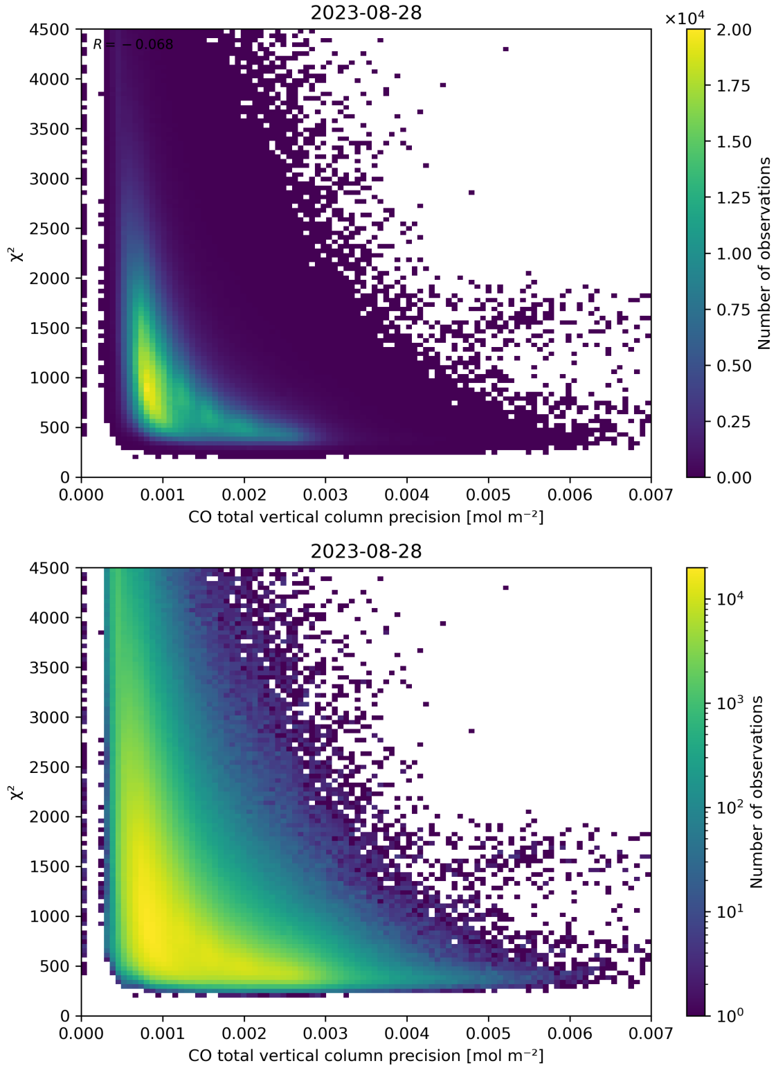
Figure 44: Scatter density plot of “CO total vertical column precision” against “ \chi^2 ” for 2023-08-27 to 2023-08-29.
