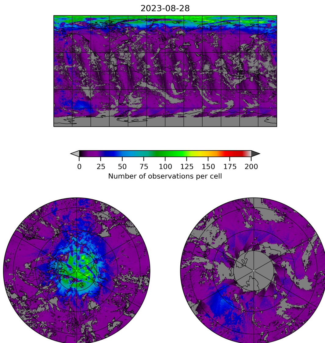
Figure 8: Map of the number of observations for 2023-08-27 to 2023-08-29
