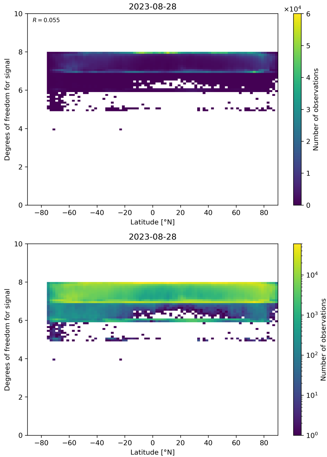
Figure 55: Scatter density plot of “Latitude” against “Degrees of freedom for signal” for 2023-08-27 to 2023-08-29.
