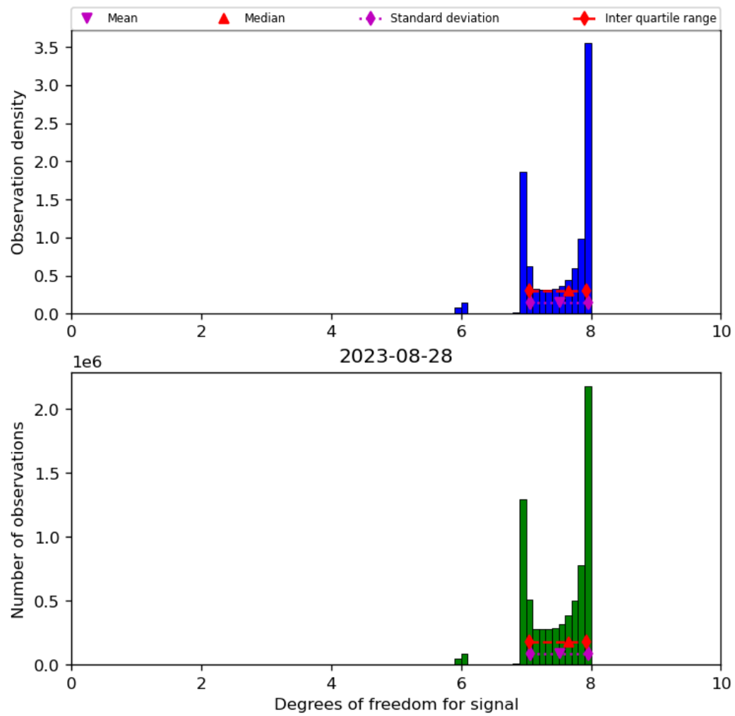
Figure 23: Histogram of “Degrees of freedom for signal” for 2023-08-27 to 2023-08-29
