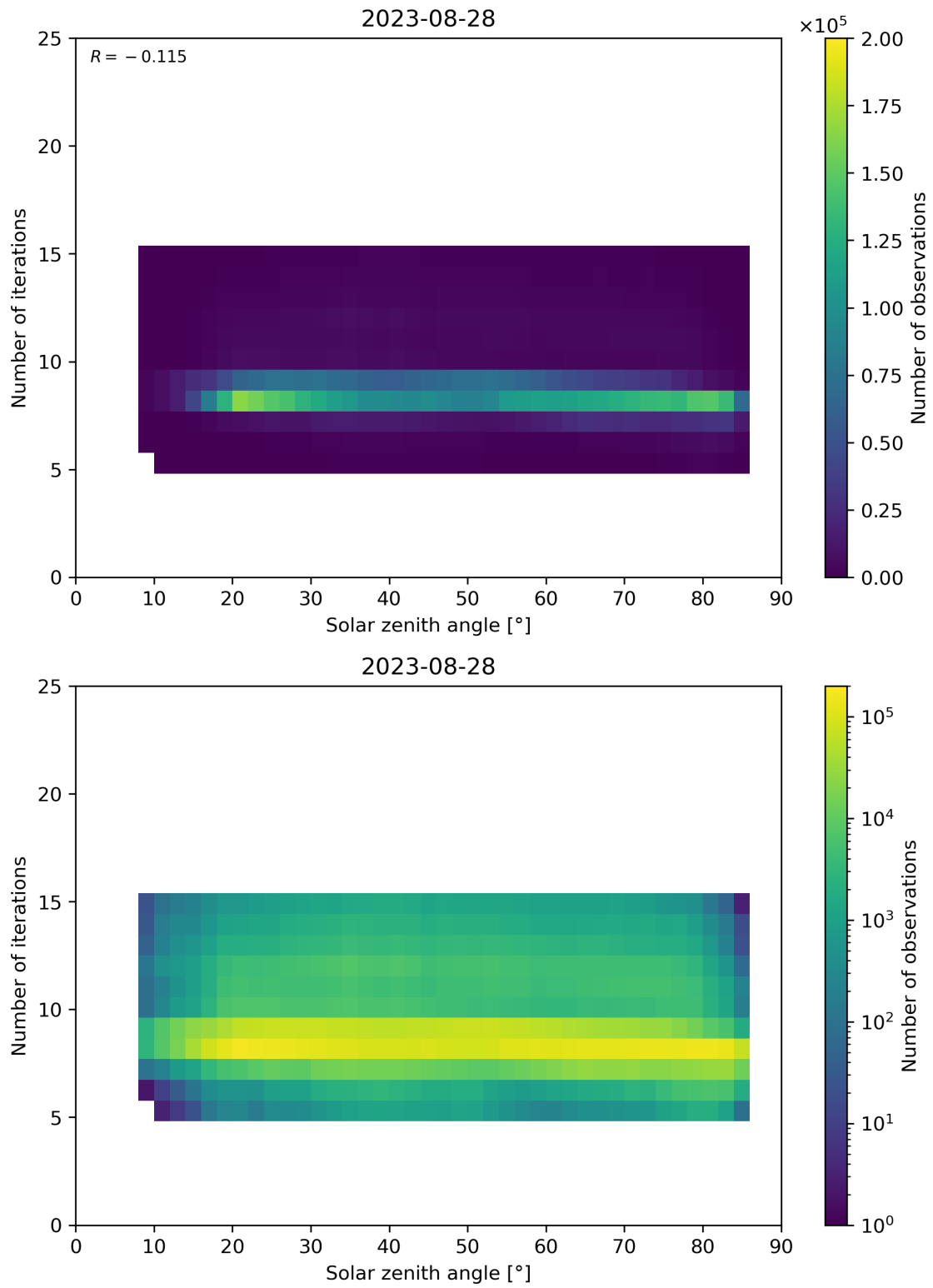
Figure 67: Scatter density plot of “Solar zenith angle” against “Number of iterations” for 2023-08-27 to 2023-08-29.
