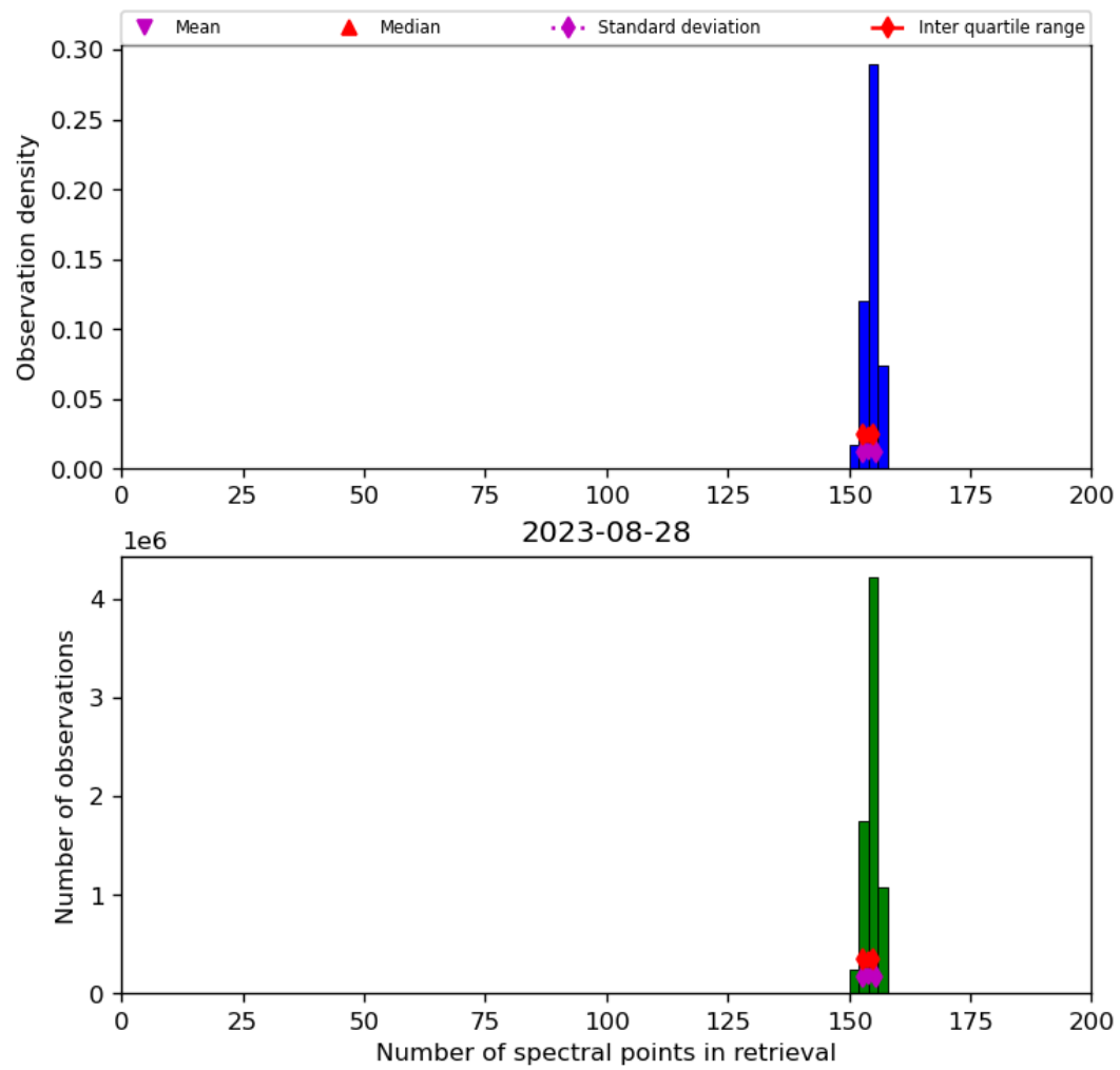
Figure 21: Histogram of “Number of spectral points in retrieval” for 2023-08-27 to 2023-08-29
