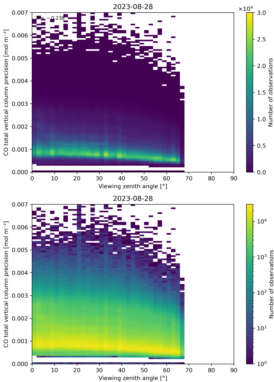
Figure 71: Scatter density plot of “Viewing zenith angle” against “CO total vertical column precision” for 2023-08-27 to 2023-08-29.
