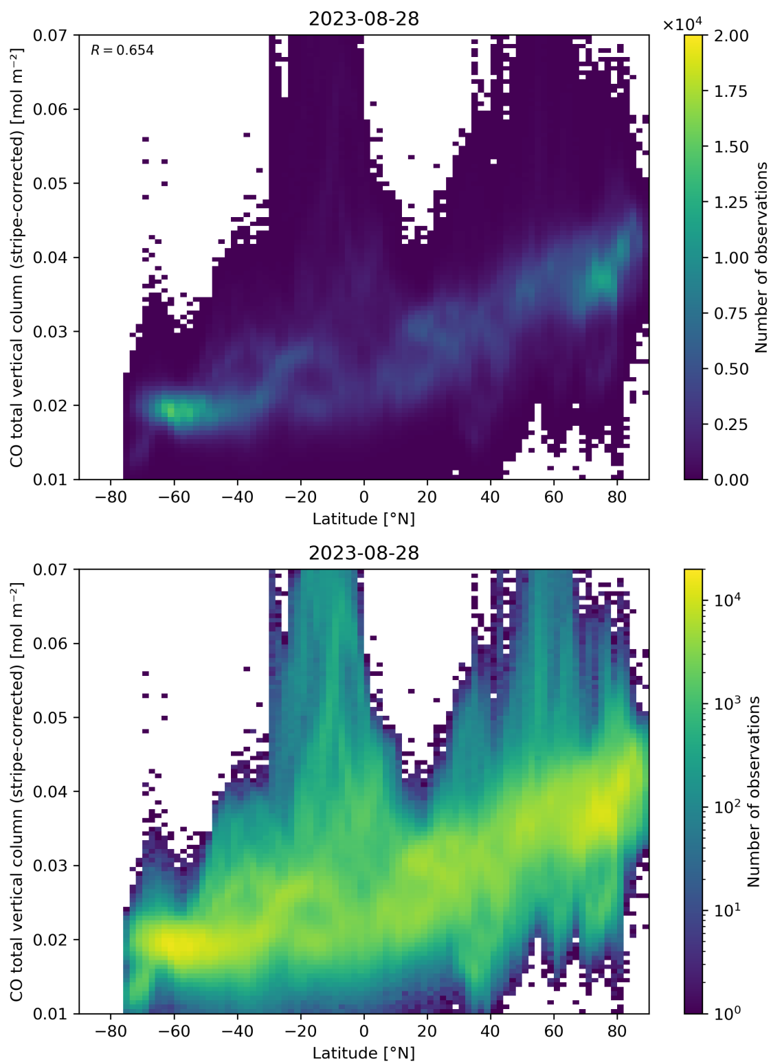
Figure 52: Scatter density plot of “Latitude” against “CO total vertical column (stripe-corrected)” for 2023-08-27 to 2023-08-29.
