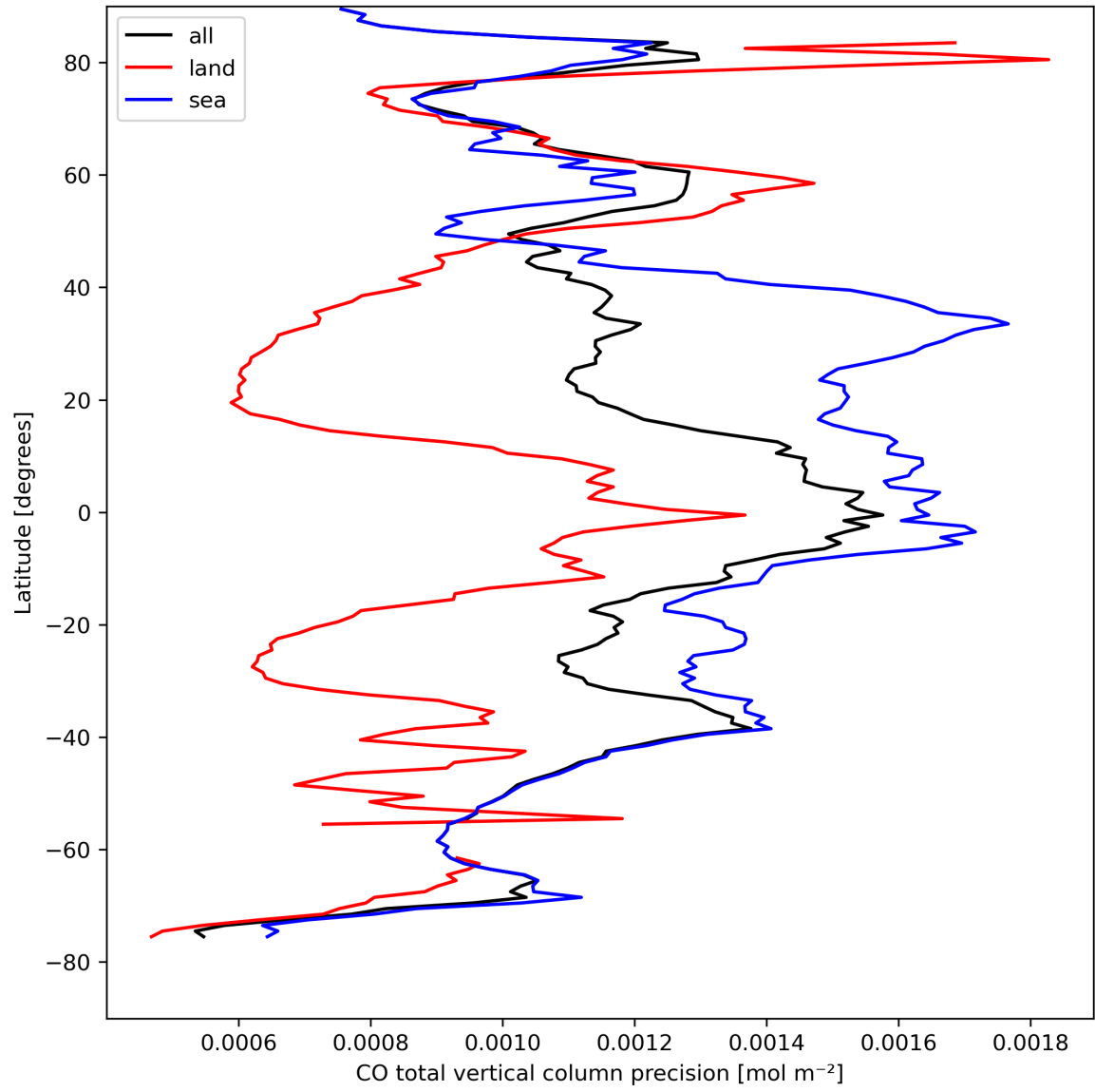
Figure 12: Zonal average of “CO total vertical column precision” for 2023-08-27 to 2023-08-29.
