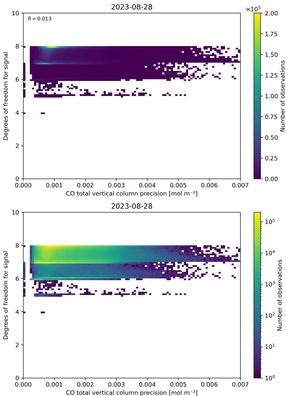
Figure 45: Scatter density plot of “CO total vertical column precision” against “Degrees of freedom for signal” for 2023-08-27 to 2023-08-29.
