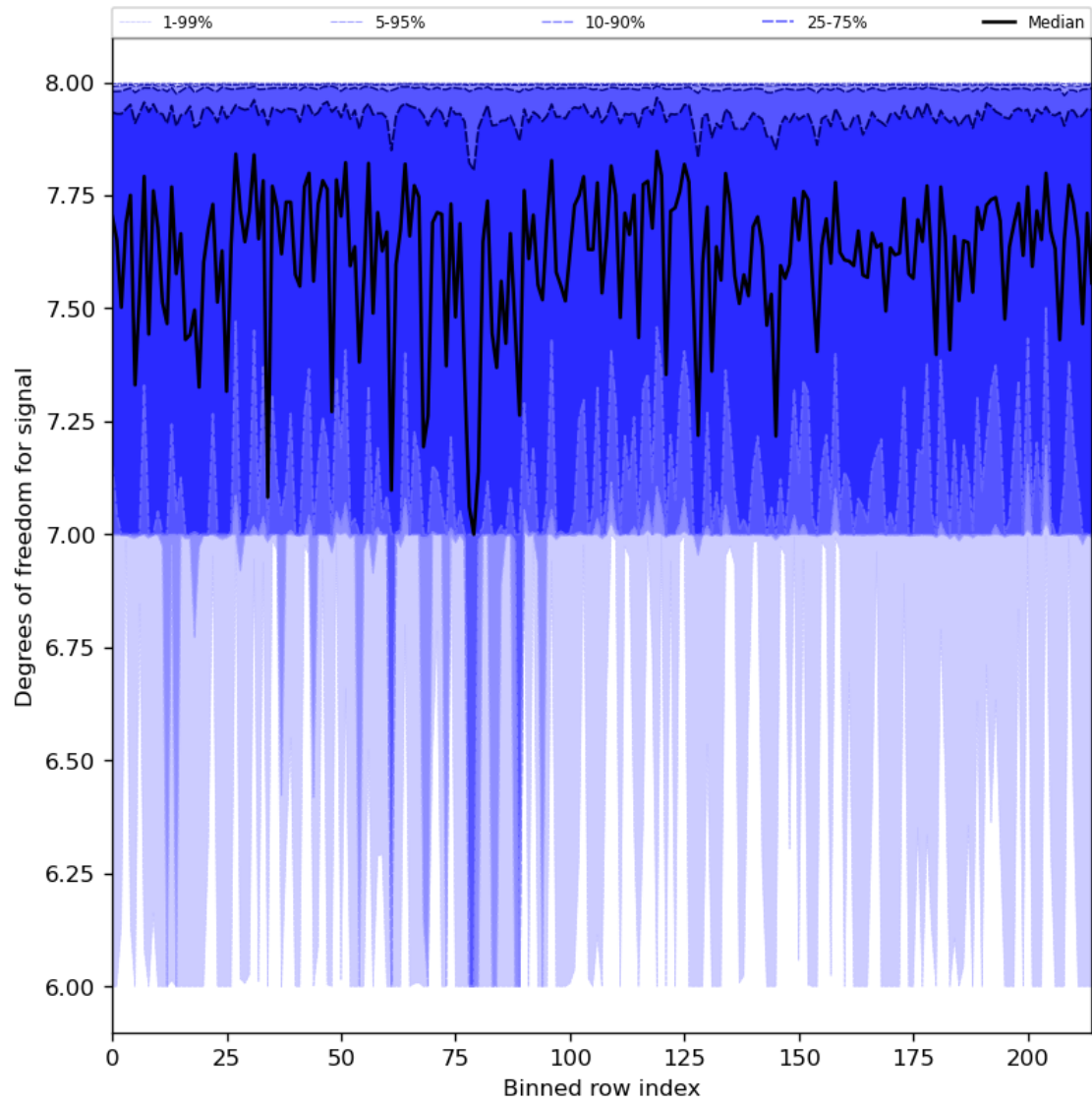
Figure 31: Along track statistics of “Degrees of freedom for signal” for 2023-08-27 to 2023-08-29
