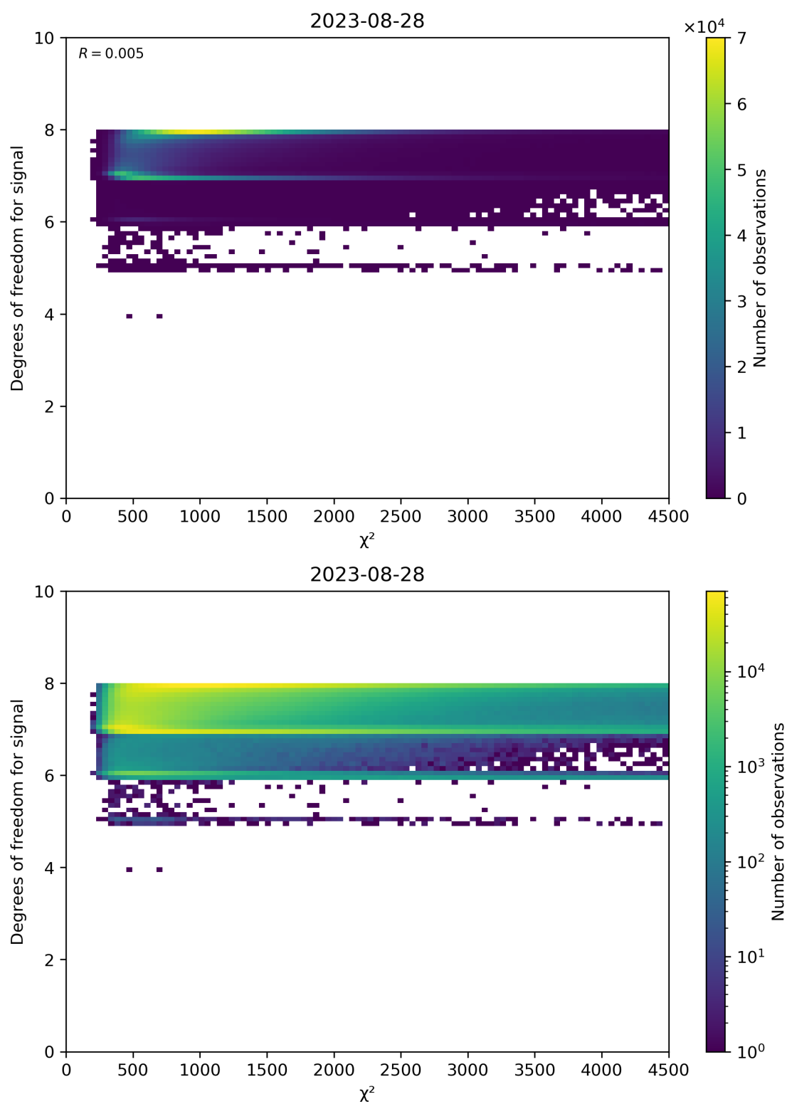
Figure 48: Scatter density plot of “ \chi^2 ” against “Degrees of freedom for signal” for 2023-08-27 to 2023-08-29.
