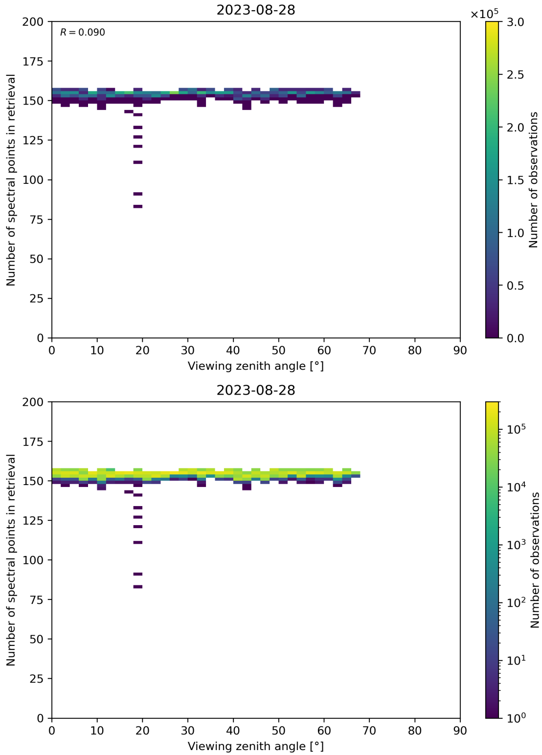
Figure 76: Scatter density plot of “Viewing zenith angle” against “Number of spectral points in retrieval” for 2023-08-27 to 2023-08-29.
