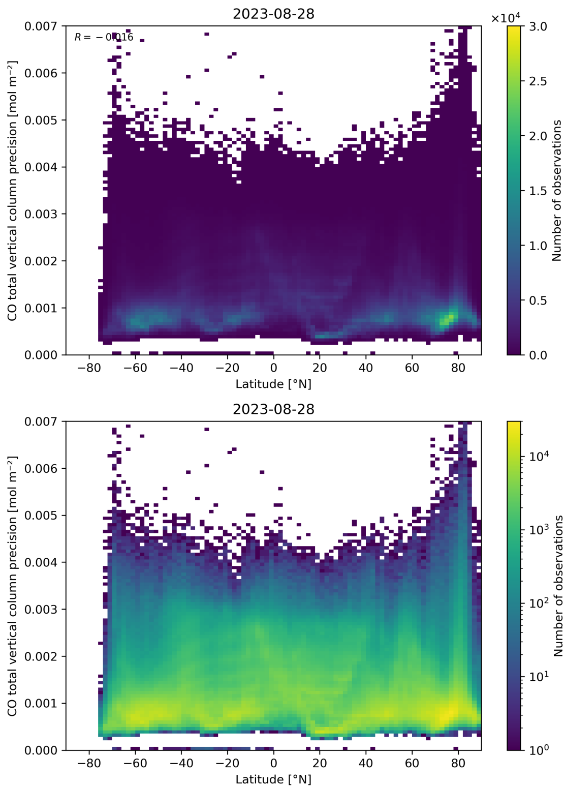
Figure 53: Scatter density plot of “Latitude” against “CO total vertical column precision” for 2023-08-27 to 2023-08-29.
