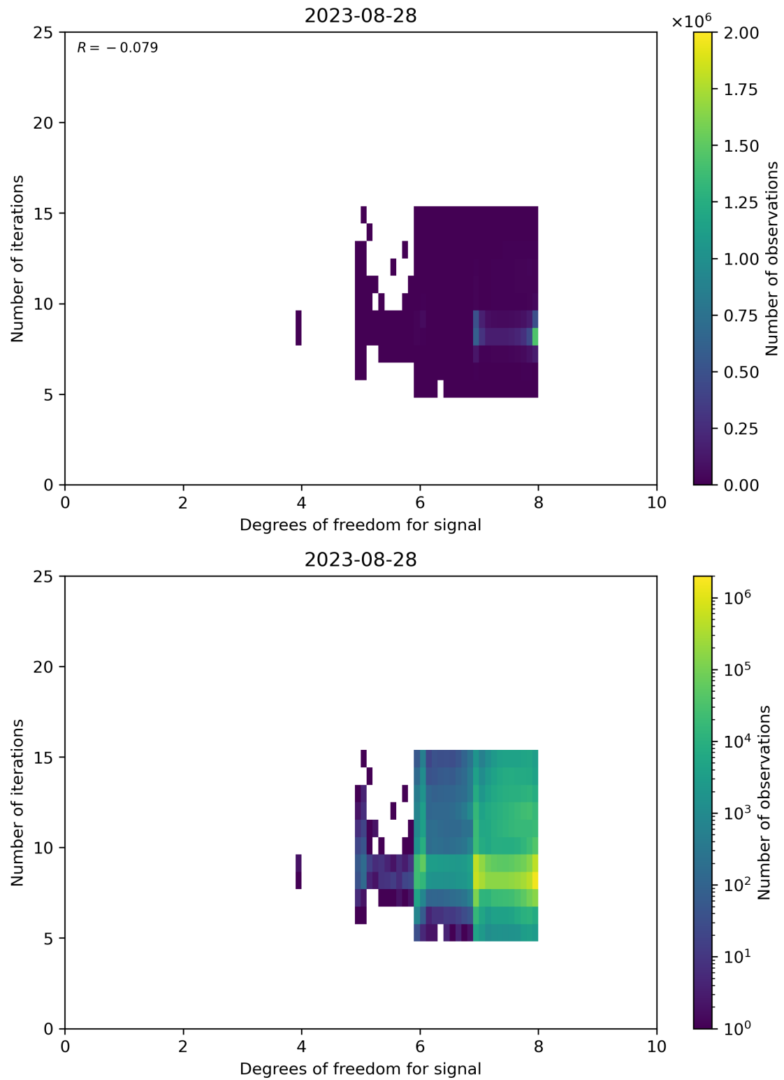
Figure 50: Scatter density plot of “Degrees of freedom for signal” against “Number of iterations” for 2023-08-27 to 2023-08-29.
