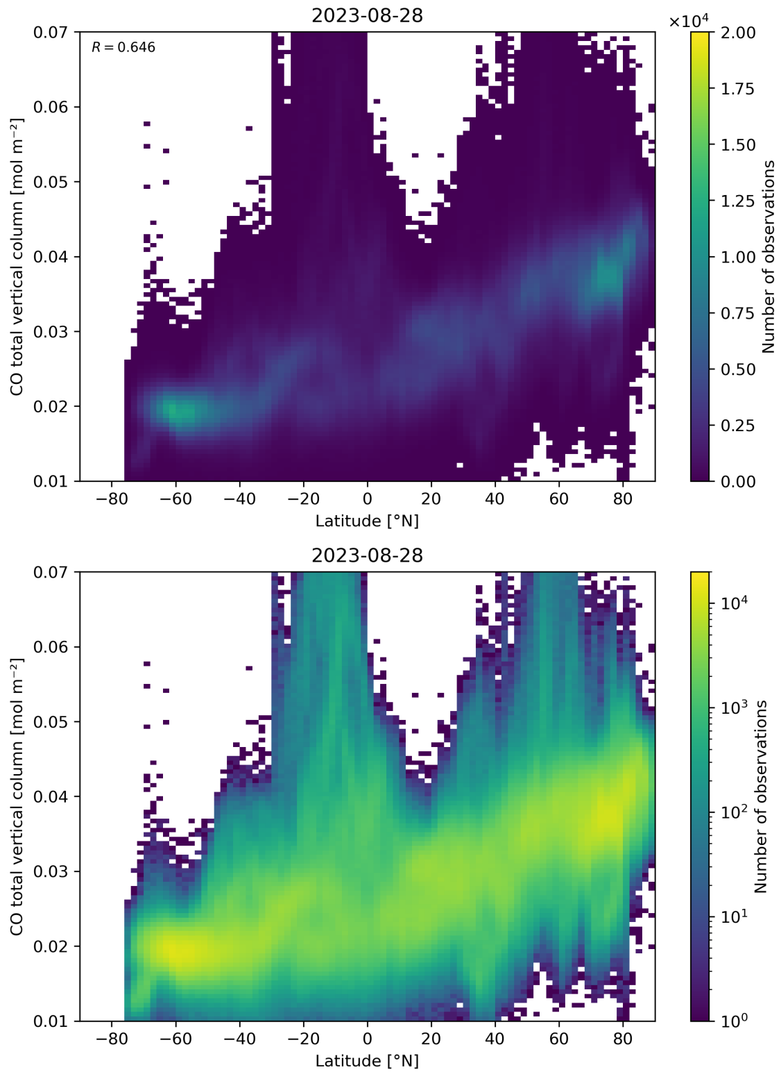
Figure 51: Scatter density plot of “Latitude” against “CO total vertical column” for 2023-08-27 to 2023-08-29.
