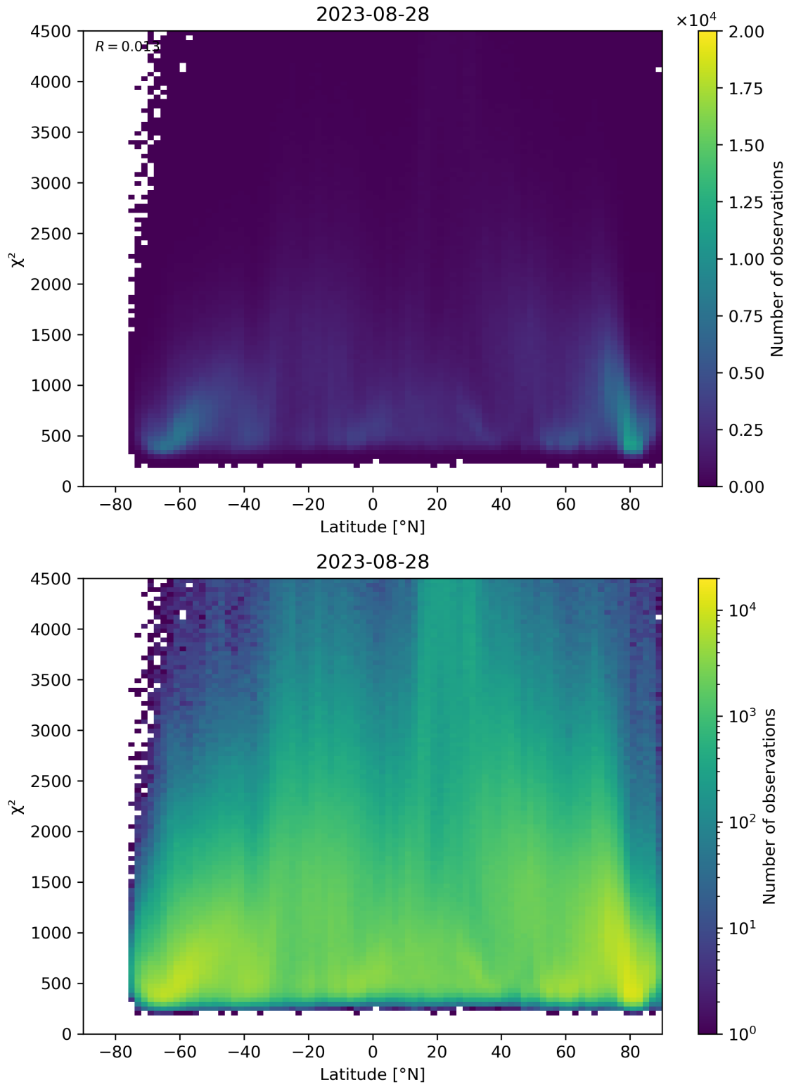
Figure 54: Scatter density plot of “Latitude” against “ \chi^2 ” for 2023-08-27 to 2023-08-29.
