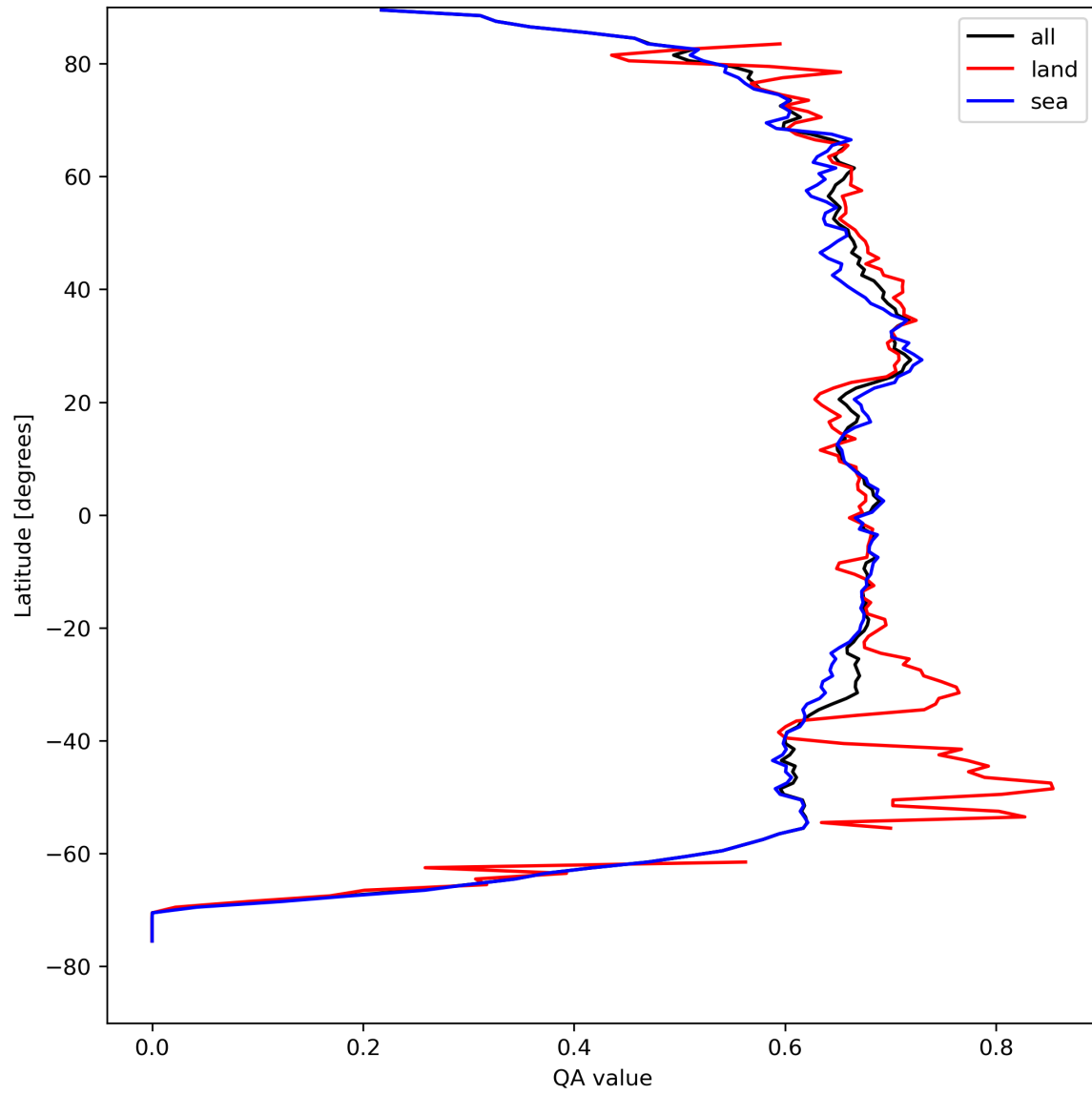
Figure 9: Zonal average of “QA value” for 2023-08-27 to 2023-08-29.
