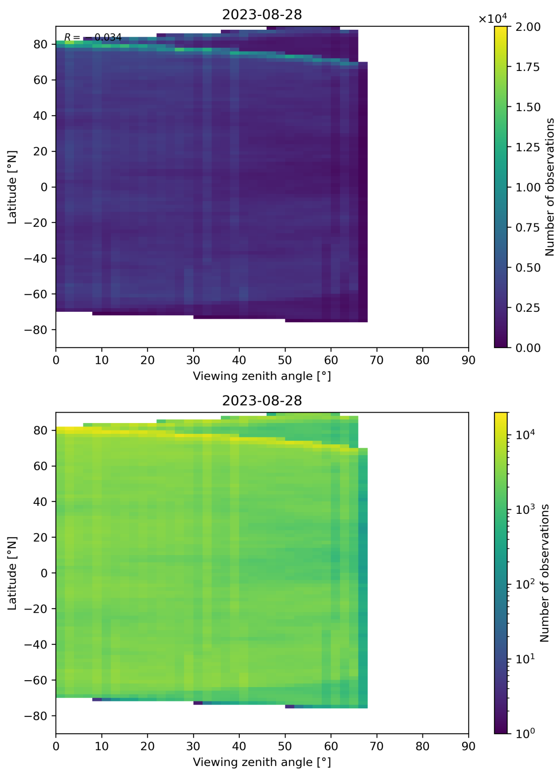
Figure 74: Scatter density plot of “Viewing zenith angle” against “Latitude” for 2023-08-27 to 2023-08-29.
