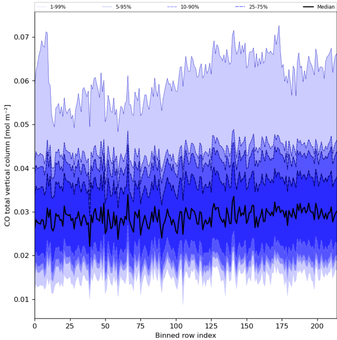
Figure 26: Along track statistics of “CO total vertical column” for 2023-08-27 to 2023-08-29
