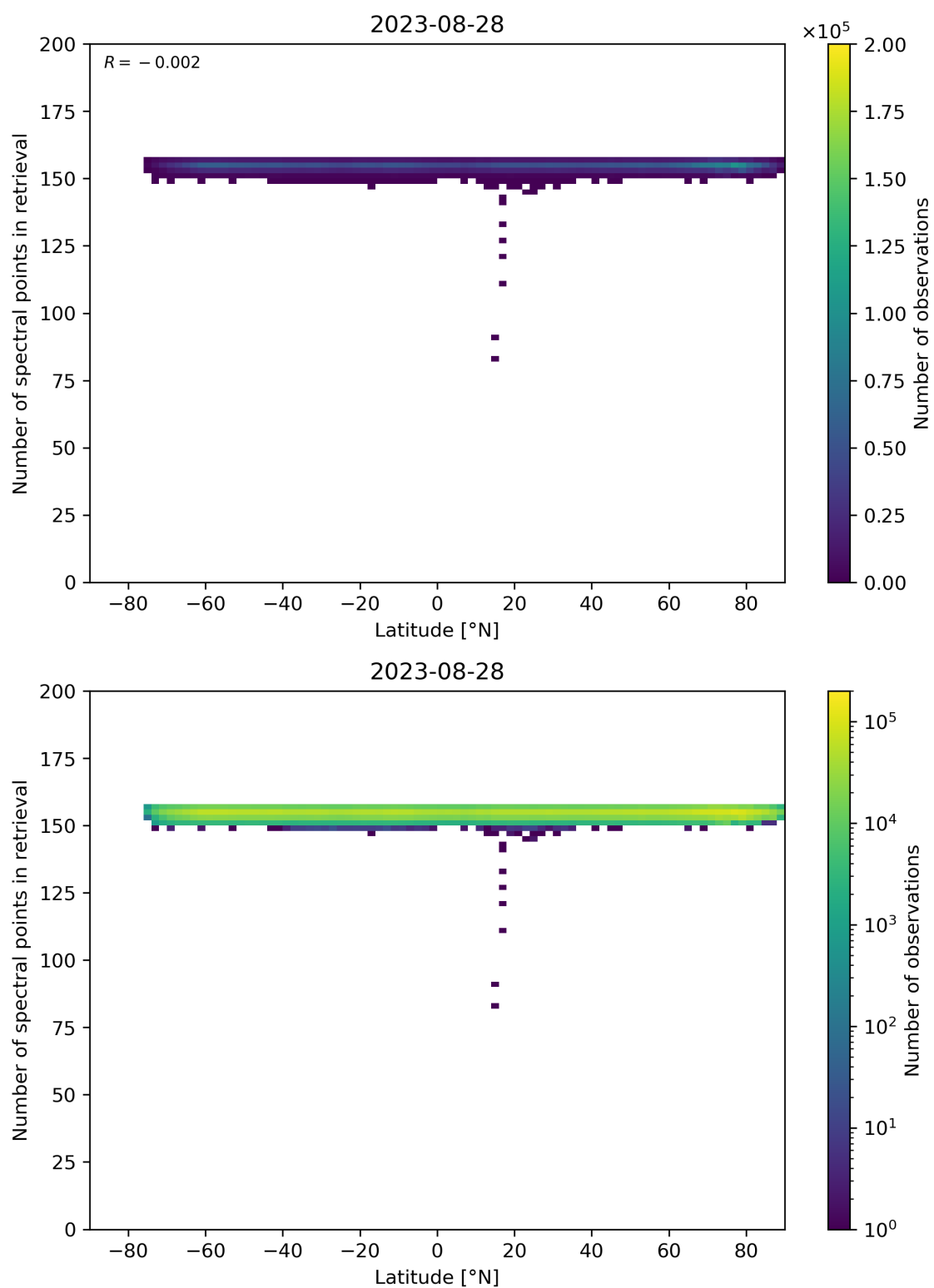
Figure 57: Scatter density plot of “Latitude” against “Number of spectral points in retrieval” for 2023-08-27 to 2023-08-29.
