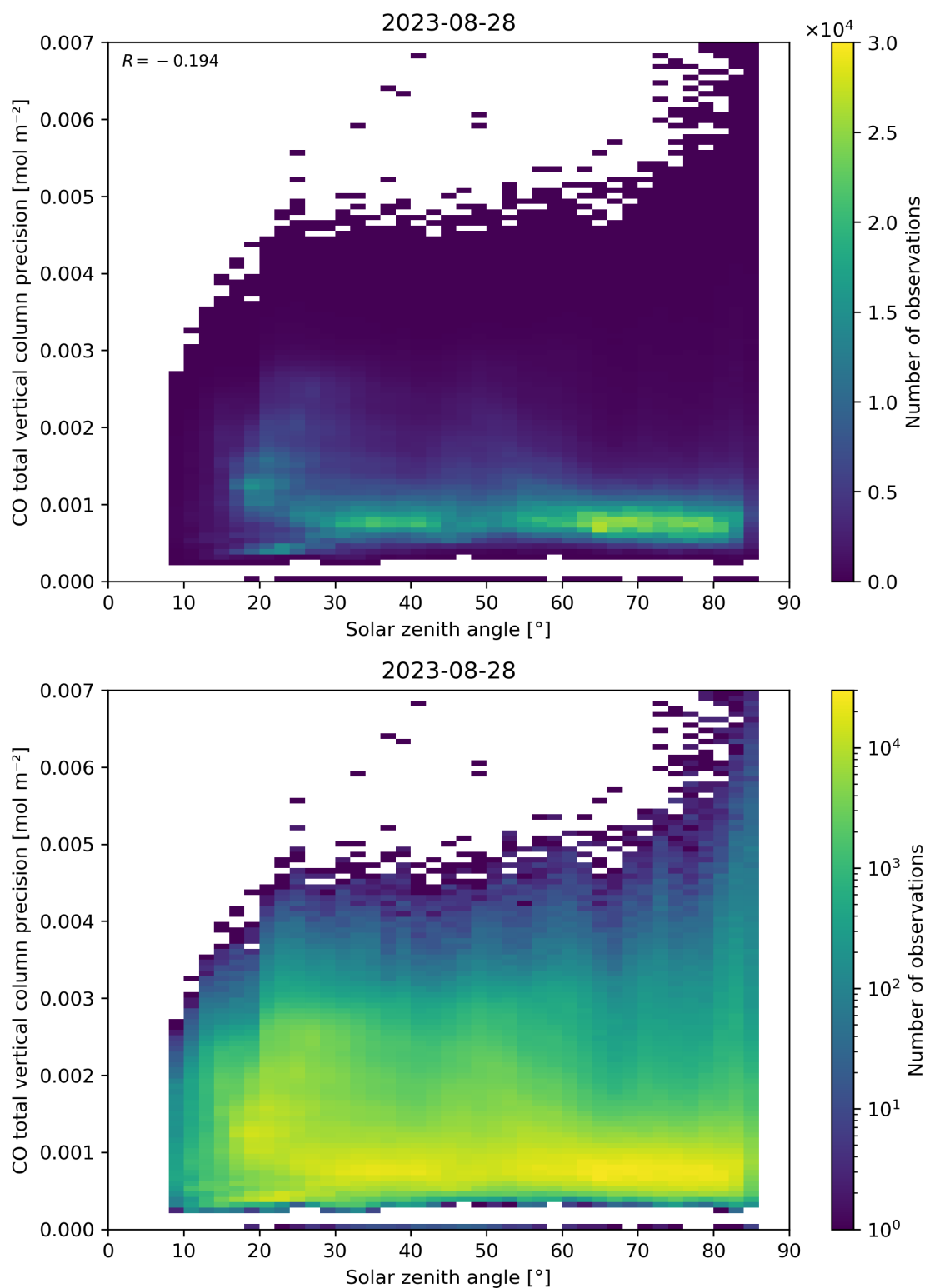
Figure 63: Scatter density plot of “Solar zenith angle” against “CO total vertical column precision” for 2023-08-27 to 2023-08-29.
