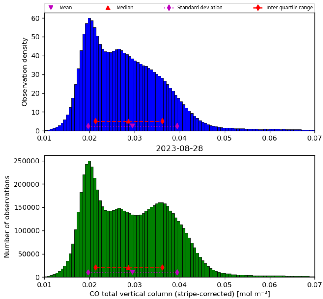
Figure 19: Histogram of “CO total vertical column (stripe-corrected)” for 2023-08-27 to 2023-08-29
