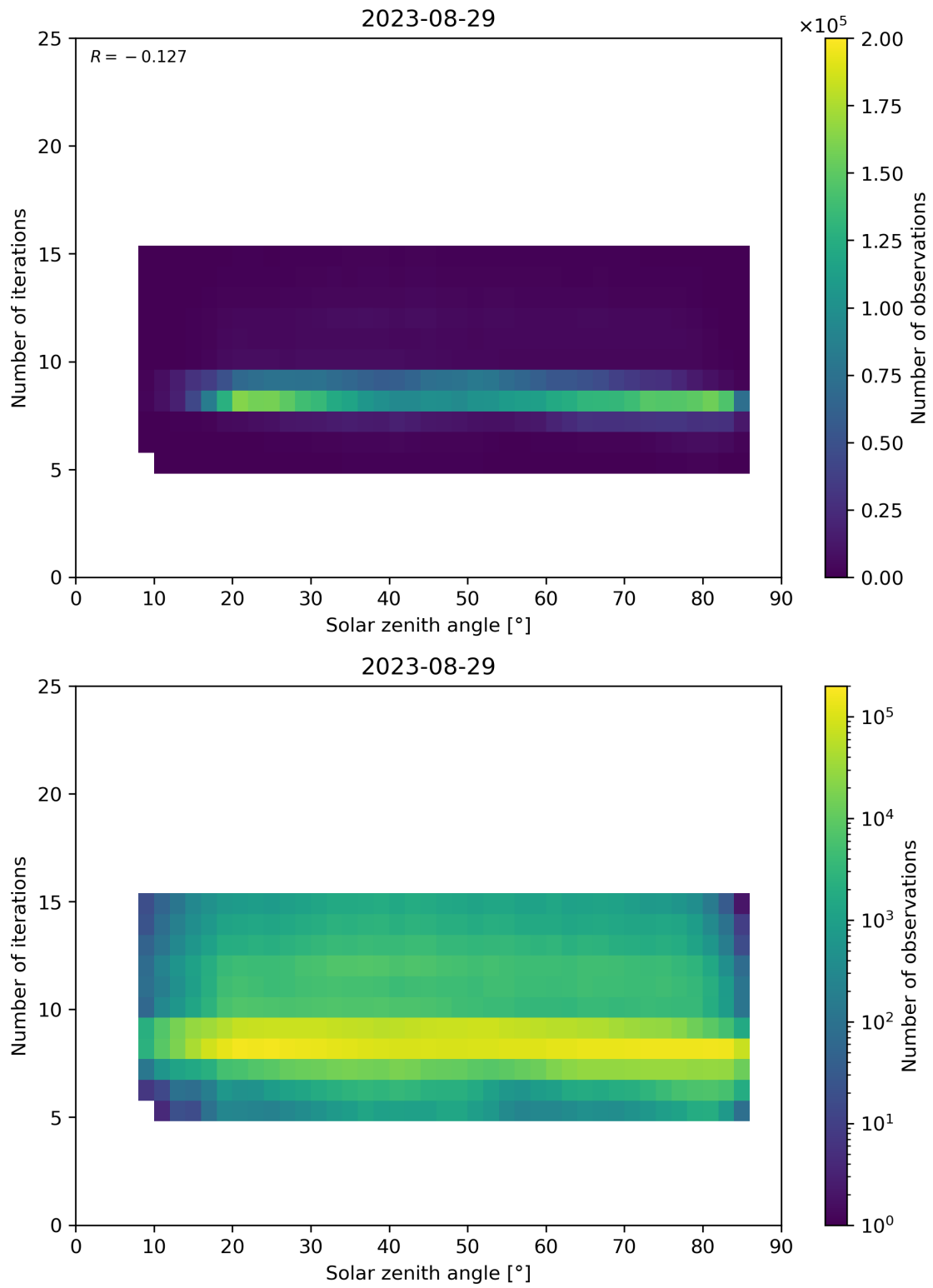
Figure 67: Scatter density plot of “Solar zenith angle” against “Number of iterations” for 2023-08-28 to 2023-08-30.
