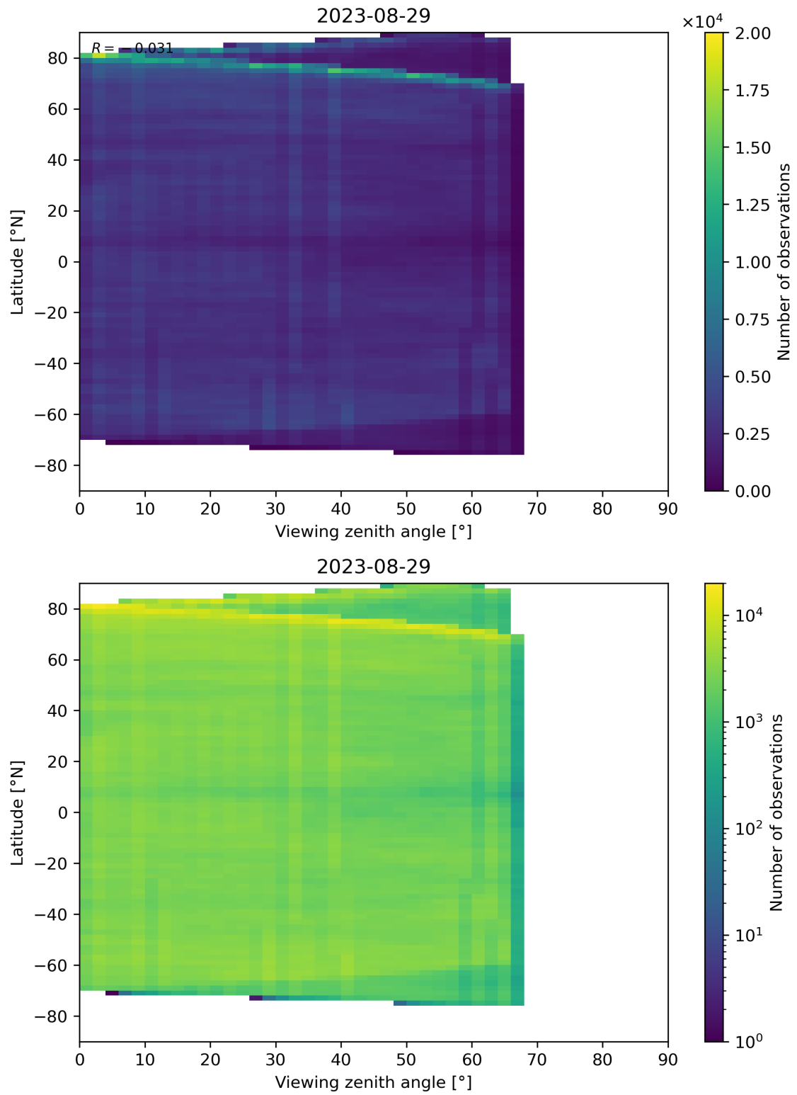
Figure 74: Scatter density plot of “Viewing zenith angle” against “Latitude” for 2023-08-28 to 2023-08-30.
