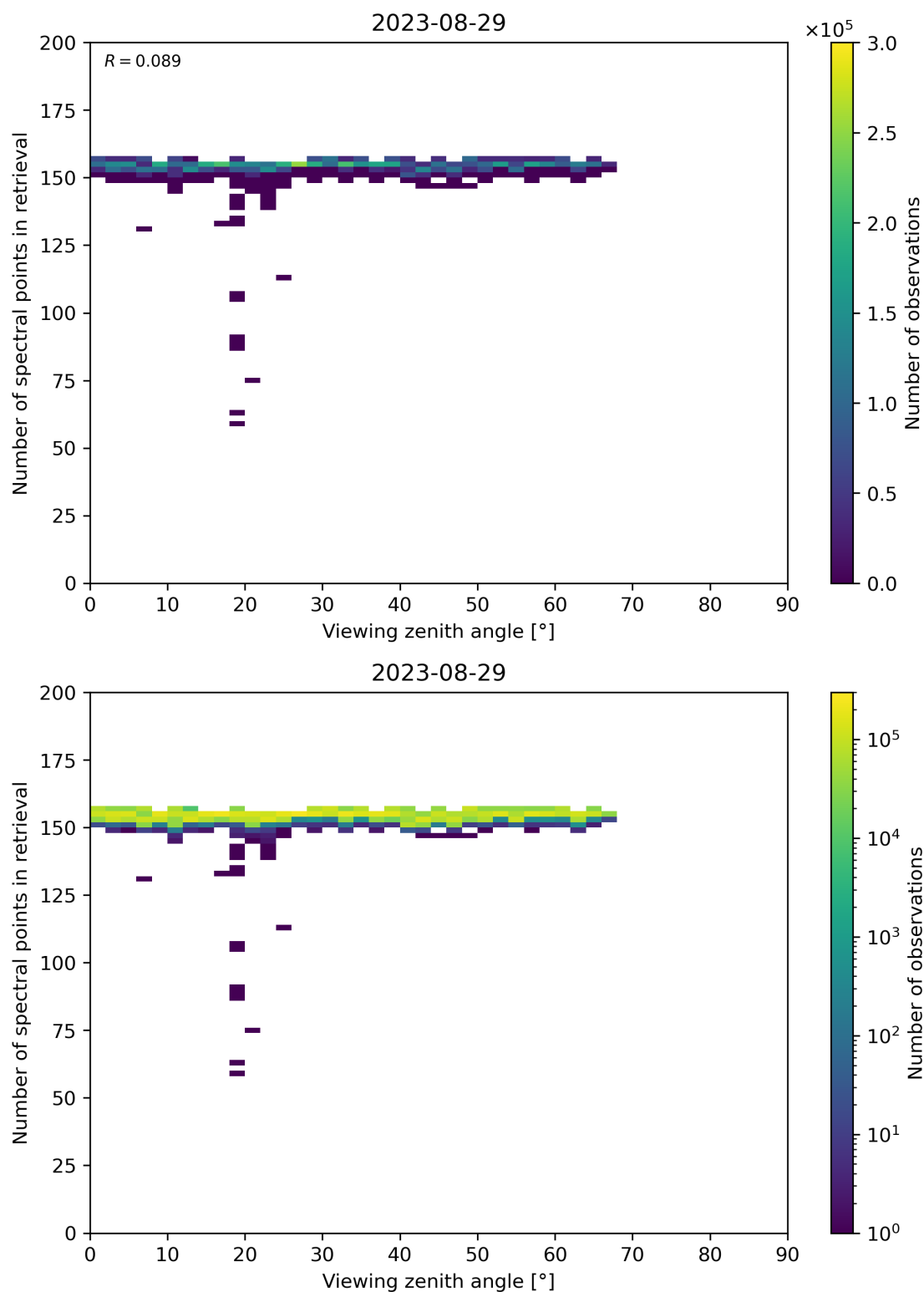
Figure 76: Scatter density plot of “Viewing zenith angle” against “Number of spectral points in retrieval” for 2023-08-28 to 2023-08-30.
