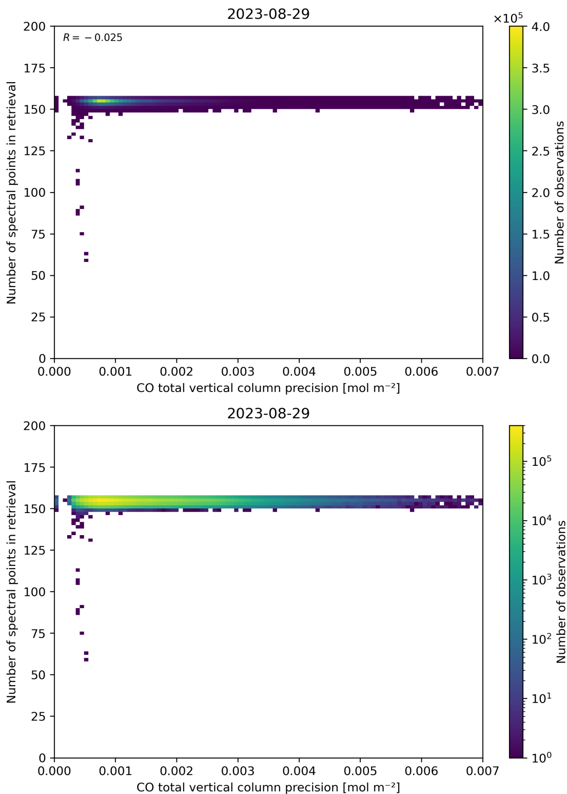
Figure 47: Scatter density plot of “CO total vertical column precision” against “Number of spectral points in retrieval” for 2023-08-28 to 2023-08-30.
