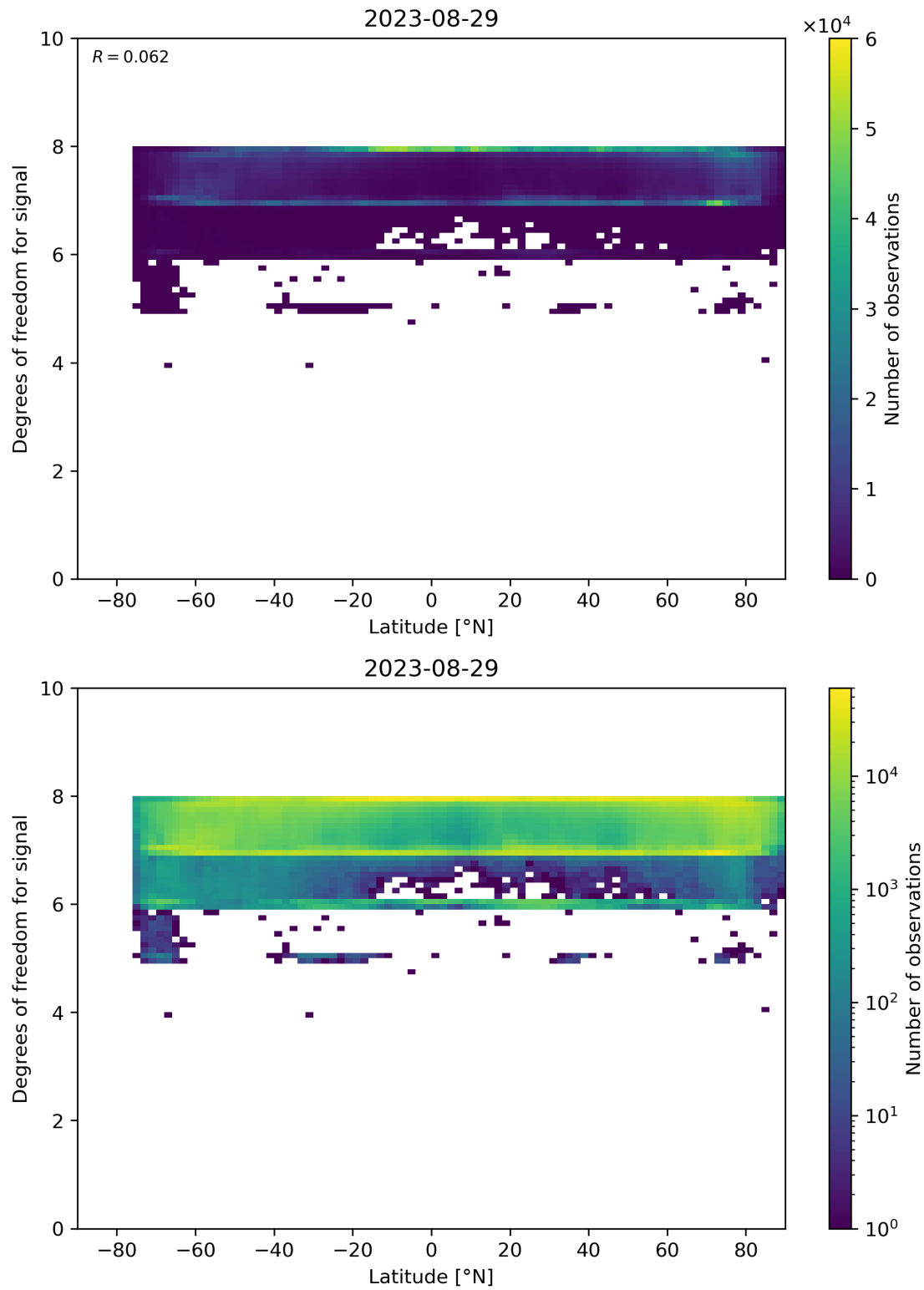
Figure 55: Scatter density plot of “Latitude” against “Degrees of freedom for signal” for 2023-08-28 to 2023-08-30.
