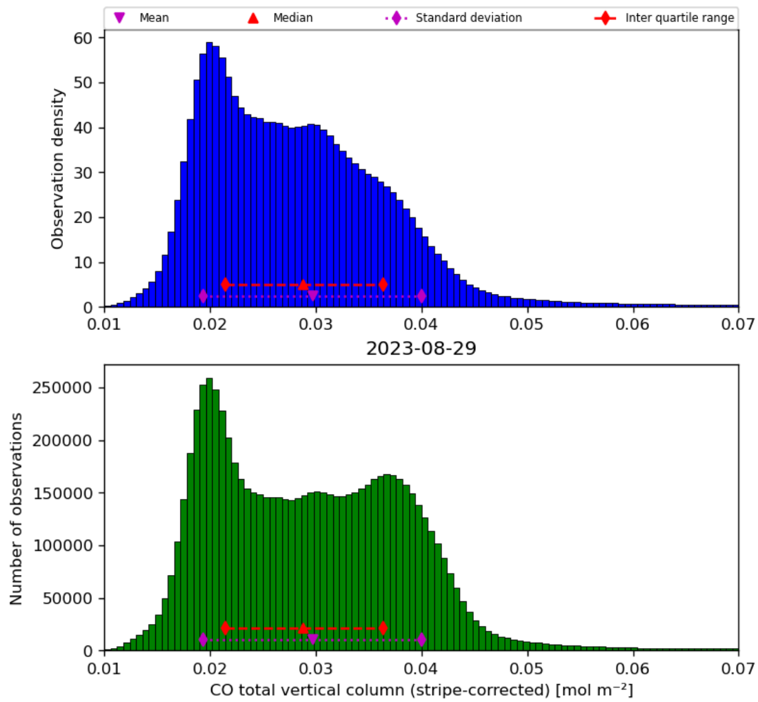
Figure 19: Histogram of “CO total vertical column (stripe-corrected)” for 2023-08-28 to 2023-08-30
