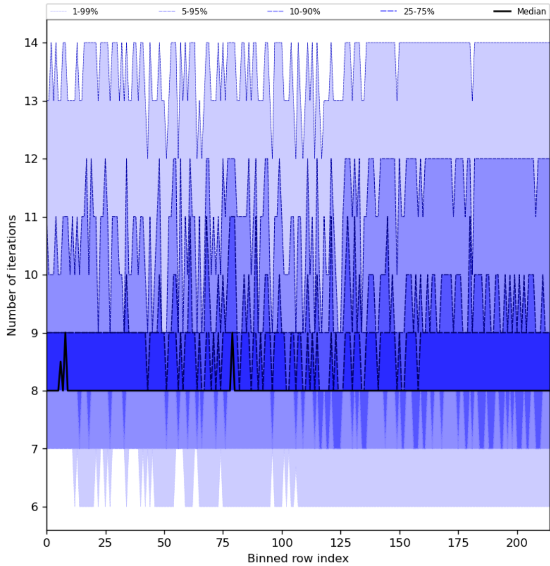
Figure 32: Along track statistics of “Number of iterations” for 2023-08-28 to 2023-08-30
