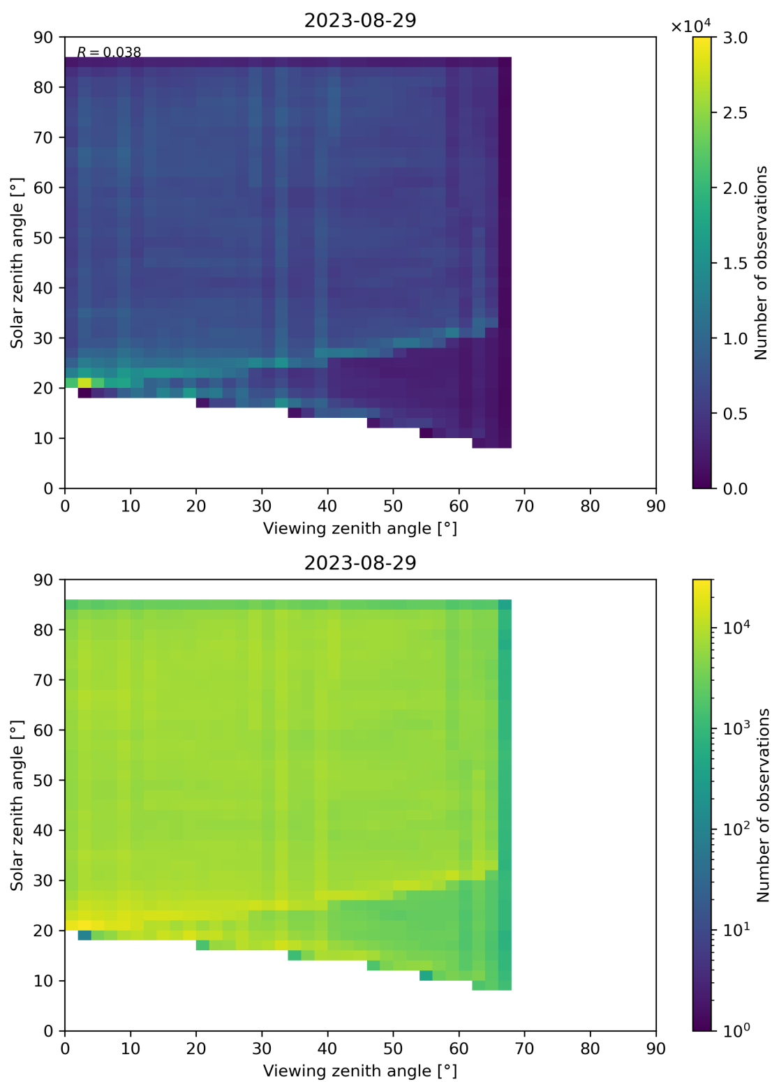
Figure 77: Scatter density plot of “Viewing zenith angle” against “Solar zenith angle” for 2023-08-28 to 2023-08-30.
