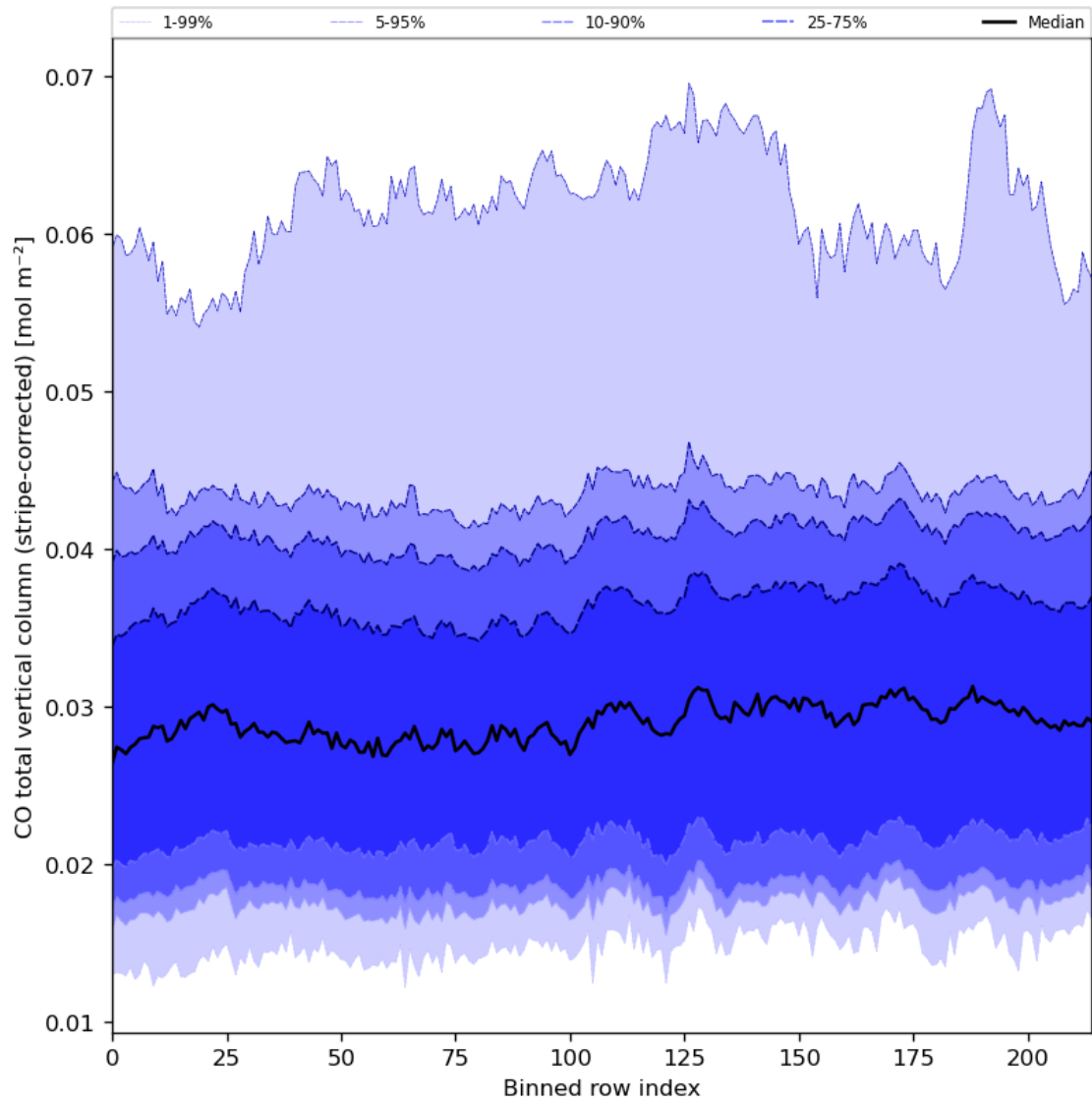
Figure 27: Along track statistics of “CO total vertical column (stripe-corrected)” for 2023-08-28 to 2023-08-30
