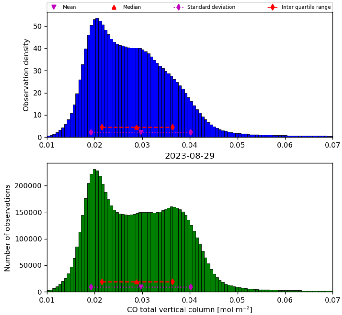
Figure 18: Histogram of “CO total vertical column” for 2023-08-28 to 2023-08-30
