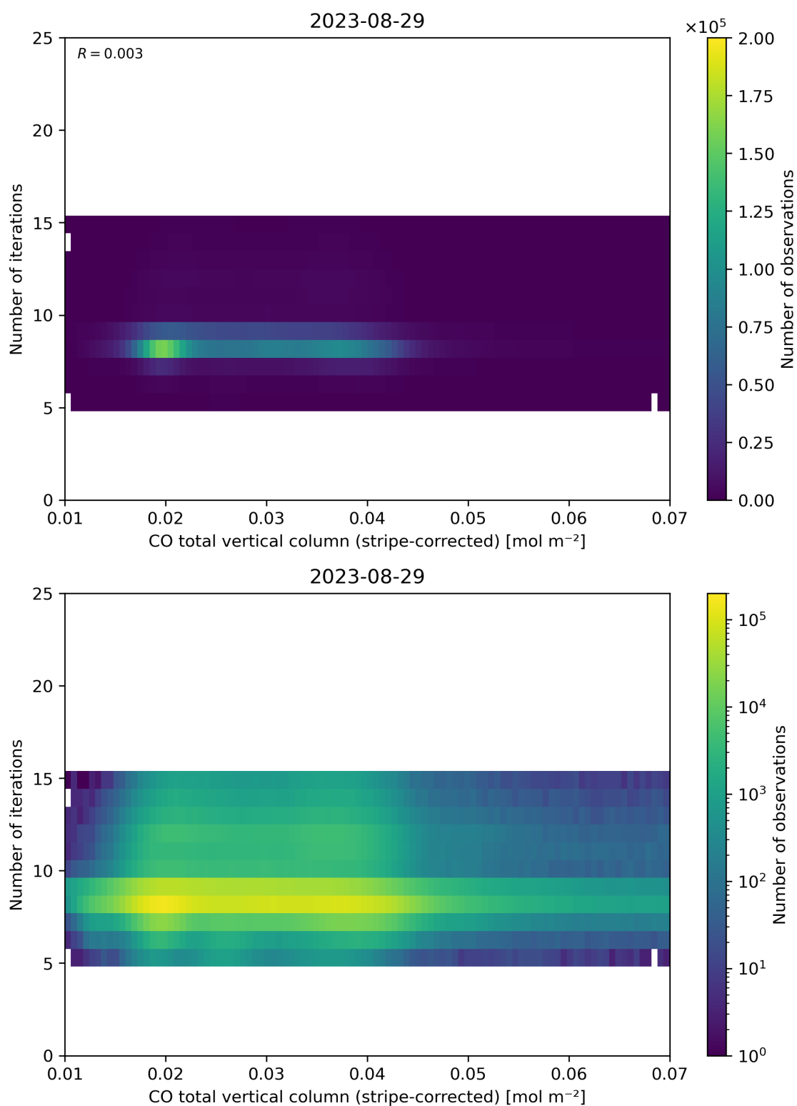
Figure 39: Scatter density plot of “CO total vertical column (stripe-corrected)” against “Number of iterations” for 2023-08-28 to 2023-08-30.
