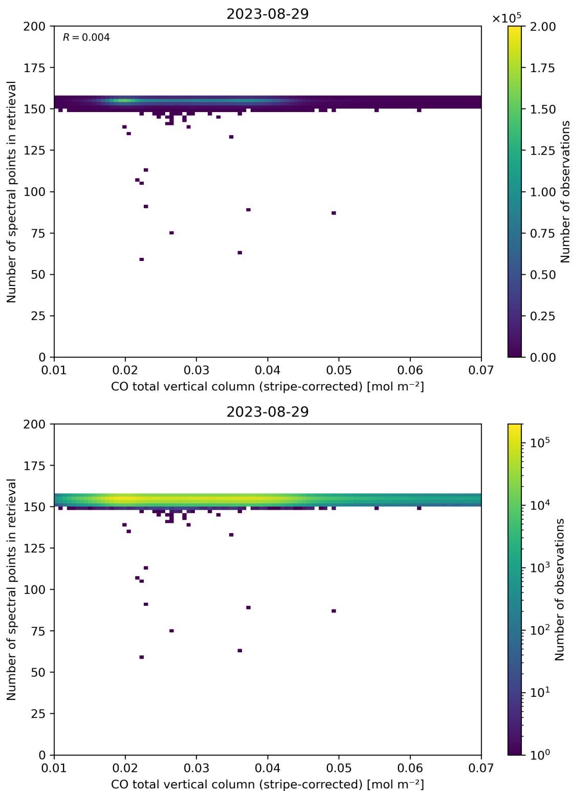
Figure 40: Scatter density plot of “CO total vertical column (stripe-corrected)” against “Number of spectral points in retrieval” for 2023-08-28 to 2023-08-30.
