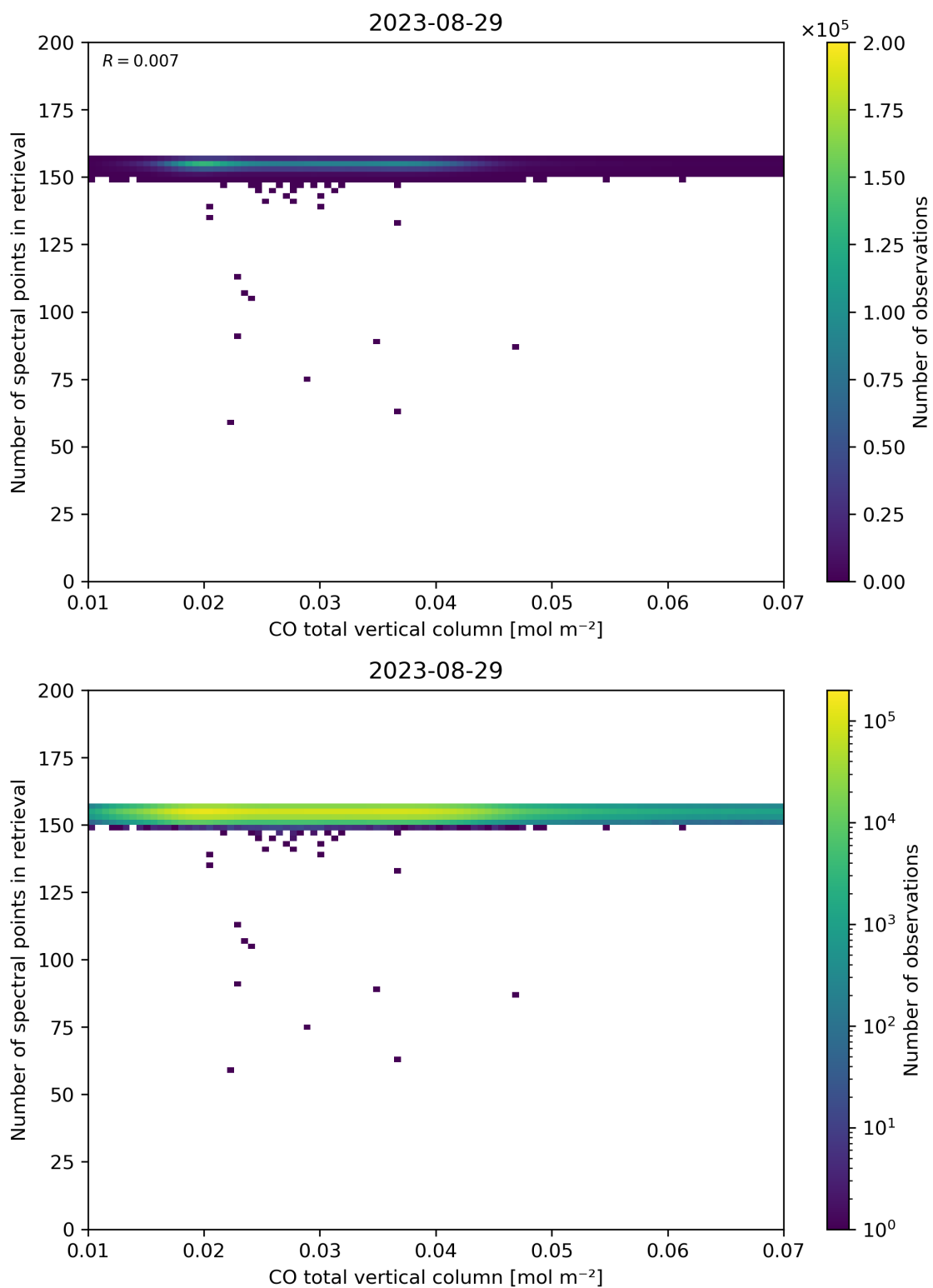
Figure 43: Scatter density plot of “CO total vertical column” against “Number of spectral points in retrieval” for 2023-08-28 to 2023-08-30.
