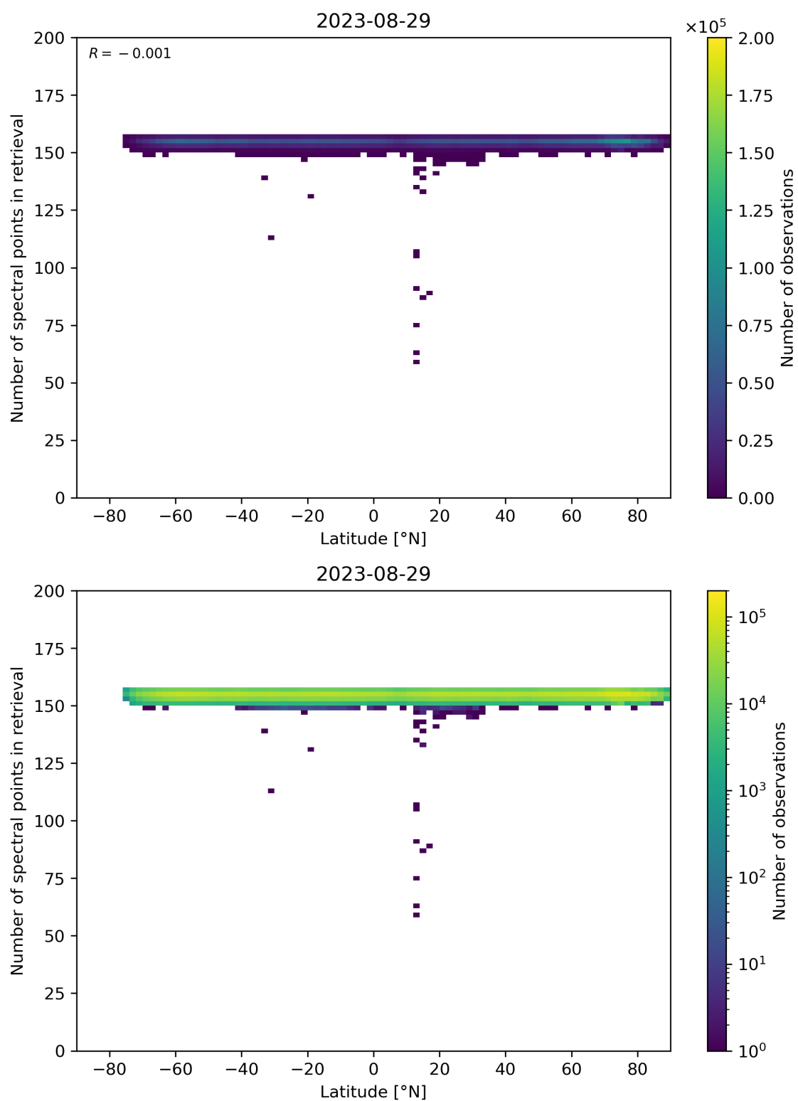
Figure 57: Scatter density plot of “Latitude” against “Number of spectral points in retrieval” for 2023-08-28 to 2023-08-30.
