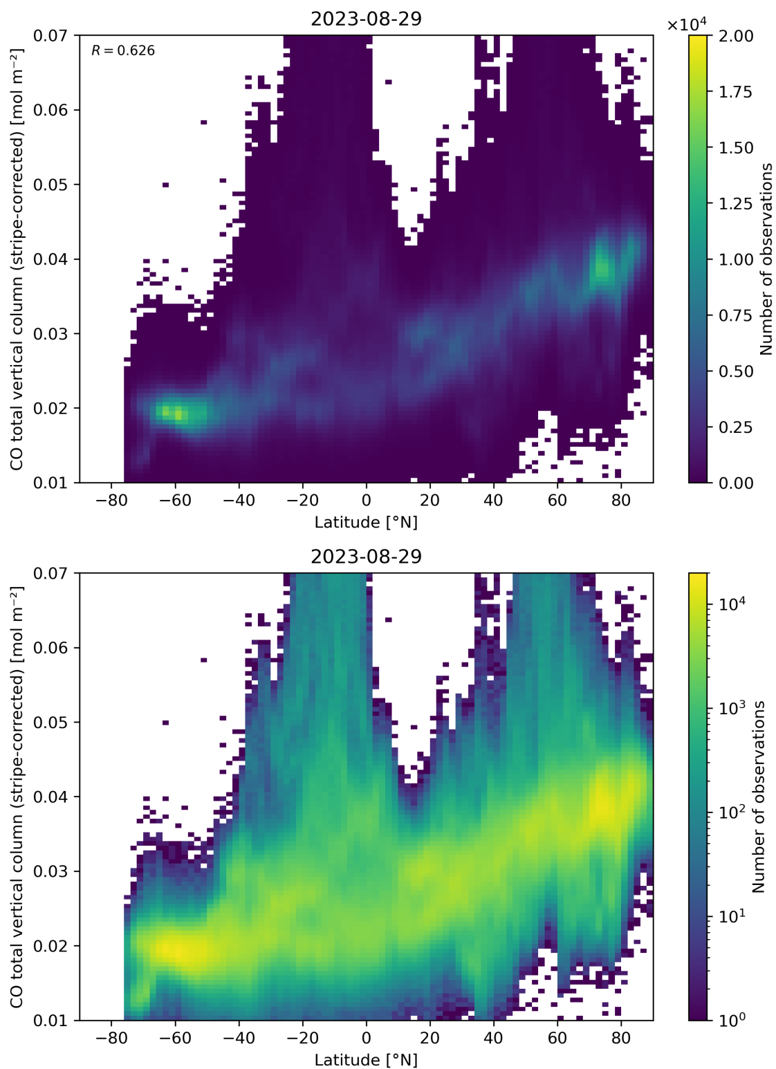
Figure 52: Scatter density plot of “Latitude” against “CO total vertical column (stripe-corrected)” for 2023-08-28 to 2023-08-30.
