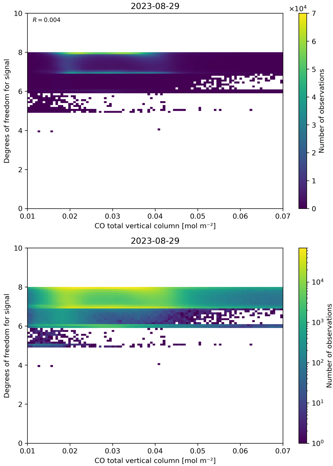
Figure 41: Scatter density plot of “CO total vertical column” against “Degrees of freedom for signal” for 2023-08-28 to 2023-08-30.
