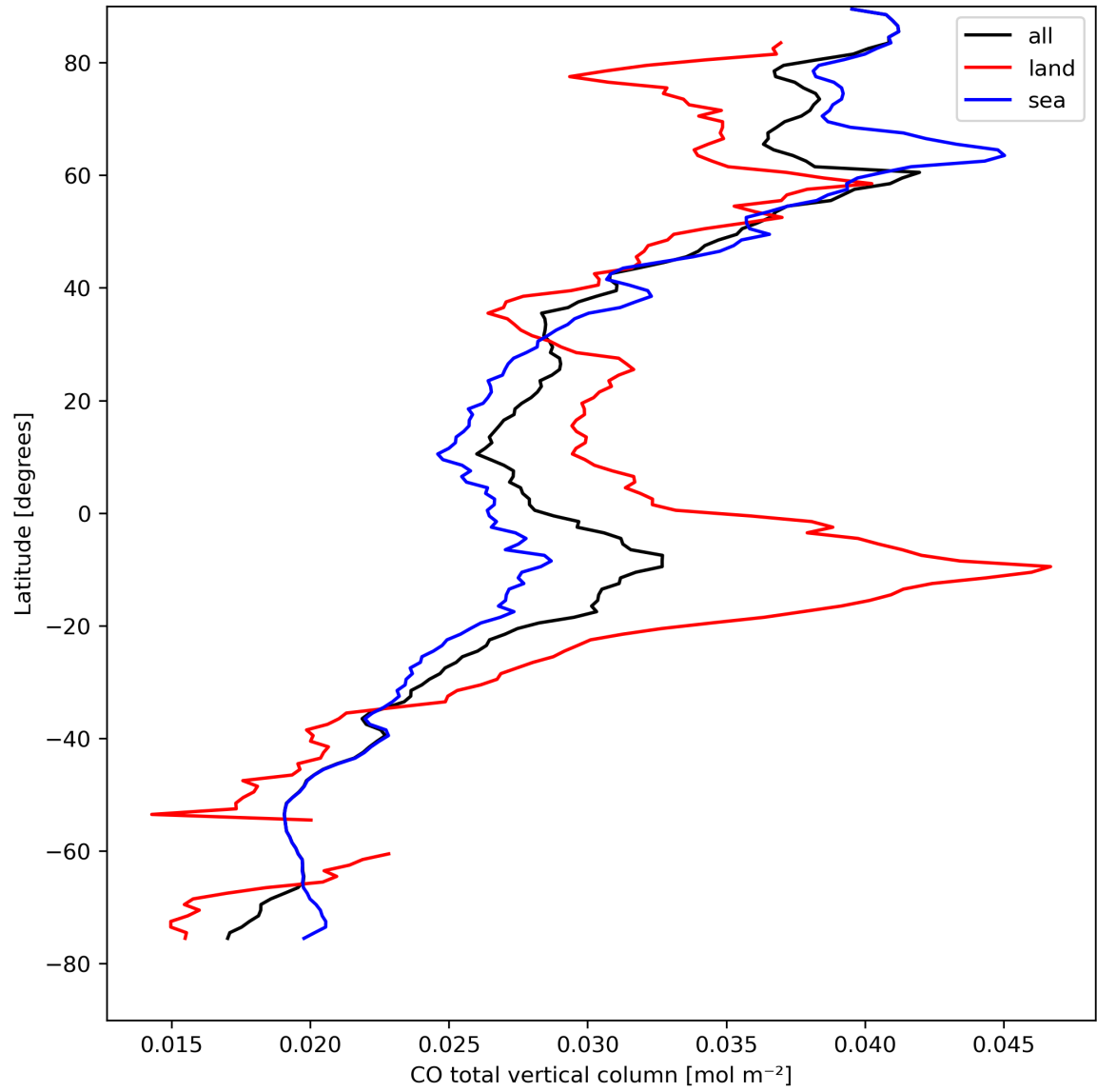
Figure 10: Zonal average of “CO total vertical column” for 2023-08-28 to 2023-08-30.
