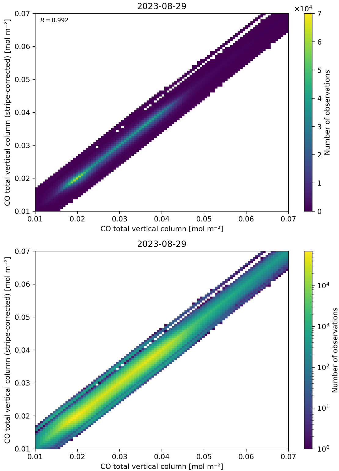
Figure 33: Scatter density plot of “CO total vertical column” against “CO total vertical column (stripe-corrected)” for 2023-08-28 to 2023-08-30.
