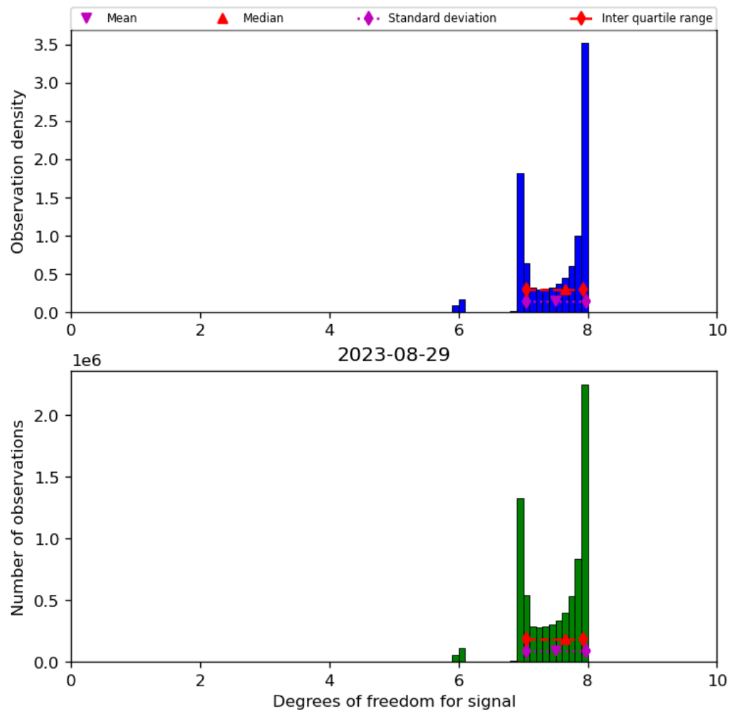
Figure 23: Histogram of “Degrees of freedom for signal” for 2023-08-28 to 2023-08-30
