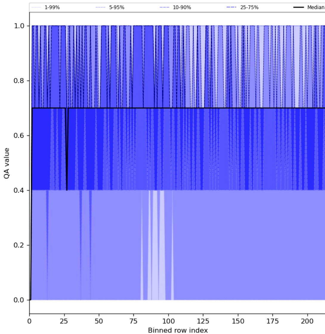
Figure 25: Along track statistics of “QA value” for 2023-08-28 to 2023-08-30
