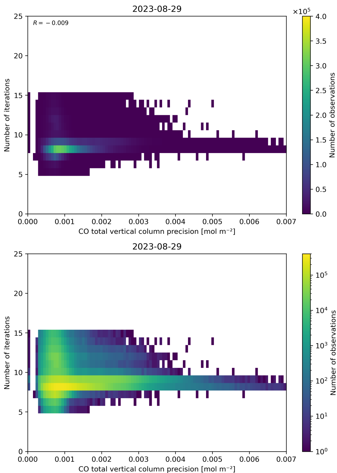
Figure 46: Scatter density plot of “CO total vertical column precision” against “Number of iterations” for 2023-08-28 to 2023-08-30.
