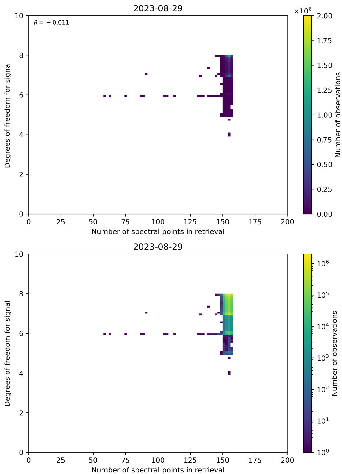
Figure 59: Scatter density plot of “Number of spectral points in retrieval” against “Degrees of freedom for signal” for 2023-08-28 to 2023-08-30.
