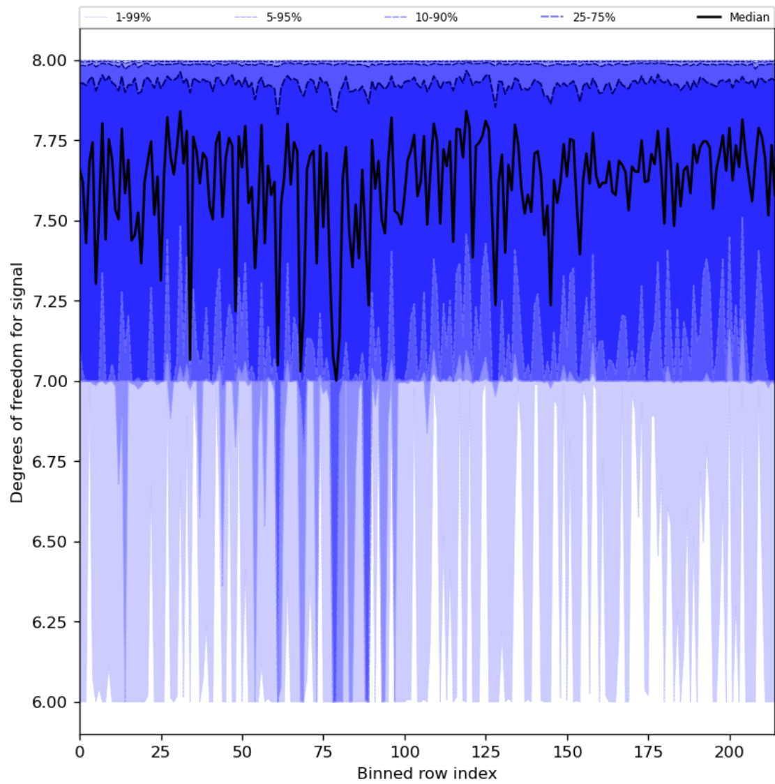
Figure 31: Along track statistics of “Degrees of freedom for signal” for 2023-08-28 to 2023-08-30
