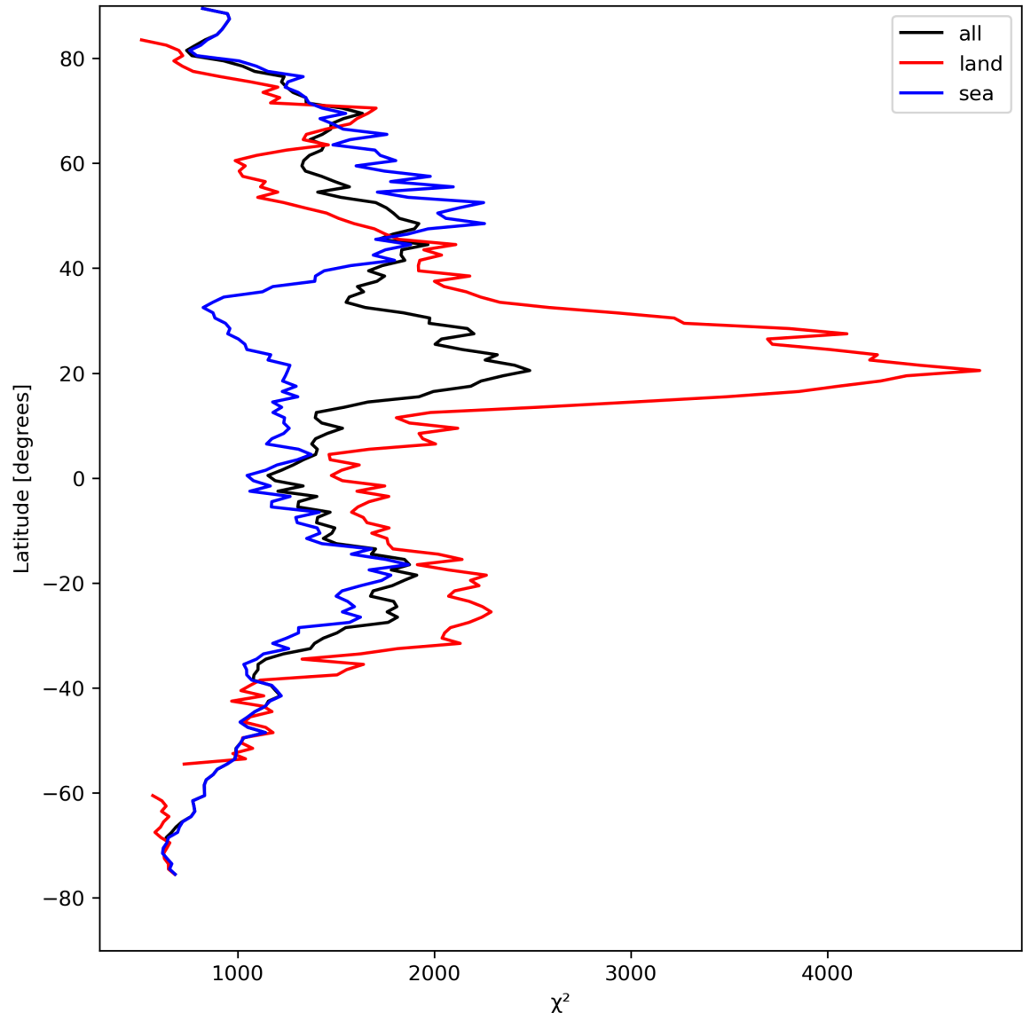
Figure 14: Zonal average of “ \chi^2 ” for 2023-08-28 to 2023-08-30.
