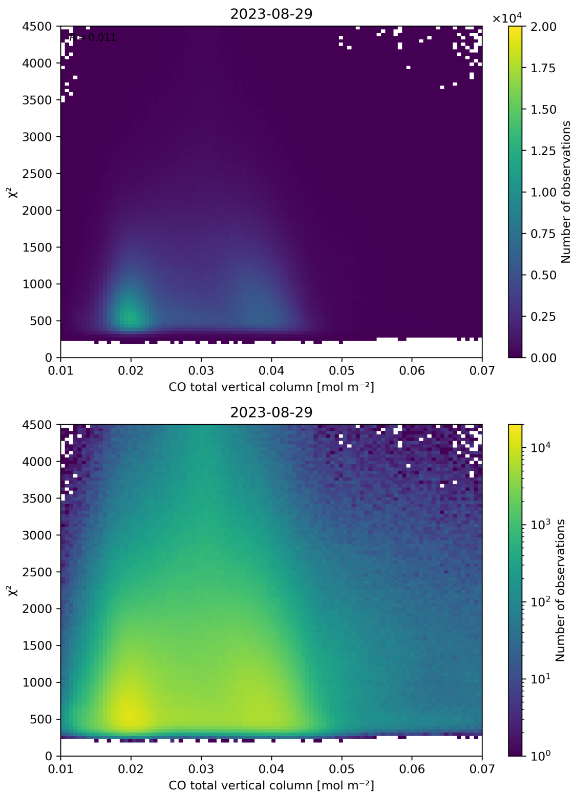
Figure 35: Scatter density plot of “CO total vertical column” against “ \chi^2 ” for 2023-08-28 to 2023-08-30.
