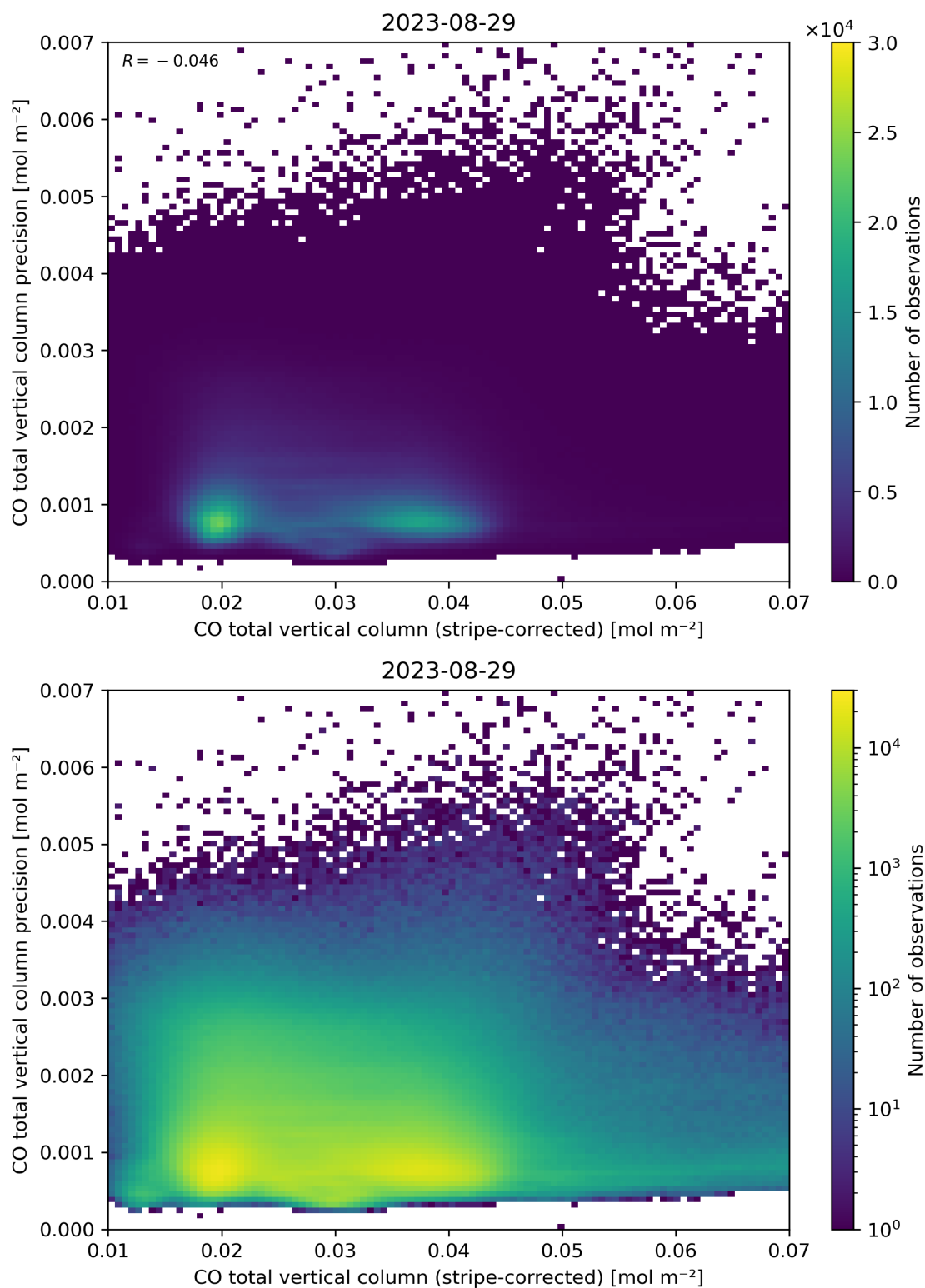
Figure 36: Scatter density plot of “CO total vertical column (stripe-corrected)” against “CO total vertical column precision” for 2023-08-28 to 2023-08-30.
