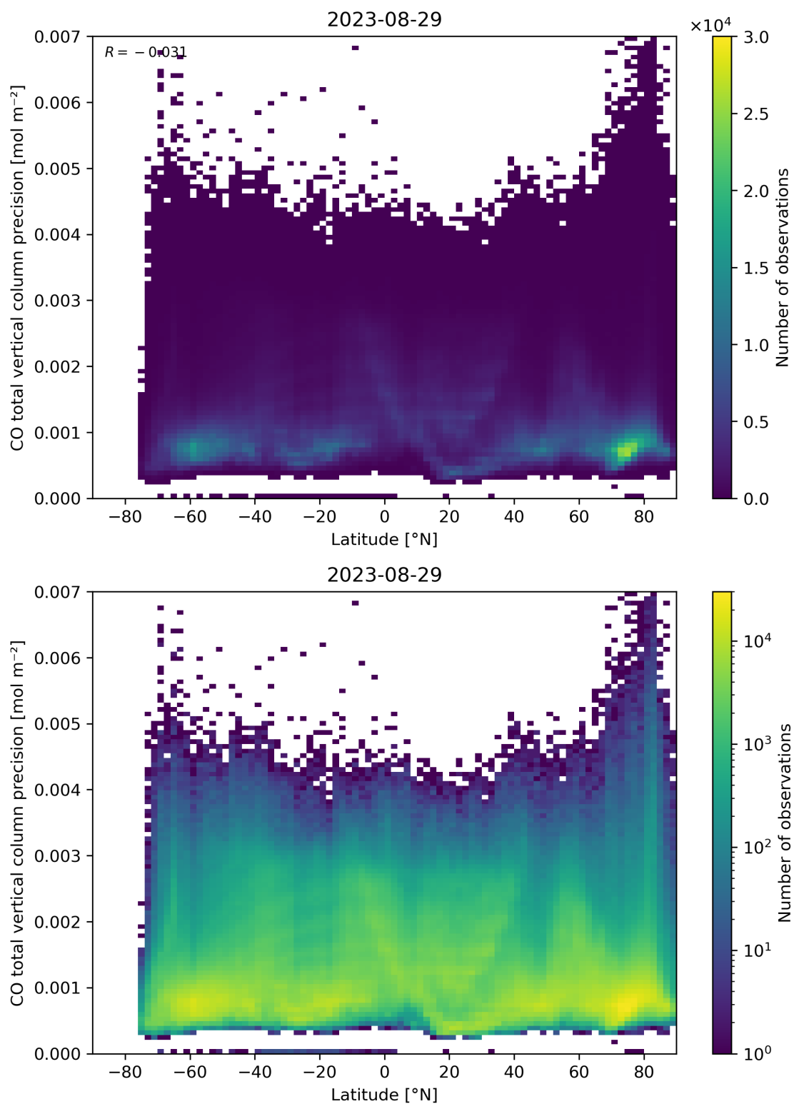
Figure 53: Scatter density plot of “Latitude” against “CO total vertical column precision” for 2023-08-28 to 2023-08-30.
