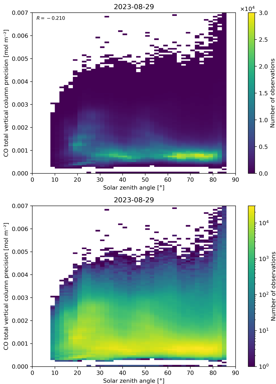
Figure 63: Scatter density plot of “Solar zenith angle” against “CO total vertical column precision” for 2023-08-28 to 2023-08-30.
