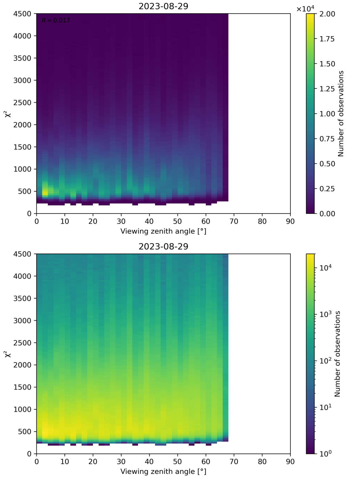
Figure 72: Scatter density plot of “Viewing zenith angle” against “ \chi^2 ” for 2023-08-28 to 2023-08-30.
