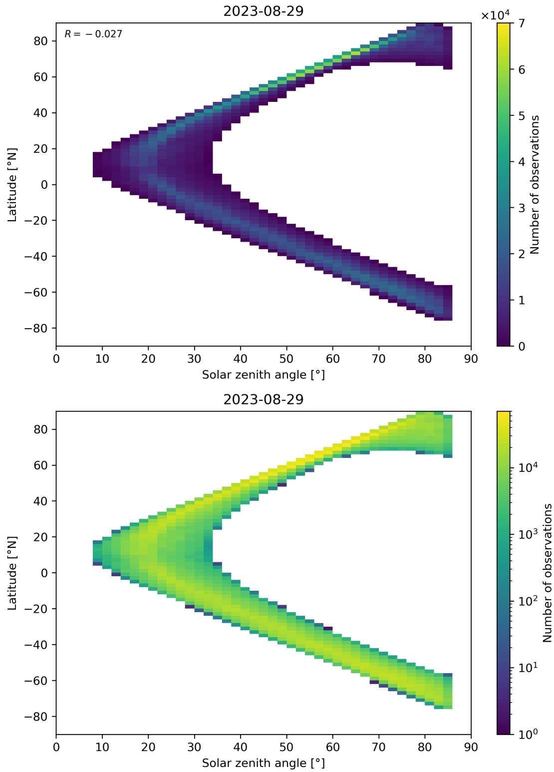
Figure 66: Scatter density plot of “Solar zenith angle” against “Latitude” for 2023-08-28 to 2023-08-30.
