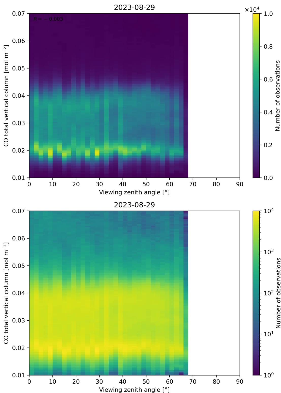
Figure 69: Scatter density plot of “Viewing zenith angle” against “CO total vertical column” for 2023-08-28 to 2023-08-30.
