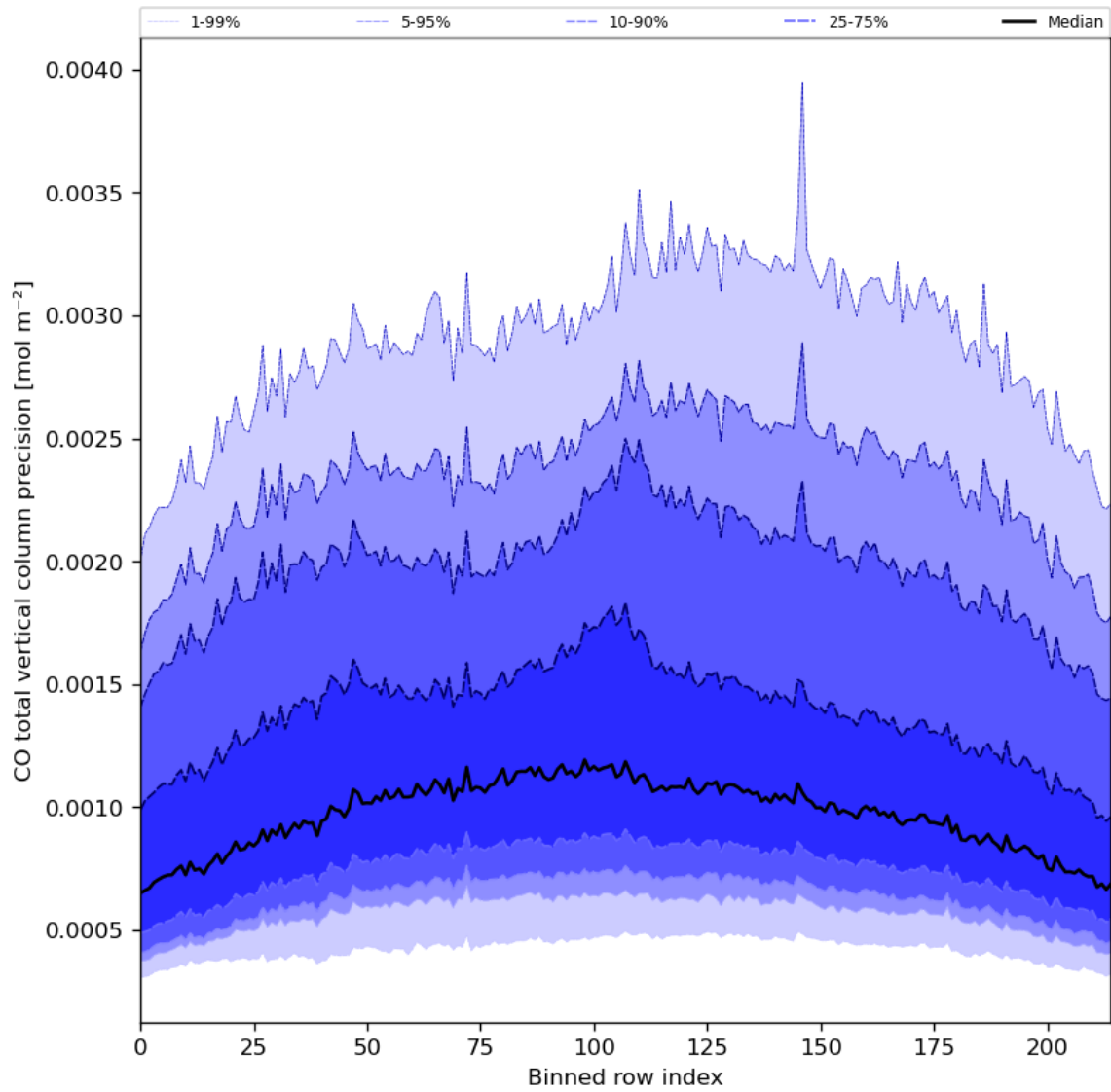
Figure 28: Along track statistics of “CO total vertical column precision” for 2023-08-28 to 2023-08-30
