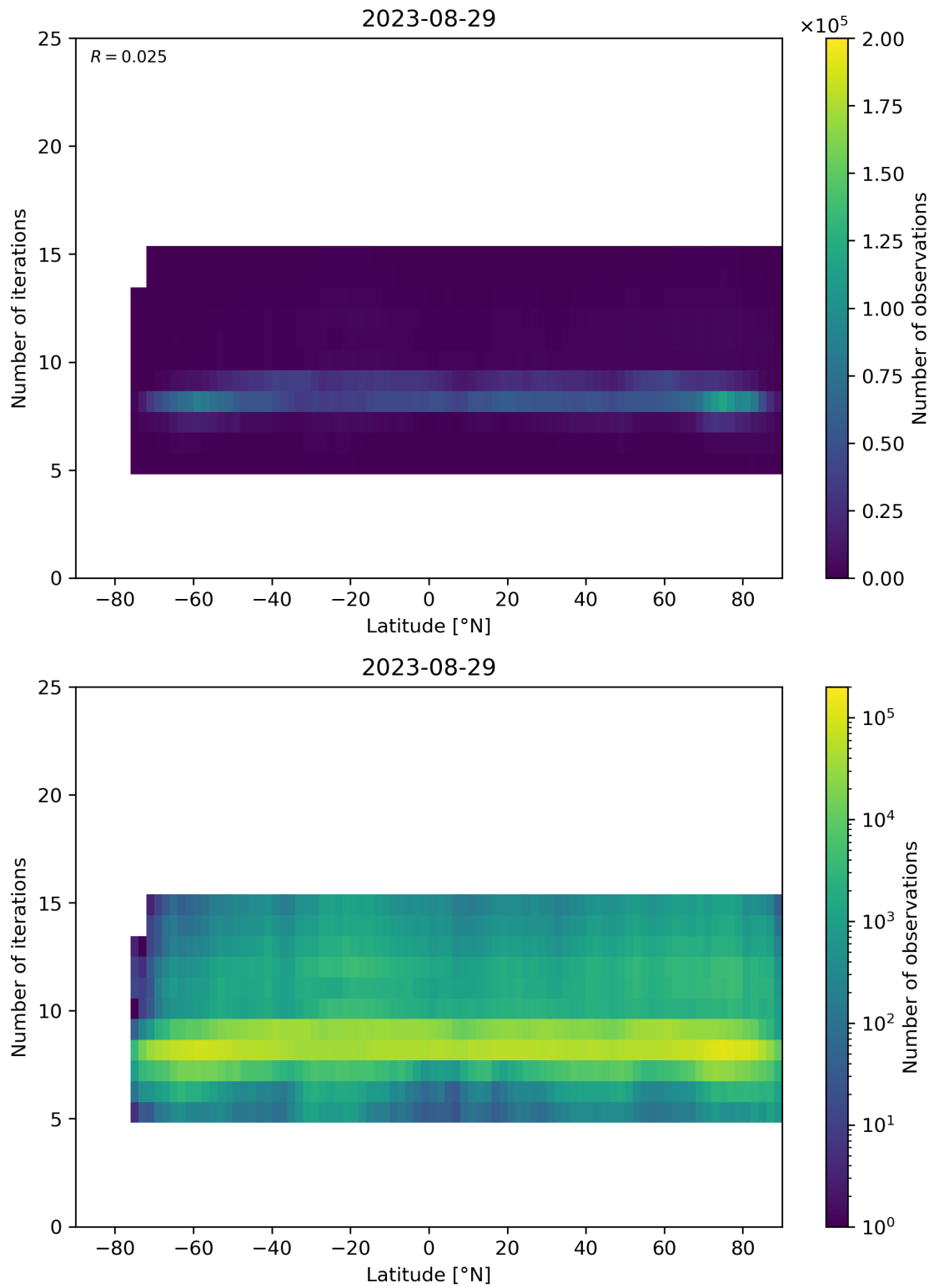
Figure 56: Scatter density plot of “Latitude” against “Number of iterations” for 2023-08-28 to 2023-08-30.
