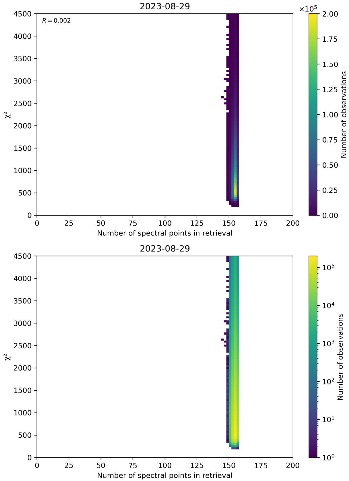
Figure 58: Scatter density plot of “Number of spectral points in retrieval” against “ \chi^2 ” for 2023-08-28 to 2023-08-30.
