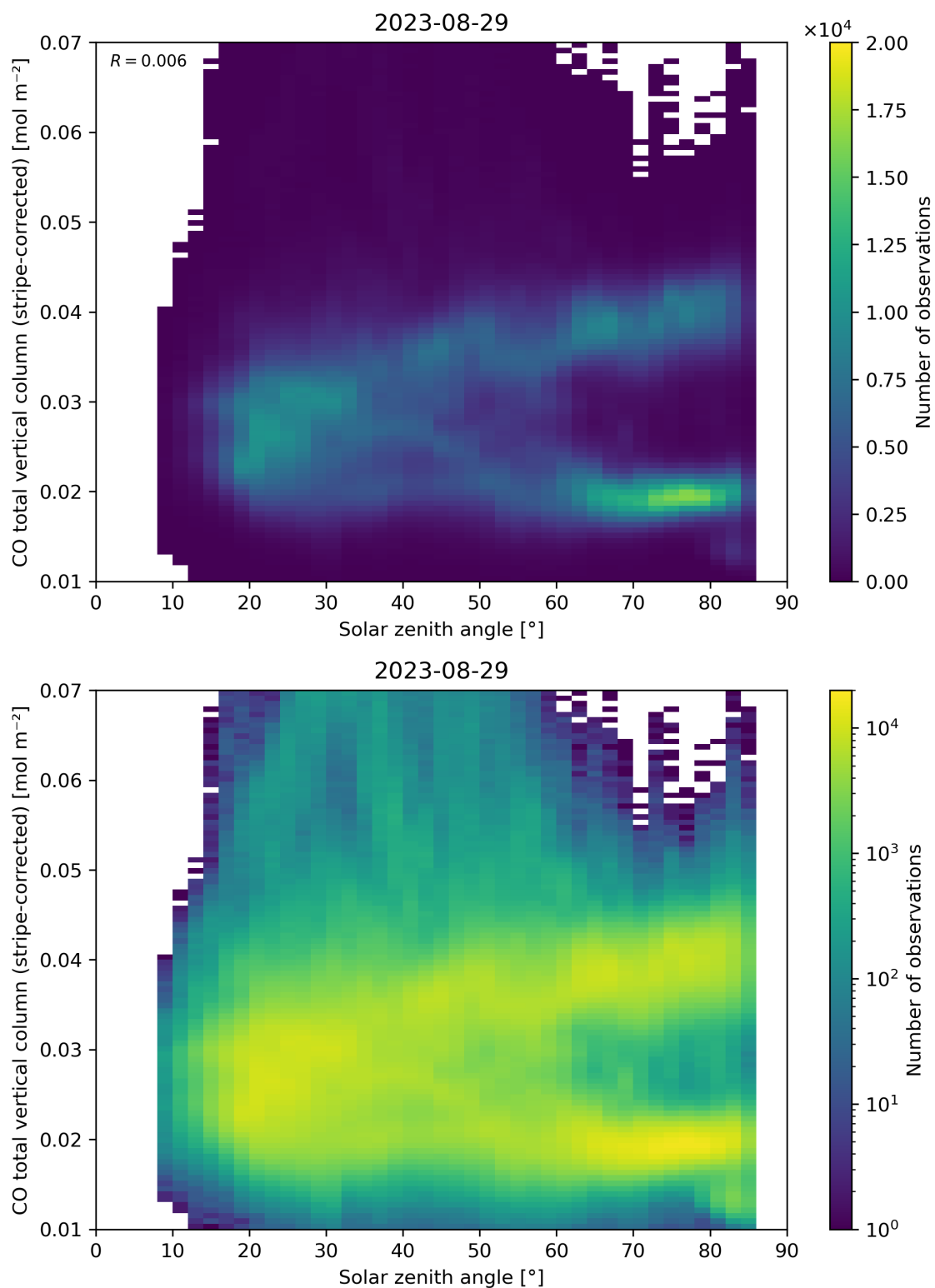
Figure 62: Scatter density plot of “Solar zenith angle” against “CO total vertical column (stripe-corrected)” for 2023-08-28 to 2023-08-30.
