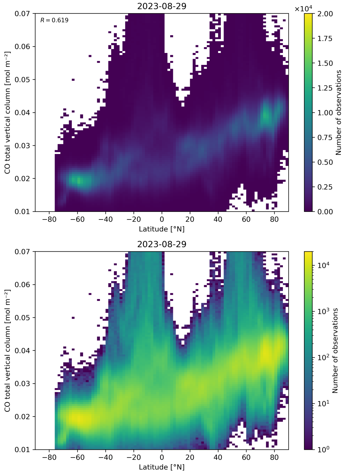
Figure 51: Scatter density plot of “Latitude” against “CO total vertical column” for 2023-08-28 to 2023-08-30.
