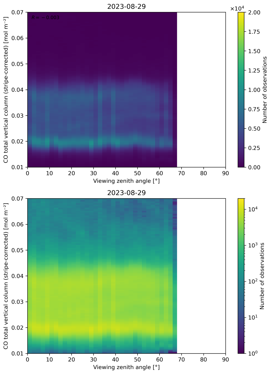
Figure 70: Scatter density plot of “Viewing zenith angle” against “CO total vertical column (stripe-corrected)” for 2023-08-28 to 2023-08-30.
