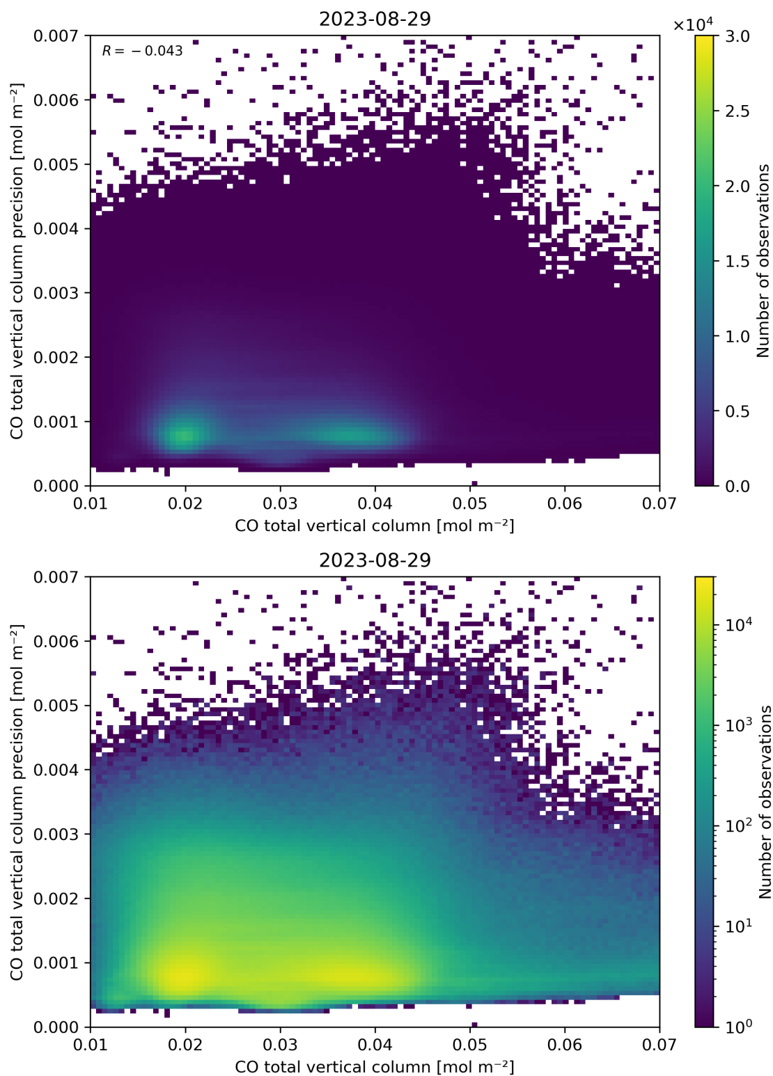
Figure 34: Scatter density plot of “CO total vertical column” against “CO total vertical column precision” for 2023-08-28 to 2023-08-30.
