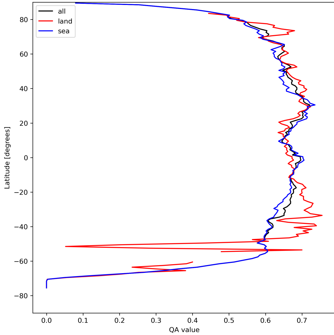
Figure 9: Zonal average of “QA value” for 2023-08-28 to 2023-08-30.
