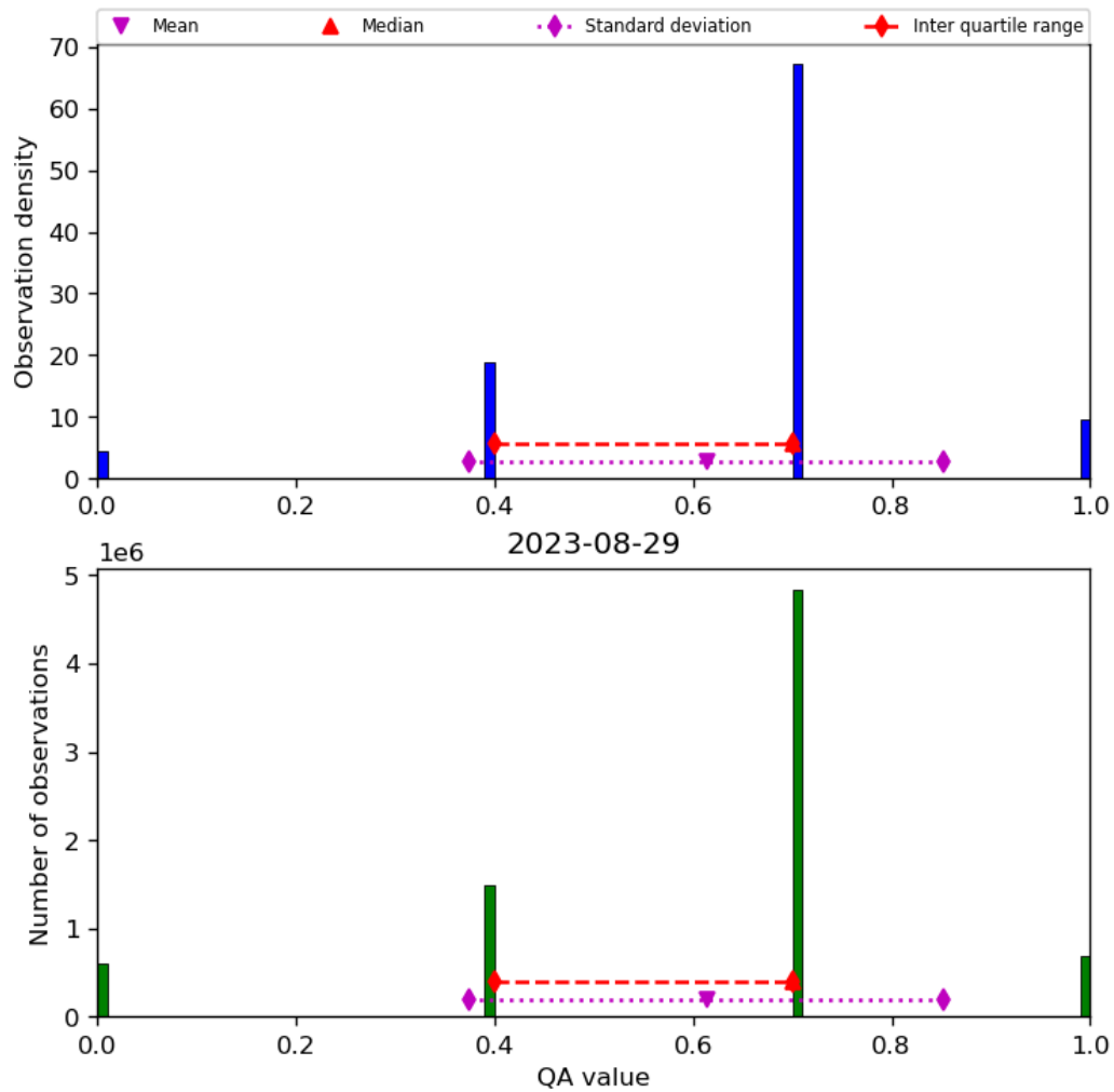
Figure 17: Histogram of “QA value” for 2023-08-28 to 2023-08-30
