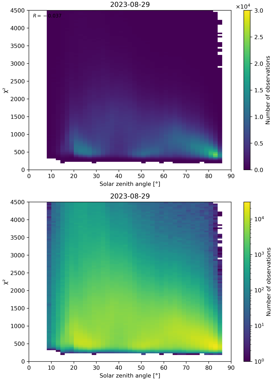
Figure 64: Scatter density plot of “Solar zenith angle” against “ \chi^2 ” for 2023-08-28 to 2023-08-30.
