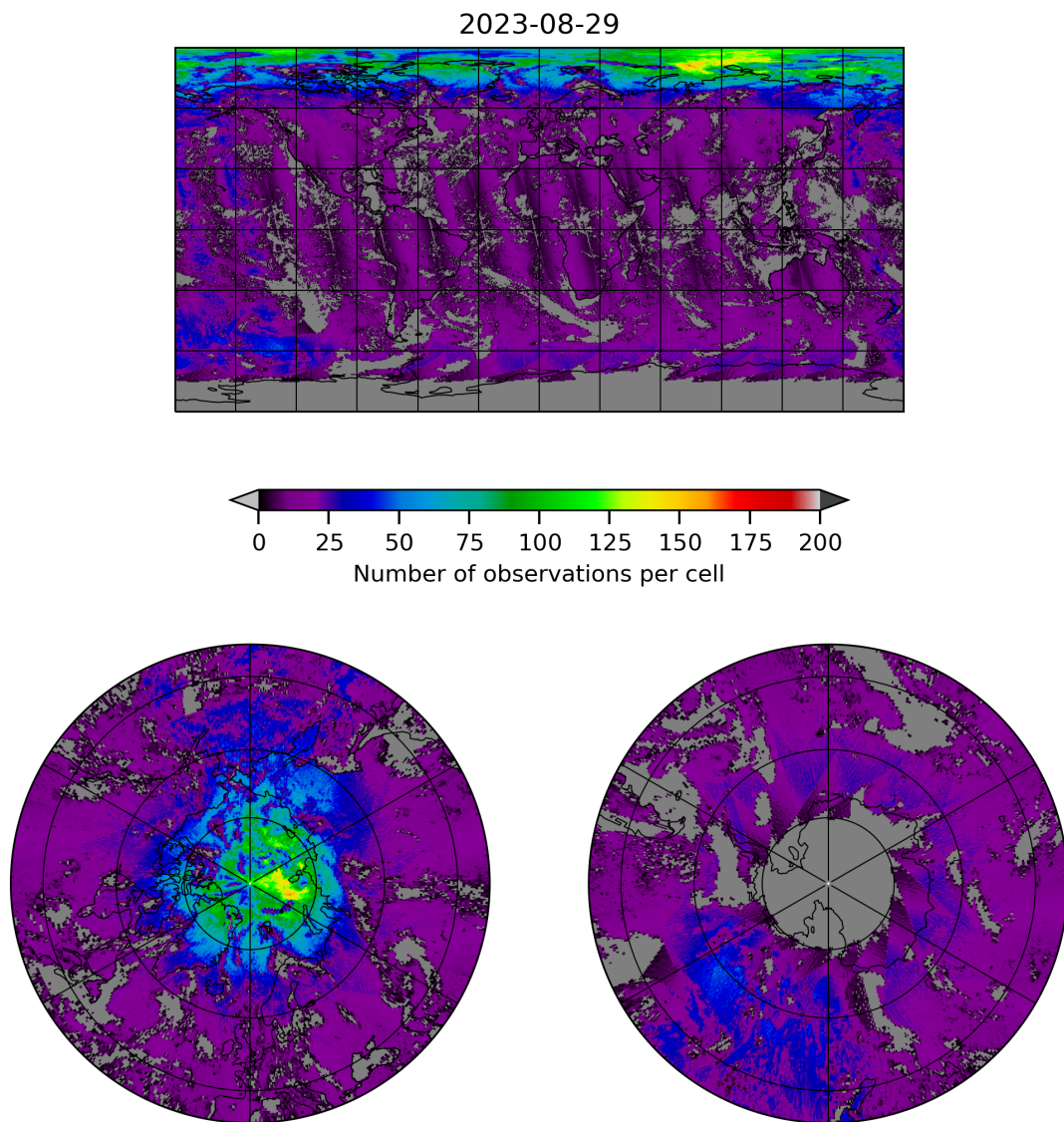
Figure 8: Map of the number of observations for 2023-08-28 to 2023-08-30
