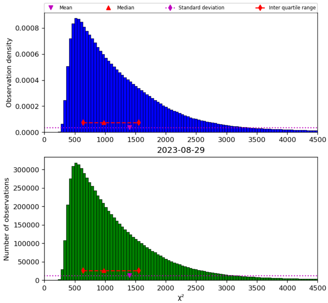
Figure 22: Histogram of “ \chi^2 ” for 2023-08-28 to 2023-08-30
