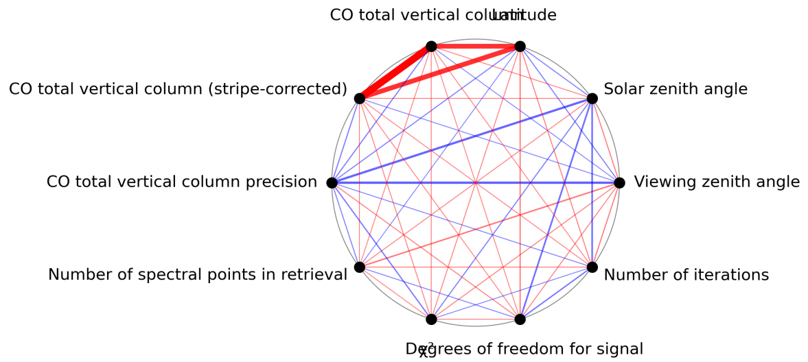
Figure 1: Map of correlation graph for 2023-08-28 to 2023-08-30.
