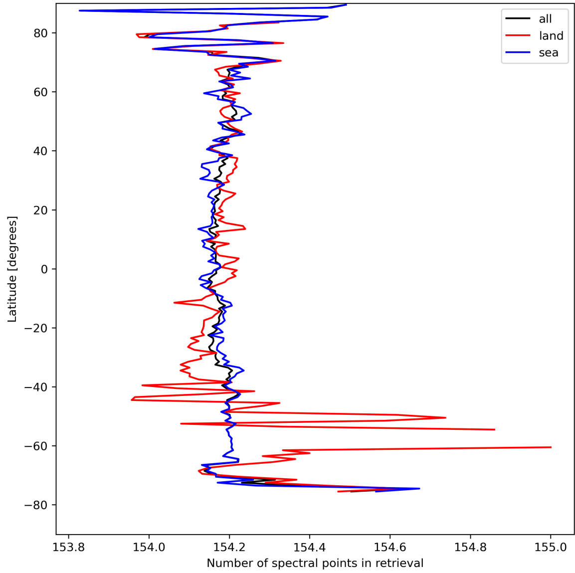
Figure 13: Zonal average of “Number of spectral points in retrieval” for 2023-08-28 to 2023-08-30.
