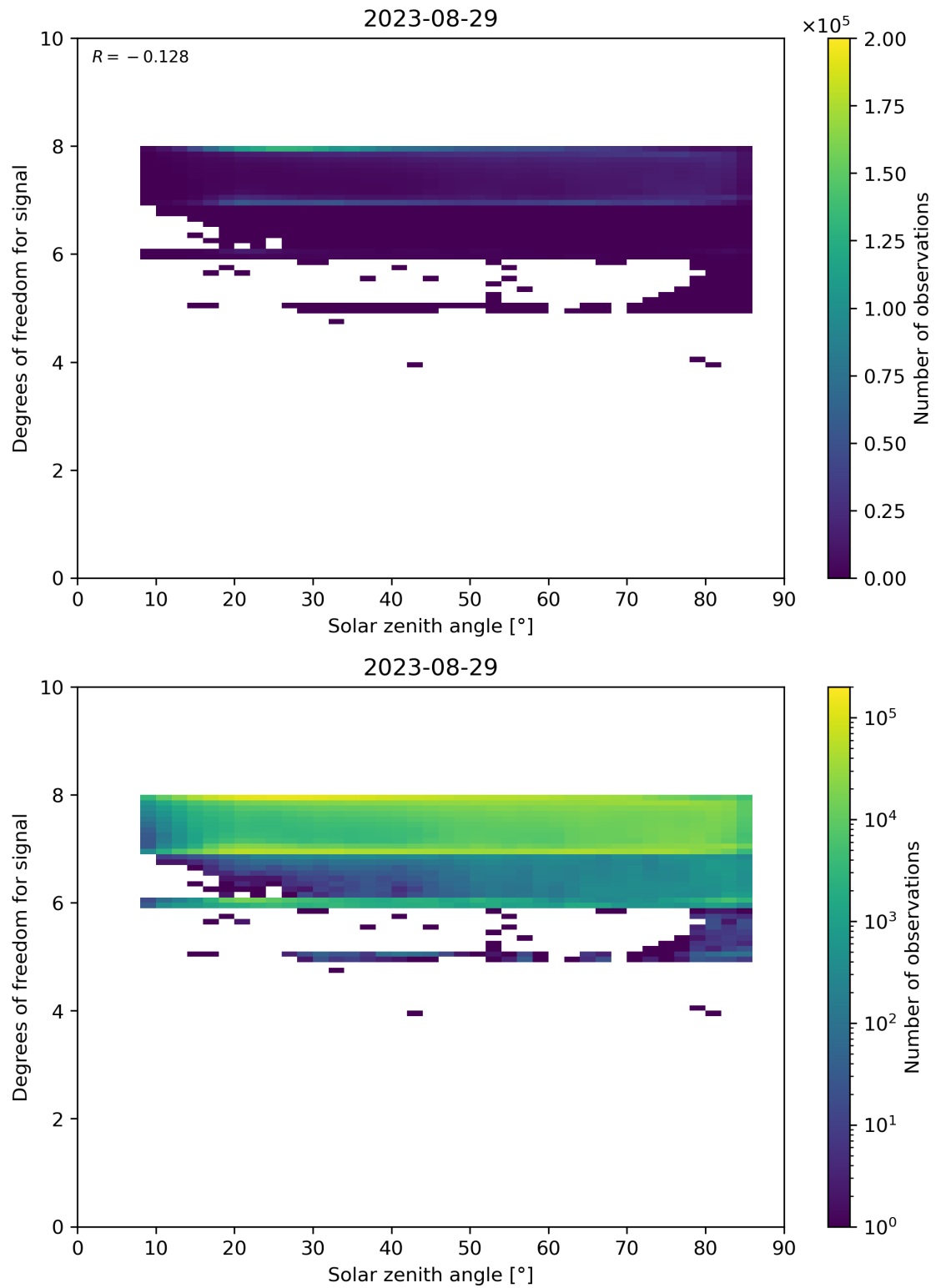
Figure 65: Scatter density plot of “Solar zenith angle” against “Degrees of freedom for signal” for 2023-08-28 to 2023-08-30.
