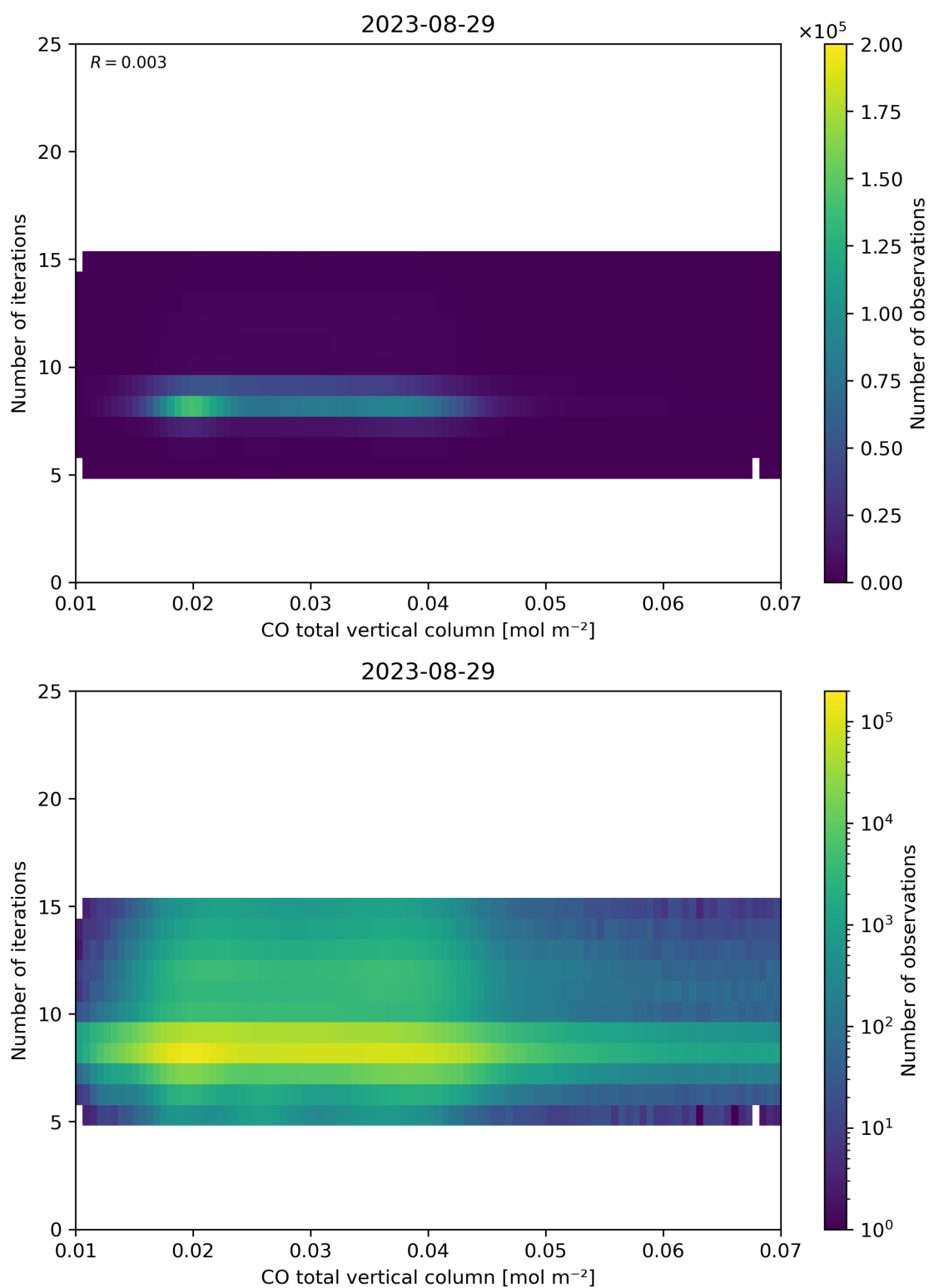
Figure 42: Scatter density plot of “CO total vertical column” against “Number of iterations” for 2023-08-28 to 2023-08-30.
