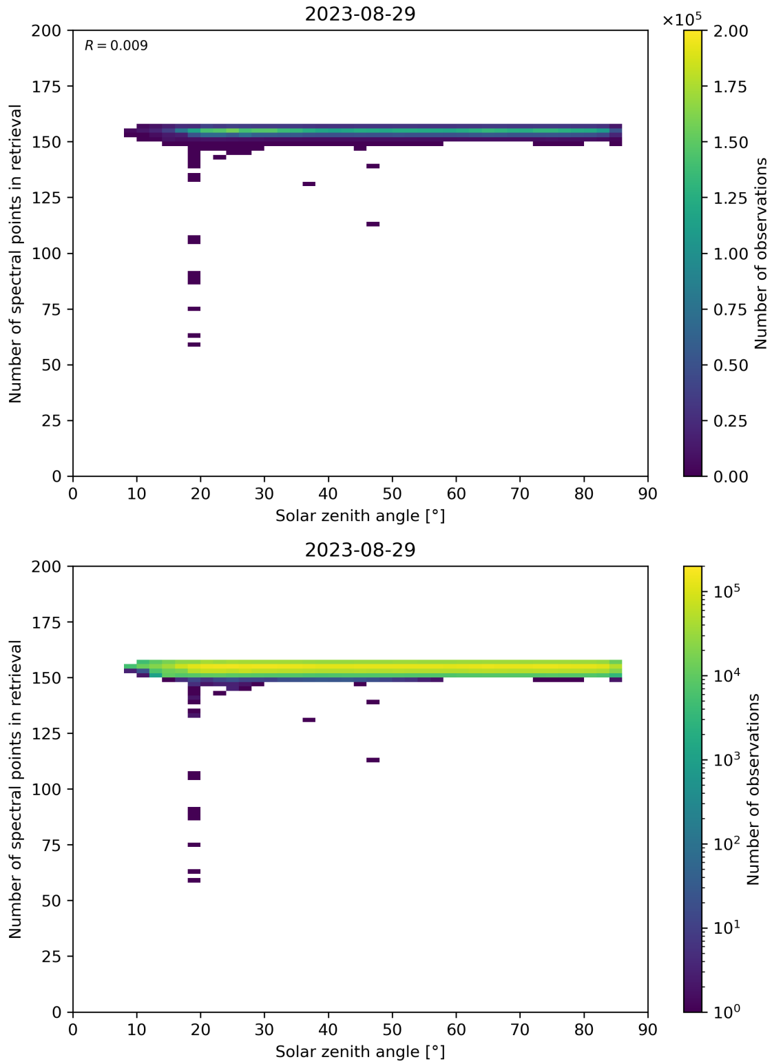
Figure 68: Scatter density plot of “Solar zenith angle” against “Number of spectral points in retrieval” for 2023-08-28 to 2023-08-30.
