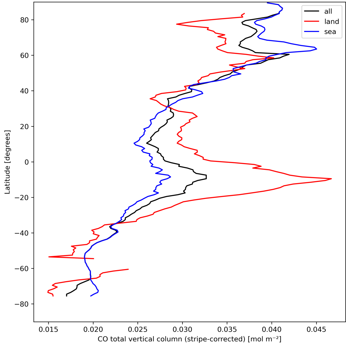
Figure 11: Zonal average of “CO total vertical column (stripe-corrected)” for 2023-08-28 to 2023-08-30.
