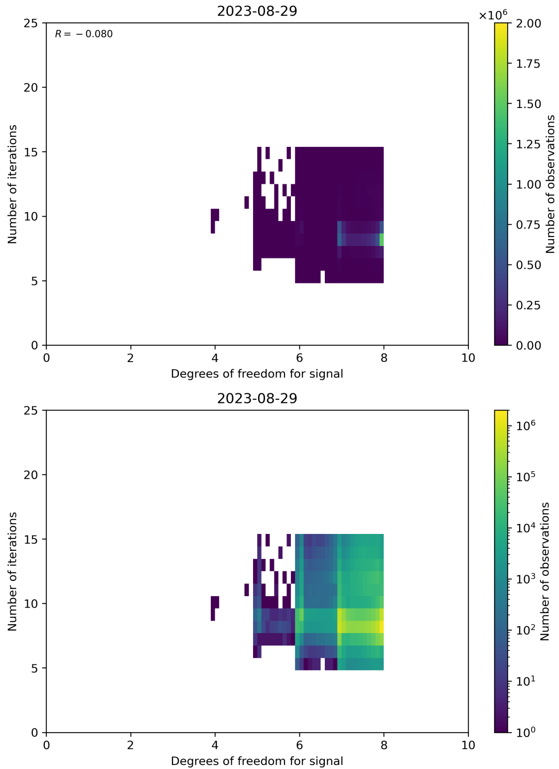
Figure 50: Scatter density plot of “Degrees of freedom for signal” against “Number of iterations” for 2023-08-28 to 2023-08-30.
