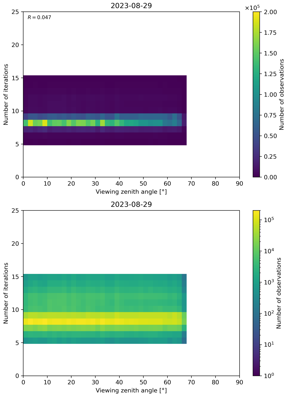
Figure 75: Scatter density plot of “Viewing zenith angle” against “Number of iterations” for 2023-08-28 to 2023-08-30.
