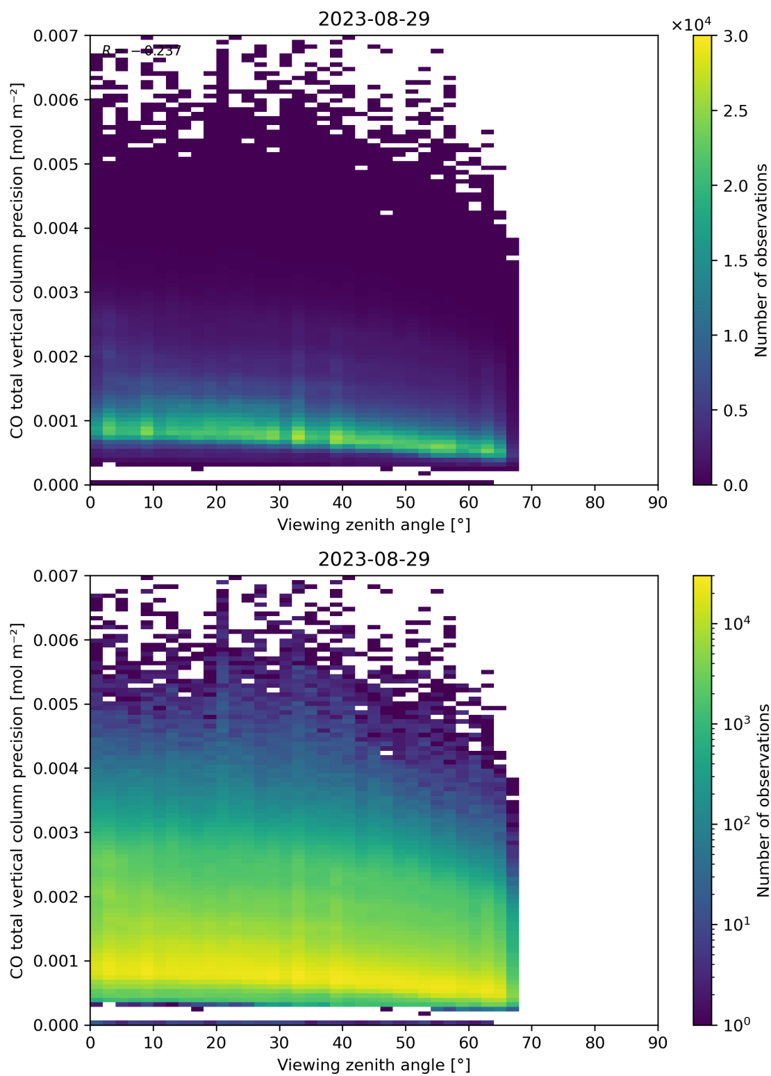
Figure 71: Scatter density plot of “Viewing zenith angle” against “CO total vertical column precision” for 2023-08-28 to 2023-08-30.
