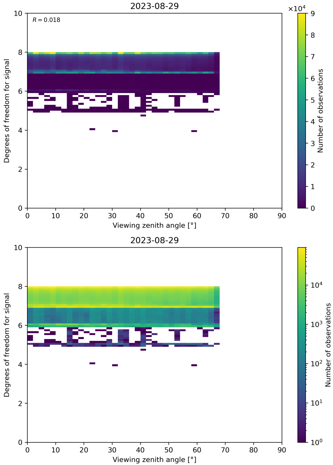
Figure 73: Scatter density plot of “Viewing zenith angle” against “Degrees of freedom for signal” for 2023-08-28 to 2023-08-30.
