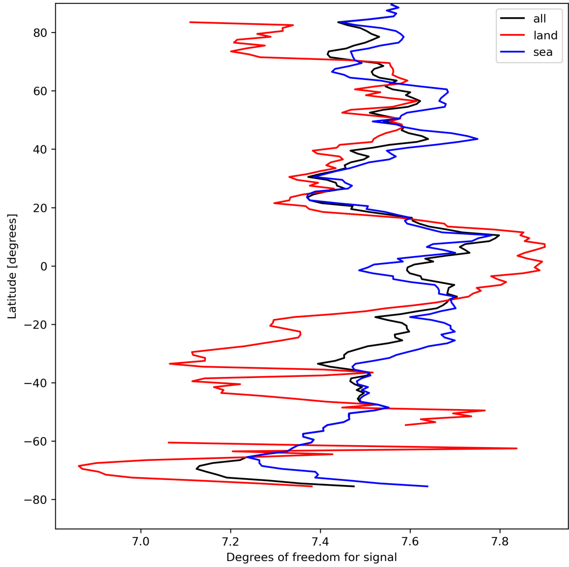
Figure 15: Zonal average of “Degrees of freedom for signal” for 2023-08-28 to 2023-08-30.
