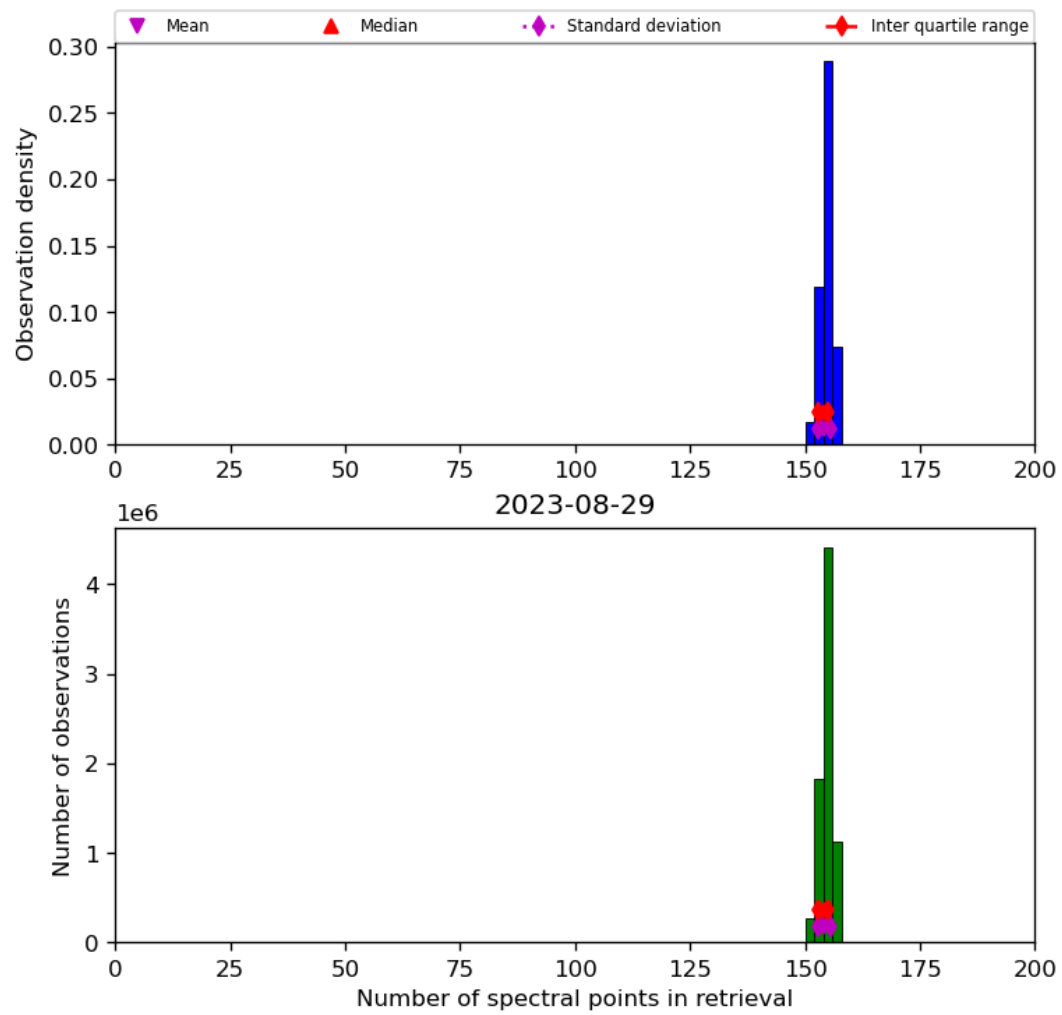
Figure 21: Histogram of “Number of spectral points in retrieval” for 2023-08-28 to 2023-08-30
