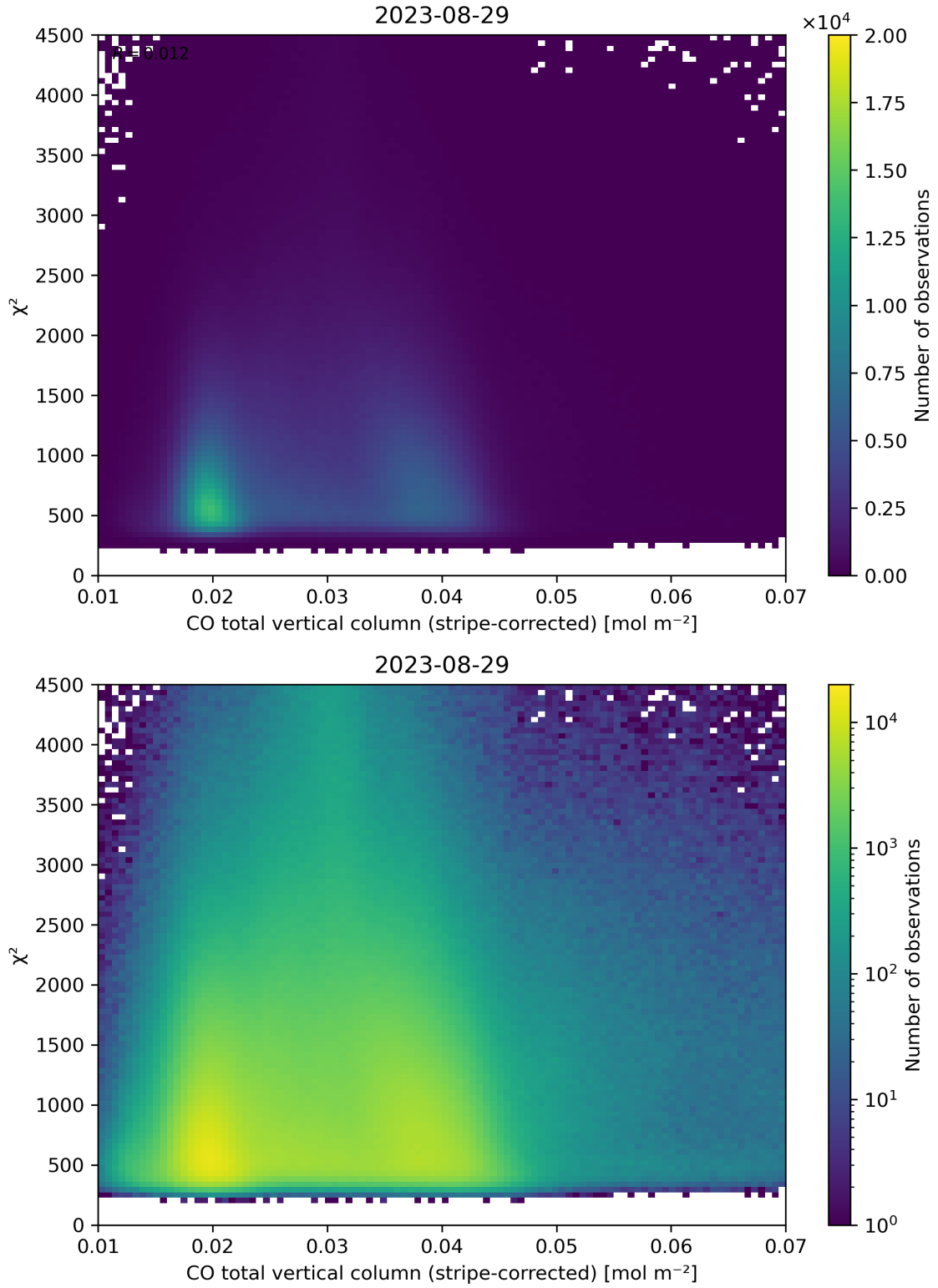
Figure 37: Scatter density plot of “CO total vertical column (stripe-corrected)” against “ \chi^2 ” for 2023-08-28 to 2023-08-30.
