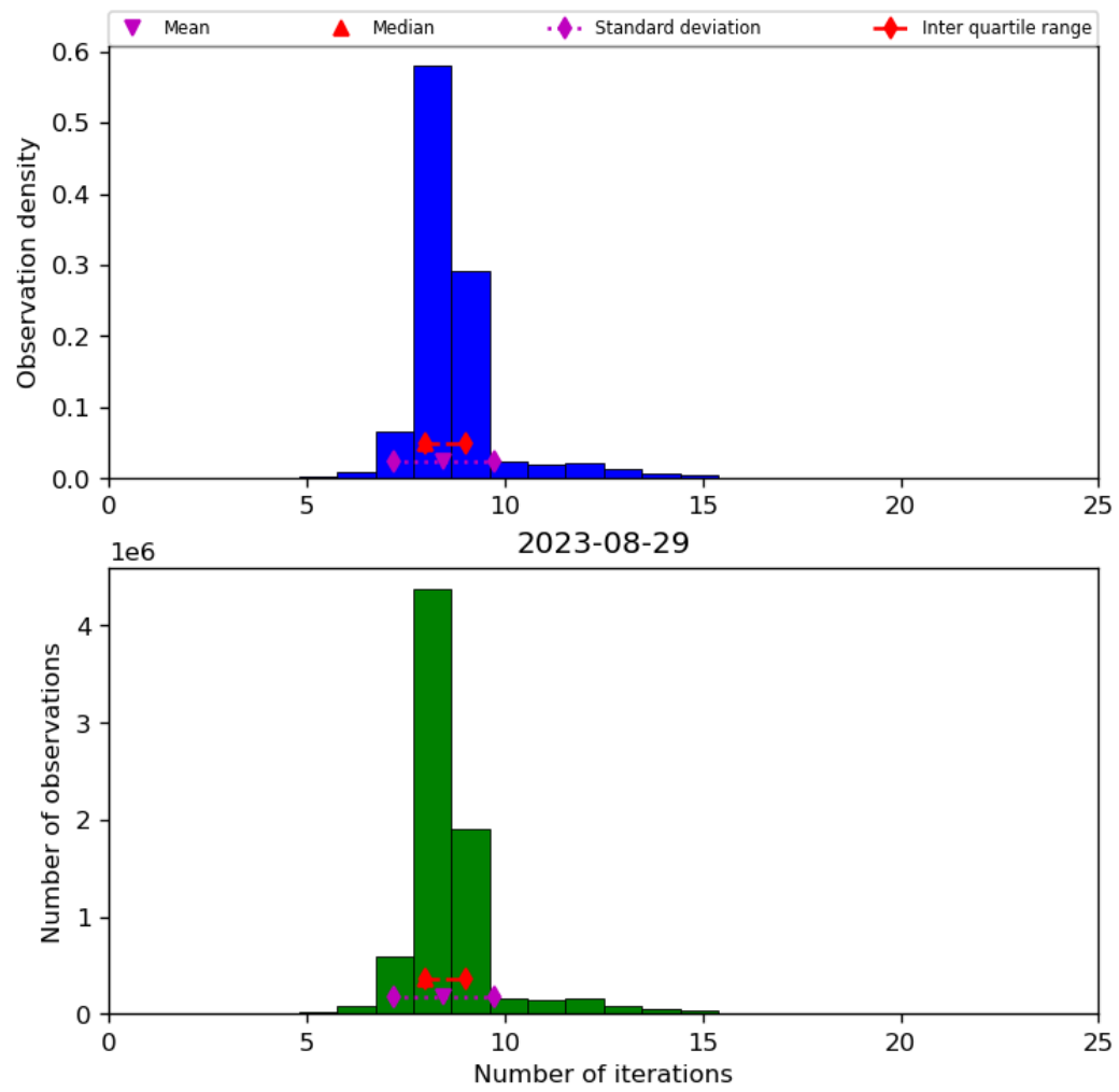
Figure 24: Histogram of “Number of iterations” for 2023-08-28 to 2023-08-30
