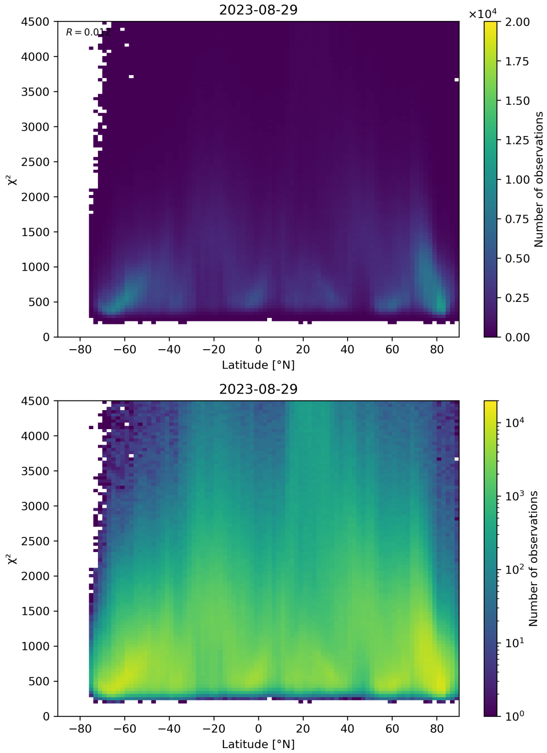
Figure 54: Scatter density plot of “Latitude” against “ \chi^2 ” for 2023-08-28 to 2023-08-30.
