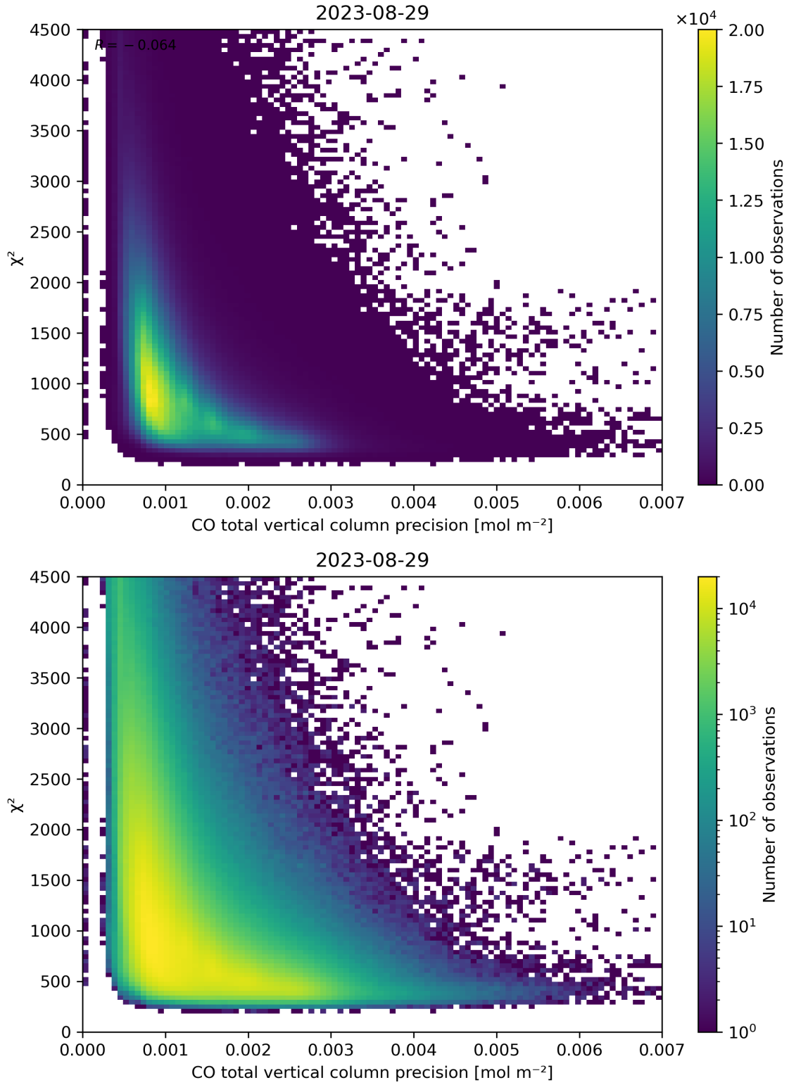
Figure 44: Scatter density plot of “CO total vertical column precision” against “ \chi^2 ” for 2023-08-28 to 2023-08-30.
