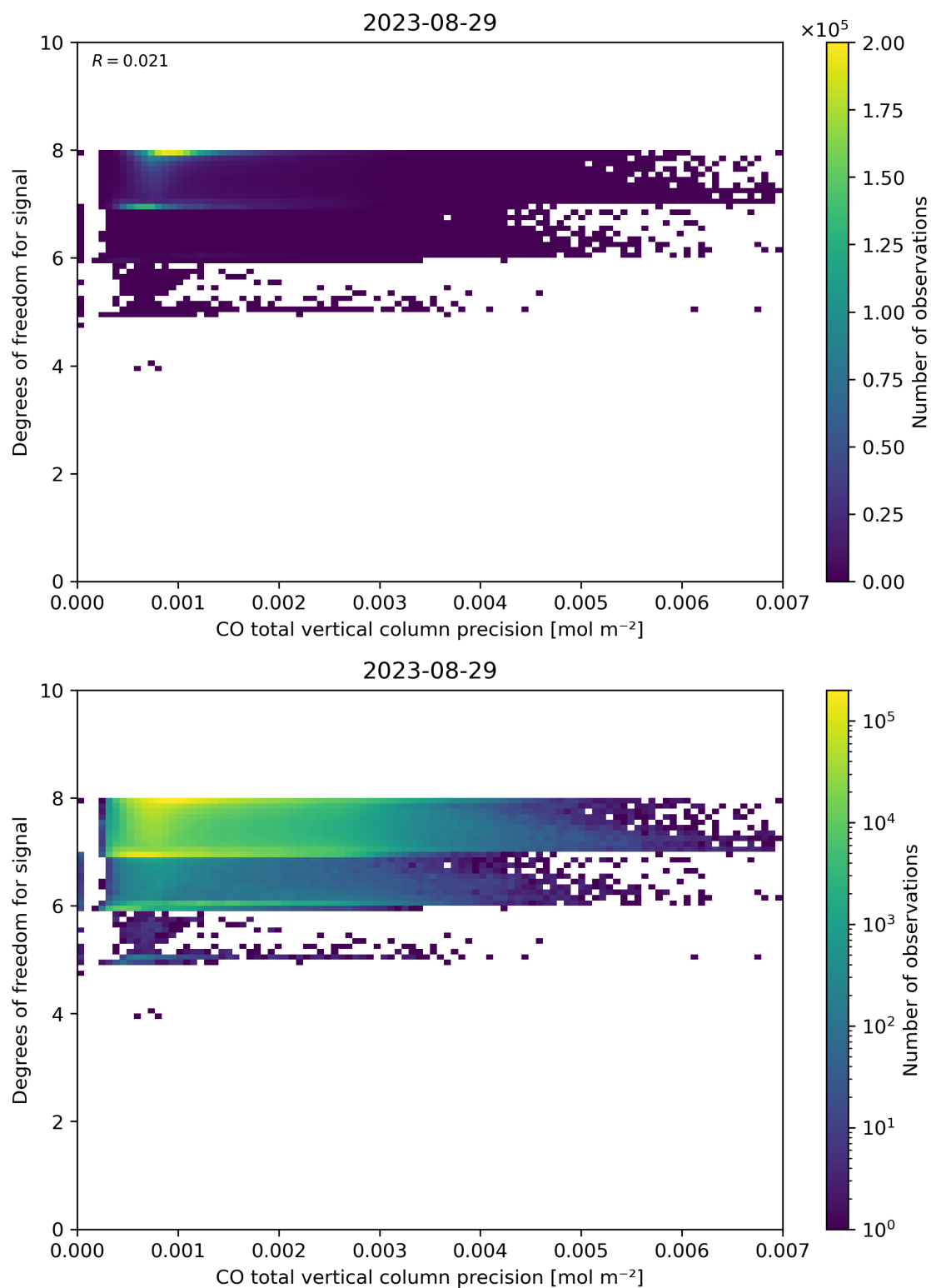
Figure 45: Scatter density plot of “CO total vertical column precision” against “Degrees of freedom for signal” for 2023-08-28 to 2023-08-30.
