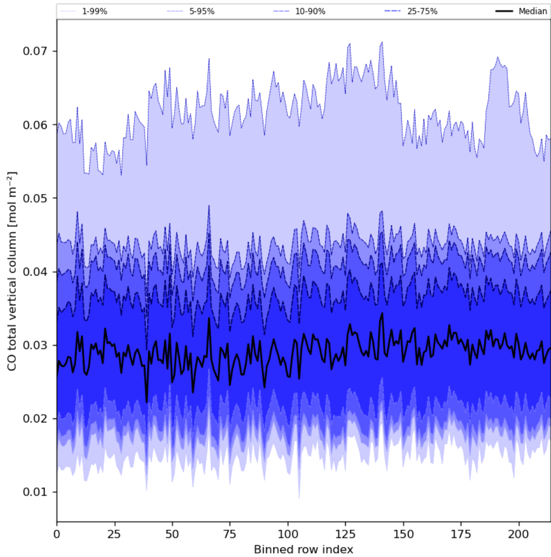
Figure 26: Along track statistics of “CO total vertical column” for 2023-08-28 to 2023-08-30
