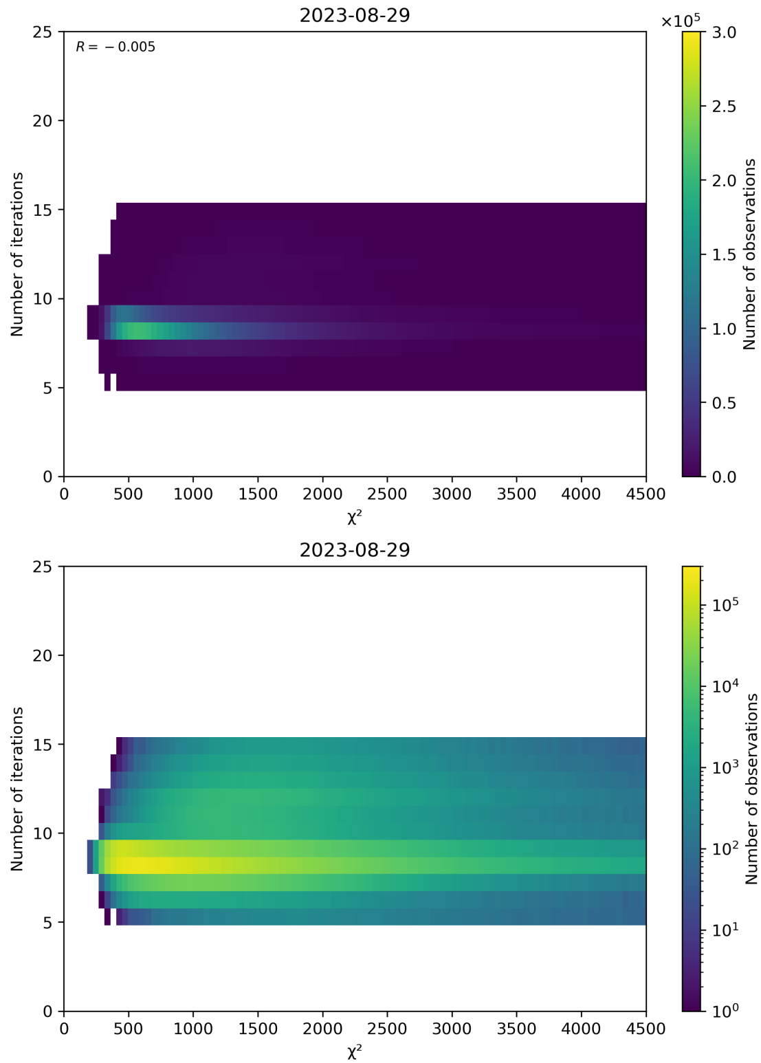
Figure 49: Scatter density plot of “ \chi^2 ” against “Number of iterations” for 2023-08-28 to 2023-08-30.
