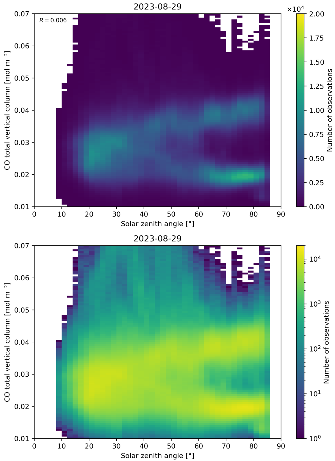
Figure 61: Scatter density plot of “Solar zenith angle” against “CO total vertical column” for 2023-08-28 to 2023-08-30.
