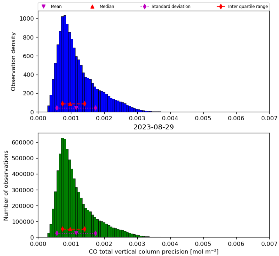
Figure 20: Histogram of “CO total vertical column precision” for 2023-08-28 to 2023-08-30
