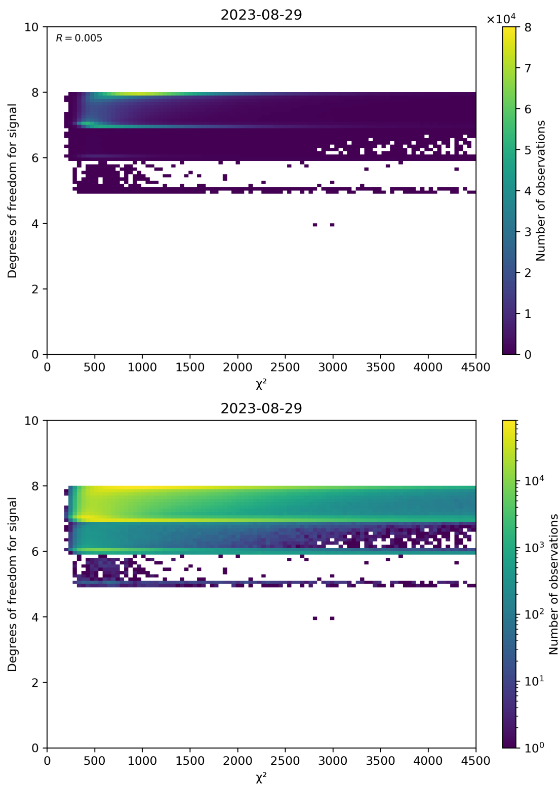
Figure 48: Scatter density plot of “ \chi^2 ” against “Degrees of freedom for signal” for 2023-08-28 to 2023-08-30.
