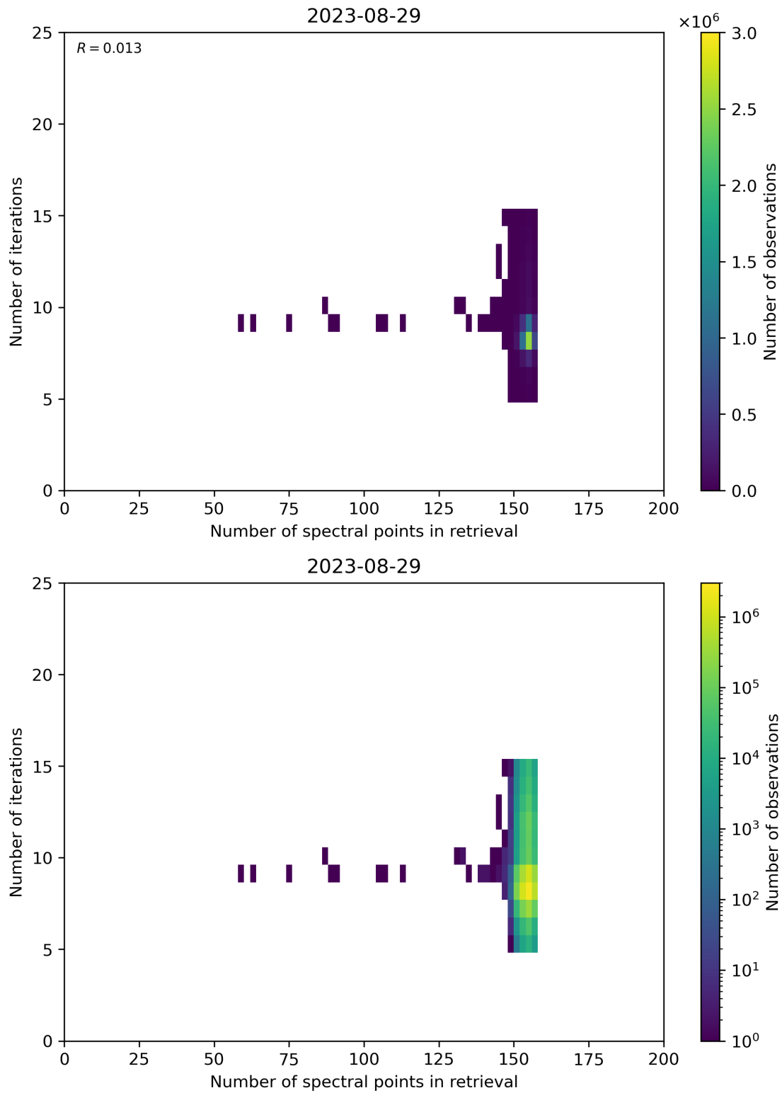
Figure 60: Scatter density plot of “Number of spectral points in retrieval” against “Number of iterations” for 2023-08-28 to 2023-08-30.
