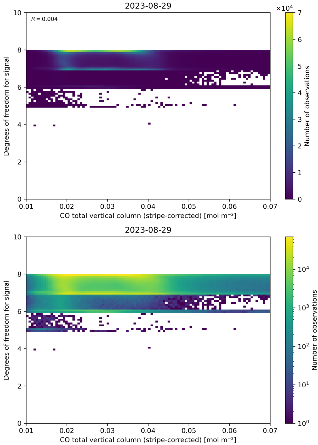
Figure 38: Scatter density plot of “CO total vertical column (stripe-corrected)” against “Degrees of freedom for signal” for 2023-08-28 to 2023-08-30.
