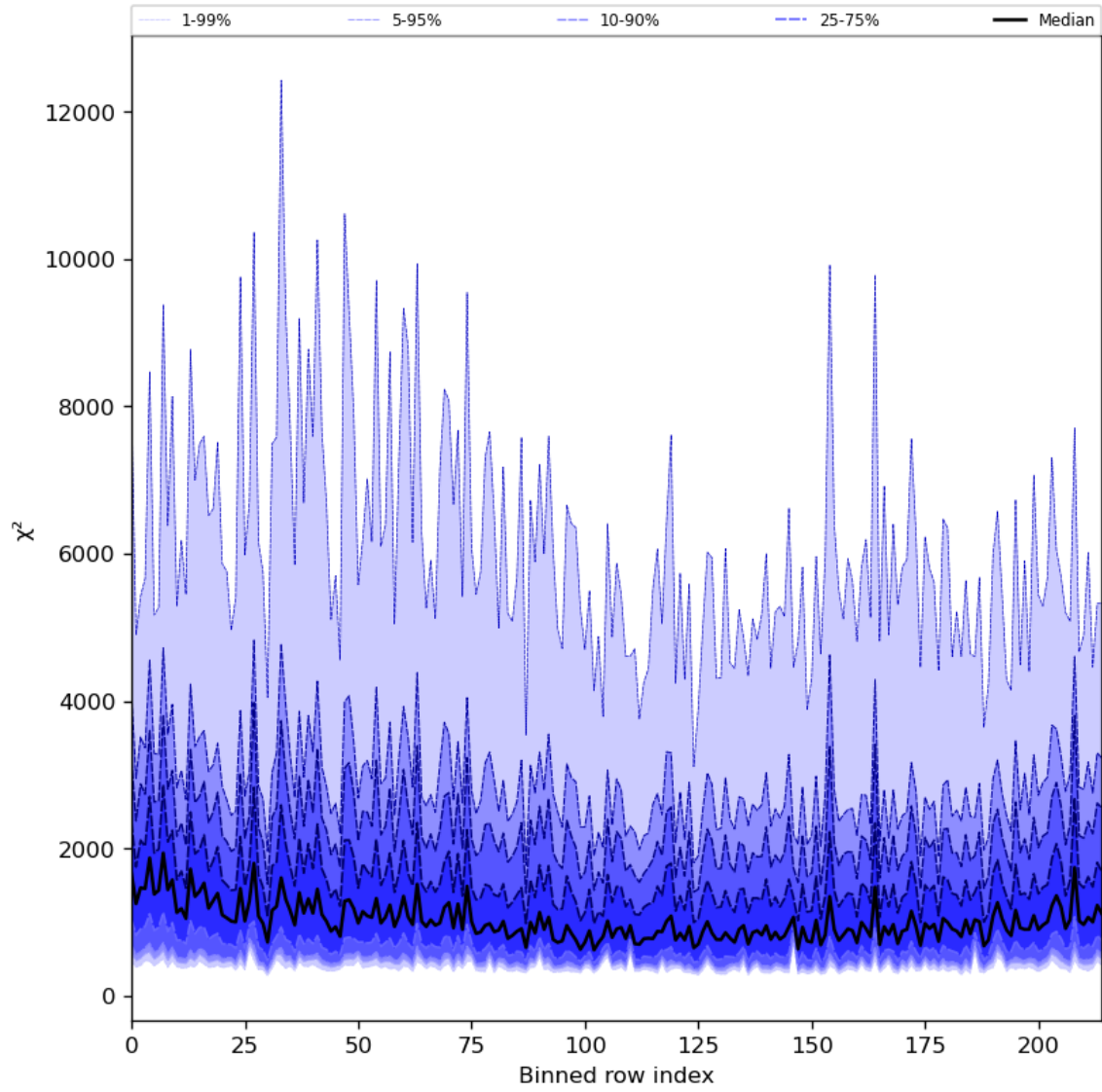
Figure 30: Along track statistics of “ \chi^2 ” for 2023-08-28 to 2023-08-30
