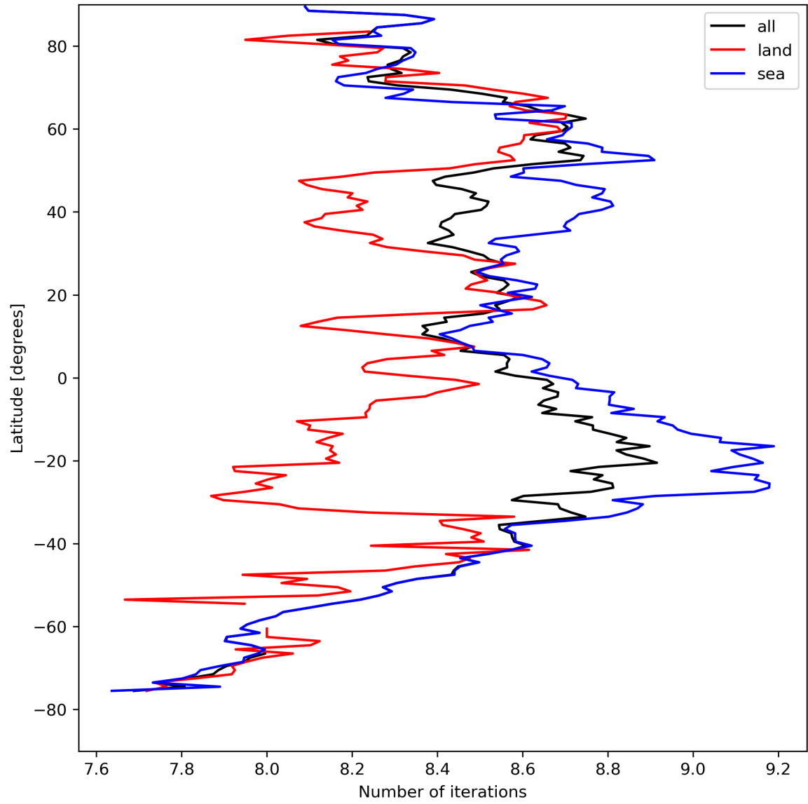
Figure 16: Zonal average of “Number of iterations” for 2023-08-28 to 2023-08-30.
