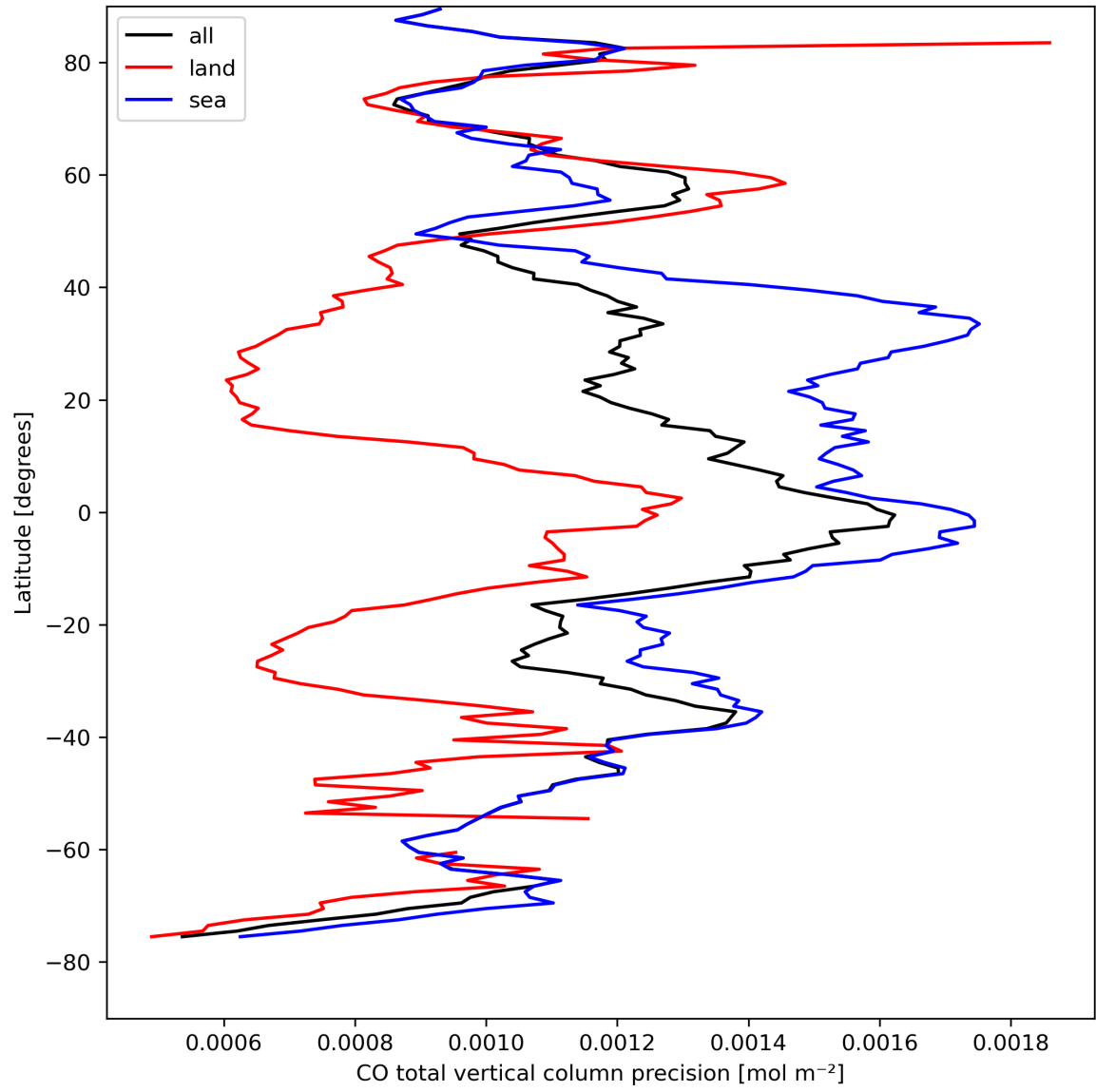
Figure 12: Zonal average of "CO total vertical column precision" for 2023-08-28 to 2023-08-30.
