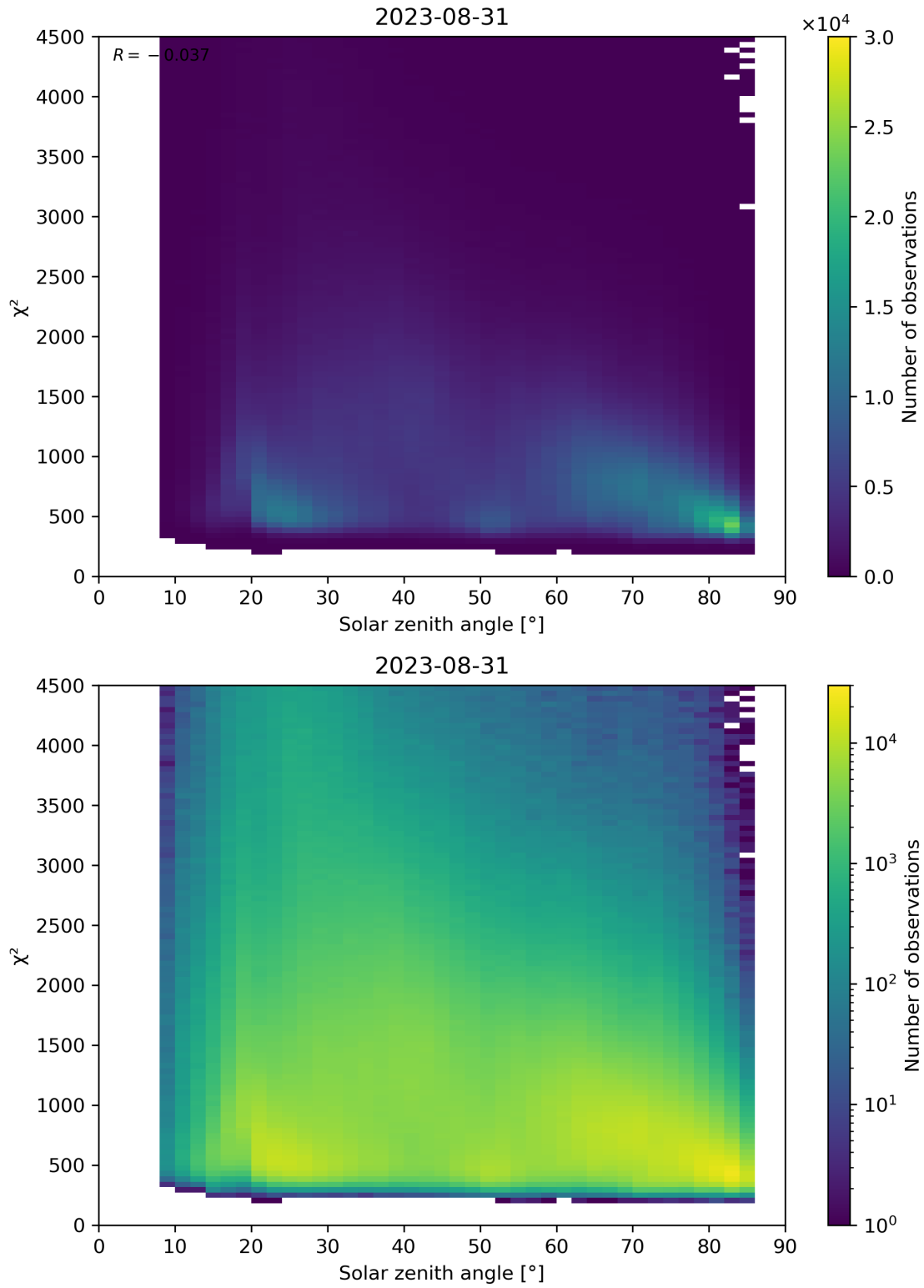
Figure 64: Scatter density plot of “Solar zenith angle” against “ \chi^2 ” for 2023-08-30 to 2023-09-01.
