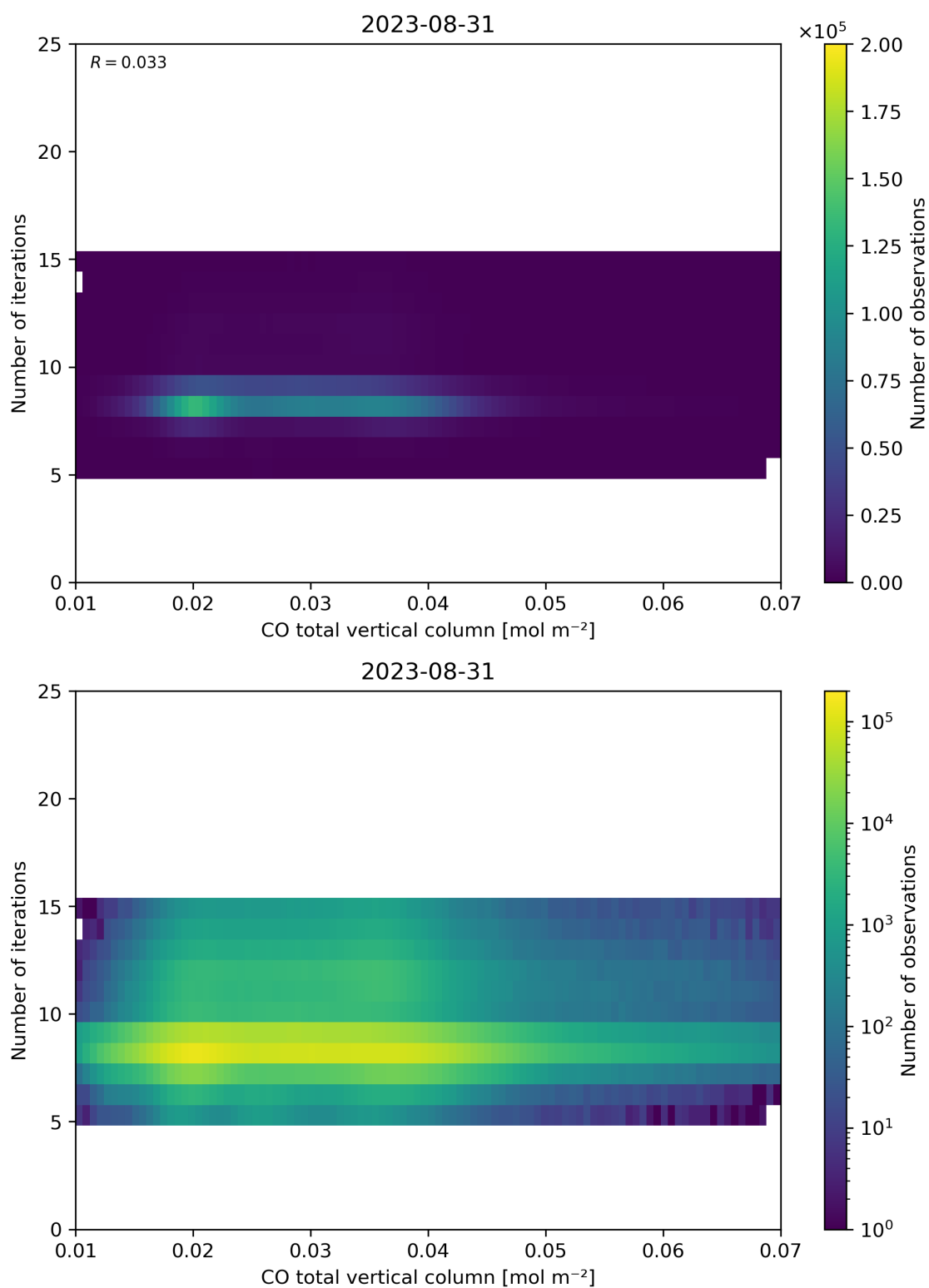
Figure 42: Scatter density plot of “CO total vertical column” against “Number of iterations” for 2023-08-30 to 2023-09-01.
