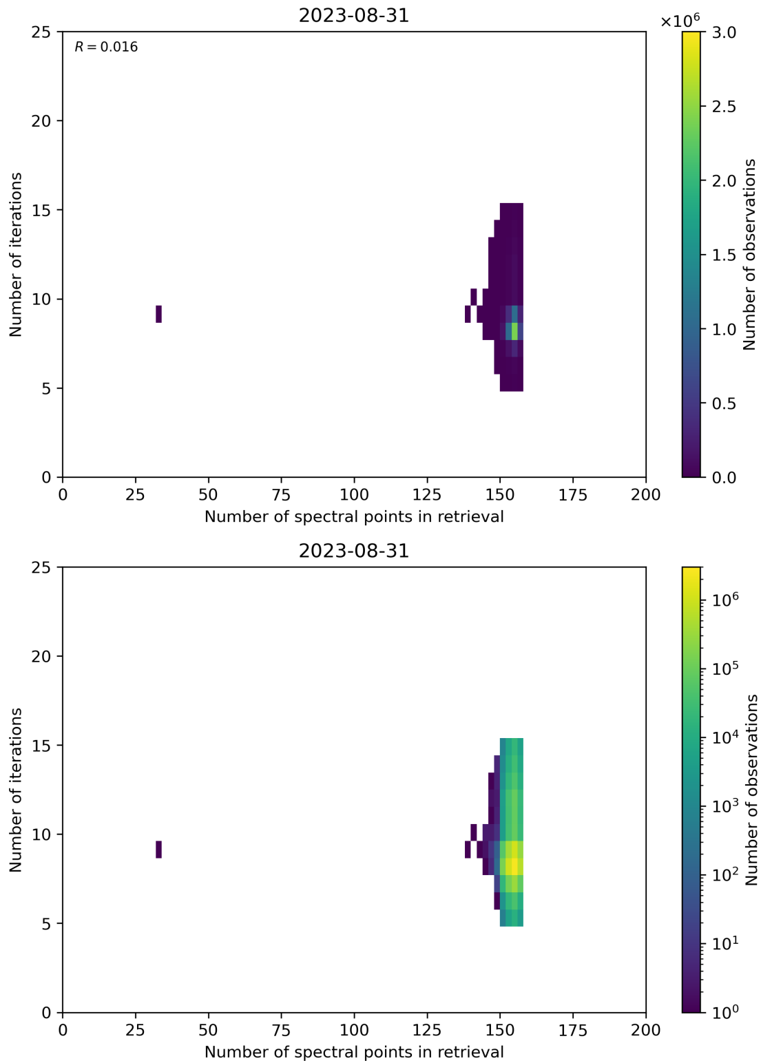
Figure 60: Scatter density plot of “Number of spectral points in retrieval” against “Number of iterations” for 2023-08-30 to 2023-09-01.
