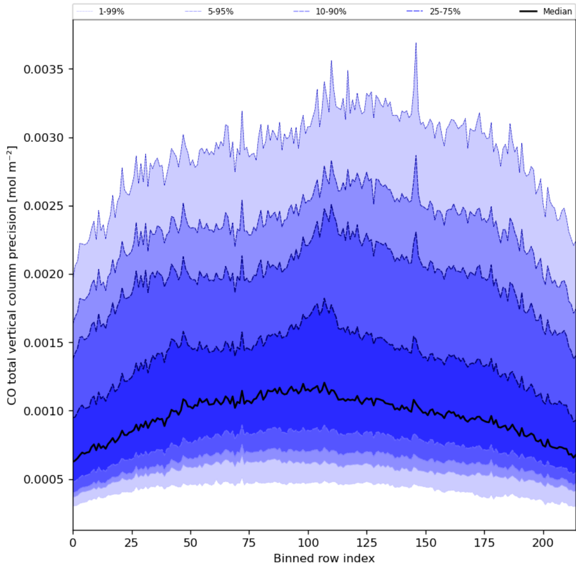
Figure 28: Along track statistics of “CO total vertical column precision” for 2023-08-30 to 2023-09-01
