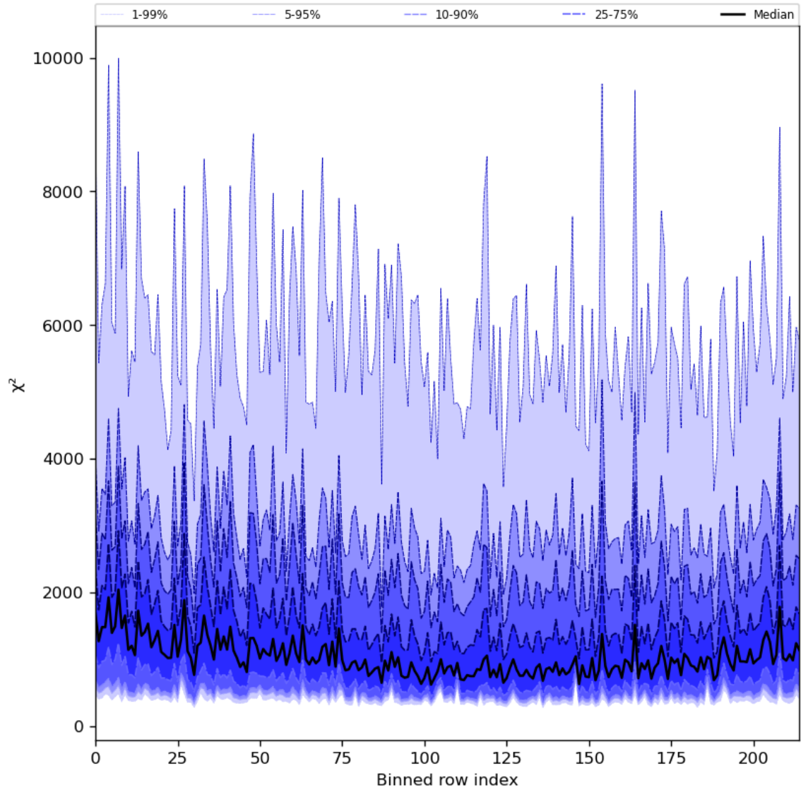
Figure 30: Along track statistics of “ \chi^2 ” for 2023-08-30 to 2023-09-01
