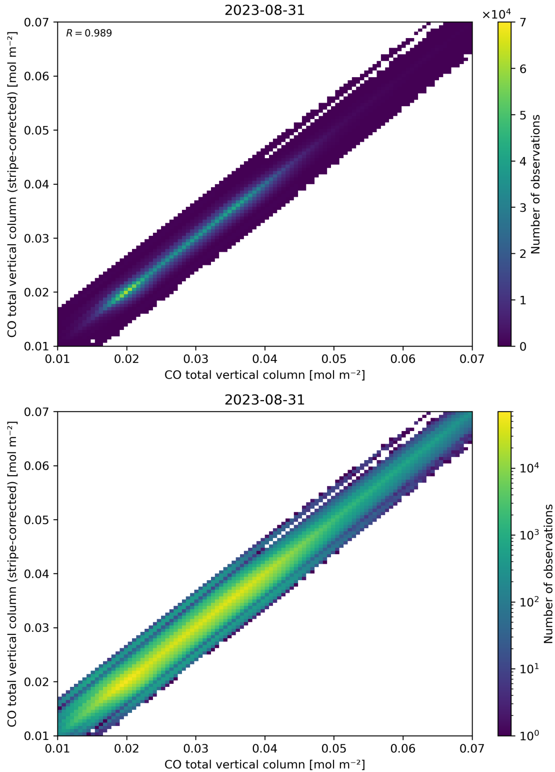
Figure 33: Scatter density plot of “CO total vertical column” against “CO total vertical column (stripe-corrected)” for 2023-08-30 to 2023-09-01.
