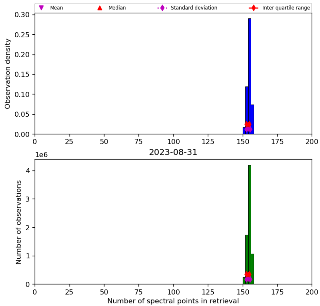
Figure 21: Histogram of “Number of spectral points in retrieval” for 2023-08-30 to 2023-09-01
