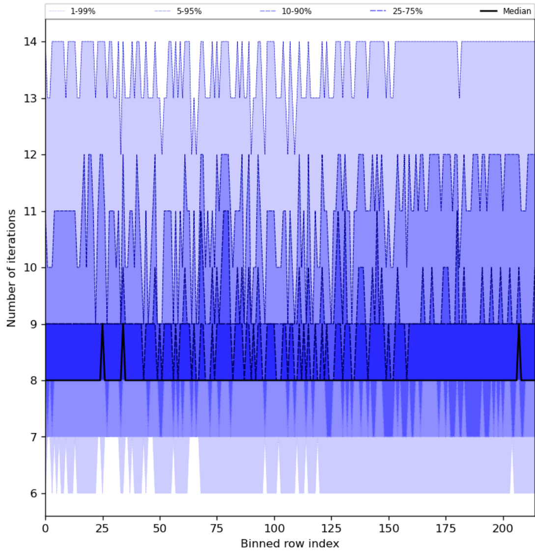
Figure 32: Along track statistics of “Number of iterations” for 2023-08-30 to 2023-09-01
