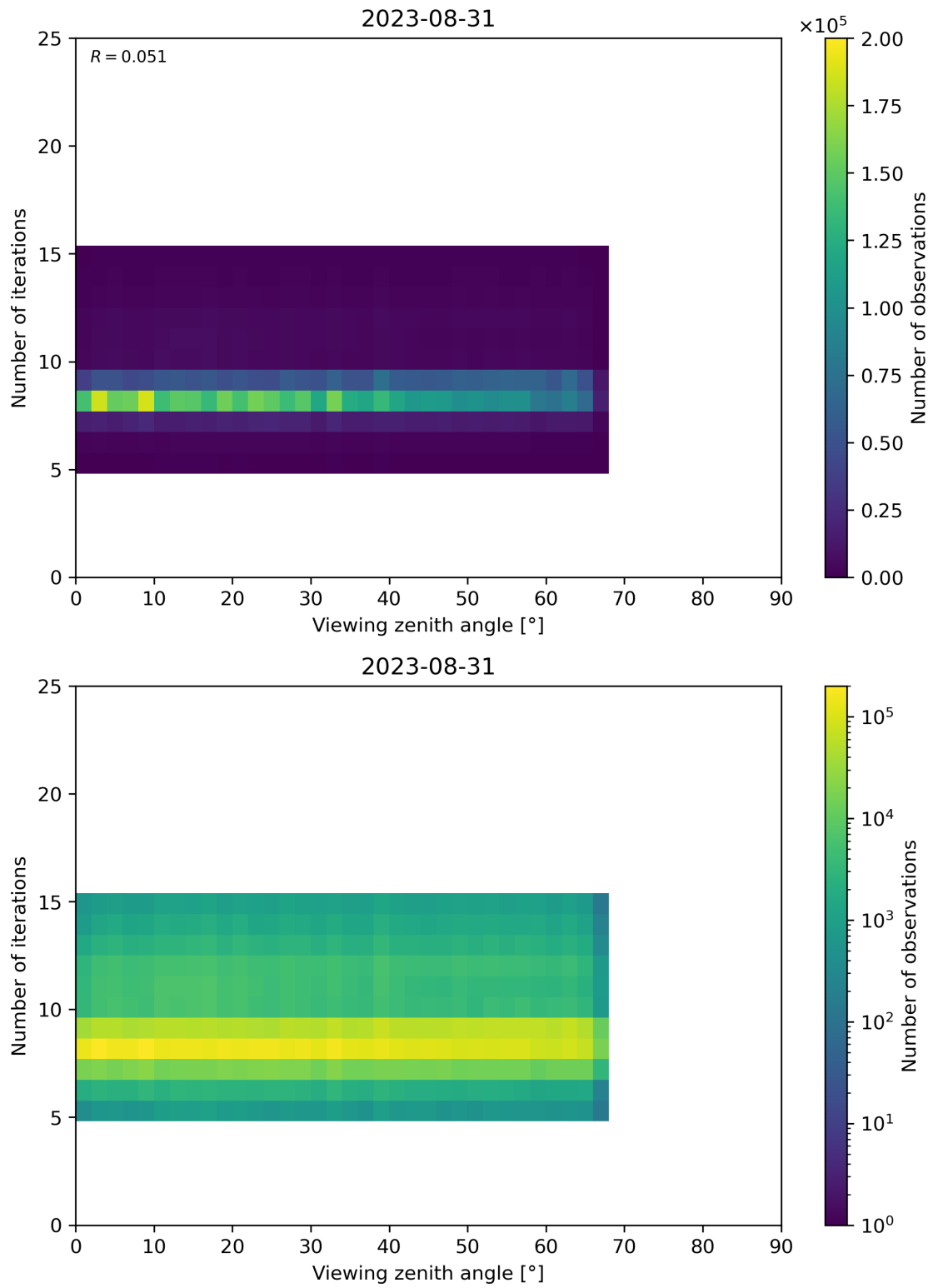
Figure 75: Scatter density plot of “Viewing zenith angle” against “Number of iterations” for 2023-08-30 to 2023-09-01.
