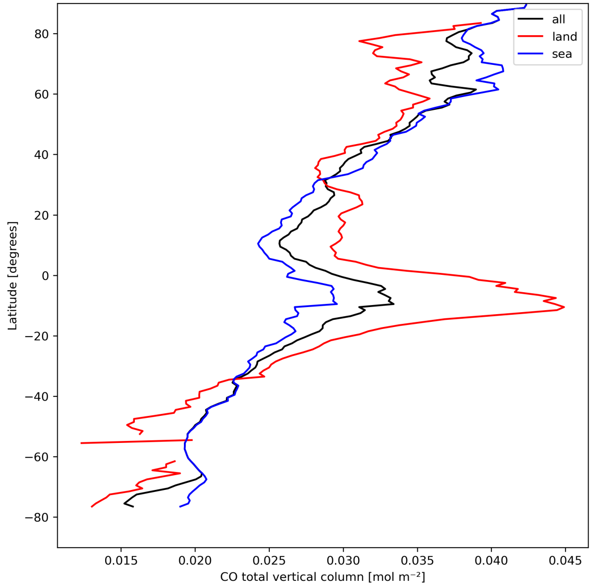
Figure 10: Zonal average of “CO total vertical column” for 2023-08-30 to 2023-09-01.
