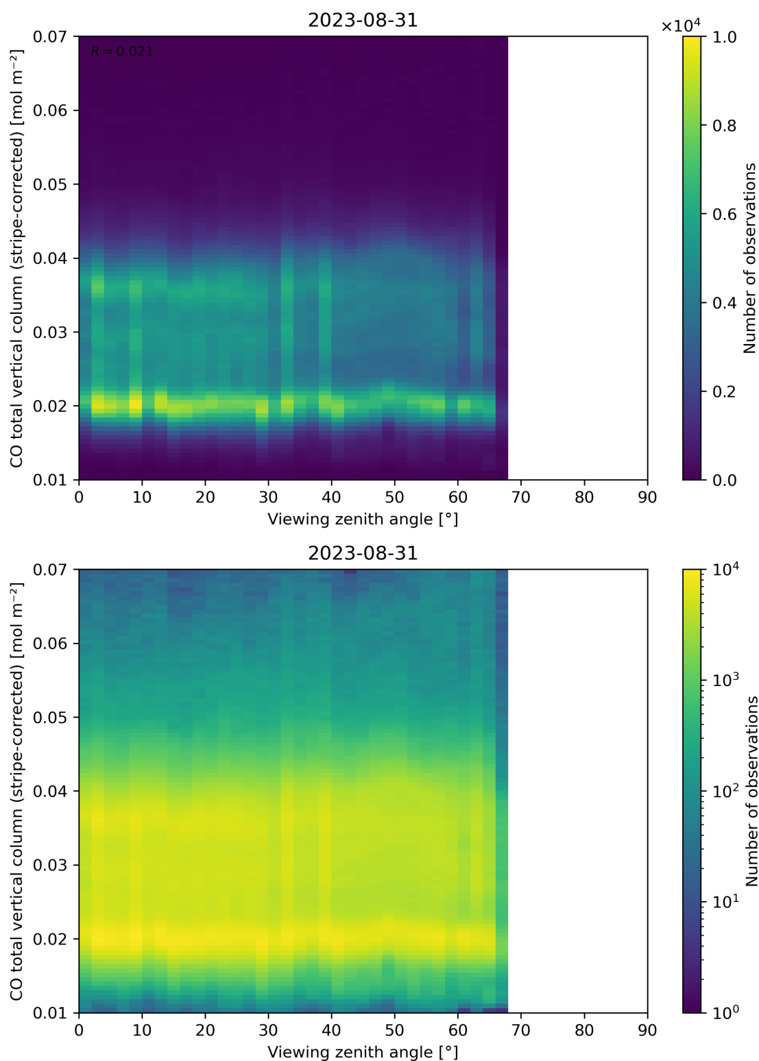
Figure 70: Scatter density plot of “Viewing zenith angle” against “CO total vertical column (stripe-corrected)” for 2023-08-30 to 2023-09-01.
