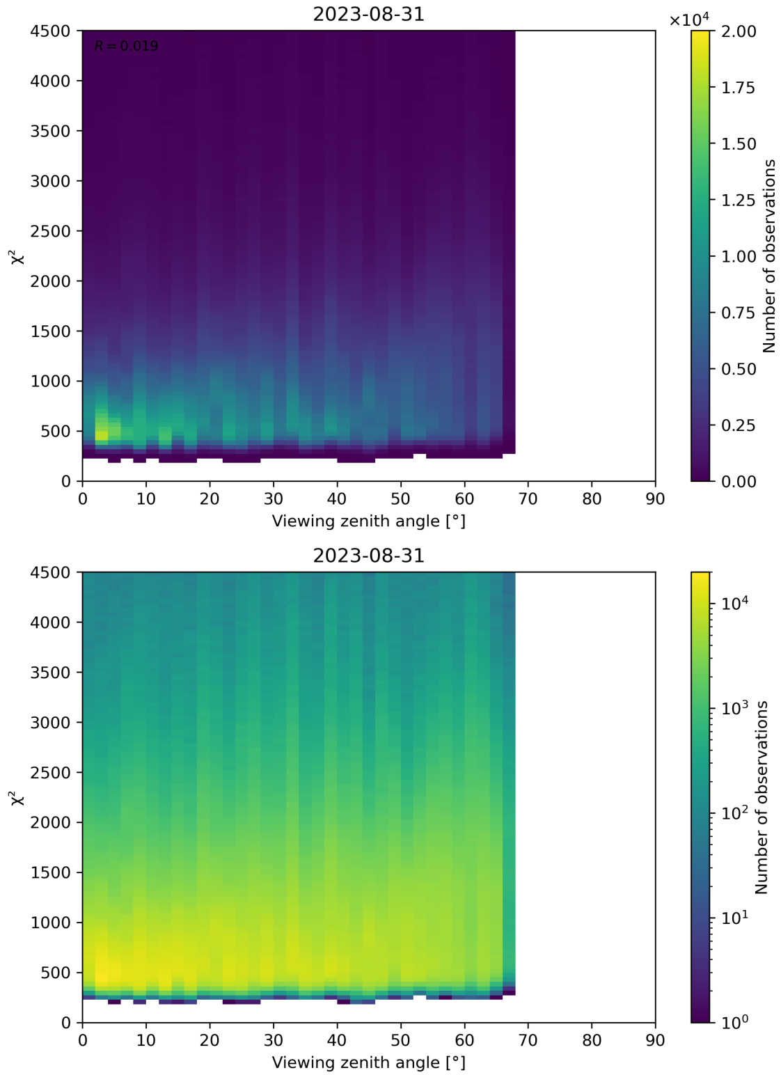
Figure 72: Scatter density plot of “Viewing zenith angle” against “ \chi^2 ” for 2023-08-30 to 2023-09-01.
