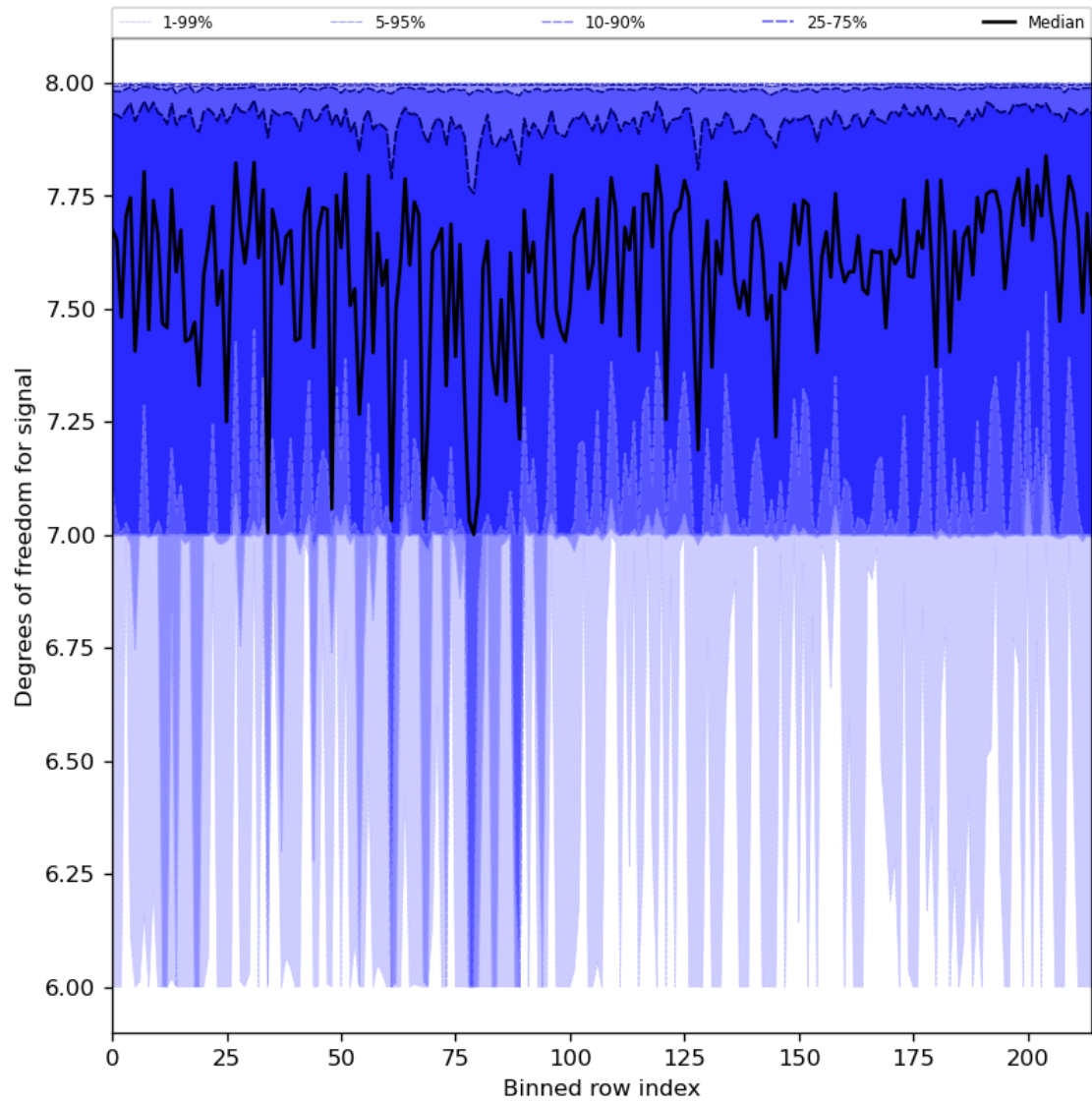
Figure 31: Along track statistics of “Degrees of freedom for signal” for 2023-08-30 to 2023-09-01
