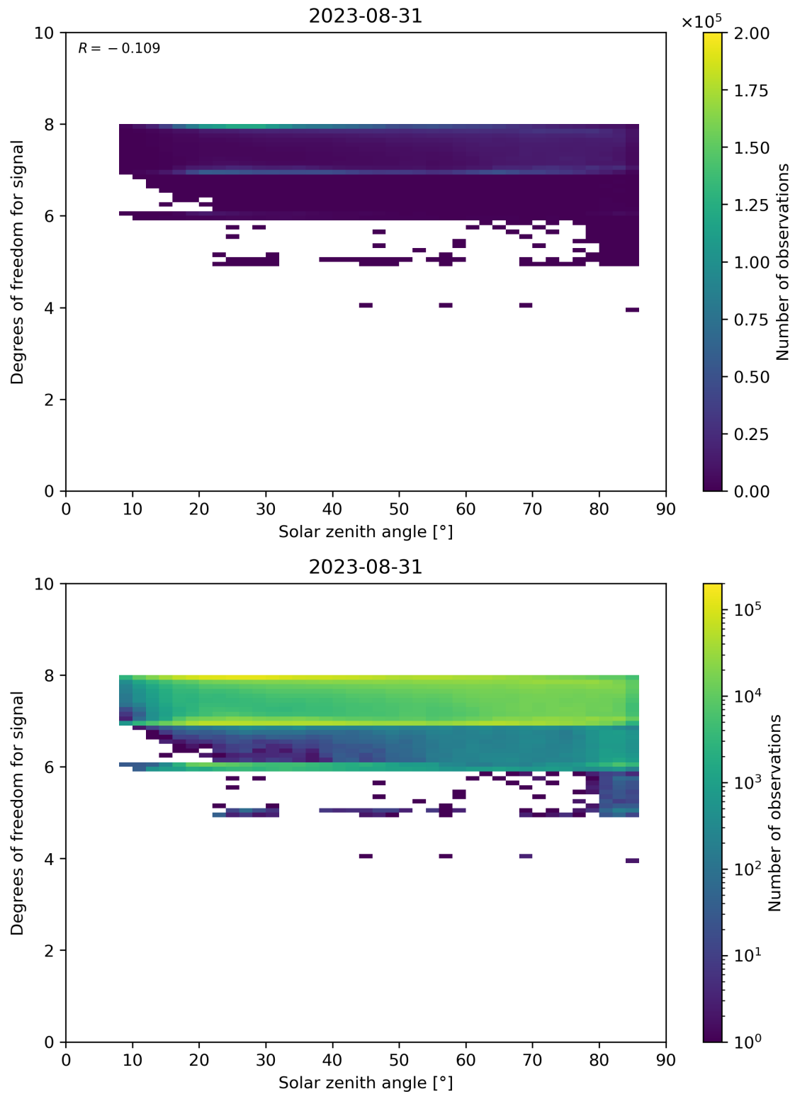
Figure 65: Scatter density plot of “Solar zenith angle” against “Degrees of freedom for signal” for 2023-08-30 to 2023-09-01.
