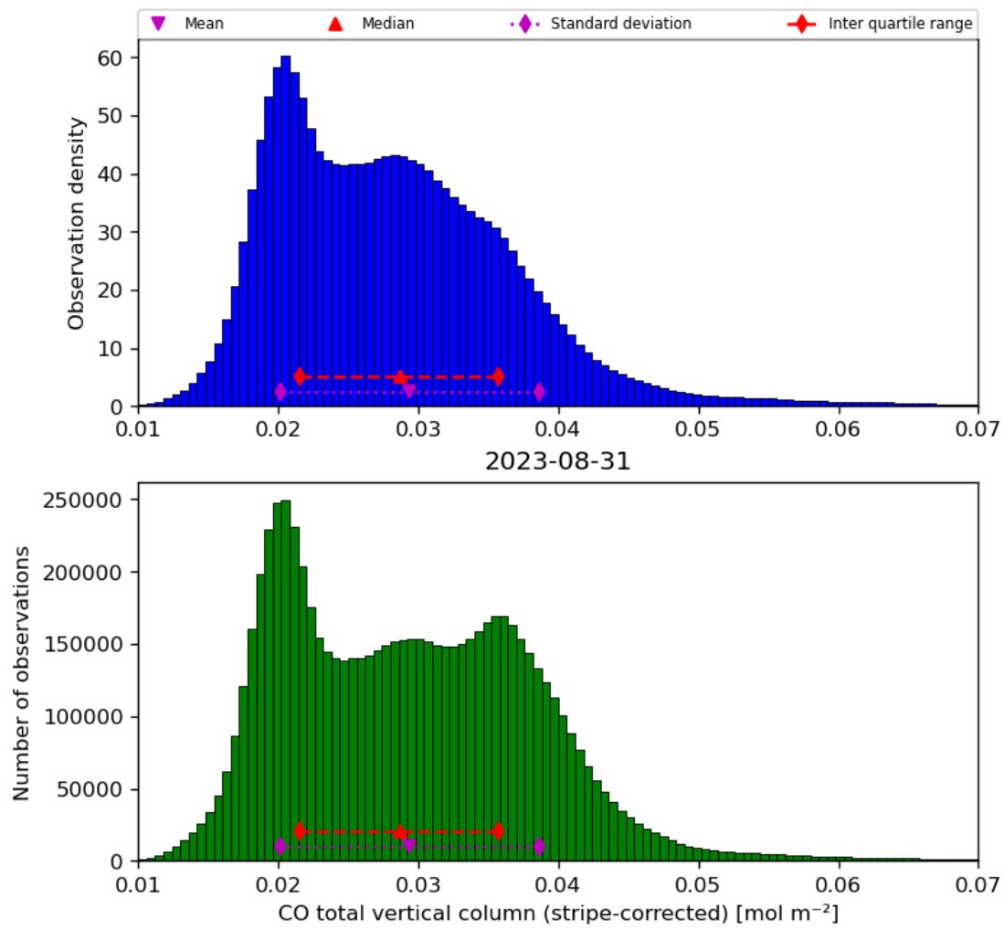
Figure 19: Histogram of “CO total vertical column (stripe-corrected)” for 2023-08-30 to 2023-09-01
