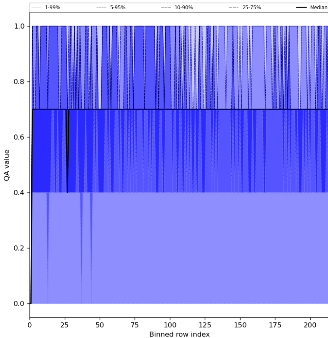
Figure 25: Along track statistics of “QA value” for 2023-08-30 to 2023-09-01
