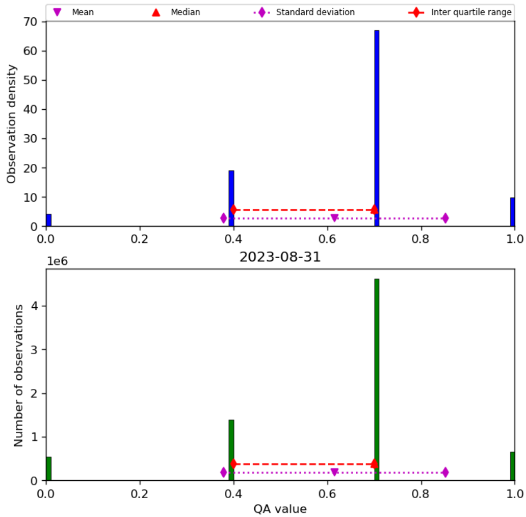
Figure 17: Histogram of "QA value" for 2023-08-30 to 2023-09-01
