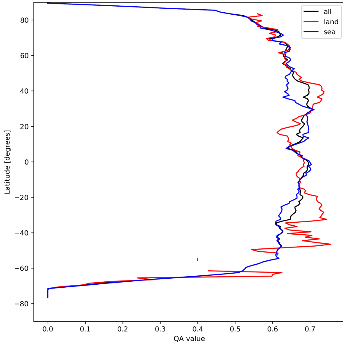
Figure 9: Zonal average of “QA value” for 2023-08-30 to 2023-09-01.
