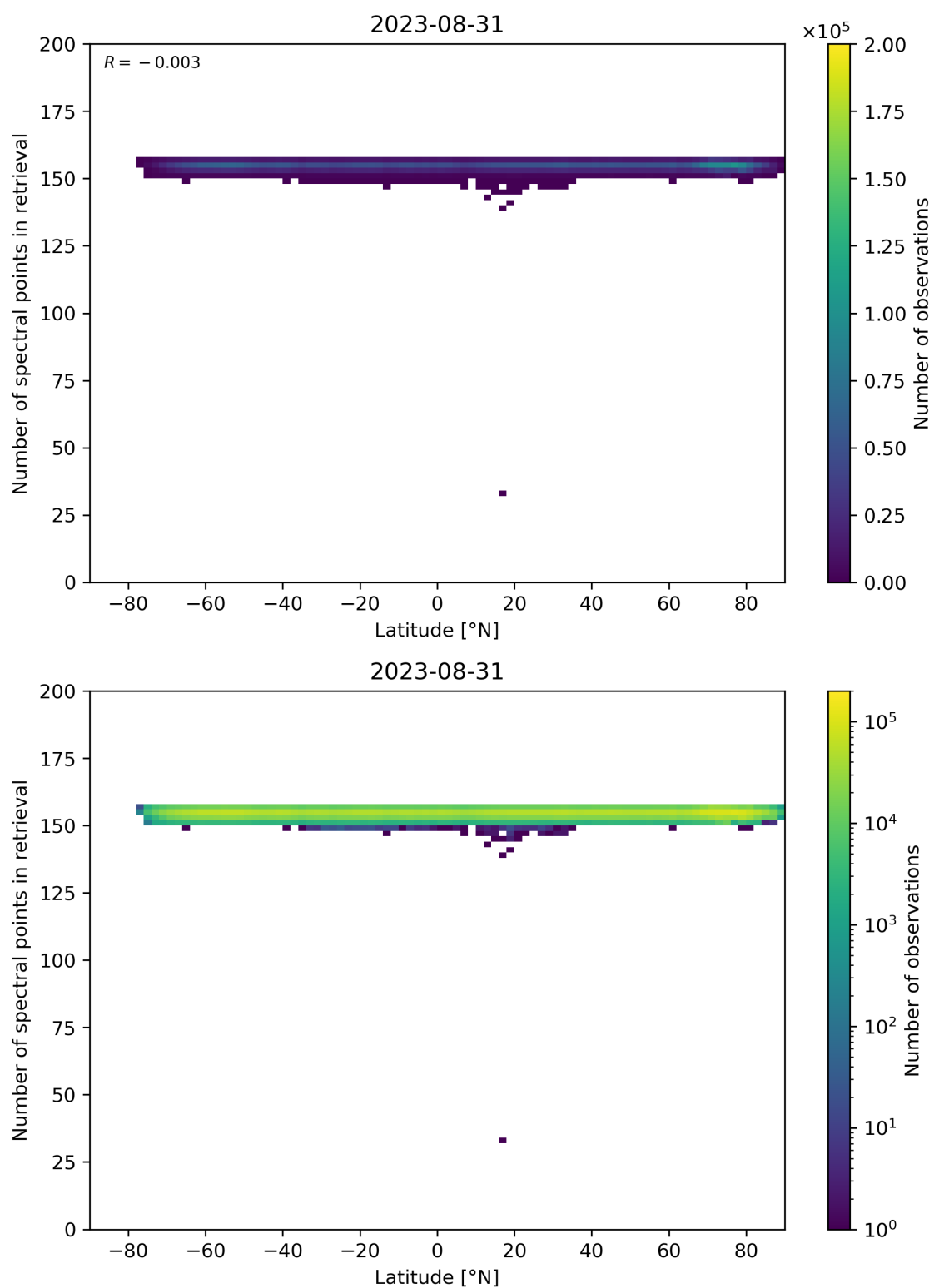
Figure 57: Scatter density plot of “Latitude” against “Number of spectral points in retrieval” for 2023-08-30 to 2023-09-01.
