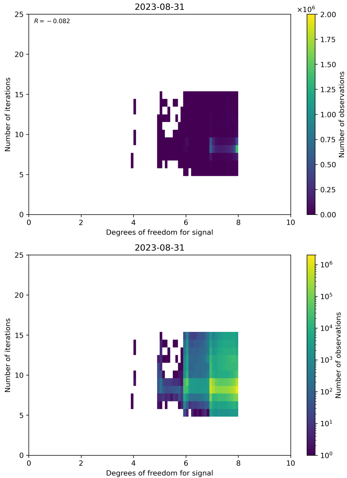
Figure 50: Scatter density plot of “Degrees of freedom for signal” against “Number of iterations” for 2023-08-30 to 2023-09-01.
