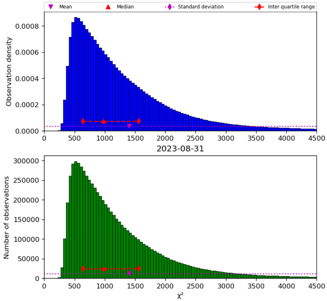
Figure 22: Histogram of “ \chi^2 ” for 2023-08-30 to 2023-09-01
