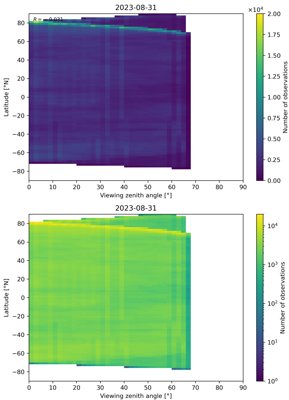
Figure 74: Scatter density plot of “Viewing zenith angle” against “Latitude” for 2023-08-30 to 2023-09-01.
