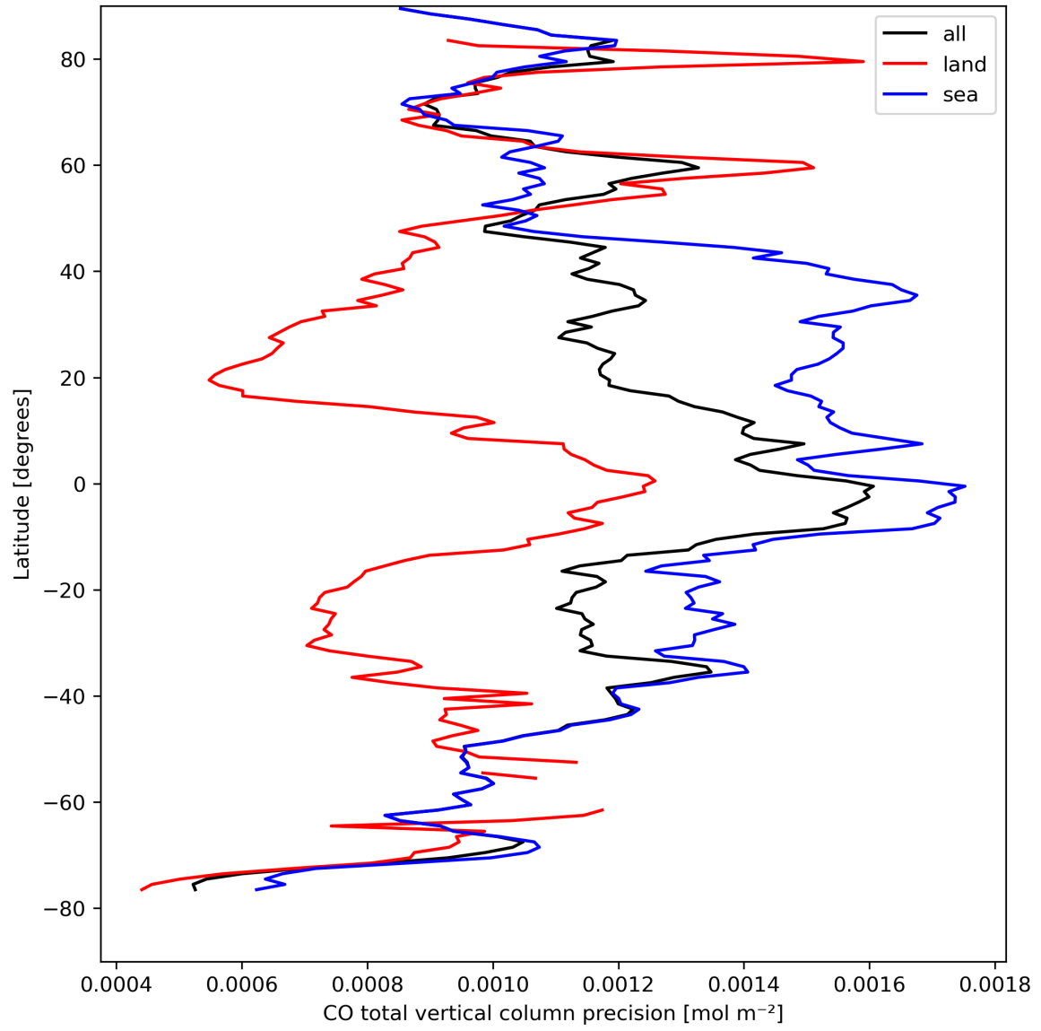
Figure 12: Zonal average of “CO total vertical column precision” for 2023-08-30 to 2023-09-01.
