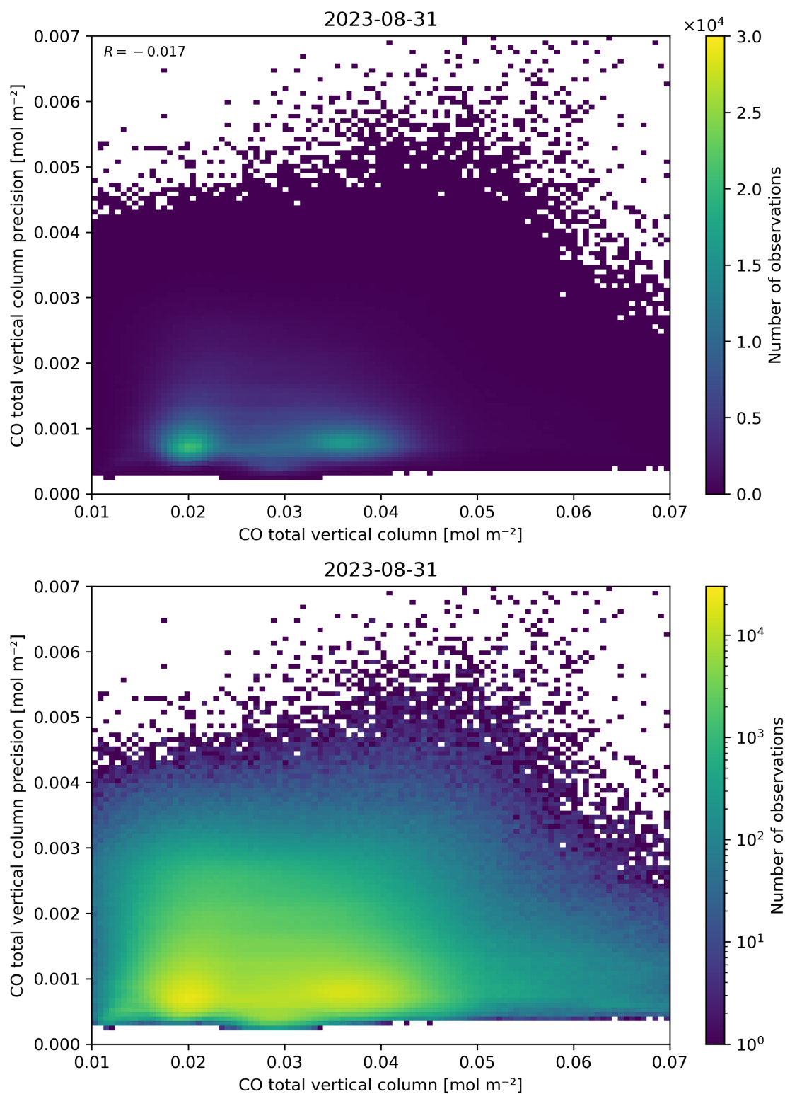
Figure 34: Scatter density plot of “CO total vertical column” against “CO total vertical column precision” for 2023-08-30 to 2023-09-01.
