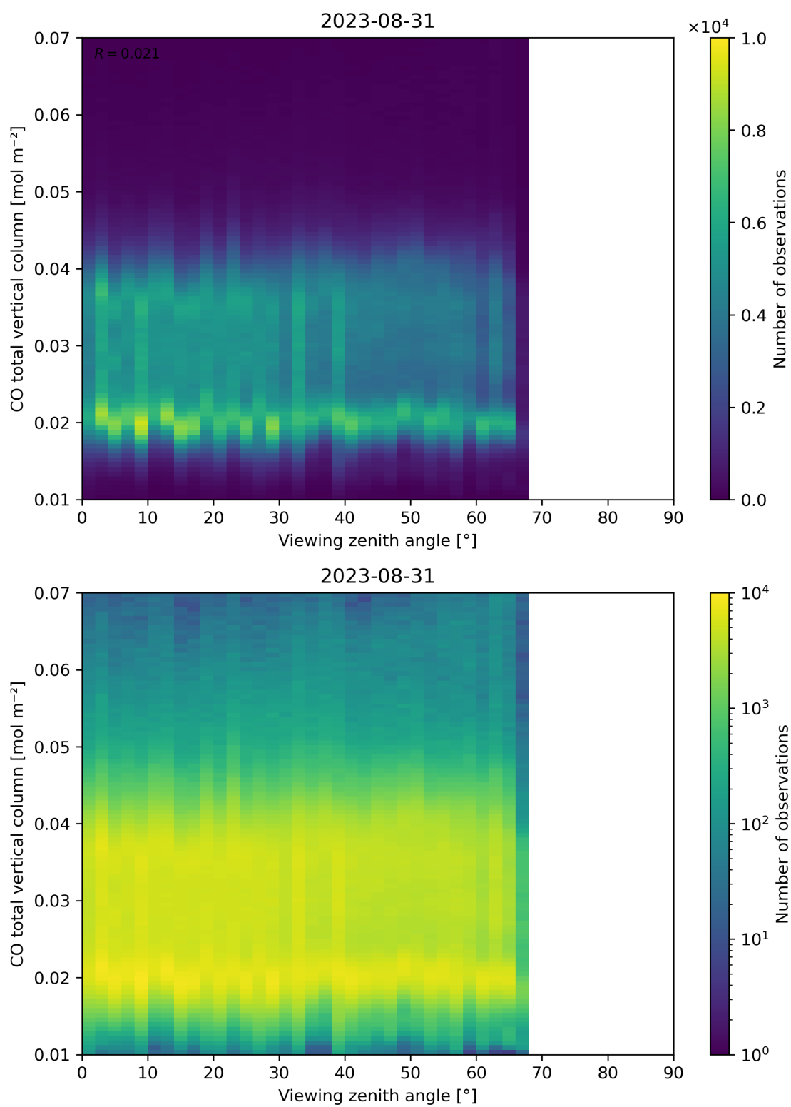
Figure 69: Scatter density plot of “Viewing zenith angle” against “CO total vertical column” for 2023-08-30 to 2023-09-01.
