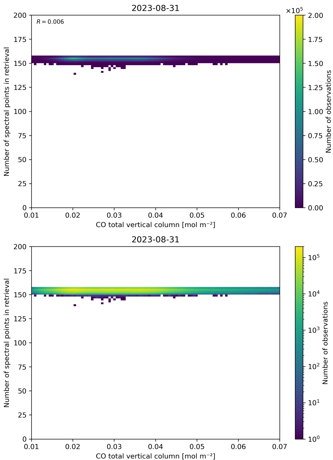
Figure 43: Scatter density plot of “CO total vertical column” against “Number of spectral points in retrieval” for 2023-08-30 to 2023-09-01.
