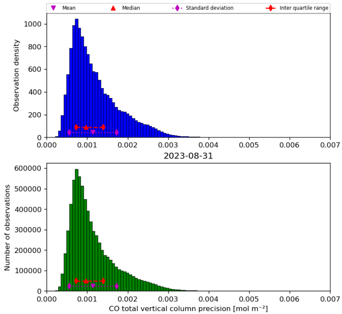
Figure 20: Histogram of “CO total vertical column precision” for 2023-08-30 to 2023-09-01
