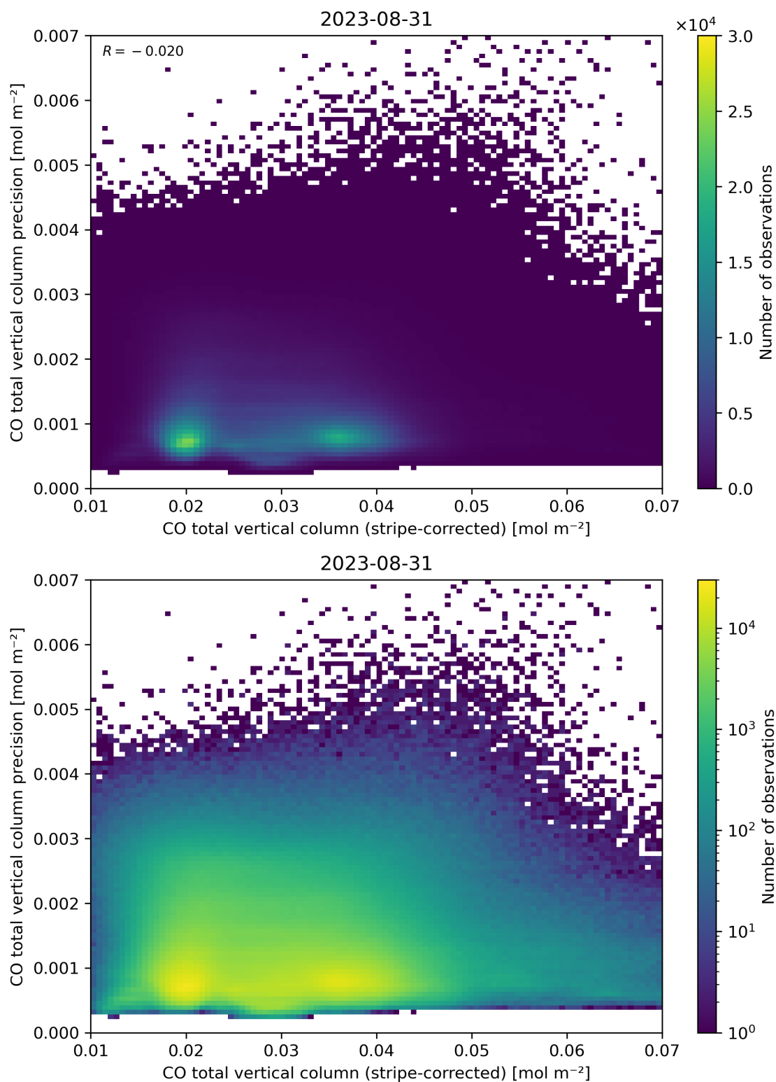
Figure 36: Scatter density plot of “CO total vertical column (stripe-corrected)” against “CO total vertical column precision” for 2023-08-30 to 2023-09-01.
