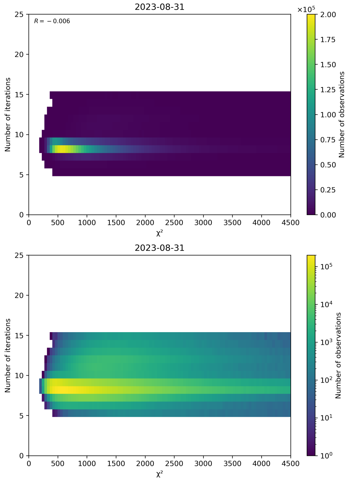
Figure 49: Scatter density plot of “ \chi^2 ” against “Number of iterations” for 2023-08-30 to 2023-09-01.
