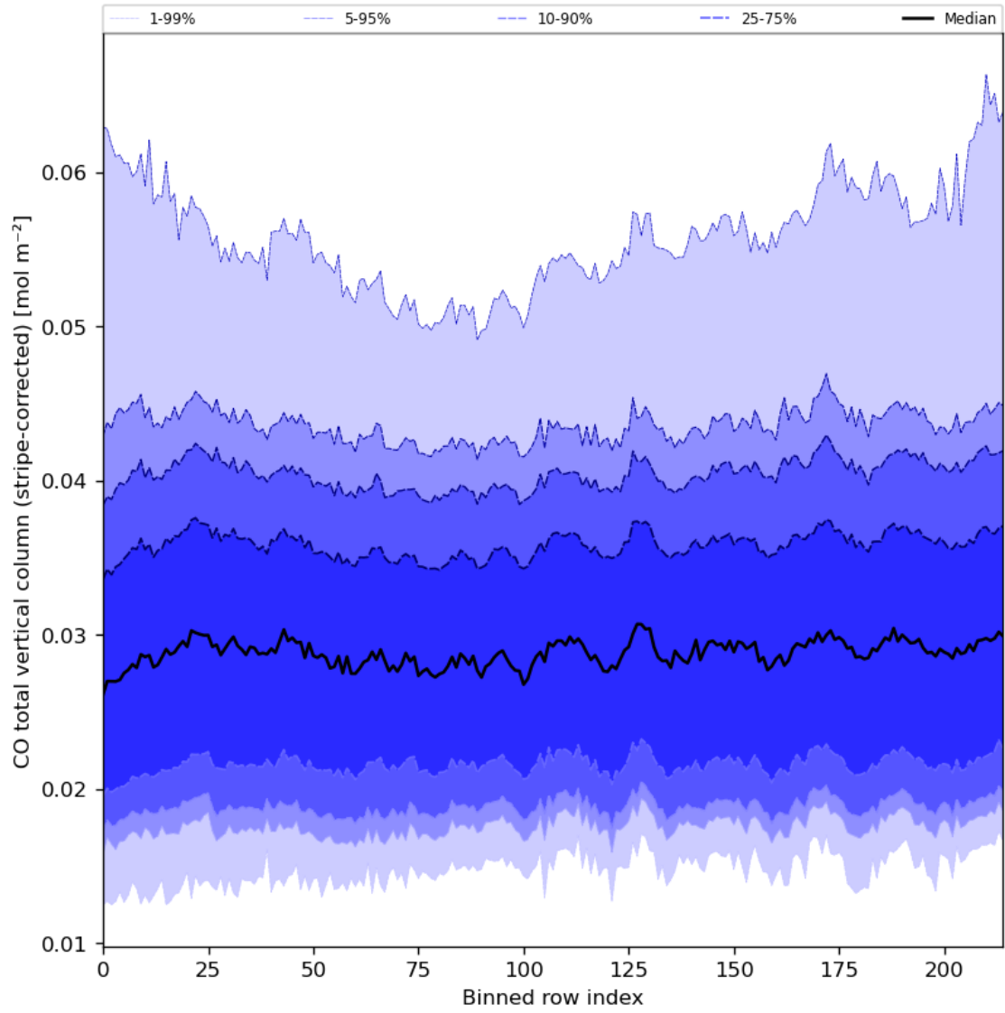
Figure 27: Along track statistics of “CO total vertical column (stripe-corrected)” for 2023-08-30 to 2023-09-01
