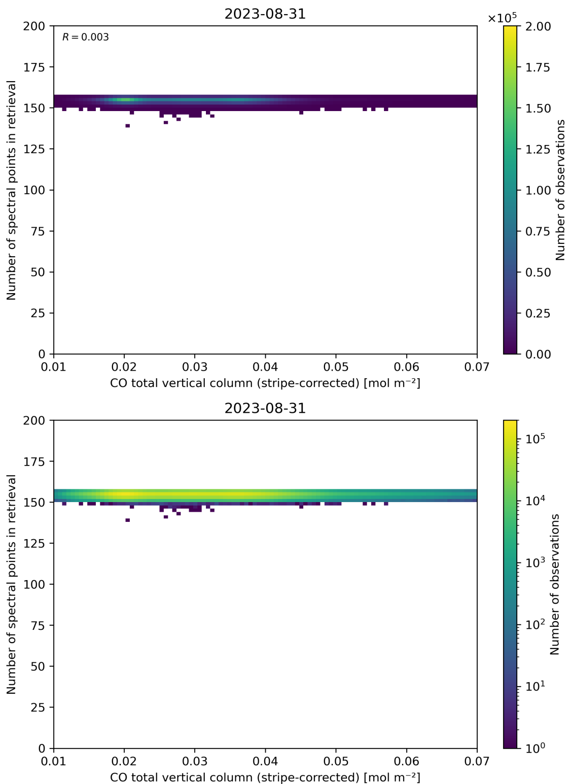
Figure 40: Scatter density plot of “CO total vertical column (stripe-corrected)” against “Number of spectral points in retrieval” for 2023-08-30 to 2023-09-01.
