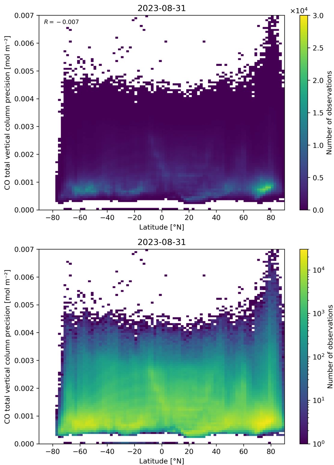
Figure 53: Scatter density plot of “Latitude” against “CO total vertical column precision” for 2023-08-30 to 2023-09-01.
