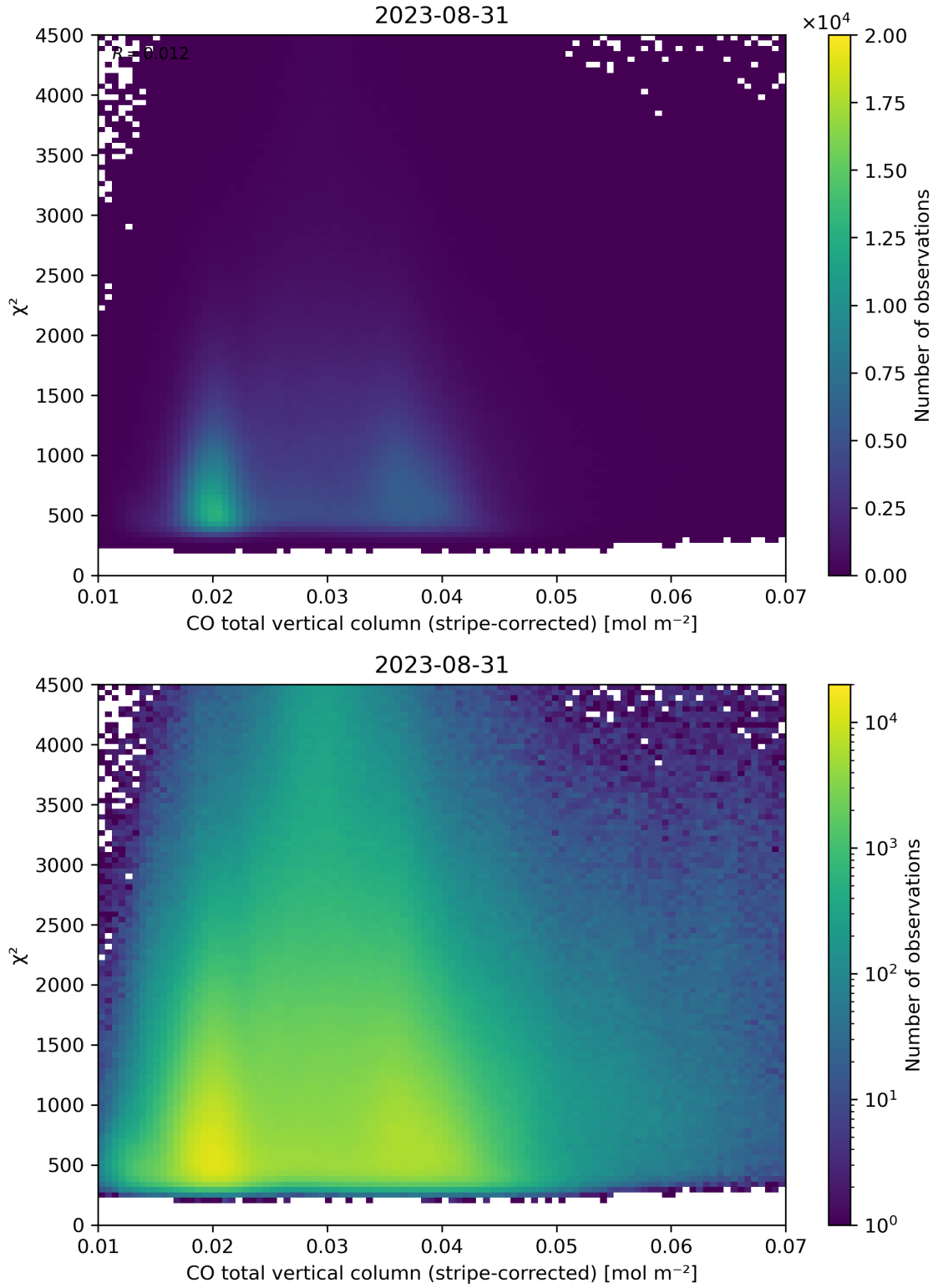
Figure 37: Scatter density plot of “CO total vertical column (stripe-corrected)” against “ \chi^2 ” for 2023-08-30 to 2023-09-01.
