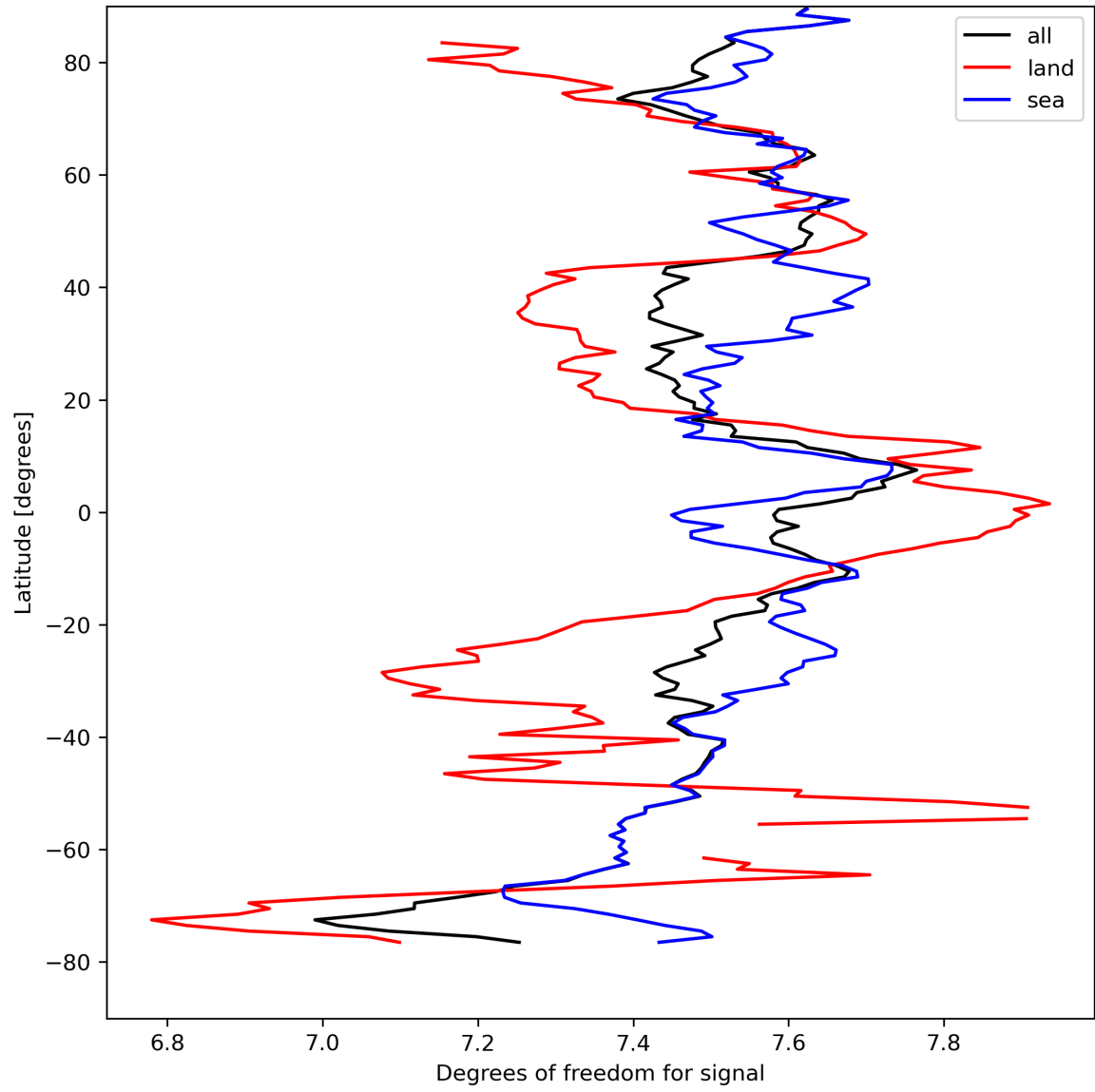
Figure 15: Zonal average of “Degrees of freedom for signal” for 2023-08-30 to 2023-09-01.
