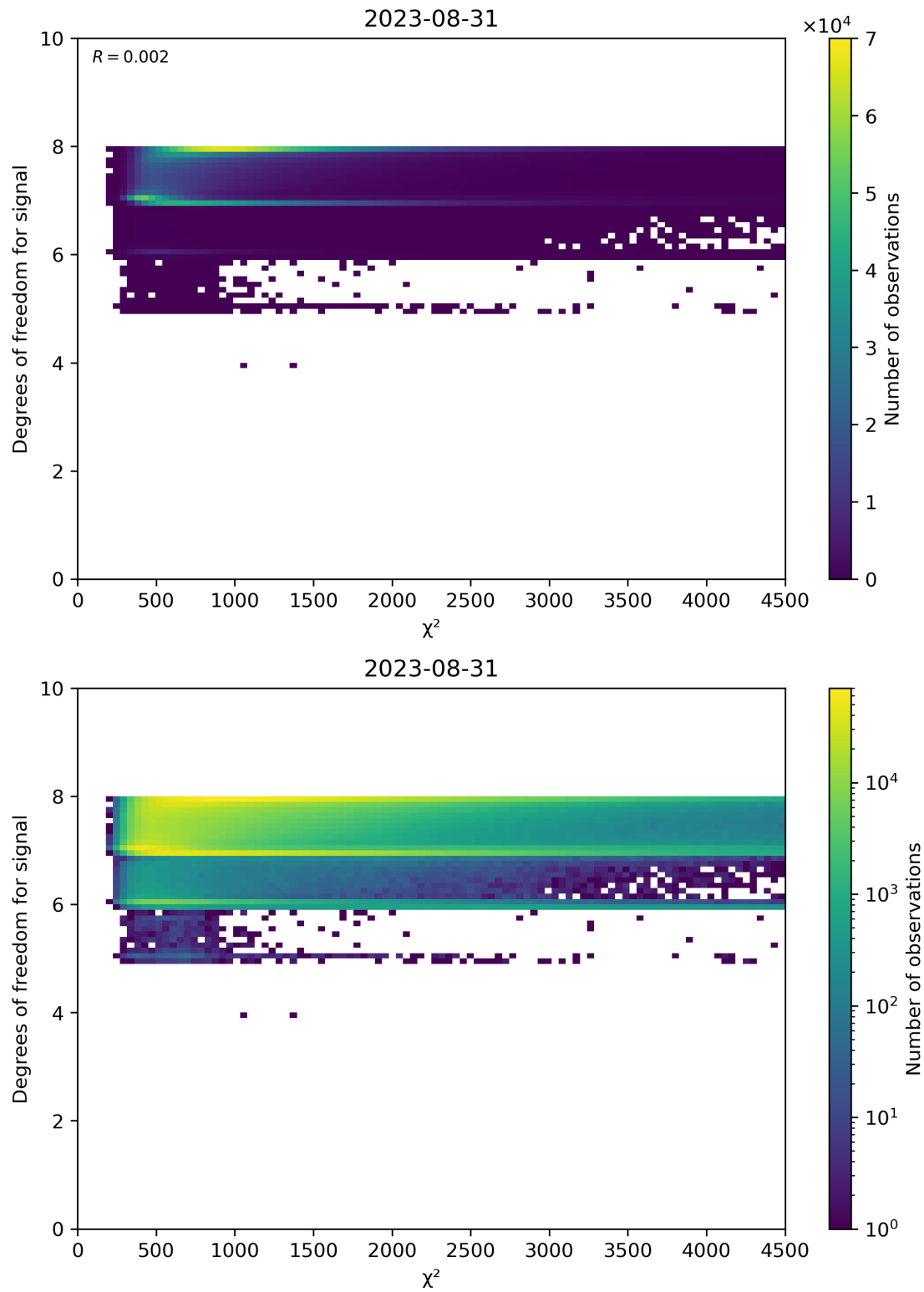
Figure 48: Scatter density plot of “ \chi^2 ” against “Degrees of freedom for signal” for 2023-08-30 to 2023-09-01.
