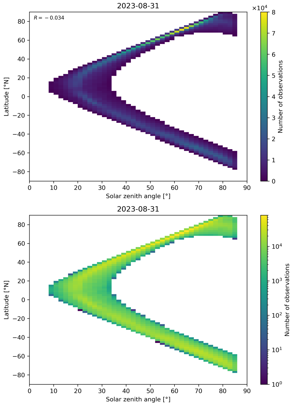
Figure 66: Scatter density plot of “Solar zenith angle” against “Latitude” for 2023-08-30 to 2023-09-01.
