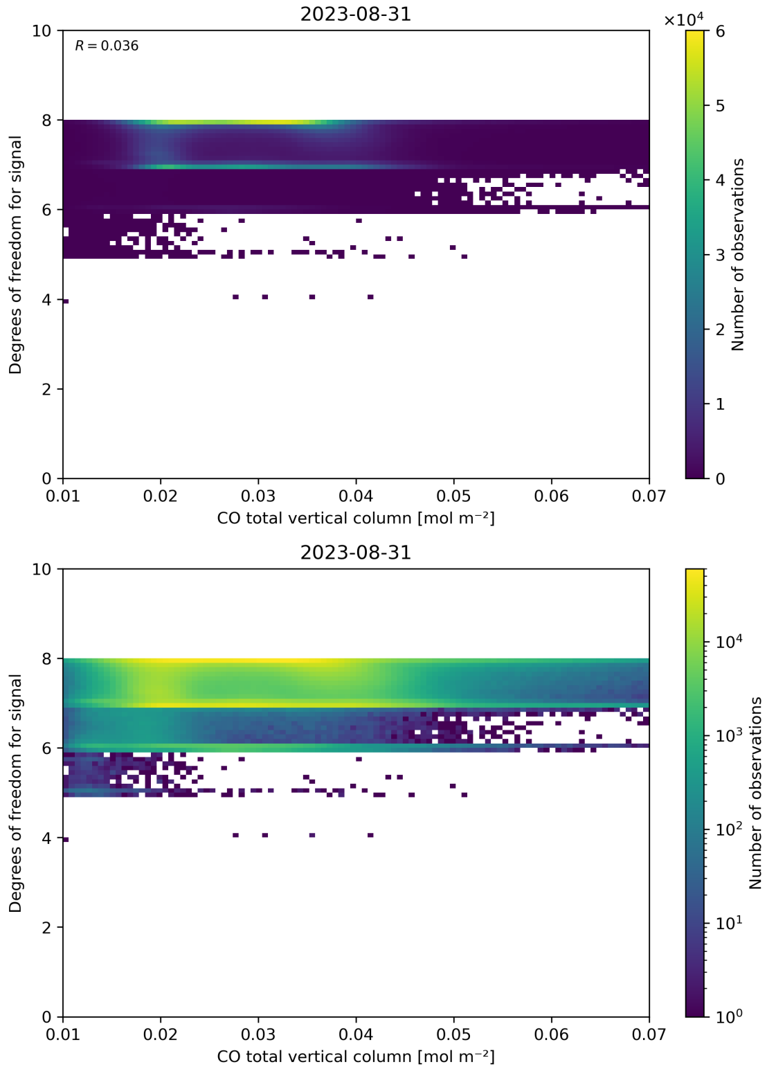
Figure 41: Scatter density plot of “CO total vertical column” against “Degrees of freedom for signal” for 2023-08-30 to 2023-09-01.
