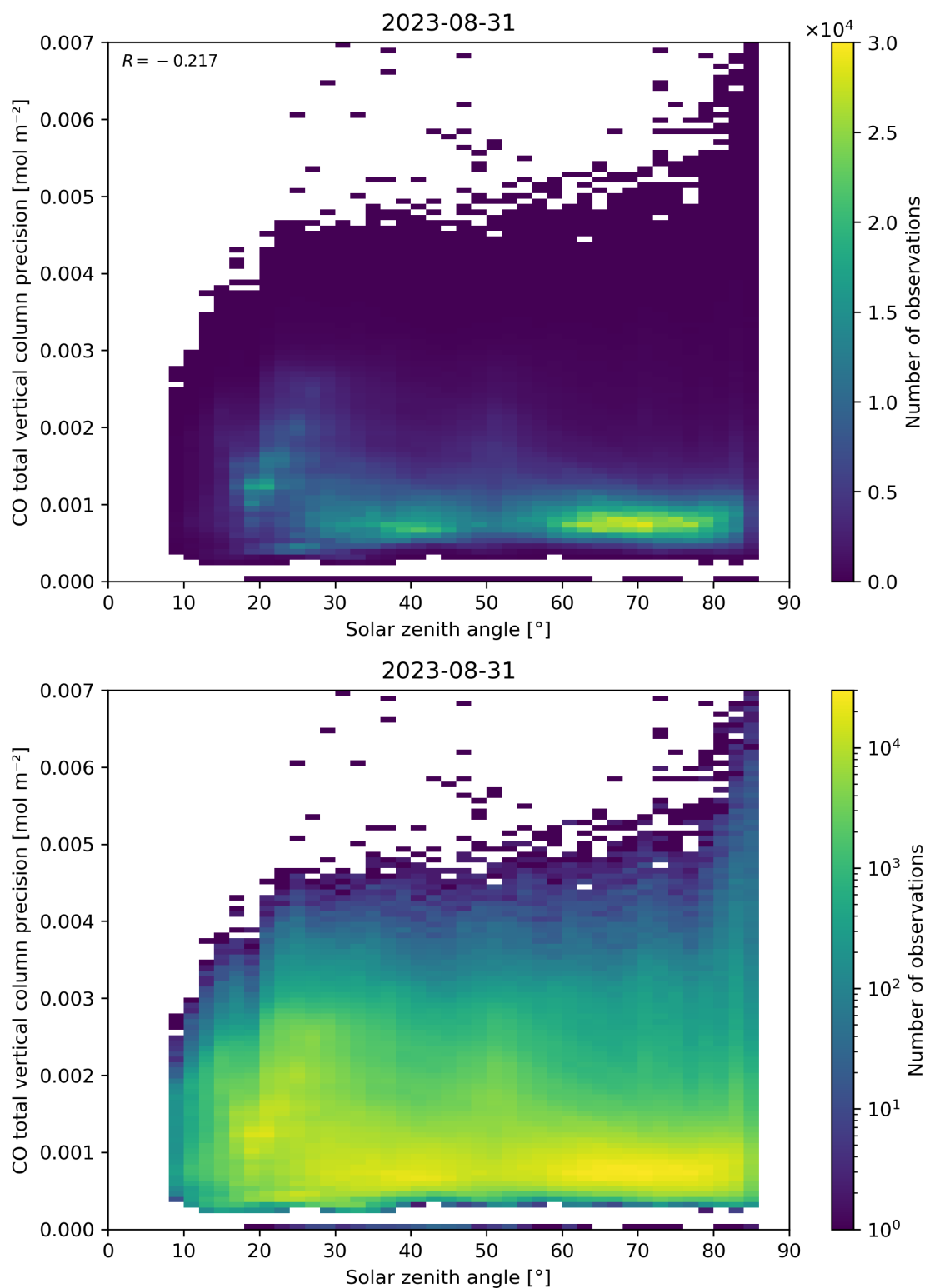
Figure 63: Scatter density plot of “Solar zenith angle” against “CO total vertical column precision” for 2023-08-30 to 2023-09-01.
