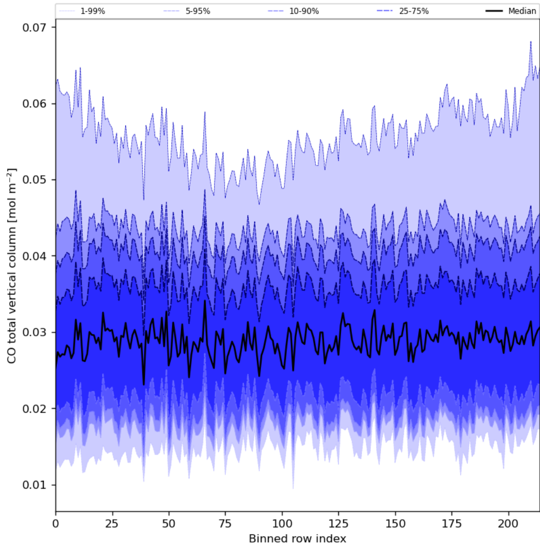
Figure 26: Along track statistics of “CO total vertical column” for 2023-08-30 to 2023-09-01
