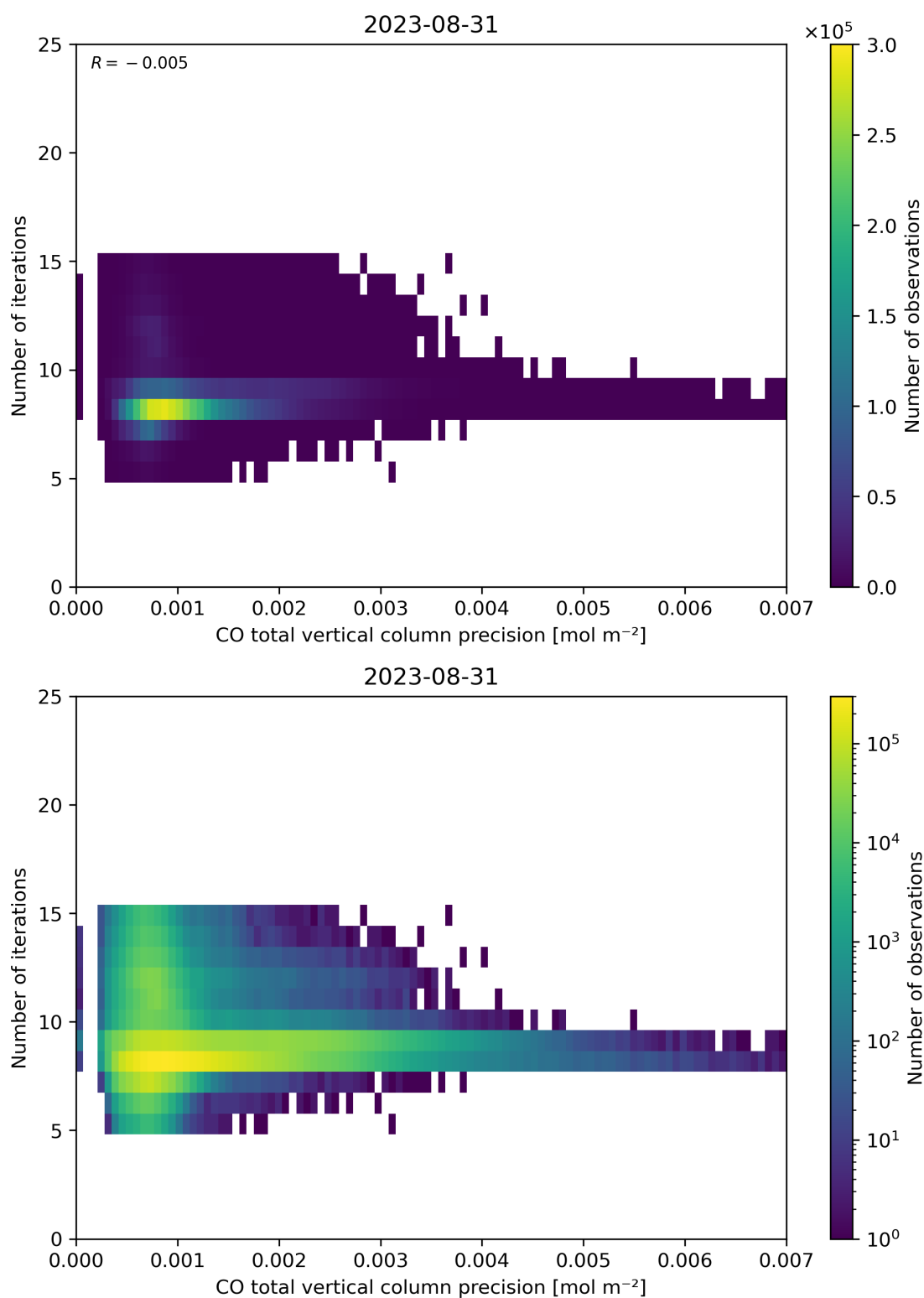
Figure 46: Scatter density plot of “CO total vertical column precision” against “Number of iterations” for 2023-08-30 to 2023-09-01.
