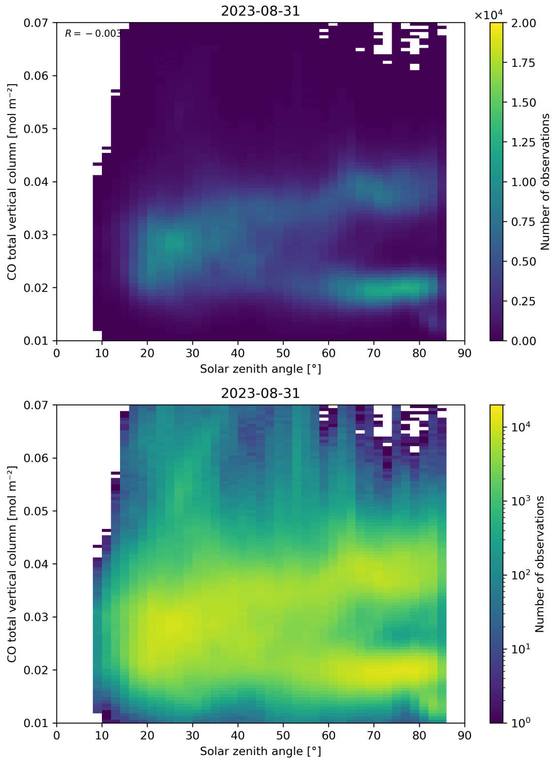
Figure 61: Scatter density plot of “Solar zenith angle” against “CO total vertical column” for 2023-08-30 to 2023-09-01.
