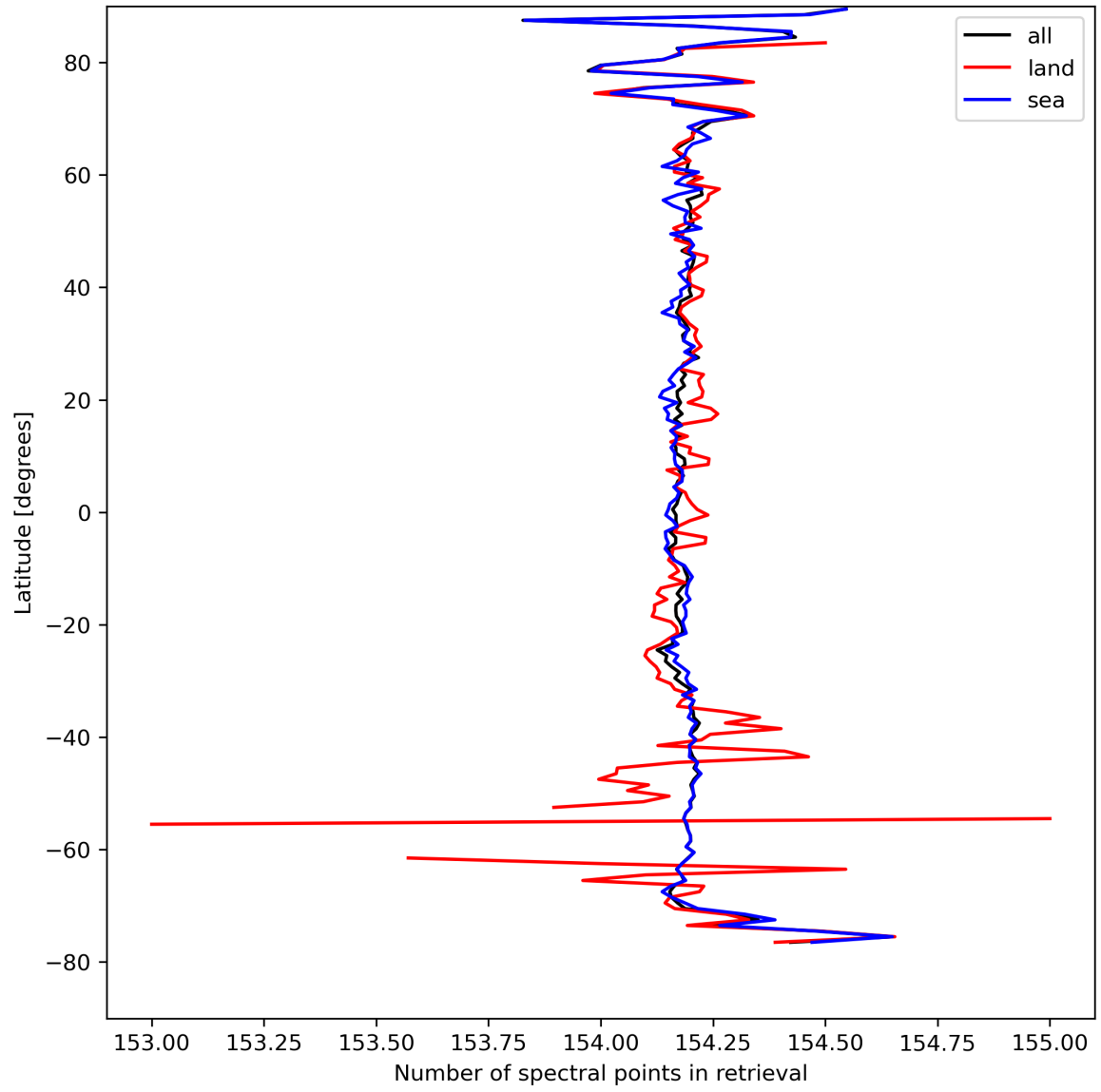
Figure 13: Zonal average of “Number of spectral points in retrieval” for 2023-08-30 to 2023-09-01.
