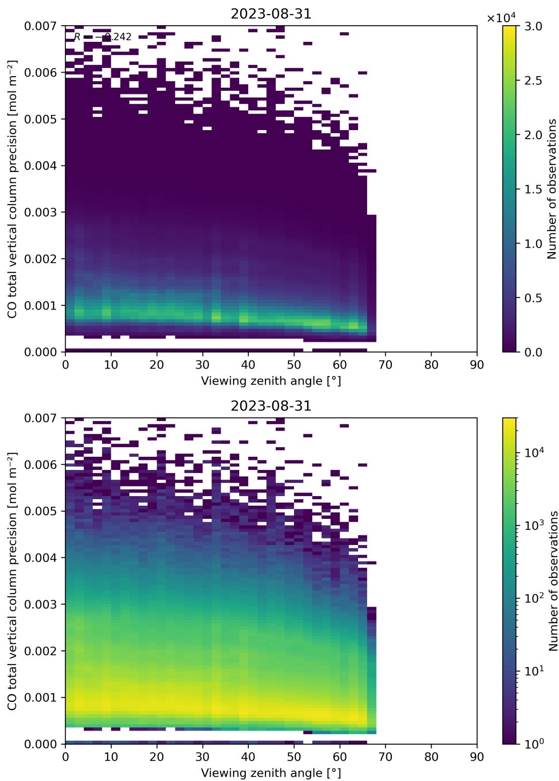
Figure 71: Scatter density plot of “Viewing zenith angle” against “CO total vertical column precision” for 2023-08-30 to 2023-09-01.
