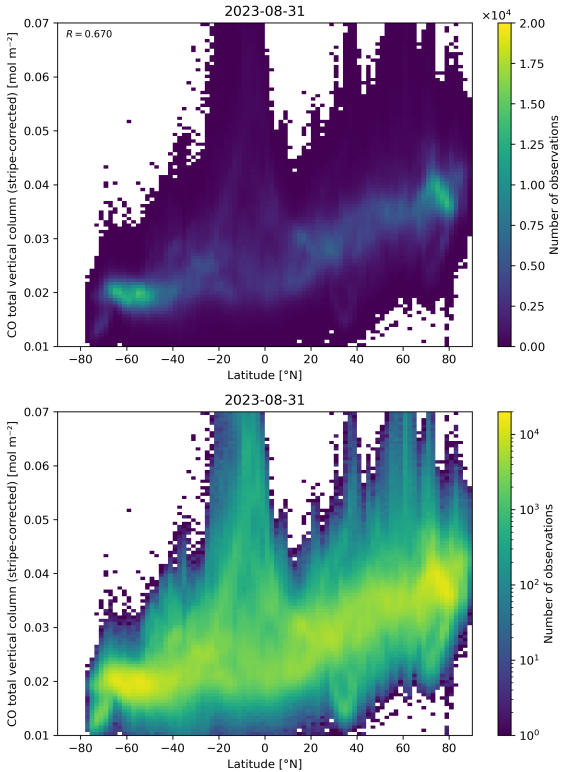
Figure 52: Scatter density plot of “Latitude” against “CO total vertical column (stripe-corrected)” for 2023-08-30 to 2023-09-01.
