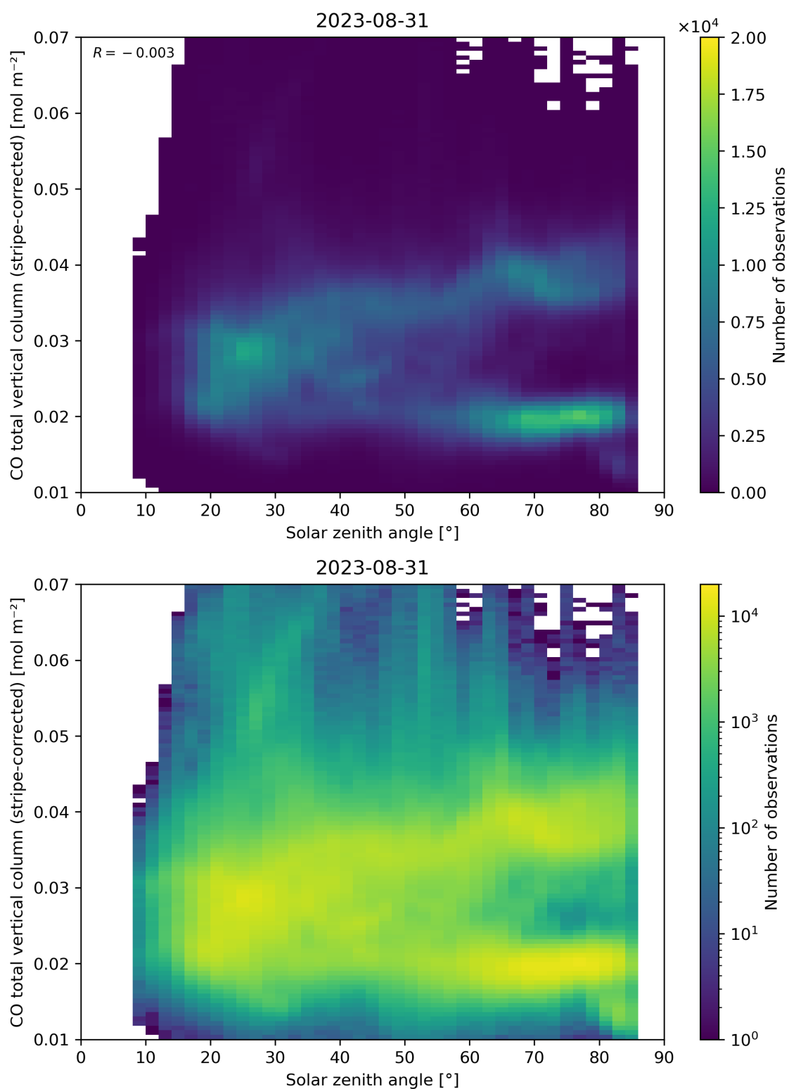
Figure 62: Scatter density plot of “Solar zenith angle” against “CO total vertical column (stripe-corrected)” for 2023-08-30 to 2023-09-01.
