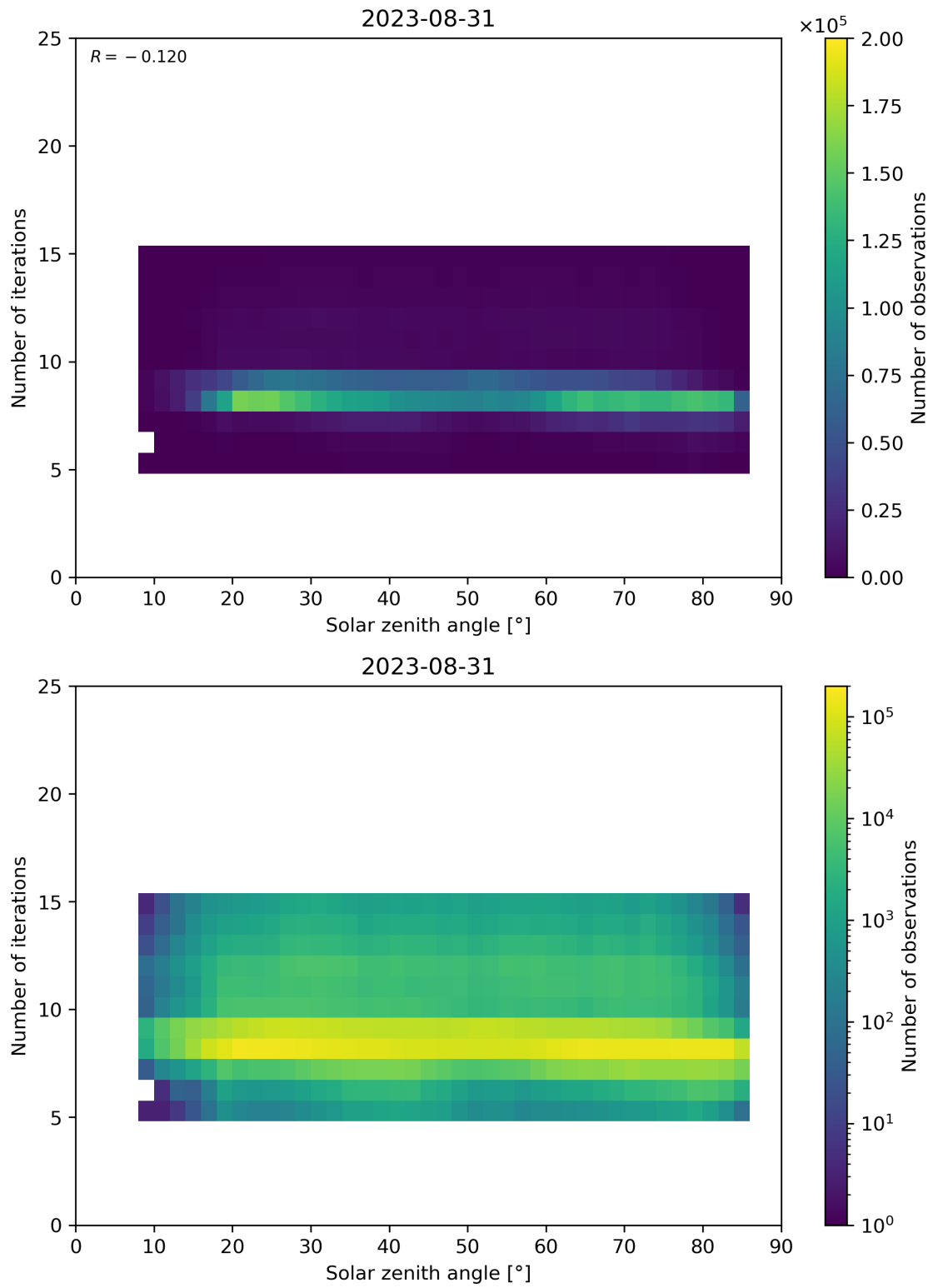
Figure 67: Scatter density plot of “Solar zenith angle” against “Number of iterations” for 2023-08-30 to 2023-09-01.
