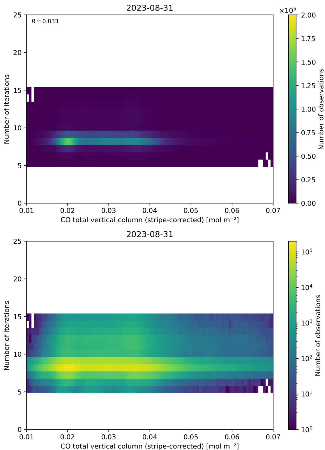
Figure 39: Scatter density plot of “CO total vertical column (stripe-corrected)” against “Number of iterations” for 2023-08-30 to 2023-09-01.
