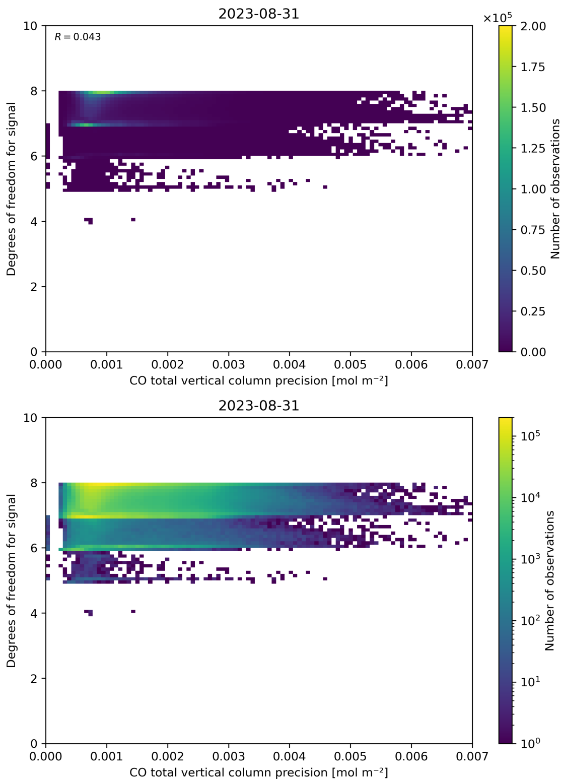
Figure 45: Scatter density plot of “CO total vertical column precision” against “Degrees of freedom for signal” for 2023-08-30 to 2023-09-01.
