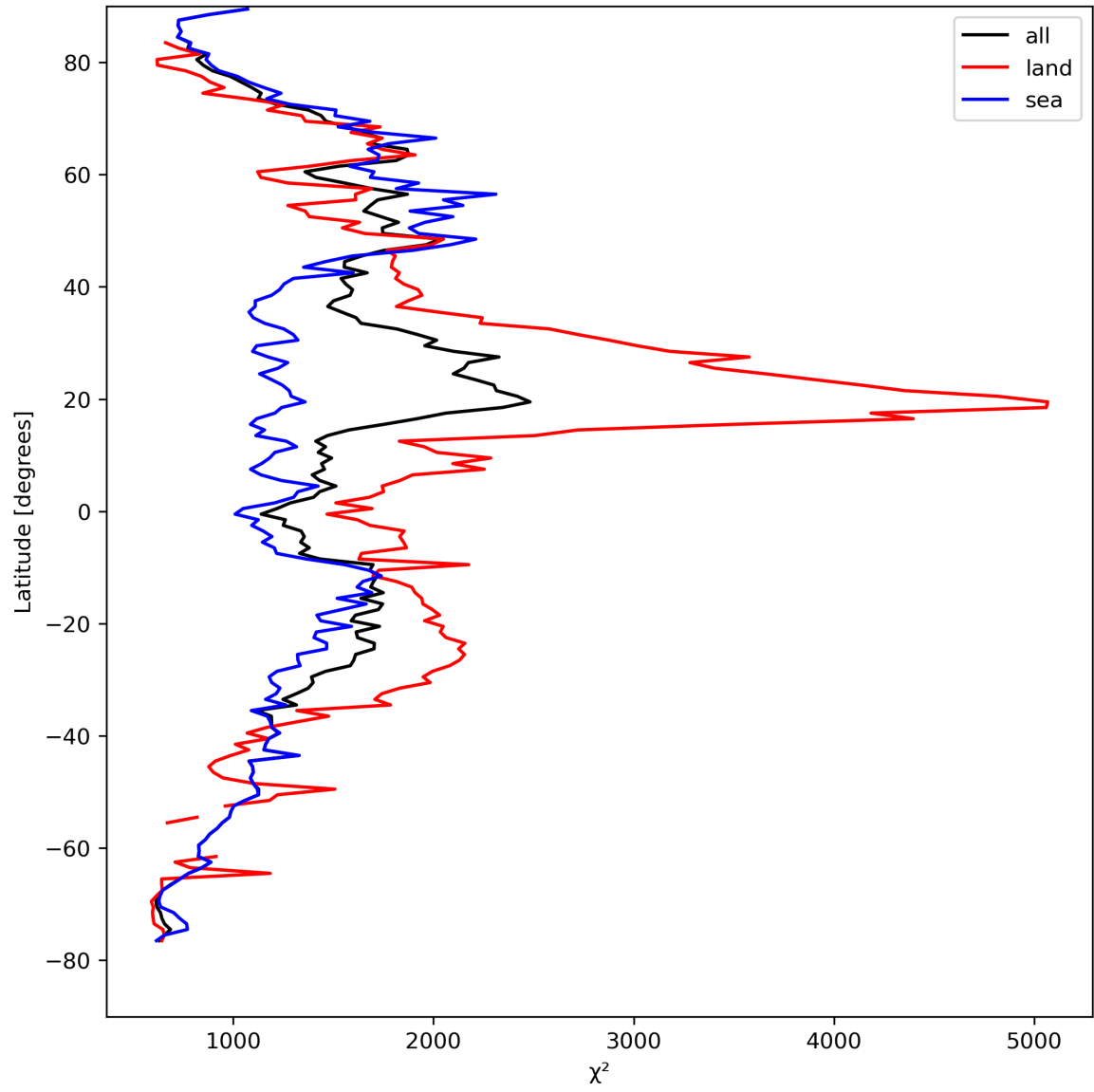
Figure 14: Zonal average of “ \chi^2 ” for 2023-08-30 to 2023-09-01.
