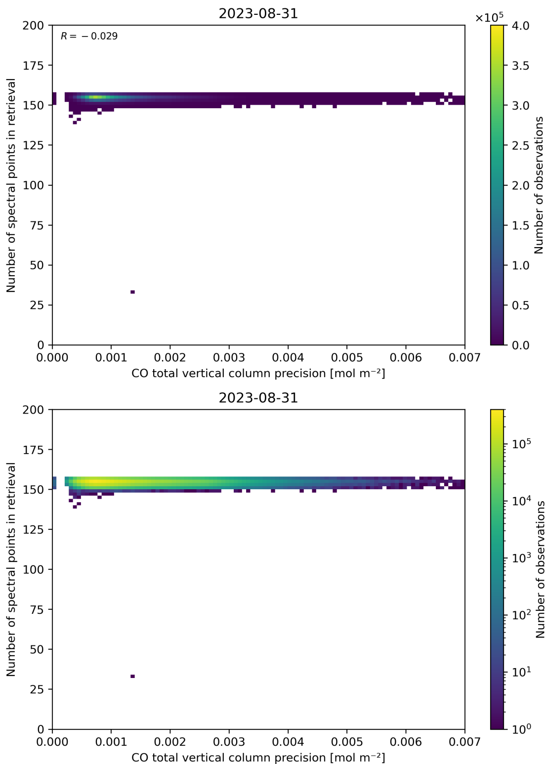
Figure 47: Scatter density plot of “CO total vertical column precision” against “Number of spectral points in retrieval” for 2023-08-30 to 2023-09-01.
