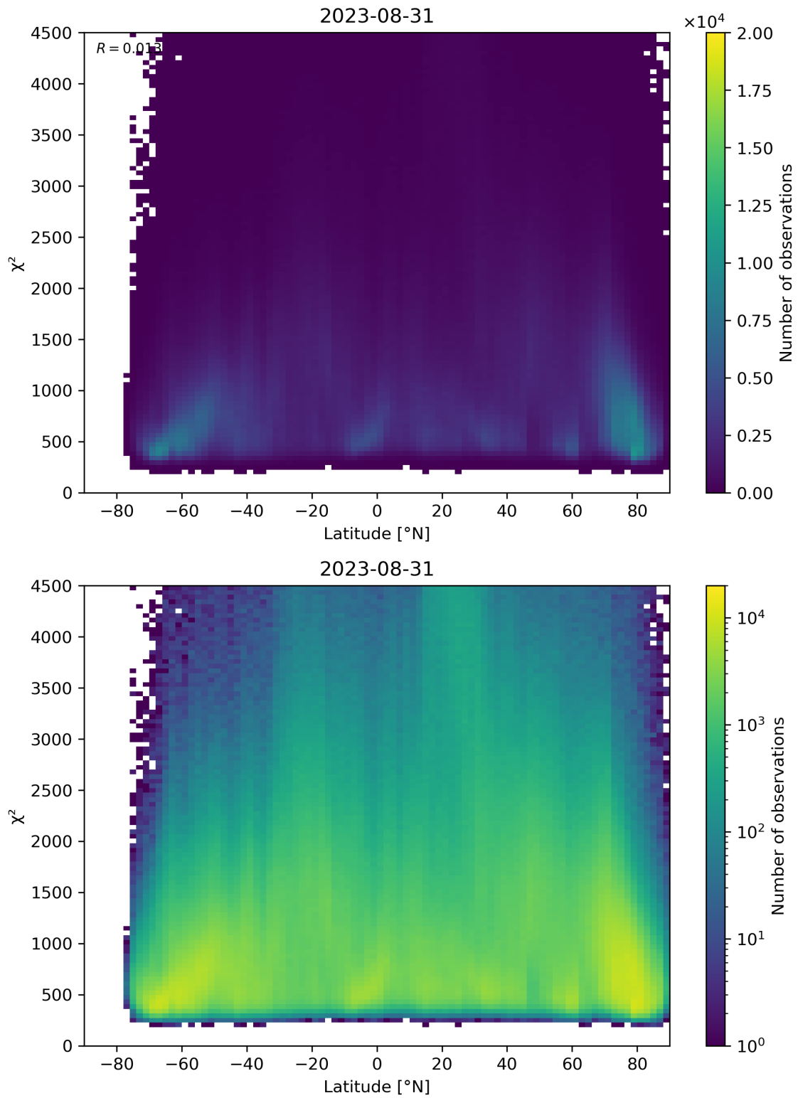
Figure 54: Scatter density plot of “Latitude” against “ \chi^2 ” for 2023-08-30 to 2023-09-01.
