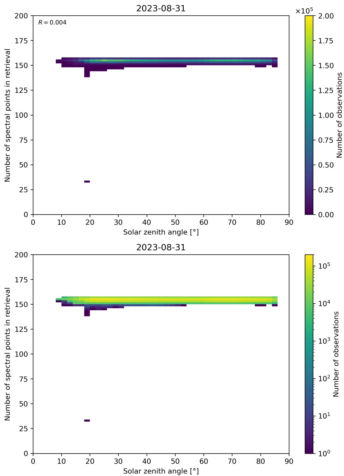
Figure 68: Scatter density plot of “Solar zenith angle” against “Number of spectral points in retrieval” for 2023-08-30 to 2023-09-01.
