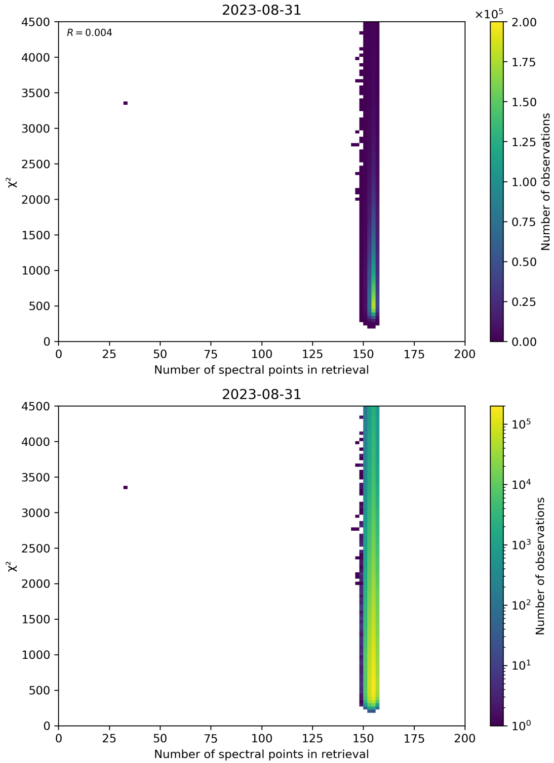
Figure 58: Scatter density plot of “Number of spectral points in retrieval” against “ \chi^2 ” for 2023-08-30 to 2023-09-01.
