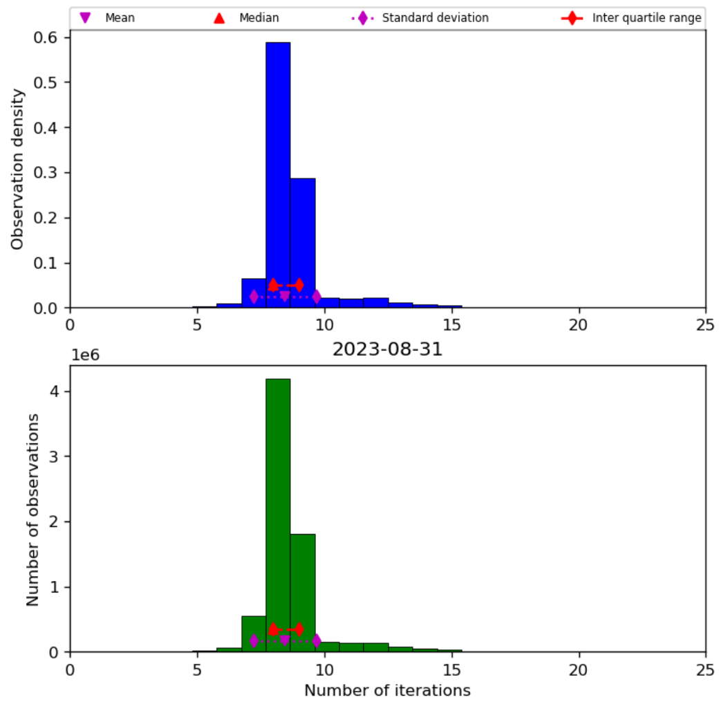
Figure 24: Histogram of “Number of iterations” for 2023-08-30 to 2023-09-01
