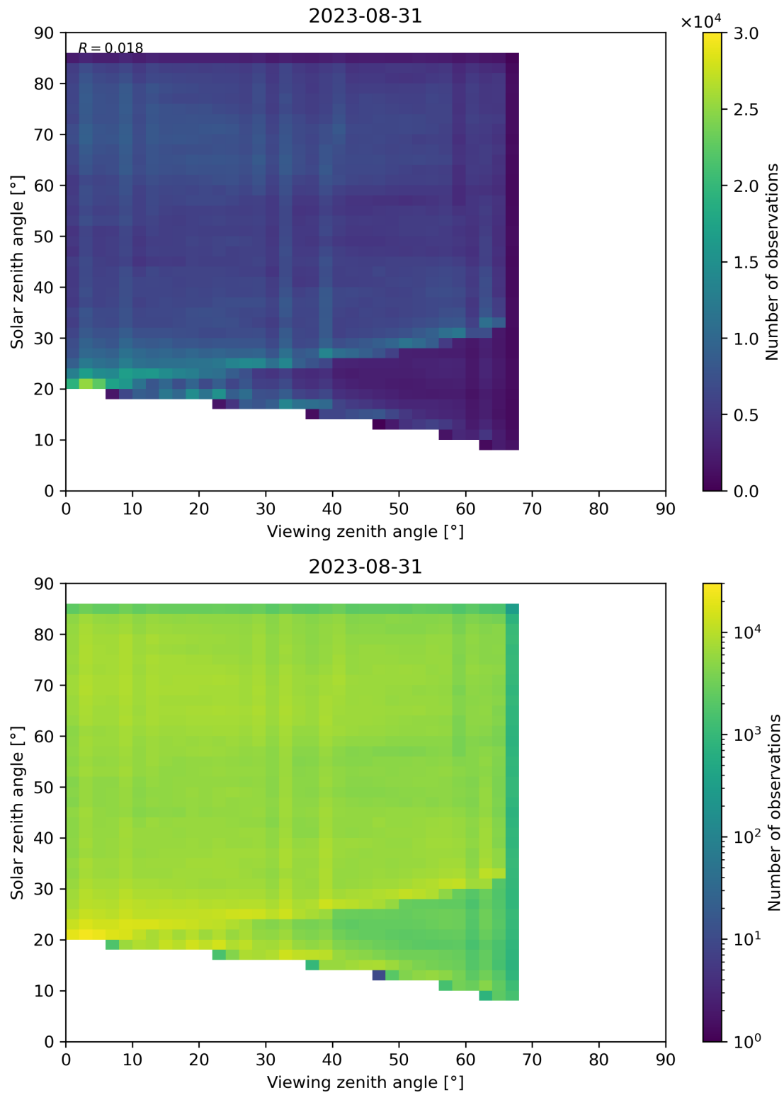
Figure 77: Scatter density plot of “Viewing zenith angle” against “Solar zenith angle” for 2023-08-30 to 2023-09-01.
