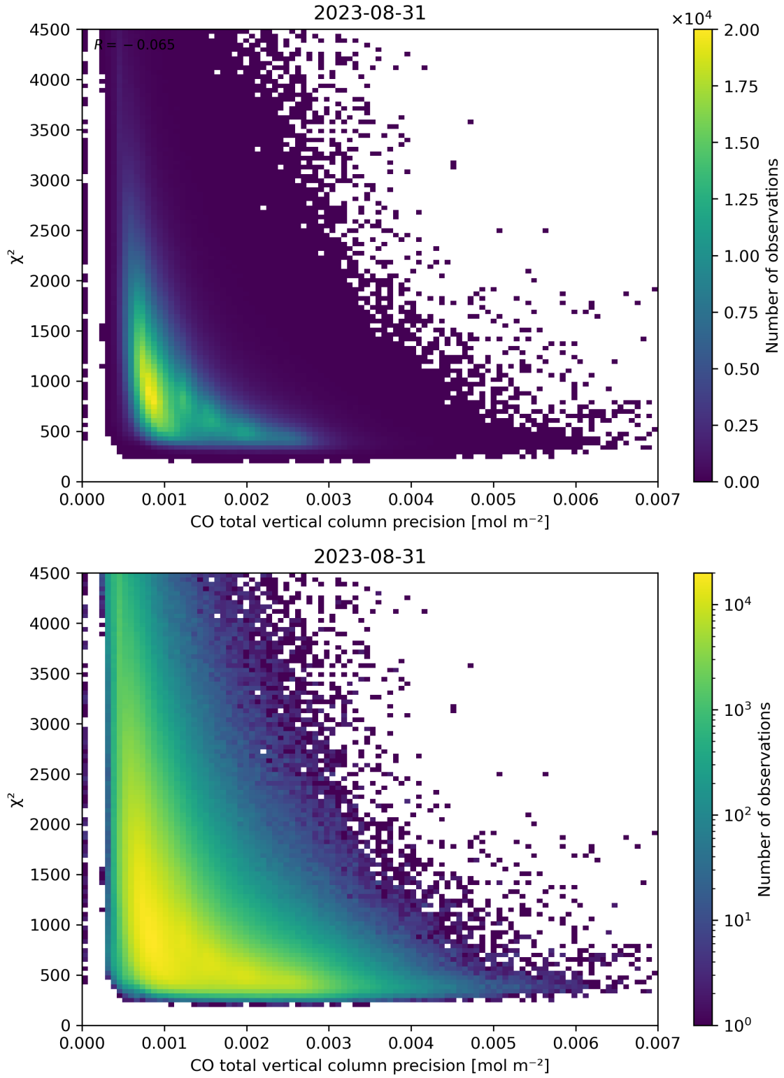
Figure 44: Scatter density plot of “CO total vertical column precision” against “ \chi^2 ” for 2023-08-30 to 2023-09-01.
