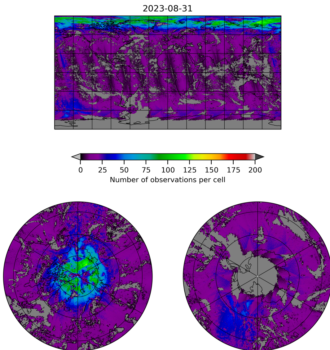
Figure 8: Map of the number of observations for 2023-08-30 to 2023-09-01
