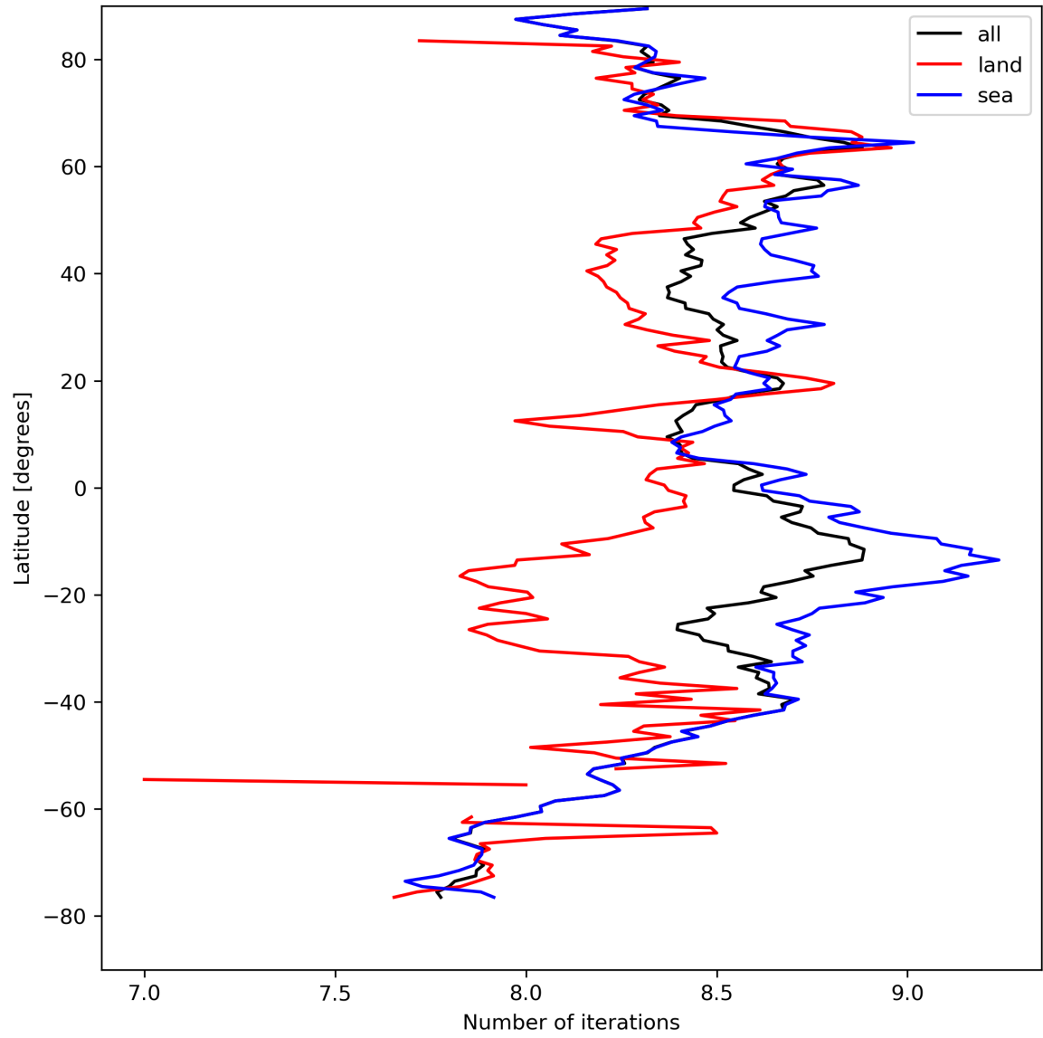
Figure 16: Zonal average of “Number of iterations” for 2023-08-30 to 2023-09-01.
