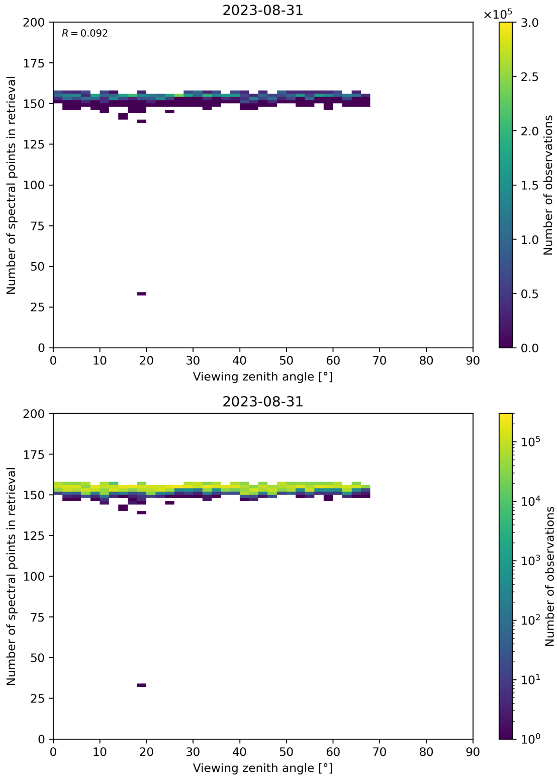
Figure 76: Scatter density plot of “Viewing zenith angle” against “Number of spectral points in retrieval” for 2023-08-30 to 2023-09-01.
