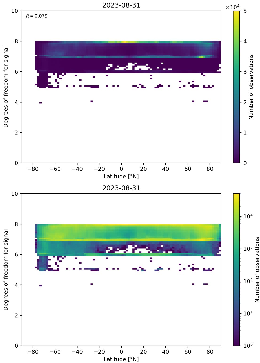
Figure 55: Scatter density plot of “Latitude” against “Degrees of freedom for signal” for 2023-08-30 to 2023-09-01.
