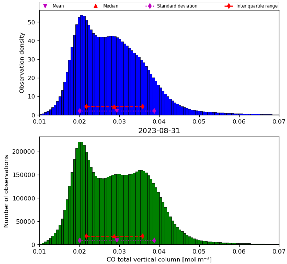
Figure 18: Histogram of “CO total vertical column” for 2023-08-30 to 2023-09-01
