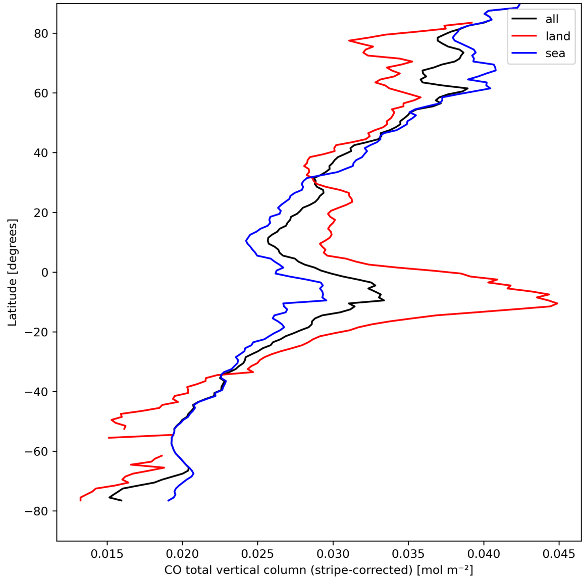
Figure 11: Zonal average of “CO total vertical column (stripe-corrected)” for 2023-08-30 to 2023-09-01.
