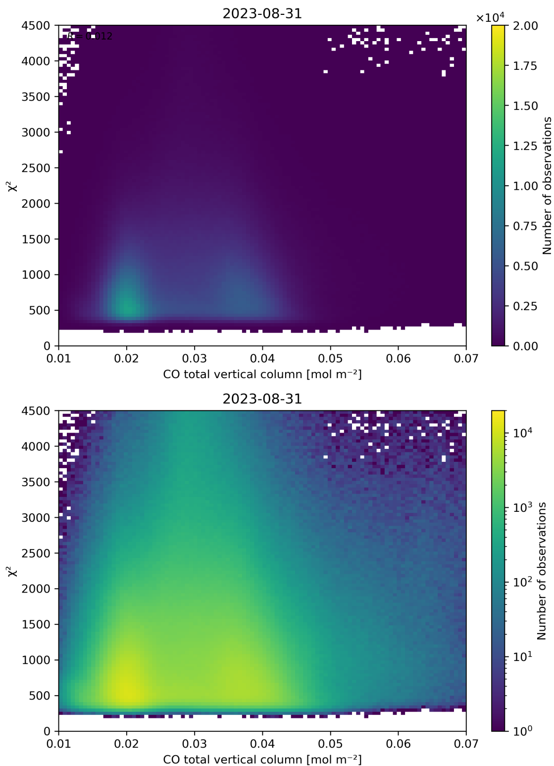
Figure 35: Scatter density plot of “CO total vertical column” against “ \chi^2 ” for 2023-08-30 to 2023-09-01.
