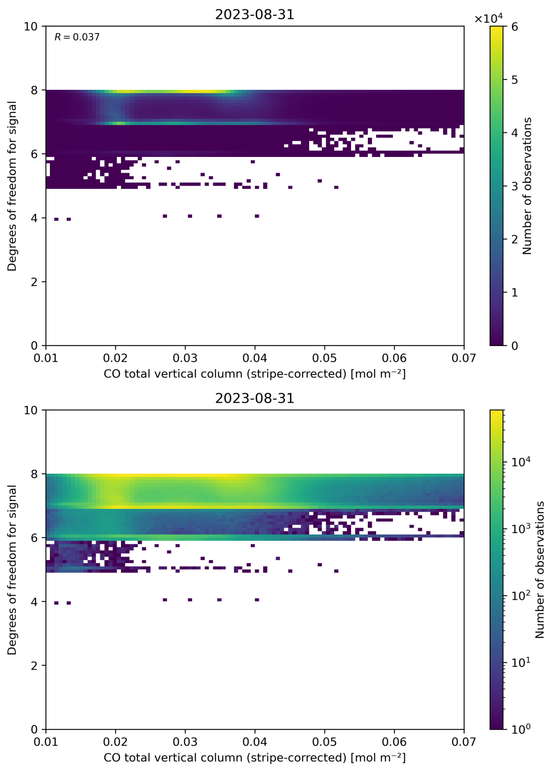
Figure 38: Scatter density plot of “CO total vertical column (stripe-corrected)” against “Degrees of freedom for signal” for 2023-08-30 to 2023-09-01.
