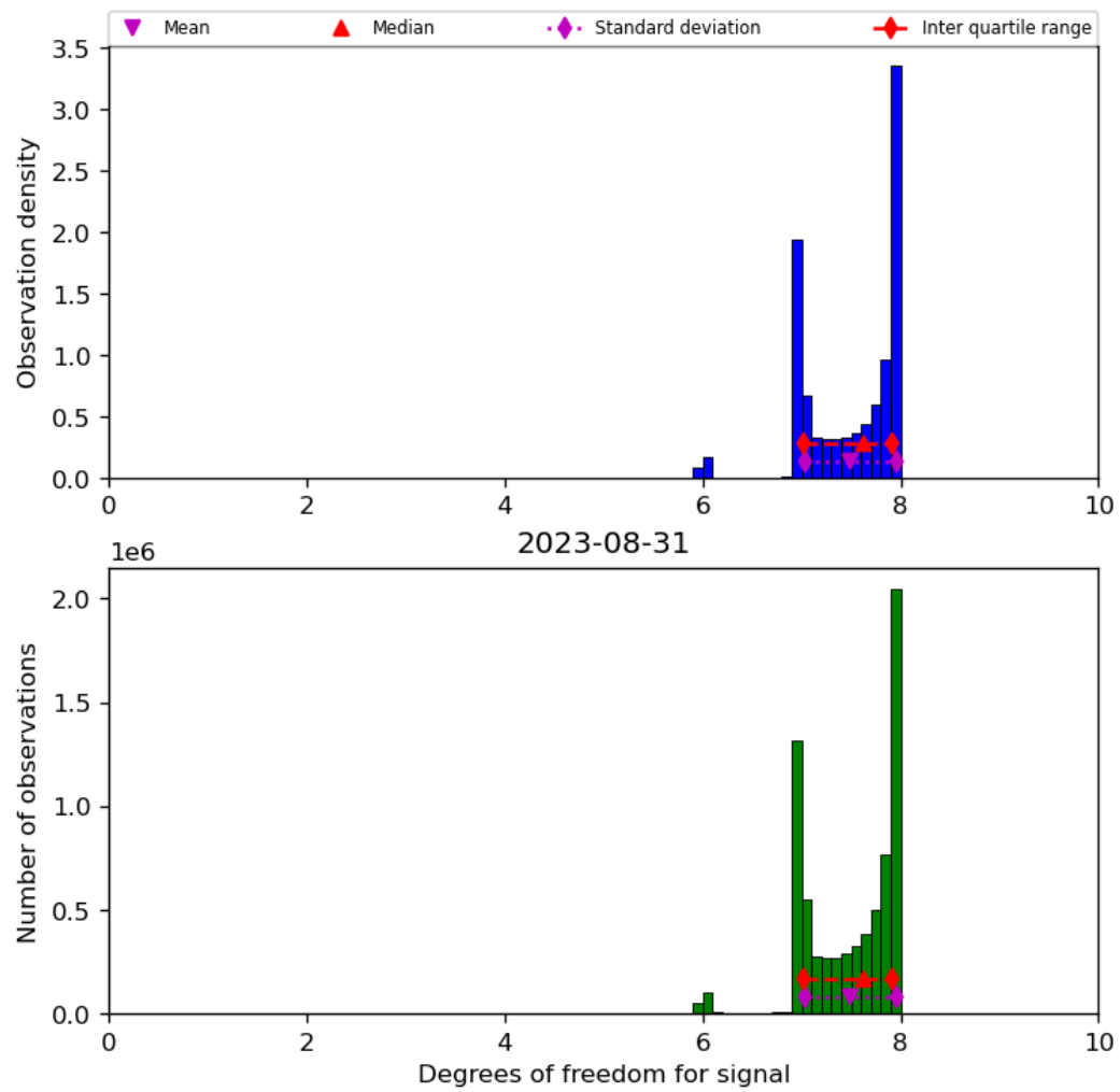
Figure 23: Histogram of “Degrees of freedom for signal” for 2023-08-30 to 2023-09-01
