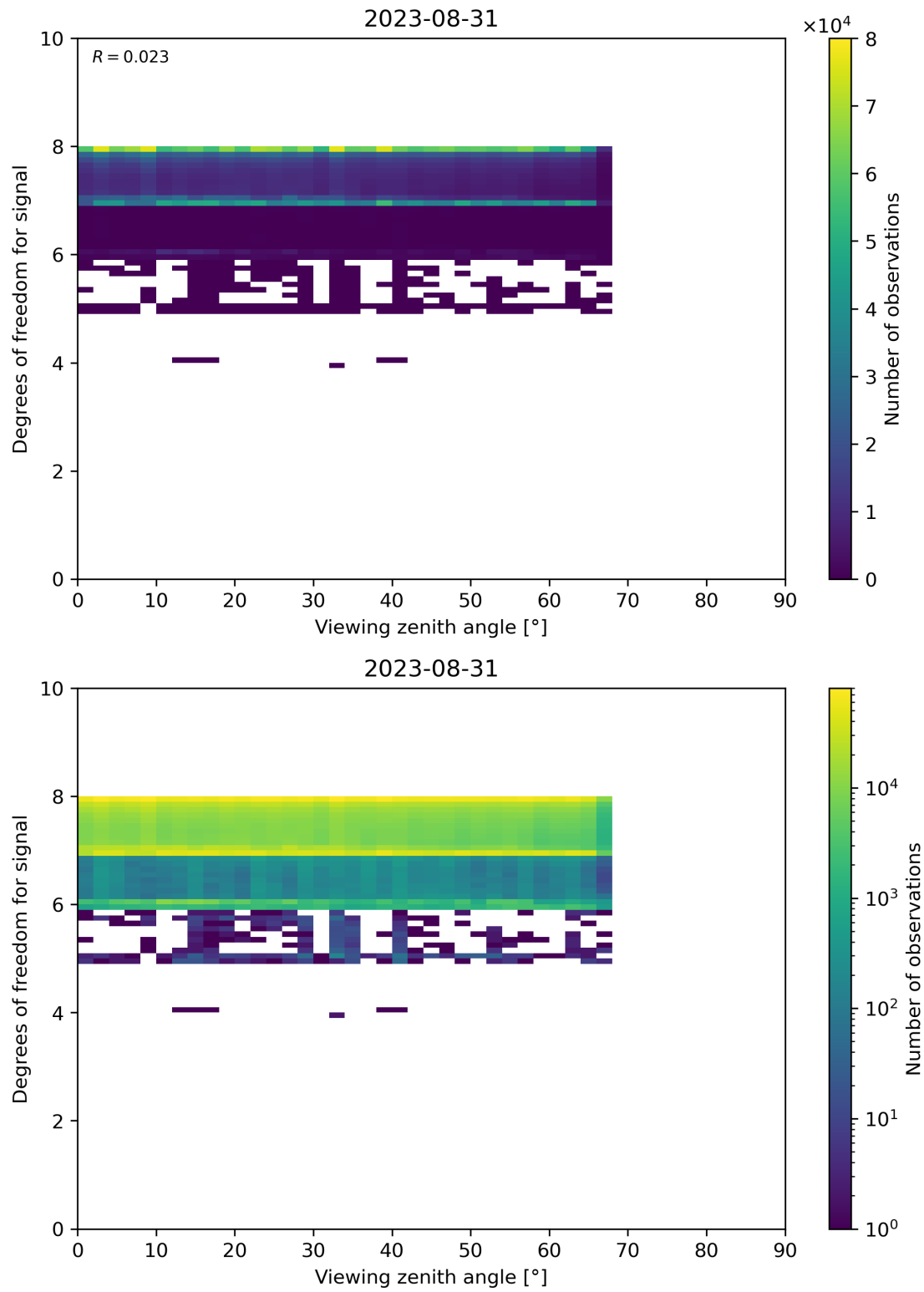
Figure 73: Scatter density plot of “Viewing zenith angle” against “Degrees of freedom for signal” for 2023-08-30 to 2023-09-01.
