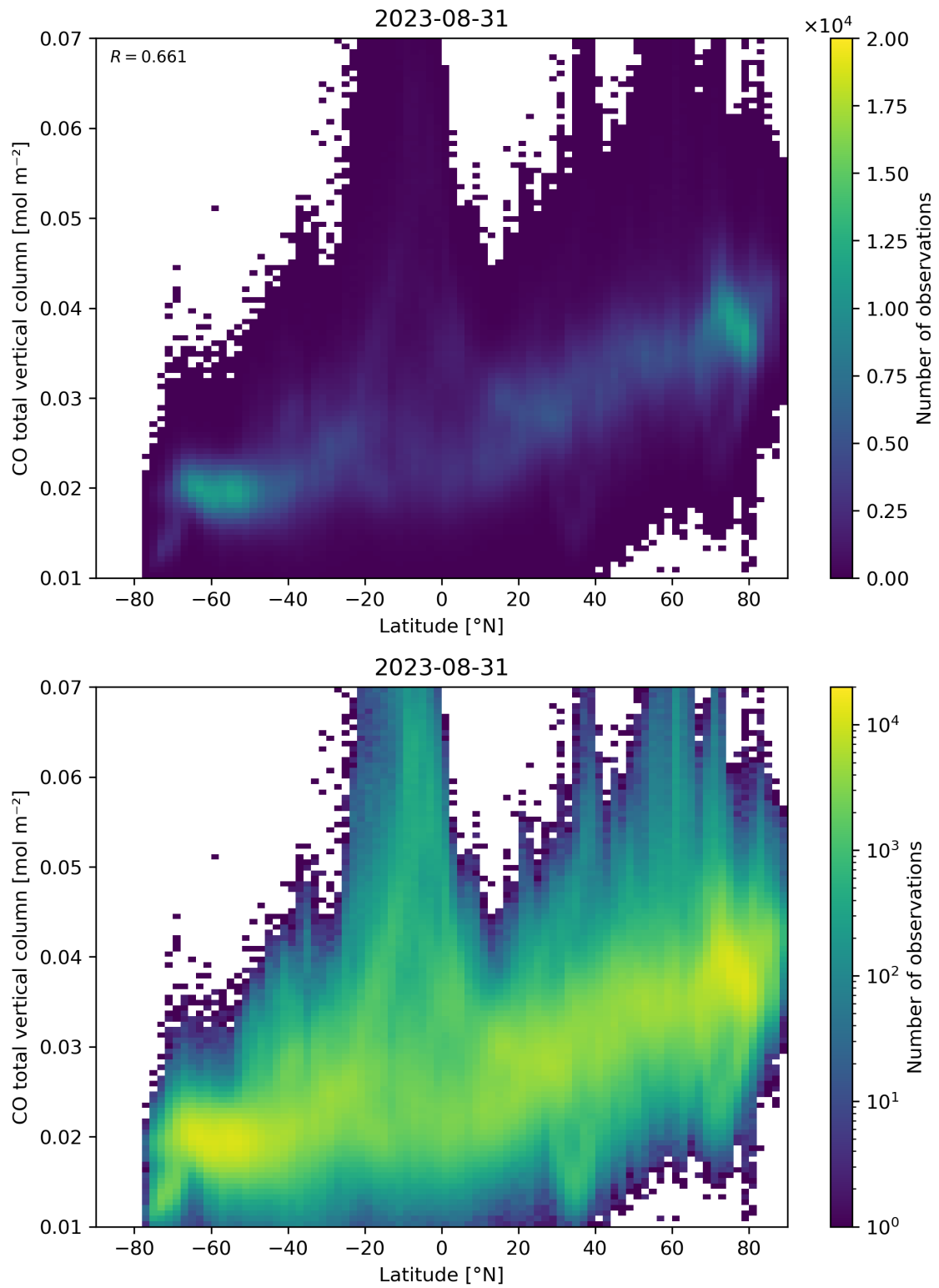
Figure 51: Scatter density plot of “Latitude” against “CO total vertical column” for 2023-08-30 to 2023-09-01.
