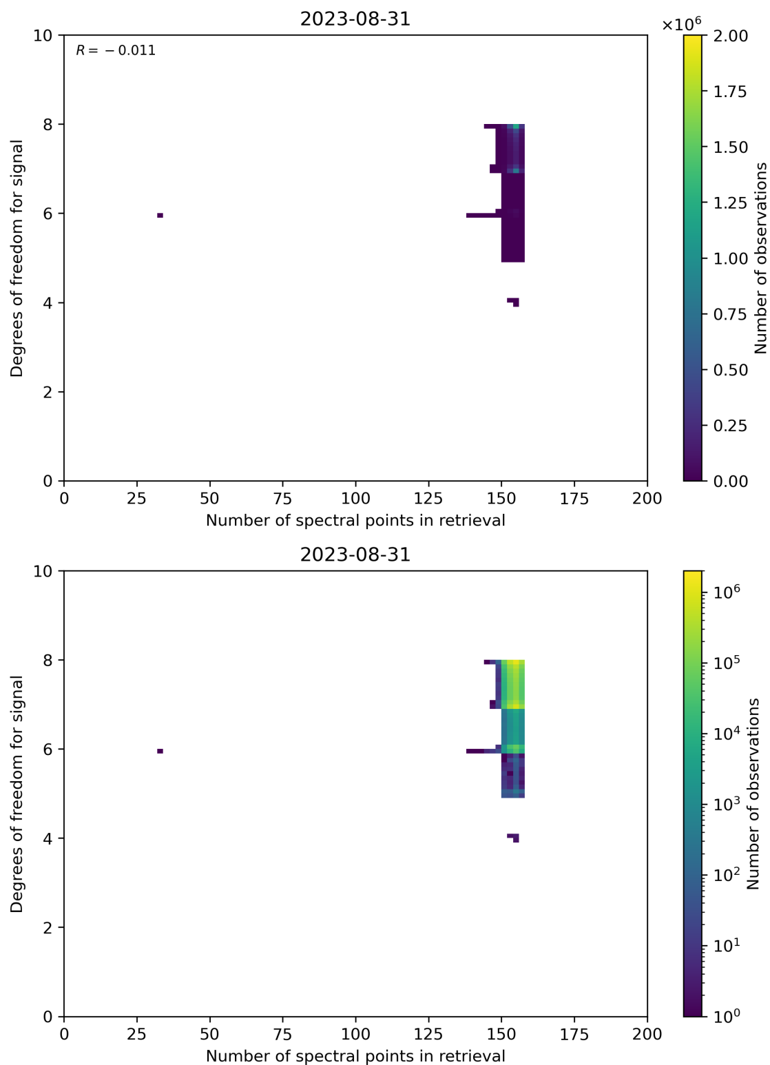
Figure 59: Scatter density plot of “Number of spectral points in retrieval” against “Degrees of freedom for signal” for 2023-08-30 to 2023-09-01.
