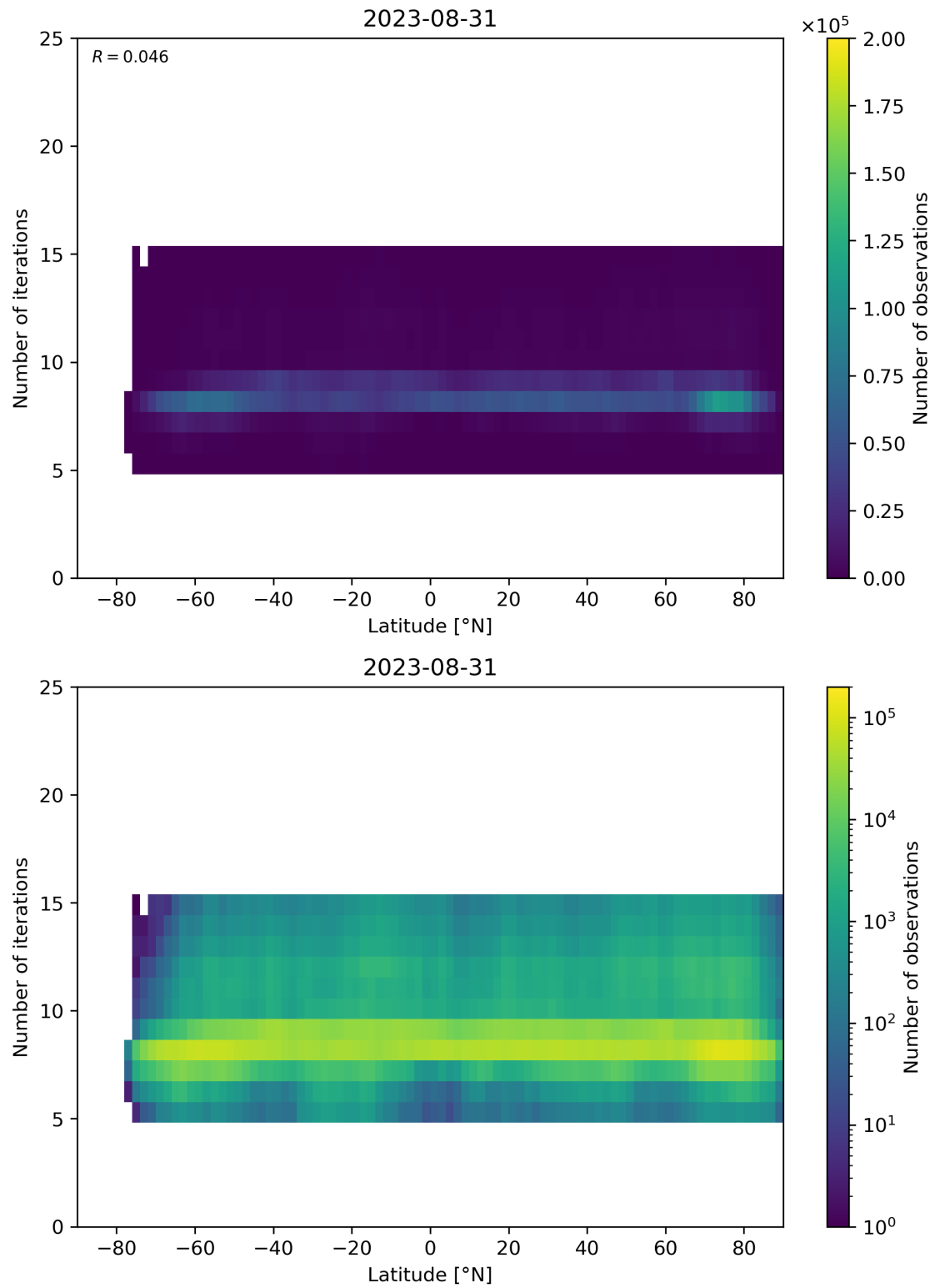
Figure 56: Scatter density plot of “Latitude” against “Number of iterations” for 2023-08-30 to 2023-09-01.
