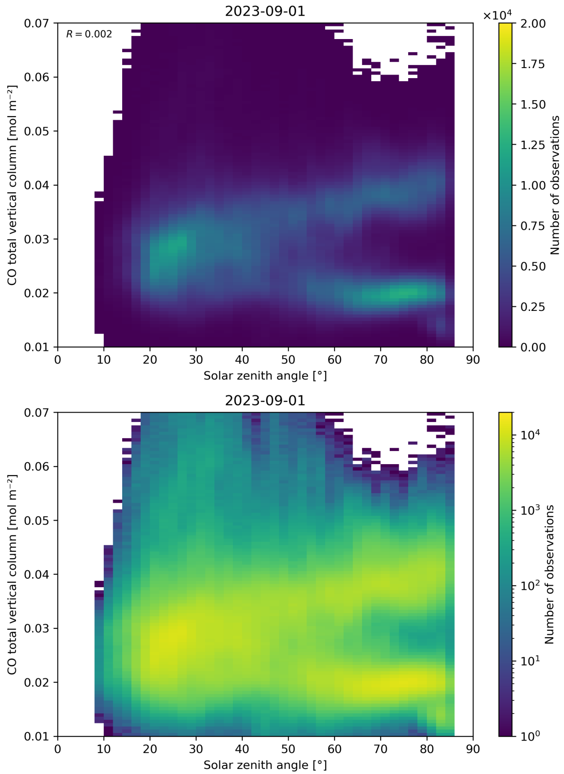
Figure 61: Scatter density plot of “Solar zenith angle” against “CO total vertical column” for 2023-08-31 to 2023-09-02.
