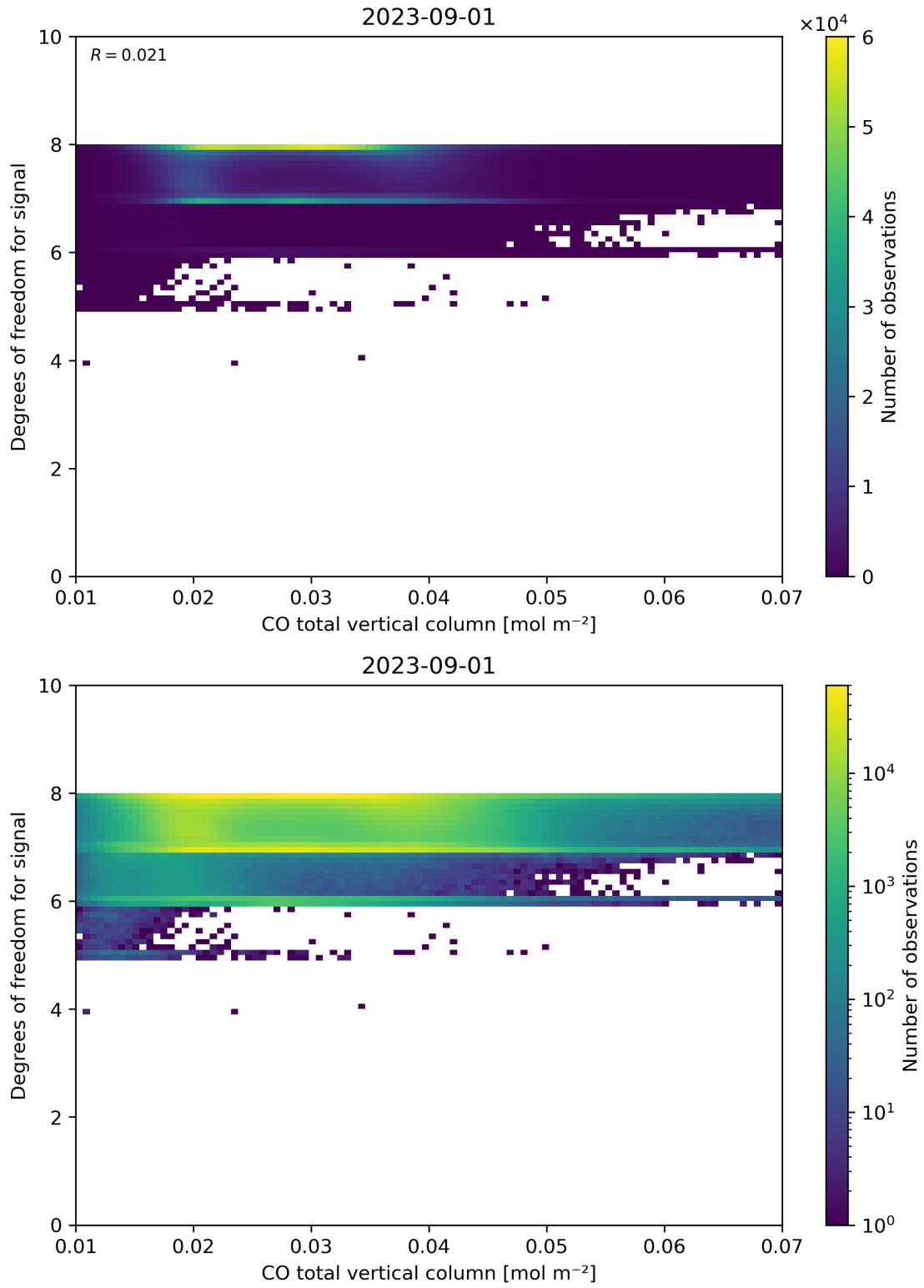
Figure 41: Scatter density plot of “CO total vertical column” against “Degrees of freedom for signal” for 2023-08-31 to 2023-09-02.
