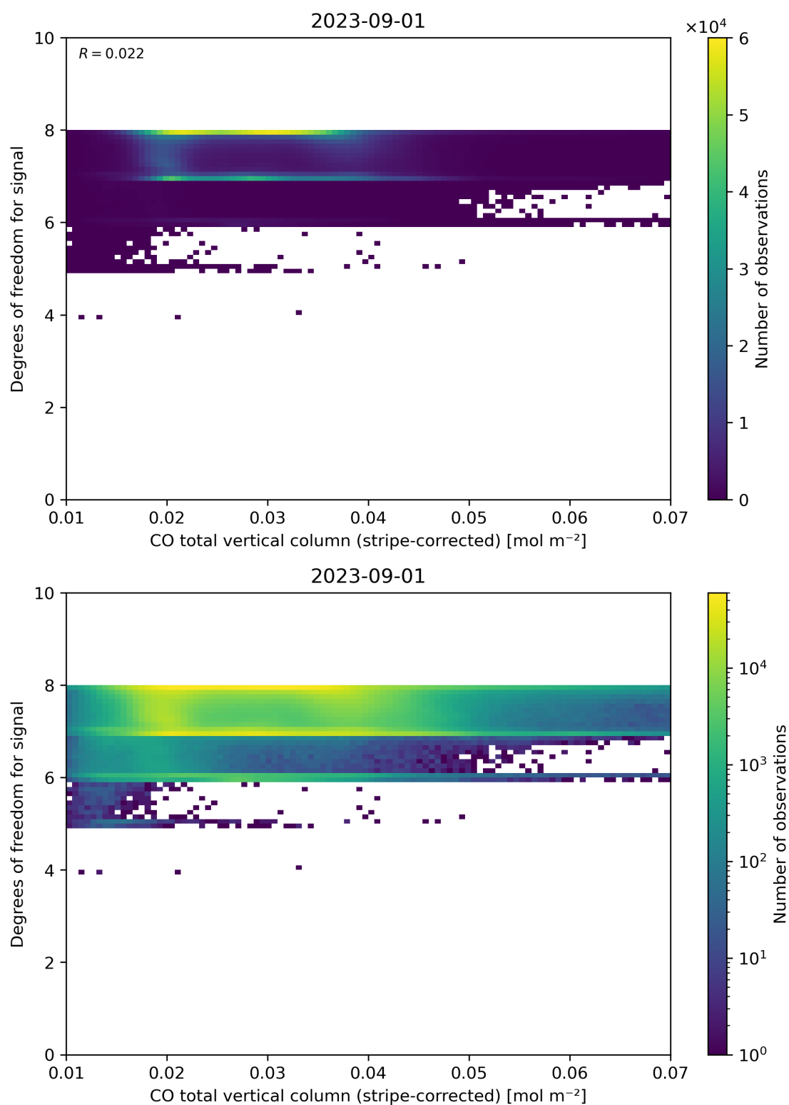
Figure 38: Scatter density plot of “CO total vertical column (stripe-corrected)” against “Degrees of freedom for signal” for 2023-08-31 to 2023-09-02.
