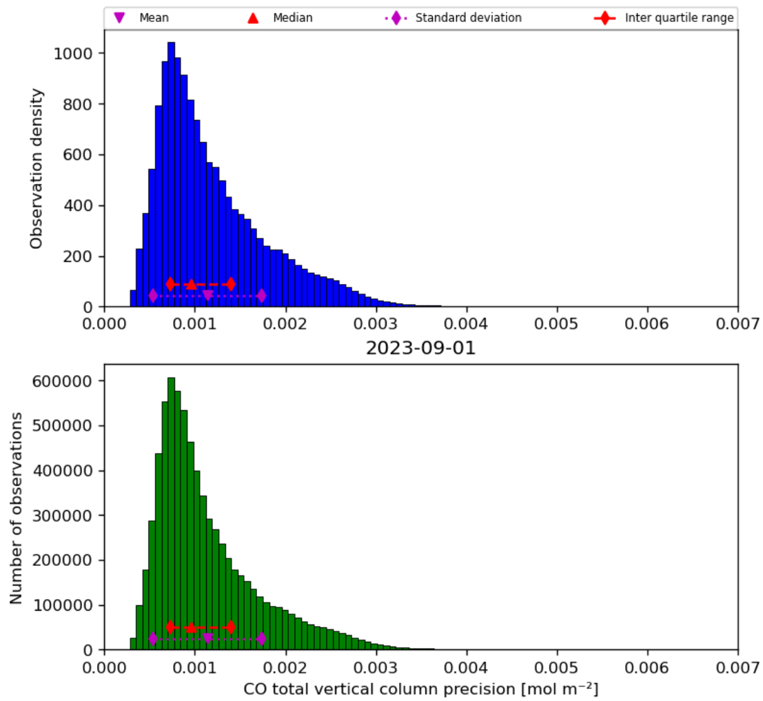
Figure 20: Histogram of “CO total vertical column precision” for 2023-08-31 to 2023-09-02
