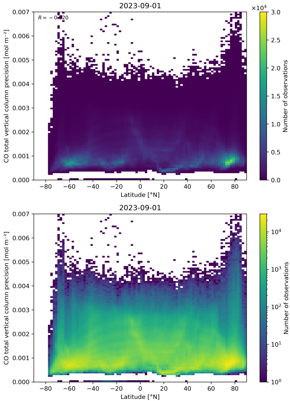
Figure 53: Scatter density plot of “Latitude” against “CO total vertical column precision” for 2023-08-31 to 2023-09-02.
