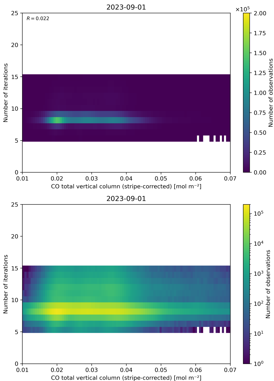
Figure 39: Scatter density plot of “CO total vertical column (stripe-corrected)” against “Number of iterations” for 2023-08-31 to 2023-09-02.
