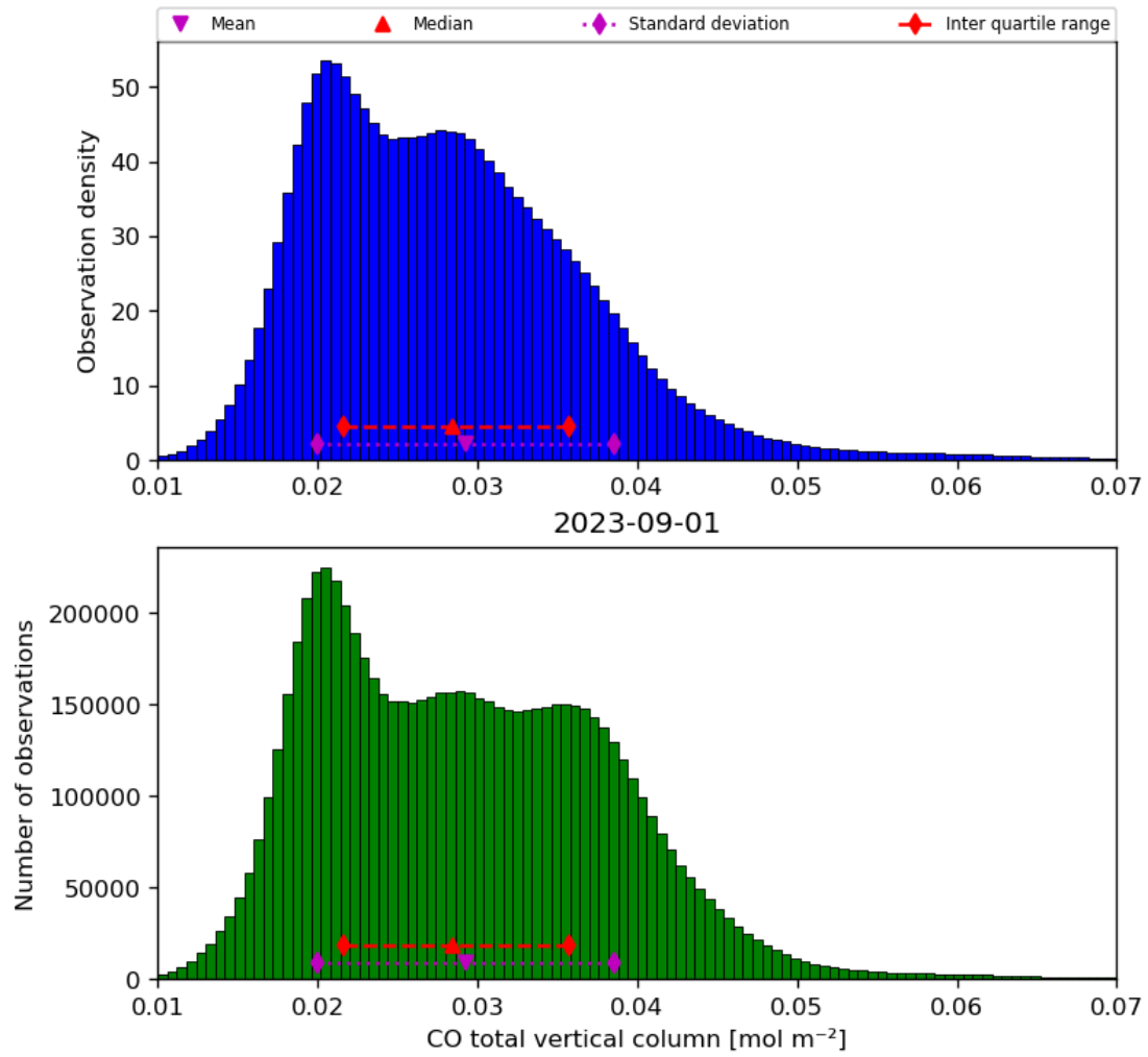
Figure 18: Histogram of “CO total vertical column” for 2023-08-31 to 2023-09-02
