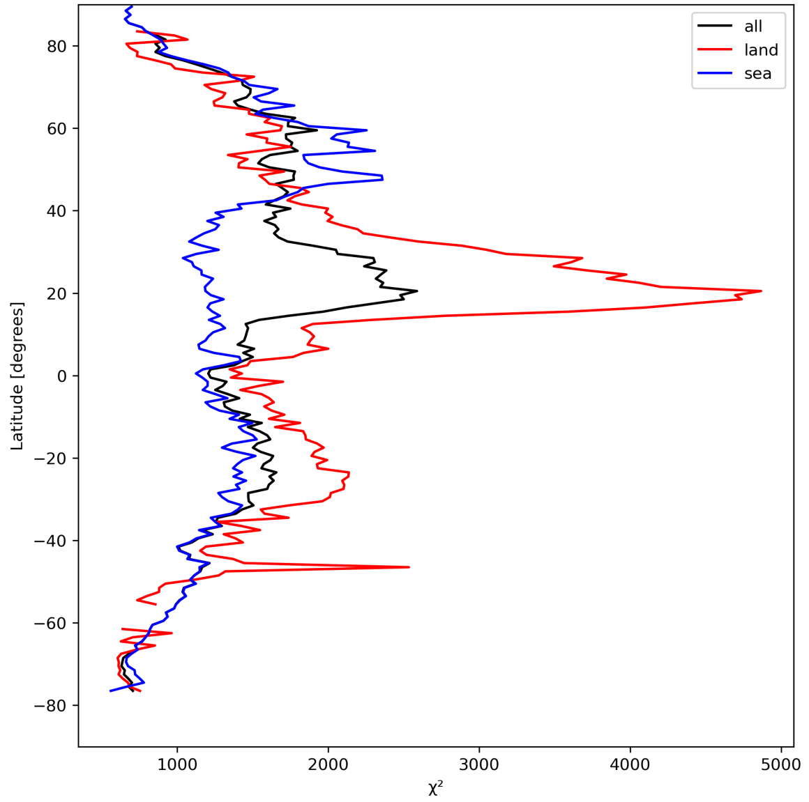
Figure 14: Zonal average of “ \chi^2 ” for 2023-08-31 to 2023-09-02.
