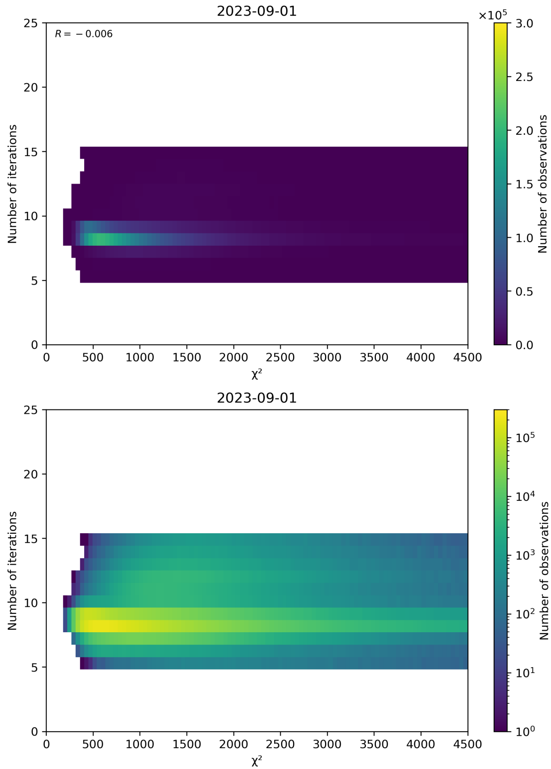
Figure 49: Scatter density plot of “ \chi^2 ” against “Number of iterations” for 2023-08-31 to 2023-09-02.
