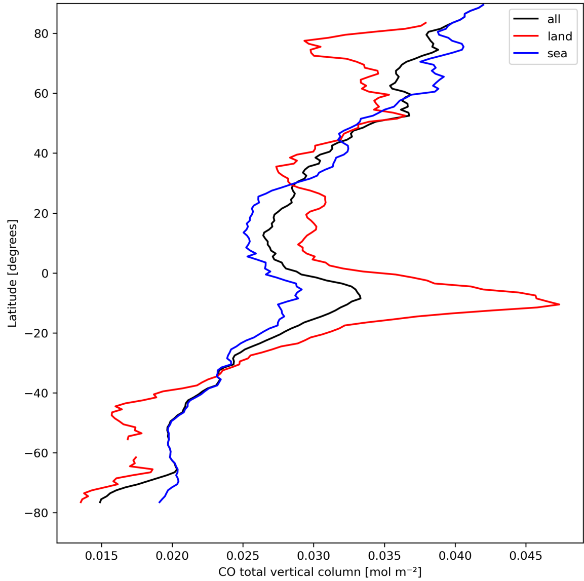
Figure 10: Zonal average of “CO total vertical column” for 2023-08-31 to 2023-09-02.
