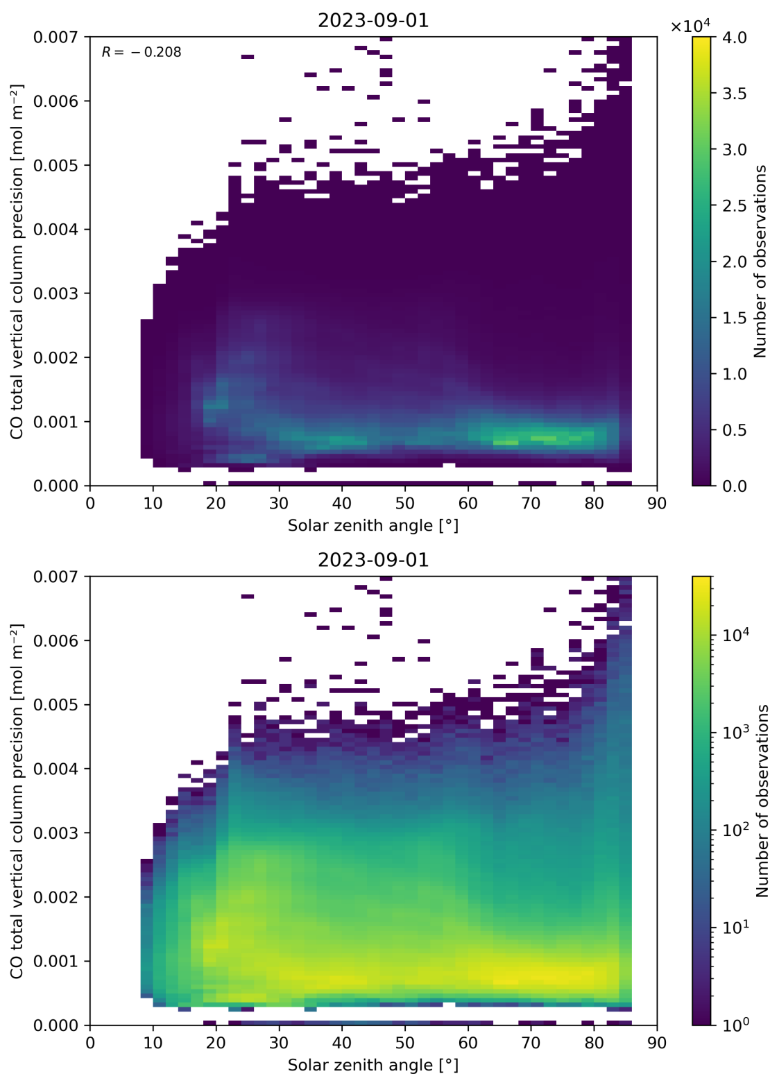
Figure 63: Scatter density plot of “Solar zenith angle” against “CO total vertical column precision” for 2023-08-31 to 2023-09-02.
