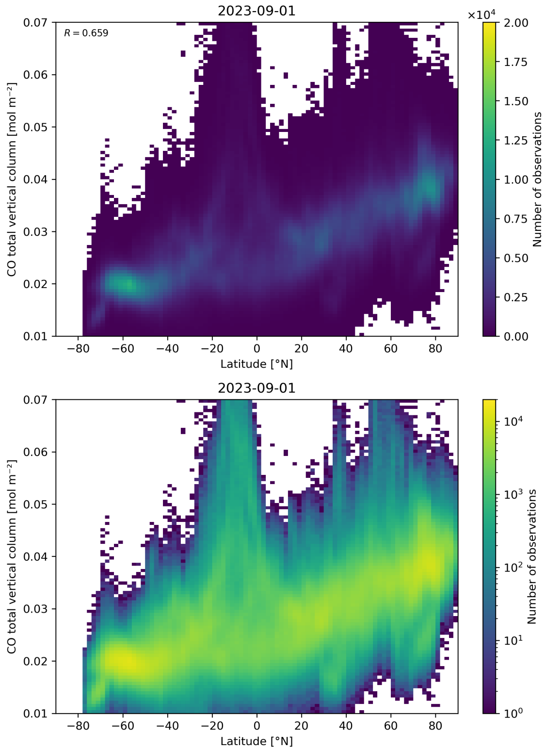
Figure 51: Scatter density plot of “Latitude” against “CO total vertical column” for 2023-08-31 to 2023-09-02.
