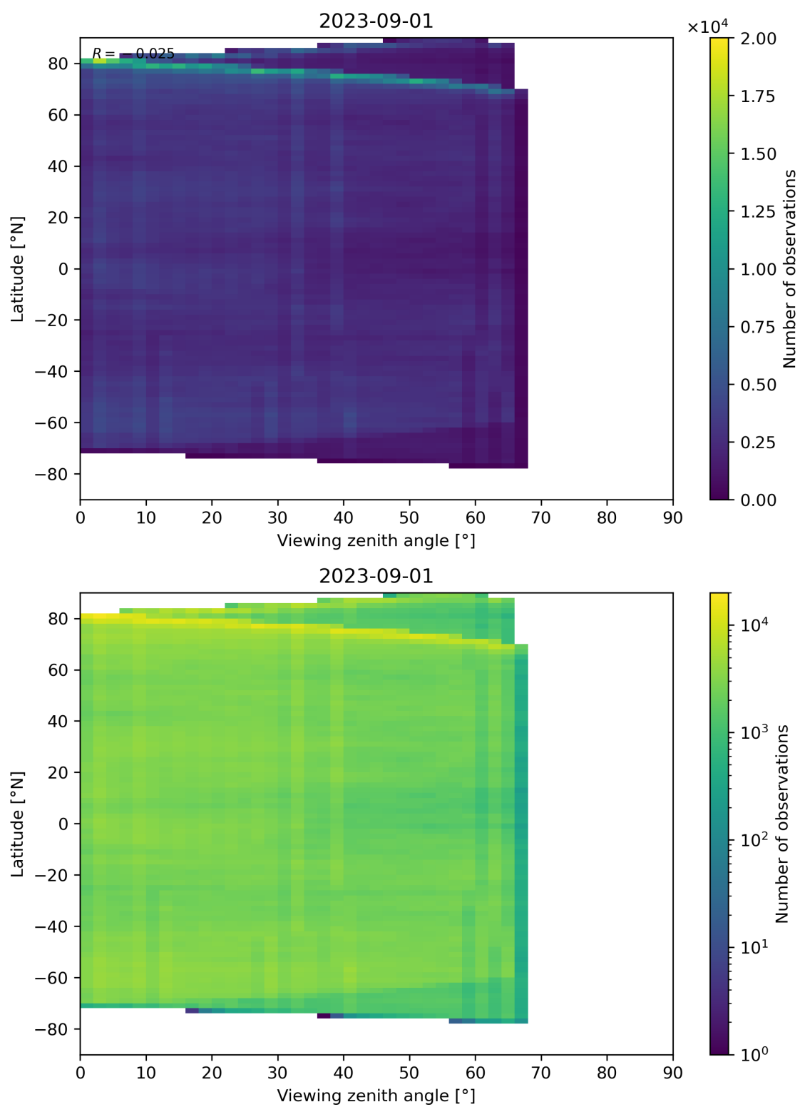
Figure 74: Scatter density plot of “Viewing zenith angle” against “Latitude” for 2023-08-31 to 2023-09-02.
