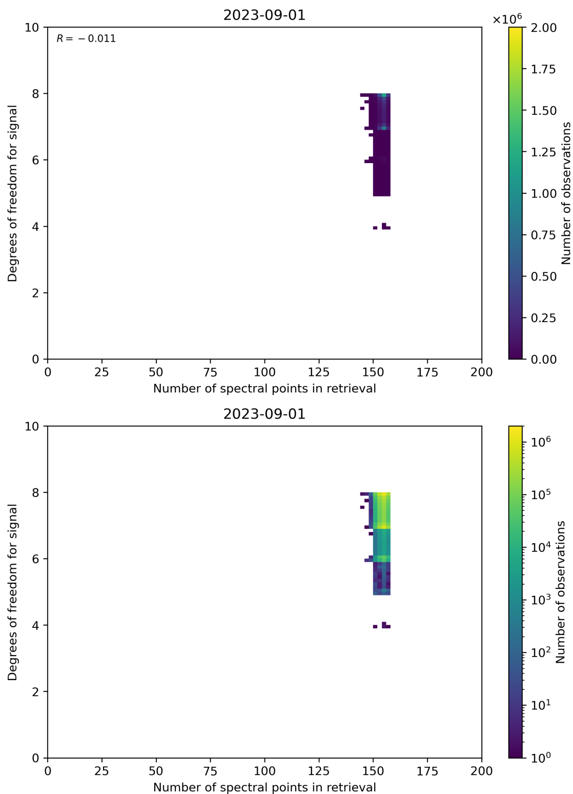
Figure 59: Scatter density plot of “Number of spectral points in retrieval” against “Degrees of freedom for signal” for 2023-08-31 to 2023-09-02.
