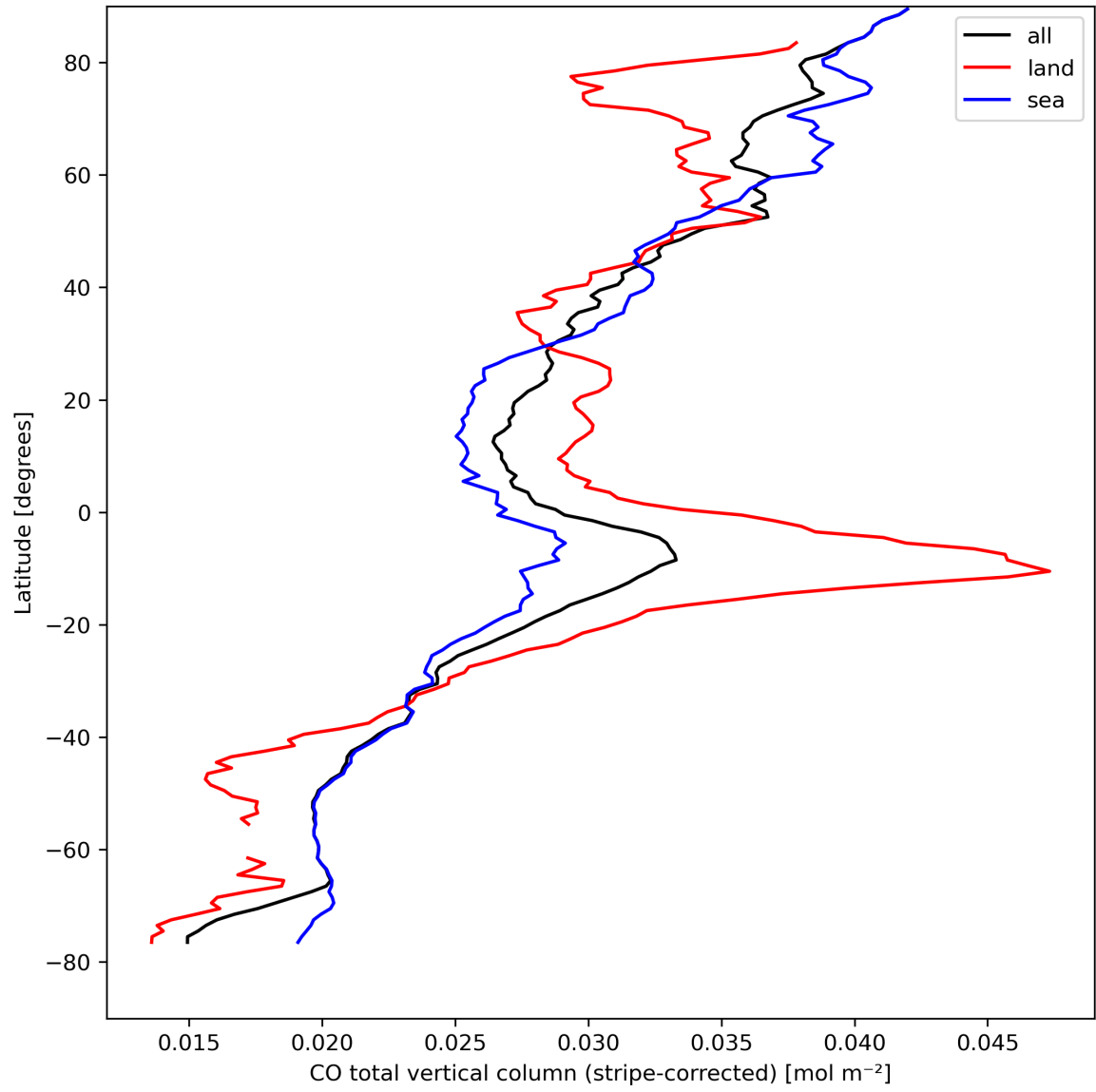
Figure 11: Zonal average of “CO total vertical column (stripe-corrected)” for 2023-08-31 to 2023-09-02.
