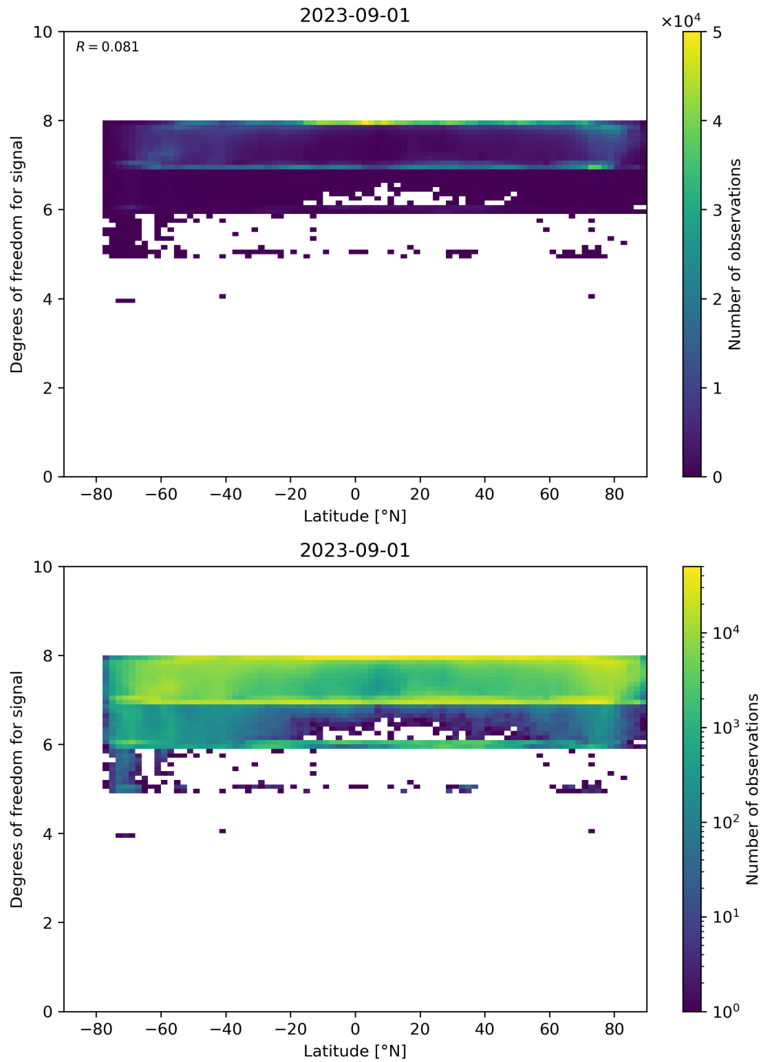
Figure 55: Scatter density plot of “Latitude” against “Degrees of freedom for signal” for 2023-08-31 to 2023-09-02.
