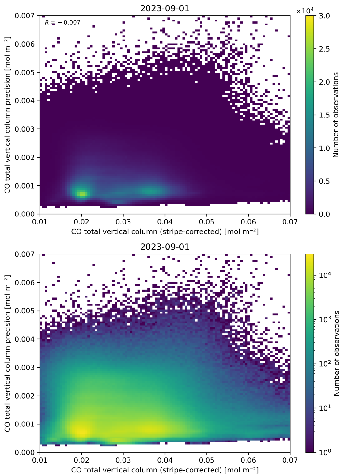
Figure 36: Scatter density plot of “CO total vertical column (stripe-corrected)” against “CO total vertical column precision” for 2023-08-31 to 2023-09-02.
