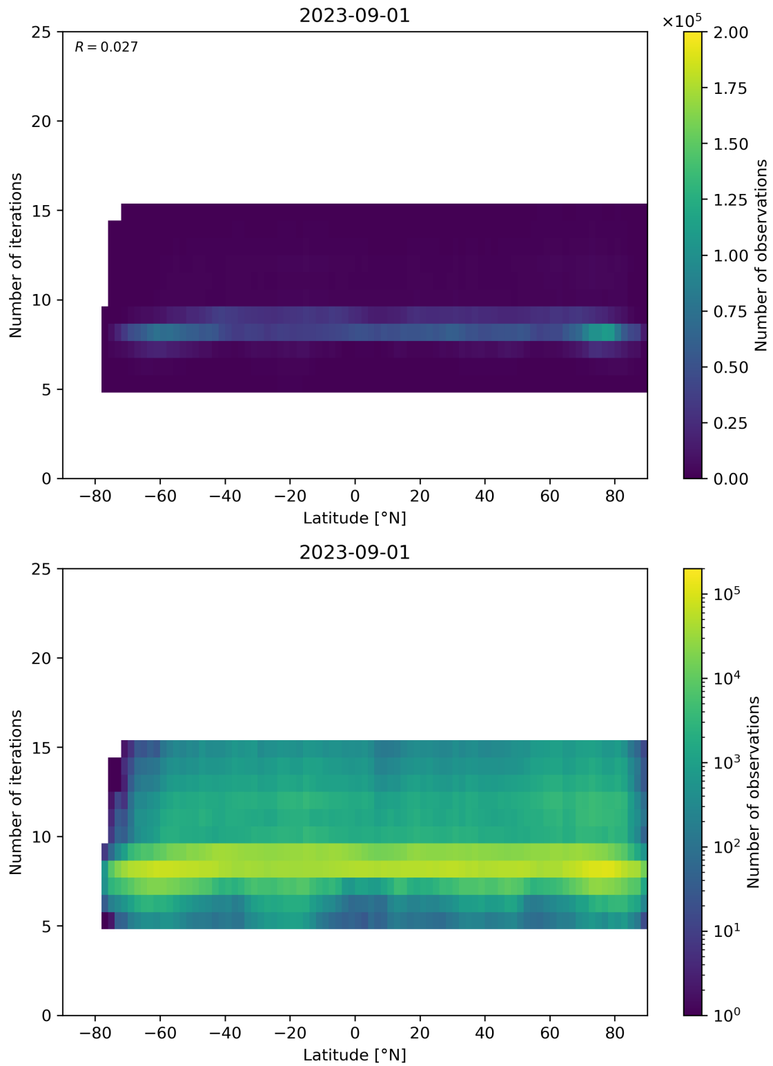
Figure 56: Scatter density plot of “Latitude” against “Number of iterations” for 2023-08-31 to 2023-09-02.
