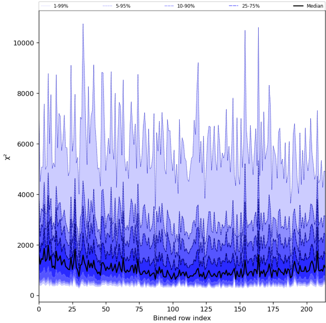
Figure 30: Along track statistics of “ \chi^2 ” for 2023-08-31 to 2023-09-02
