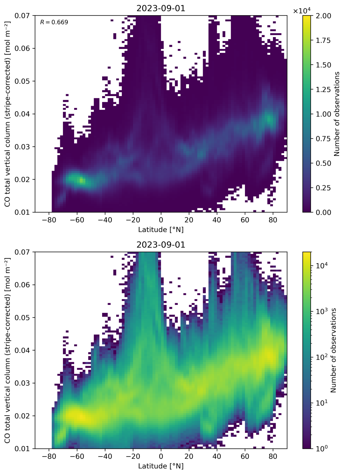
Figure 52: Scatter density plot of “Latitude” against “CO total vertical column (stripe-corrected)” for 2023-08-31 to 2023-09-02.
