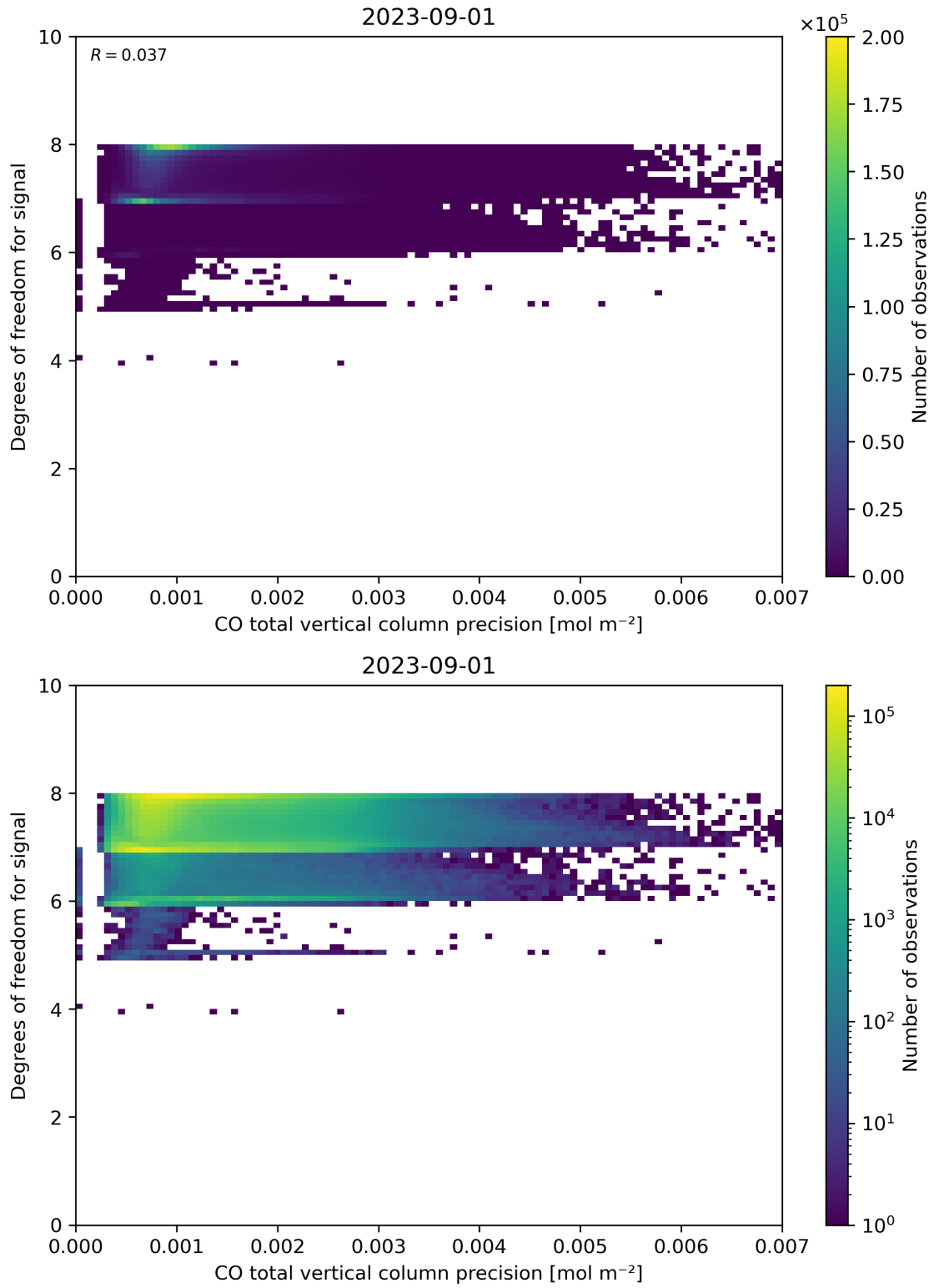
Figure 45: Scatter density plot of “CO total vertical column precision” against “Degrees of freedom for signal” for 2023-08-31 to 2023-09-02.
