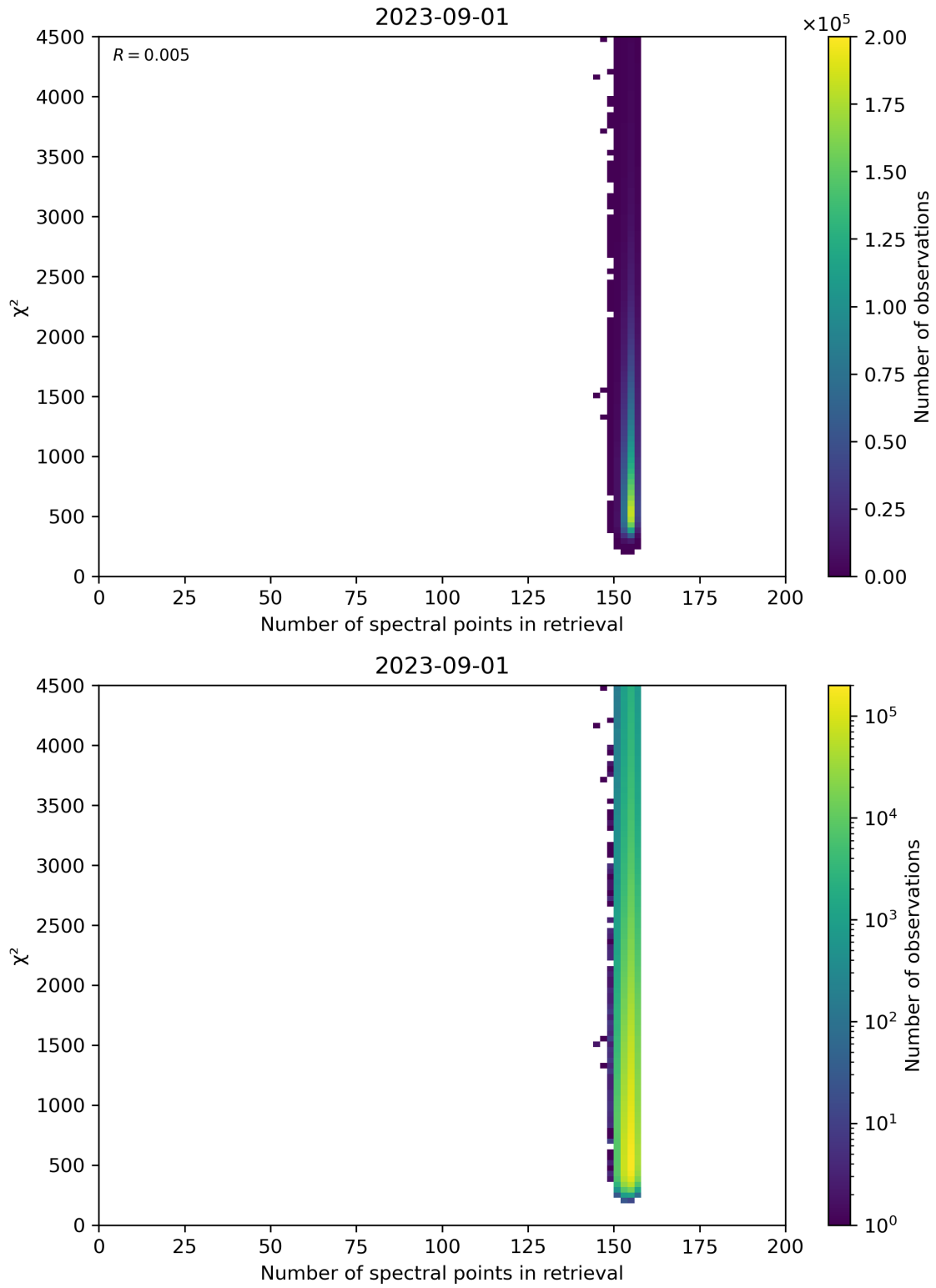
Figure 58: Scatter density plot of “Number of spectral points in retrieval” against “ \chi^2 ” for 2023-08-31 to 2023-09-02.
