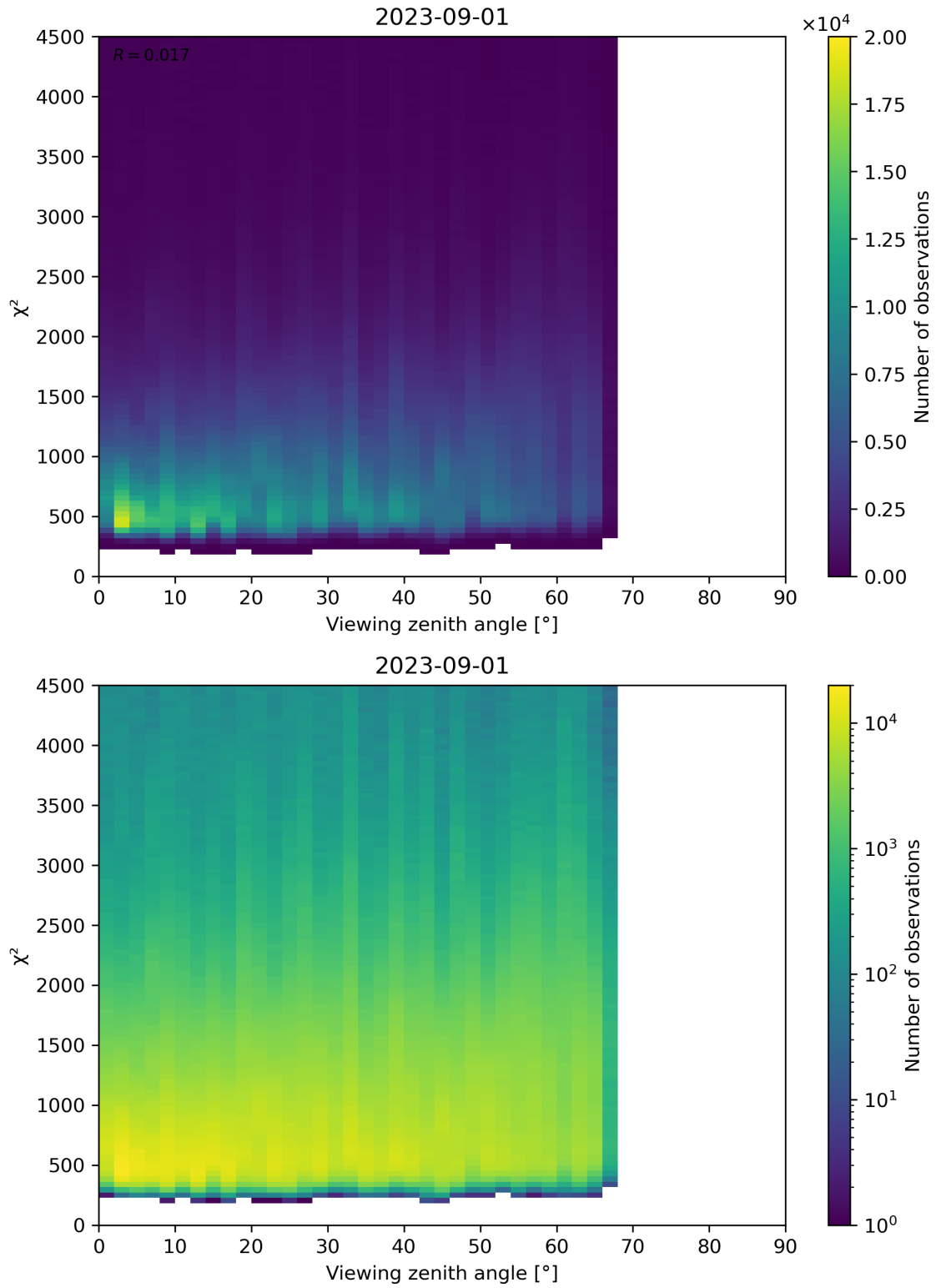
Figure 72: Scatter density plot of “Viewing zenith angle” against “ \chi^2 ” for 2023-08-31 to 2023-09-02.
