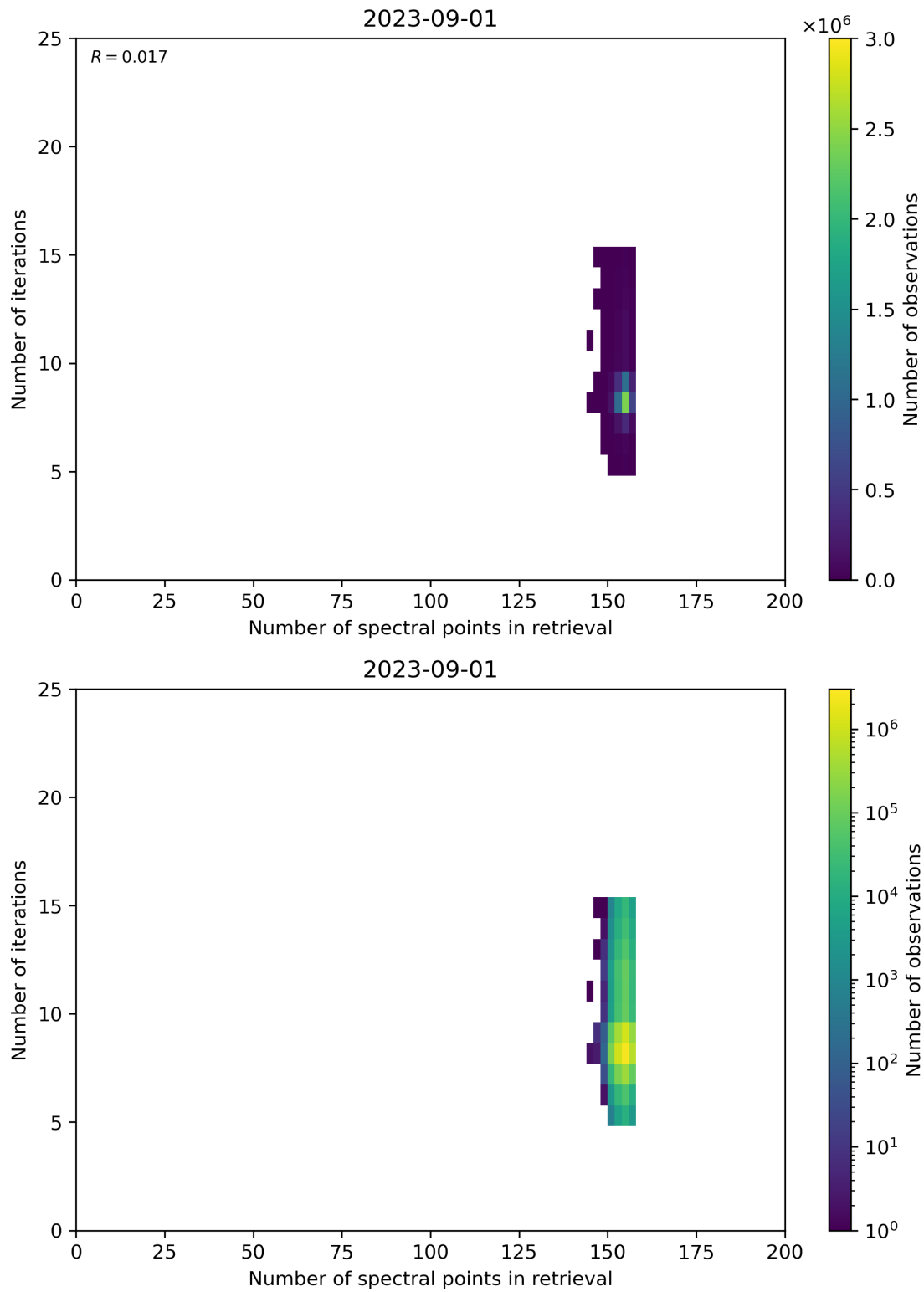
Figure 60: Scatter density plot of “Number of spectral points in retrieval” against “Number of iterations” for 2023-08-31 to 2023-09-02.
