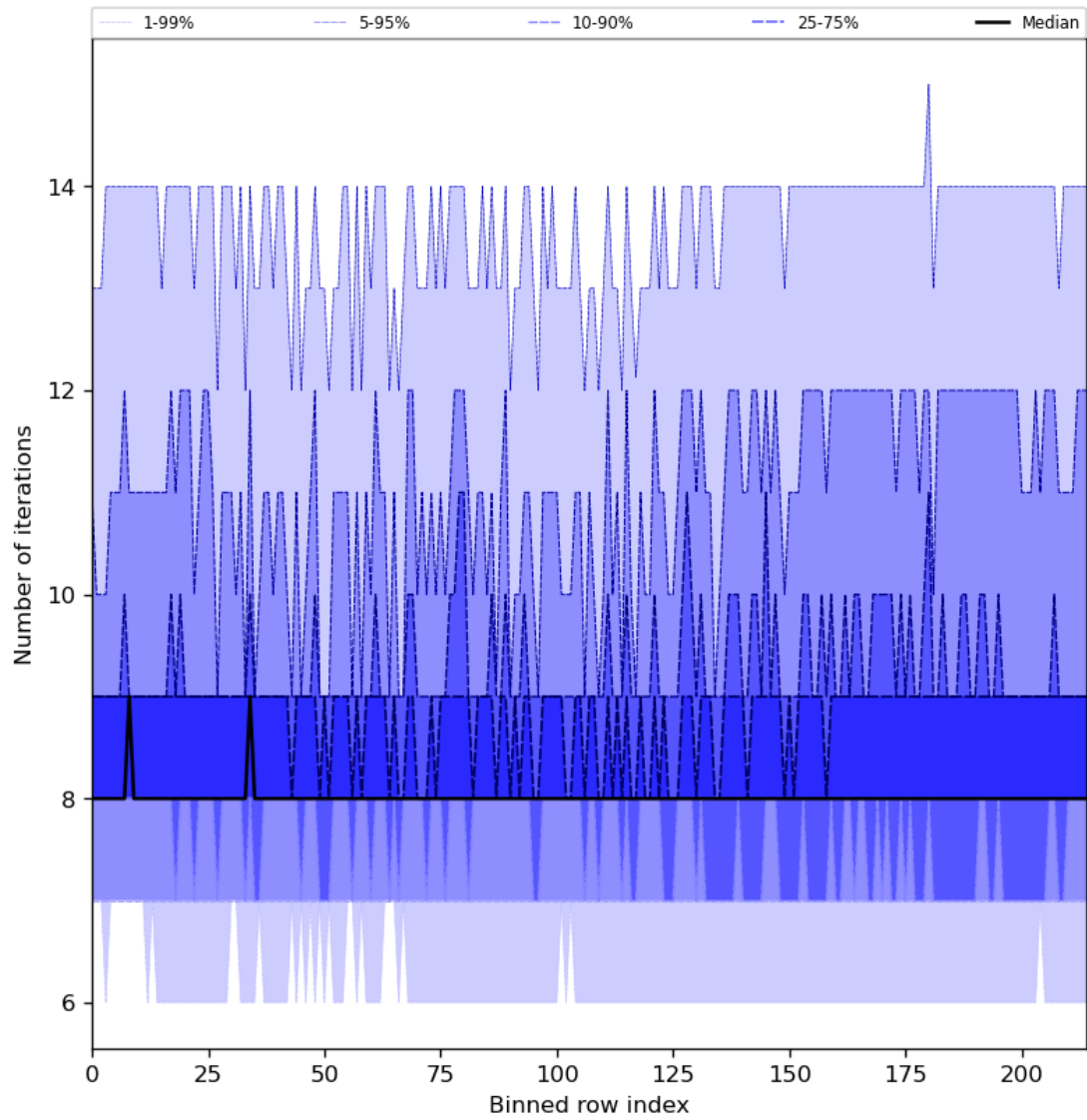
Figure 32: Along track statistics of “Number of iterations” for 2023-08-31 to 2023-09-02
