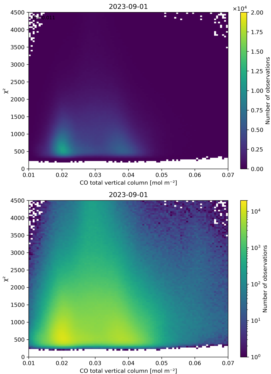
Figure 35: Scatter density plot of “CO total vertical column” against “ \chi^2 ” for 2023-08-31 to 2023-09-02.
