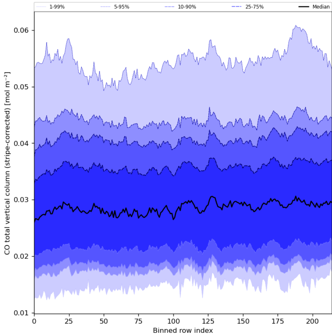
Figure 27: Along track statistics of “CO total vertical column (stripe-corrected)” for 2023-08-31 to 2023-09-02
