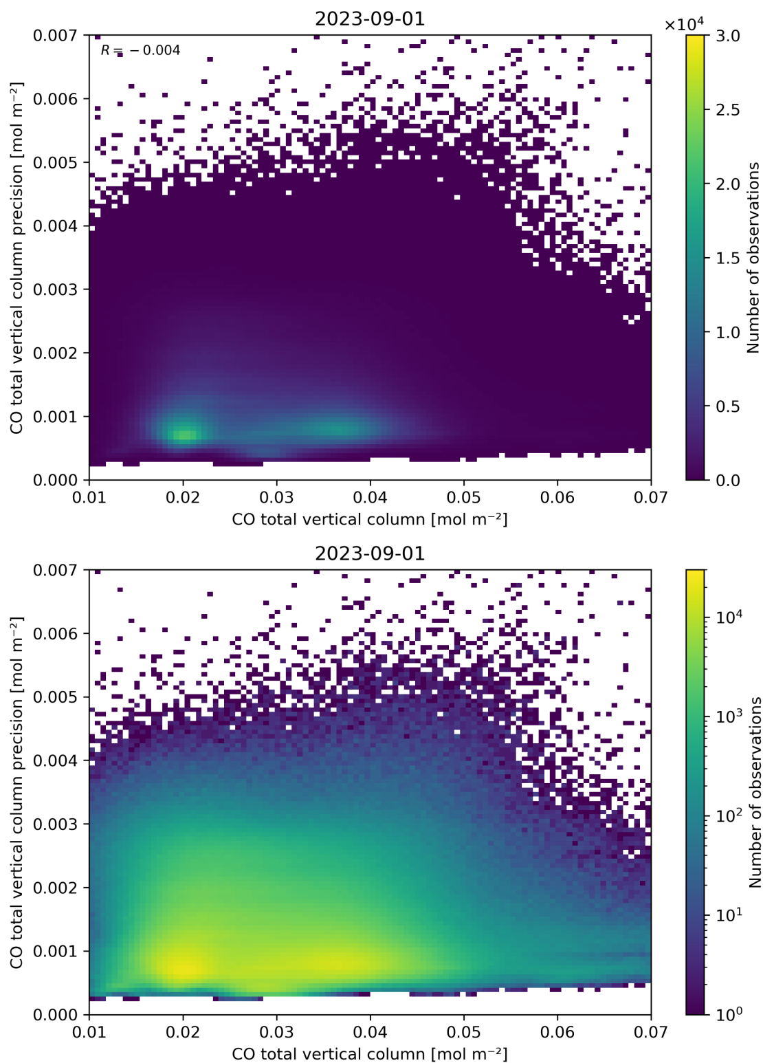
Figure 34: Scatter density plot of “CO total vertical column” against “CO total vertical column precision” for 2023-08-31 to 2023-09-02.
