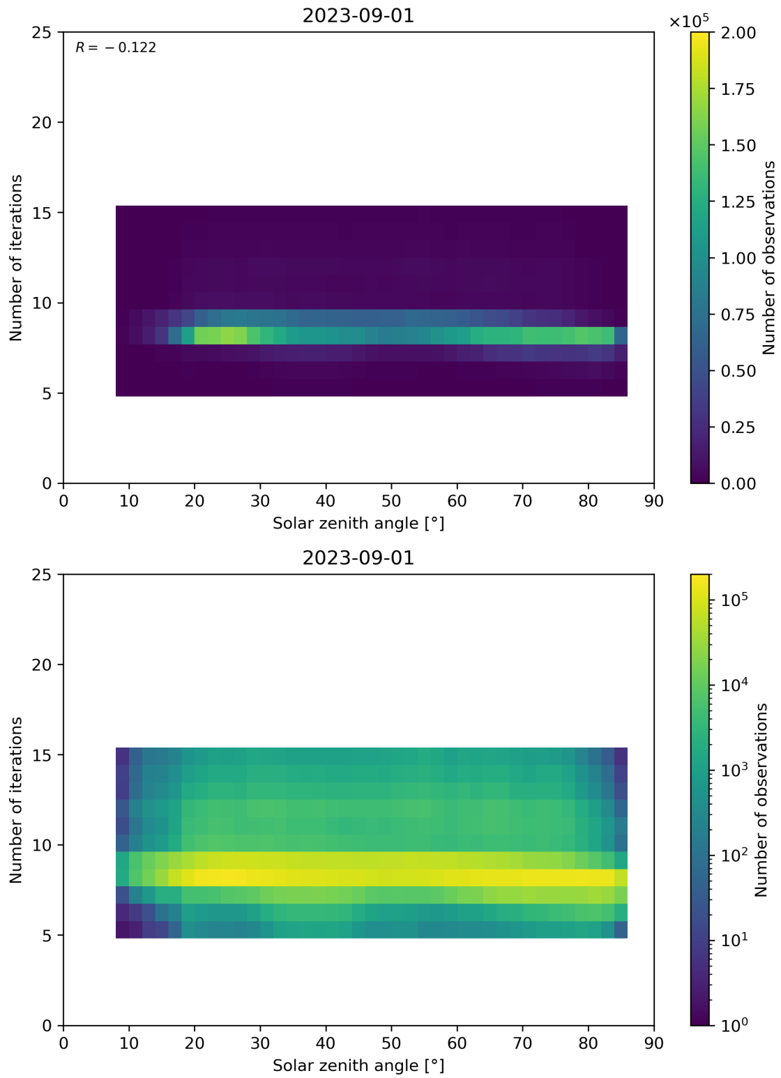
Figure 67: Scatter density plot of “Solar zenith angle” against “Number of iterations” for 2023-08-31 to 2023-09-02.
