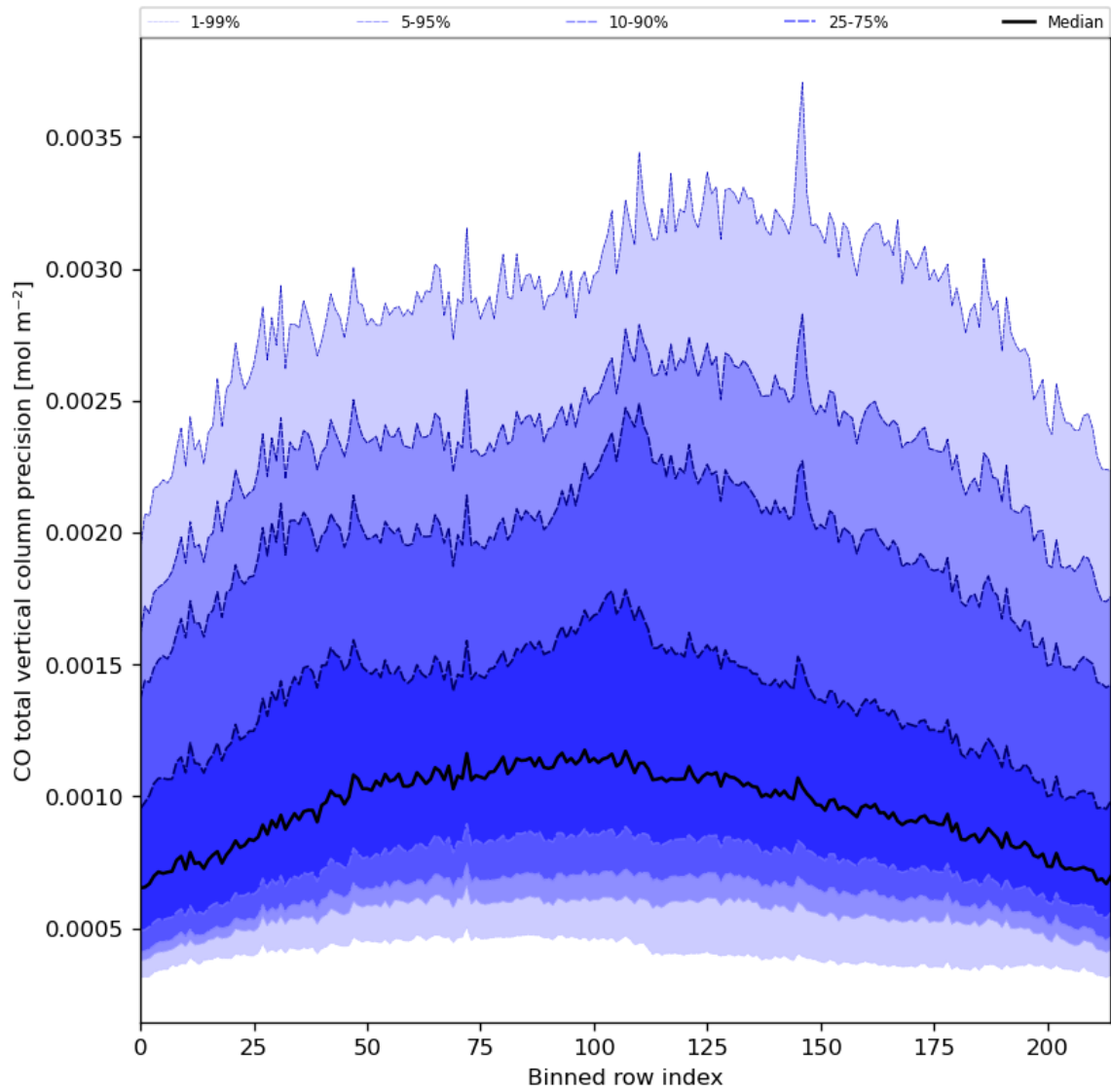
Figure 28: Along track statistics of “CO total vertical column precision” for 2023-08-31 to 2023-09-02
