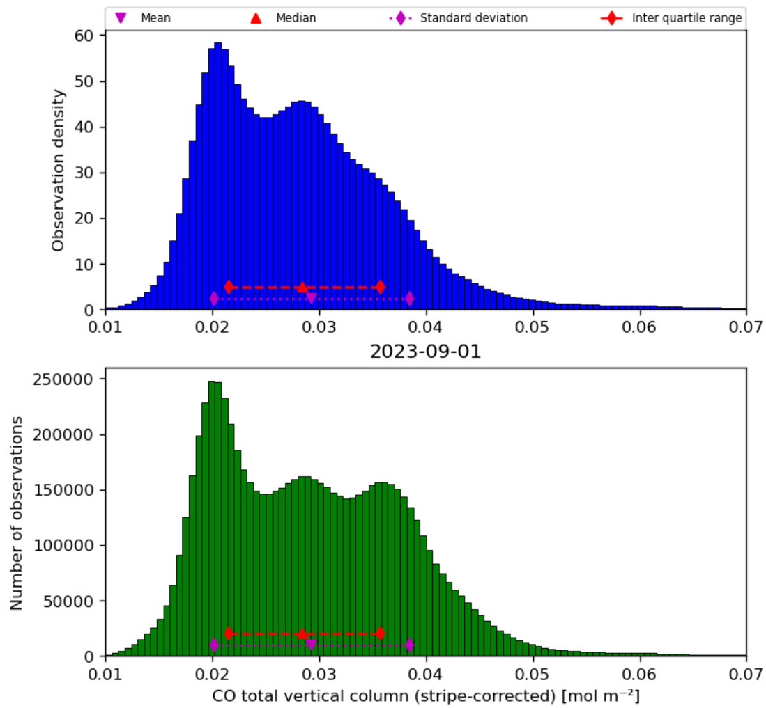
Figure 19: Histogram of “CO total vertical column (stripe-corrected)” for 2023-08-31 to 2023-09-02
