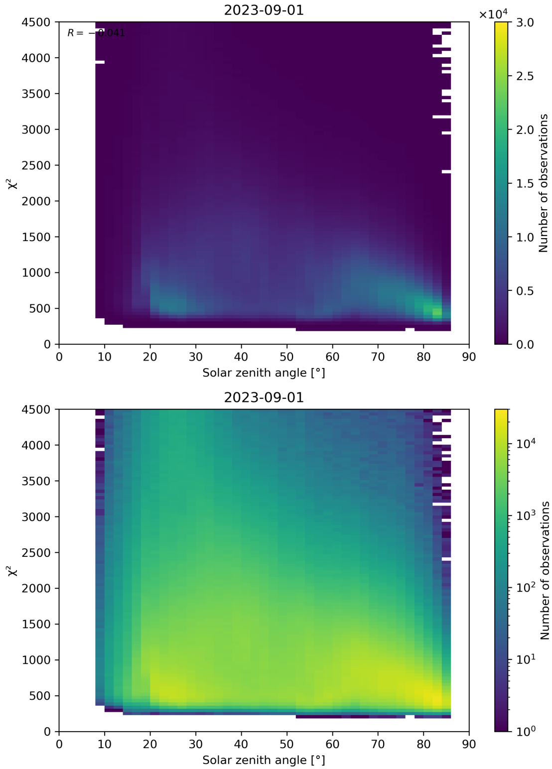
Figure 64: Scatter density plot of “Solar zenith angle” against “ \chi^2 ” for 2023-08-31 to 2023-09-02.
