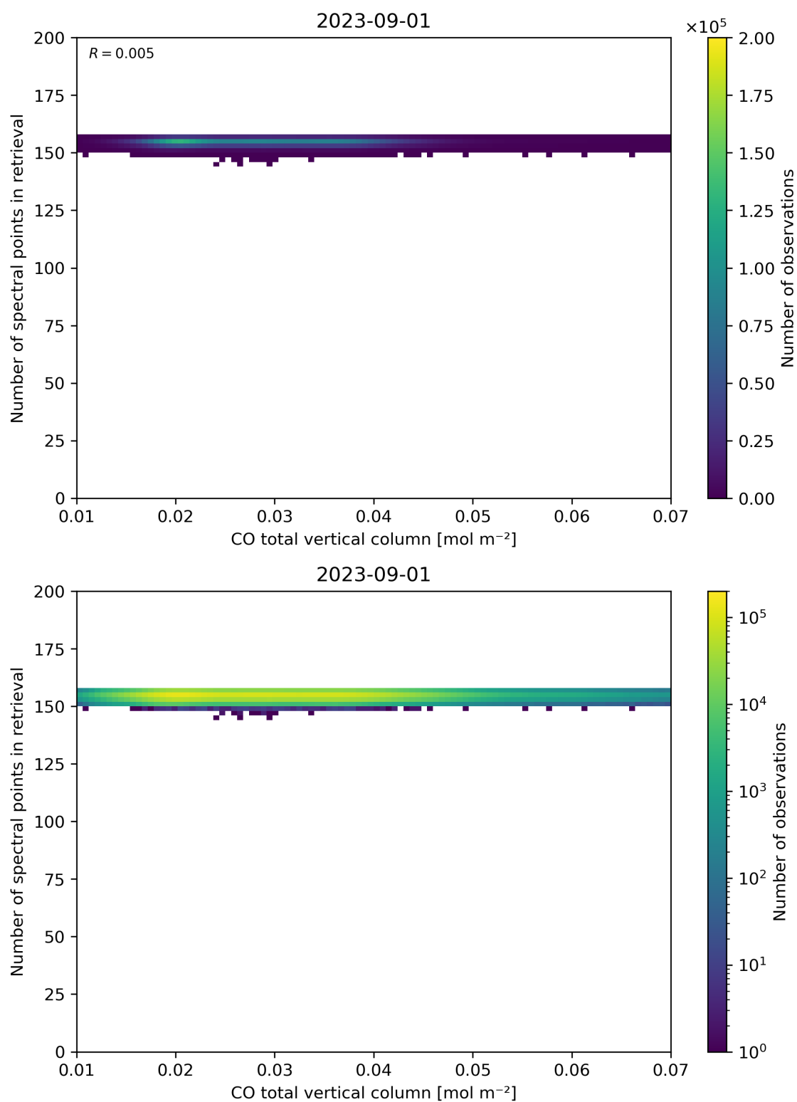
Figure 43: Scatter density plot of “CO total vertical column” against “Number of spectral points in retrieval” for 2023-08-31 to 2023-09-02.
