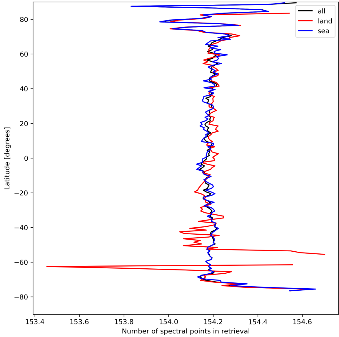
Figure 13: Zonal average of “Number of spectral points in retrieval” for 2023-08-31 to 2023-09-02.
