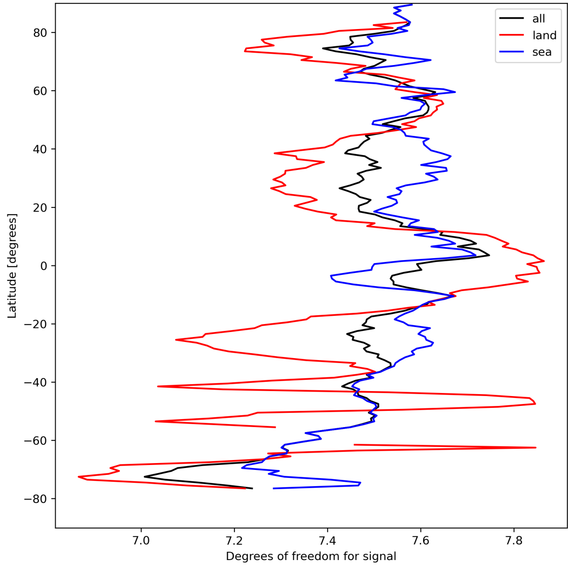
Figure 15: Zonal average of “Degrees of freedom for signal” for 2023-08-31 to 2023-09-02.
