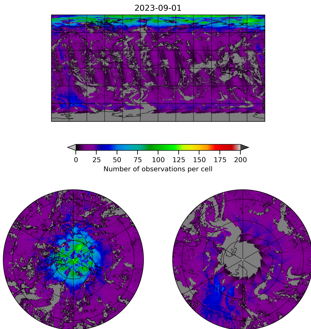
Figure 8: Map of the number of observations for 2023-08-31 to 2023-09-02
