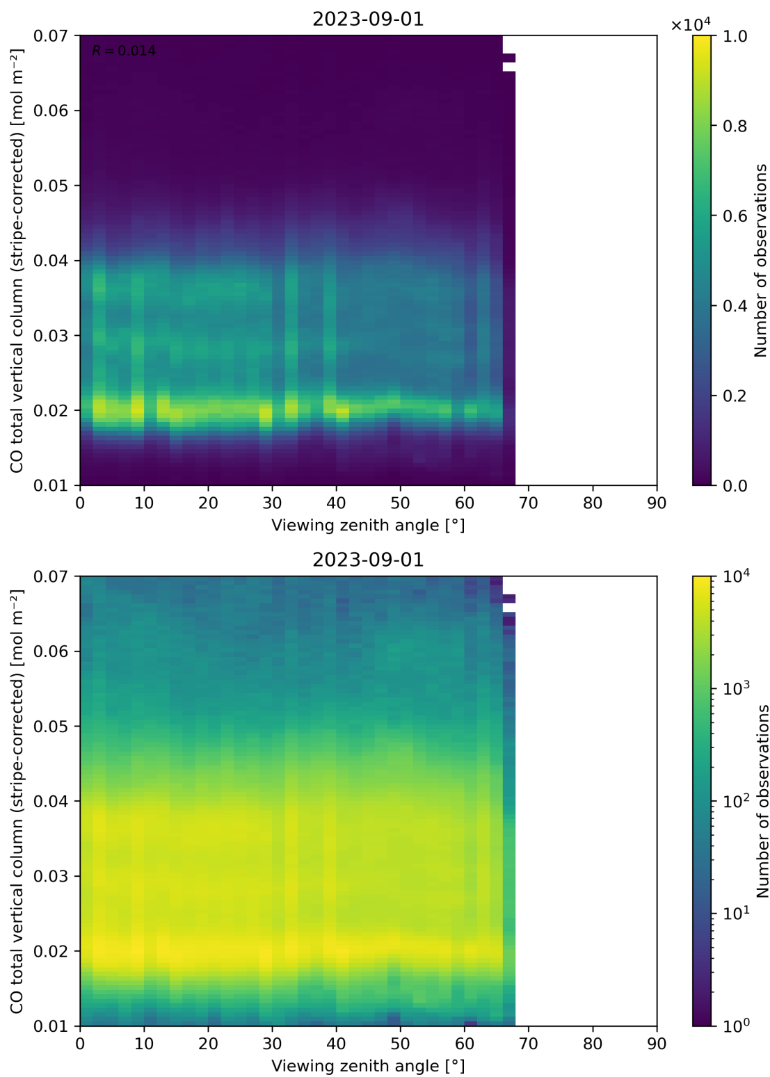
Figure 70: Scatter density plot of “Viewing zenith angle” against “CO total vertical column (stripe-corrected)” for 2023-08-31 to 2023-09-02.
