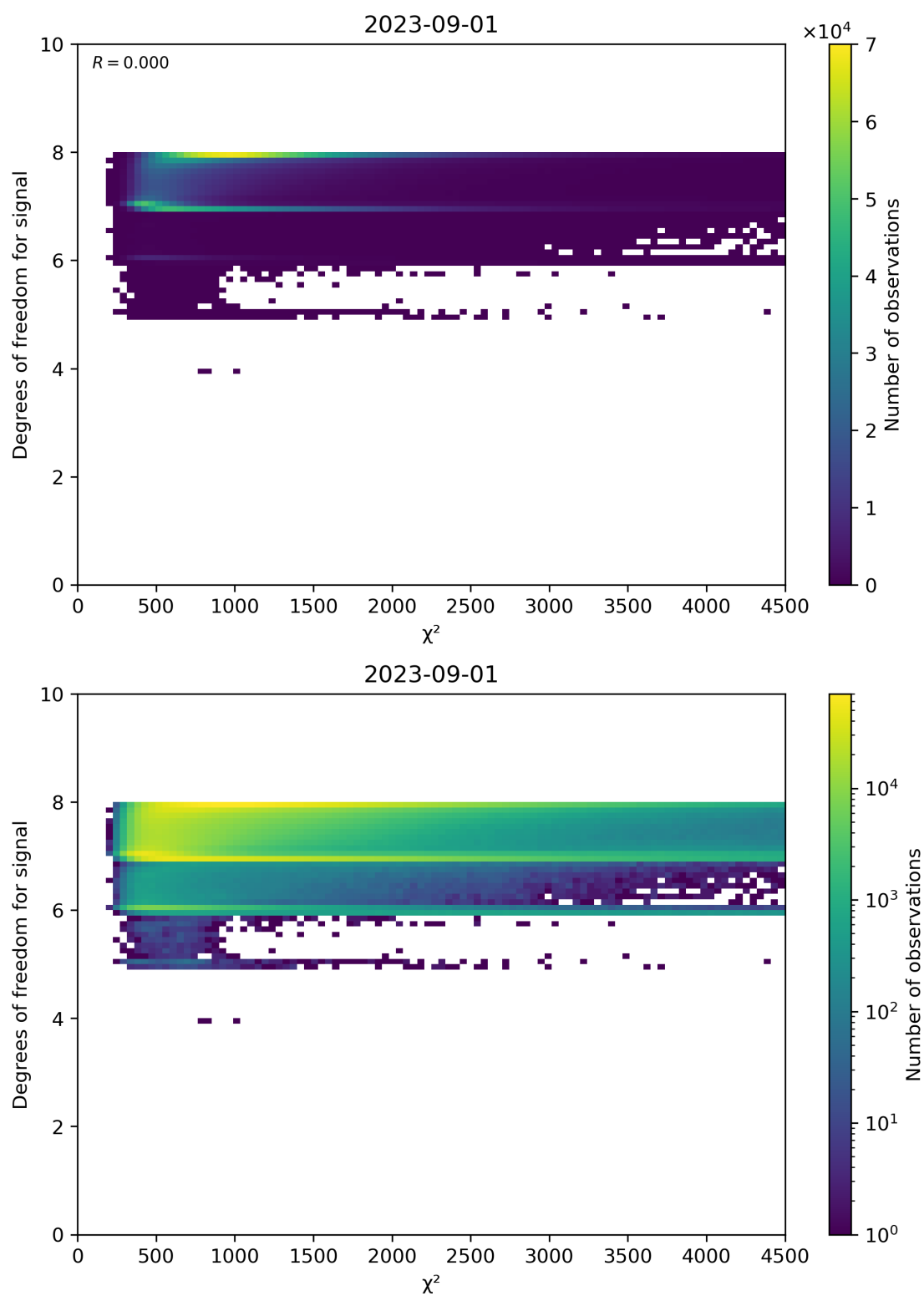
Figure 48: Scatter density plot of " \chi^2 " against "Degrees of freedom for signal" for 2023-08-31 to 2023-09-02.
