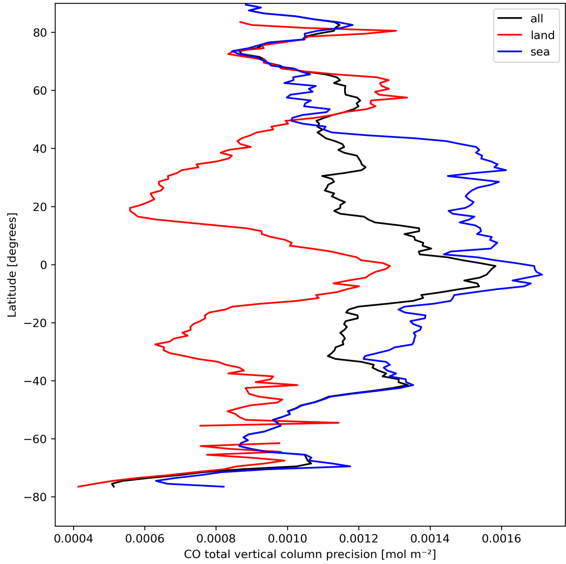
Figure 12: Zonal average of “CO total vertical column precision” for 2023-08-31 to 2023-09-02.
