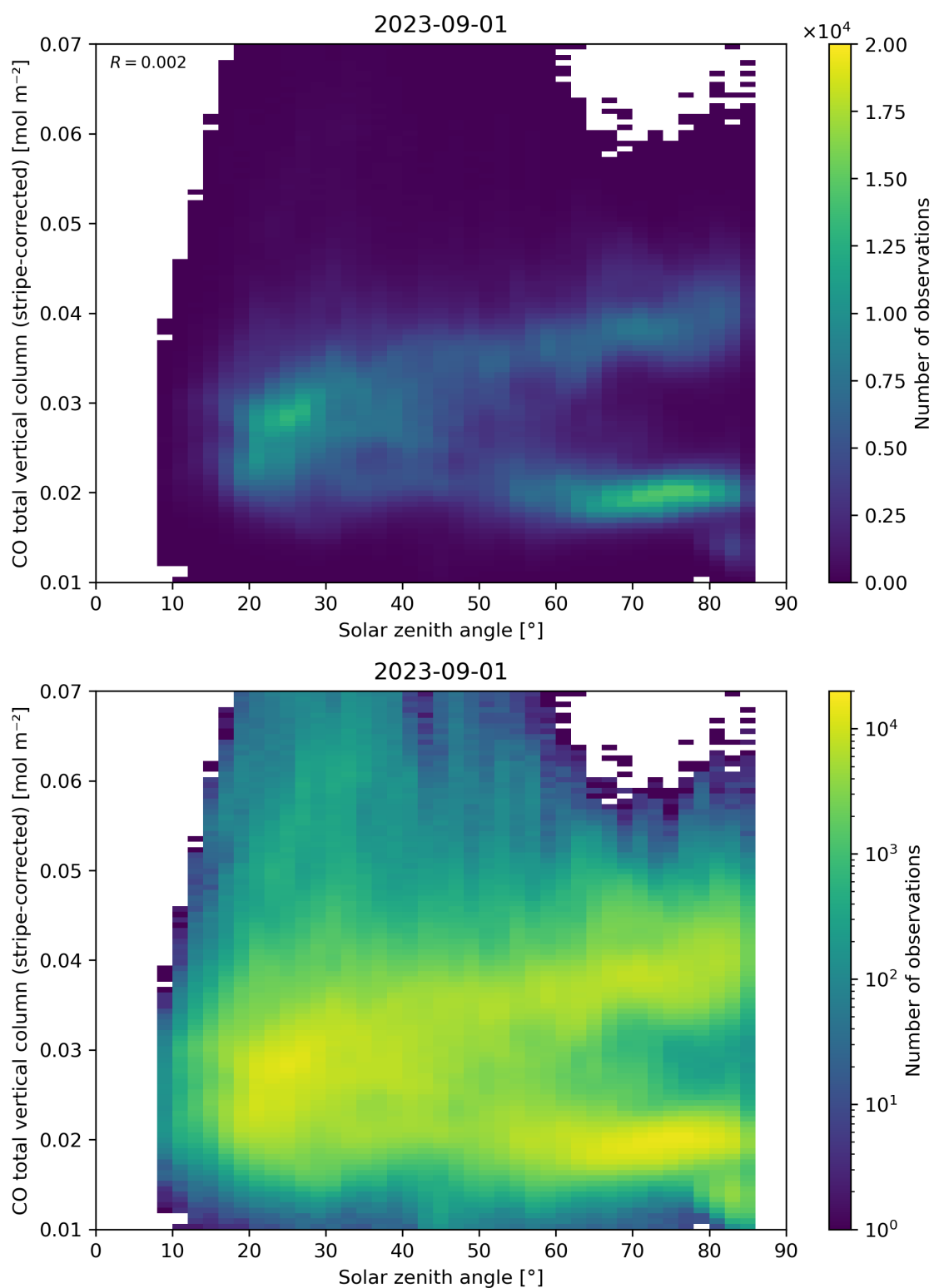
Figure 62: Scatter density plot of “Solar zenith angle” against “CO total vertical column (stripe-corrected)” for 2023-08-31 to 2023-09-02.
