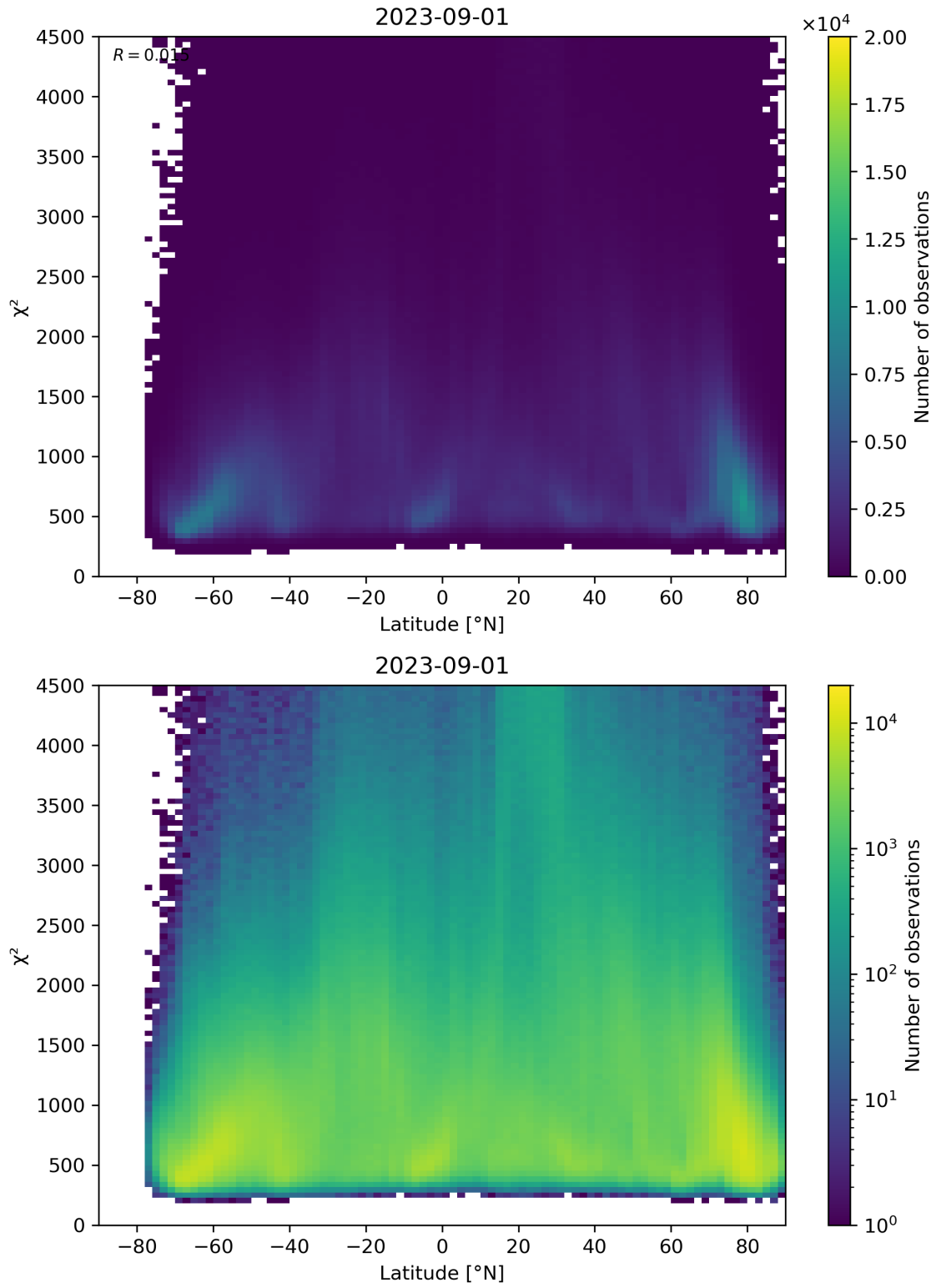
Figure 54: Scatter density plot of “Latitude” against “ \chi^2 ” for 2023-08-31 to 2023-09-02.
