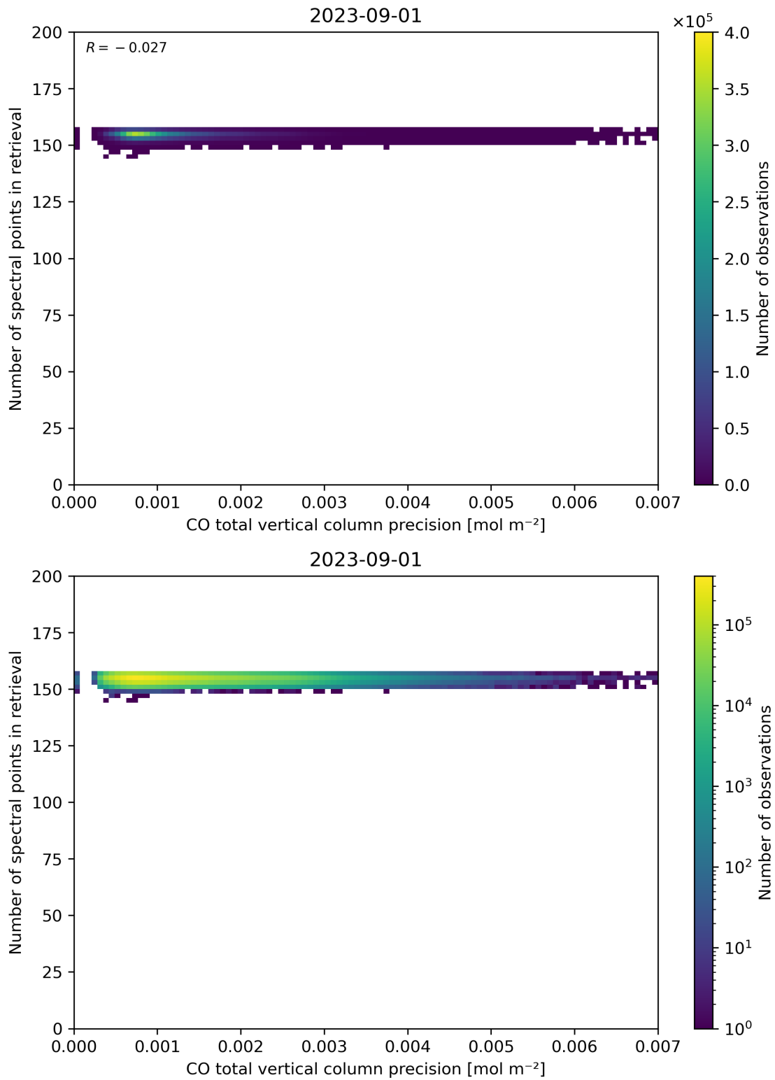
Figure 47: Scatter density plot of “CO total vertical column precision” against “Number of spectral points in retrieval” for 2023-08-31 to 2023-09-02.
