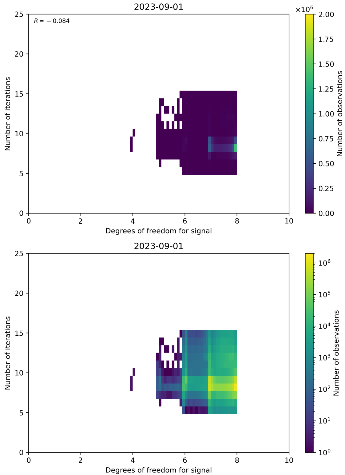
Figure 50: Scatter density plot of “Degrees of freedom for signal” against “Number of iterations” for 2023-08-31 to 2023-09-02.
