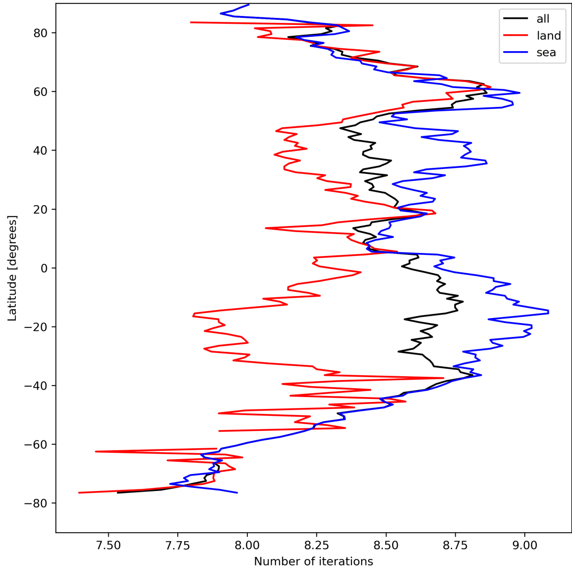
Figure 16: Zonal average of “Number of iterations” for 2023-08-31 to 2023-09-02.
