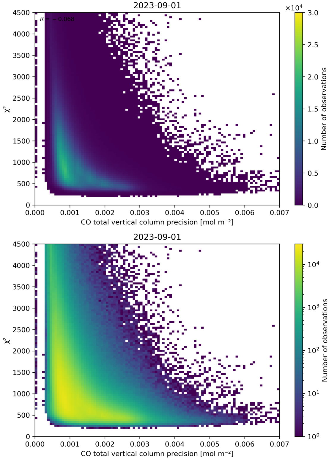
Figure 44: Scatter density plot of “CO total vertical column precision” against “ \chi^2 ” for 2023-08-31 to 2023-09-02.
