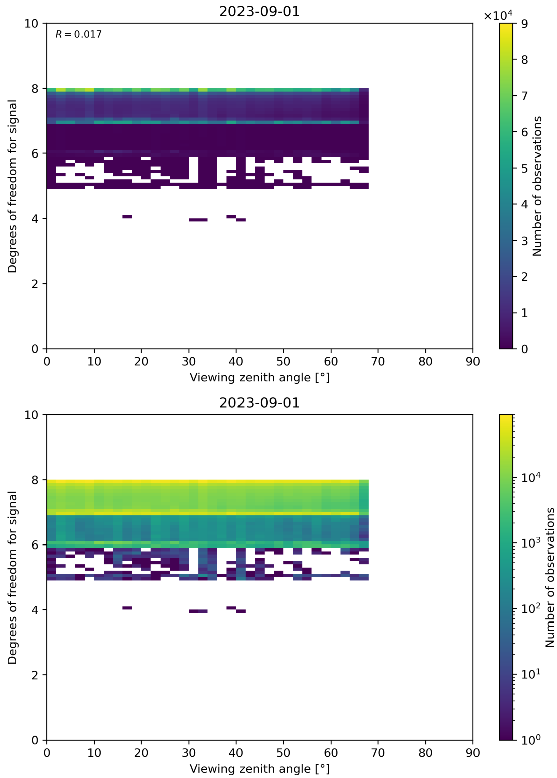
Figure 73: Scatter density plot of “Viewing zenith angle” against “Degrees of freedom for signal” for 2023-08-31 to 2023-09-02.
