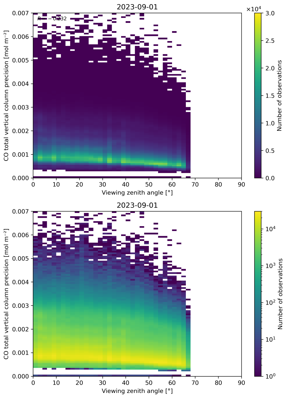
Figure 71: Scatter density plot of “Viewing zenith angle” against “CO total vertical column precision” for 2023-08-31 to 2023-09-02.
