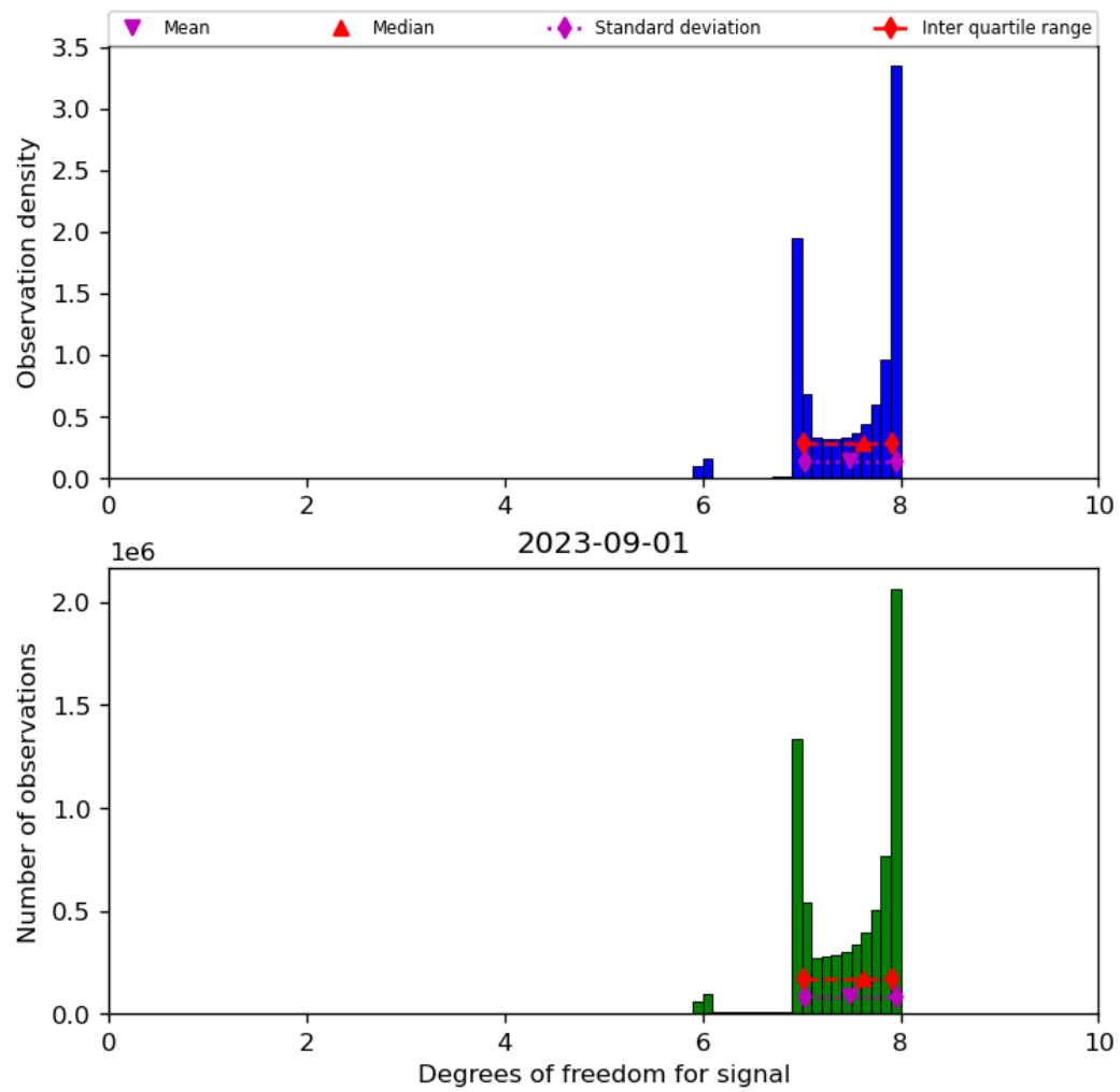
Figure 23: Histogram of “Degrees of freedom for signal” for 2023-08-31 to 2023-09-02
