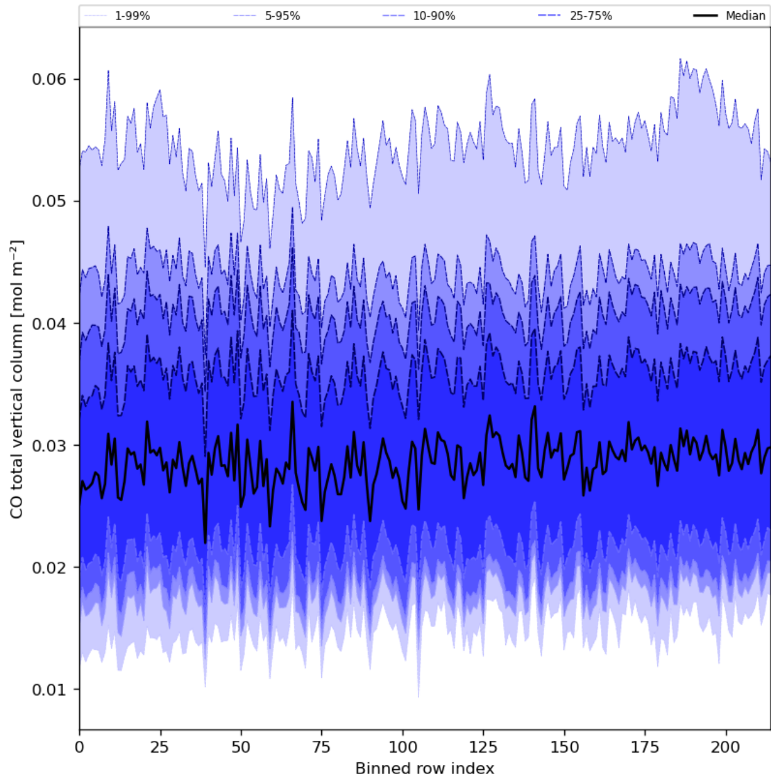
Figure 26: Along track statistics of “CO total vertical column” for 2023-08-31 to 2023-09-02
