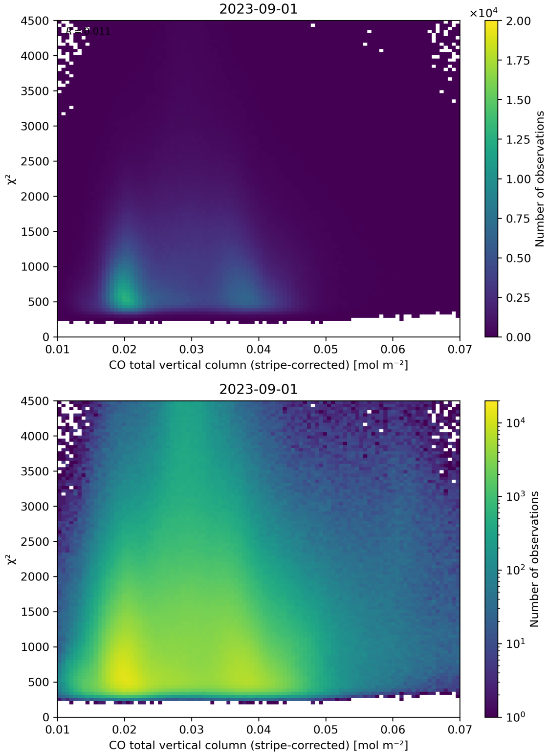
Figure 37: Scatter density plot of “CO total vertical column (stripe-corrected)” against “ \chi^2 ” for 2023-08-31 to 2023-09-02.
