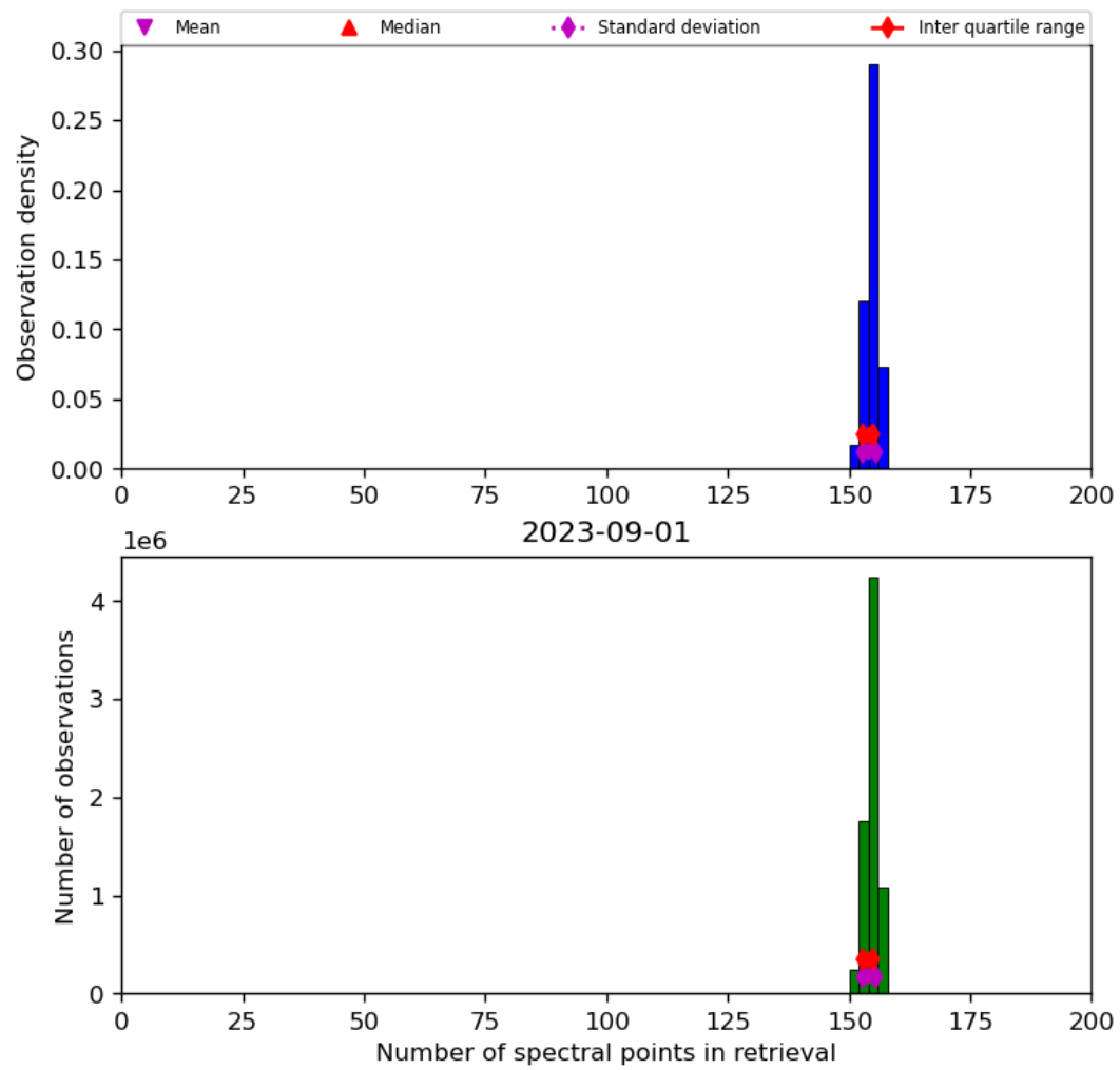
Figure 21: Histogram of “Number of spectral points in retrieval” for 2023-08-31 to 2023-09-02
