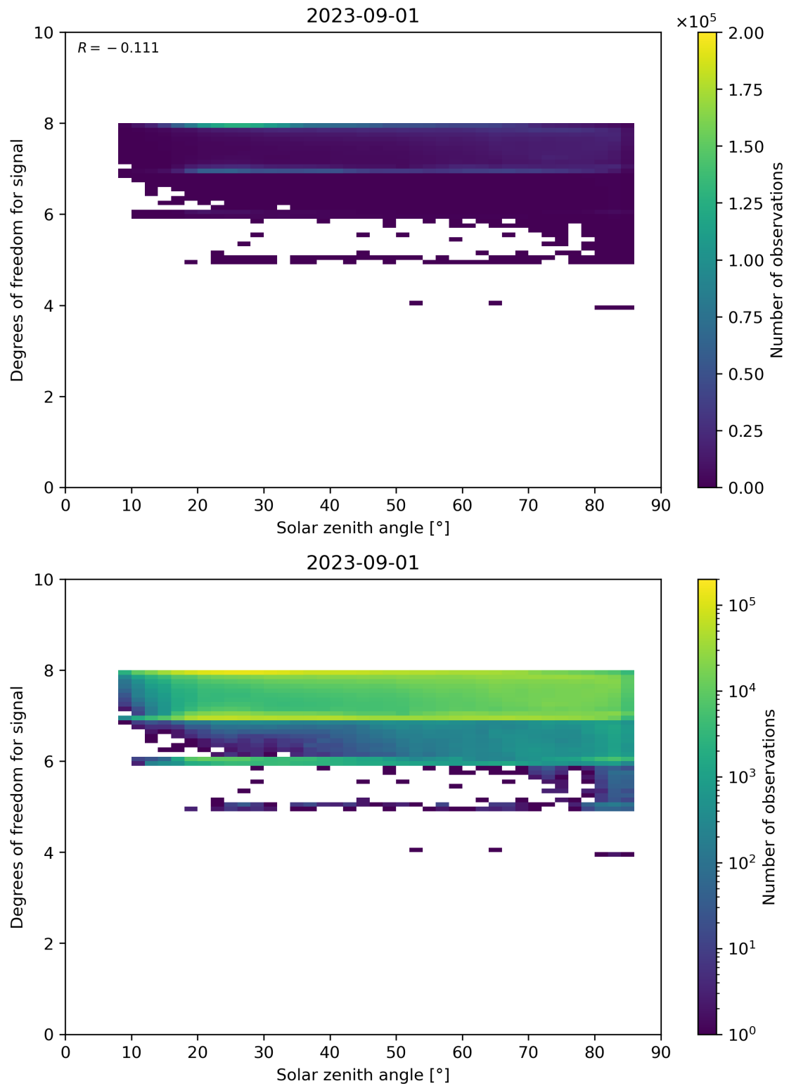
Figure 65: Scatter density plot of “Solar zenith angle” against “Degrees of freedom for signal” for 2023-08-31 to 2023-09-02.
