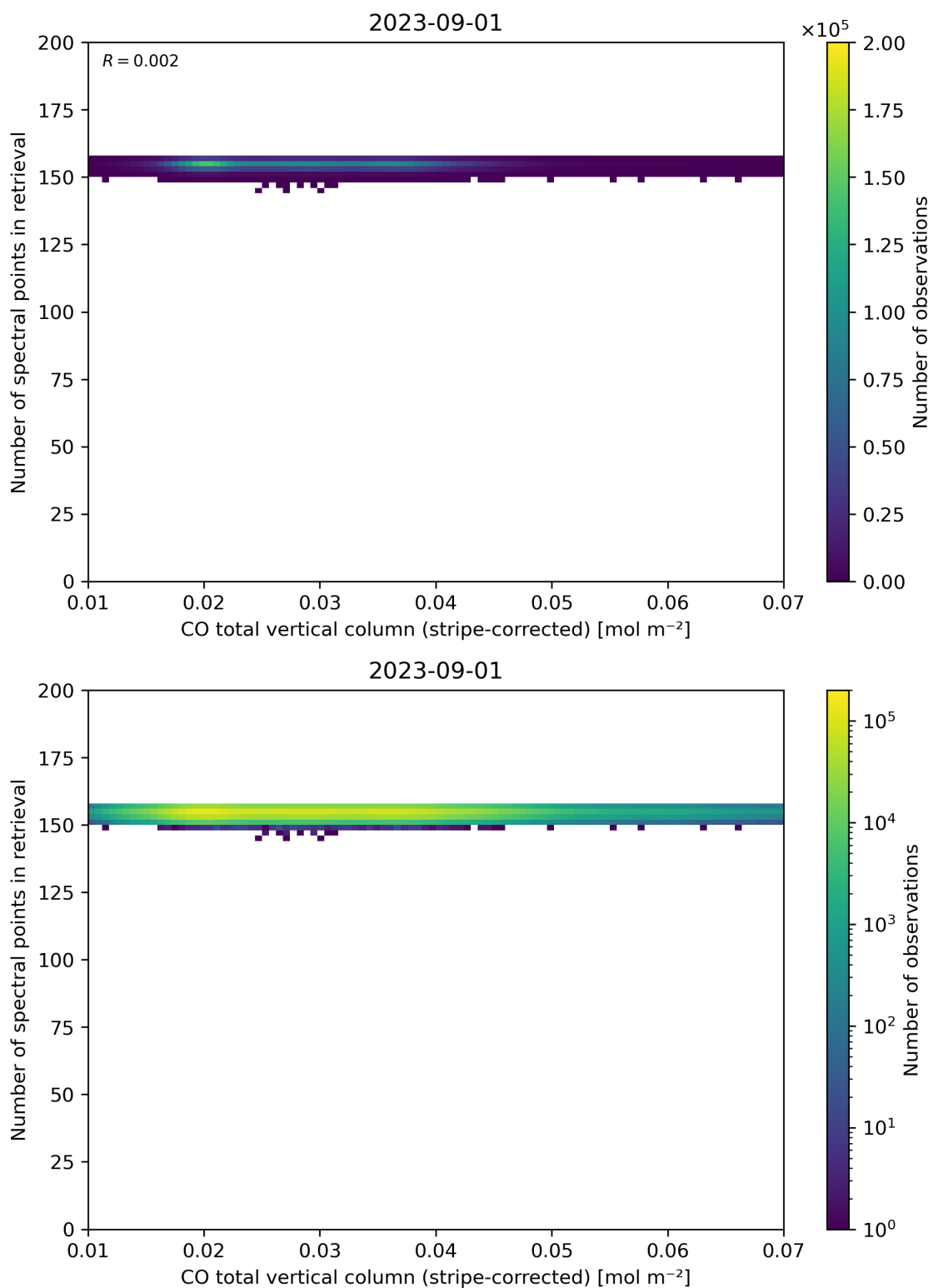
Figure 40: Scatter density plot of “CO total vertical column (stripe-corrected)” against “Number of spectral points in retrieval” for 2023-08-31 to 2023-09-02.
