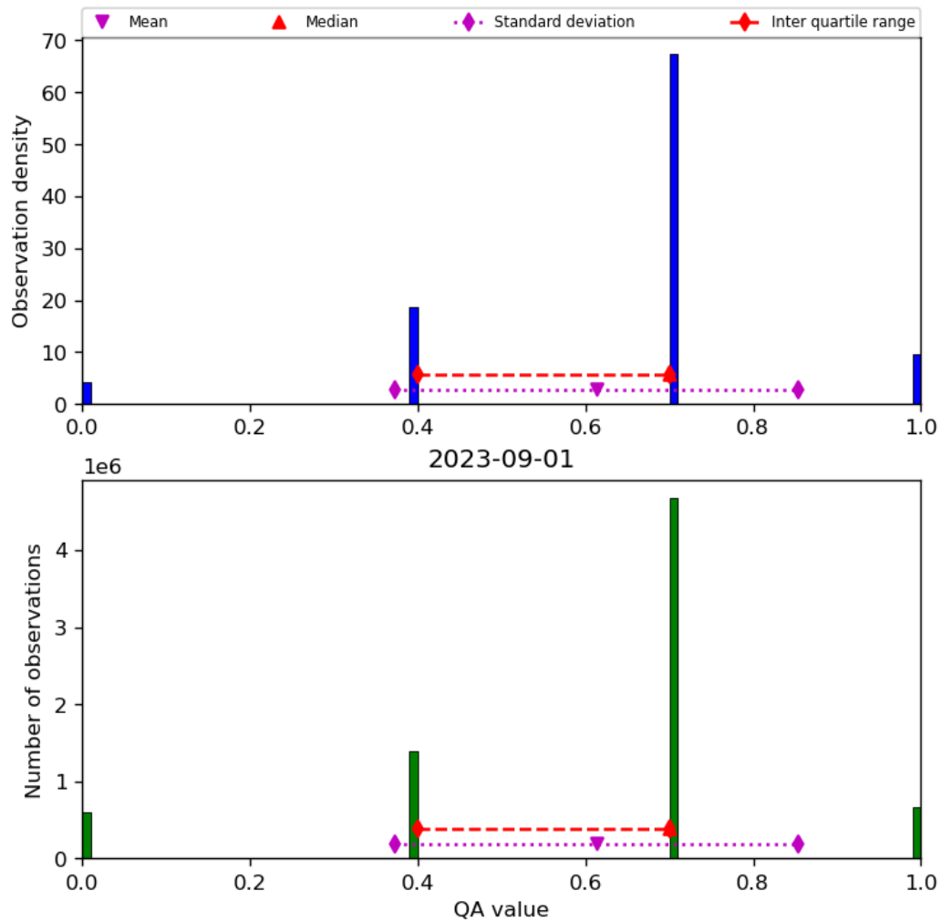
Figure 17: Histogram of “QA value” for 2023-08-31 to 2023-09-02
