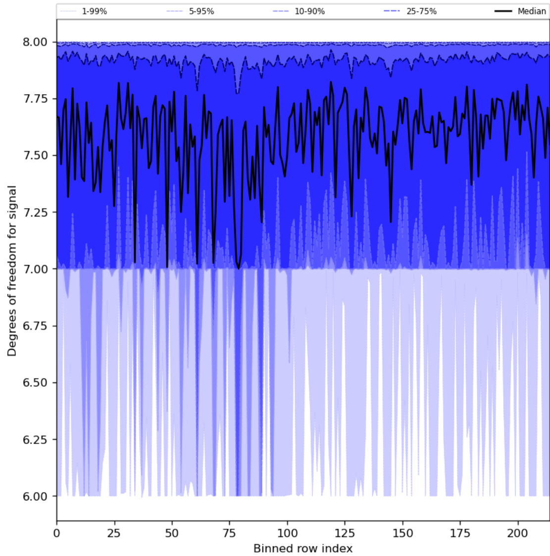
Figure 31: Along track statistics of “Degrees of freedom for signal” for 2023-08-31 to 2023-09-02
