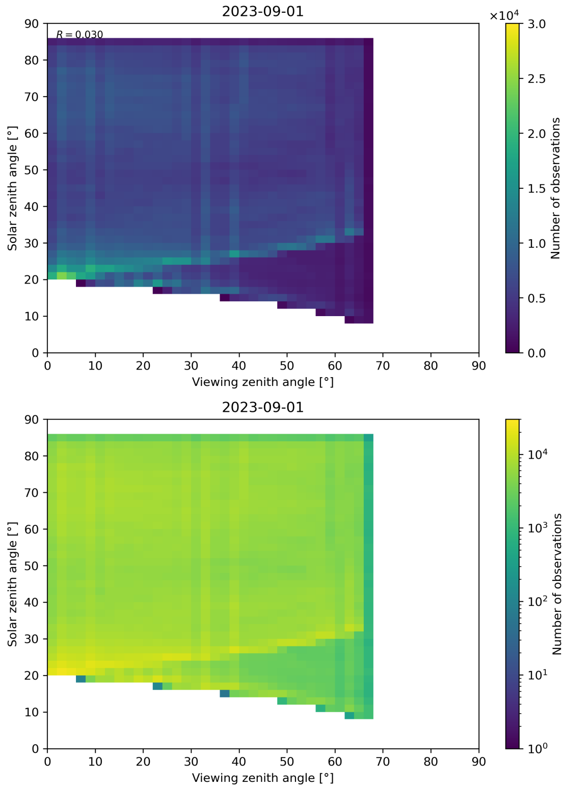
Figure 77: Scatter density plot of “Viewing zenith angle” against “Solar zenith angle” for 2023-08-31 to 2023-09-02.
