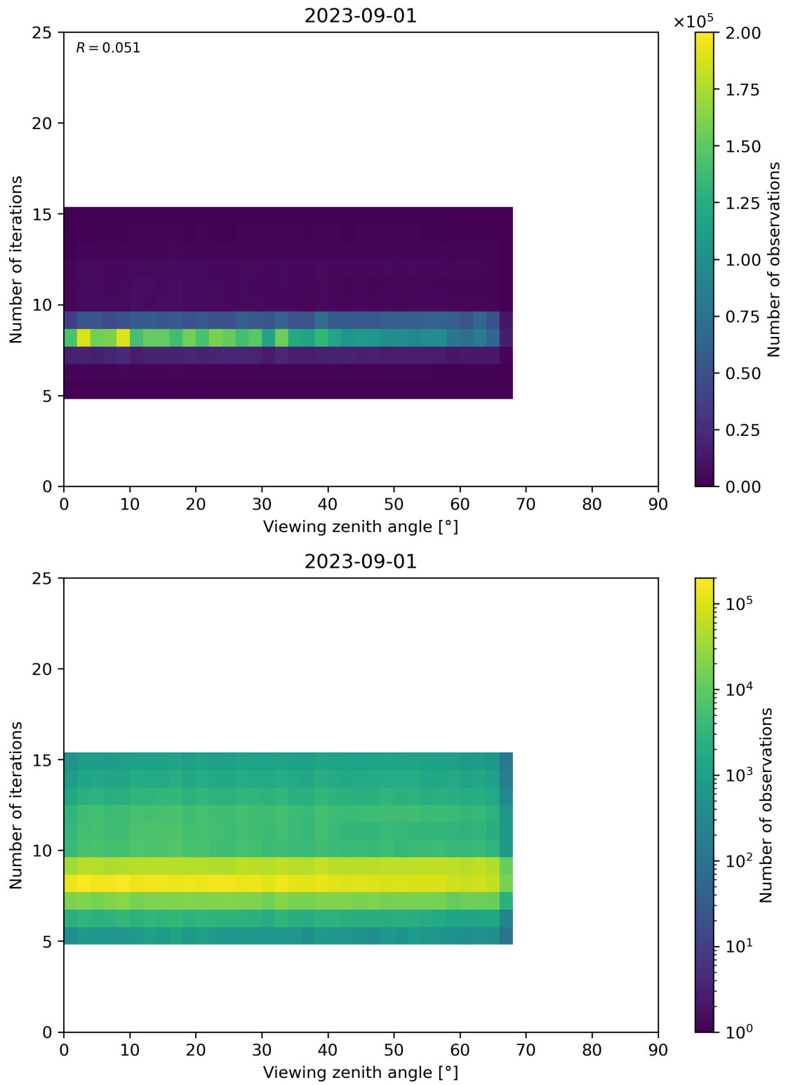
Figure 75: Scatter density plot of “Viewing zenith angle” against “Number of iterations” for 2023-08-31 to 2023-09-02.
