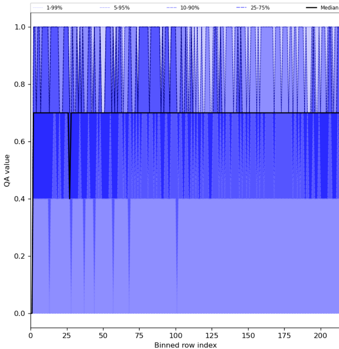
Figure 25: Along track statistics of “QA value” for 2023-08-31 to 2023-09-02
