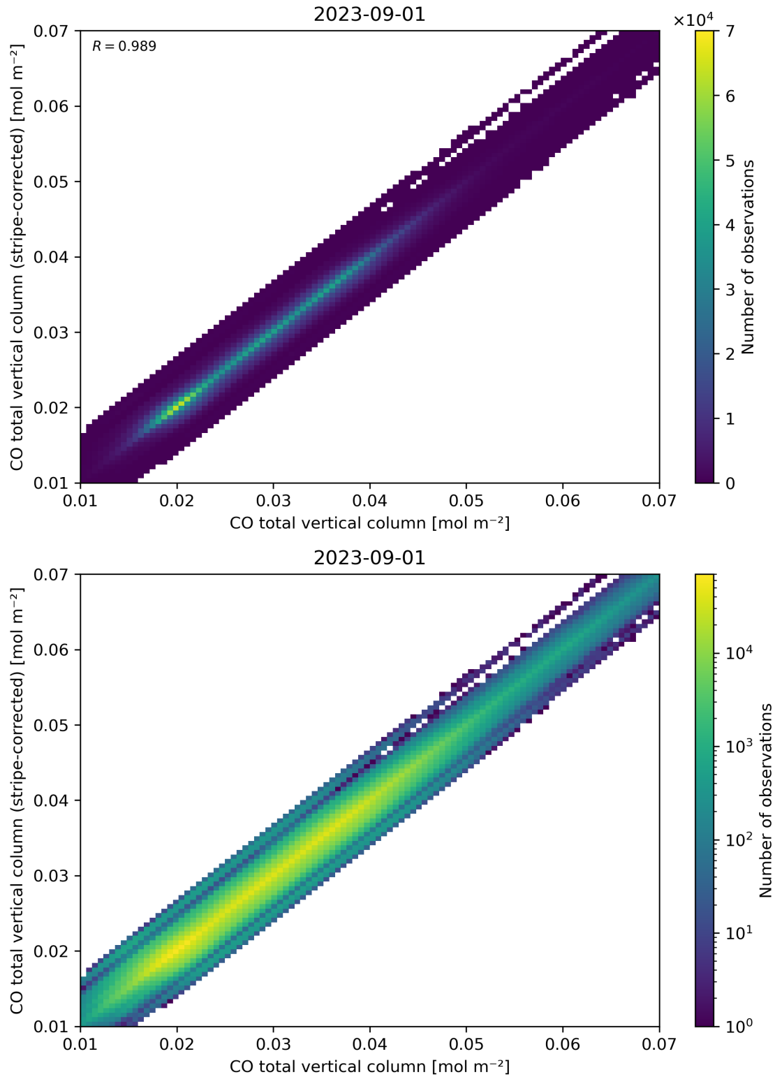
Figure 33: Scatter density plot of “CO total vertical column” against “CO total vertical column (stripe-corrected)” for 2023-08-31 to 2023-09-02.
