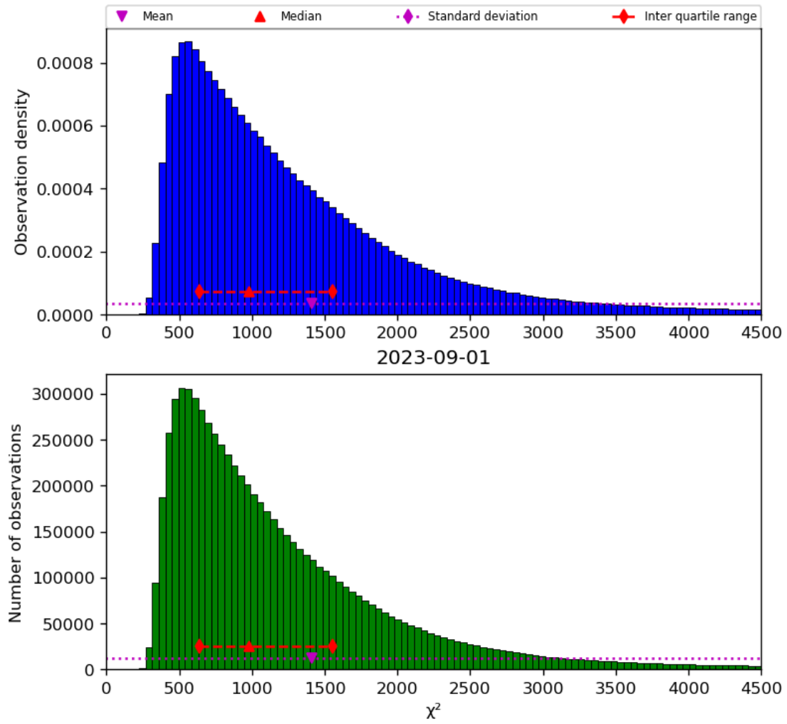
Figure 22: Histogram of " \chi^2 " for 2023-08-31 to 2023-09-02
