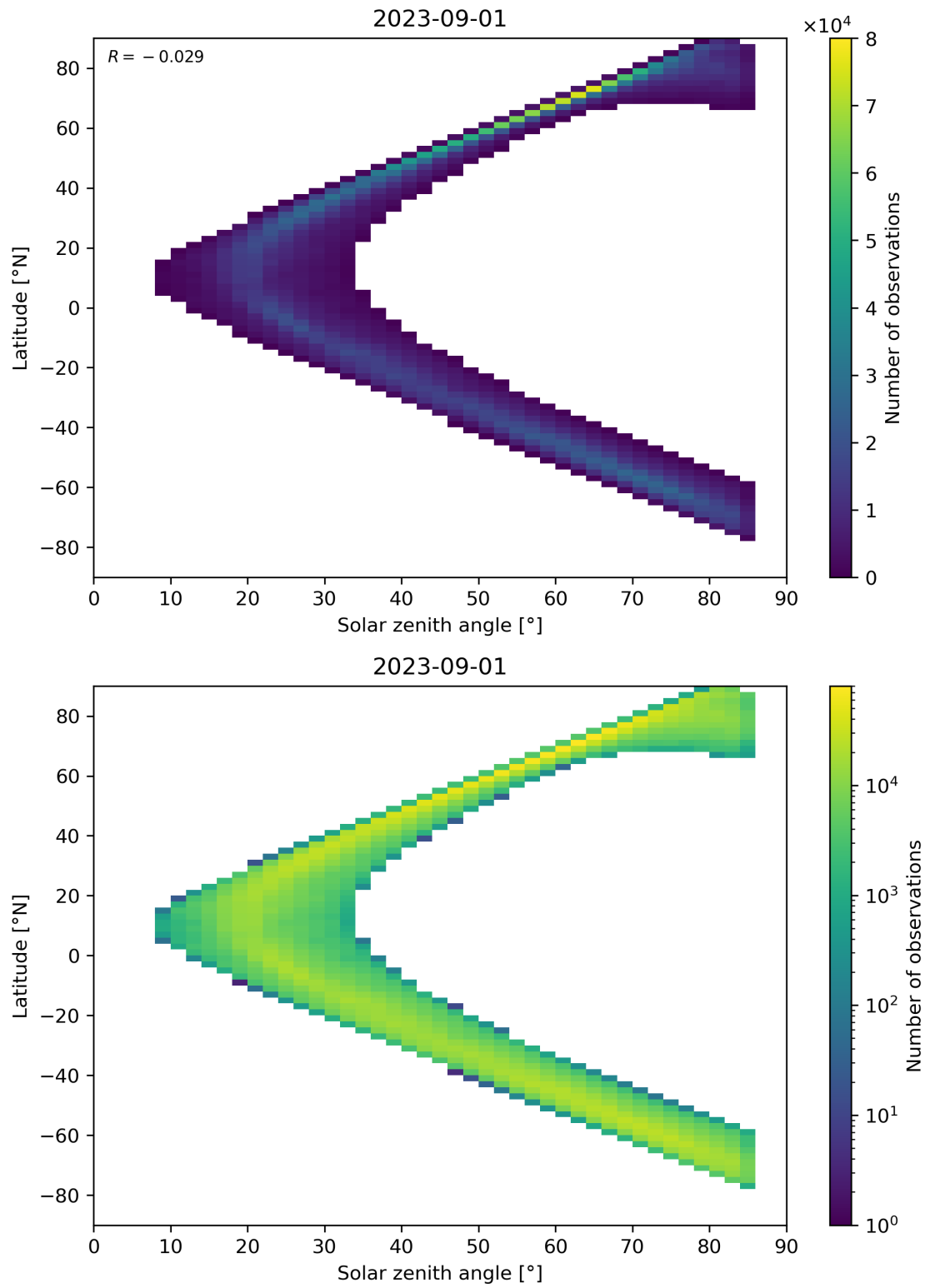
Figure 66: Scatter density plot of “Solar zenith angle” against “Latitude” for 2023-08-31 to 2023-09-02.
