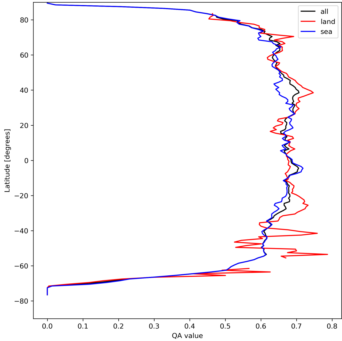
Figure 9: Zonal average of “QA value” for 2023-08-31 to 2023-09-02.
