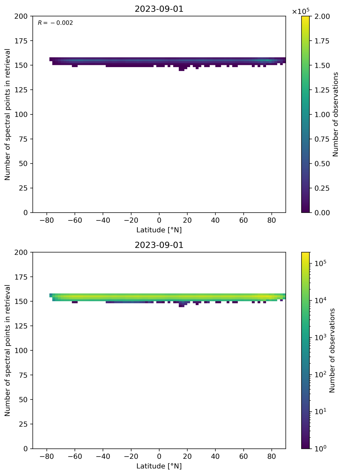
Figure 57: Scatter density plot of “Latitude” against “Number of spectral points in retrieval” for 2023-08-31 to 2023-09-02.
