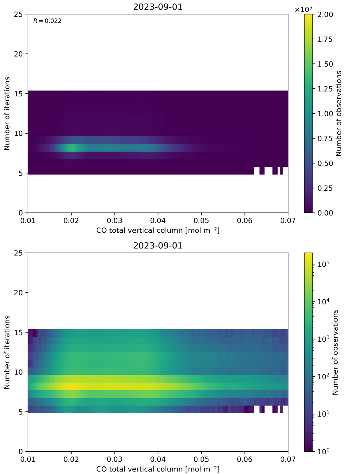
Figure 42: Scatter density plot of “CO total vertical column” against “Number of iterations” for 2023-08-31 to 2023-09-02.
