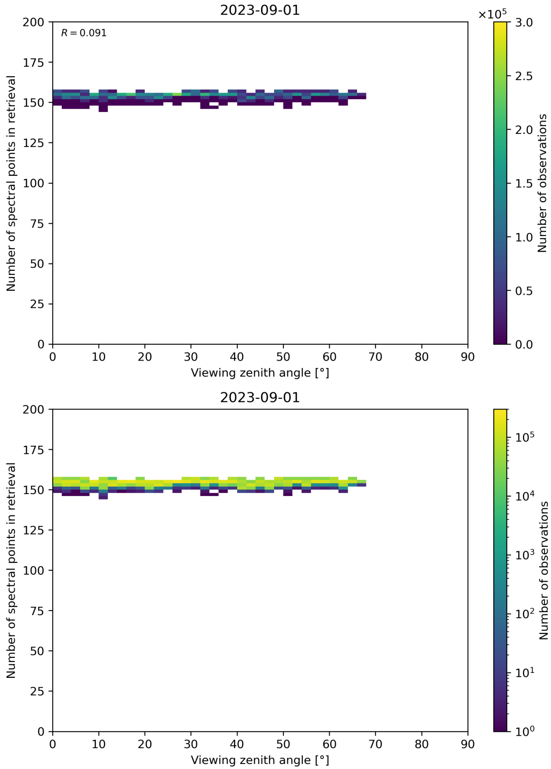
Figure 76: Scatter density plot of “Viewing zenith angle” against “Number of spectral points in retrieval” for 2023-08-31 to 2023-09-02.
