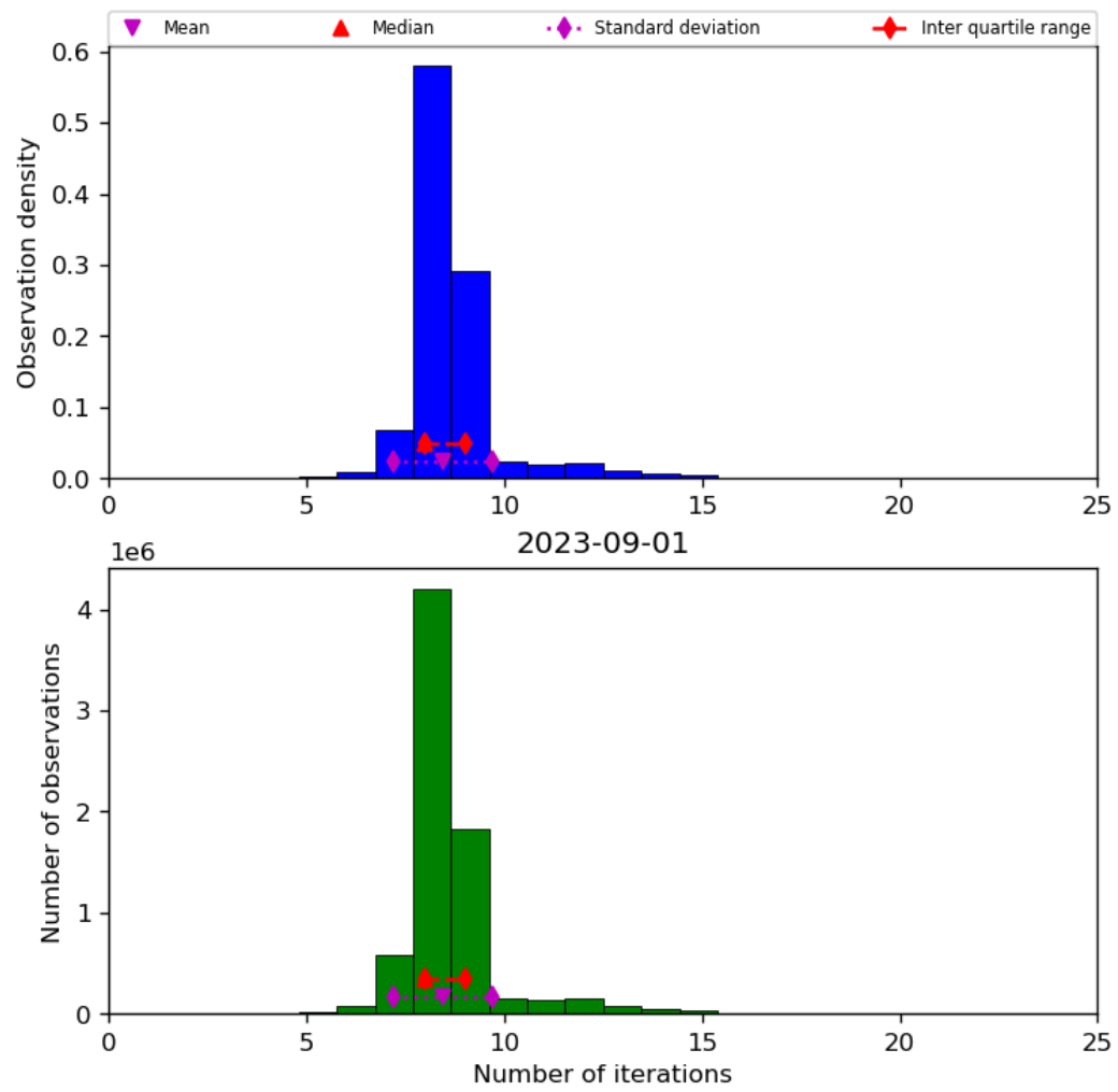
Figure 24: Histogram of “Number of iterations” for 2023-08-31 to 2023-09-02
