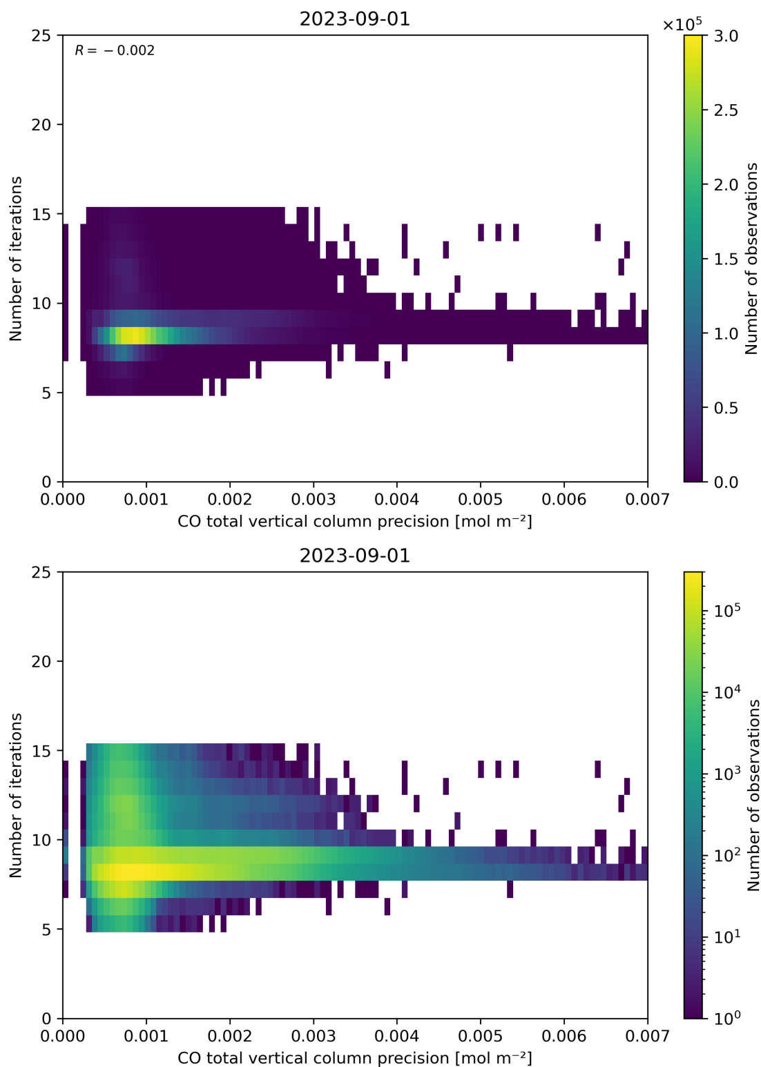
Figure 46: Scatter density plot of “CO total vertical column precision” against “Number of iterations” for 2023-08-31 to 2023-09-02.
