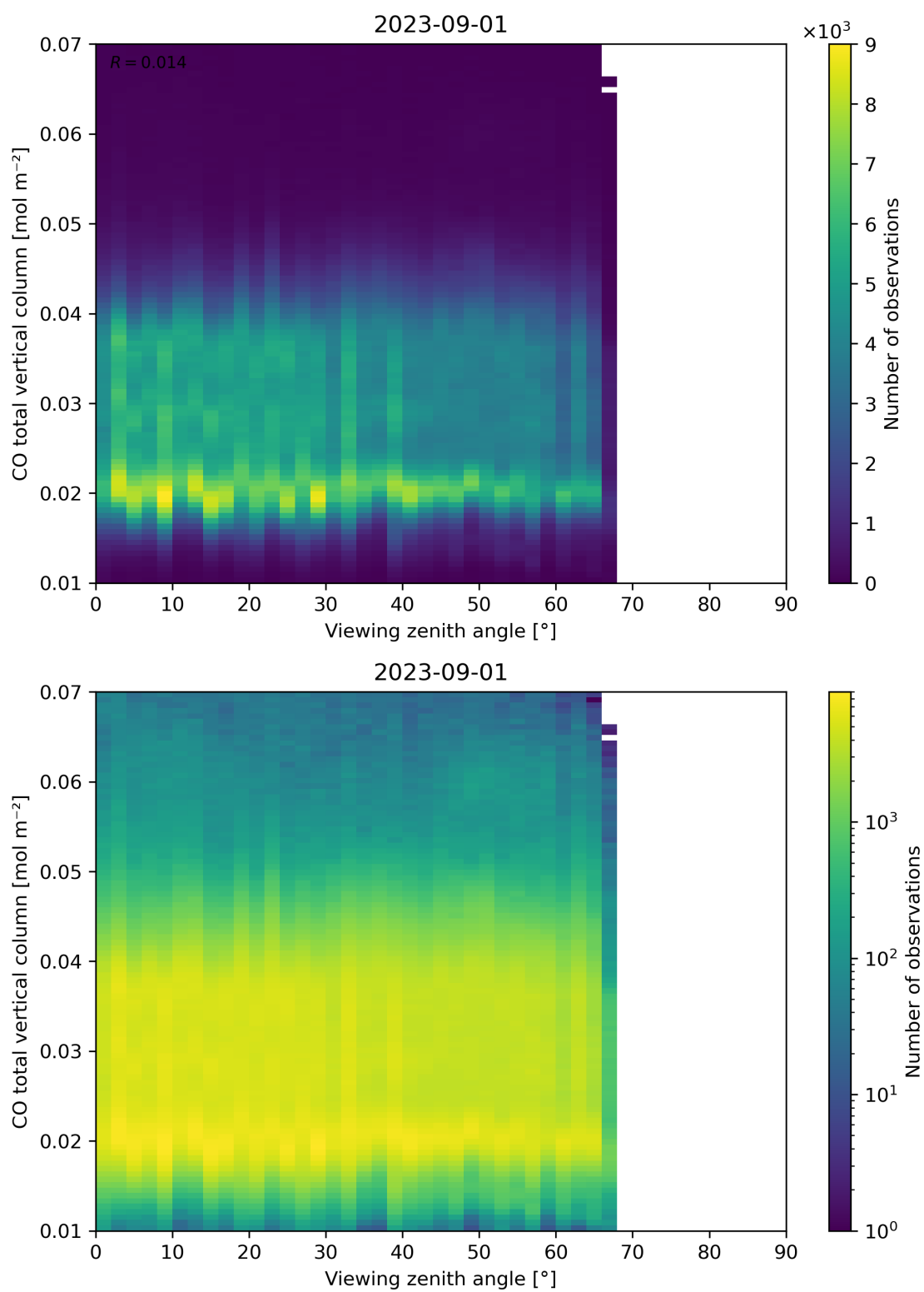
Figure 69: Scatter density plot of “Viewing zenith angle” against “CO total vertical column” for 2023-08-31 to 2023-09-02.
