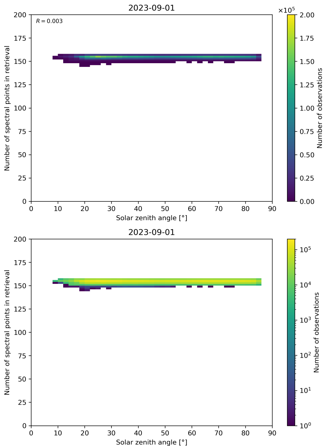
Figure 68: Scatter density plot of “Solar zenith angle” against “Number of spectral points in retrieval” for 2023-08-31 to 2023-09-02.
