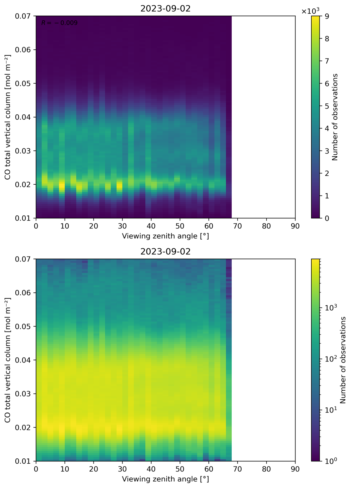
Figure 69: Scatter density plot of “Viewing zenith angle” against “CO total vertical column” for 2023-09-01 to 2023-09-03.
