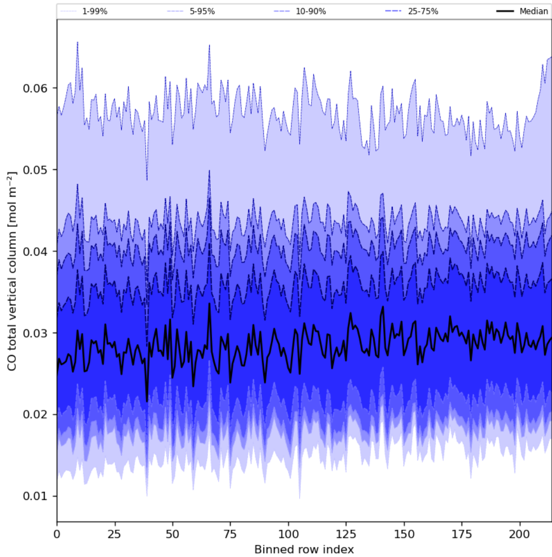
Figure 26: Along track statistics of “CO total vertical column” for 2023-09-01 to 2023-09-03
