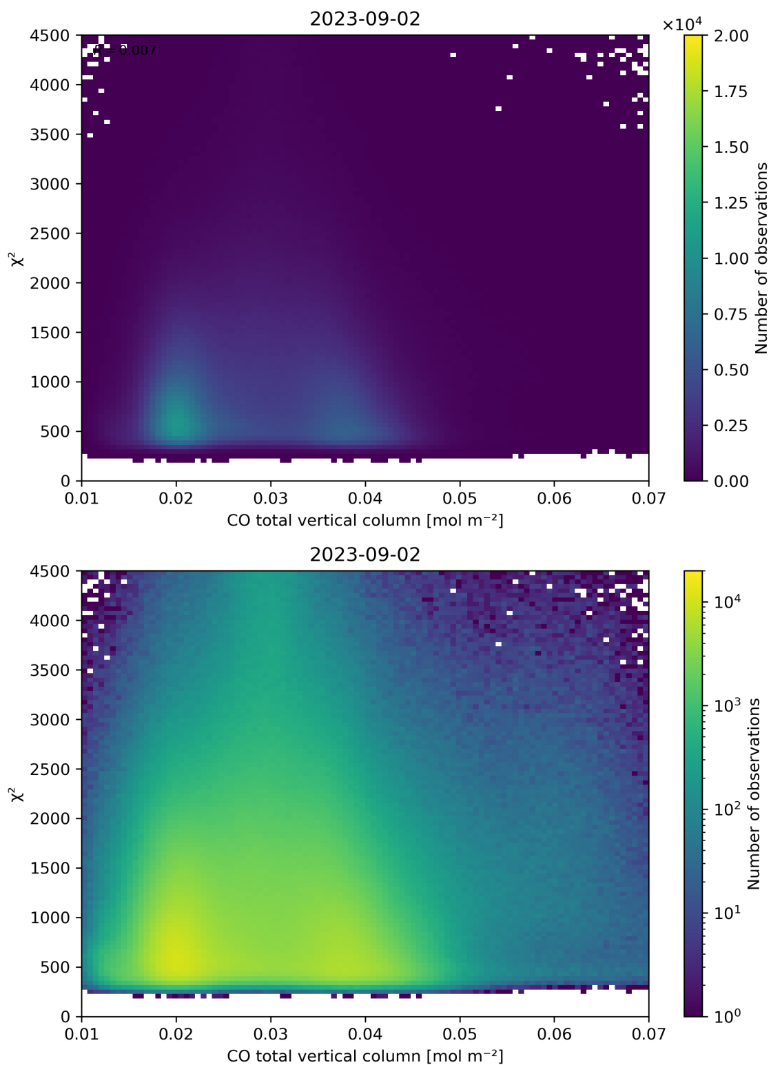
Figure 35: Scatter density plot of “CO total vertical column” against “ \chi^2 ” for 2023-09-01 to 2023-09-03.
