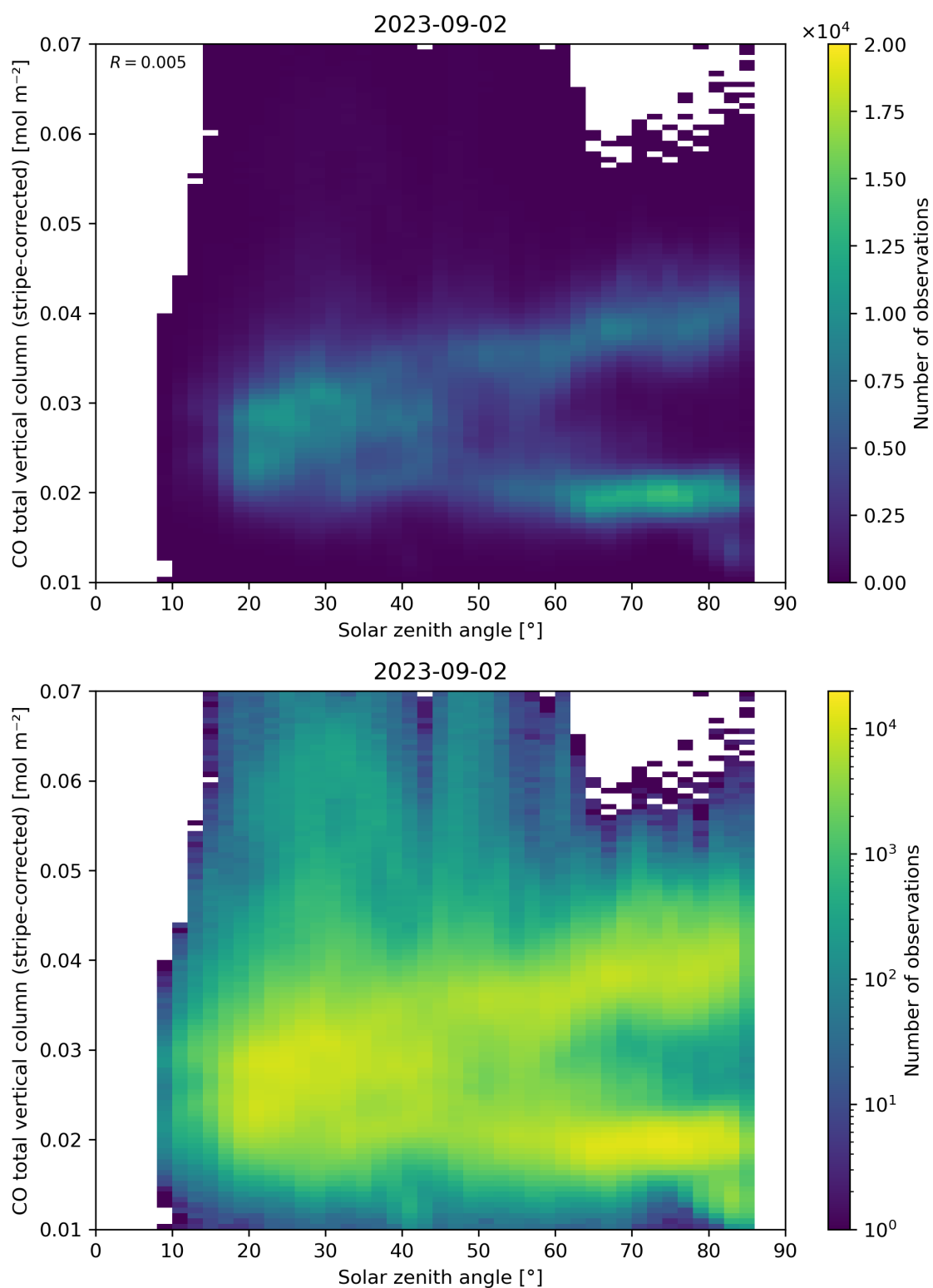
Figure 62: Scatter density plot of “Solar zenith angle” against “CO total vertical column (stripe-corrected)” for 2023-09-01 to 2023-09-03.
