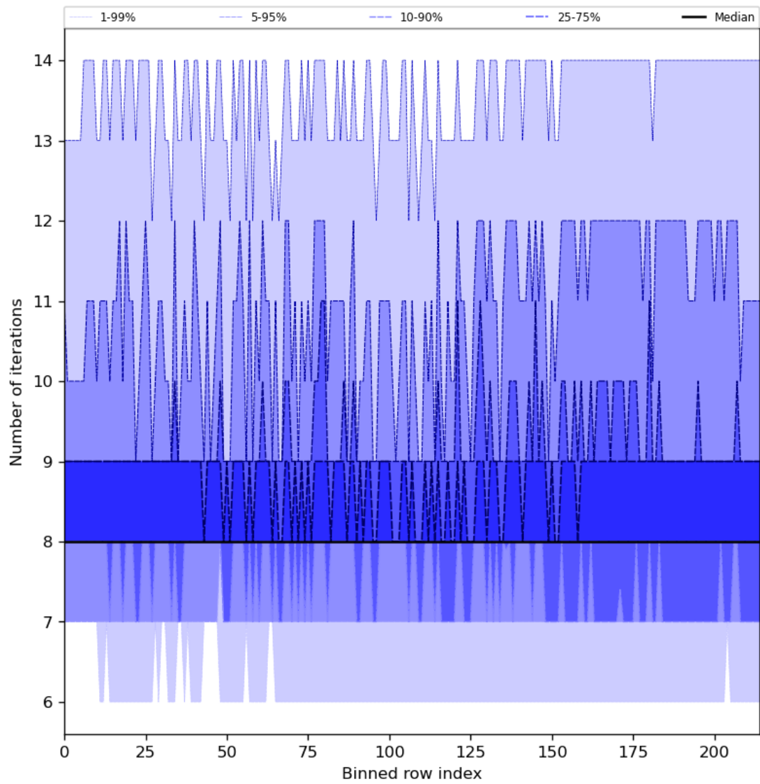
Figure 32: Along track statistics of “Number of iterations” for 2023-09-01 to 2023-09-03
