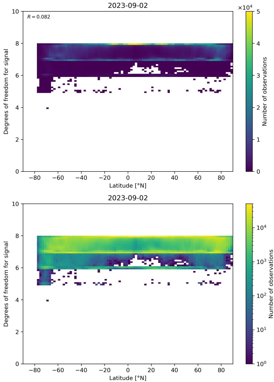
Figure 55: Scatter density plot of “Latitude” against “Degrees of freedom for signal” for 2023-09-01 to 2023-09-03.
