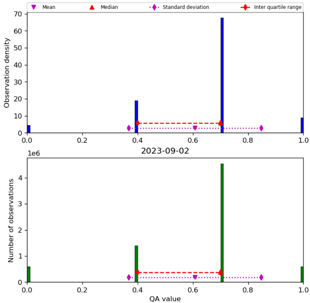
Figure 17: Histogram of “QA value” for 2023-09-01 to 2023-09-03
