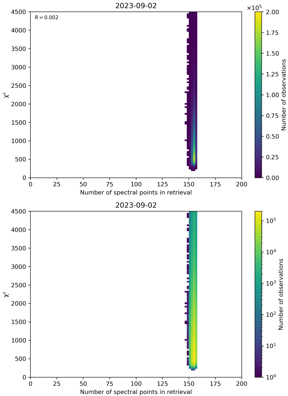
Figure 58: Scatter density plot of “Number of spectral points in retrieval” against “ \chi^2 ” for 2023-09-01 to 2023-09-03.
