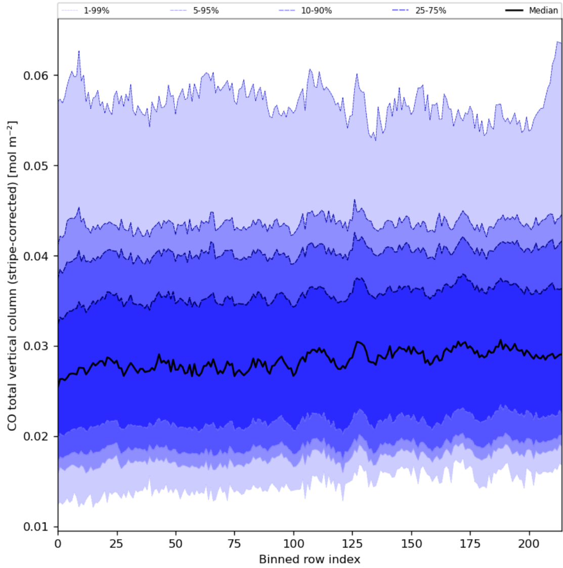
Figure 27: Along track statistics of “CO total vertical column (stripe-corrected)” for 2023-09-01 to 2023-09-03
