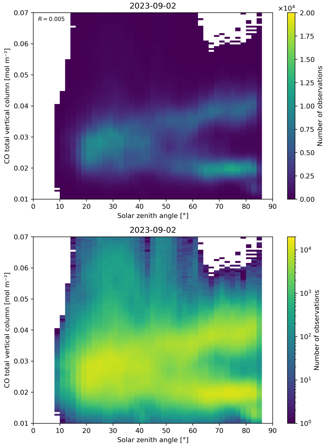
Figure 61: Scatter density plot of “Solar zenith angle” against “CO total vertical column” for 2023-09-01 to 2023-09-03.
