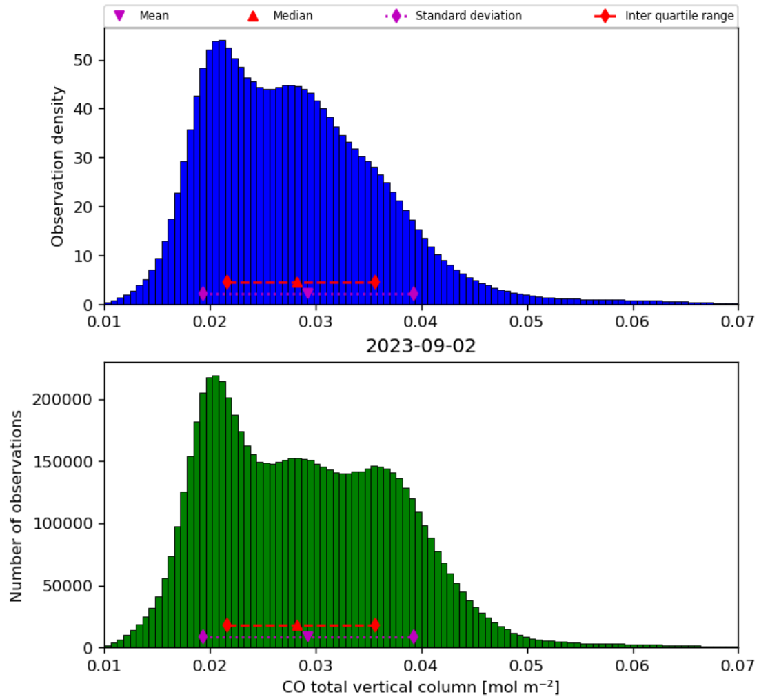
Figure 18: Histogram of “CO total vertical column” for 2023-09-01 to 2023-09-03
