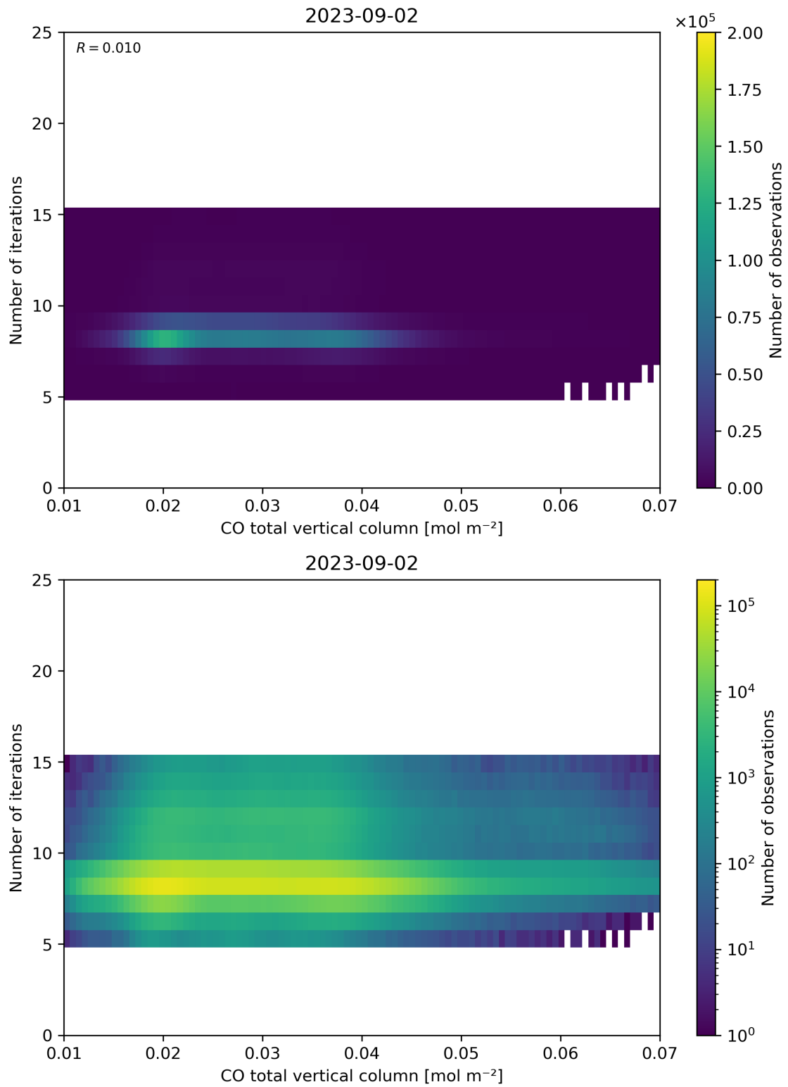
Figure 42: Scatter density plot of “CO total vertical column” against “Number of iterations” for 2023-09-01 to 2023-09-03.
