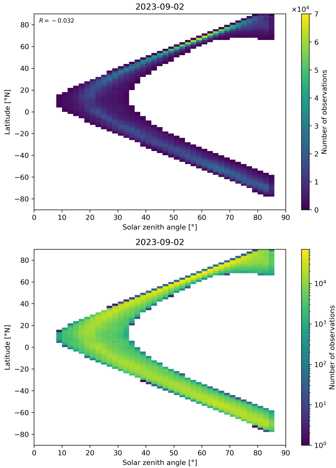
Figure 66: Scatter density plot of “Solar zenith angle” against “Latitude” for 2023-09-01 to 2023-09-03.
