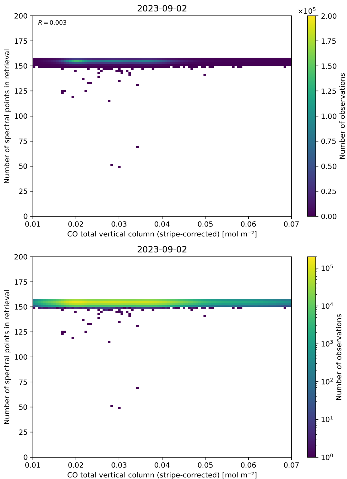
Figure 40: Scatter density plot of “CO total vertical column (stripe-corrected)” against “Number of spectral points in retrieval” for 2023-09-01 to 2023-09-03.
