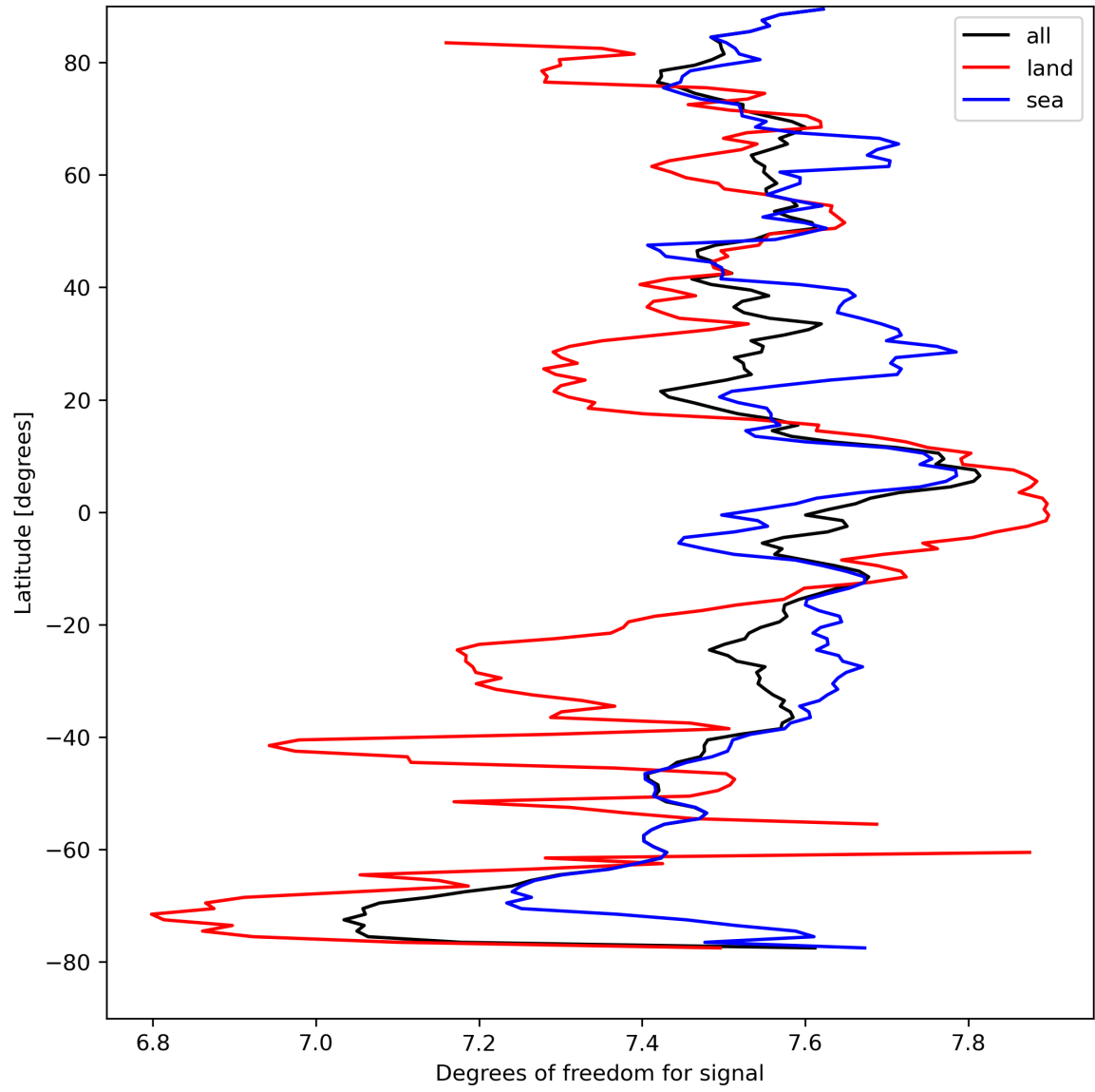
Figure 15: Zonal average of “Degrees of freedom for signal” for 2023-09-01 to 2023-09-03.
