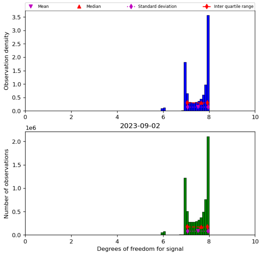
Figure 23: Histogram of “Degrees of freedom for signal” for 2023-09-01 to 2023-09-03
