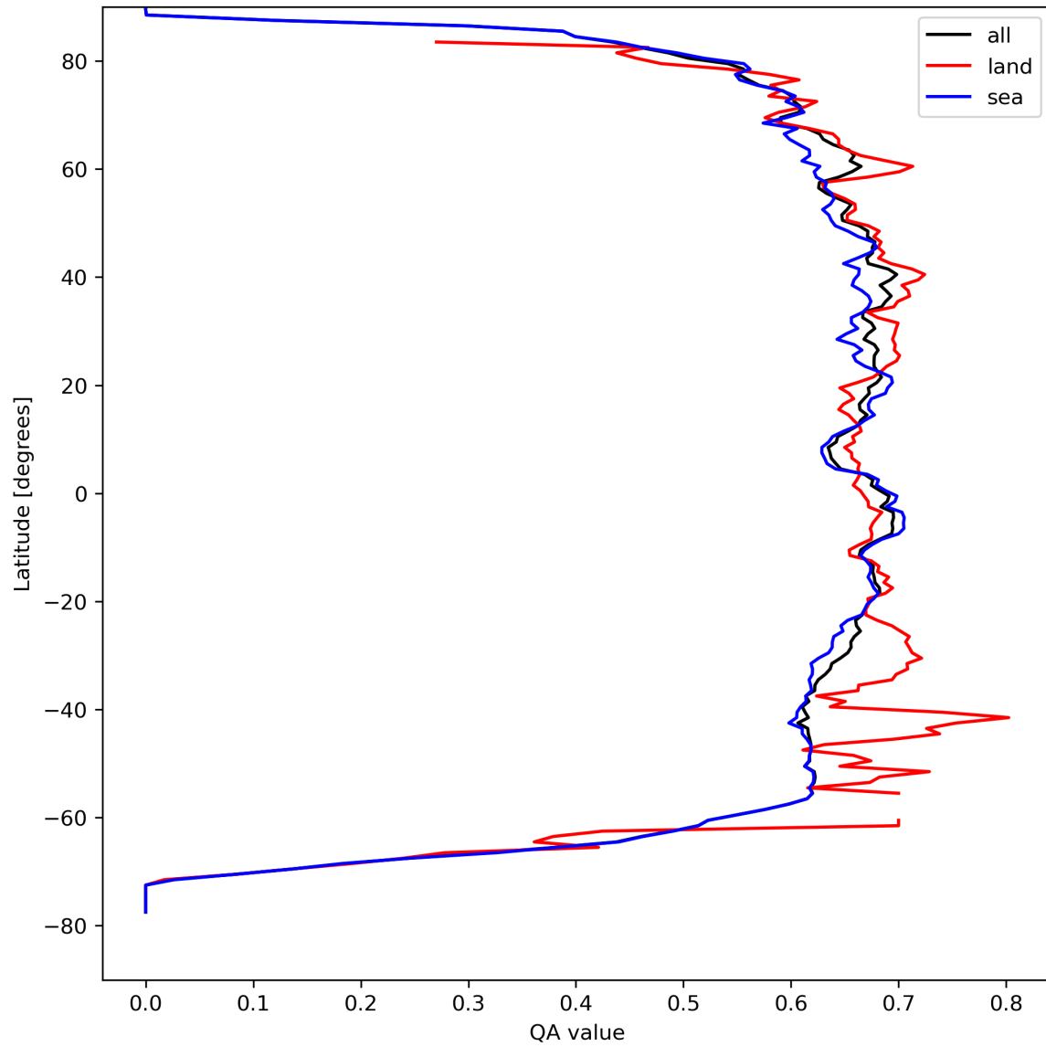
Figure 9: Zonal average of “QA value” for 2023-09-01 to 2023-09-03.
