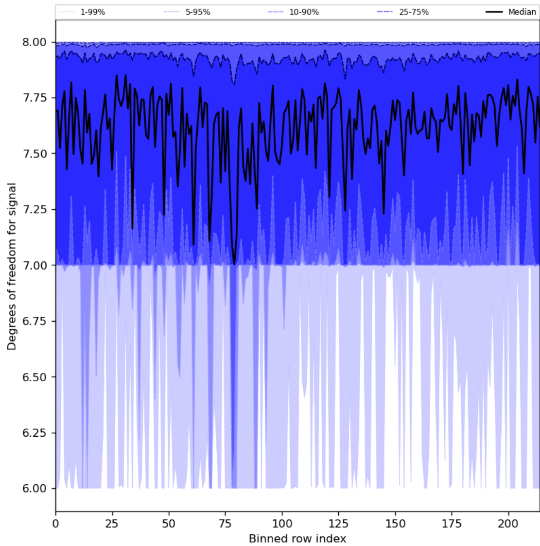
Figure 31: Along track statistics of “Degrees of freedom for signal” for 2023-09-01 to 2023-09-03
