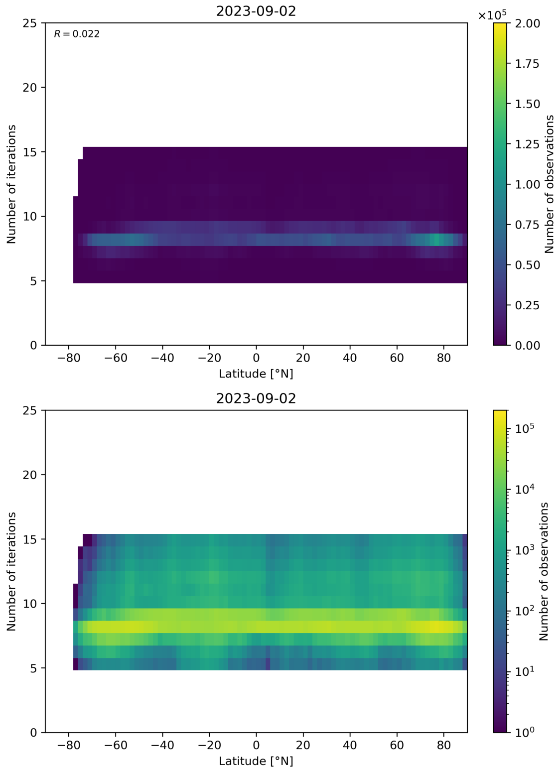
Figure 56: Scatter density plot of “Latitude” against “Number of iterations” for 2023-09-01 to 2023-09-03.
