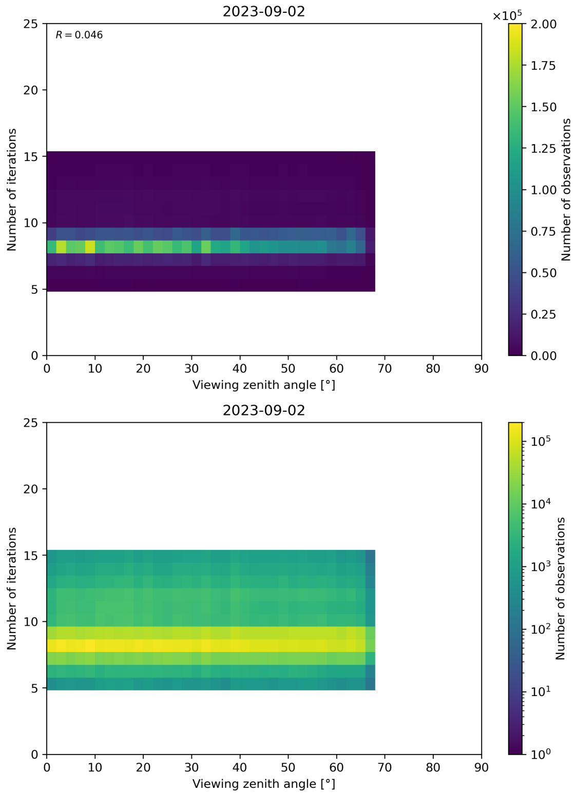
Figure 75: Scatter density plot of “Viewing zenith angle” against “Number of iterations” for 2023-09-01 to 2023-09-03.
