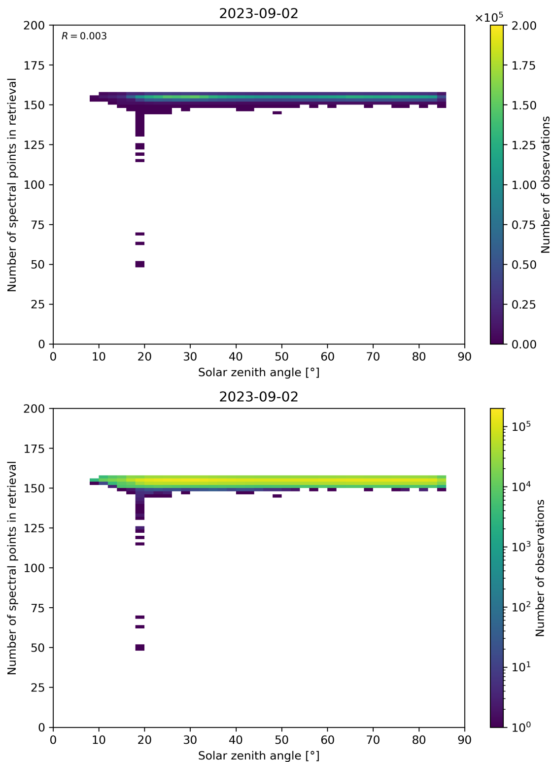
Figure 68: Scatter density plot of “Solar zenith angle” against “Number of spectral points in retrieval” for 2023-09-01 to 2023-09-03.
