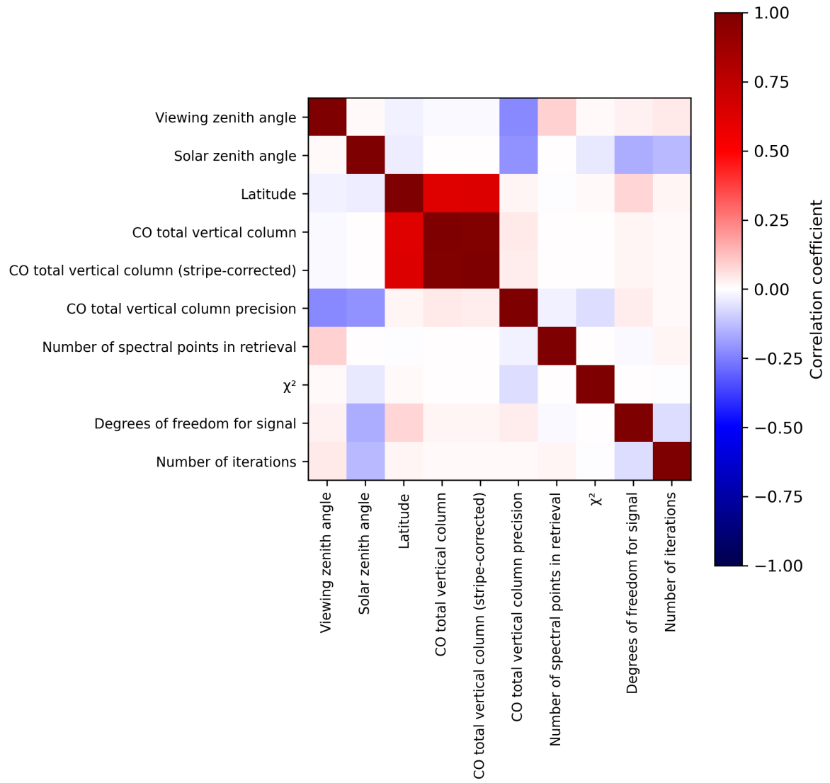
Figure 2: Map of correlation matrix for 2023-09-01 to 2023-09-03.
