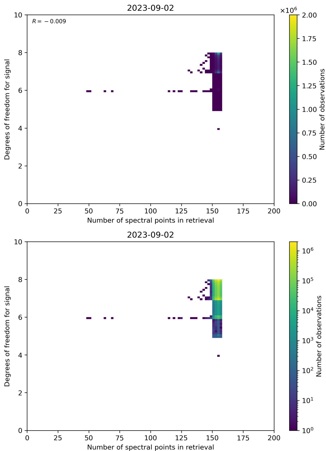
Figure 59: Scatter density plot of “Number of spectral points in retrieval” against “Degrees of freedom for signal” for 2023-09-01 to 2023-09-03.
