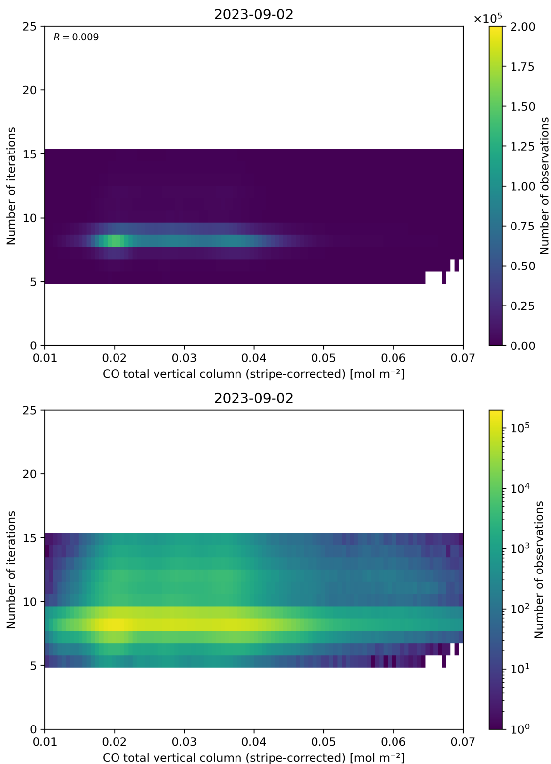
Figure 39: Scatter density plot of “CO total vertical column (stripe-corrected)” against “Number of iterations” for 2023-09-01 to 2023-09-03.
