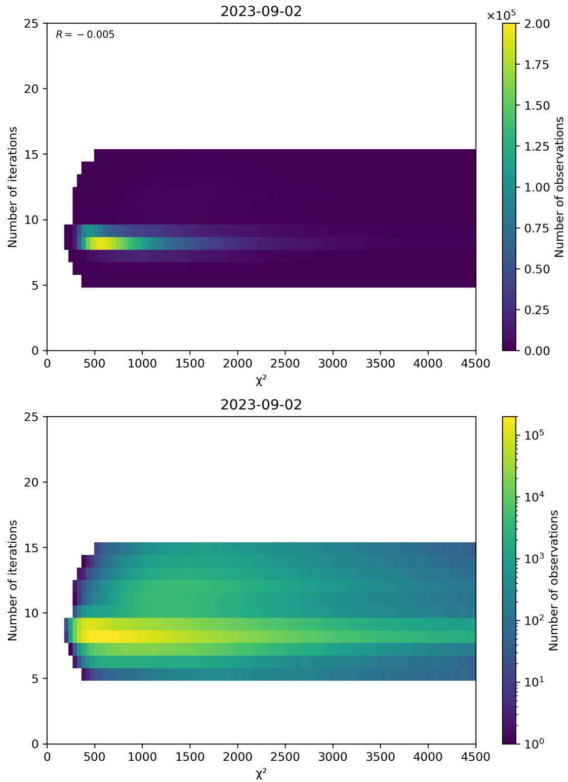
Figure 49: Scatter density plot of “ \chi^2 ” against “Number of iterations” for 2023-09-01 to 2023-09-03.
