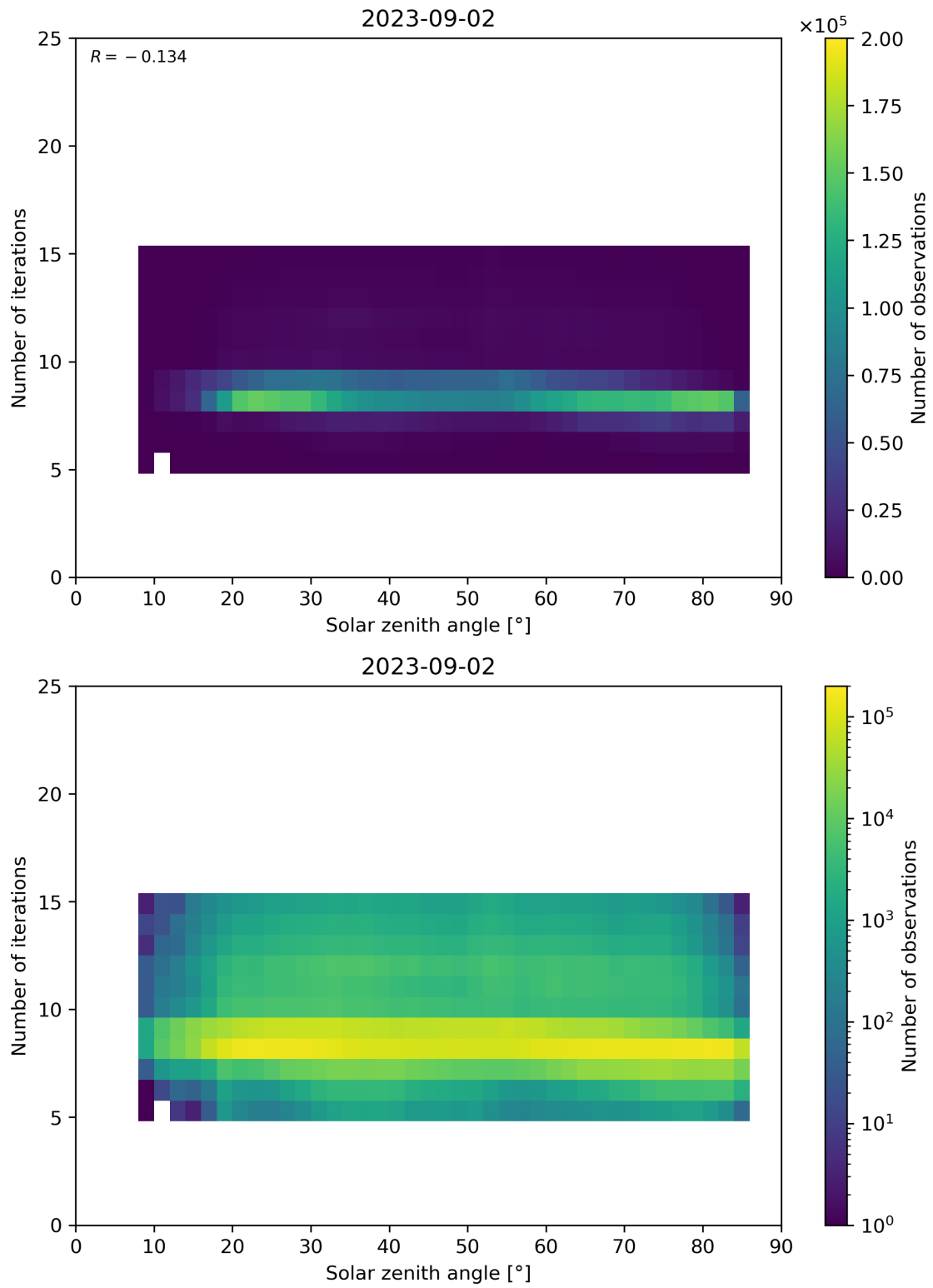
Figure 67: Scatter density plot of “Solar zenith angle” against “Number of iterations” for 2023-09-01 to 2023-09-03.
