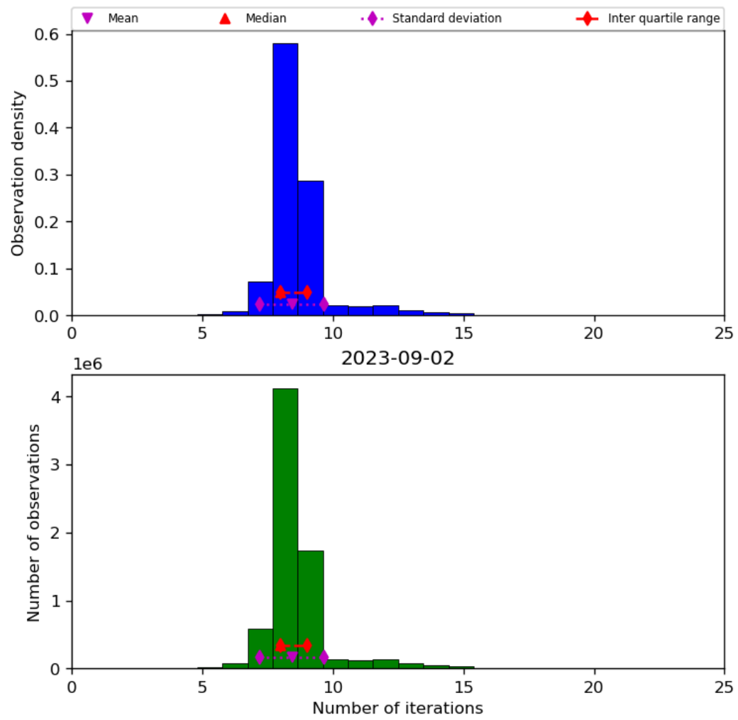
Figure 24: Histogram of “Number of iterations” for 2023-09-01 to 2023-09-03
