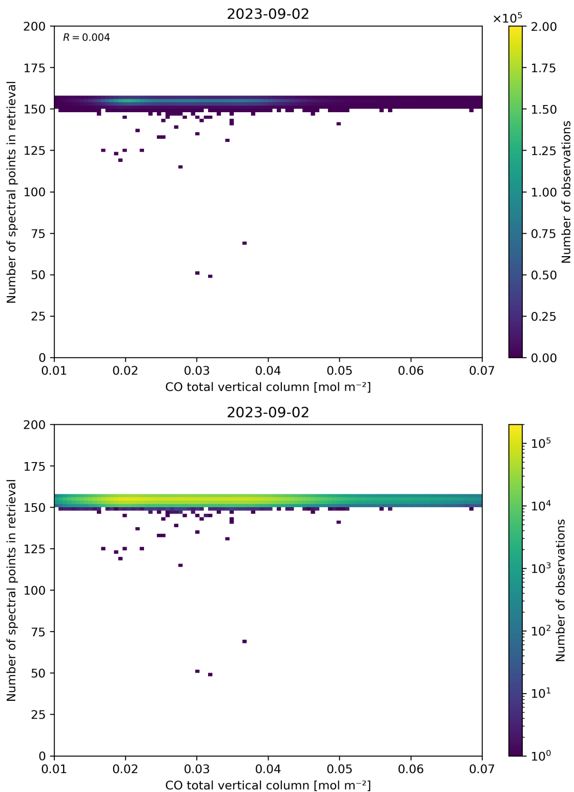
Figure 43: Scatter density plot of “CO total vertical column” against “Number of spectral points in retrieval” for 2023-09-01 to 2023-09-03.
