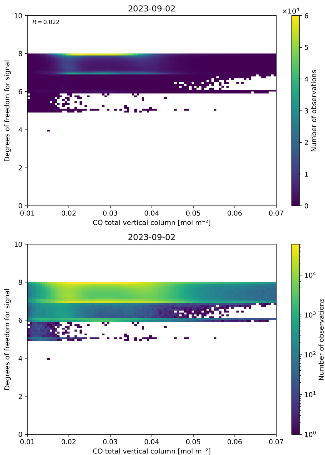
Figure 41: Scatter density plot of “CO total vertical column” against “Degrees of freedom for signal” for 2023-09-01 to 2023-09-03.
