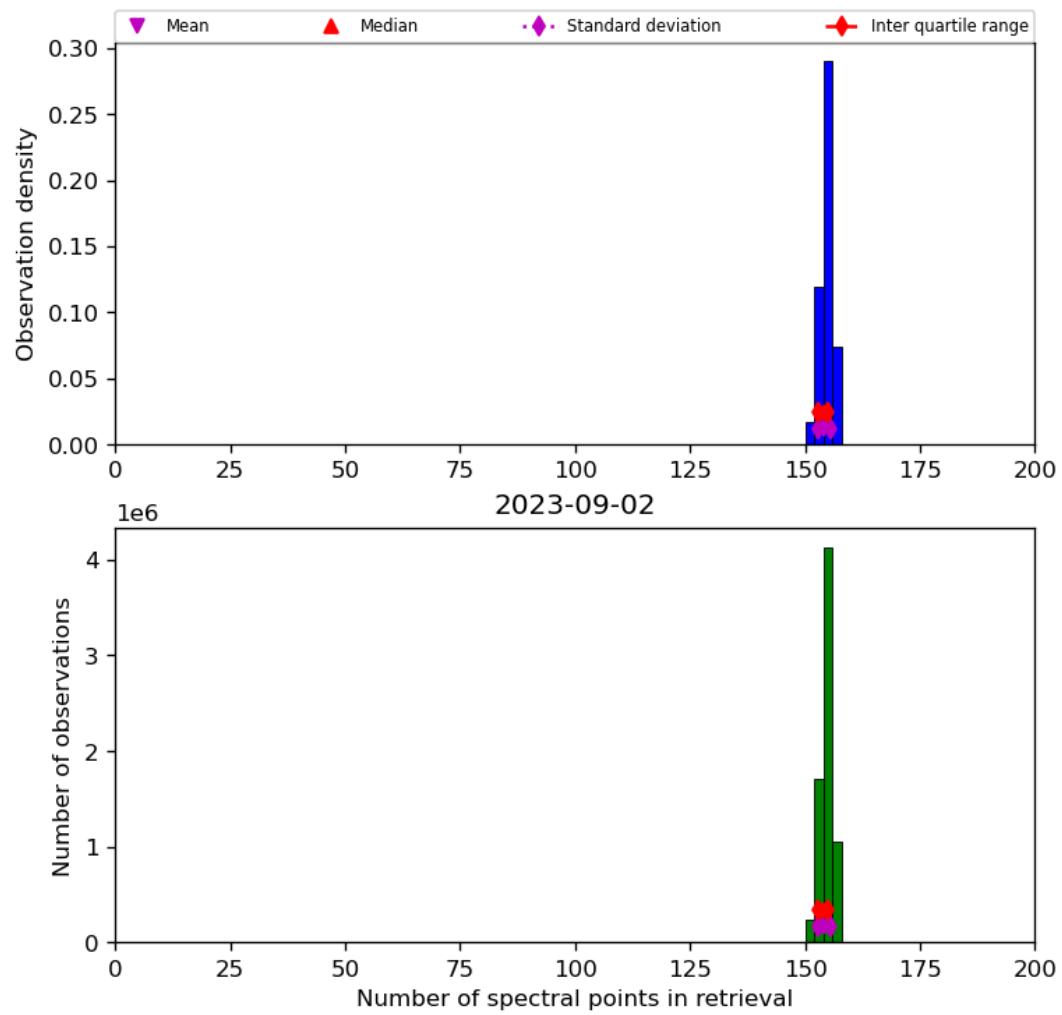
Figure 21: Histogram of “Number of spectral points in retrieval” for 2023-09-01 to 2023-09-03
