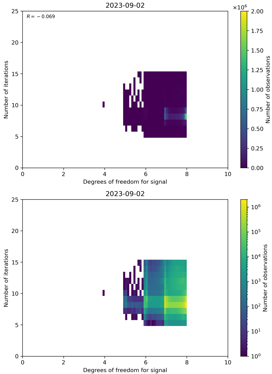
Figure 50: Scatter density plot of “Degrees of freedom for signal” against “Number of iterations” for 2023-09-01 to 2023-09-03.
