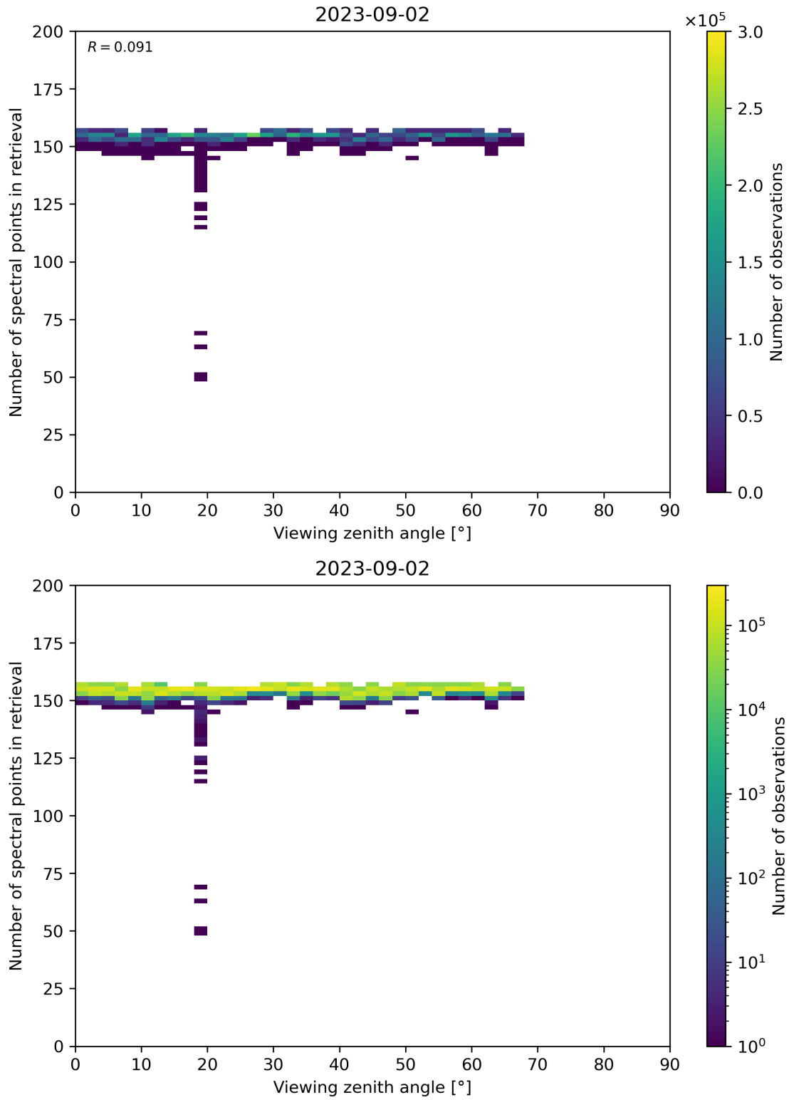
Figure 76: Scatter density plot of “Viewing zenith angle” against “Number of spectral points in retrieval” for 2023-09-01 to 2023-09-03.
