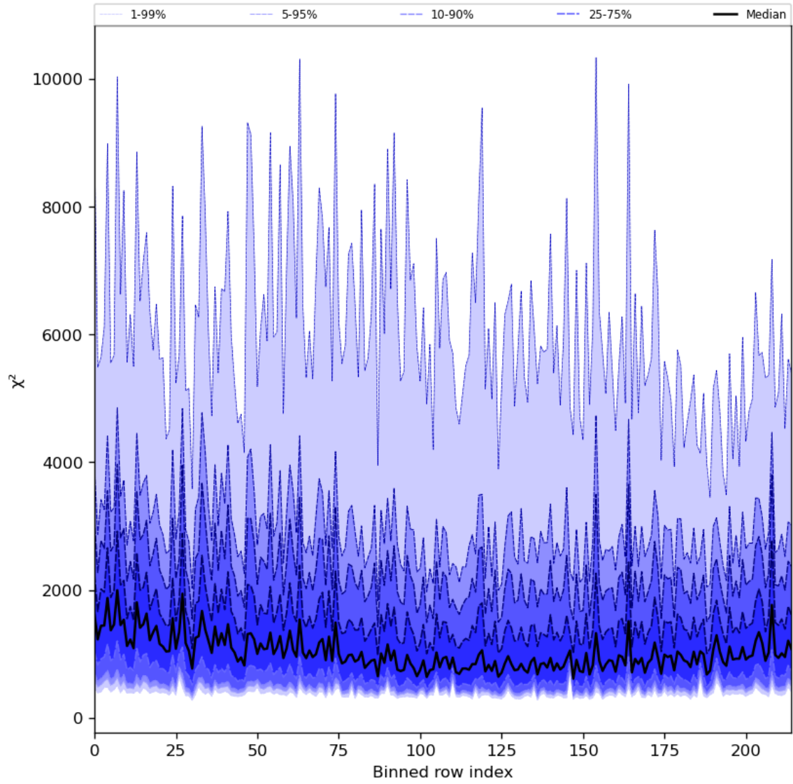
Figure 30: Along track statistics of “ \chi^2 ” for 2023-09-01 to 2023-09-03
