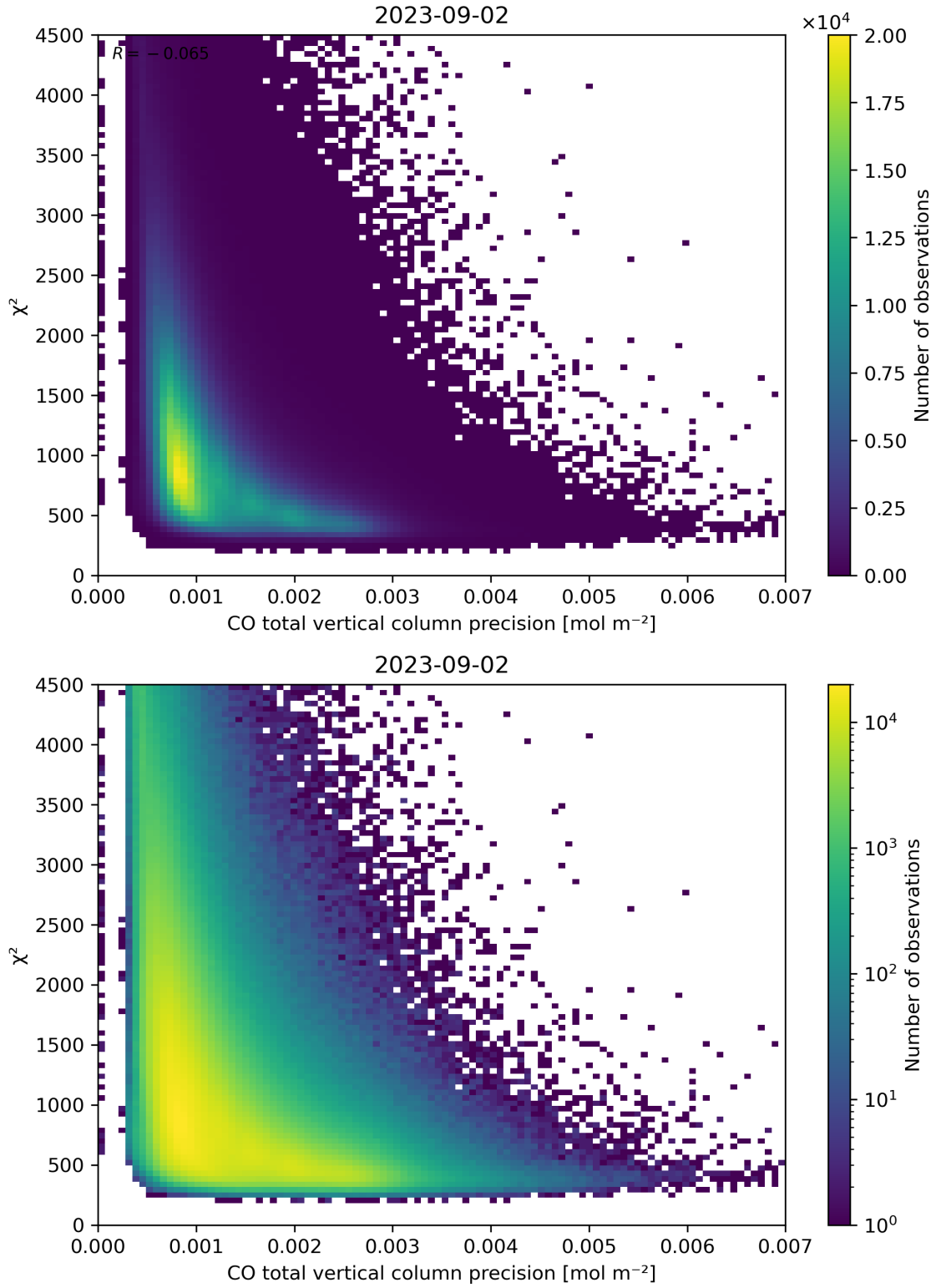
Figure 44: Scatter density plot of “CO total vertical column precision” against “ \chi^2 ” for 2023-09-01 to 2023-09-03.
