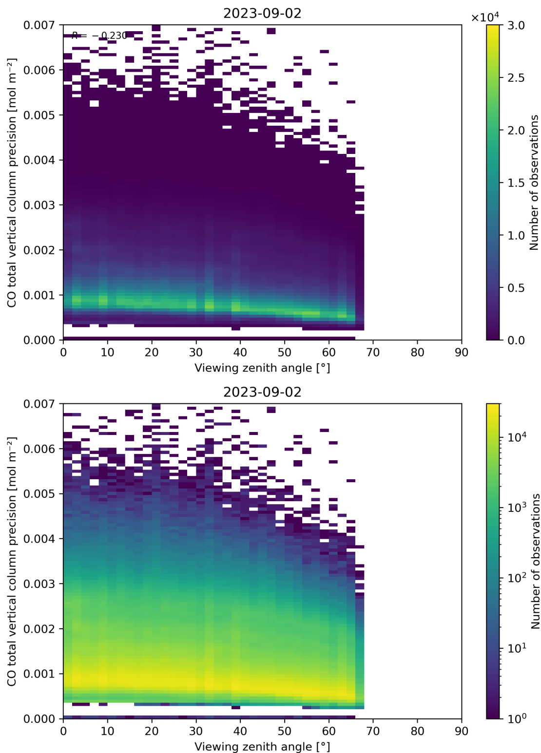
Figure 71: Scatter density plot of “Viewing zenith angle” against “CO total vertical column precision” for 2023-09-01 to 2023-09-03.
