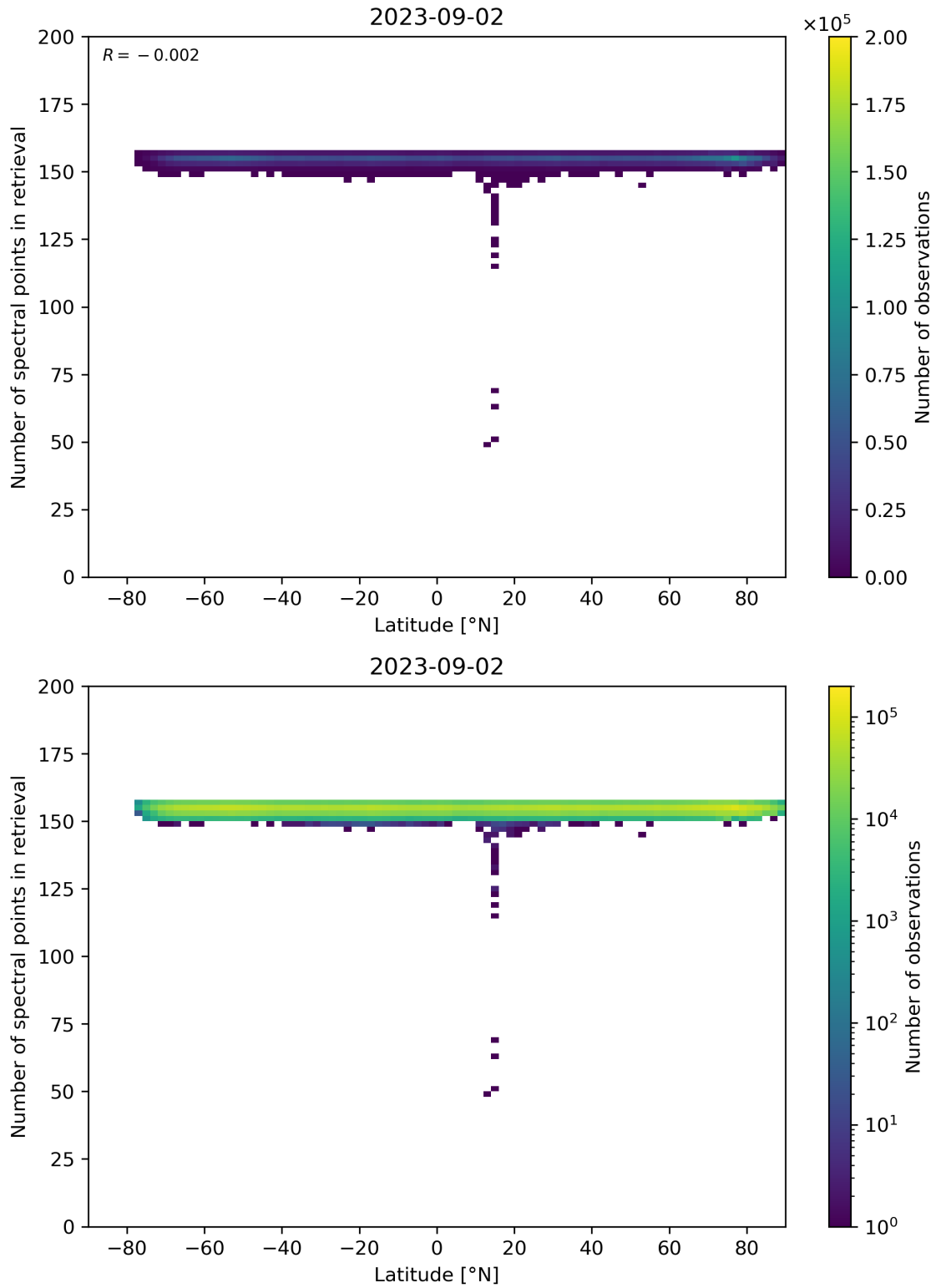
Figure 57: Scatter density plot of “Latitude” against “Number of spectral points in retrieval” for 2023-09-01 to 2023-09-03.
