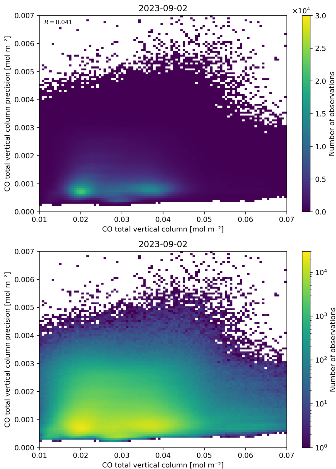
Figure 34: Scatter density plot of “CO total vertical column” against “CO total vertical column precision” for 2023-09-01 to 2023-09-03.
