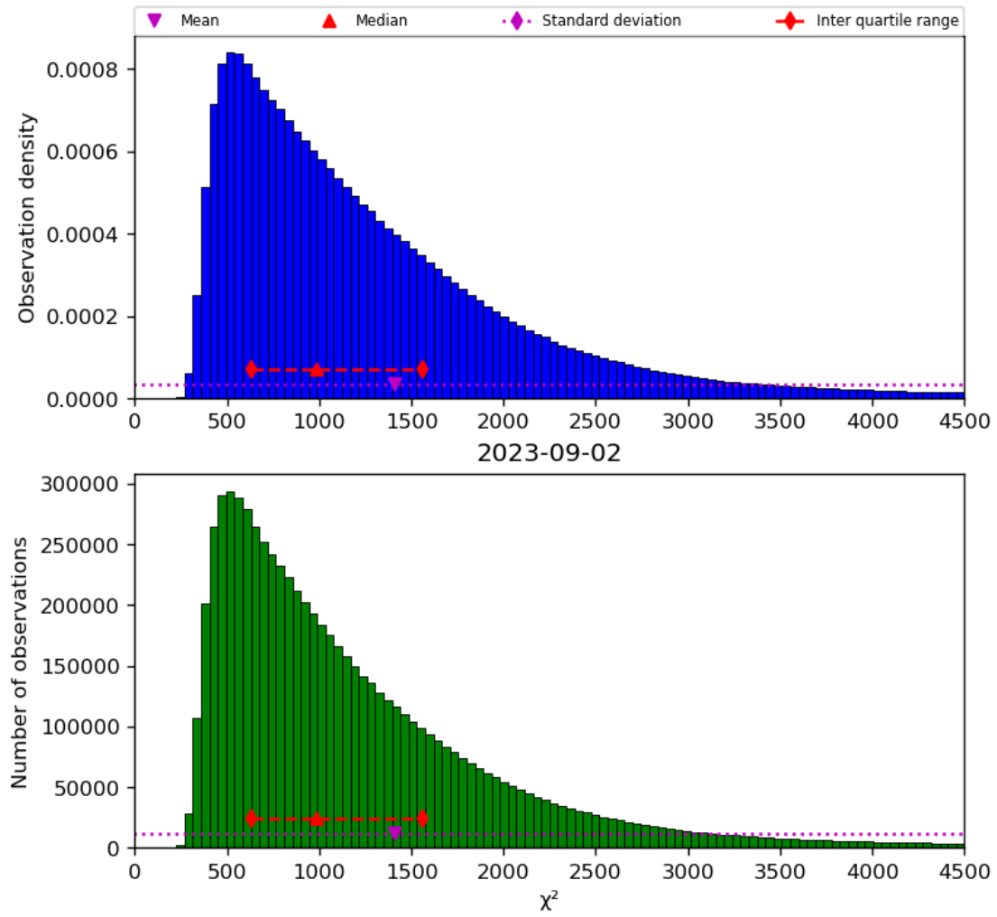
Figure 22: Histogram of “ \chi^2 ” for 2023-09-01 to 2023-09-03
