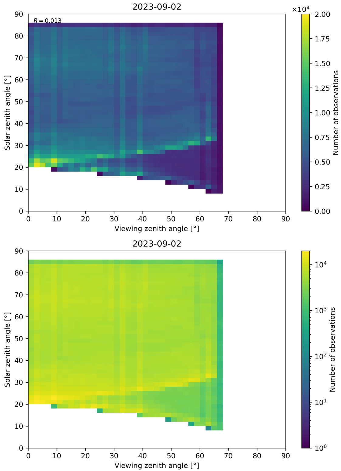
Figure 77: Scatter density plot of “Viewing zenith angle” against “Solar zenith angle” for 2023-09-01 to 2023-09-03.
