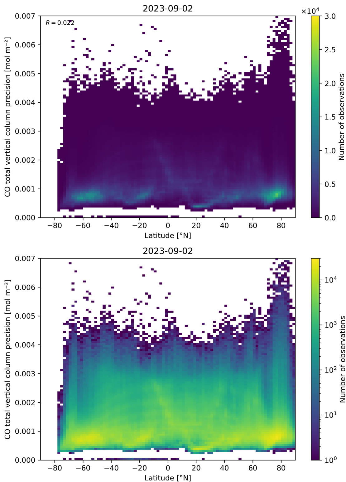
Figure 53: Scatter density plot of “Latitude” against “CO total vertical column precision” for 2023-09-01 to 2023-09-03.
