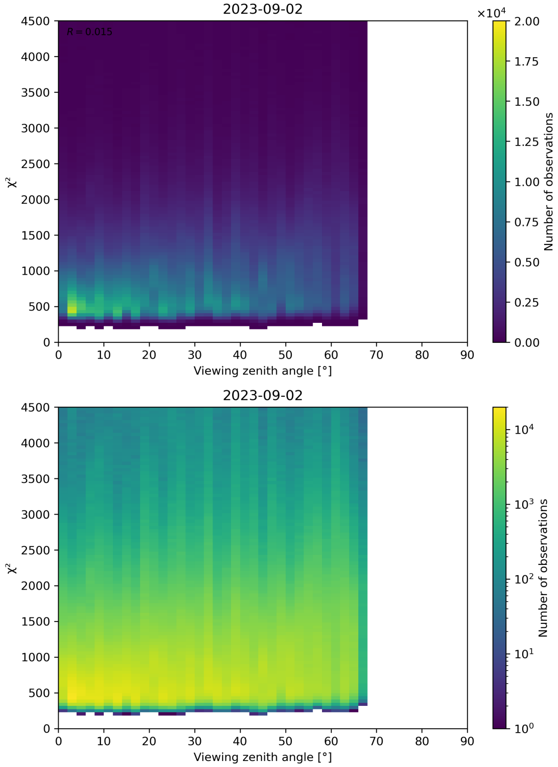
Figure 72: Scatter density plot of “Viewing zenith angle” against “ \chi^2 ” for 2023-09-01 to 2023-09-03.
