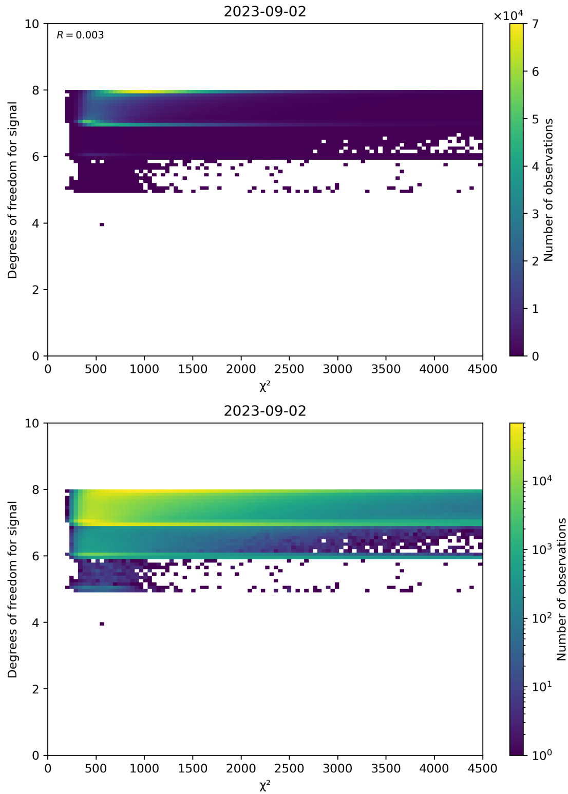
Figure 48: Scatter density plot of “ \chi^2 ” against “Degrees of freedom for signal” for 2023-09-01 to 2023-09-03.
