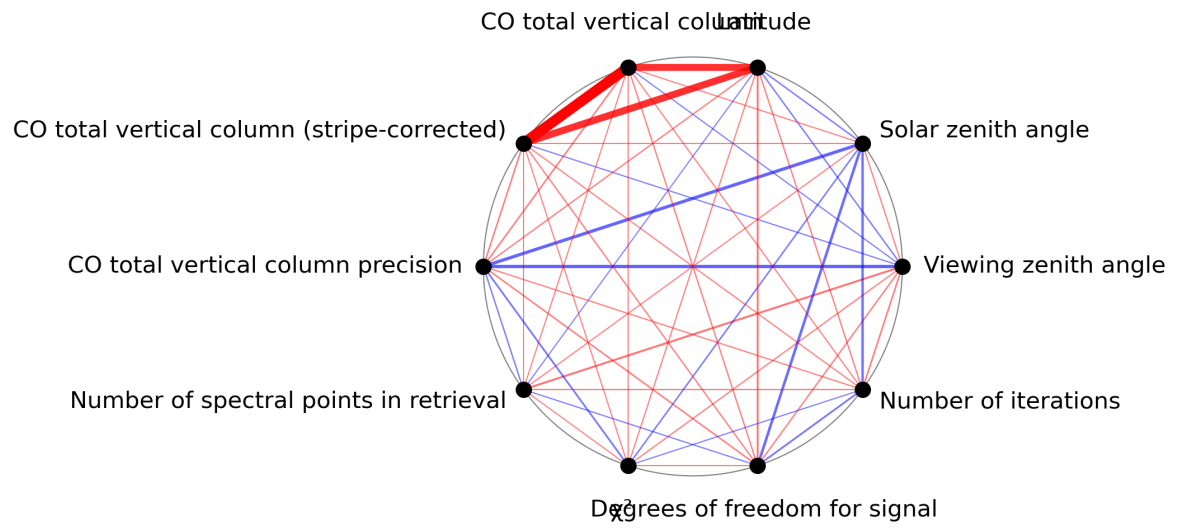
Figure 1: Map of correlation graph for 2023-09-01 to 2023-09-03.
