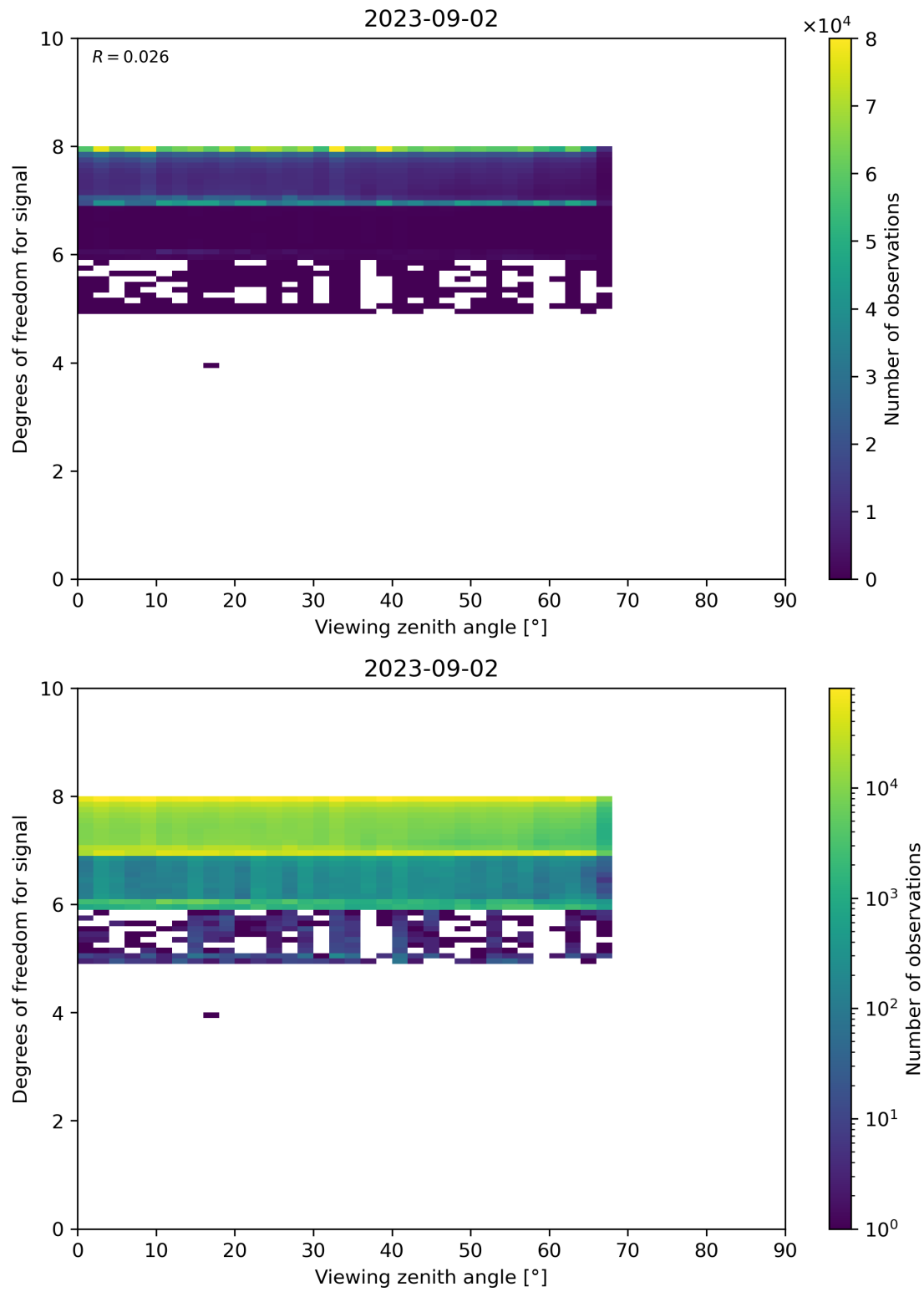
Figure 73: Scatter density plot of “Viewing zenith angle” against “Degrees of freedom for signal” for 2023-09-01 to 2023-09-03.
