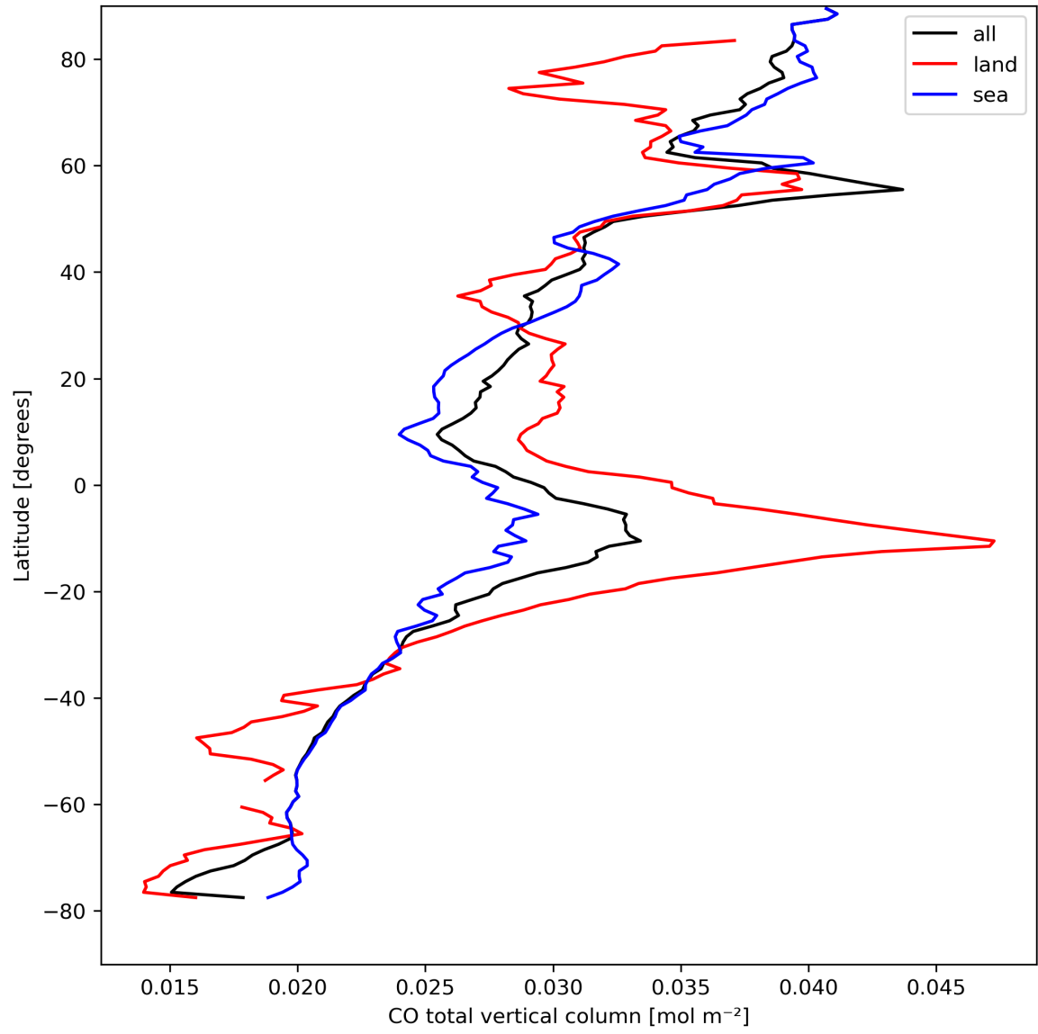
Figure 10: Zonal average of “CO total vertical column” for 2023-09-01 to 2023-09-03.
