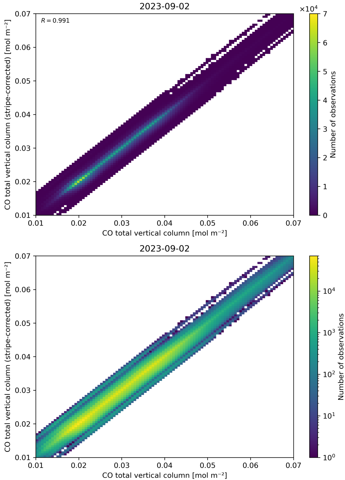
Figure 33: Scatter density plot of “CO total vertical column” against “CO total vertical column (stripe-corrected)” for 2023-09-01 to 2023-09-03.
