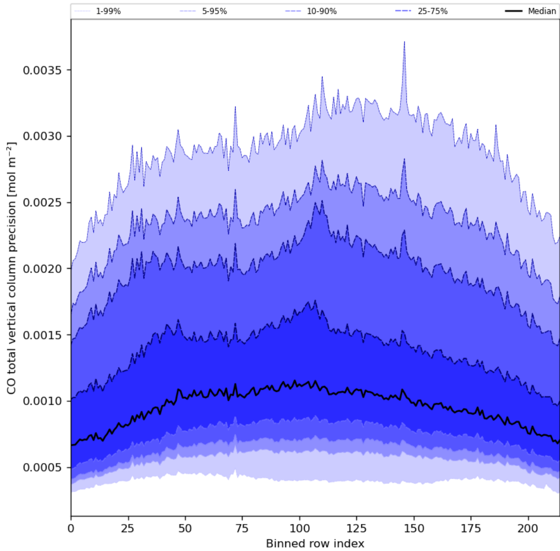
Figure 28: Along track statistics of “CO total vertical column precision” for 2023-09-01 to 2023-09-03
