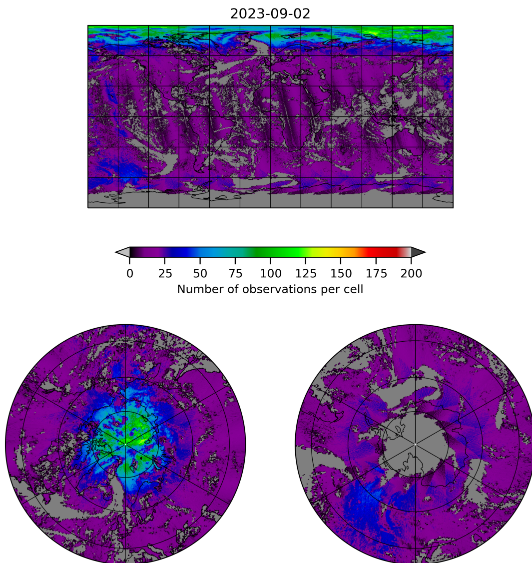
Figure 8: Map of the number of observations for 2023-09-01 to 2023-09-03
