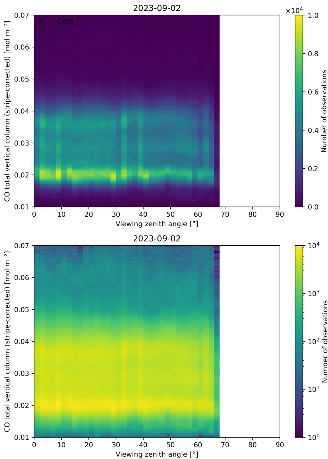
Figure 70: Scatter density plot of “Viewing zenith angle” against “CO total vertical column (stripe-corrected)” for 2023-09-01 to 2023-09-03.
