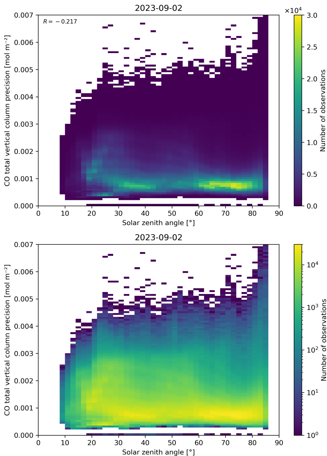
Figure 63: Scatter density plot of “Solar zenith angle” against “CO total vertical column precision” for 2023-09-01 to 2023-09-03.
