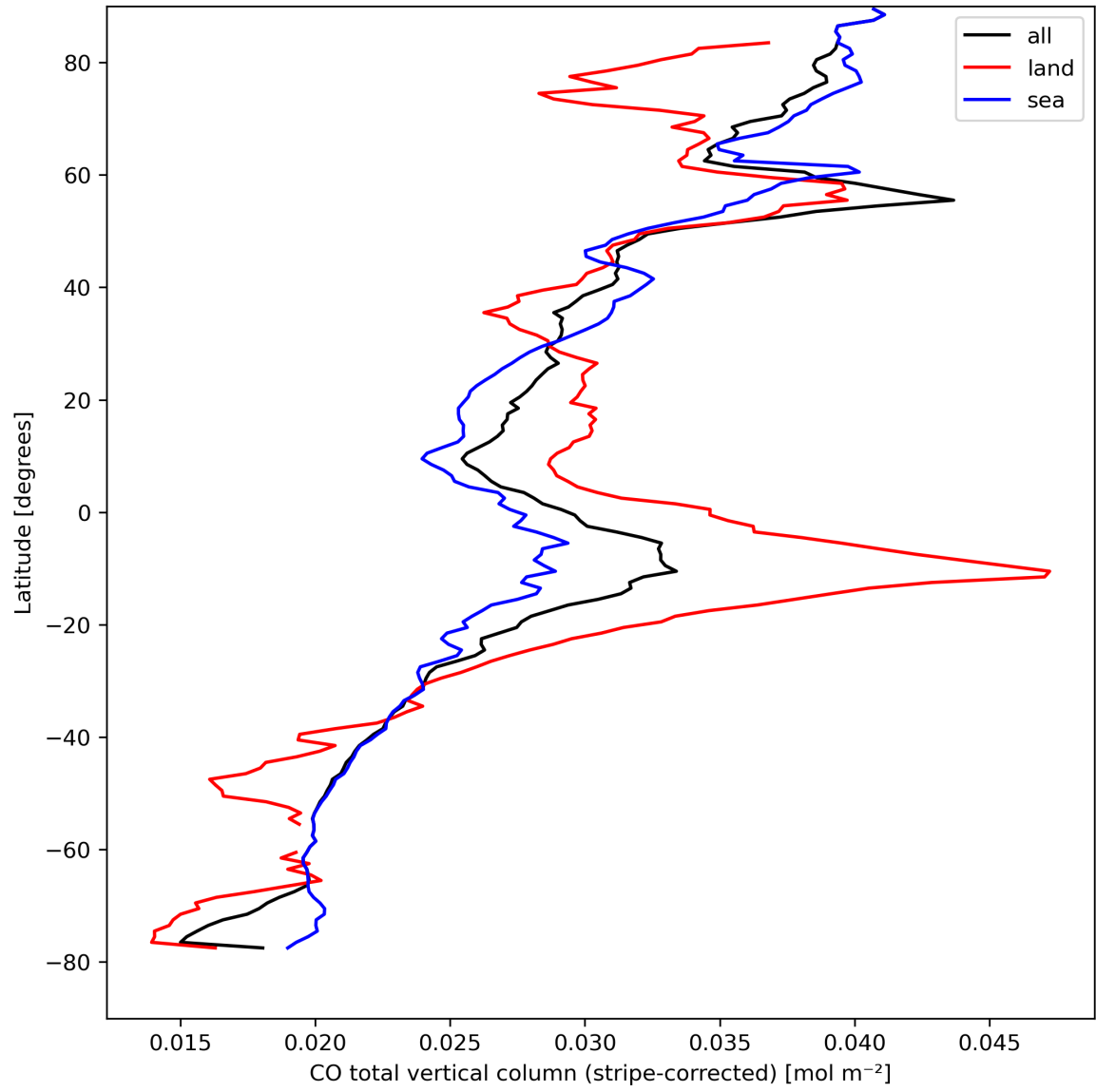
Figure 11: Zonal average of “CO total vertical column (stripe-corrected)” for 2023-09-01 to 2023-09-03.
