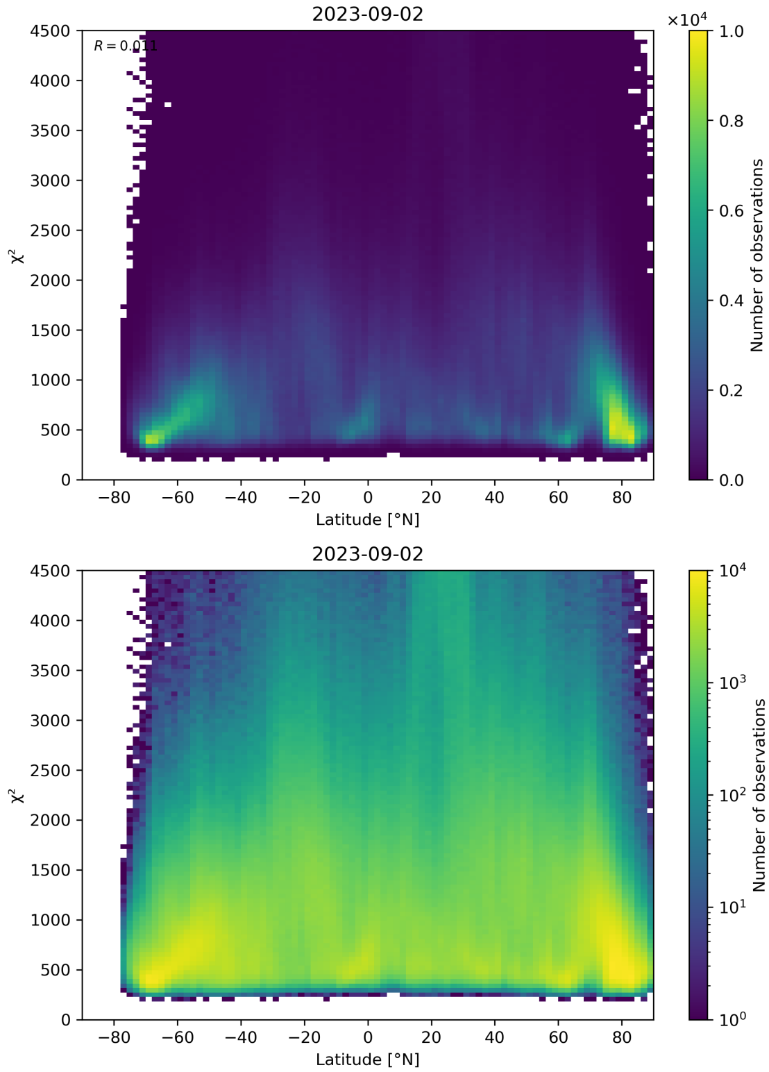
Figure 54: Scatter density plot of “Latitude” against “ \chi^2 ” for 2023-09-01 to 2023-09-03.
