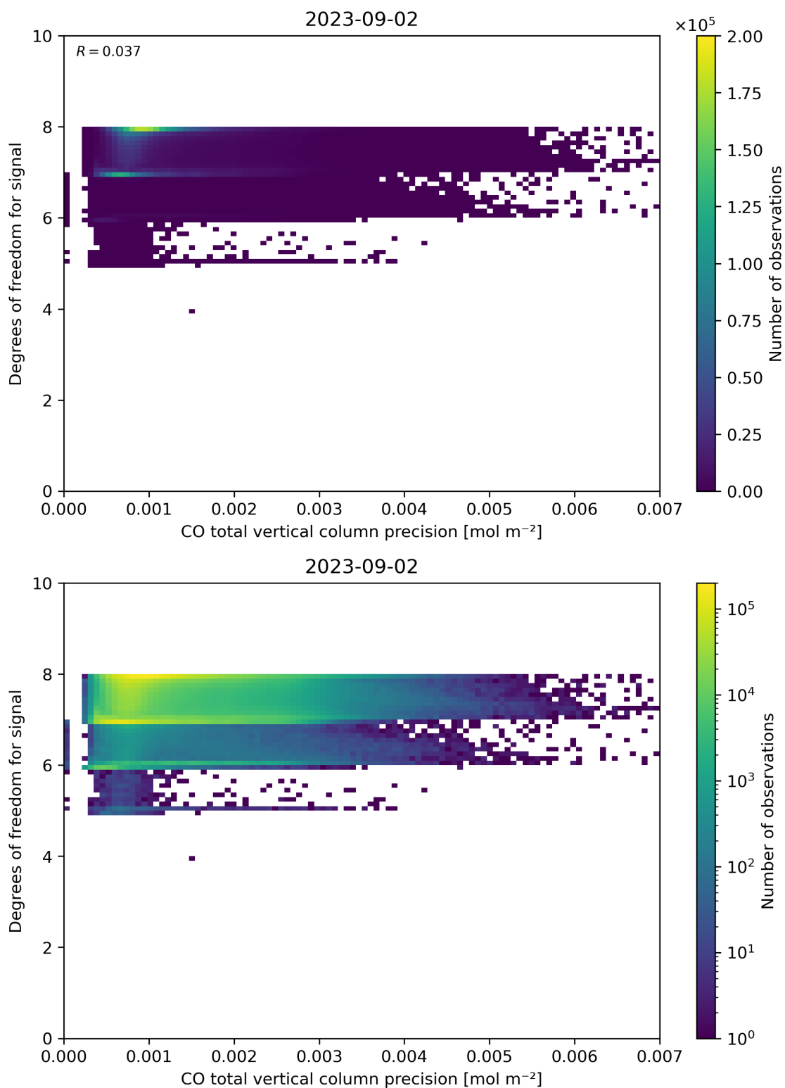
Figure 45: Scatter density plot of “CO total vertical column precision” against “Degrees of freedom for signal” for 2023-09-01 to 2023-09-03.
