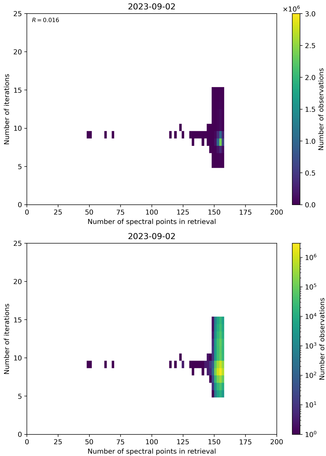
Figure 60: Scatter density plot of “Number of spectral points in retrieval” against “Number of iterations” for 2023-09-01 to 2023-09-03.
