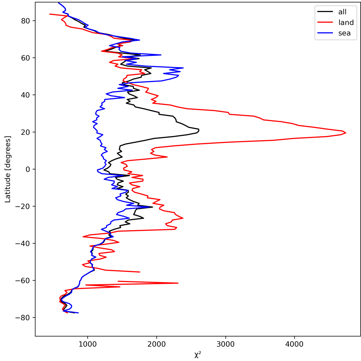
Figure 14: Zonal average of “ \chi^2 ” for 2023-09-01 to 2023-09-03.
