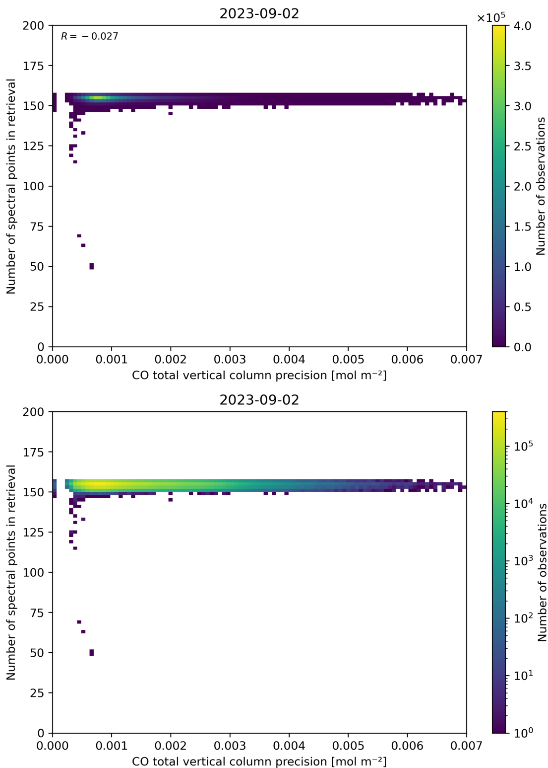
Figure 47: Scatter density plot of “CO total vertical column precision” against “Number of spectral points in retrieval” for 2023-09-01 to 2023-09-03.
