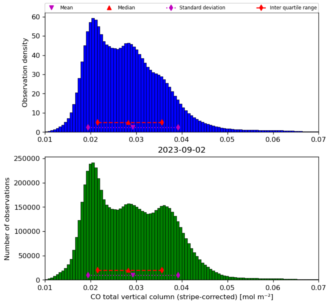
Figure 19: Histogram of “CO total vertical column (stripe-corrected)” for 2023-09-01 to 2023-09-03
