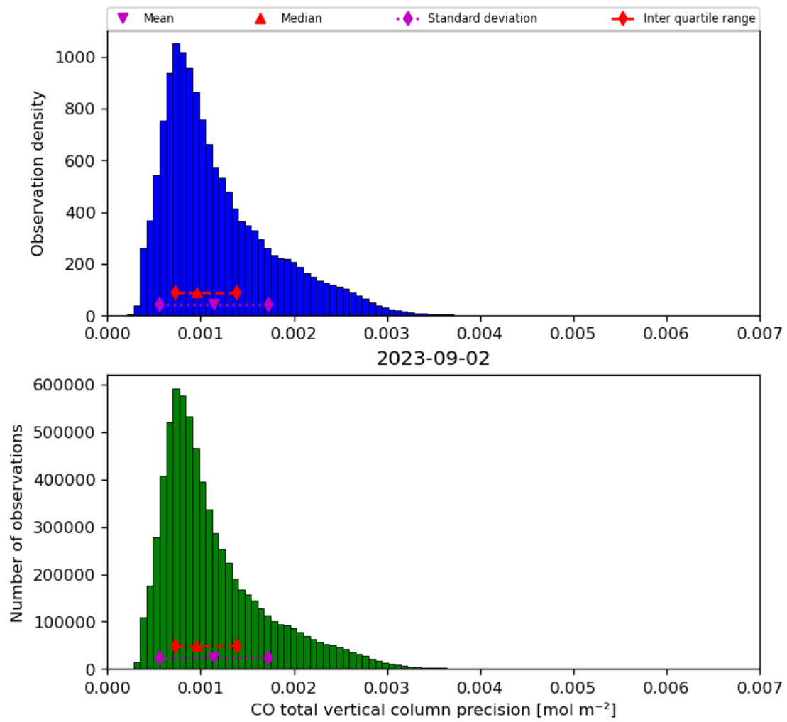
Figure 20: Histogram of “CO total vertical column precision” for 2023-09-01 to 2023-09-03
