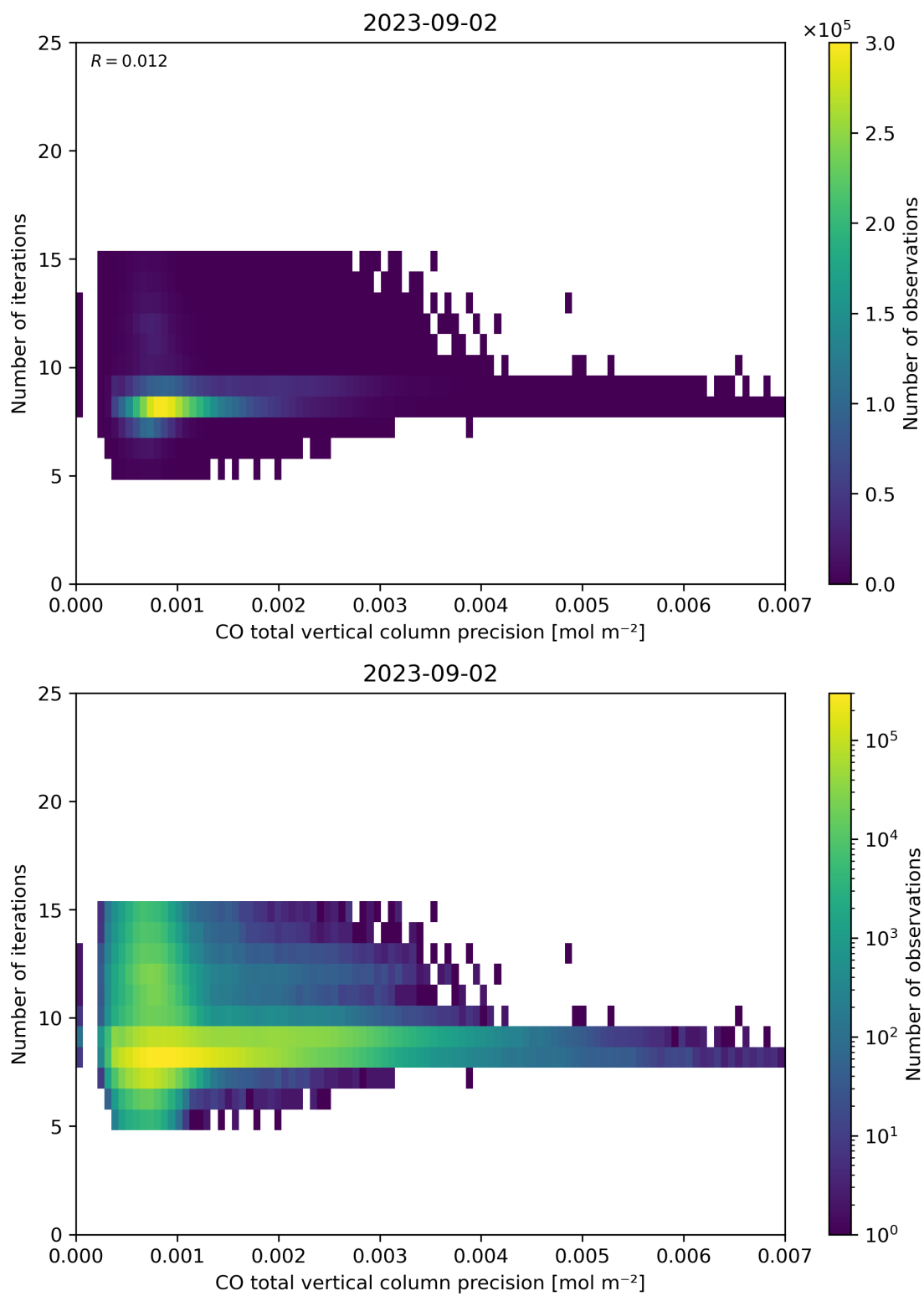
Figure 46: Scatter density plot of “CO total vertical column precision” against “Number of iterations” for 2023-09-01 to 2023-09-03.
