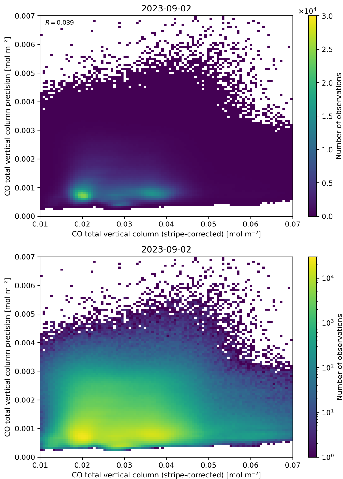
Figure 36: Scatter density plot of “CO total vertical column (stripe-corrected)” against “CO total vertical column precision” for 2023-09-01 to 2023-09-03.
