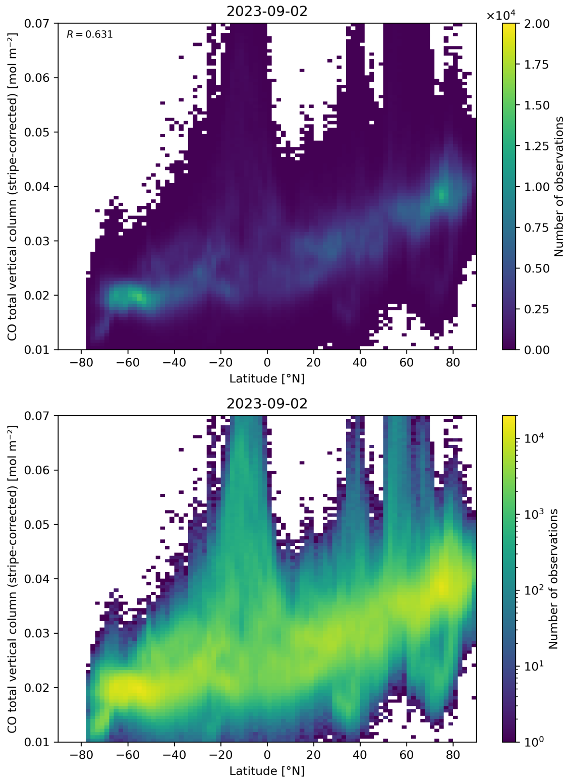
Figure 52: Scatter density plot of “Latitude” against “CO total vertical column (stripe-corrected)” for 2023-09-01 to 2023-09-03.
