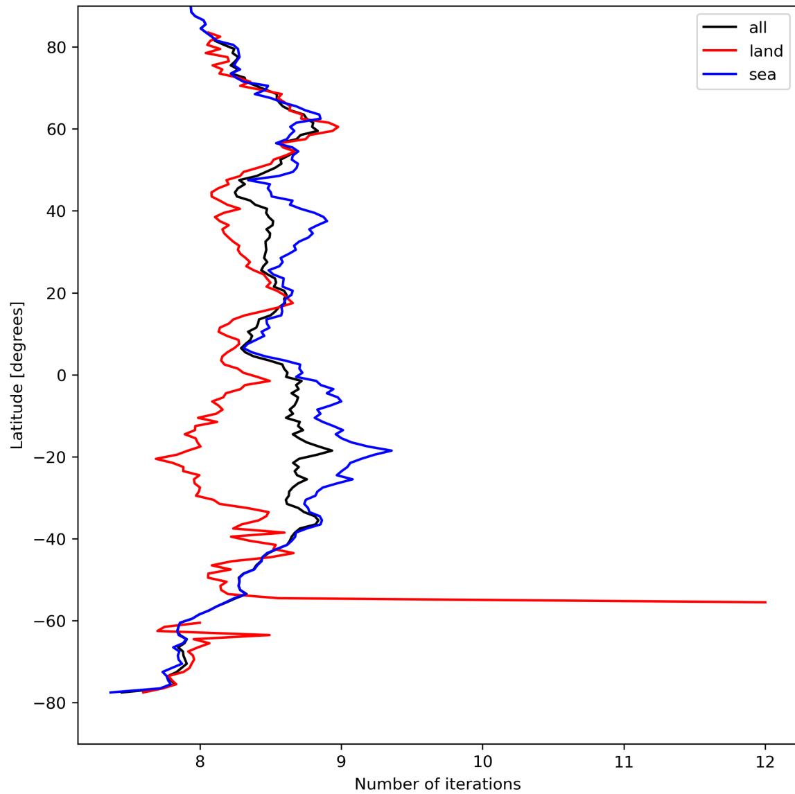
Figure 16: Zonal average of “Number of iterations” for 2023-09-01 to 2023-09-03.
