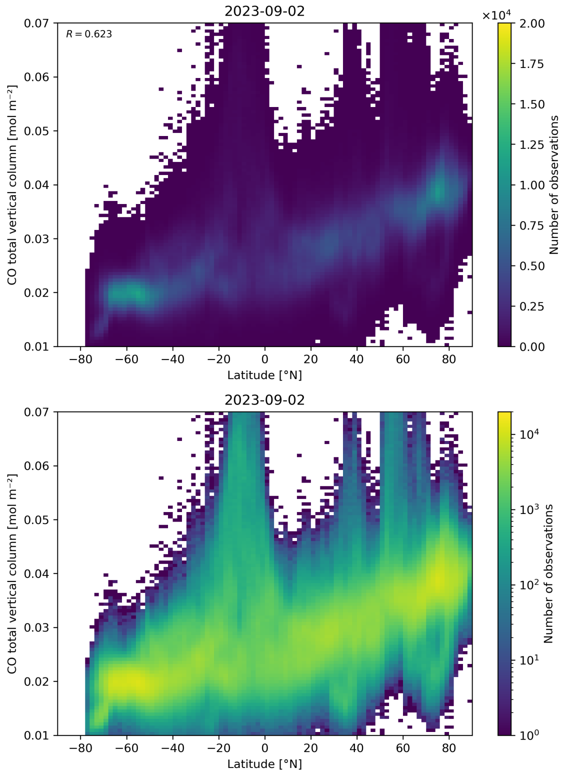
Figure 51: Scatter density plot of “Latitude” against “CO total vertical column” for 2023-09-01 to 2023-09-03.
