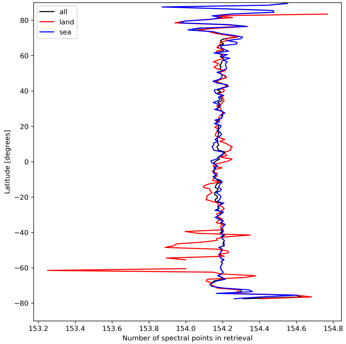
Figure 13: Zonal average of “Number of spectral points in retrieval” for 2023-09-01 to 2023-09-03.
