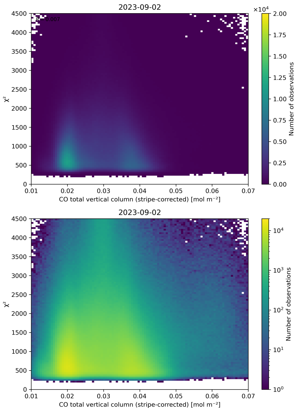
Figure 37: Scatter density plot of “CO total vertical column (stripe-corrected)” against “ \chi^2 ” for 2023-09-01 to 2023-09-03.
