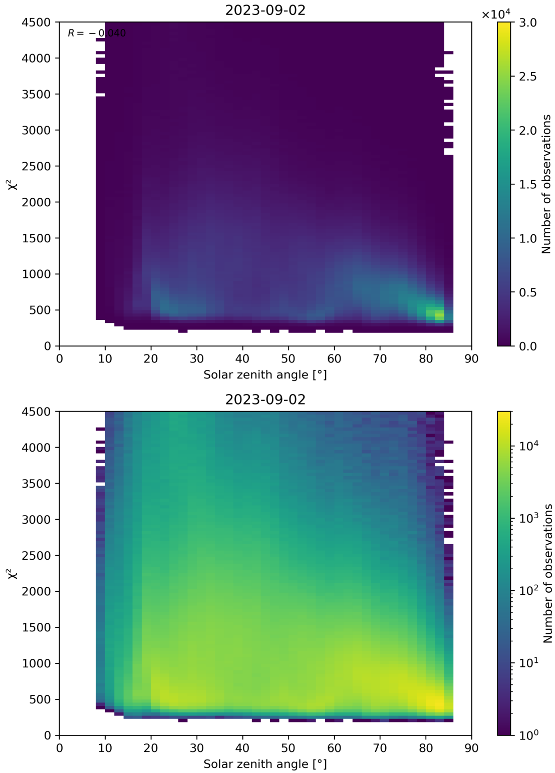
Figure 64: Scatter density plot of “Solar zenith angle” against “ \chi^2 ” for 2023-09-01 to 2023-09-03.
