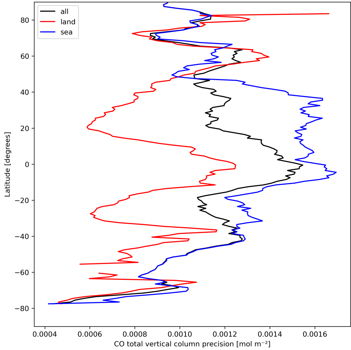
Figure 12: Zonal average of “CO total vertical column precision” for 2023-09-01 to 2023-09-03.
