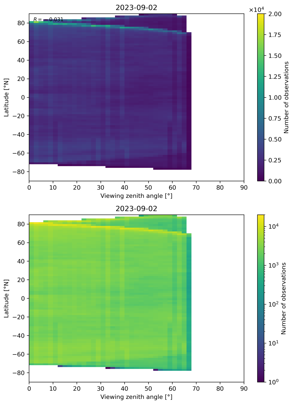
Figure 74: Scatter density plot of “Viewing zenith angle” against “Latitude” for 2023-09-01 to 2023-09-03.
