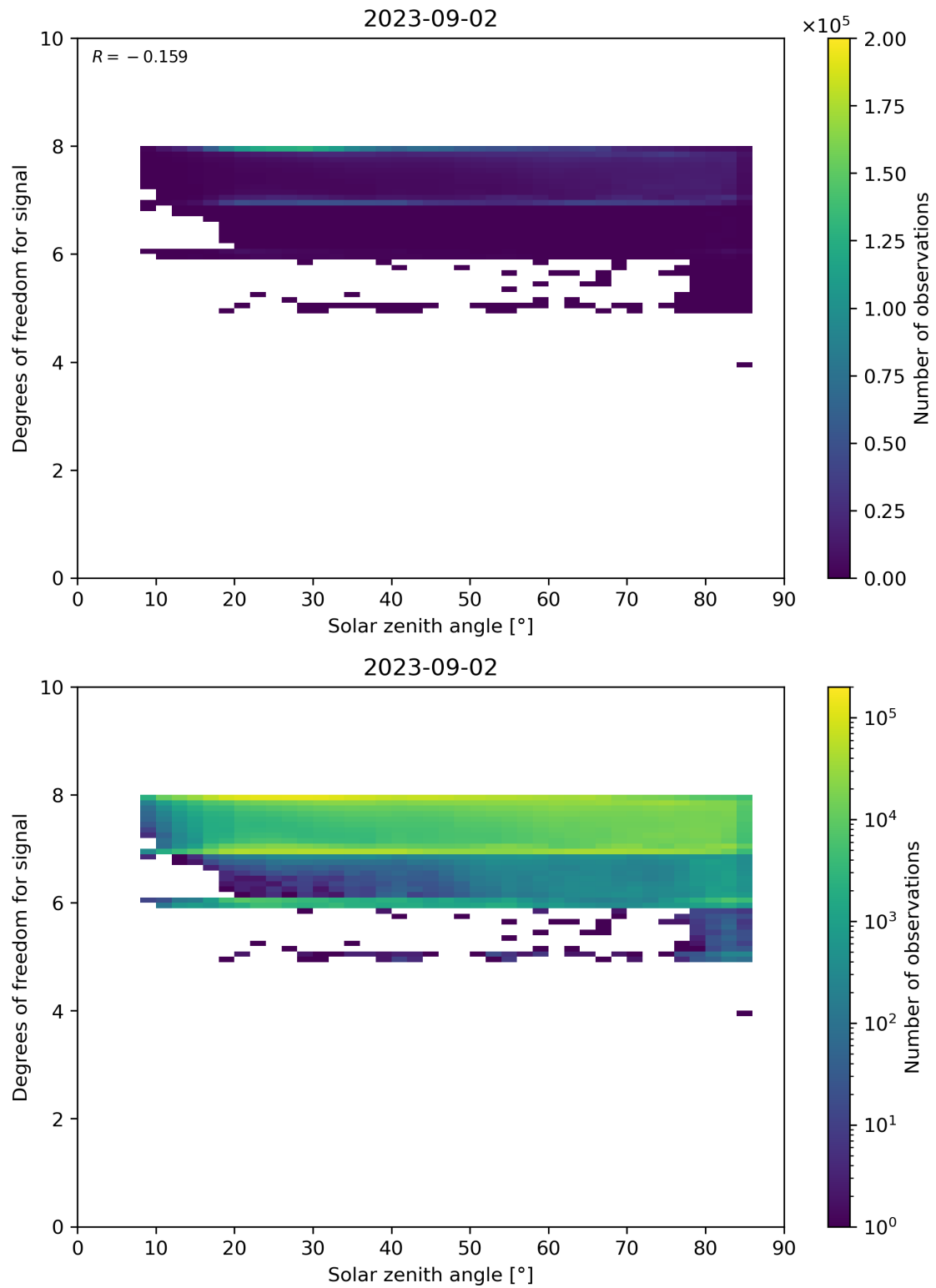
Figure 65: Scatter density plot of “Solar zenith angle” against “Degrees of freedom for signal” for 2023-09-01 to 2023-09-03.
