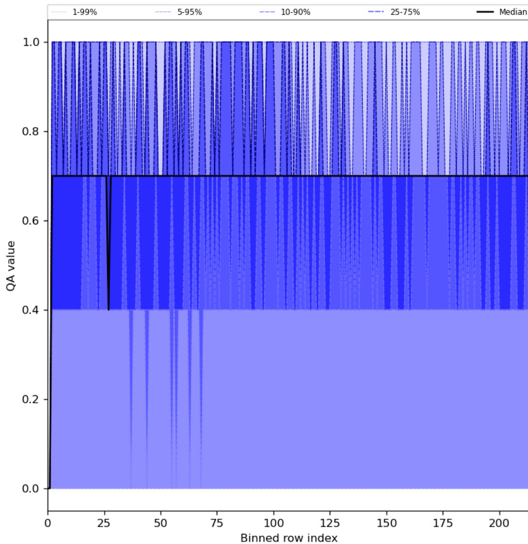
Figure 25: Along track statistics of “QA value” for 2023-09-01 to 2023-09-03
