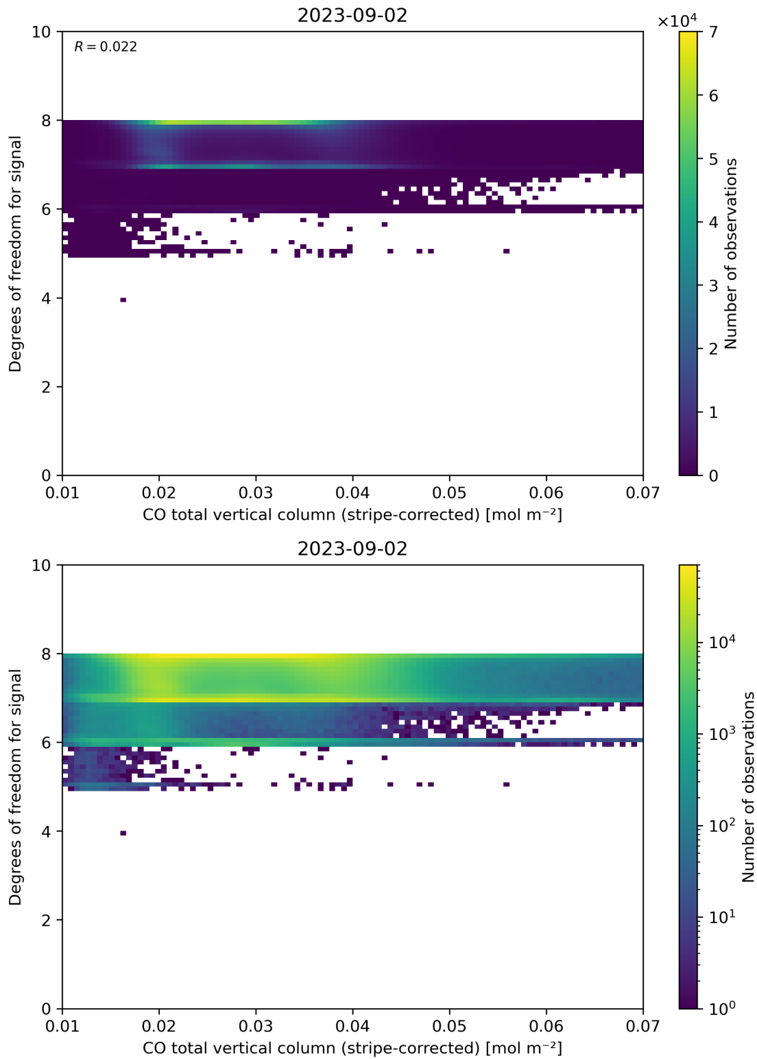
Figure 38: Scatter density plot of “CO total vertical column (stripe-corrected)” against “Degrees of freedom for signal” for 2023-09-01 to 2023-09-03.
