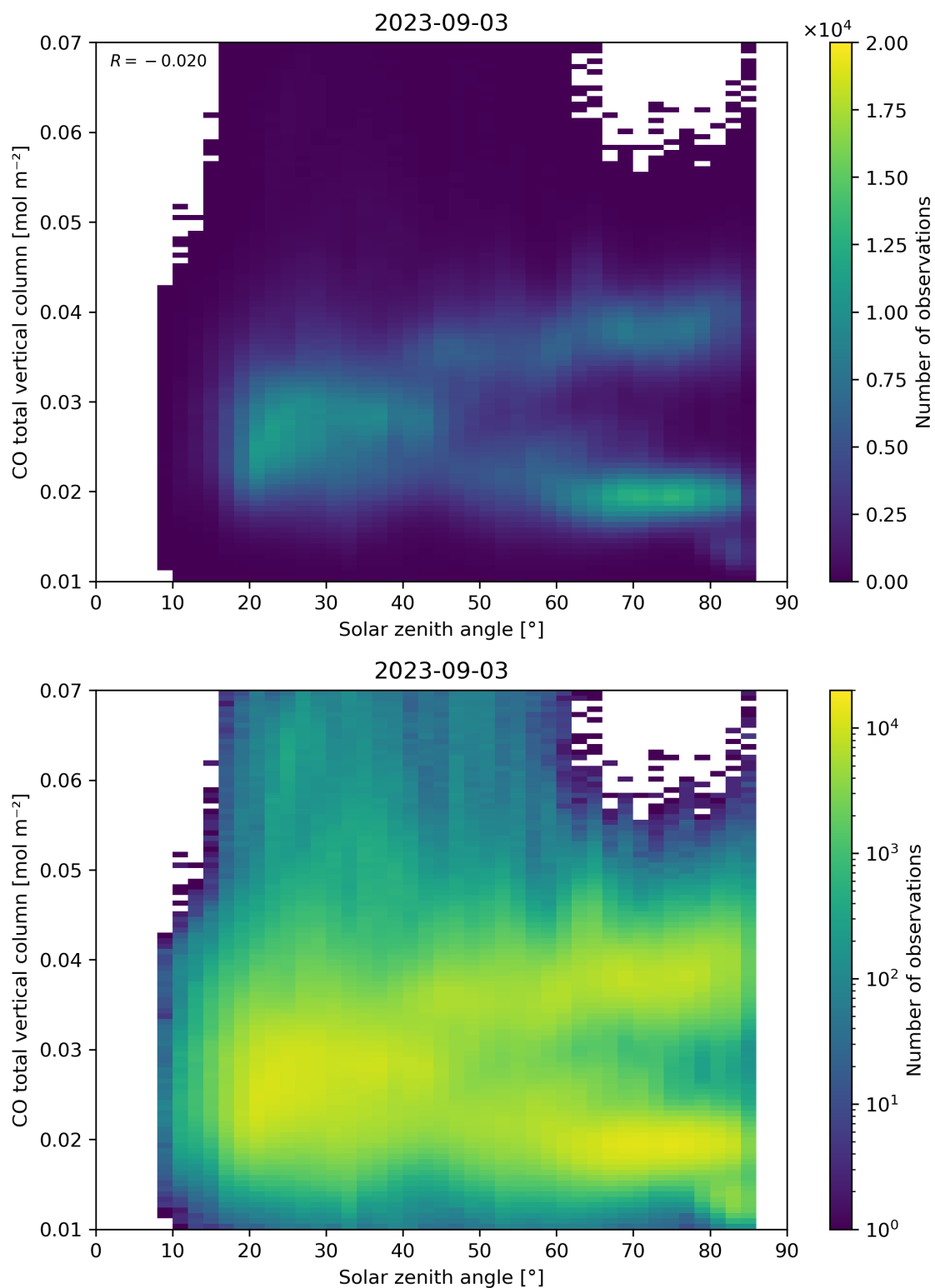
Figure 61: Scatter density plot of “Solar zenith angle” against “CO total vertical column” for 2023-09-02 to 2023-09-04.
