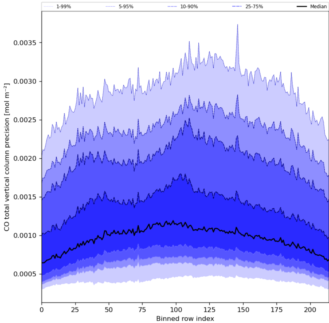
Figure 28: Along track statistics of “CO total vertical column precision” for 2023-09-02 to 2023-09-04
