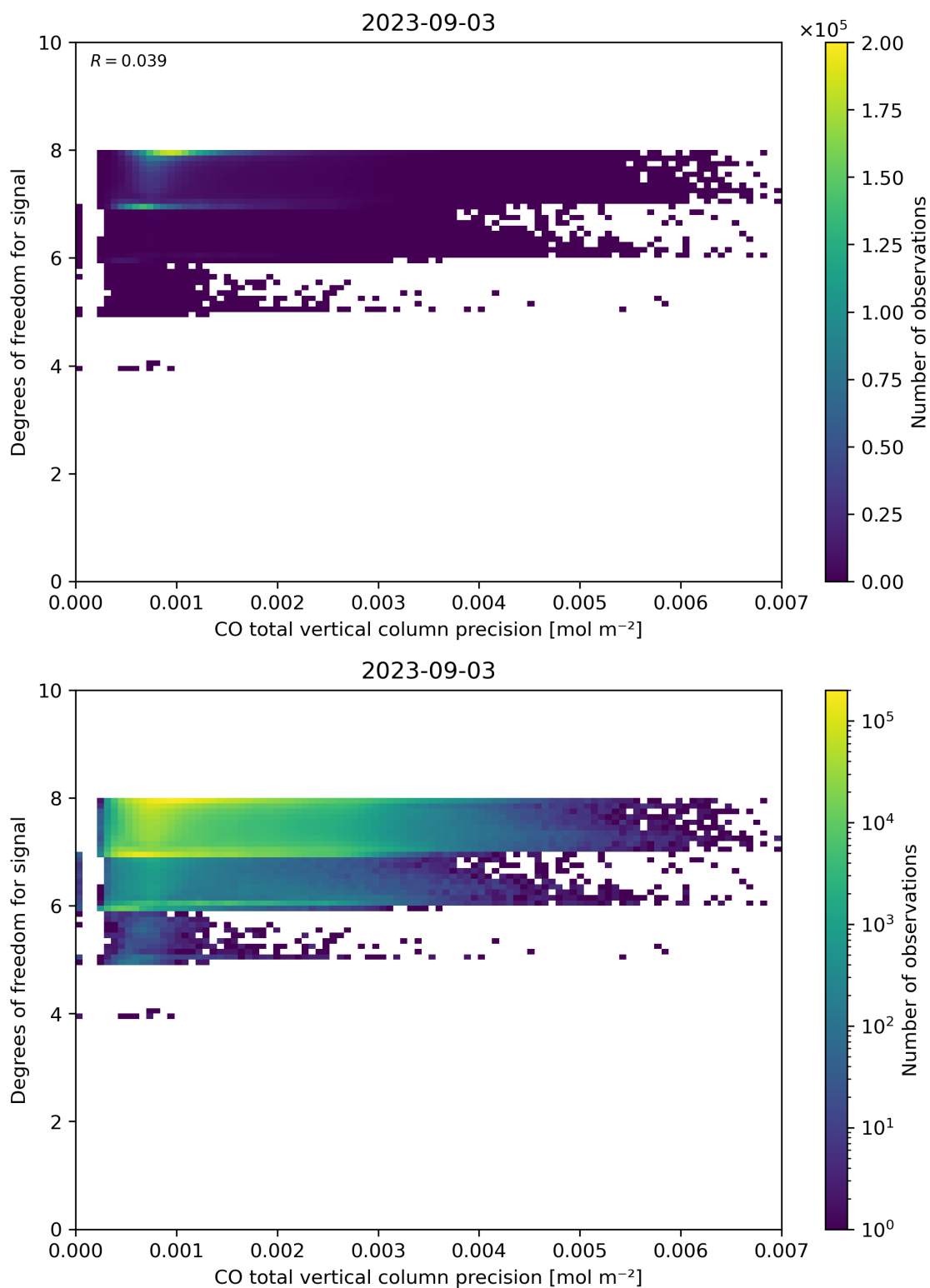
Figure 45: Scatter density plot of “CO total vertical column precision” against “Degrees of freedom for signal” for 2023-09-02 to 2023-09-04.
