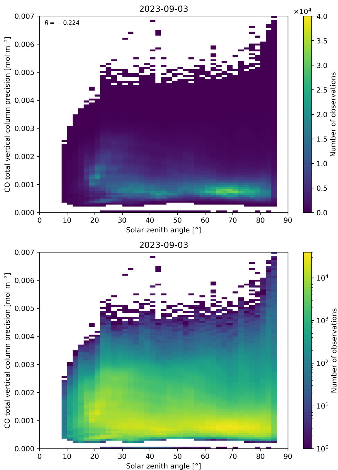
Figure 63: Scatter density plot of “Solar zenith angle” against “CO total vertical column precision” for 2023-09-02 to 2023-09-04.
