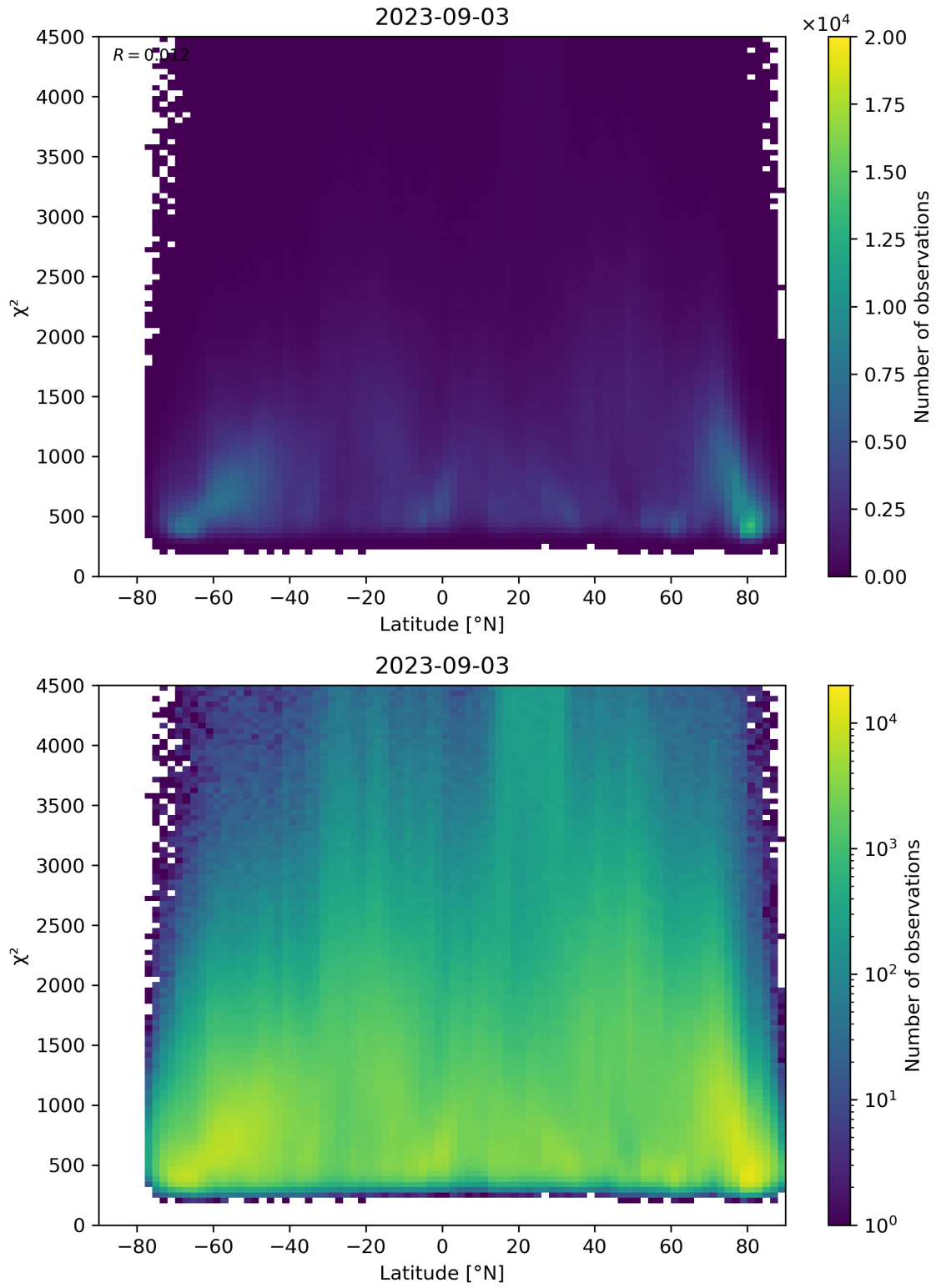
Figure 54: Scatter density plot of “Latitude” against “ \chi^2 ” for 2023-09-02 to 2023-09-04.
