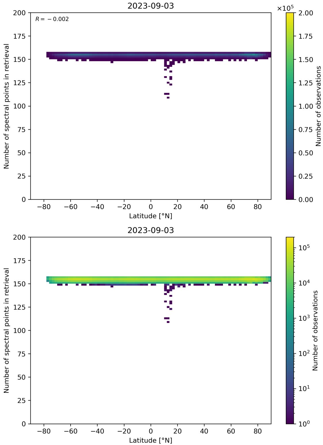
Figure 57: Scatter density plot of “Latitude” against “Number of spectral points in retrieval” for 2023-09-02 to 2023-09-04.
