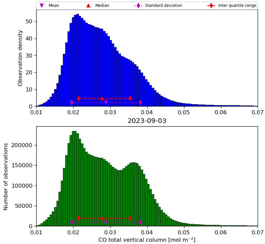
Figure 18: Histogram of “CO total vertical column” for 2023-09-02 to 2023-09-04
