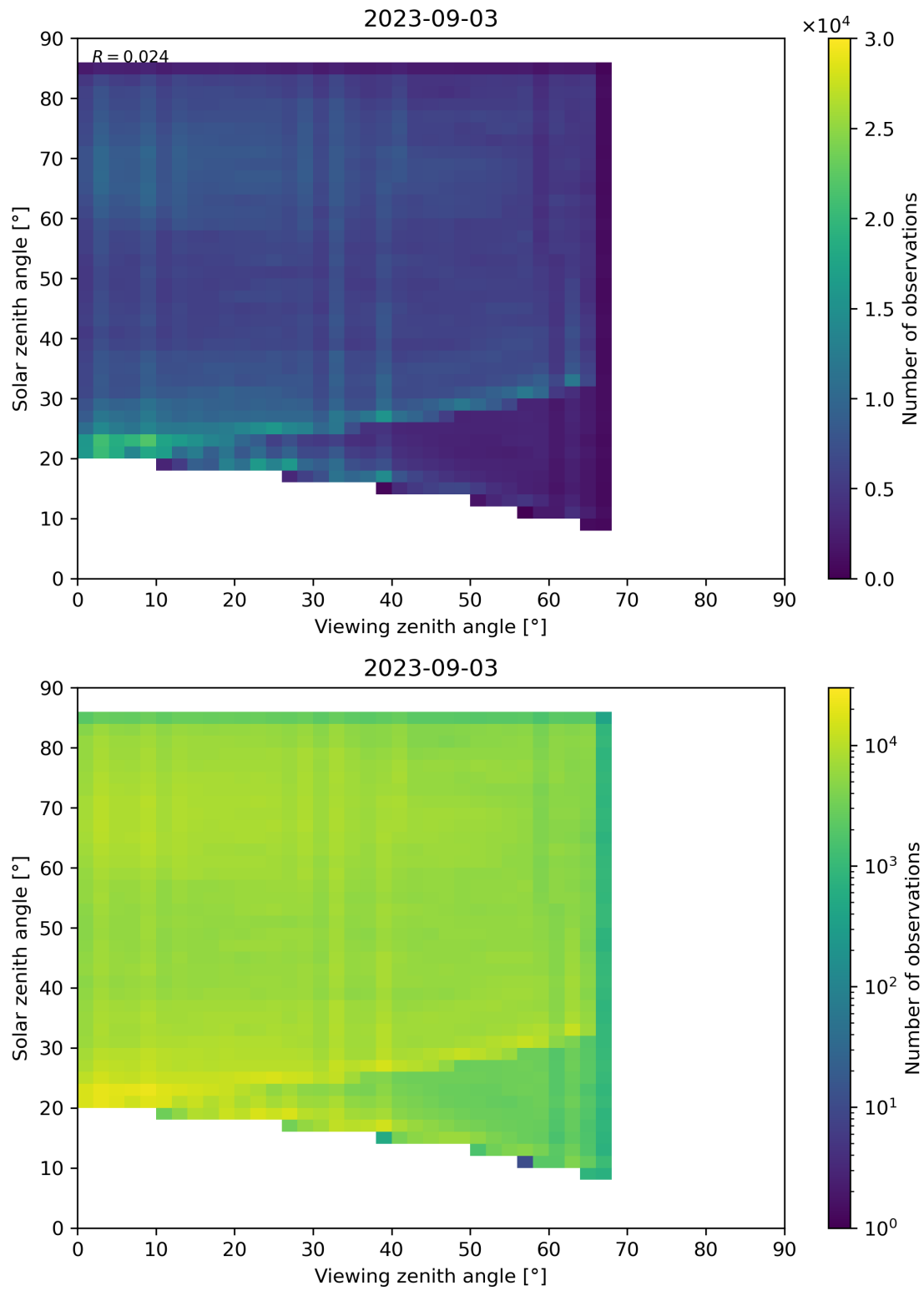
Figure 77: Scatter density plot of “Viewing zenith angle” against “Solar zenith angle” for 2023-09-02 to 2023-09-04.
