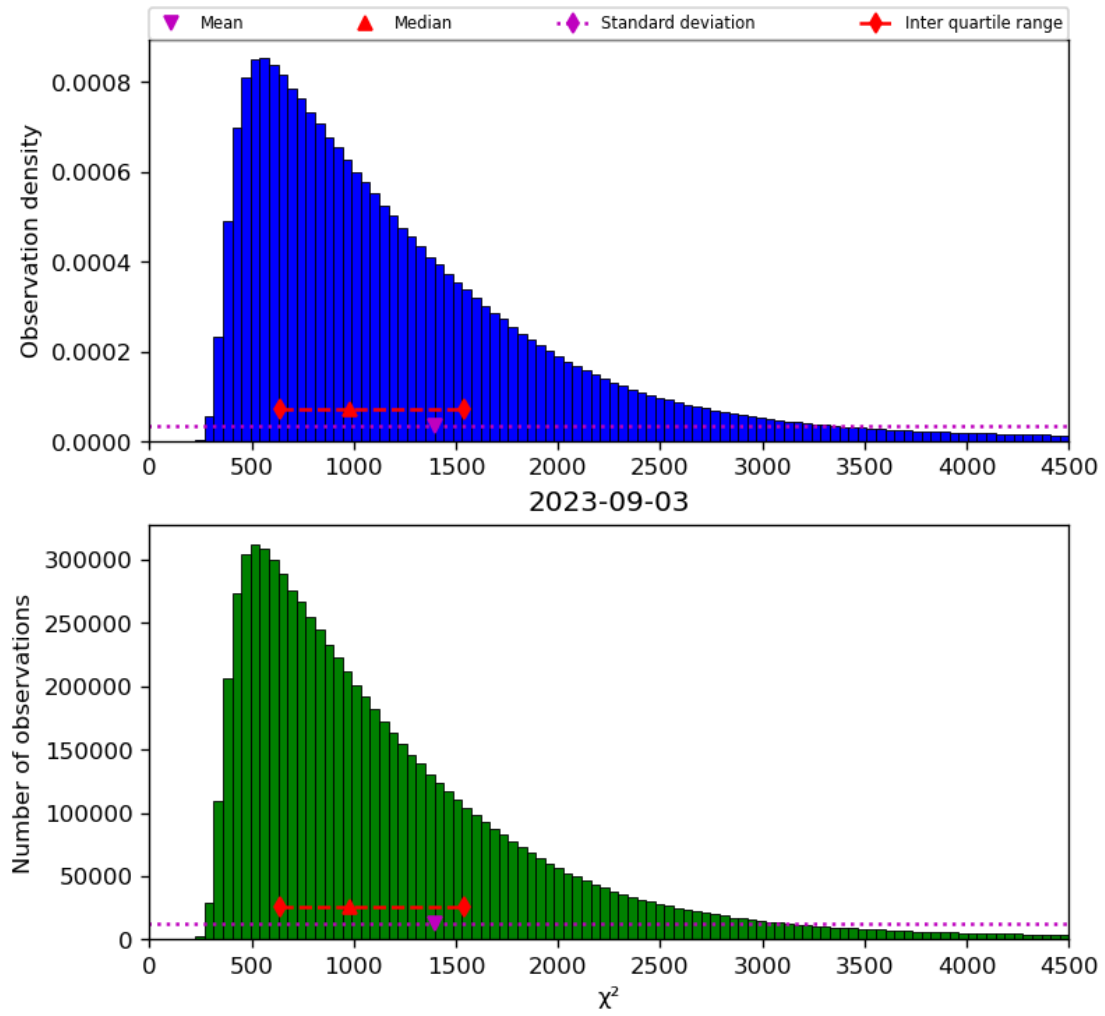
Figure 22: Histogram of “ \chi^2 ” for 2023-09-02 to 2023-09-04
