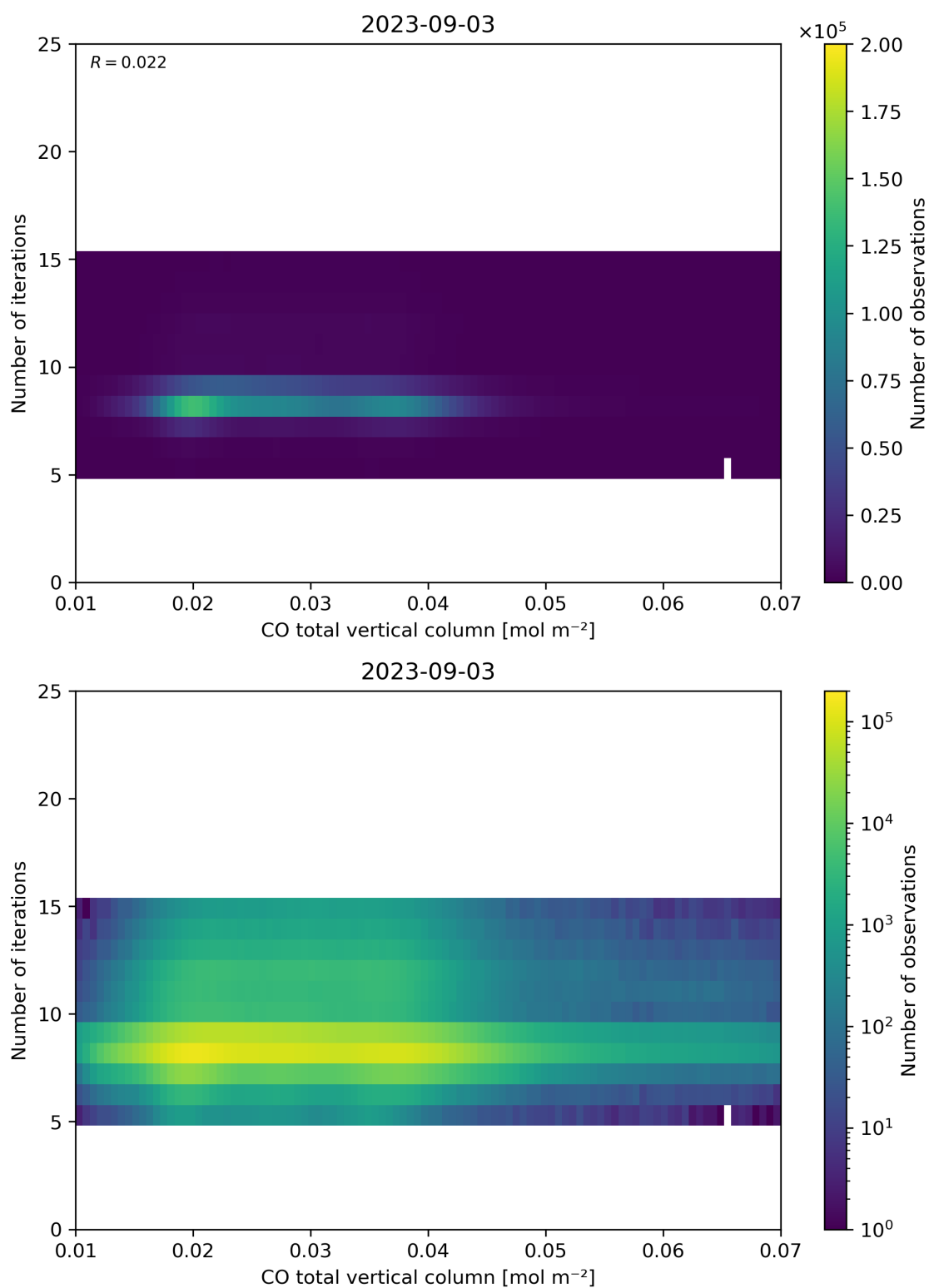
Figure 42: Scatter density plot of “CO total vertical column” against “Number of iterations” for 2023-09-02 to 2023-09-04.
