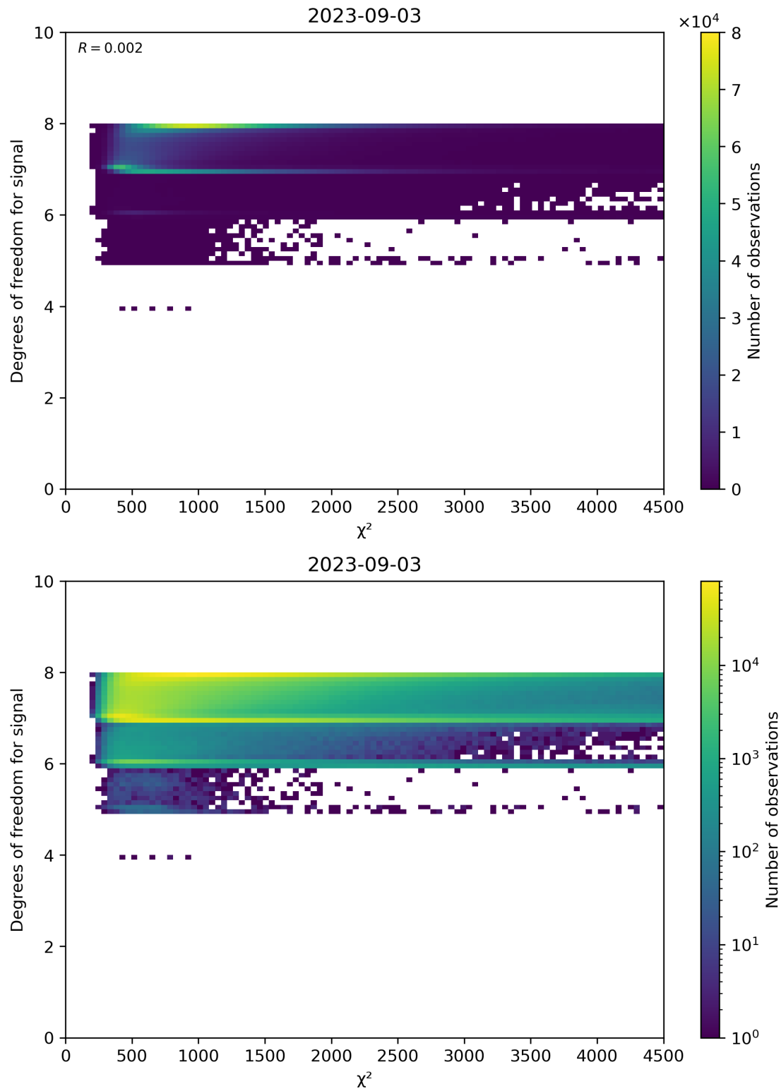
Figure 48: Scatter density plot of “ \chi^2 ” against “Degrees of freedom for signal” for 2023-09-02 to 2023-09-04.
