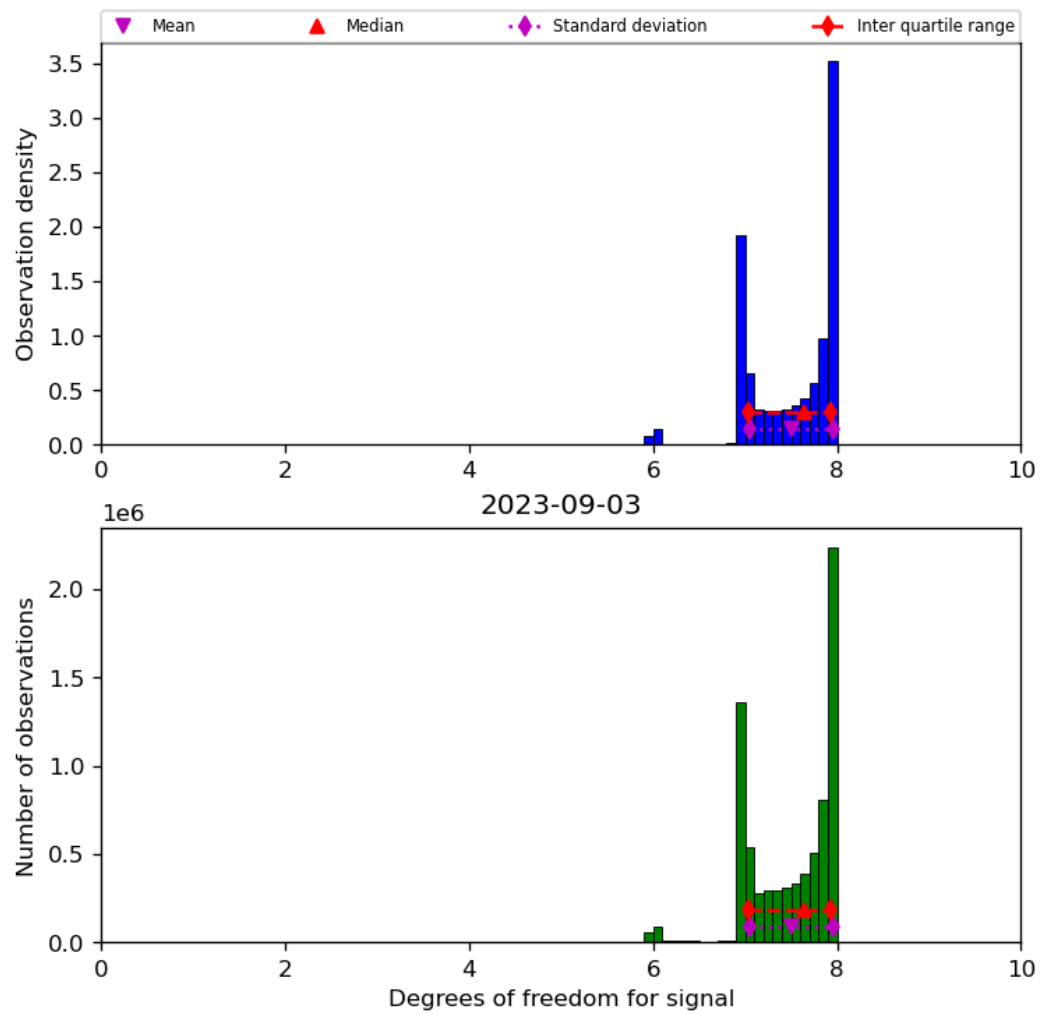
Figure 23: Histogram of “Degrees of freedom for signal” for 2023-09-02 to 2023-09-04
