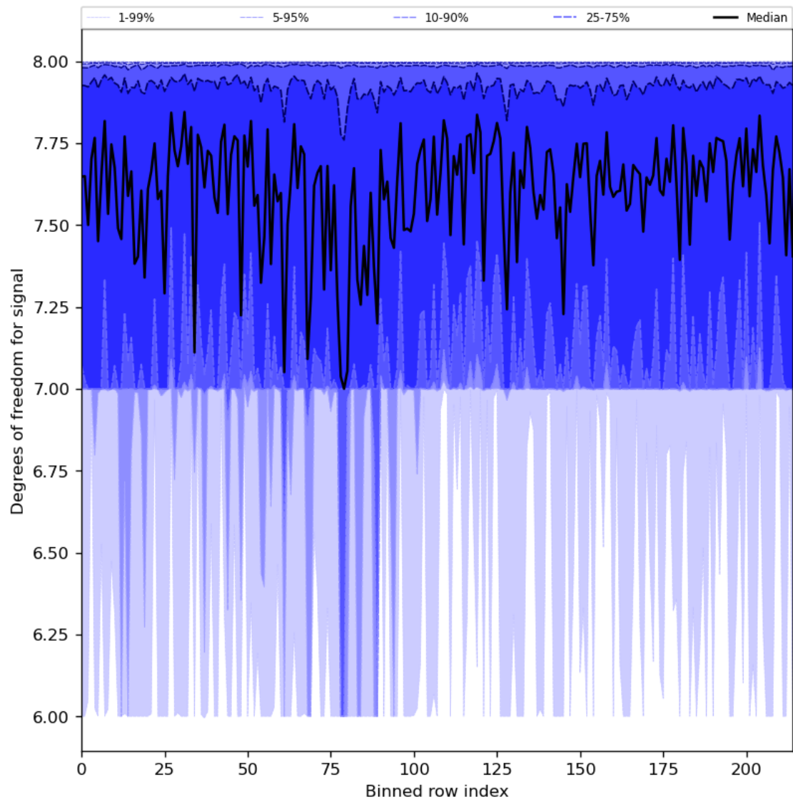
Figure 31: Along track statistics of “Degrees of freedom for signal” for 2023-09-02 to 2023-09-04
