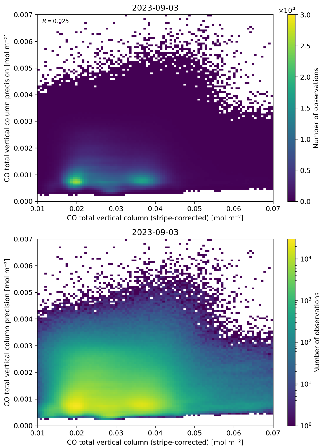
Figure 36: Scatter density plot of “CO total vertical column (stripe-corrected)” against “CO total vertical column precision” for 2023-09-02 to 2023-09-04.
