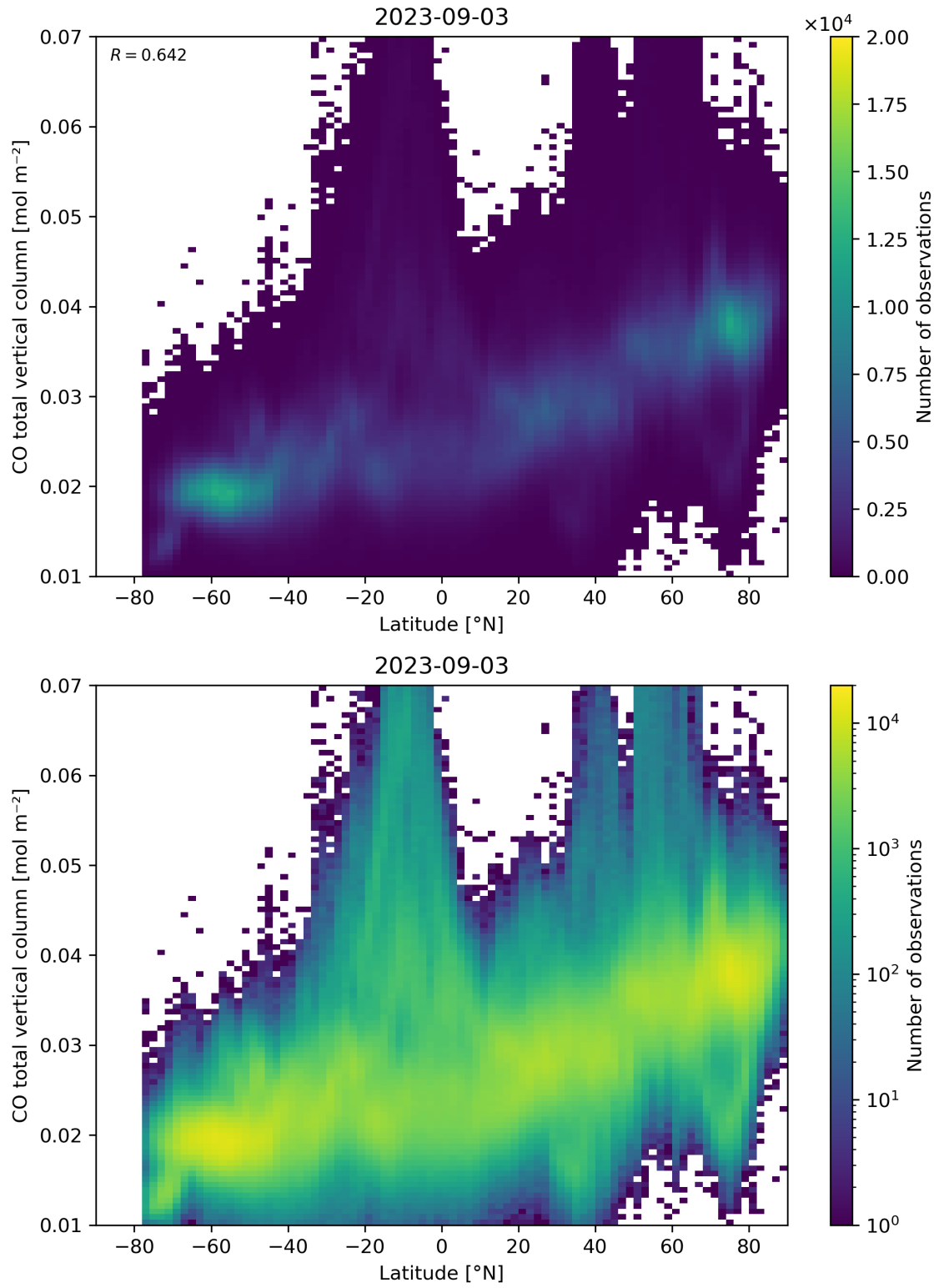
Figure 51: Scatter density plot of “Latitude” against “CO total vertical column” for 2023-09-02 to 2023-09-04.
