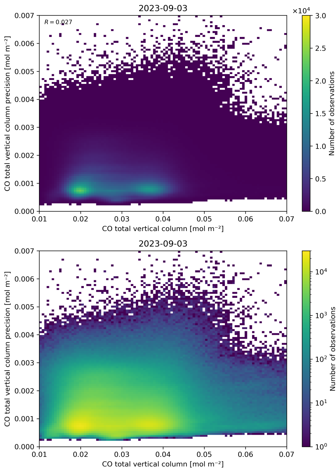
Figure 34: Scatter density plot of “CO total vertical column” against “CO total vertical column precision” for 2023-09-02 to 2023-09-04.
