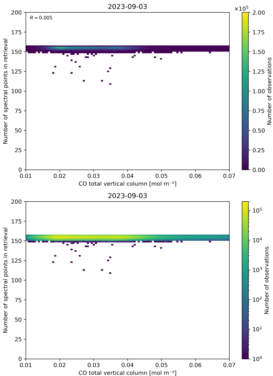
Figure 43: Scatter density plot of “CO total vertical column” against “Number of spectral points in retrieval” for 2023-09-02 to 2023-09-04.
