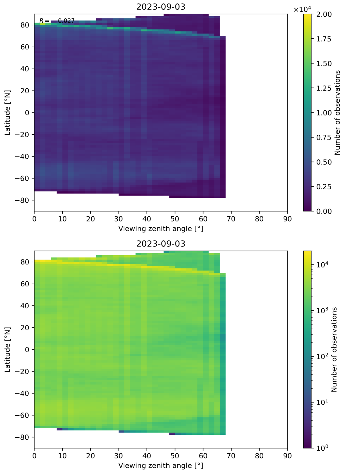
Figure 74: Scatter density plot of “Viewing zenith angle” against “Latitude” for 2023-09-02 to 2023-09-04.
