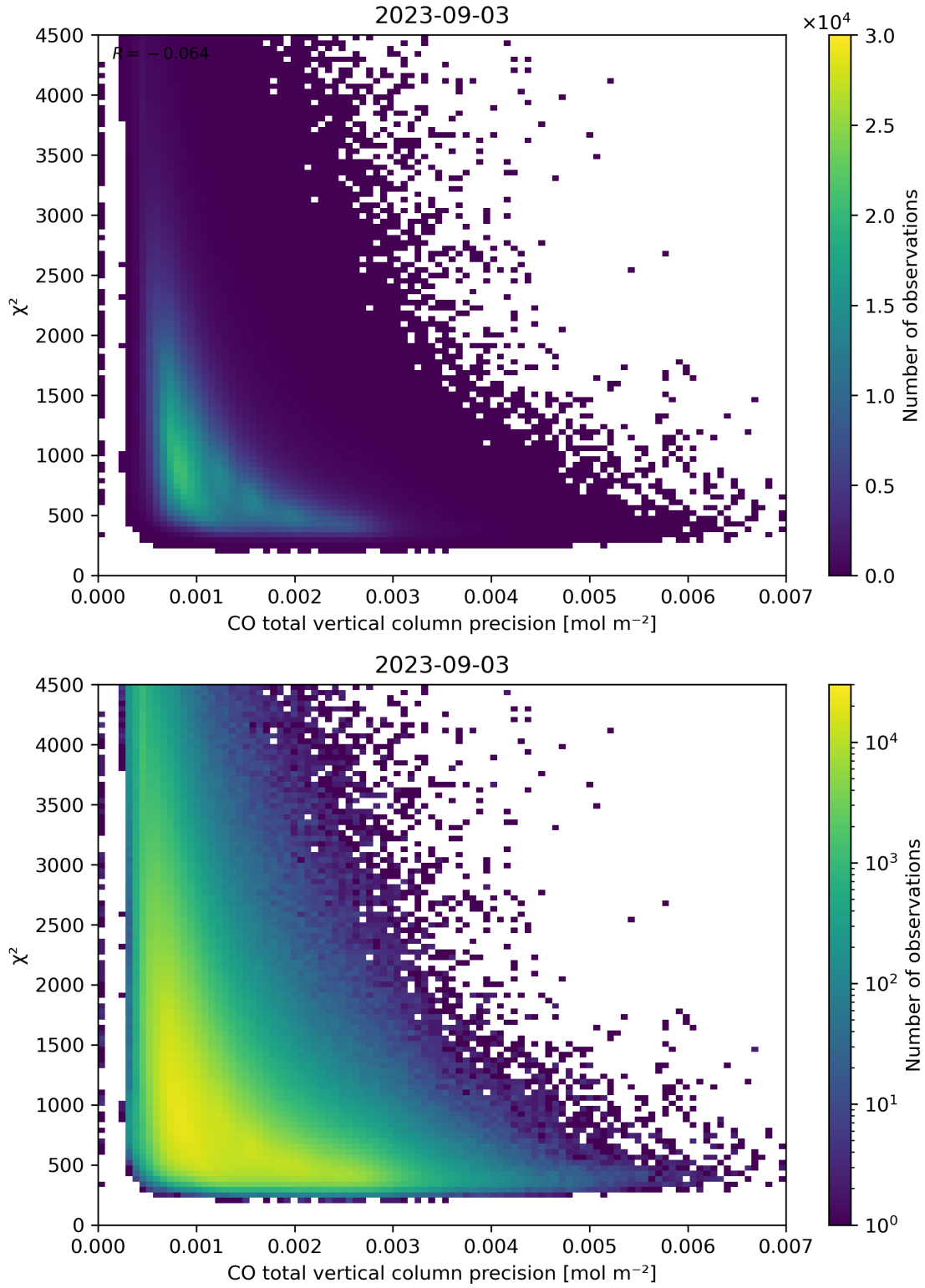
Figure 44: Scatter density plot of “CO total vertical column precision” against “ \chi^2 ” for 2023-09-02 to 2023-09-04.
