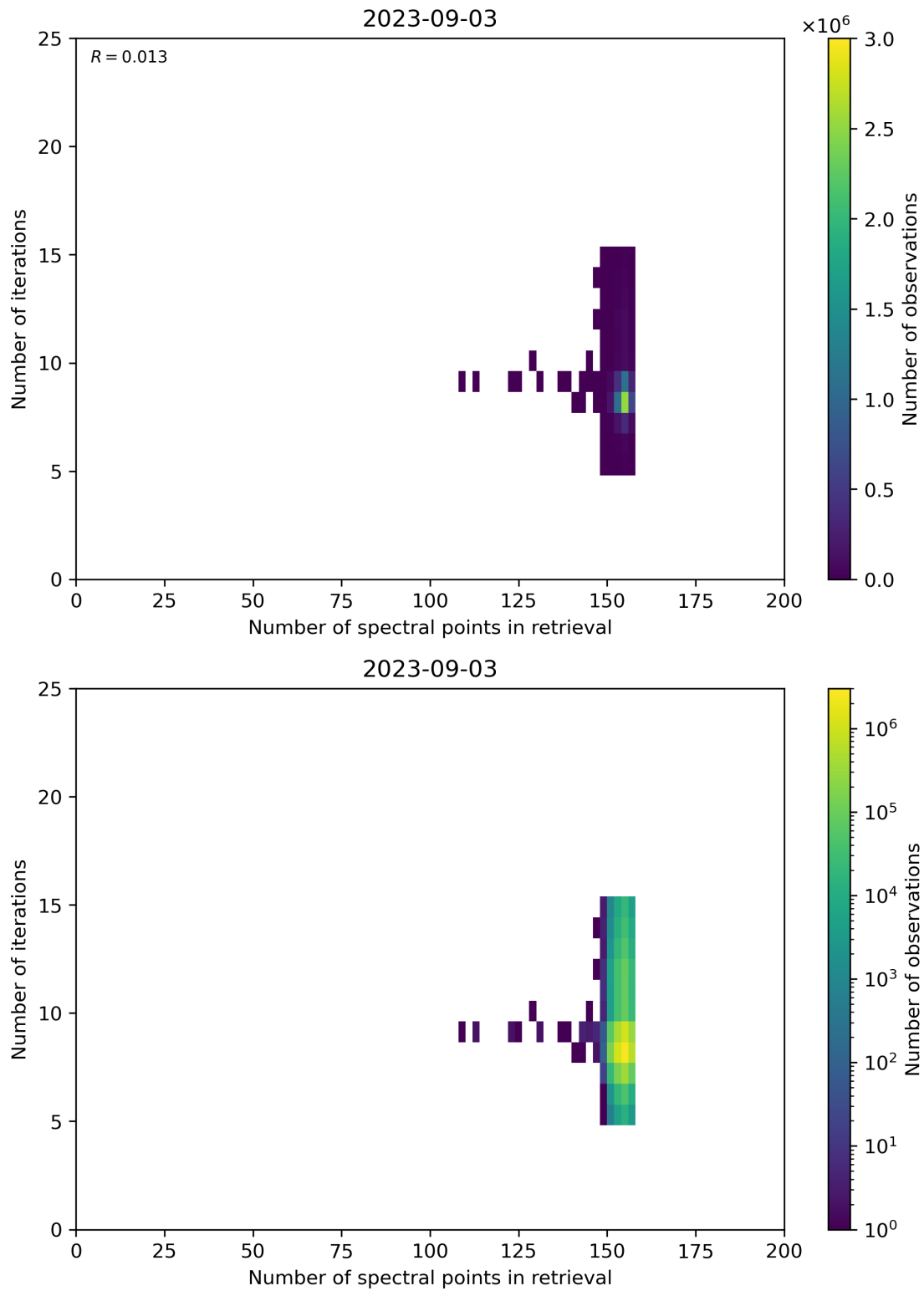
Figure 60: Scatter density plot of “Number of spectral points in retrieval” against “Number of iterations” for 2023-09-02 to 2023-09-04.
