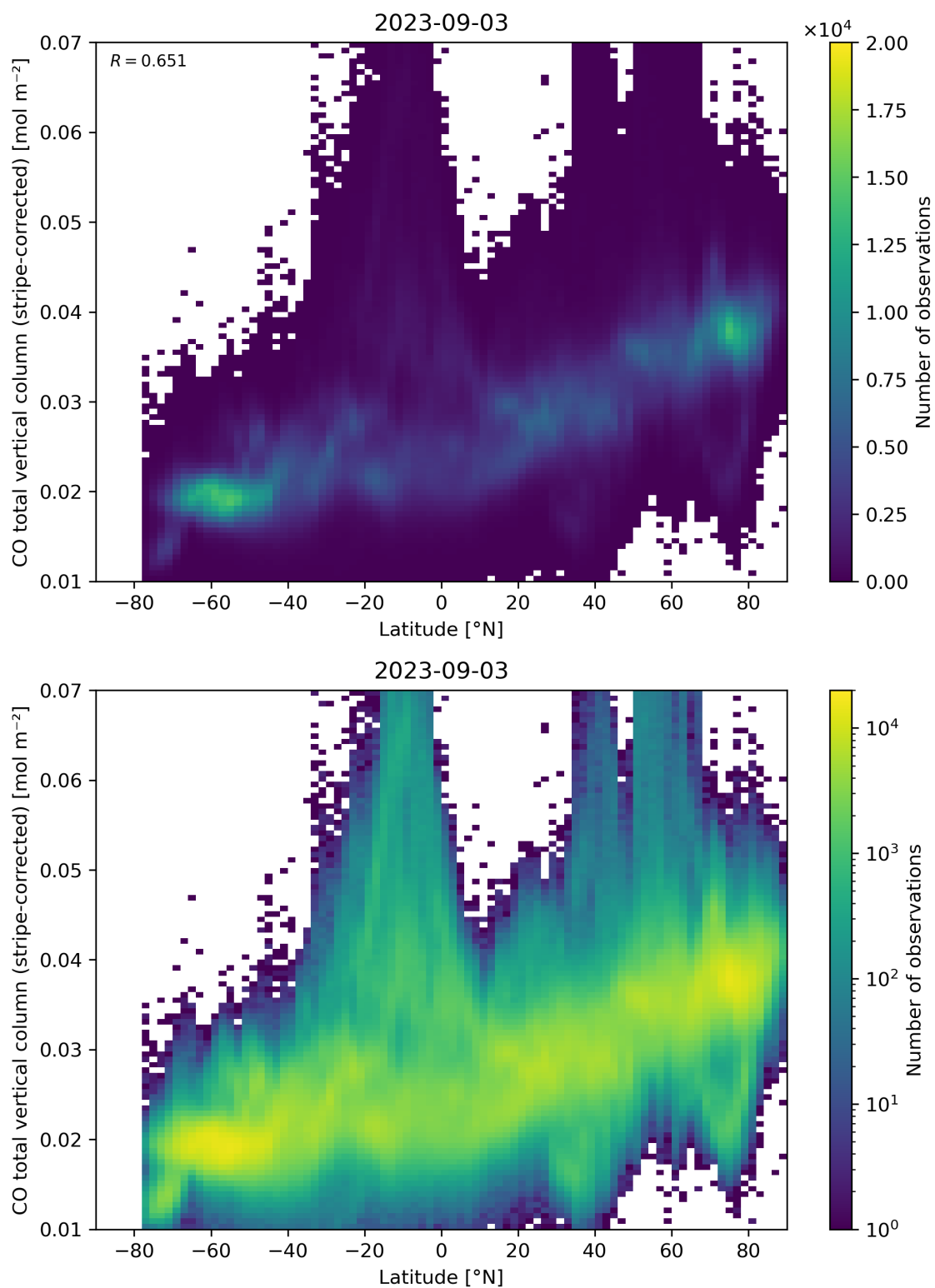
Figure 52: Scatter density plot of “Latitude” against “CO total vertical column (stripe-corrected)” for 2023-09-02 to 2023-09-04.
