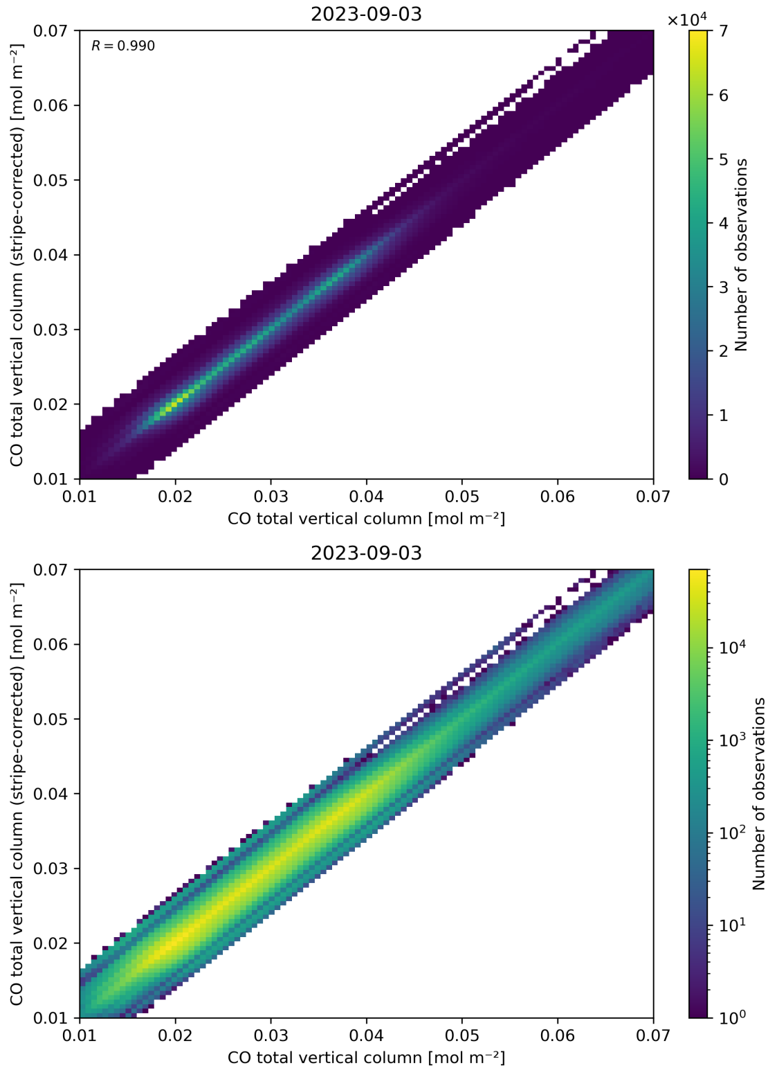
Figure 33: Scatter density plot of “CO total vertical column” against “CO total vertical column (stripe-corrected)” for 2023-09-02 to 2023-09-04.
