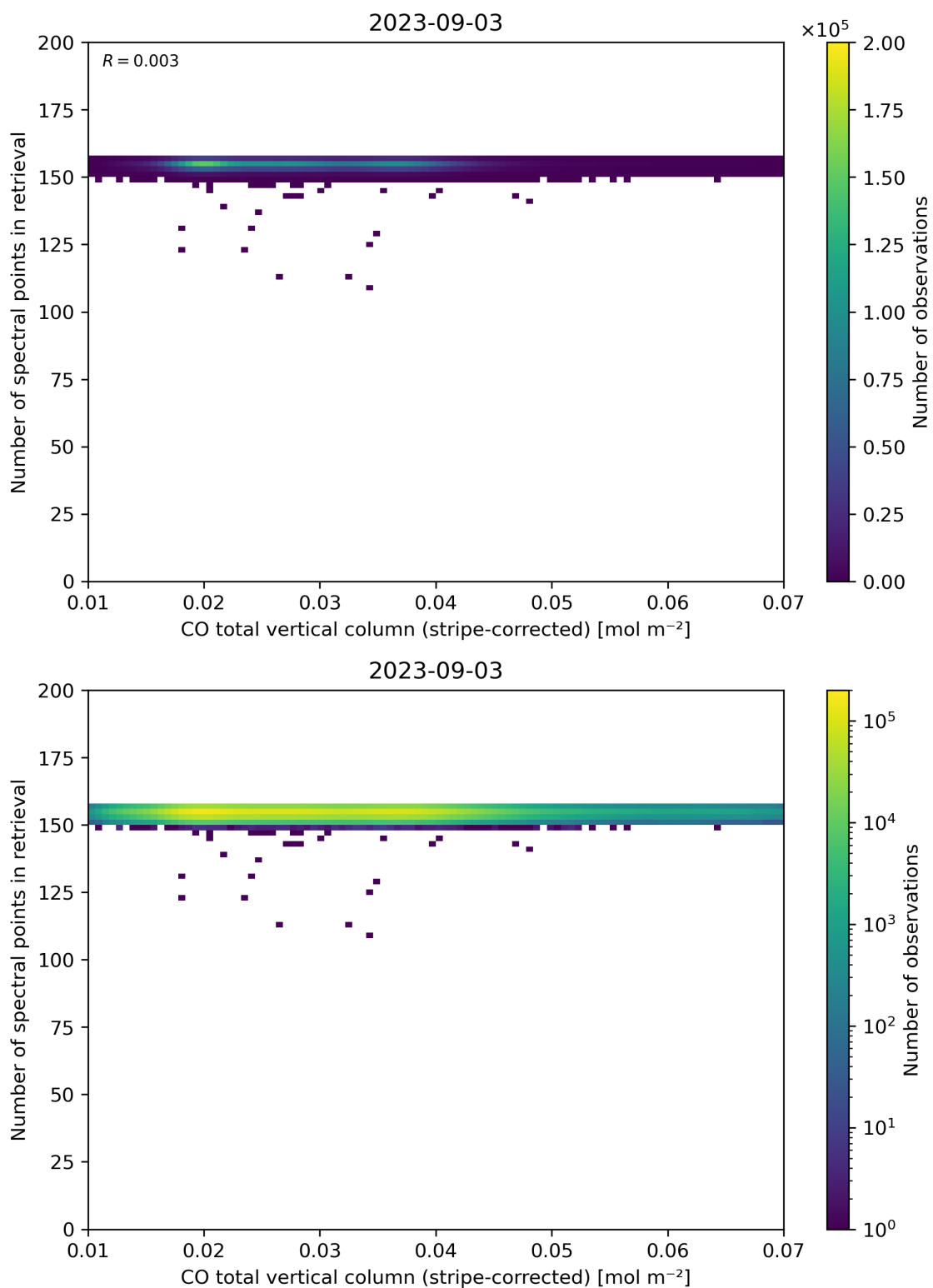
Figure 40: Scatter density plot of “CO total vertical column (stripe-corrected)” against “Number of spectral points in retrieval” for 2023-09-02 to 2023-09-04.
