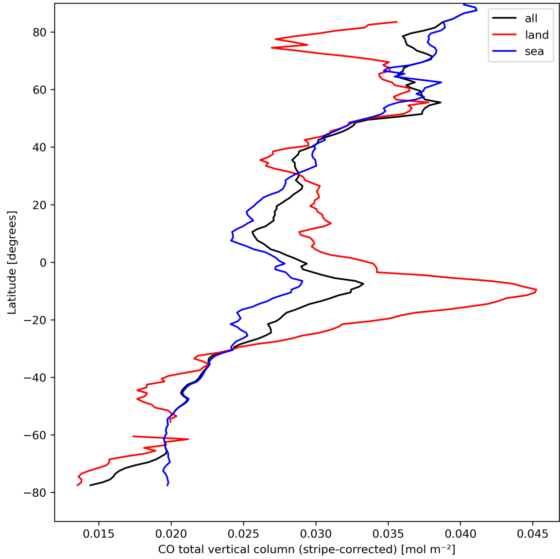
Figure 11: Zonal average of “CO total vertical column (stripe-corrected)” for 2023-09-02 to 2023-09-04.
