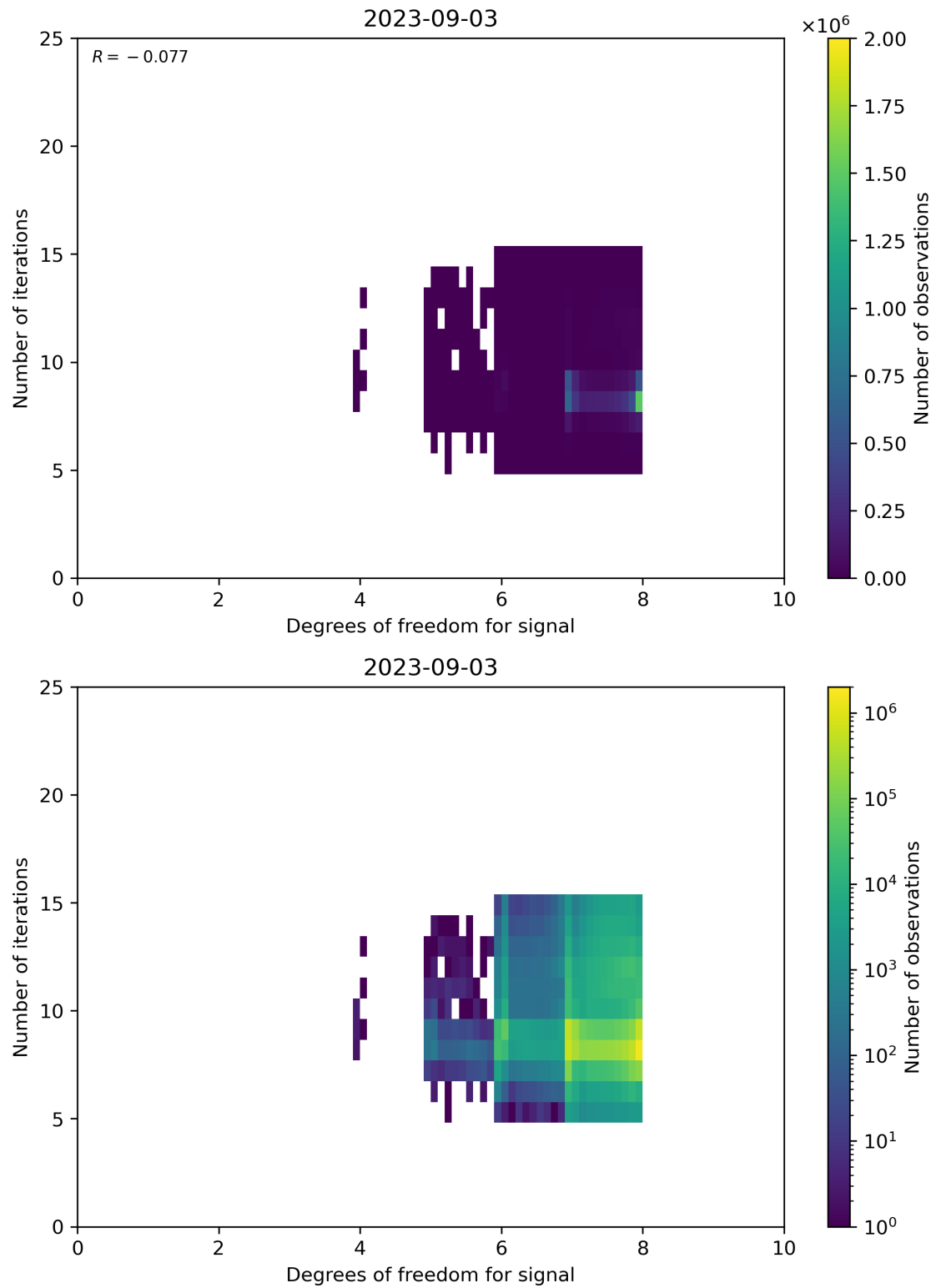
Figure 50: Scatter density plot of “Degrees of freedom for signal” against “Number of iterations” for 2023-09-02 to 2023-09-04.
