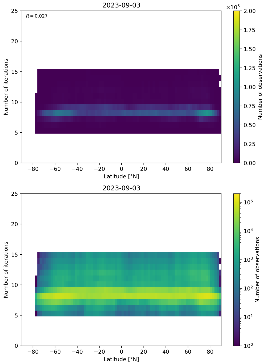
Figure 56: Scatter density plot of “Latitude” against “Number of iterations” for 2023-09-02 to 2023-09-04.
