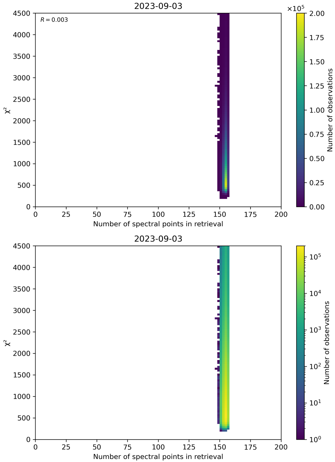
Figure 58: Scatter density plot of “Number of spectral points in retrieval” against “ \chi^2 ” for 2023-09-02 to 2023-09-04.
