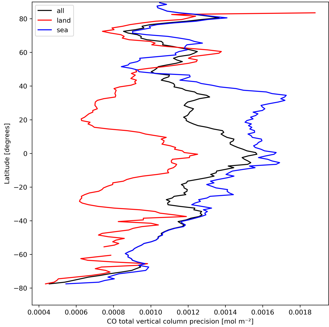
Figure 12: Zonal average of “CO total vertical column precision” for 2023-09-02 to 2023-09-04.
