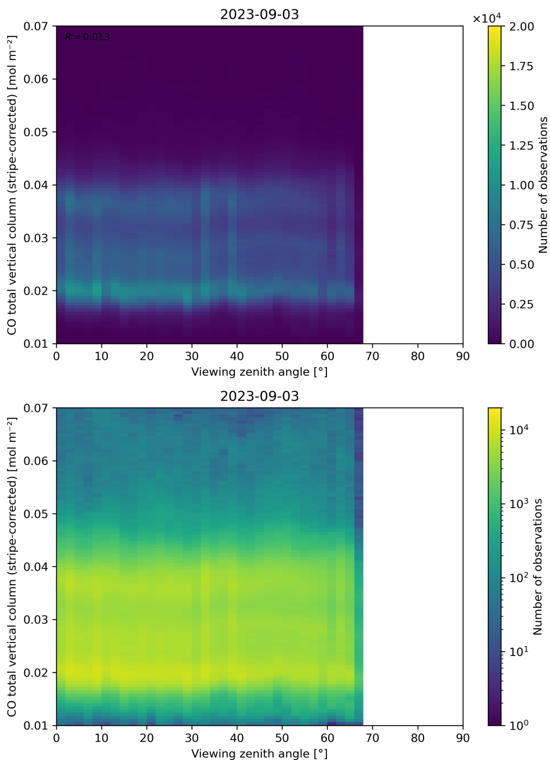
Figure 70: Scatter density plot of “Viewing zenith angle” against “CO total vertical column (stripe-corrected)” for 2023-09-02 to 2023-09-04.
