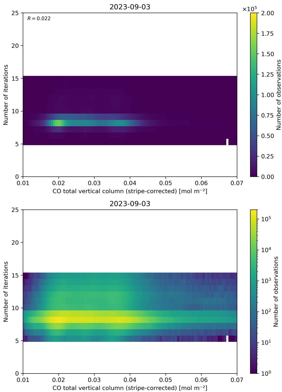
Figure 39: Scatter density plot of “CO total vertical column (stripe-corrected)” against “Number of iterations” for 2023-09-02 to 2023-09-04.
