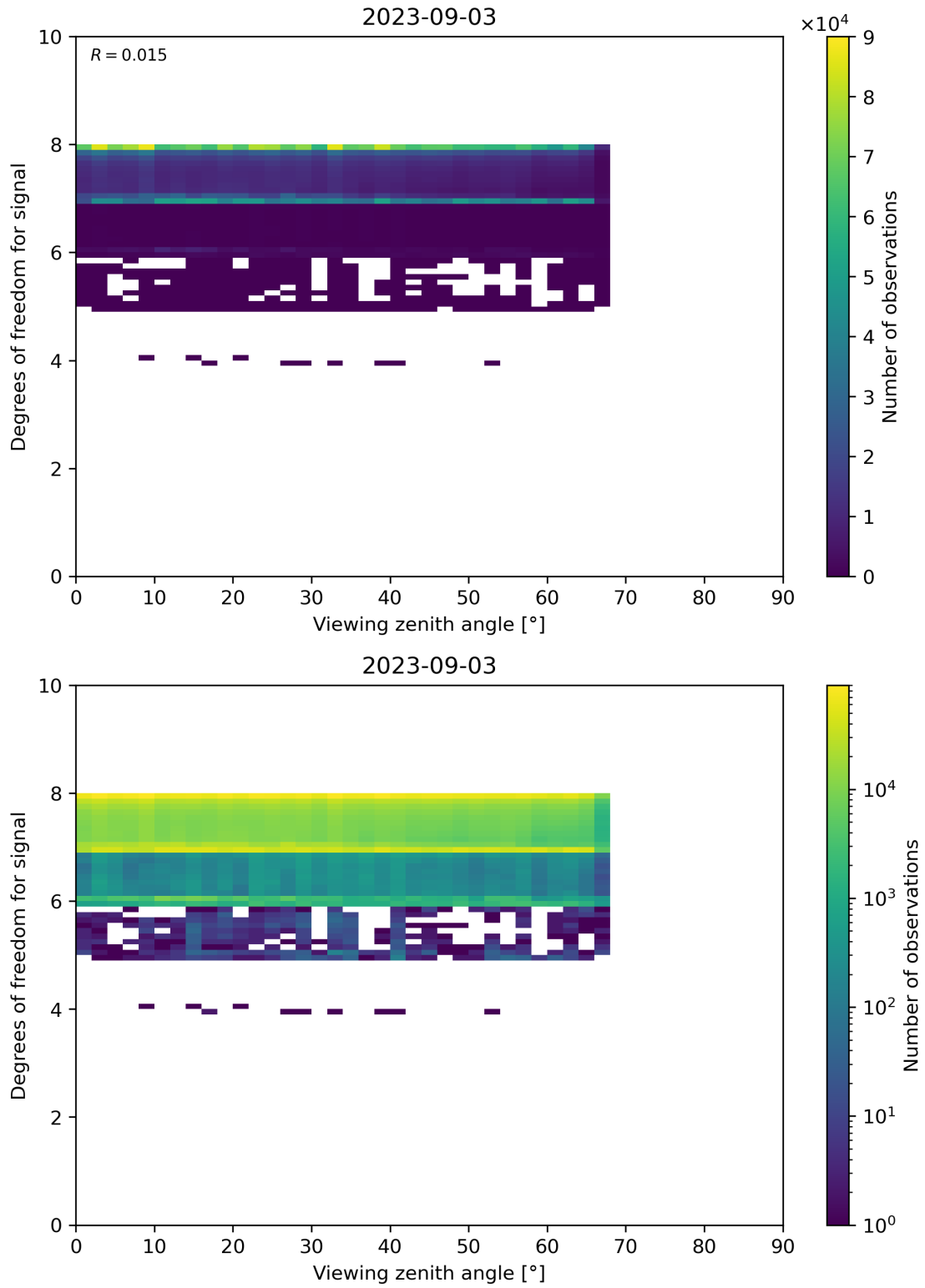
Figure 73: Scatter density plot of “Viewing zenith angle” against “Degrees of freedom for signal” for 2023-09-02 to 2023-09-04.
