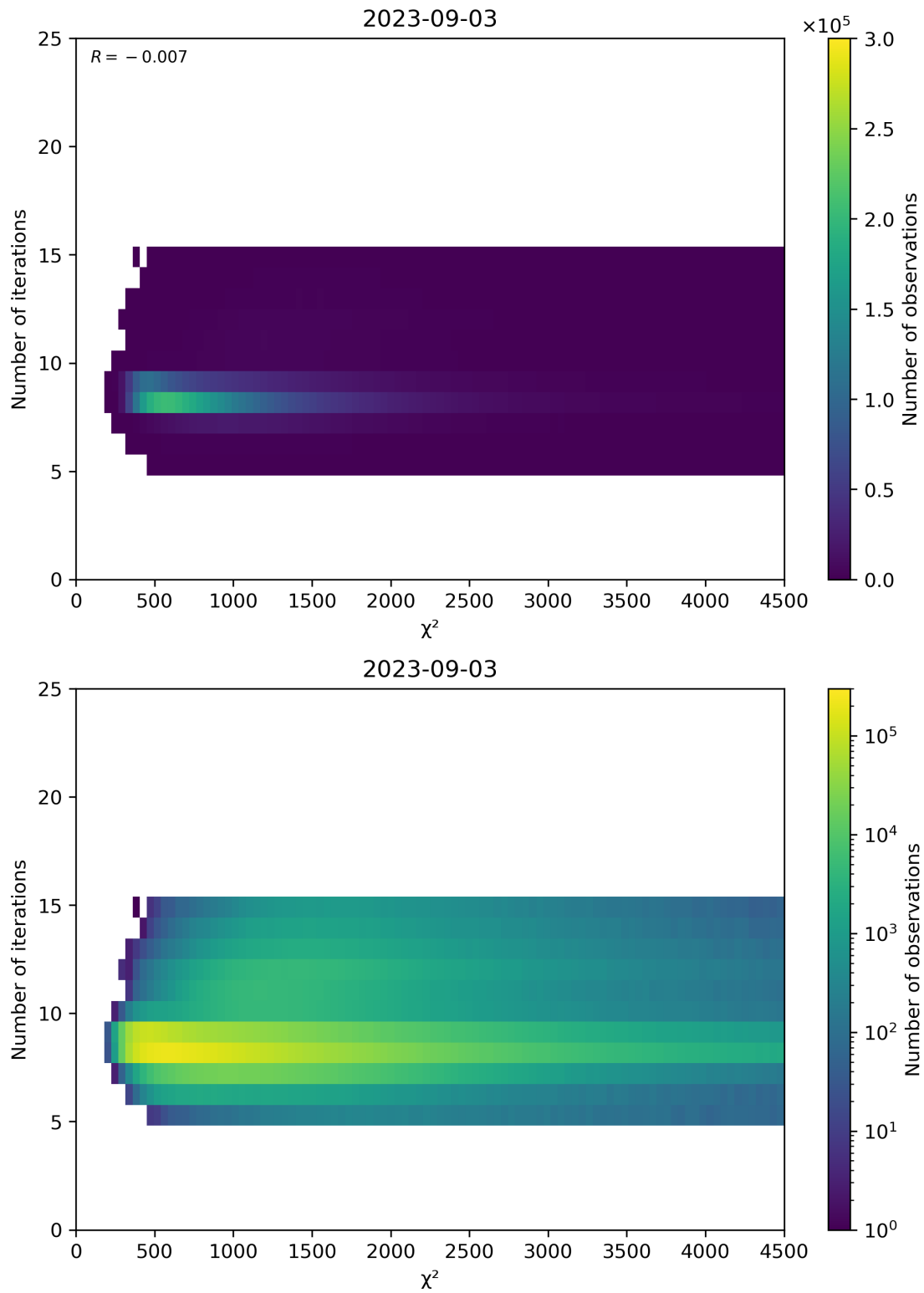
Figure 49: Scatter density plot of “ \chi^2 ” against “Number of iterations” for 2023-09-02 to 2023-09-04.
