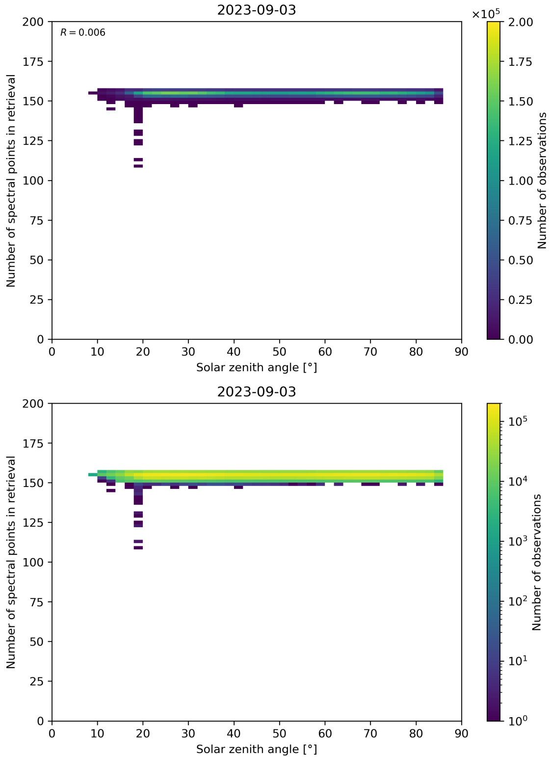
Figure 68: Scatter density plot of “Solar zenith angle” against “Number of spectral points in retrieval” for 2023-09-02 to 2023-09-04.
