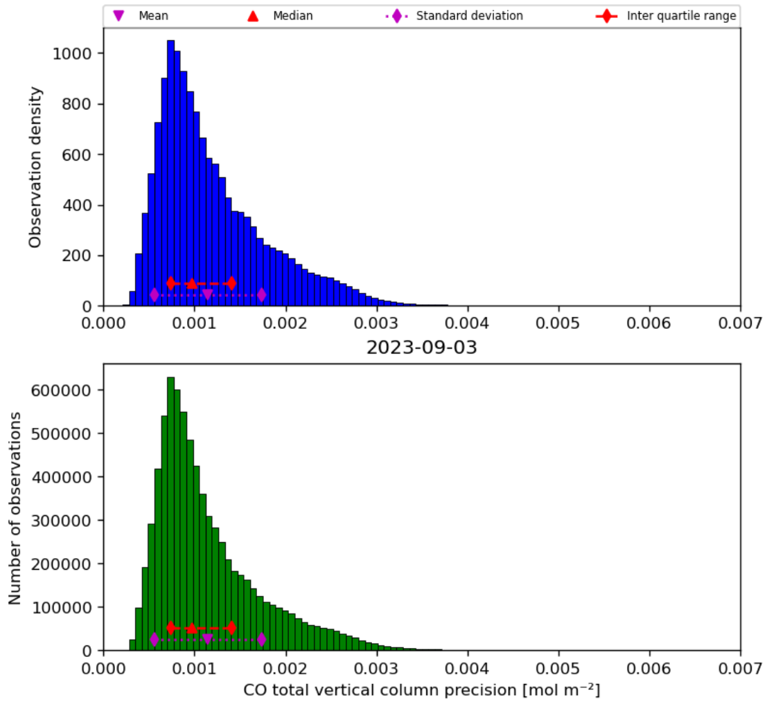
Figure 20: Histogram of “CO total vertical column precision” for 2023-09-02 to 2023-09-04
