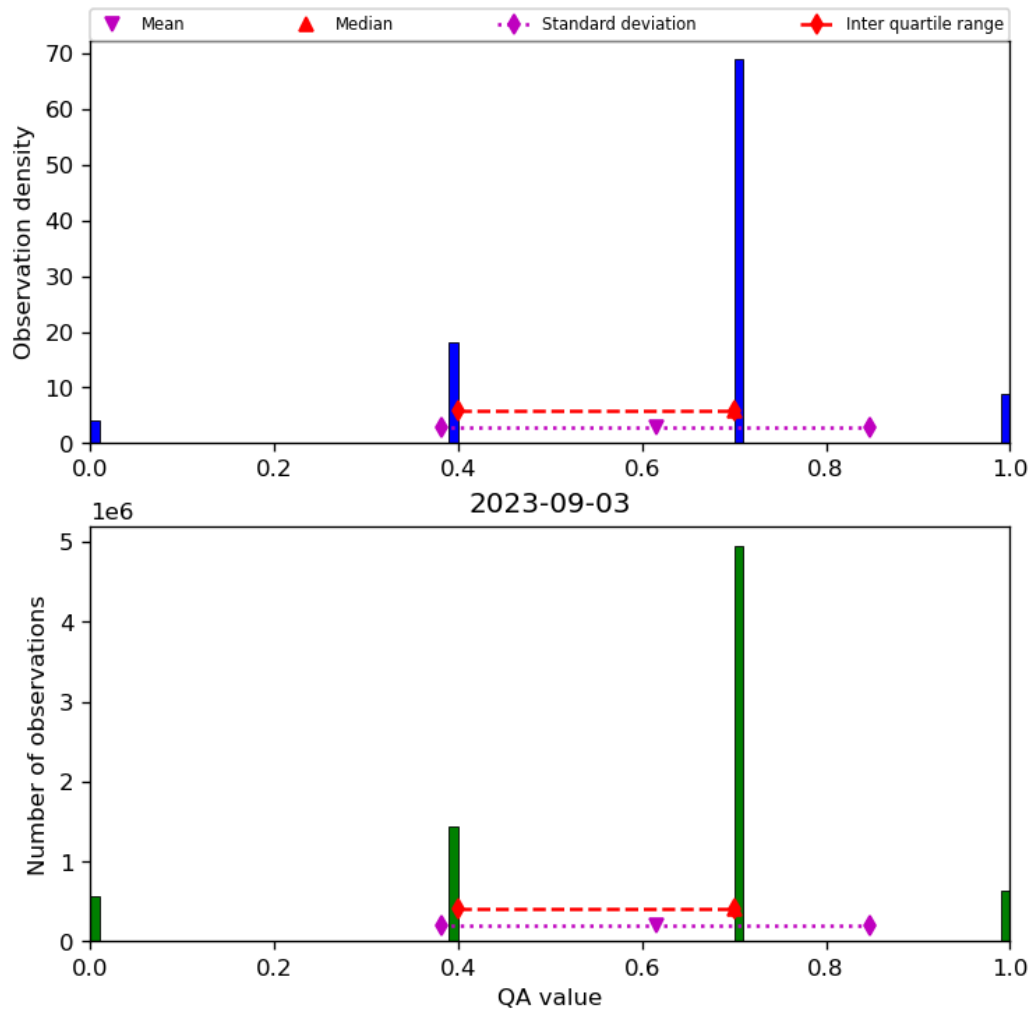
Figure 17: Histogram of “QA value” for 2023-09-02 to 2023-09-04
