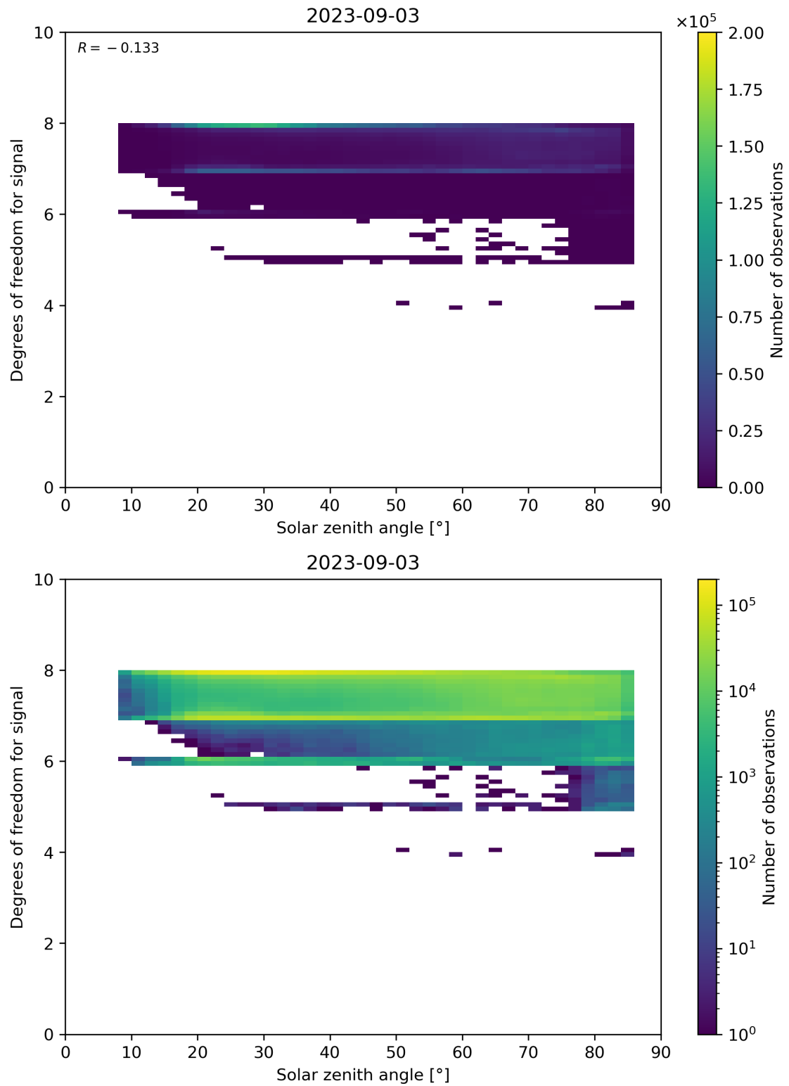
Figure 65: Scatter density plot of “Solar zenith angle” against “Degrees of freedom for signal” for 2023-09-02 to 2023-09-04.
