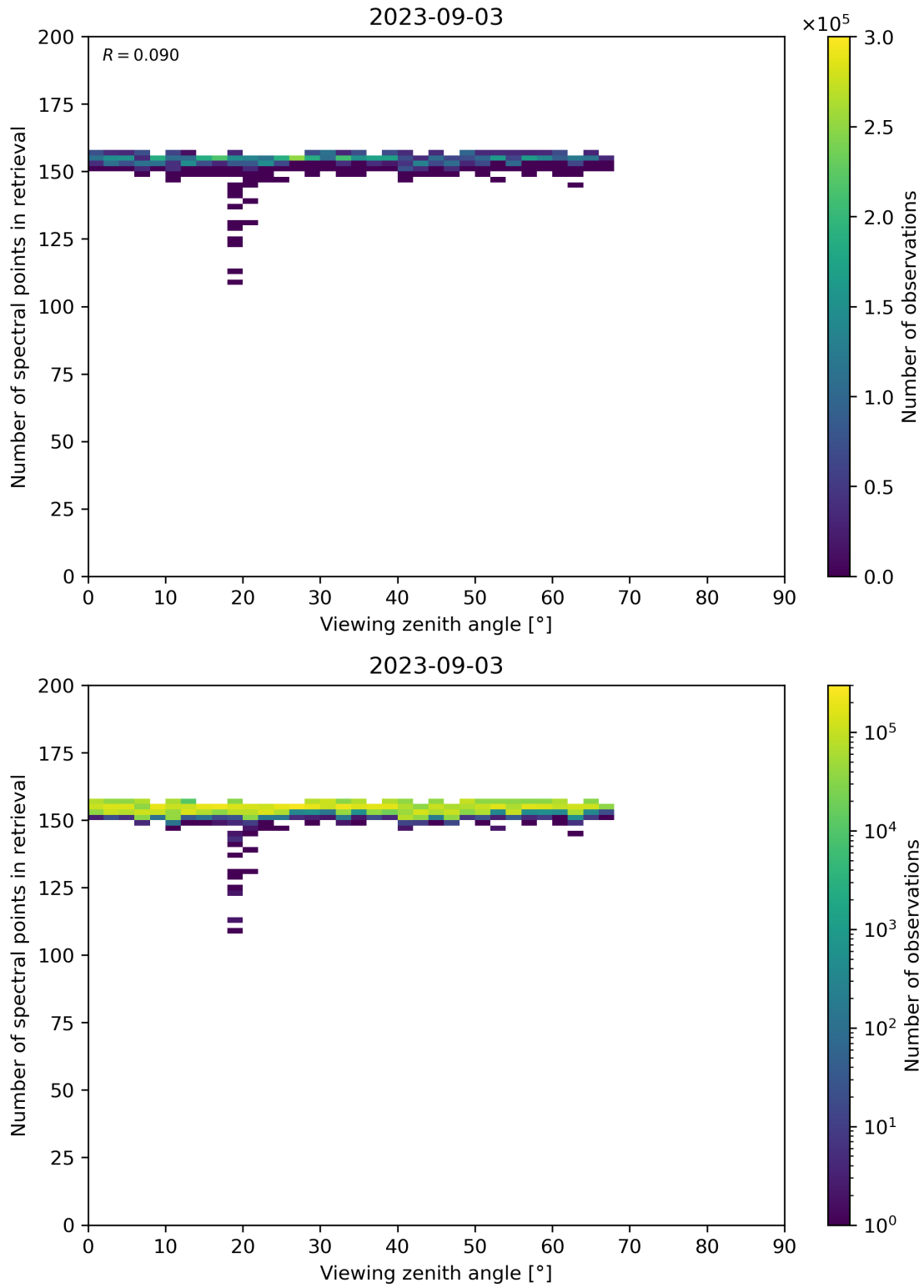
Figure 76: Scatter density plot of “Viewing zenith angle” against “Number of spectral points in retrieval” for 2023-09-02 to 2023-09-04.
