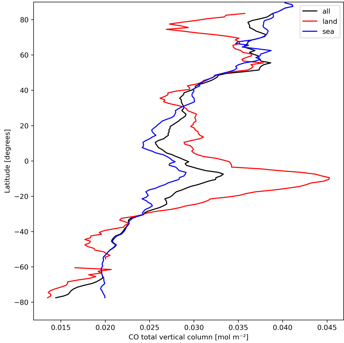
Figure 10: Zonal average of “CO total vertical column” for 2023-09-02 to 2023-09-04.
