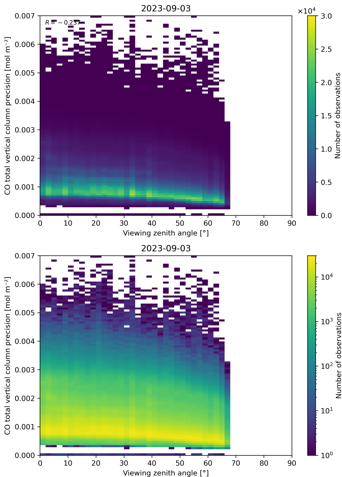
Figure 71: Scatter density plot of “Viewing zenith angle” against “CO total vertical column precision” for 2023-09-02 to 2023-09-04.
