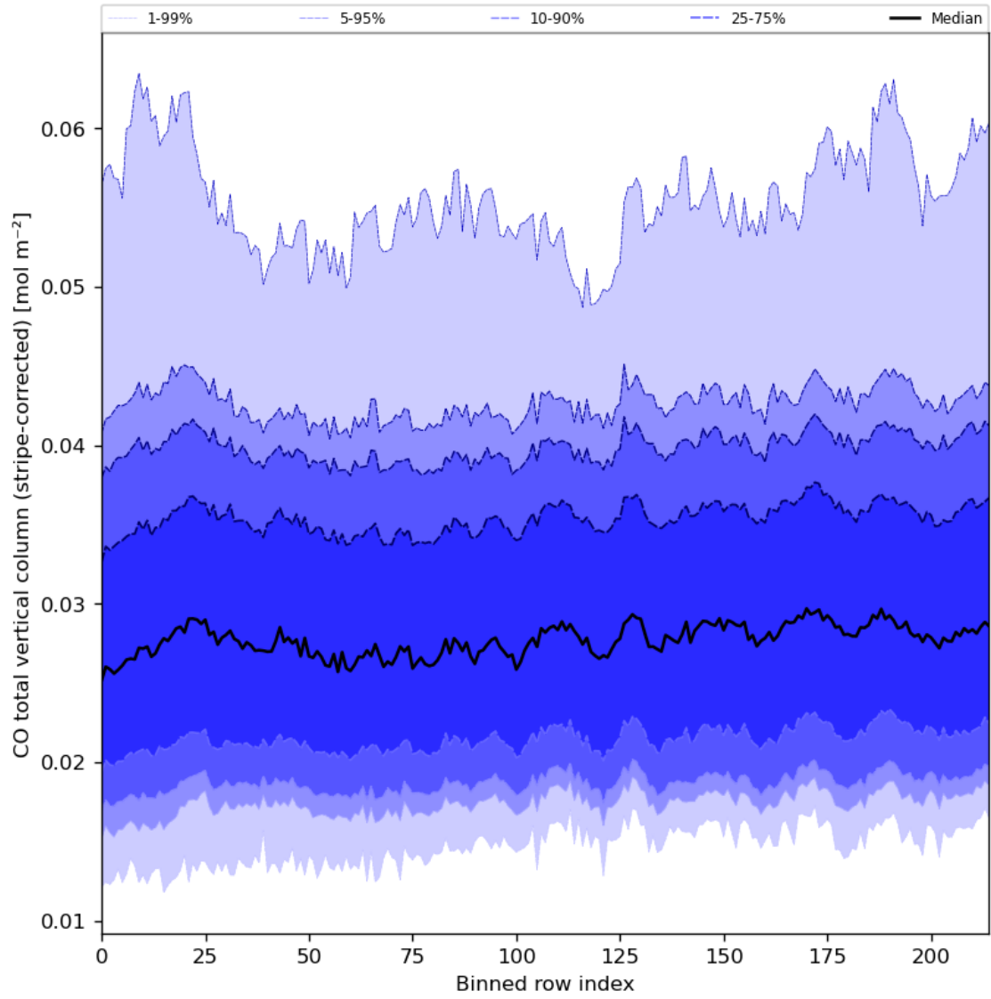
Figure 27: Along track statistics of “CO total vertical column (stripe-corrected)” for 2023-09-02 to 2023-09-04
