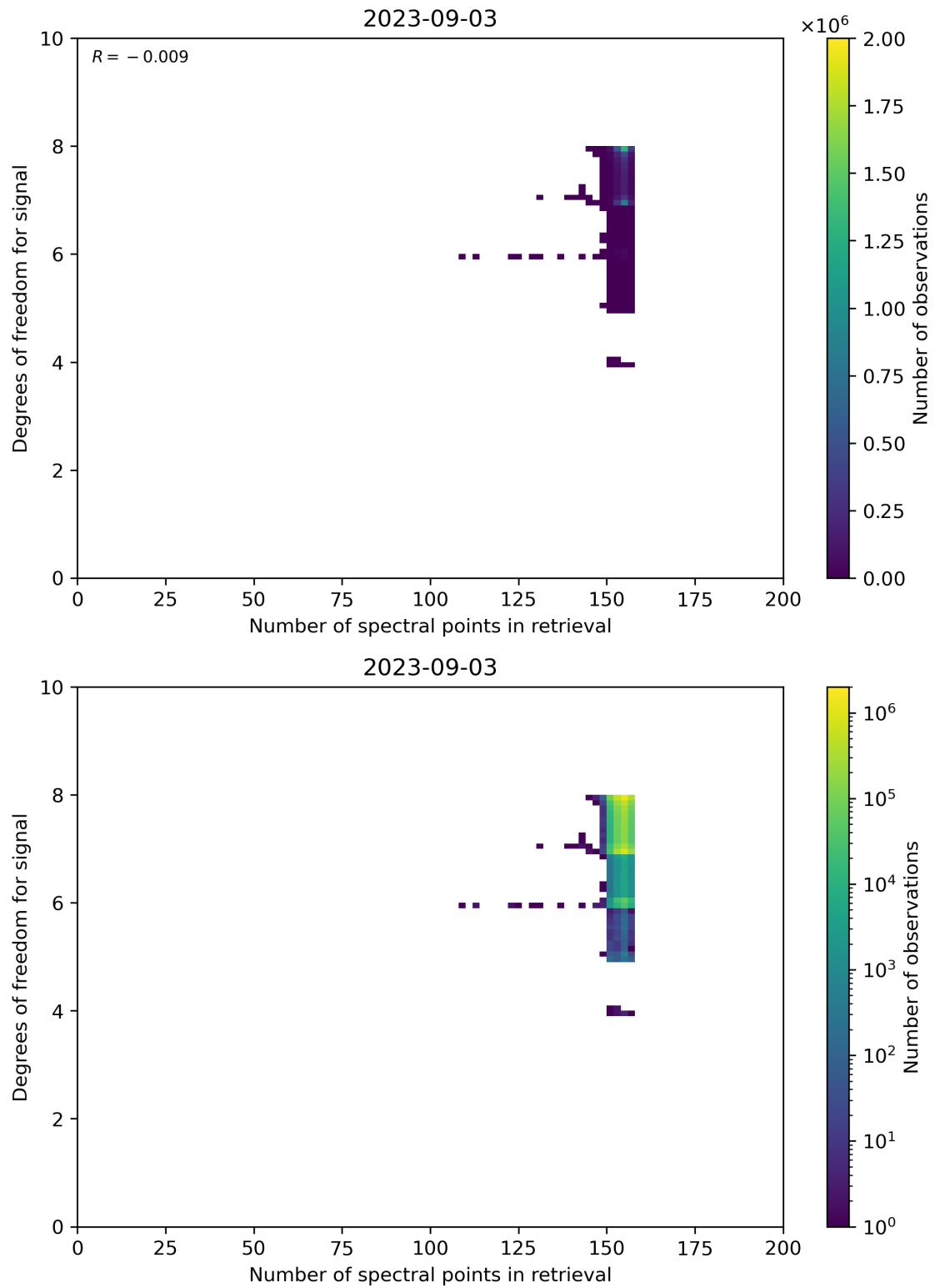
Figure 59: Scatter density plot of “Number of spectral points in retrieval” against “Degrees of freedom for signal” for 2023-09-02 to 2023-09-04.
