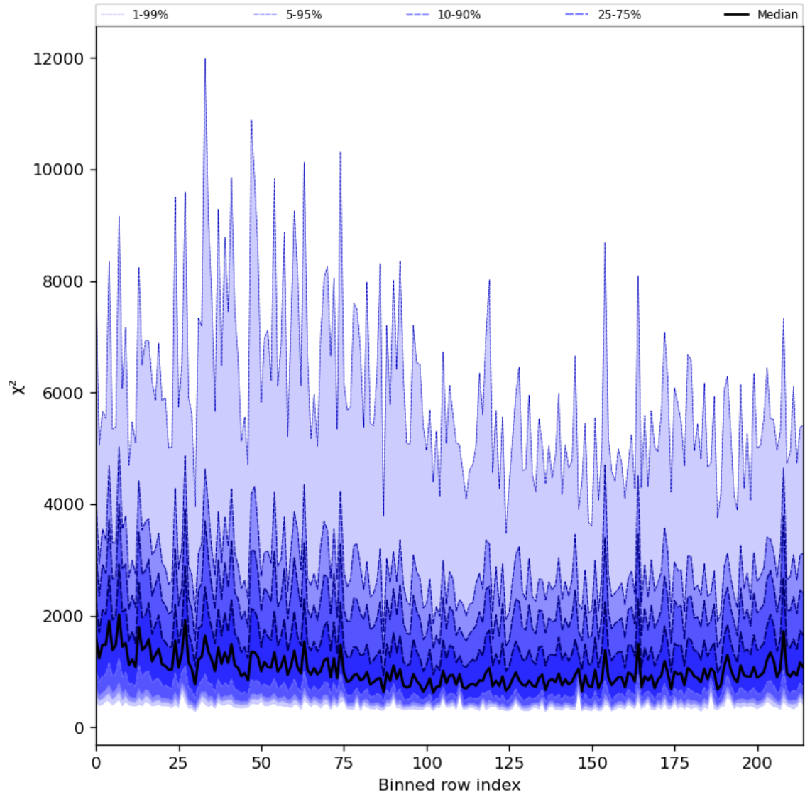
Figure 30: Along track statistics of “ \chi^2 ” for 2023-09-02 to 2023-09-04
