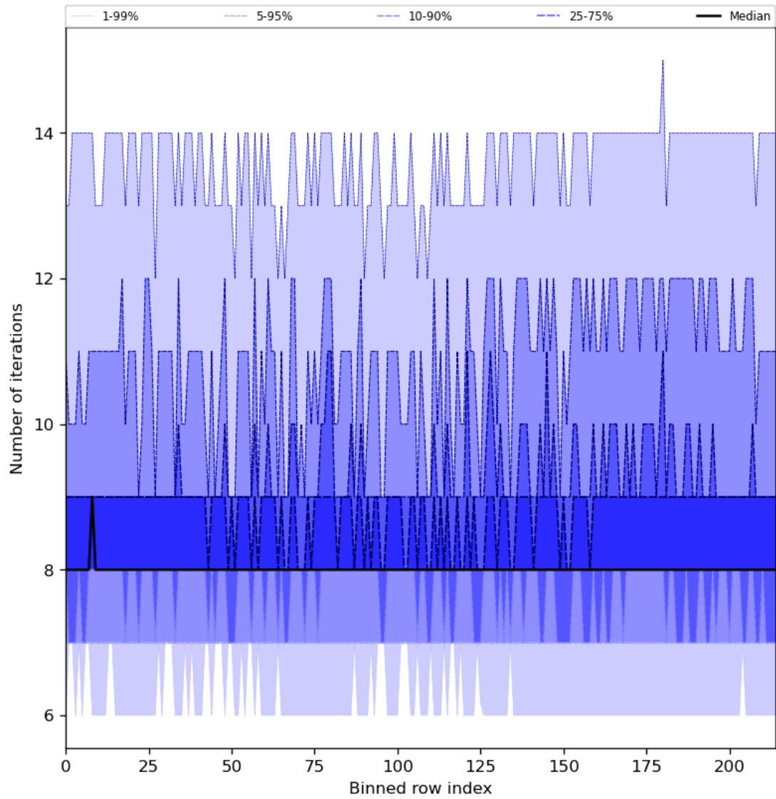
Figure 32: Along track statistics of “Number of iterations” for 2023-09-02 to 2023-09-04
