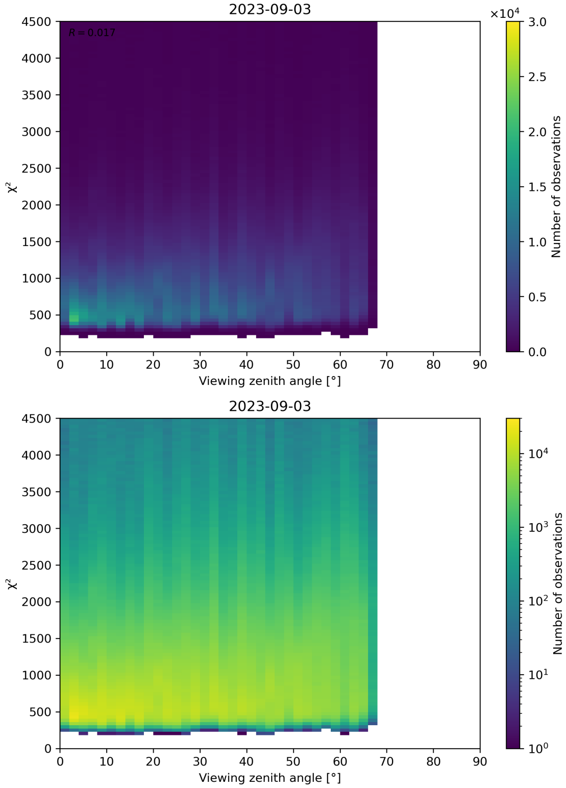
Figure 72: Scatter density plot of “Viewing zenith angle” against “ \chi^2 ” for 2023-09-02 to 2023-09-04.
