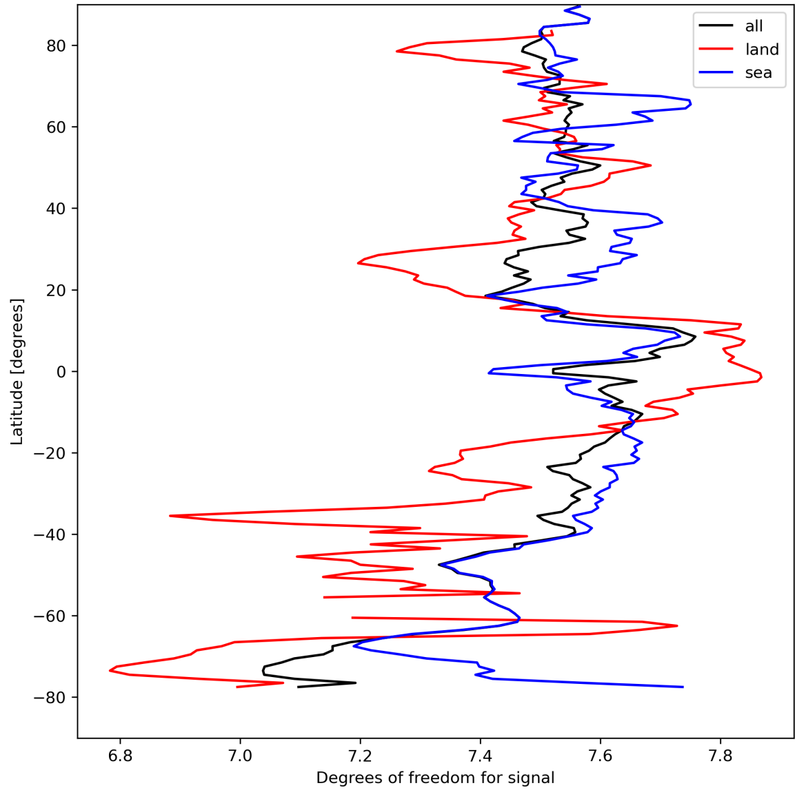
Figure 15: Zonal average of “Degrees of freedom for signal” for 2023-09-02 to 2023-09-04.
