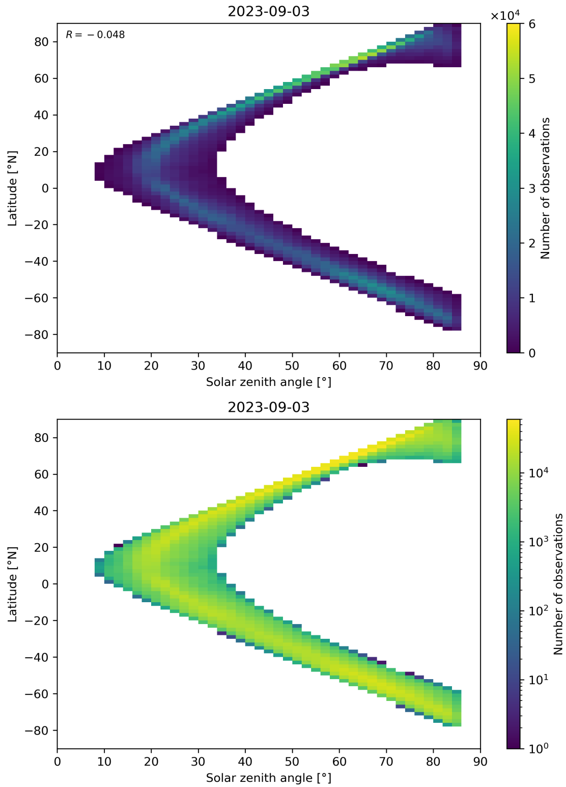
Figure 66: Scatter density plot of “Solar zenith angle” against “Latitude” for 2023-09-02 to 2023-09-04.
