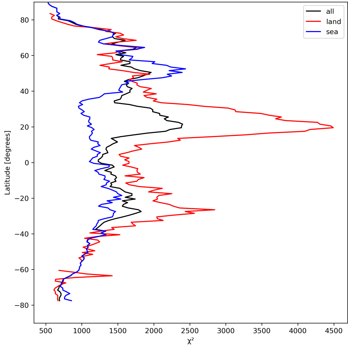
Figure 14: Zonal average of “ \chi^2 ” for 2023-09-02 to 2023-09-04.
