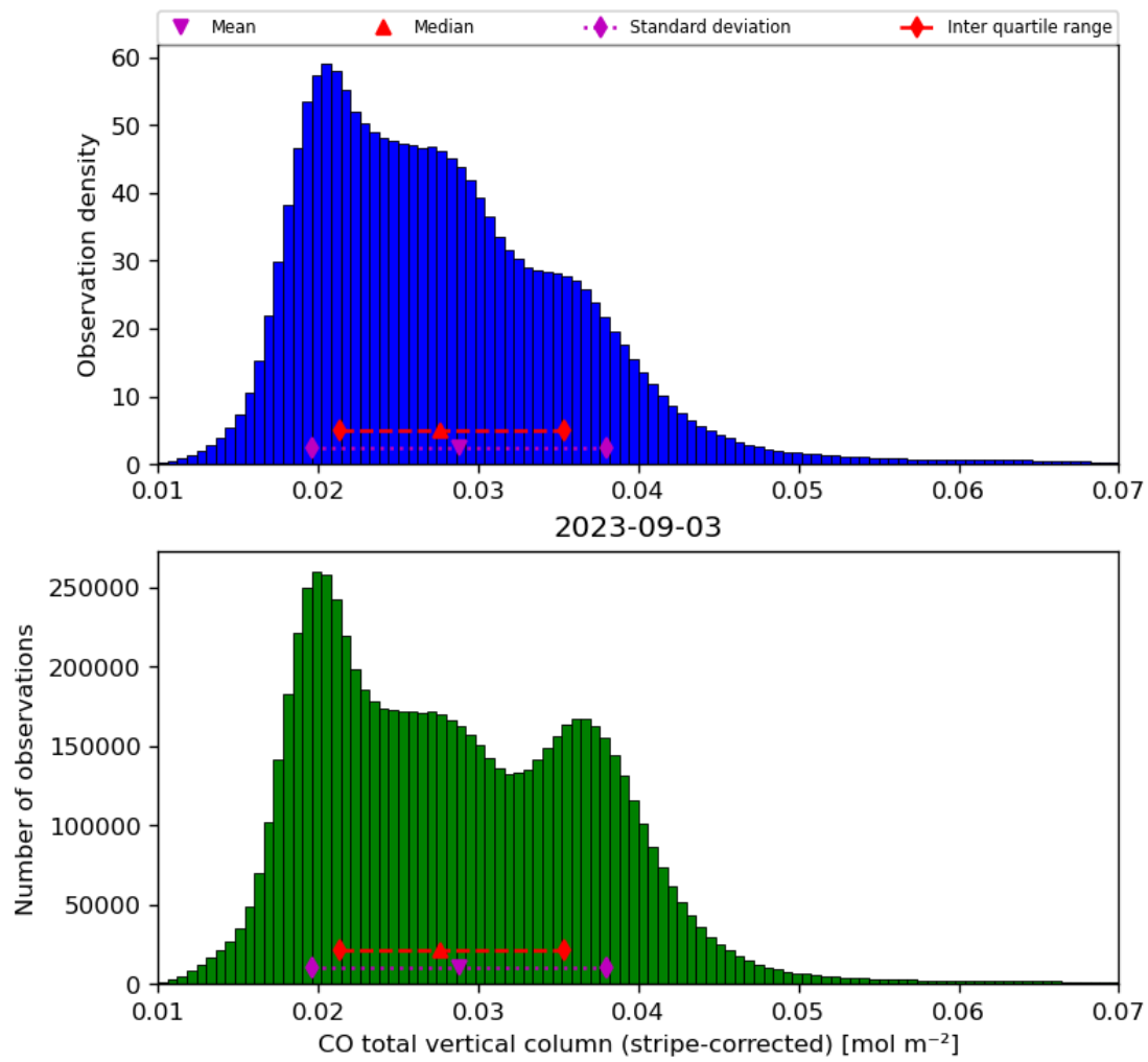
Figure 19: Histogram of “CO total vertical column (stripe-corrected)” for 2023-09-02 to 2023-09-04
