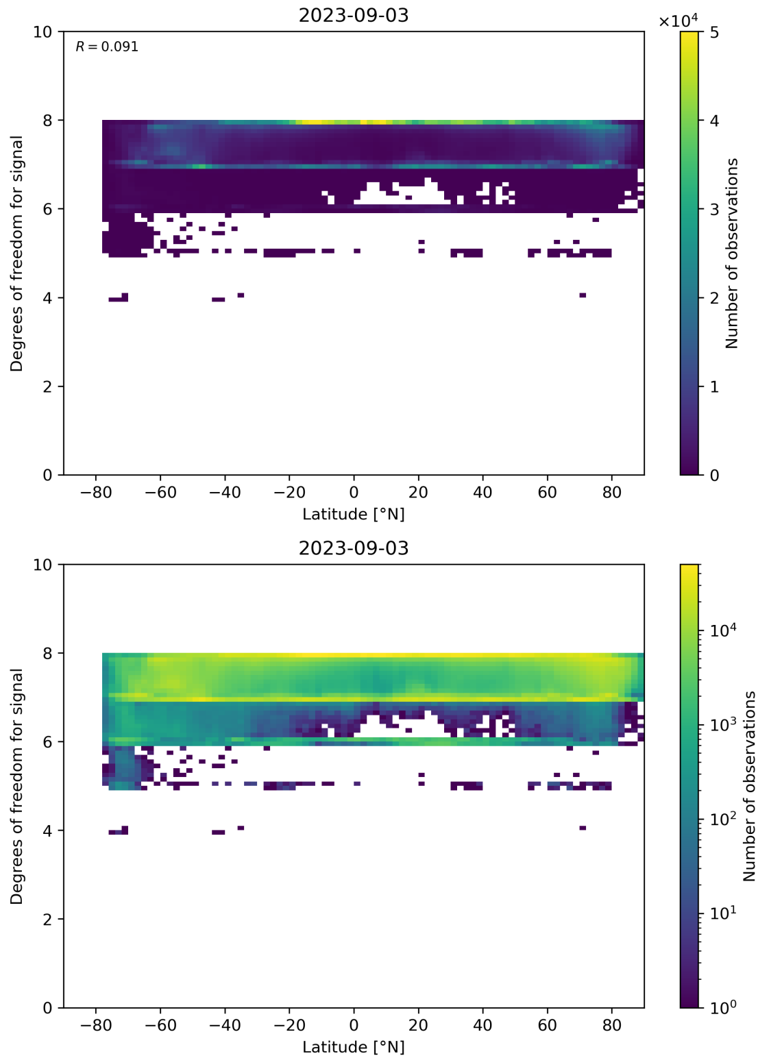
Figure 55: Scatter density plot of “Latitude” against “Degrees of freedom for signal” for 2023-09-02 to 2023-09-04.
