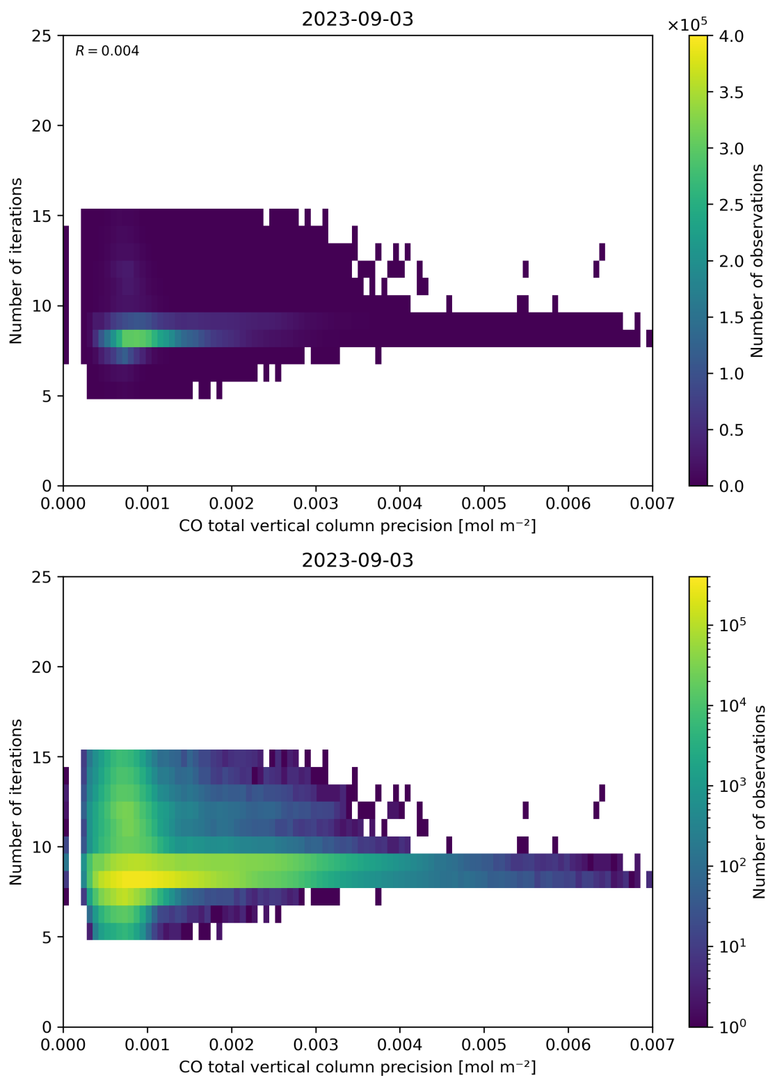
Figure 46: Scatter density plot of “CO total vertical column precision” against “Number of iterations” for 2023-09-02 to 2023-09-04.
