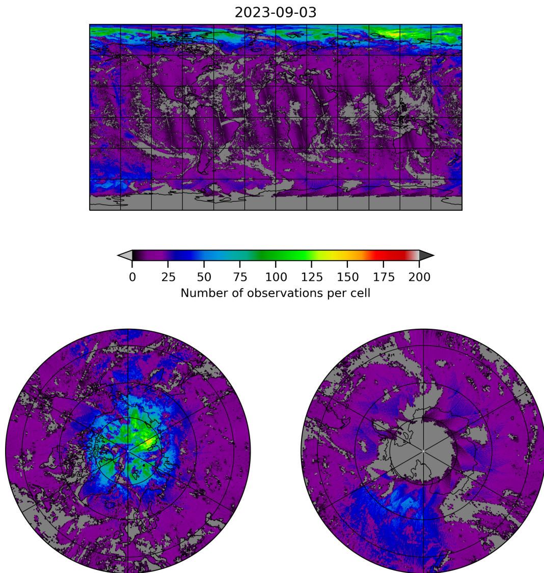
Figure 8: Map of the number of observations for 2023-09-02 to 2023-09-04
