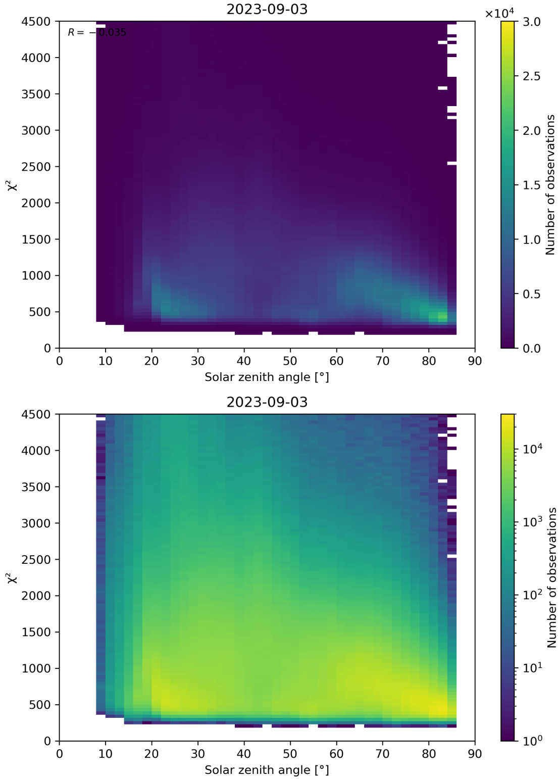
Figure 64: Scatter density plot of “Solar zenith angle” against “ \chi^2 ” for 2023-09-02 to 2023-09-04.
