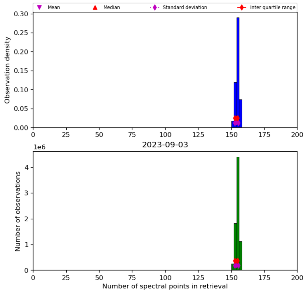
Figure 21: Histogram of “Number of spectral points in retrieval” for 2023-09-02 to 2023-09-04
