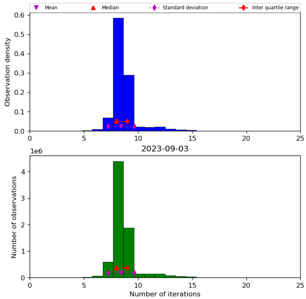
Figure 24: Histogram of “Number of iterations” for 2023-09-02 to 2023-09-04
