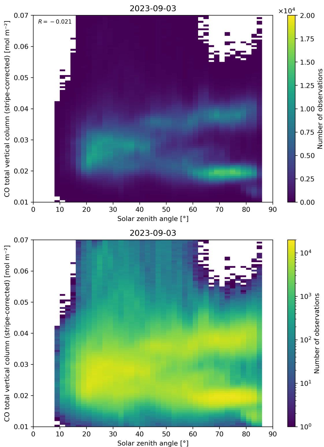
Figure 62: Scatter density plot of “Solar zenith angle” against “CO total vertical column (stripe-corrected)” for 2023-09-02 to 2023-09-04.
