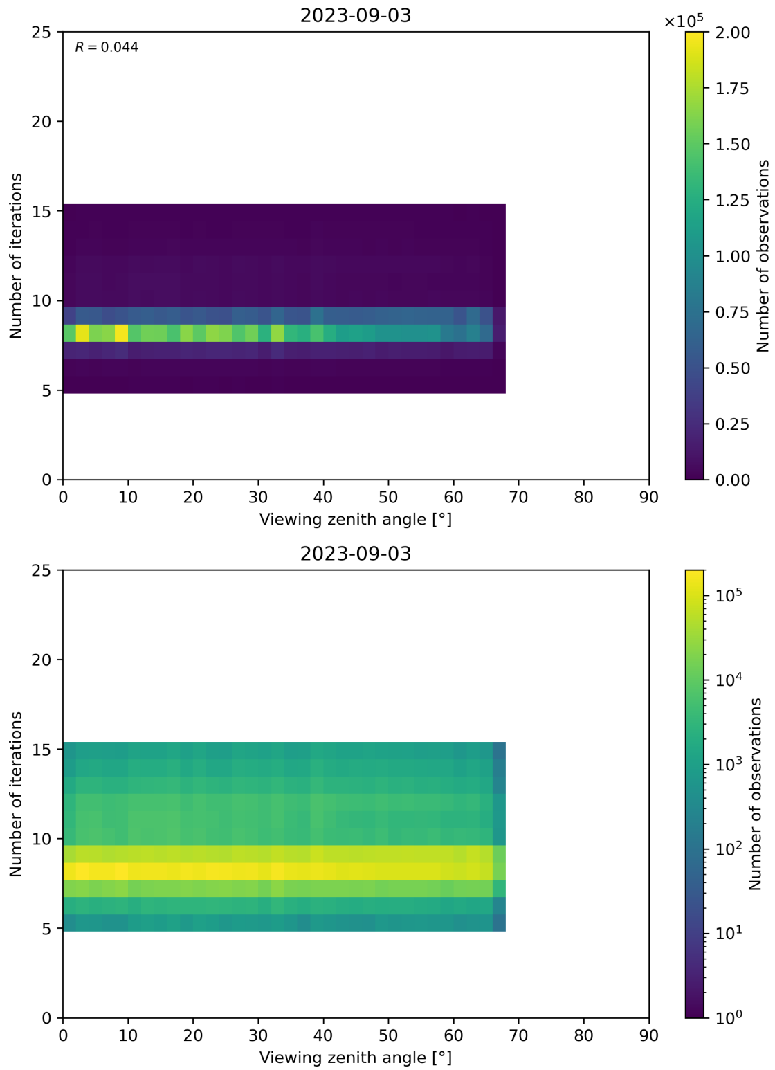
Figure 75: Scatter density plot of “Viewing zenith angle” against “Number of iterations” for 2023-09-02 to 2023-09-04.
