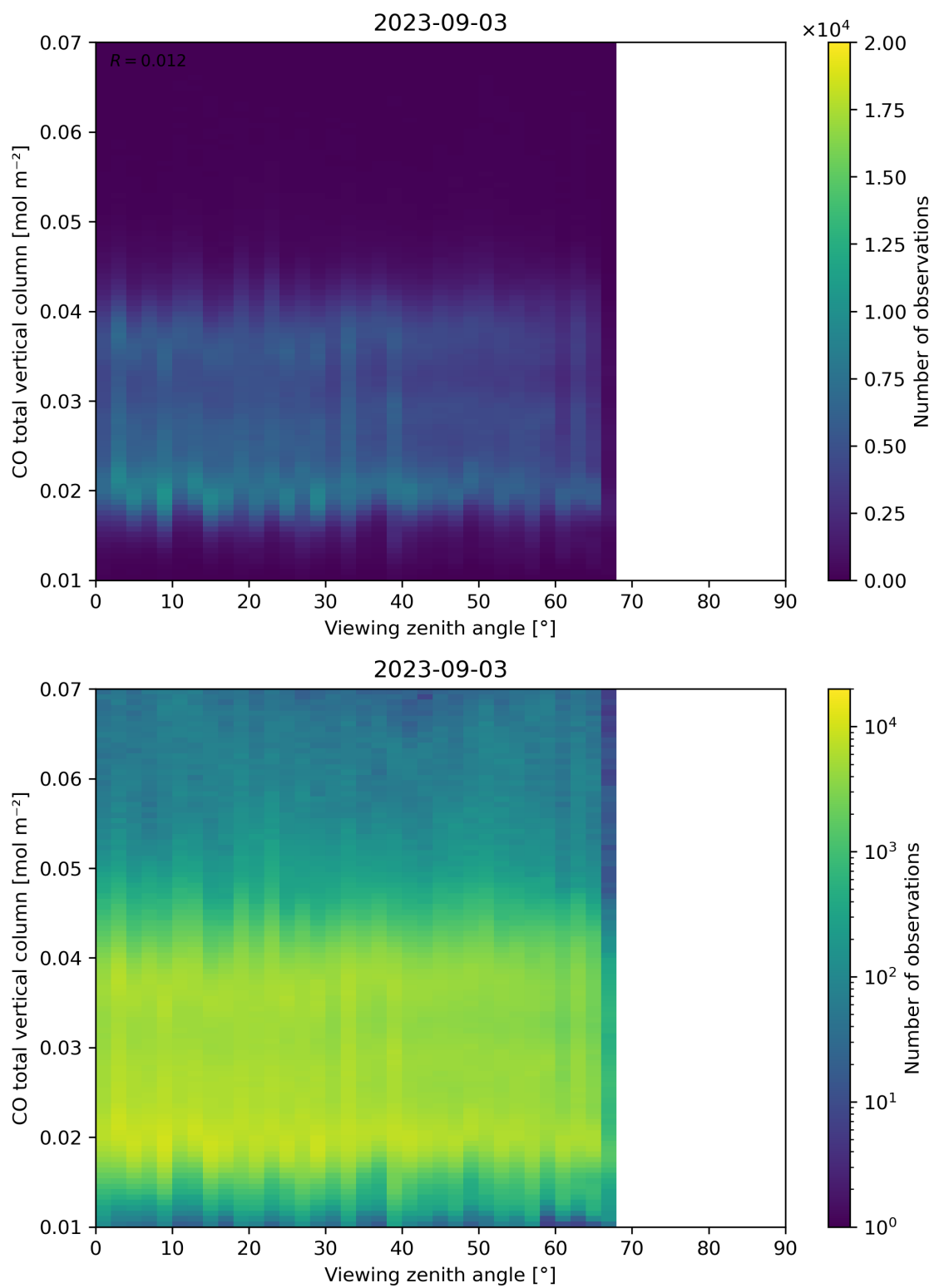
Figure 69: Scatter density plot of “Viewing zenith angle” against “CO total vertical column” for 2023-09-02 to 2023-09-04.
