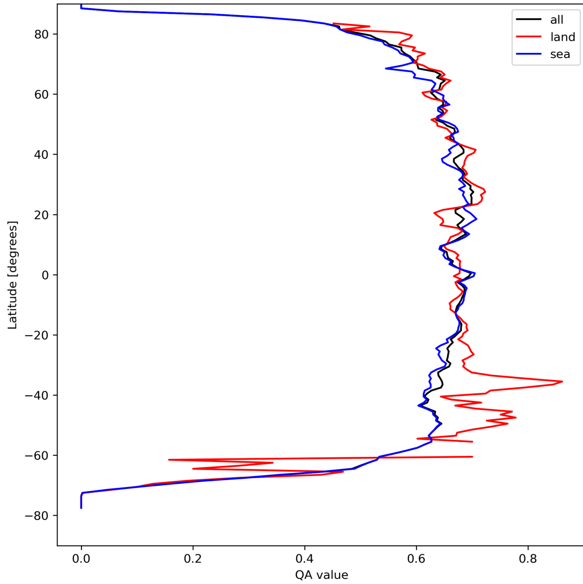
Figure 9: Zonal average of “QA value” for 2023-09-02 to 2023-09-04.
