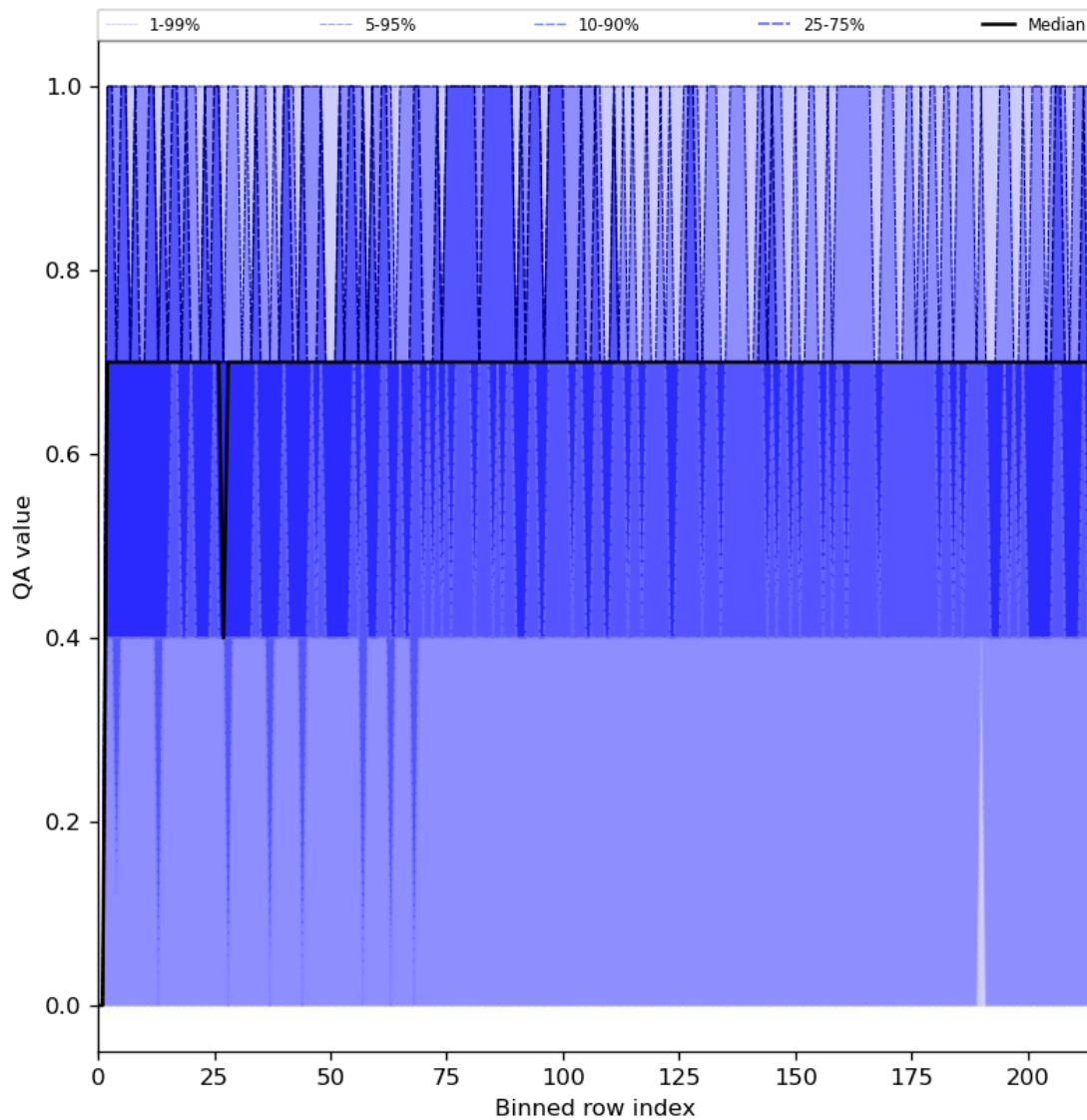
Figure 25: Along track statistics of “QA value” for 2023-09-02 to 2023-09-04
