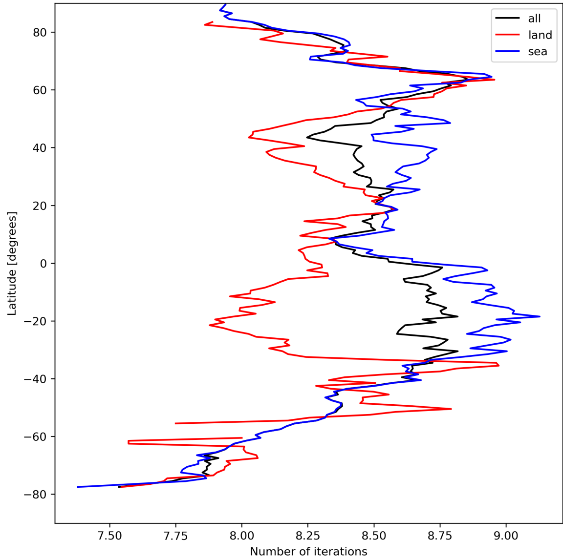
Figure 16: Zonal average of “Number of iterations” for 2023-09-02 to 2023-09-04.
