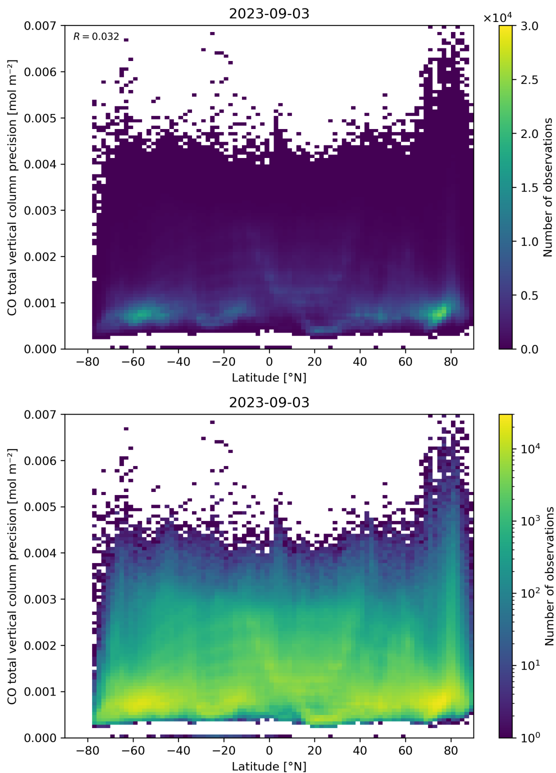
Figure 53: Scatter density plot of “Latitude” against “CO total vertical column precision” for 2023-09-02 to 2023-09-04.
