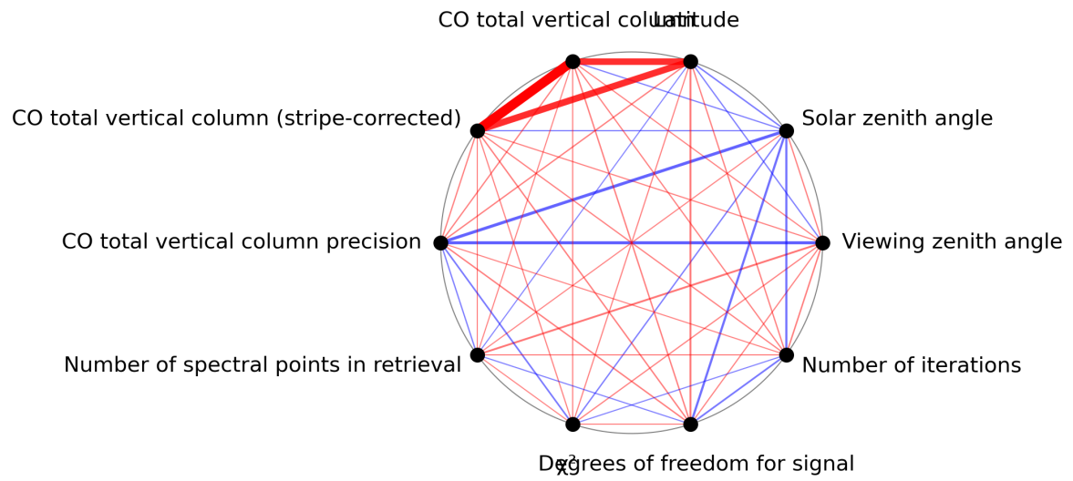
Figure 1: Map of correlation graph for 2023-09-02 to 2023-09-04.
