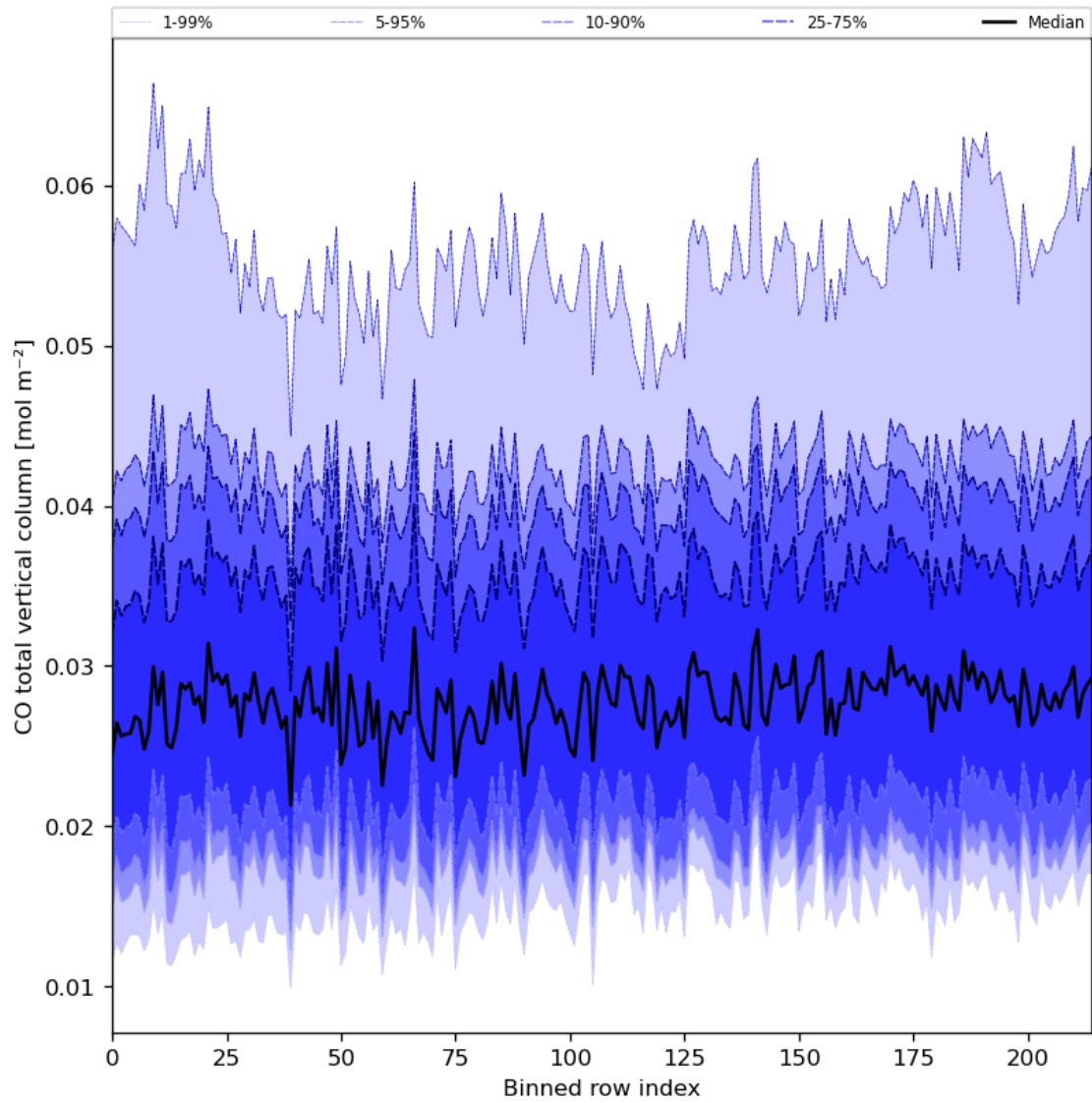
Figure 26: Along track statistics of “CO total vertical column” for 2023-09-02 to 2023-09-04
