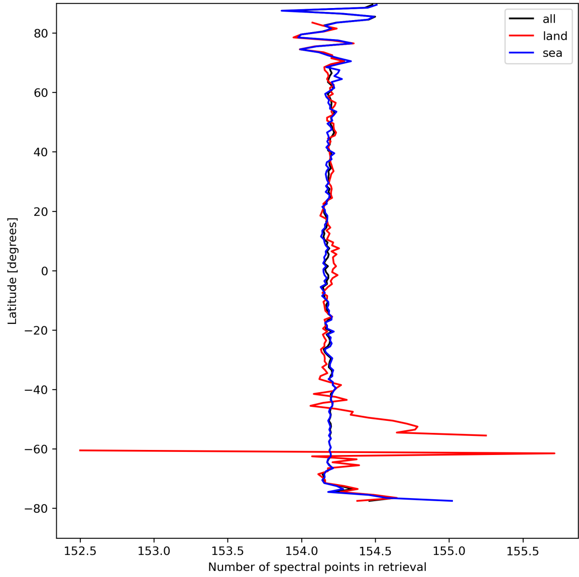
Figure 13: Zonal average of “Number of spectral points in retrieval” for 2023-09-02 to 2023-09-04.
