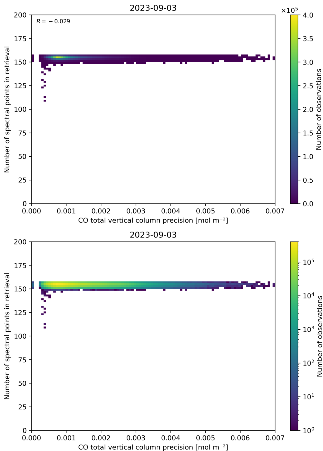
Figure 47: Scatter density plot of “CO total vertical column precision” against “Number of spectral points in retrieval” for 2023-09-02 to 2023-09-04.
