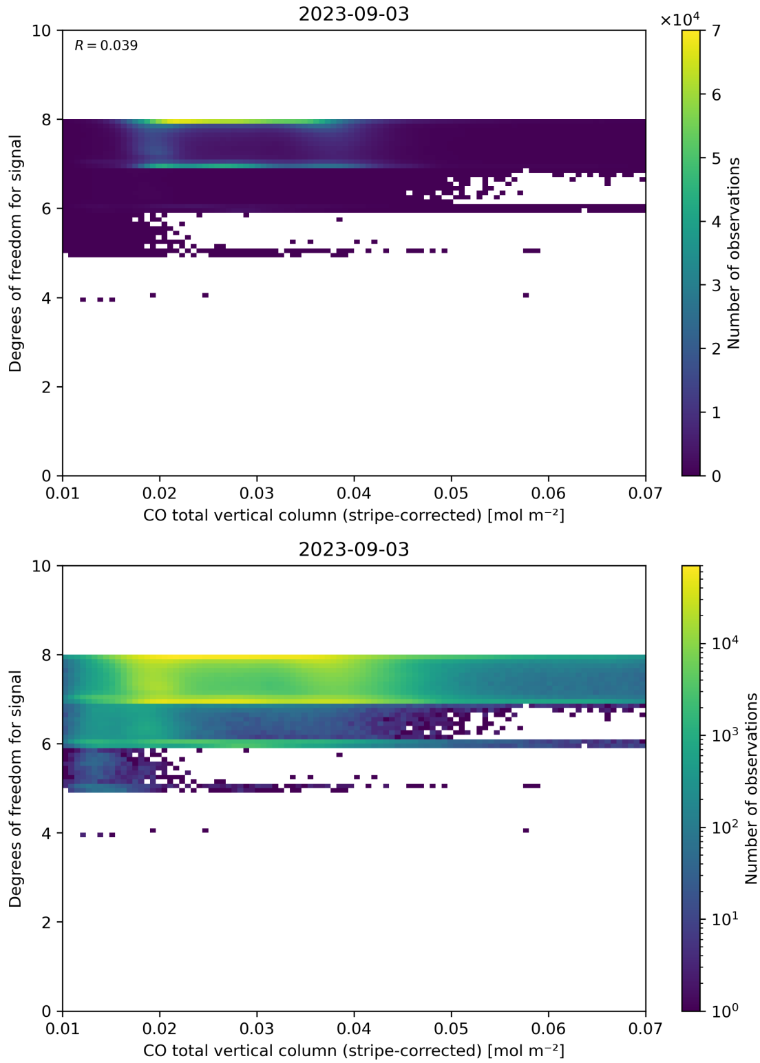
Figure 38: Scatter density plot of “CO total vertical column (stripe-corrected)” against “Degrees of freedom for signal” for 2023-09-02 to 2023-09-04.
