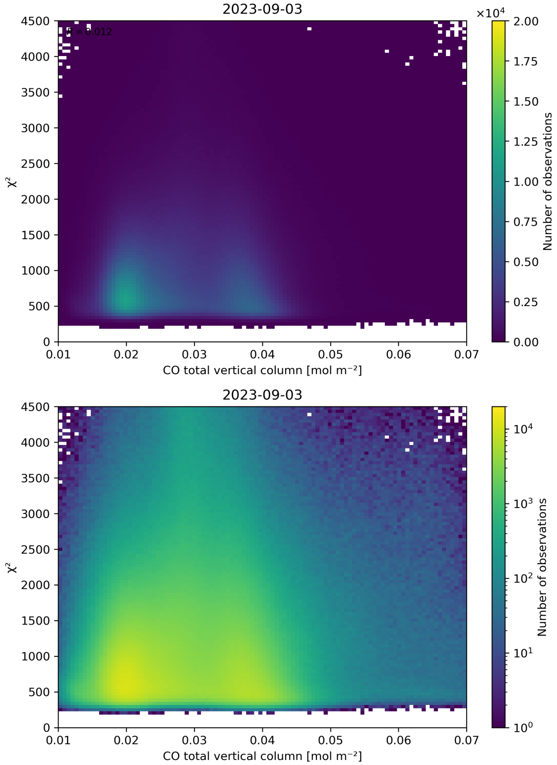
Figure 35: Scatter density plot of “CO total vertical column” against “ \chi^2 ” for 2023-09-02 to 2023-09-04.
