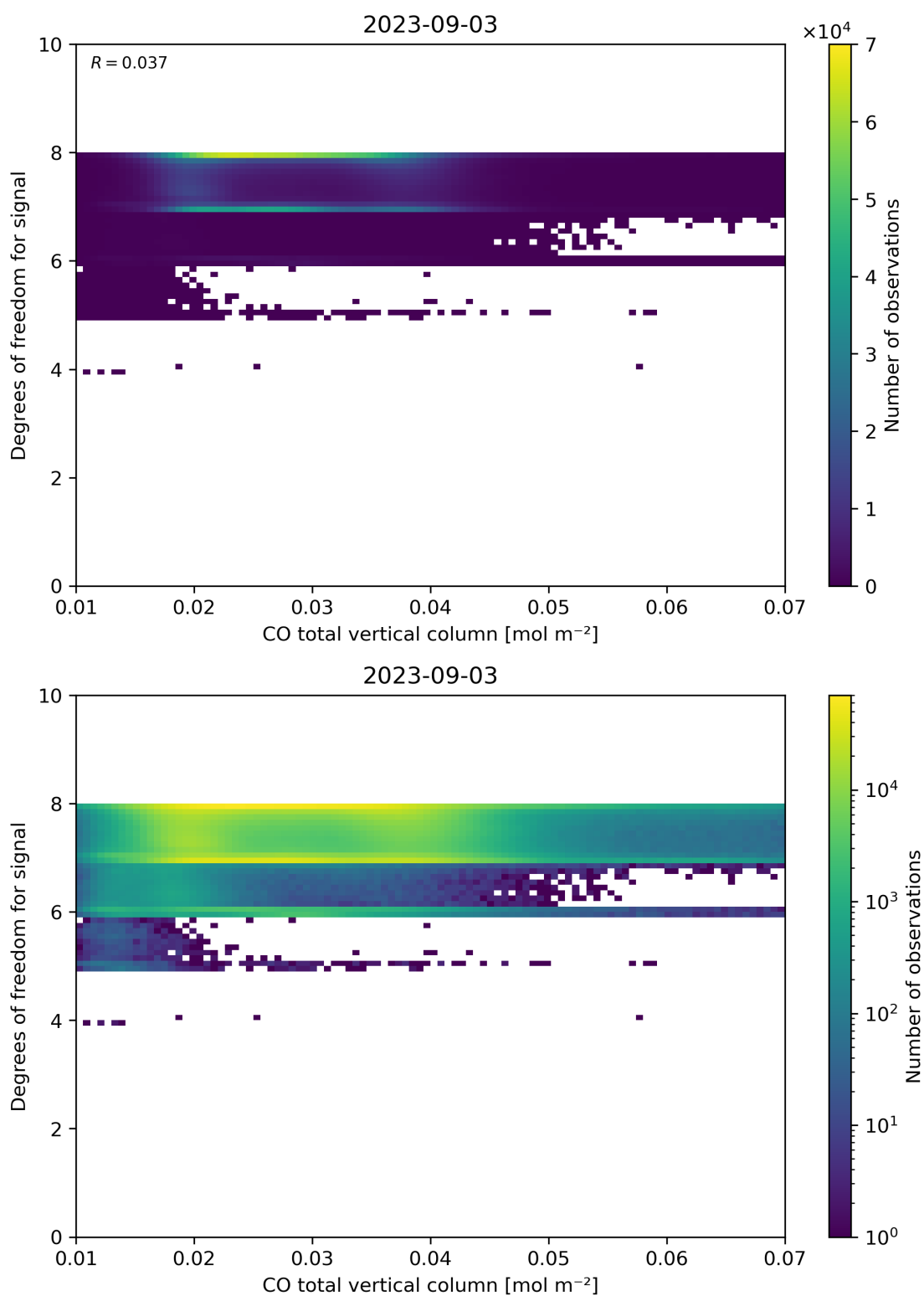
Figure 41: Scatter density plot of “CO total vertical column” against “Degrees of freedom for signal” for 2023-09-02 to 2023-09-04.
