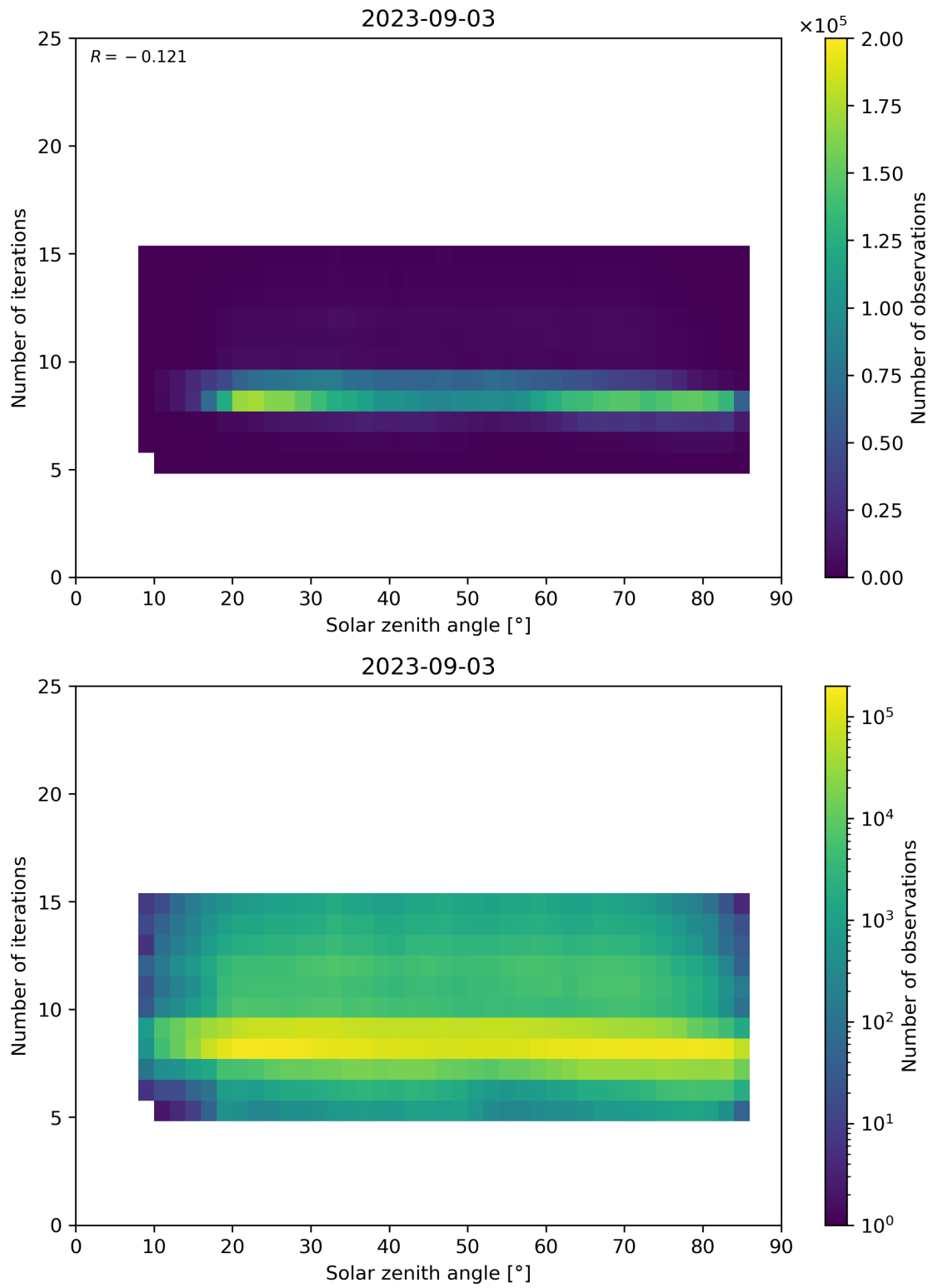
Figure 67: Scatter density plot of “Solar zenith angle” against “Number of iterations” for 2023-09-02 to 2023-09-04.
