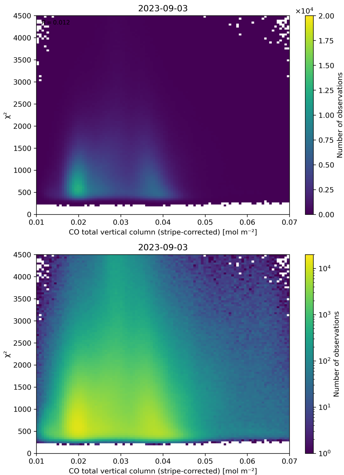
Figure 37: Scatter density plot of “CO total vertical column (stripe-corrected)” against “ \chi^2 ” for 2023-09-02 to 2023-09-04.
