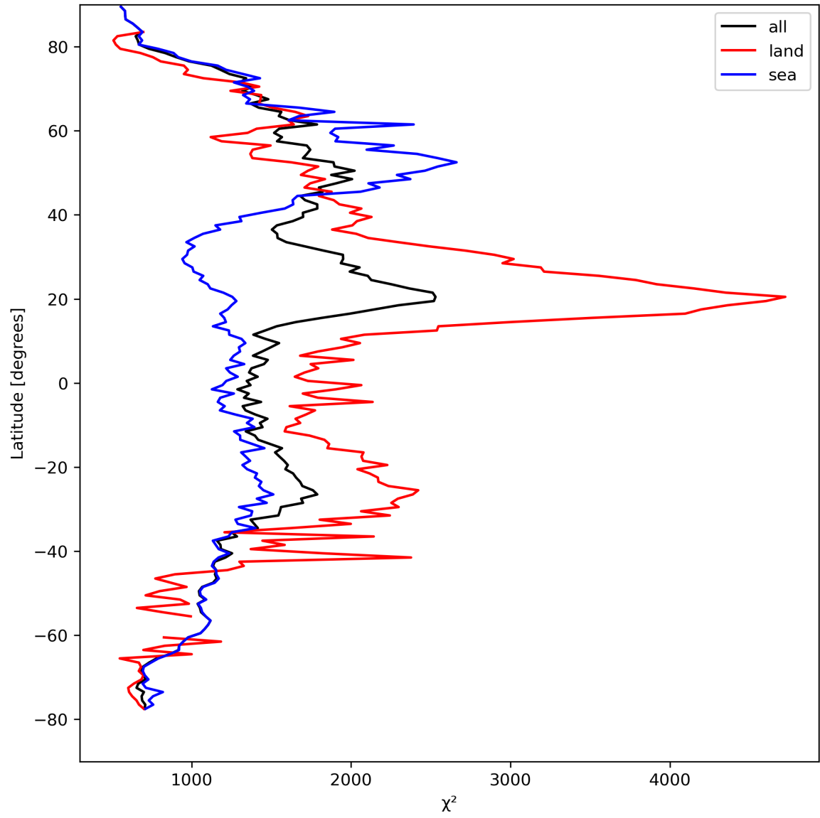
Figure 14: Zonal average of “ \chi^2 ” for 2023-09-04 to 2023-09-05.
