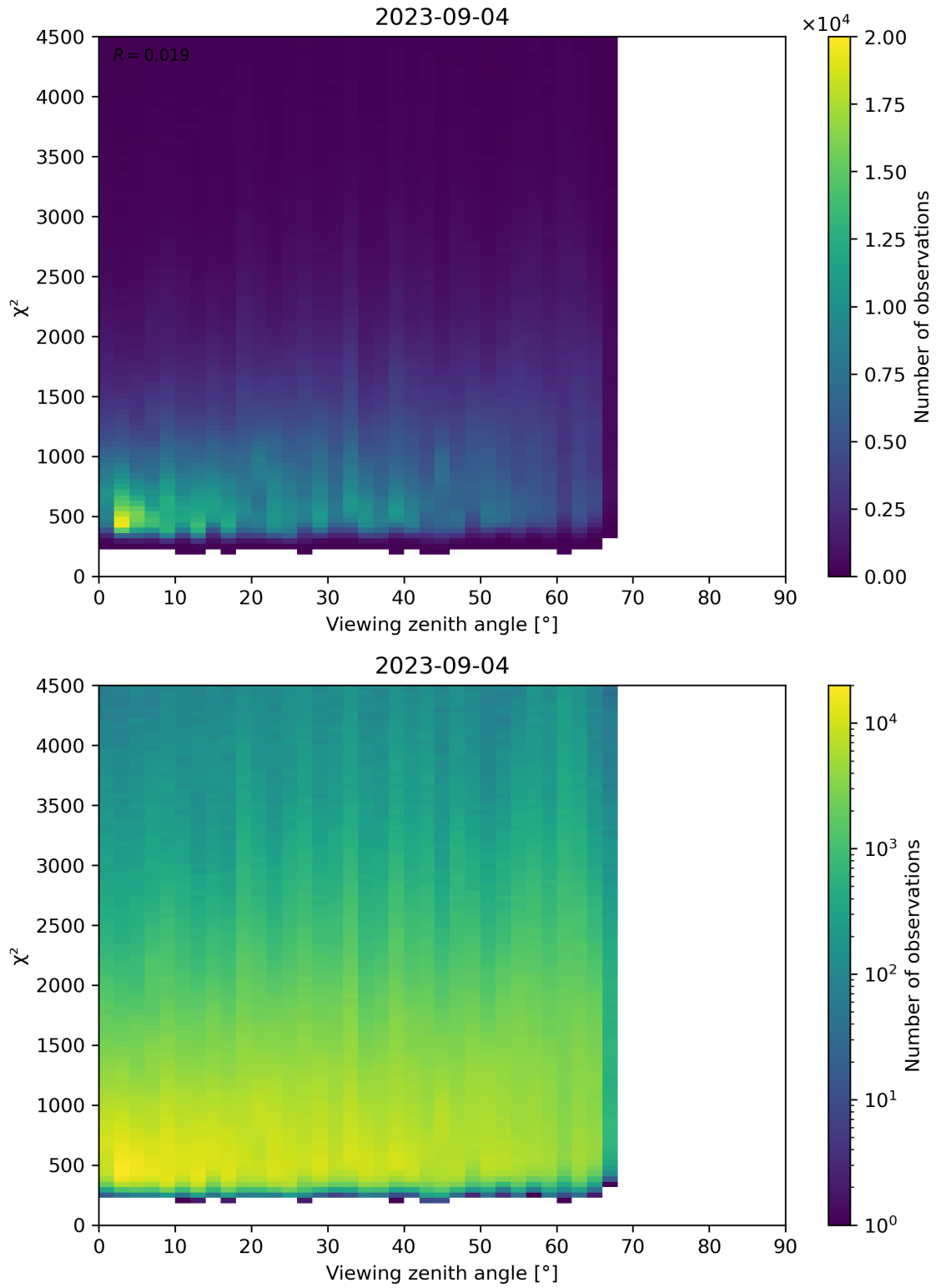
Figure 72: Scatter density plot of “Viewing zenith angle” against “ \chi^2 ” for 2023-09-04 to 2023-09-05.
