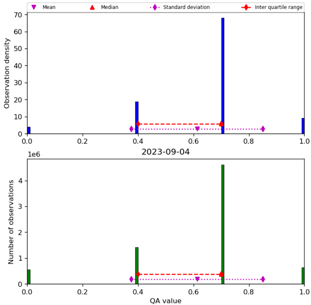
Figure 17: Histogram of “QA value” for 2023-09-04 to 2023-09-05
