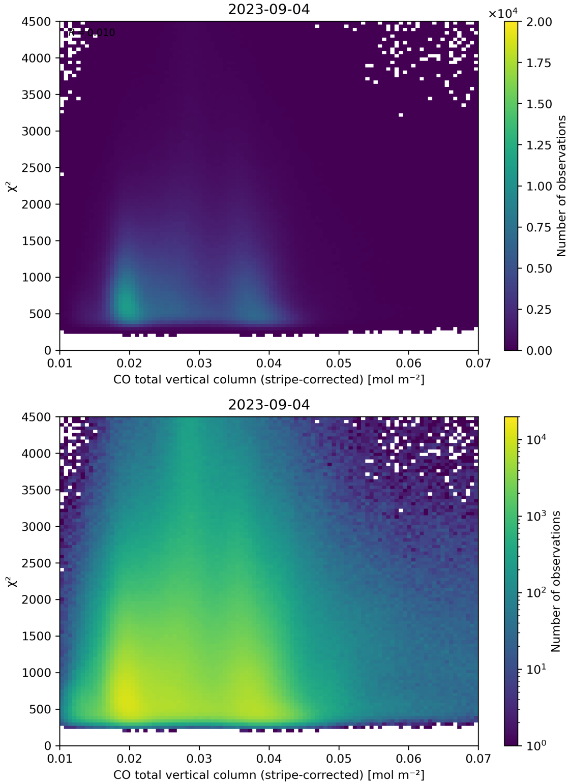
Figure 37: Scatter density plot of “CO total vertical column (stripe-corrected)” against “ \chi^2 ” for 2023-09-04 to 2023-09-05.
