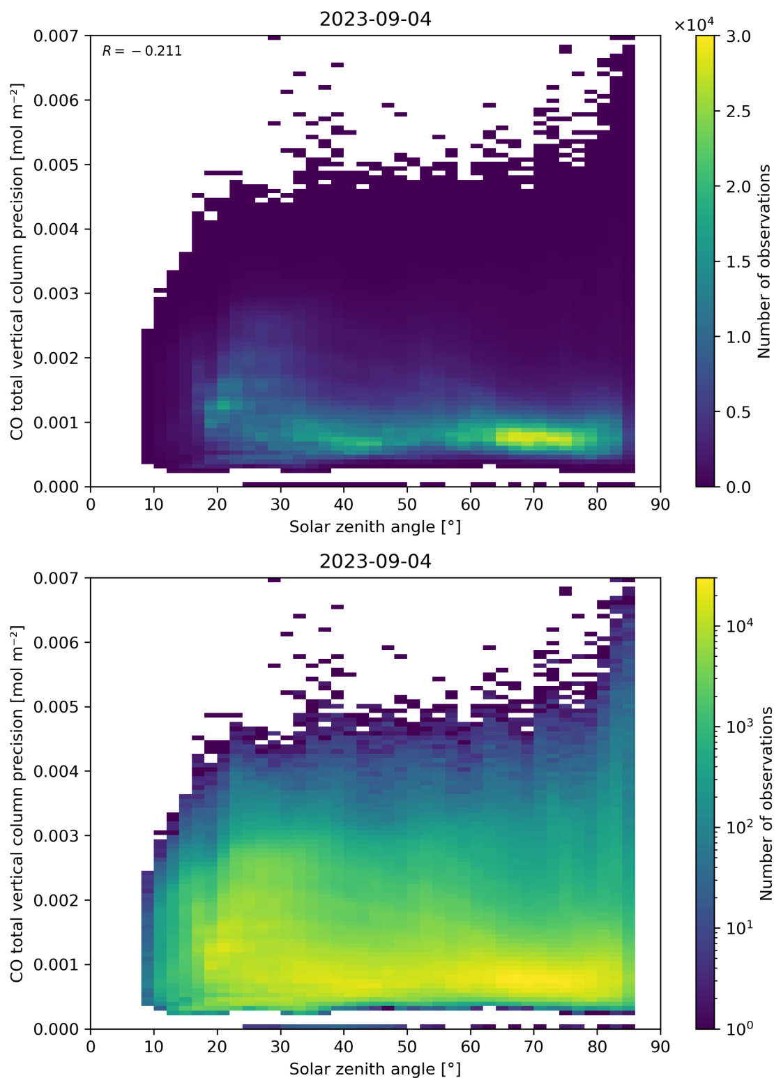
Figure 63: Scatter density plot of “Solar zenith angle” against “CO total vertical column precision” for 2023-09-04 to 2023-09-05.
