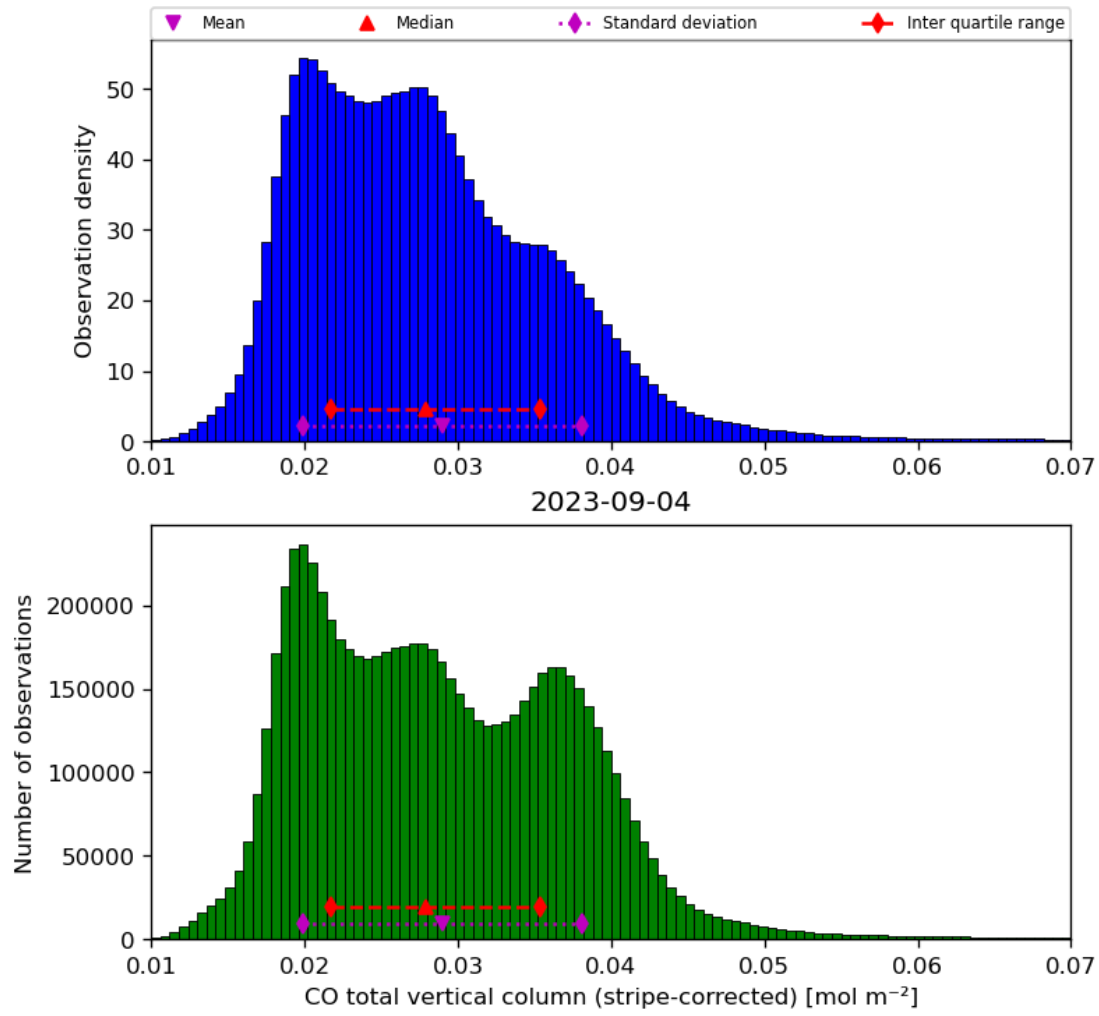
Figure 19: Histogram of “CO total vertical column (stripe-corrected)” for 2023-09-04 to 2023-09-05
