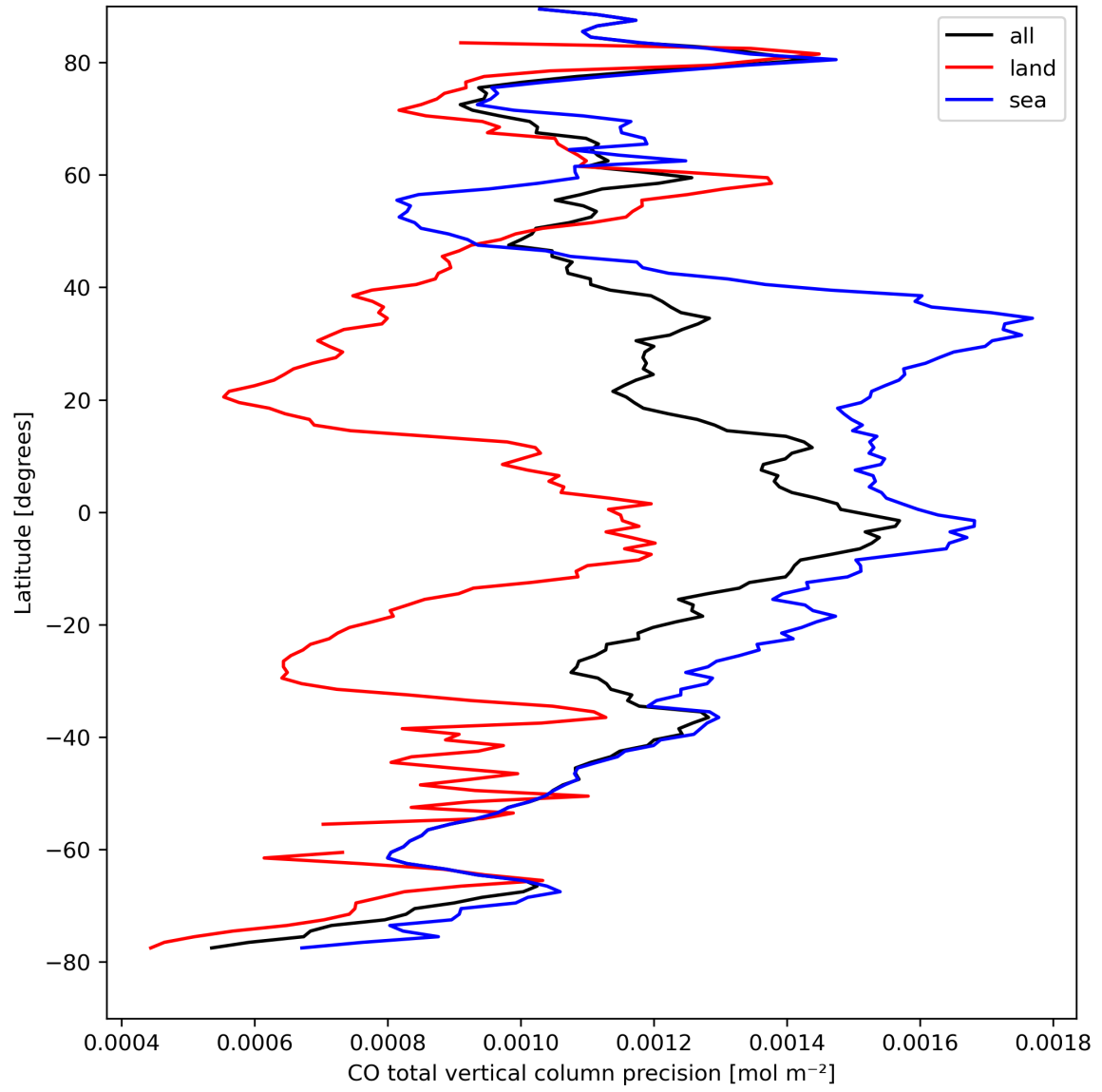
Figure 12: Zonal average of “CO total vertical column precision” for 2023-09-04 to 2023-09-05.
