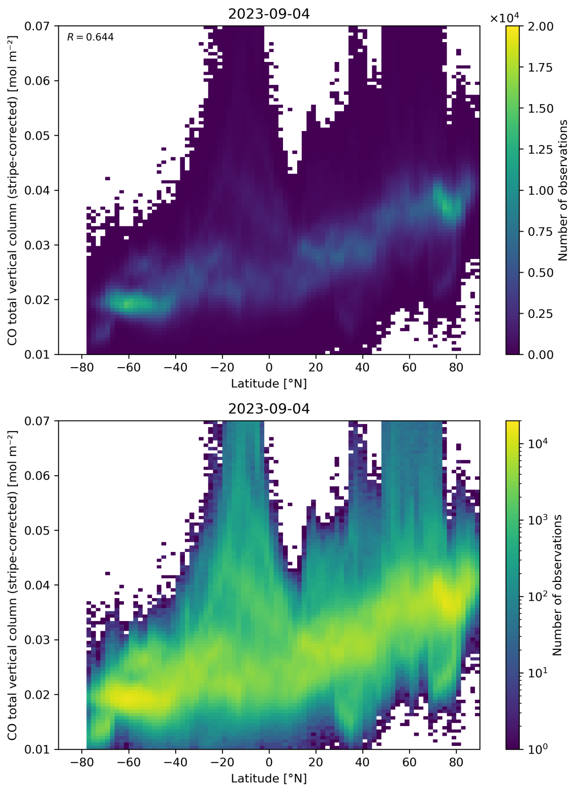
Figure 52: Scatter density plot of “Latitude” against “CO total vertical column (stripe-corrected)” for 2023-09-04 to 2023-09-05.
