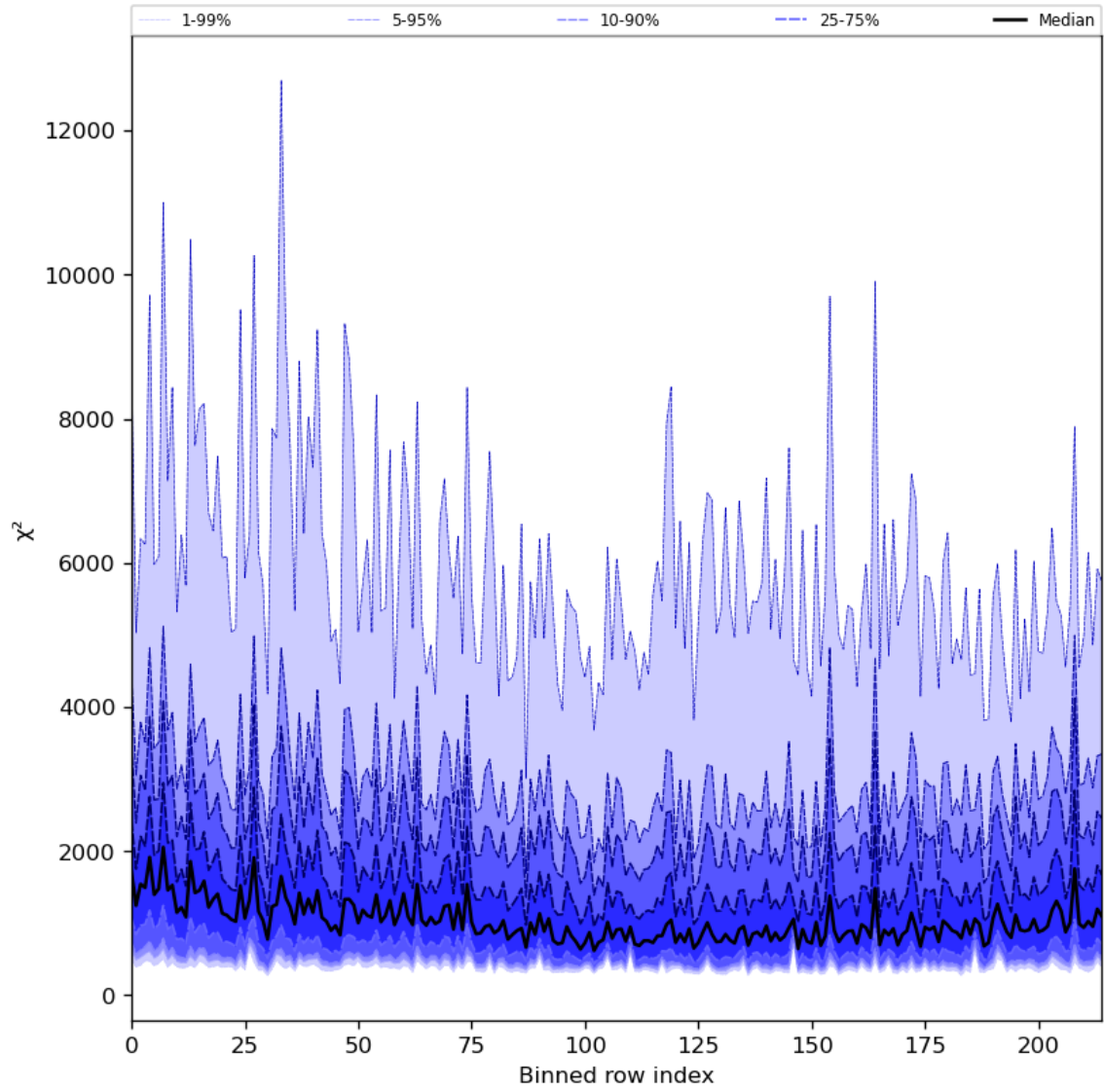
Figure 30: Along track statistics of “ \chi^2 ” for 2023-09-04 to 2023-09-05
