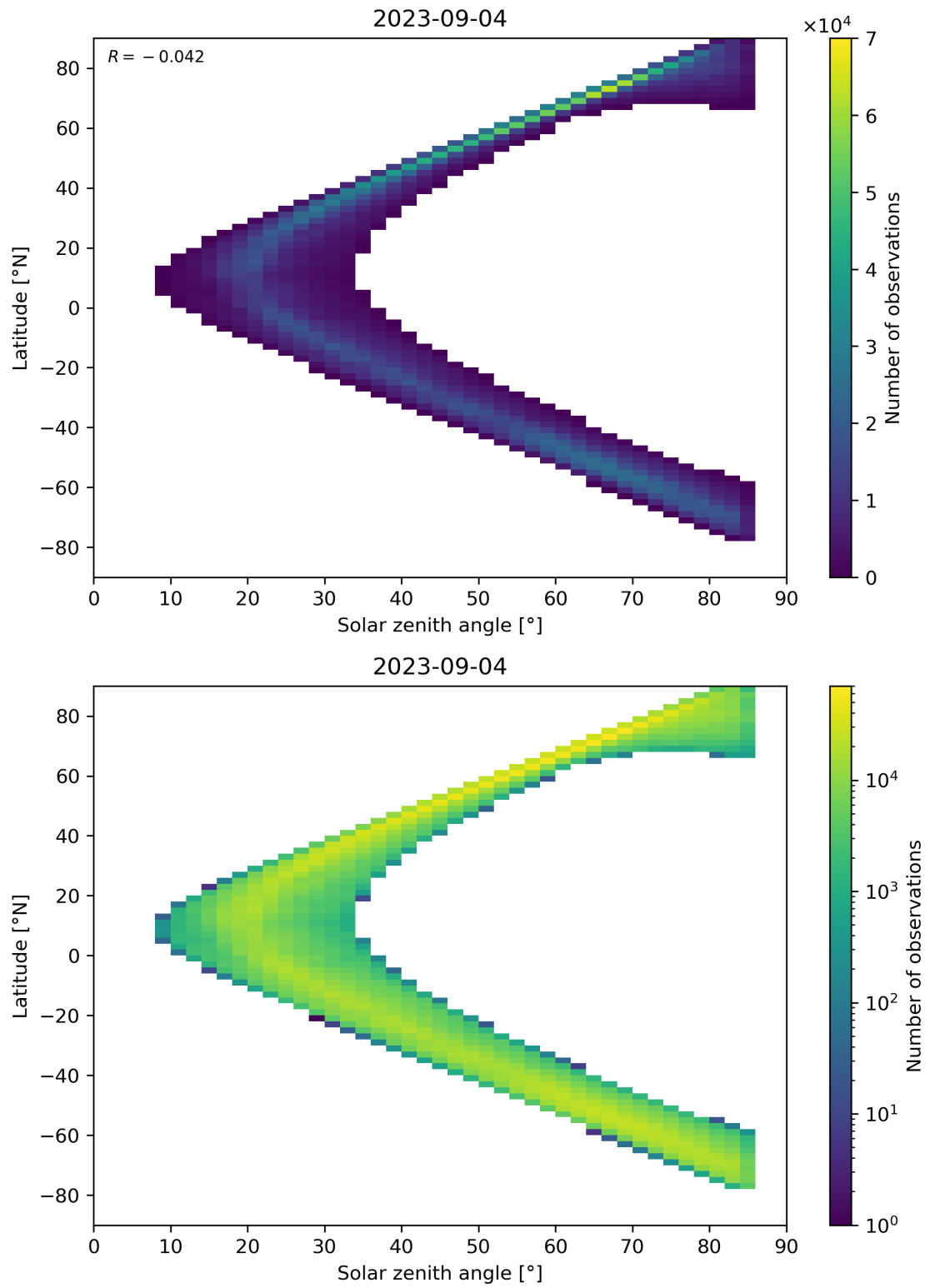
Figure 66: Scatter density plot of “Solar zenith angle” against “Latitude” for 2023-09-04 to 2023-09-05.
