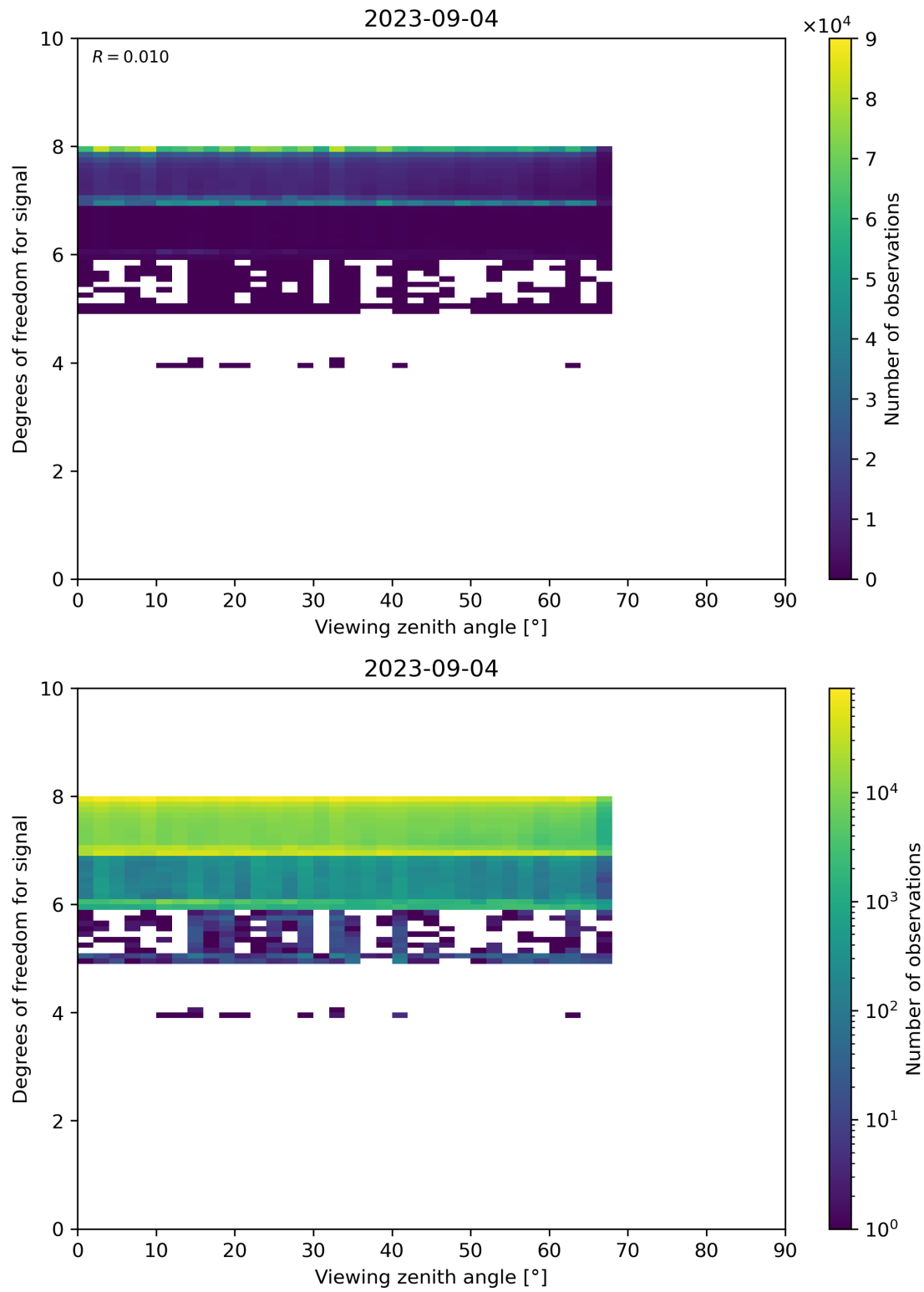
Figure 73: Scatter density plot of “Viewing zenith angle” against “Degrees of freedom for signal” for 2023-09-04 to 2023-09-05.
