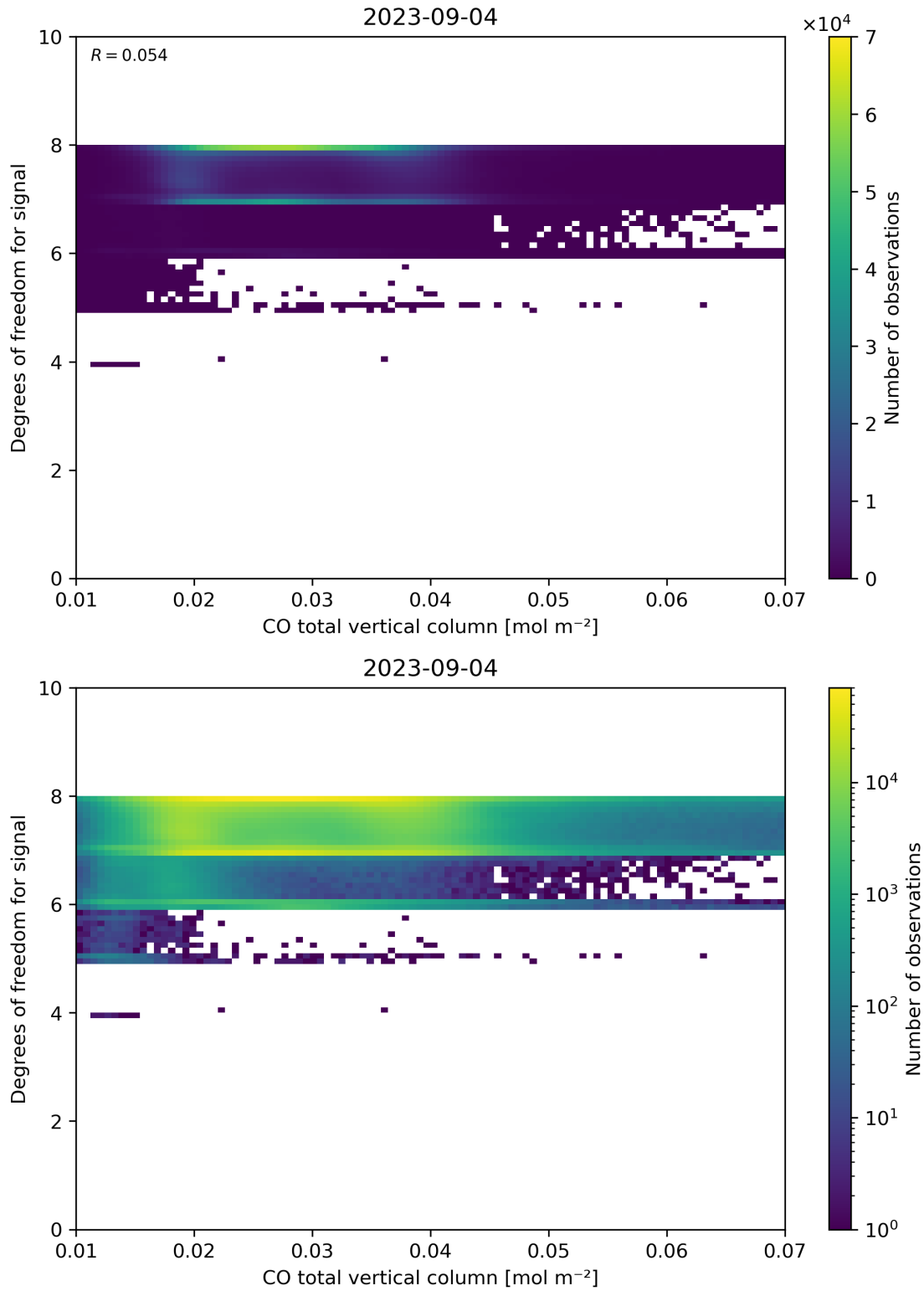
Figure 41: Scatter density plot of “CO total vertical column” against “Degrees of freedom for signal” for 2023-09-04 to 2023-09-05.
