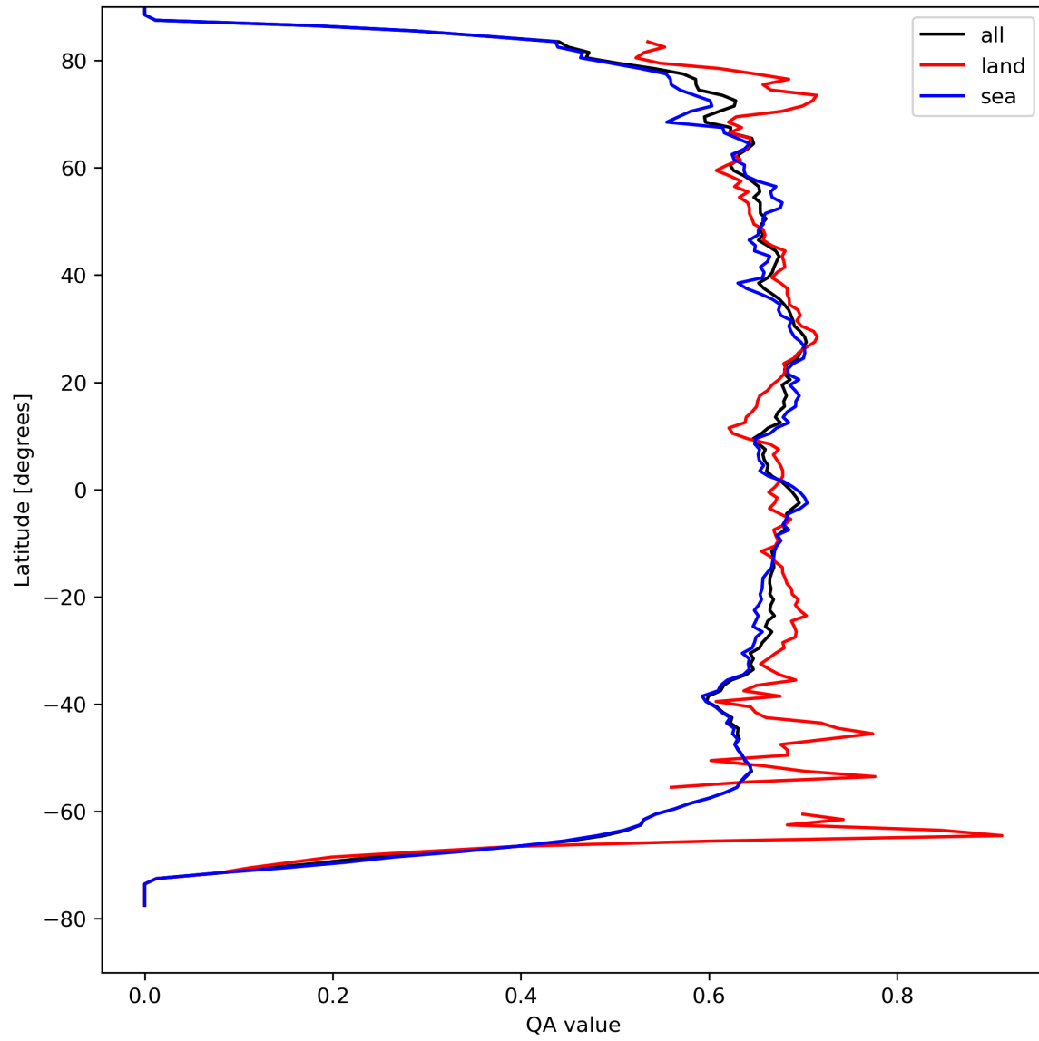
Figure 9: Zonal average of “QA value” for 2023-09-04 to 2023-09-05.
