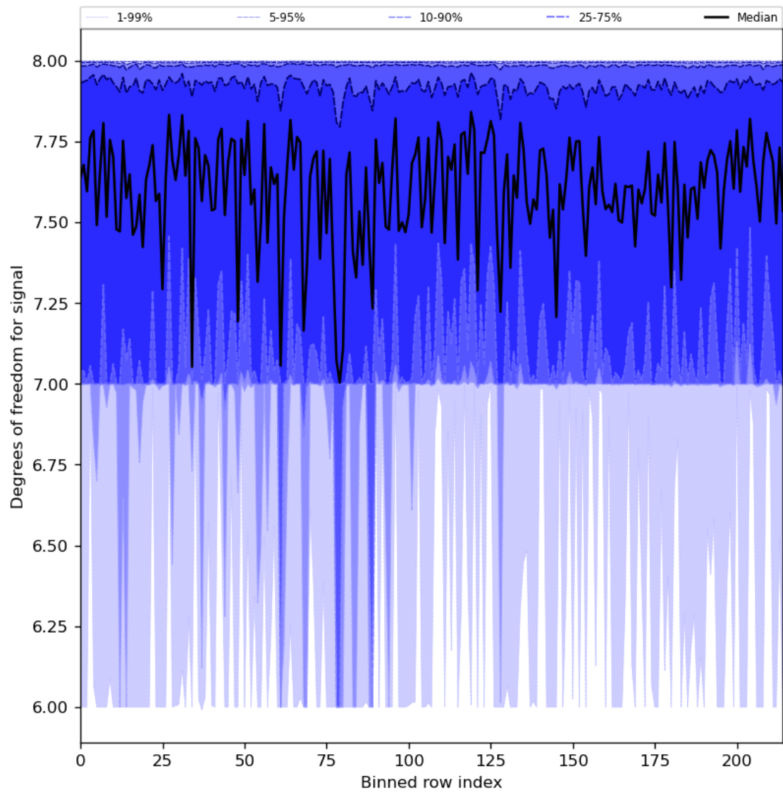
Figure 31: Along track statistics of “Degrees of freedom for signal” for 2023-09-04 to 2023-09-05
