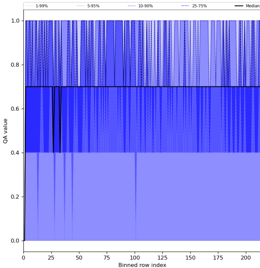
Figure 25: Along track statistics of “QA value” for 2023-09-04 to 2023-09-05
