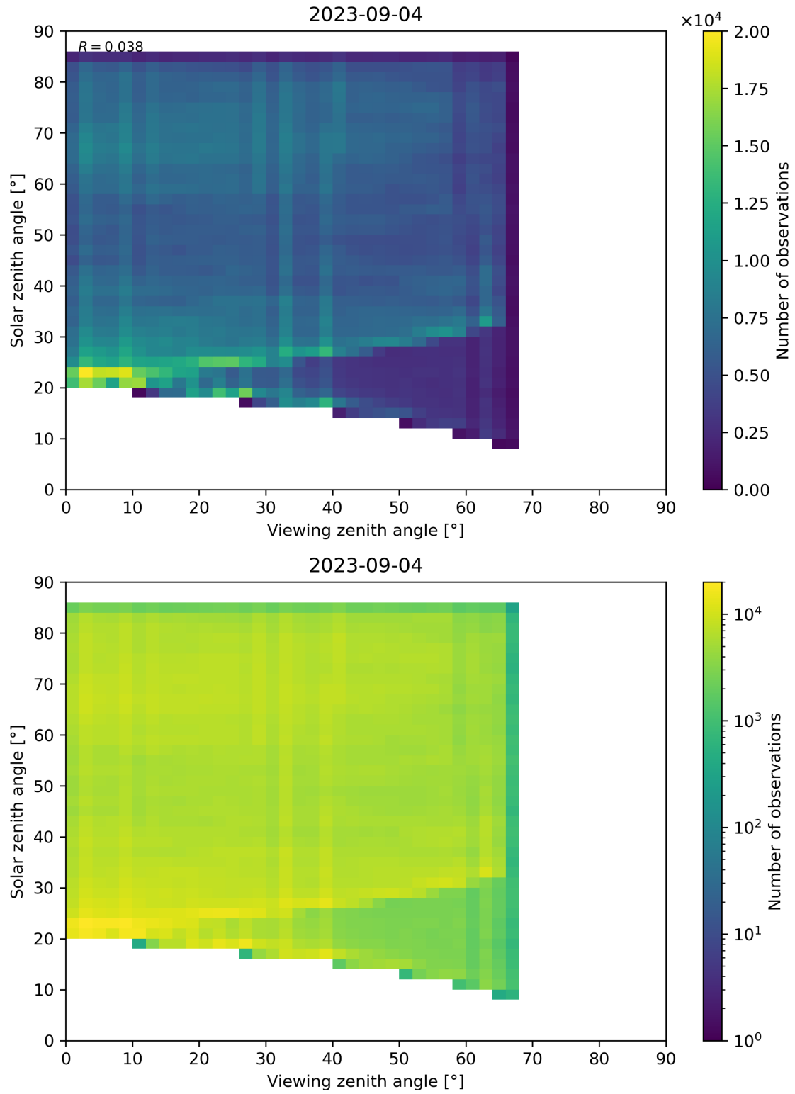
Figure 77: Scatter density plot of “Viewing zenith angle” against “Solar zenith angle” for 2023-09-04 to 2023-09-05.
