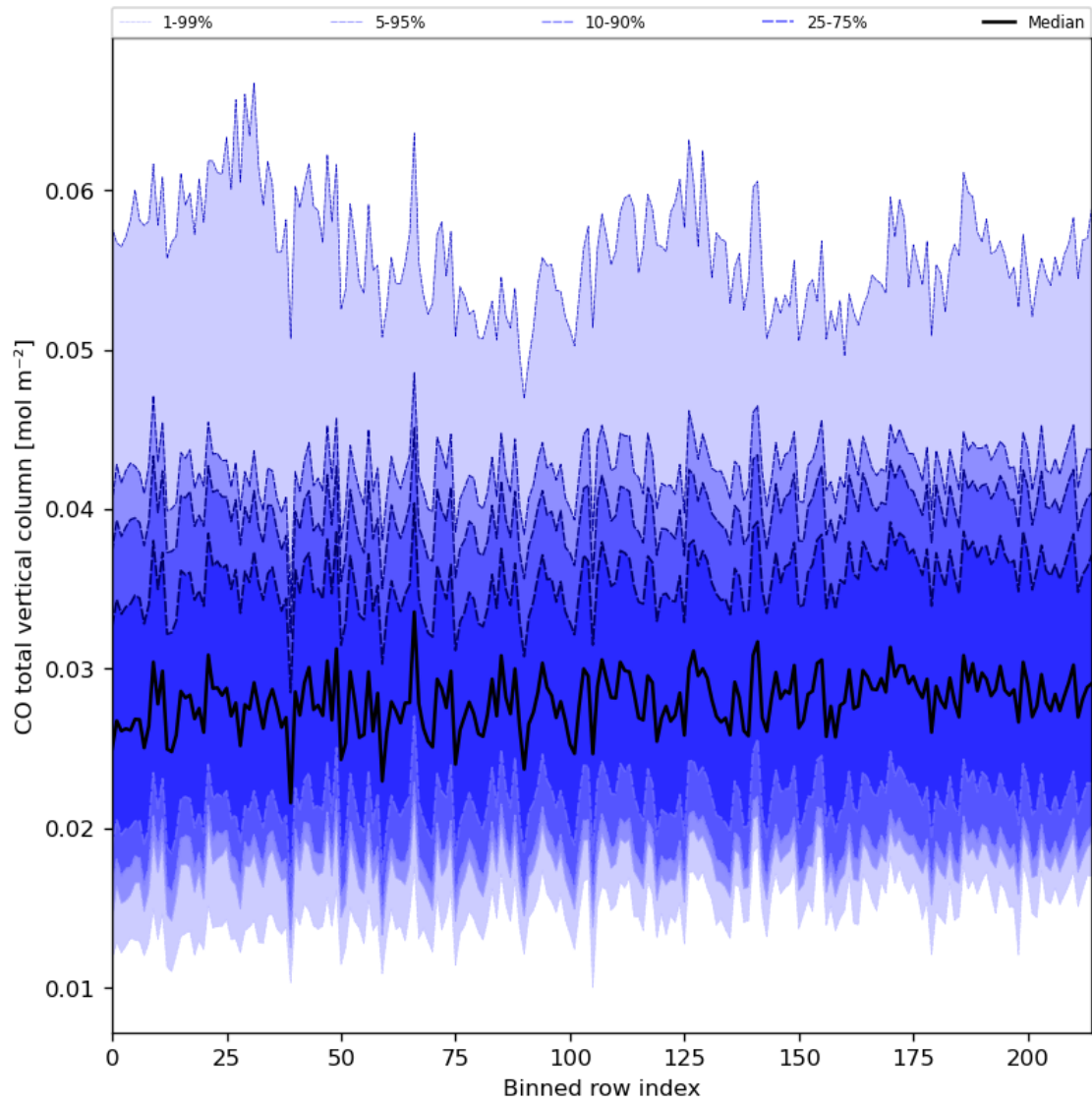
Figure 26: Along track statistics of “CO total vertical column” for 2023-09-04 to 2023-09-05
