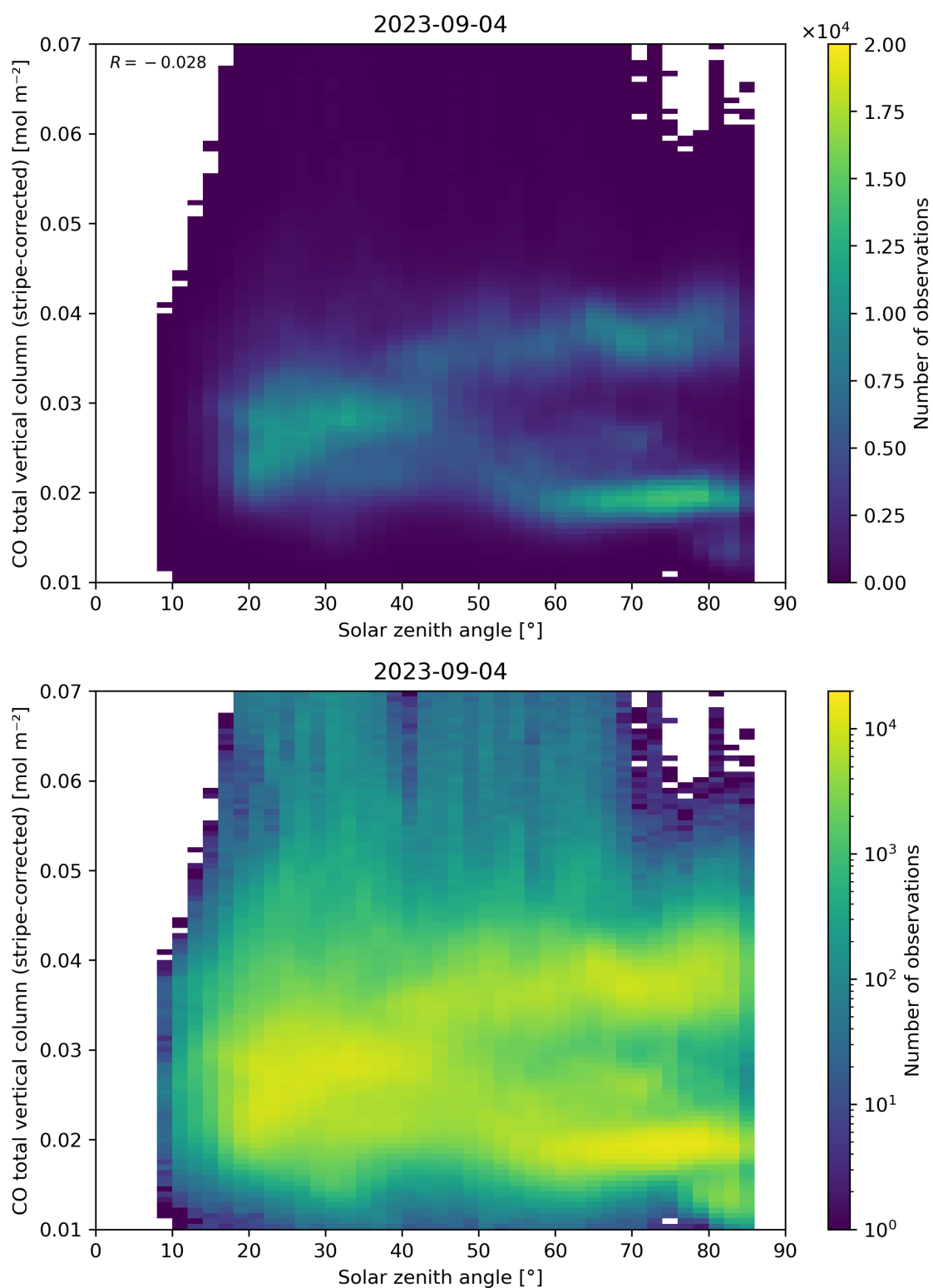
Figure 62: Scatter density plot of “Solar zenith angle” against “CO total vertical column (stripe-corrected)” for 2023-09-04 to 2023-09-05.
