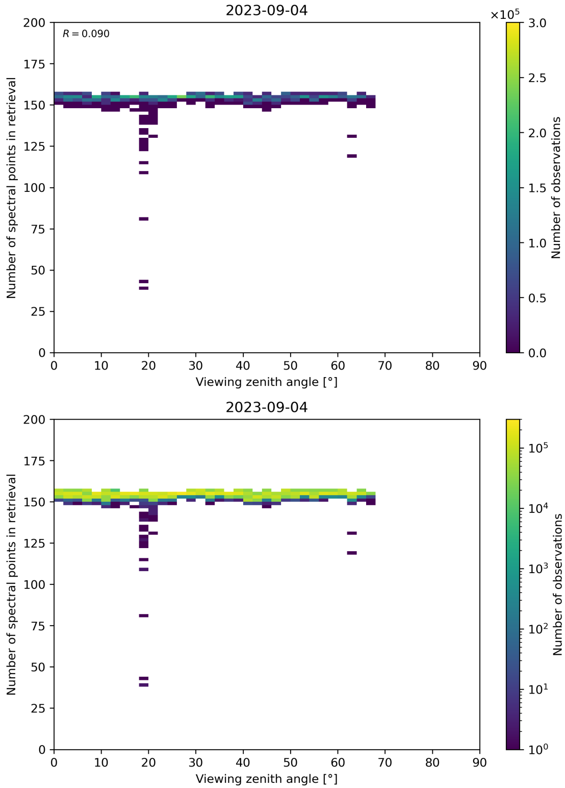
Figure 76: Scatter density plot of “Viewing zenith angle” against “Number of spectral points in retrieval” for 2023-09-04 to 2023-09-05.
