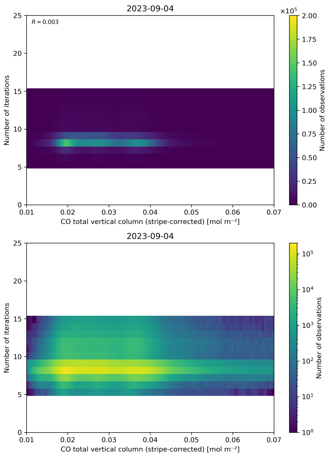
Figure 39: Scatter density plot of “CO total vertical column (stripe-corrected)” against “Number of iterations” for 2023-09-04 to 2023-09-05.
