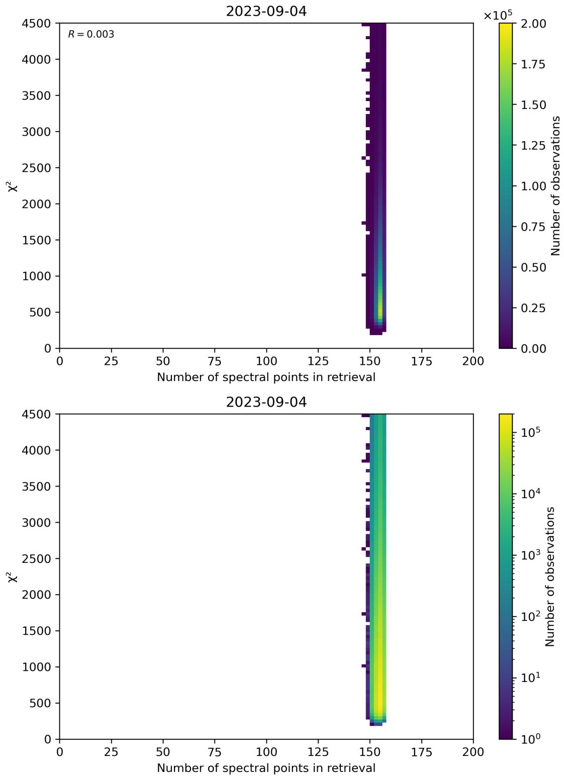
Figure 58: Scatter density plot of “Number of spectral points in retrieval” against “ \chi^2 ” for 2023-09-04 to 2023-09-05.
