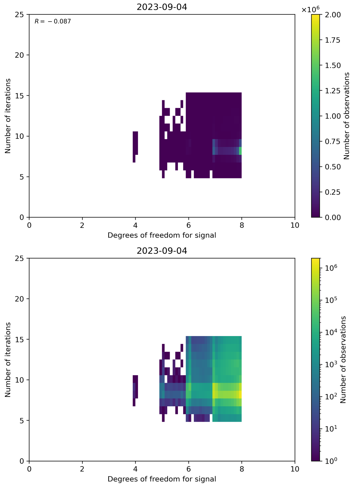
Figure 50: Scatter density plot of “Degrees of freedom for signal” against “Number of iterations” for 2023-09-04 to 2023-09-05.
