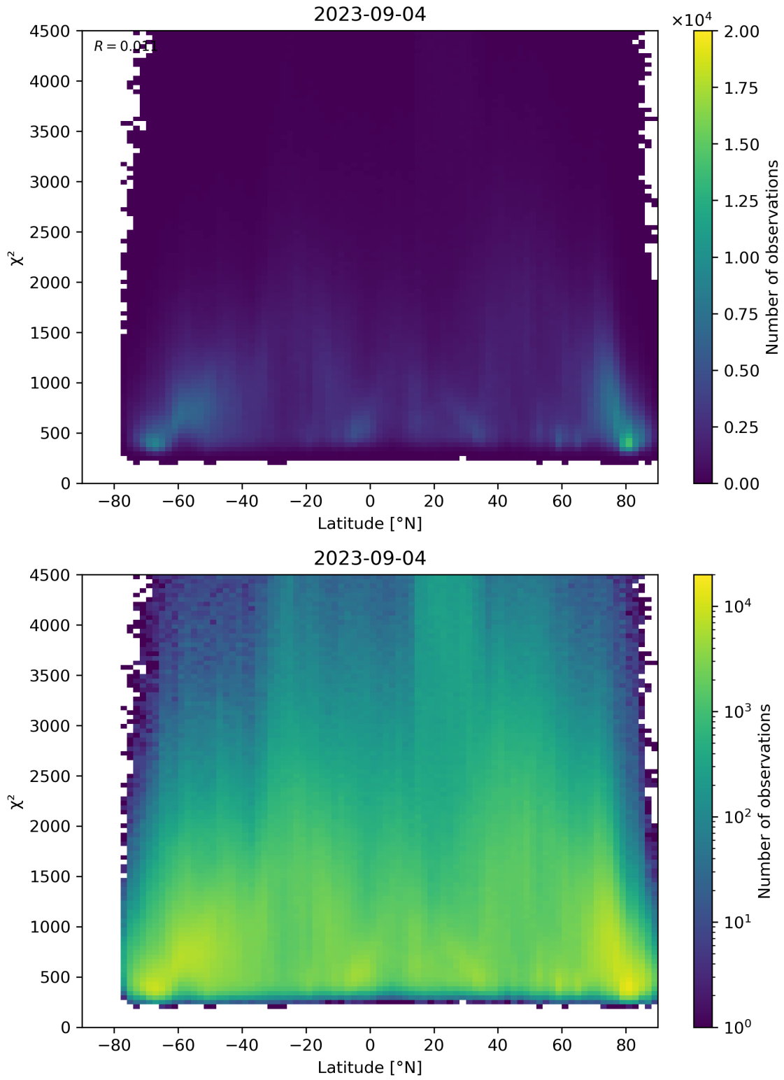
Figure 54: Scatter density plot of “Latitude” against “ \chi^2 ” for 2023-09-04 to 2023-09-05.
