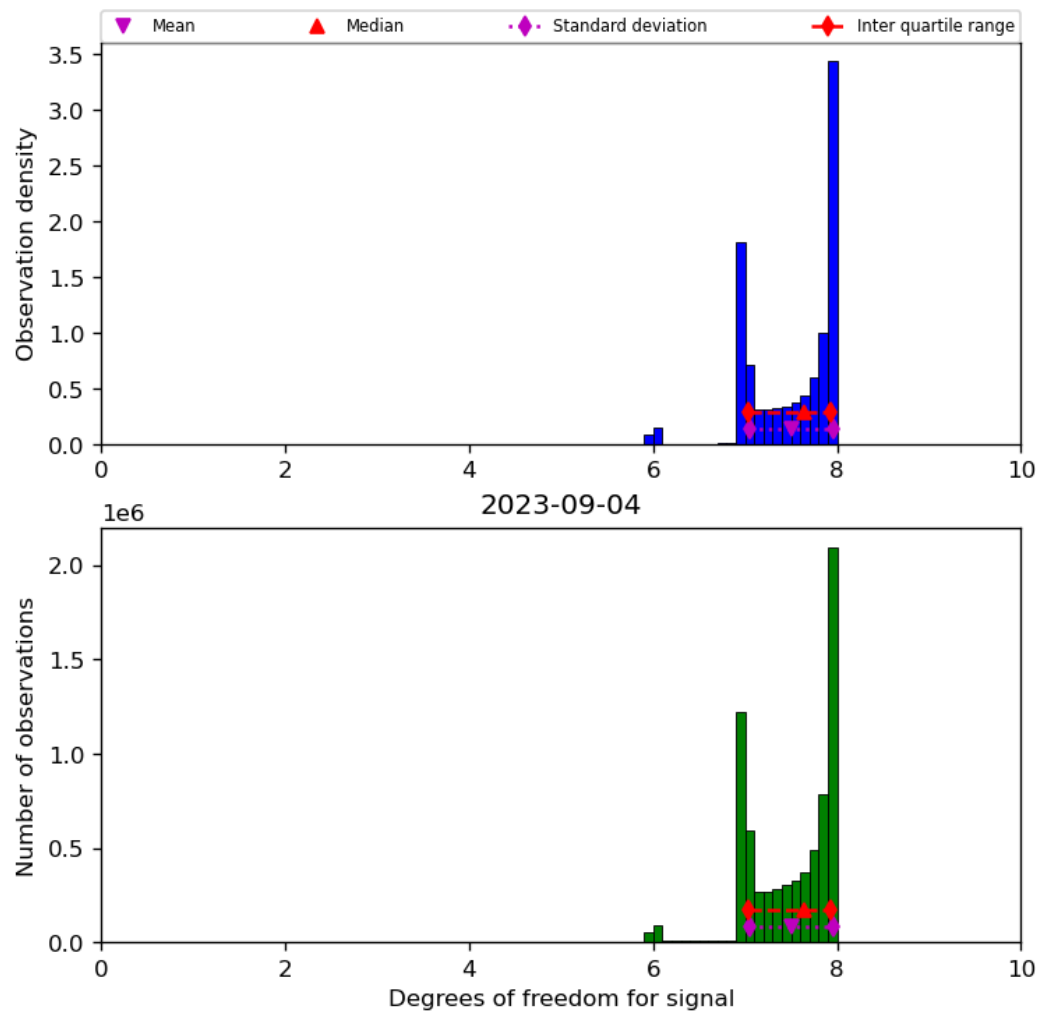
Figure 23: Histogram of “Degrees of freedom for signal” for 2023-09-04 to 2023-09-05
