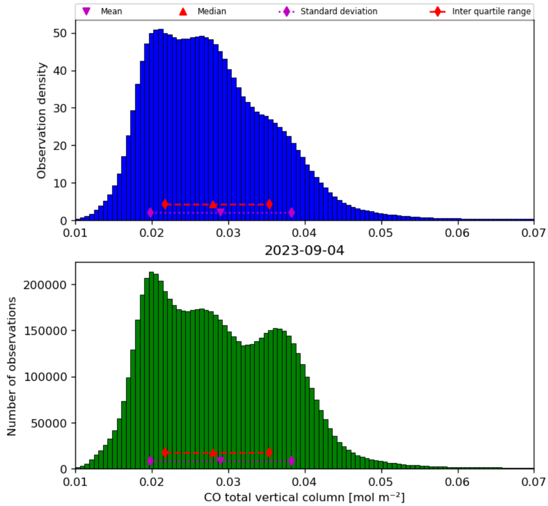
Figure 18: Histogram of “CO total vertical column” for 2023-09-04 to 2023-09-05
