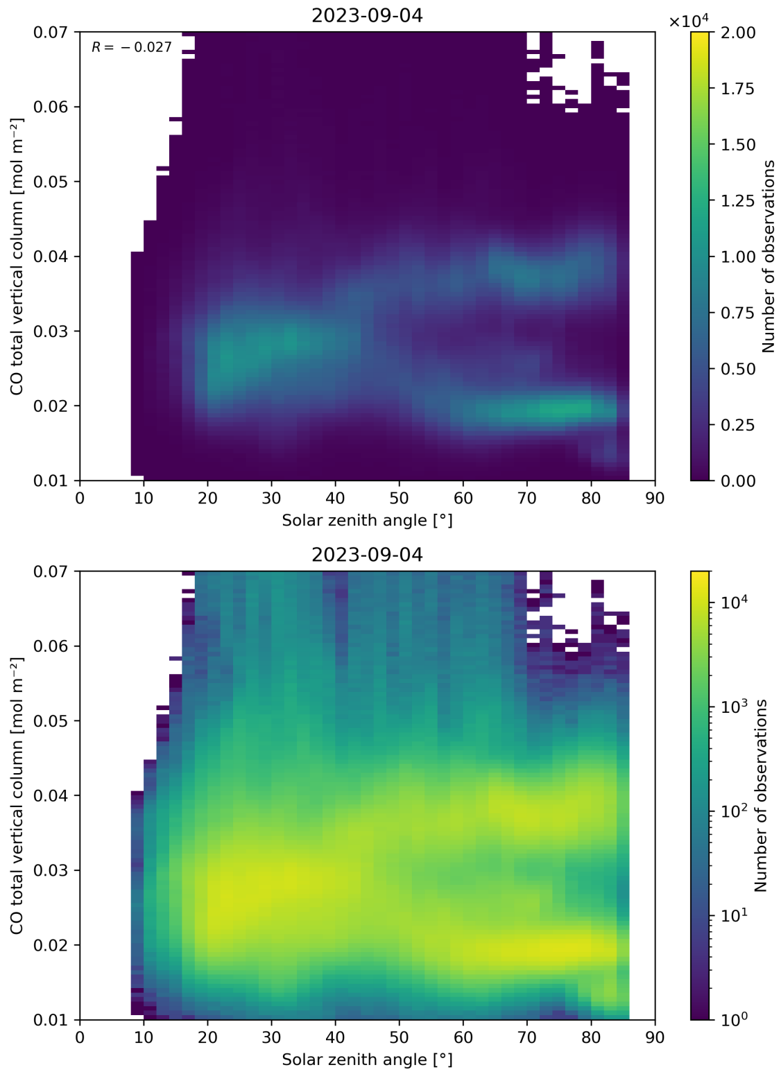
Figure 61: Scatter density plot of “Solar zenith angle” against “CO total vertical column” for 2023-09-04 to 2023-09-05.
