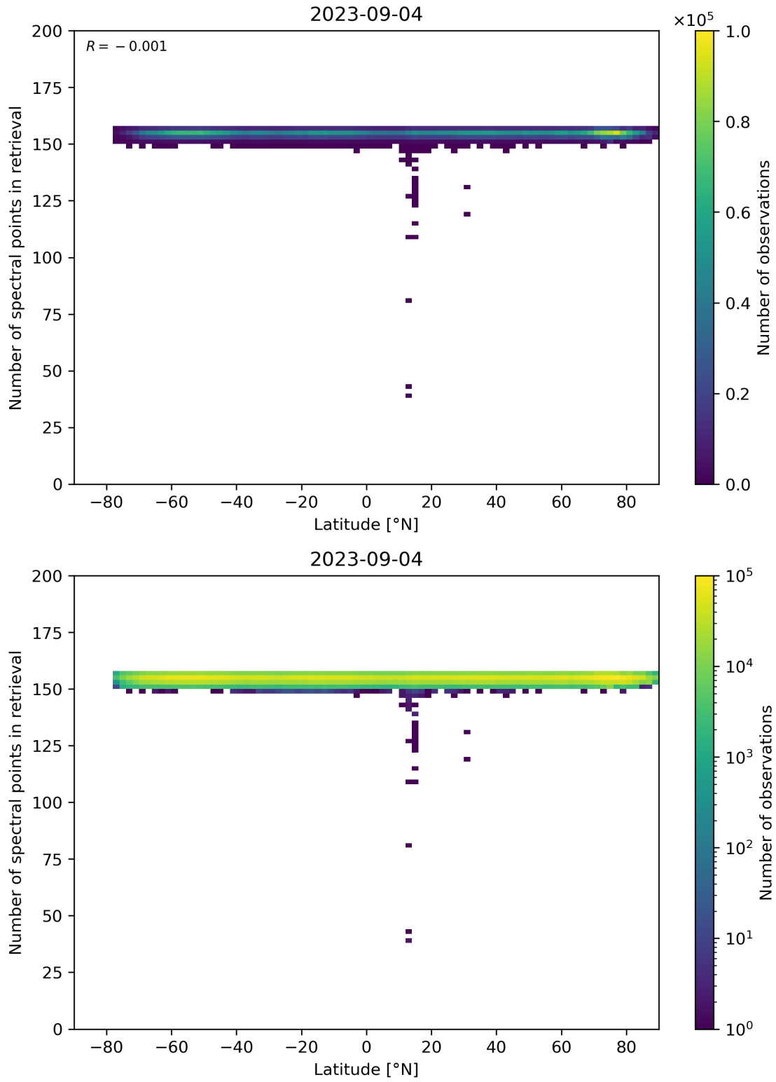
Figure 57: Scatter density plot of “Latitude” against “Number of spectral points in retrieval” for 2023-09-04 to 2023-09-05.
