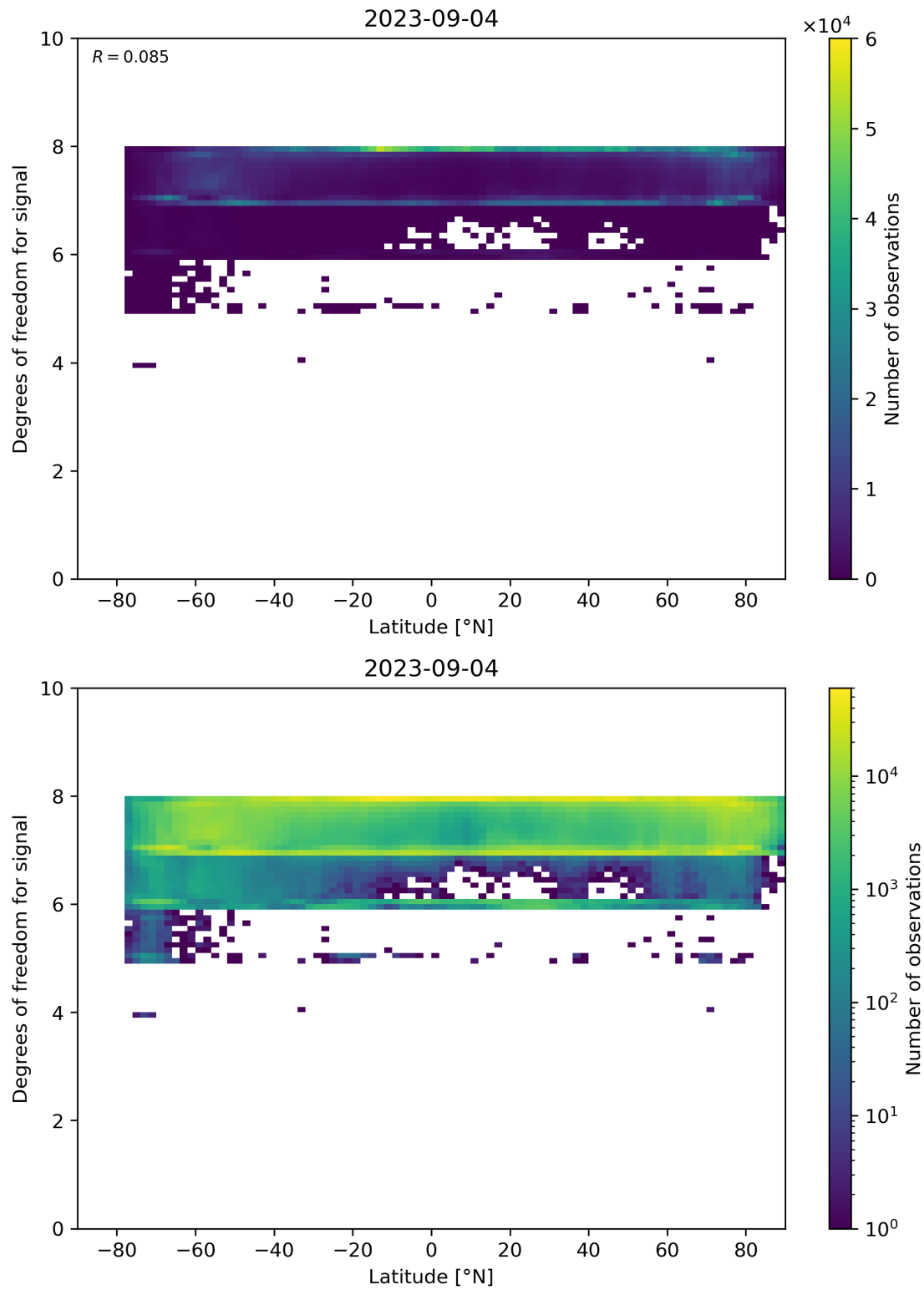
Figure 55: Scatter density plot of “Latitude” against “Degrees of freedom for signal” for 2023-09-04 to 2023-09-05.
