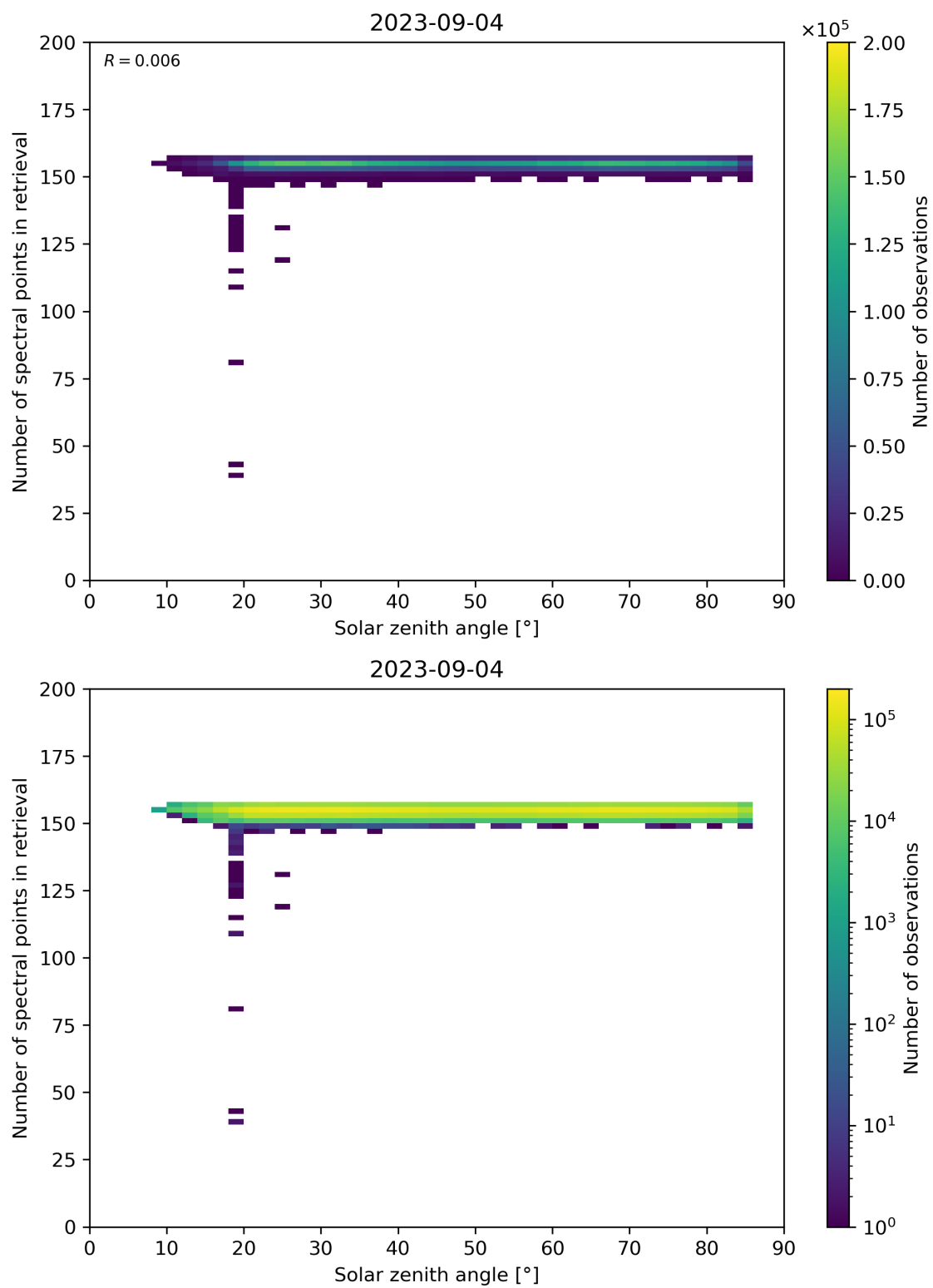
Figure 68: Scatter density plot of “Solar zenith angle” against “Number of spectral points in retrieval” for 2023-09-04 to 2023-09-05.
