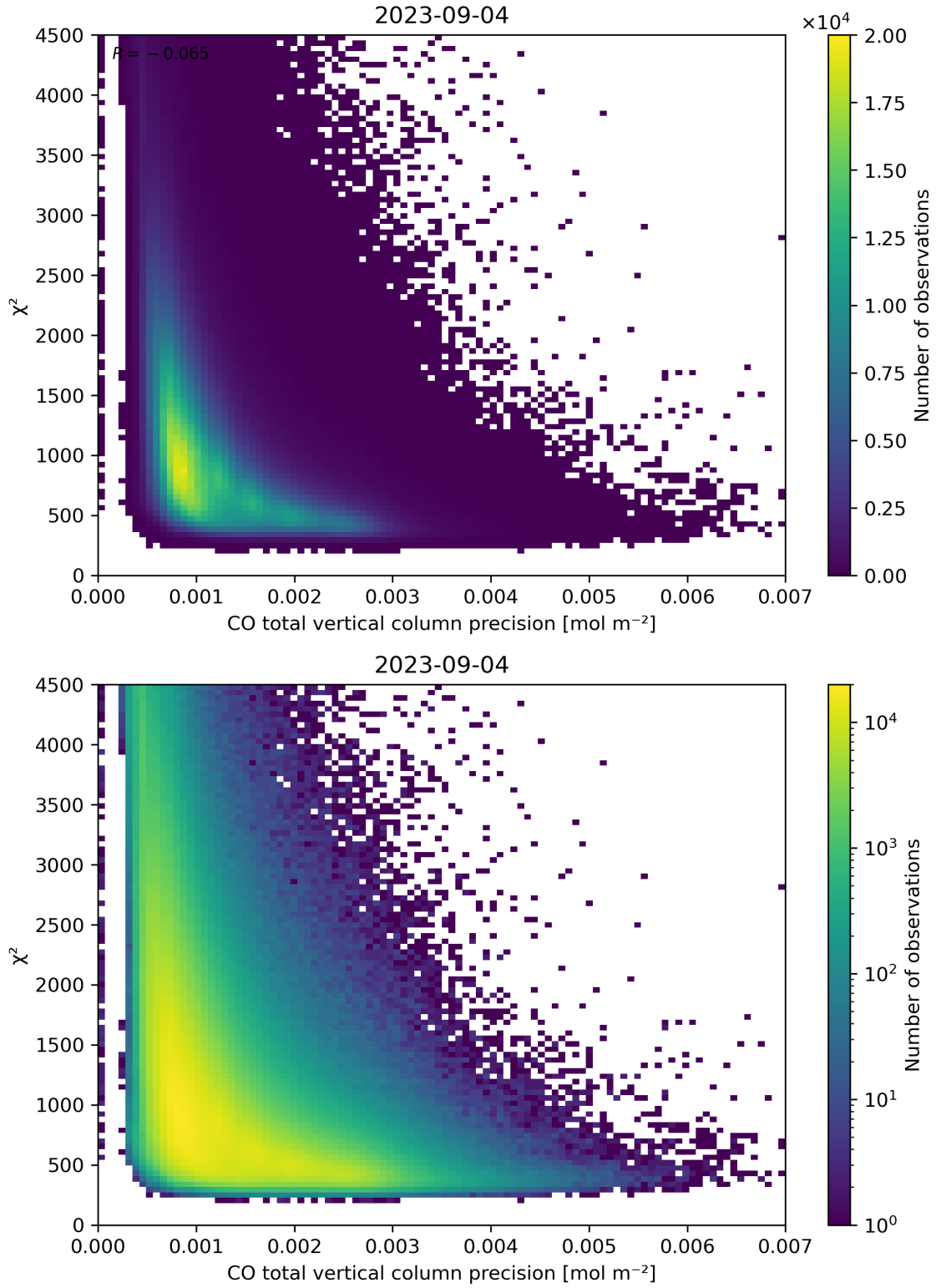
Figure 44: Scatter density plot of “CO total vertical column precision” against “ \chi^2 ” for 2023-09-04 to 2023-09-05.
