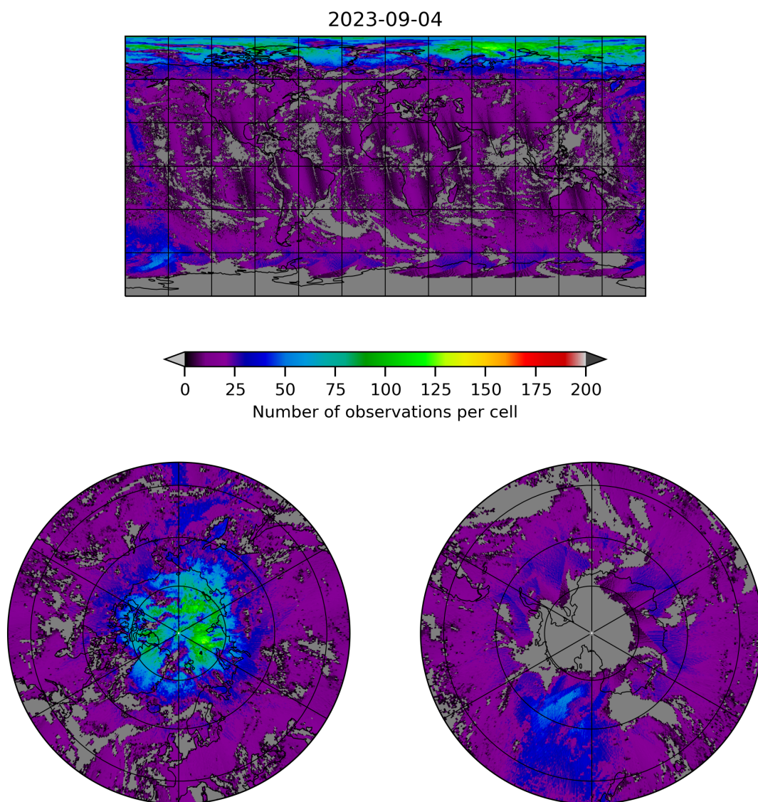
Figure 8: Map of the number of observations for 2023-09-04 to 2023-09-05
