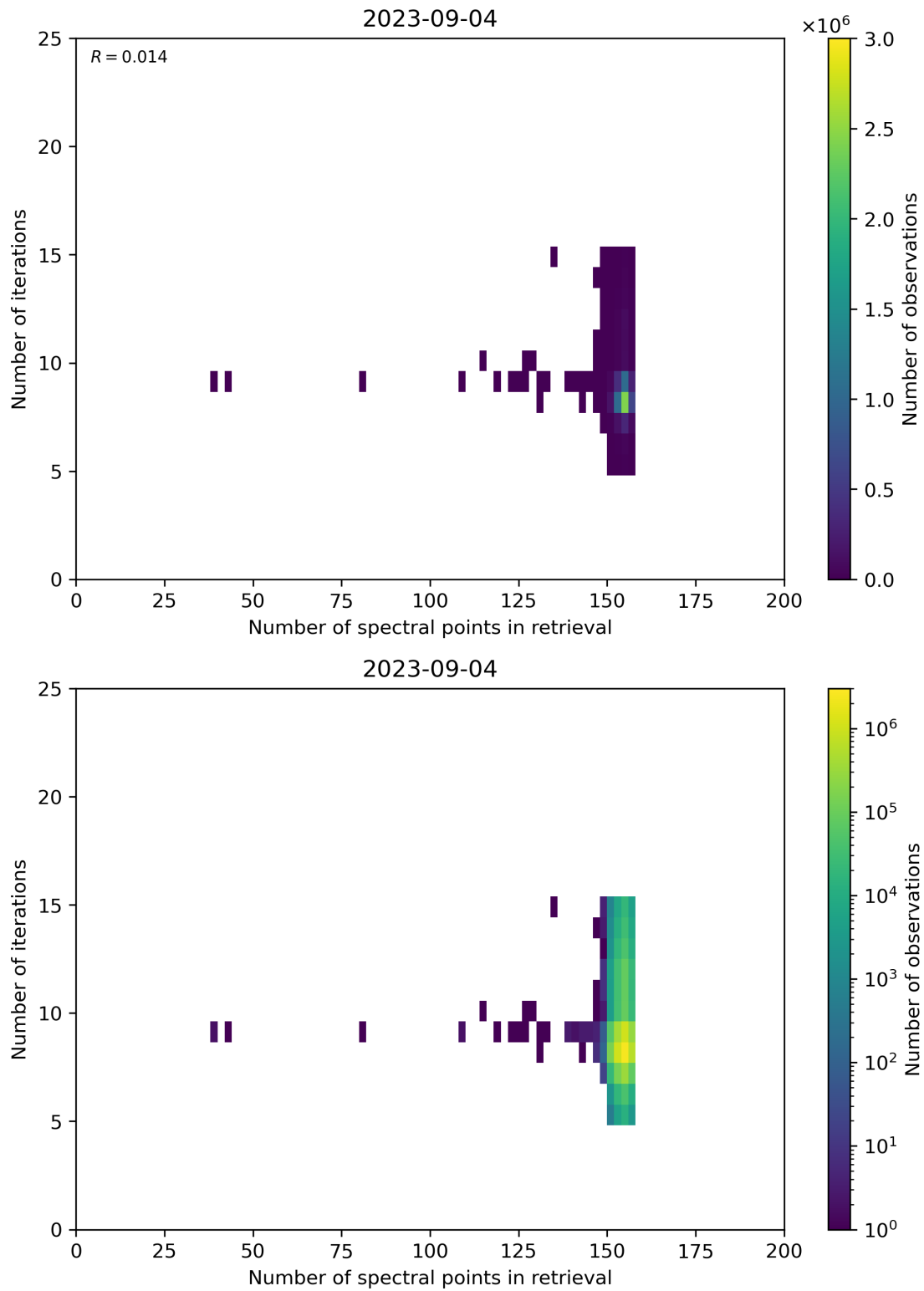
Figure 60: Scatter density plot of “Number of spectral points in retrieval” against “Number of iterations” for 2023-09-04 to 2023-09-05.
