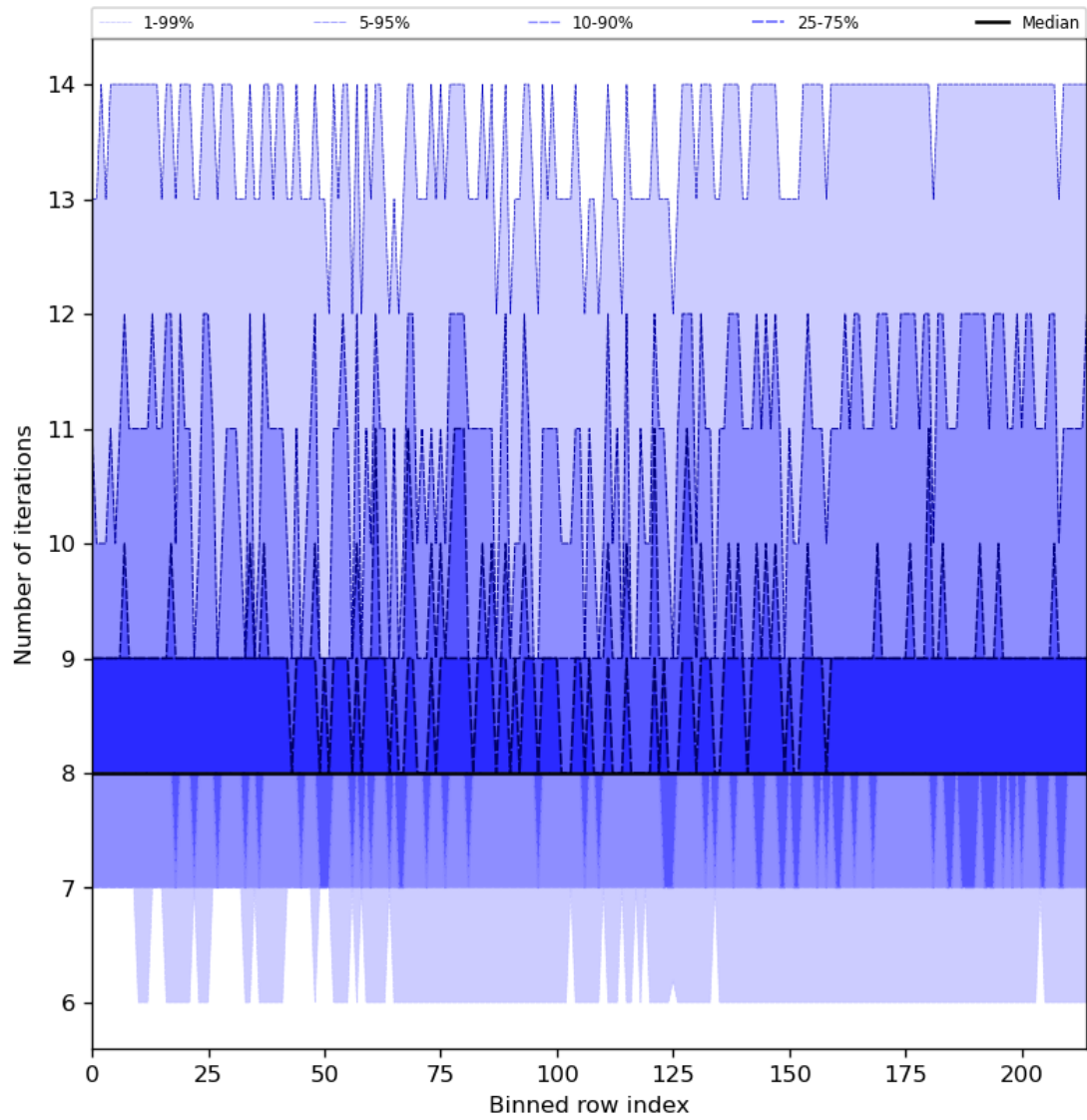
Figure 32: Along track statistics of “Number of iterations” for 2023-09-04 to 2023-09-05
