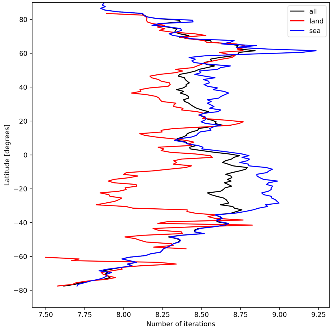
Figure 16: Zonal average of “Number of iterations” for 2023-09-04 to 2023-09-05.
