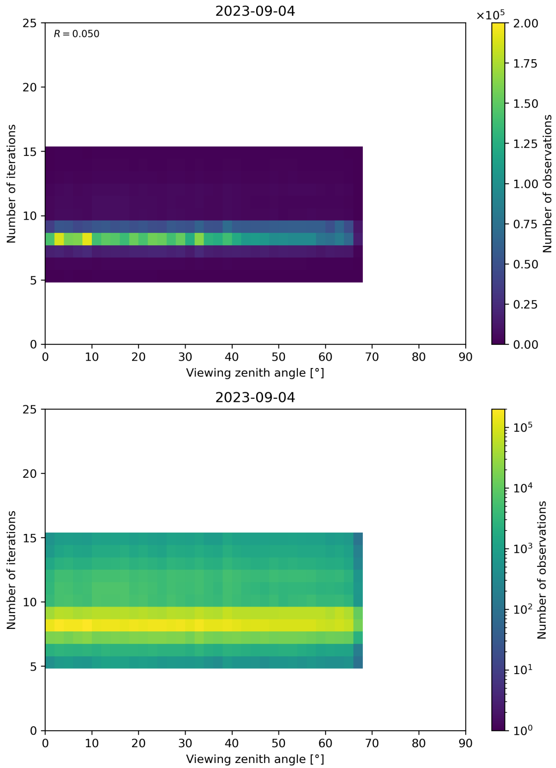
Figure 75: Scatter density plot of “Viewing zenith angle” against “Number of iterations” for 2023-09-04 to 2023-09-05.
