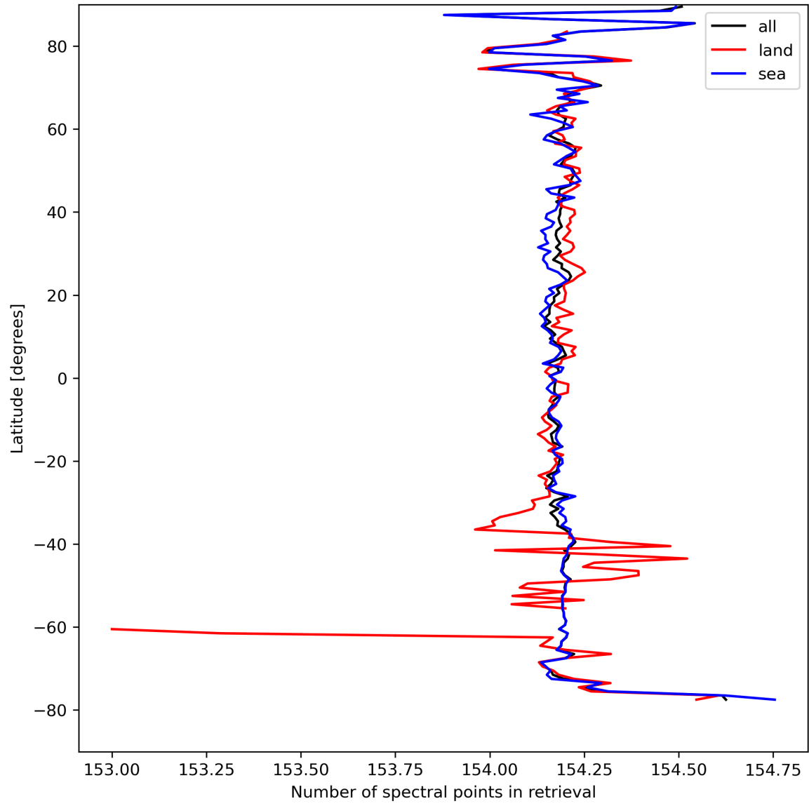
Figure 13: Zonal average of “Number of spectral points in retrieval” for 2023-09-04 to 2023-09-05.
