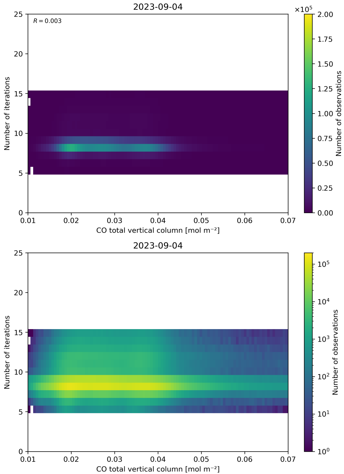
Figure 42: Scatter density plot of “CO total vertical column” against “Number of iterations” for 2023-09-04 to 2023-09-05.
