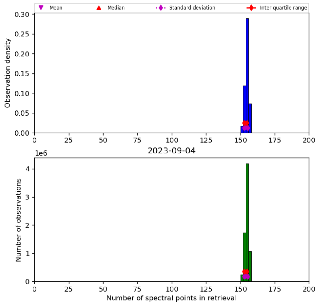
Figure 21: Histogram of “Number of spectral points in retrieval” for 2023-09-04 to 2023-09-05
