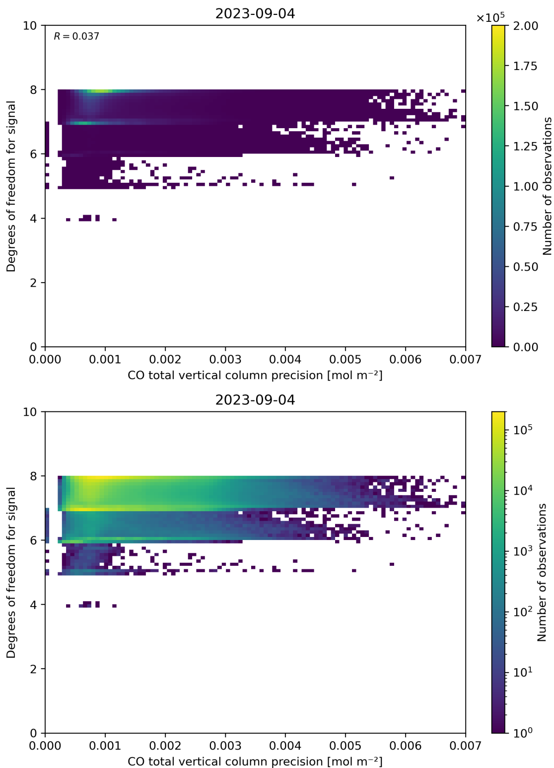
Figure 45: Scatter density plot of “CO total vertical column precision” against “Degrees of freedom for signal” for 2023-09-04 to 2023-09-05.
