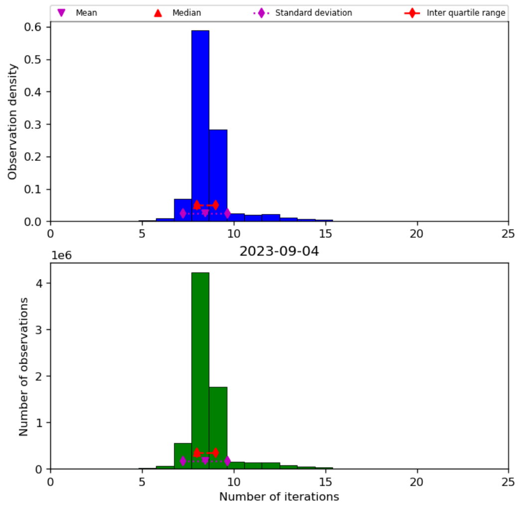
Figure 24: Histogram of “Number of iterations” for 2023-09-04 to 2023-09-05
