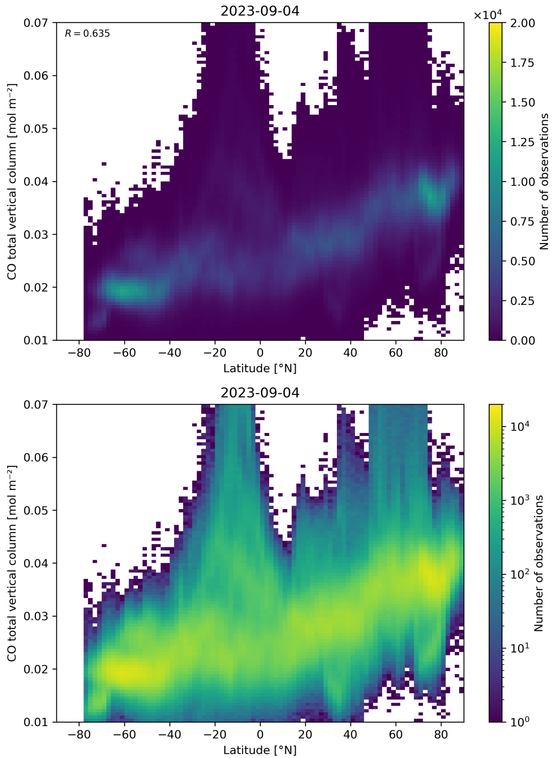
Figure 51: Scatter density plot of “Latitude” against “CO total vertical column” for 2023-09-04 to 2023-09-05.
