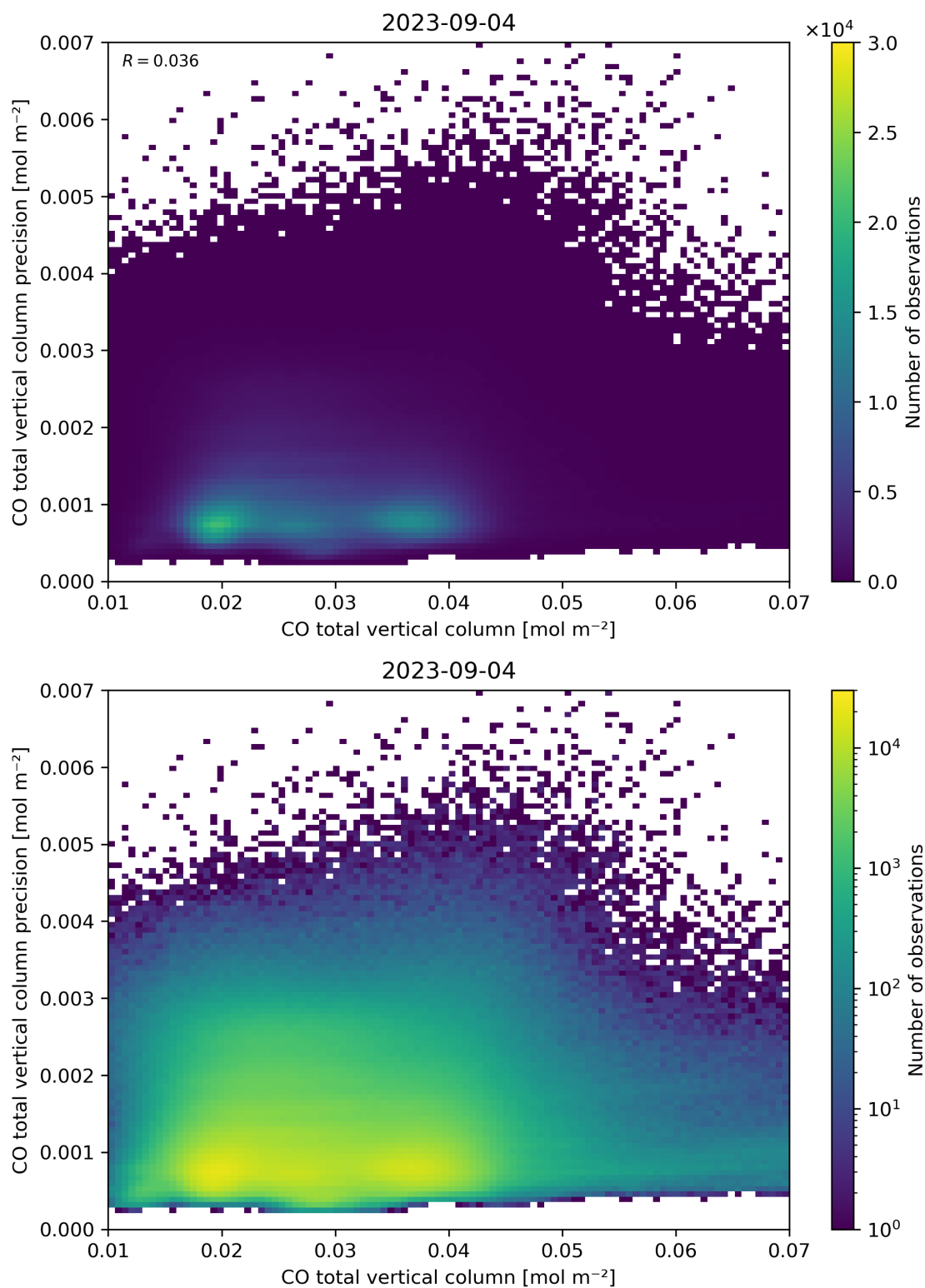
Figure 34: Scatter density plot of “CO total vertical column” against “CO total vertical column precision” for 2023-09-04 to 2023-09-05.
