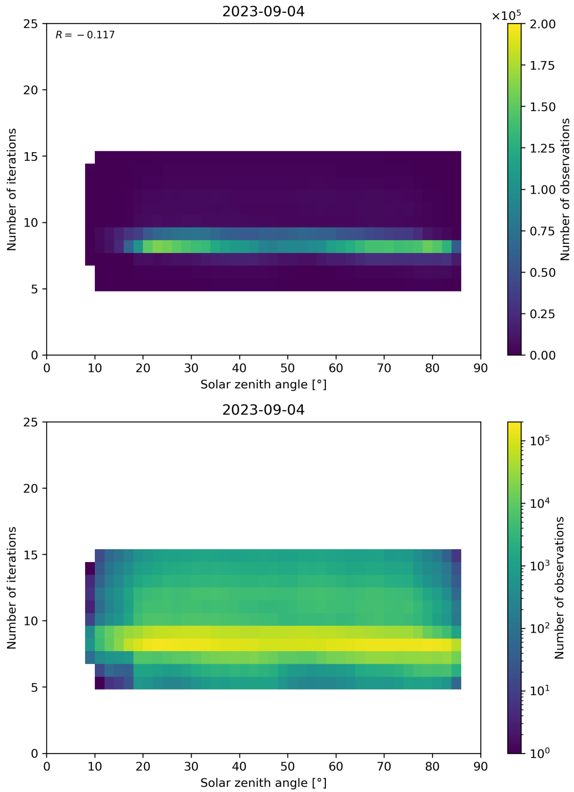
Figure 67: Scatter density plot of “Solar zenith angle” against “Number of iterations” for 2023-09-04 to 2023-09-05.
