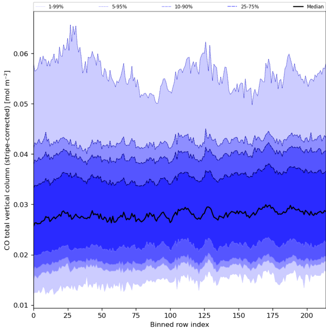
Figure 27: Along track statistics of “CO total vertical column (stripe-corrected)” for 2023-09-04 to 2023-09-05
