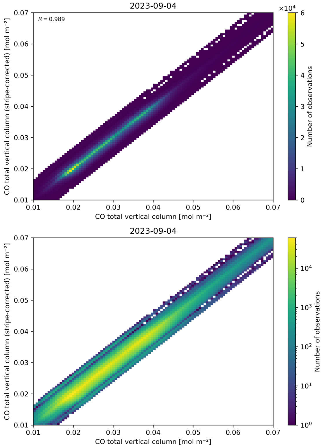
Figure 33: Scatter density plot of “CO total vertical column” against “CO total vertical column (stripe-corrected)” for 2023-09-04 to 2023-09-05.
