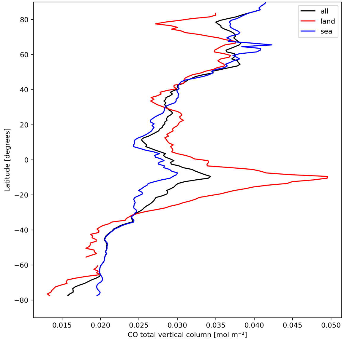
Figure 10: Zonal average of “CO total vertical column” for 2023-09-04 to 2023-09-05.
