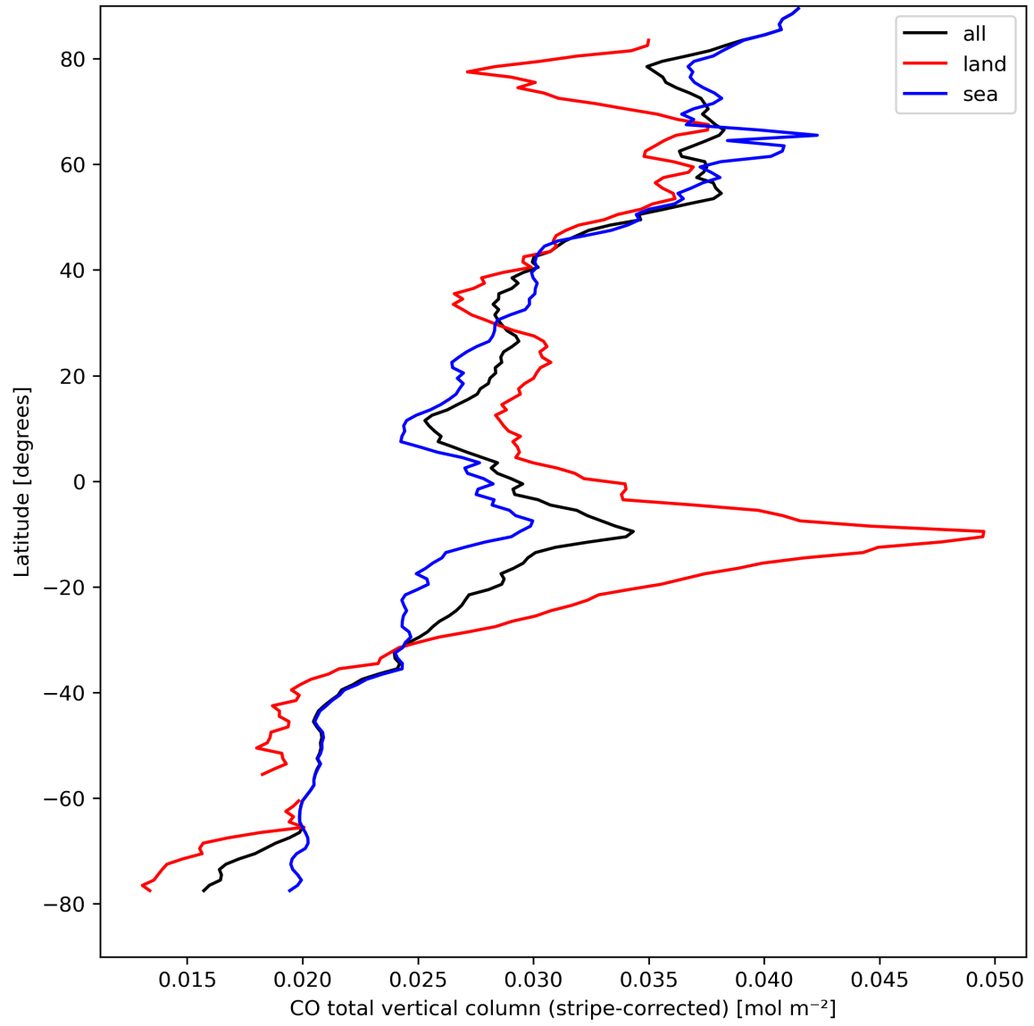
Figure 11: Zonal average of “CO total vertical column (stripe-corrected)” for 2023-09-04 to 2023-09-05.
