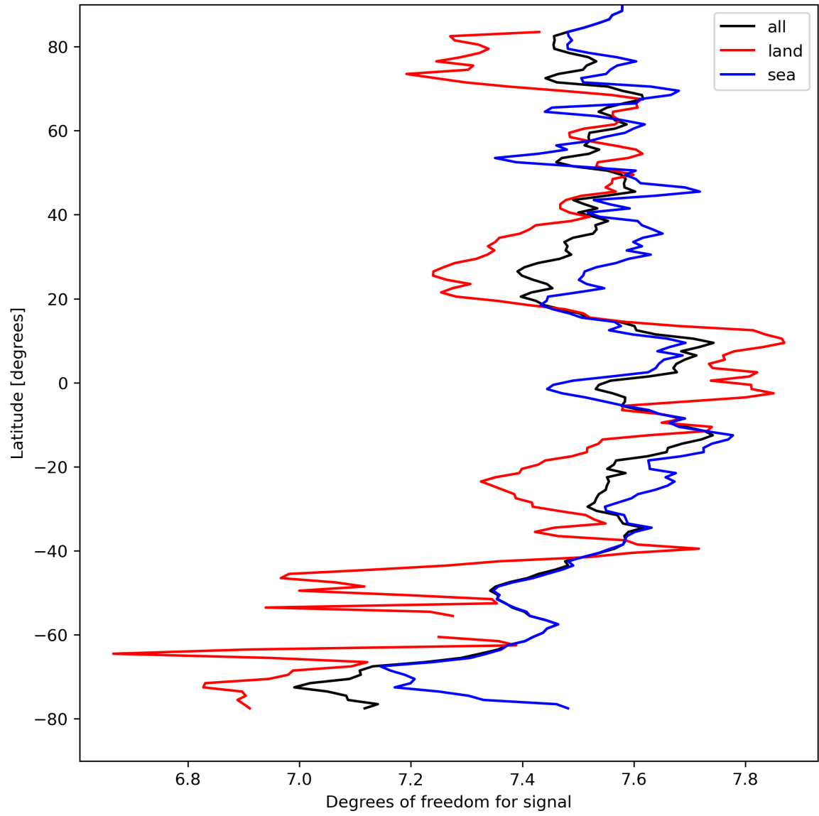
Figure 15: Zonal average of “Degrees of freedom for signal” for 2023-09-04 to 2023-09-05.
