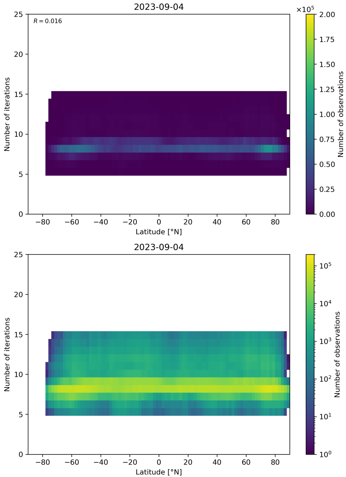
Figure 56: Scatter density plot of “Latitude” against “Number of iterations” for 2023-09-04 to 2023-09-05.
