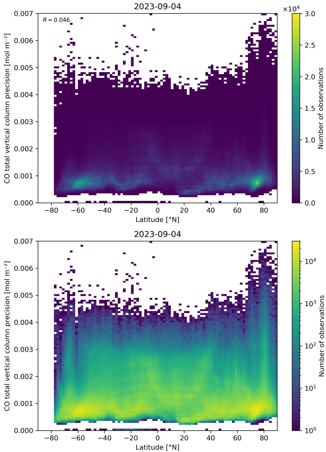
Figure 53: Scatter density plot of “Latitude” against “CO total vertical column precision” for 2023-09-04 to 2023-09-05.
