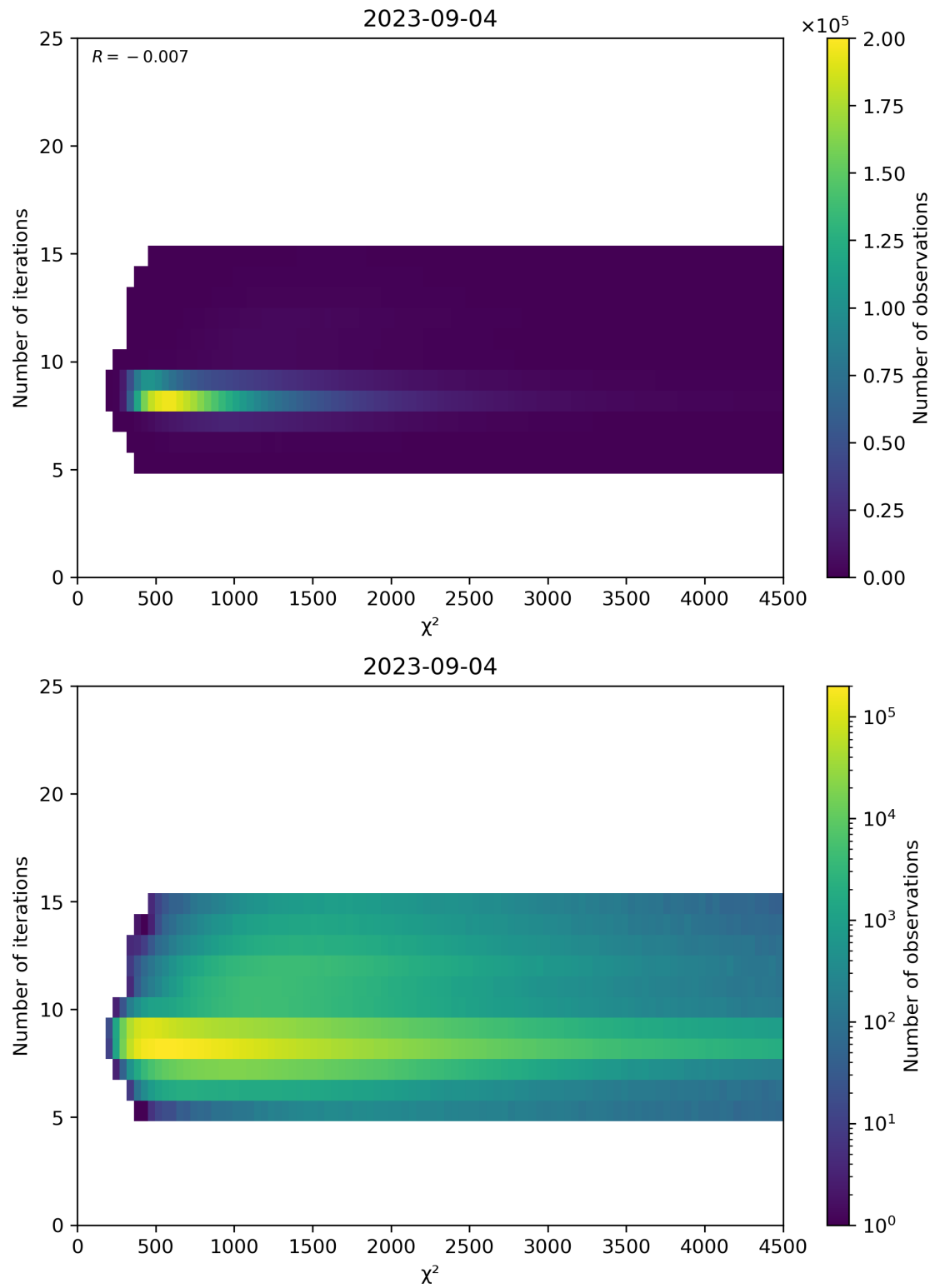
Figure 49: Scatter density plot of “ \chi^2 ” against “Number of iterations” for 2023-09-04 to 2023-09-05.
