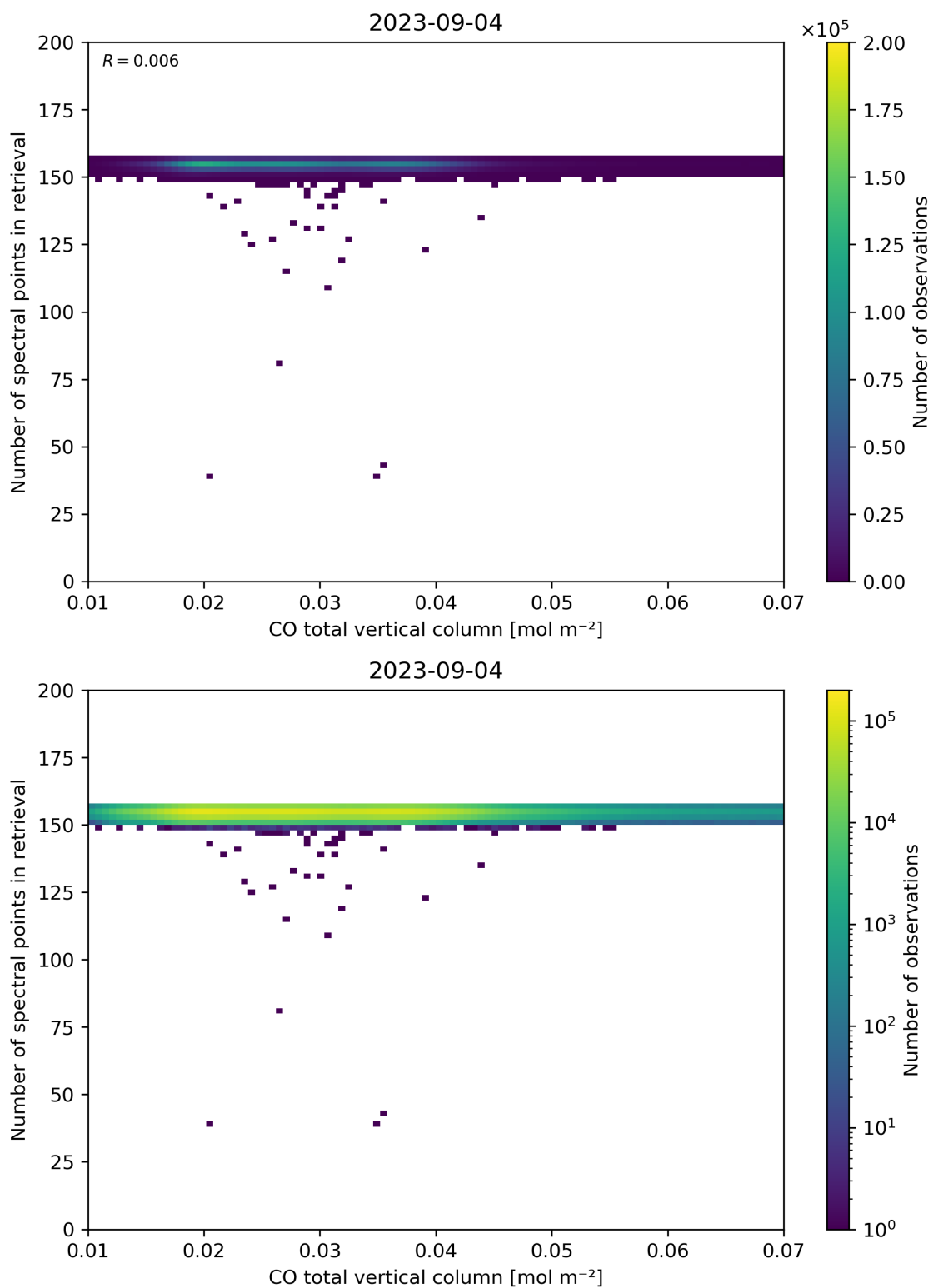
Figure 43: Scatter density plot of “CO total vertical column” against “Number of spectral points in retrieval” for 2023-09-04 to 2023-09-05.
