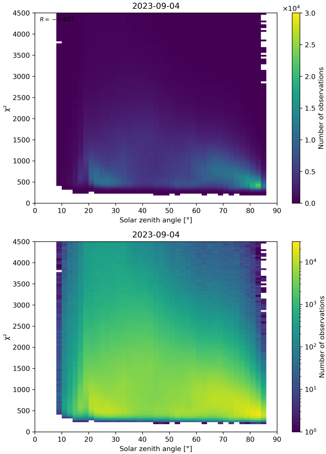
Figure 64: Scatter density plot of “Solar zenith angle” against “ \chi^2 ” for 2023-09-04 to 2023-09-05.
