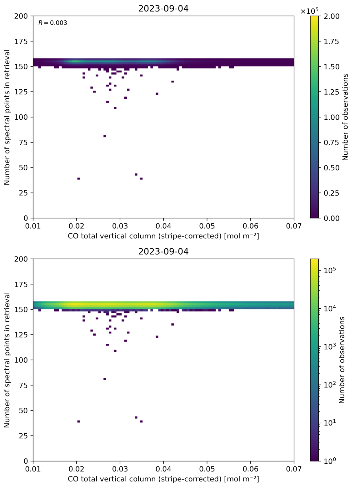
Figure 40: Scatter density plot of “CO total vertical column (stripe-corrected)” against “Number of spectral points in retrieval” for 2023-09-04 to 2023-09-05.
