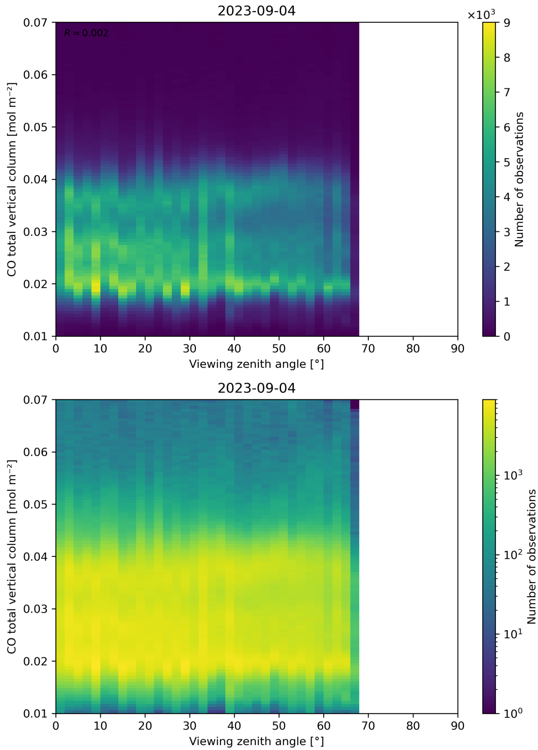
Figure 69: Scatter density plot of “Viewing zenith angle” against “CO total vertical column” for 2023-09-04 to 2023-09-05.
