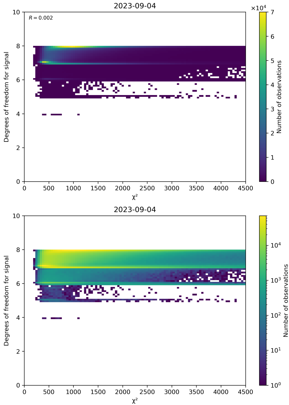
Figure 48: Scatter density plot of " \chi^2 " against "Degrees of freedom for signal" for 2023-09-04 to 2023-09-05.
