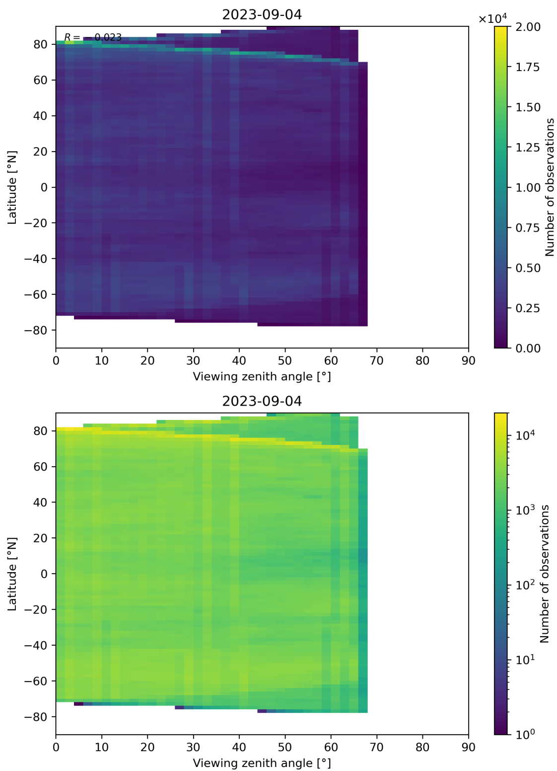
Figure 74: Scatter density plot of “Viewing zenith angle” against “Latitude” for 2023-09-04 to 2023-09-05.
