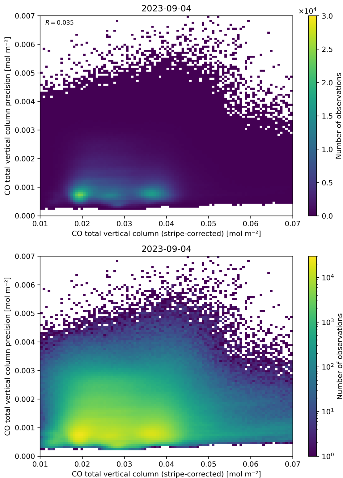
Figure 36: Scatter density plot of “CO total vertical column (stripe-corrected)” against “CO total vertical column precision” for 2023-09-04 to 2023-09-05.
