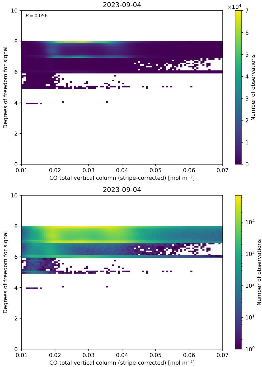
Figure 38: Scatter density plot of “CO total vertical column (stripe-corrected)” against “Degrees of freedom for signal” for 2023-09-04 to 2023-09-05.
