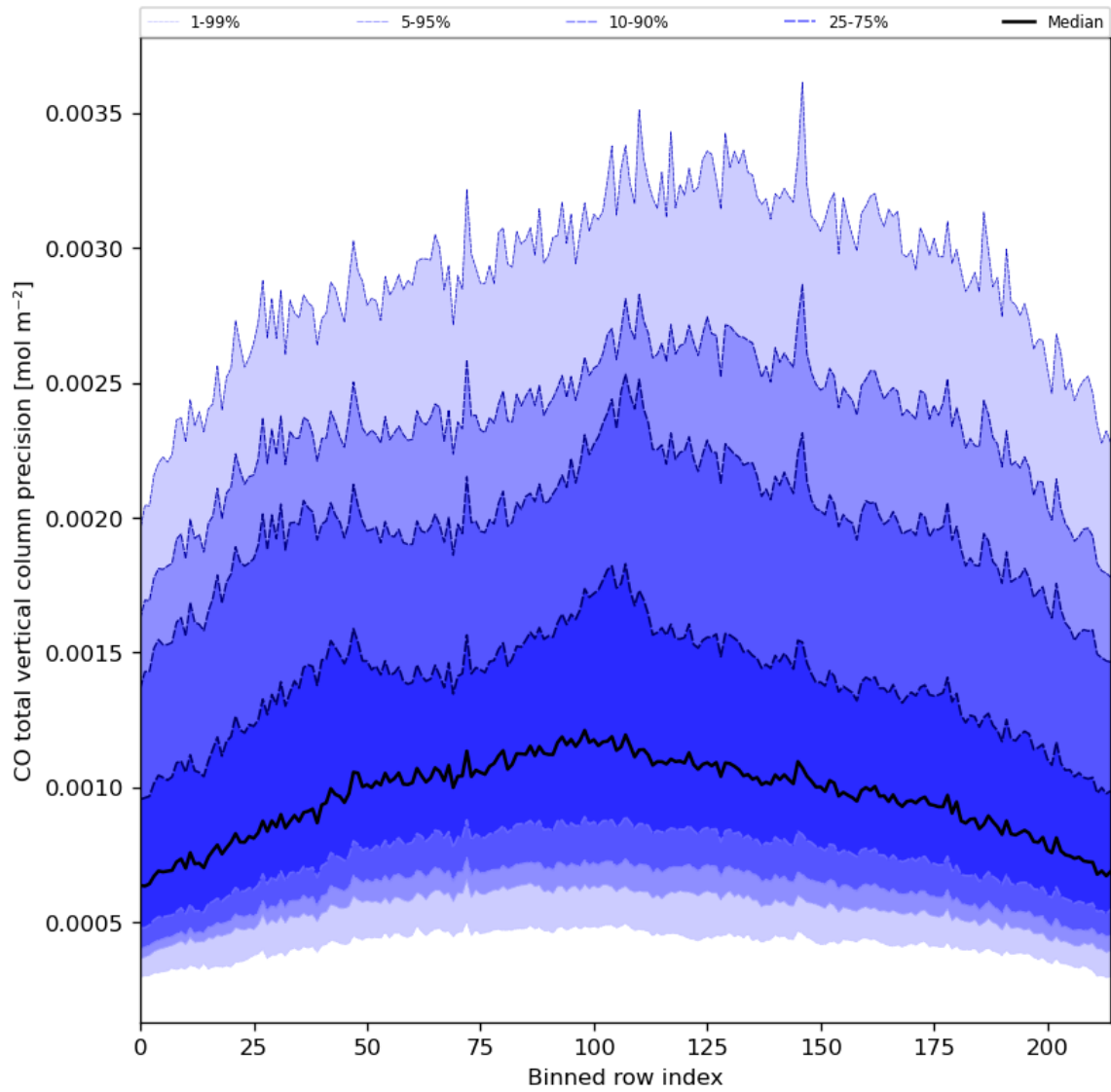
Figure 28: Along track statistics of “CO total vertical column precision” for 2023-09-04 to 2023-09-05
