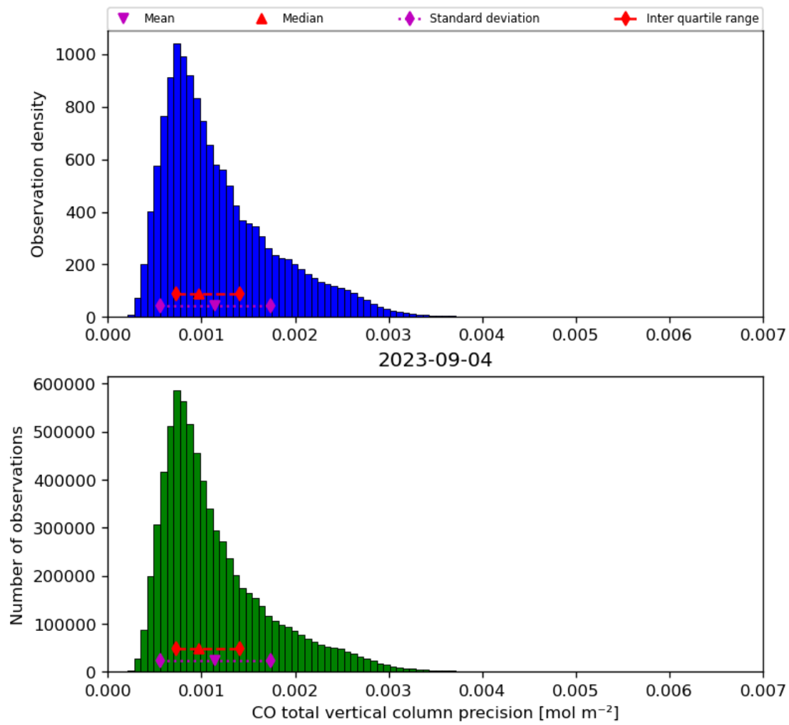
Figure 20: Histogram of “CO total vertical column precision” for 2023-09-04 to 2023-09-05
