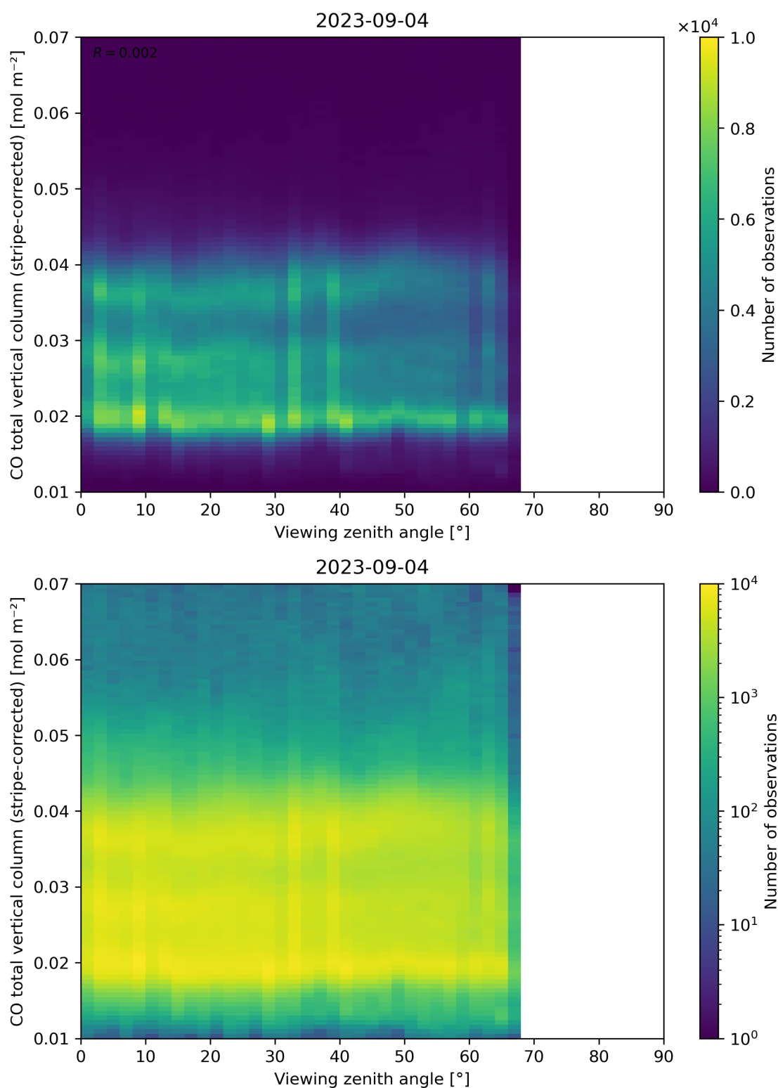
Figure 70: Scatter density plot of “Viewing zenith angle” against “CO total vertical column (stripe-corrected)” for 2023-09-04 to 2023-09-05.
