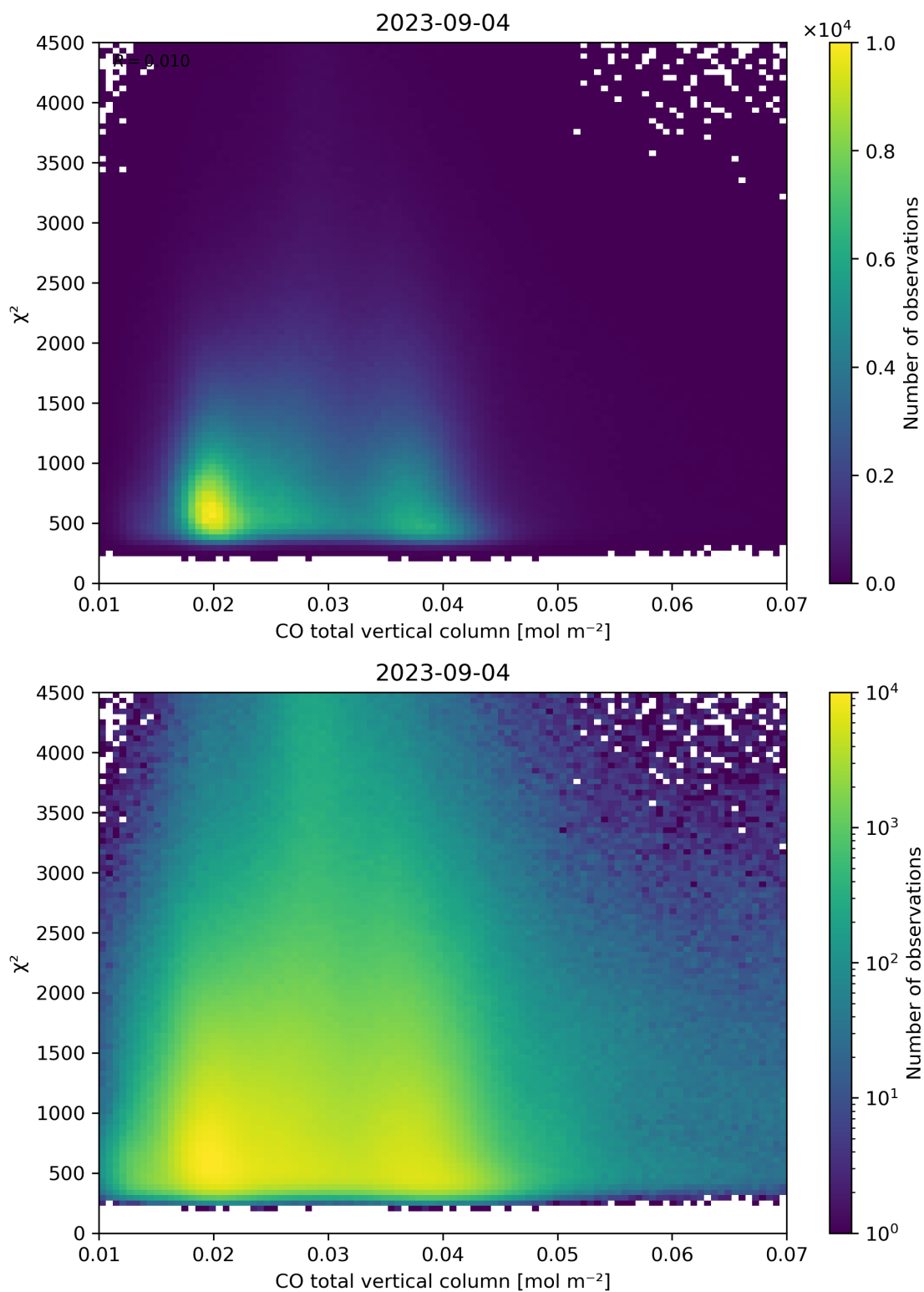
Figure 35: Scatter density plot of “CO total vertical column” against “ \chi^2 ” for 2023-09-04 to 2023-09-05.
