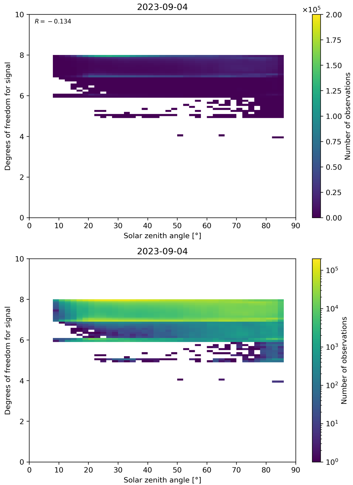
Figure 65: Scatter density plot of “Solar zenith angle” against “Degrees of freedom for signal” for 2023-09-04 to 2023-09-05.
