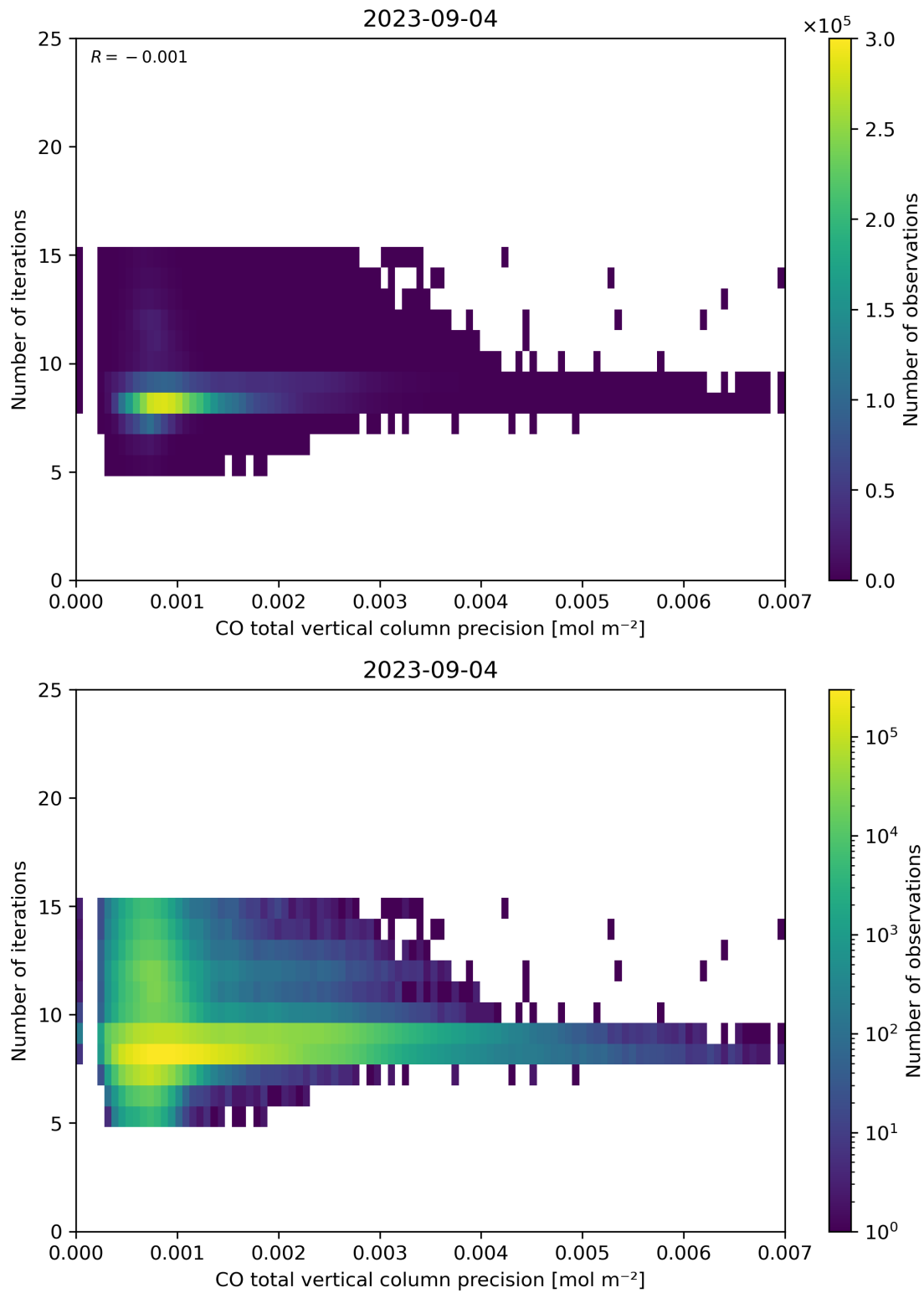
Figure 46: Scatter density plot of “CO total vertical column precision” against “Number of iterations” for 2023-09-04 to 2023-09-05.
