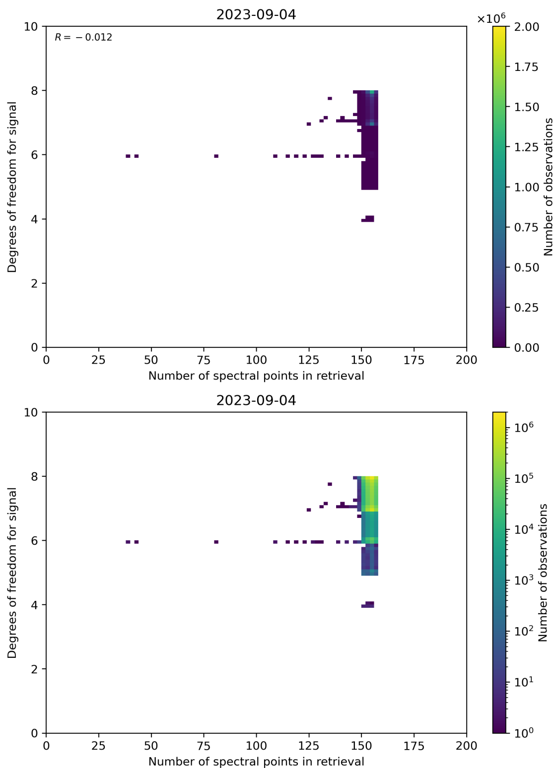
Figure 59: Scatter density plot of “Number of spectral points in retrieval” against “Degrees of freedom for signal” for 2023-09-04 to 2023-09-05.
