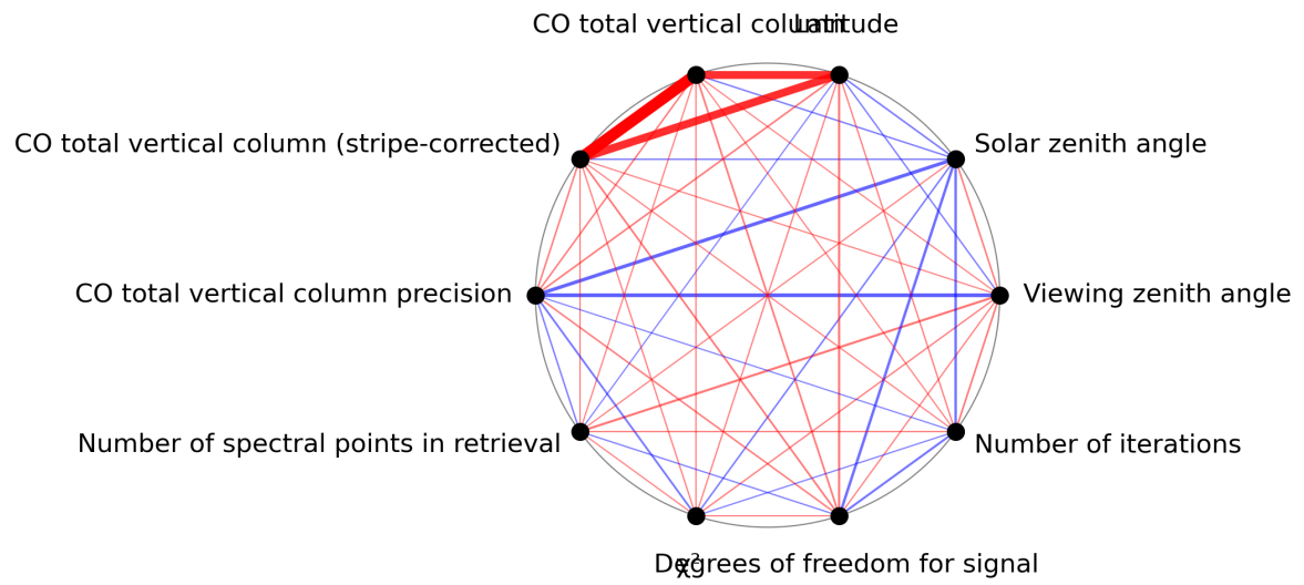
Figure 1: Map of correlation graph for 2023-09-04 to 2023-09-05.
