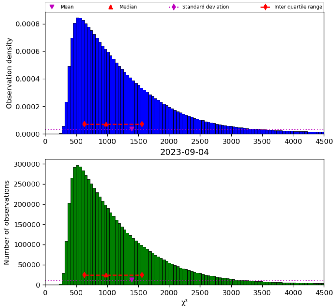
Figure 22: Histogram of “ \chi^2 ” for 2023-09-04 to 2023-09-05
