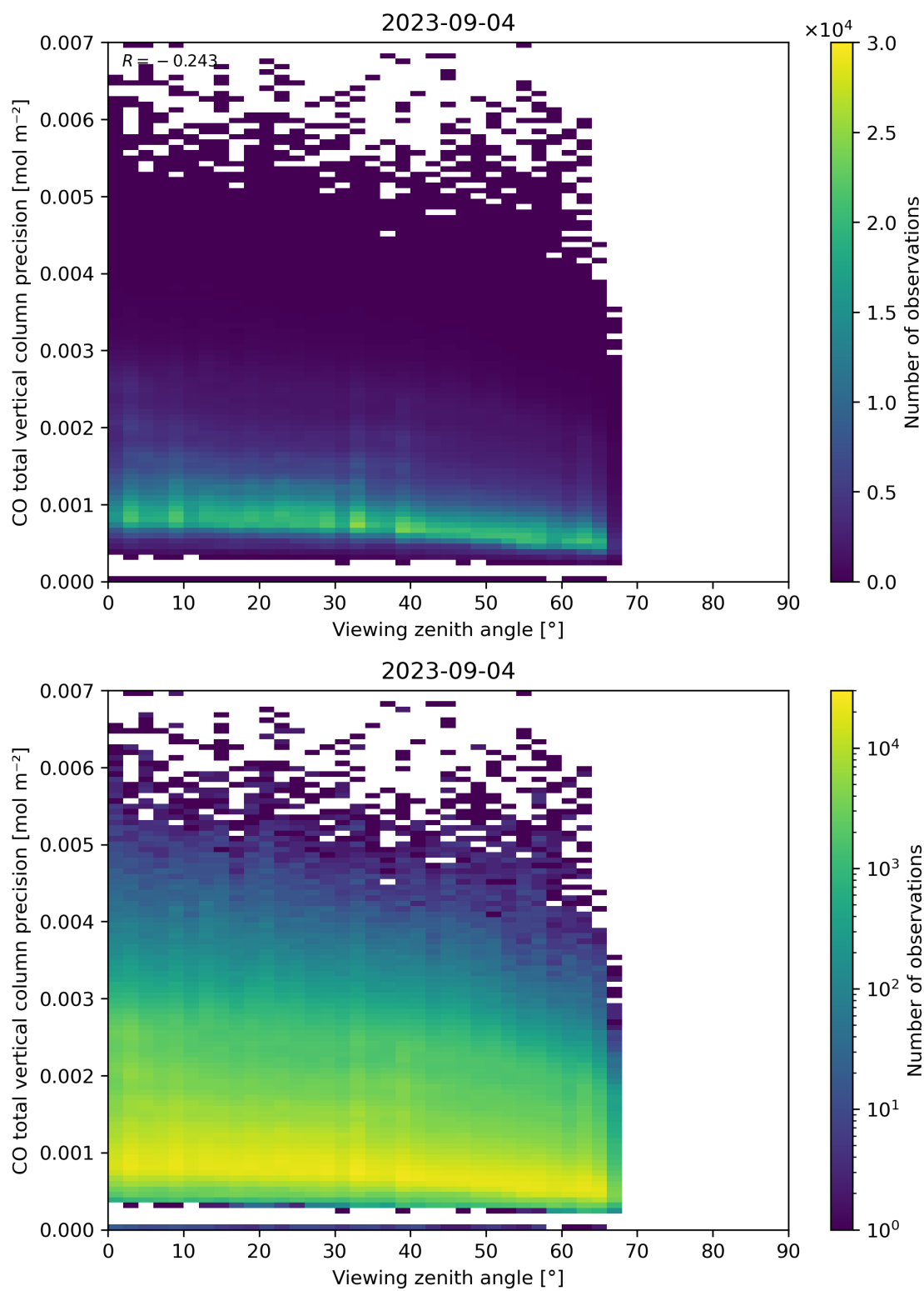
Figure 71: Scatter density plot of “Viewing zenith angle” against “CO total vertical column precision” for 2023-09-04 to 2023-09-05.
