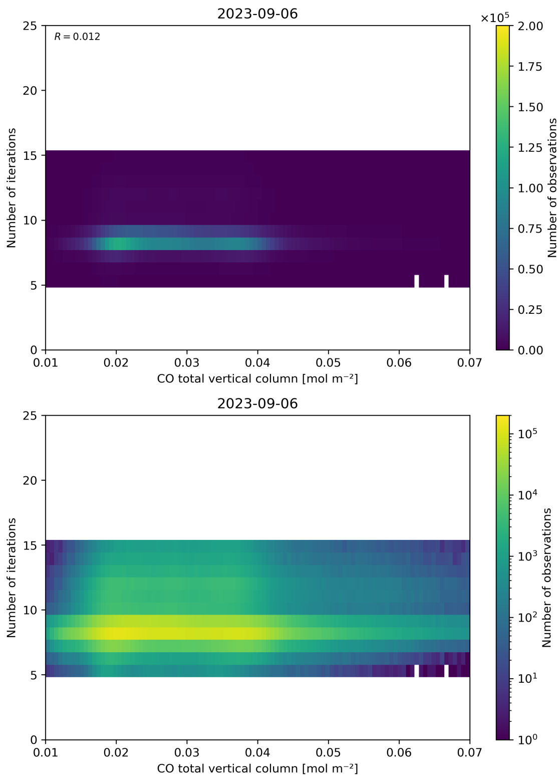
Figure 42: Scatter density plot of “CO total vertical column” against “Number of iterations” for 2023-09-05 to 2023-09-07.
