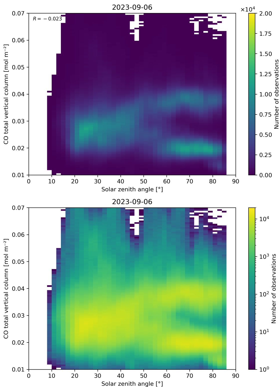
Figure 61: Scatter density plot of “Solar zenith angle” against “CO total vertical column” for 2023-09-05 to 2023-09-07.
