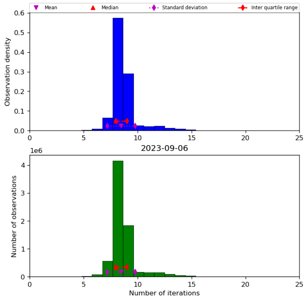
Figure 24: Histogram of “Number of iterations” for 2023-09-05 to 2023-09-07
