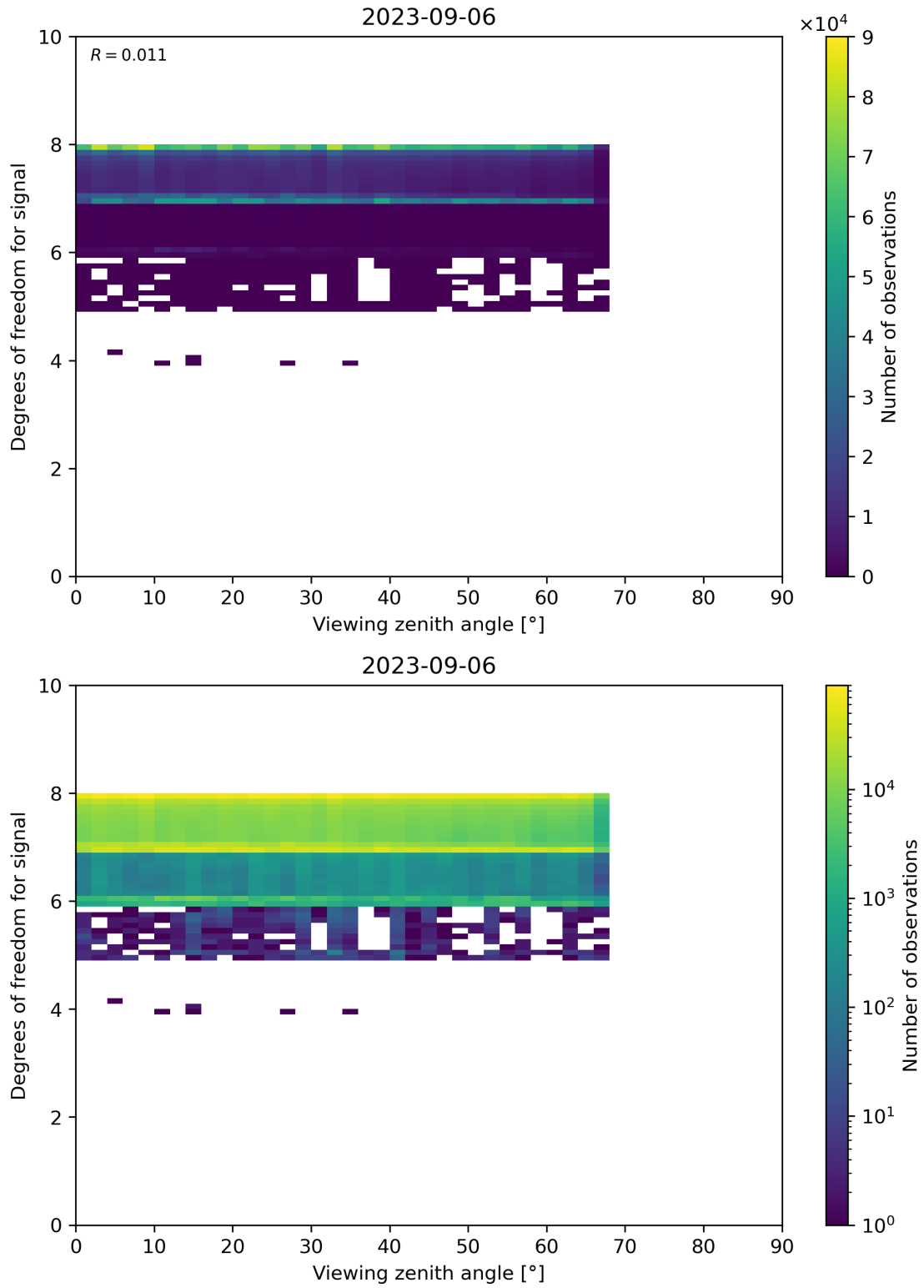
Figure 73: Scatter density plot of “Viewing zenith angle” against “Degrees of freedom for signal” for 2023-09-05 to 2023-09-07.
