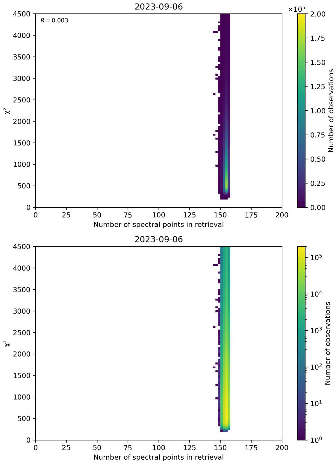
Figure 58: Scatter density plot of “Number of spectral points in retrieval” against “ \chi^2 ” for 2023-09-05 to 2023-09-07.
