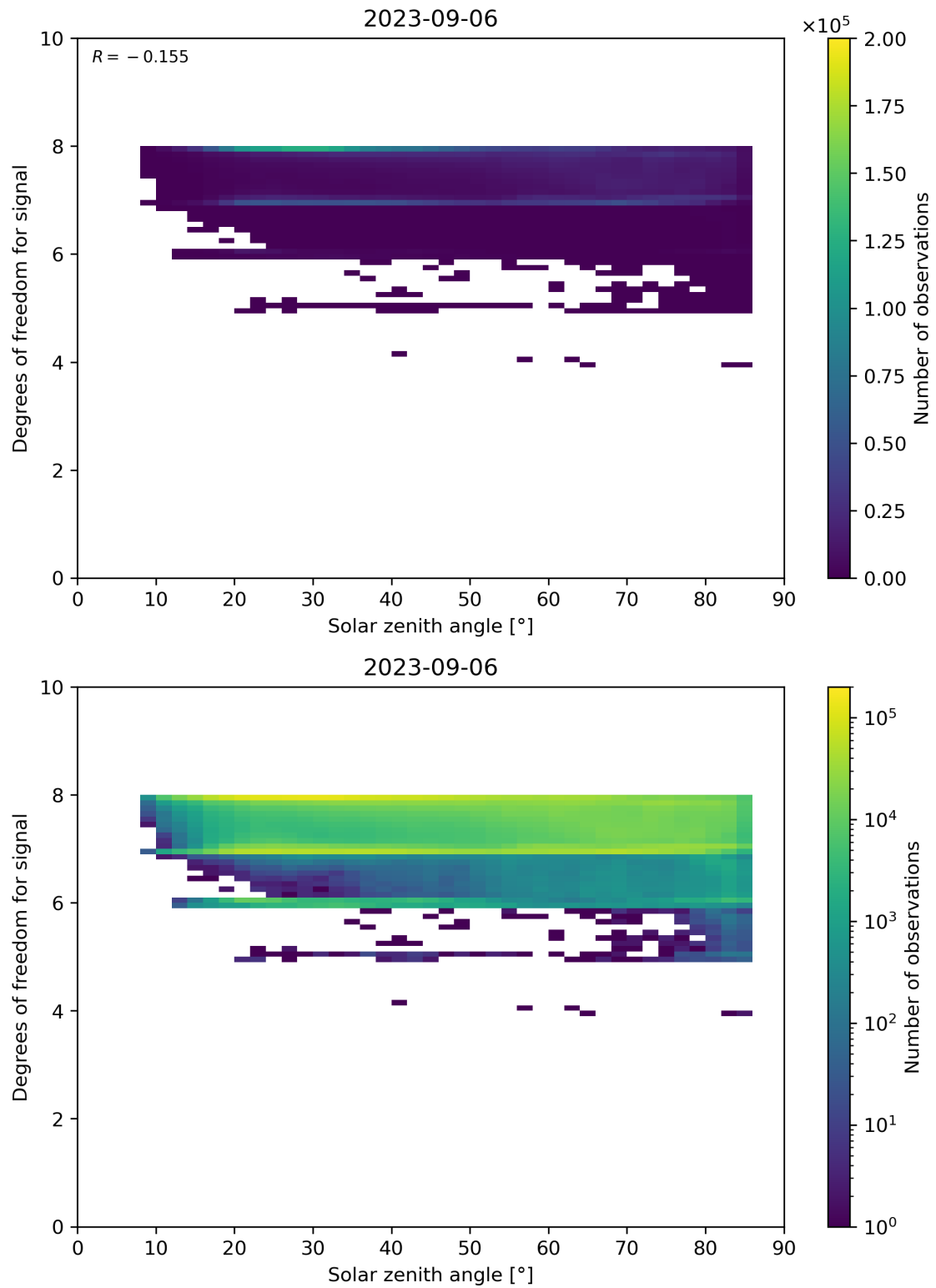
Figure 65: Scatter density plot of “Solar zenith angle” against “Degrees of freedom for signal” for 2023-09-05 to 2023-09-07.
