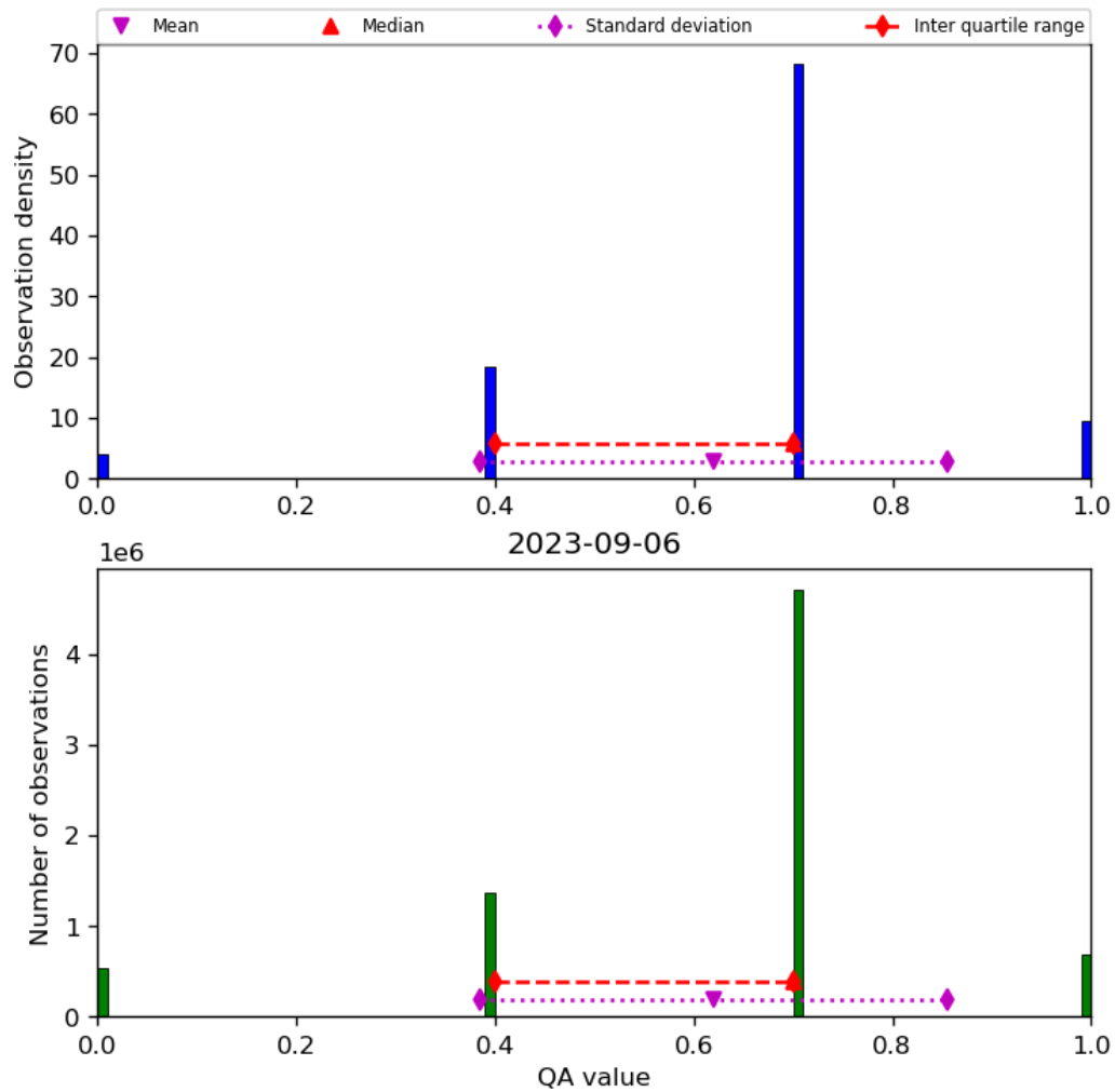
Figure 17: Histogram of “QA value” for 2023-09-05 to 2023-09-07
