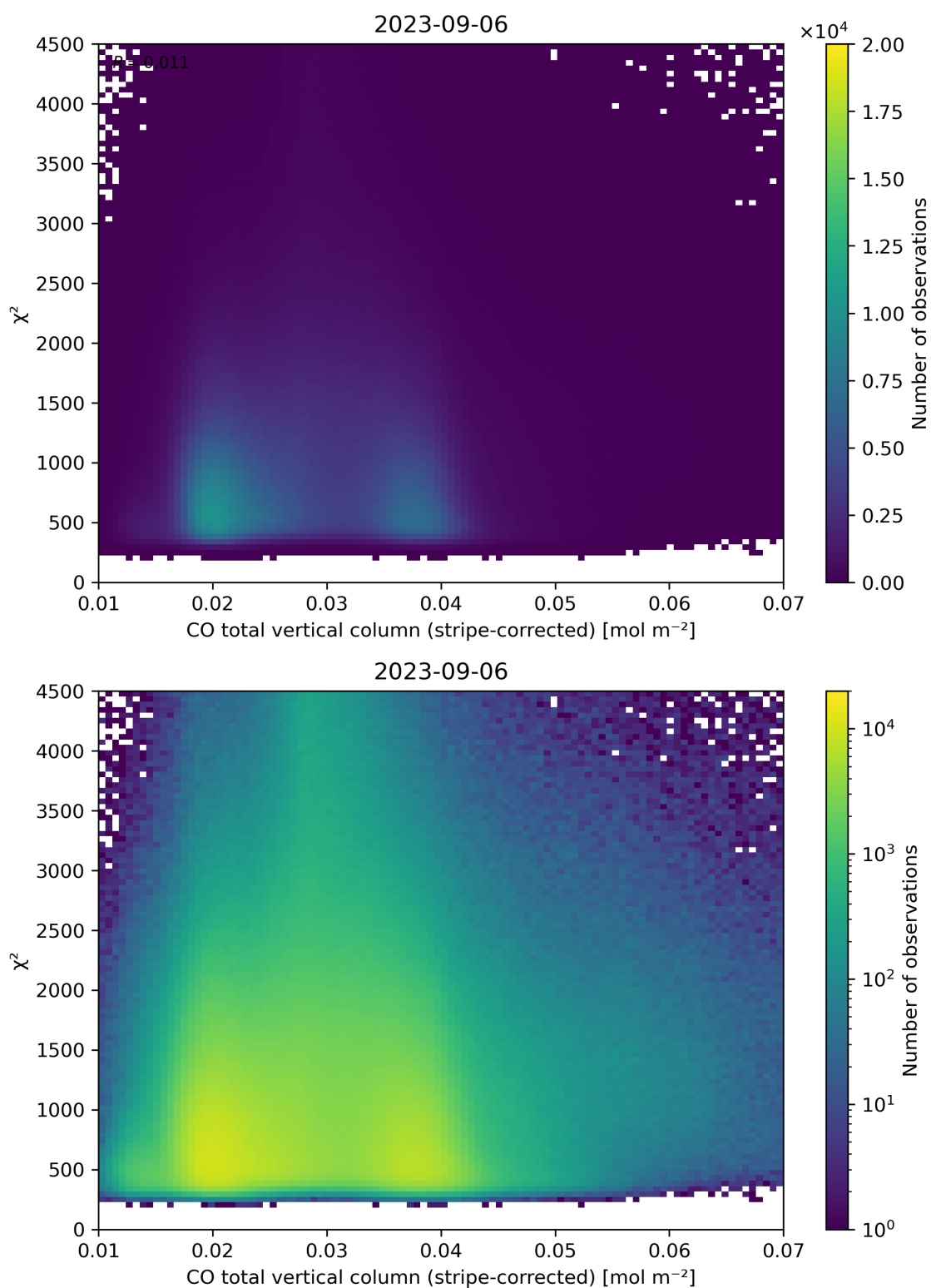
Figure 37: Scatter density plot of “CO total vertical column (stripe-corrected)” against “ \chi^2 ” for 2023-09-05 to 2023-09-07.
