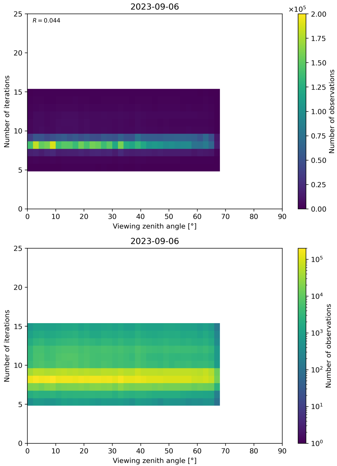
Figure 75: Scatter density plot of “Viewing zenith angle” against “Number of iterations” for 2023-09-05 to 2023-09-07.
