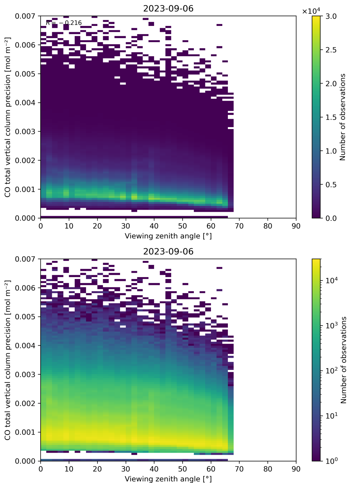
Figure 71: Scatter density plot of “Viewing zenith angle” against “CO total vertical column precision” for 2023-09-05 to 2023-09-07.
