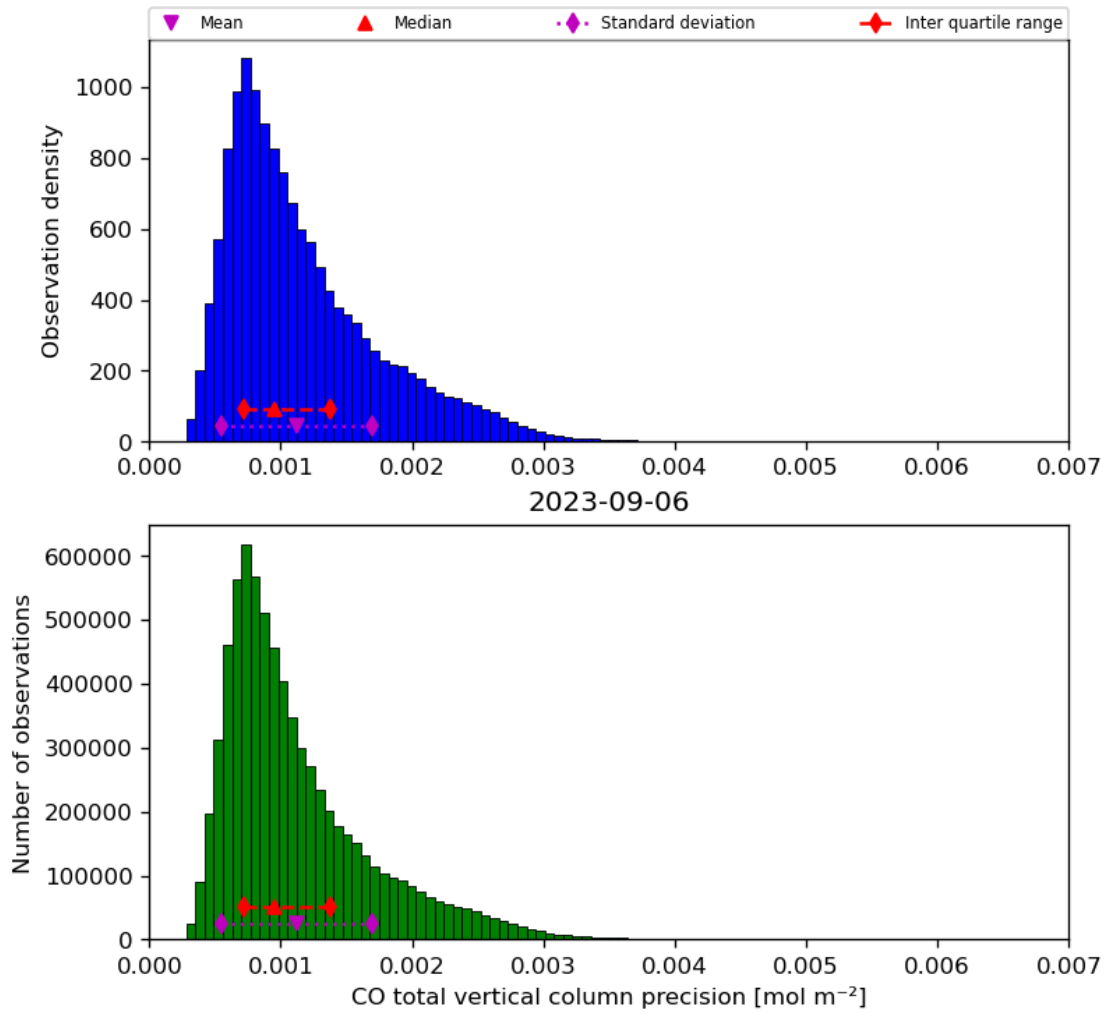
Figure 20: Histogram of “CO total vertical column precision” for 2023-09-05 to 2023-09-07
