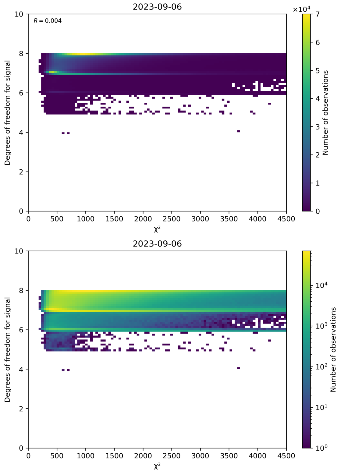
Figure 48: Scatter density plot of “ \chi^2 ” against “Degrees of freedom for signal” for 2023-09-05 to 2023-09-07.
