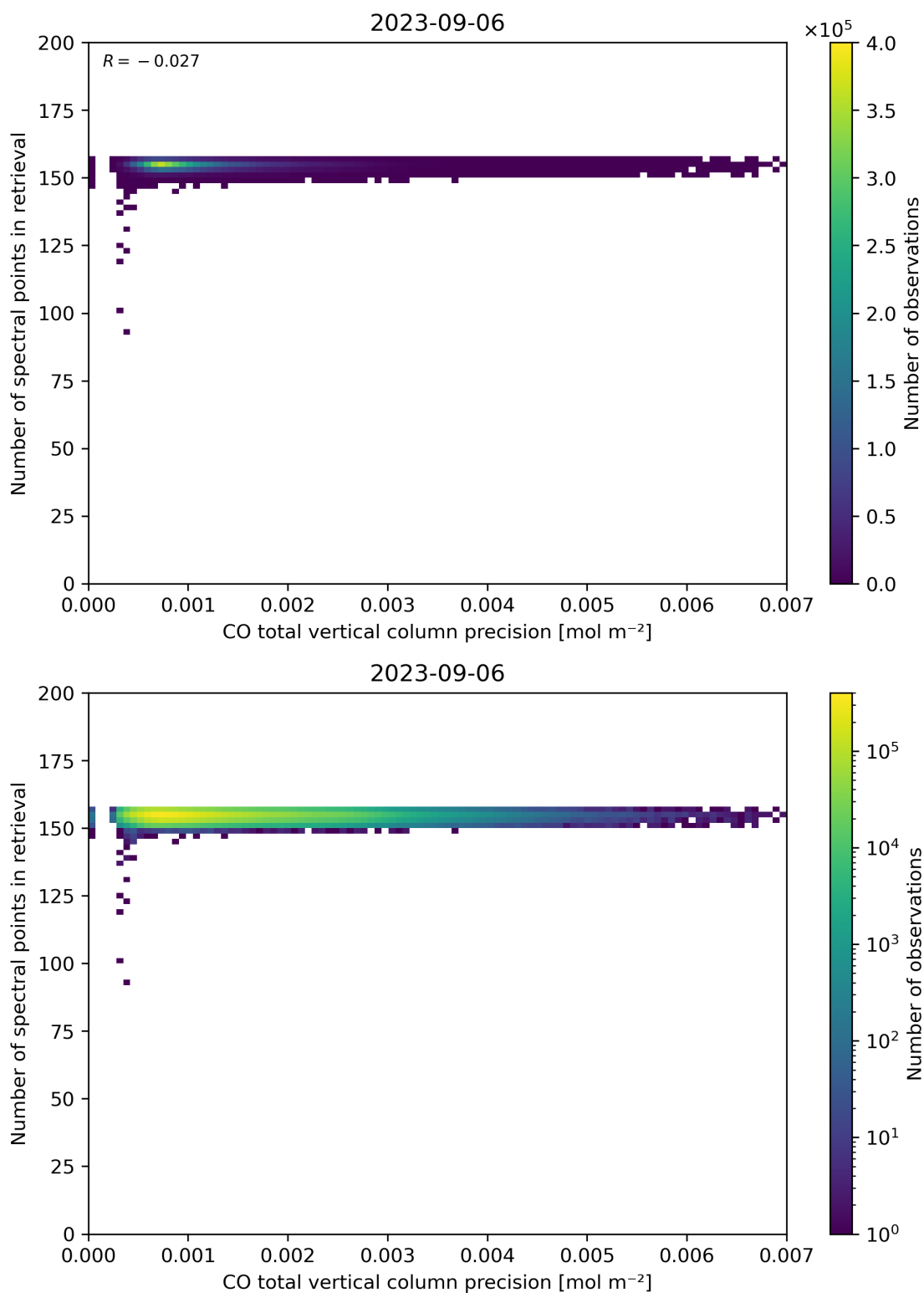
Figure 47: Scatter density plot of “CO total vertical column precision” against “Number of spectral points in retrieval” for 2023-09-05 to 2023-09-07.
