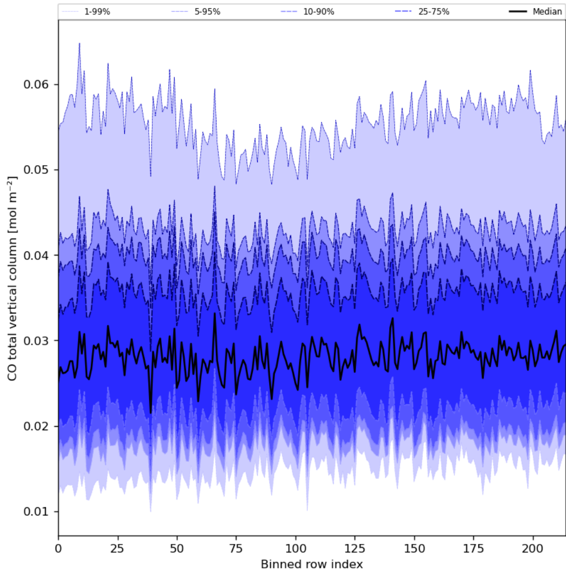
Figure 26: Along track statistics of “CO total vertical column” for 2023-09-05 to 2023-09-07
