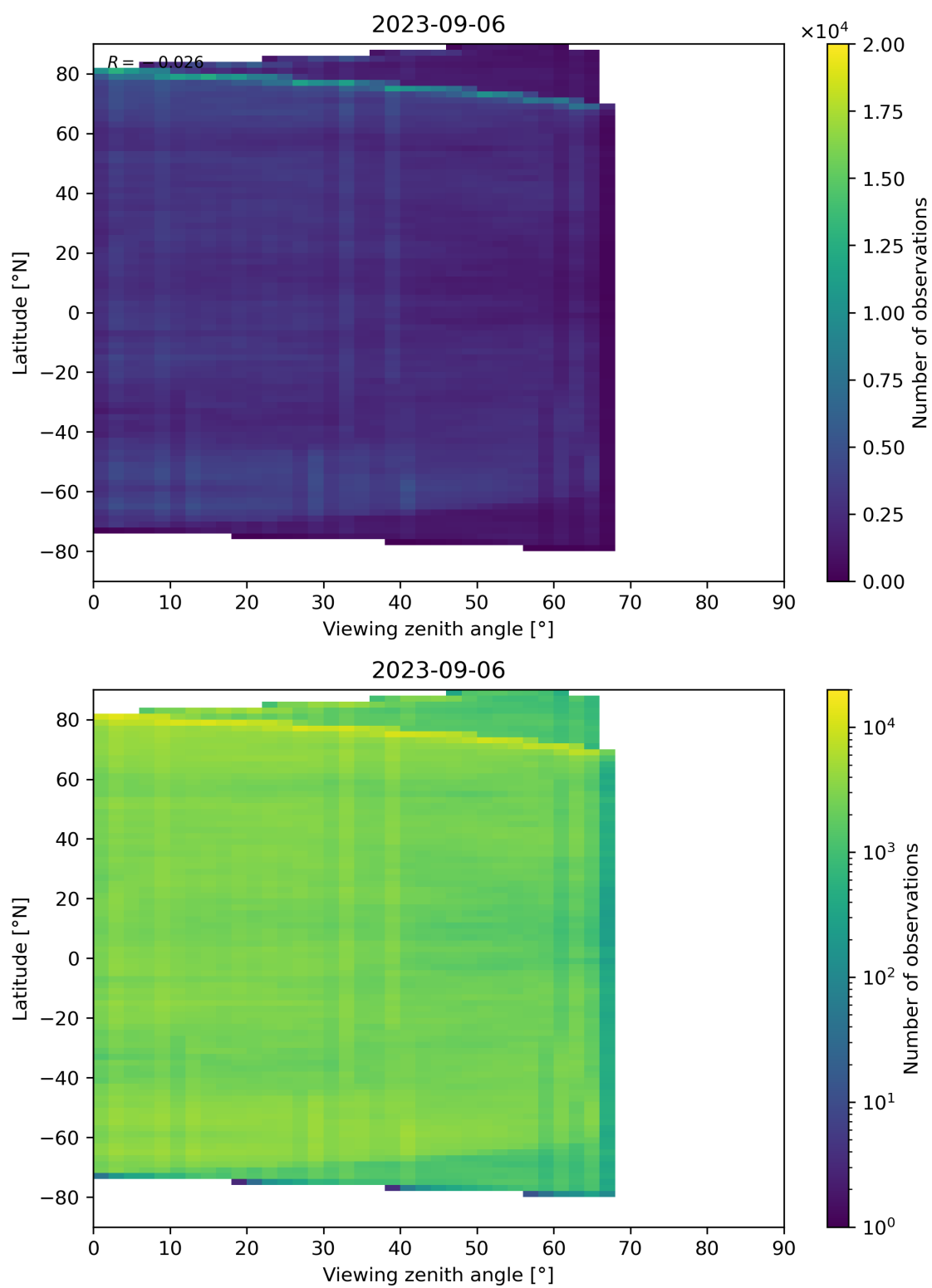
Figure 74: Scatter density plot of “Viewing zenith angle” against “Latitude” for 2023-09-05 to 2023-09-07.
