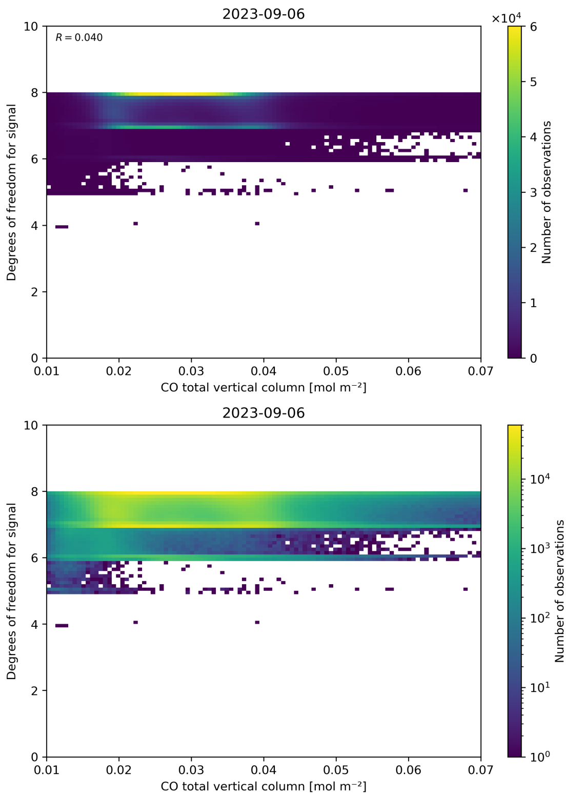
Figure 41: Scatter density plot of “CO total vertical column” against “Degrees of freedom for signal” for 2023-09-05 to 2023-09-07.
