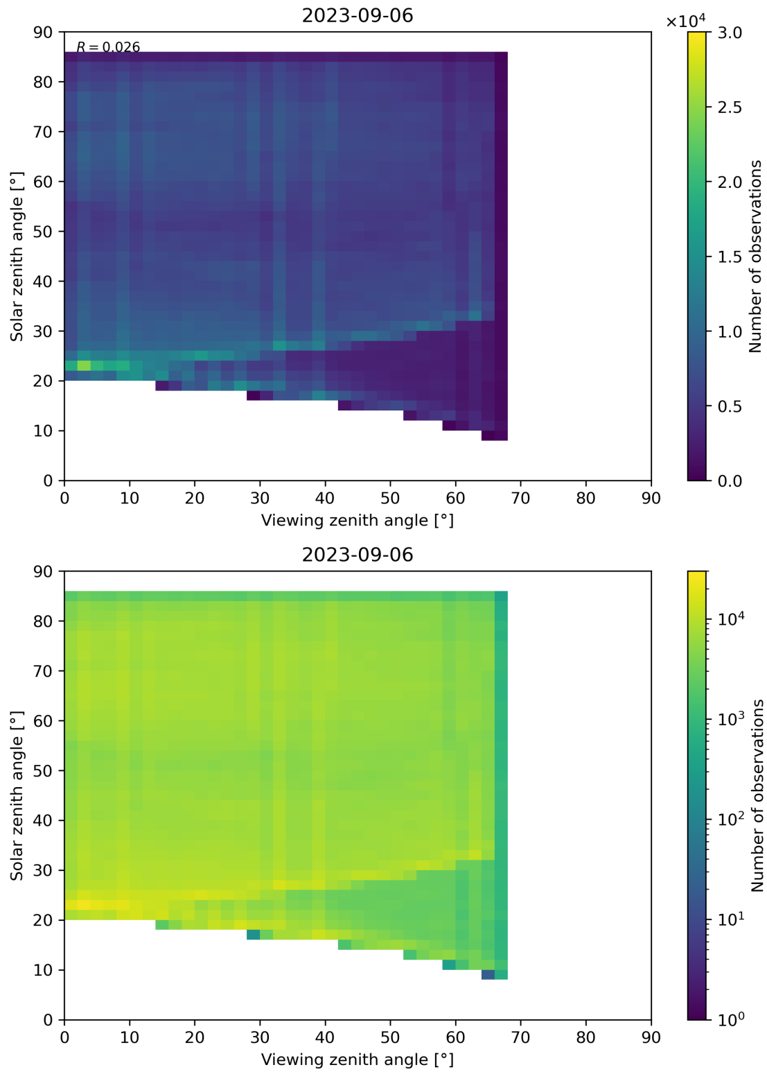
Figure 77: Scatter density plot of “Viewing zenith angle” against “Solar zenith angle” for 2023-09-05 to 2023-09-07.
