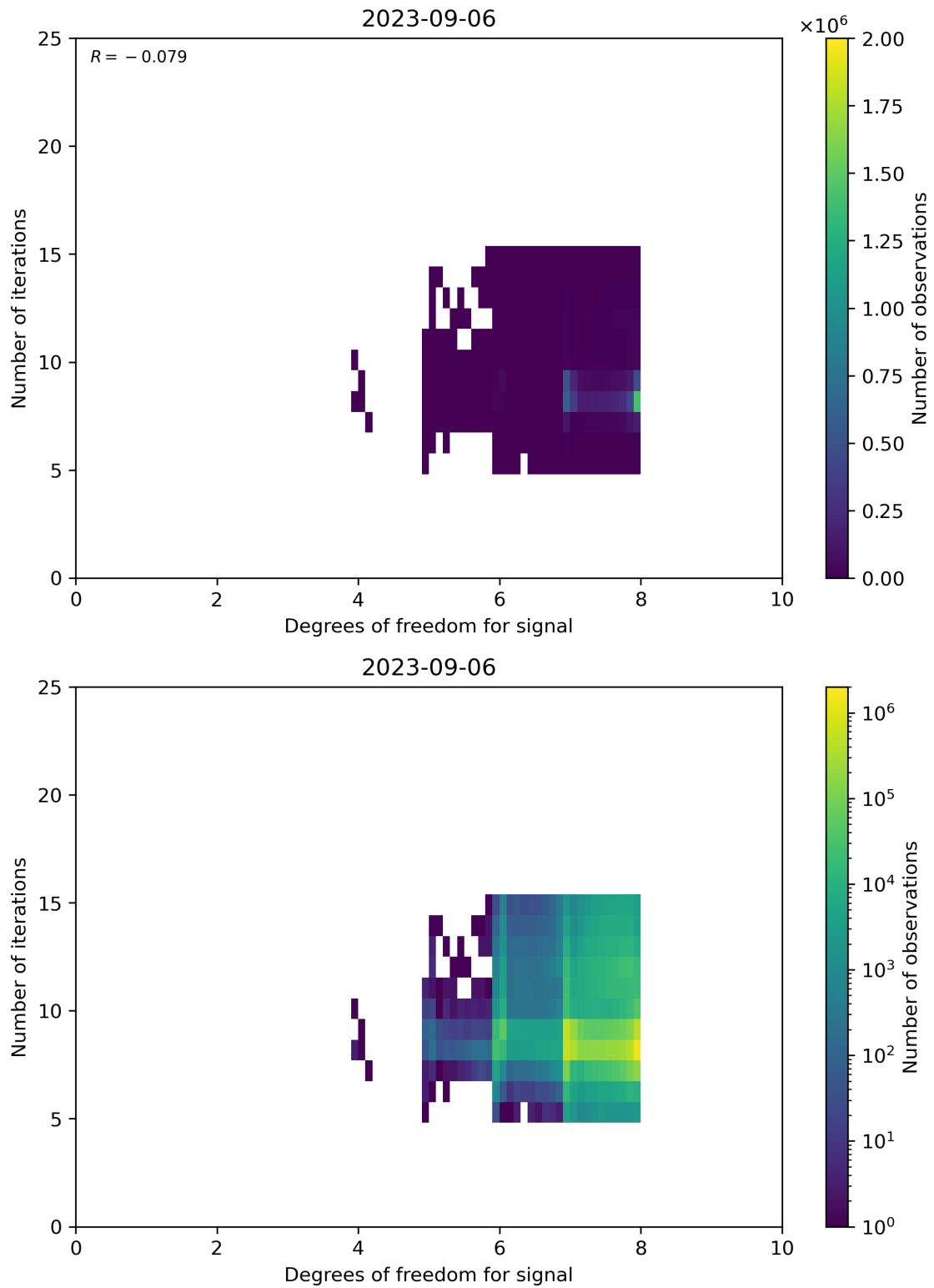
Figure 50: Scatter density plot of “Degrees of freedom for signal” against “Number of iterations” for 2023-09-05 to 2023-09-07.
