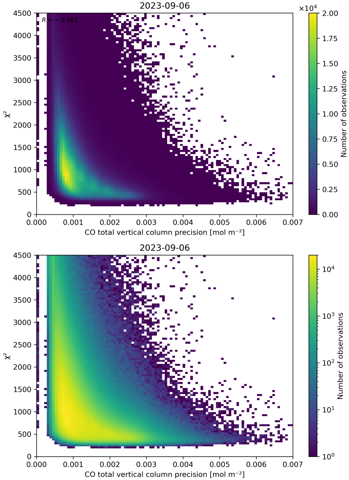
Figure 44: Scatter density plot of “CO total vertical column precision” against “ \chi^2 ” for 2023-09-05 to 2023-09-07.
