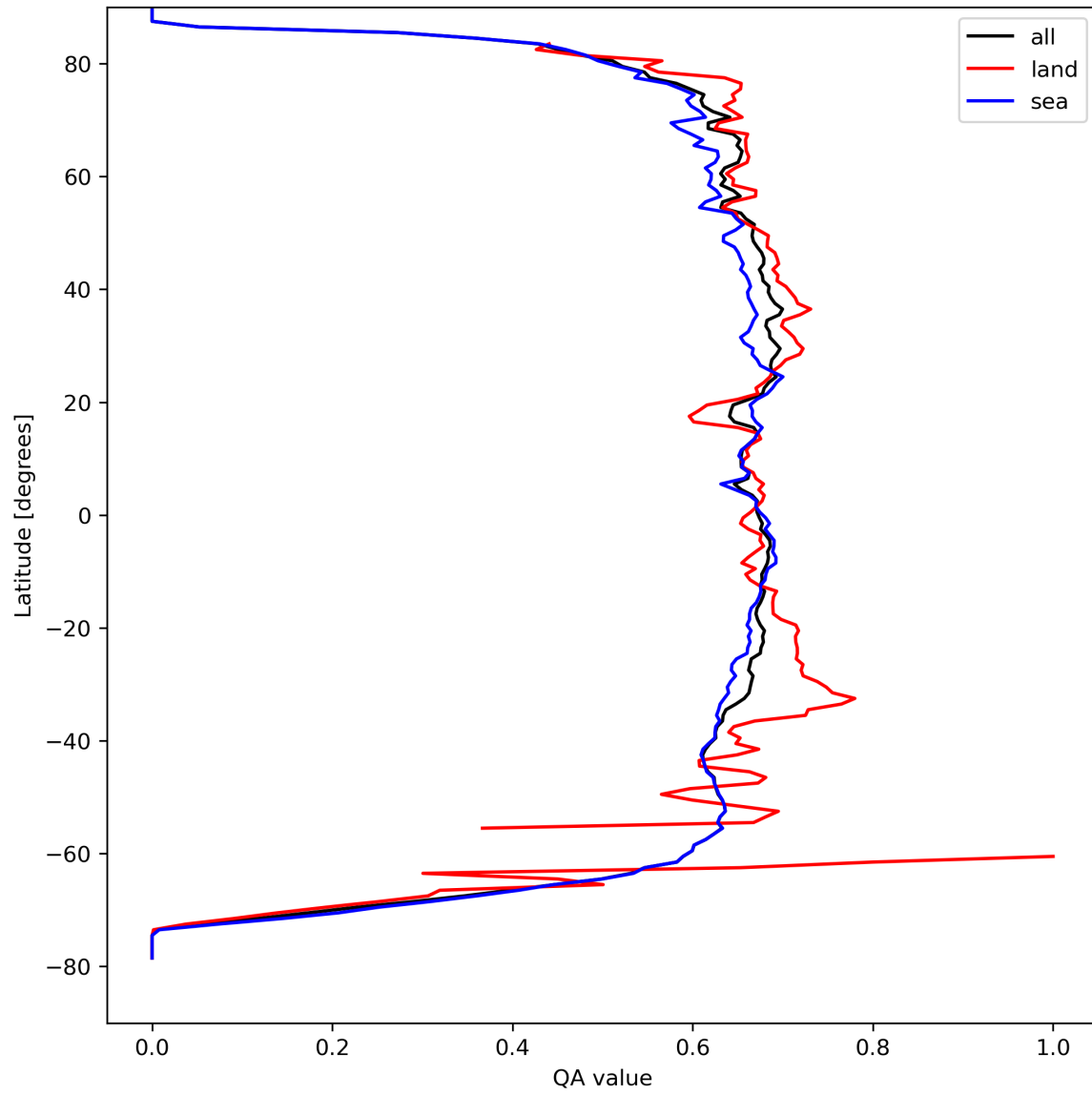
Figure 9: Zonal average of “QA value” for 2023-09-05 to 2023-09-07.
