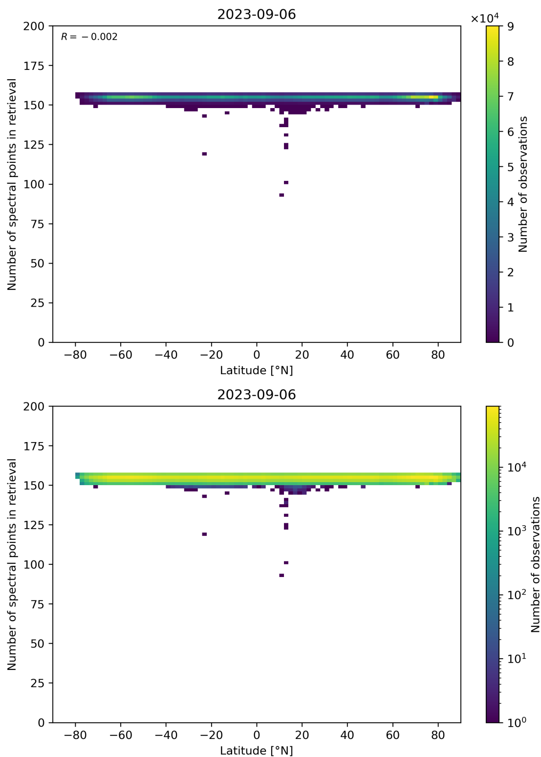
Figure 57: Scatter density plot of “Latitude” against “Number of spectral points in retrieval” for 2023-09-05 to 2023-09-07.
