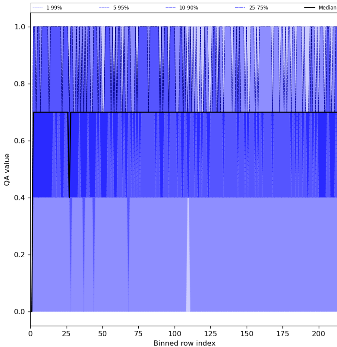
Figure 25: Along track statistics of “QA value” for 2023-09-05 to 2023-09-07
