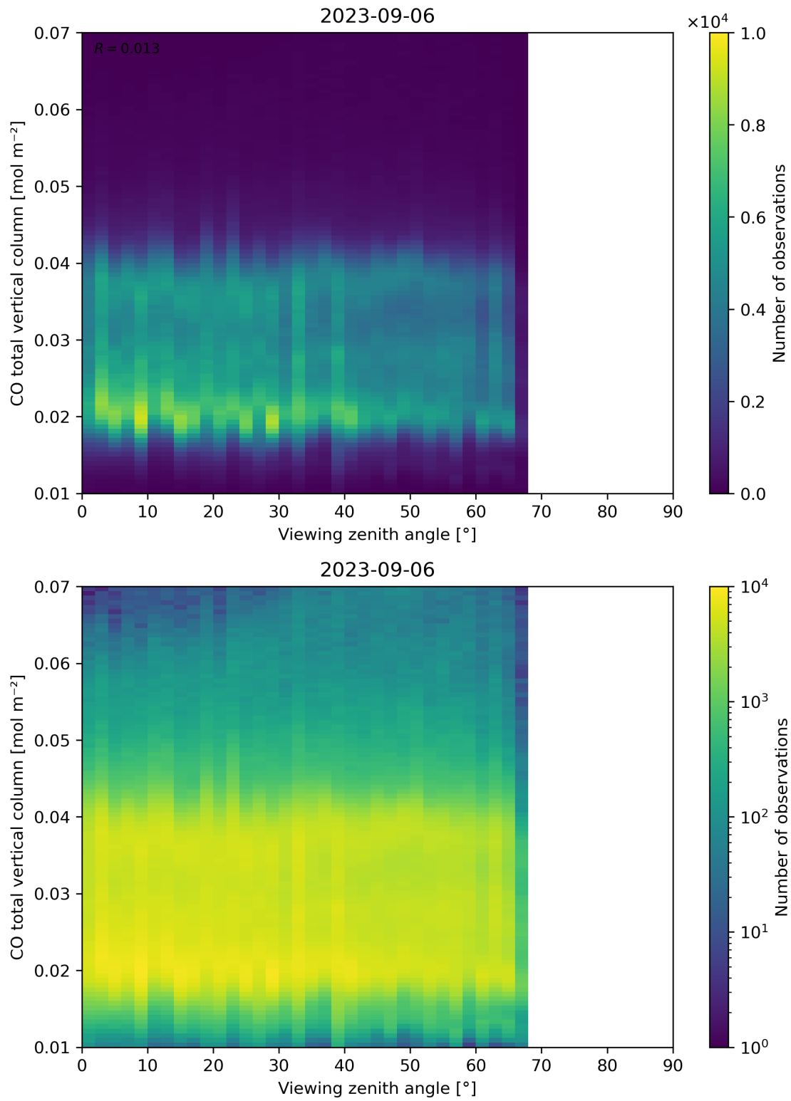
Figure 69: Scatter density plot of “Viewing zenith angle” against “CO total vertical column” for 2023-09-05 to 2023-09-07.
