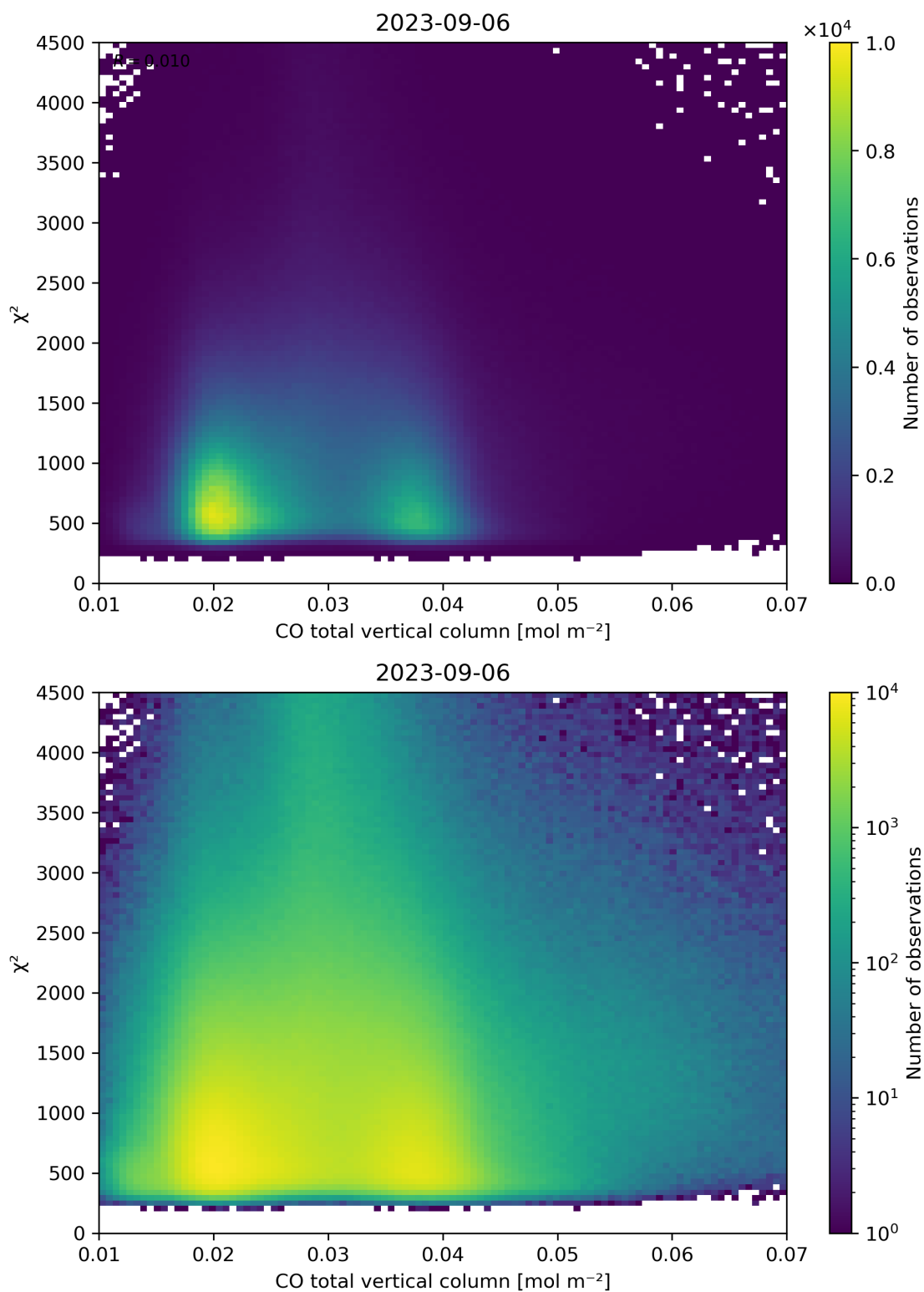
Figure 35: Scatter density plot of “CO total vertical column” against “ \chi^2 ” for 2023-09-05 to 2023-09-07.
