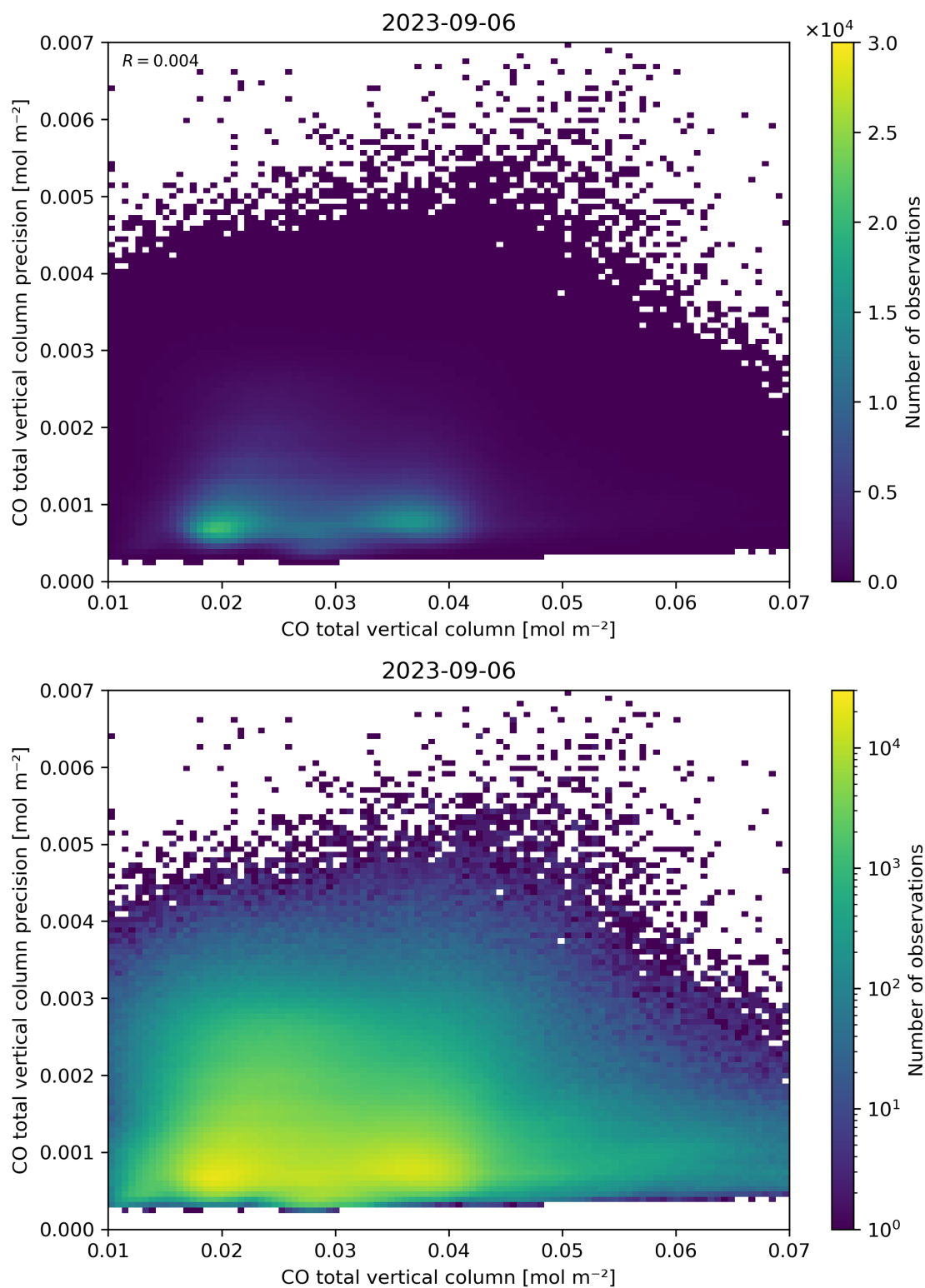
Figure 34: Scatter density plot of “CO total vertical column” against “CO total vertical column precision” for 2023-09-05 to 2023-09-07.
