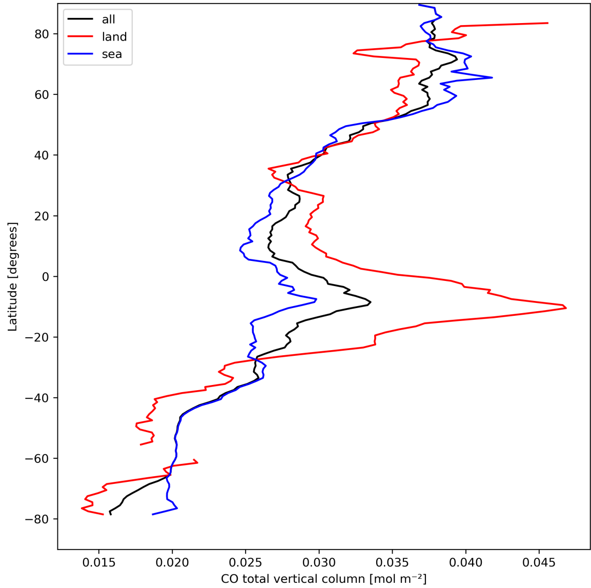
Figure 10: Zonal average of “CO total vertical column” for 2023-09-05 to 2023-09-07.
