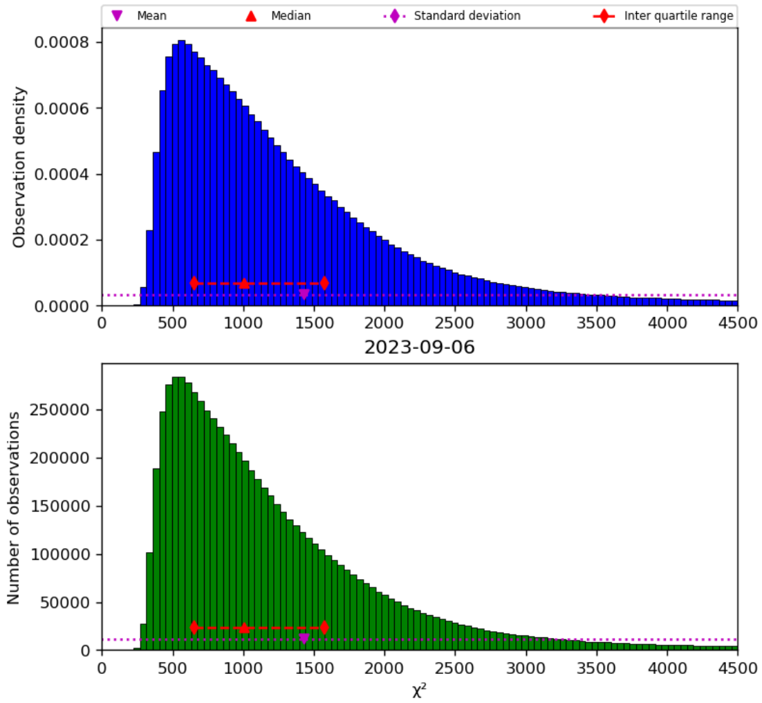
Figure 22: Histogram of “ \chi^2 ” for 2023-09-05 to 2023-09-07
