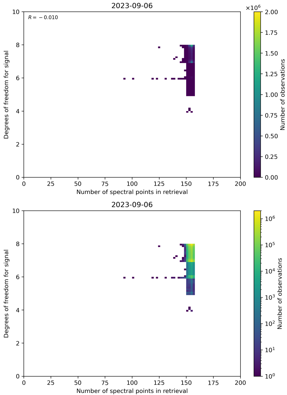
Figure 59: Scatter density plot of “Number of spectral points in retrieval” against “Degrees of freedom for signal” for 2023-09-05 to 2023-09-07.
