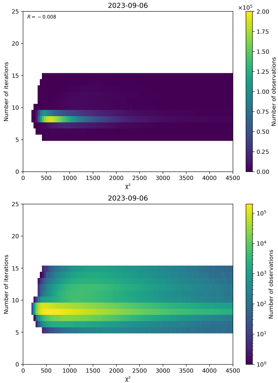
Figure 49: Scatter density plot of “ \chi^2 ” against “Number of iterations” for 2023-09-05 to 2023-09-07.
