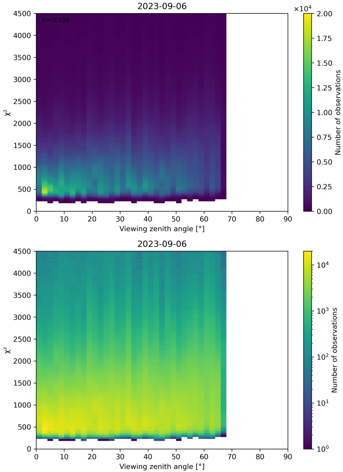
Figure 72: Scatter density plot of “Viewing zenith angle” against “ \chi^2 ” for 2023-09-05 to 2023-09-07.
