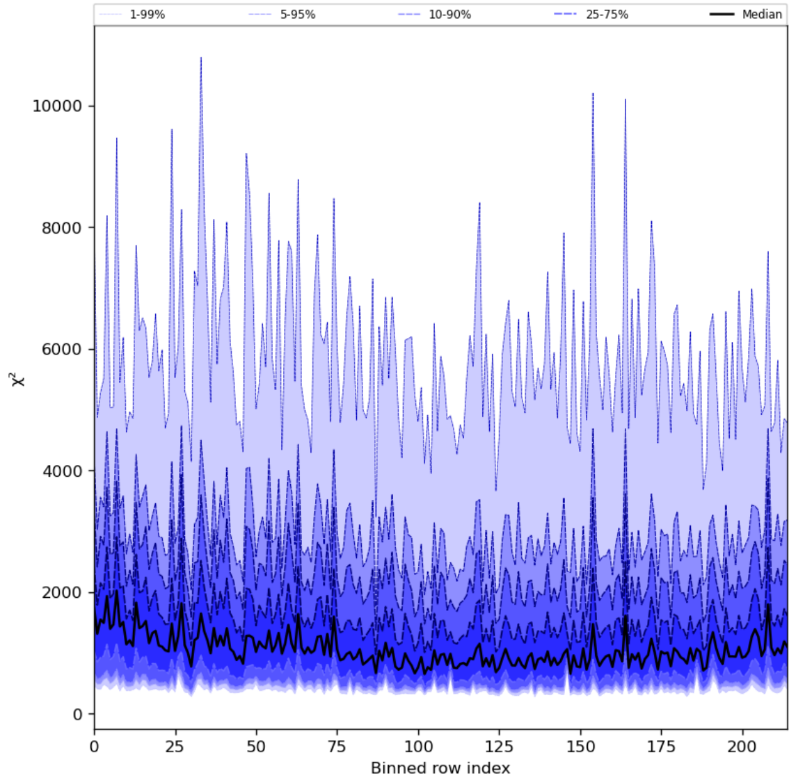
Figure 30: Along track statistics of “ \chi^2 ” for 2023-09-05 to 2023-09-07
