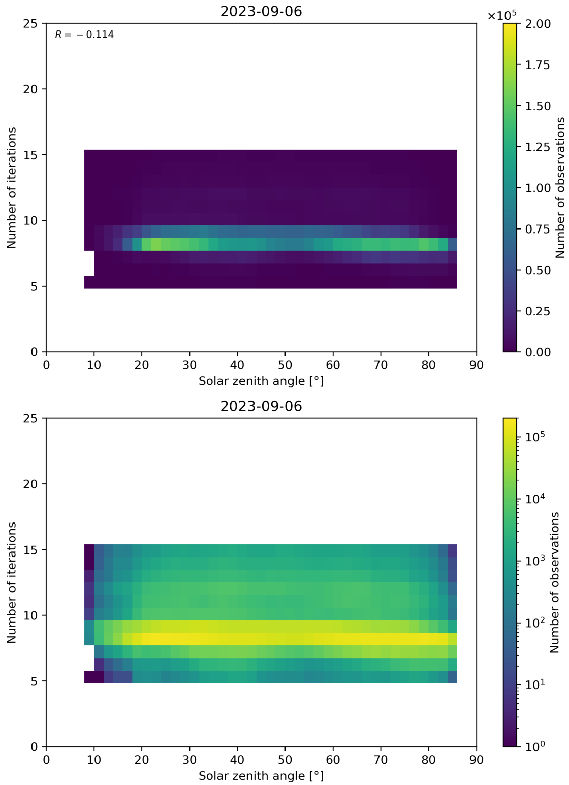
Figure 67: Scatter density plot of “Solar zenith angle” against “Number of iterations” for 2023-09-05 to 2023-09-07.
