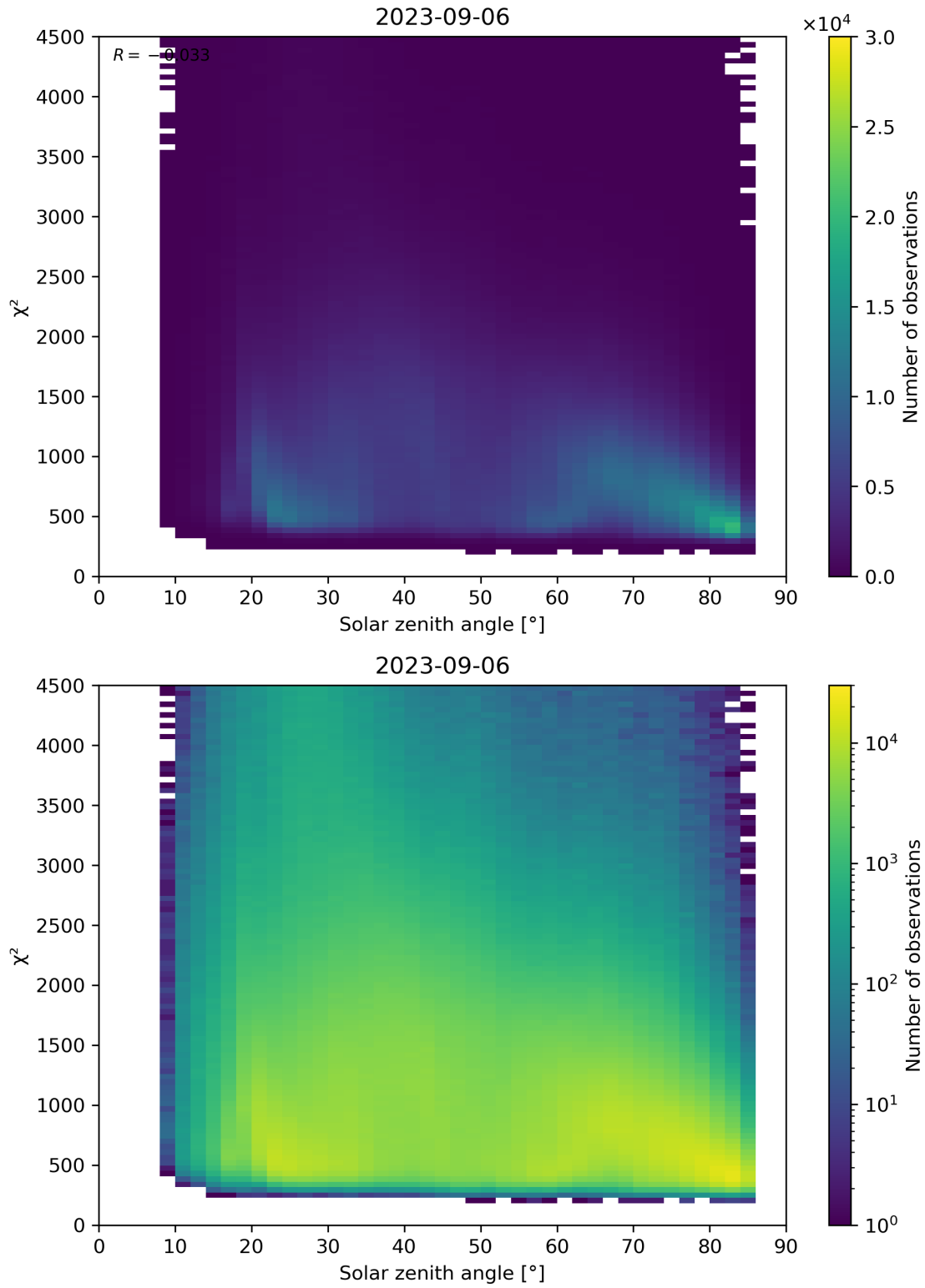
Figure 64: Scatter density plot of “Solar zenith angle” against “ \chi^2 ” for 2023-09-05 to 2023-09-07.
