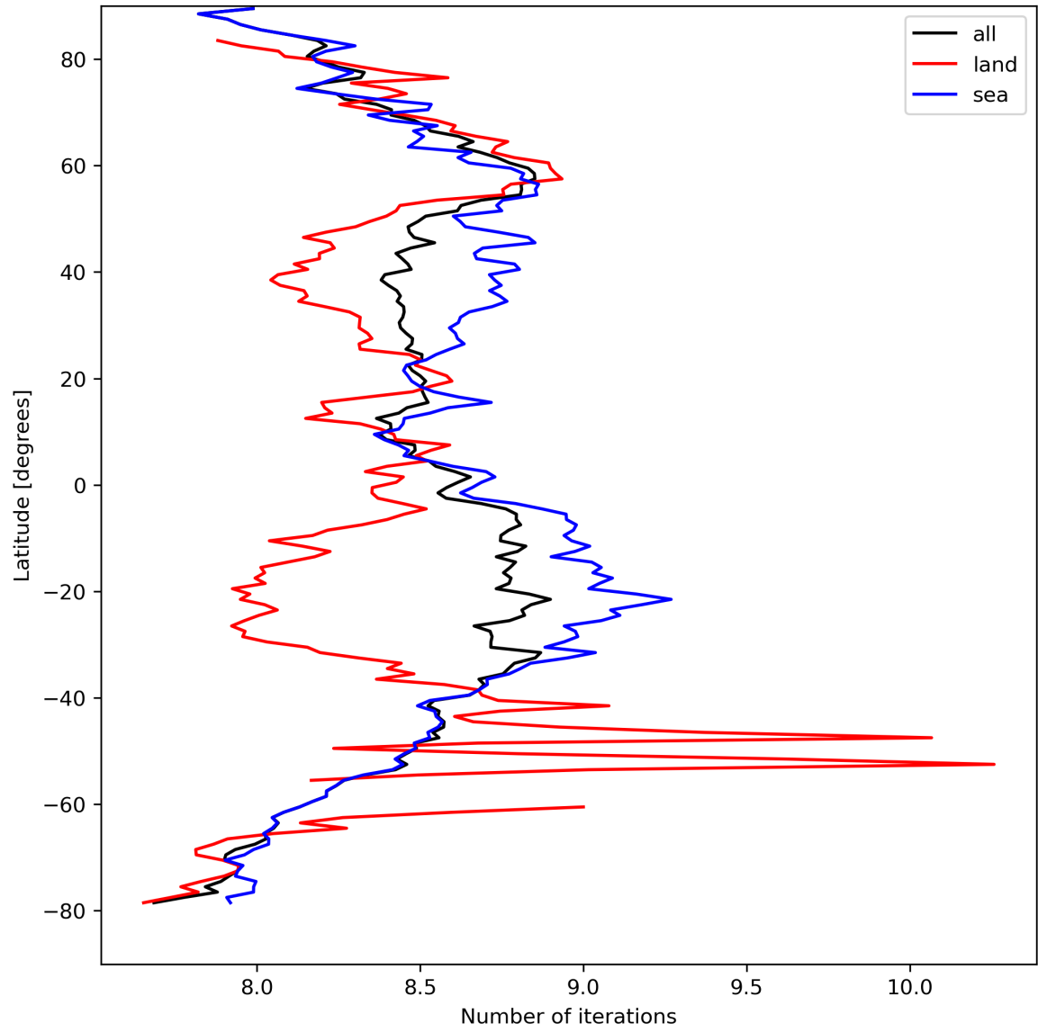
Figure 16: Zonal average of “Number of iterations” for 2023-09-05 to 2023-09-07.
