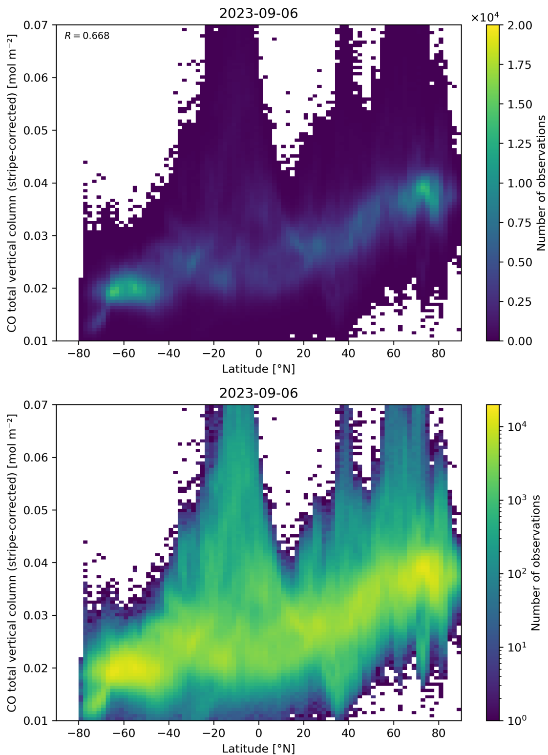
Figure 52: Scatter density plot of “Latitude” against “CO total vertical column (stripe-corrected)” for 2023-09-05 to 2023-09-07.
