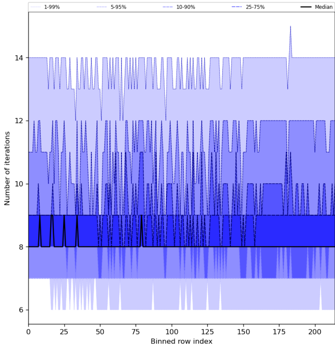
Figure 32: Along track statistics of “Number of iterations” for 2023-09-05 to 2023-09-07
