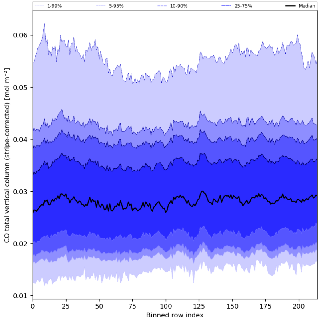
Figure 27: Along track statistics of “CO total vertical column (stripe-corrected)” for 2023-09-05 to 2023-09-07
