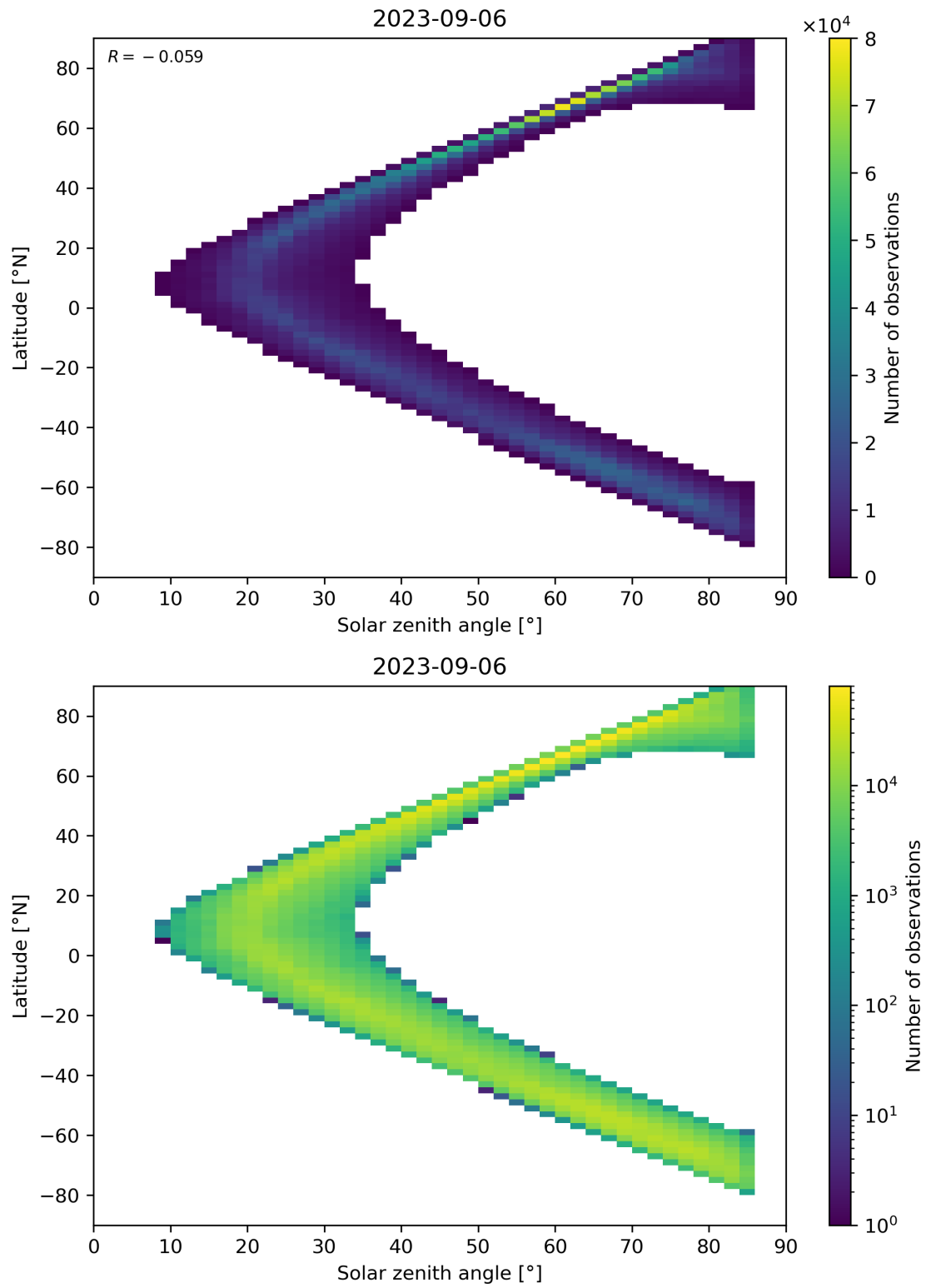
Figure 66: Scatter density plot of “Solar zenith angle” against “Latitude” for 2023-09-05 to 2023-09-07.
