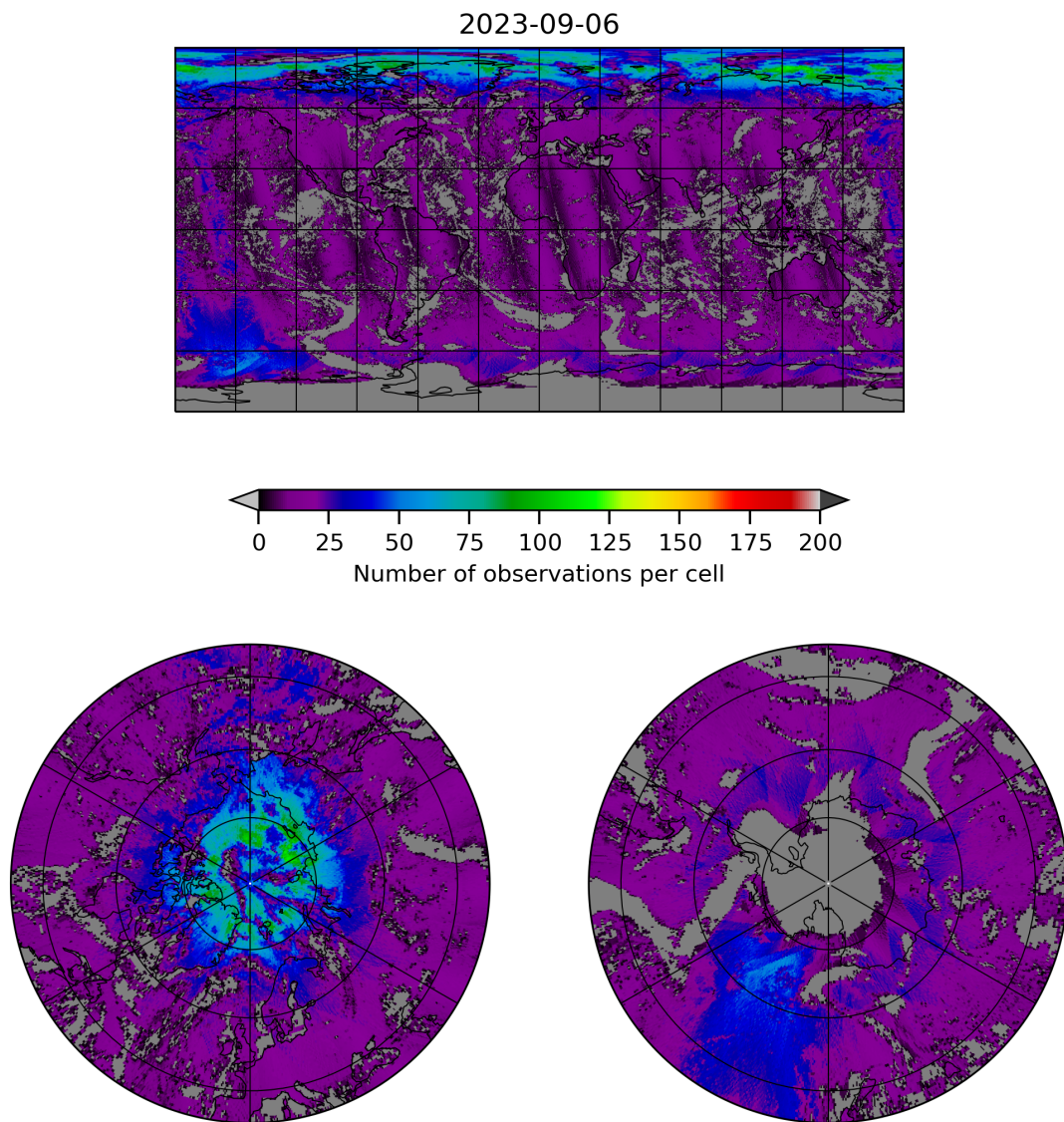
Figure 8: Map of the number of observations for 2023-09-05 to 2023-09-07
