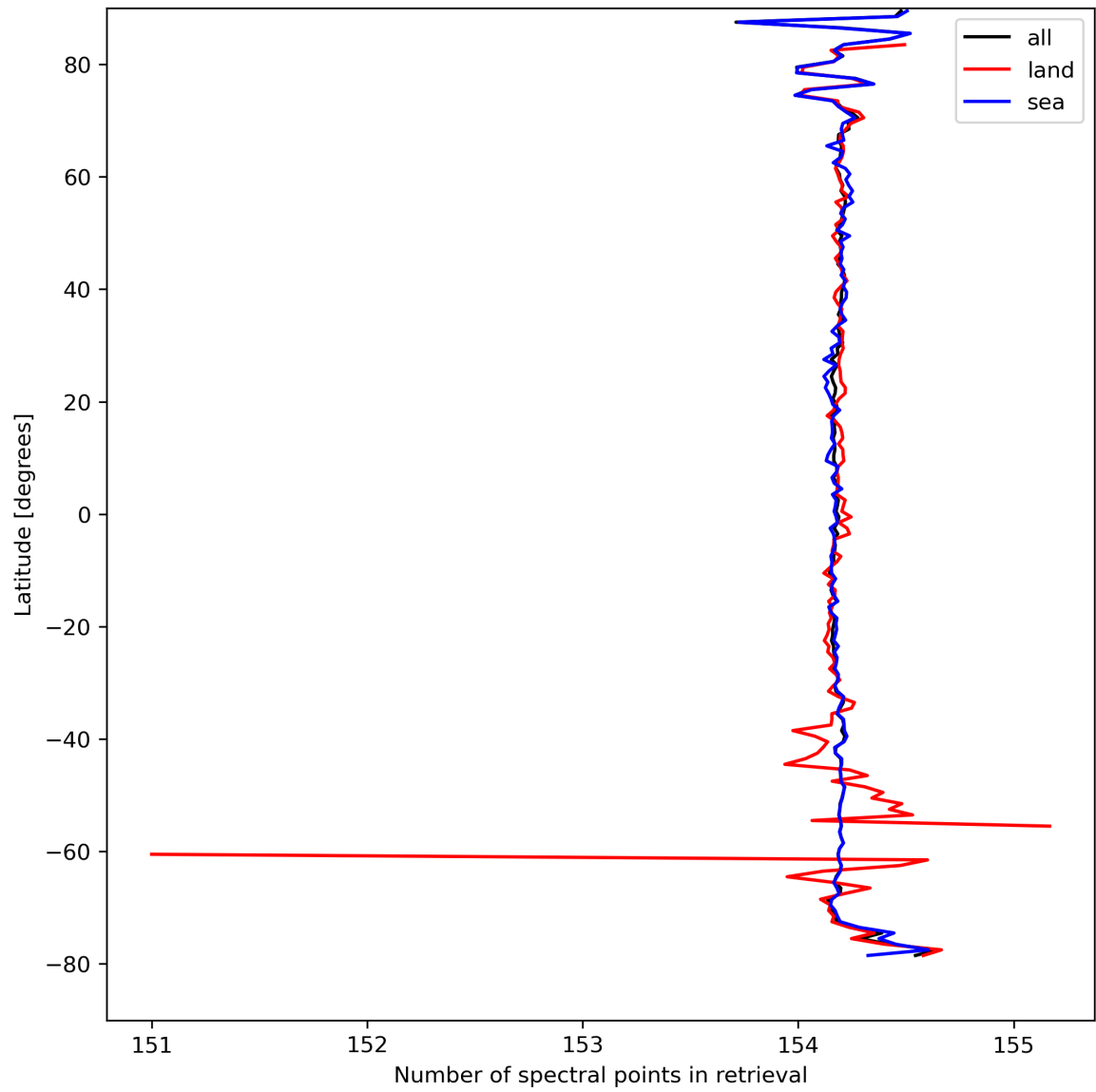
Figure 13: Zonal average of “Number of spectral points in retrieval” for 2023-09-05 to 2023-09-07.
