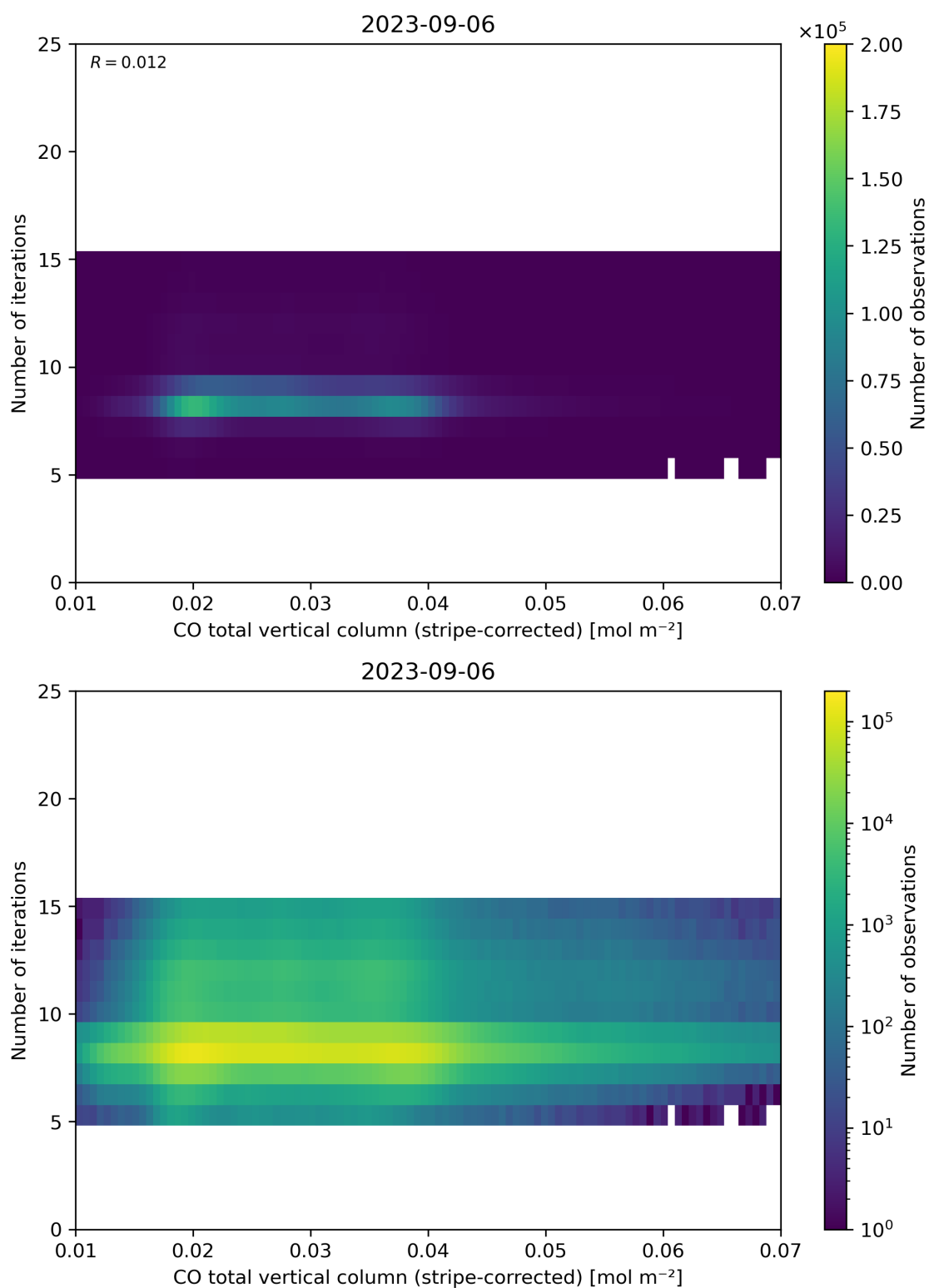
Figure 39: Scatter density plot of “CO total vertical column (stripe-corrected)” against “Number of iterations” for 2023-09-05 to 2023-09-07.
