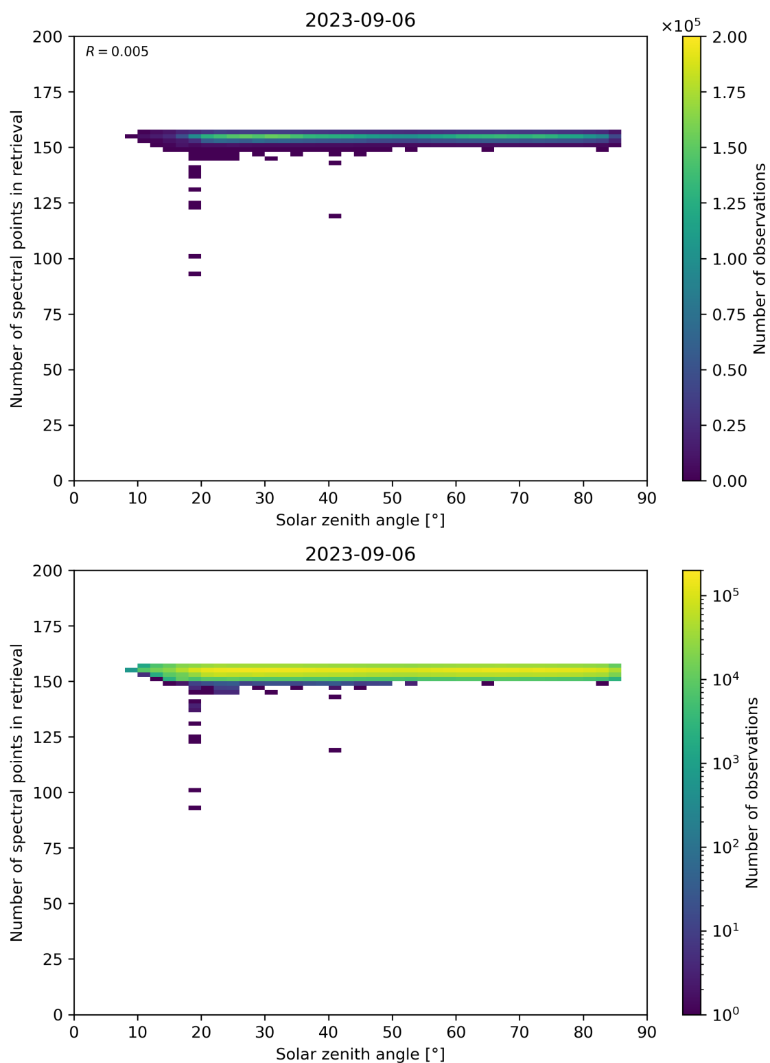
Figure 68: Scatter density plot of “Solar zenith angle” against “Number of spectral points in retrieval” for 2023-09-05 to 2023-09-07.
