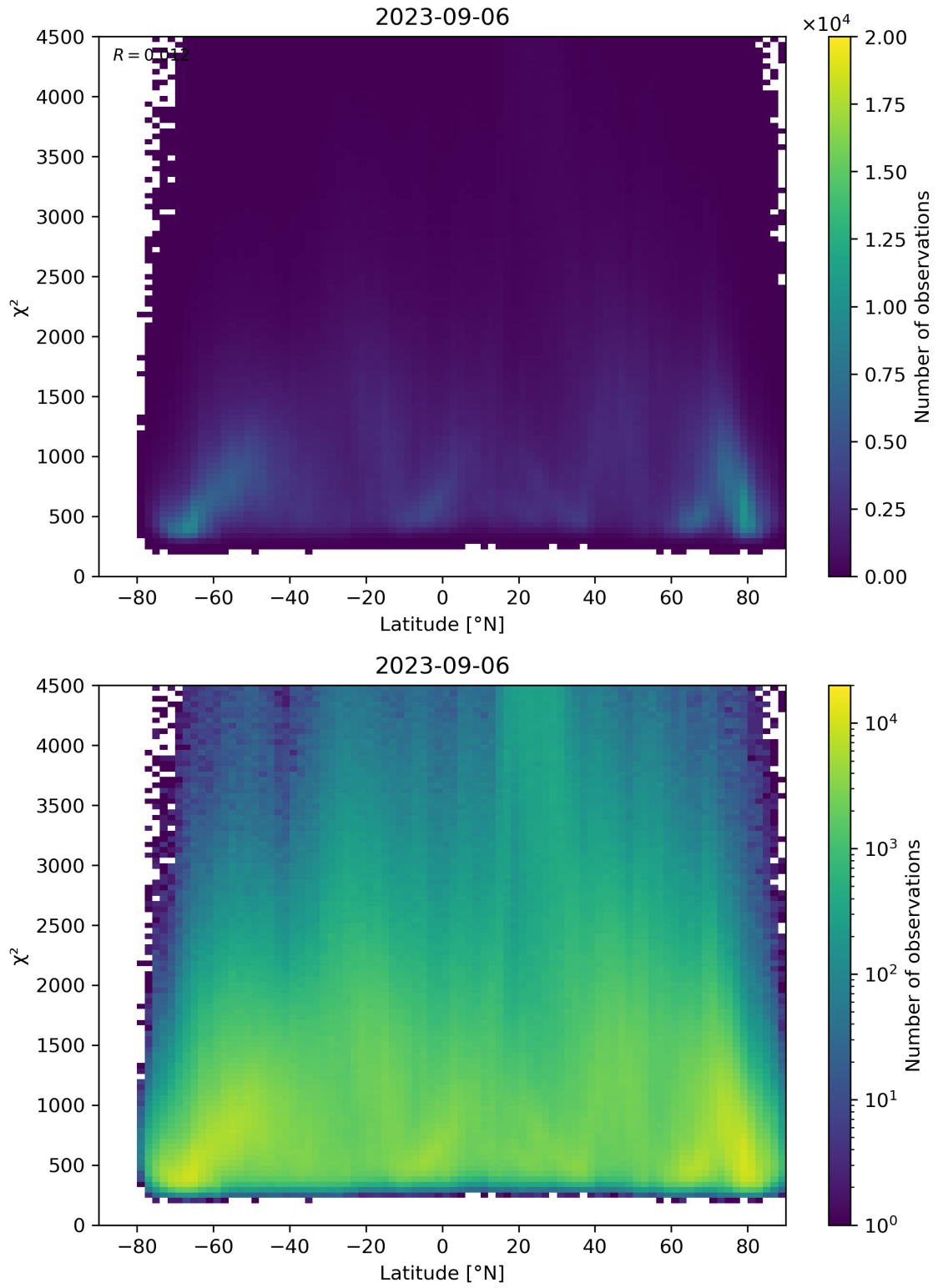
Figure 54: Scatter density plot of “Latitude” against “ \chi^2 ” for 2023-09-05 to 2023-09-07.
