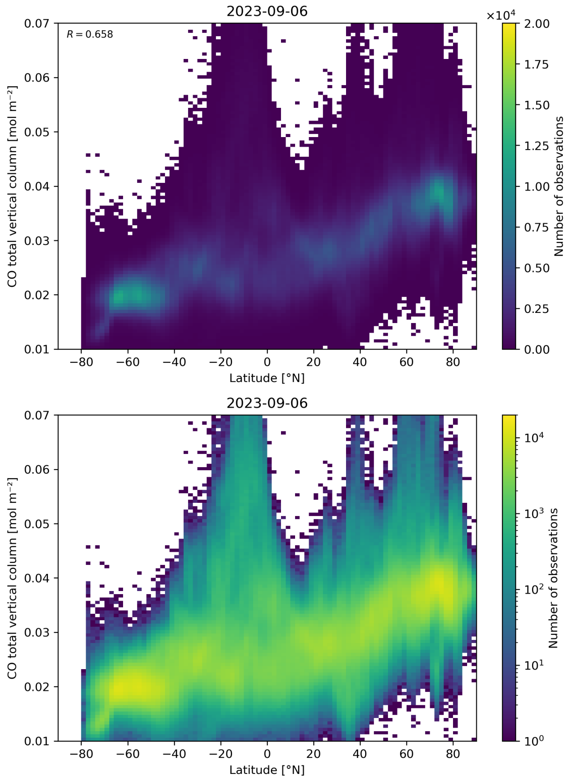
Figure 51: Scatter density plot of “Latitude” against “CO total vertical column” for 2023-09-05 to 2023-09-07.
