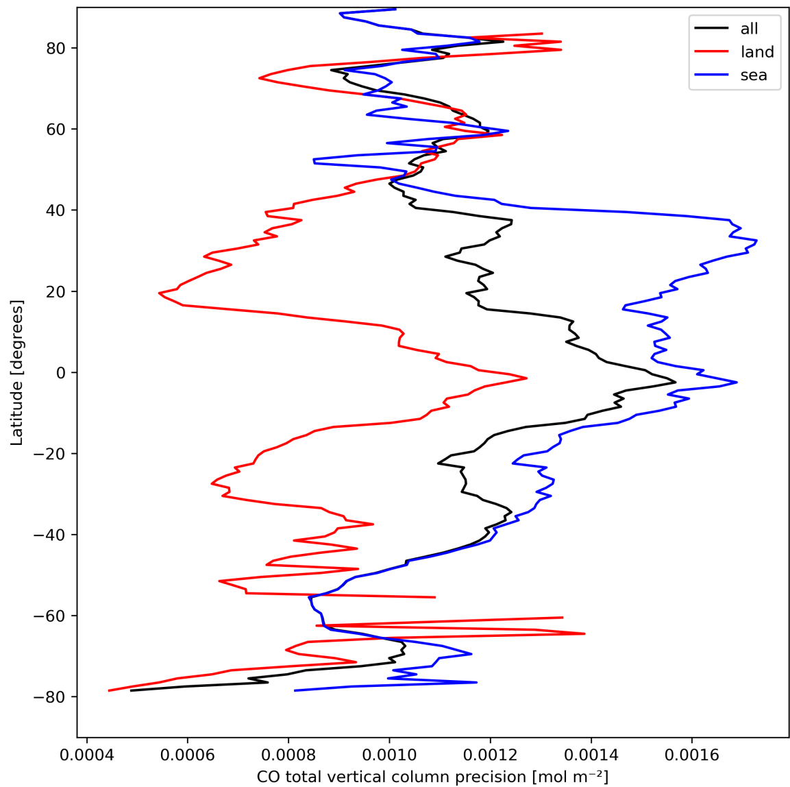
Figure 12: Zonal average of “CO total vertical column precision” for 2023-09-05 to 2023-09-07.
