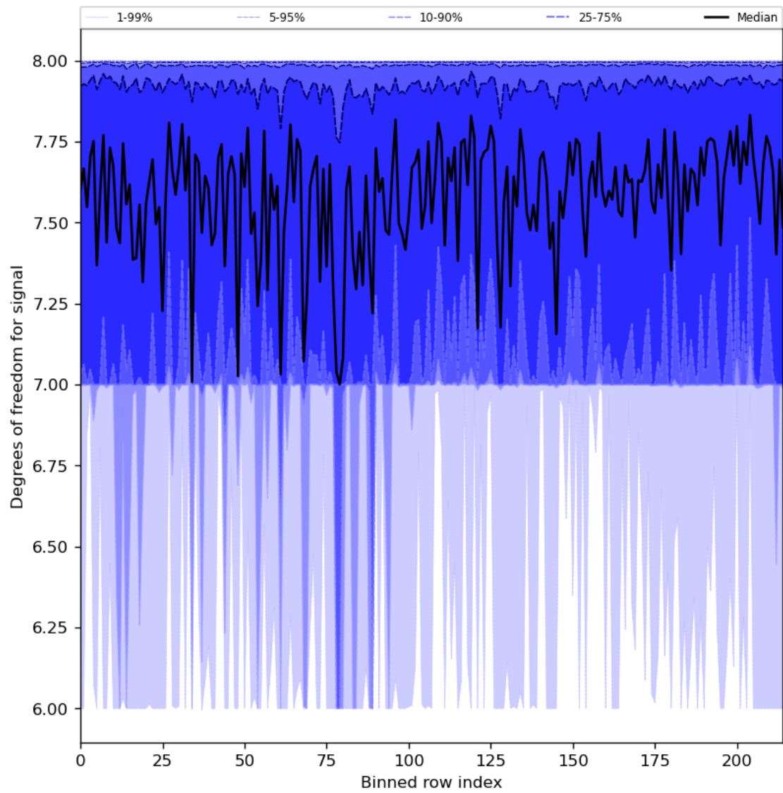
Figure 31: Along track statistics of “Degrees of freedom for signal” for 2023-09-05 to 2023-09-07
