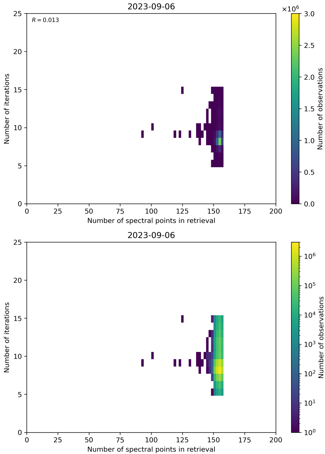
Figure 60: Scatter density plot of “Number of spectral points in retrieval” against “Number of iterations” for 2023-09-05 to 2023-09-07.
