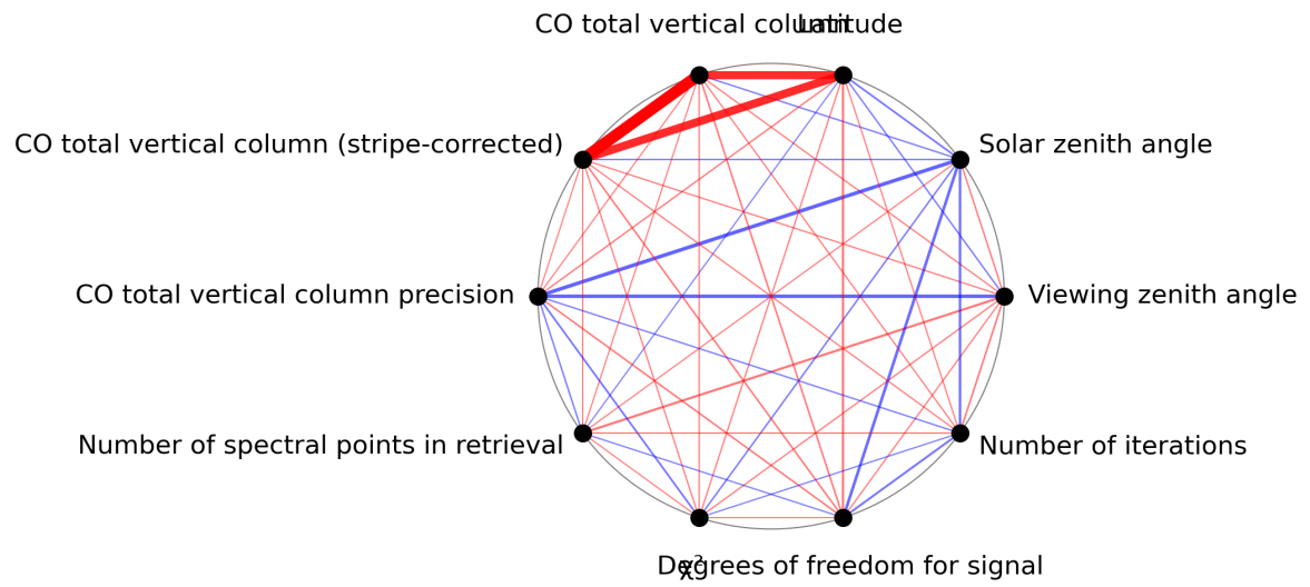
Figure 1: Map of correlation graph for 2023-09-05 to 2023-09-07.
