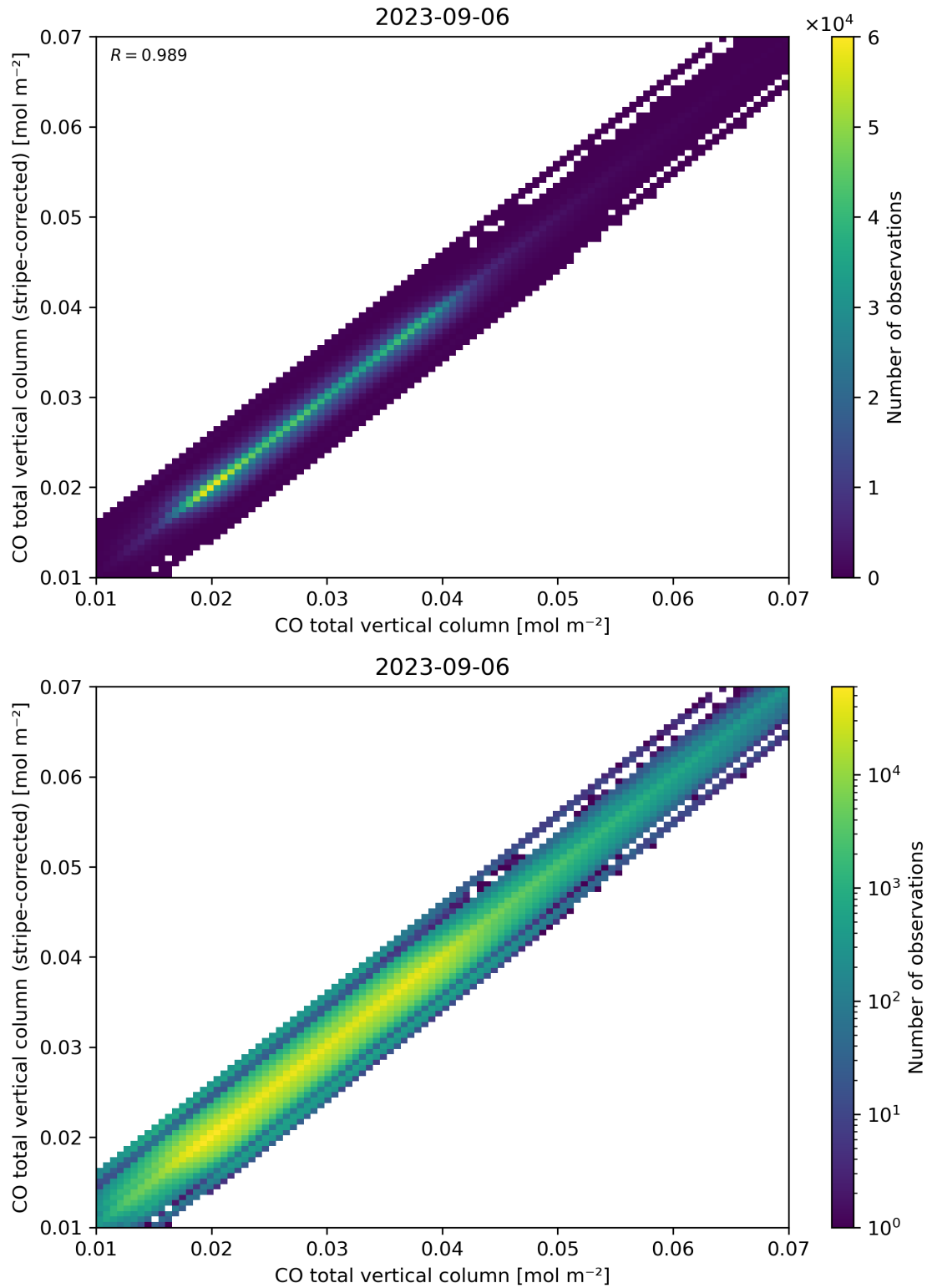
Figure 33: Scatter density plot of “CO total vertical column” against “CO total vertical column (stripe-corrected)” for 2023-09-05 to 2023-09-07.
