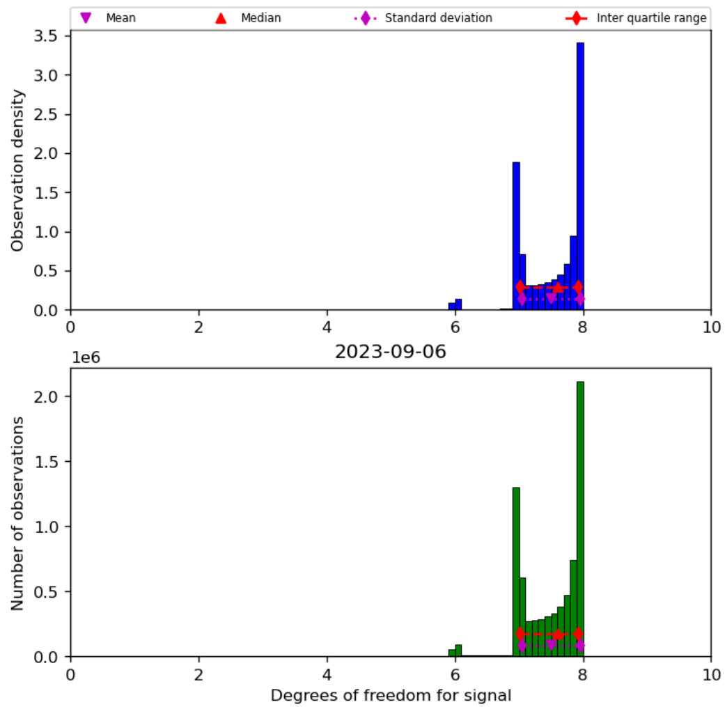
Figure 23: Histogram of “Degrees of freedom for signal” for 2023-09-05 to 2023-09-07
