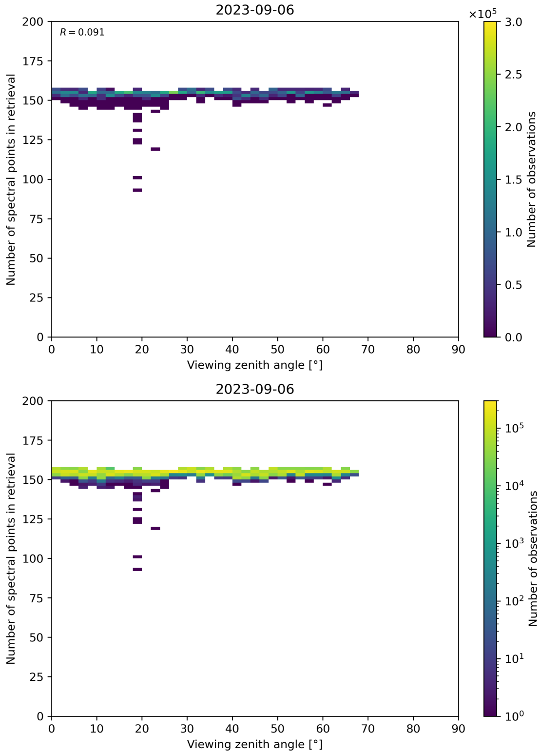
Figure 76: Scatter density plot of “Viewing zenith angle” against “Number of spectral points in retrieval” for 2023-09-05 to 2023-09-07.
