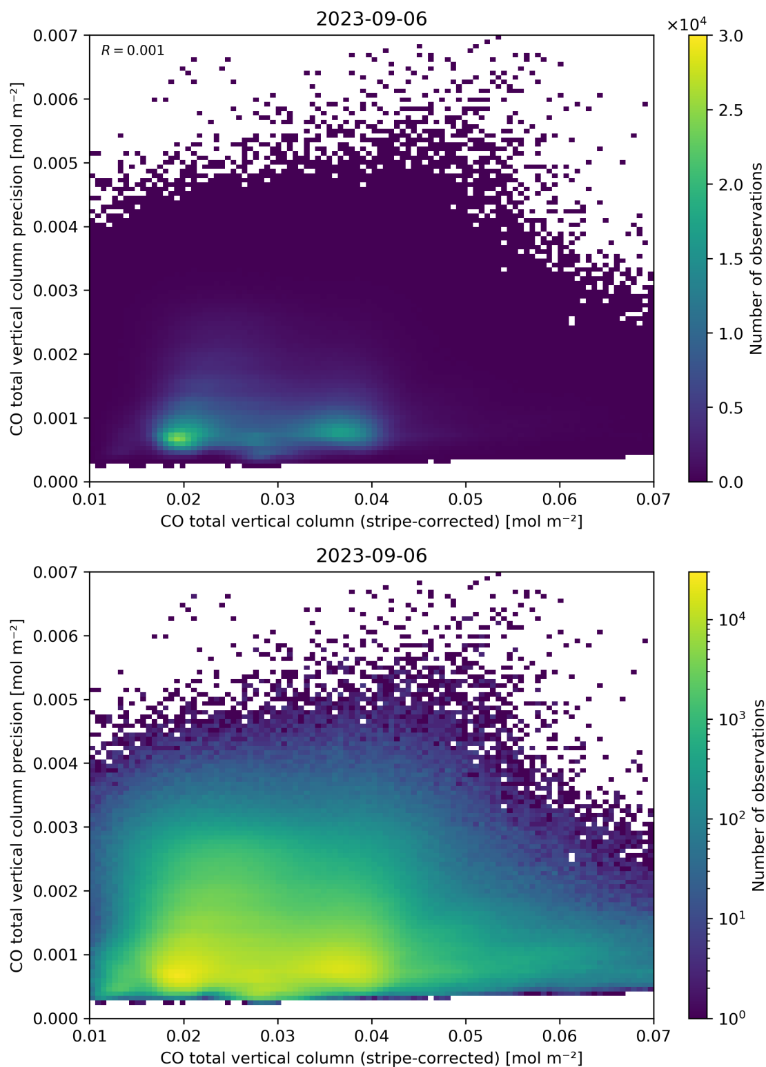
Figure 36: Scatter density plot of “CO total vertical column (stripe-corrected)” against “CO total vertical column precision” for 2023-09-05 to 2023-09-07.
