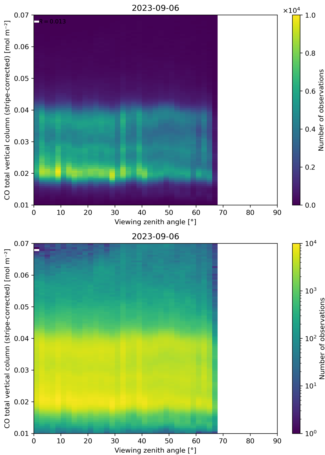
Figure 70: Scatter density plot of “Viewing zenith angle” against “CO total vertical column (stripe-corrected)” for 2023-09-05 to 2023-09-07.
