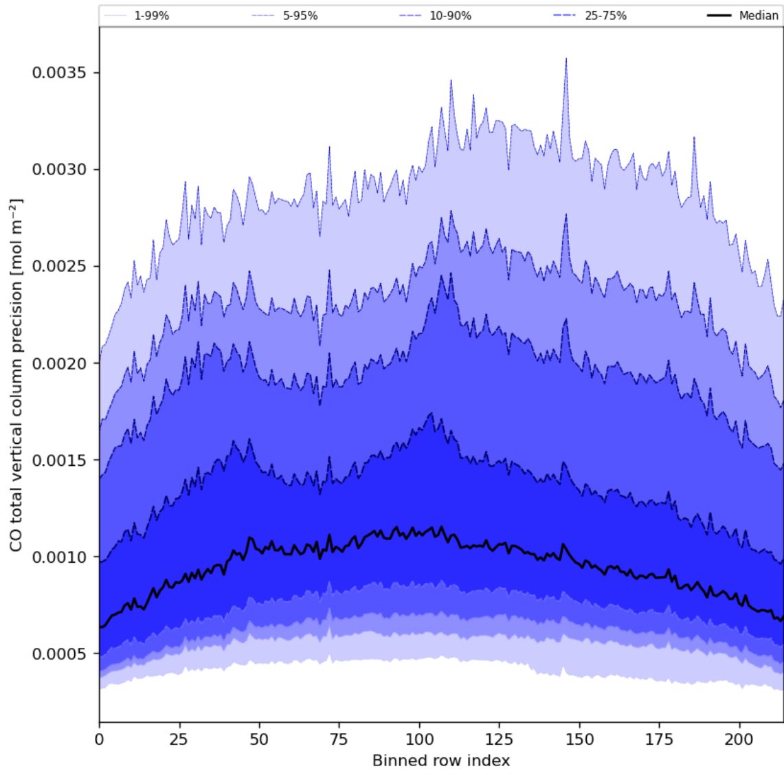
Figure 28: Along track statistics of “CO total vertical column precision” for 2023-09-05 to 2023-09-07
