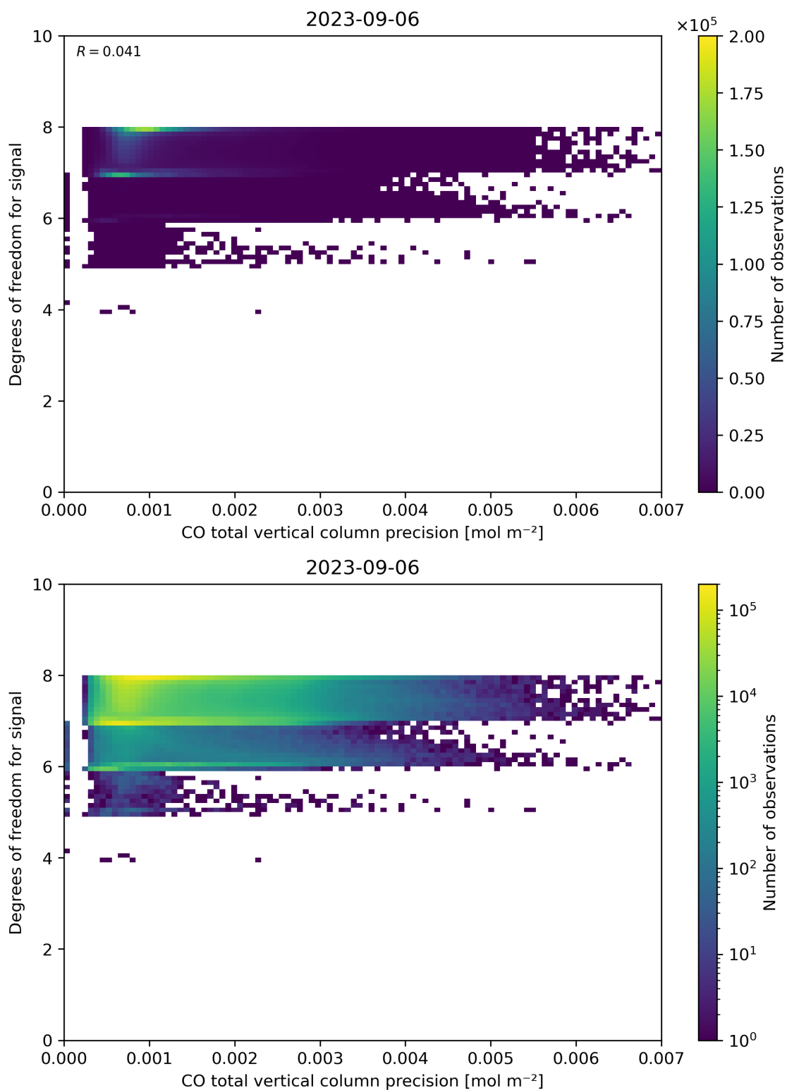
Figure 45: Scatter density plot of “CO total vertical column precision” against “Degrees of freedom for signal” for 2023-09-05 to 2023-09-07.
