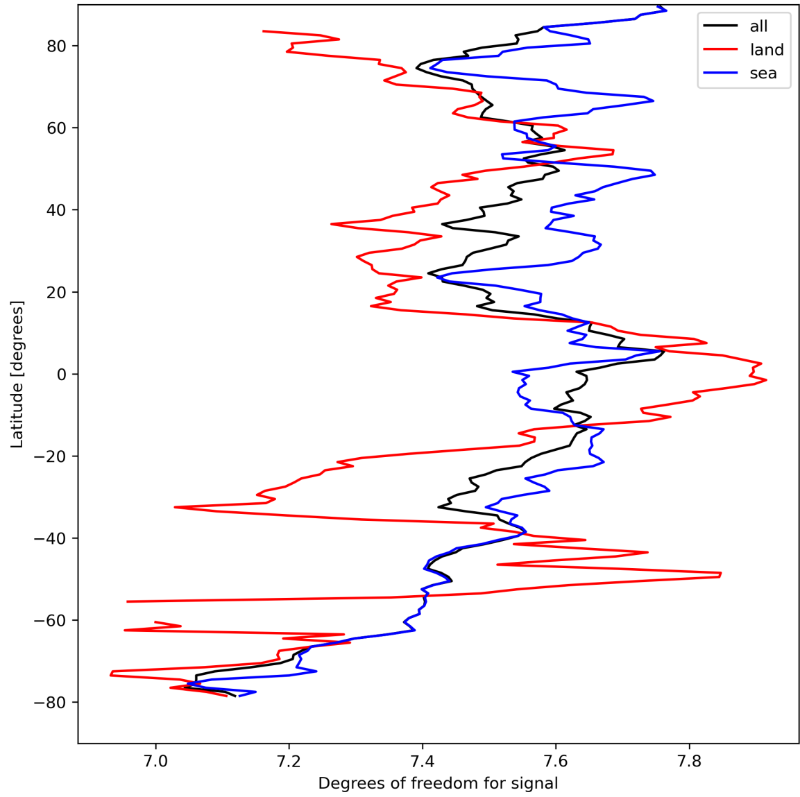
Figure 15: Zonal average of “Degrees of freedom for signal” for 2023-09-05 to 2023-09-07.
