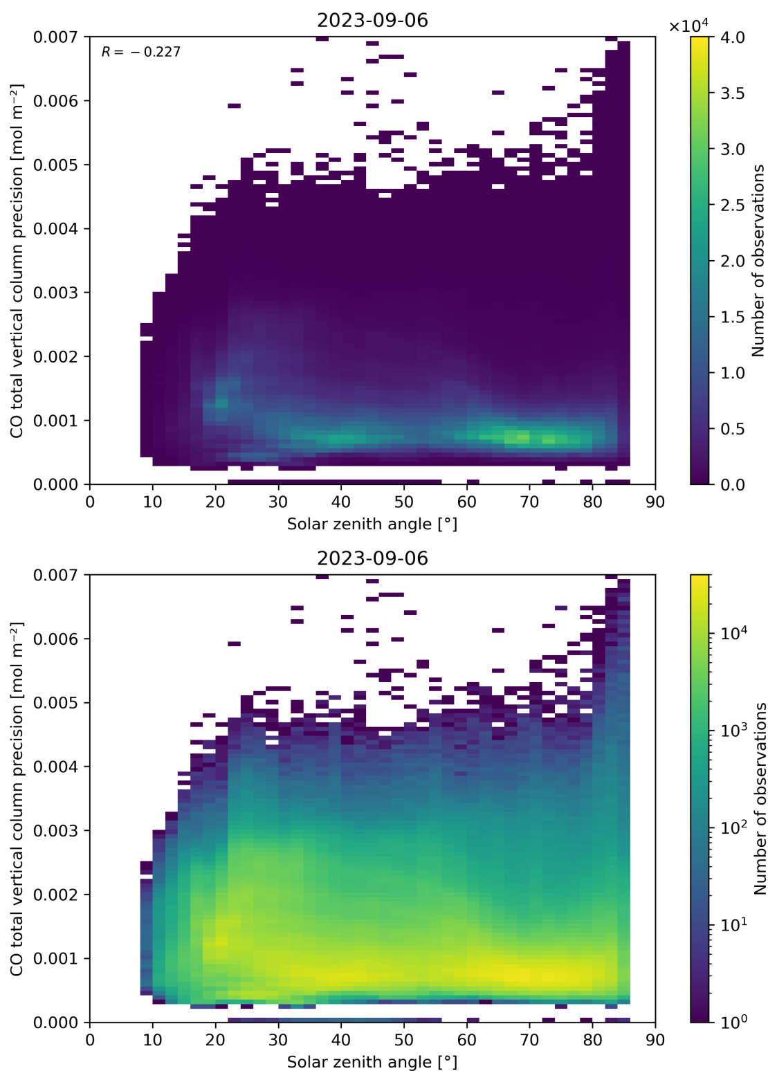
Figure 63: Scatter density plot of “Solar zenith angle” against “CO total vertical column precision” for 2023-09-05 to 2023-09-07.
