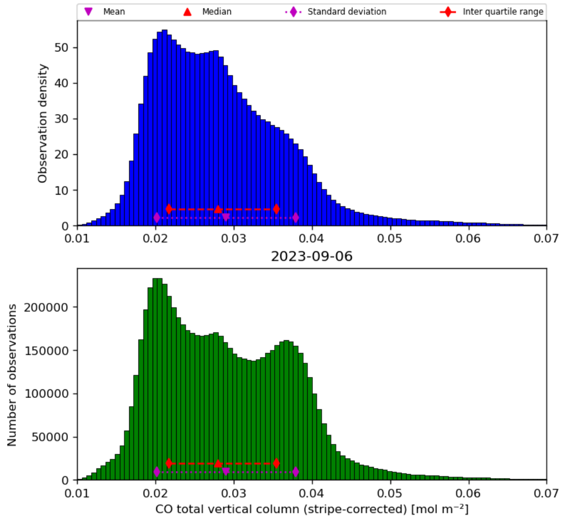
Figure 19: Histogram of “CO total vertical column (stripe-corrected)” for 2023-09-05 to 2023-09-07
