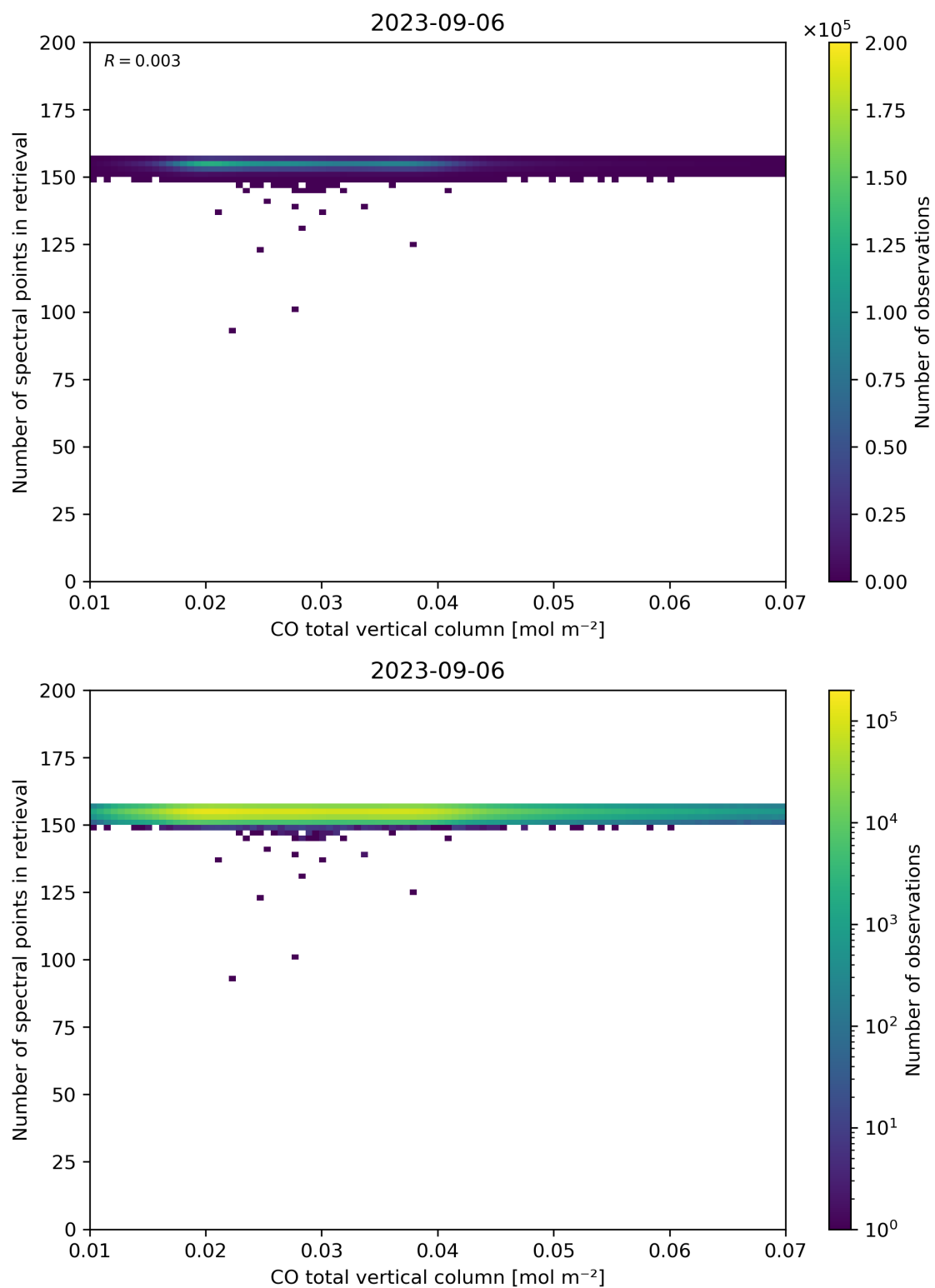
Figure 43: Scatter density plot of “CO total vertical column” against “Number of spectral points in retrieval” for 2023-09-05 to 2023-09-07.
