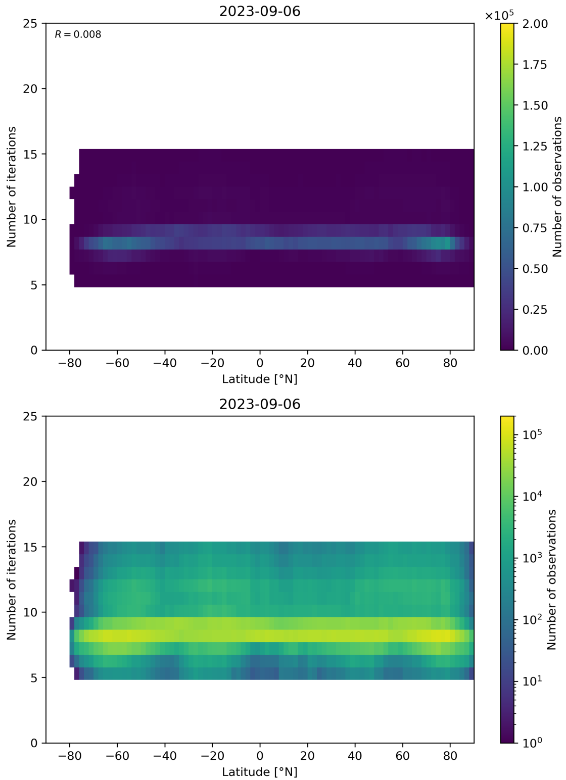
Figure 56: Scatter density plot of “Latitude” against “Number of iterations” for 2023-09-05 to 2023-09-07.
