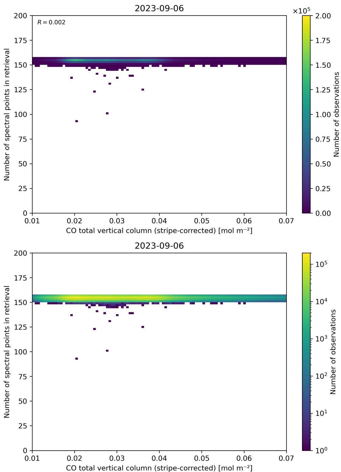
Figure 40: Scatter density plot of “CO total vertical column (stripe-corrected)” against “Number of spectral points in retrieval” for 2023-09-05 to 2023-09-07.
