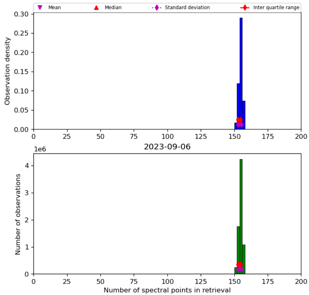
Figure 21: Histogram of “Number of spectral points in retrieval” for 2023-09-05 to 2023-09-07
