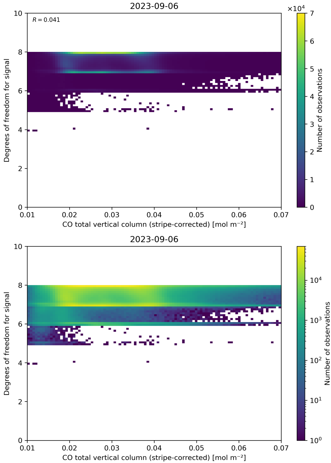
Figure 38: Scatter density plot of “CO total vertical column (stripe-corrected)” against “Degrees of freedom for signal” for 2023-09-05 to 2023-09-07.
