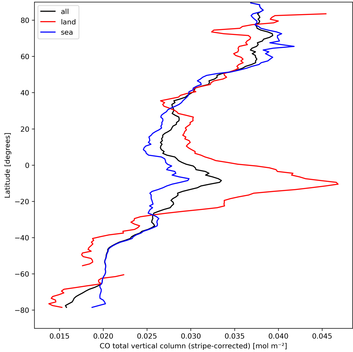
Figure 11: Zonal average of “CO total vertical column (stripe-corrected)” for 2023-09-05 to 2023-09-07.
