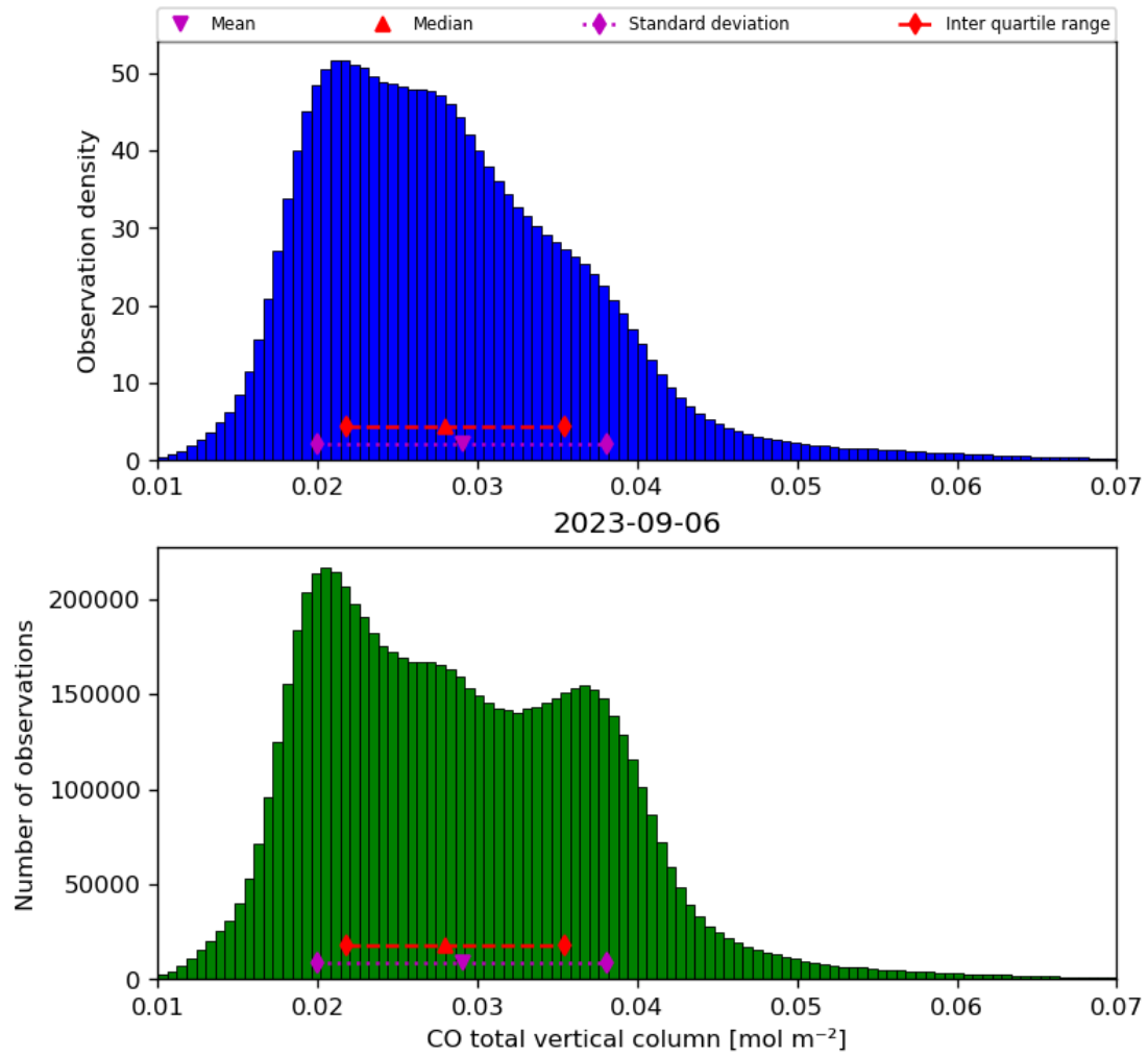
Figure 18: Histogram of “CO total vertical column” for 2023-09-05 to 2023-09-07
