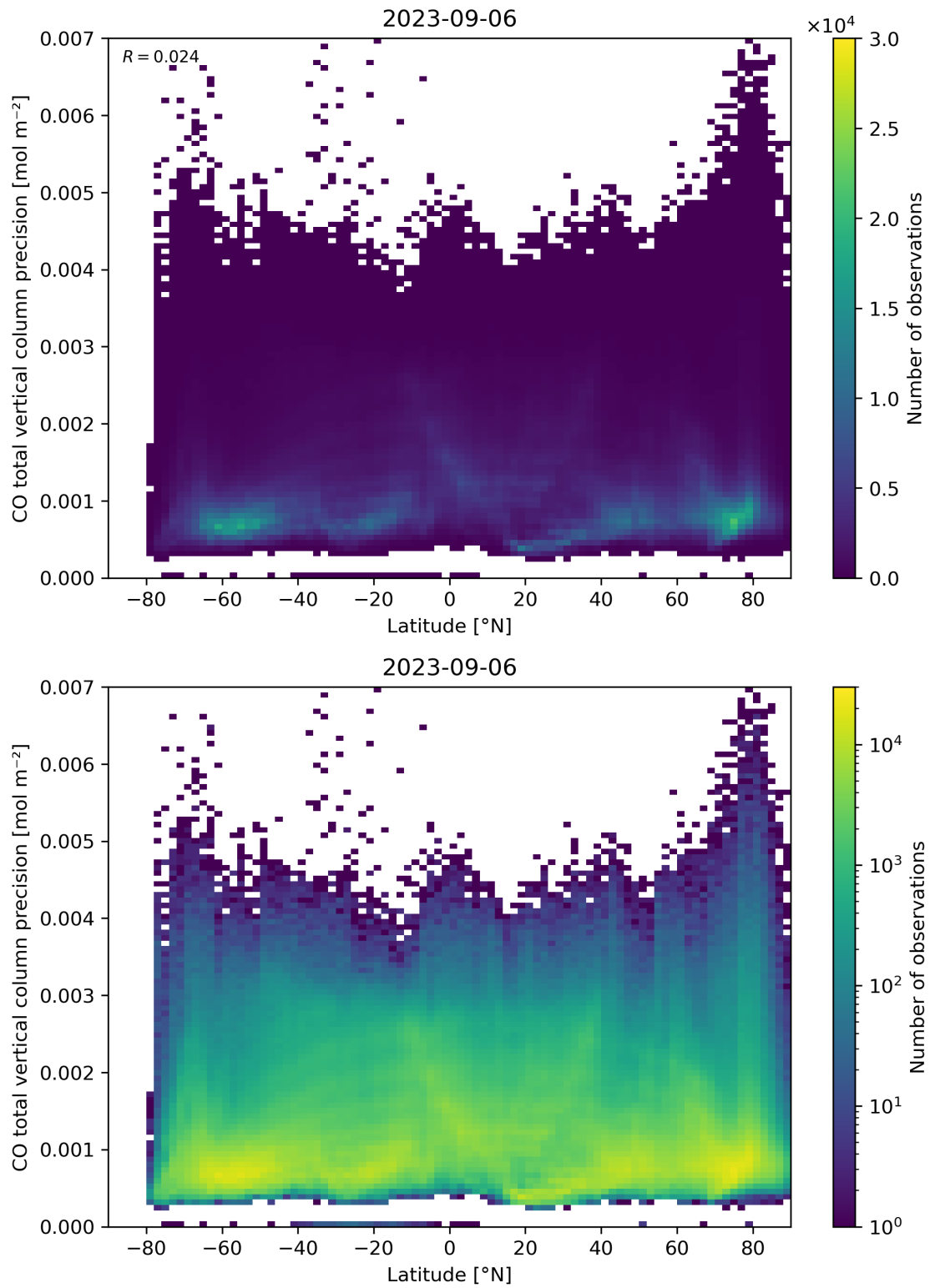
Figure 53: Scatter density plot of “Latitude” against “CO total vertical column precision” for 2023-09-05 to 2023-09-07.
