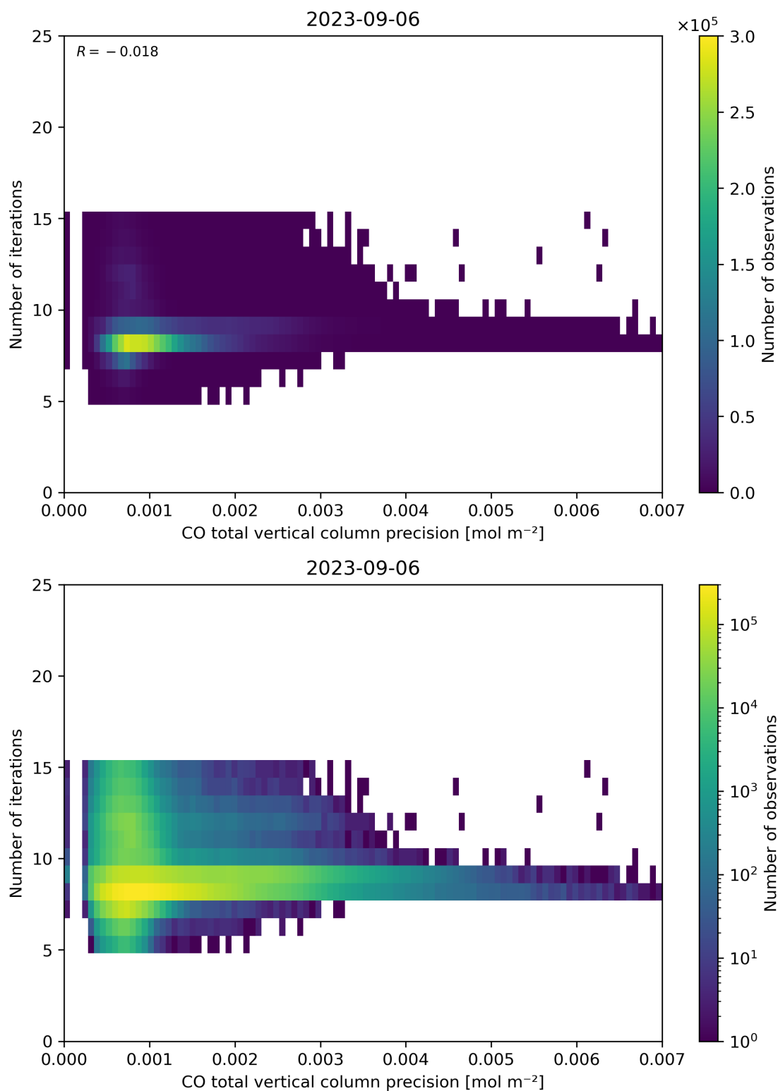
Figure 46: Scatter density plot of “CO total vertical column precision” against “Number of iterations” for 2023-09-05 to 2023-09-07.
