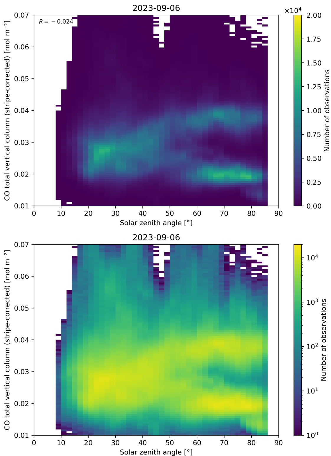
Figure 62: Scatter density plot of “Solar zenith angle” against “CO total vertical column (stripe-corrected)” for 2023-09-05 to 2023-09-07.
