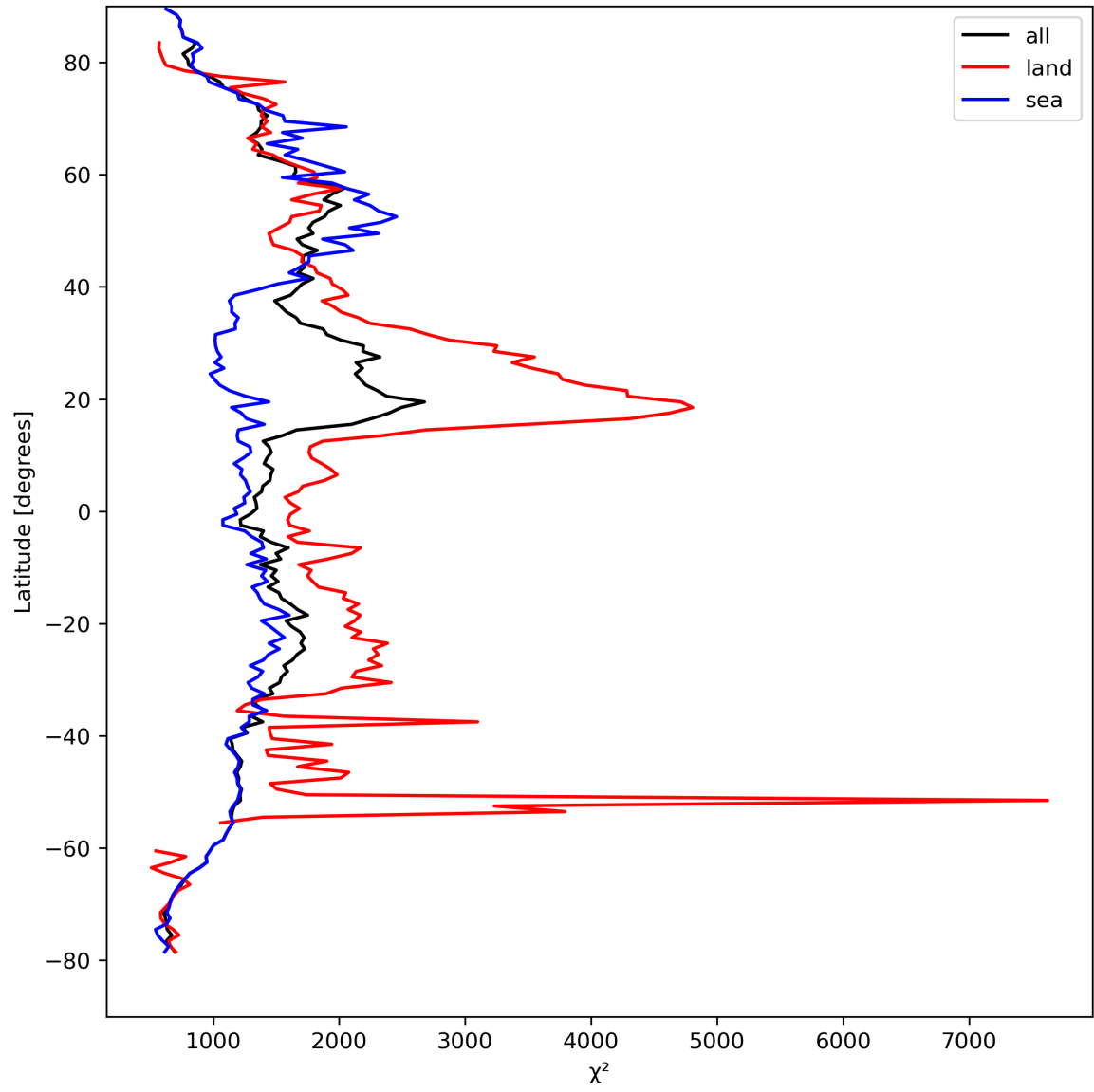
Figure 14: Zonal average of “ \chi^2 ” for 2023-09-05 to 2023-09-07.
