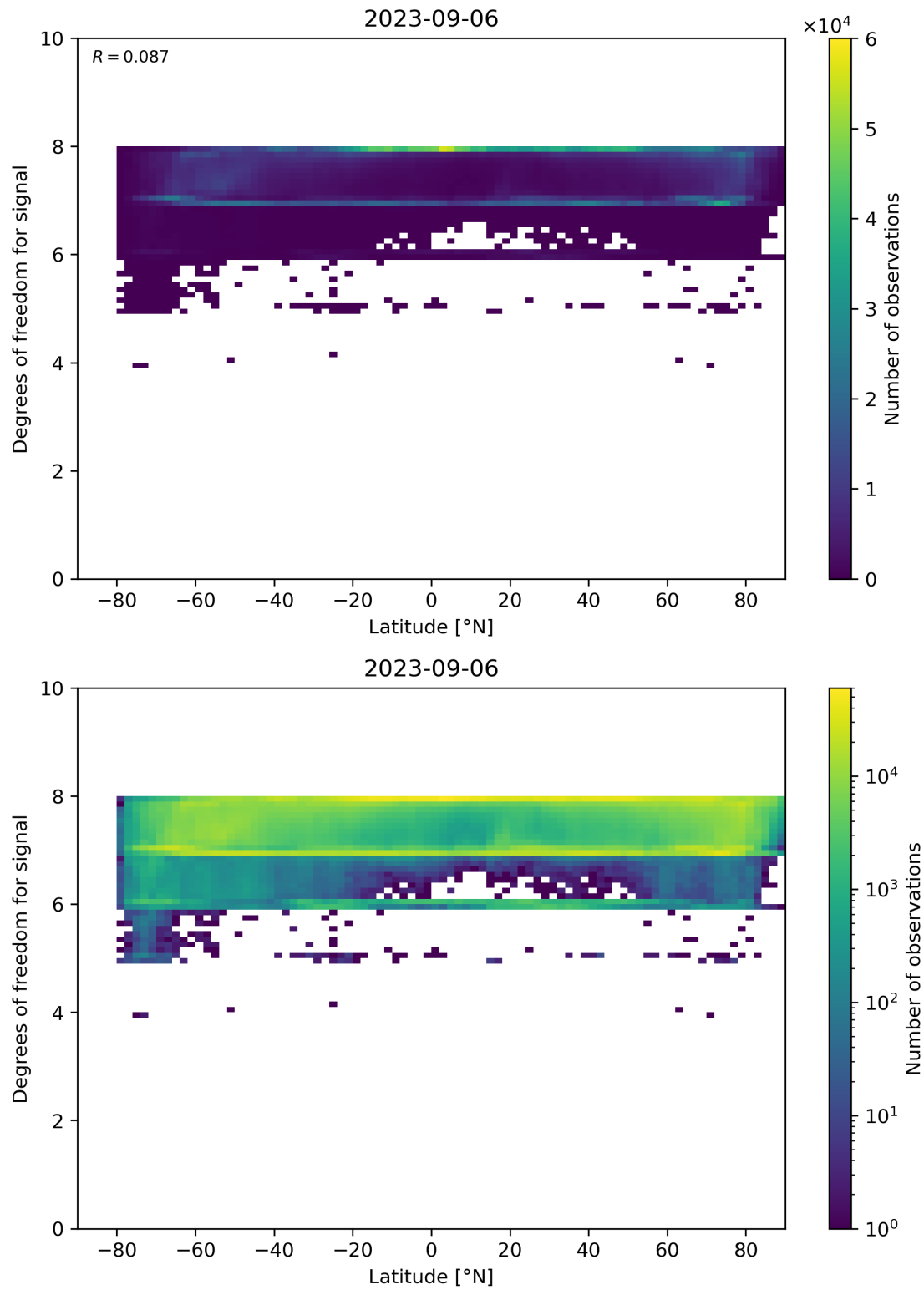
Figure 55: Scatter density plot of “Latitude” against “Degrees of freedom for signal” for 2023-09-05 to 2023-09-07.
