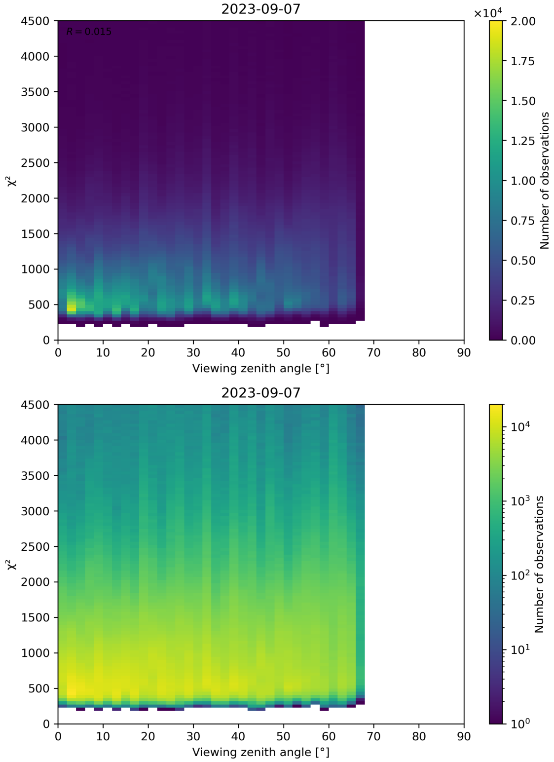
Figure 72: Scatter density plot of “Viewing zenith angle” against “ \chi^2 ” for 2023-09-06 to 2023-09-08.
