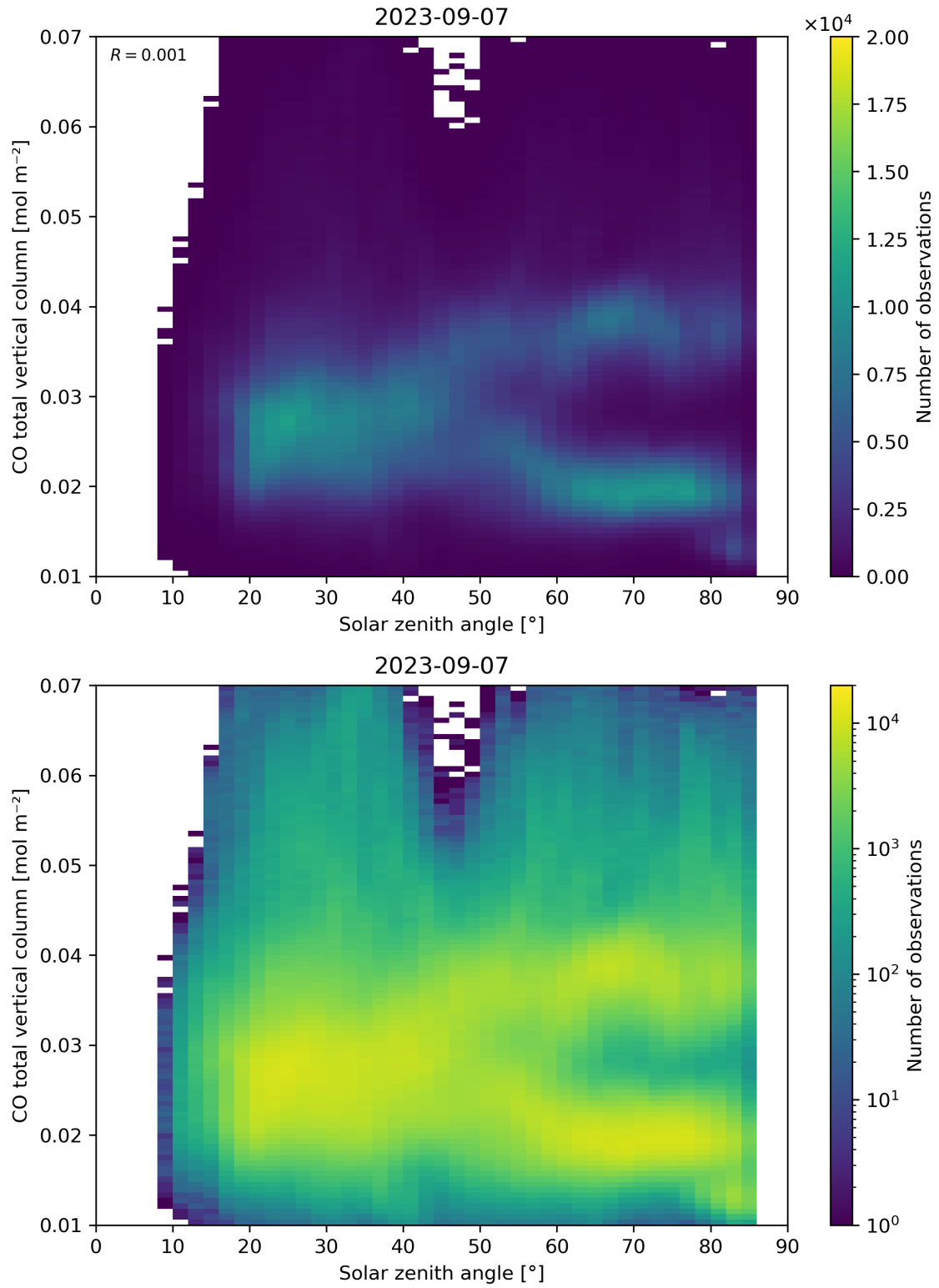
Figure 61: Scatter density plot of “Solar zenith angle” against “CO total vertical column” for 2023-09-06 to 2023-09-08.
