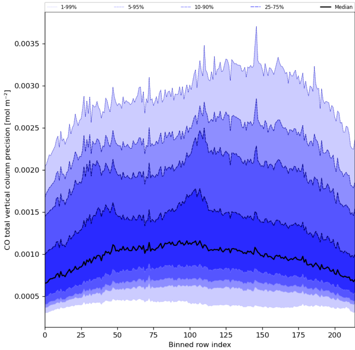
Figure 28: Along track statistics of “CO total vertical column precision” for 2023-09-06 to 2023-09-08
