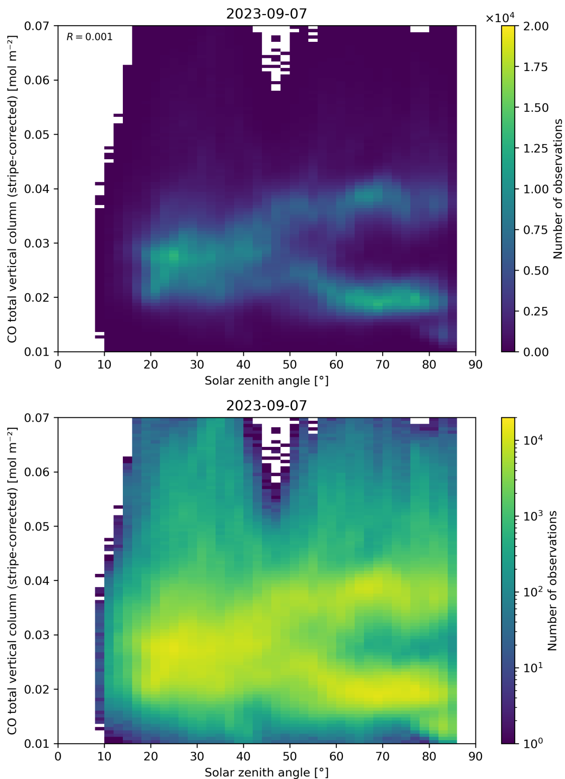
Figure 62: Scatter density plot of “Solar zenith angle” against “CO total vertical column (stripe-corrected)” for 2023-09-06 to 2023-09-08.
