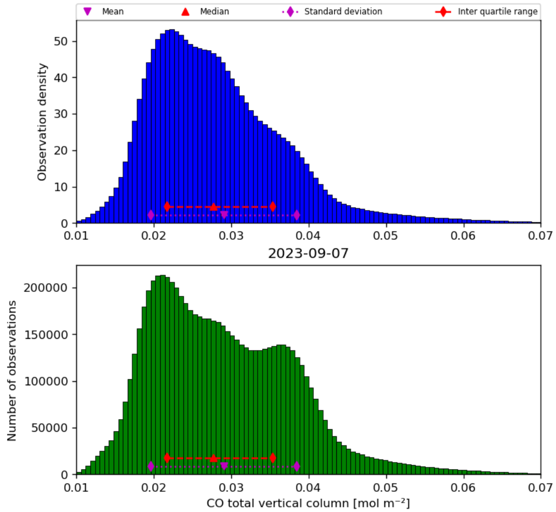
Figure 18: Histogram of “CO total vertical column” for 2023-09-06 to 2023-09-08
