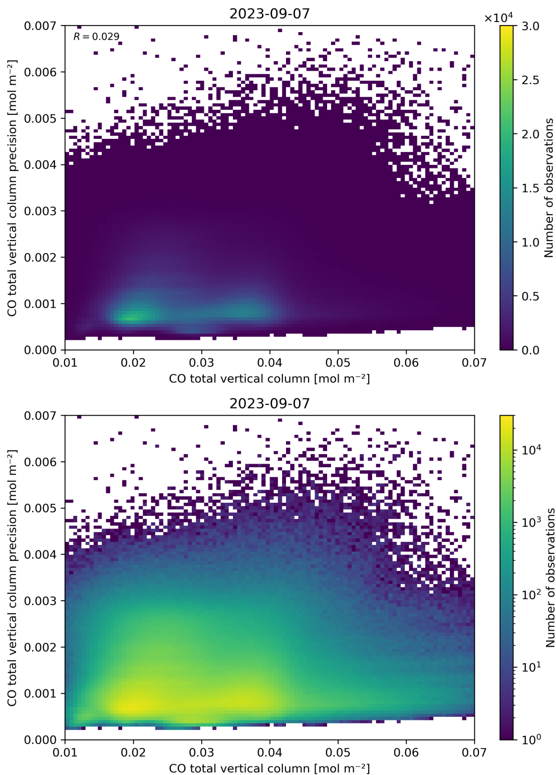
Figure 34: Scatter density plot of “CO total vertical column” against “CO total vertical column precision” for 2023-09-06 to 2023-09-08.
