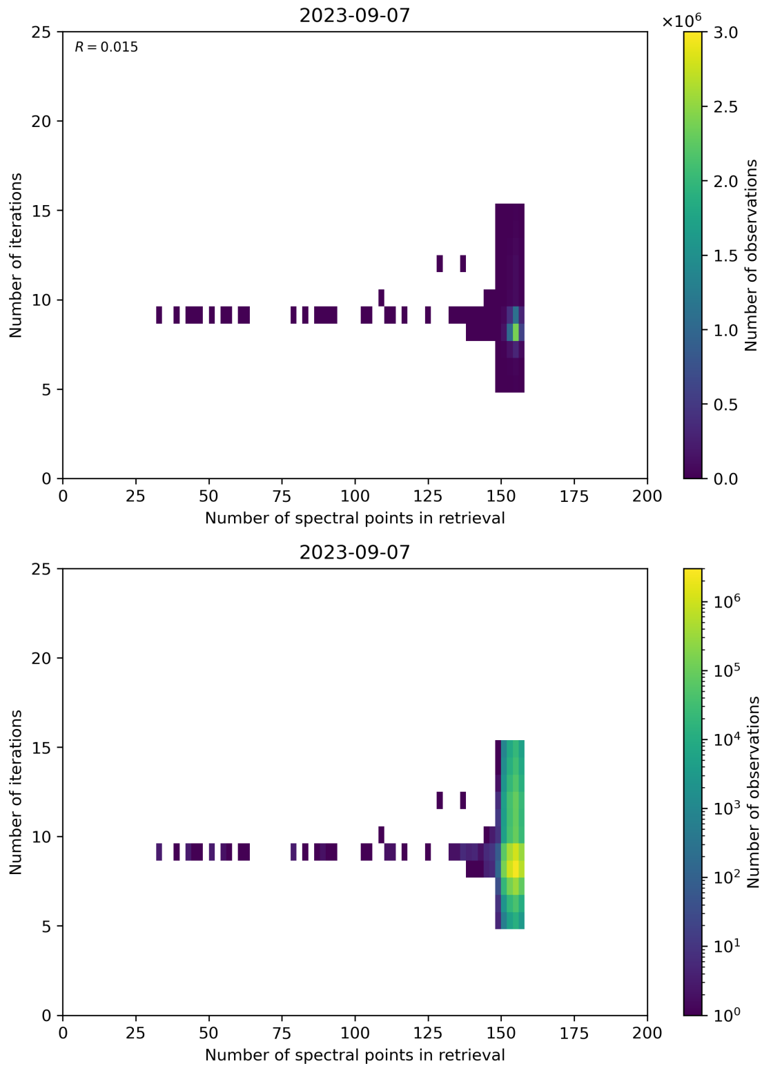
Figure 60: Scatter density plot of “Number of spectral points in retrieval” against “Number of iterations” for 2023-09-06 to 2023-09-08.
