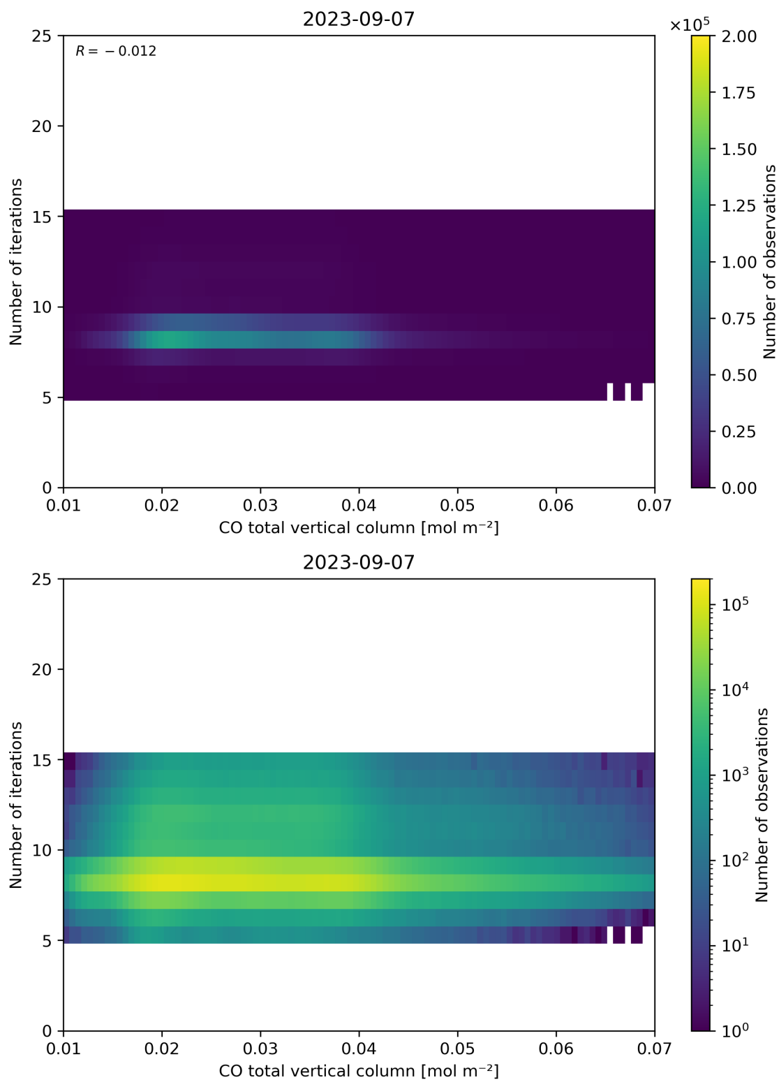
Figure 42: Scatter density plot of “CO total vertical column” against “Number of iterations” for 2023-09-06 to 2023-09-08.
