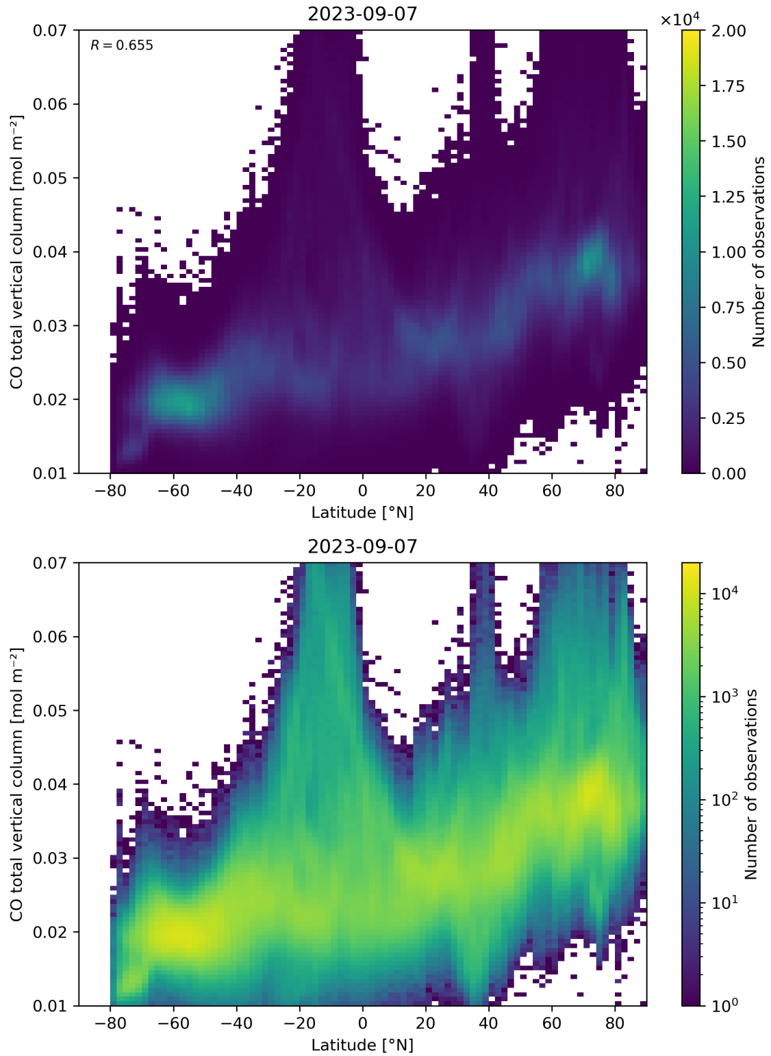
Figure 51: Scatter density plot of “Latitude” against “CO total vertical column” for 2023-09-06 to 2023-09-08.
