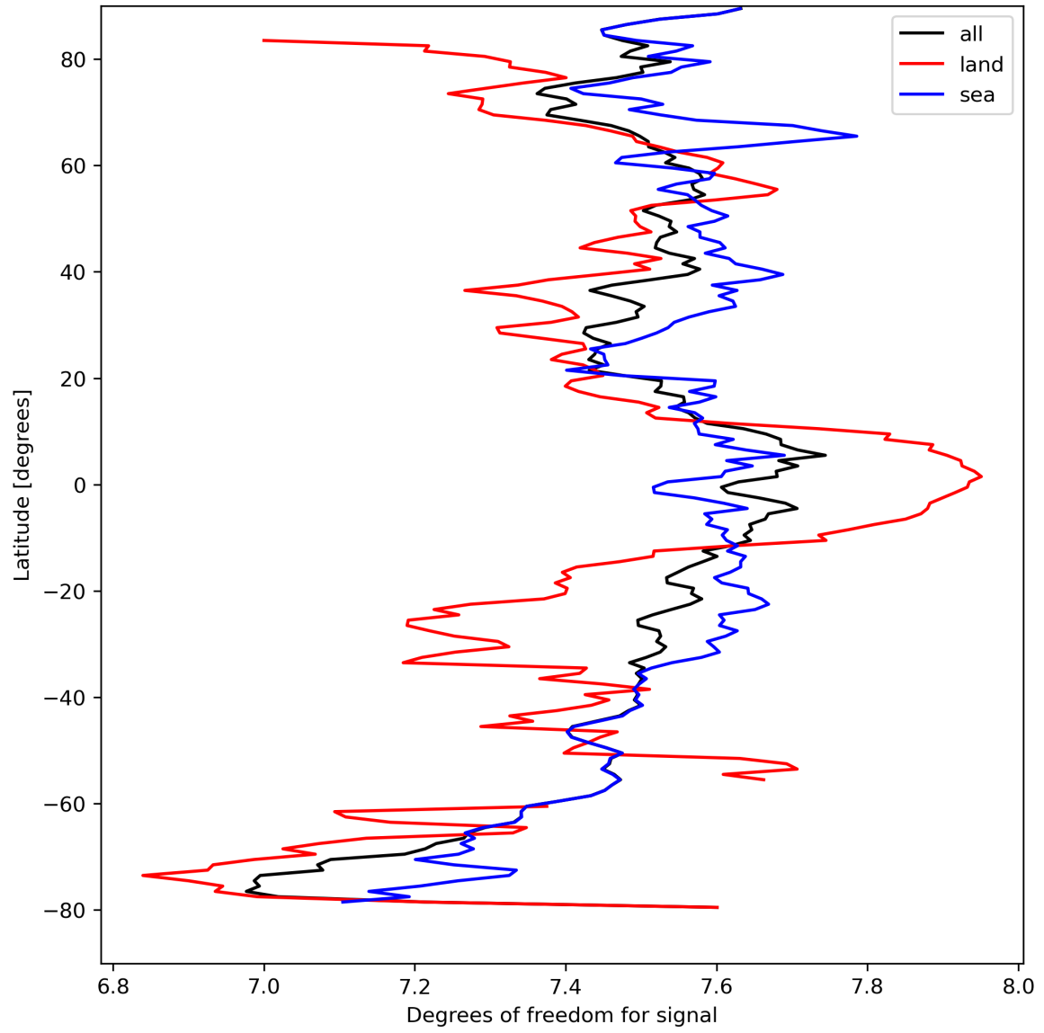
Figure 15: Zonal average of “Degrees of freedom for signal” for 2023-09-06 to 2023-09-08.
