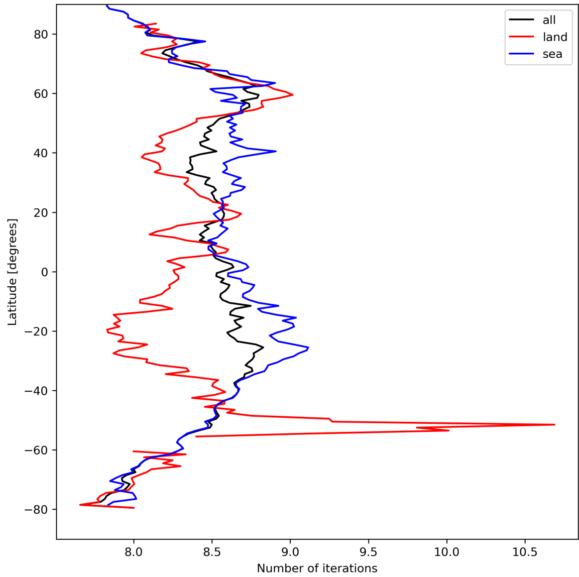
Figure 16: Zonal average of “Number of iterations” for 2023-09-06 to 2023-09-08.
