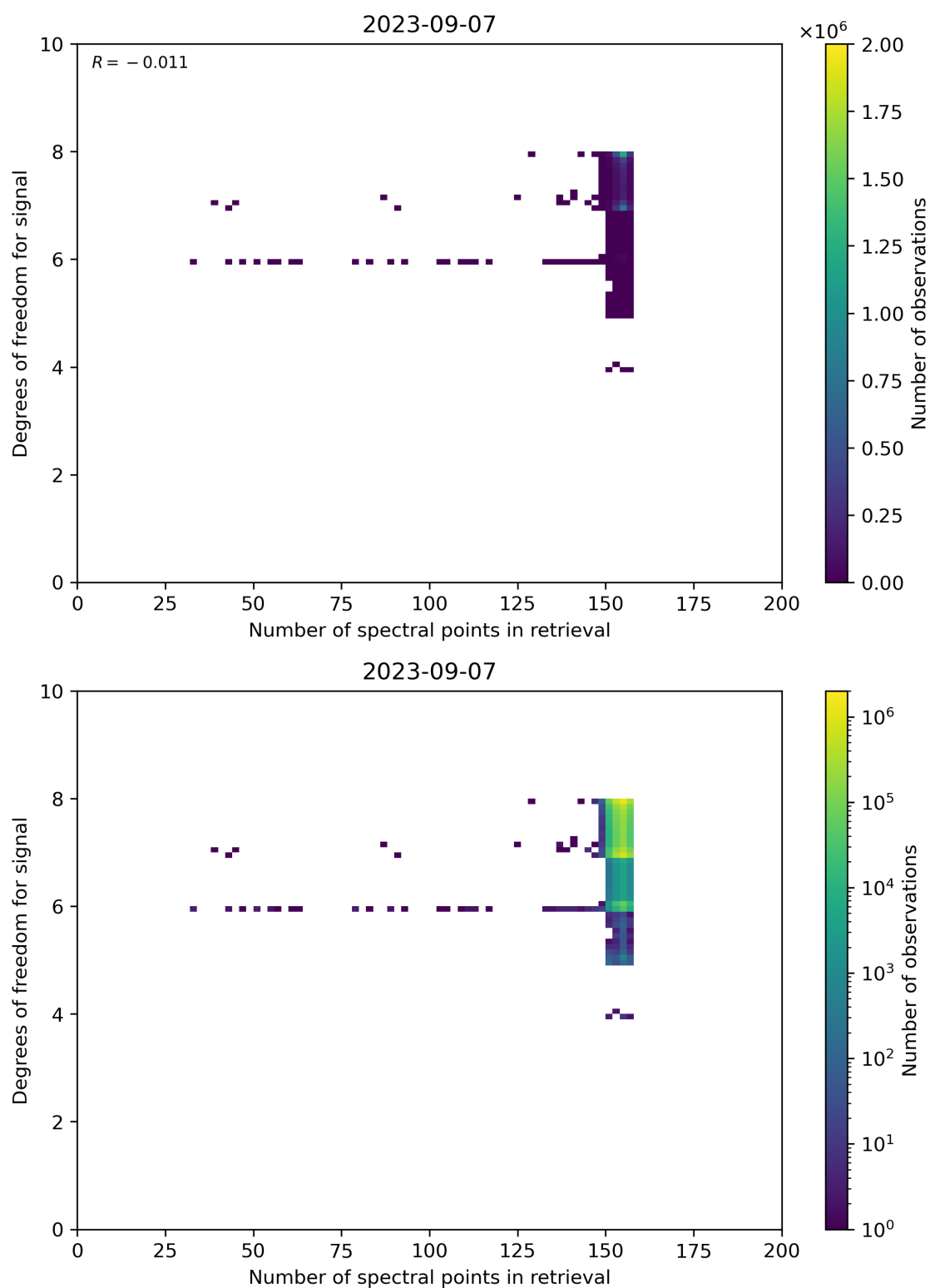
Figure 59: Scatter density plot of “Number of spectral points in retrieval” against “Degrees of freedom for signal” for 2023-09-06 to 2023-09-08.
