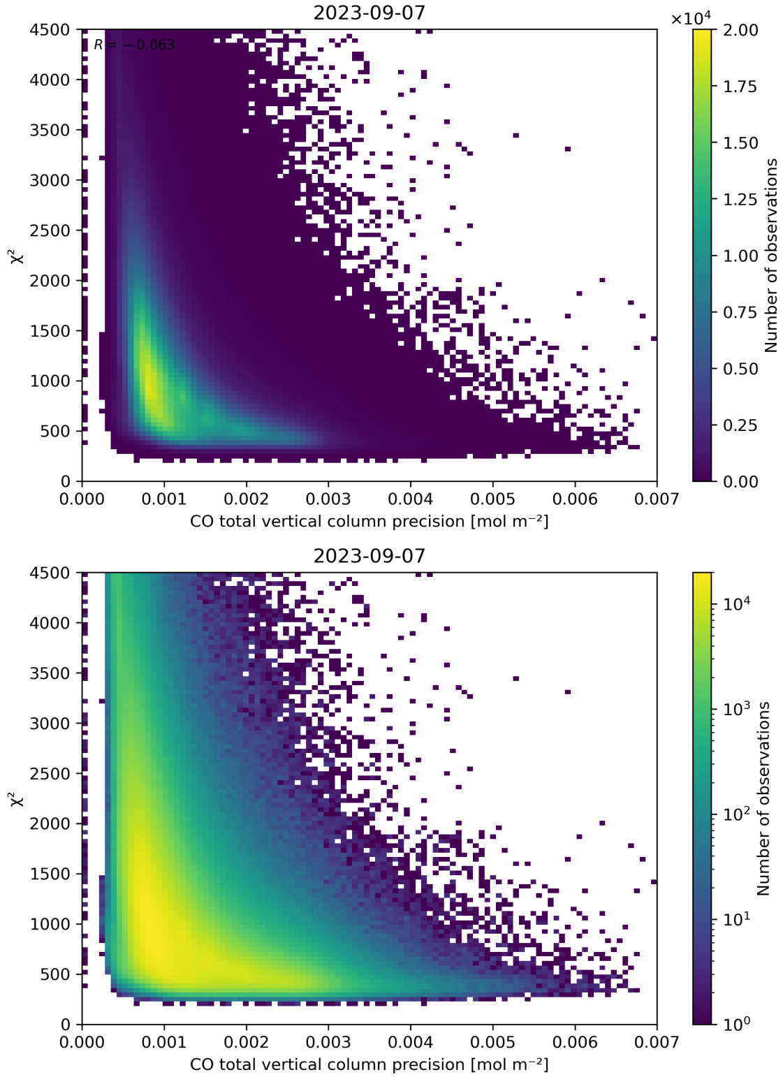
Figure 44: Scatter density plot of “CO total vertical column precision” against “ \chi^2 ” for 2023-09-06 to 2023-09-08.
