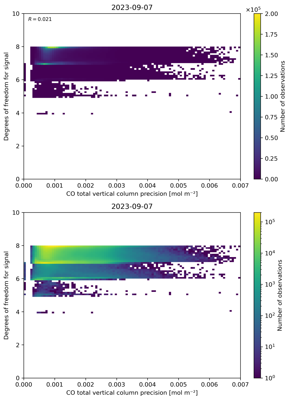
Figure 45: Scatter density plot of “CO total vertical column precision” against “Degrees of freedom for signal” for 2023-09-06 to 2023-09-08.
