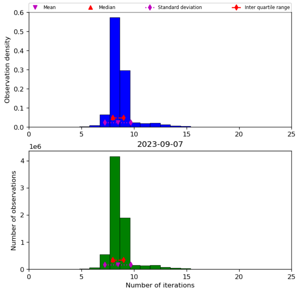
Figure 24: Histogram of “Number of iterations” for 2023-09-06 to 2023-09-08
