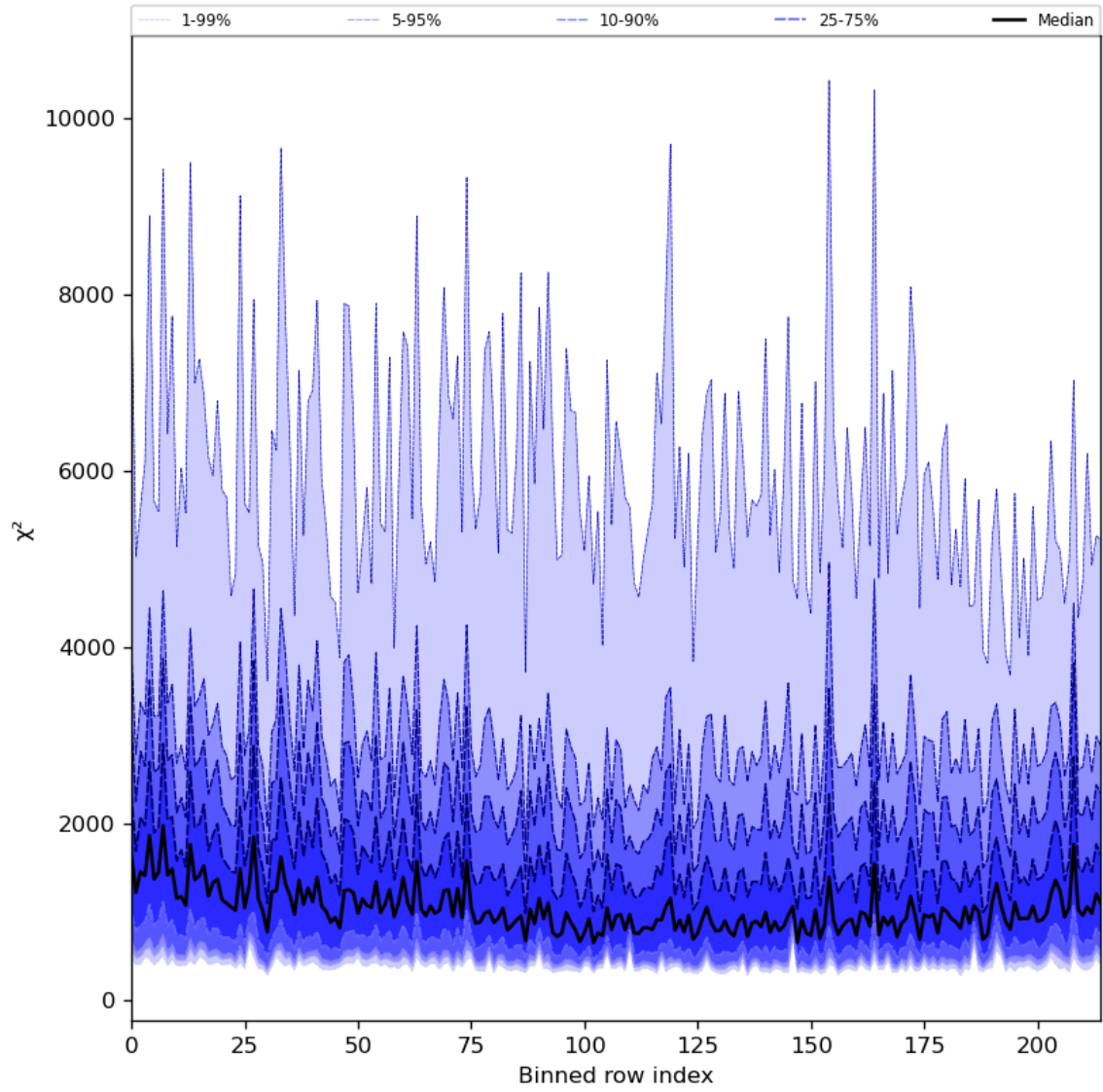
Figure 30: Along track statistics of “ \chi^2 ” for 2023-09-06 to 2023-09-08
