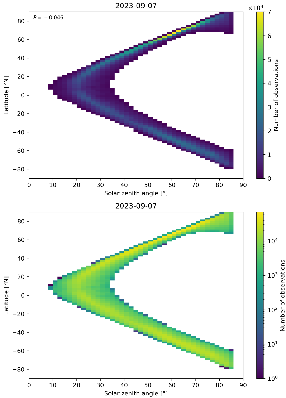
Figure 66: Scatter density plot of “Solar zenith angle” against “Latitude” for 2023-09-06 to 2023-09-08.
