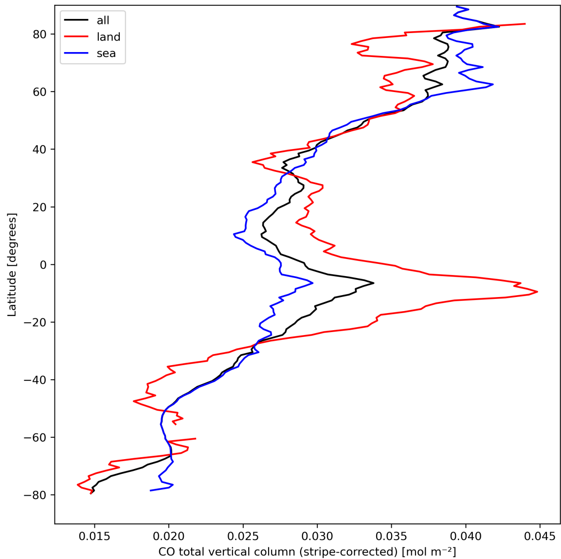
Figure 11: Zonal average of “CO total vertical column (stripe-corrected)” for 2023-09-06 to 2023-09-08.
