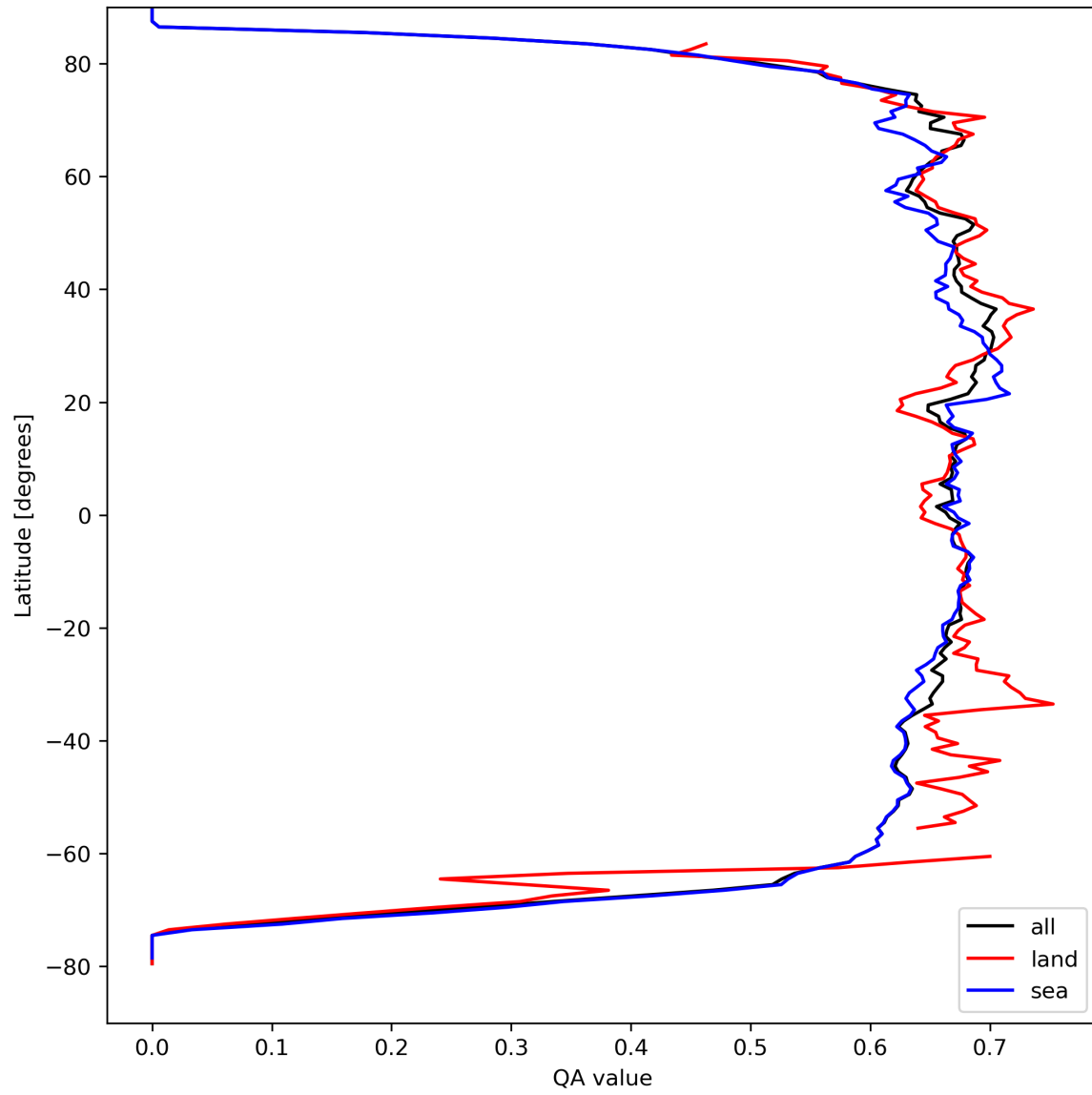
Figure 9: Zonal average of “QA value” for 2023-09-06 to 2023-09-08.
