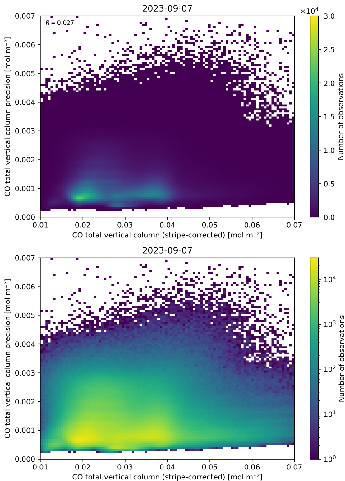
Figure 36: Scatter density plot of “CO total vertical column (stripe-corrected)” against “CO total vertical column precision” for 2023-09-06 to 2023-09-08.
