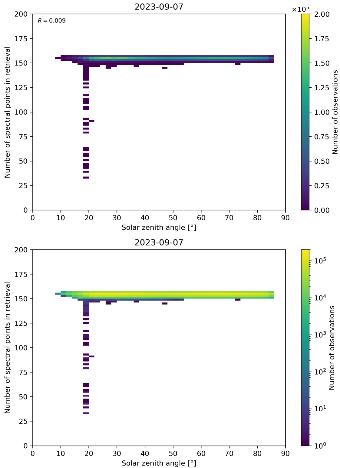
Figure 68: Scatter density plot of “Solar zenith angle” against “Number of spectral points in retrieval” for 2023-09-06 to 2023-09-08.
