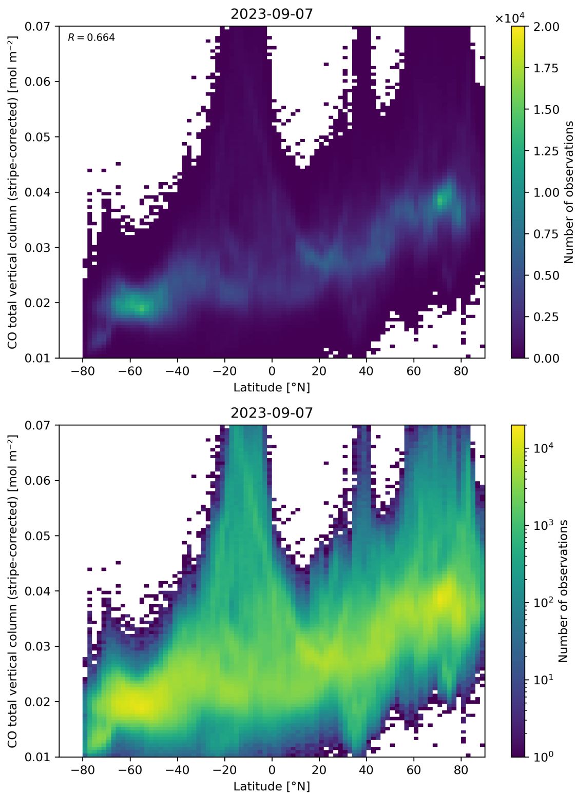
Figure 52: Scatter density plot of “Latitude” against “CO total vertical column (stripe-corrected)” for 2023-09-06 to 2023-09-08.
