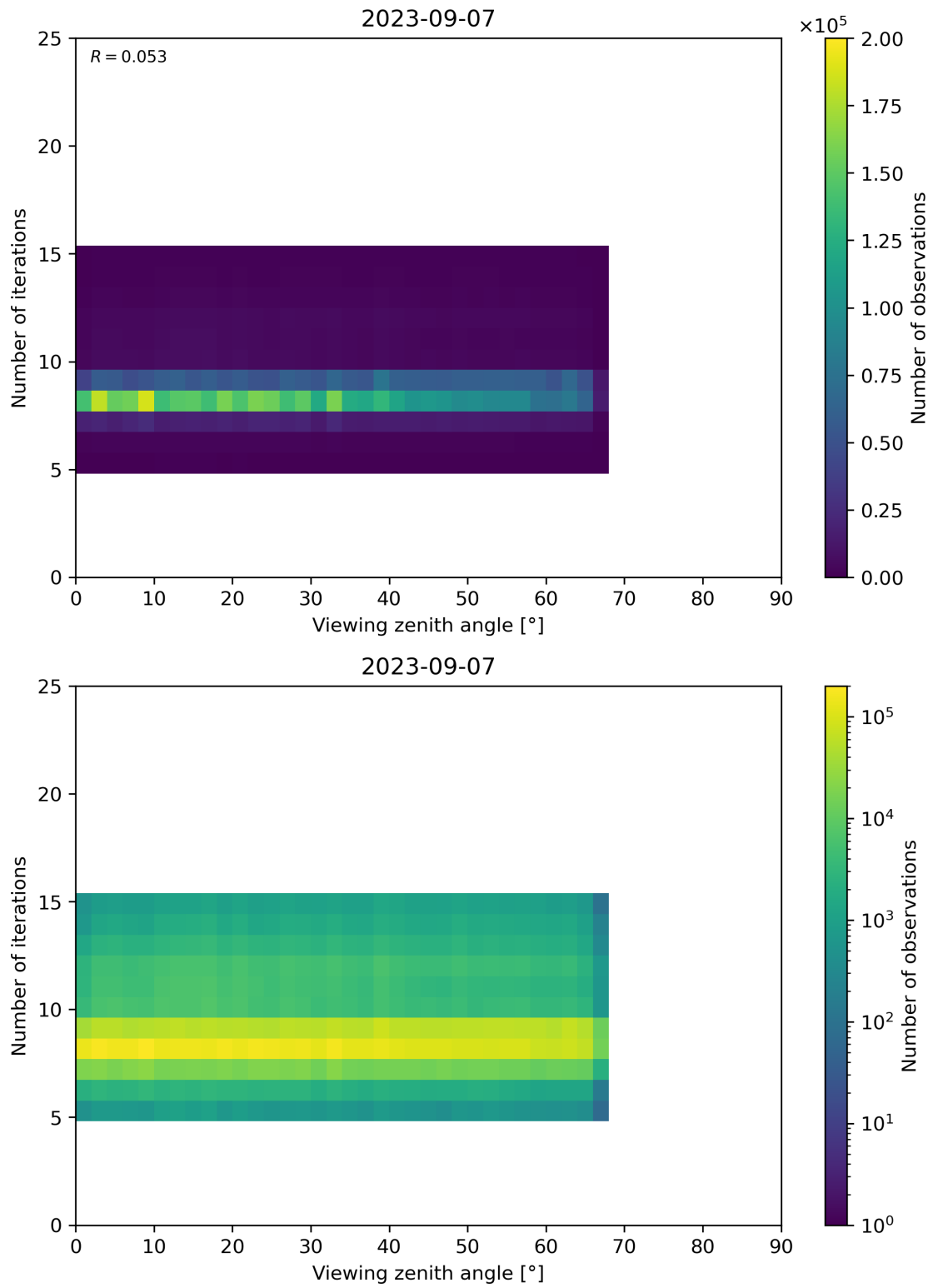
Figure 75: Scatter density plot of “Viewing zenith angle” against “Number of iterations” for 2023-09-06 to 2023-09-08.
