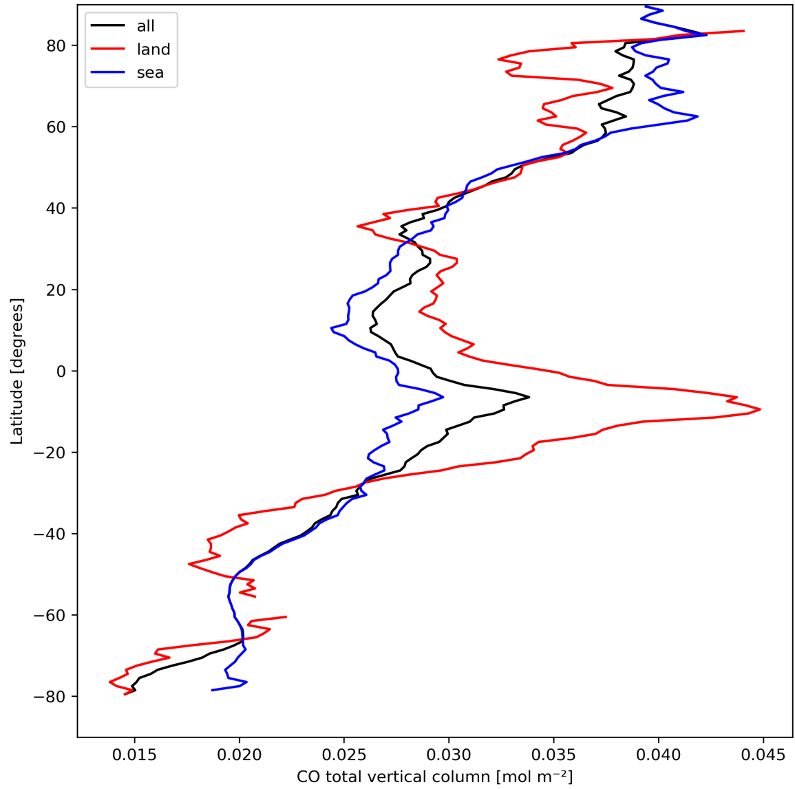
Figure 10: Zonal average of “CO total vertical column” for 2023-09-06 to 2023-09-08.
