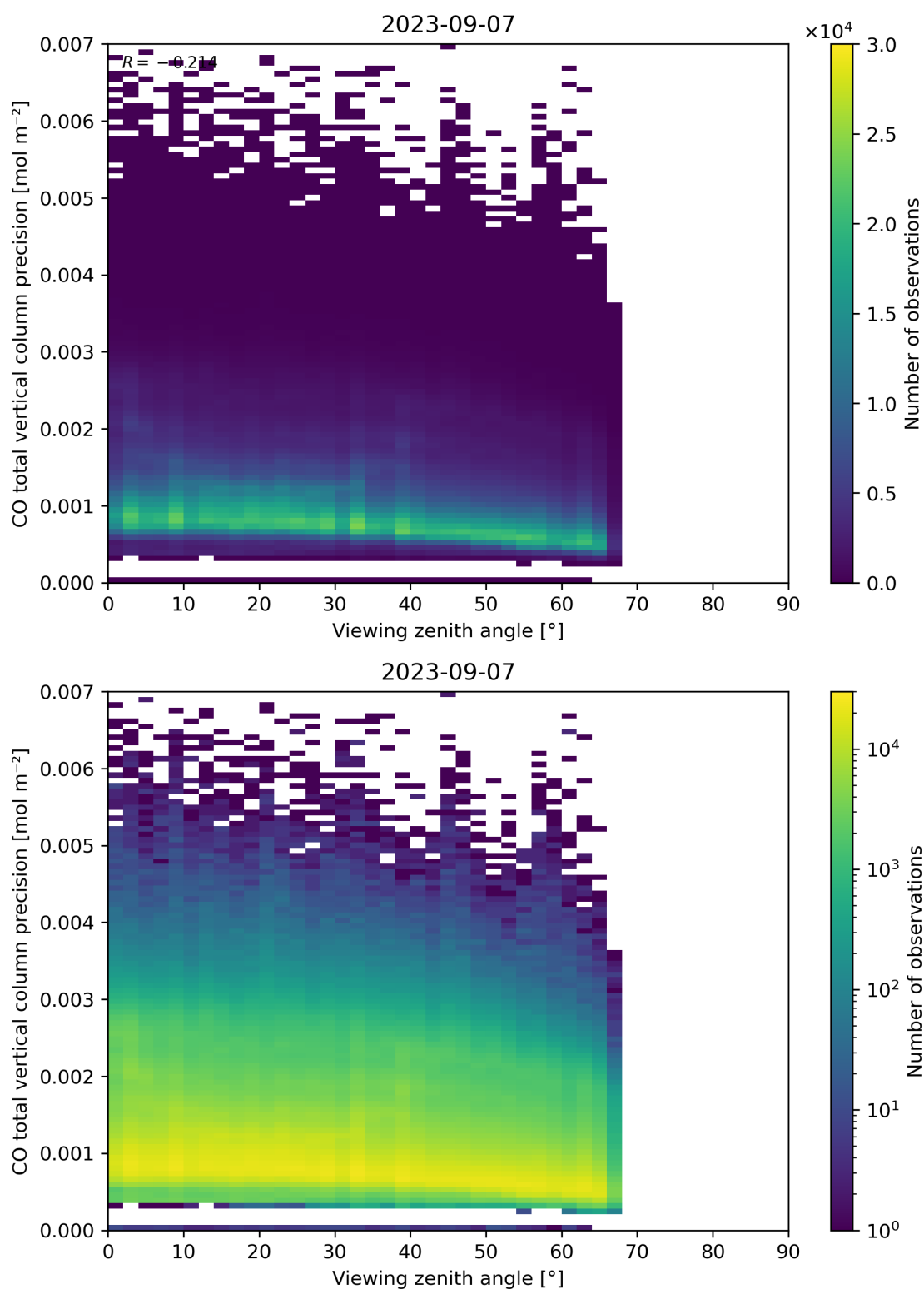
Figure 71: Scatter density plot of “Viewing zenith angle” against “CO total vertical column precision” for 2023-09-06 to 2023-09-08.
