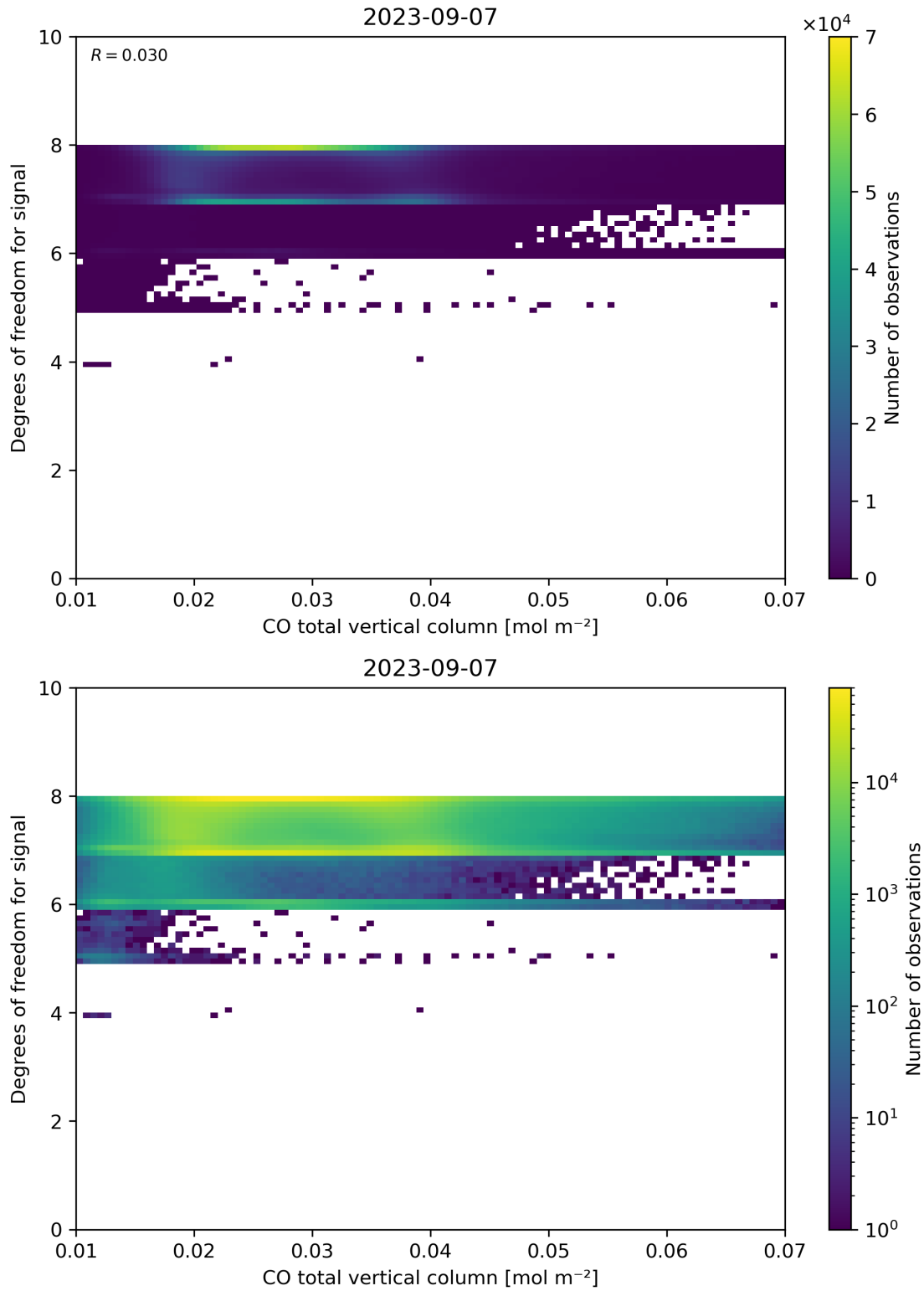
Figure 41: Scatter density plot of “CO total vertical column” against “Degrees of freedom for signal” for 2023-09-06 to 2023-09-08.
