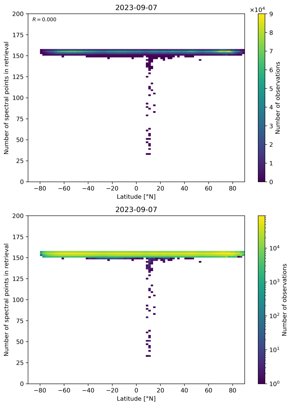
Figure 57: Scatter density plot of “Latitude” against “Number of spectral points in retrieval” for 2023-09-06 to 2023-09-08.
