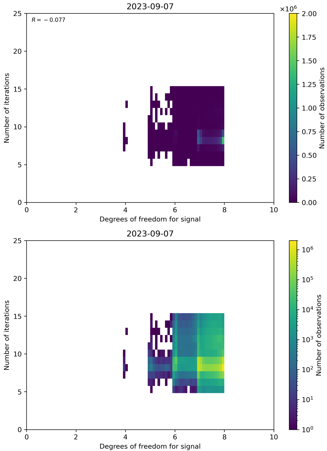
Figure 50: Scatter density plot of “Degrees of freedom for signal” against “Number of iterations” for 2023-09-06 to 2023-09-08.
