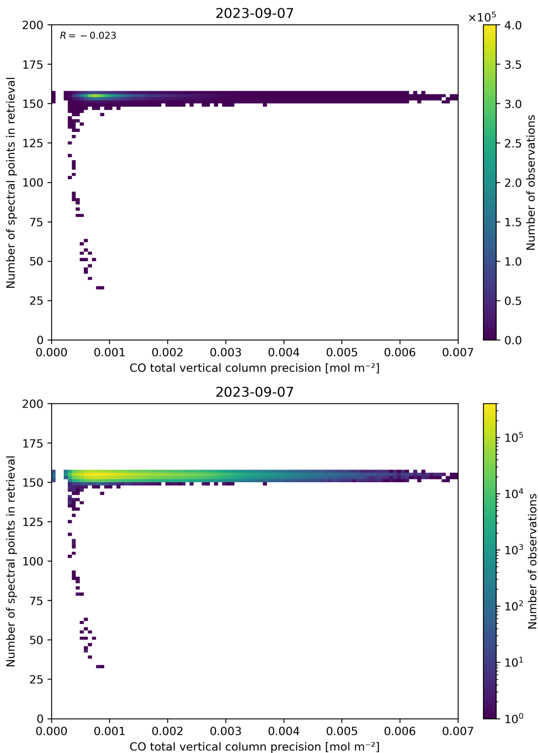
Figure 47: Scatter density plot of “CO total vertical column precision” against “Number of spectral points in retrieval” for 2023-09-06 to 2023-09-08.
