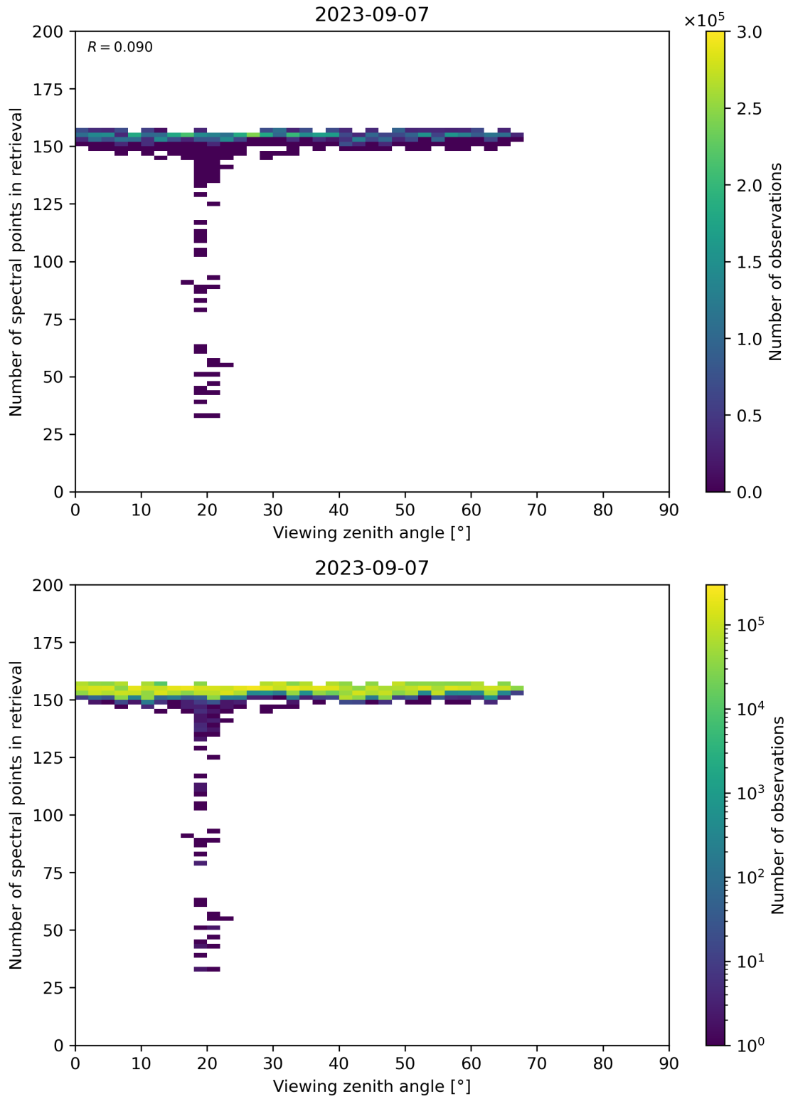
Figure 76: Scatter density plot of “Viewing zenith angle” against “Number of spectral points in retrieval” for 2023-09-06 to 2023-09-08.
