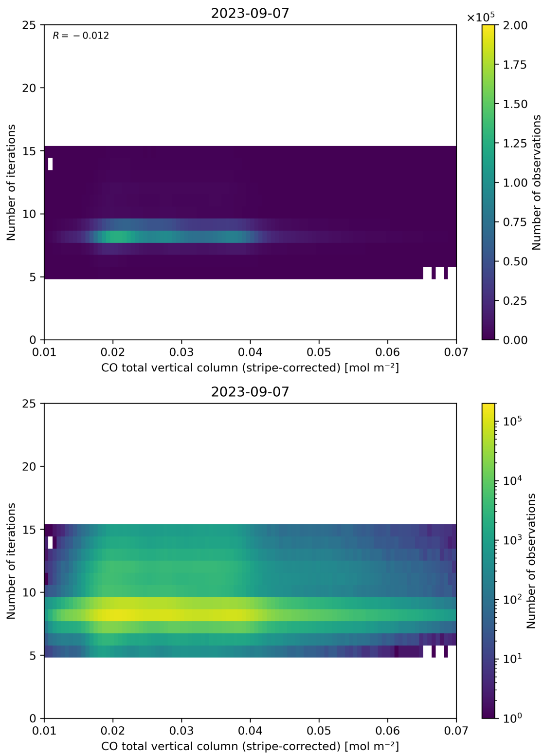
Figure 39: Scatter density plot of “CO total vertical column (stripe-corrected)” against “Number of iterations” for 2023-09-06 to 2023-09-08.
