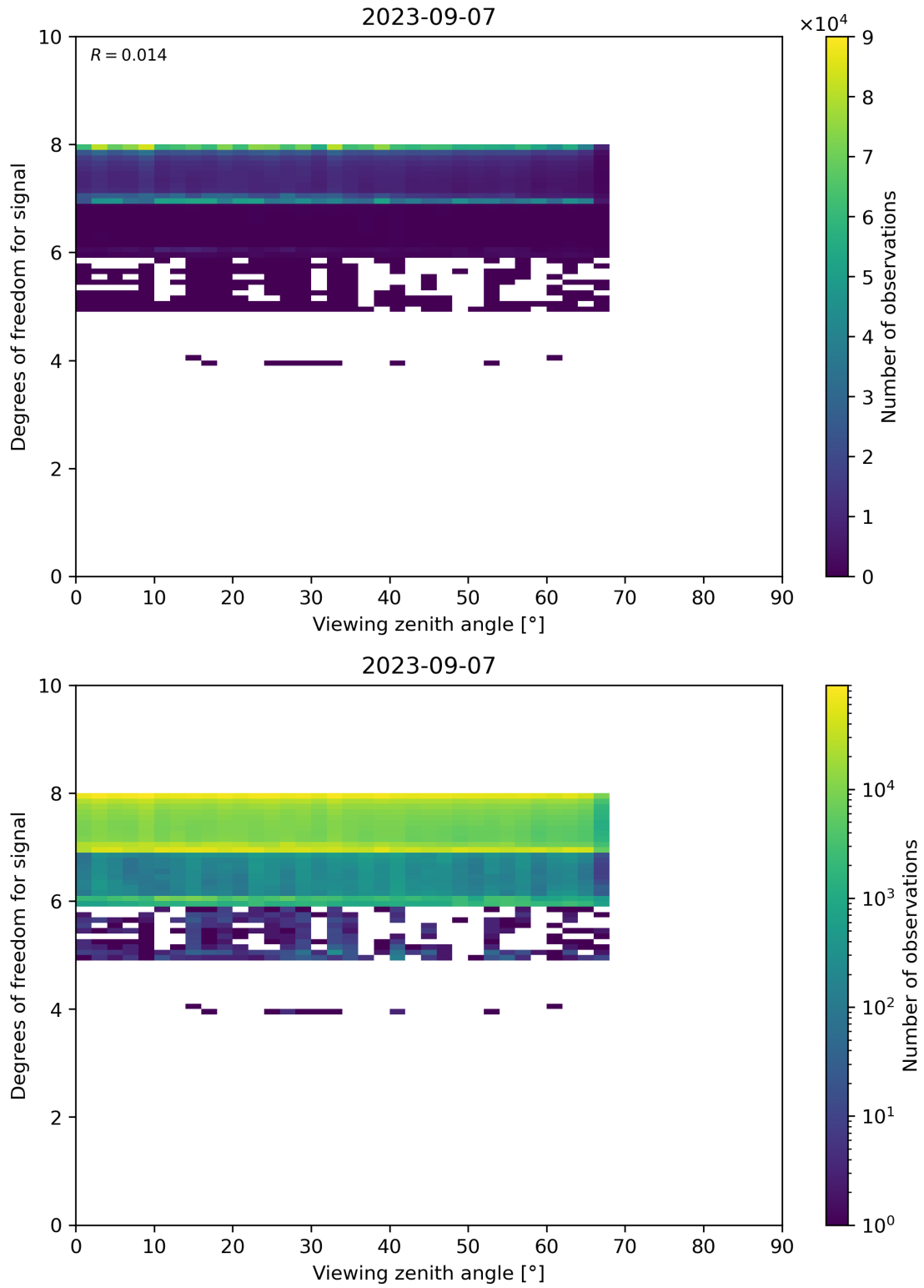
Figure 73: Scatter density plot of “Viewing zenith angle” against “Degrees of freedom for signal” for 2023-09-06 to 2023-09-08.
