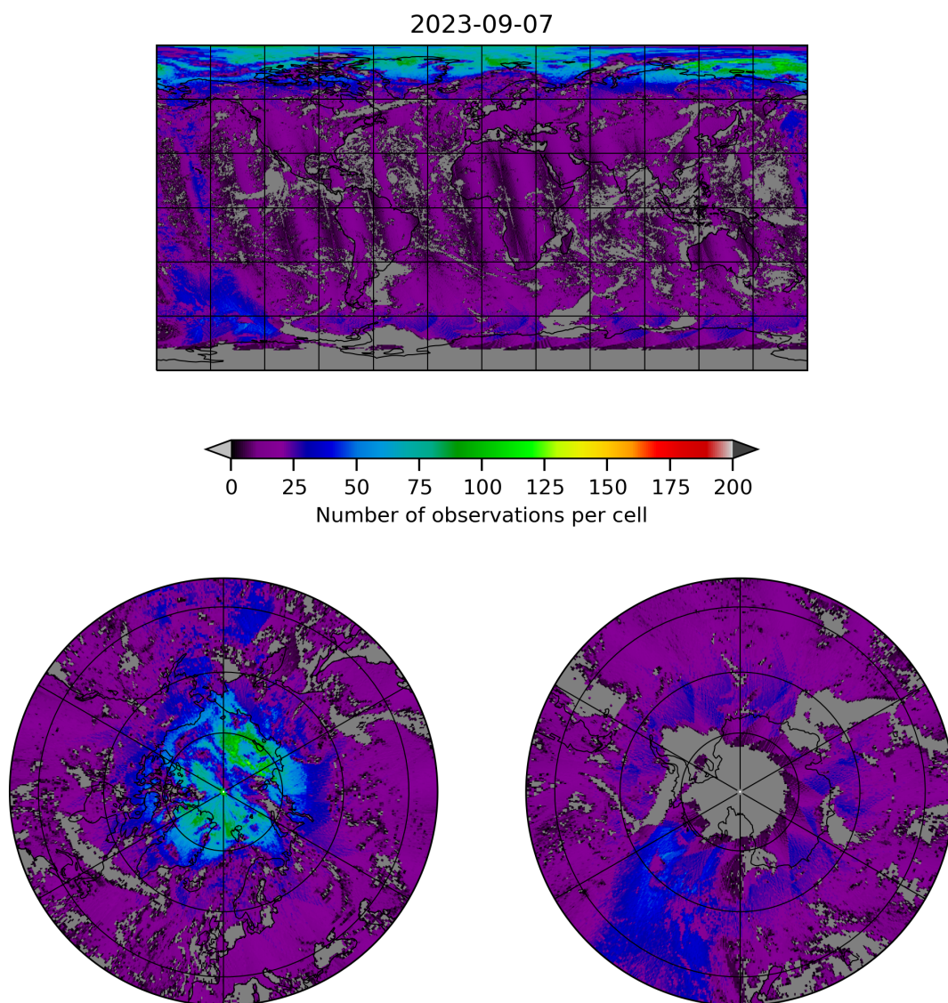
Figure 8: Map of the number of observations for 2023-09-06 to 2023-09-08
