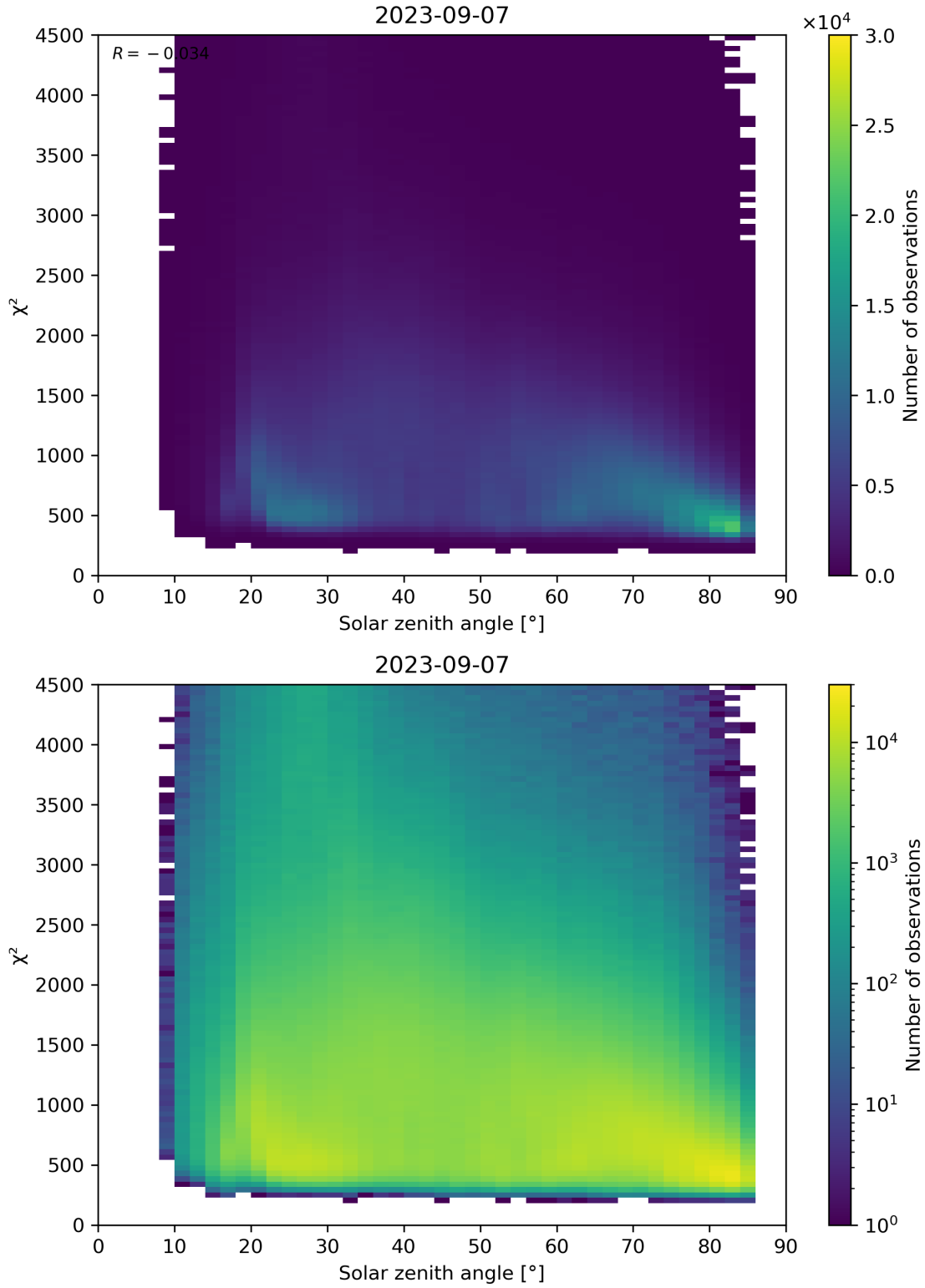
Figure 64: Scatter density plot of “Solar zenith angle” against “ \chi^2 ” for 2023-09-06 to 2023-09-08.
