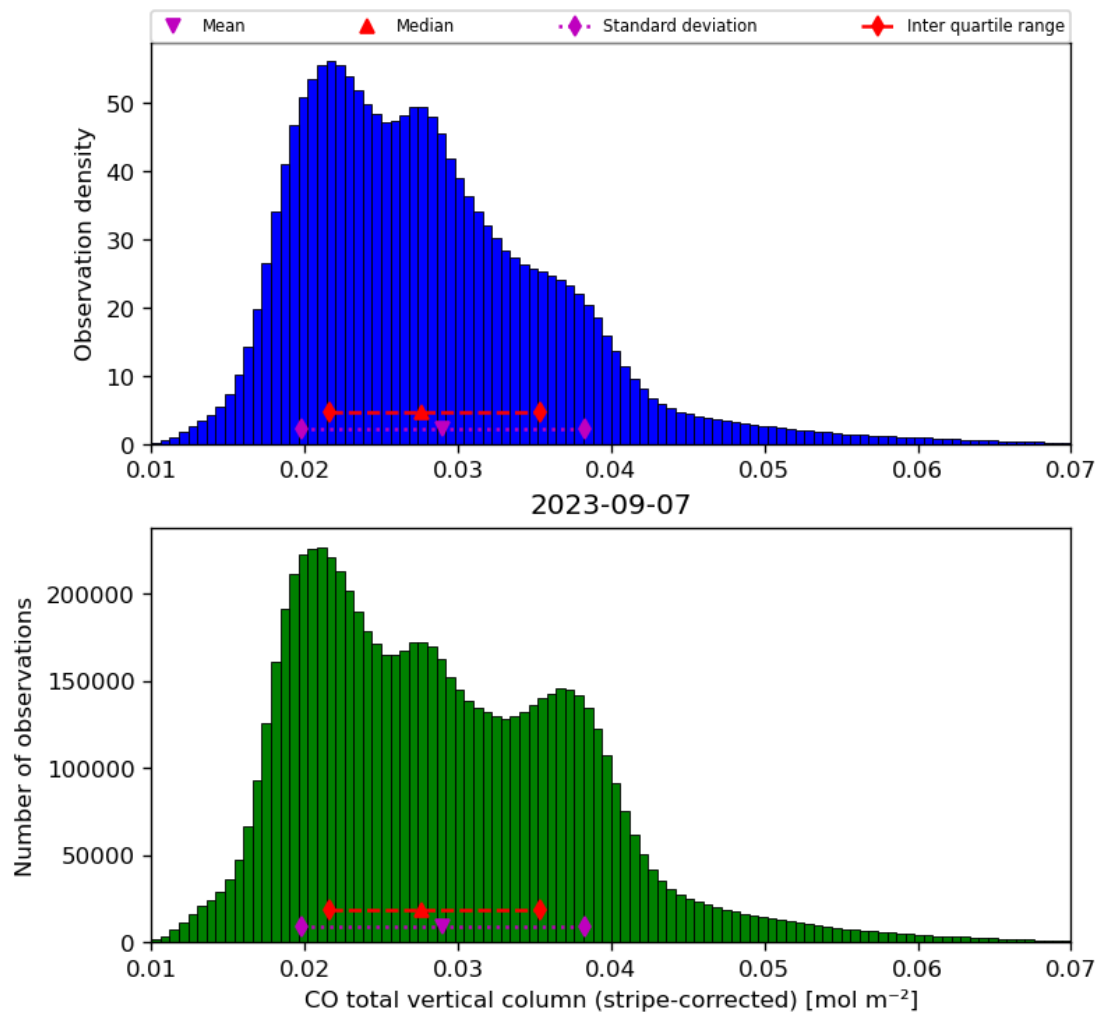
Figure 19: Histogram of “CO total vertical column (stripe-corrected)” for 2023-09-06 to 2023-09-08
