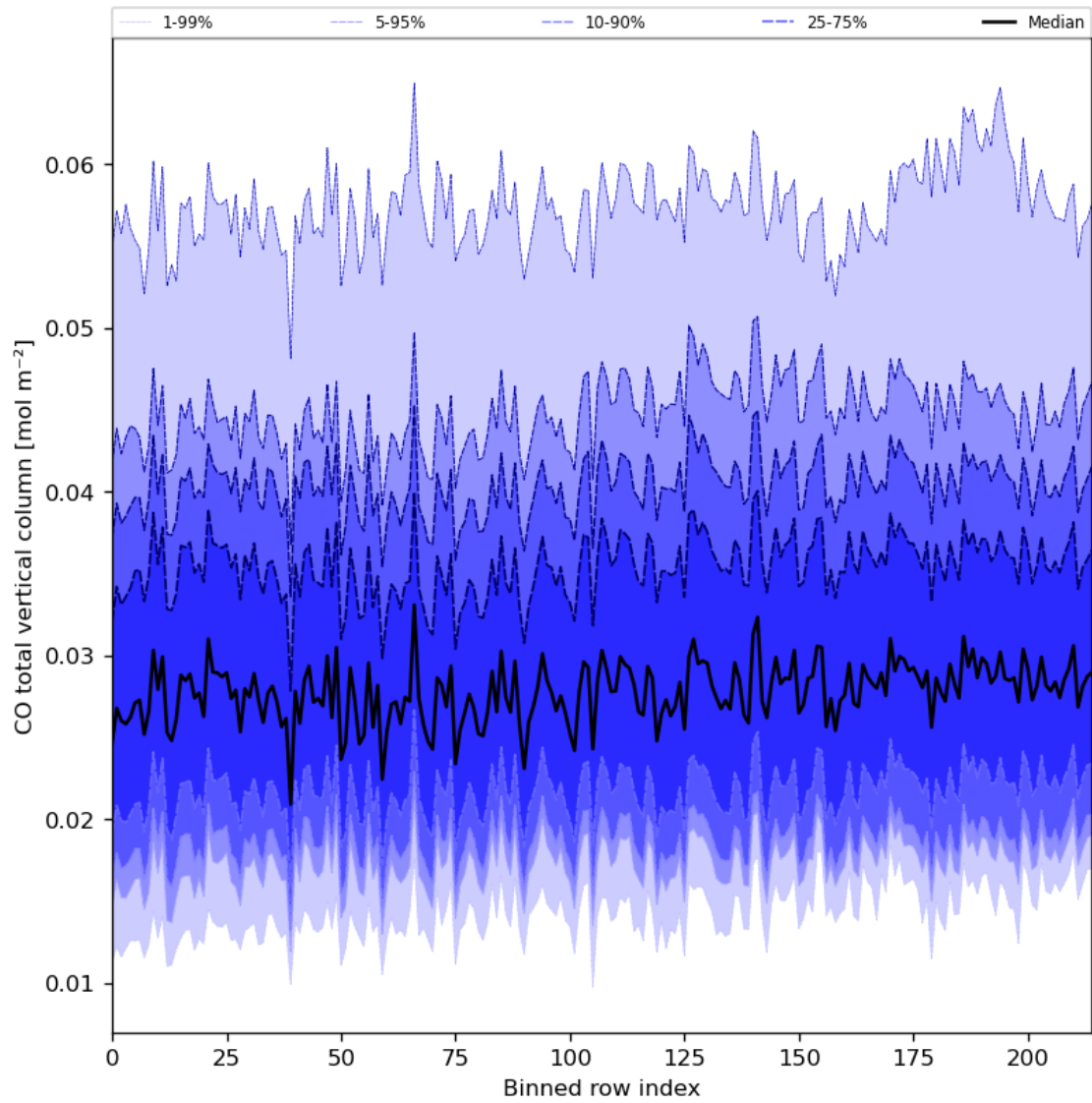
Figure 26: Along track statistics of “CO total vertical column” for 2023-09-06 to 2023-09-08
