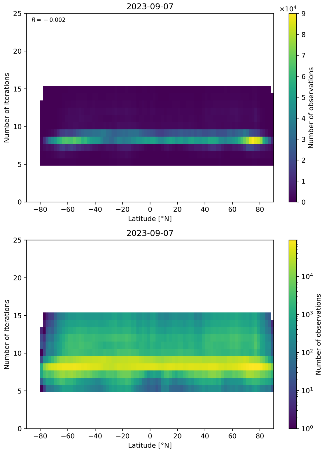
Figure 56: Scatter density plot of “Latitude” against “Number of iterations” for 2023-09-06 to 2023-09-08.
