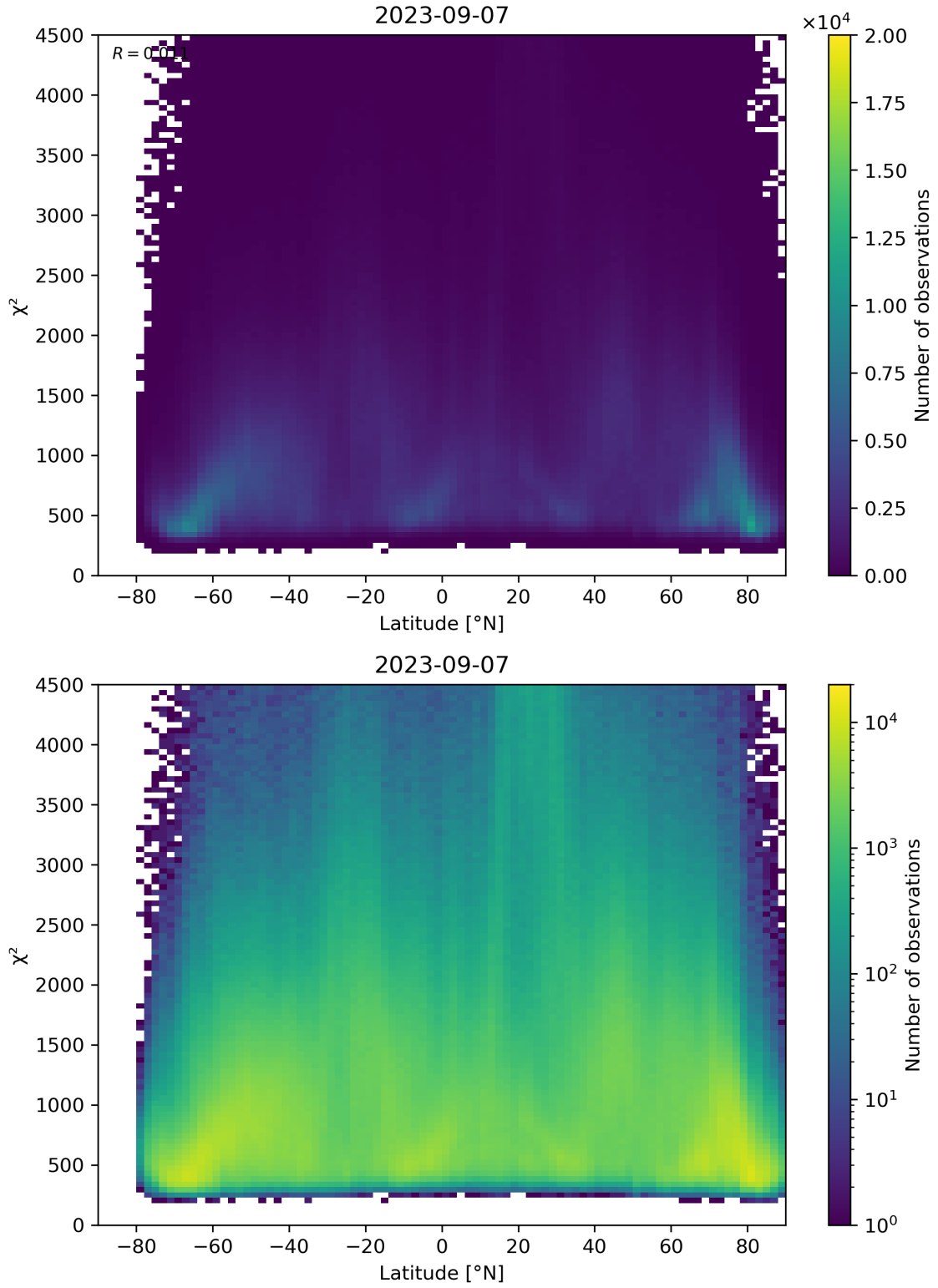
Figure 54: Scatter density plot of “Latitude” against “ \chi^2 ” for 2023-09-06 to 2023-09-08.
