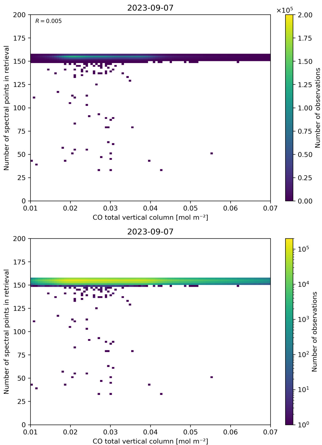
Figure 43: Scatter density plot of “CO total vertical column” against “Number of spectral points in retrieval” for 2023-09-06 to 2023-09-08.
