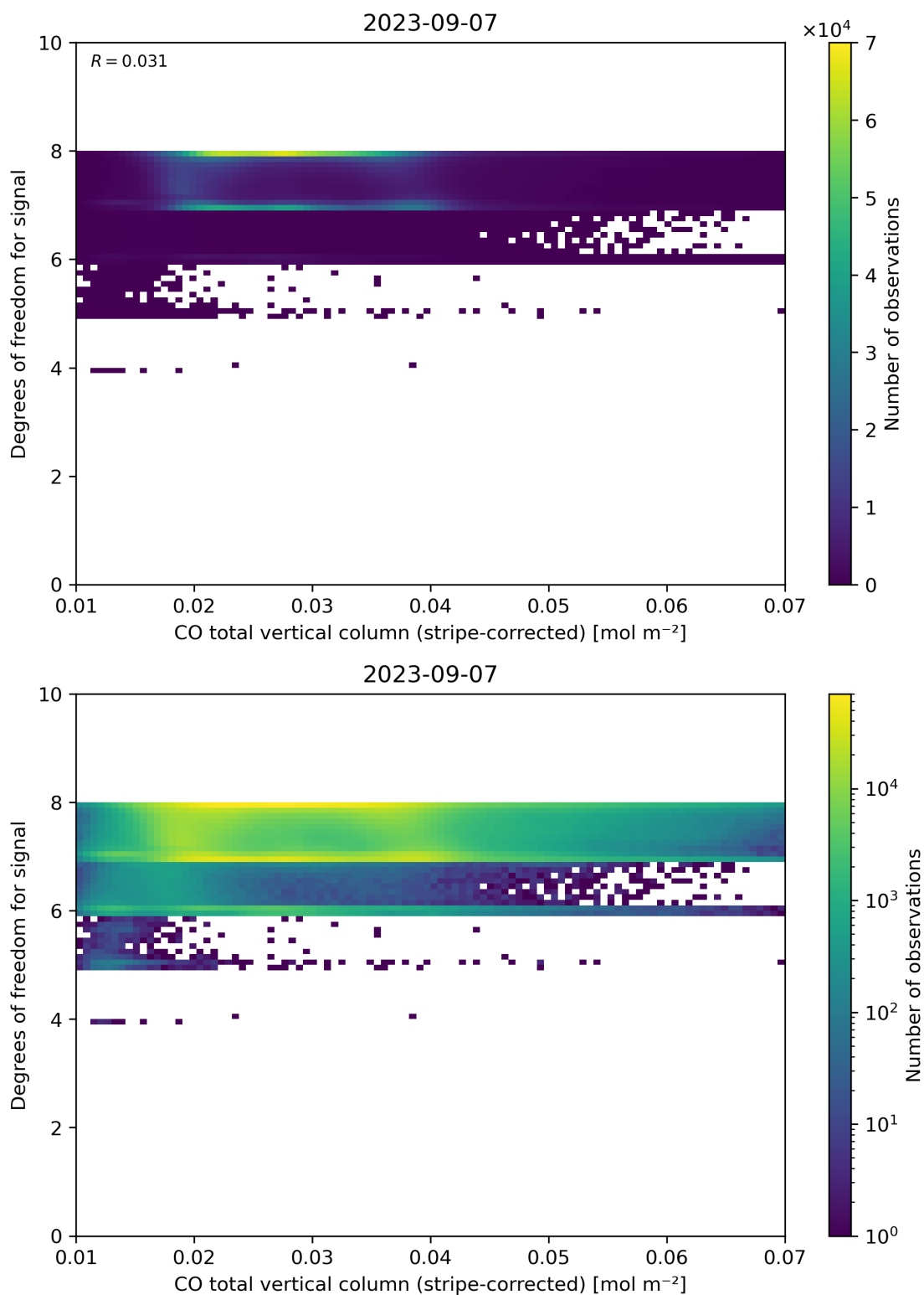
Figure 38: Scatter density plot of “CO total vertical column (stripe-corrected)” against “Degrees of freedom for signal” for 2023-09-06 to 2023-09-08.
