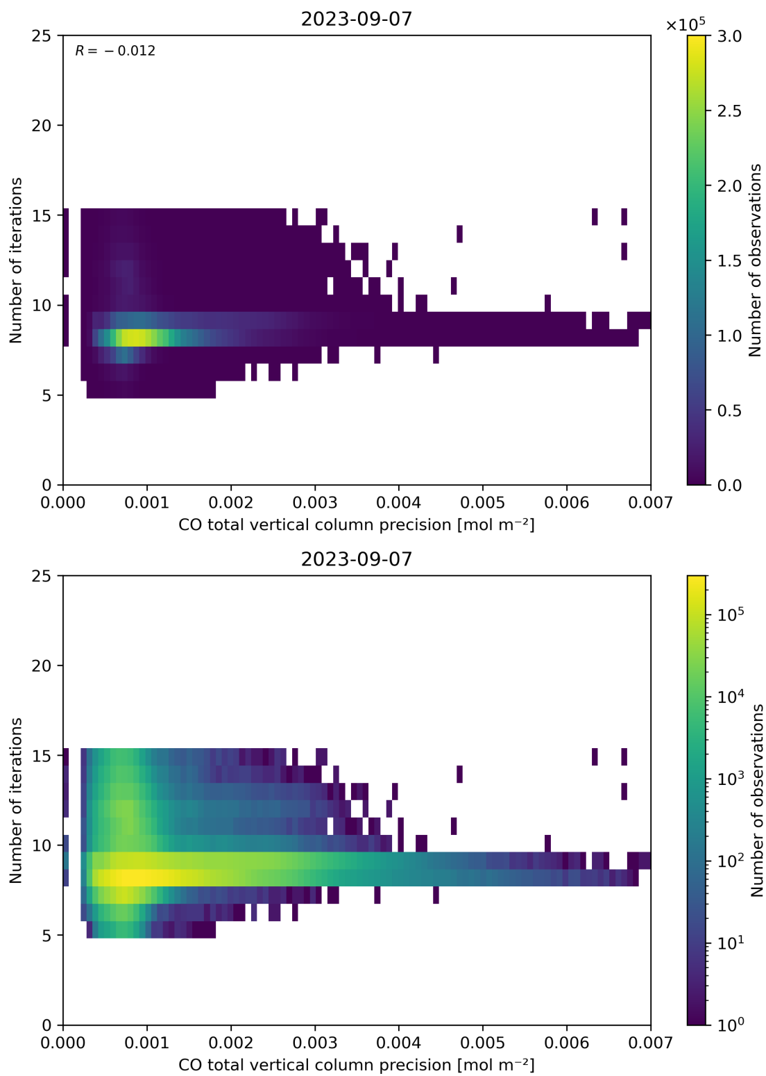
Figure 46: Scatter density plot of “CO total vertical column precision” against “Number of iterations” for 2023-09-06 to 2023-09-08.
