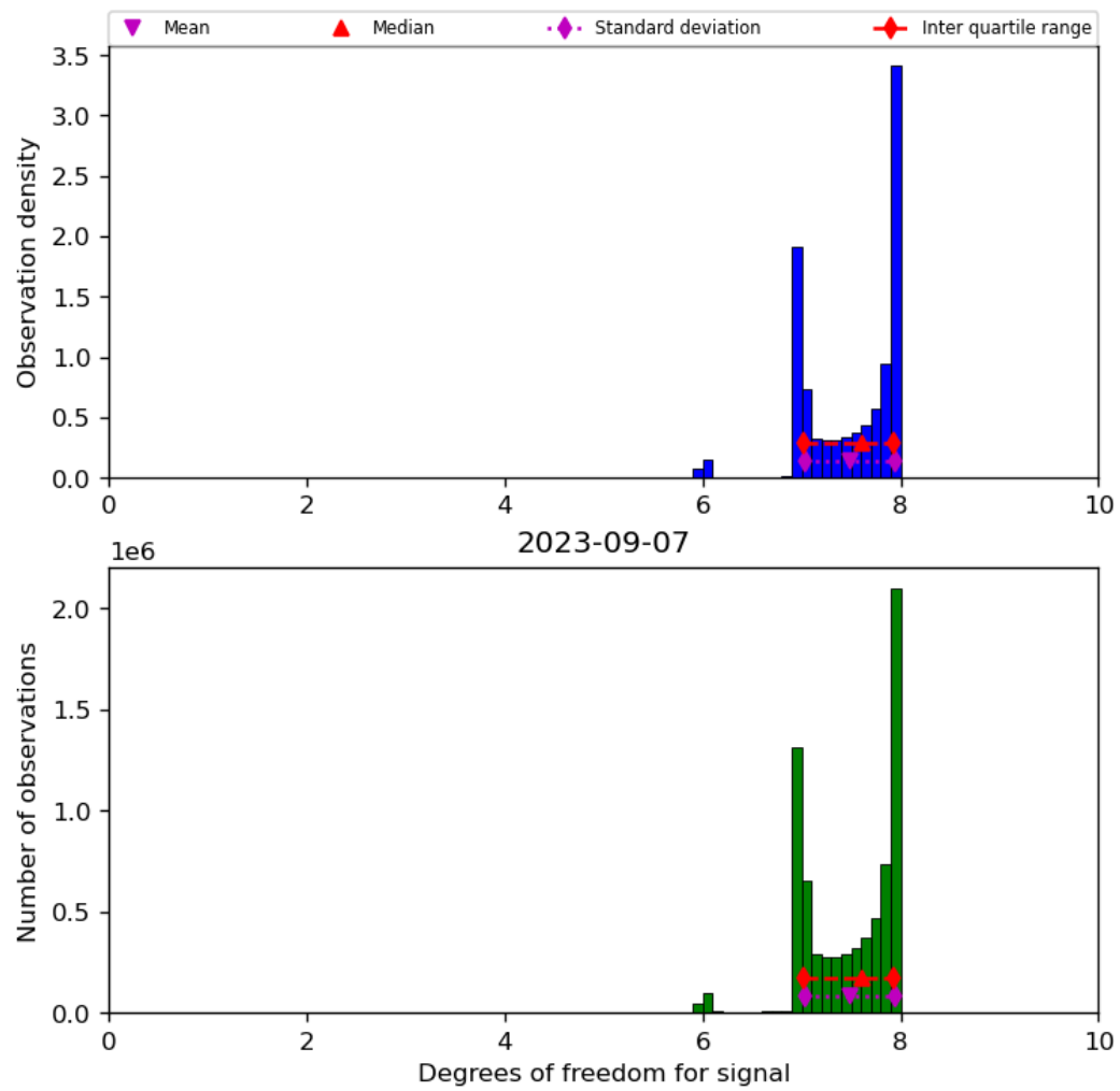
Figure 23: Histogram of “Degrees of freedom for signal” for 2023-09-06 to 2023-09-08
