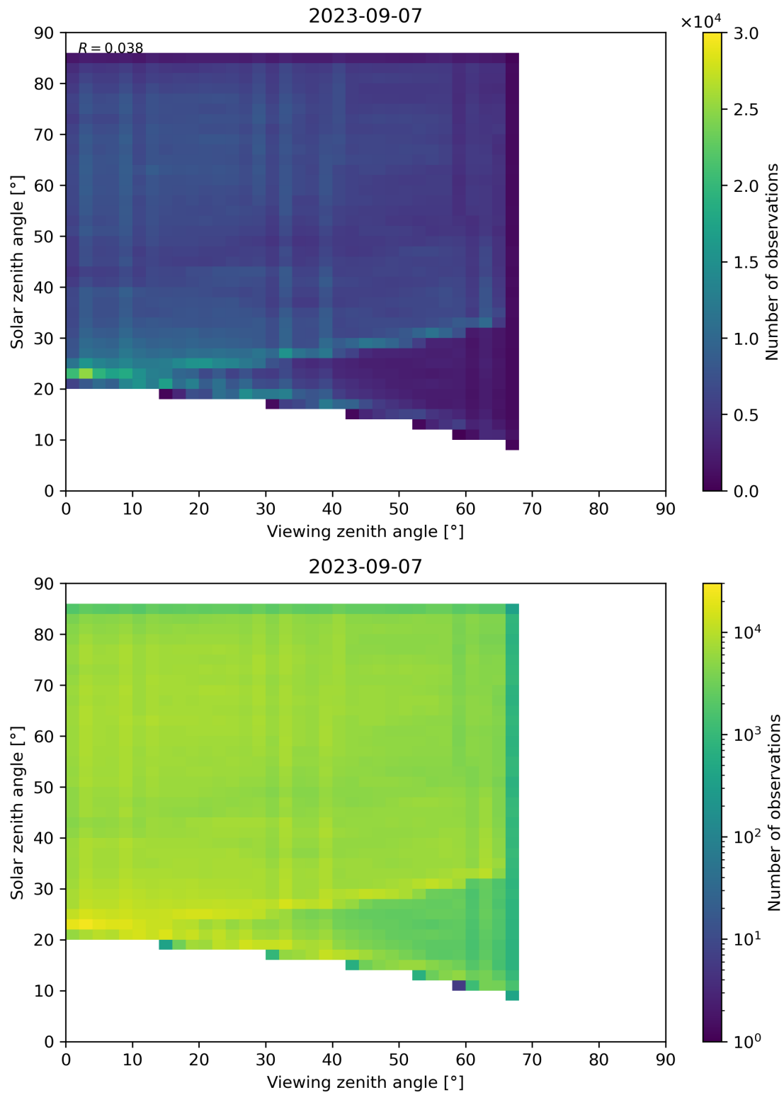
Figure 77: Scatter density plot of “Viewing zenith angle” against “Solar zenith angle” for 2023-09-06 to 2023-09-08.
