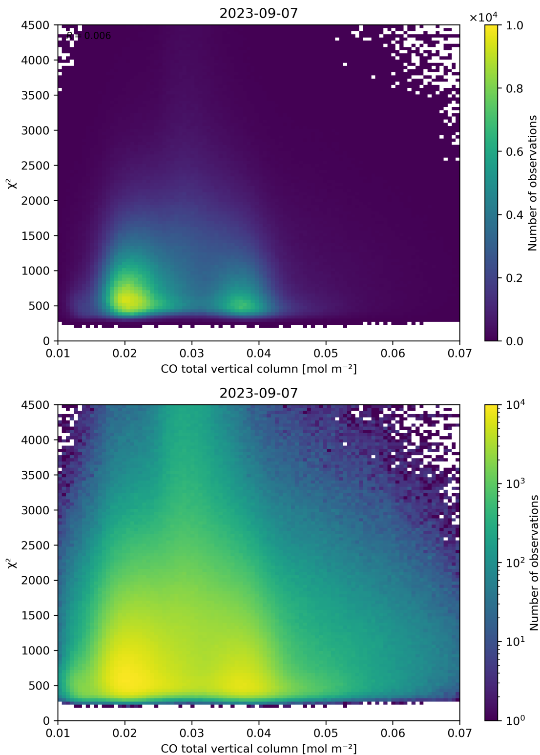
Figure 35: Scatter density plot of “CO total vertical column” against “ \chi^2 ” for 2023-09-06 to 2023-09-08.
