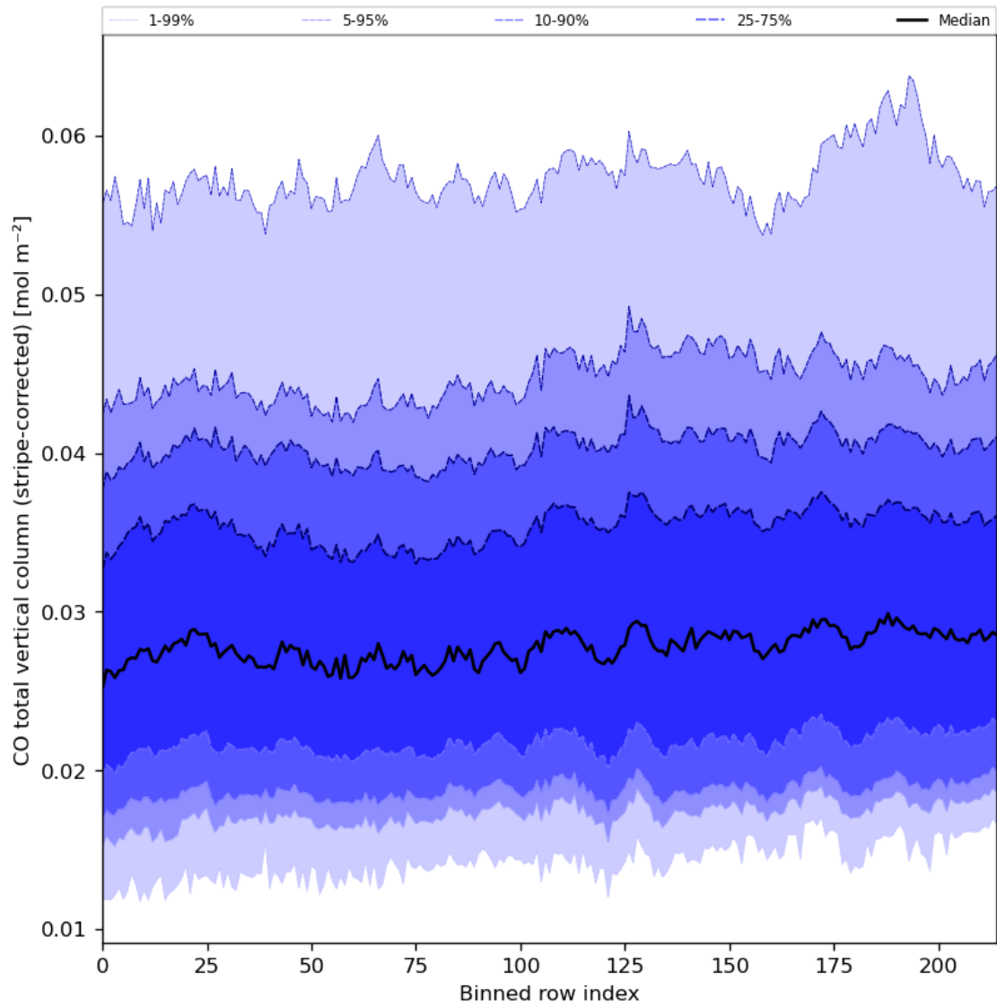
Figure 27: Along track statistics of “CO total vertical column (stripe-corrected)” for 2023-09-06 to 2023-09-08
