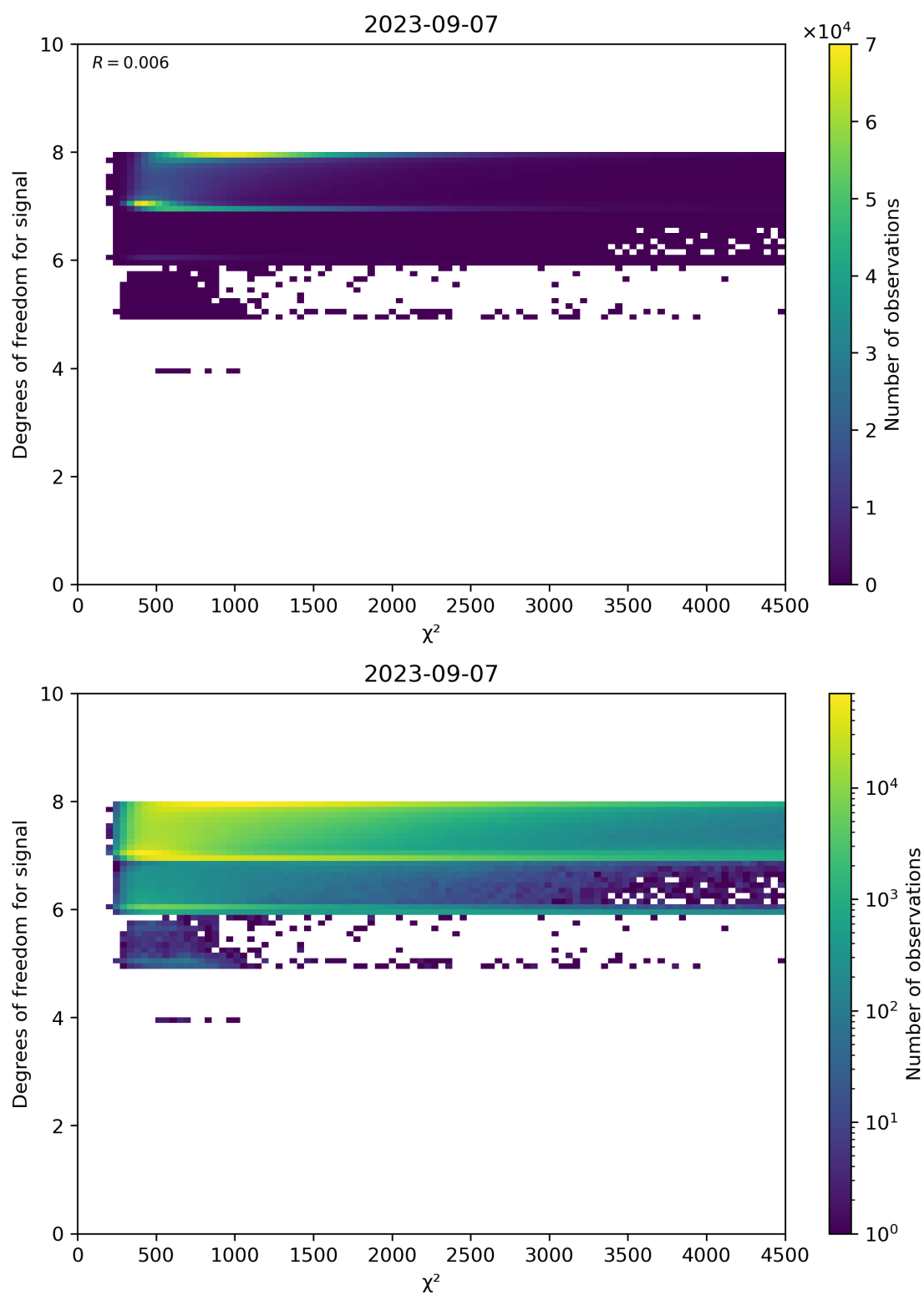
Figure 48: Scatter density plot of “ \chi^2 ” against “Degrees of freedom for signal” for 2023-09-06 to 2023-09-08.
