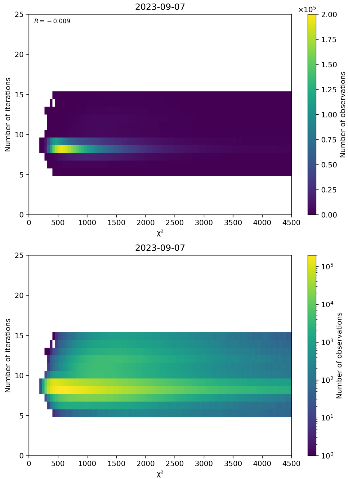
Figure 49: Scatter density plot of “ \chi^2 ” against “Number of iterations” for 2023-09-06 to 2023-09-08.
