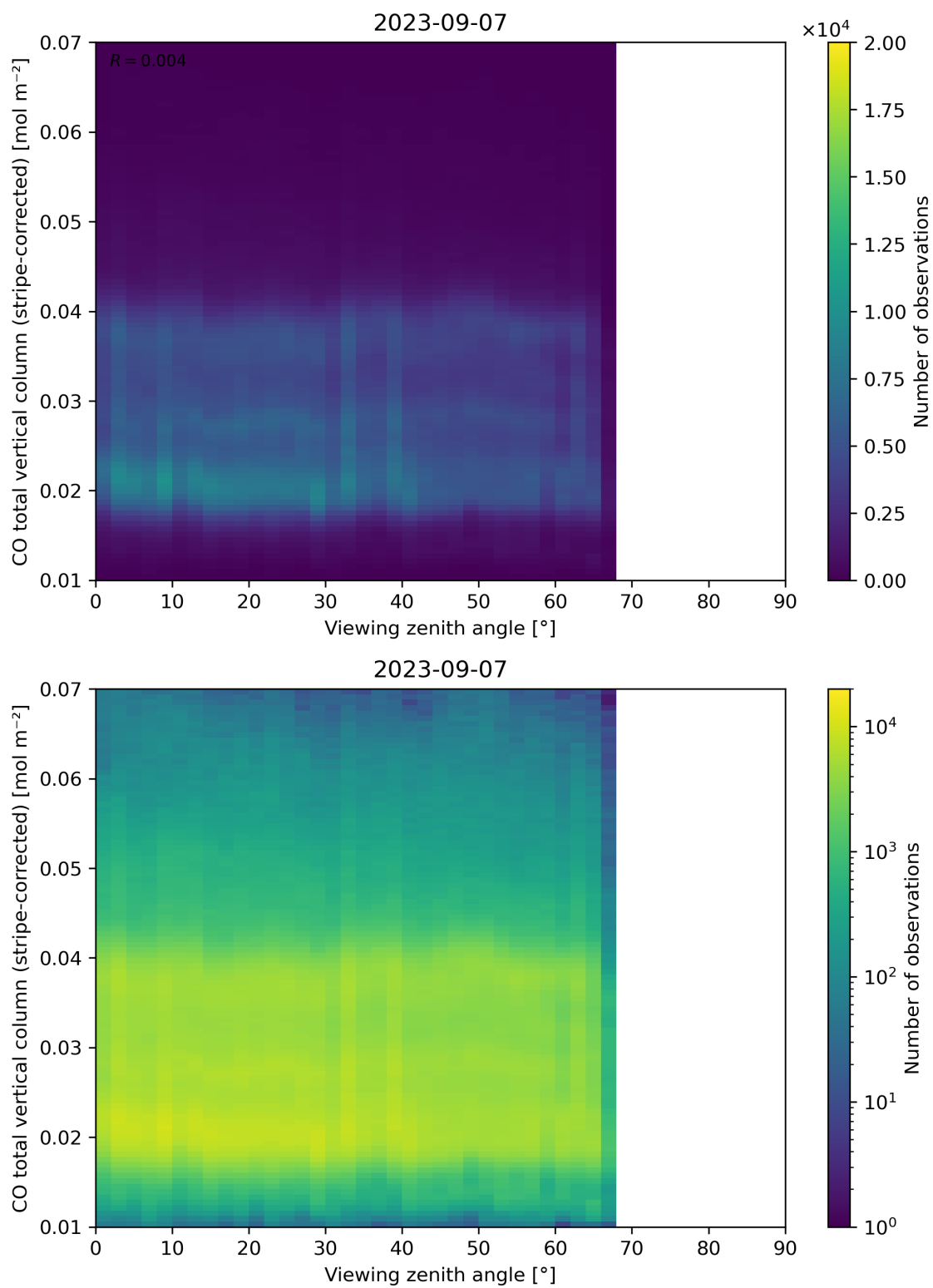
Figure 70: Scatter density plot of “Viewing zenith angle” against “CO total vertical column (stripe-corrected)” for 2023-09-06 to 2023-09-08.
