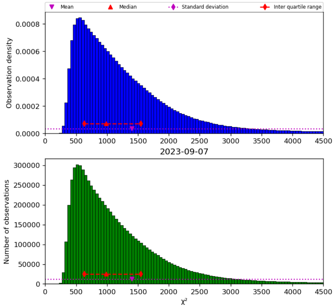
Figure 22: Histogram of “ \chi^2 ” for 2023-09-06 to 2023-09-08
