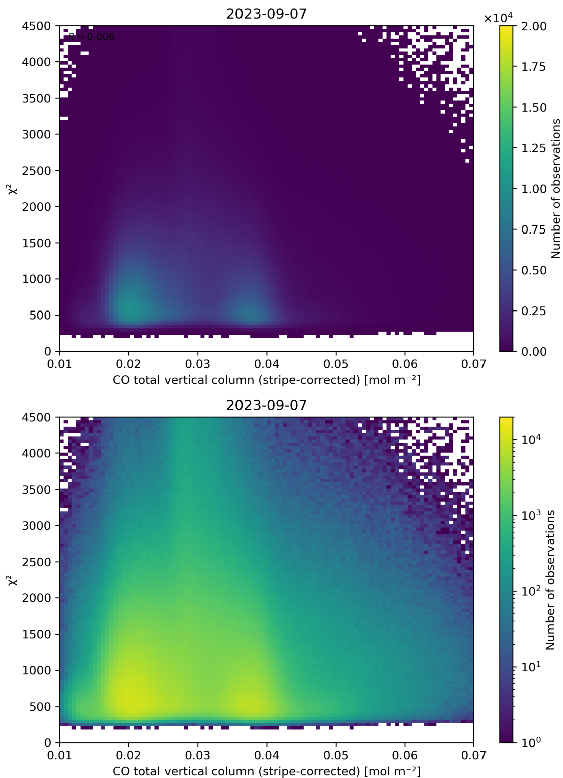
Figure 37: Scatter density plot of “CO total vertical column (stripe-corrected)” against “ \chi^2 ” for 2023-09-06 to 2023-09-08.
