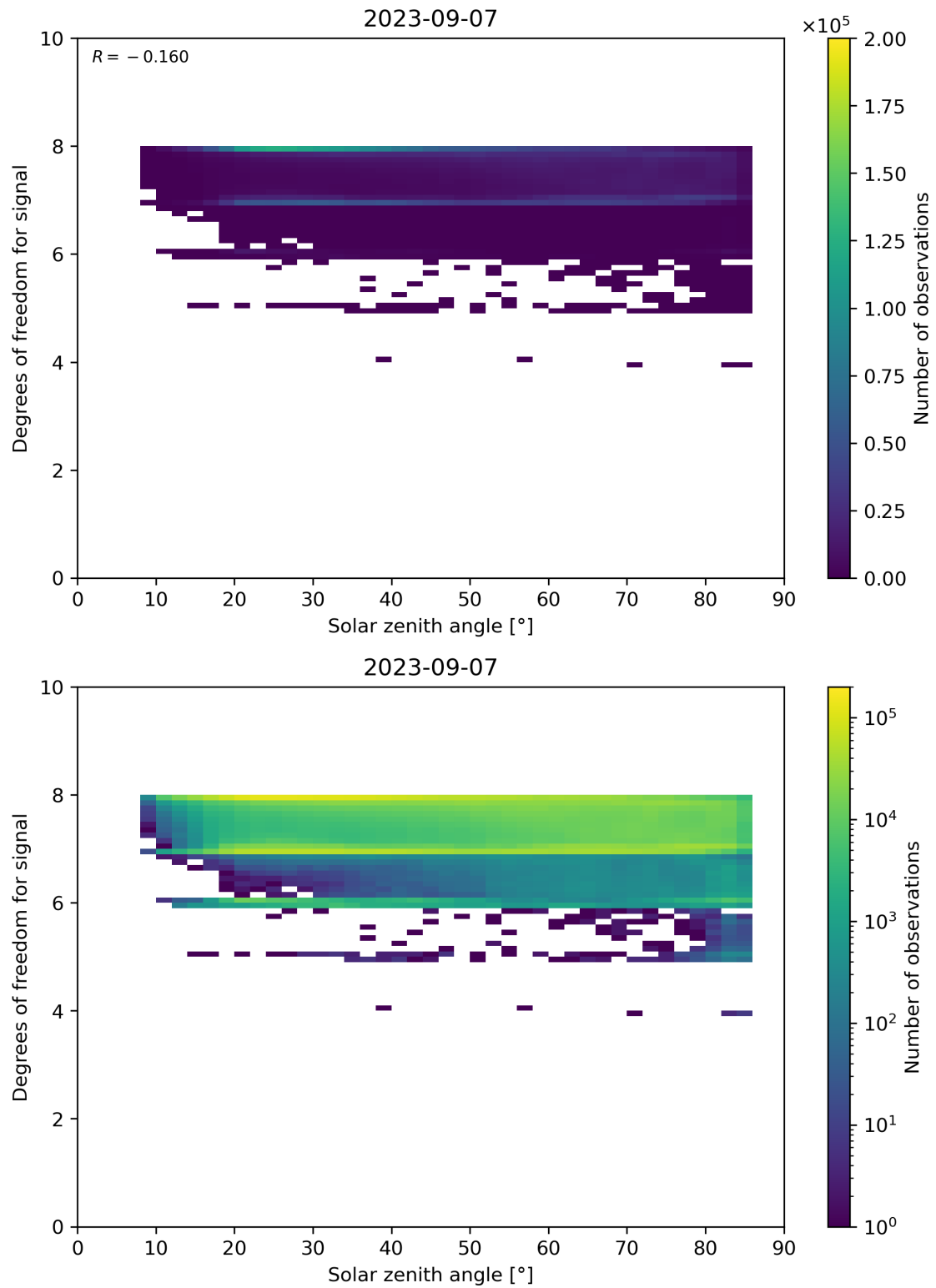
Figure 65: Scatter density plot of “Solar zenith angle” against “Degrees of freedom for signal” for 2023-09-06 to 2023-09-08.
