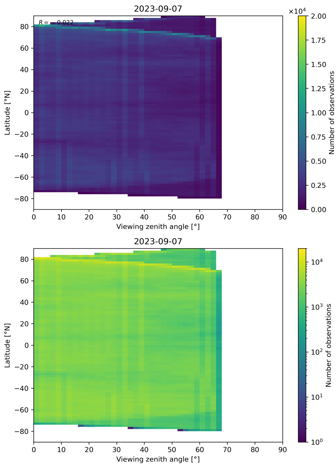
Figure 74: Scatter density plot of “Viewing zenith angle” against “Latitude” for 2023-09-06 to 2023-09-08.
