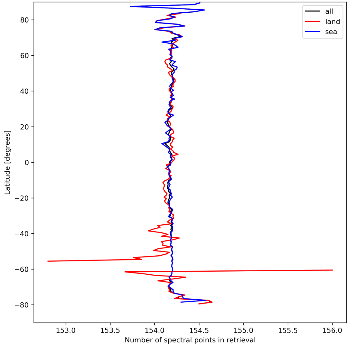
Figure 13: Zonal average of “Number of spectral points in retrieval” for 2023-09-06 to 2023-09-08.
