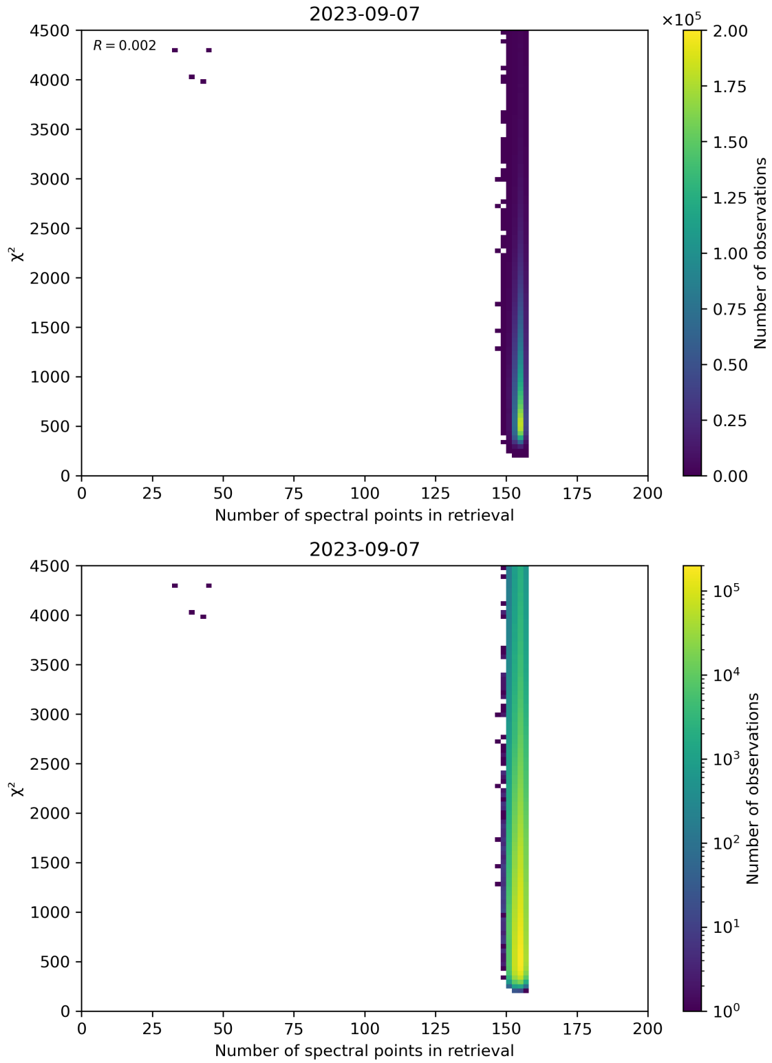
Figure 58: Scatter density plot of “Number of spectral points in retrieval” against “ \chi^2 ” for 2023-09-06 to 2023-09-08.
