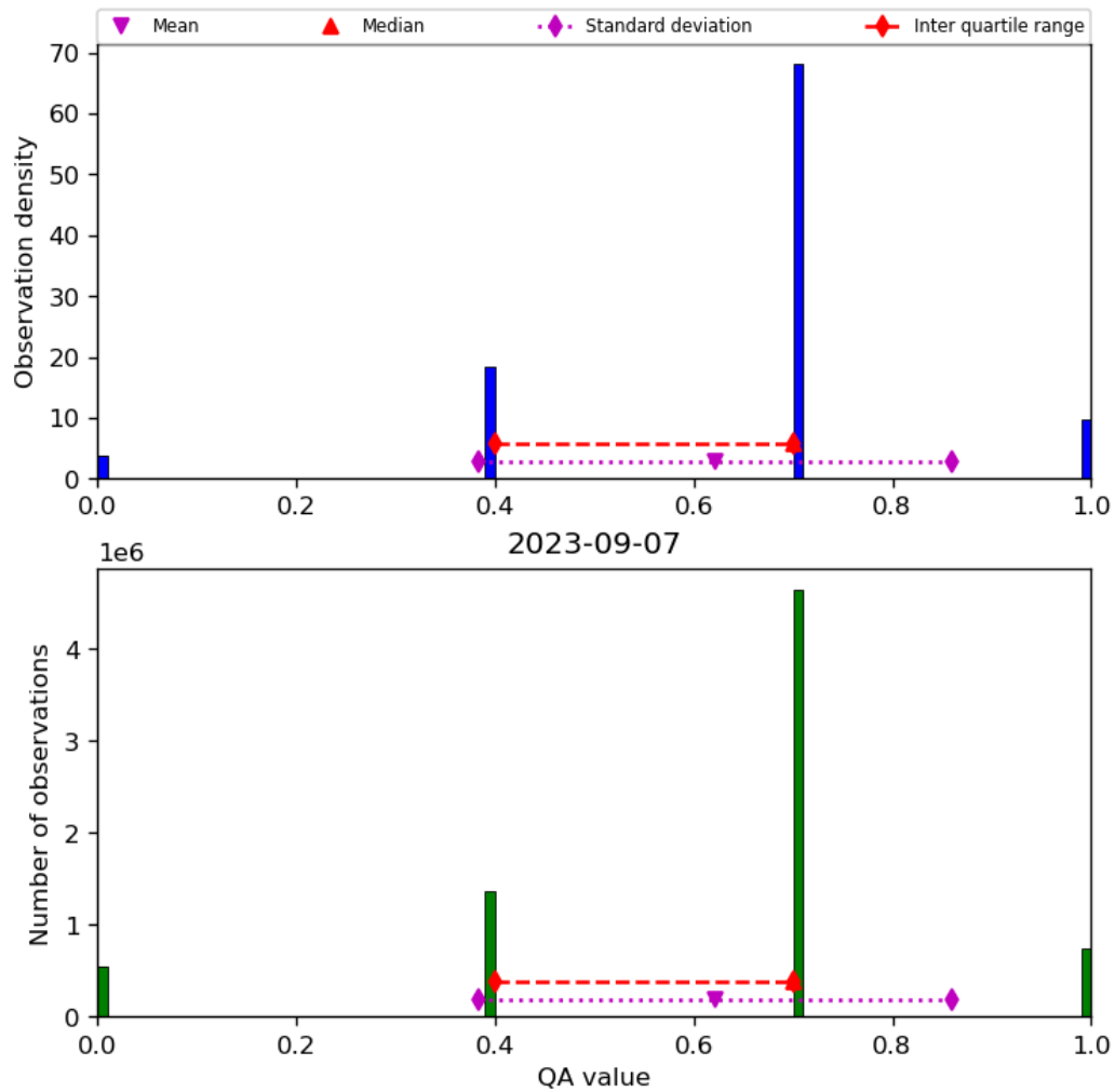
Figure 17: Histogram of “QA value” for 2023-09-06 to 2023-09-08
