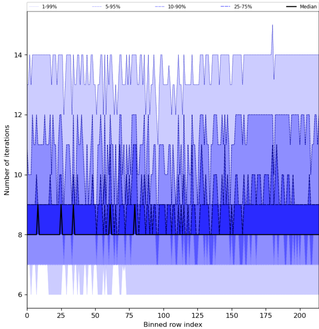
Figure 32: Along track statistics of “Number of iterations” for 2023-09-06 to 2023-09-08
