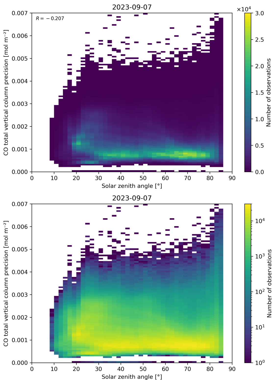
Figure 63: Scatter density plot of “Solar zenith angle” against “CO total vertical column precision” for 2023-09-06 to 2023-09-08.
