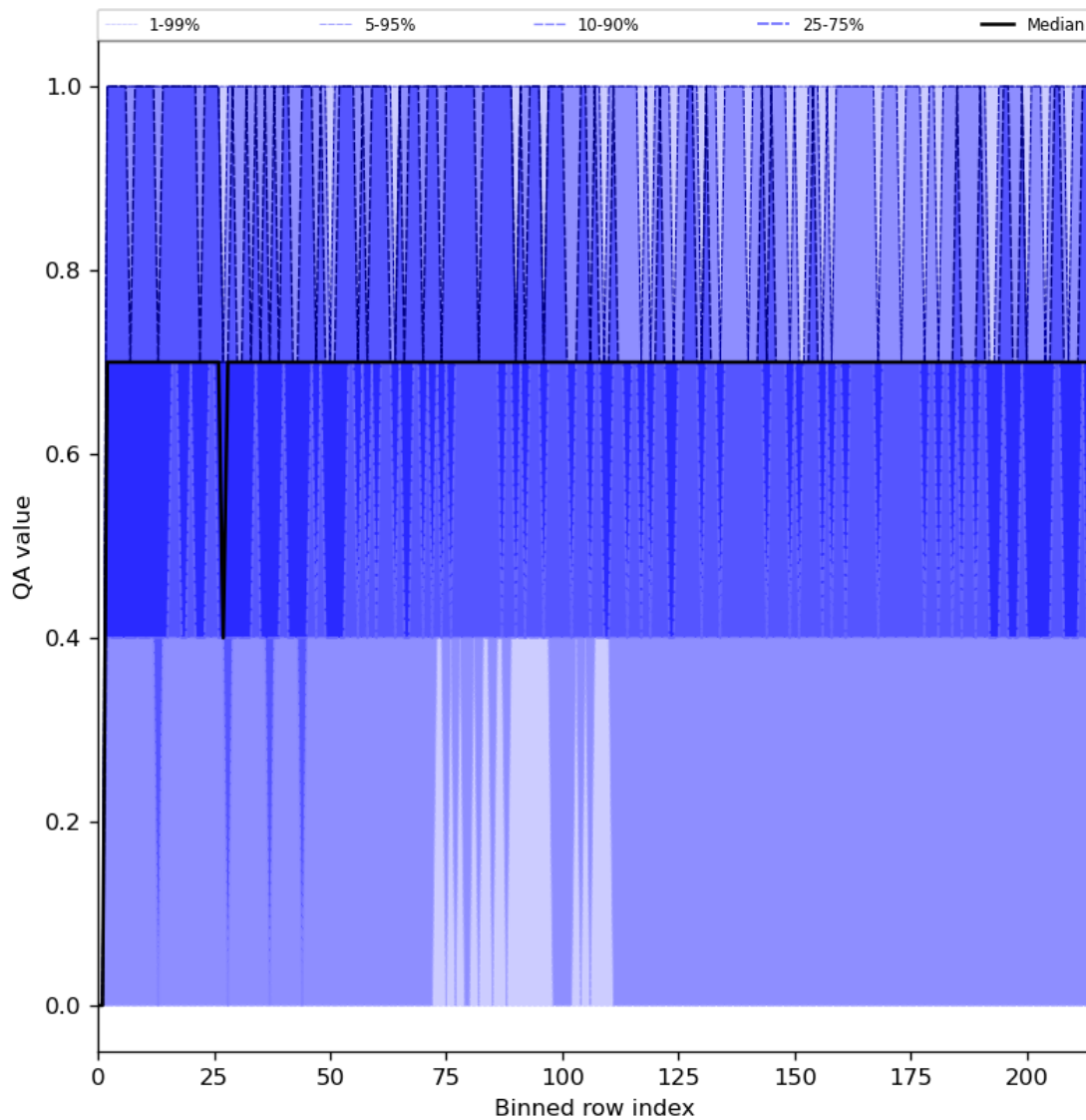
Figure 25: Along track statistics of “QA value” for 2023-09-06 to 2023-09-08
