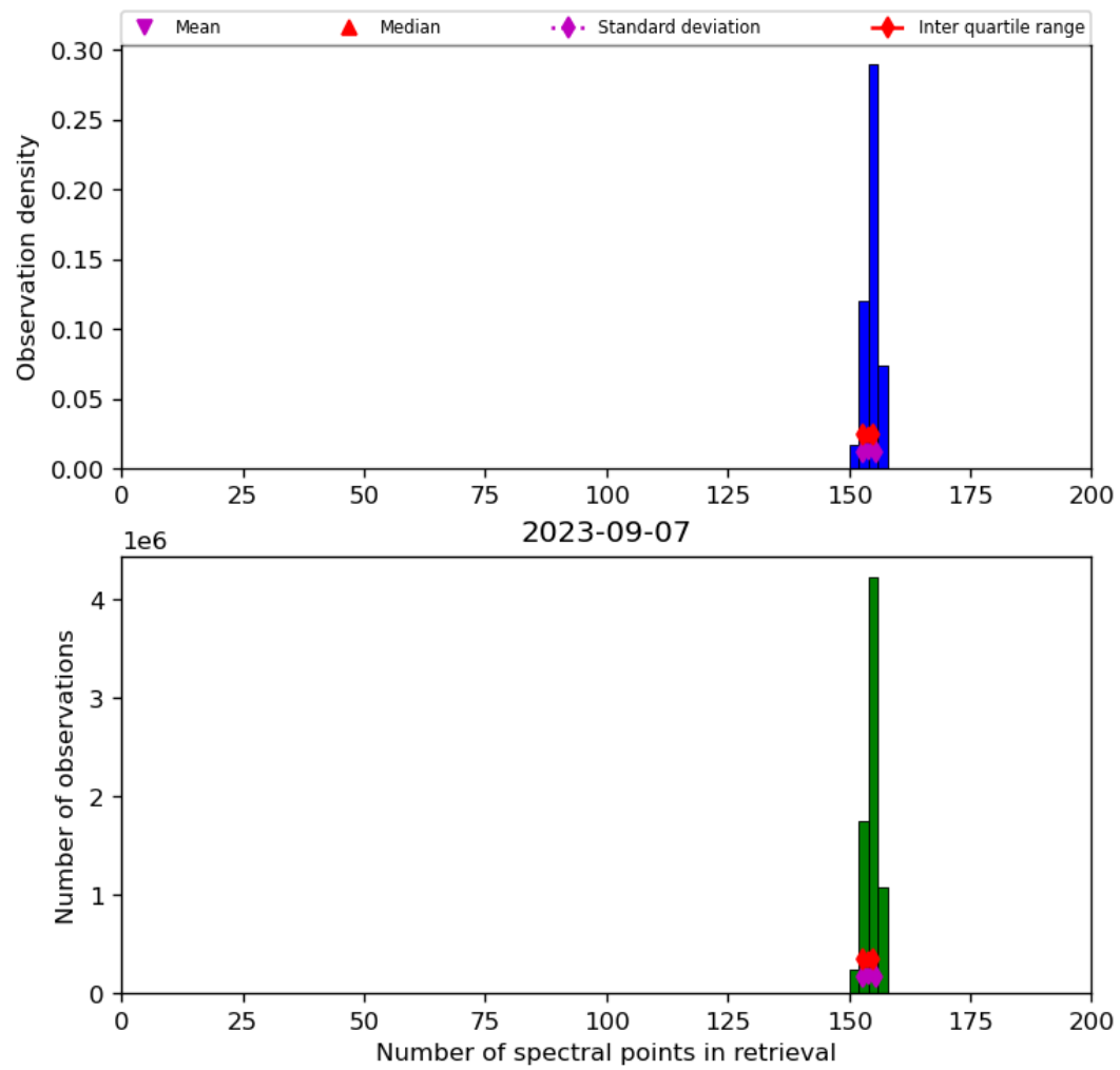
Figure 21: Histogram of “Number of spectral points in retrieval” for 2023-09-06 to 2023-09-08
