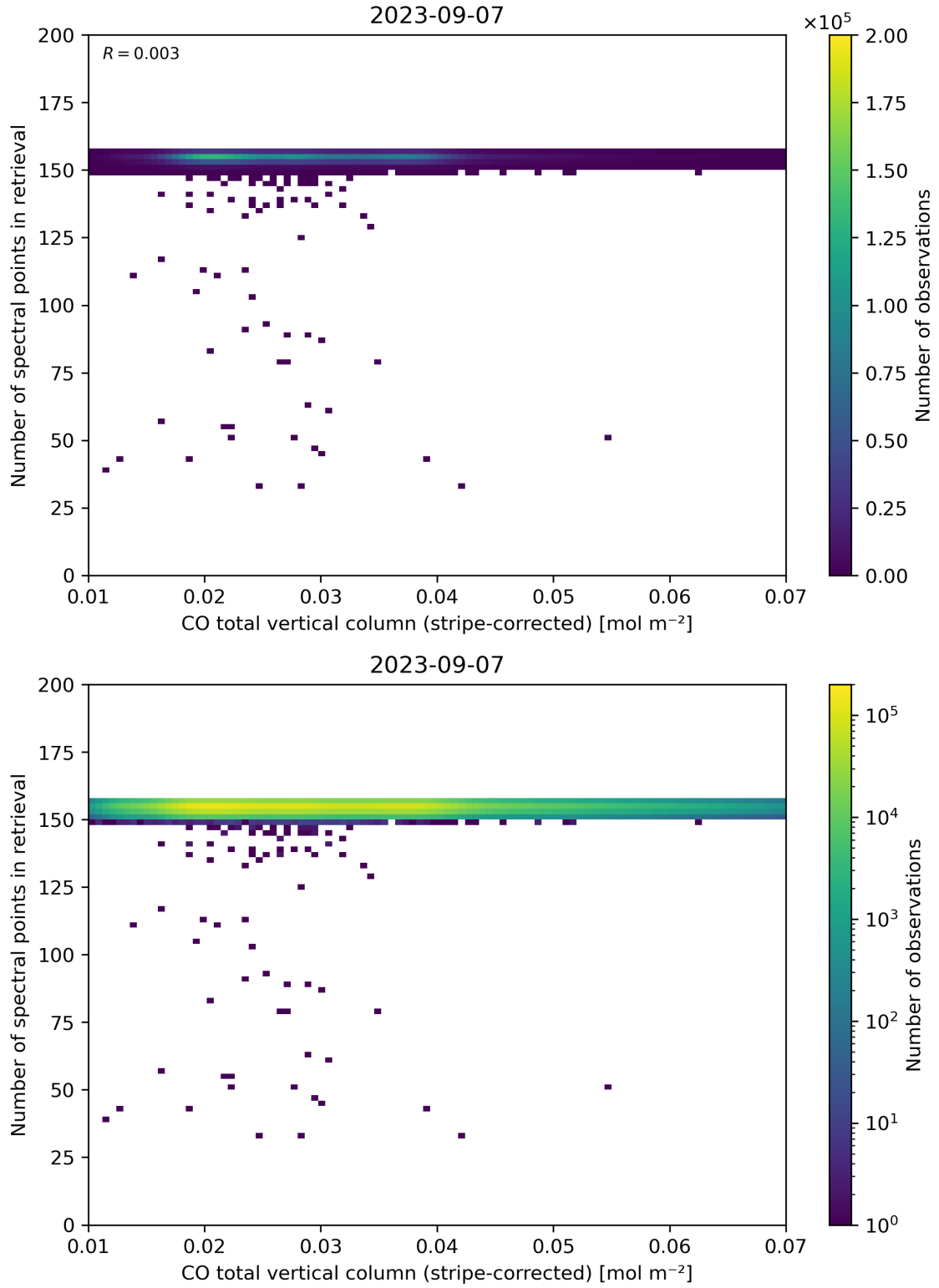
Figure 40: Scatter density plot of “CO total vertical column (stripe-corrected)” against “Number of spectral points in retrieval” for 2023-09-06 to 2023-09-08.
