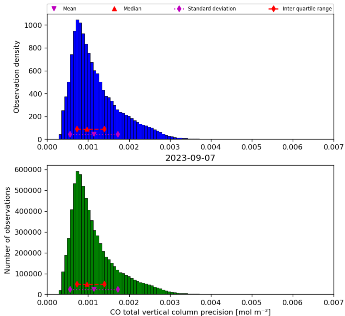
Figure 20: Histogram of “CO total vertical column precision” for 2023-09-06 to 2023-09-08
