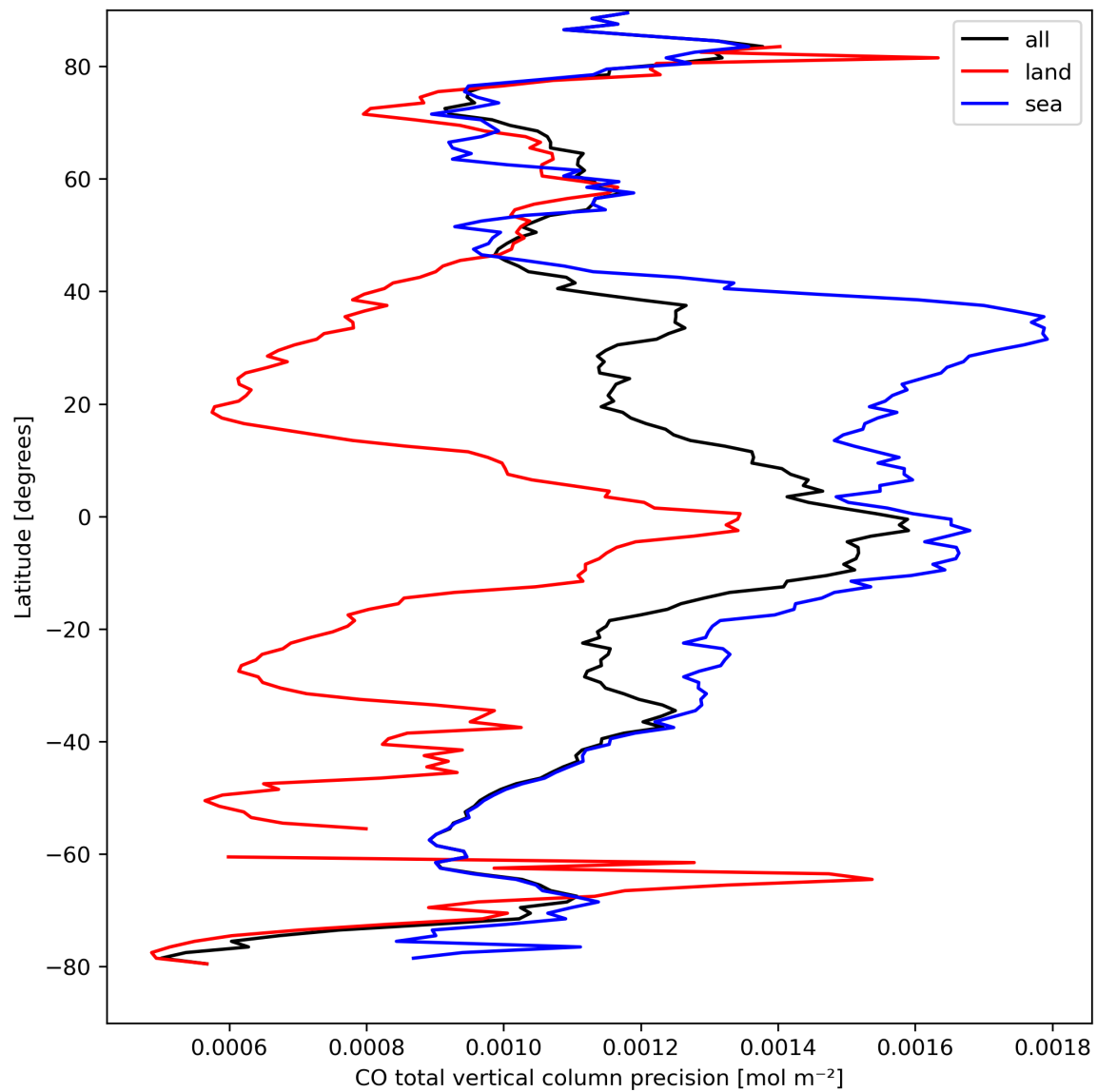
Figure 12: Zonal average of “CO total vertical column precision” for 2023-09-06 to 2023-09-08.
