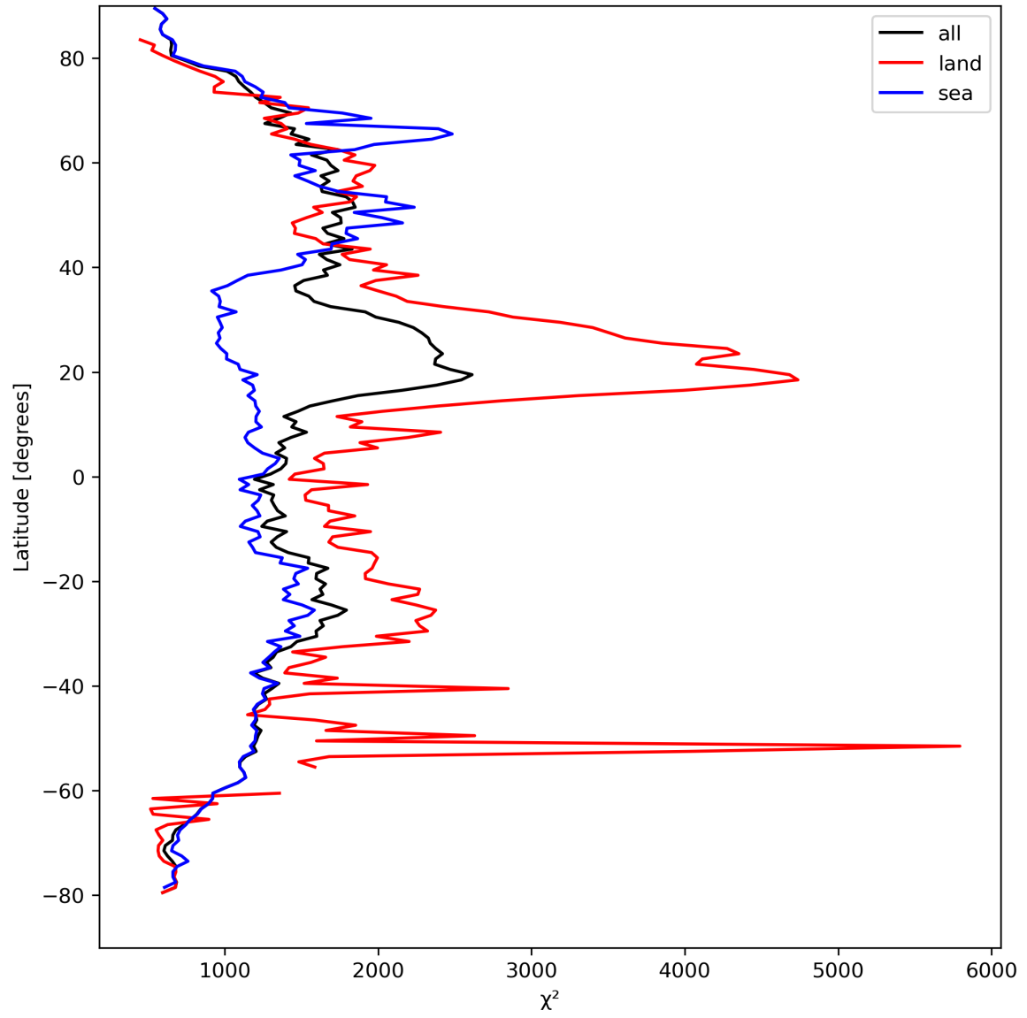
Figure 14: Zonal average of “ \chi^2 ” for 2023-09-06 to 2023-09-08.
