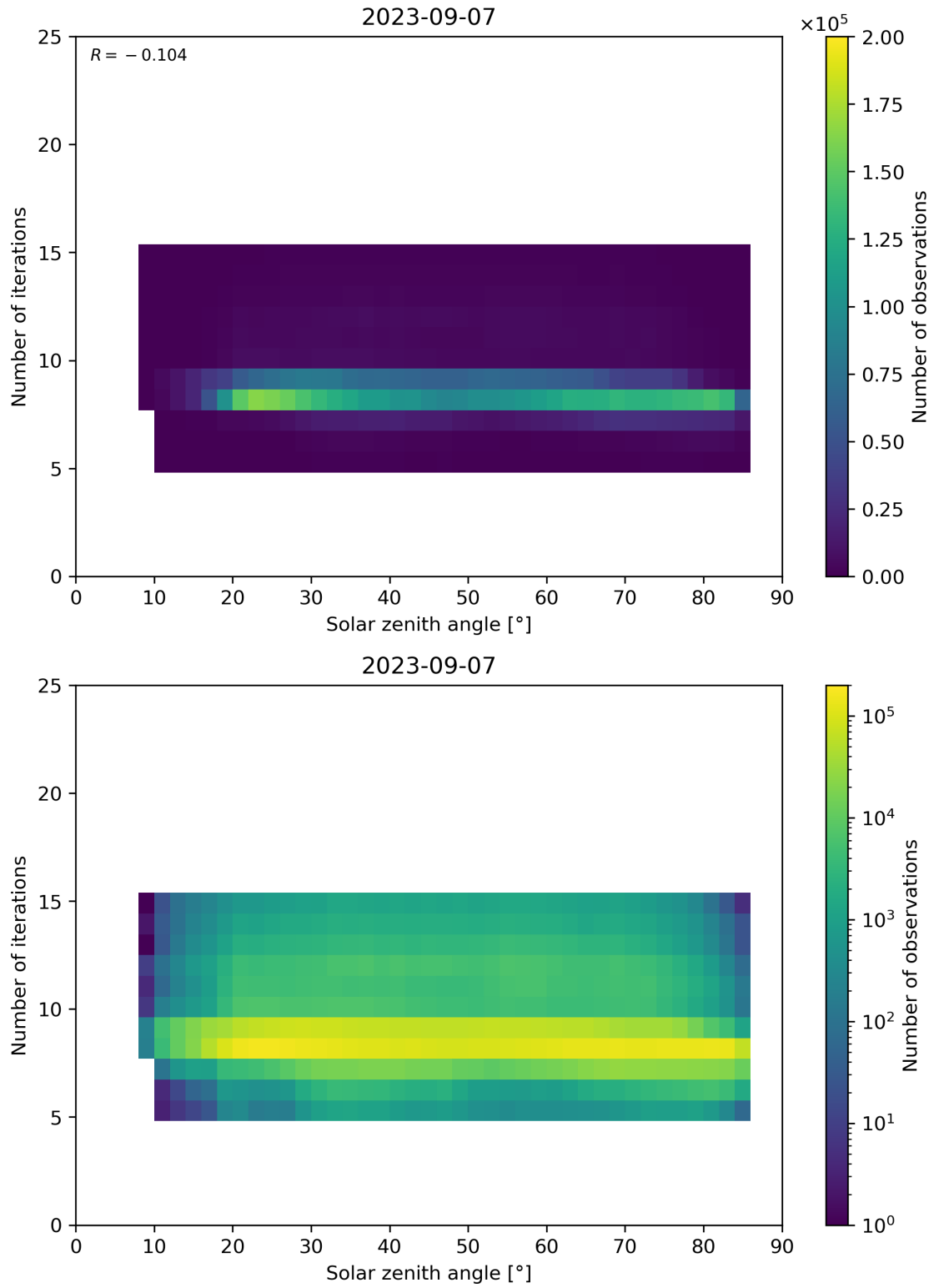
Figure 67: Scatter density plot of “Solar zenith angle” against “Number of iterations” for 2023-09-06 to 2023-09-08.
