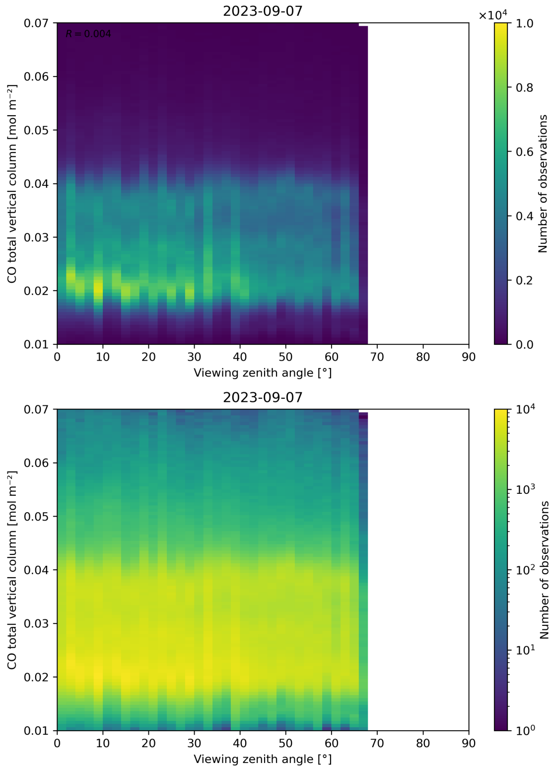
Figure 69: Scatter density plot of “Viewing zenith angle” against “CO total vertical column” for 2023-09-06 to 2023-09-08.
