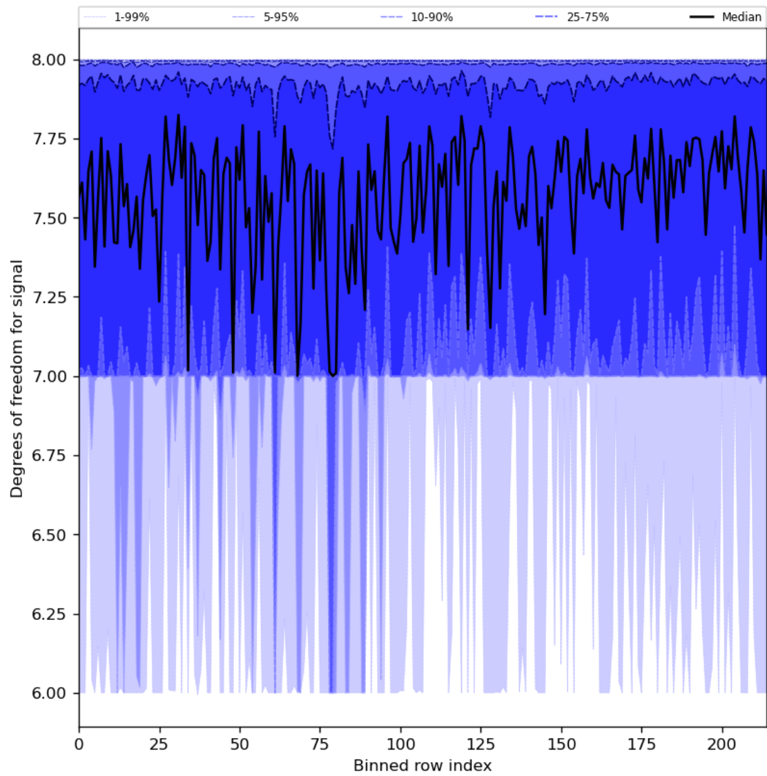
Figure 31: Along track statistics of “Degrees of freedom for signal” for 2023-09-06 to 2023-09-08
