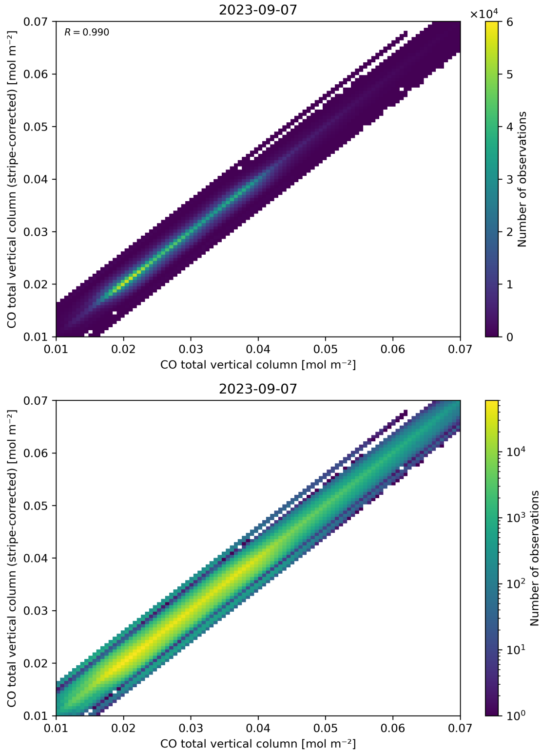
Figure 33: Scatter density plot of “CO total vertical column” against “CO total vertical column (stripe-corrected)” for 2023-09-06 to 2023-09-08.
