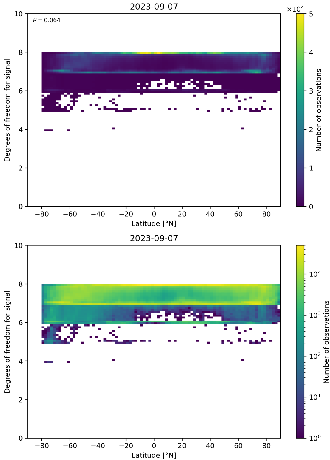
Figure 55: Scatter density plot of “Latitude” against “Degrees of freedom for signal” for 2023-09-06 to 2023-09-08.
