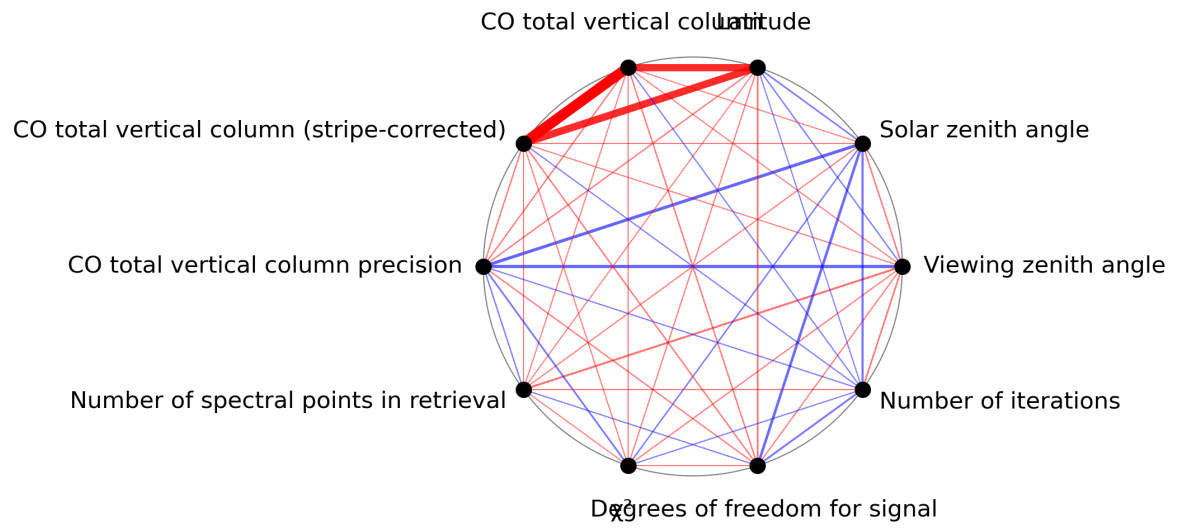
Figure 1: Map of correlation graph for 2023-09-06 to 2023-09-08.
