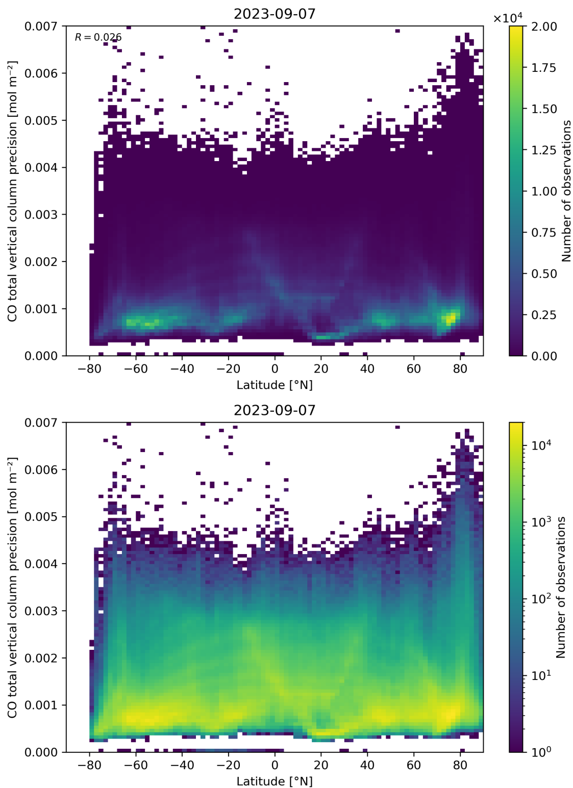
Figure 53: Scatter density plot of “Latitude” against “CO total vertical column precision” for 2023-09-06 to 2023-09-08.
