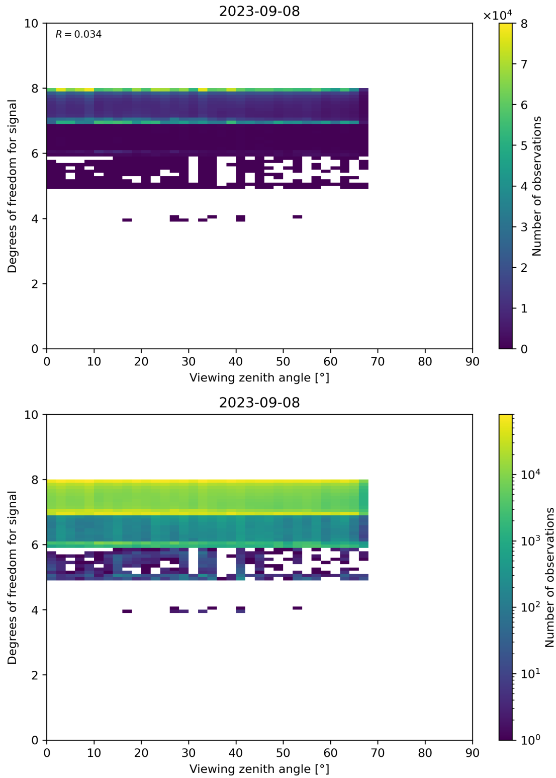
Figure 73: Scatter density plot of “Viewing zenith angle” against “Degrees of freedom for signal” for 2023-09-07 to 2023-09-09.
