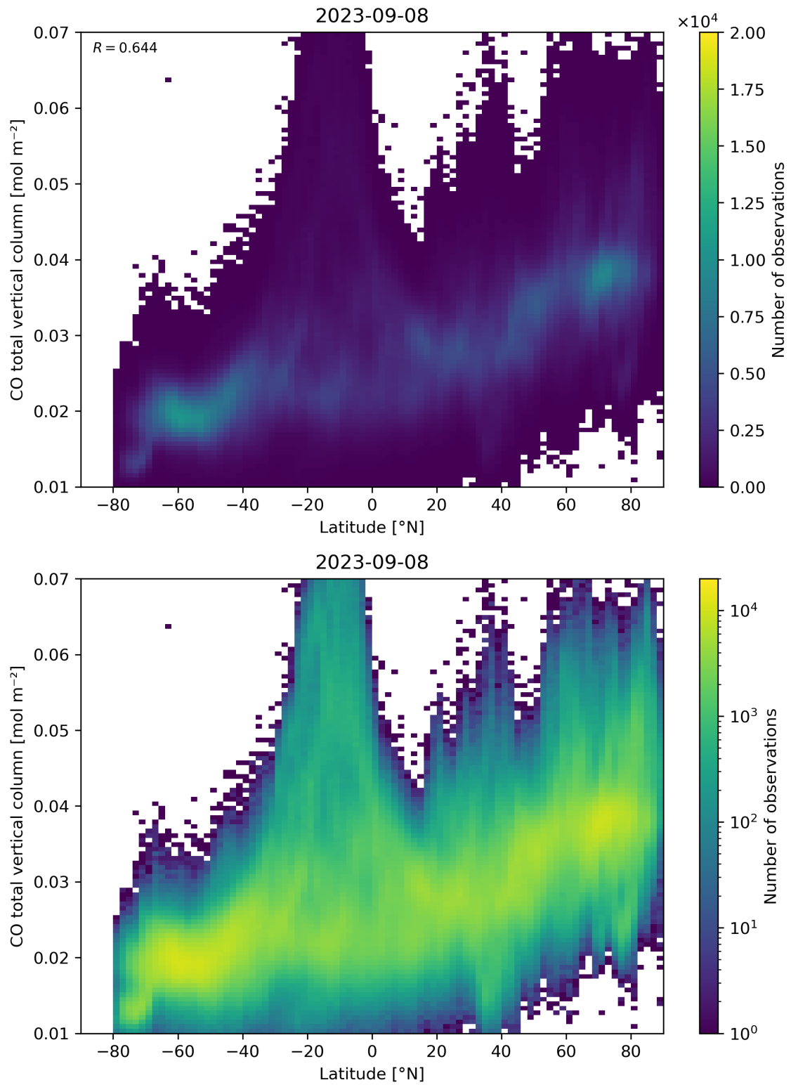
Figure 51: Scatter density plot of “Latitude” against “CO total vertical column” for 2023-09-07 to 2023-09-09.
