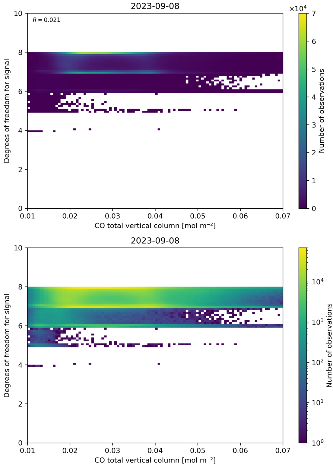
Figure 41: Scatter density plot of “CO total vertical column” against “Degrees of freedom for signal” for 2023-09-07 to 2023-09-09.
