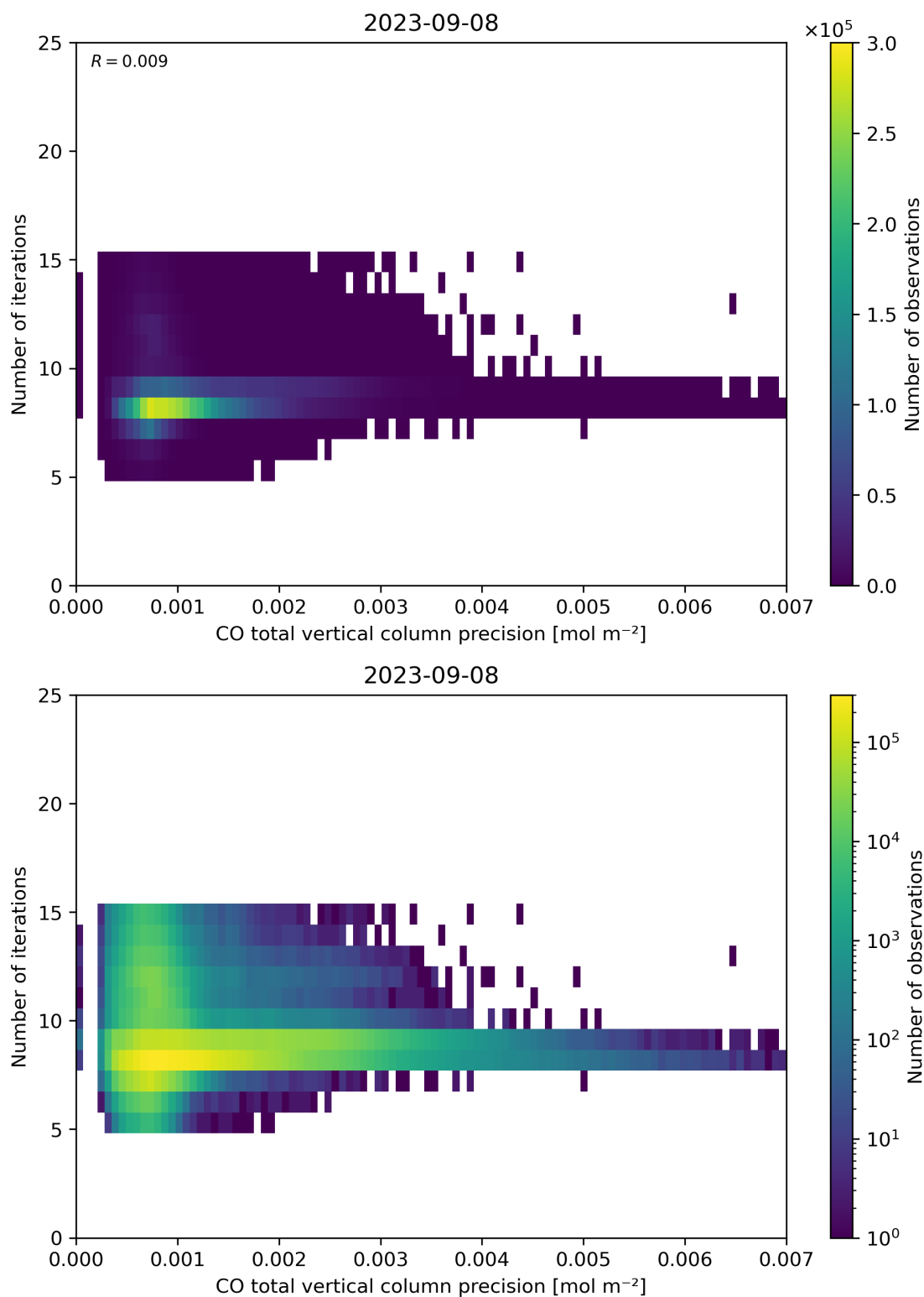
Figure 46: Scatter density plot of “CO total vertical column precision” against “Number of iterations” for 2023-09-07 to 2023-09-09.
