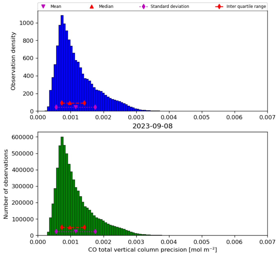
Figure 20: Histogram of “CO total vertical column precision” for 2023-09-07 to 2023-09-09
