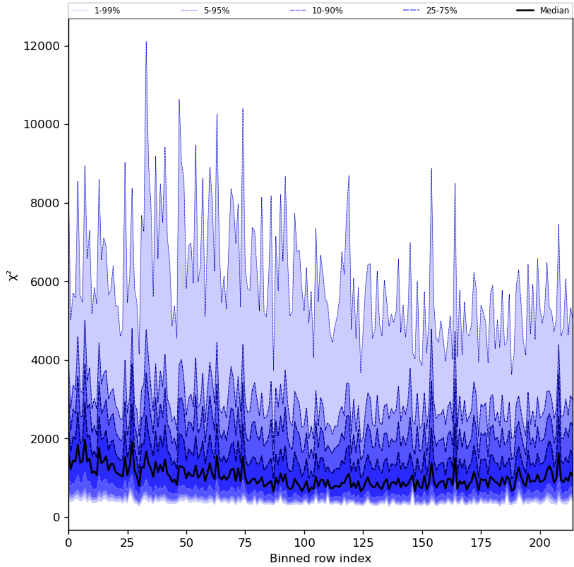
Figure 30: Along track statistics of “ \chi^2 ” for 2023-09-07 to 2023-09-09
