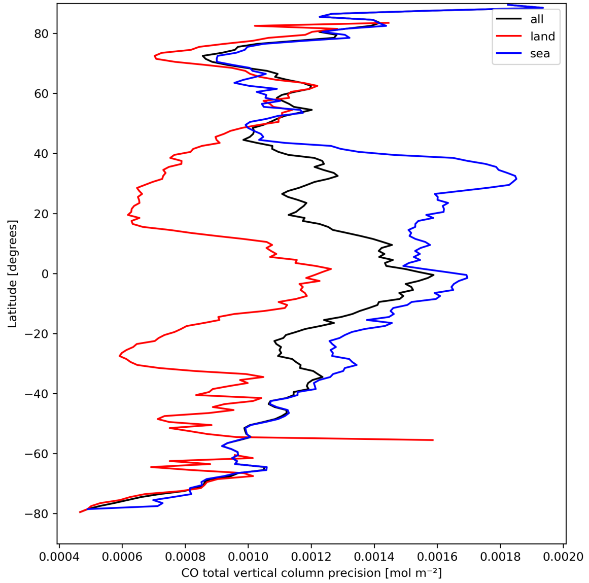
Figure 12: Zonal average of "CO total vertical column precision" for 2023-09-07 to 2023-09-09.
