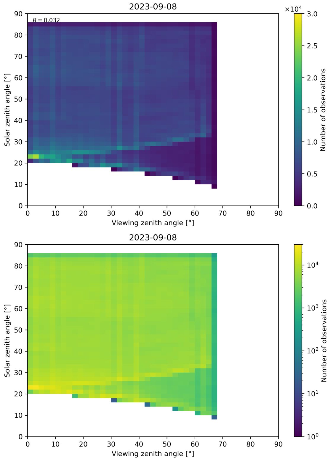
Figure 77: Scatter density plot of “Viewing zenith angle” against “Solar zenith angle” for 2023-09-07 to 2023-09-09.
