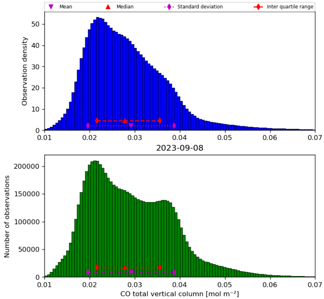
Figure 18: Histogram of “CO total vertical column” for 2023-09-07 to 2023-09-09
