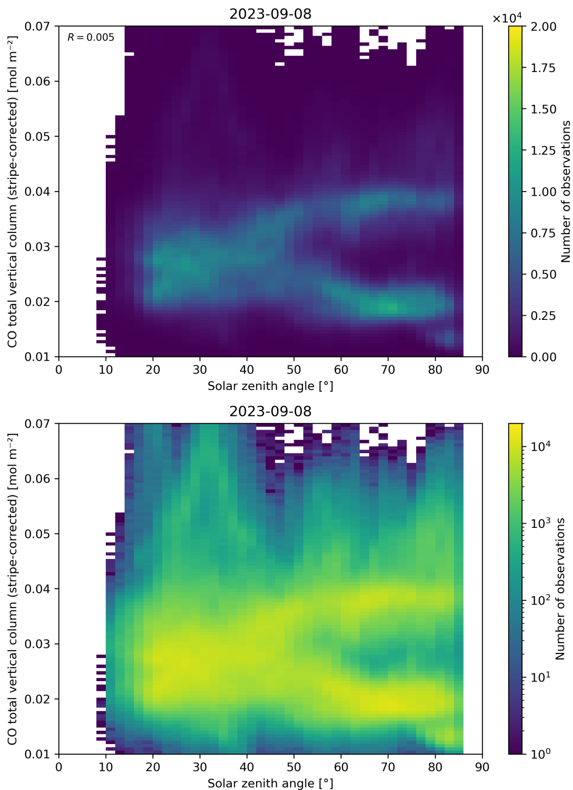
Figure 62: Scatter density plot of “Solar zenith angle” against “CO total vertical column (stripe-corrected)” for 2023-09-07 to 2023-09-09.
