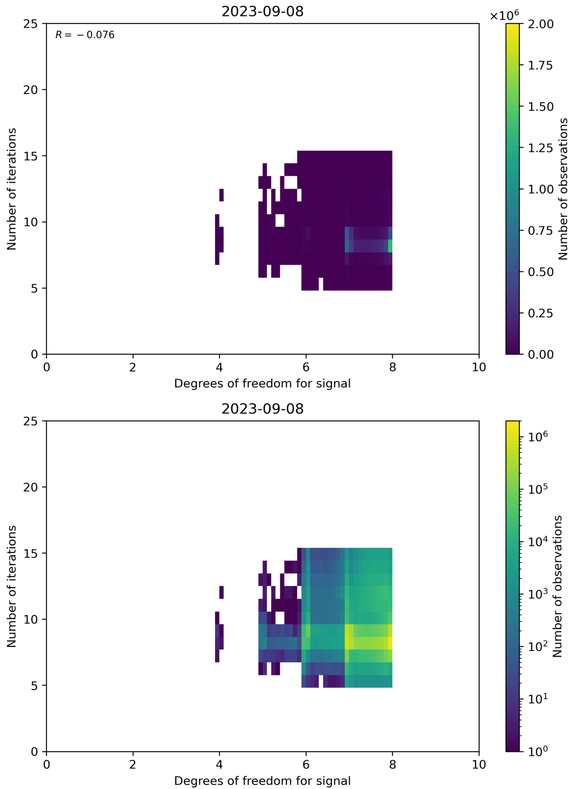
Figure 50: Scatter density plot of “Degrees of freedom for signal” against “Number of iterations” for 2023-09-07 to 2023-09-09.
