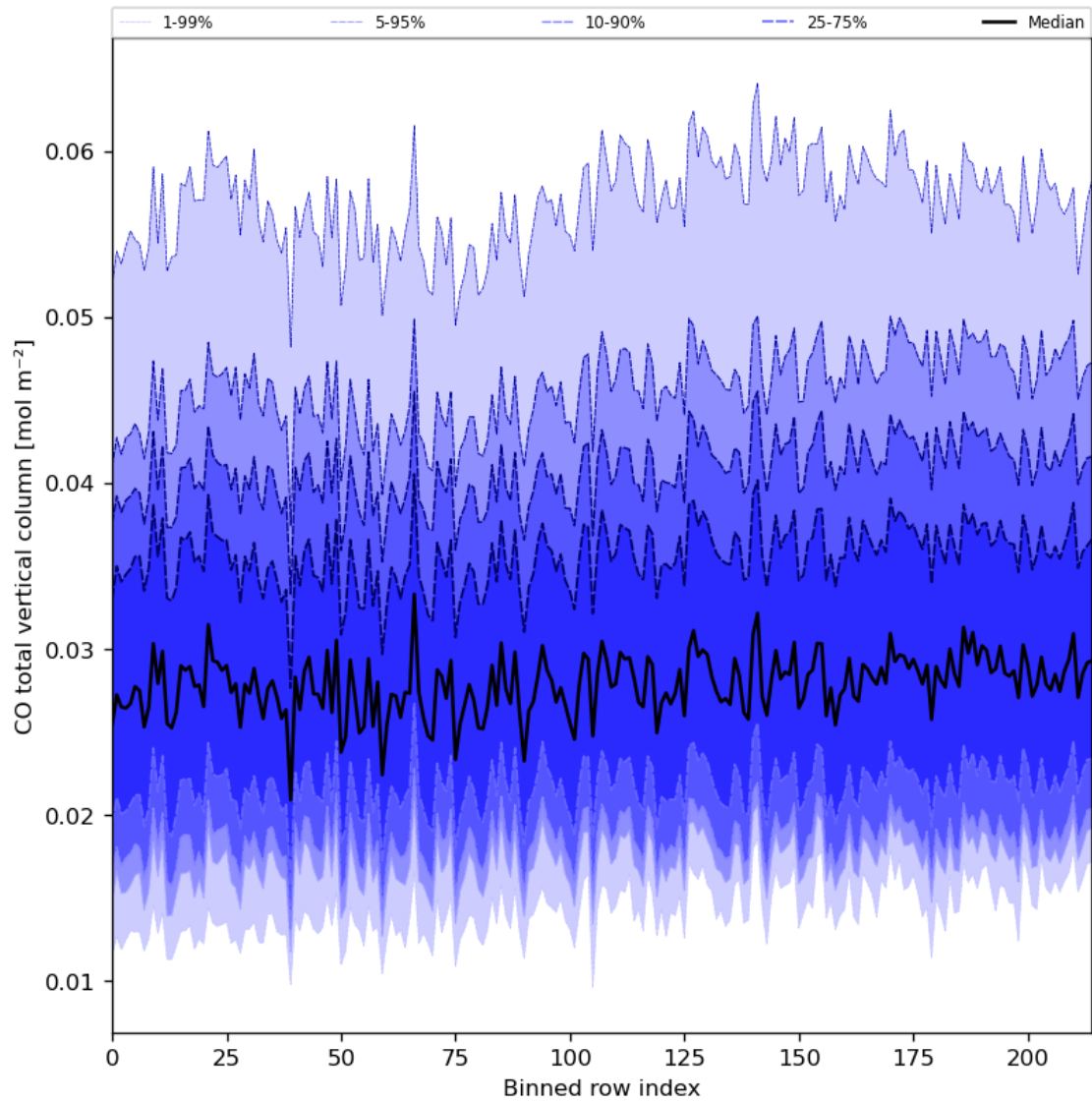
Figure 26: Along track statistics of “CO total vertical column” for 2023-09-07 to 2023-09-09
