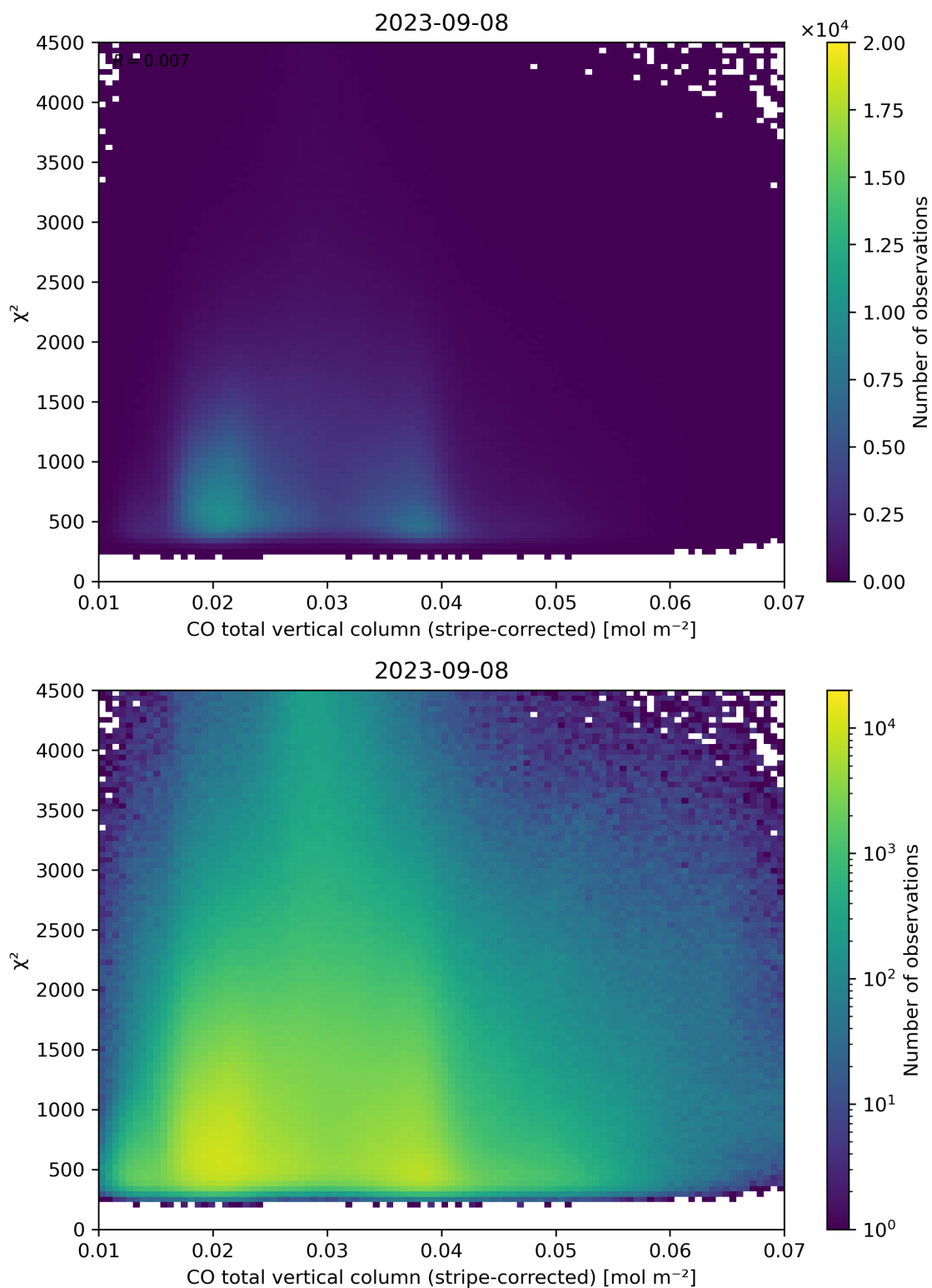
Figure 37: Scatter density plot of “CO total vertical column (stripe-corrected)” against “ \chi^2 ” for 2023-09-07 to 2023-09-09.
