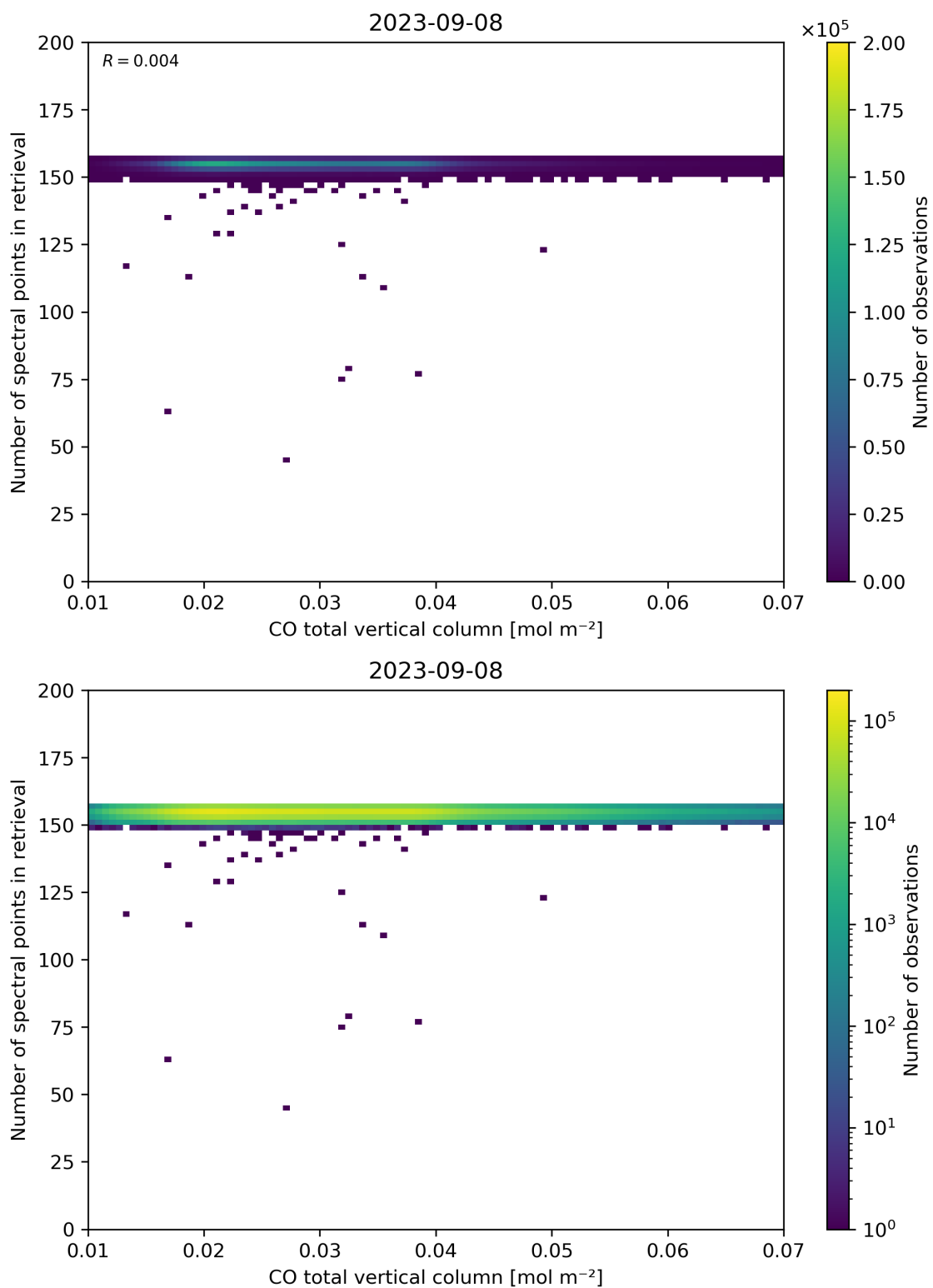
Figure 43: Scatter density plot of “CO total vertical column” against “Number of spectral points in retrieval” for 2023-09-07 to 2023-09-09.
