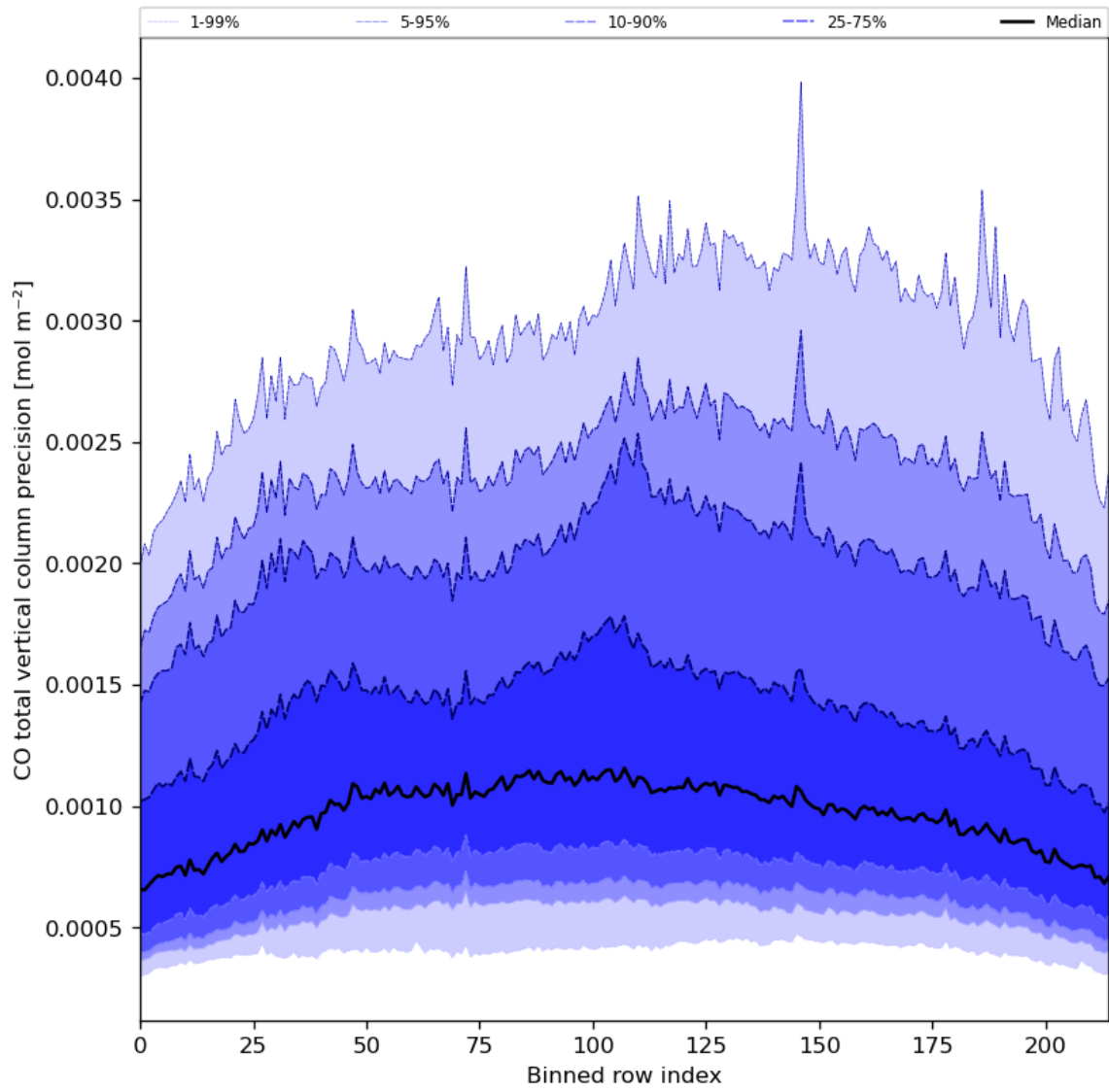
Figure 28: Along track statistics of “CO total vertical column precision” for 2023-09-07 to 2023-09-09
