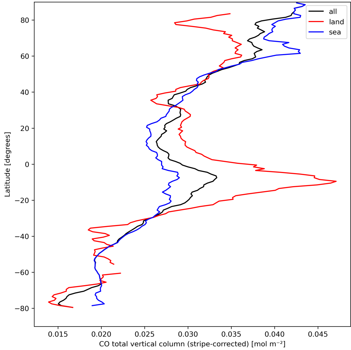
Figure 11: Zonal average of “CO total vertical column (stripe-corrected)” for 2023-09-07 to 2023-09-09.
