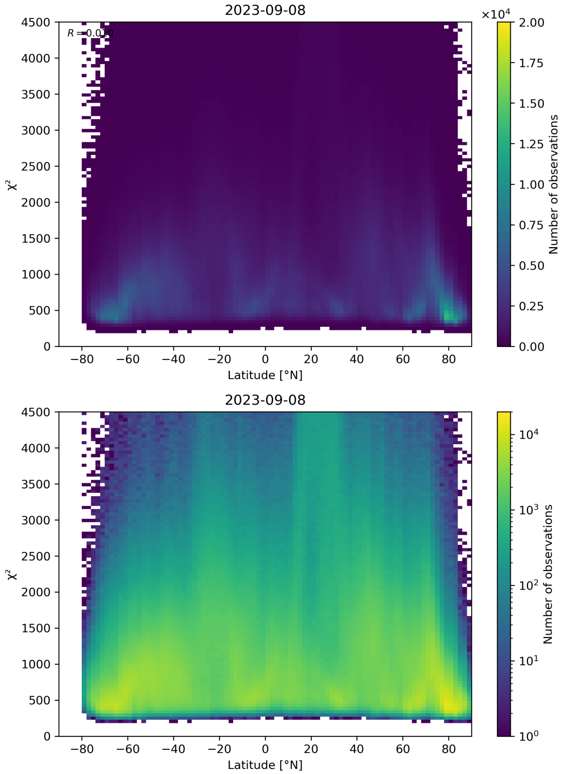
Figure 54: Scatter density plot of “Latitude” against “ \chi^2 ” for 2023-09-07 to 2023-09-09.
