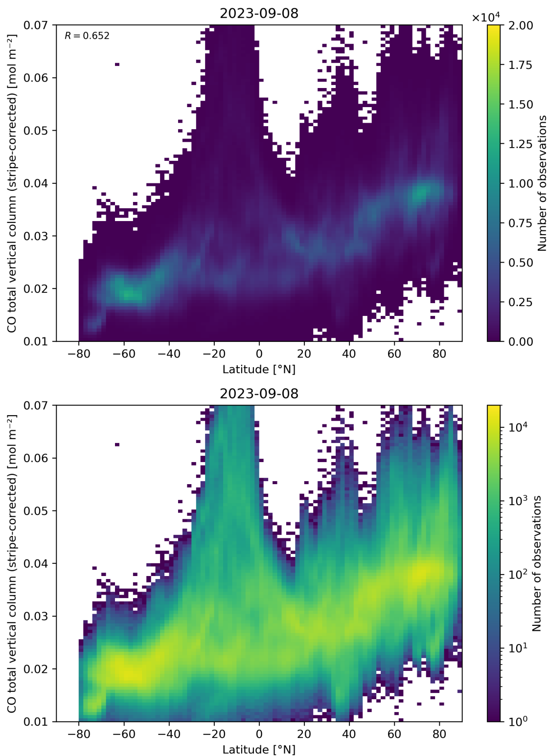
Figure 52: Scatter density plot of “Latitude” against “CO total vertical column (stripe-corrected)” for 2023-09-07 to 2023-09-09.
