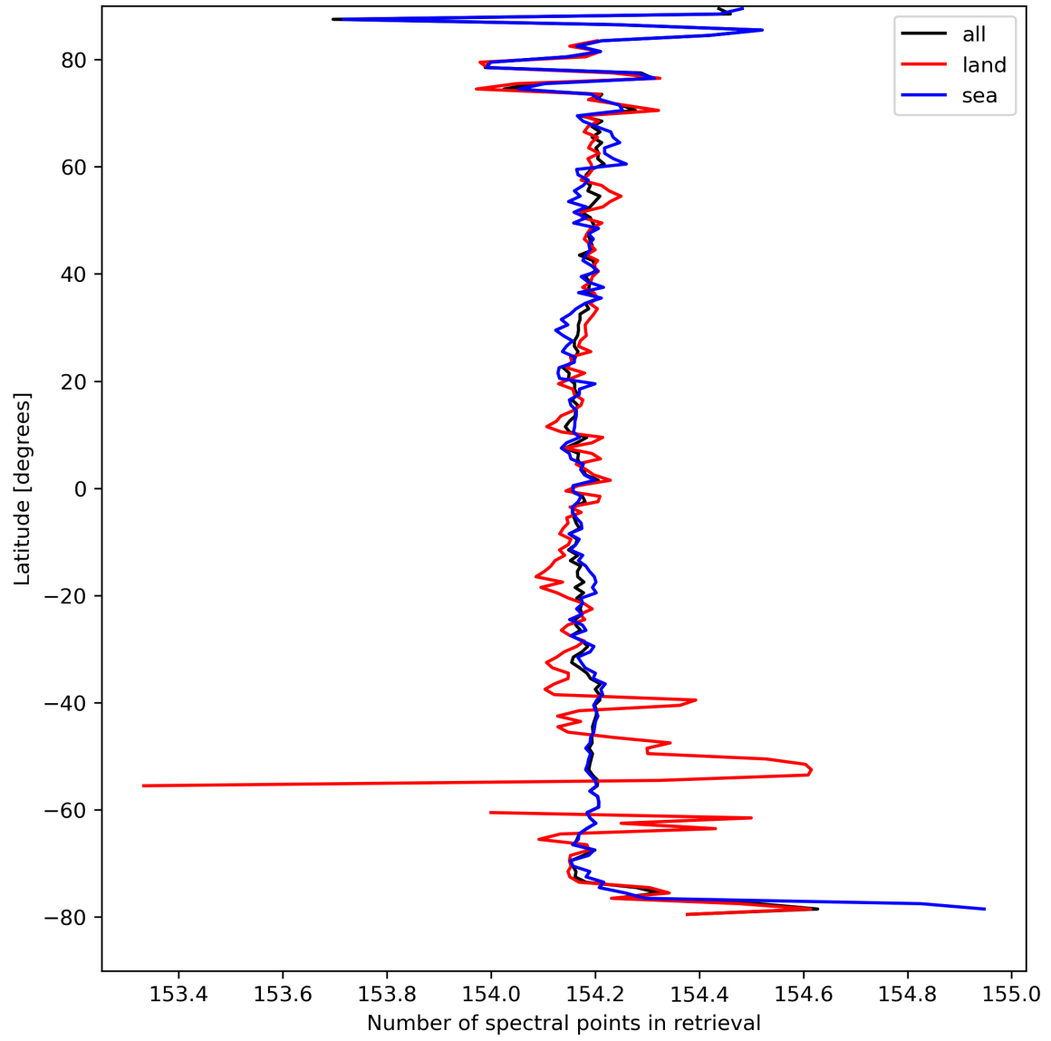
Figure 13: Zonal average of “Number of spectral points in retrieval” for 2023-09-07 to 2023-09-09.
