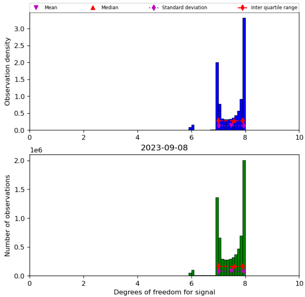
Figure 23: Histogram of “Degrees of freedom for signal” for 2023-09-07 to 2023-09-09
