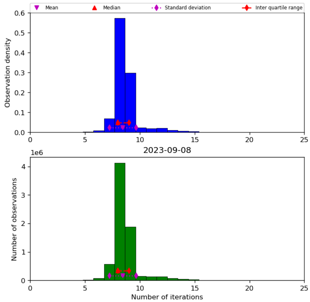
Figure 24: Histogram of “Number of iterations” for 2023-09-07 to 2023-09-09
