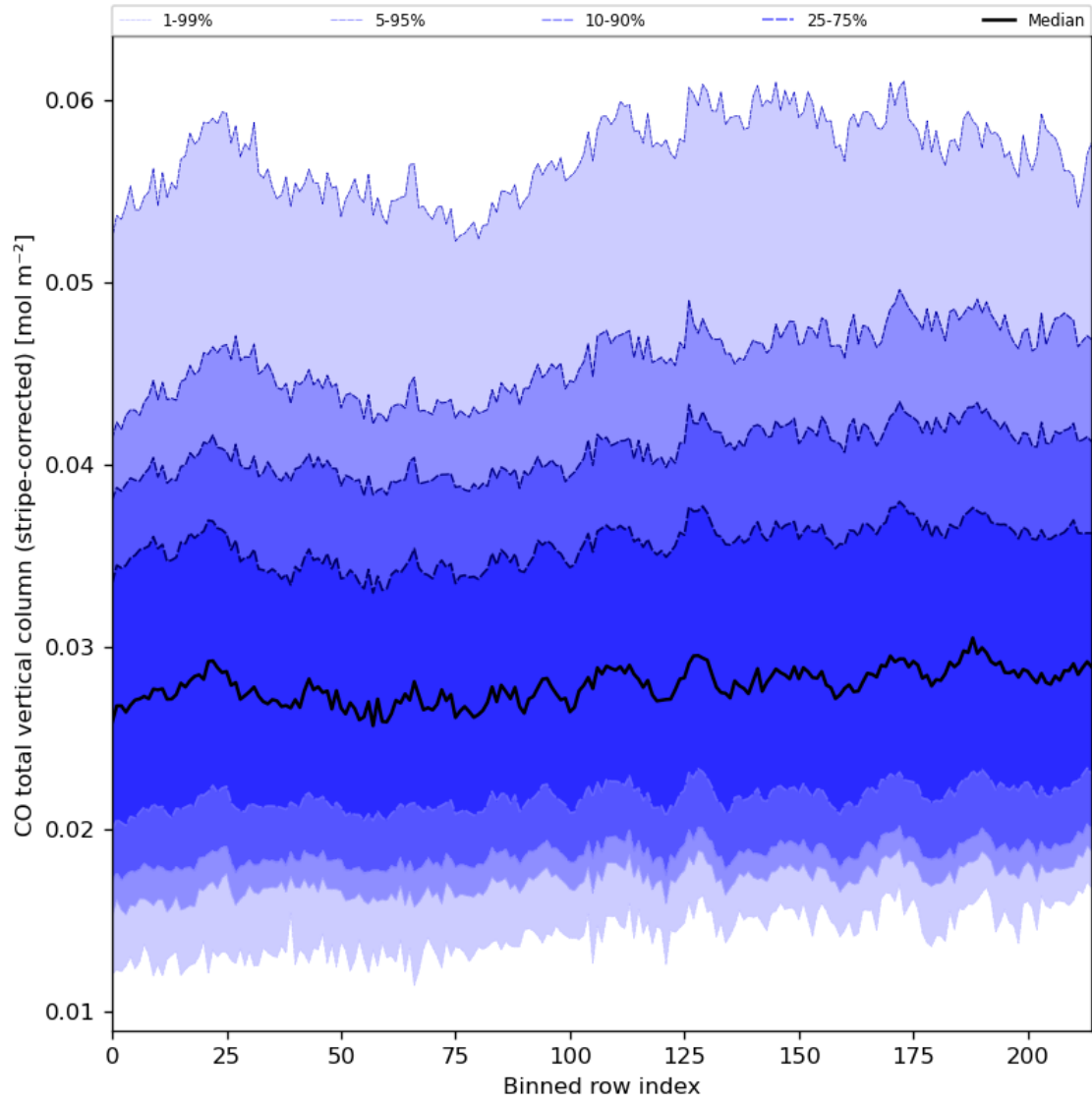
Figure 27: Along track statistics of “CO total vertical column (stripe-corrected)” for 2023-09-07 to 2023-09-09
