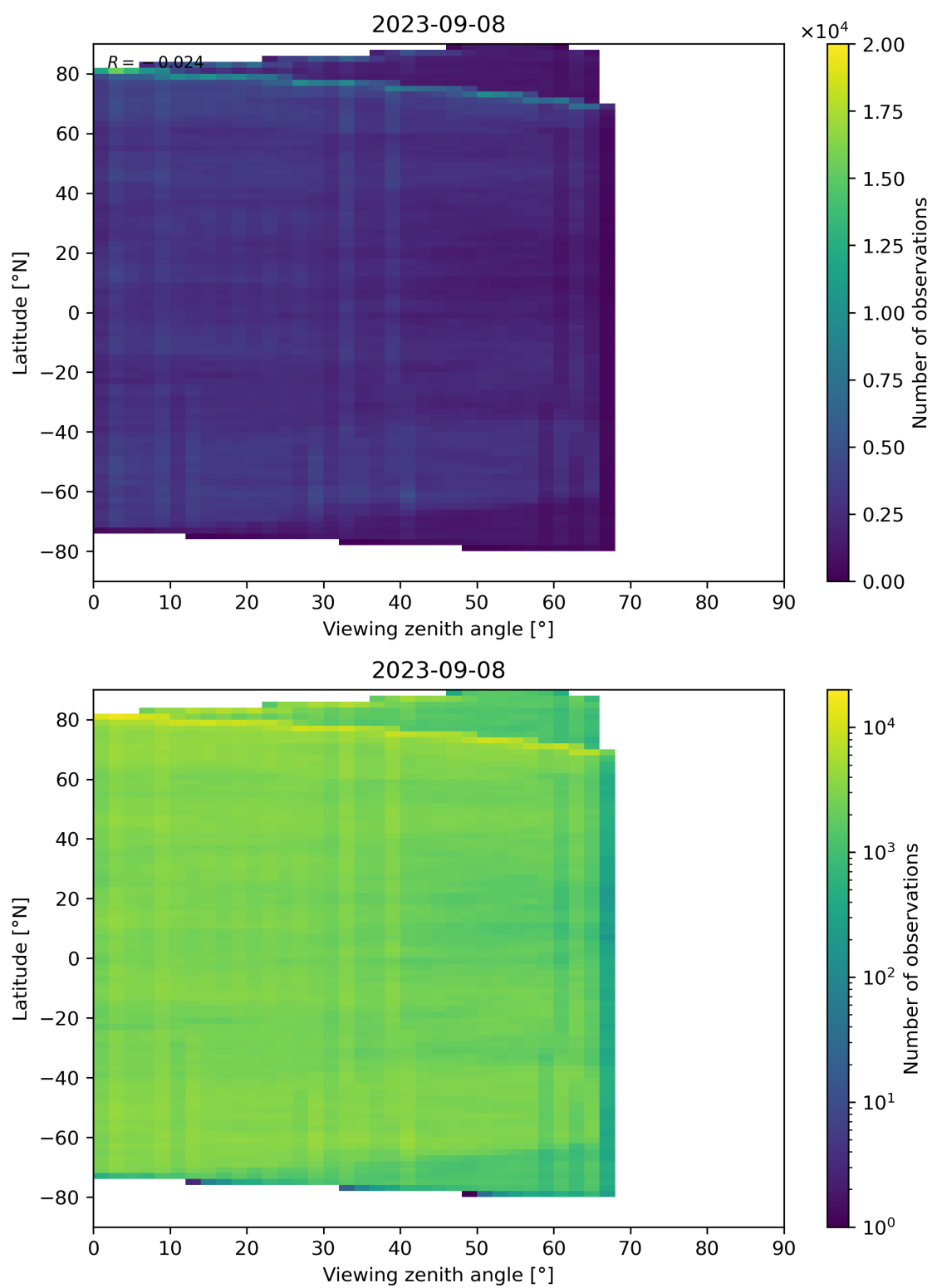
Figure 74: Scatter density plot of “Viewing zenith angle” against “Latitude” for 2023-09-07 to 2023-09-09.
