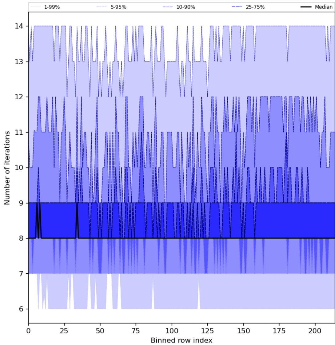
Figure 32: Along track statistics of “Number of iterations” for 2023-09-07 to 2023-09-09
