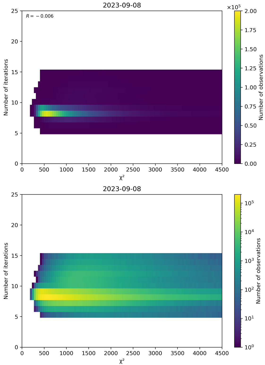
Figure 49: Scatter density plot of “ \chi^2 ” against “Number of iterations” for 2023-09-07 to 2023-09-09.
