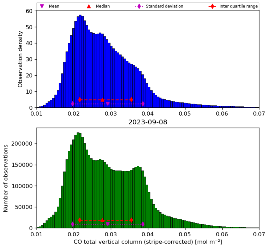
Figure 19: Histogram of “CO total vertical column (stripe-corrected)” for 2023-09-07 to 2023-09-09
