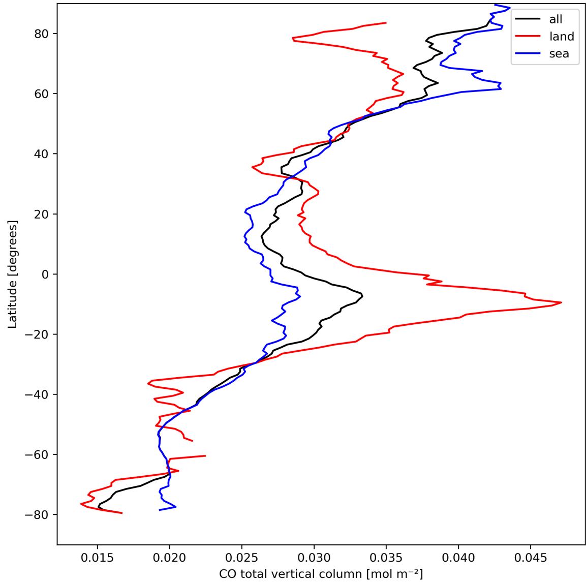
Figure 10: Zonal average of “CO total vertical column” for 2023-09-07 to 2023-09-09.
