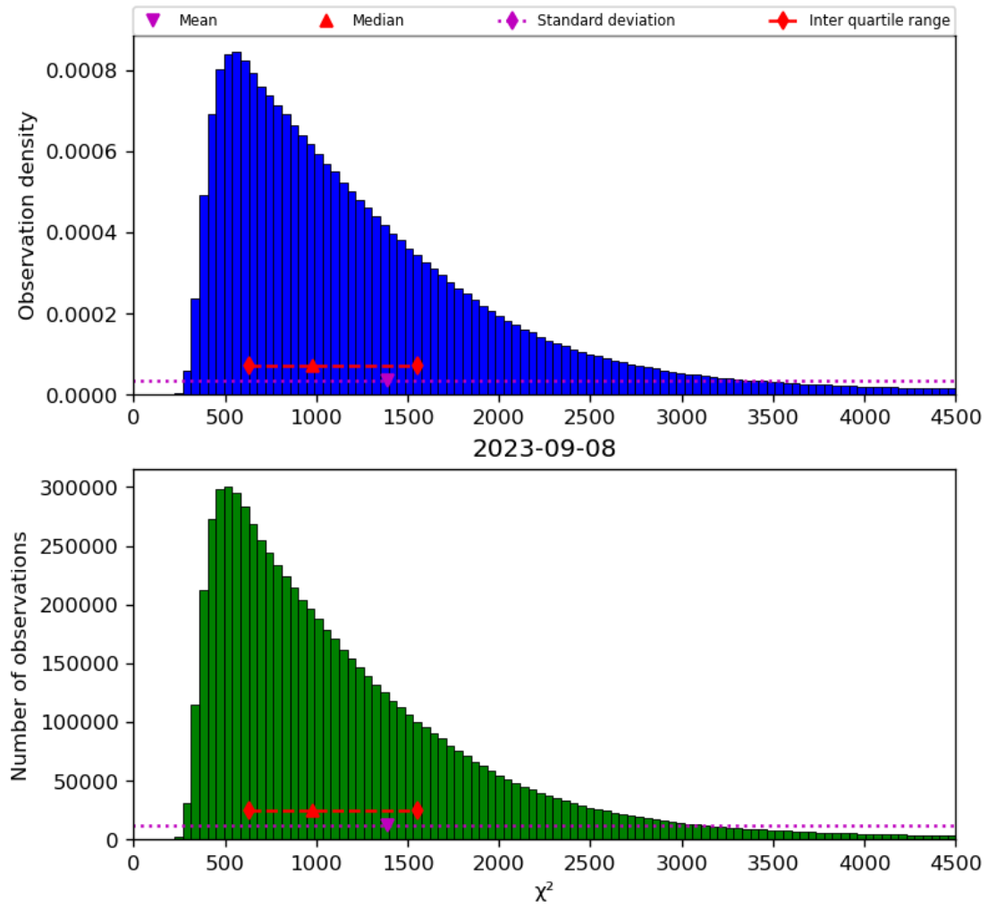
Figure 22: Histogram of “ \chi^2 ” for 2023-09-07 to 2023-09-09
