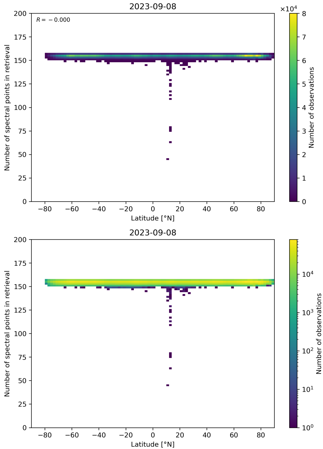
Figure 57: Scatter density plot of “Latitude” against “Number of spectral points in retrieval” for 2023-09-07 to 2023-09-09.
