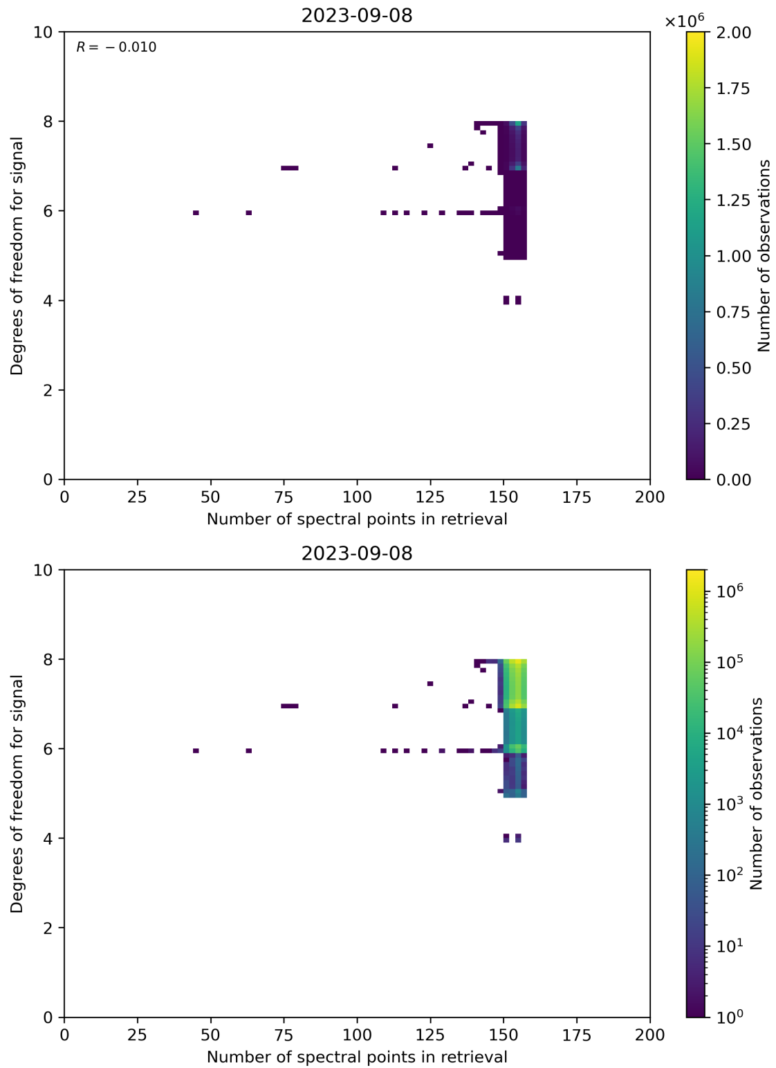
Figure 59: Scatter density plot of “Number of spectral points in retrieval” against “Degrees of freedom for signal” for 2023-09-07 to 2023-09-09.
