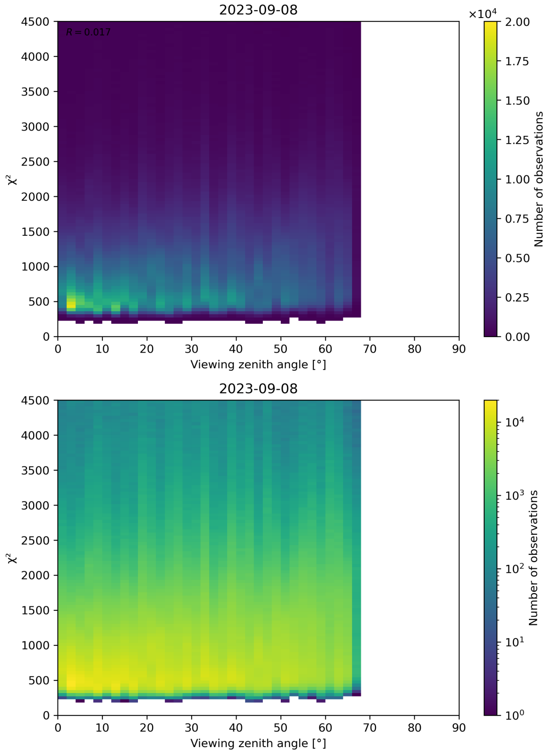
Figure 72: Scatter density plot of “Viewing zenith angle” against “ \chi^2 ” for 2023-09-07 to 2023-09-09.
