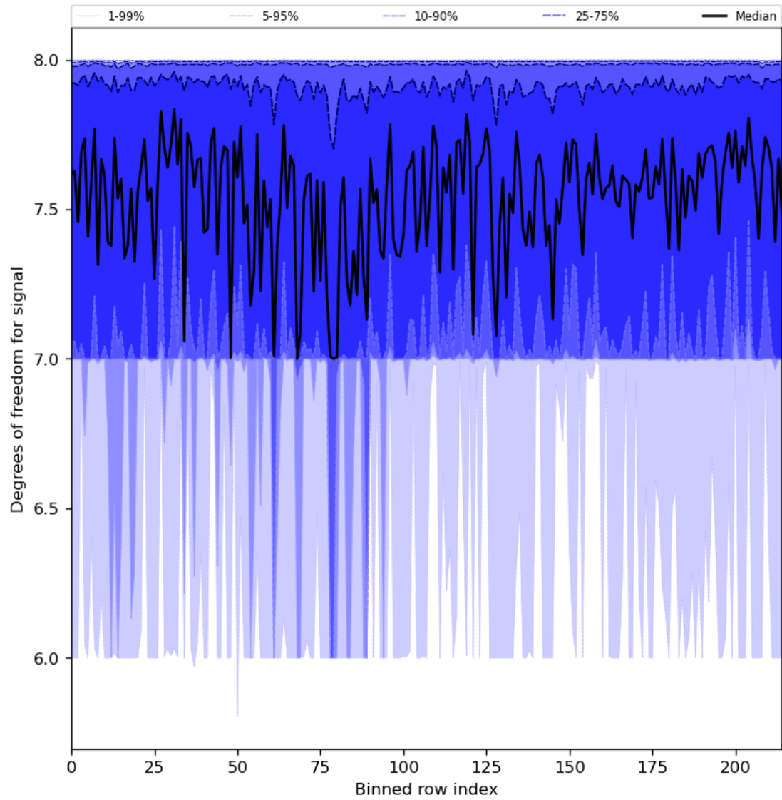
Figure 31: Along track statistics of “Degrees of freedom for signal” for 2023-09-07 to 2023-09-09
