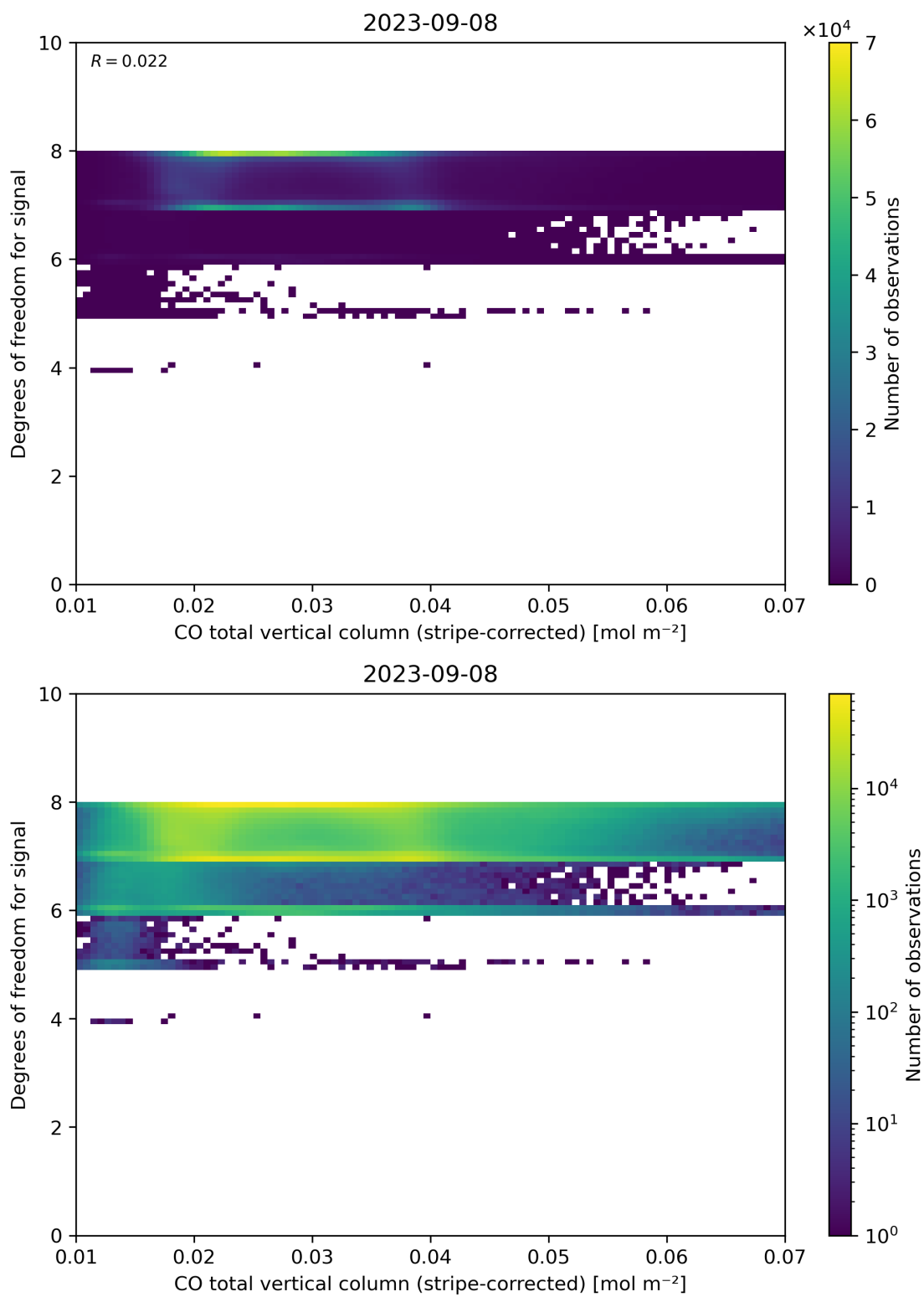
Figure 38: Scatter density plot of “CO total vertical column (stripe-corrected)” against “Degrees of freedom for signal” for 2023-09-07 to 2023-09-09.
