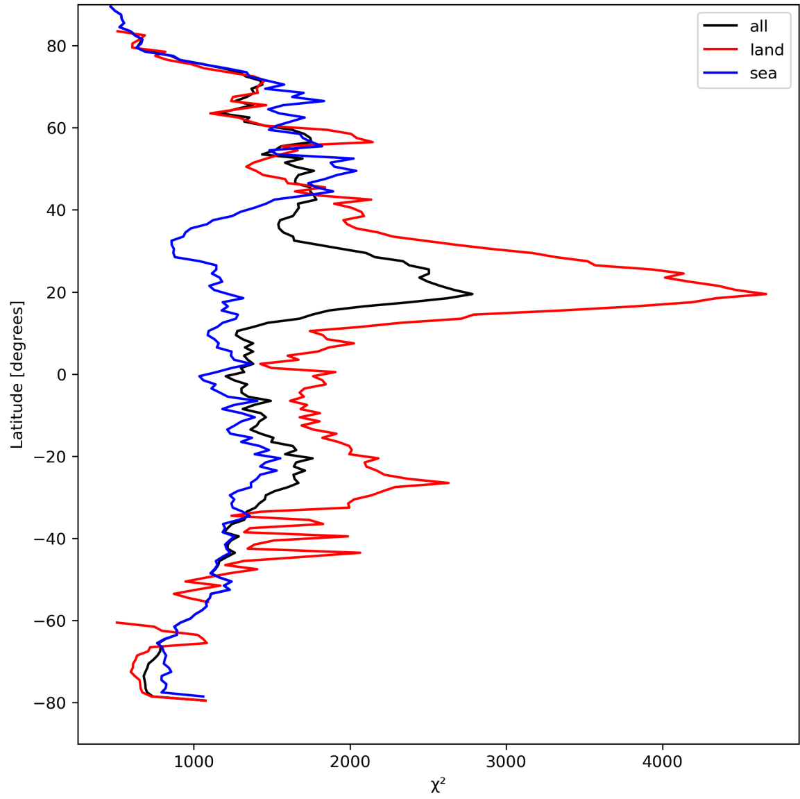
Figure 14: Zonal average of “ \chi^2 ” for 2023-09-07 to 2023-09-09.
