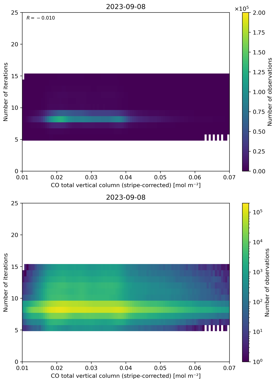
Figure 39: Scatter density plot of “CO total vertical column (stripe-corrected)” against “Number of iterations” for 2023-09-07 to 2023-09-09.
