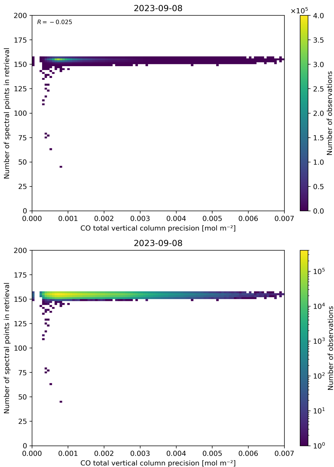
Figure 47: Scatter density plot of “CO total vertical column precision” against “Number of spectral points in retrieval” for 2023-09-07 to 2023-09-09.
