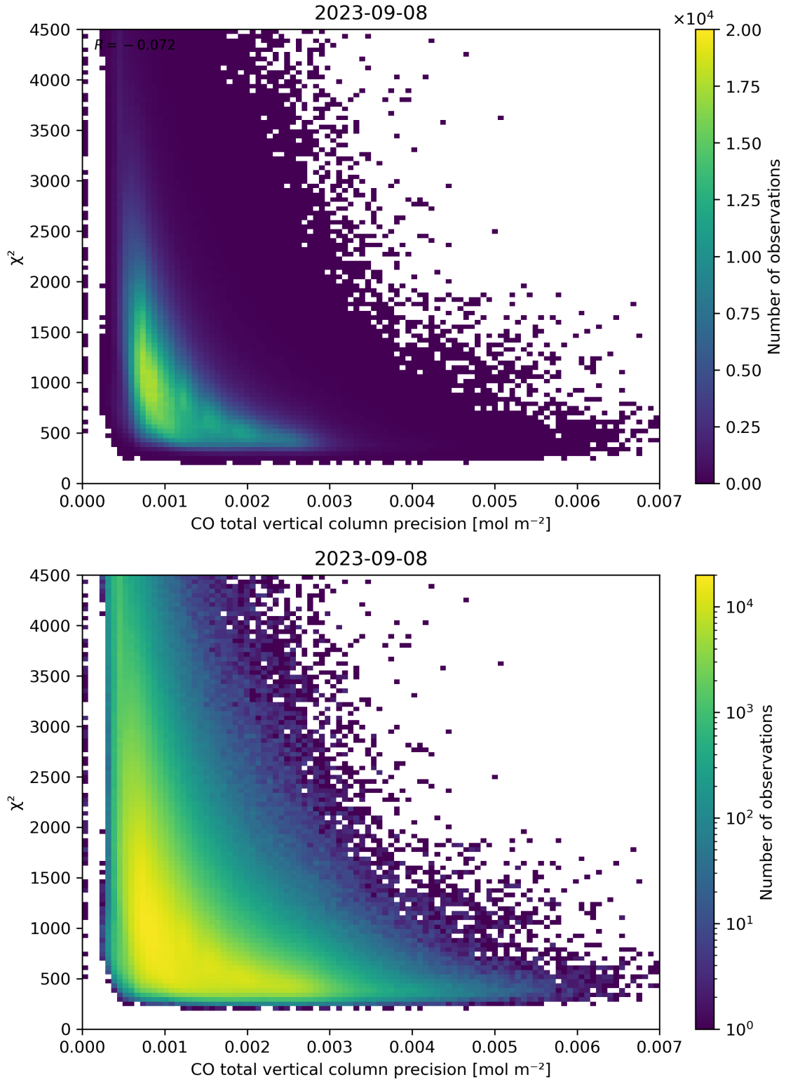
Figure 44: Scatter density plot of “CO total vertical column precision” against “ \chi^2 ” for 2023-09-07 to 2023-09-09.
