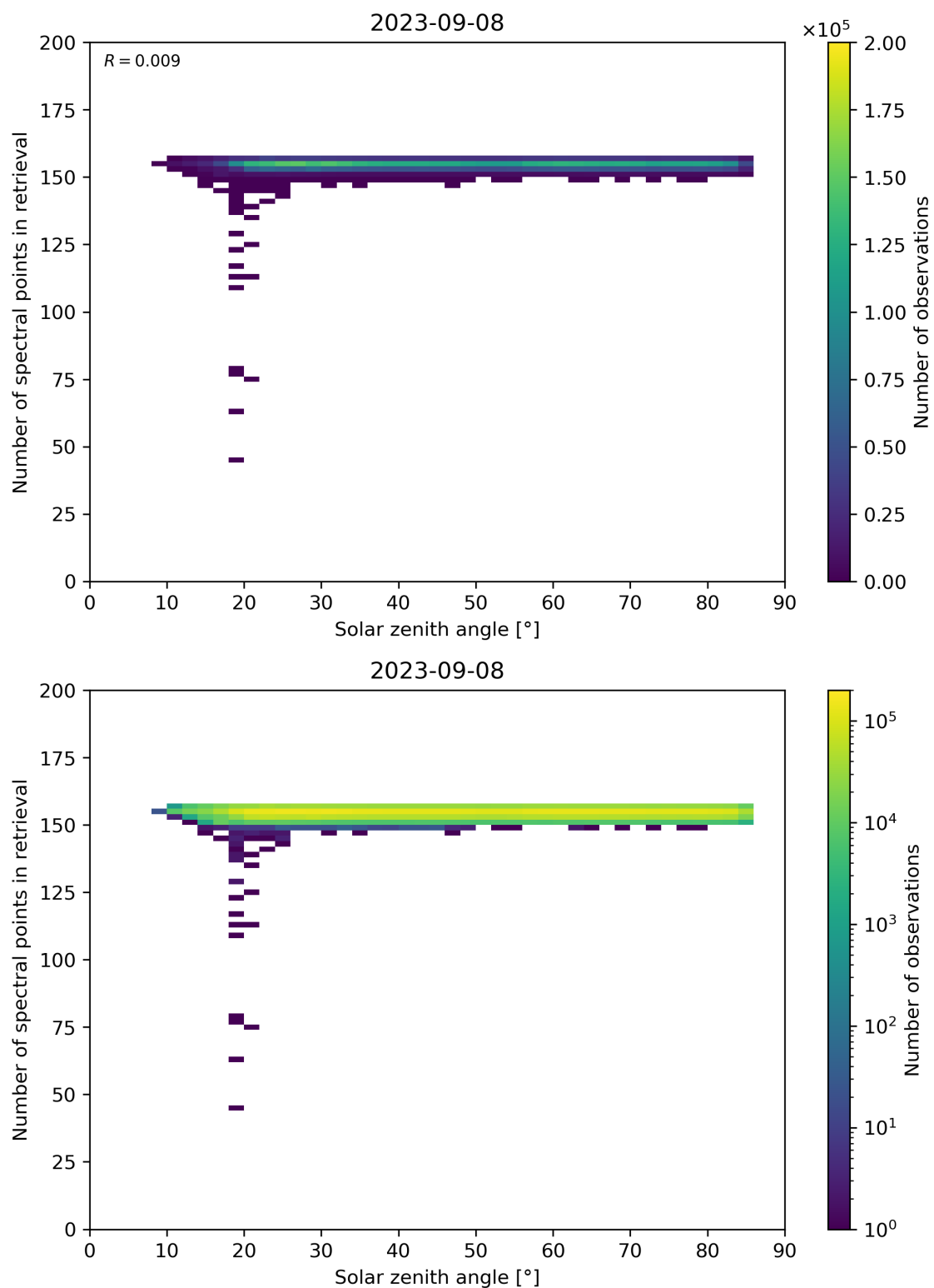
Figure 68: Scatter density plot of “Solar zenith angle” against “Number of spectral points in retrieval” for 2023-09-07 to 2023-09-09.
