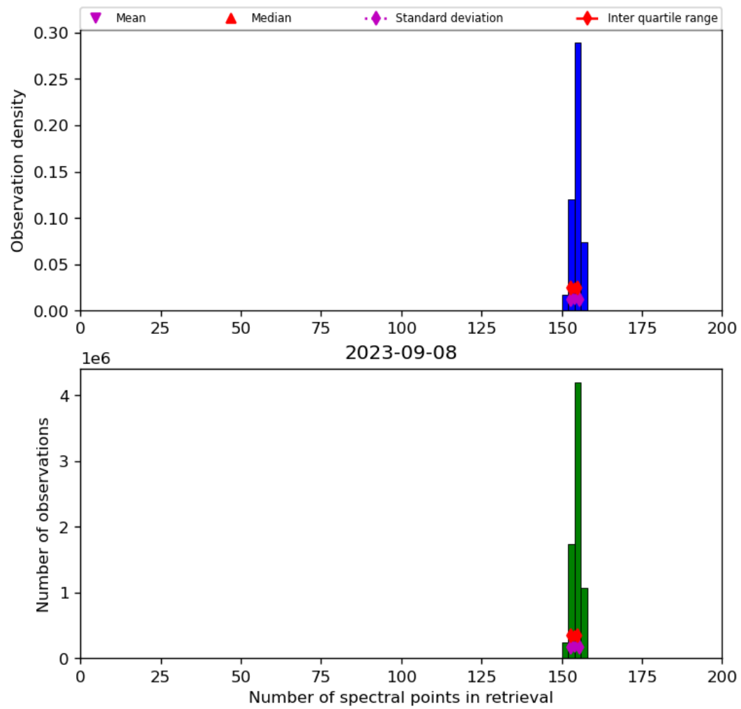
Figure 21: Histogram of “Number of spectral points in retrieval” for 2023-09-07 to 2023-09-09
