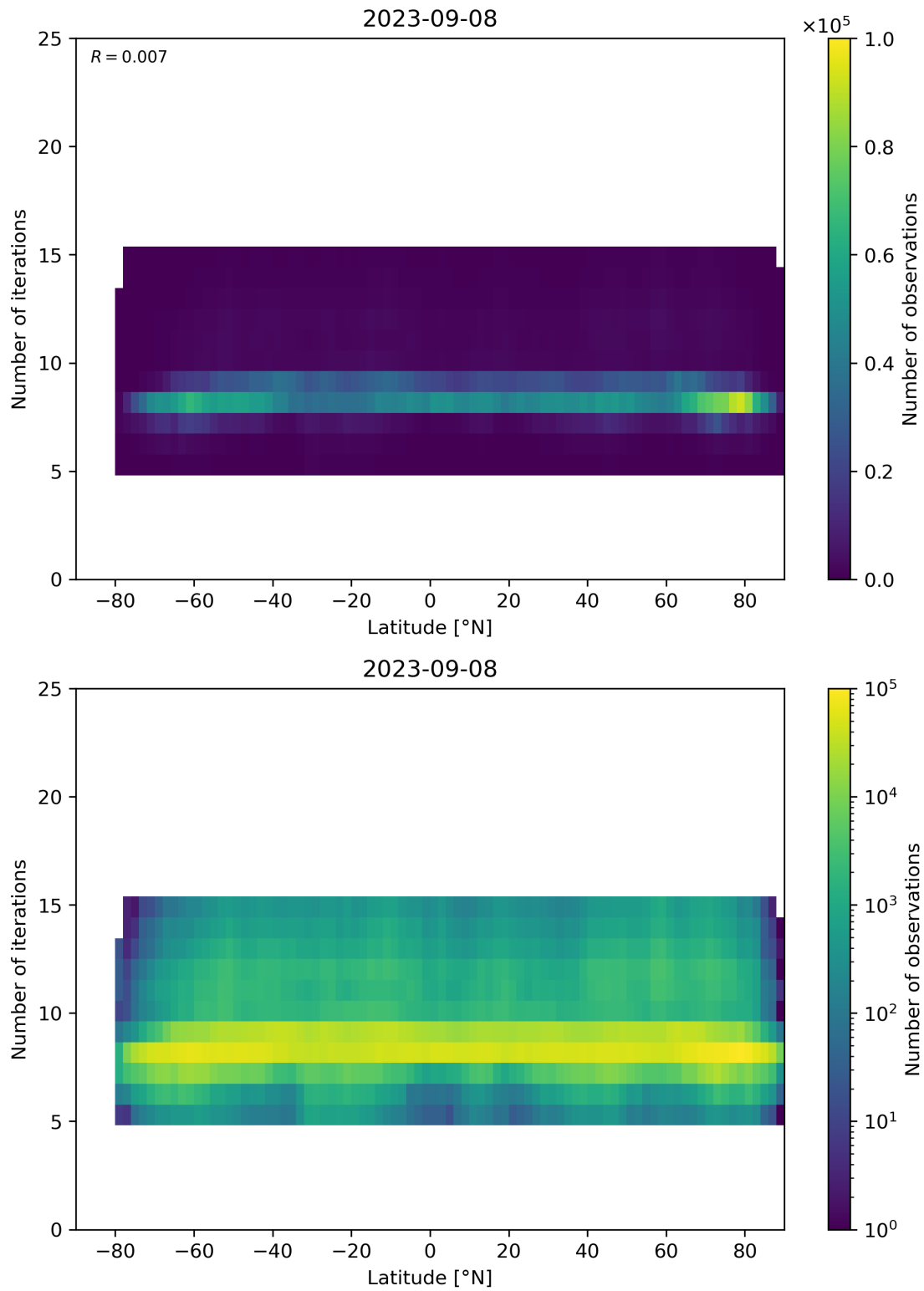
Figure 56: Scatter density plot of “Latitude” against “Number of iterations” for 2023-09-07 to 2023-09-09.
