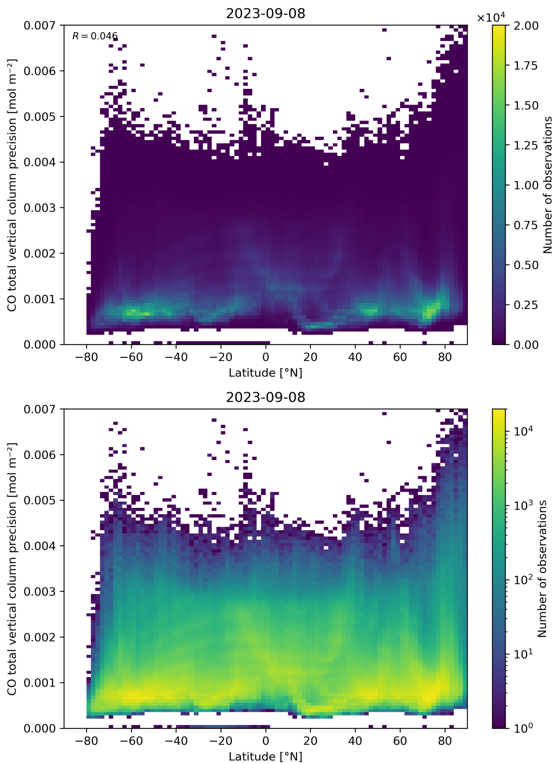
Figure 53: Scatter density plot of “Latitude” against “CO total vertical column precision” for 2023-09-07 to 2023-09-09.
