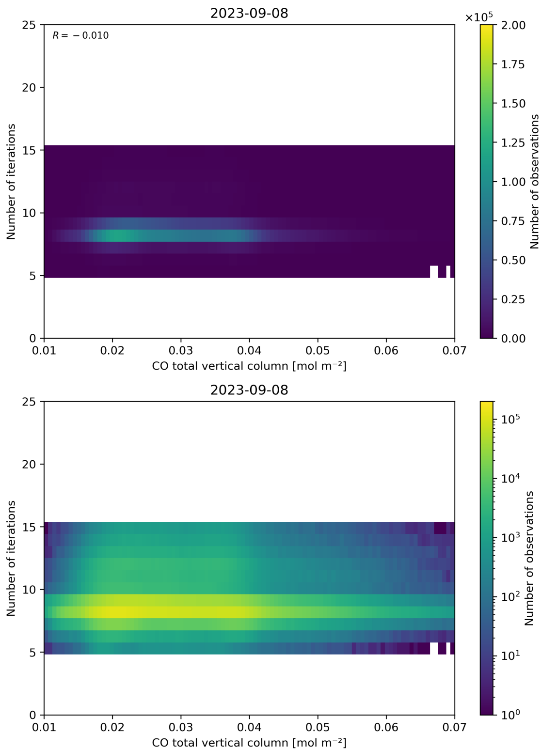
Figure 42: Scatter density plot of “CO total vertical column” against “Number of iterations” for 2023-09-07 to 2023-09-09.
