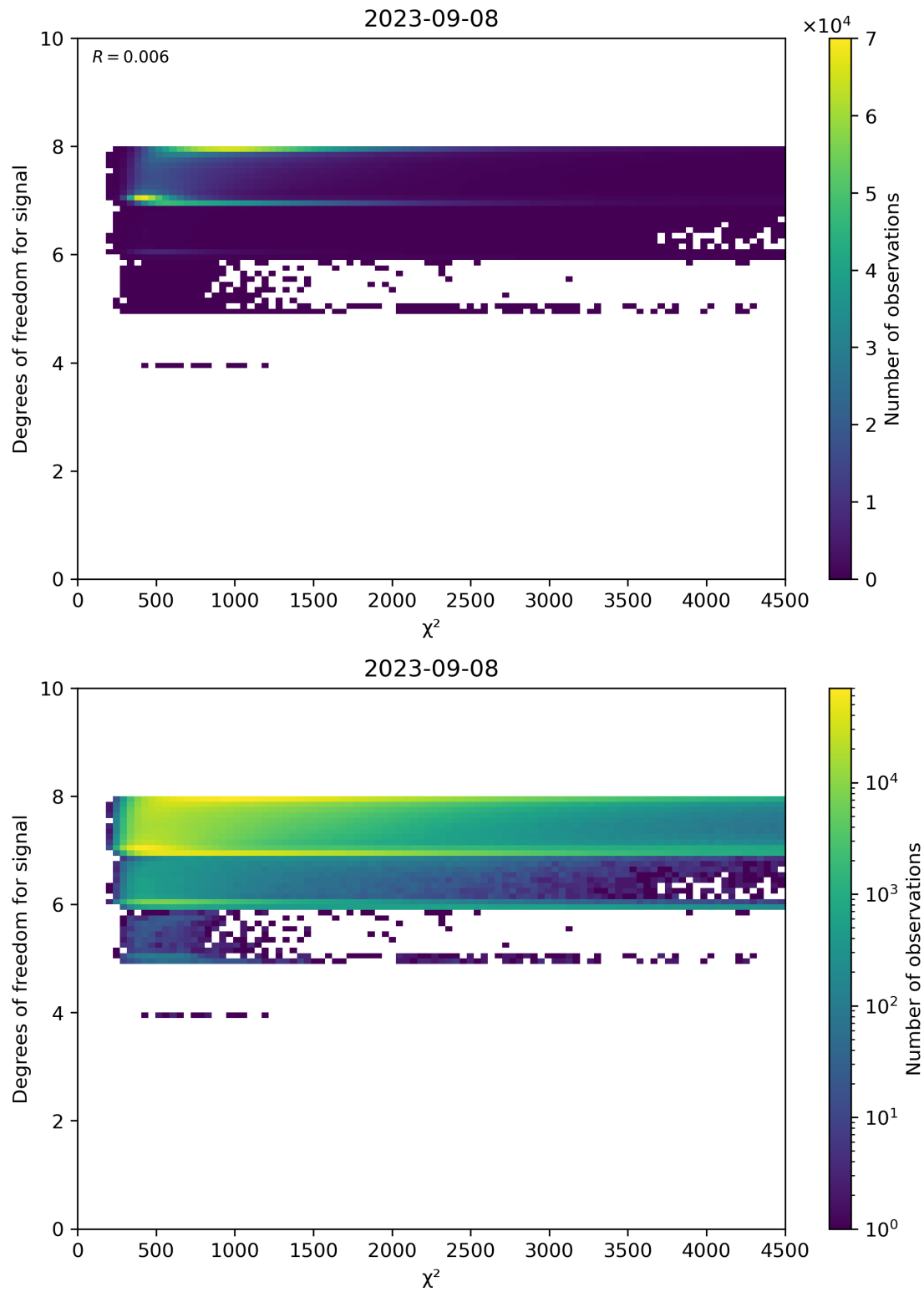
Figure 48: Scatter density plot of “ \chi^2 ” against “Degrees of freedom for signal” for 2023-09-07 to 2023-09-09.
