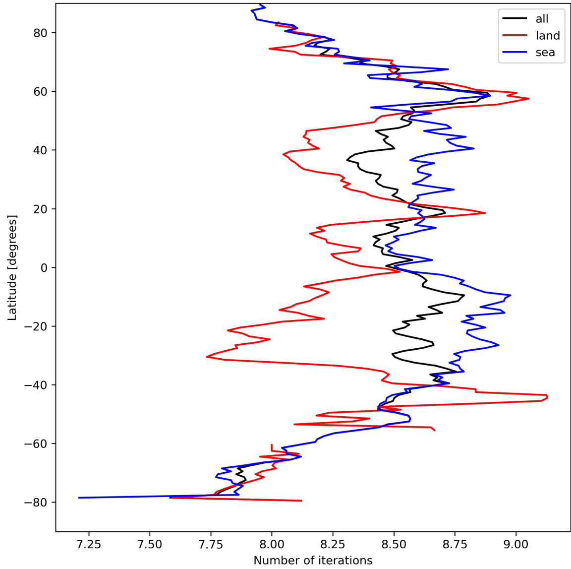
Figure 16: Zonal average of “Number of iterations” for 2023-09-07 to 2023-09-09.
