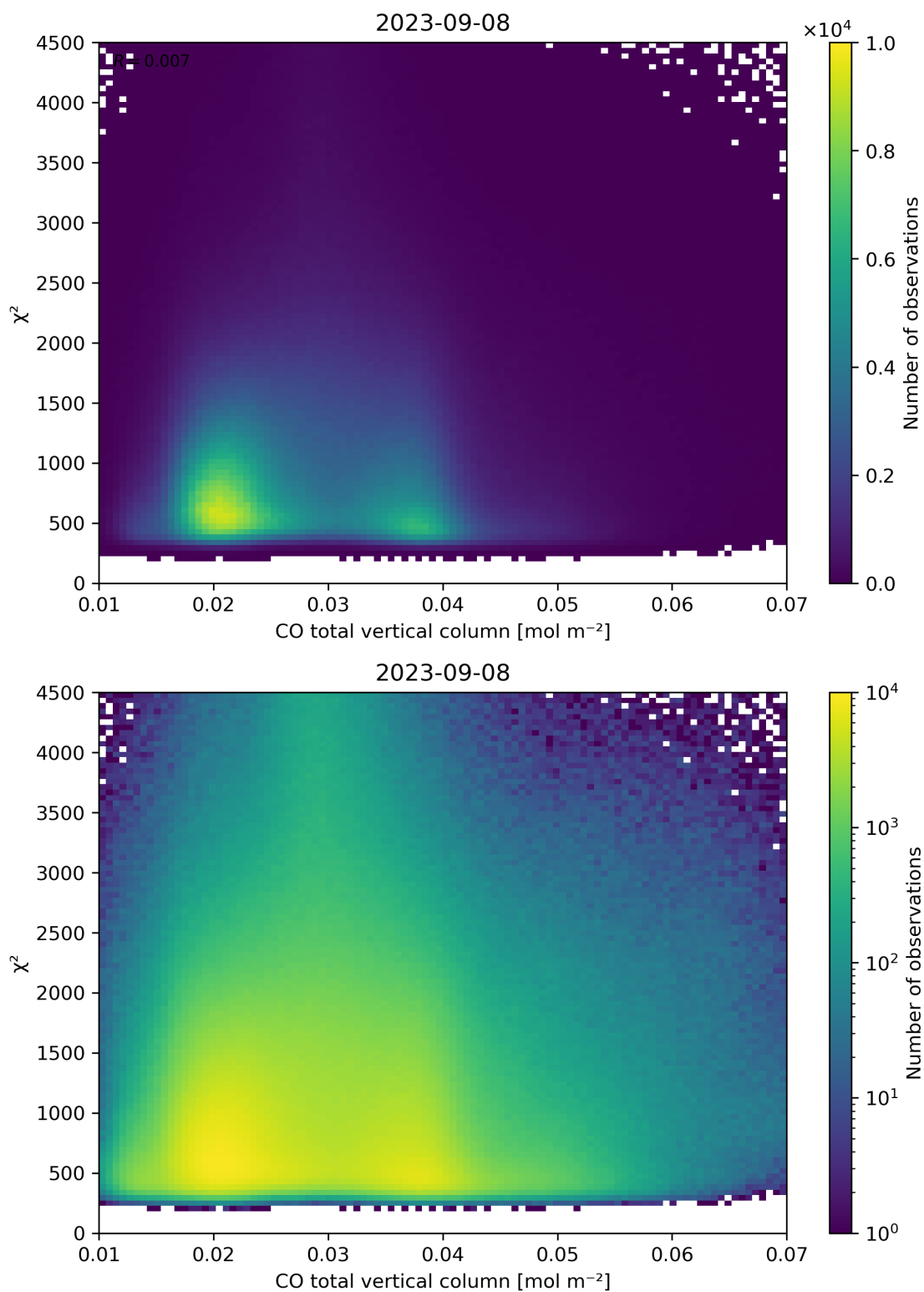
Figure 35: Scatter density plot of “CO total vertical column” against “ \chi^2 ” for 2023-09-07 to 2023-09-09.
