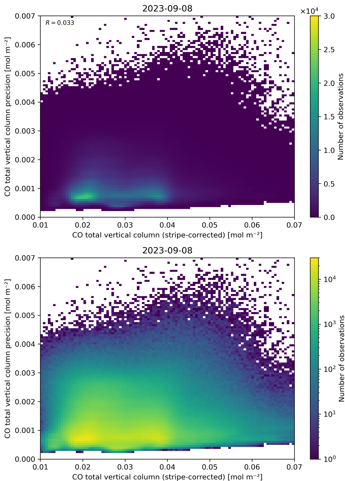
Figure 36: Scatter density plot of “CO total vertical column (stripe-corrected)” against “CO total vertical column precision” for 2023-09-07 to 2023-09-09.
