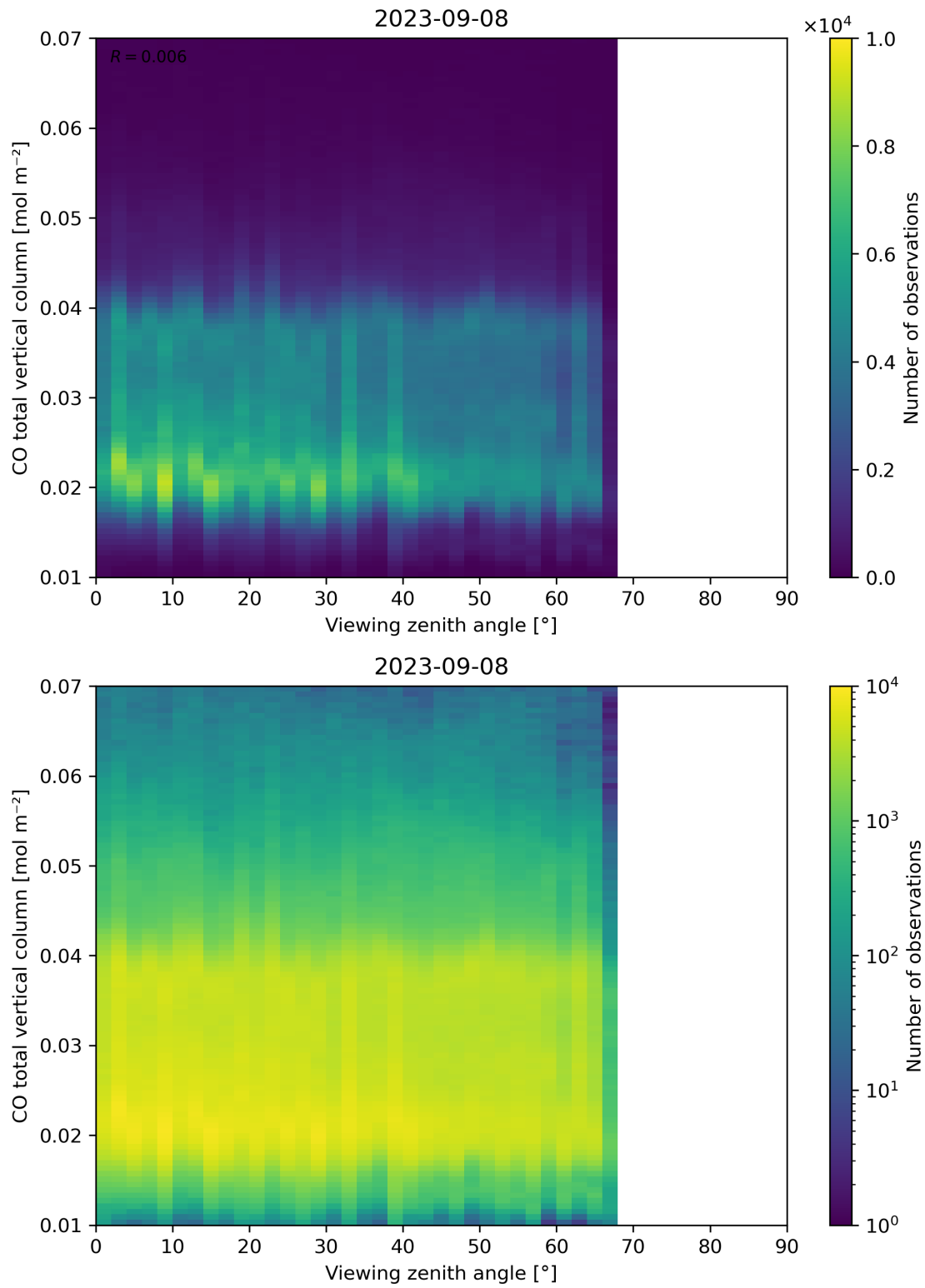
Figure 69: Scatter density plot of “Viewing zenith angle” against “CO total vertical column” for 2023-09-07 to 2023-09-09.
