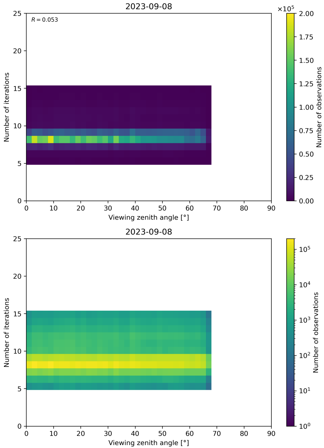
Figure 75: Scatter density plot of “Viewing zenith angle” against “Number of iterations” for 2023-09-07 to 2023-09-09.
