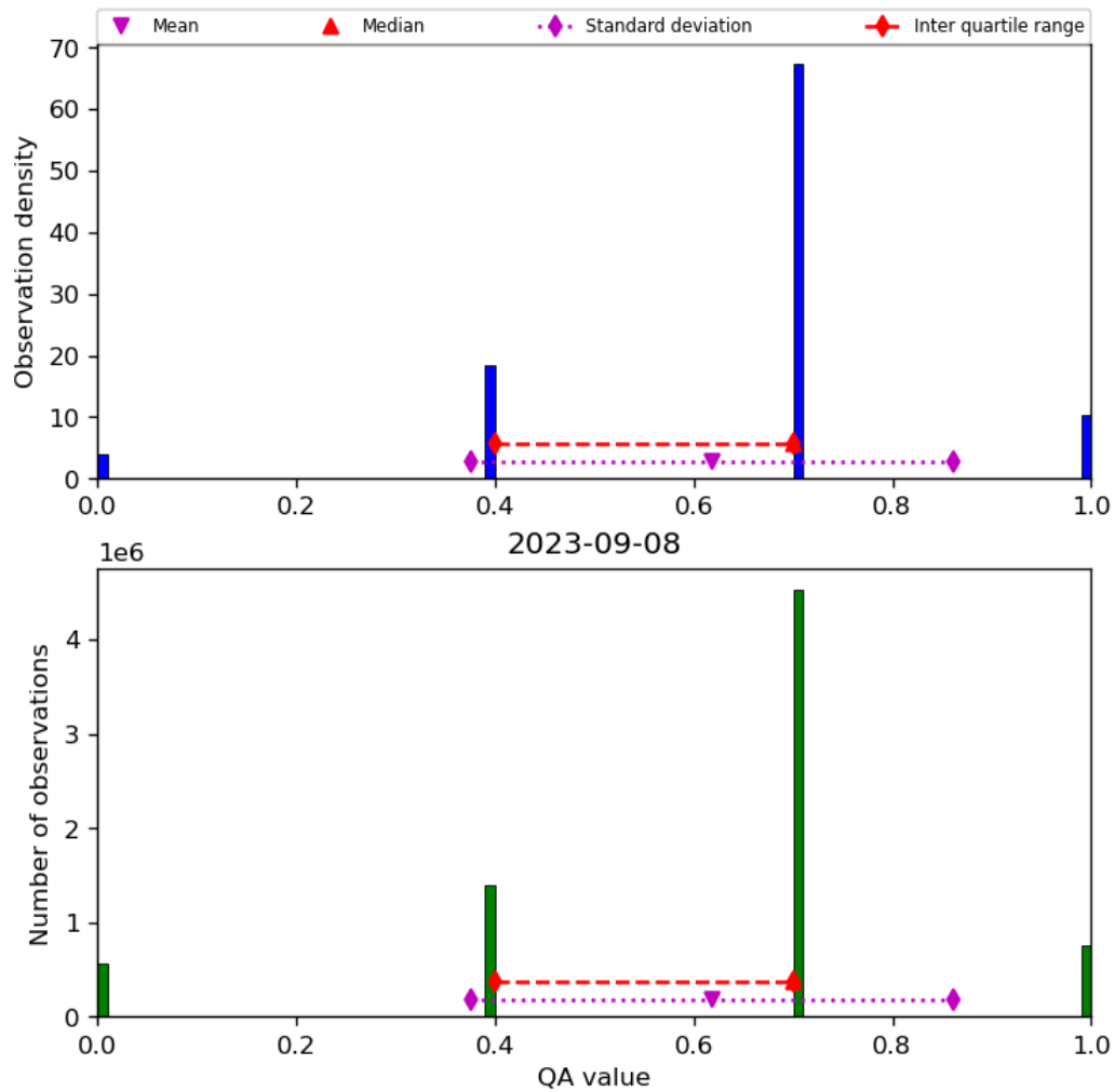
Figure 17: Histogram of “QA value” for 2023-09-07 to 2023-09-09
