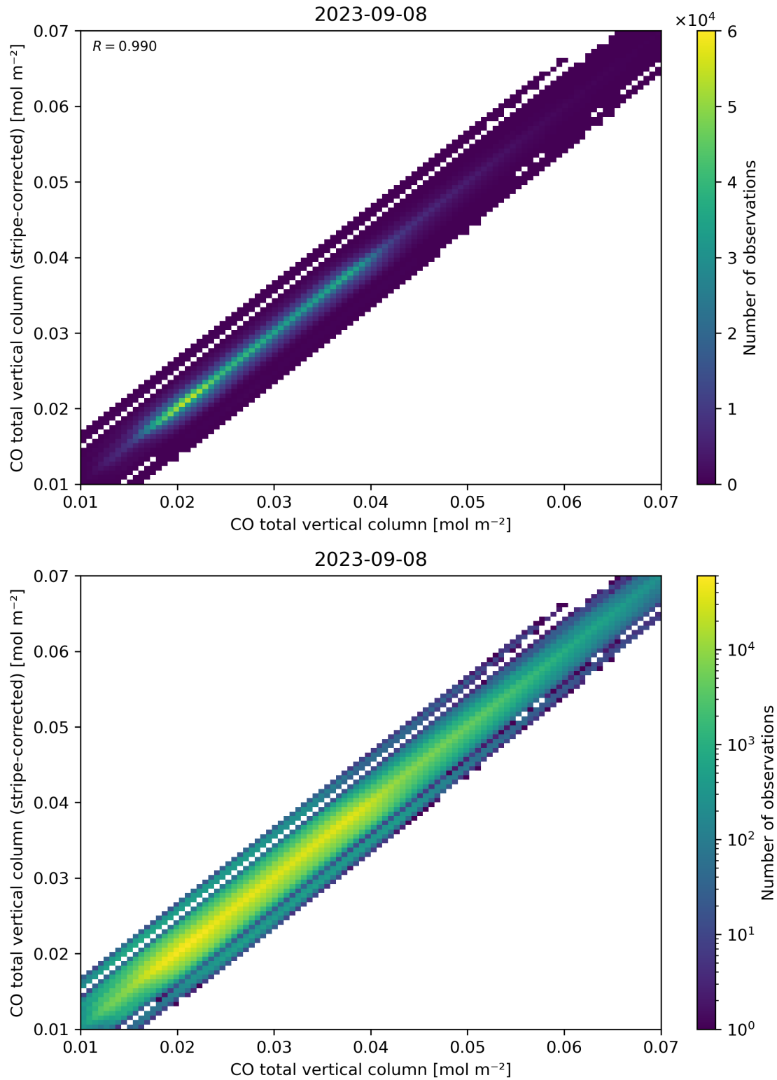
Figure 33: Scatter density plot of “CO total vertical column” against “CO total vertical column (stripe-corrected)” for 2023-09-07 to 2023-09-09.
