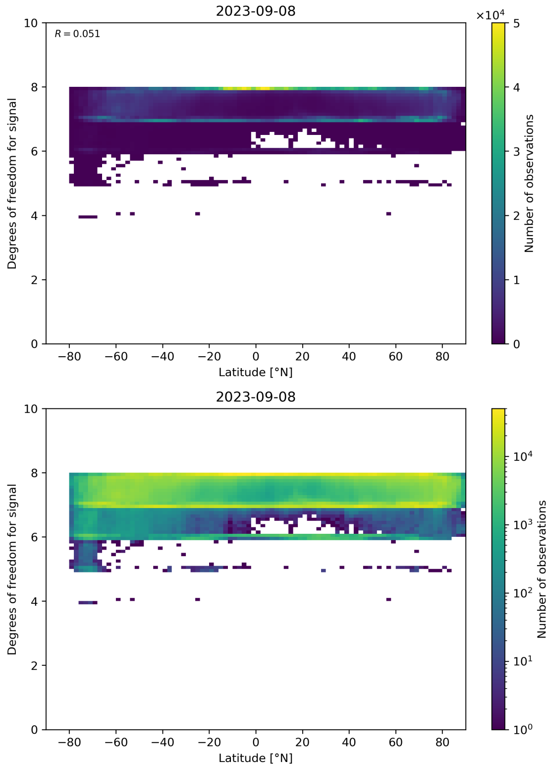
Figure 55: Scatter density plot of “Latitude” against “Degrees of freedom for signal” for 2023-09-07 to 2023-09-09.
