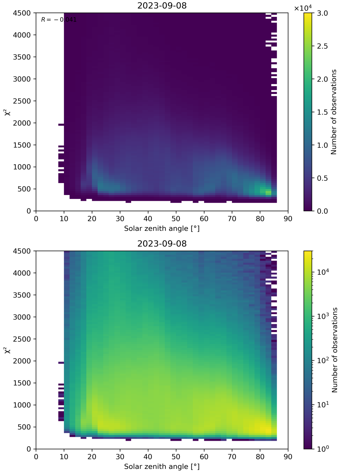
Figure 64: Scatter density plot of “Solar zenith angle” against “ \chi^2 ” for 2023-09-07 to 2023-09-09.
