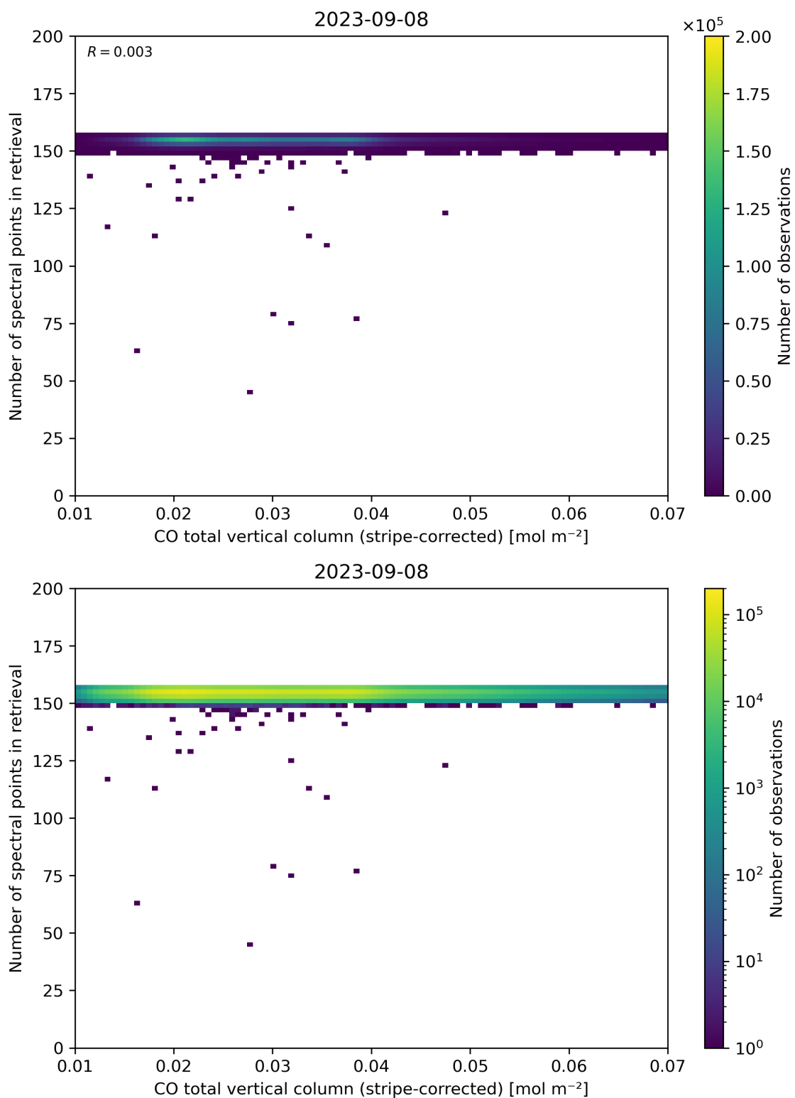
Figure 40: Scatter density plot of “CO total vertical column (stripe-corrected)” against “Number of spectral points in retrieval” for 2023-09-07 to 2023-09-09.
