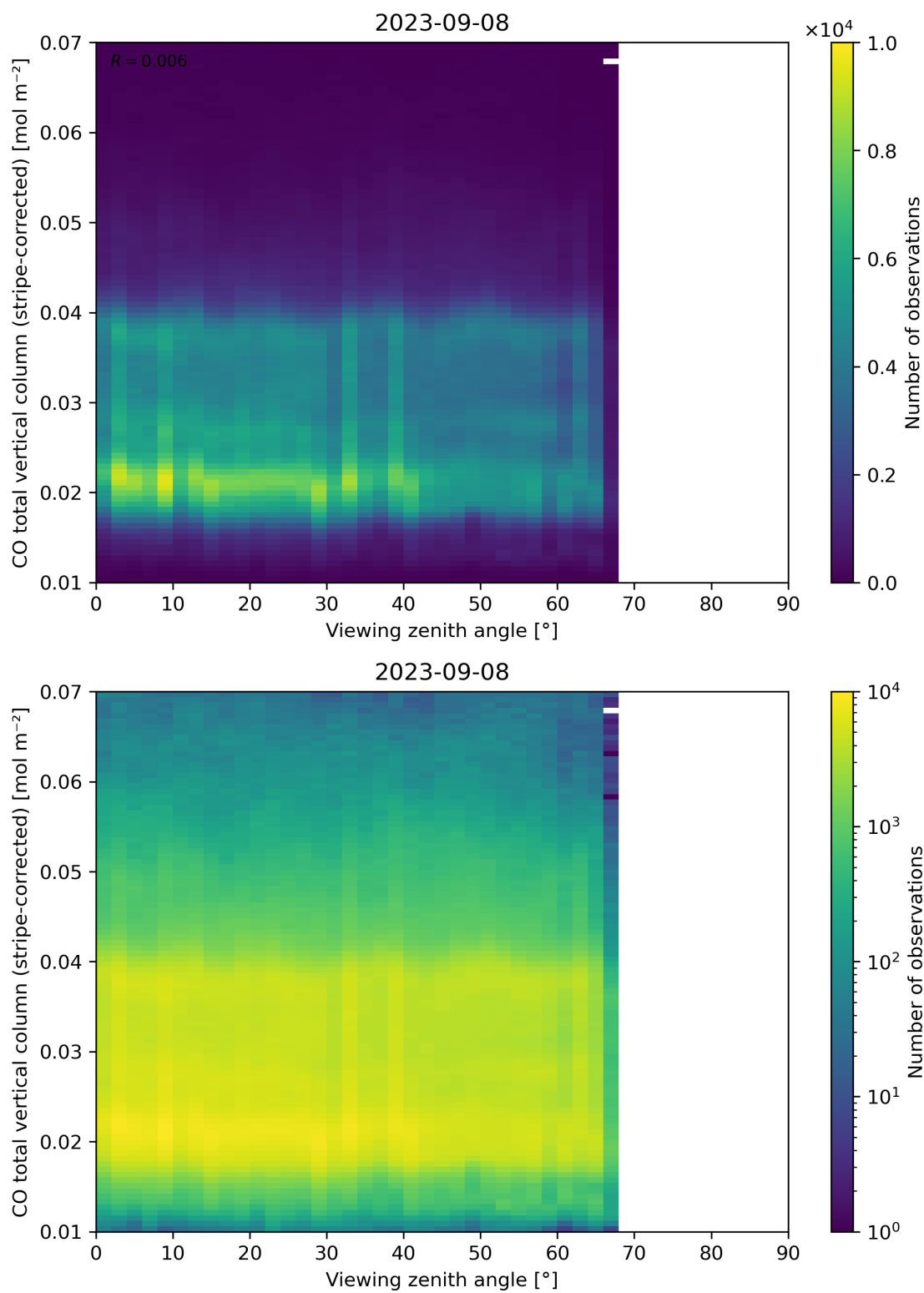
Figure 70: Scatter density plot of “Viewing zenith angle” against “CO total vertical column (stripe-corrected)” for 2023-09-07 to 2023-09-09.
