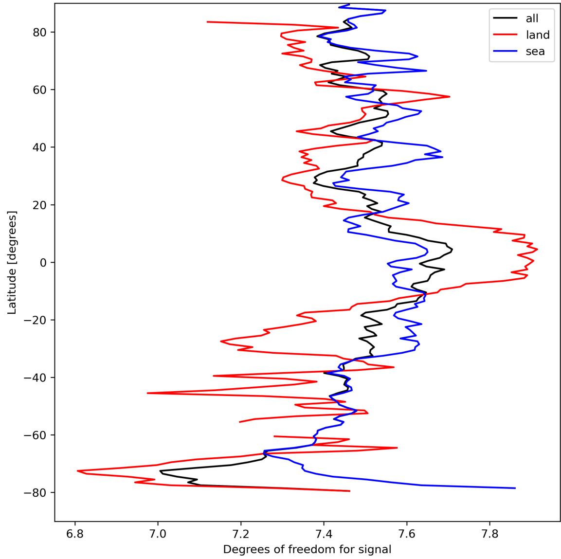
Figure 15: Zonal average of “Degrees of freedom for signal” for 2023-09-07 to 2023-09-09.
