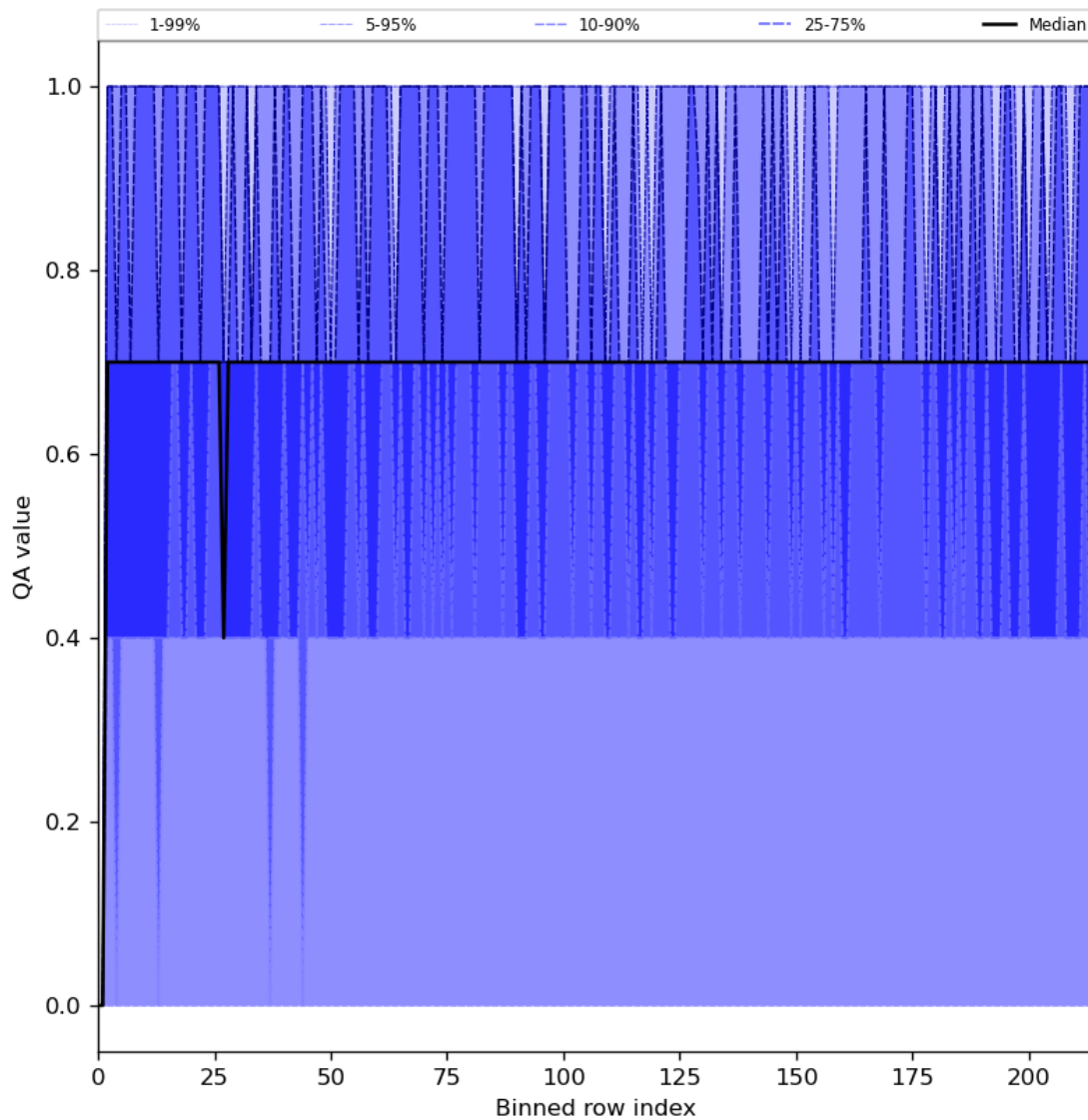
Figure 25: Along track statistics of “QA value” for 2023-09-07 to 2023-09-09
