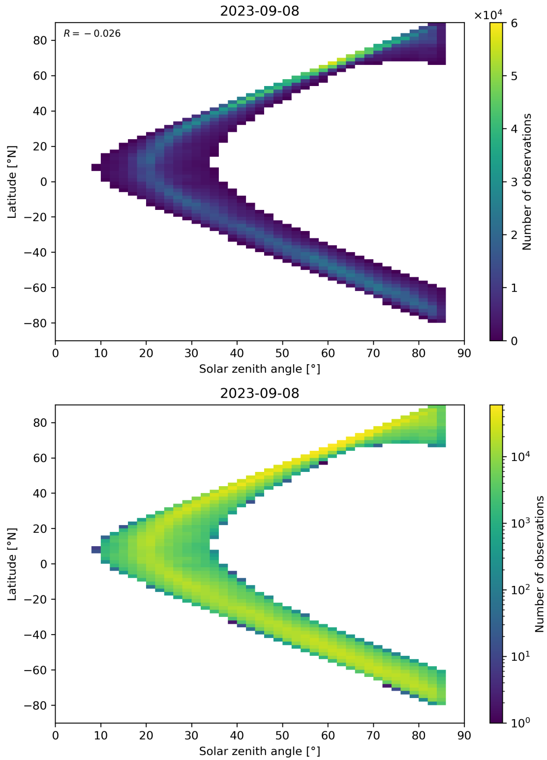
Figure 66: Scatter density plot of “Solar zenith angle” against “Latitude” for 2023-09-07 to 2023-09-09.
