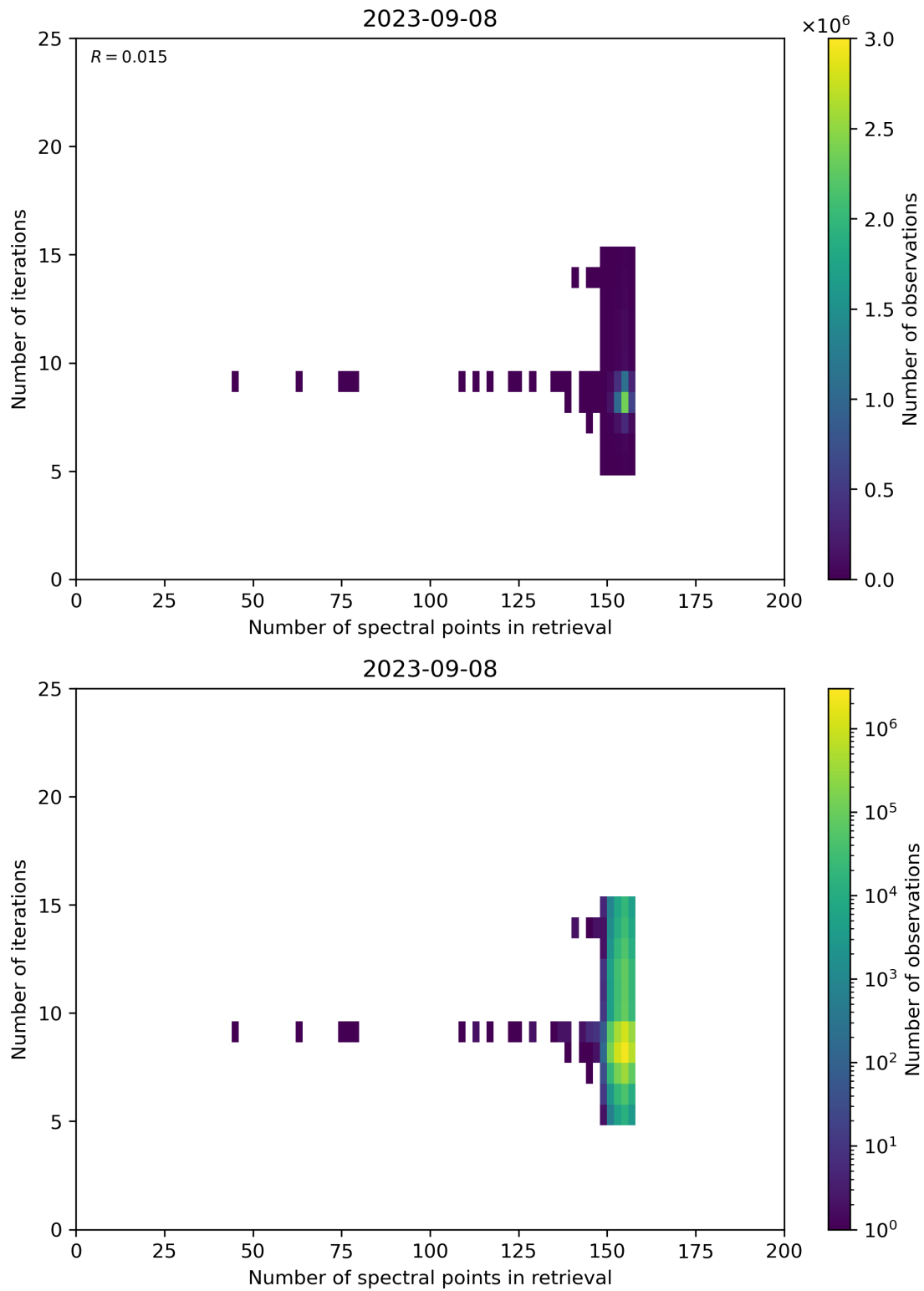
Figure 60: Scatter density plot of “Number of spectral points in retrieval” against “Number of iterations” for 2023-09-07 to 2023-09-09.
