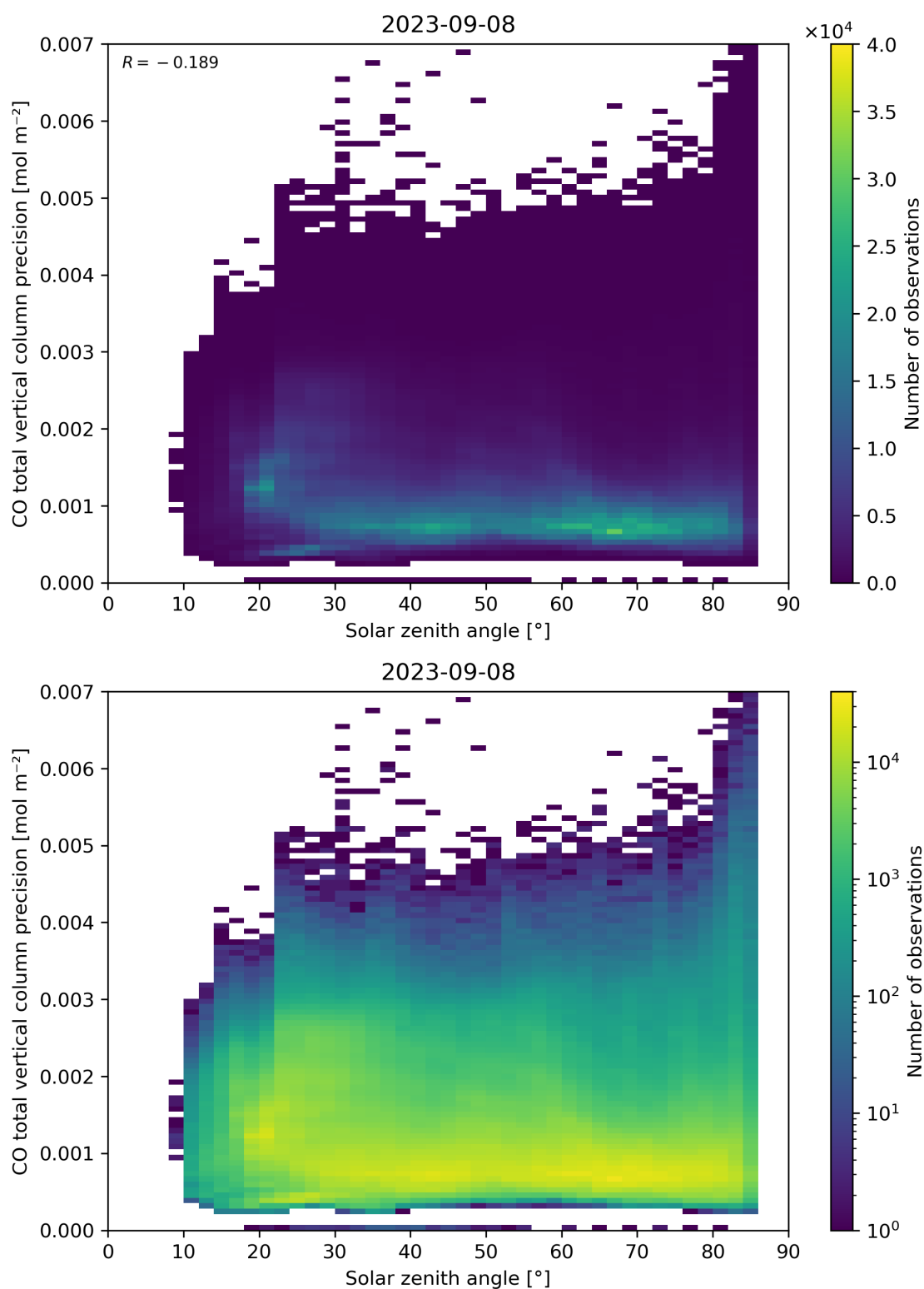
Figure 63: Scatter density plot of “Solar zenith angle” against “CO total vertical column precision” for 2023-09-07 to 2023-09-09.
