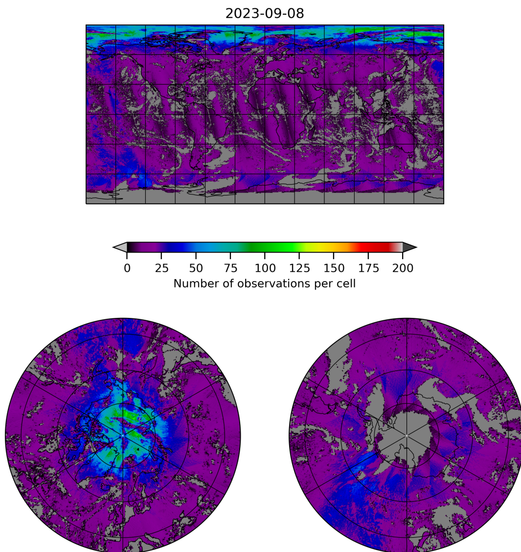
Figure 8: Map of the number of observations for 2023-09-07 to 2023-09-09
