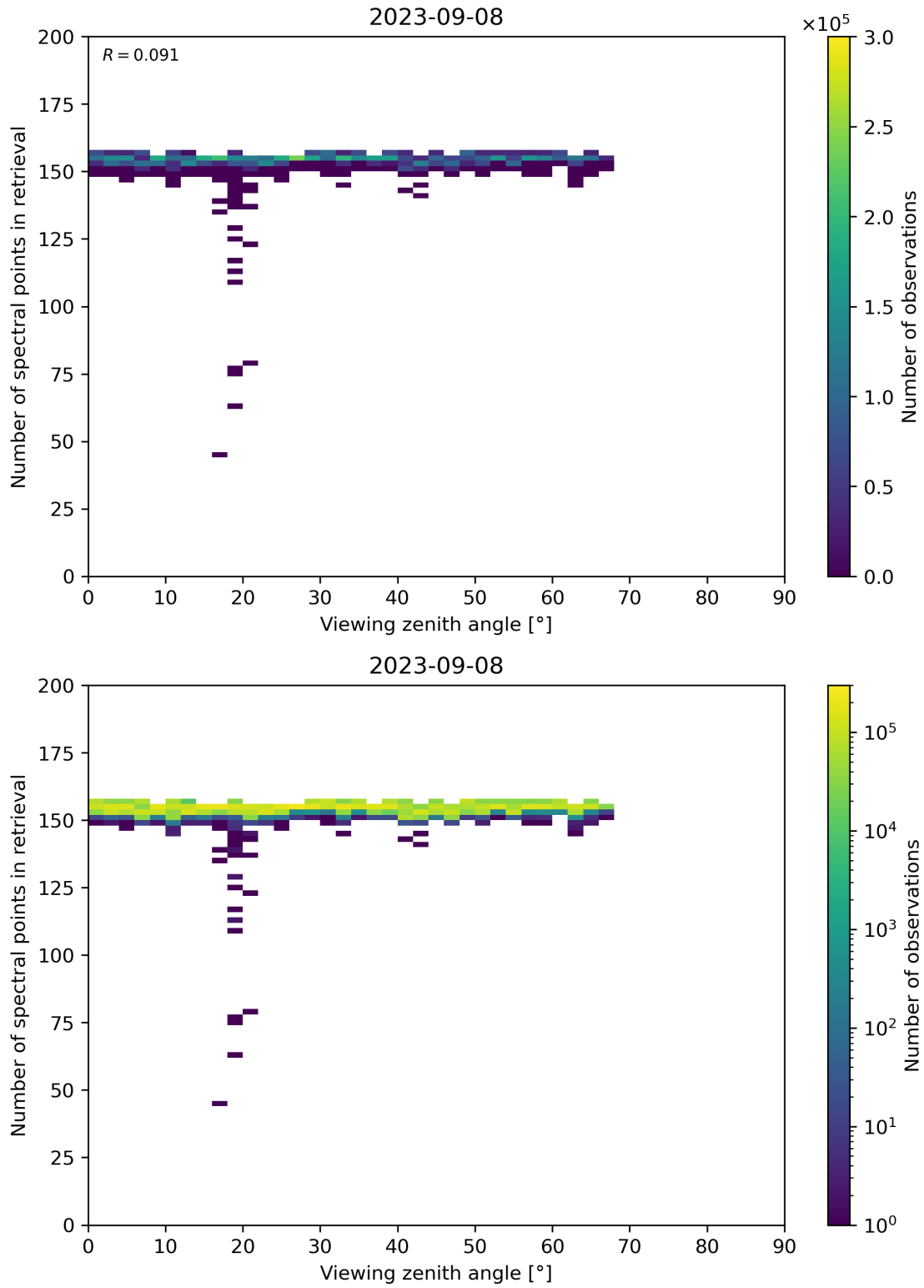
Figure 76: Scatter density plot of “Viewing zenith angle” against “Number of spectral points in retrieval” for 2023-09-07 to 2023-09-09.
