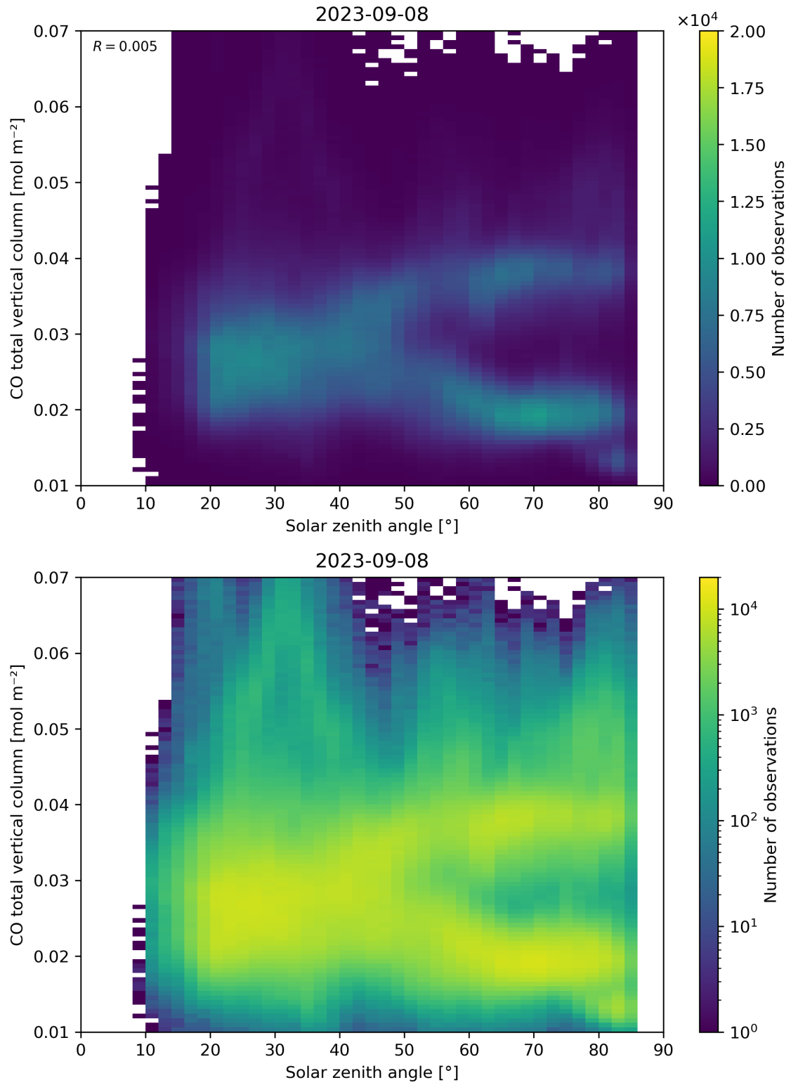
Figure 61: Scatter density plot of “Solar zenith angle” against “CO total vertical column” for 2023-09-07 to 2023-09-09.
