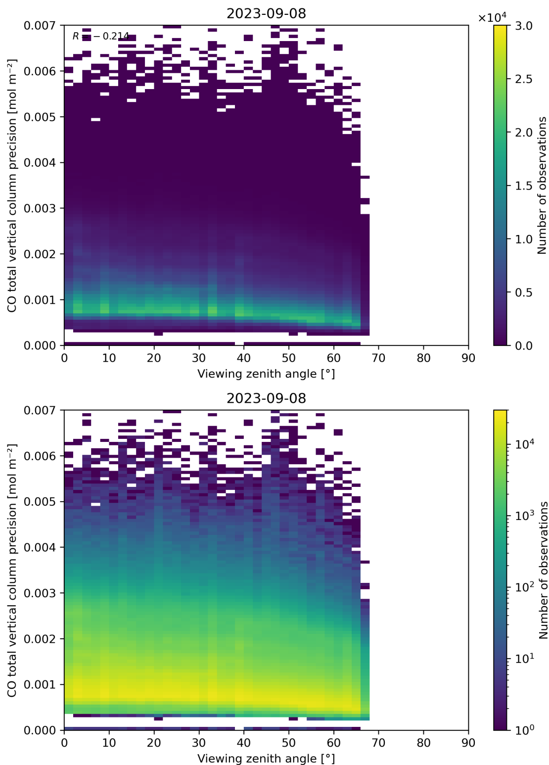
Figure 71: Scatter density plot of “Viewing zenith angle” against “CO total vertical column precision” for 2023-09-07 to 2023-09-09.
