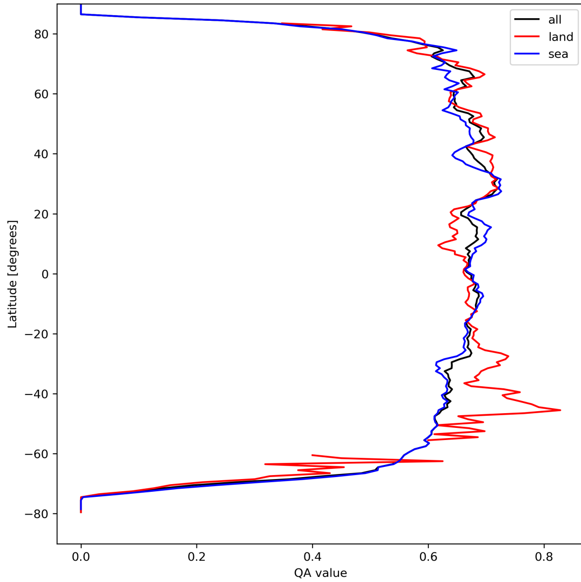
Figure 9: Zonal average of “QA value” for 2023-09-07 to 2023-09-09.
