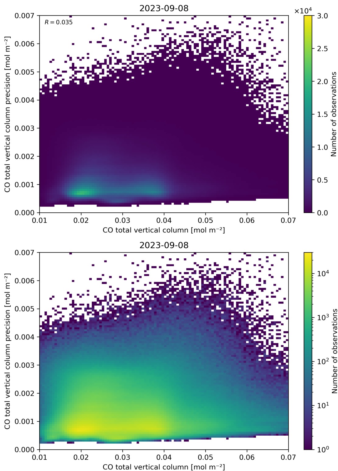
Figure 34: Scatter density plot of “CO total vertical column” against “CO total vertical column precision” for 2023-09-07 to 2023-09-09.
