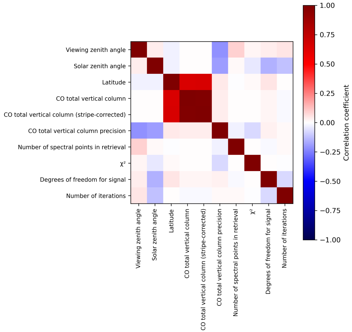
Figure 2: Map of correlation matrix for 2023-09-07 to 2023-09-09.
