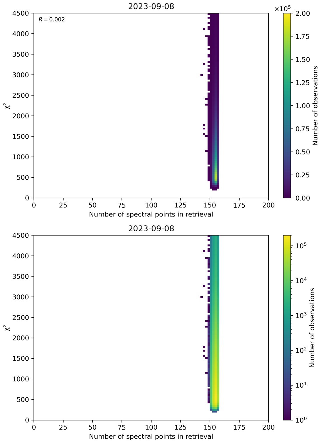
Figure 58: Scatter density plot of “Number of spectral points in retrieval” against “ \chi^2 ” for 2023-09-07 to 2023-09-09.
