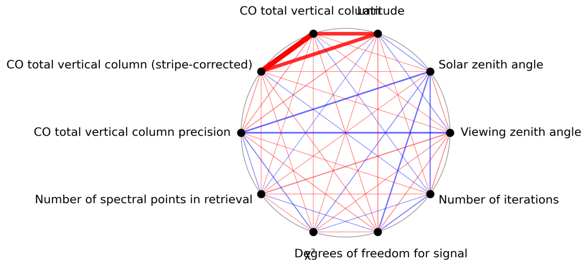
Figure 1: Map of correlation graph for 2023-09-07 to 2023-09-09.
