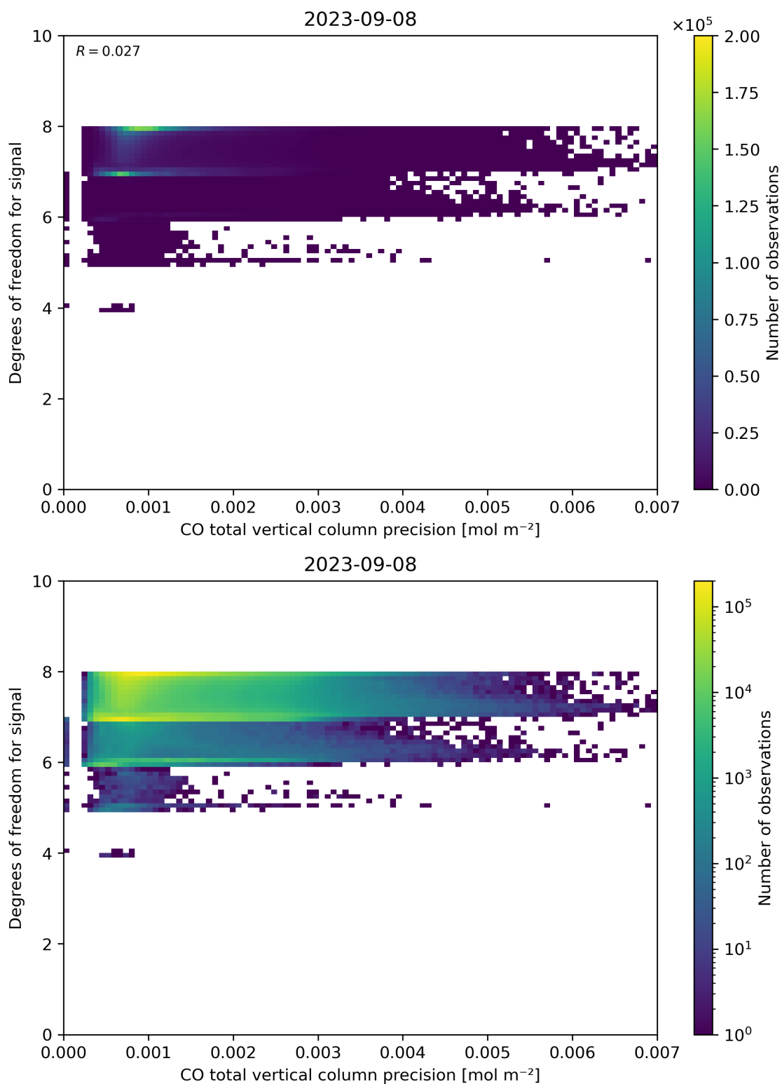
Figure 45: Scatter density plot of “CO total vertical column precision” against “Degrees of freedom for signal” for 2023-09-07 to 2023-09-09.
