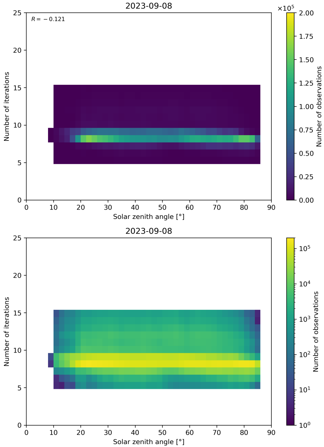
Figure 67: Scatter density plot of “Solar zenith angle” against “Number of iterations” for 2023-09-07 to 2023-09-09.
