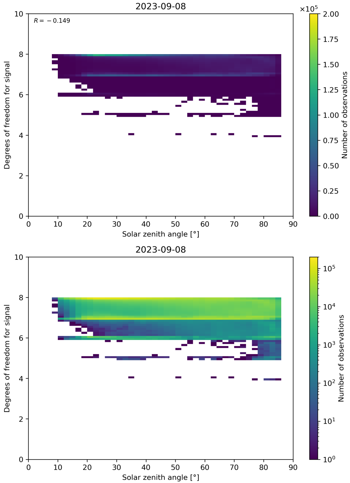
Figure 65: Scatter density plot of “Solar zenith angle” against “Degrees of freedom for signal” for 2023-09-07 to 2023-09-09.
