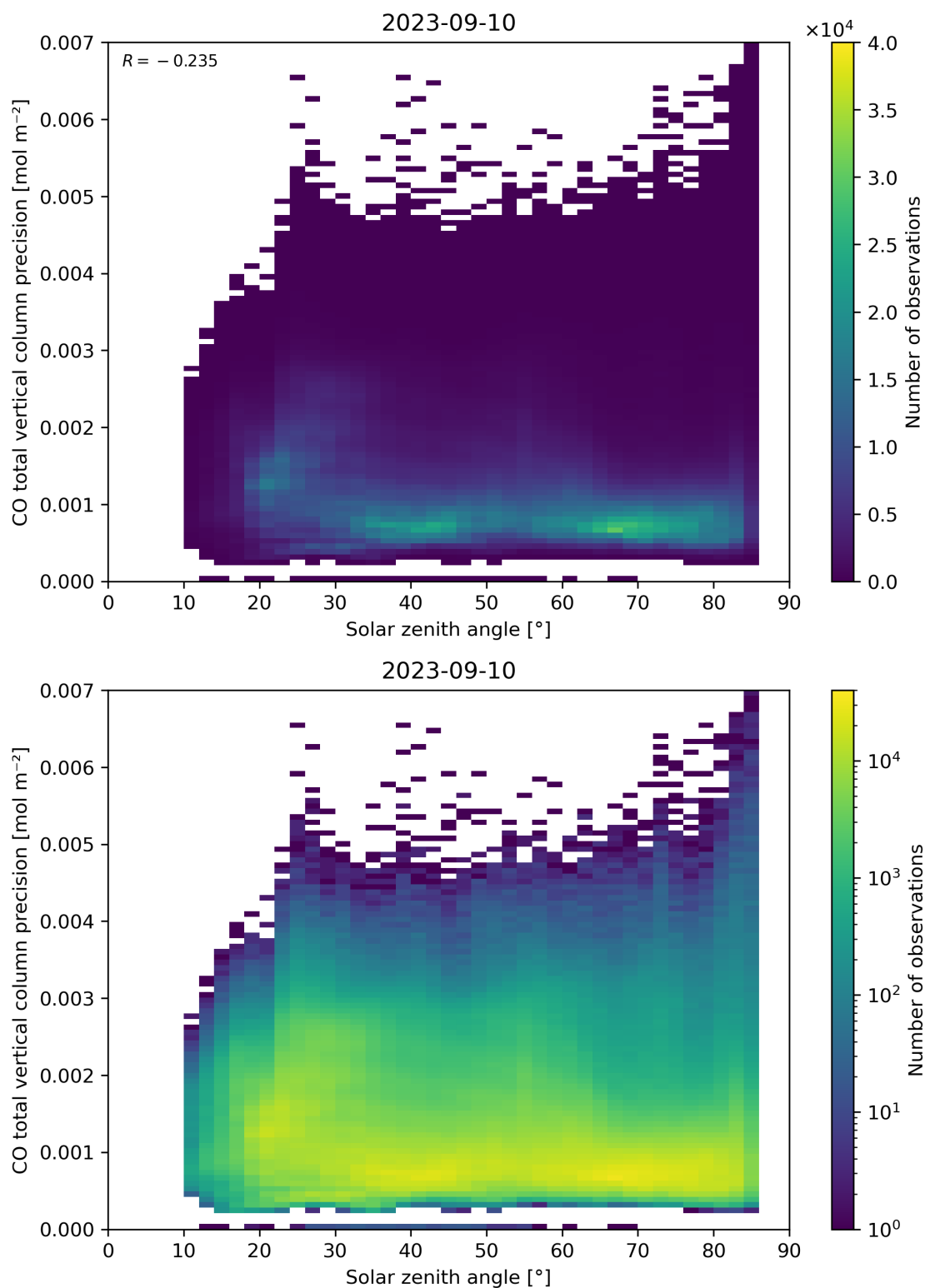
Figure 63: Scatter density plot of “Solar zenith angle” against “CO total vertical column precision” for 2023-09-10 to 2023-09-11.
