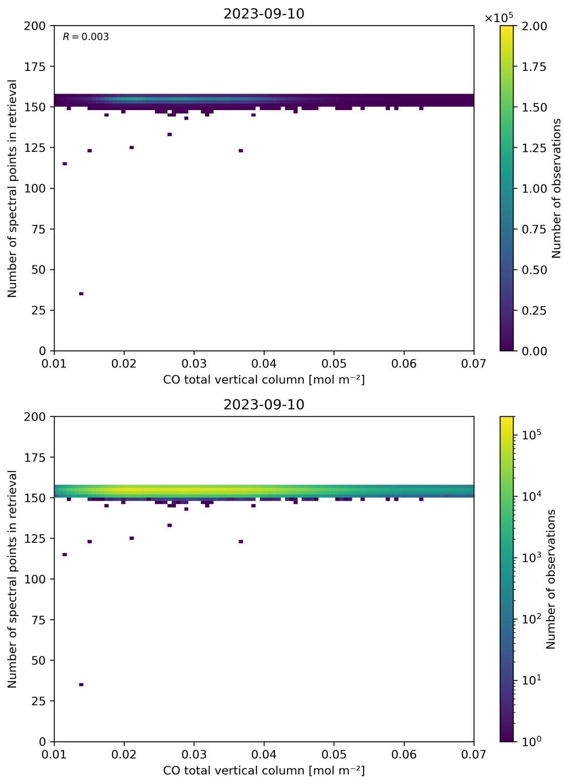
Figure 43: Scatter density plot of “CO total vertical column” against “Number of spectral points in retrieval” for 2023-09-10 to 2023-09-11.
