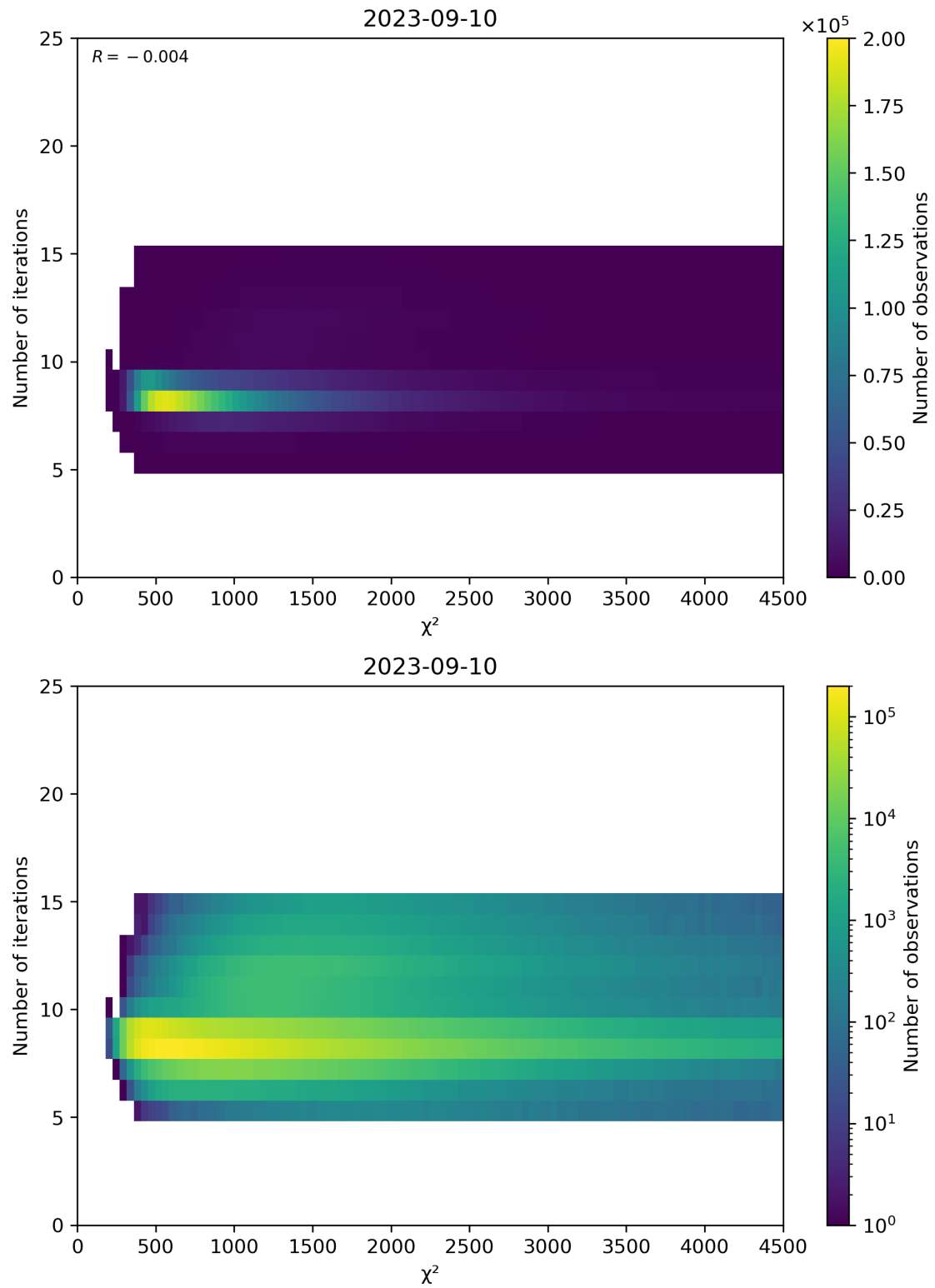
Figure 49: Scatter density plot of “ \chi^2 ” against “Number of iterations” for 2023-09-10 to 2023-09-11.
