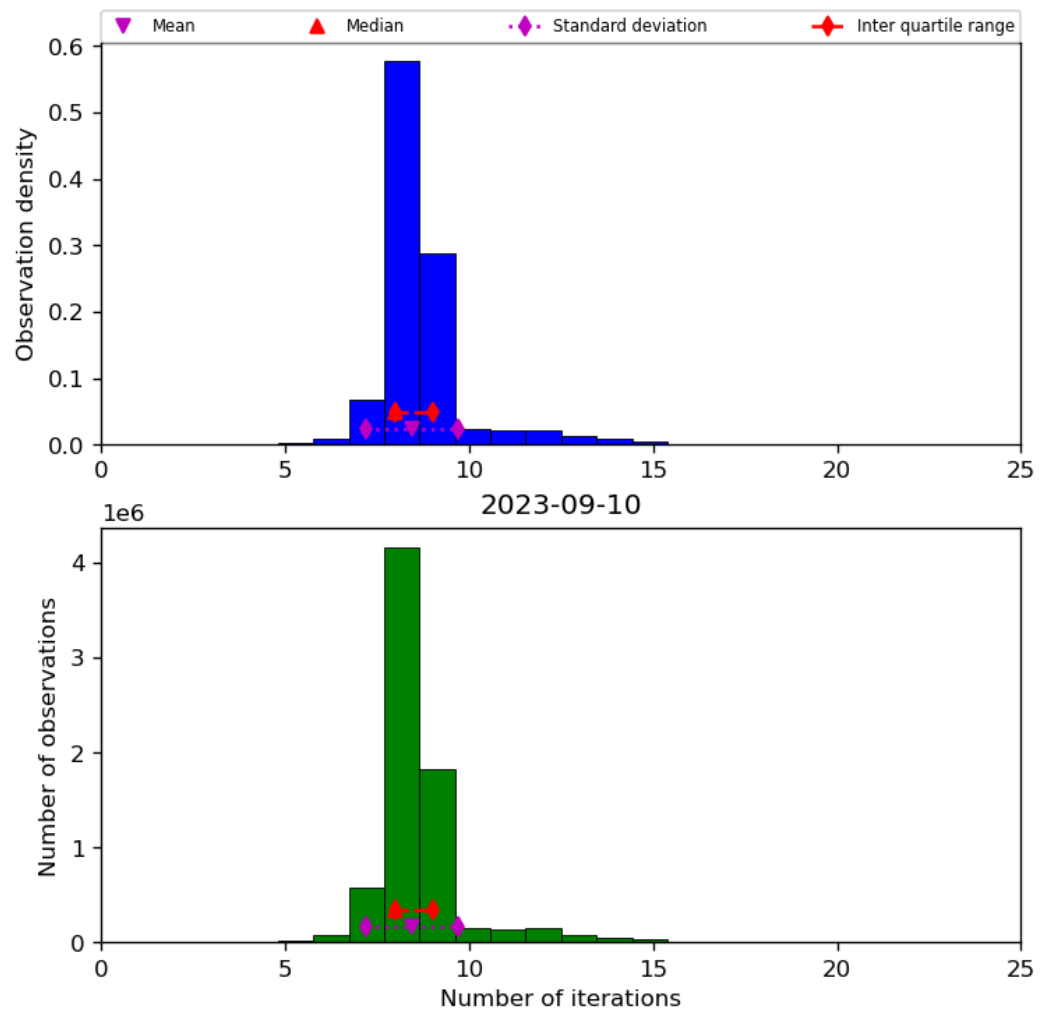
Figure 24: Histogram of “Number of iterations” for 2023-09-10 to 2023-09-11
