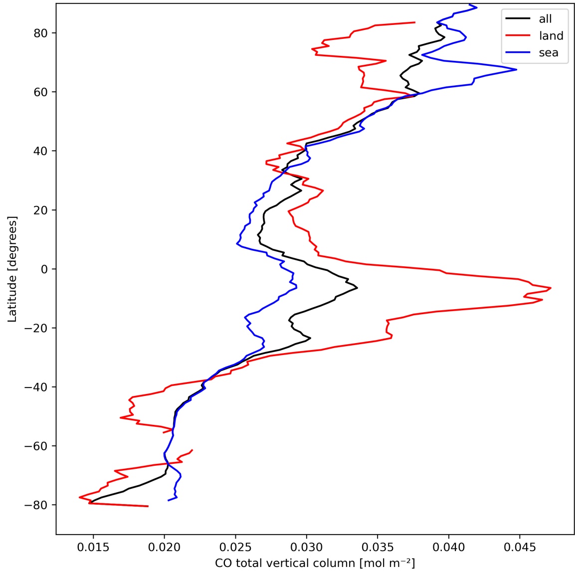
Figure 10: Zonal average of “CO total vertical column” for 2023-09-10 to 2023-09-11.
