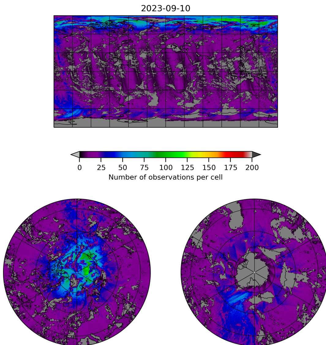
Figure 8: Map of the number of observations for 2023-09-10 to 2023-09-11
