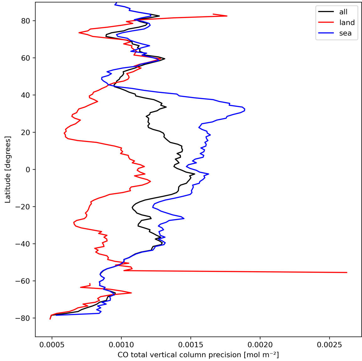
Figure 12: Zonal average of “CO total vertical column precision” for 2023-09-10 to 2023-09-11.
