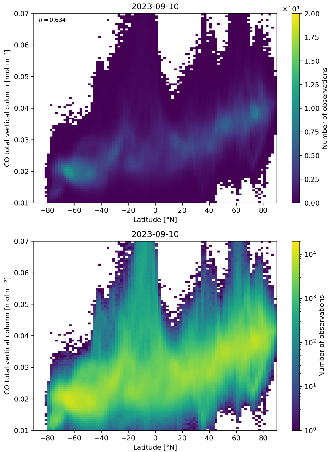
Figure 51: Scatter density plot of “Latitude” against “CO total vertical column” for 2023-09-10 to 2023-09-11.
