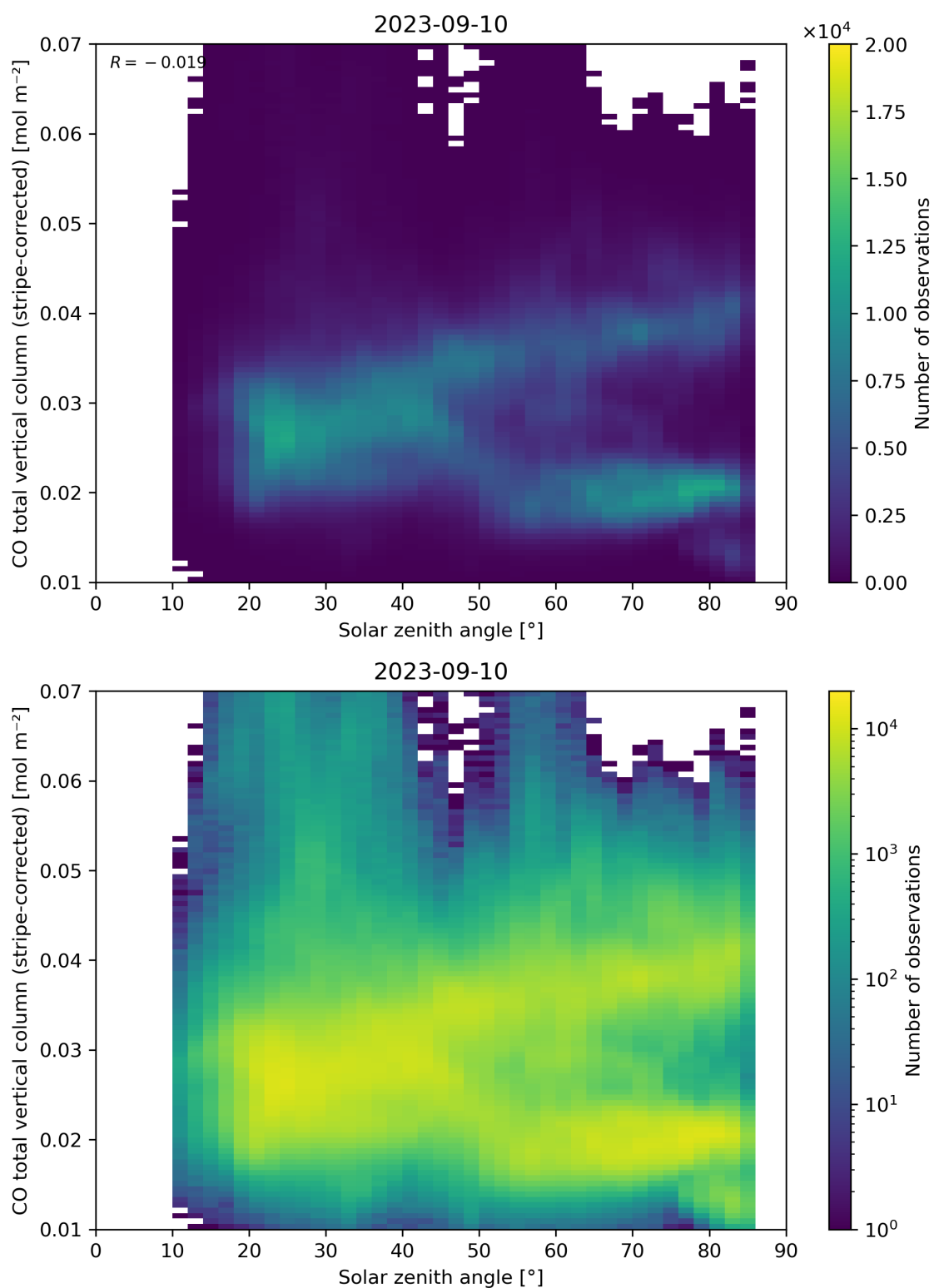
Figure 62: Scatter density plot of “Solar zenith angle” against “CO total vertical column (stripe-corrected)” for 2023-09-10 to 2023-09-11.
