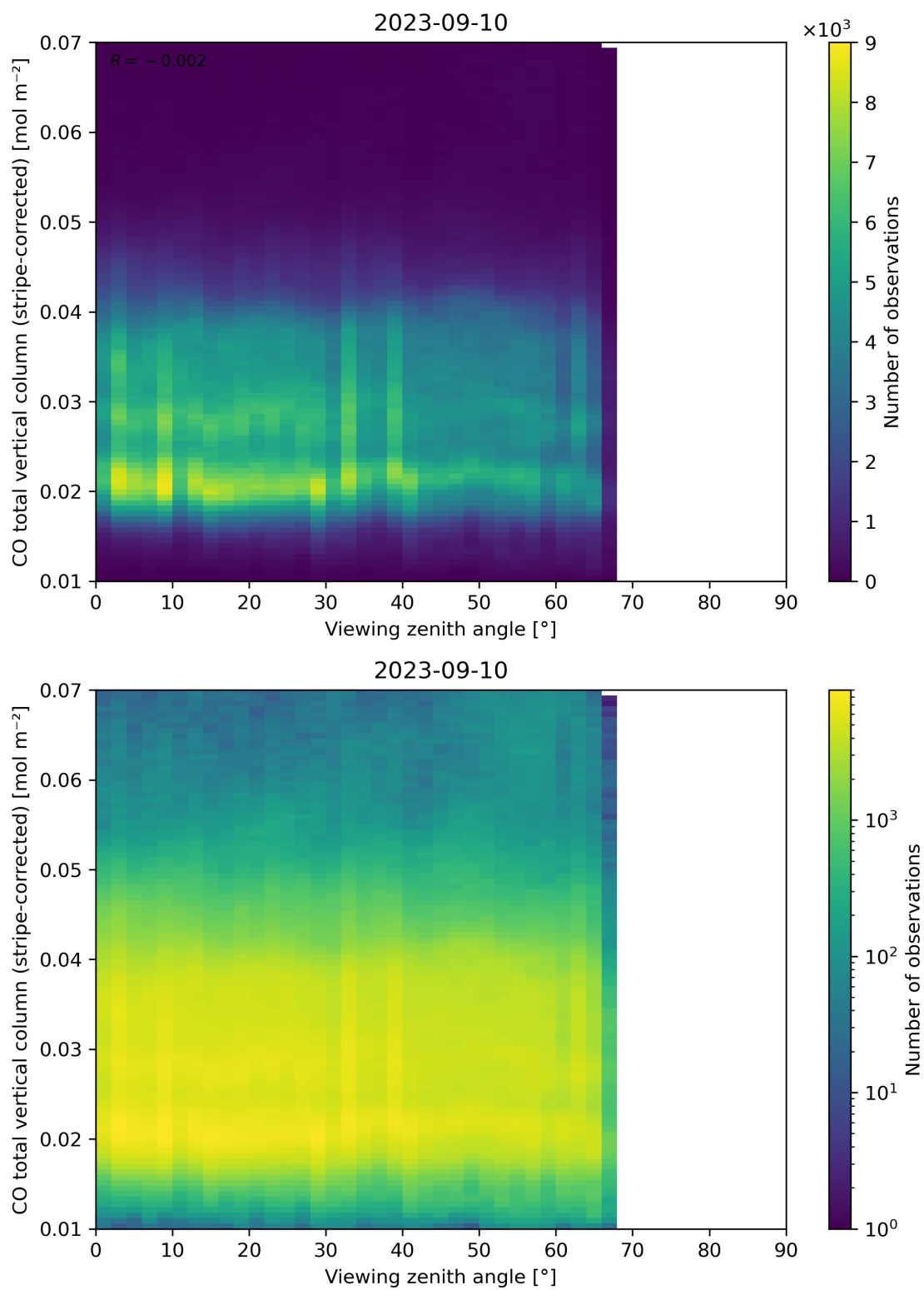
Figure 70: Scatter density plot of “Viewing zenith angle” against “CO total vertical column (stripe-corrected)” for 2023-09-10 to 2023-09-11.
