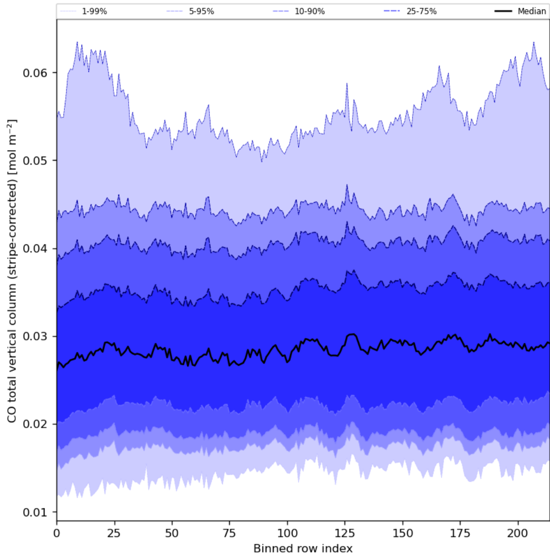
Figure 27: Along track statistics of “CO total vertical column (stripe-corrected)” for 2023-09-10 to 2023-09-11
