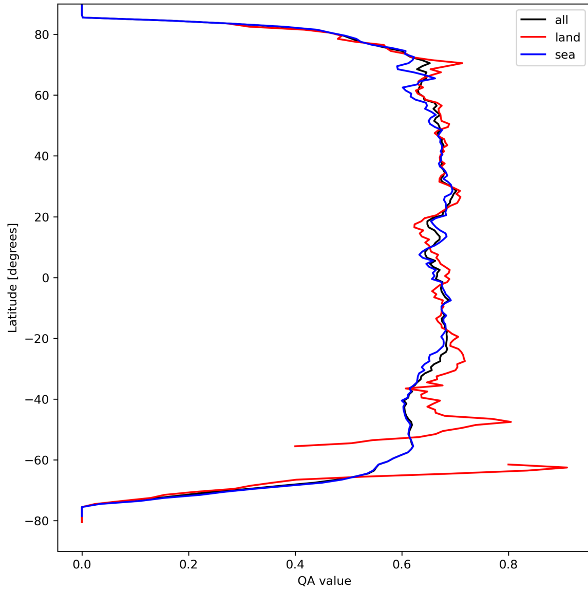
Figure 9: Zonal average of “QA value” for 2023-09-10 to 2023-09-11.
