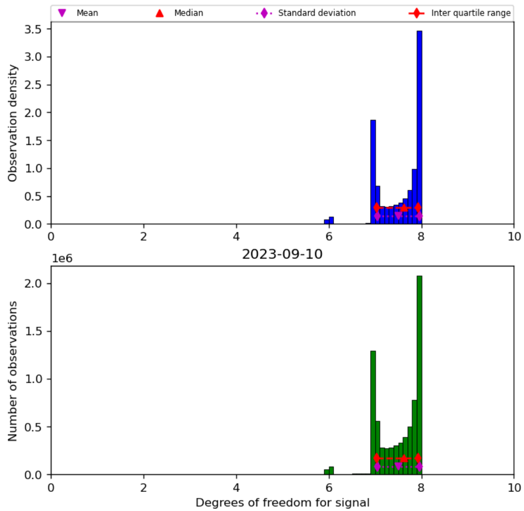
Figure 23: Histogram of “Degrees of freedom for signal” for 2023-09-10 to 2023-09-11
