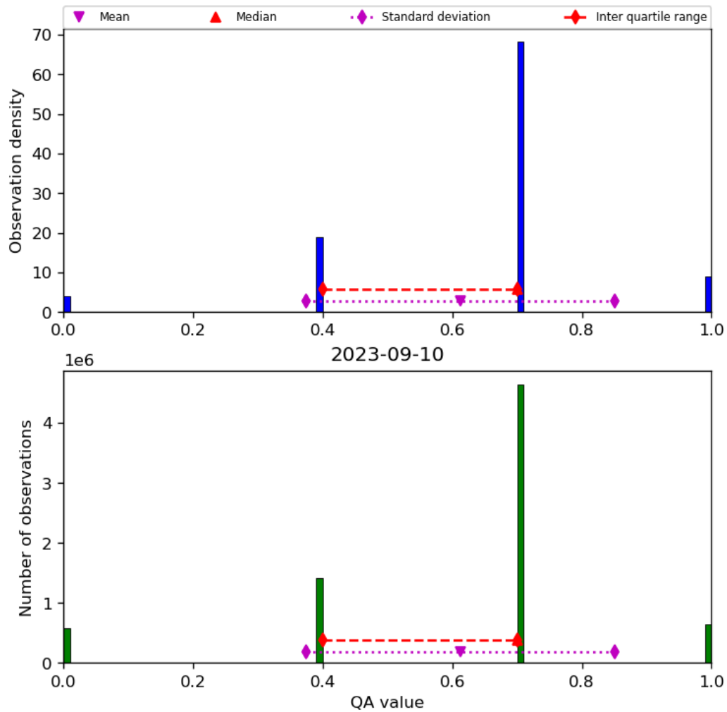
Figure 17: Histogram of “QA value” for 2023-09-10 to 2023-09-11
