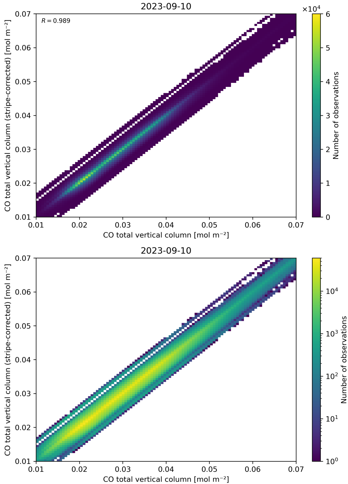
Figure 33: Scatter density plot of “CO total vertical column” against “CO total vertical column (stripe-corrected)” for 2023-09-10 to 2023-09-11.
