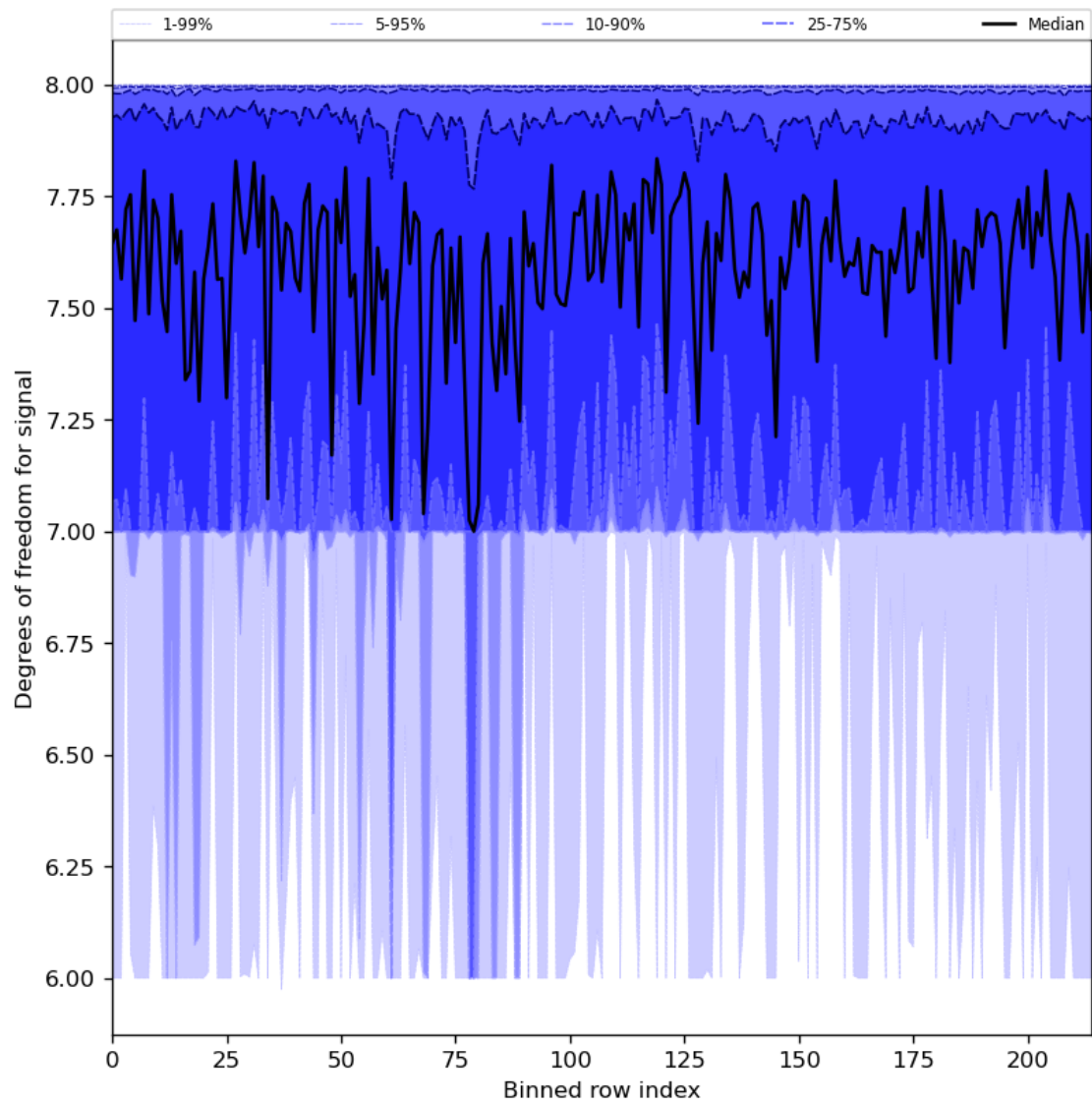
Figure 31: Along track statistics of “Degrees of freedom for signal” for 2023-09-10 to 2023-09-11
