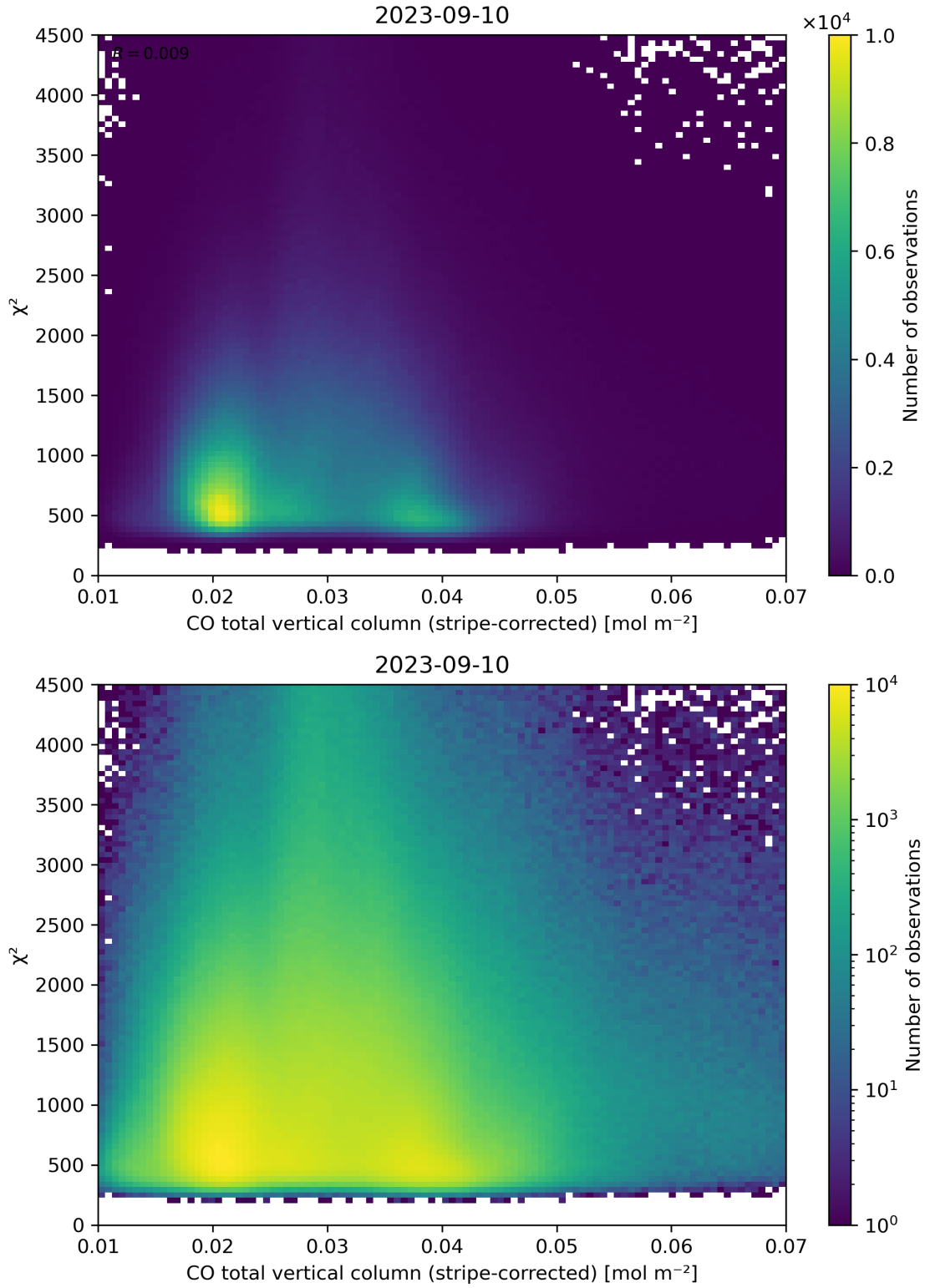
Figure 37: Scatter density plot of “CO total vertical column (stripe-corrected)” against “ \chi^2 ” for 2023-09-10 to 2023-09-11.
