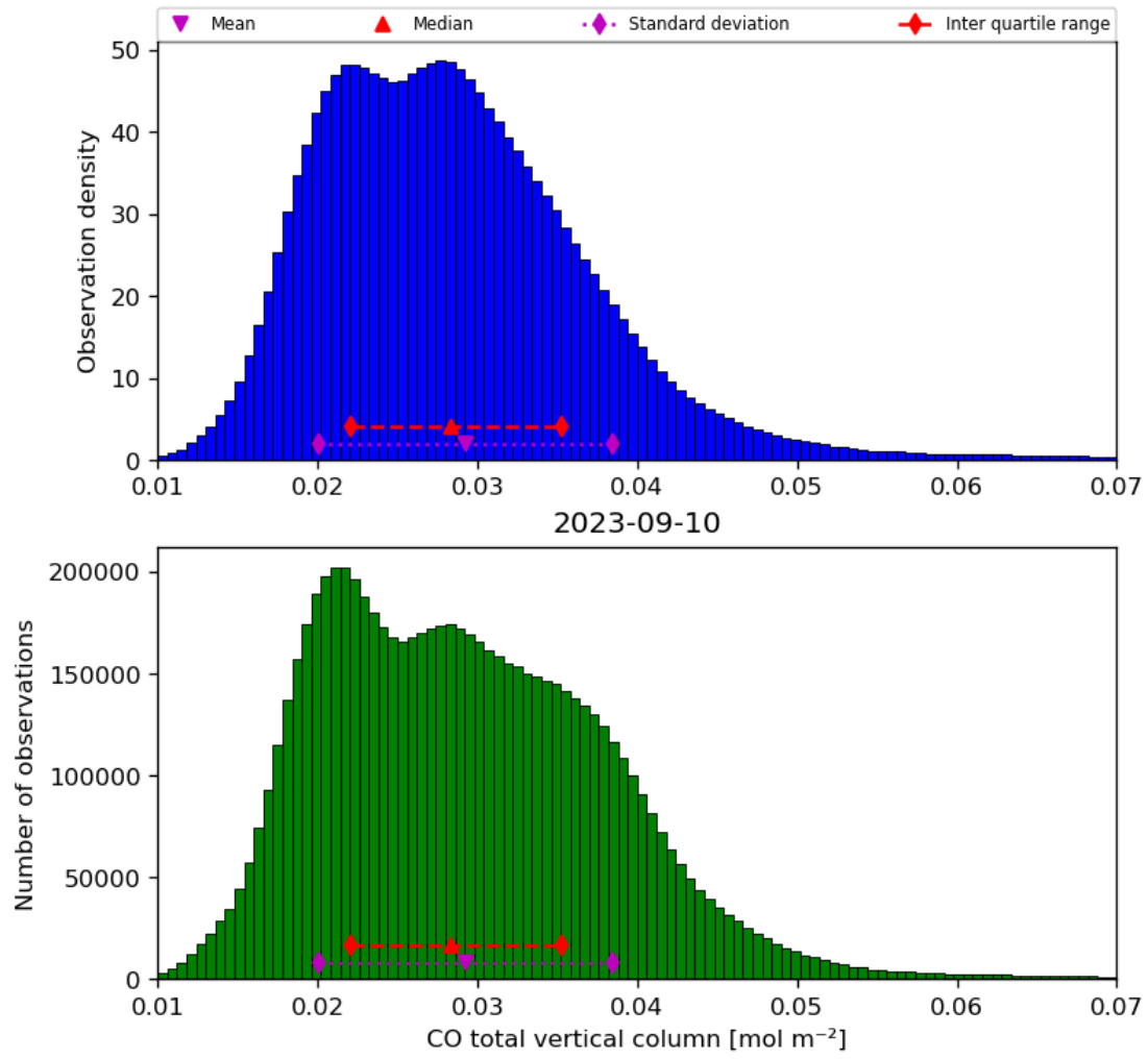
Figure 18: Histogram of “CO total vertical column” for 2023-09-10 to 2023-09-11
