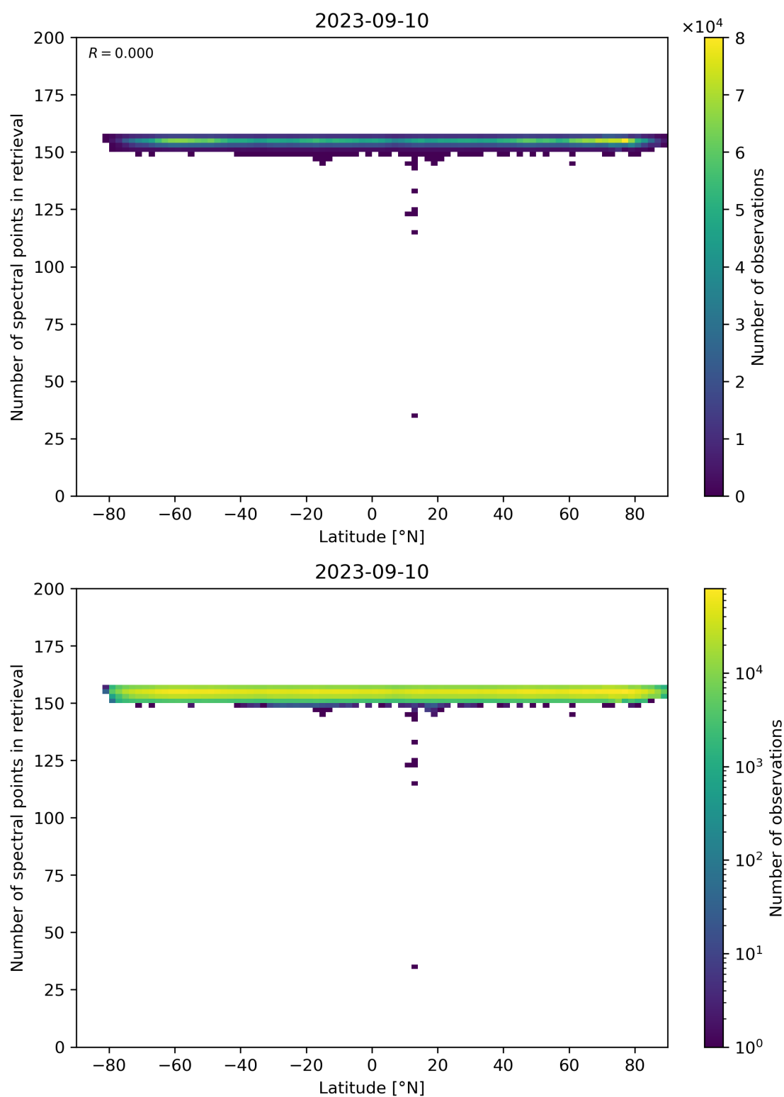
Figure 57: Scatter density plot of “Latitude” against “Number of spectral points in retrieval” for 2023-09-10 to 2023-09-11.
