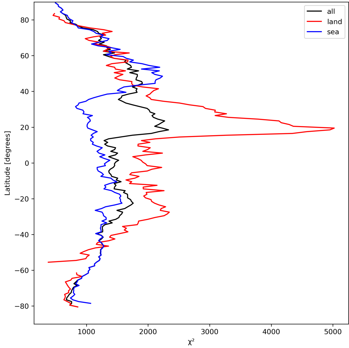
Figure 14: Zonal average of “ \chi^2 ” for 2023-09-10 to 2023-09-11.
