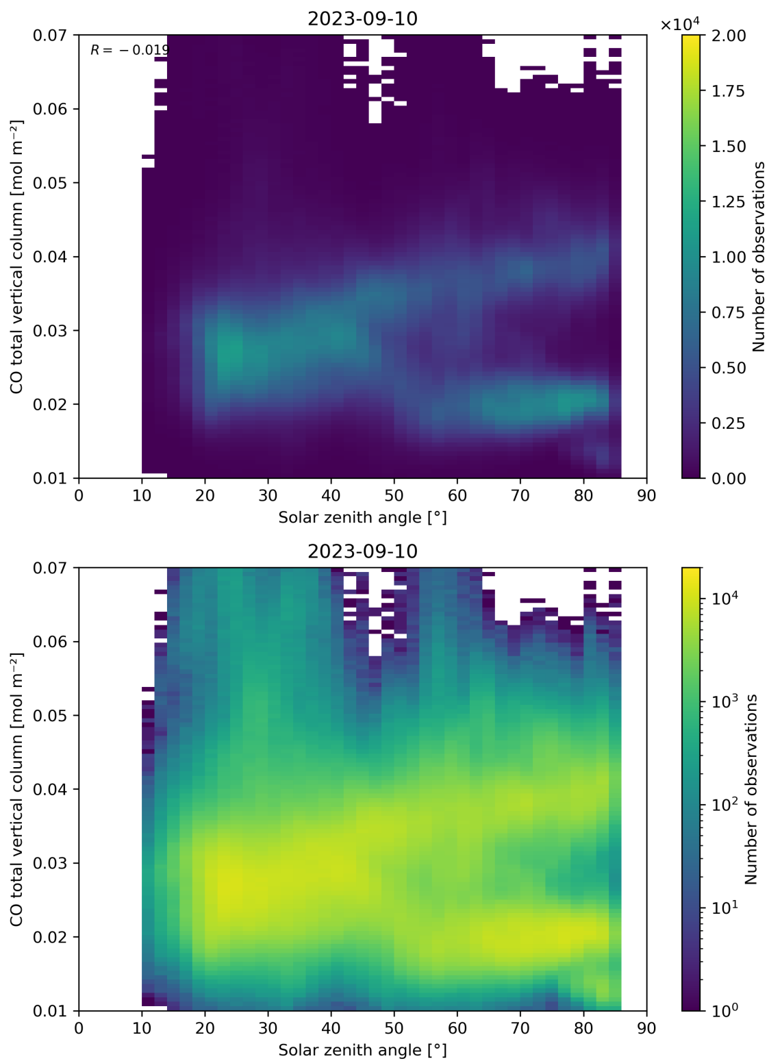
Figure 61: Scatter density plot of “Solar zenith angle” against “CO total vertical column” for 2023-09-10 to 2023-09-11.
