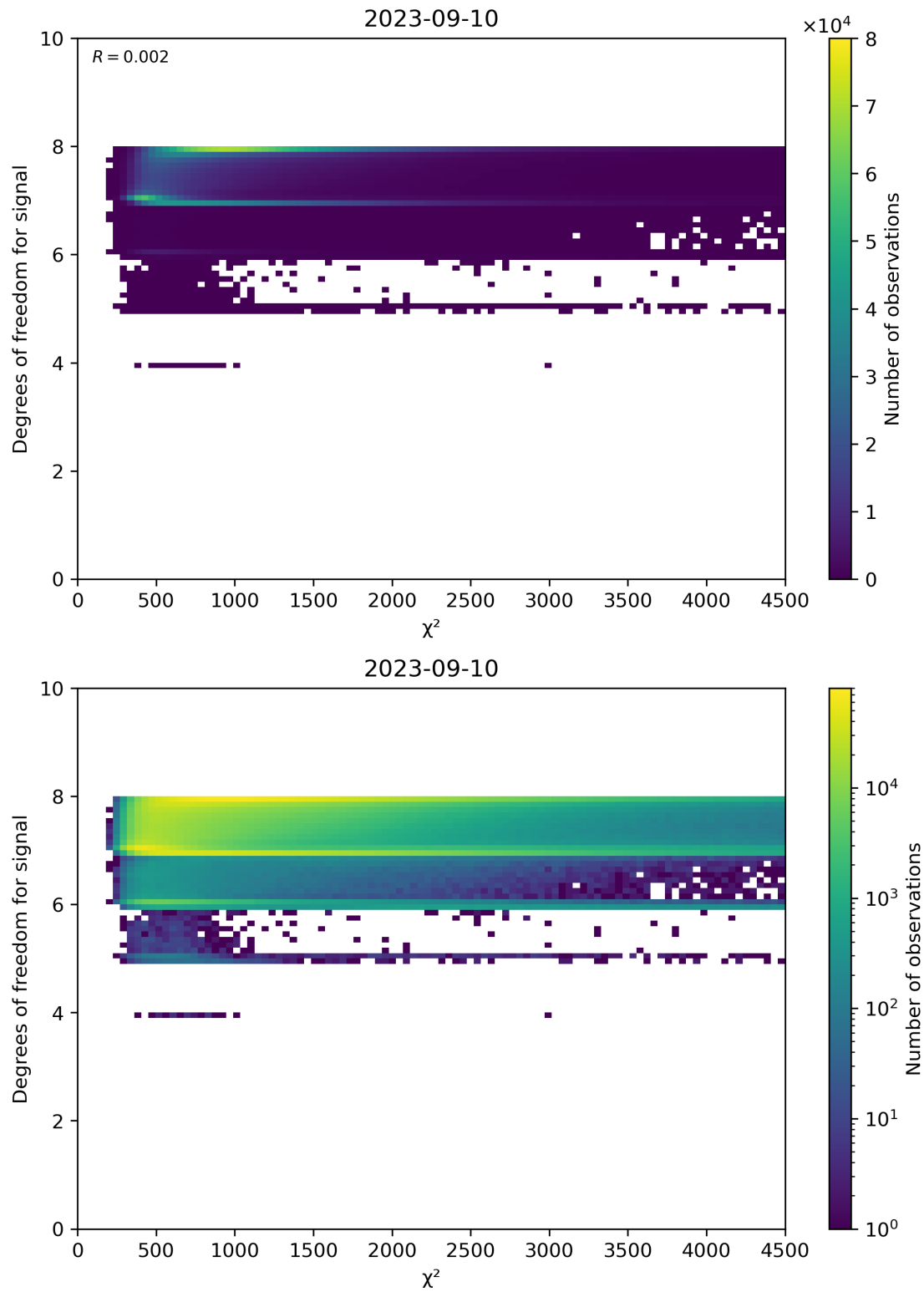
Figure 48: Scatter density plot of " \chi^2 " against "Degrees of freedom for signal" for 2023-09-10 to 2023-09-11.
