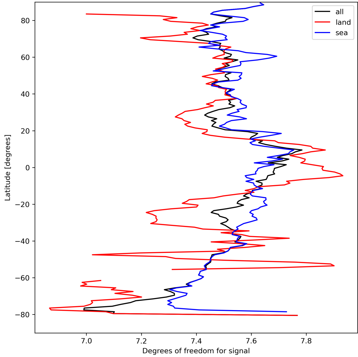
Figure 15: Zonal average of “Degrees of freedom for signal” for 2023-09-10 to 2023-09-11.
