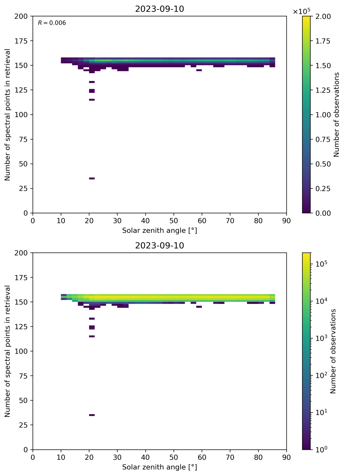
Figure 68: Scatter density plot of “Solar zenith angle” against “Number of spectral points in retrieval” for 2023-09-10 to 2023-09-11.
