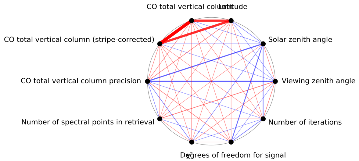
Figure 1: Map of correlation graph for 2023-09-10 to 2023-09-11.
