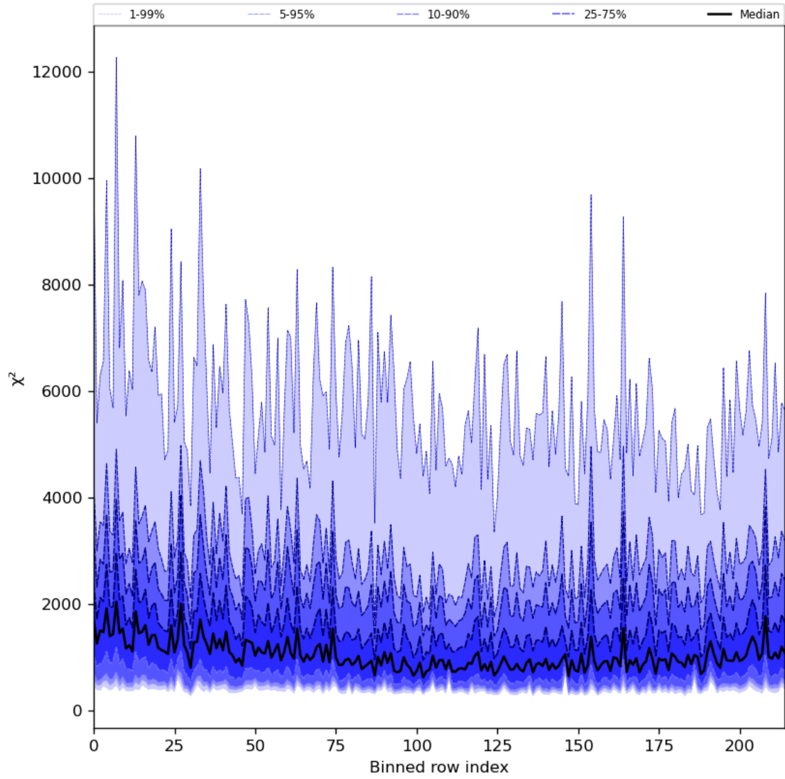
Figure 30: Along track statistics of “ \chi^2 ” for 2023-09-10 to 2023-09-11
