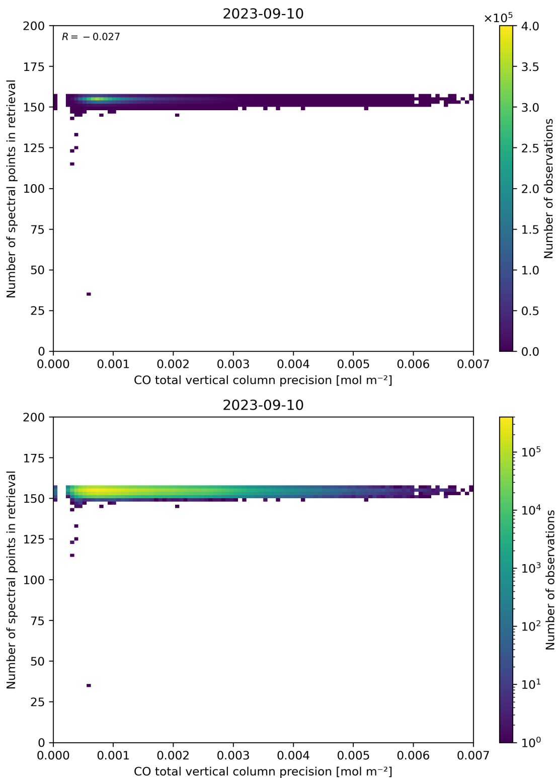
Figure 47: Scatter density plot of “CO total vertical column precision” against “Number of spectral points in retrieval” for 2023-09-10 to 2023-09-11.
