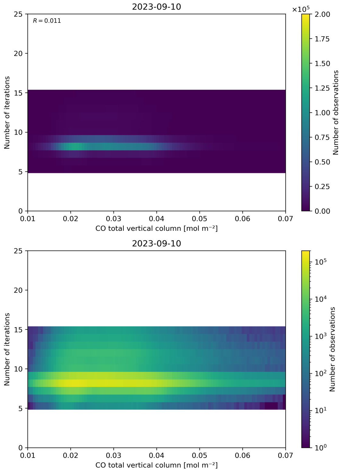
Figure 42: Scatter density plot of “CO total vertical column” against “Number of iterations” for 2023-09-10 to 2023-09-11.
