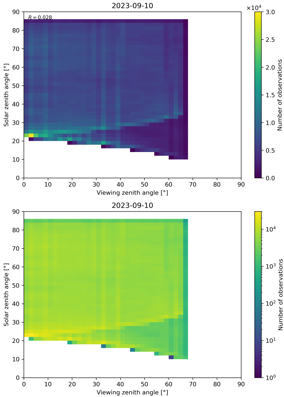
Figure 77: Scatter density plot of “Viewing zenith angle” against “Solar zenith angle” for 2023-09-10 to 2023-09-11.
