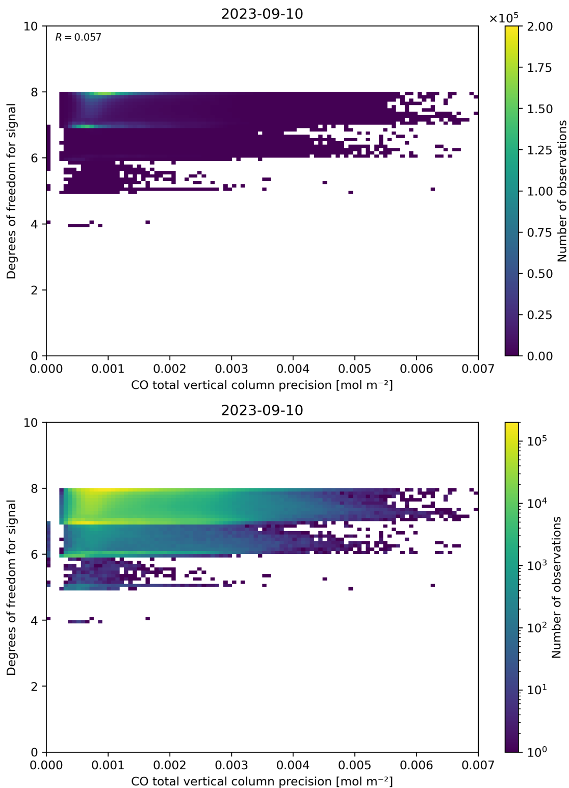
Figure 45: Scatter density plot of “CO total vertical column precision” against “Degrees of freedom for signal” for 2023-09-10 to 2023-09-11.
