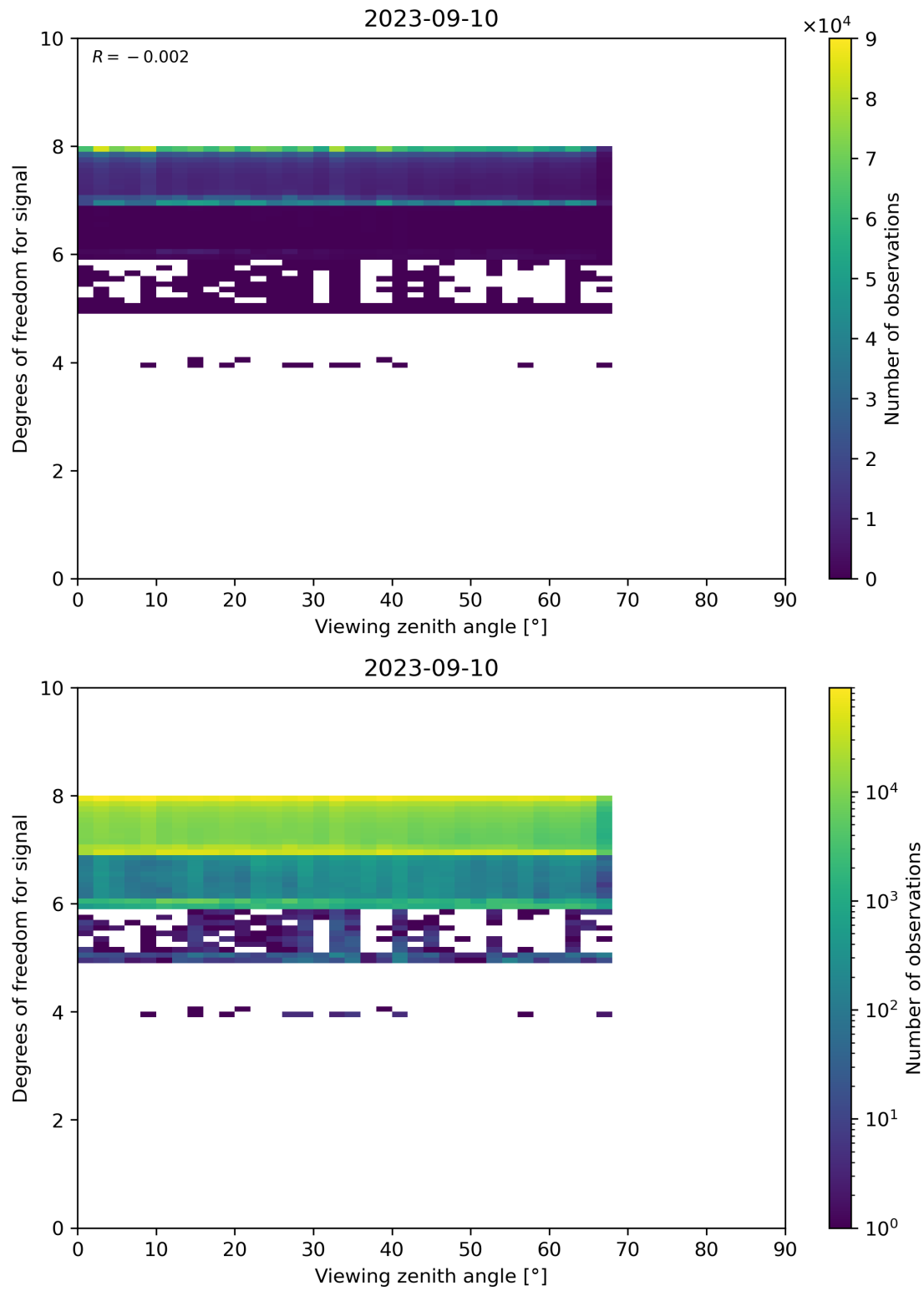
Figure 73: Scatter density plot of “Viewing zenith angle” against “Degrees of freedom for signal” for 2023-09-10 to 2023-09-11.
