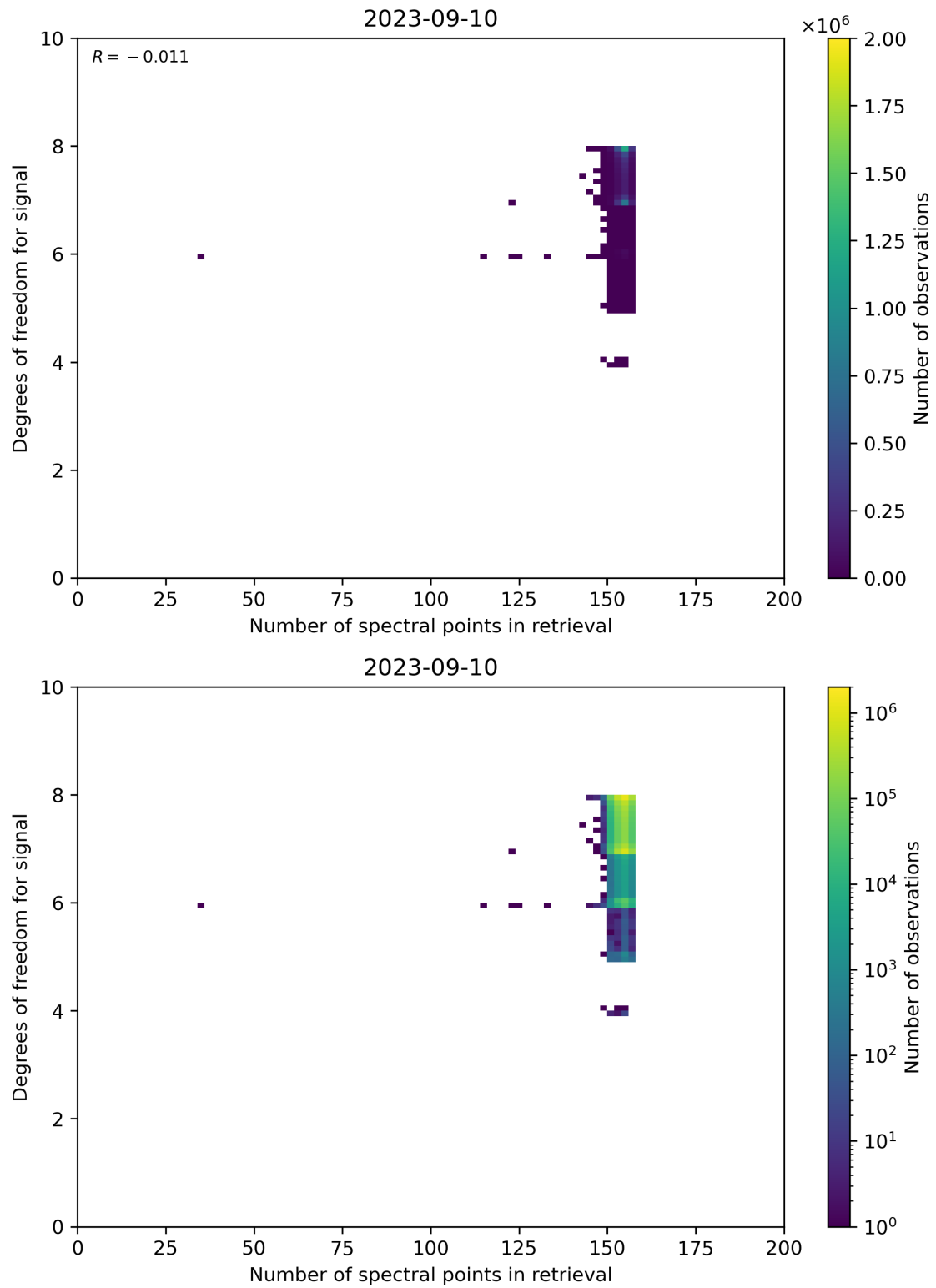
Figure 59: Scatter density plot of “Number of spectral points in retrieval” against “Degrees of freedom for signal” for 2023-09-10 to 2023-09-11.
