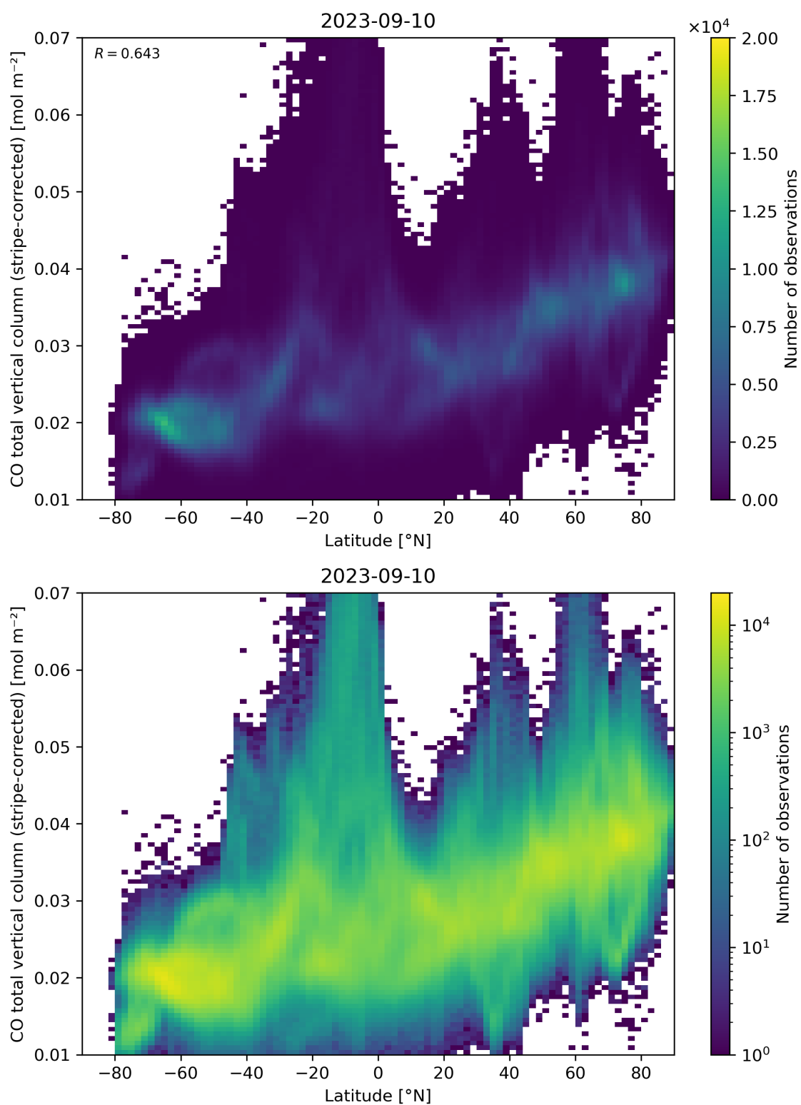
Figure 52: Scatter density plot of “Latitude” against “CO total vertical column (stripe-corrected)” for 2023-09-10 to 2023-09-11.
