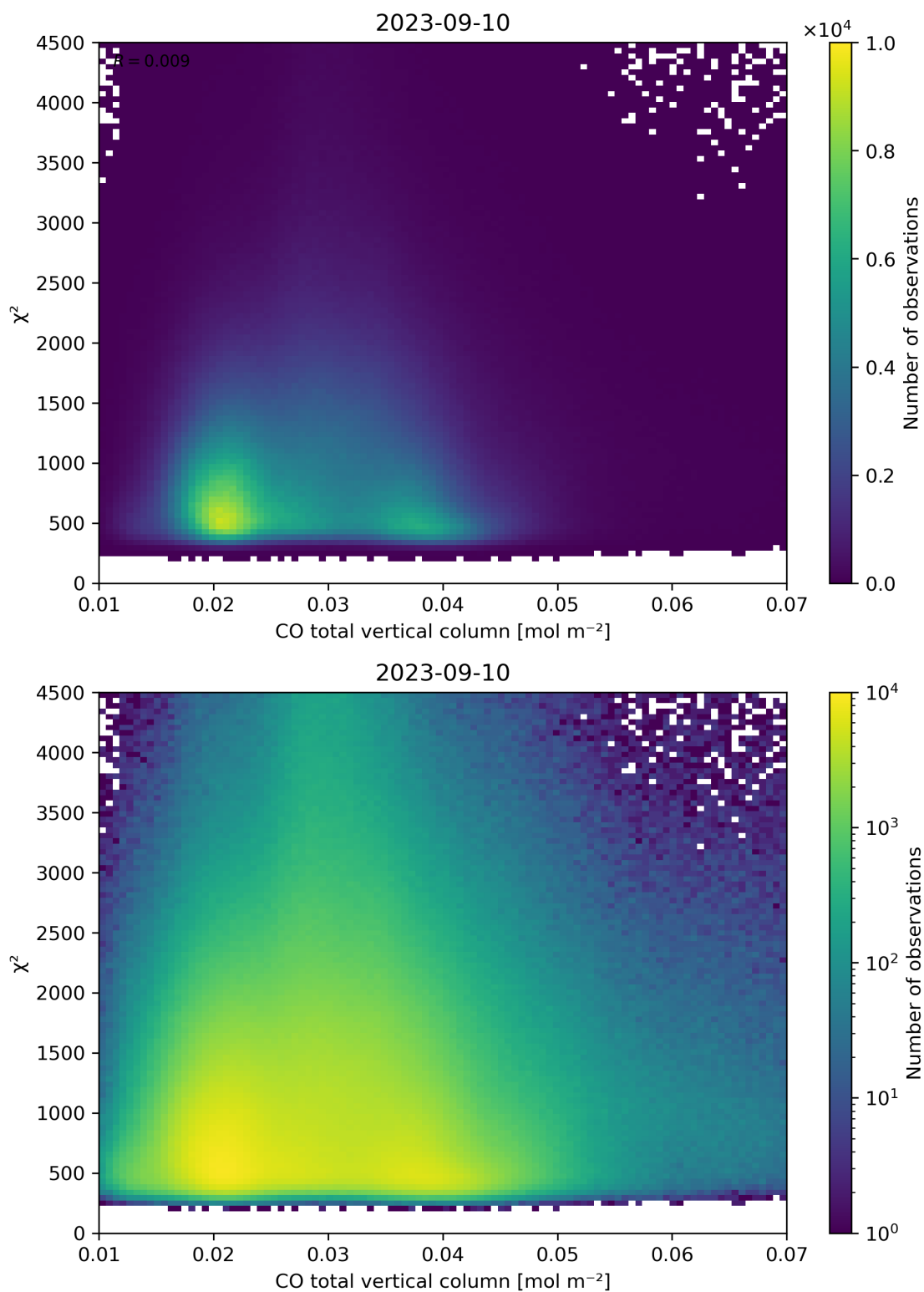
Figure 35: Scatter density plot of “CO total vertical column” against “ \chi^2 ” for 2023-09-10 to 2023-09-11.
