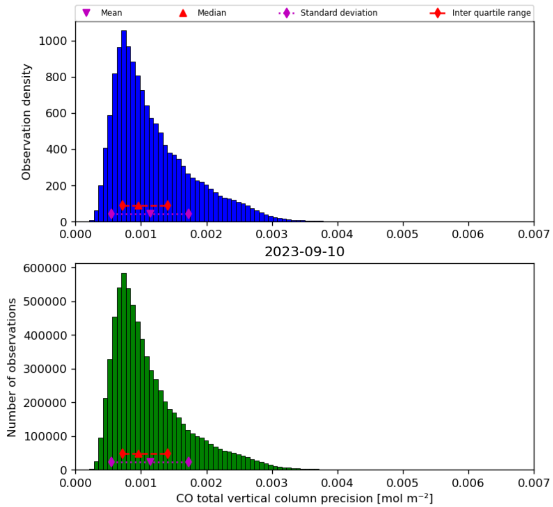
Figure 20: Histogram of “CO total vertical column precision” for 2023-09-10 to 2023-09-11
