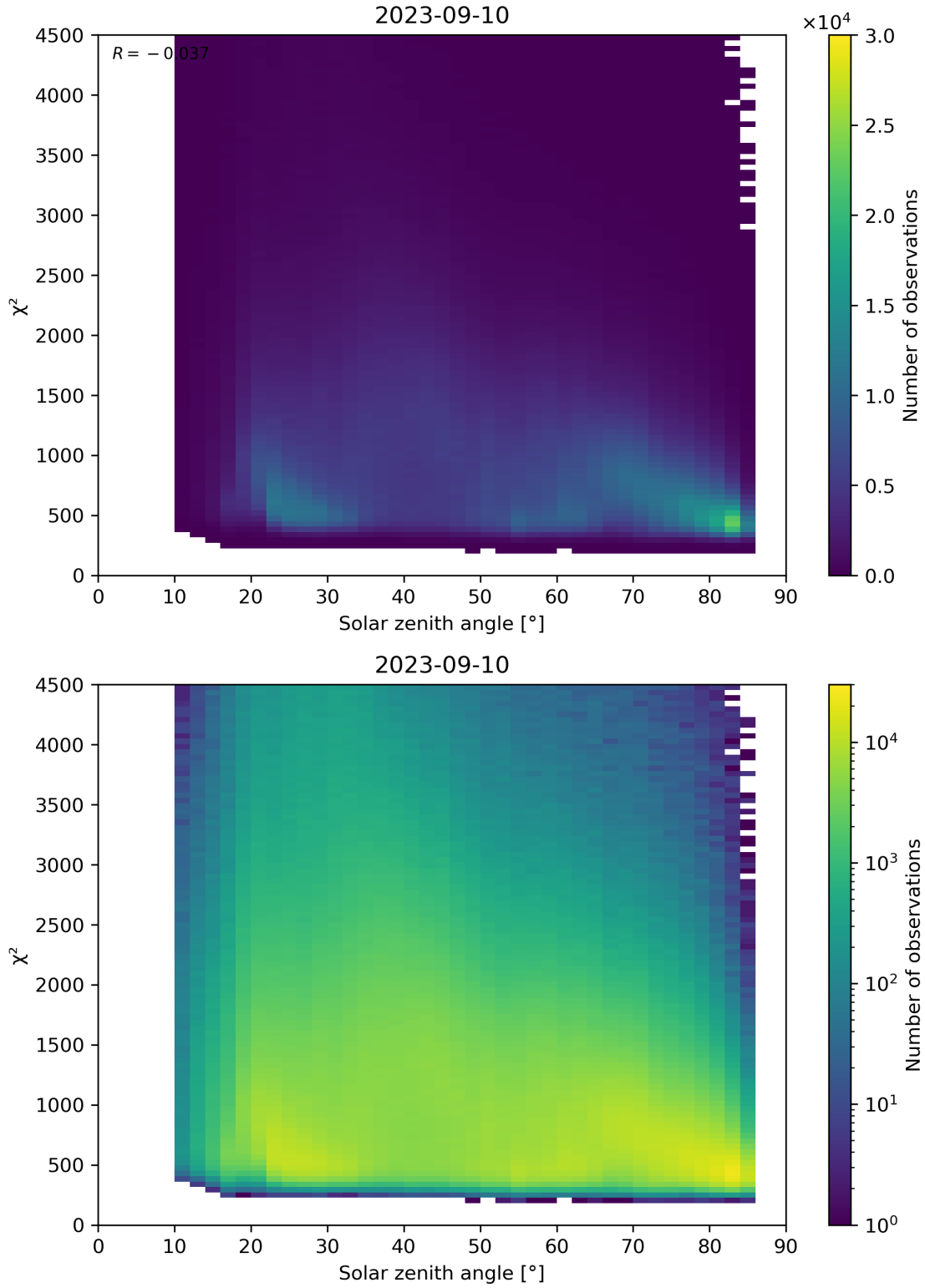
Figure 64: Scatter density plot of “Solar zenith angle” against “ \chi^2 ” for 2023-09-10 to 2023-09-11.
