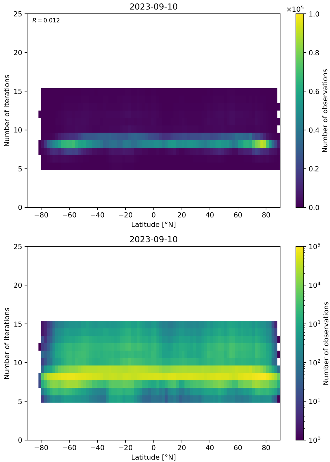
Figure 56: Scatter density plot of “Latitude” against “Number of iterations” for 2023-09-10 to 2023-09-11.
