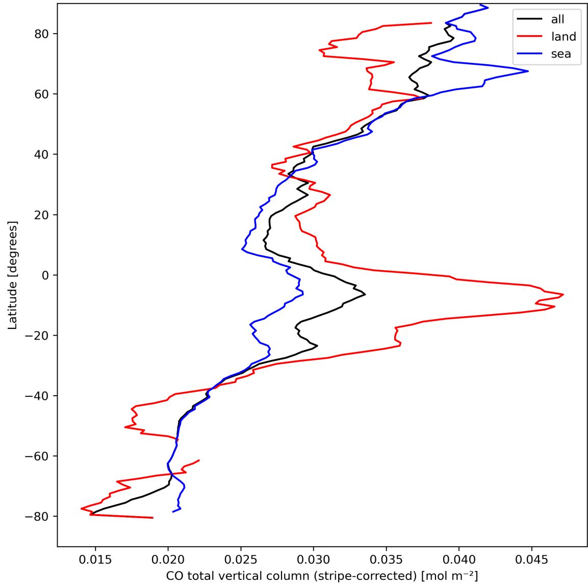
Figure 11: Zonal average of “CO total vertical column (stripe-corrected)” for 2023-09-10 to 2023-09-11.
