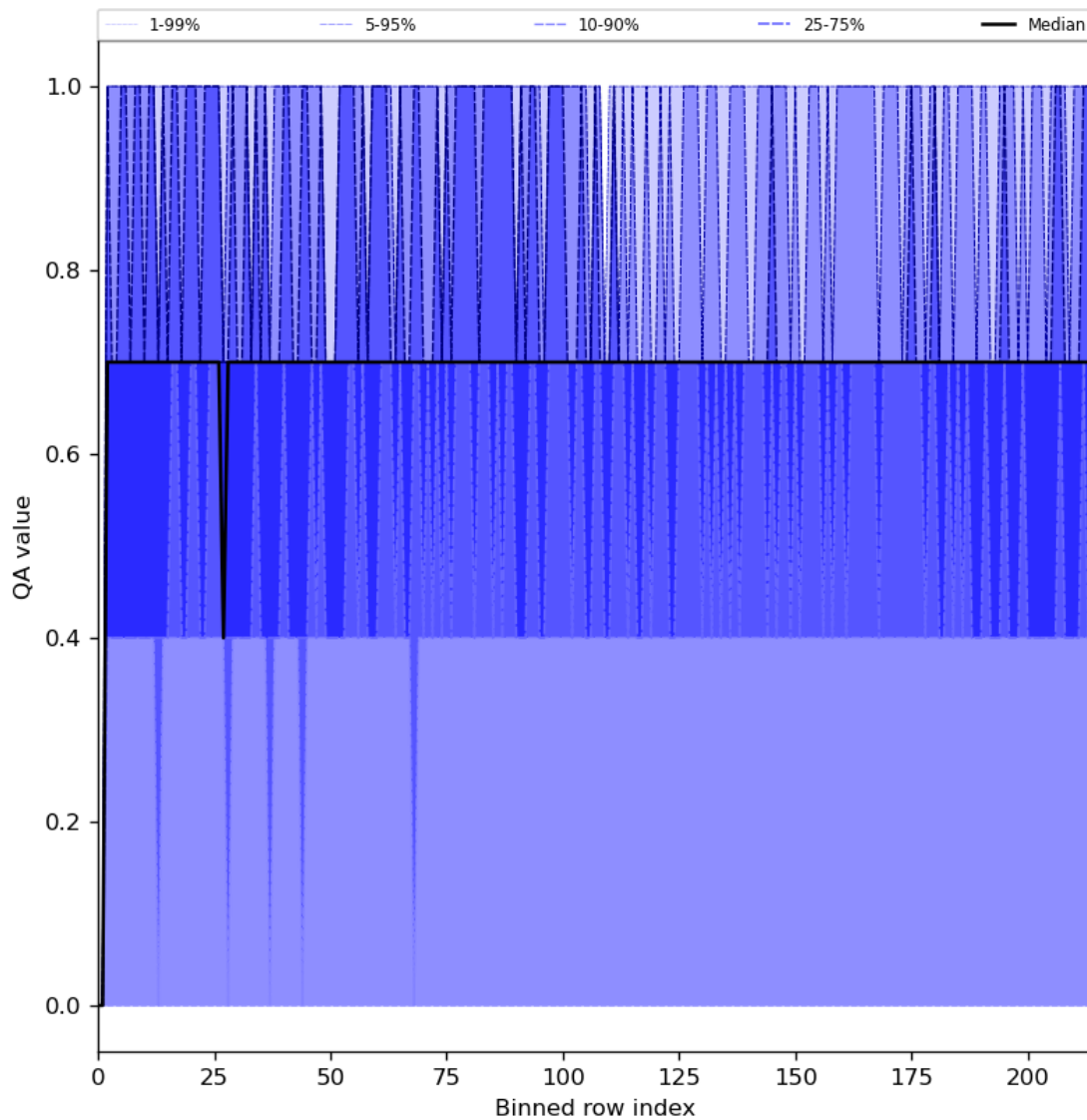
Figure 25: Along track statistics of “QA value” for 2023-09-10 to 2023-09-11
