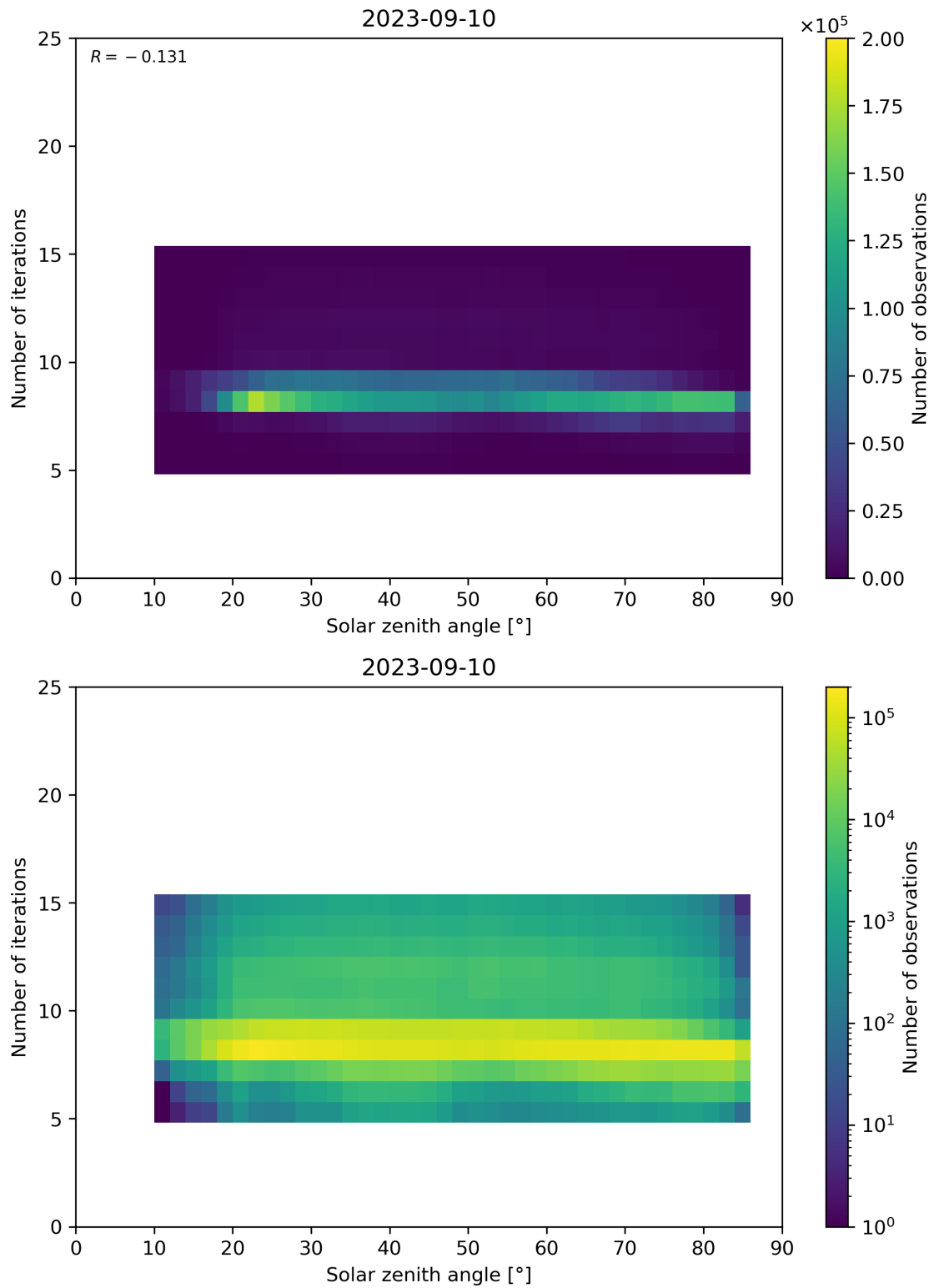
Figure 67: Scatter density plot of “Solar zenith angle” against “Number of iterations” for 2023-09-10 to 2023-09-11.
