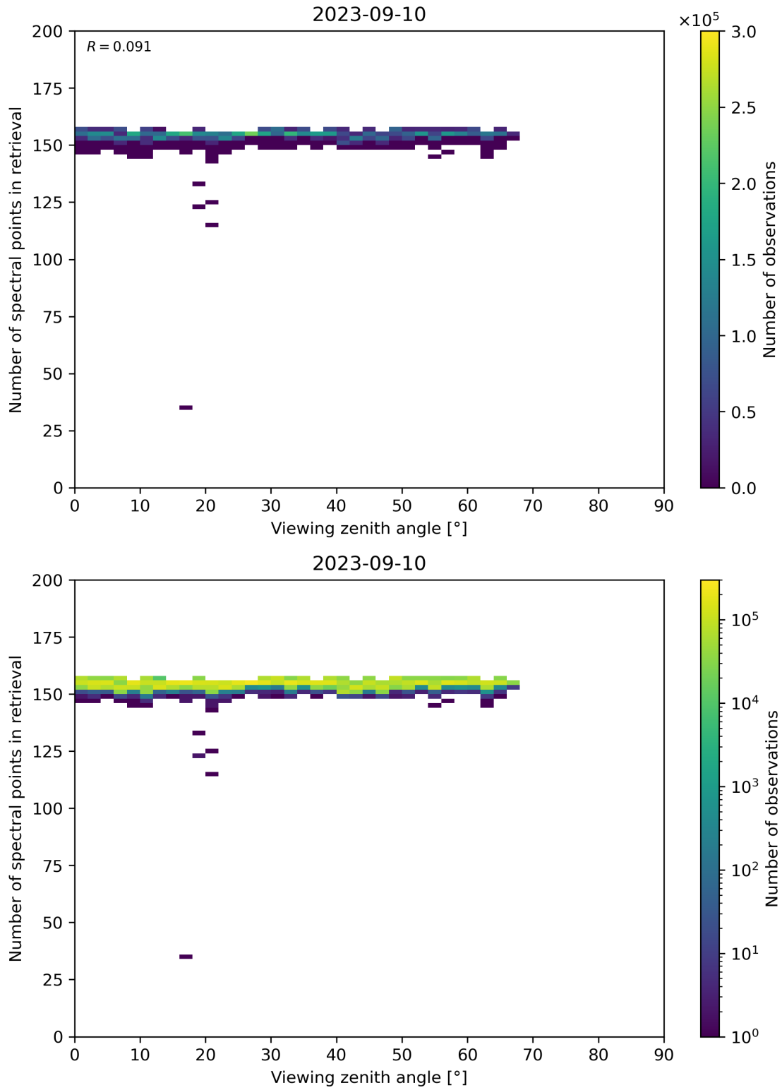
Figure 76: Scatter density plot of “Viewing zenith angle” against “Number of spectral points in retrieval” for 2023-09-10 to 2023-09-11.
