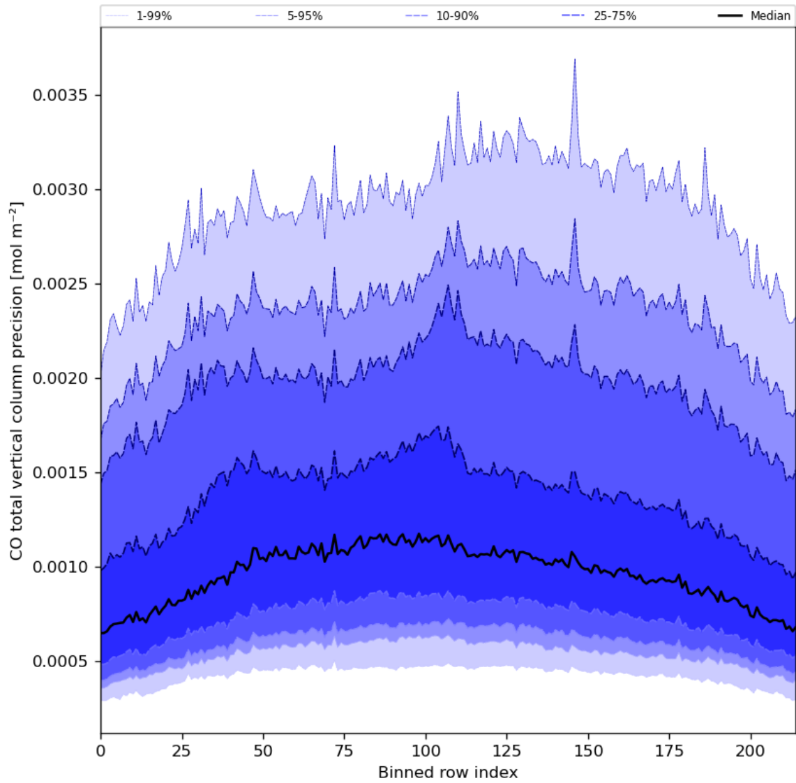
Figure 28: Along track statistics of “CO total vertical column precision” for 2023-09-10 to 2023-09-11
