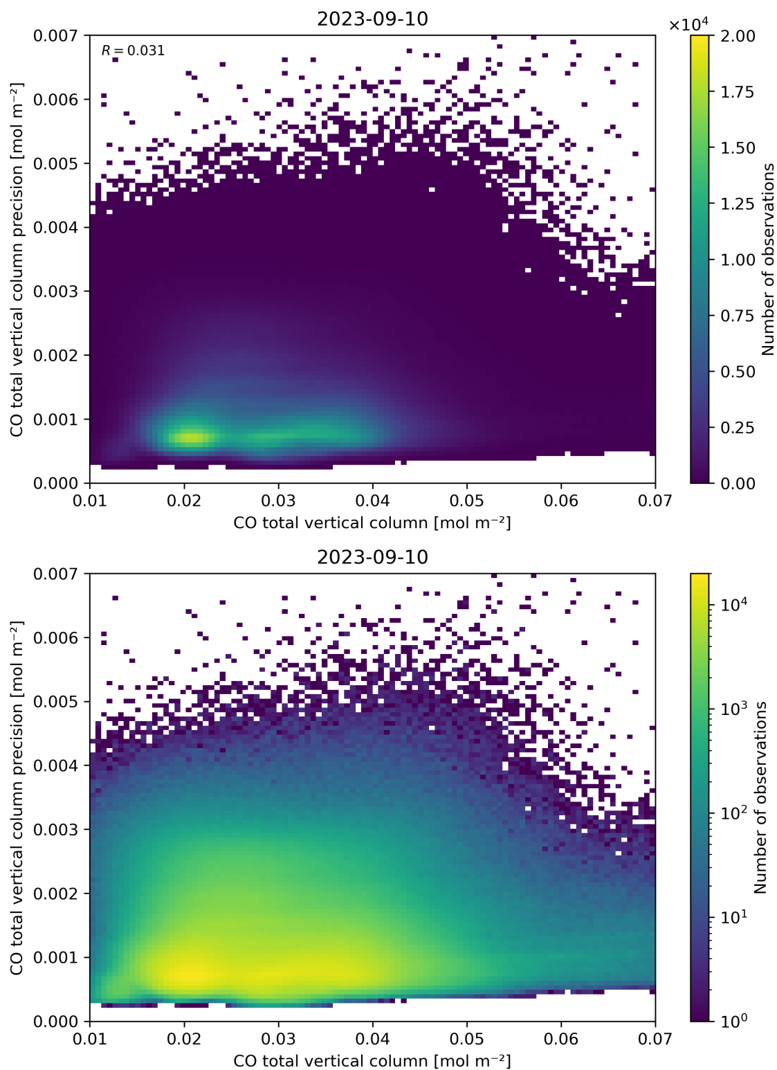
Figure 34: Scatter density plot of “CO total vertical column” against “CO total vertical column precision” for 2023-09-10 to 2023-09-11.
