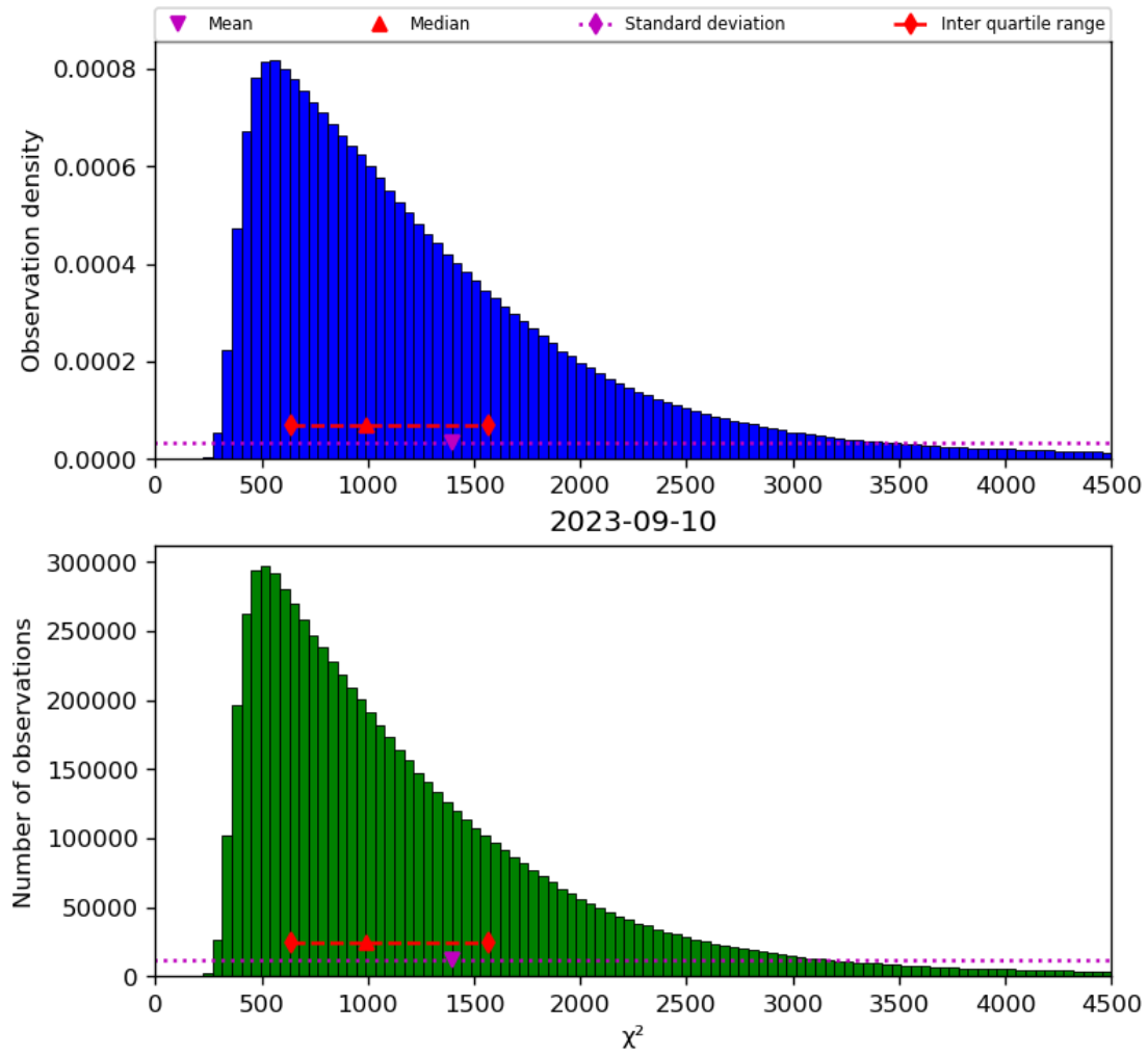
Figure 22: Histogram of “ \chi^2 ” for 2023-09-10 to 2023-09-11
