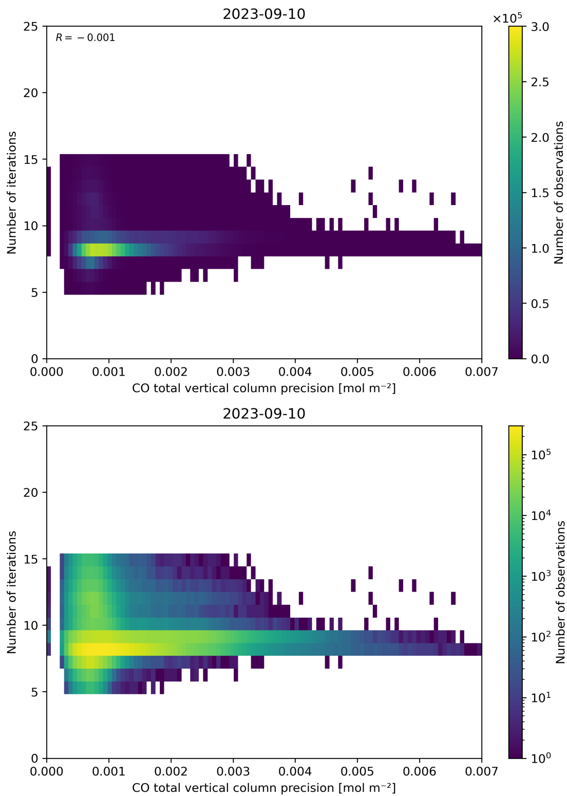
Figure 46: Scatter density plot of “CO total vertical column precision” against “Number of iterations” for 2023-09-10 to 2023-09-11.
