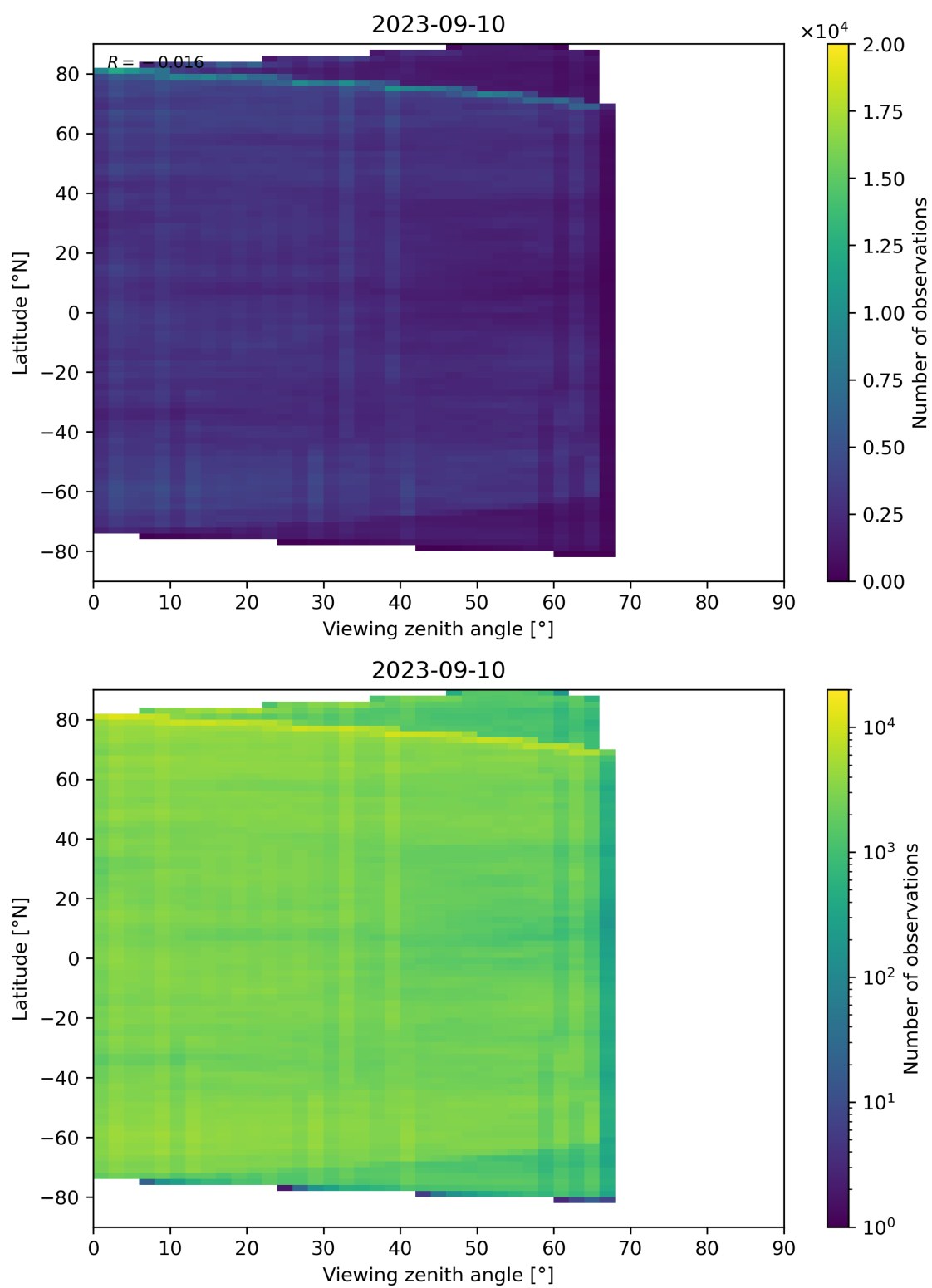
Figure 74: Scatter density plot of “Viewing zenith angle” against “Latitude” for 2023-09-10 to 2023-09-11.
