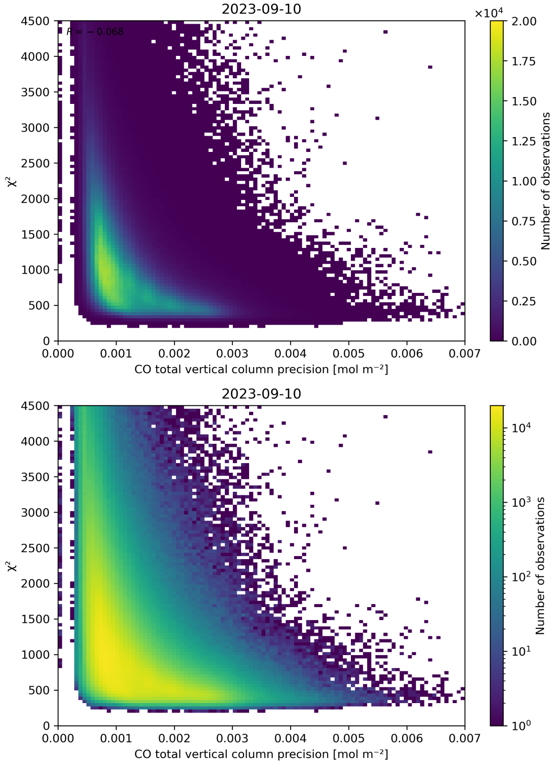
Figure 44: Scatter density plot of “CO total vertical column precision” against “ \chi^2 ” for 2023-09-10 to 2023-09-11.
