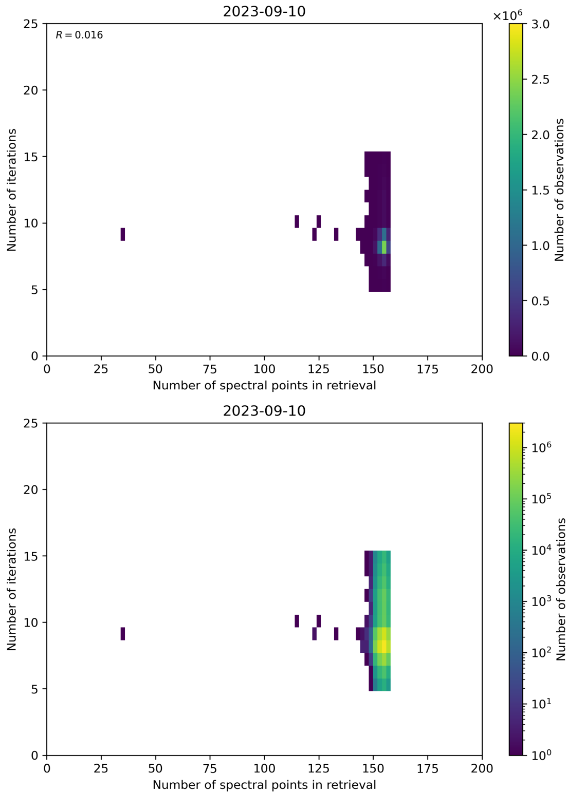
Figure 60: Scatter density plot of “Number of spectral points in retrieval” against “Number of iterations” for 2023-09-10 to 2023-09-11.
