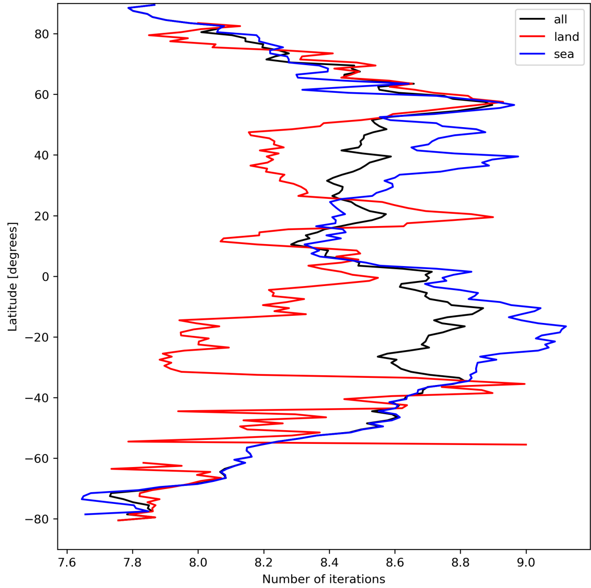
Figure 16: Zonal average of “Number of iterations” for 2023-09-10 to 2023-09-11.
