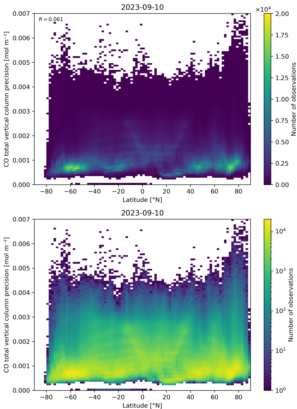
Figure 53: Scatter density plot of “Latitude” against “CO total vertical column precision” for 2023-09-10 to 2023-09-11.
