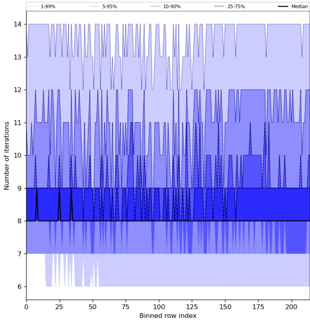
Figure 32: Along track statistics of “Number of iterations” for 2023-09-10 to 2023-09-11
