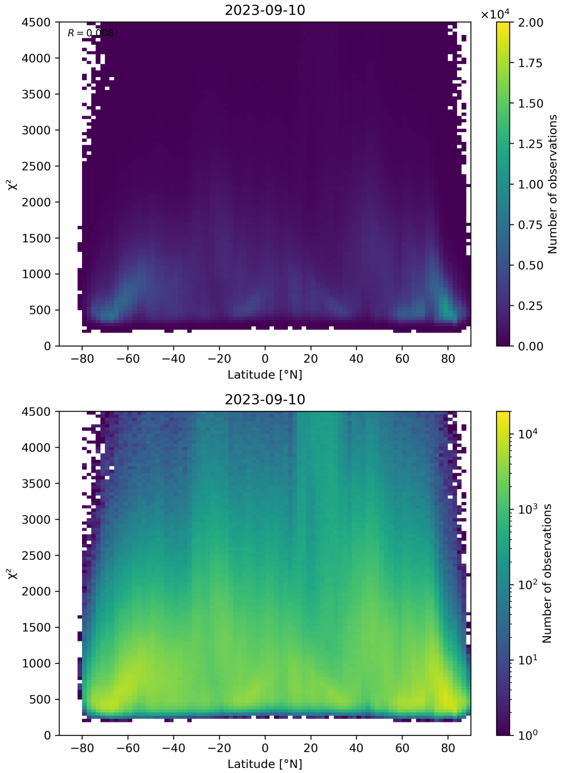
Figure 54: Scatter density plot of “Latitude” against “ \chi^2 ” for 2023-09-10 to 2023-09-11.
