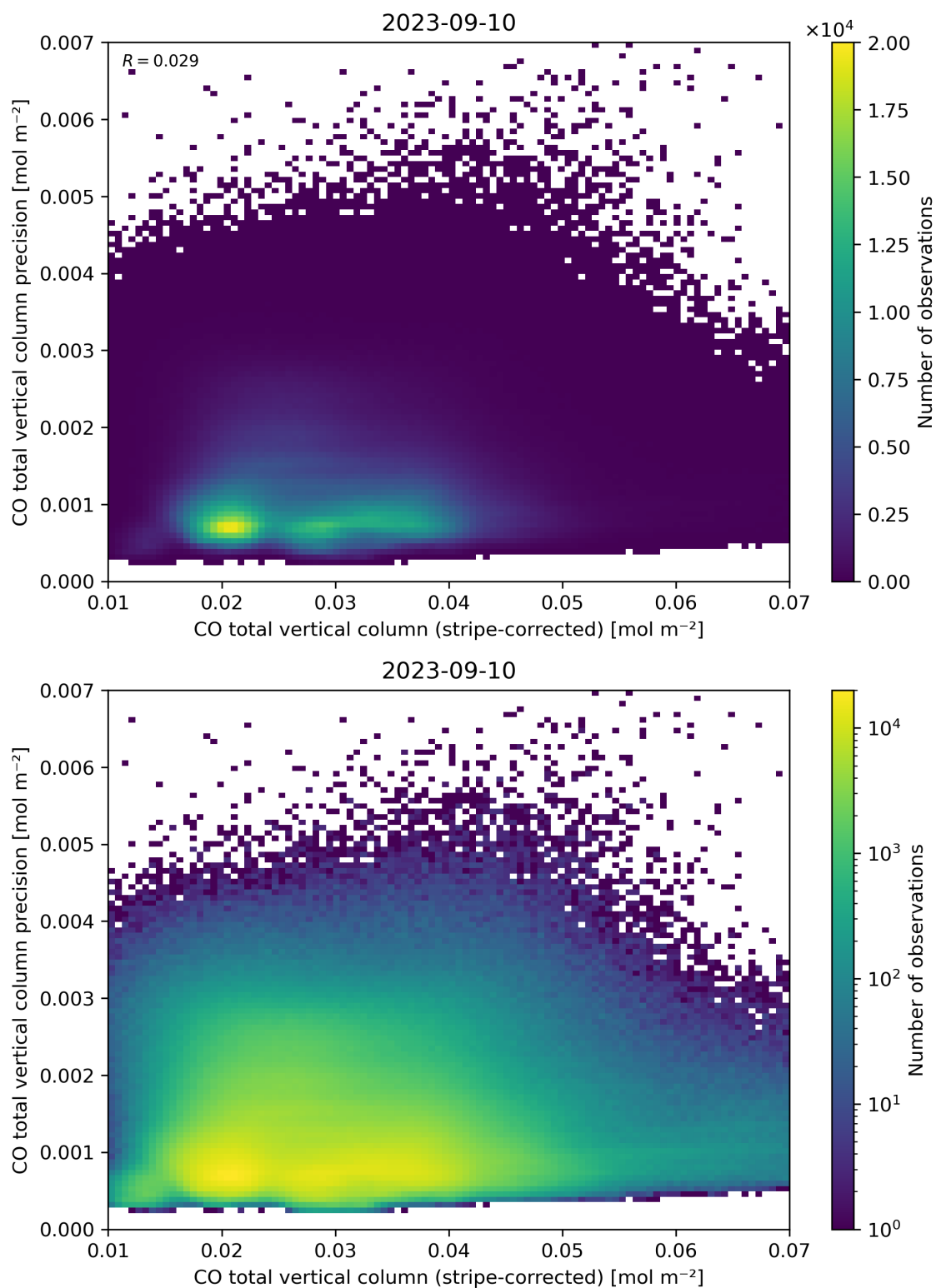
Figure 36: Scatter density plot of “CO total vertical column (stripe-corrected)” against “CO total vertical column precision” for 2023-09-10 to 2023-09-11.
