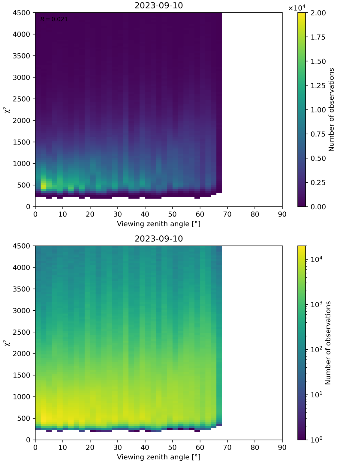
Figure 72: Scatter density plot of “Viewing zenith angle” against “ \chi^2 ” for 2023-09-10 to 2023-09-11.
