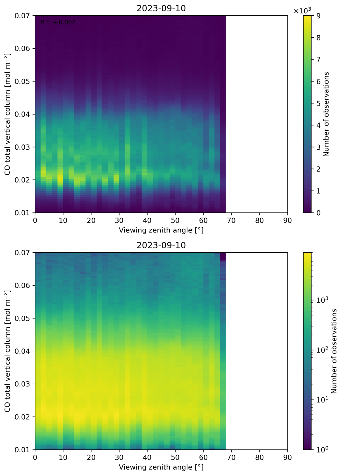
Figure 69: Scatter density plot of “Viewing zenith angle” against “CO total vertical column” for 2023-09-10 to 2023-09-11.
