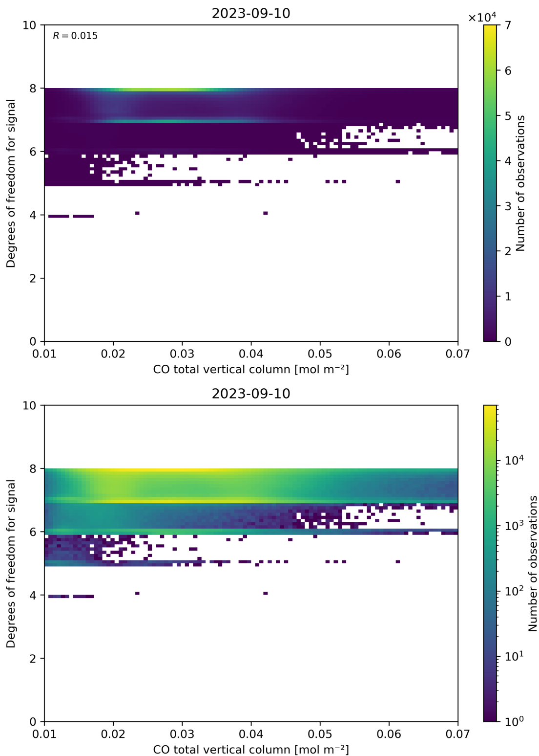
Figure 41: Scatter density plot of “CO total vertical column” against “Degrees of freedom for signal” for 2023-09-10 to 2023-09-11.
