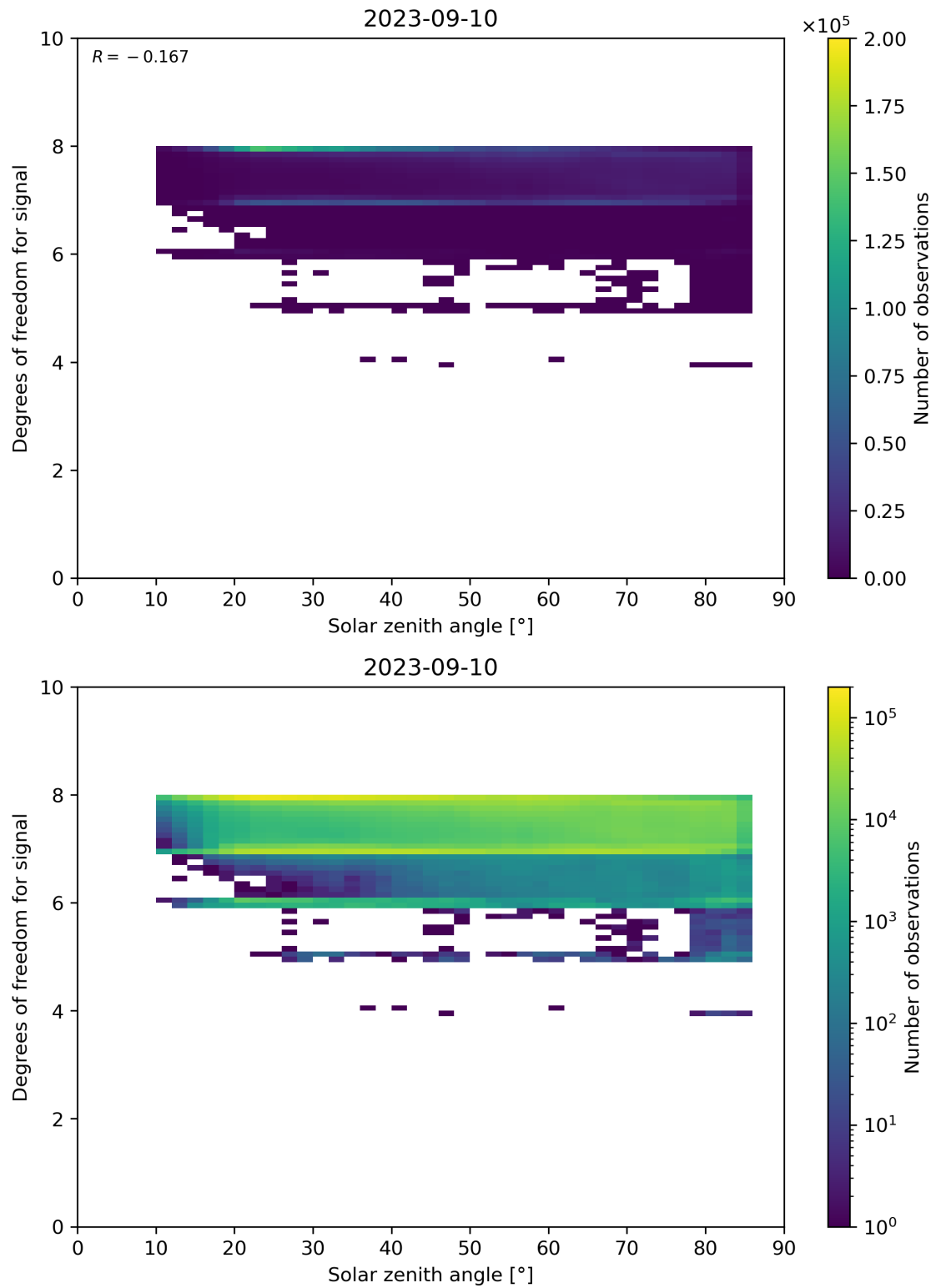
Figure 65: Scatter density plot of “Solar zenith angle” against “Degrees of freedom for signal” for 2023-09-10 to 2023-09-11.
