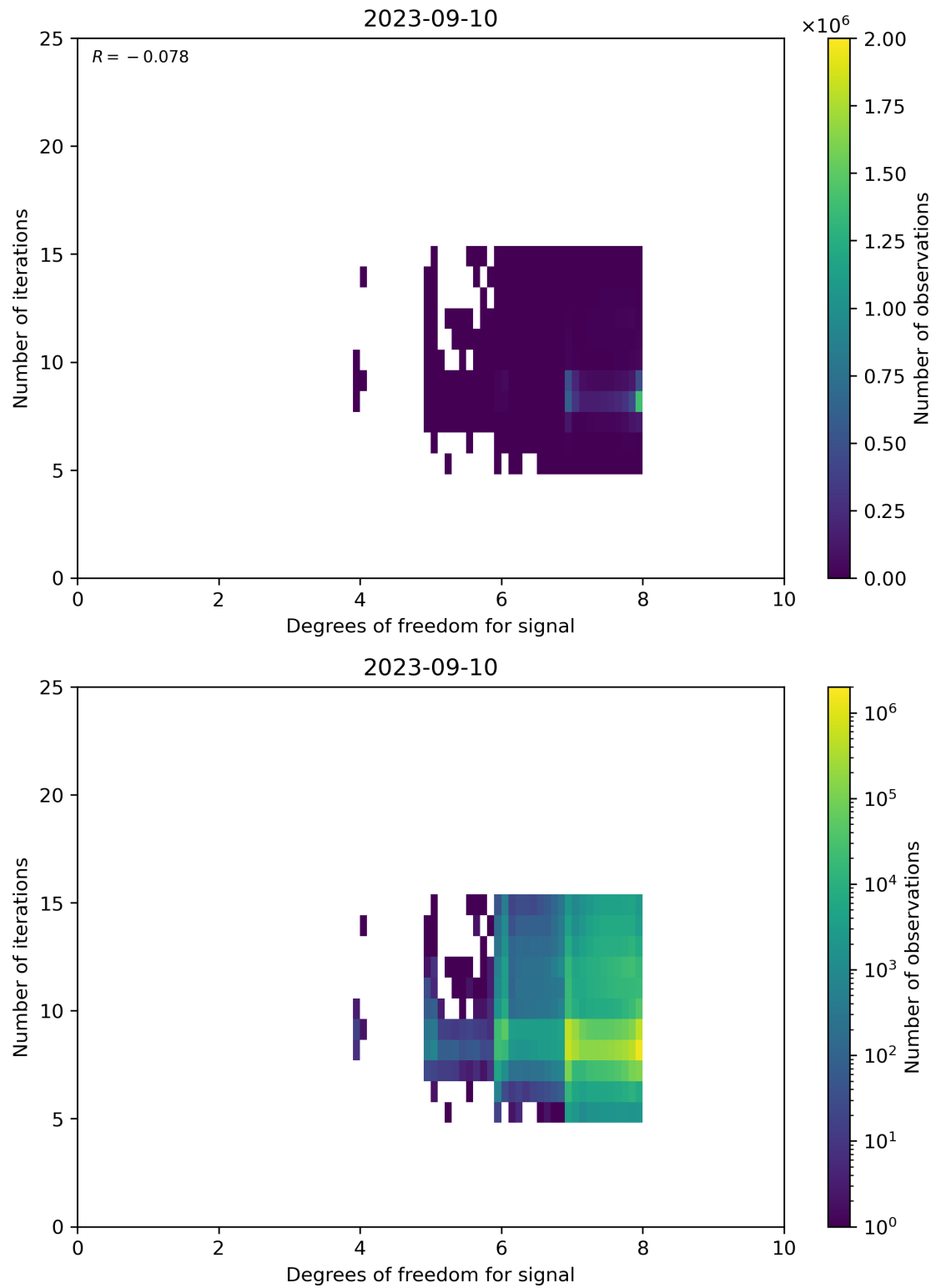
Figure 50: Scatter density plot of “Degrees of freedom for signal” against “Number of iterations” for 2023-09-10 to 2023-09-11.
