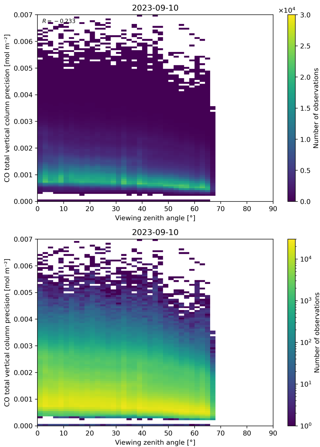
Figure 71: Scatter density plot of “Viewing zenith angle” against “CO total vertical column precision” for 2023-09-10 to 2023-09-11.
