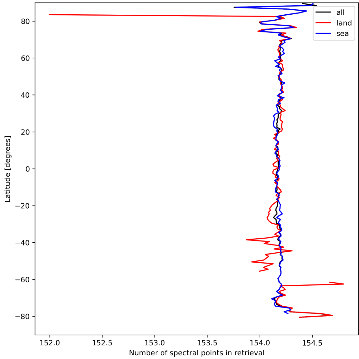
Figure 13: Zonal average of “Number of spectral points in retrieval” for 2023-09-10 to 2023-09-11.
