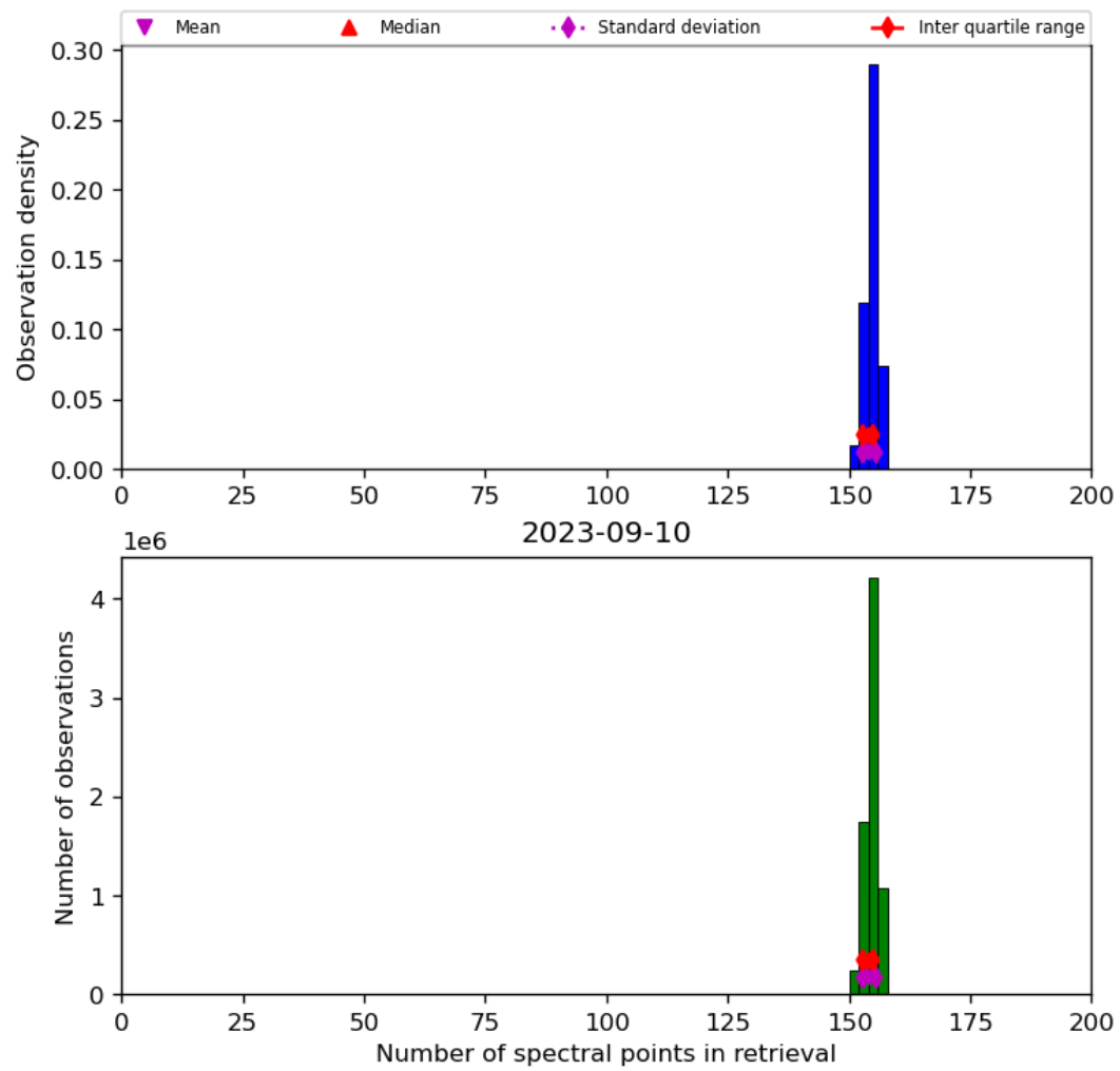
Figure 21: Histogram of “Number of spectral points in retrieval” for 2023-09-10 to 2023-09-11
