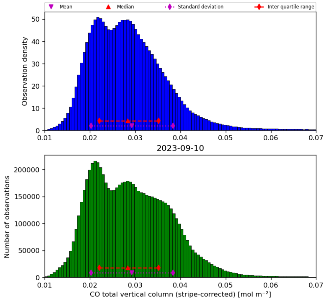
Figure 19: Histogram of “CO total vertical column (stripe-corrected)” for 2023-09-10 to 2023-09-11
