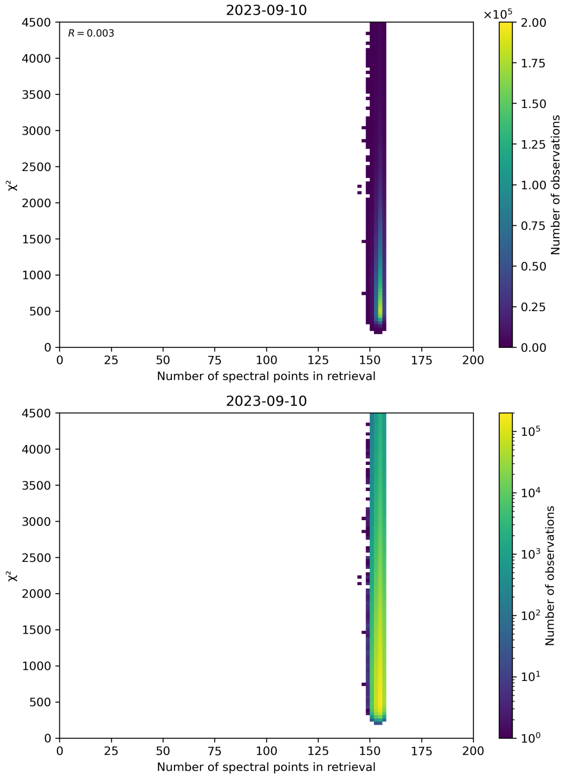
Figure 58: Scatter density plot of “Number of spectral points in retrieval” against “ \chi^2 ” for 2023-09-10 to 2023-09-11.
