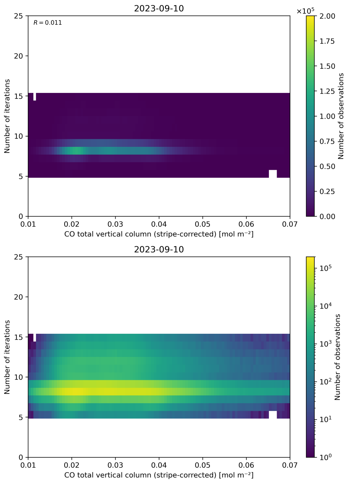
Figure 39: Scatter density plot of “CO total vertical column (stripe-corrected)” against “Number of iterations” for 2023-09-10 to 2023-09-11.
