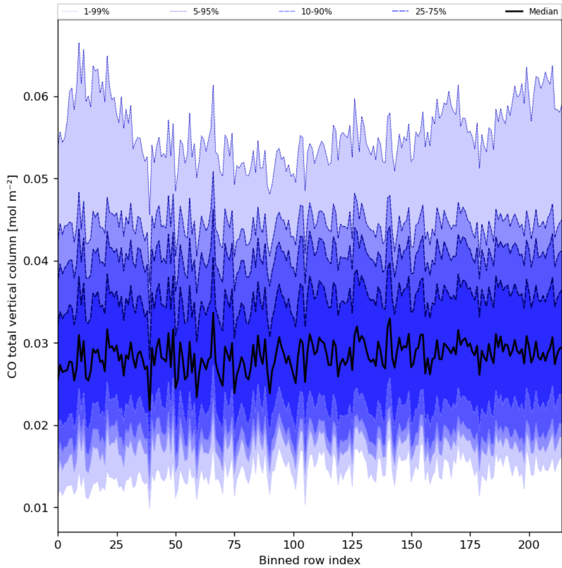
Figure 26: Along track statistics of “CO total vertical column” for 2023-09-10 to 2023-09-11
