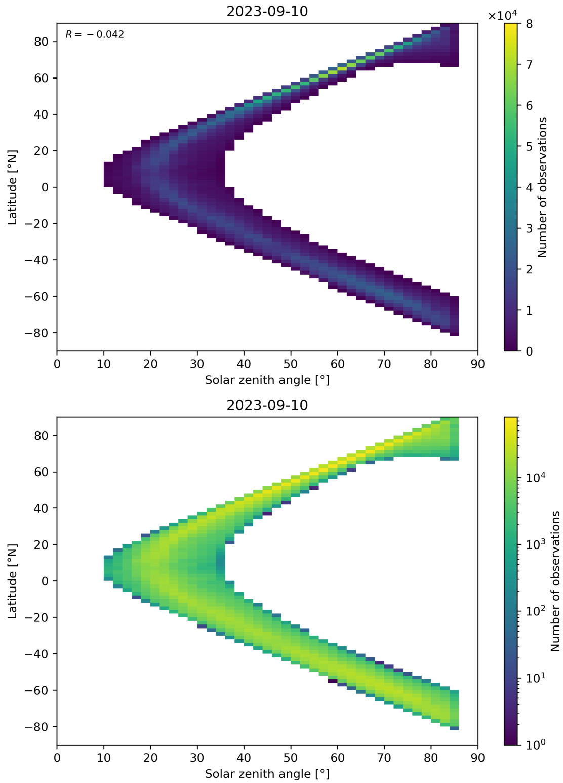
Figure 66: Scatter density plot of “Solar zenith angle” against “Latitude” for 2023-09-10 to 2023-09-11.
