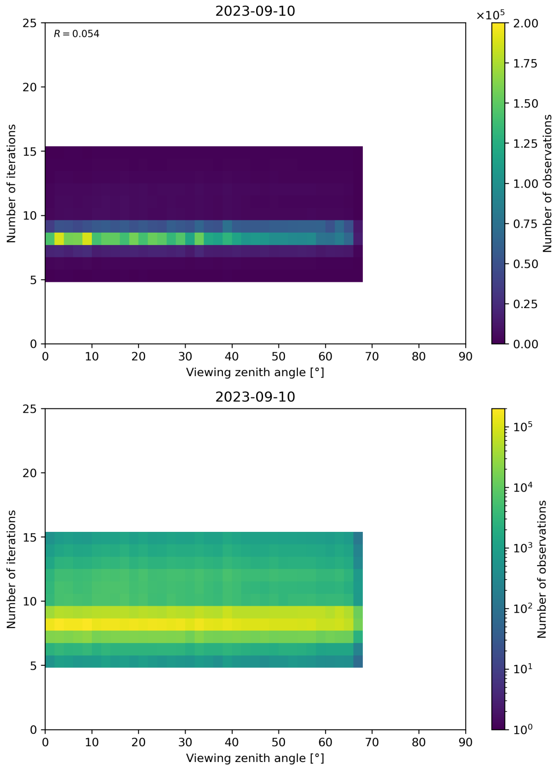
Figure 75: Scatter density plot of “Viewing zenith angle” against “Number of iterations” for 2023-09-10 to 2023-09-11.
