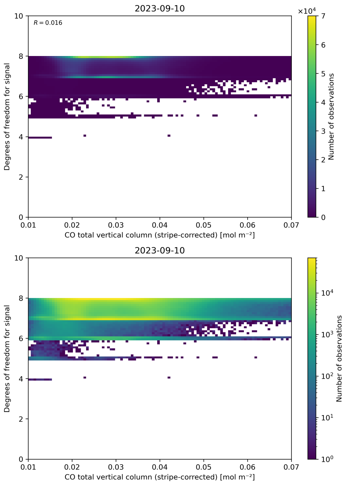
Figure 38: Scatter density plot of “CO total vertical column (stripe-corrected)” against “Degrees of freedom for signal” for 2023-09-10 to 2023-09-11.
