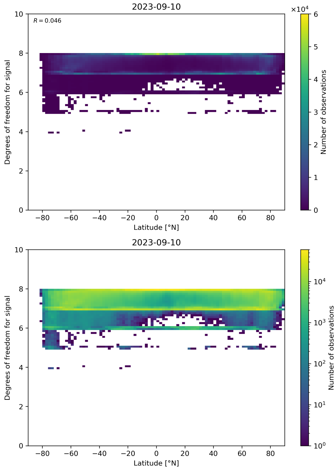
Figure 55: Scatter density plot of “Latitude” against “Degrees of freedom for signal” for 2023-09-10 to 2023-09-11.
