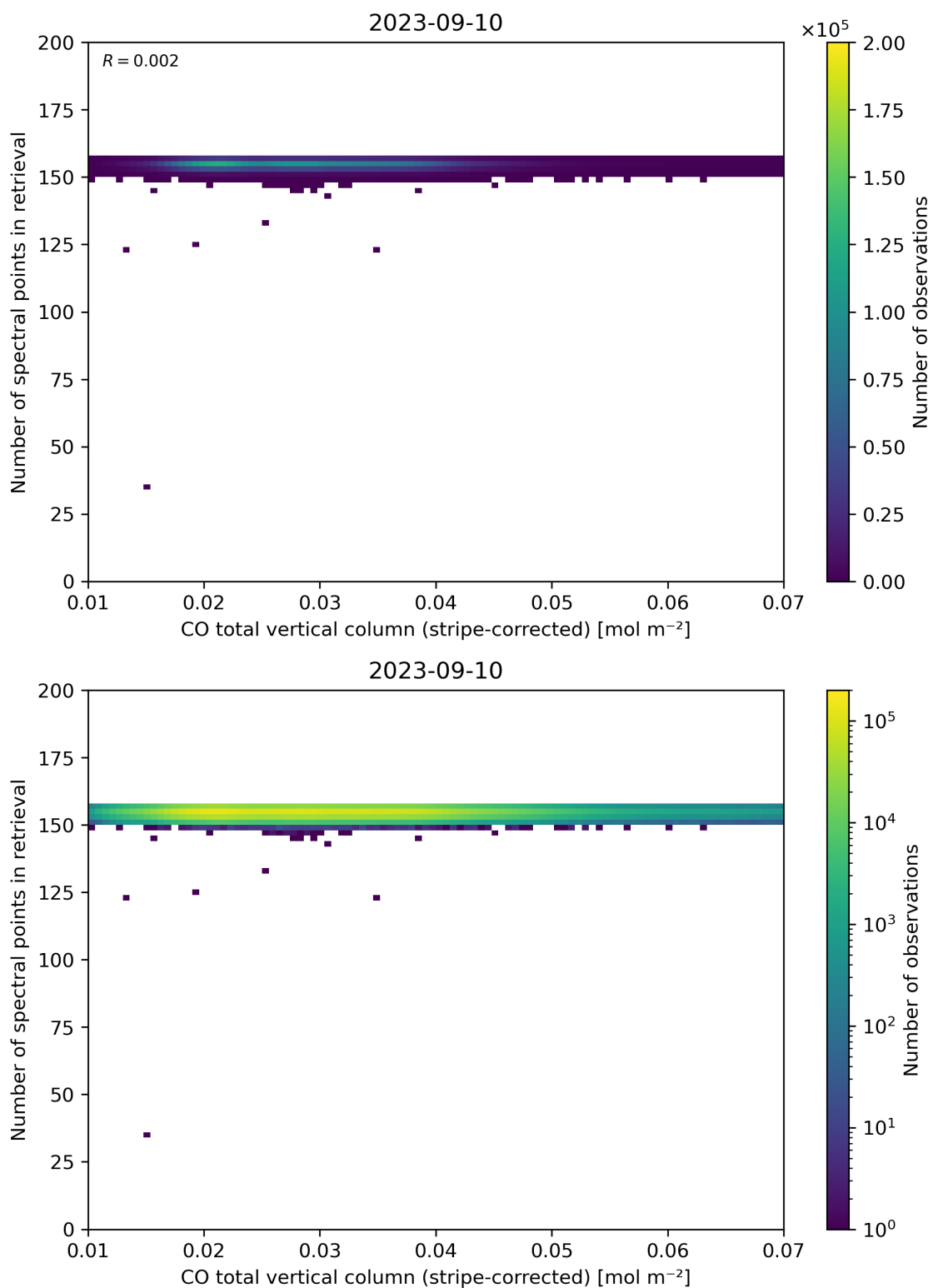
Figure 40: Scatter density plot of “CO total vertical column (stripe-corrected)” against “Number of spectral points in retrieval” for 2023-09-10 to 2023-09-11.
