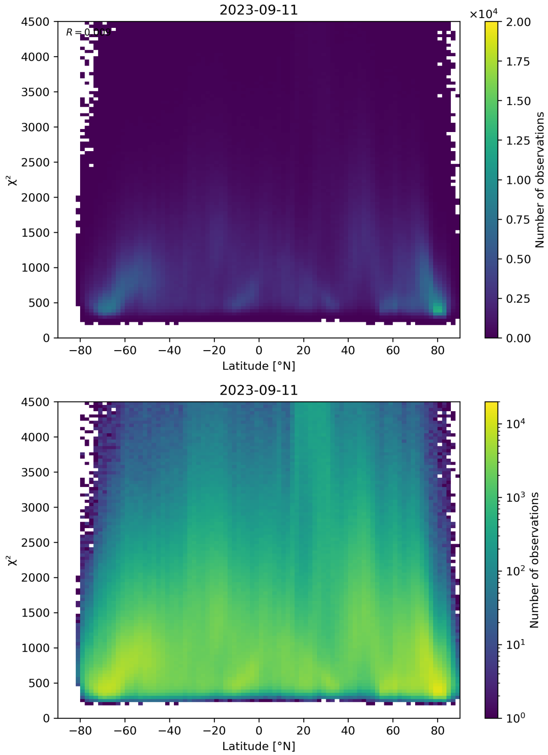
Figure 54: Scatter density plot of “Latitude” against “ \chi^2 ” for 2023-09-10 to 2023-09-12.
