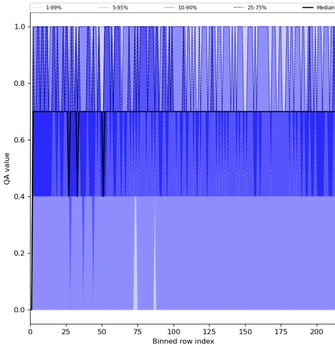
Figure 25: Along track statistics of “QA value” for 2023-09-10 to 2023-09-12
