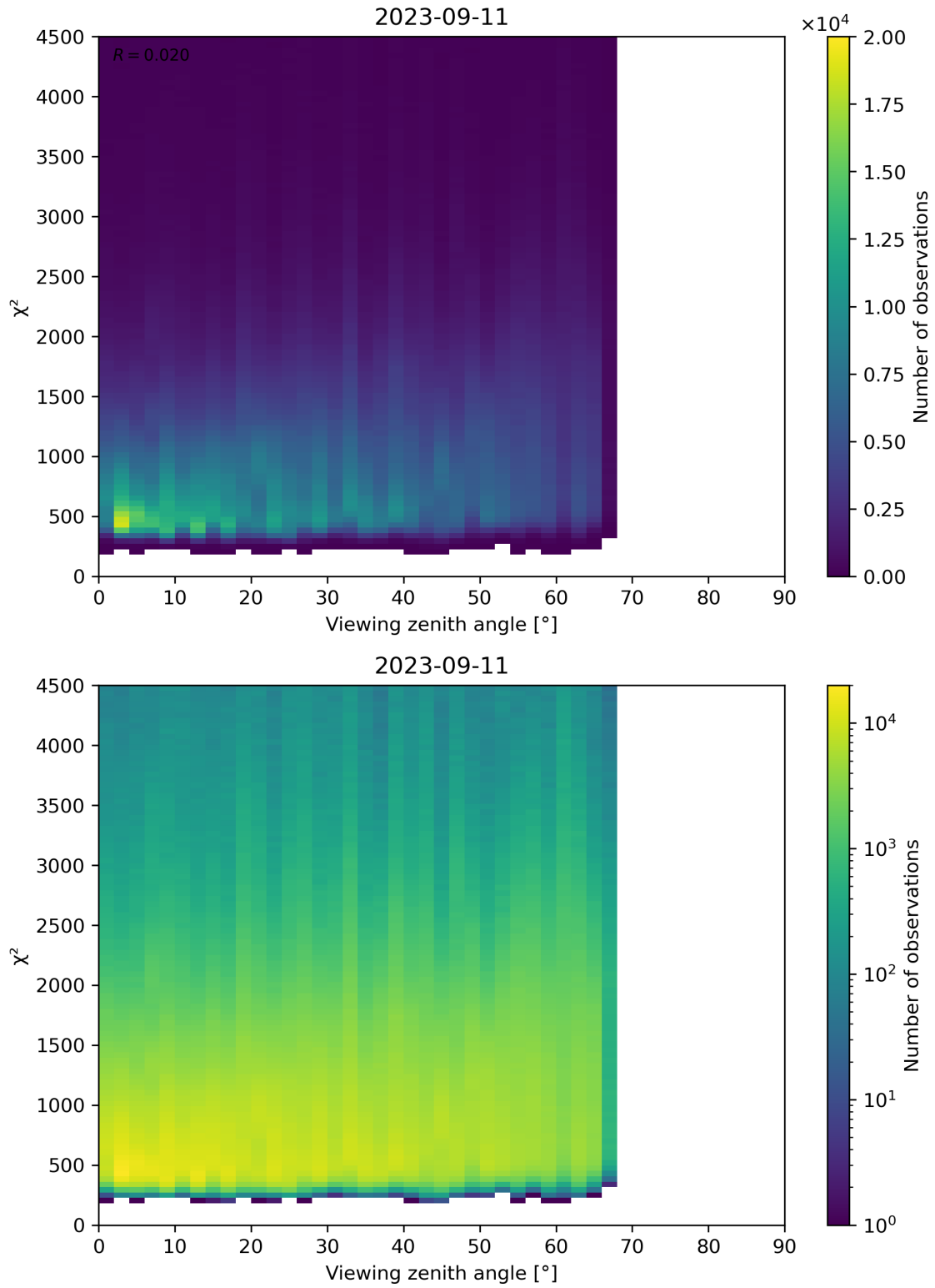
Figure 72: Scatter density plot of “Viewing zenith angle” against “ \chi^2 ” for 2023-09-10 to 2023-09-12.
