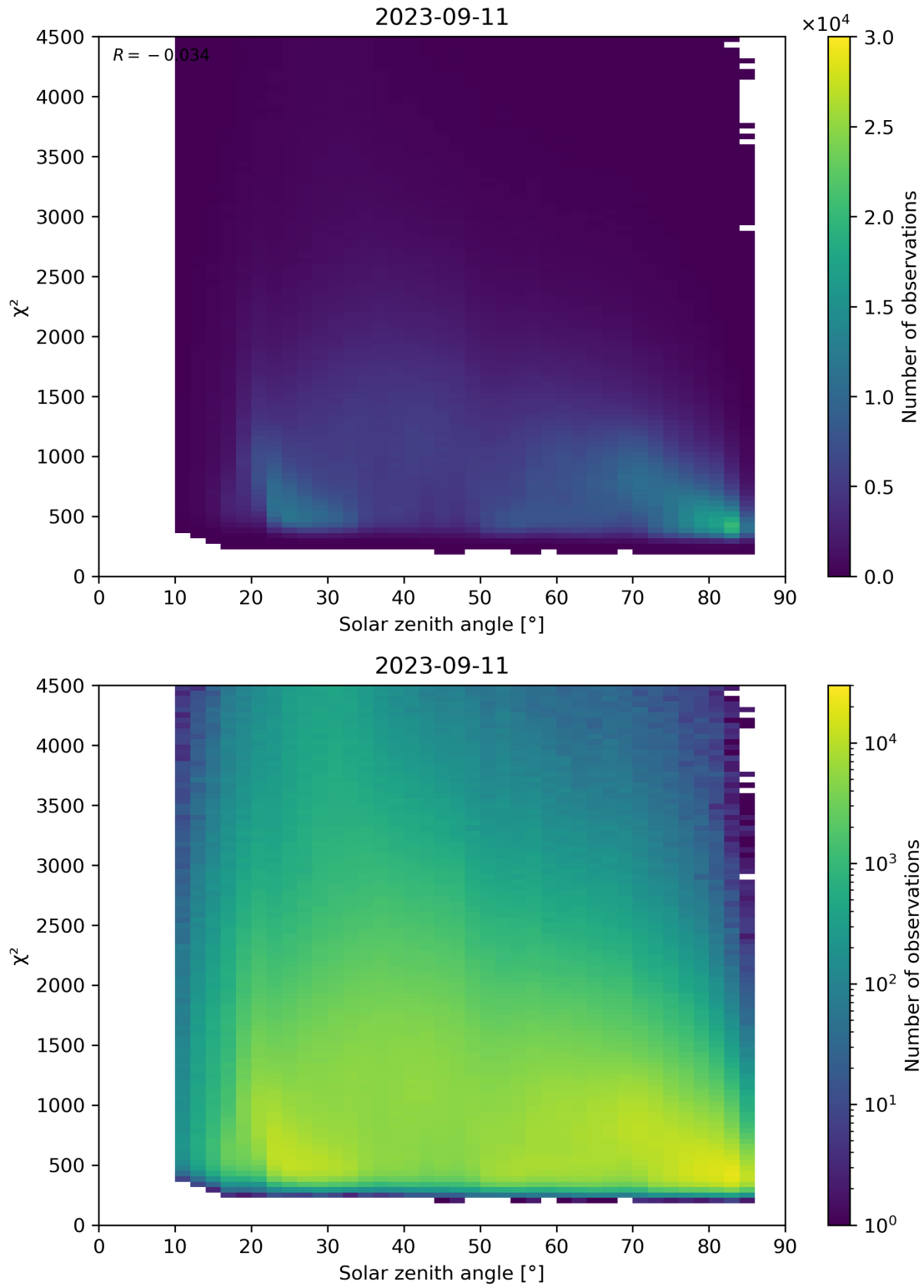
Figure 64: Scatter density plot of “Solar zenith angle” against “ \chi^2 ” for 2023-09-10 to 2023-09-12.
