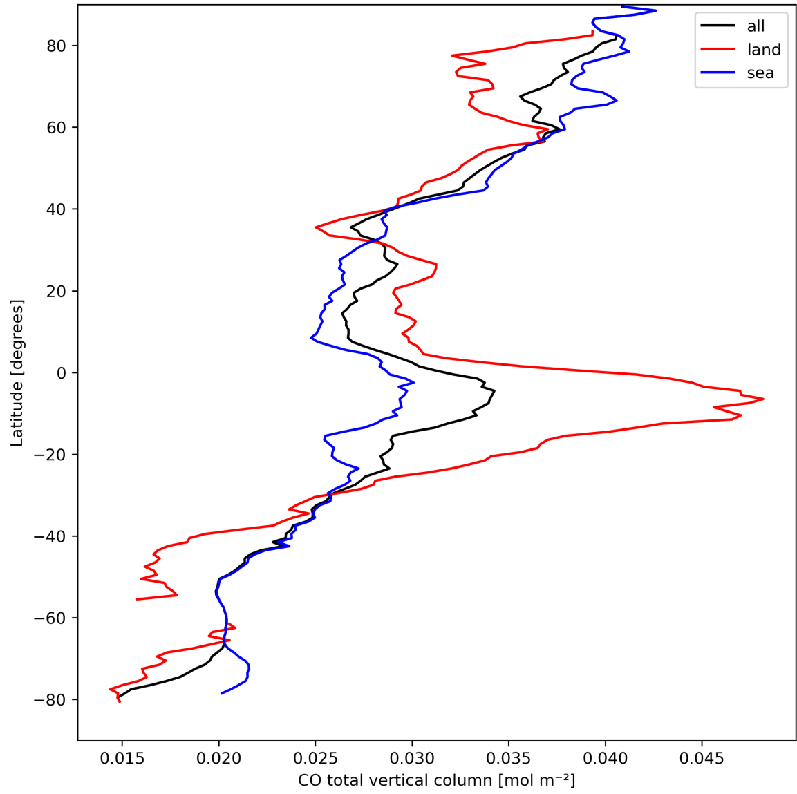
Figure 10: Zonal average of “CO total vertical column” for 2023-09-10 to 2023-09-12.
