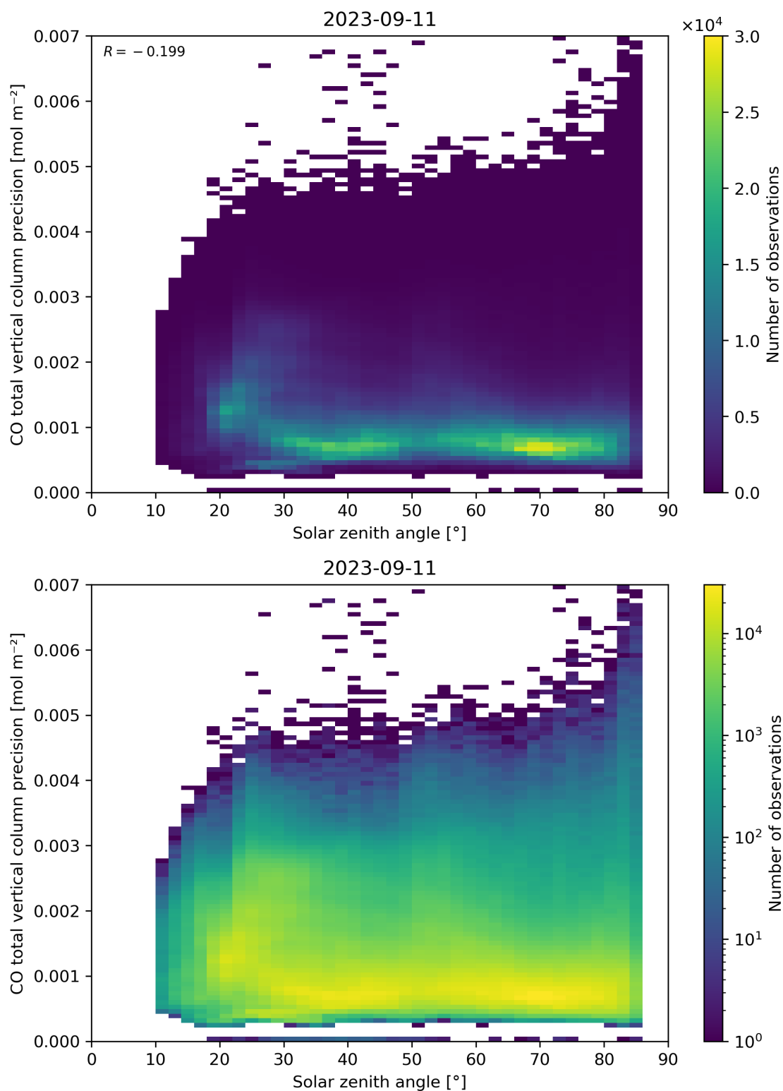
Figure 63: Scatter density plot of “Solar zenith angle” against “CO total vertical column precision” for 2023-09-10 to 2023-09-12.
