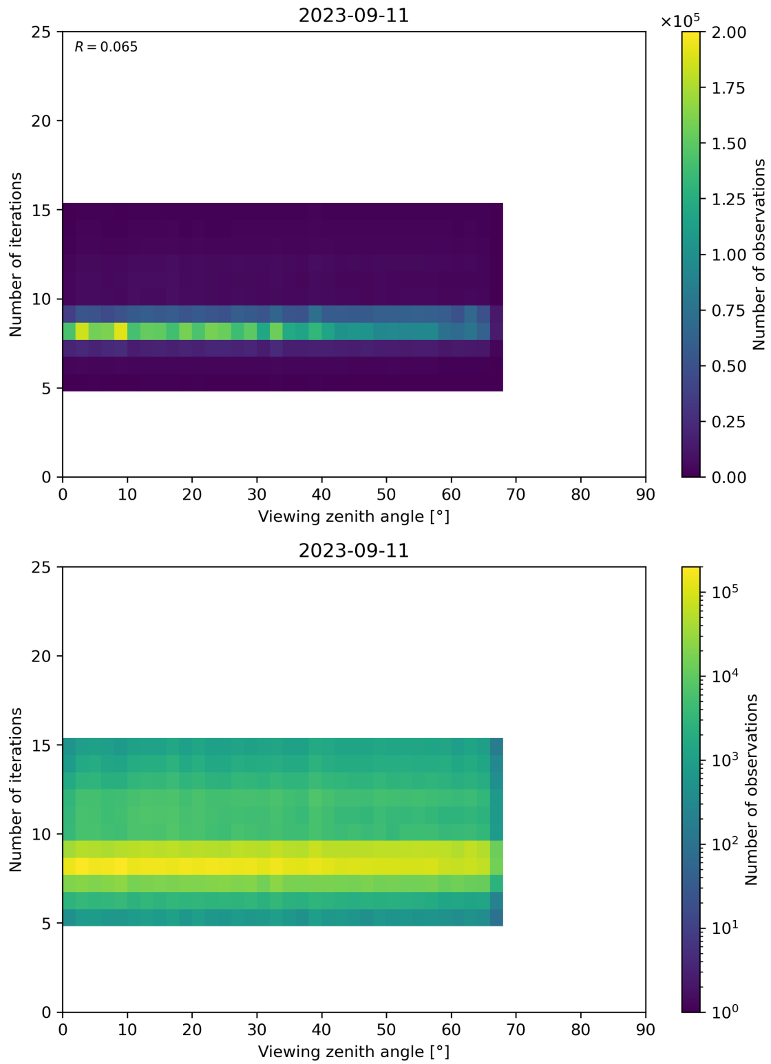
Figure 75: Scatter density plot of “Viewing zenith angle” against “Number of iterations” for 2023-09-10 to 2023-09-12.
