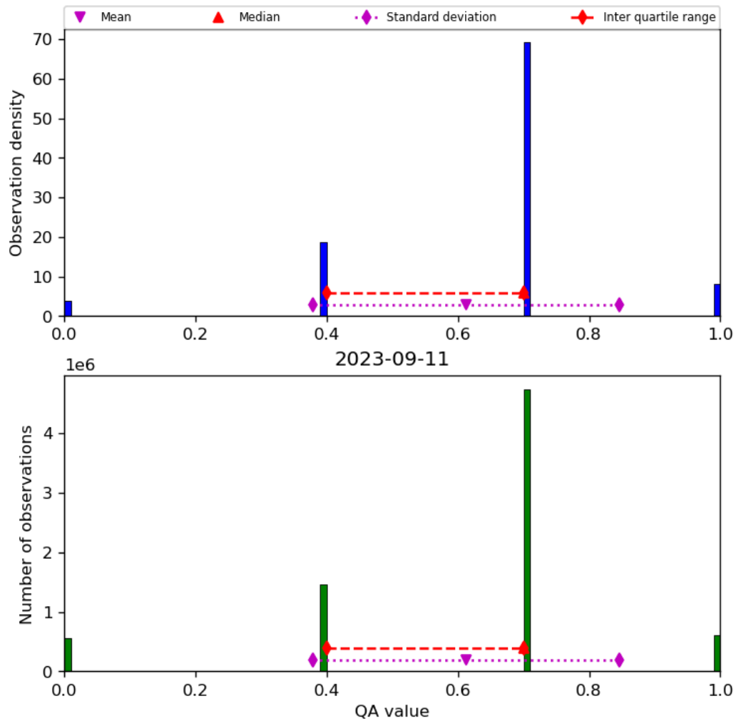
Figure 17: Histogram of “QA value” for 2023-09-10 to 2023-09-12
