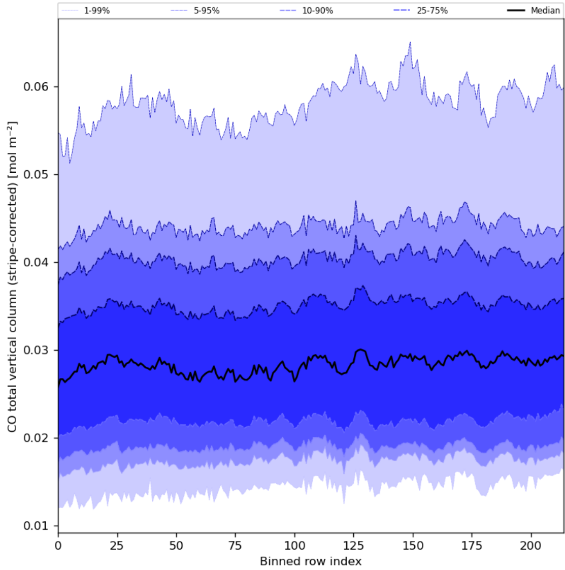
Figure 27: Along track statistics of “CO total vertical column (stripe-corrected)” for 2023-09-10 to 2023-09-12
