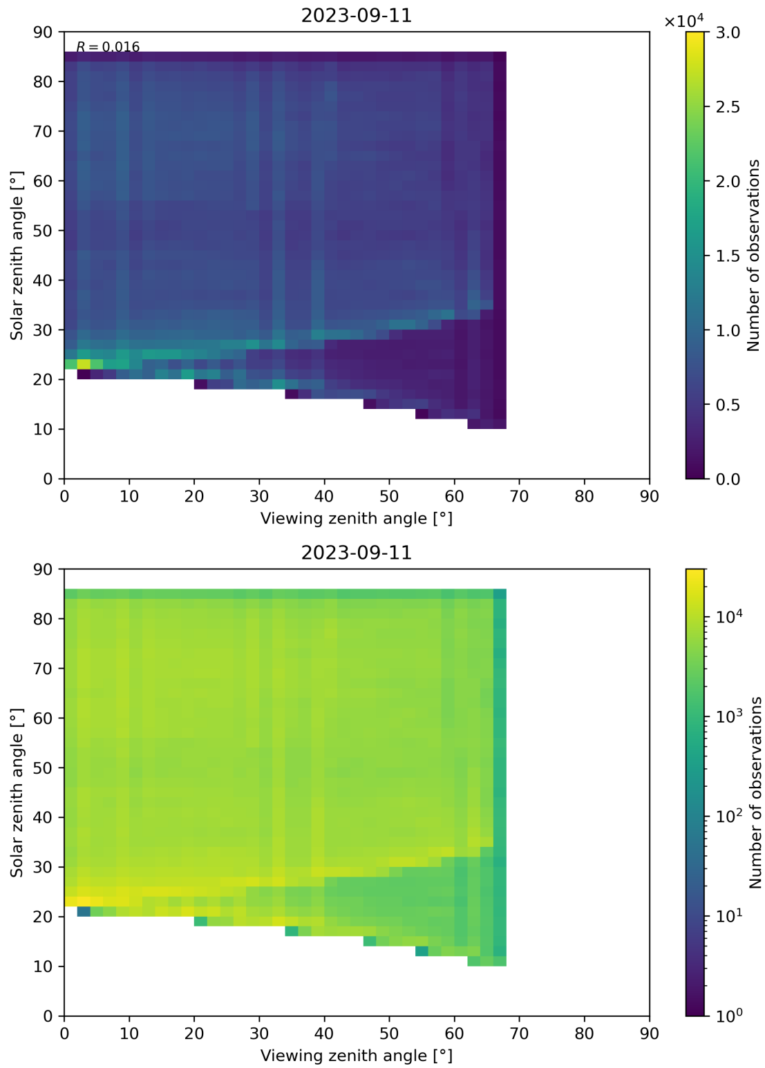
Figure 77: Scatter density plot of “Viewing zenith angle” against “Solar zenith angle” for 2023-09-10 to 2023-09-12.
