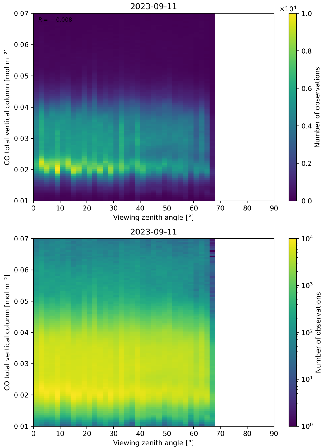
Figure 69: Scatter density plot of “Viewing zenith angle” against “CO total vertical column” for 2023-09-10 to 2023-09-12.
