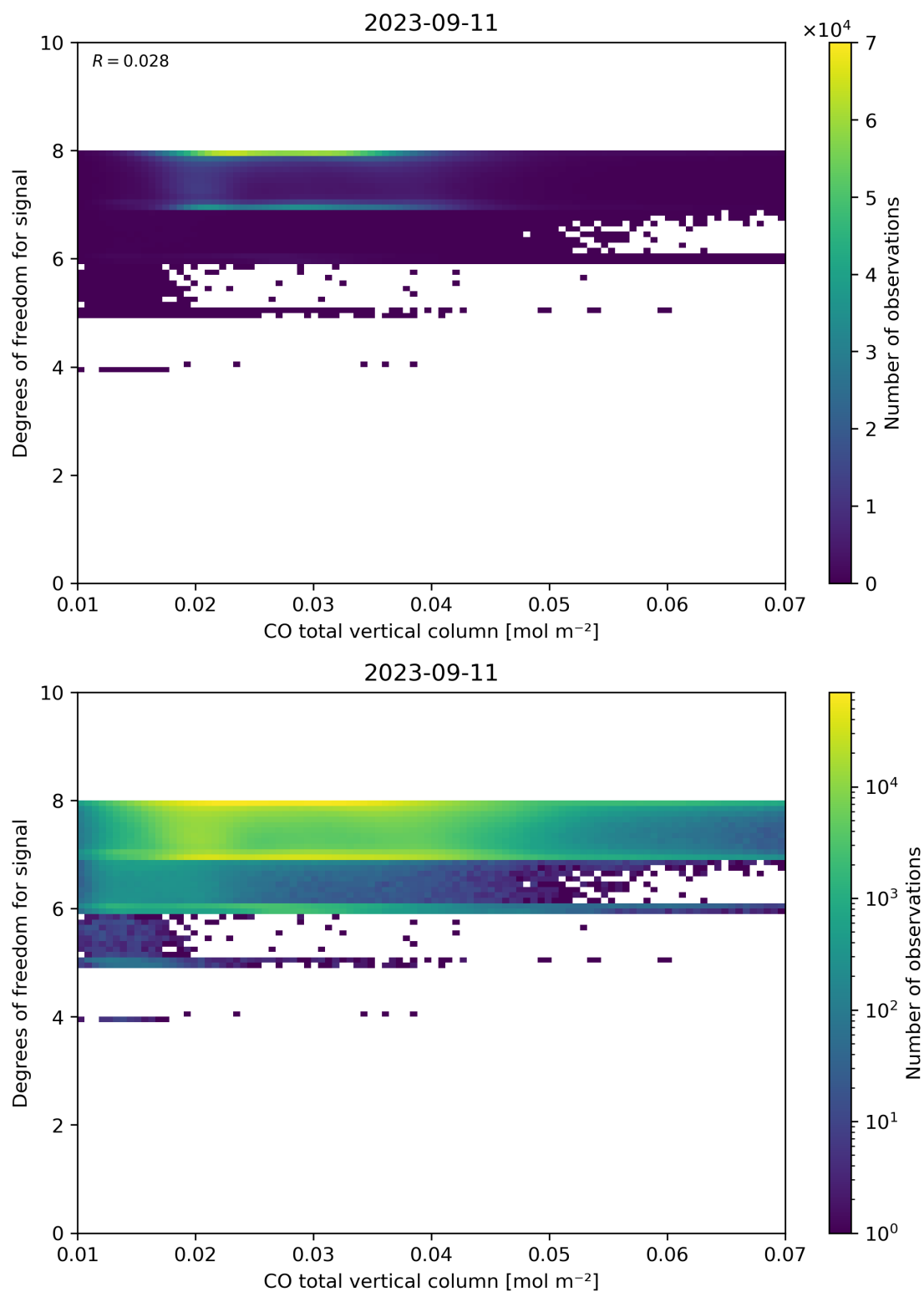
Figure 41: Scatter density plot of “CO total vertical column” against “Degrees of freedom for signal” for 2023-09-10 to 2023-09-12.
