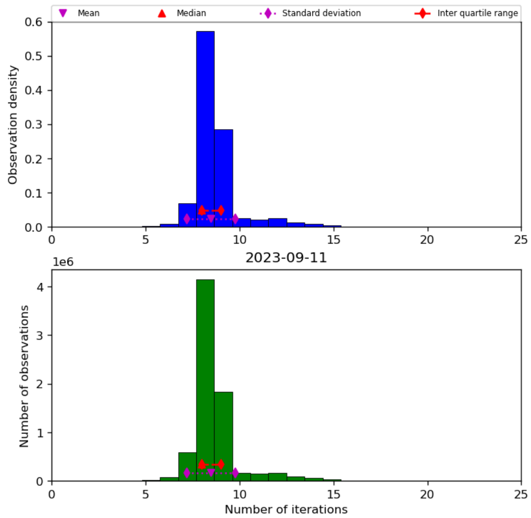
Figure 24: Histogram of “Number of iterations” for 2023-09-10 to 2023-09-12
