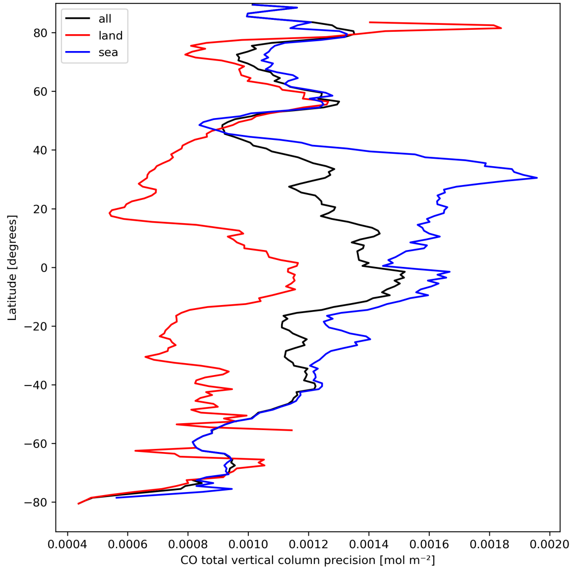
Figure 12: Zonal average of “CO total vertical column precision” for 2023-09-10 to 2023-09-12.
