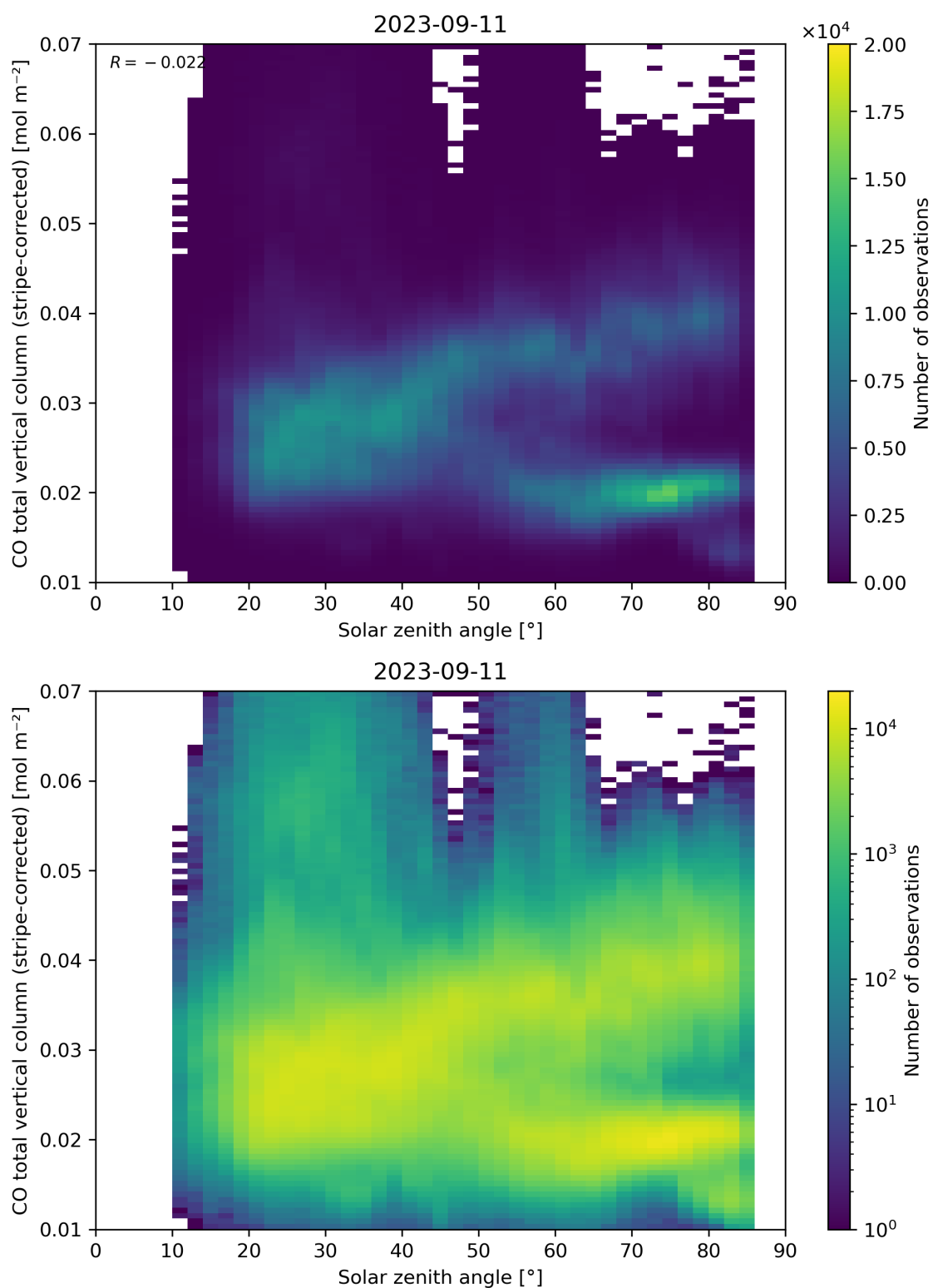
Figure 62: Scatter density plot of “Solar zenith angle” against “CO total vertical column (stripe-corrected)” for 2023-09-10 to 2023-09-12.
