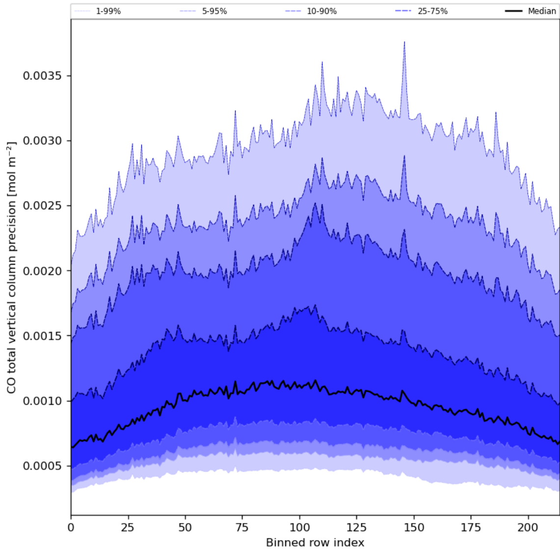
Figure 28: Along track statistics of “CO total vertical column precision” for 2023-09-10 to 2023-09-12
