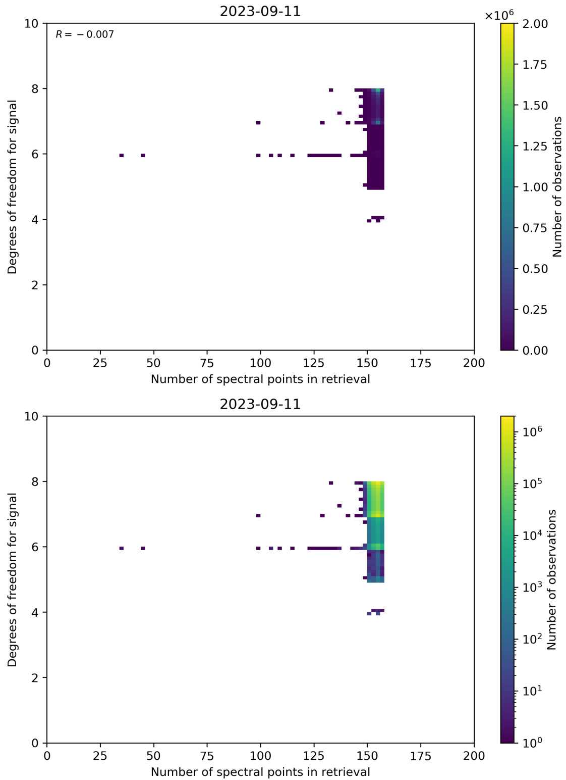
Figure 59: Scatter density plot of “Number of spectral points in retrieval” against “Degrees of freedom for signal” for 2023-09-10 to 2023-09-12.
