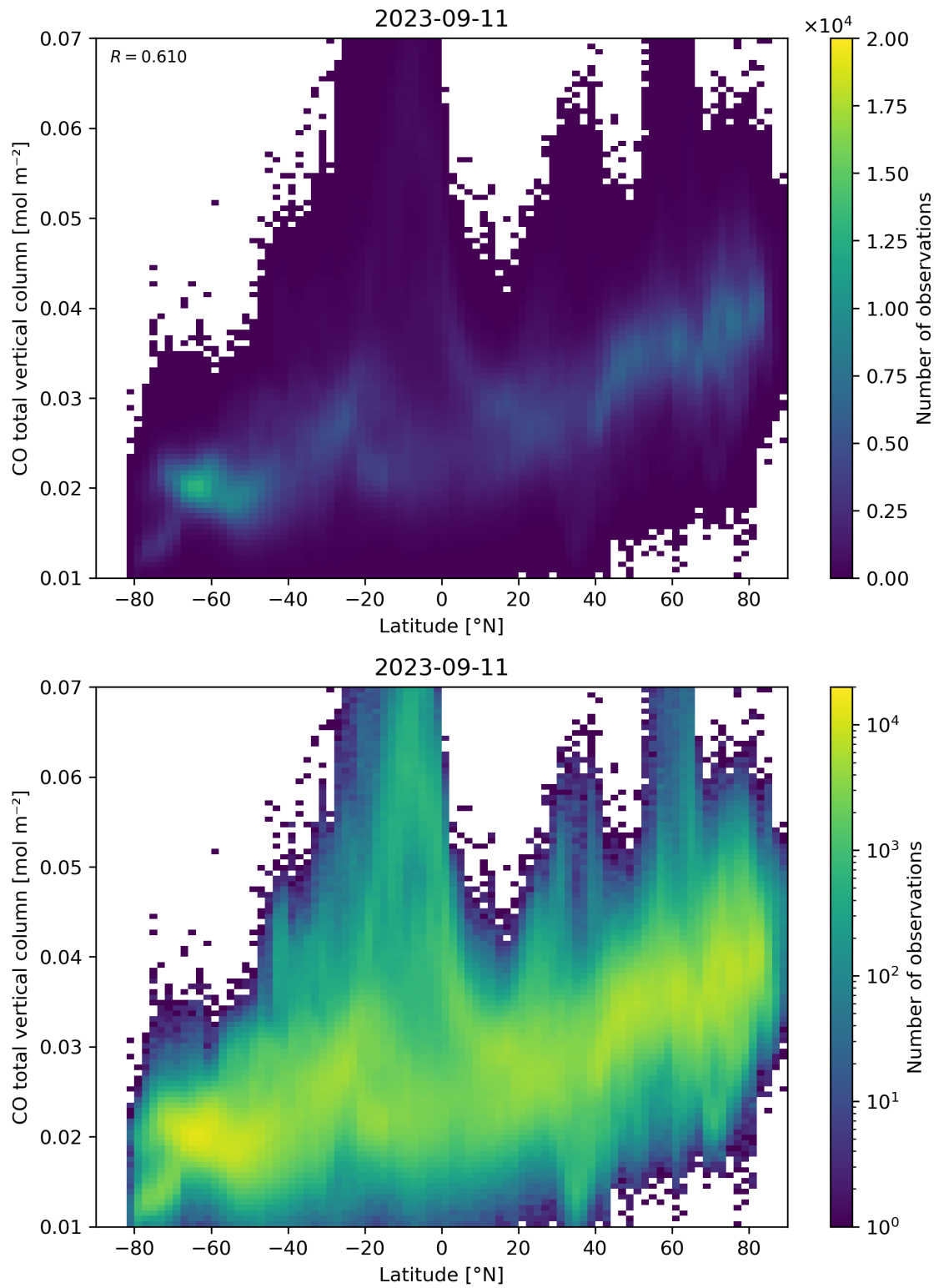
Figure 51: Scatter density plot of “Latitude” against “CO total vertical column” for 2023-09-10 to 2023-09-12.
