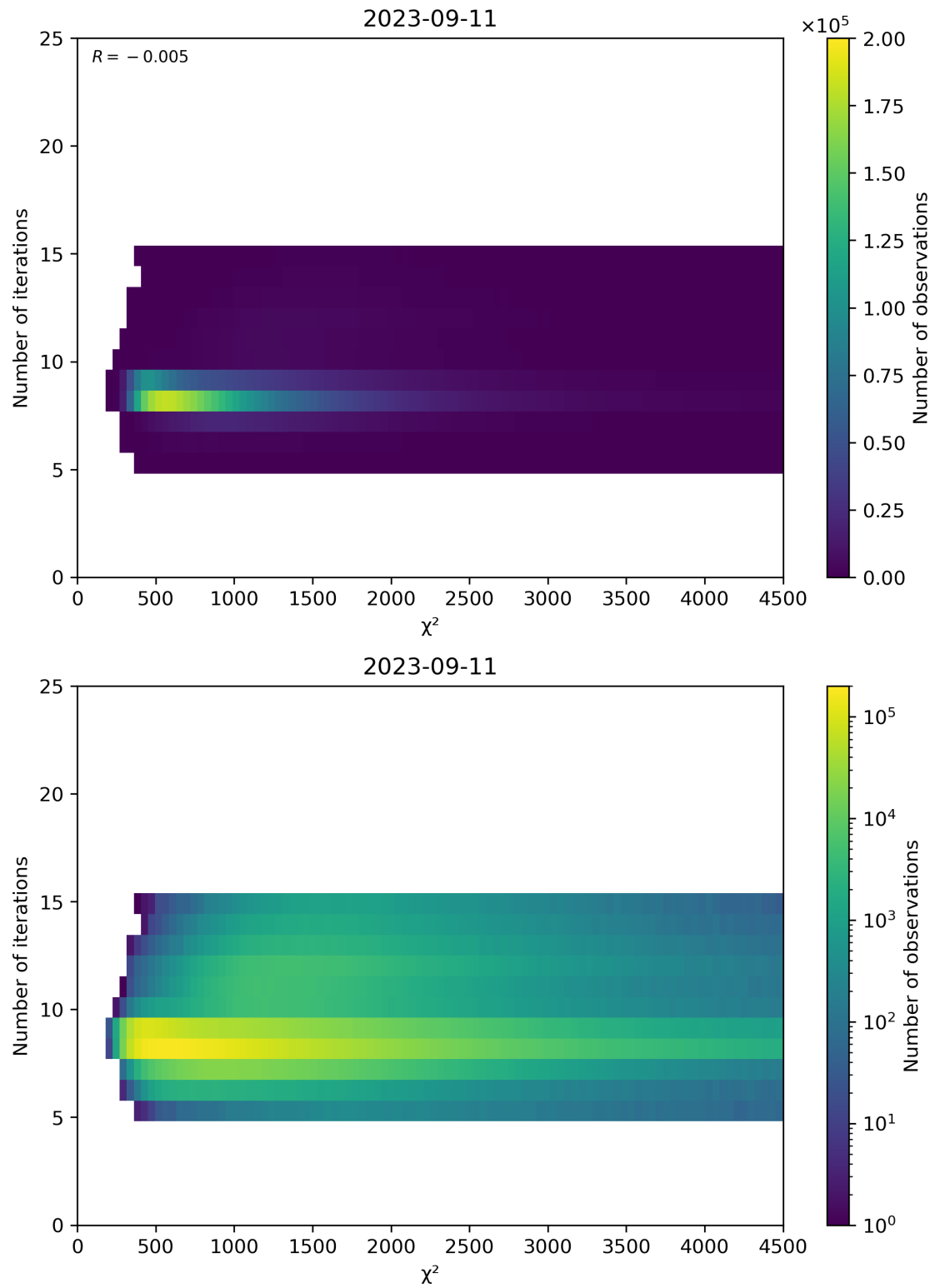
Figure 49: Scatter density plot of “ \chi^2 ” against “Number of iterations” for 2023-09-10 to 2023-09-12.
