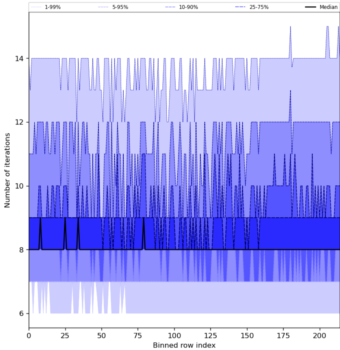
Figure 32: Along track statistics of “Number of iterations” for 2023-09-10 to 2023-09-12
