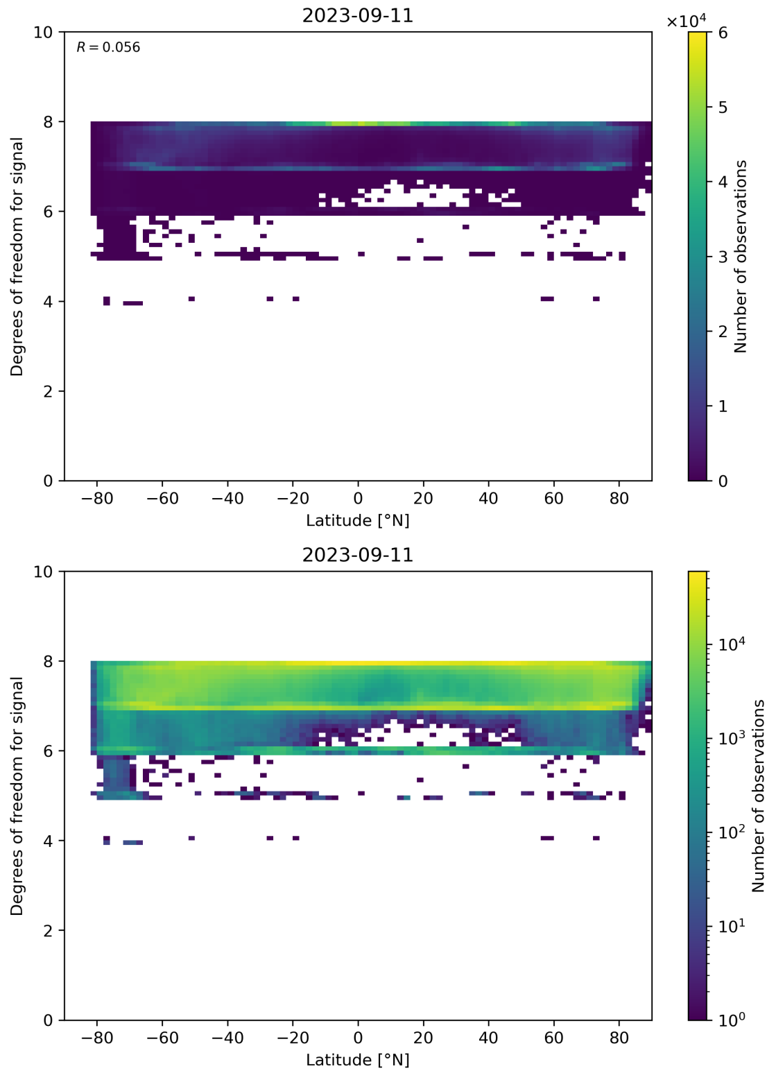
Figure 55: Scatter density plot of “Latitude” against “Degrees of freedom for signal” for 2023-09-10 to 2023-09-12.
