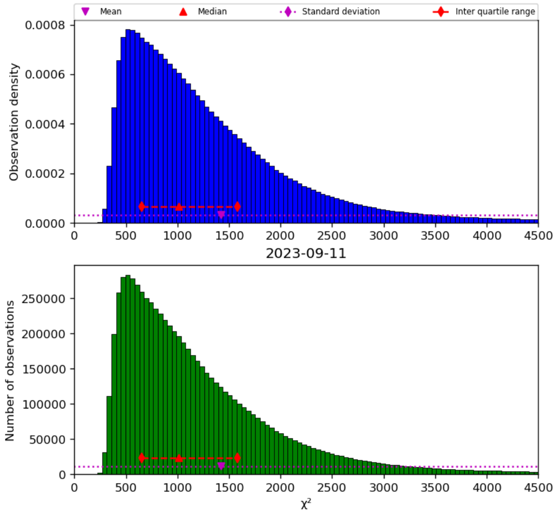
Figure 22: Histogram of “ \chi^2 ” for 2023-09-10 to 2023-09-12
