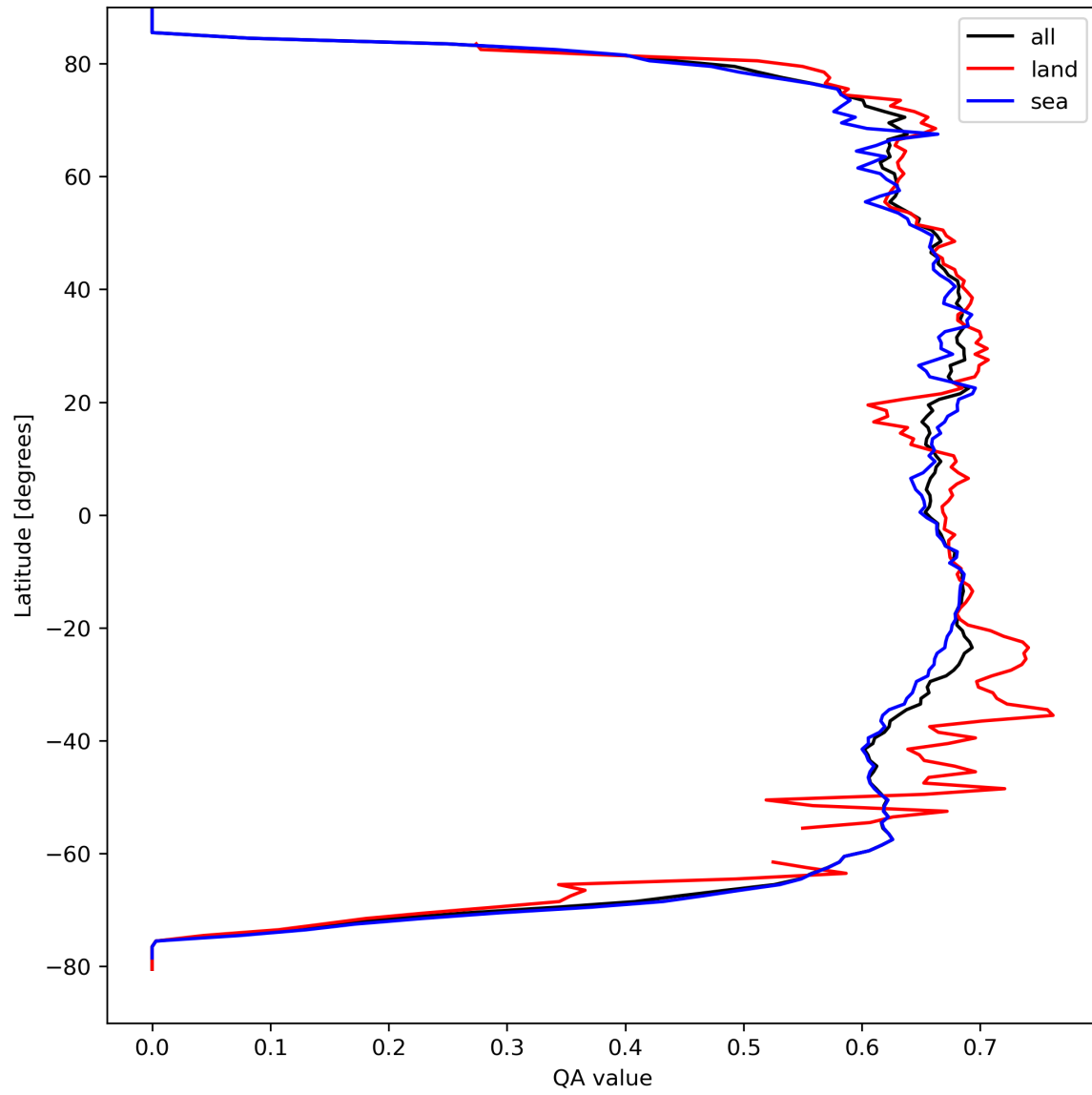
Figure 9: Zonal average of “QA value” for 2023-09-10 to 2023-09-12.
