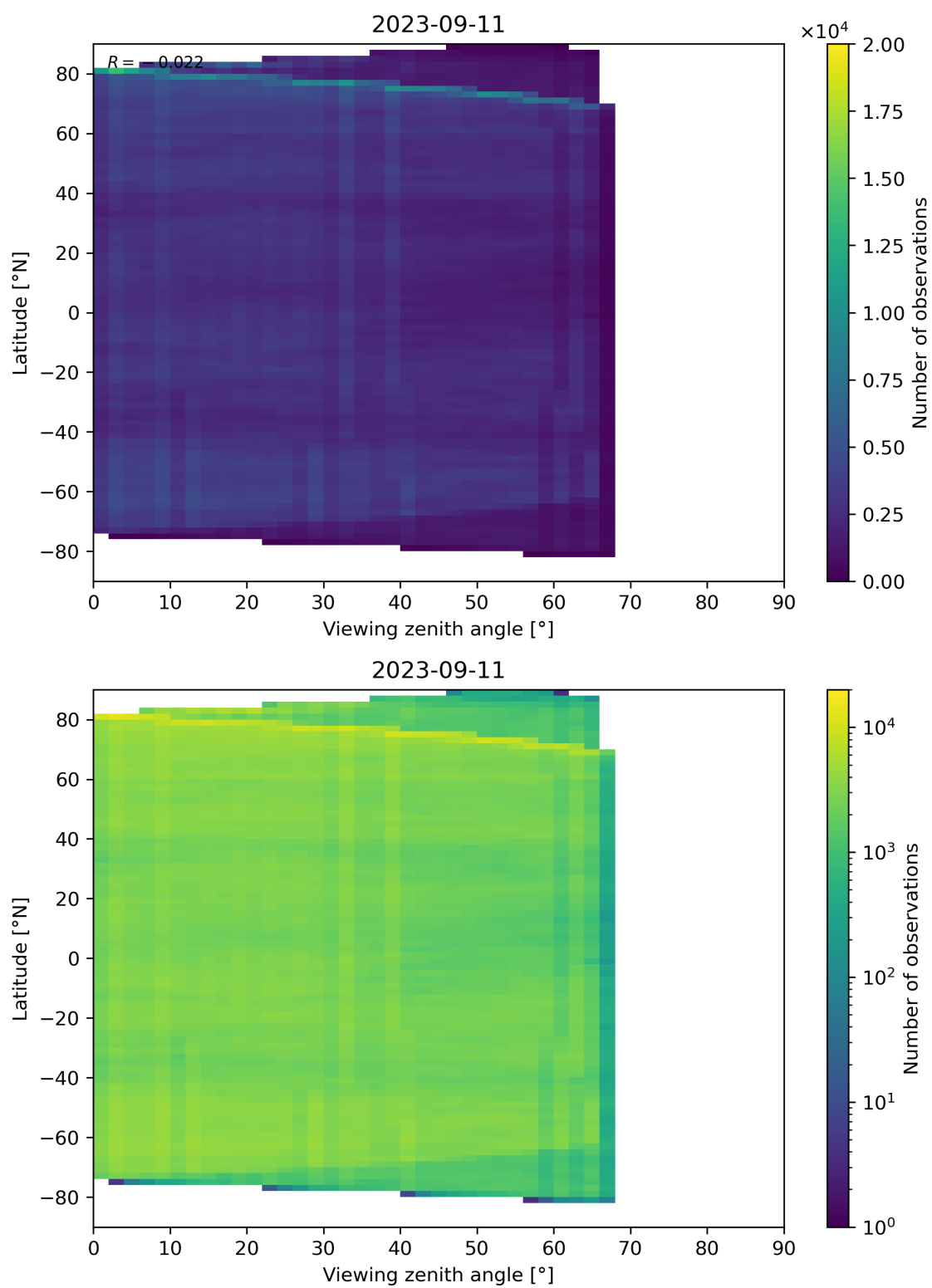
Figure 74: Scatter density plot of “Viewing zenith angle” against “Latitude” for 2023-09-10 to 2023-09-12.
