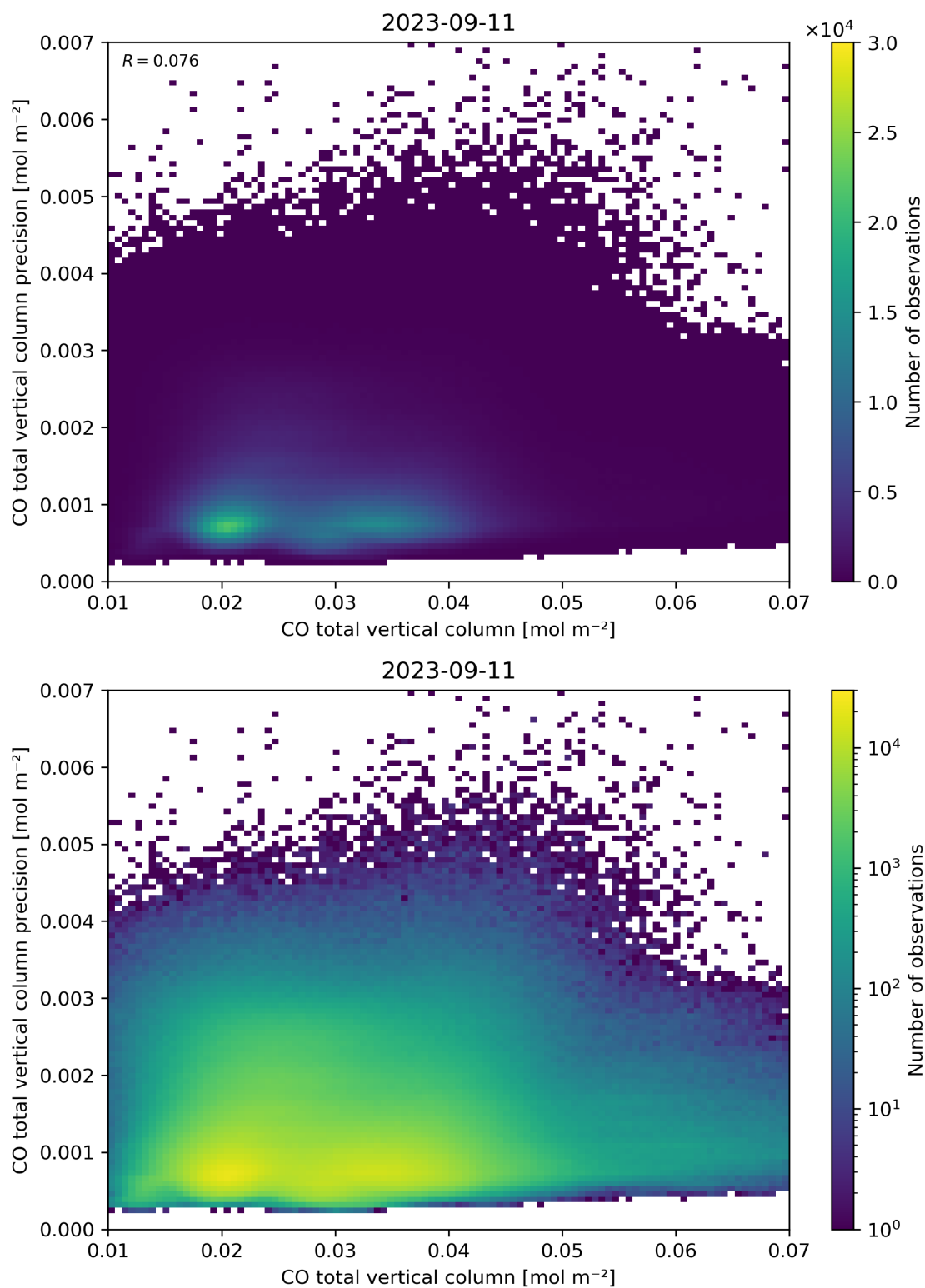
Figure 34: Scatter density plot of “CO total vertical column” against “CO total vertical column precision” for 2023-09-10 to 2023-09-12.
