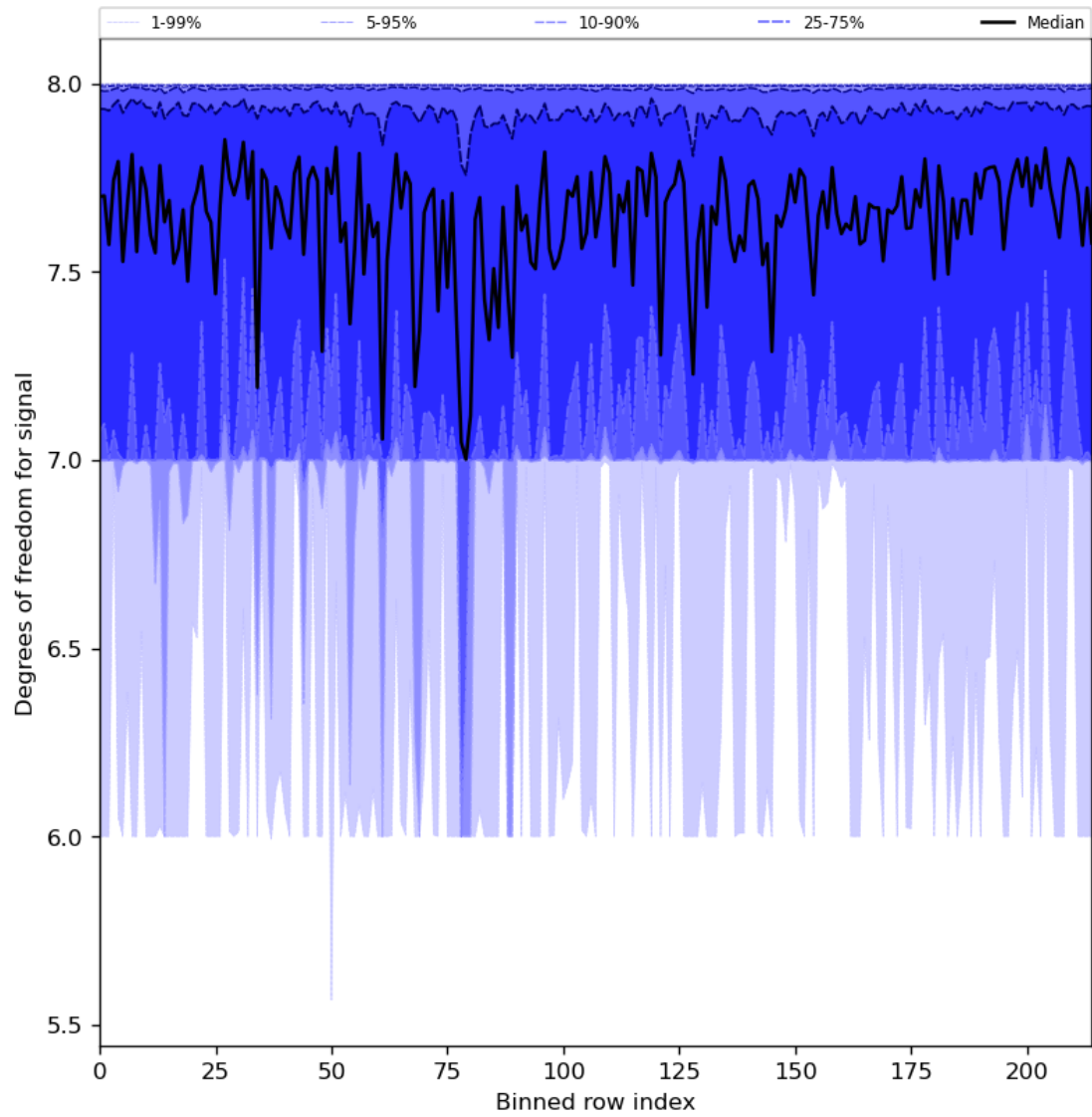
Figure 31: Along track statistics of “Degrees of freedom for signal” for 2023-09-10 to 2023-09-12
