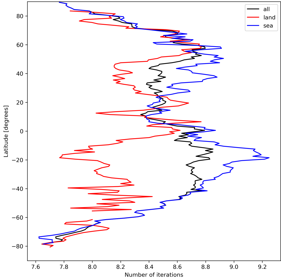
Figure 16: Zonal average of “Number of iterations” for 2023-09-10 to 2023-09-12.
