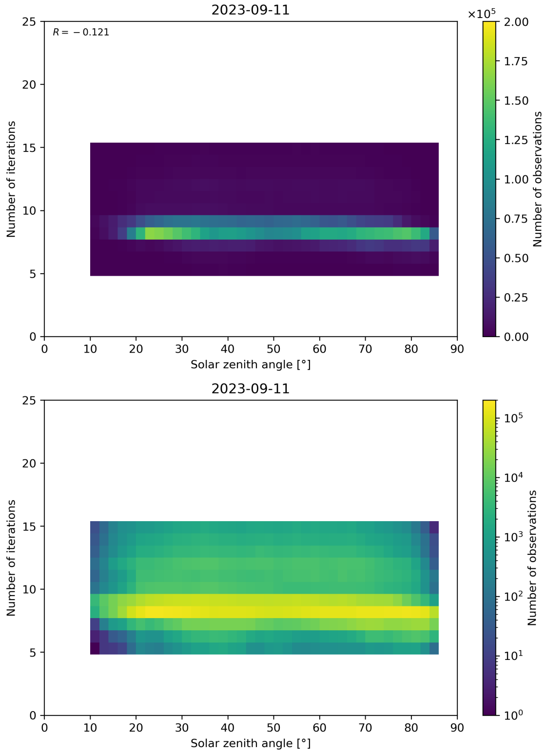
Figure 67: Scatter density plot of “Solar zenith angle” against “Number of iterations” for 2023-09-10 to 2023-09-12.
