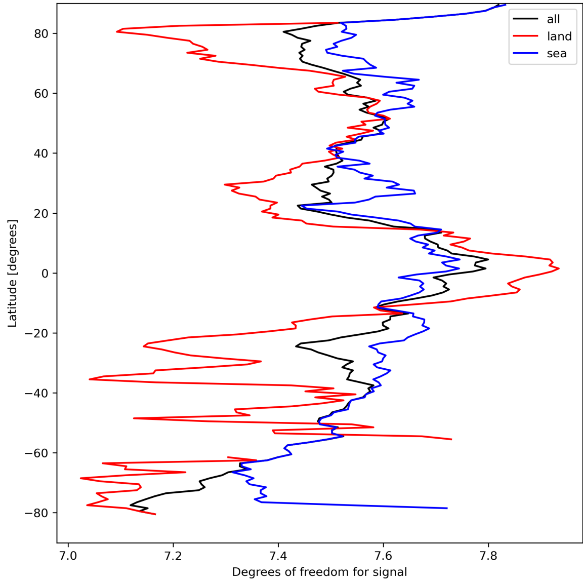
Figure 15: Zonal average of “Degrees of freedom for signal” for 2023-09-10 to 2023-09-12.
