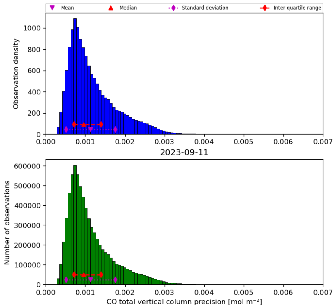
Figure 20: Histogram of “CO total vertical column precision” for 2023-09-10 to 2023-09-12
