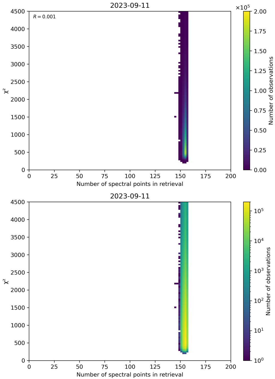
Figure 58: Scatter density plot of “Number of spectral points in retrieval” against “ \chi^2 ” for 2023-09-10 to 2023-09-12.
