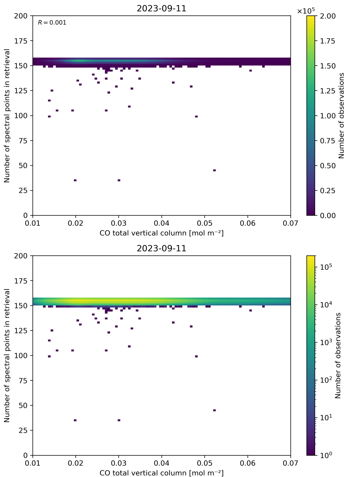
Figure 43: Scatter density plot of “CO total vertical column” against “Number of spectral points in retrieval” for 2023-09-10 to 2023-09-12.
