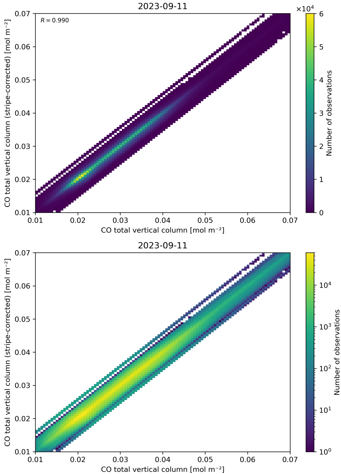
Figure 33: Scatter density plot of “CO total vertical column” against “CO total vertical column (stripe-corrected)” for 2023-09-10 to 2023-09-12.
