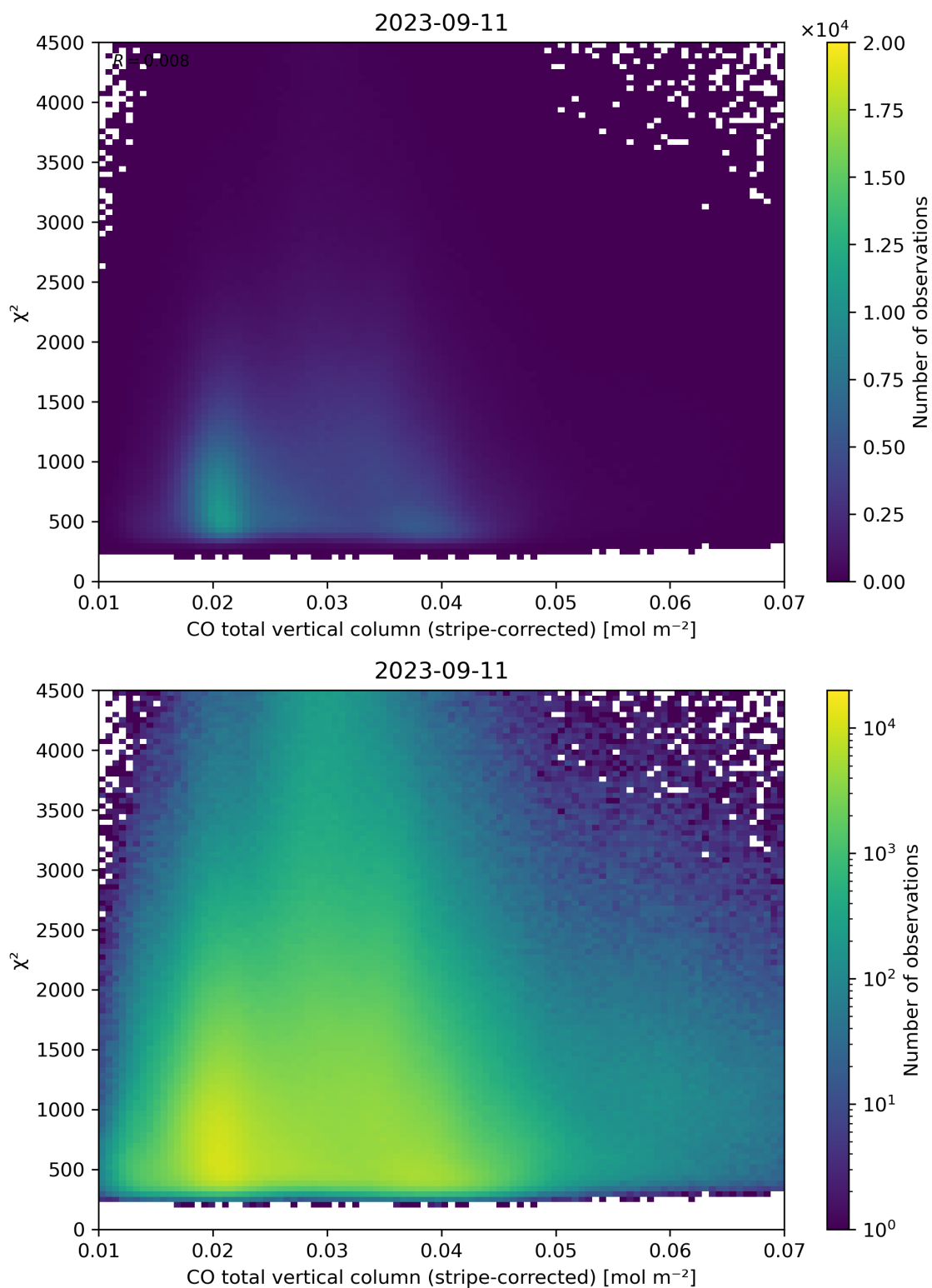
Figure 37: Scatter density plot of “CO total vertical column (stripe-corrected)” against “ \chi^2 ” for 2023-09-10 to 2023-09-12.
