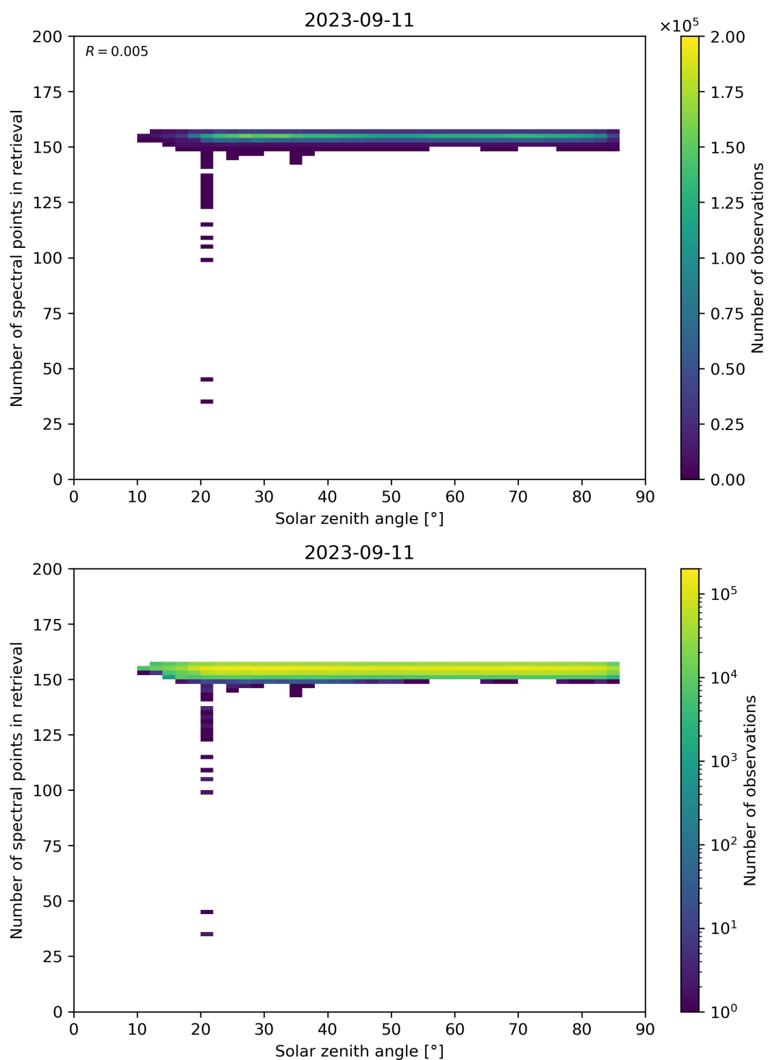
Figure 68: Scatter density plot of “Solar zenith angle” against “Number of spectral points in retrieval” for 2023-09-10 to 2023-09-12.
