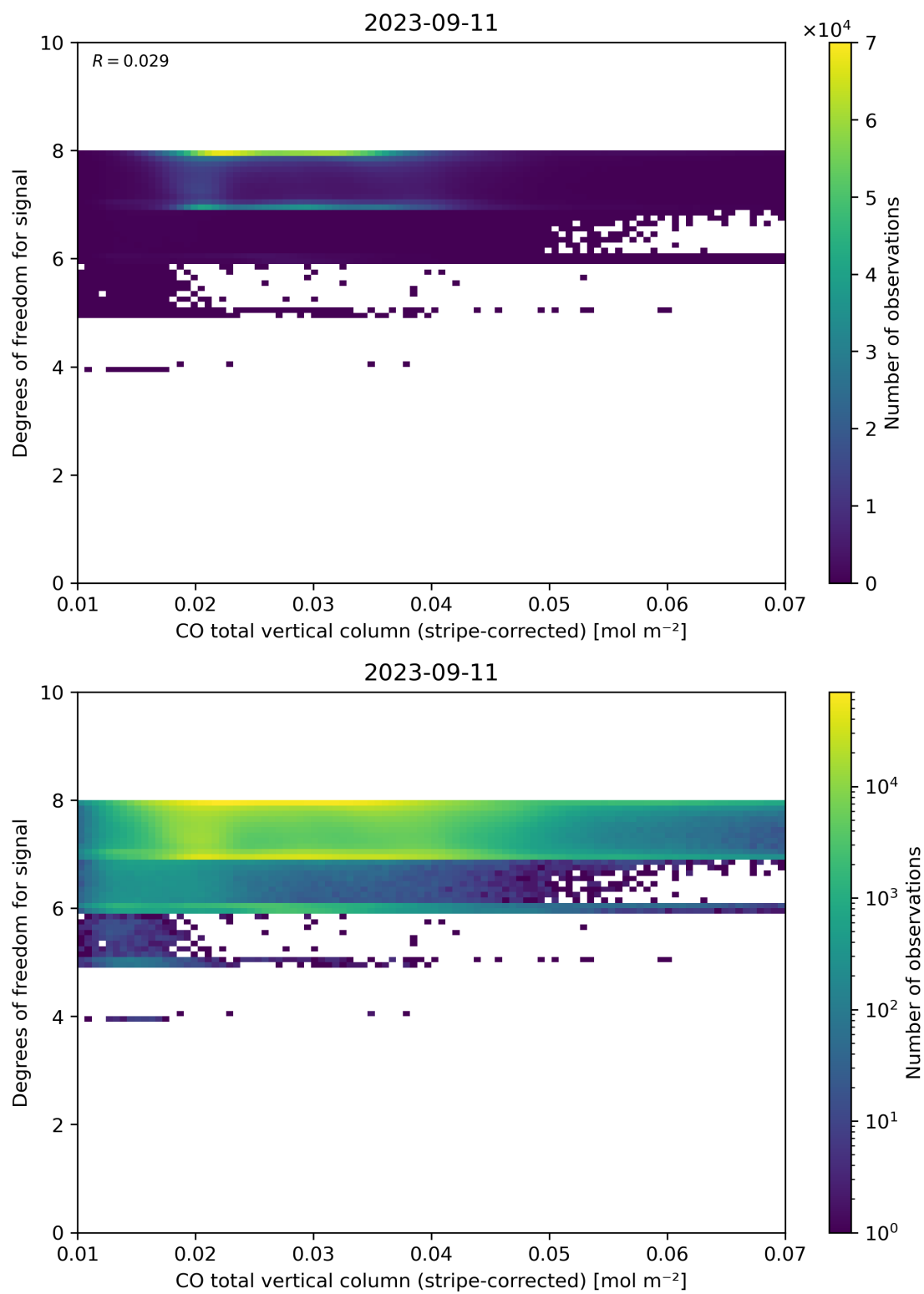
Figure 38: Scatter density plot of “CO total vertical column (stripe-corrected)” against “Degrees of freedom for signal” for 2023-09-10 to 2023-09-12.
