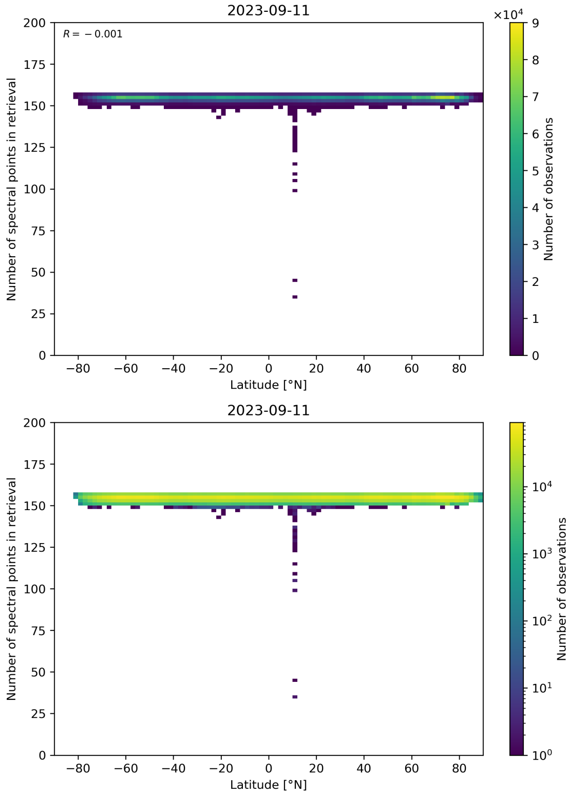
Figure 57: Scatter density plot of “Latitude” against “Number of spectral points in retrieval” for 2023-09-10 to 2023-09-12.
