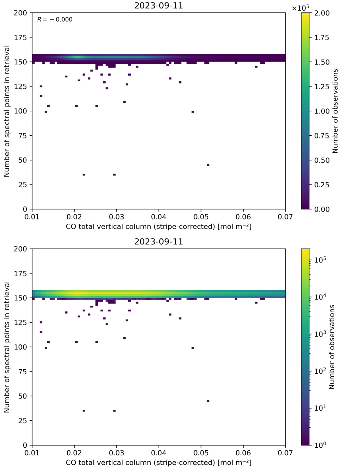
Figure 40: Scatter density plot of “CO total vertical column (stripe-corrected)” against “Number of spectral points in retrieval” for 2023-09-10 to 2023-09-12.
