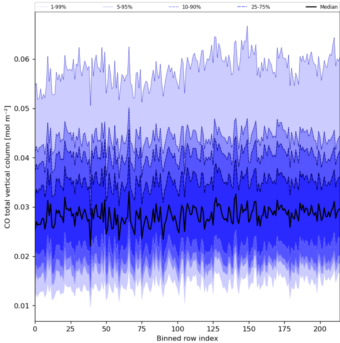
Figure 26: Along track statistics of “CO total vertical column” for 2023-09-10 to 2023-09-12
