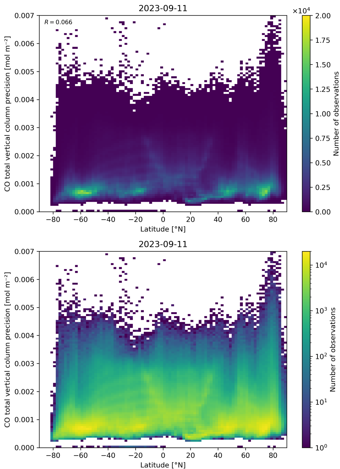
Figure 53: Scatter density plot of “Latitude” against “CO total vertical column precision” for 2023-09-10 to 2023-09-12.
