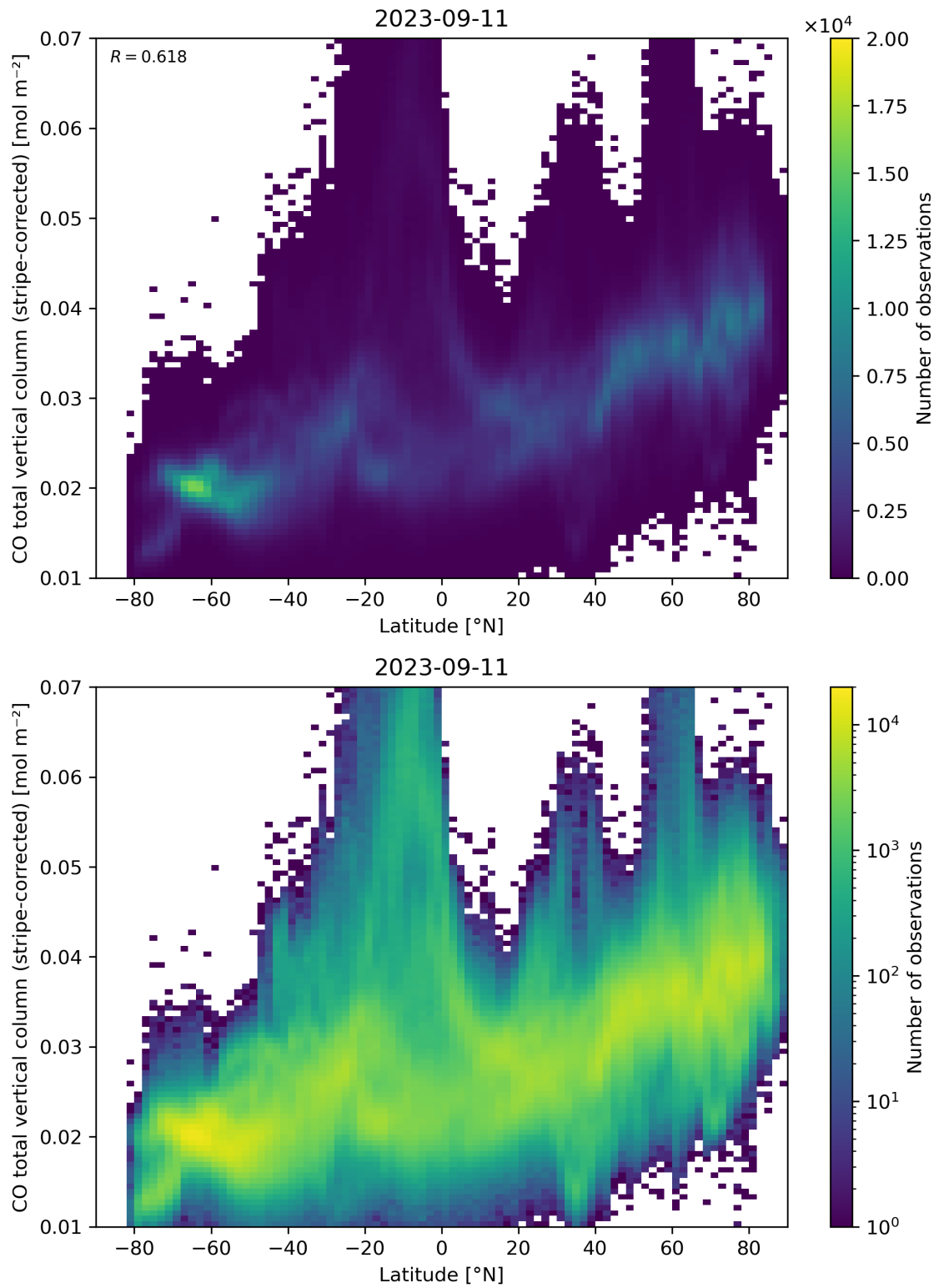
Figure 52: Scatter density plot of “Latitude” against “CO total vertical column (stripe-corrected)” for 2023-09-10 to 2023-09-12.
