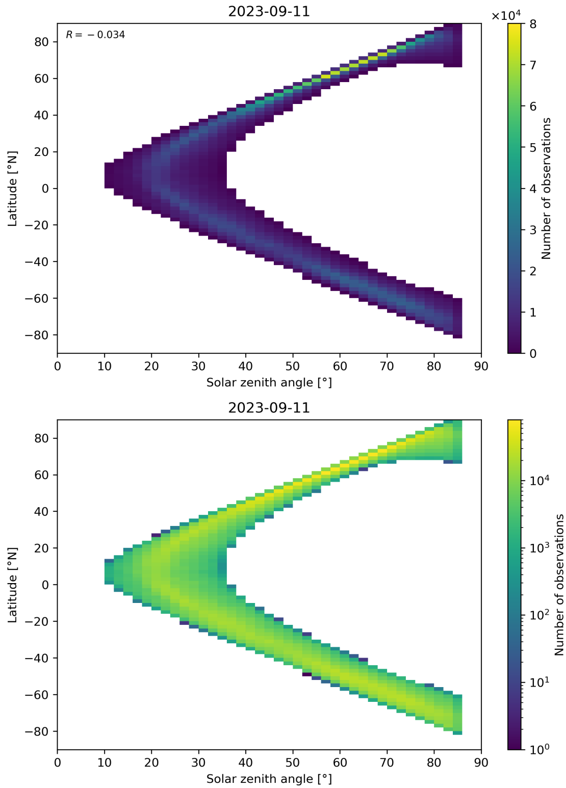
Figure 66: Scatter density plot of “Solar zenith angle” against “Latitude” for 2023-09-10 to 2023-09-12.
