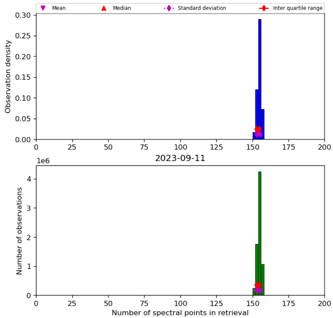
Figure 21: Histogram of “Number of spectral points in retrieval” for 2023-09-10 to 2023-09-12
