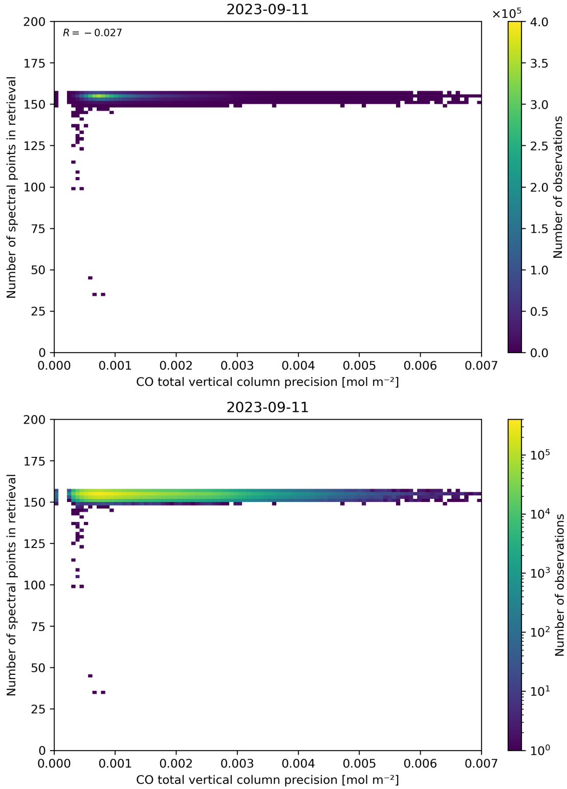
Figure 47: Scatter density plot of “CO total vertical column precision” against “Number of spectral points in retrieval” for 2023-09-10 to 2023-09-12.
