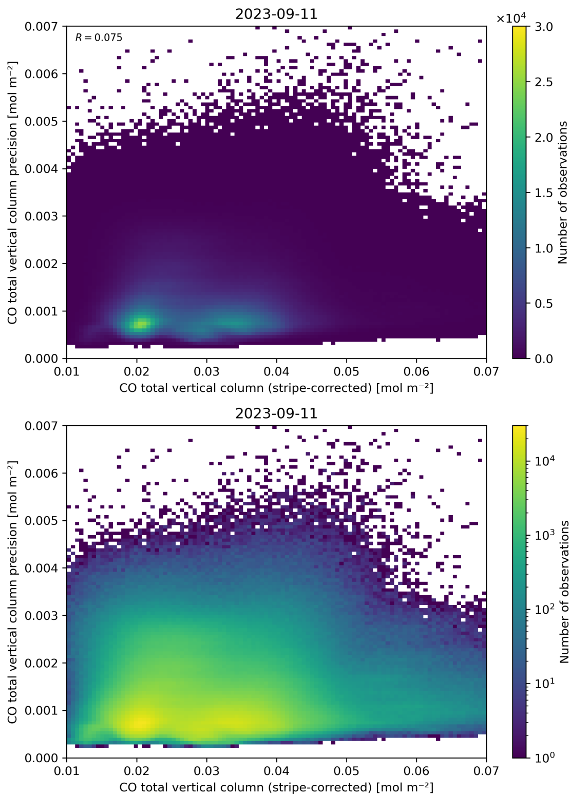
Figure 36: Scatter density plot of “CO total vertical column (stripe-corrected)” against “CO total vertical column precision” for 2023-09-10 to 2023-09-12.
