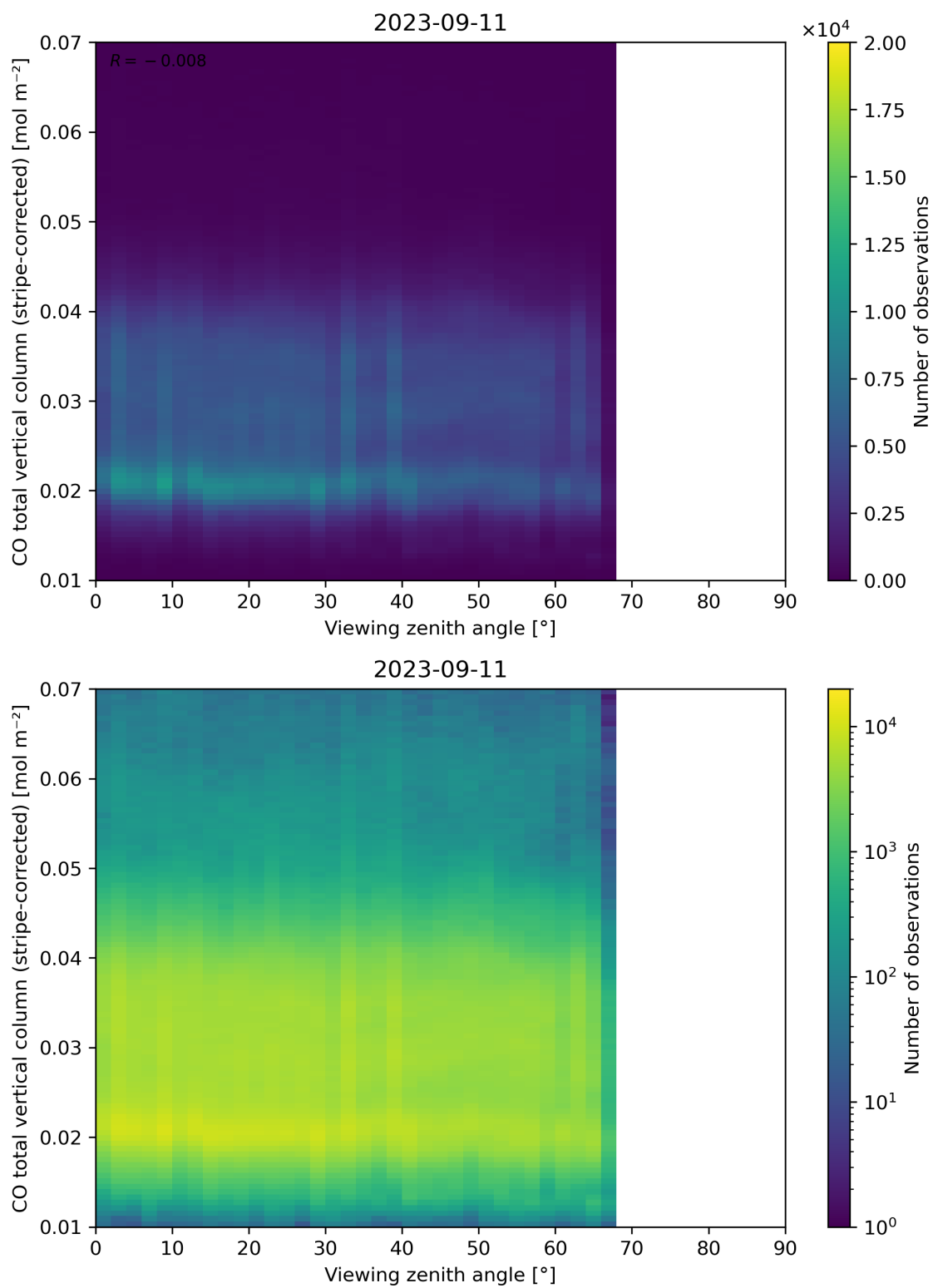
Figure 70: Scatter density plot of “Viewing zenith angle” against “CO total vertical column (stripe-corrected)” for 2023-09-10 to 2023-09-12.
