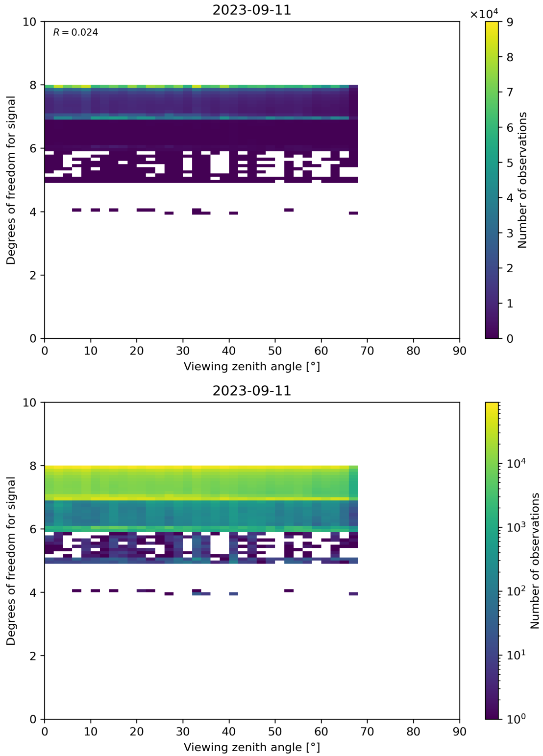
Figure 73: Scatter density plot of “Viewing zenith angle” against “Degrees of freedom for signal” for 2023-09-10 to 2023-09-12.
