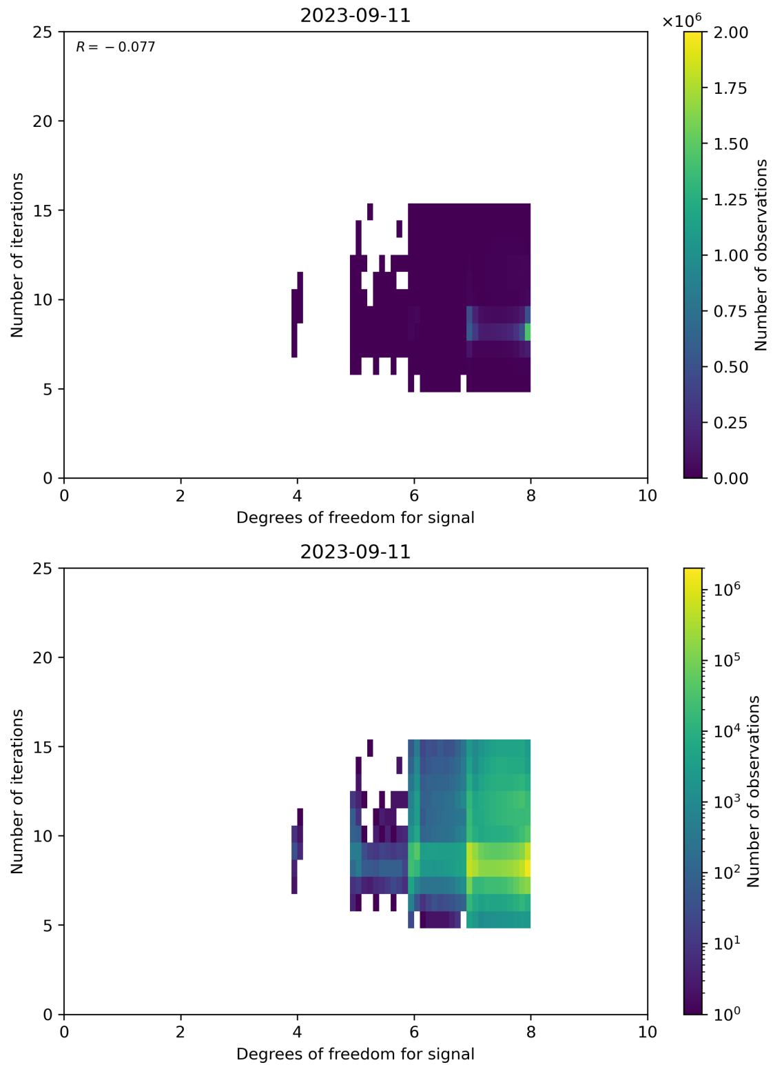
Figure 50: Scatter density plot of “Degrees of freedom for signal” against “Number of iterations” for 2023-09-10 to 2023-09-12.
