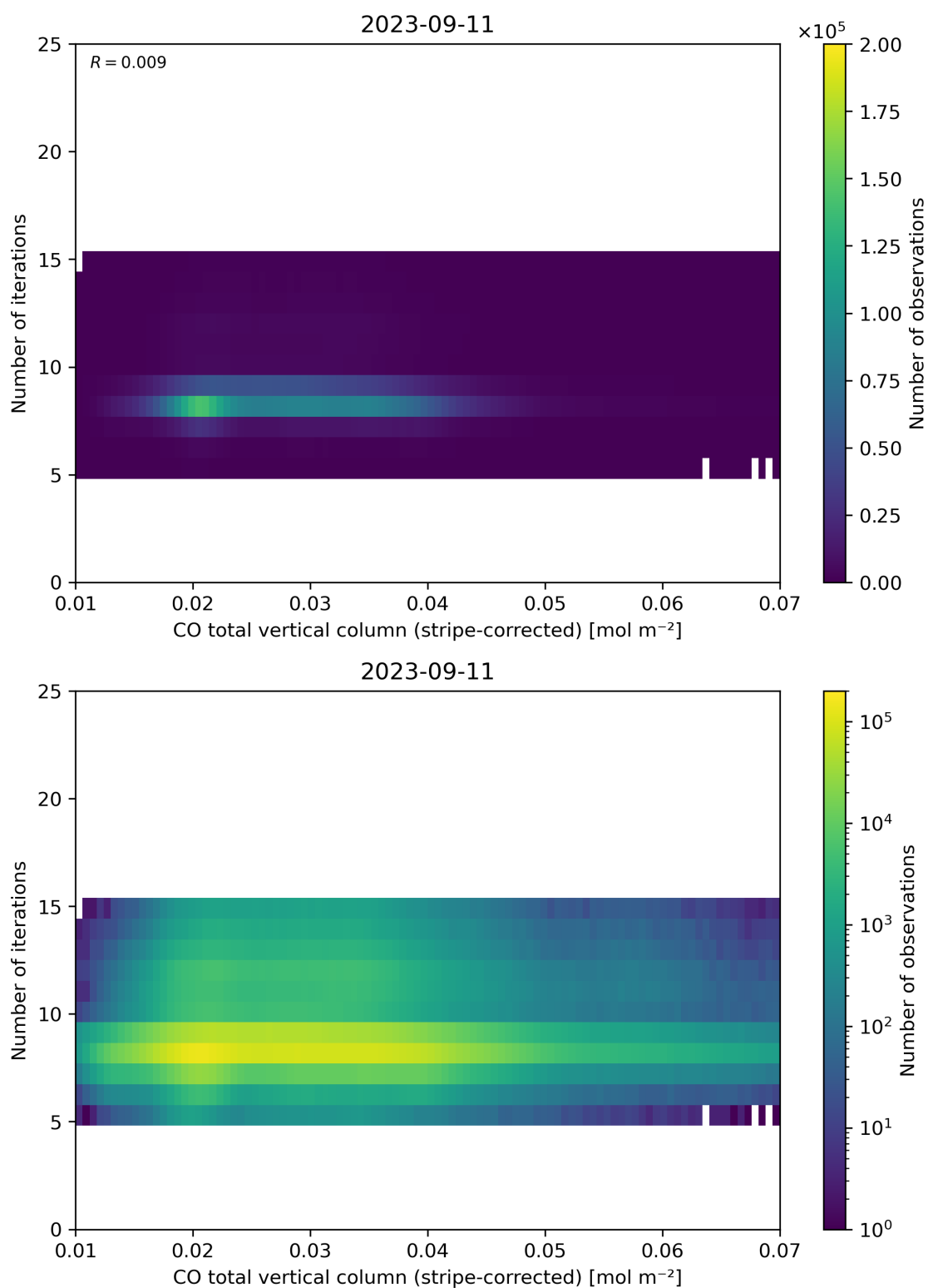
Figure 39: Scatter density plot of “CO total vertical column (stripe-corrected)” against “Number of iterations” for 2023-09-10 to 2023-09-12.
