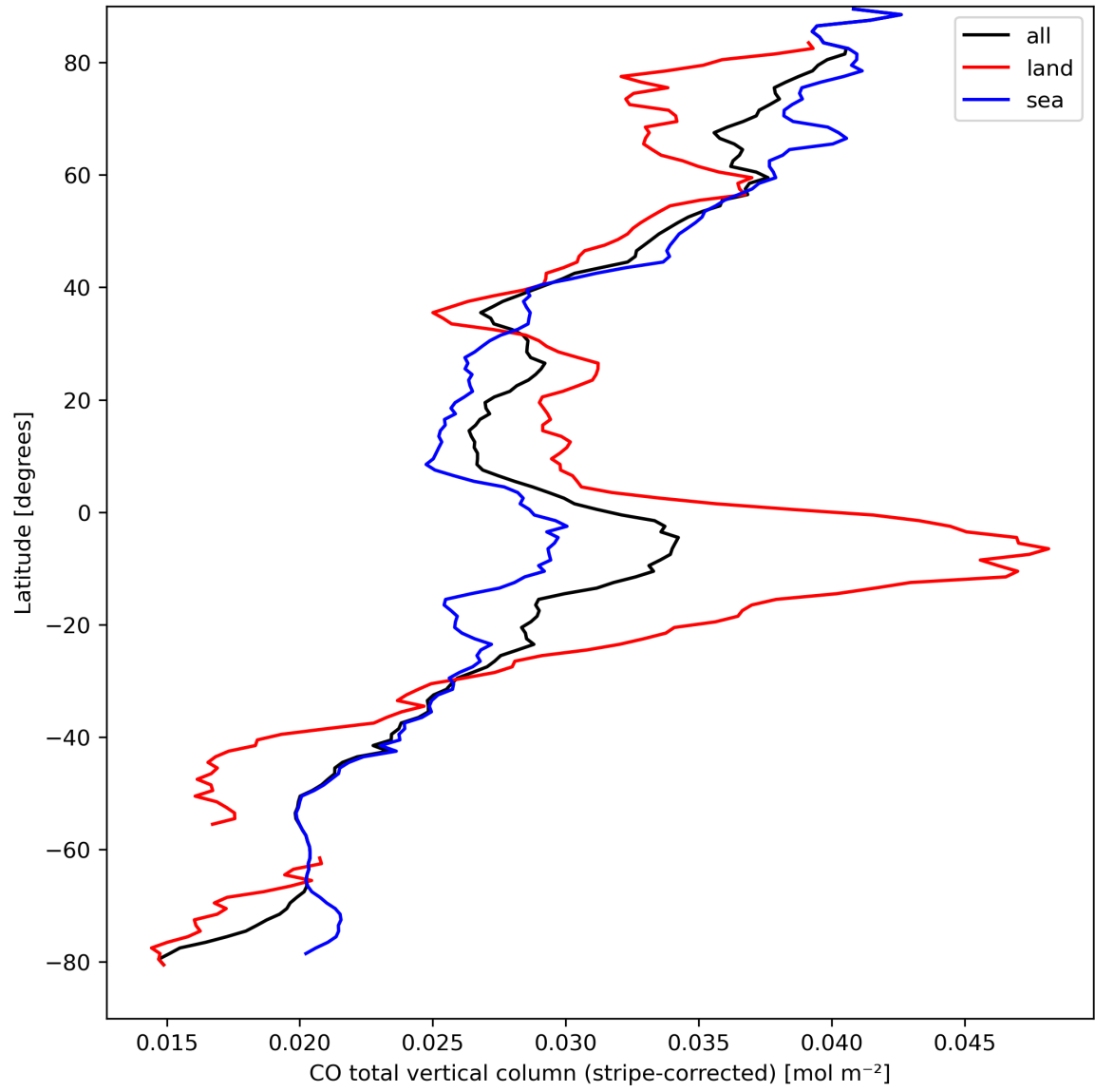
Figure 11: Zonal average of “CO total vertical column (stripe-corrected)” for 2023-09-10 to 2023-09-12.
