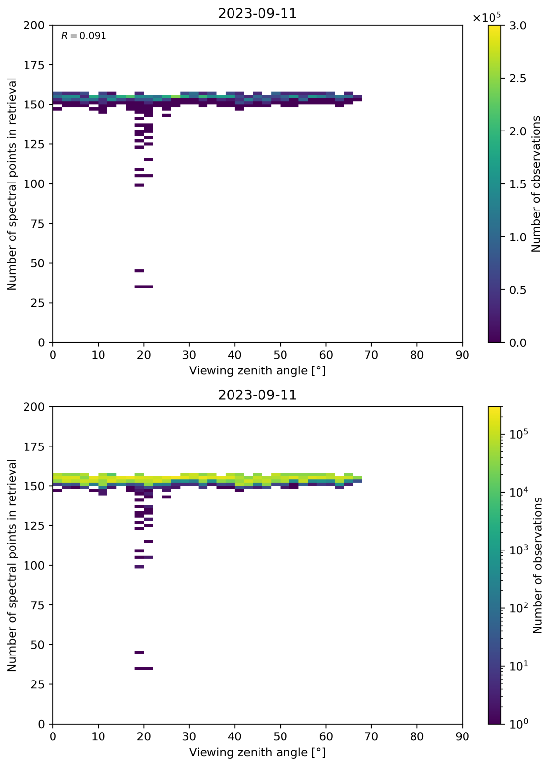
Figure 76: Scatter density plot of “Viewing zenith angle” against “Number of spectral points in retrieval” for 2023-09-10 to 2023-09-12.
