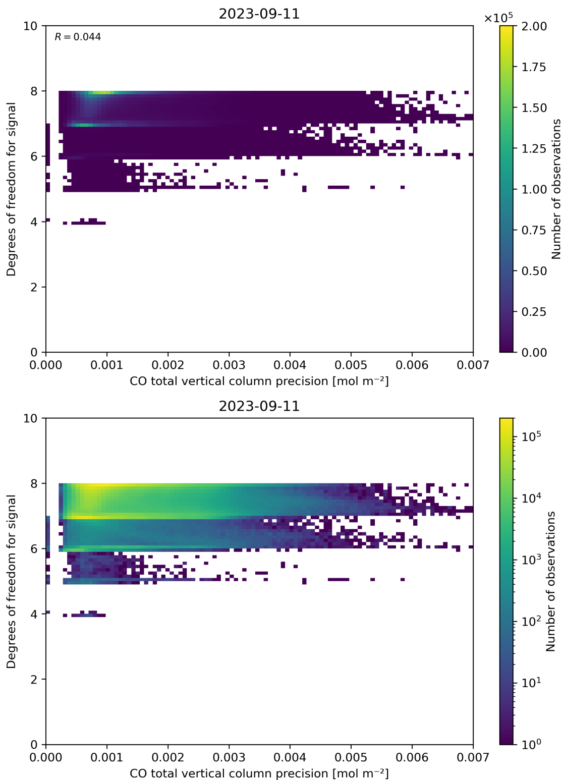
Figure 45: Scatter density plot of “CO total vertical column precision” against “Degrees of freedom for signal” for 2023-09-10 to 2023-09-12.
