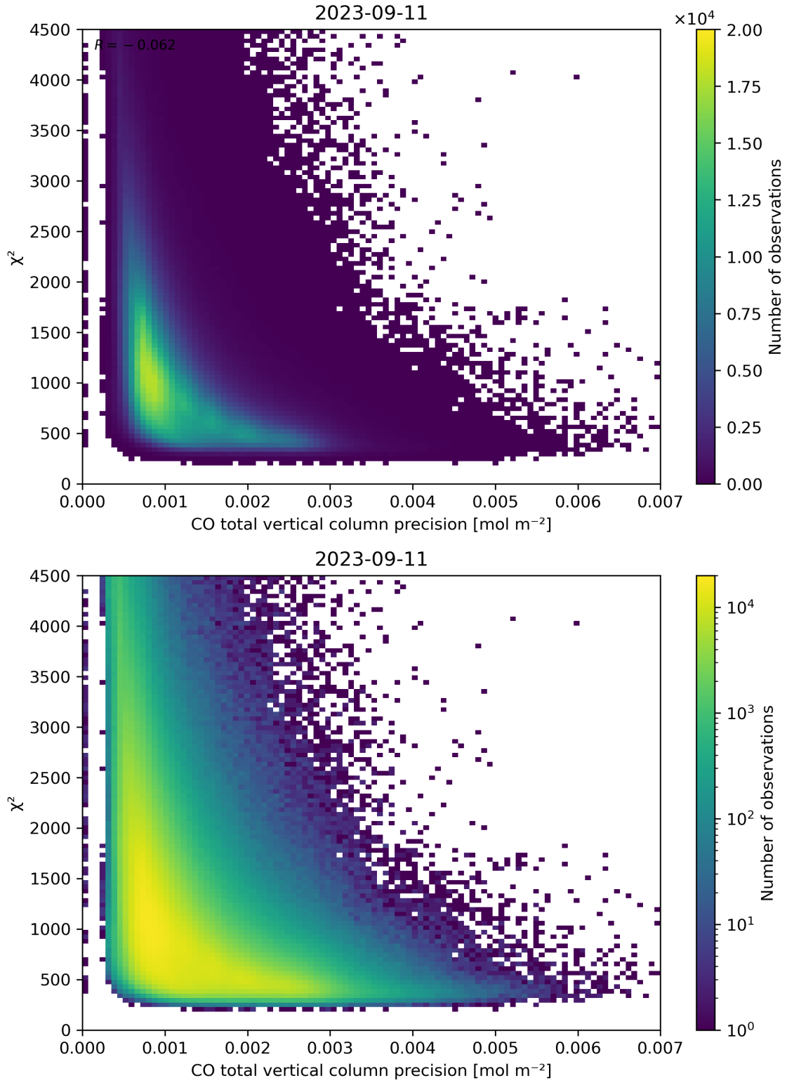
Figure 44: Scatter density plot of “CO total vertical column precision” against “ \chi^2 ” for 2023-09-10 to 2023-09-12.
