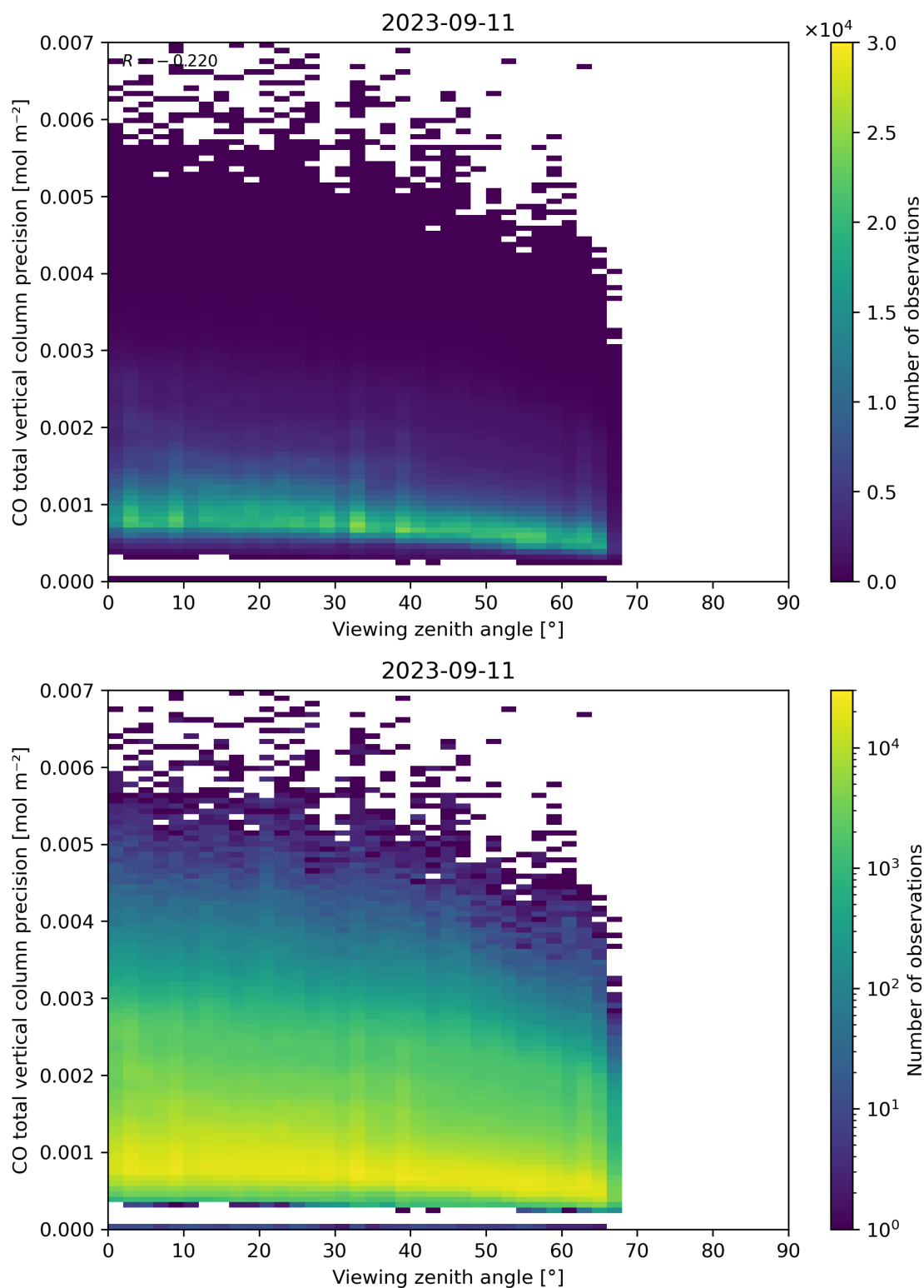
Figure 71: Scatter density plot of “Viewing zenith angle” against “CO total vertical column precision” for 2023-09-10 to 2023-09-12.
