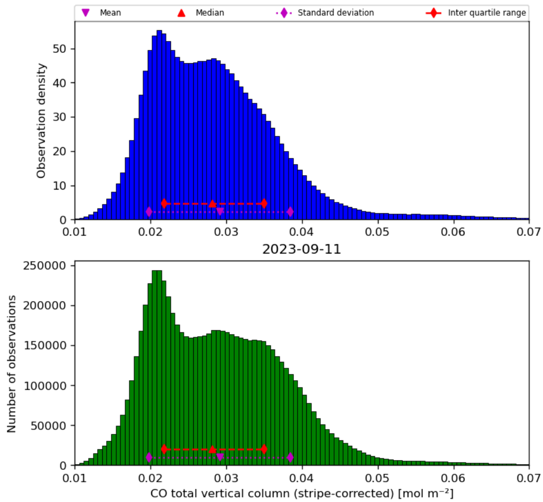
Figure 19: Histogram of “CO total vertical column (stripe-corrected)” for 2023-09-10 to 2023-09-12
