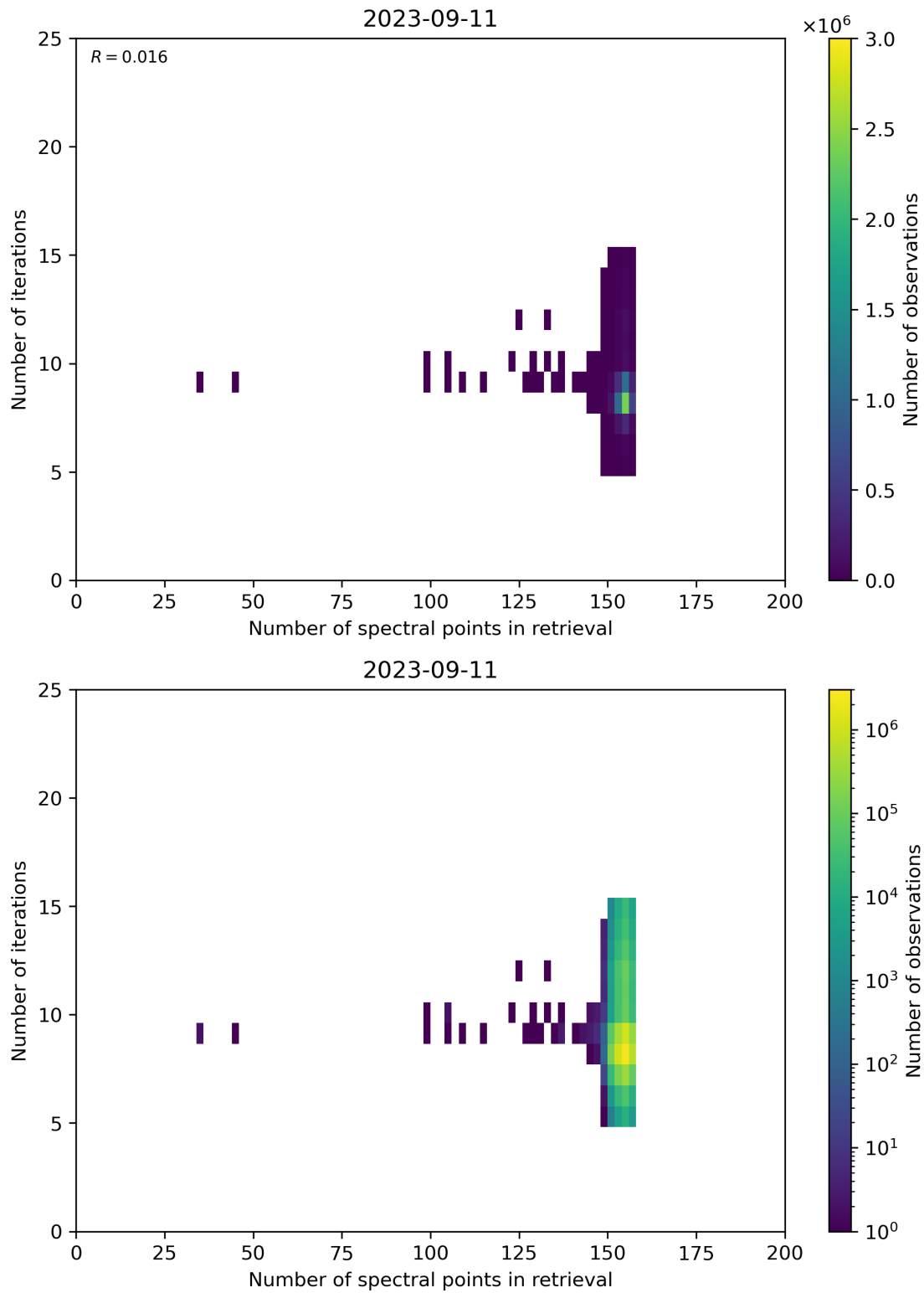
Figure 60: Scatter density plot of “Number of spectral points in retrieval” against “Number of iterations” for 2023-09-10 to 2023-09-12.
