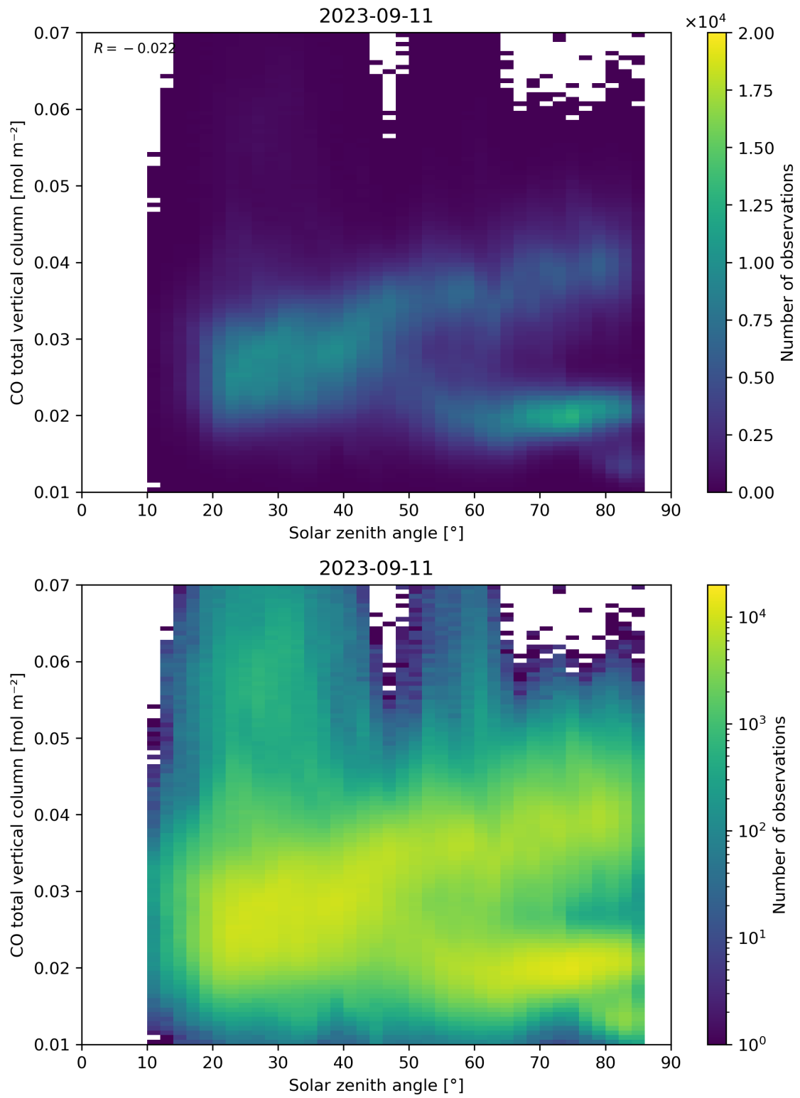
Figure 61: Scatter density plot of “Solar zenith angle” against “CO total vertical column” for 2023-09-10 to 2023-09-12.
