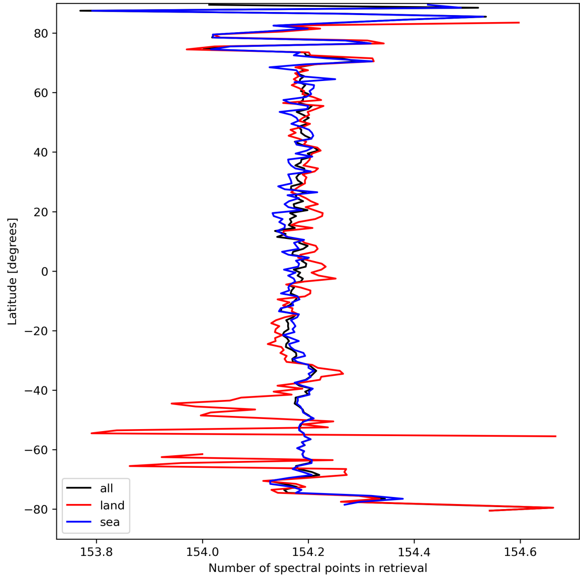
Figure 13: Zonal average of “Number of spectral points in retrieval” for 2023-09-10 to 2023-09-12.
