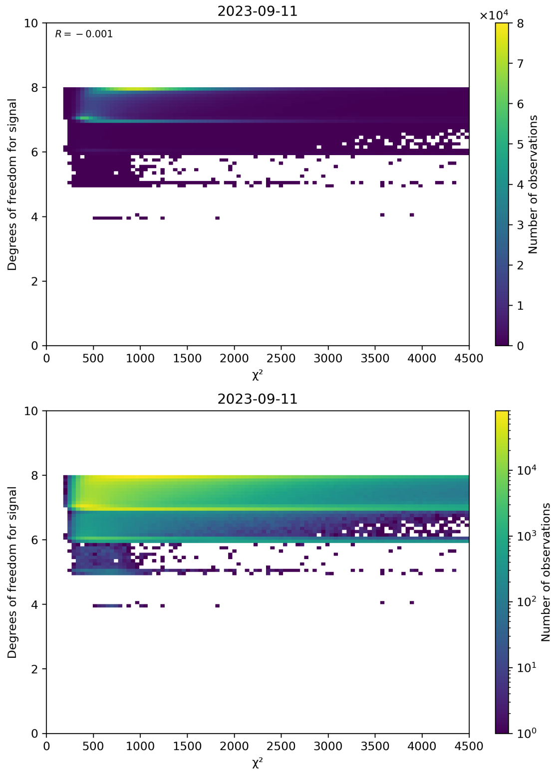
Figure 48: Scatter density plot of “ \chi^2 ” against “Degrees of freedom for signal” for 2023-09-10 to 2023-09-12.
