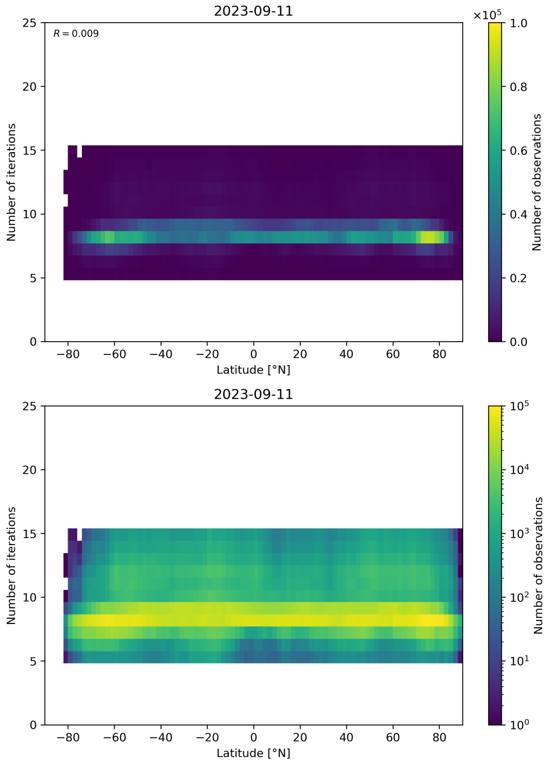
Figure 56: Scatter density plot of “Latitude” against “Number of iterations” for 2023-09-10 to 2023-09-12.
