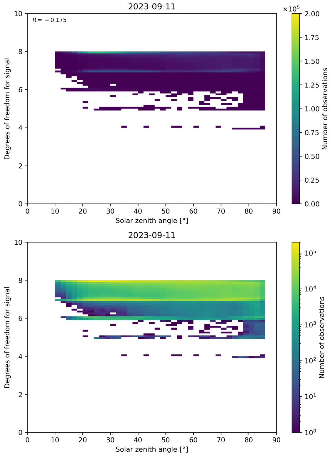
Figure 65: Scatter density plot of “Solar zenith angle” against “Degrees of freedom for signal” for 2023-09-10 to 2023-09-12.
