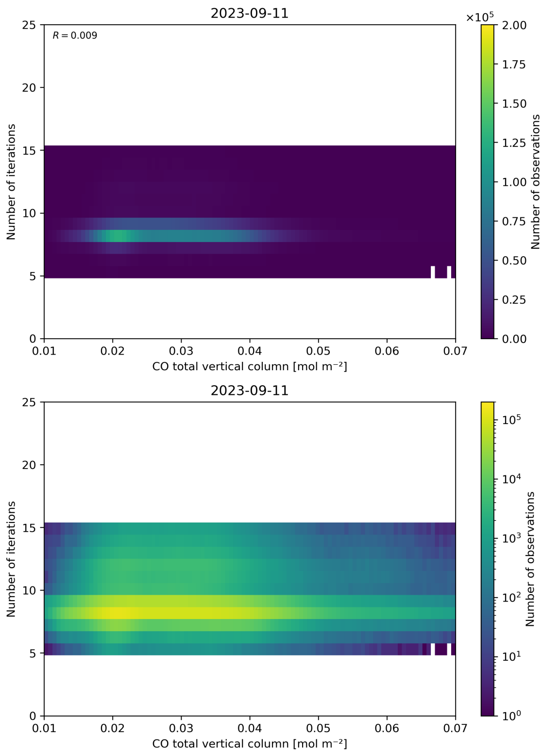
Figure 42: Scatter density plot of “CO total vertical column” against “Number of iterations” for 2023-09-10 to 2023-09-12.
