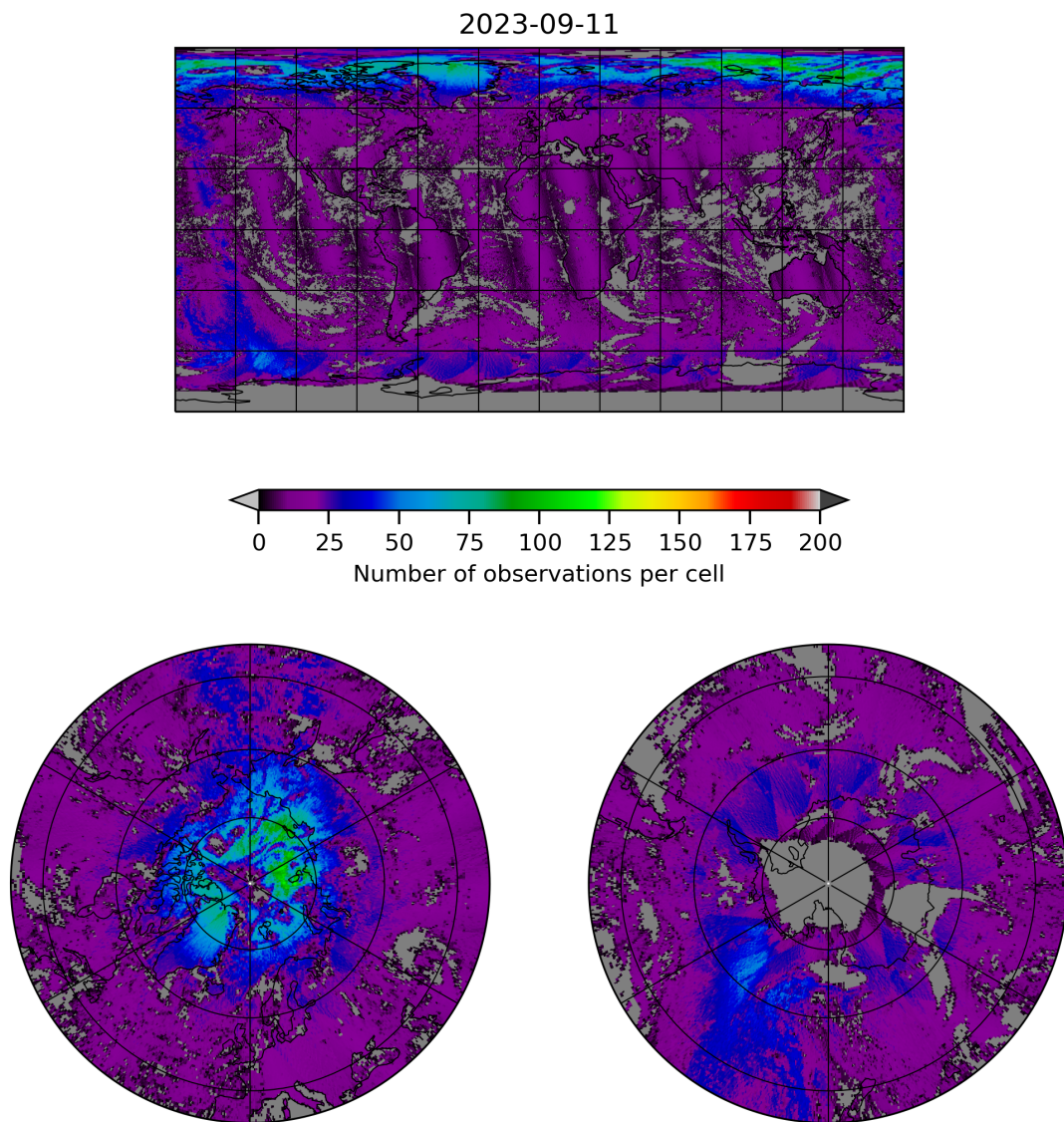
Figure 8: Map of the number of observations for 2023-09-10 to 2023-09-12
