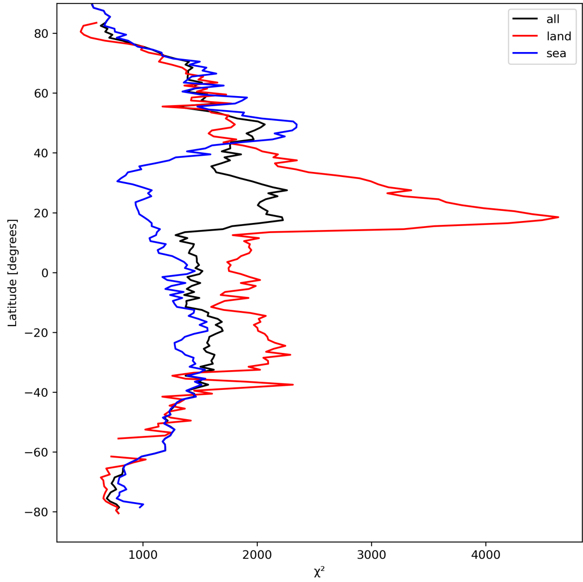
Figure 14: Zonal average of “ \chi^2 ” for 2023-09-10 to 2023-09-12.
