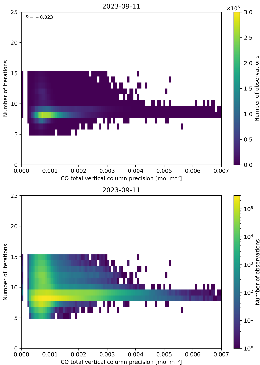
Figure 46: Scatter density plot of “CO total vertical column precision” against “Number of iterations” for 2023-09-10 to 2023-09-12.
