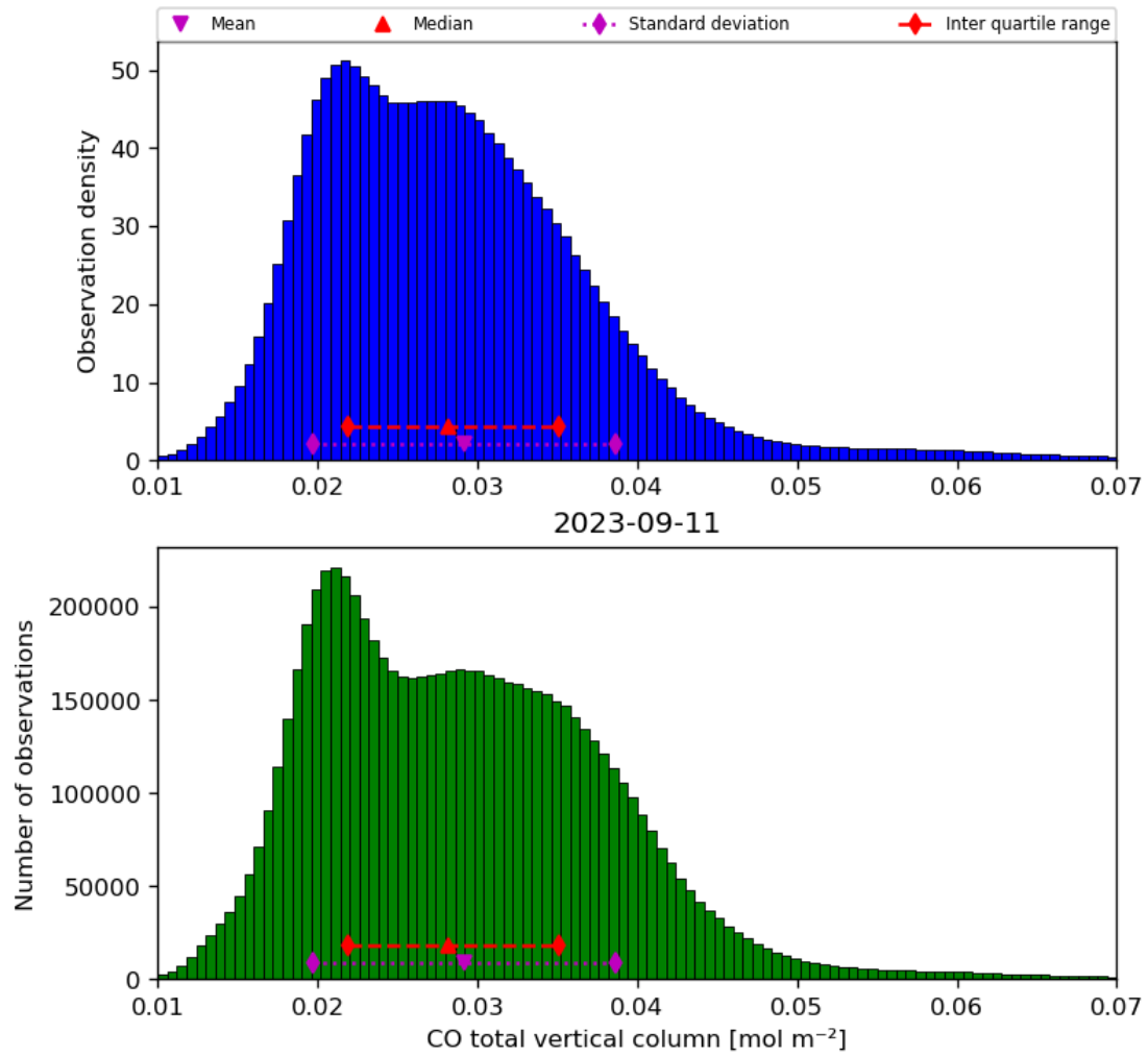
Figure 18: Histogram of “CO total vertical column” for 2023-09-10 to 2023-09-12
