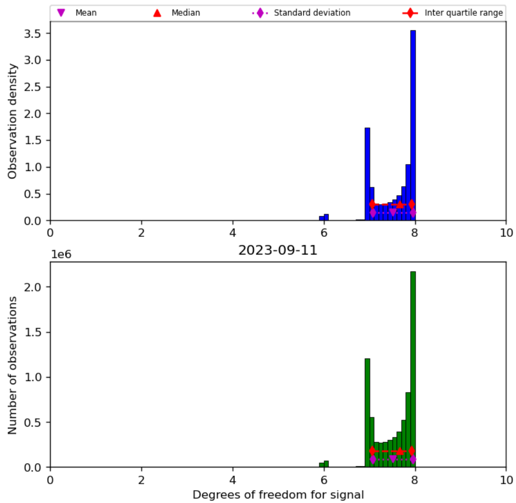
Figure 23: Histogram of “Degrees of freedom for signal” for 2023-09-10 to 2023-09-12
