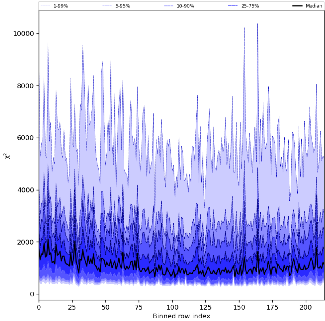
Figure 30: Along track statistics of “ \chi^2 ” for 2023-09-10 to 2023-09-12
