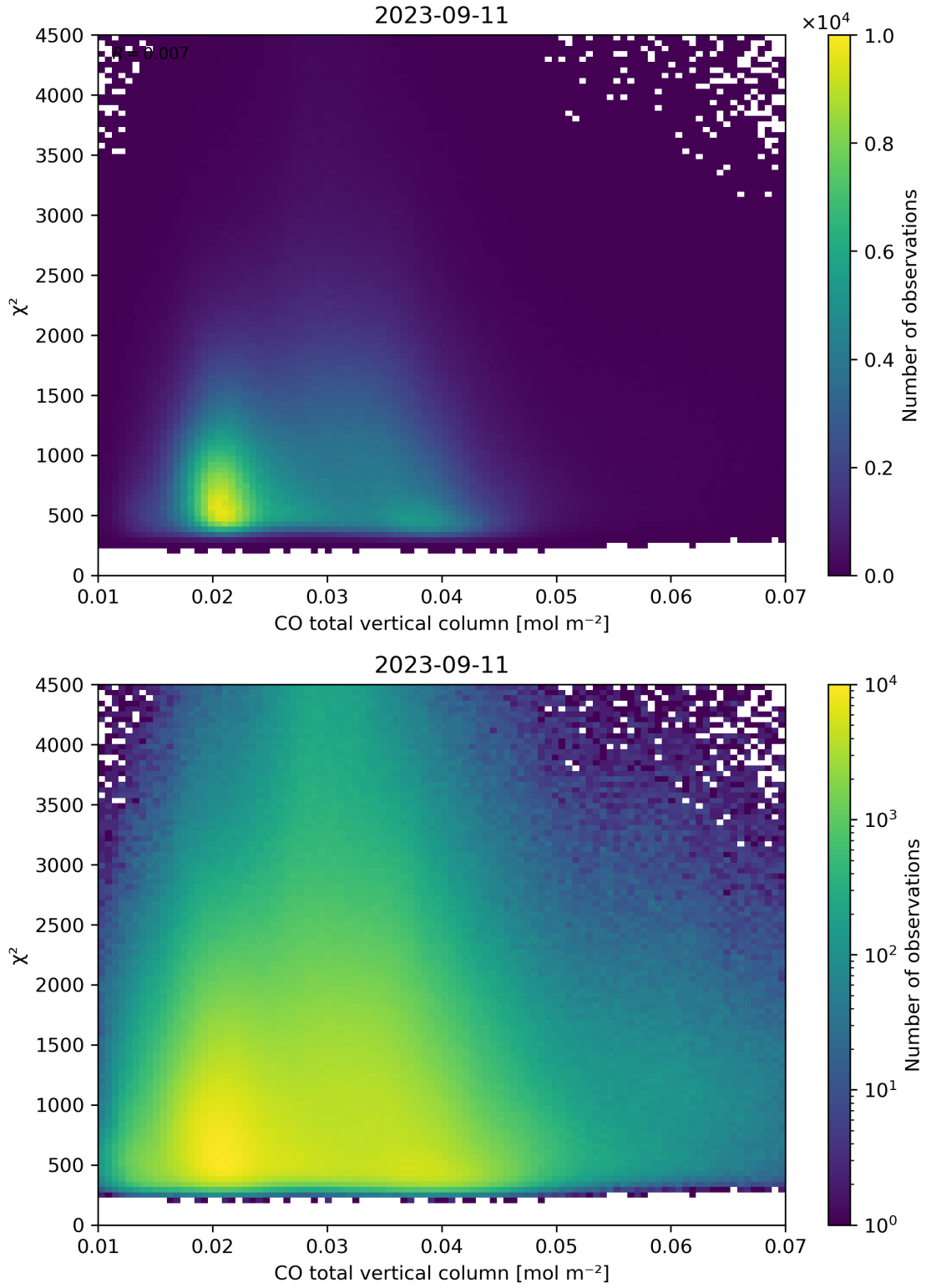
Figure 35: Scatter density plot of “CO total vertical column” against “ \chi^2 ” for 2023-09-10 to 2023-09-12.
