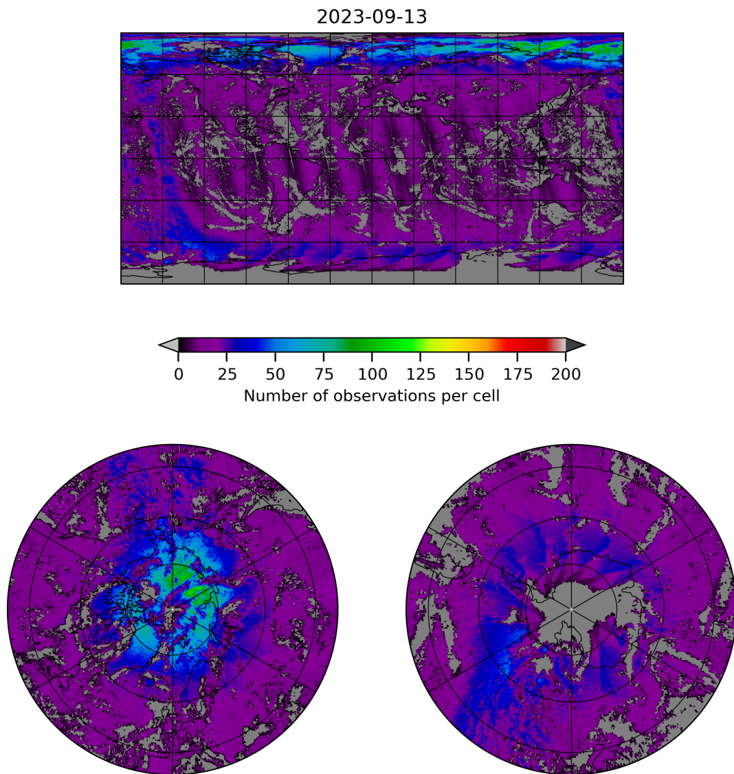
Figure 8: Map of the number of observations for 2023-09-12 to 2023-09-14
