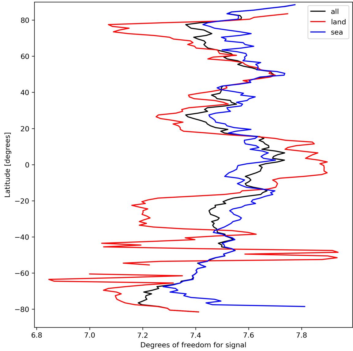
Figure 15: Zonal average of “Degrees of freedom for signal” for 2023-09-12 to 2023-09-14.
