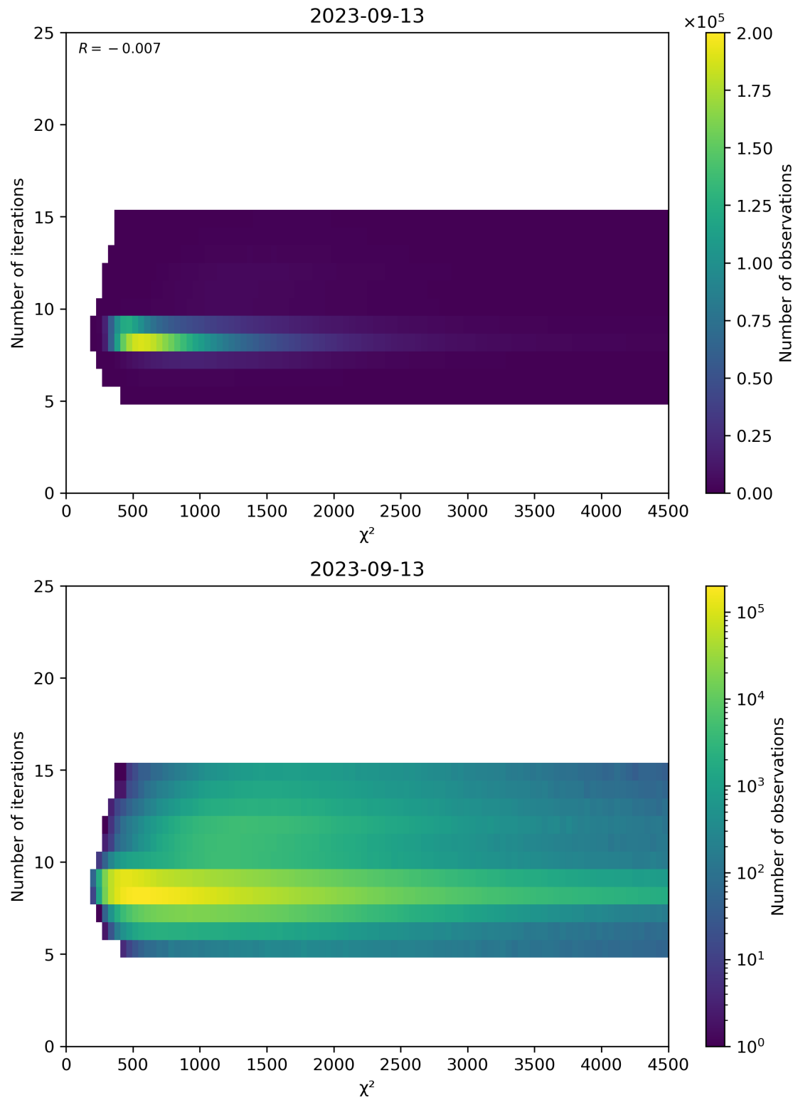
Figure 49: Scatter density plot of “ \chi^2 ” against “Number of iterations” for 2023-09-12 to 2023-09-14.
