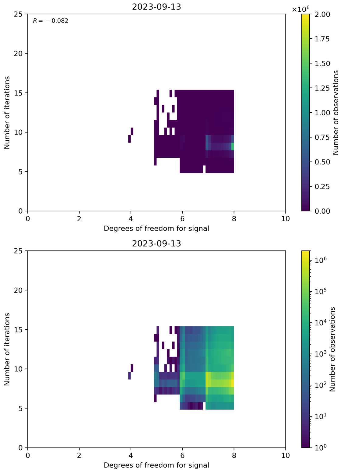
Figure 50: Scatter density plot of “Degrees of freedom for signal” against “Number of iterations” for 2023-09-12 to 2023-09-14.
