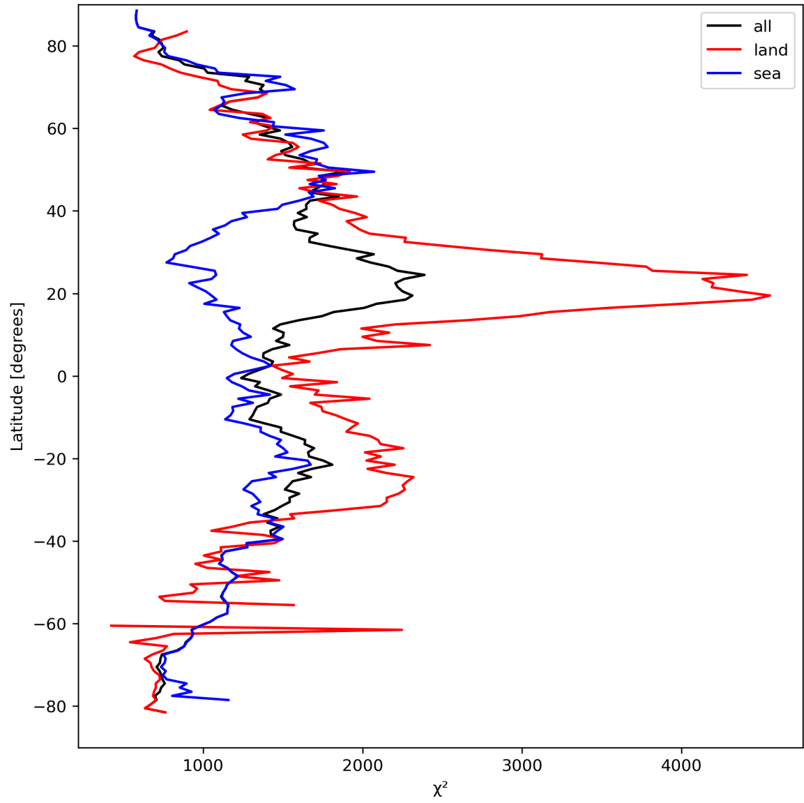
Figure 14: Zonal average of “ \chi^2 ” for 2023-09-12 to 2023-09-14.
