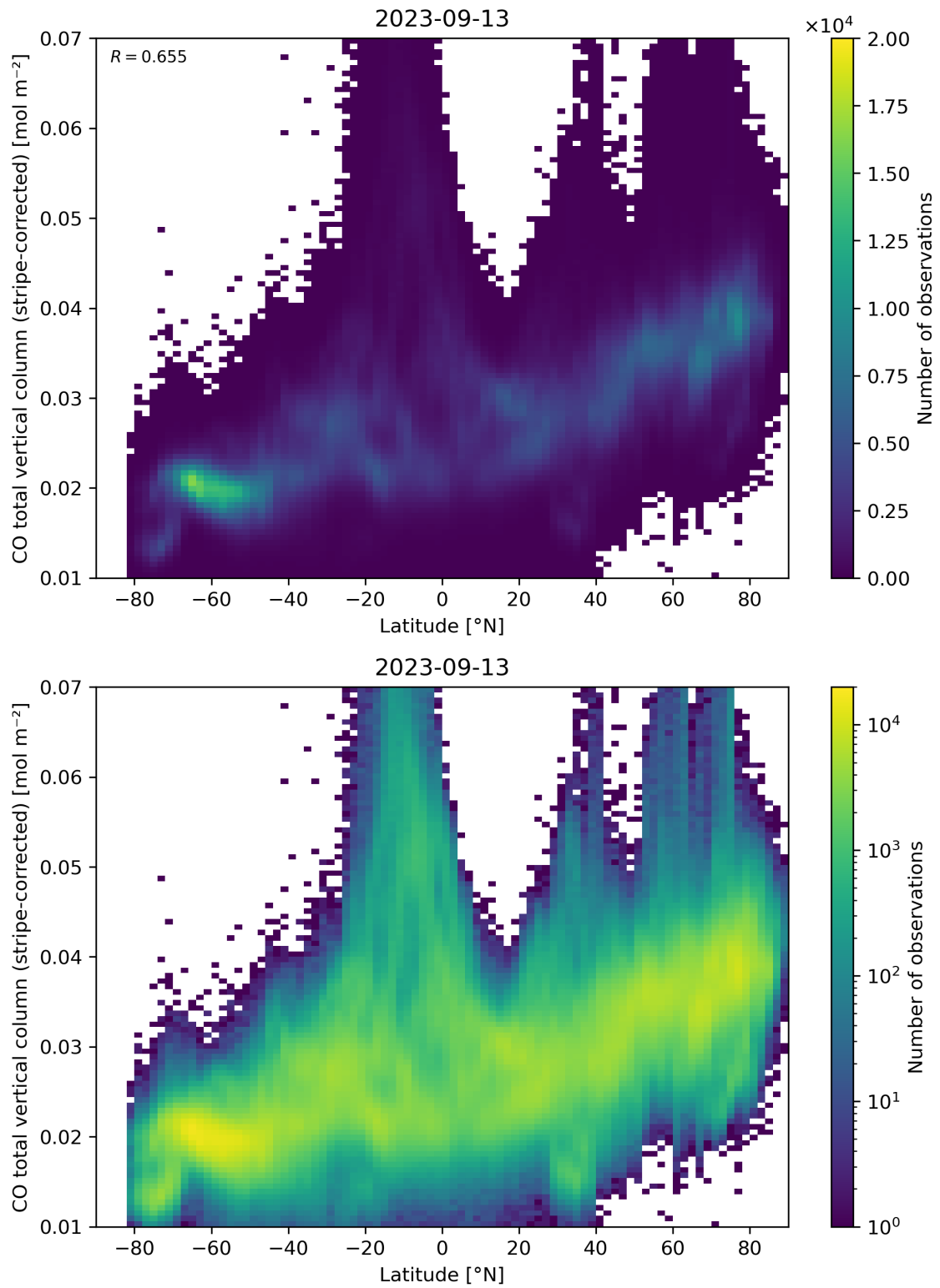
Figure 52: Scatter density plot of “Latitude” against “CO total vertical column (stripe-corrected)” for 2023-09-12 to 2023-09-14.
