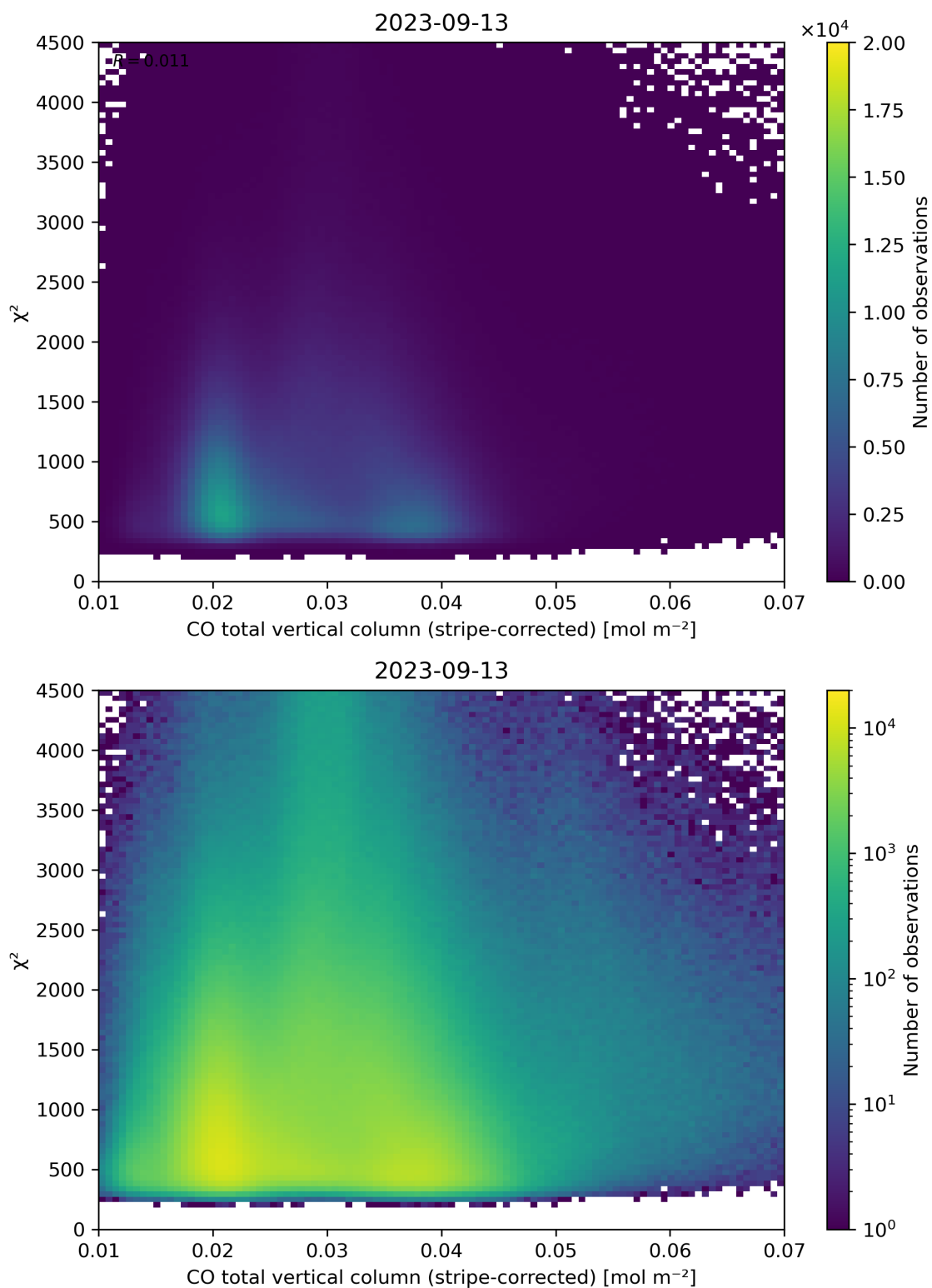
Figure 37: Scatter density plot of “CO total vertical column (stripe-corrected)” against “ \chi^2 ” for 2023-09-12 to 2023-09-14.
