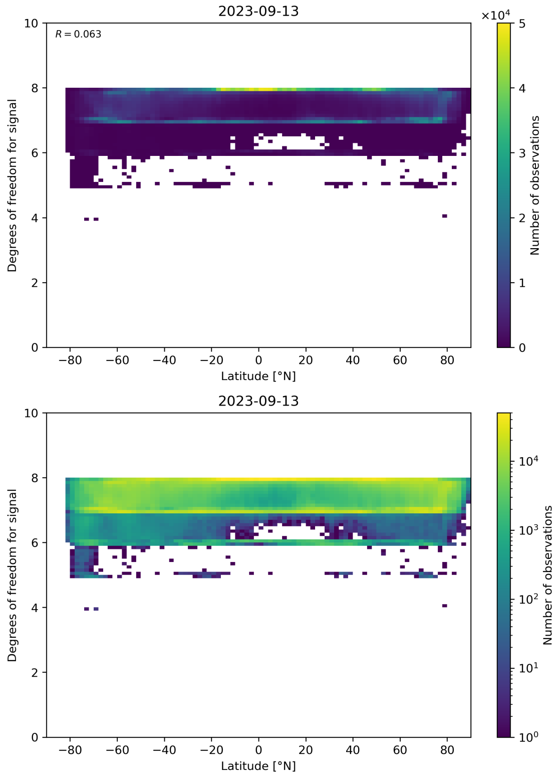
Figure 55: Scatter density plot of “Latitude” against “Degrees of freedom for signal” for 2023-09-12 to 2023-09-14.
