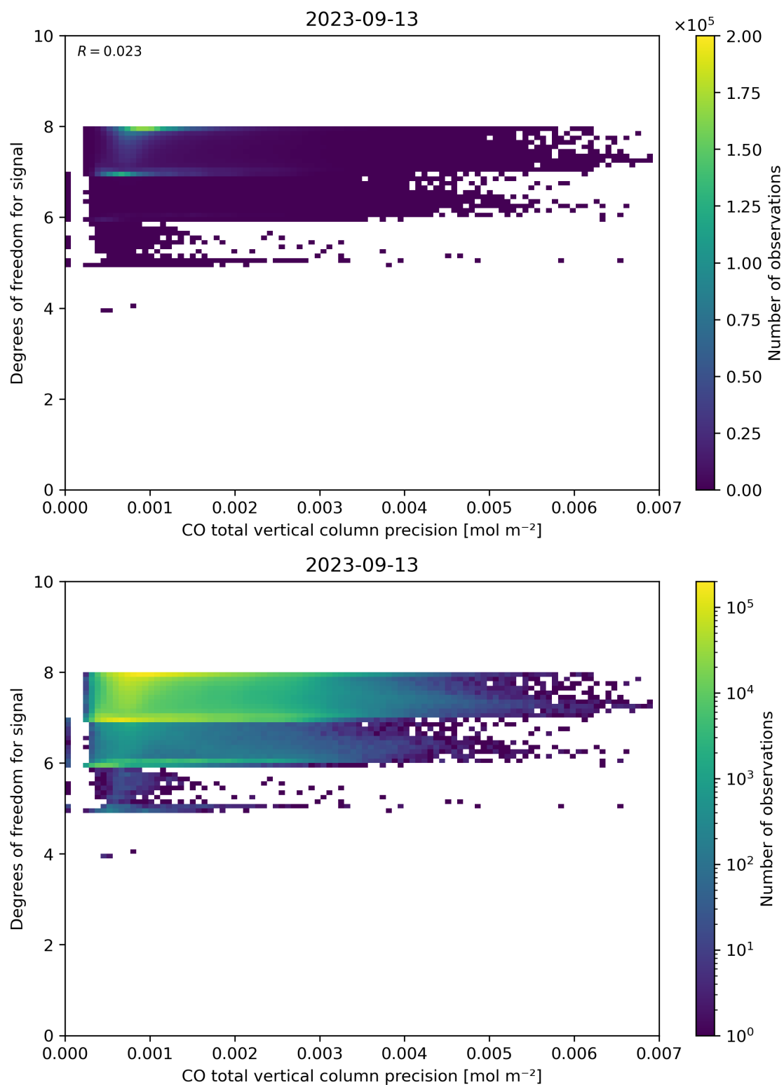
Figure 45: Scatter density plot of “CO total vertical column precision” against “Degrees of freedom for signal” for 2023-09-12 to 2023-09-14.
