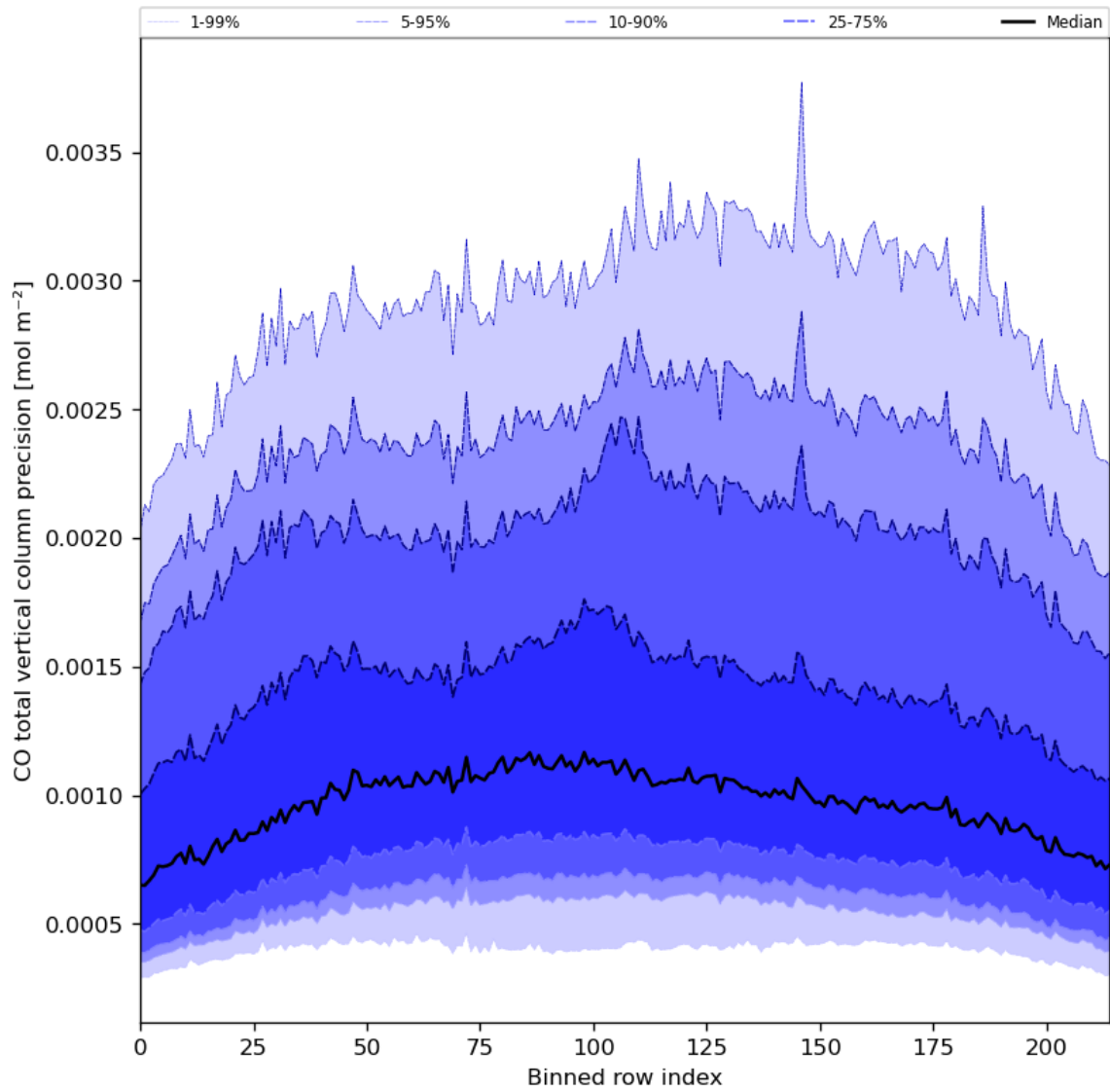
Figure 28: Along track statistics of “CO total vertical column precision” for 2023-09-12 to 2023-09-14
