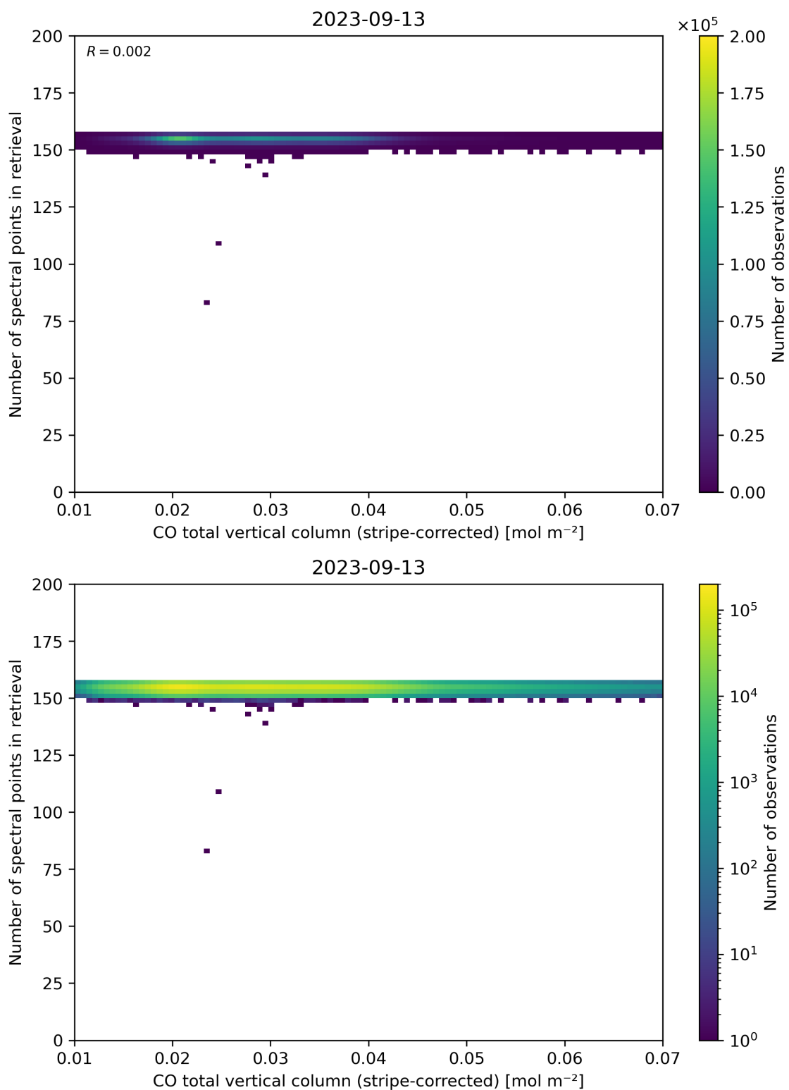
Figure 40: Scatter density plot of “CO total vertical column (stripe-corrected)” against “Number of spectral points in retrieval” for 2023-09-12 to 2023-09-14.
