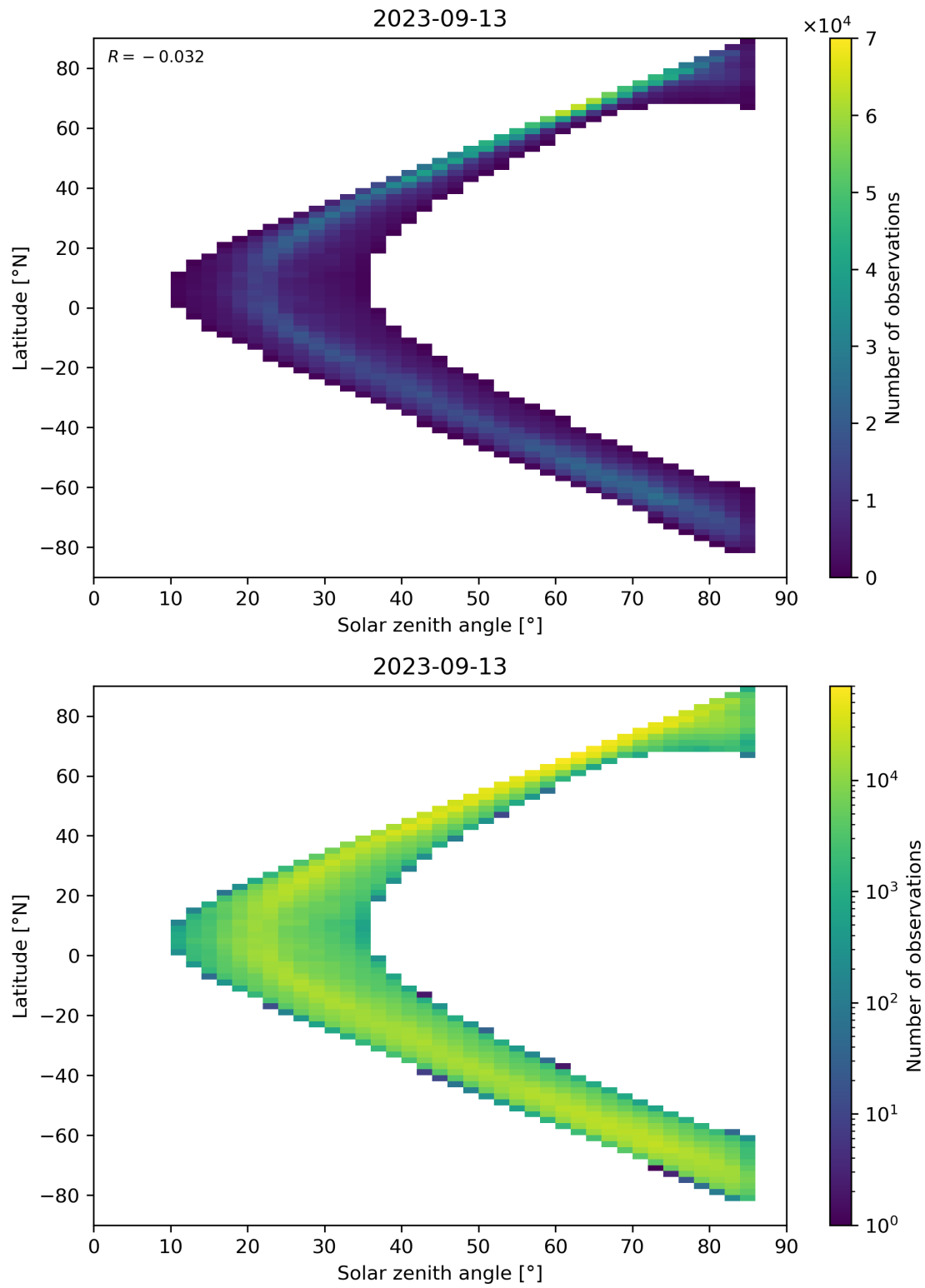
Figure 66: Scatter density plot of “Solar zenith angle” against “Latitude” for 2023-09-12 to 2023-09-14.
