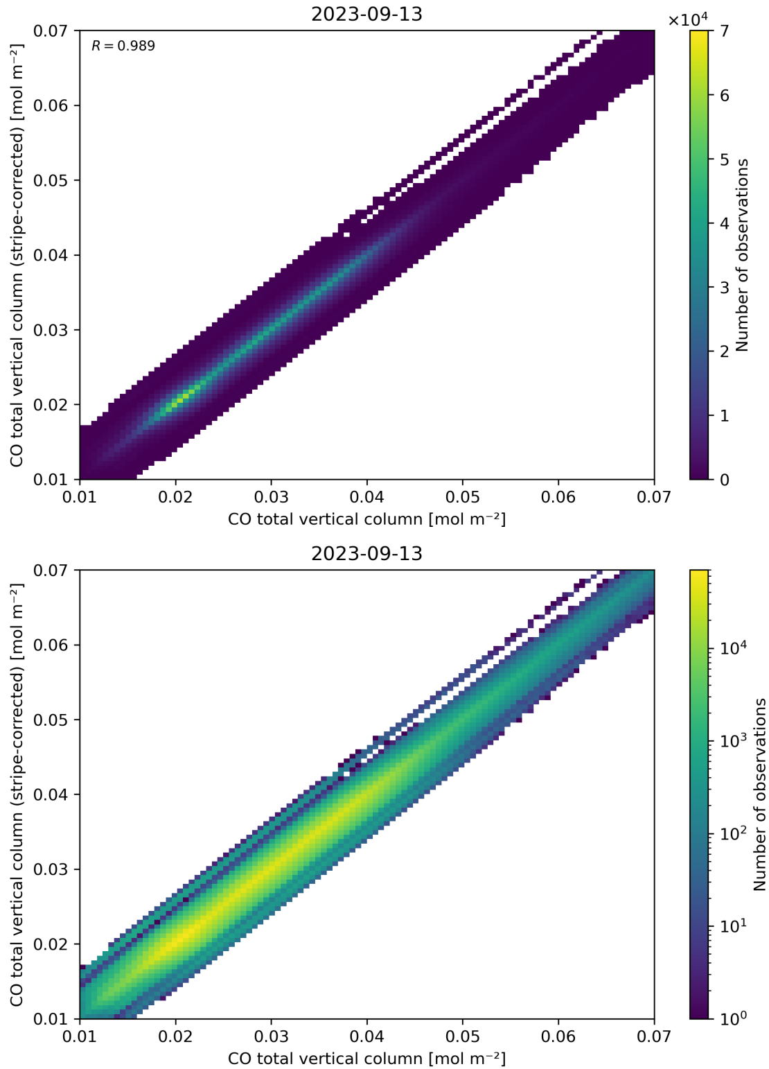
Figure 33: Scatter density plot of “CO total vertical column” against “CO total vertical column (stripe-corrected)” for 2023-09-12 to 2023-09-14.
