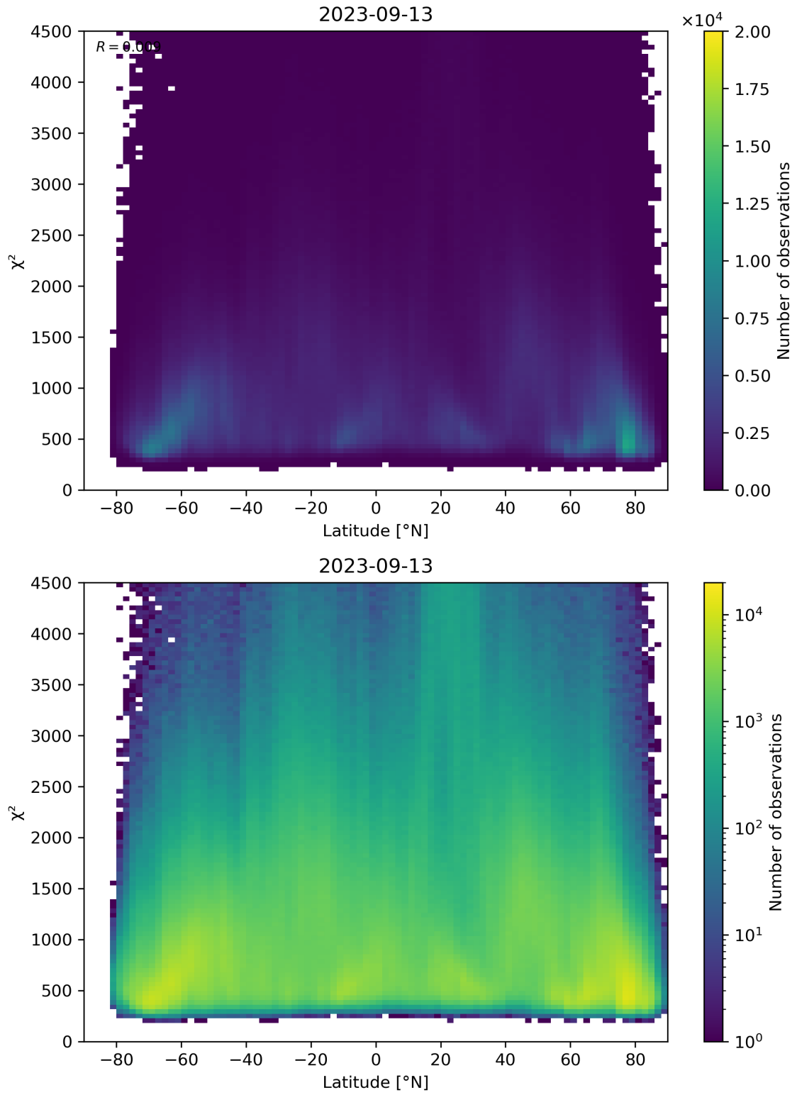
Figure 54: Scatter density plot of “Latitude” against “ \chi^2 ” for 2023-09-12 to 2023-09-14.
