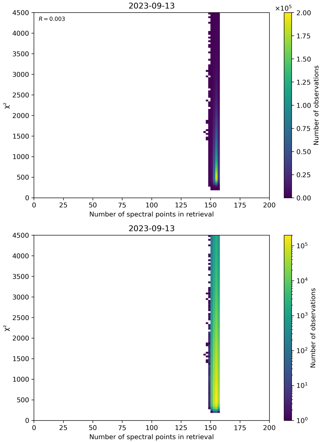
Figure 58: Scatter density plot of “Number of spectral points in retrieval” against “ \chi^2 ” for 2023-09-12 to 2023-09-14.
