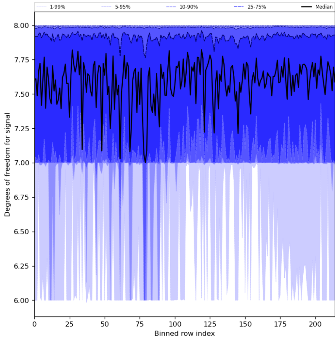
Figure 31: Along track statistics of “Degrees of freedom for signal” for 2023-09-12 to 2023-09-14
