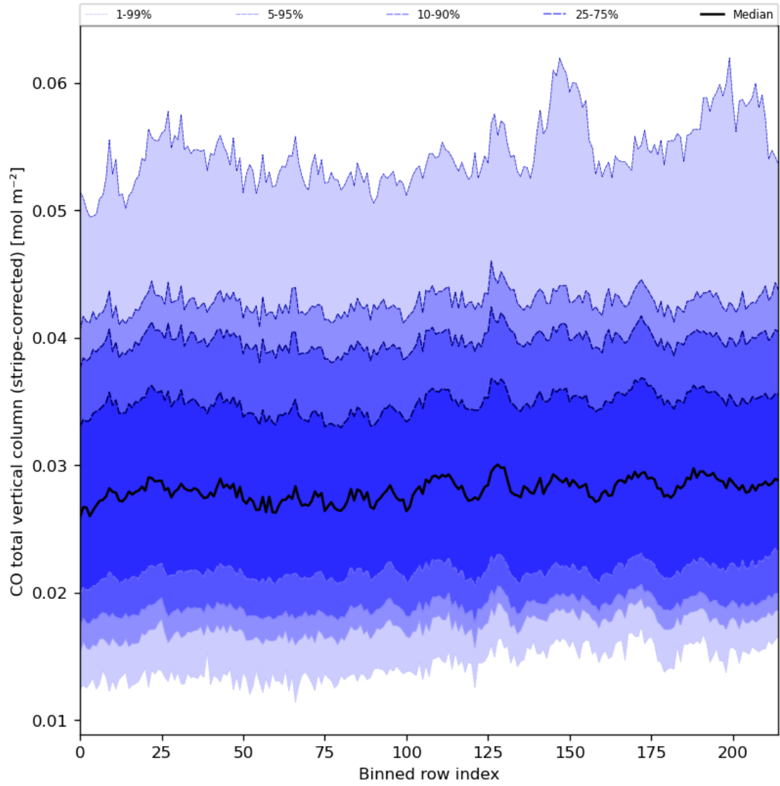
Figure 27: Along track statistics of “CO total vertical column (stripe-corrected)” for 2023-09-12 to 2023-09-14
