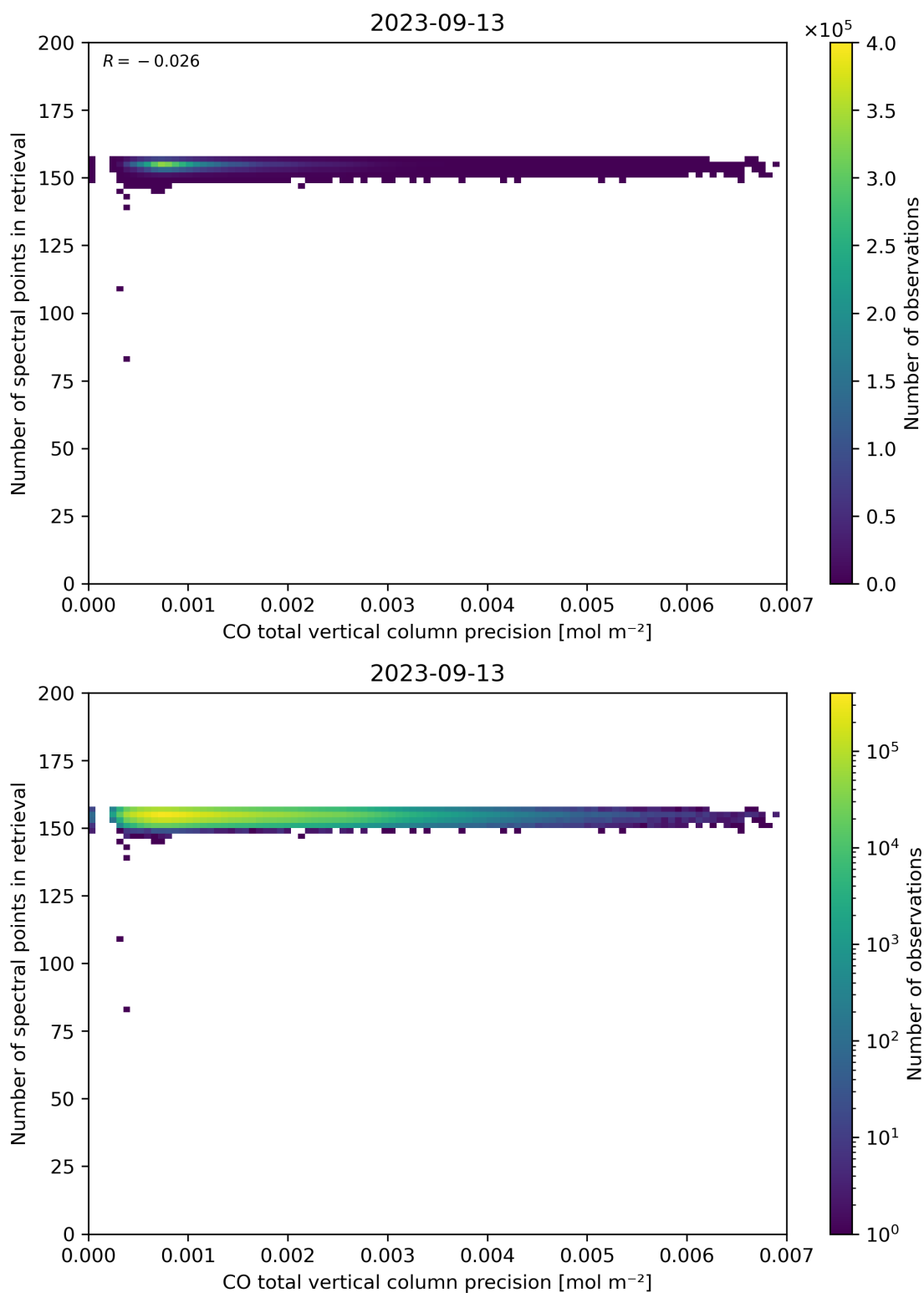
Figure 47: Scatter density plot of “CO total vertical column precision” against “Number of spectral points in retrieval” for 2023-09-12 to 2023-09-14.
