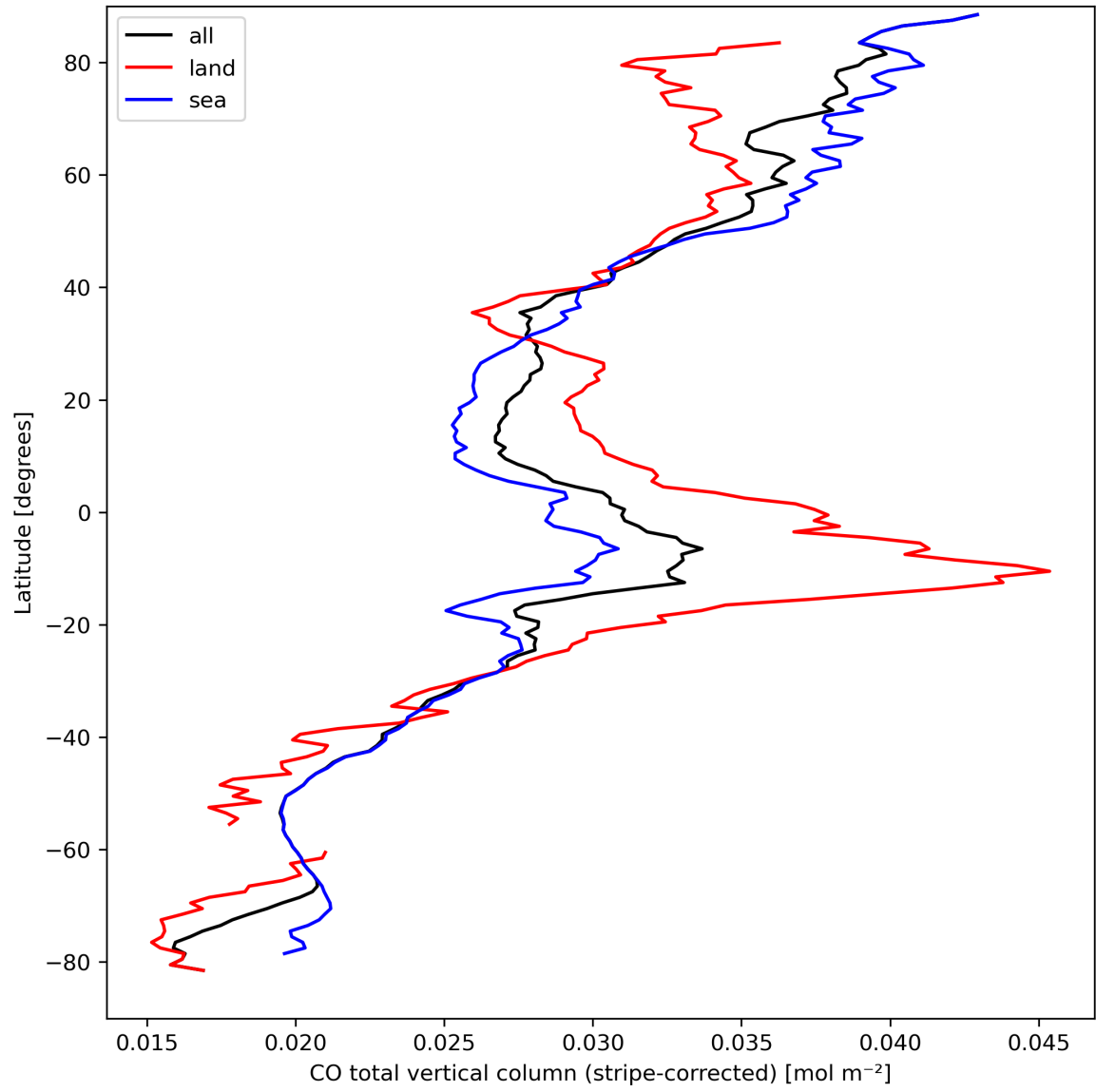
Figure 11: Zonal average of “CO total vertical column (stripe-corrected)” for 2023-09-12 to 2023-09-14.
