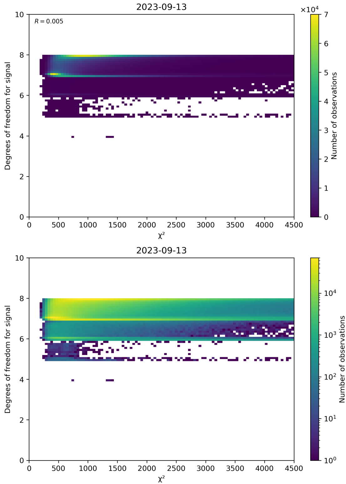
Figure 48: Scatter density plot of “ \chi^2 ” against “Degrees of freedom for signal” for 2023-09-12 to 2023-09-14.
