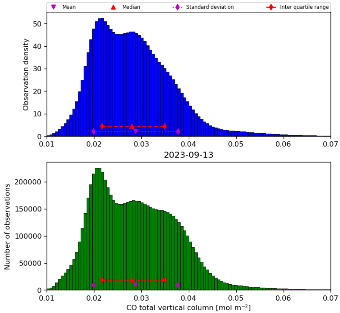
Figure 18: Histogram of “CO total vertical column” for 2023-09-12 to 2023-09-14
