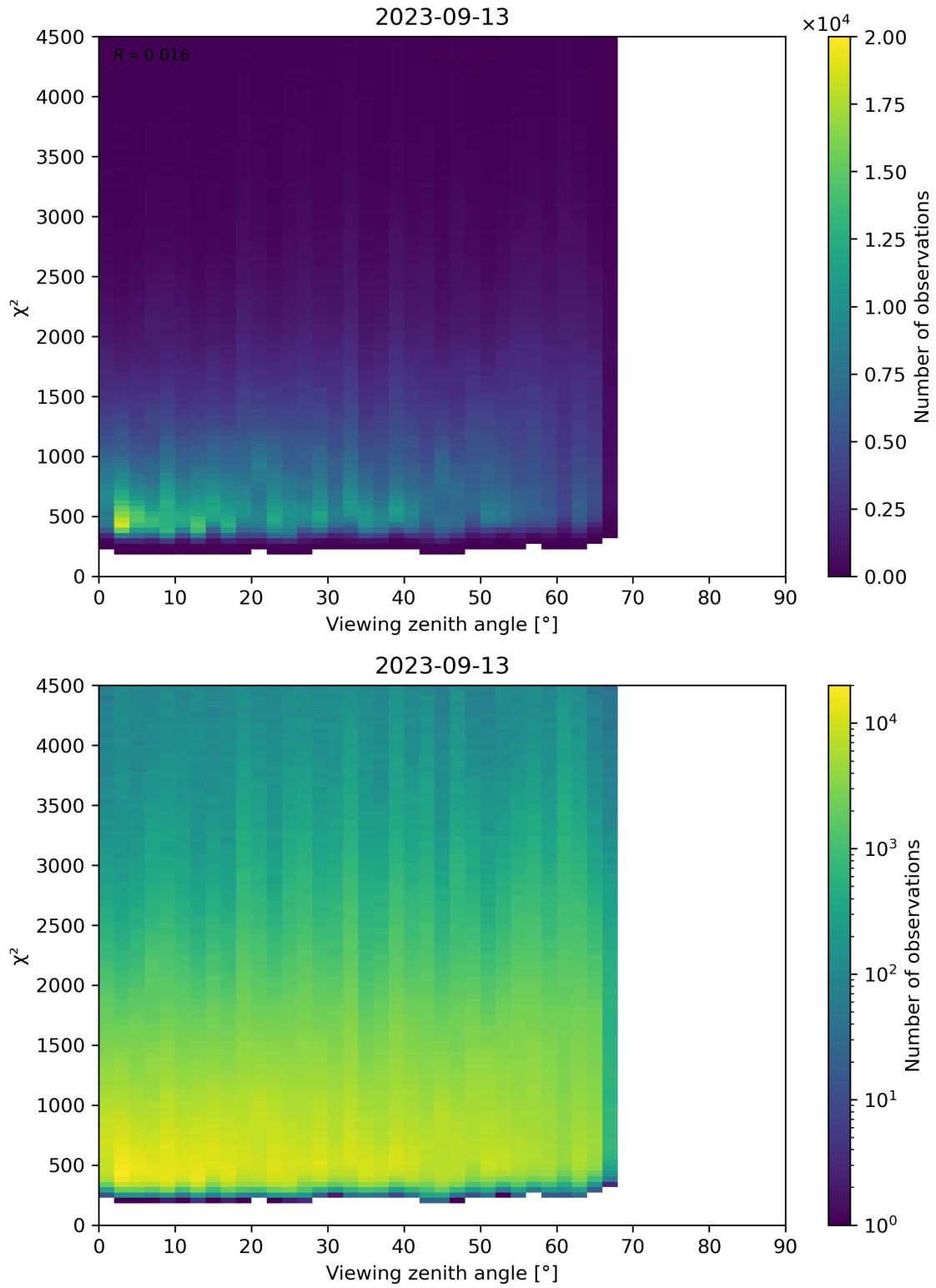
Figure 72: Scatter density plot of “Viewing zenith angle” against “ \chi^2 ” for 2023-09-12 to 2023-09-14.
