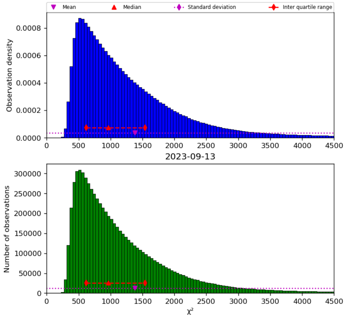
Figure 22: Histogram of “ \chi^2 ” for 2023-09-12 to 2023-09-14
