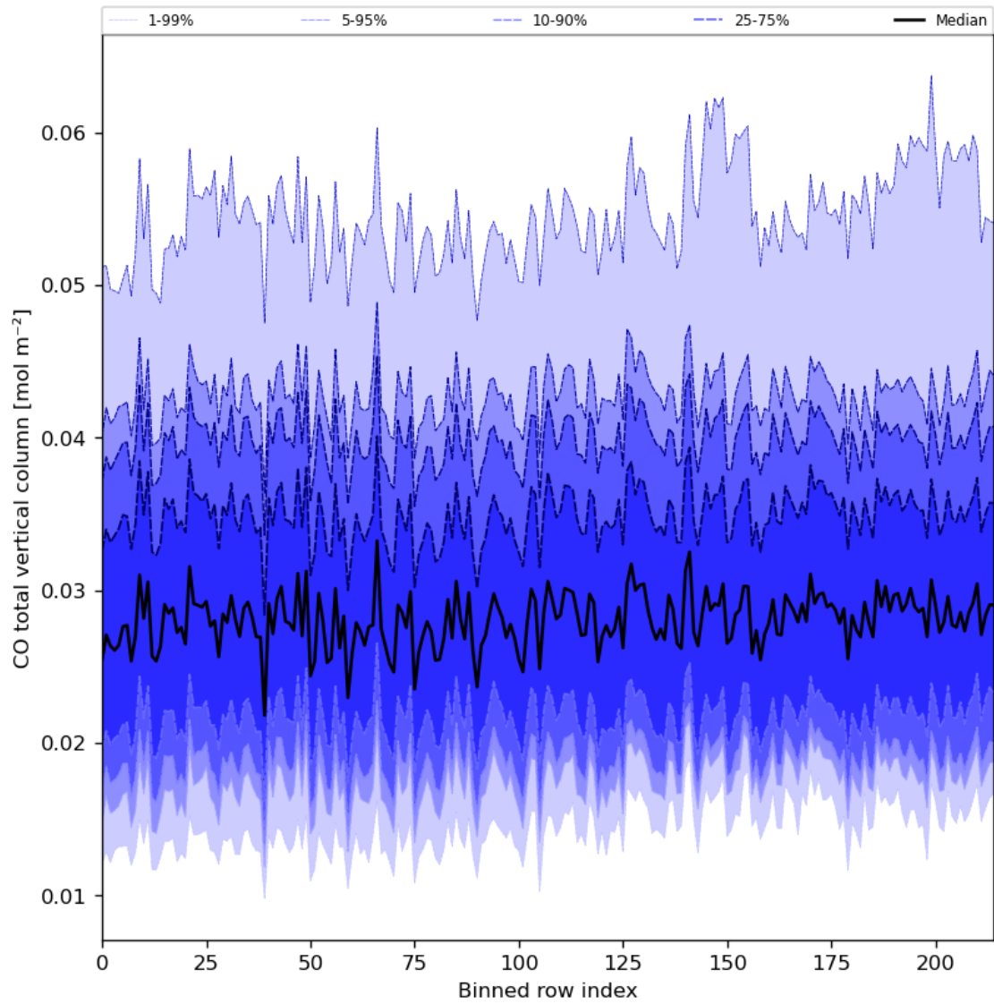
Figure 26: Along track statistics of “CO total vertical column” for 2023-09-12 to 2023-09-14
