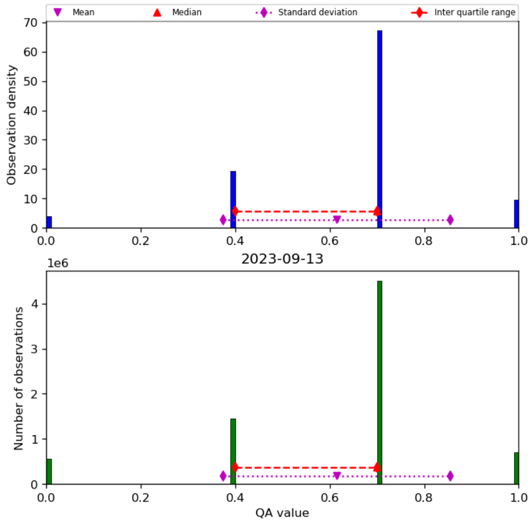
Figure 17: Histogram of “QA value” for 2023-09-12 to 2023-09-14
