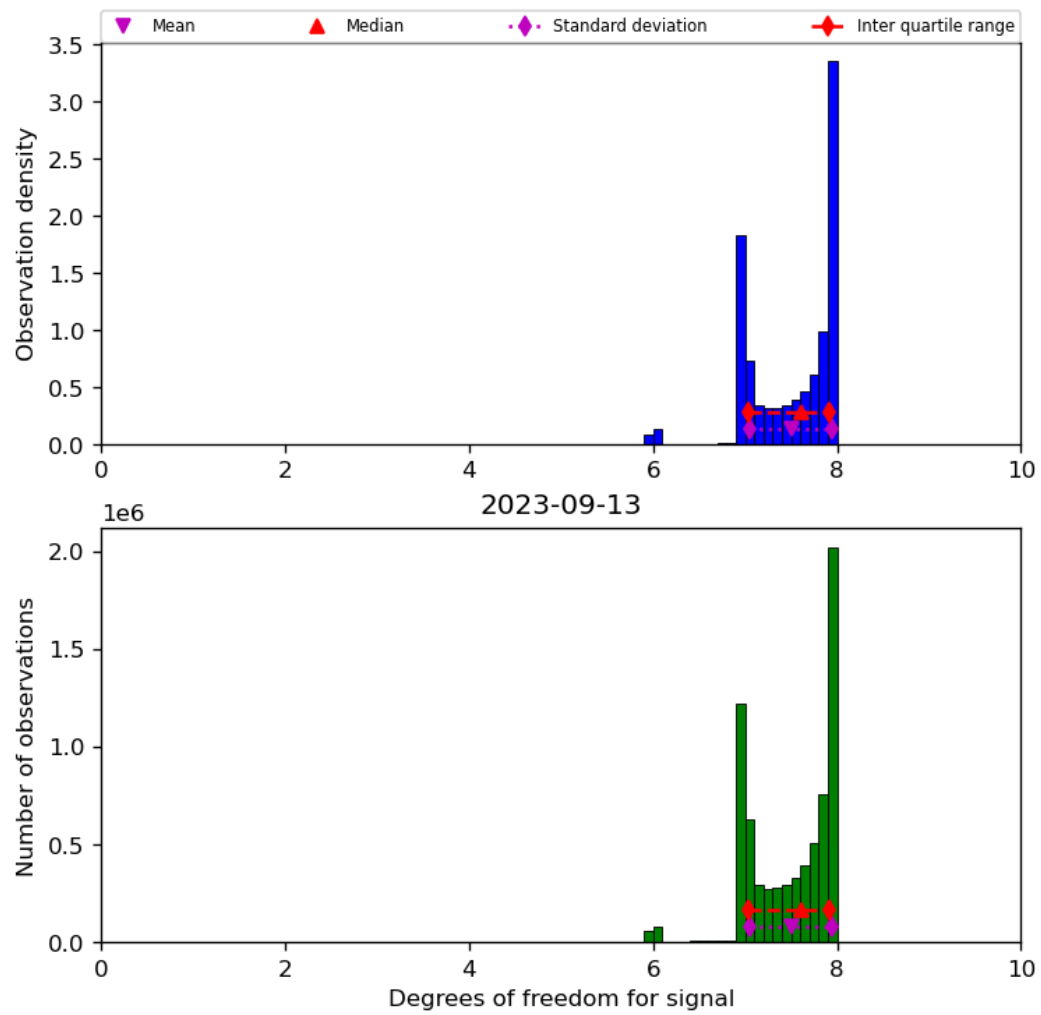
Figure 23: Histogram of “Degrees of freedom for signal” for 2023-09-12 to 2023-09-14
