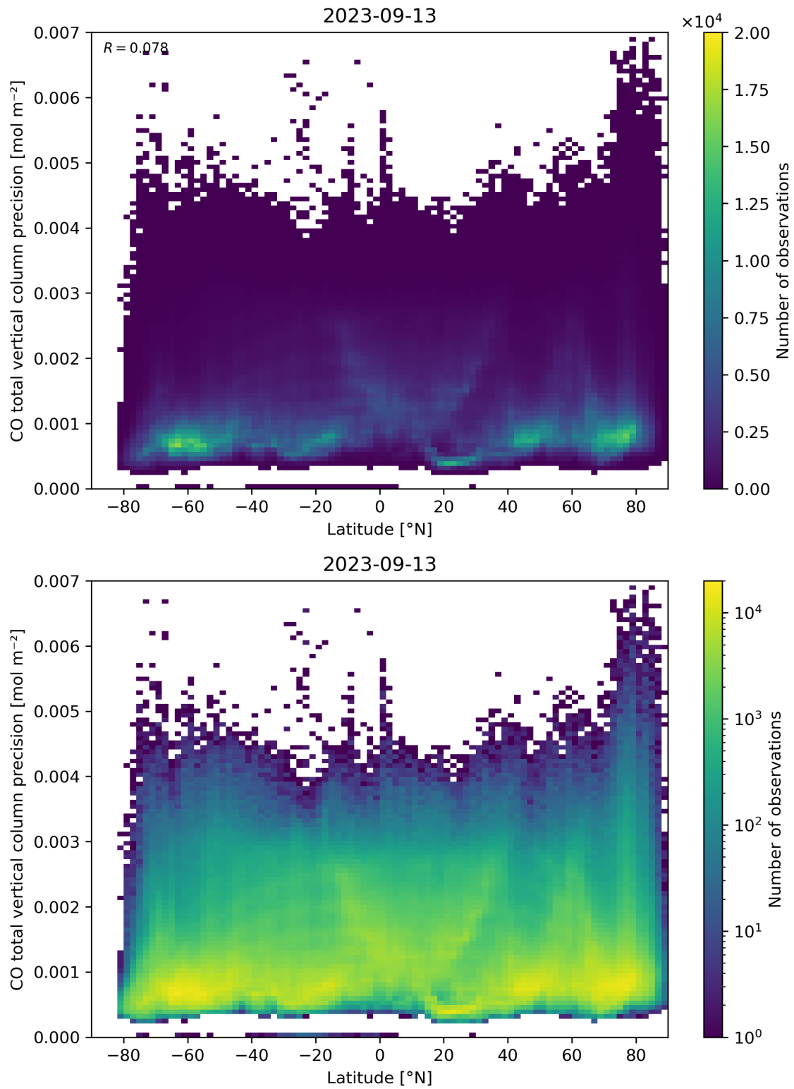
Figure 53: Scatter density plot of “Latitude” against “CO total vertical column precision” for 2023-09-12 to 2023-09-14.
