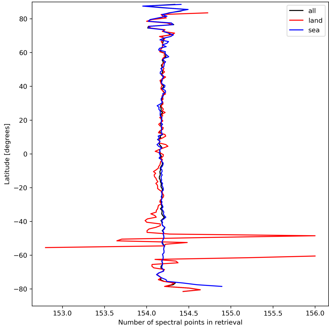
Figure 13: Zonal average of “Number of spectral points in retrieval” for 2023-09-12 to 2023-09-14.
