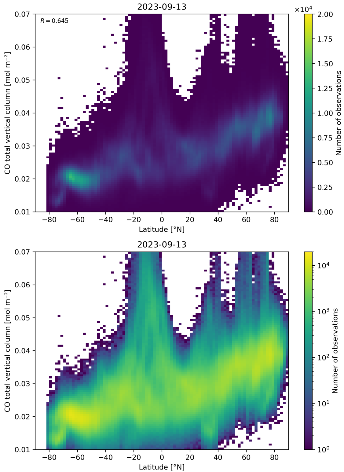
Figure 51: Scatter density plot of “Latitude” against “CO total vertical column” for 2023-09-12 to 2023-09-14.
