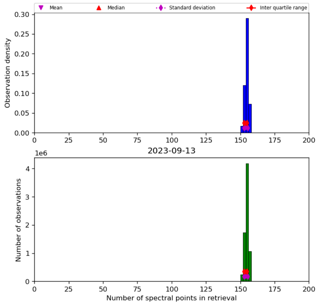
Figure 21: Histogram of “Number of spectral points in retrieval” for 2023-09-12 to 2023-09-14
