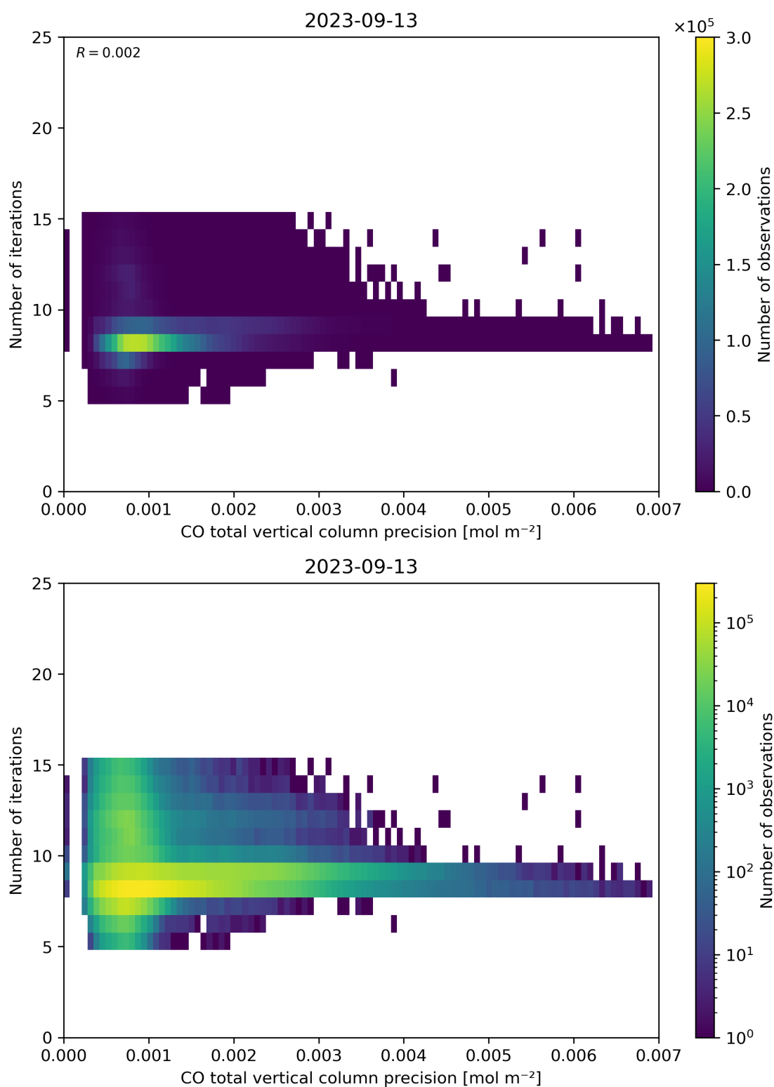
Figure 46: Scatter density plot of “CO total vertical column precision” against “Number of iterations” for 2023-09-12 to 2023-09-14.
