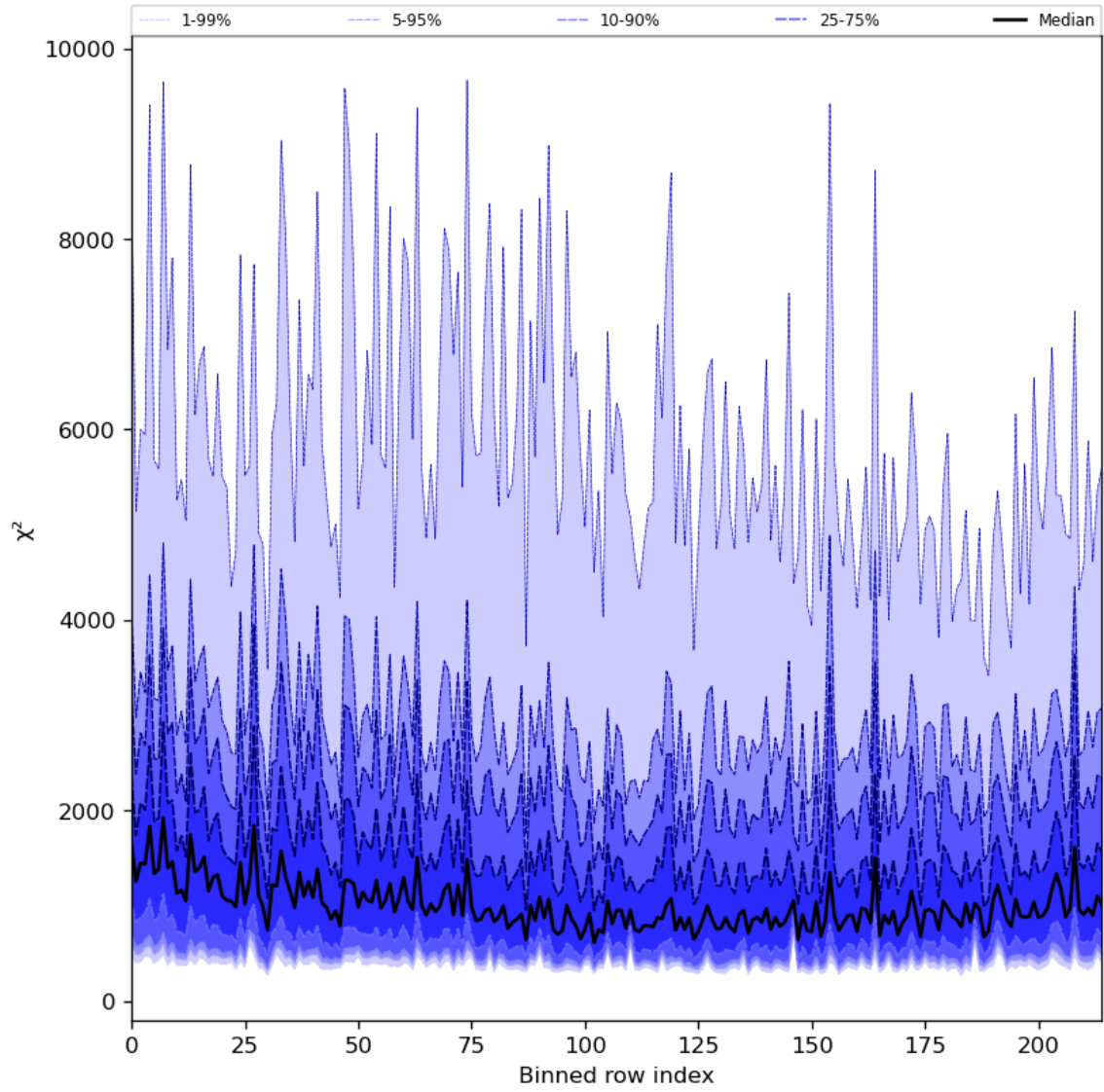
Figure 30: Along track statistics of “ \chi^2 ” for 2023-09-12 to 2023-09-14
