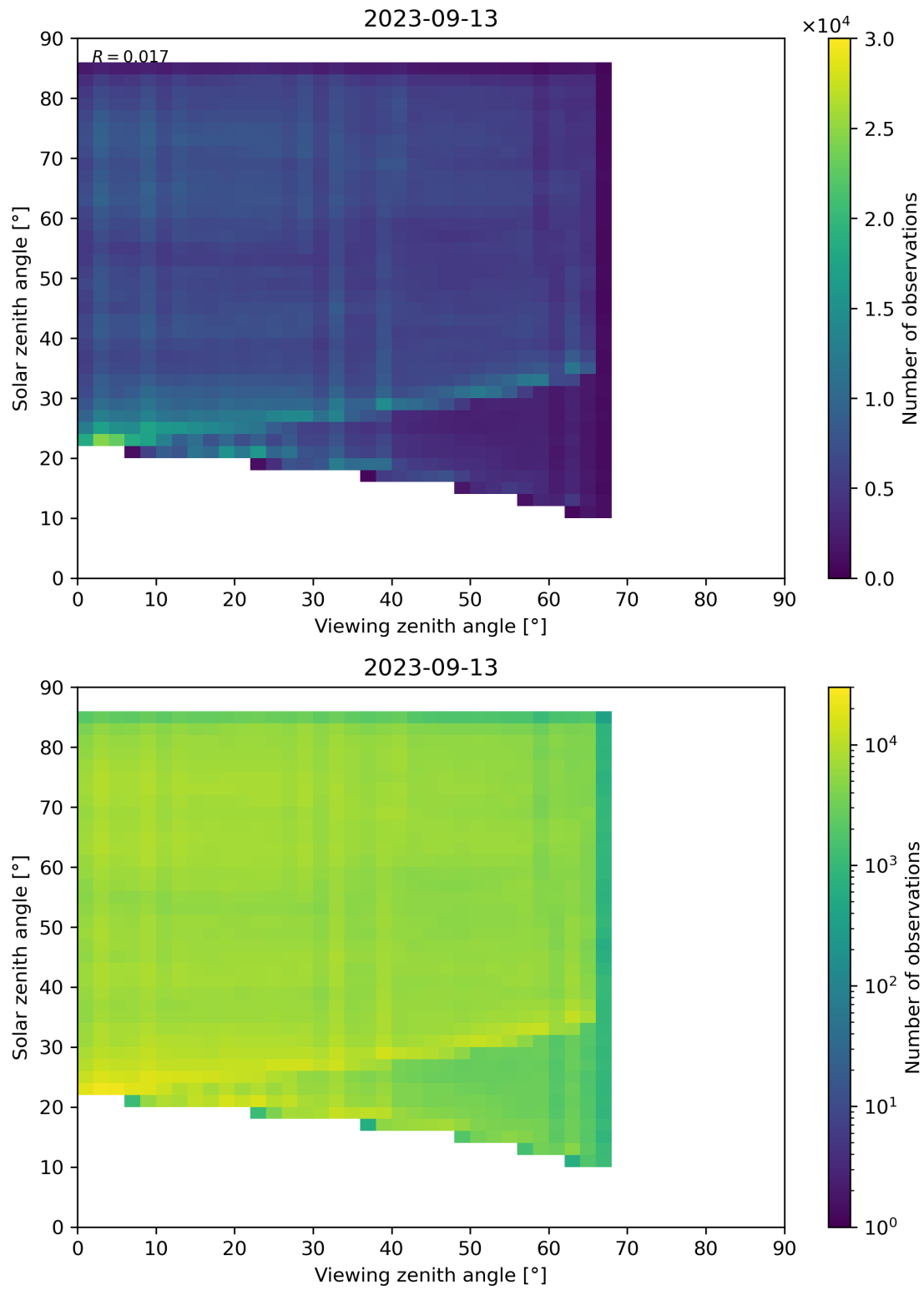
Figure 77: Scatter density plot of “Viewing zenith angle” against “Solar zenith angle” for 2023-09-12 to 2023-09-14.
