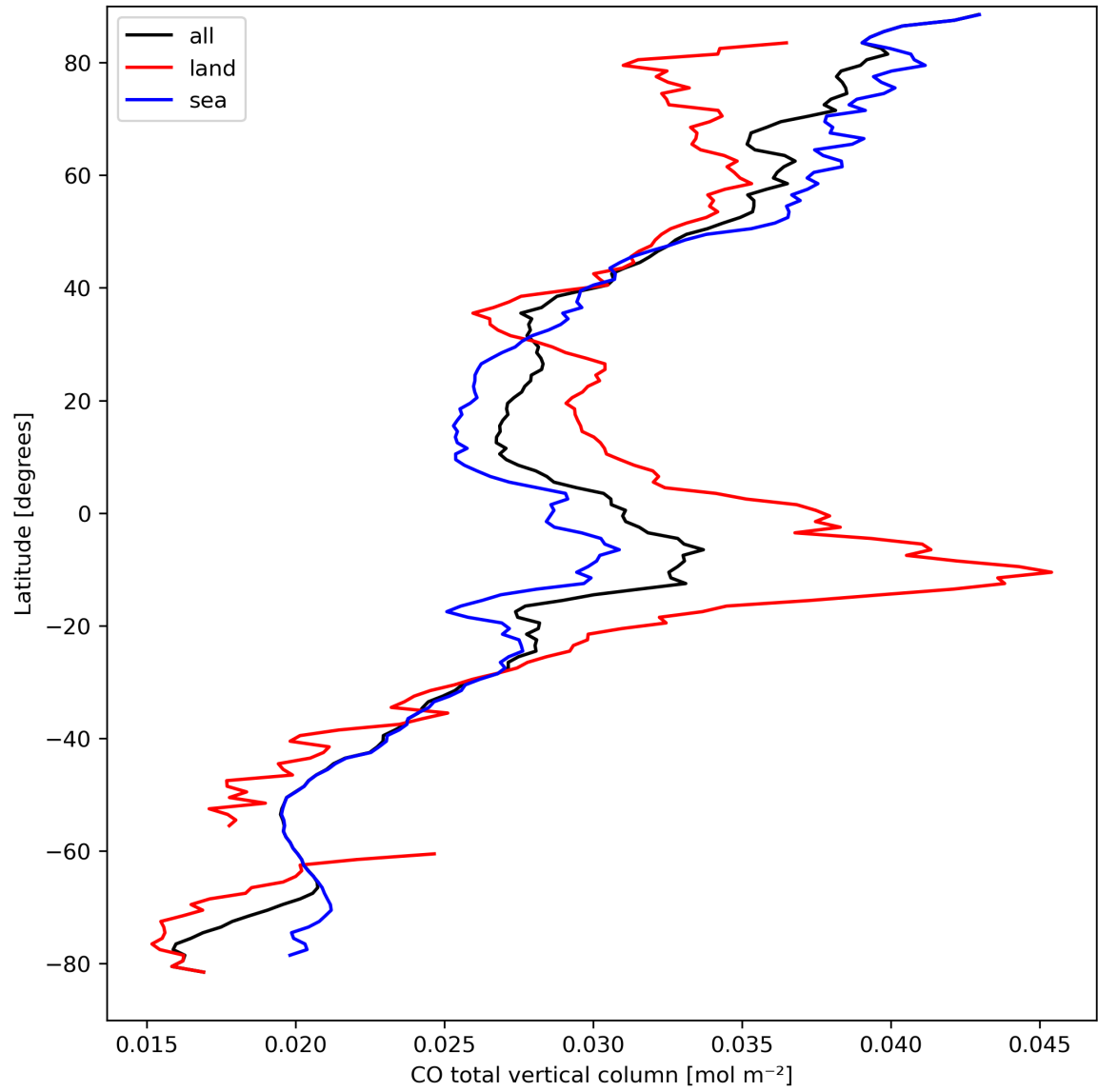
Figure 10: Zonal average of “CO total vertical column” for 2023-09-12 to 2023-09-14.
