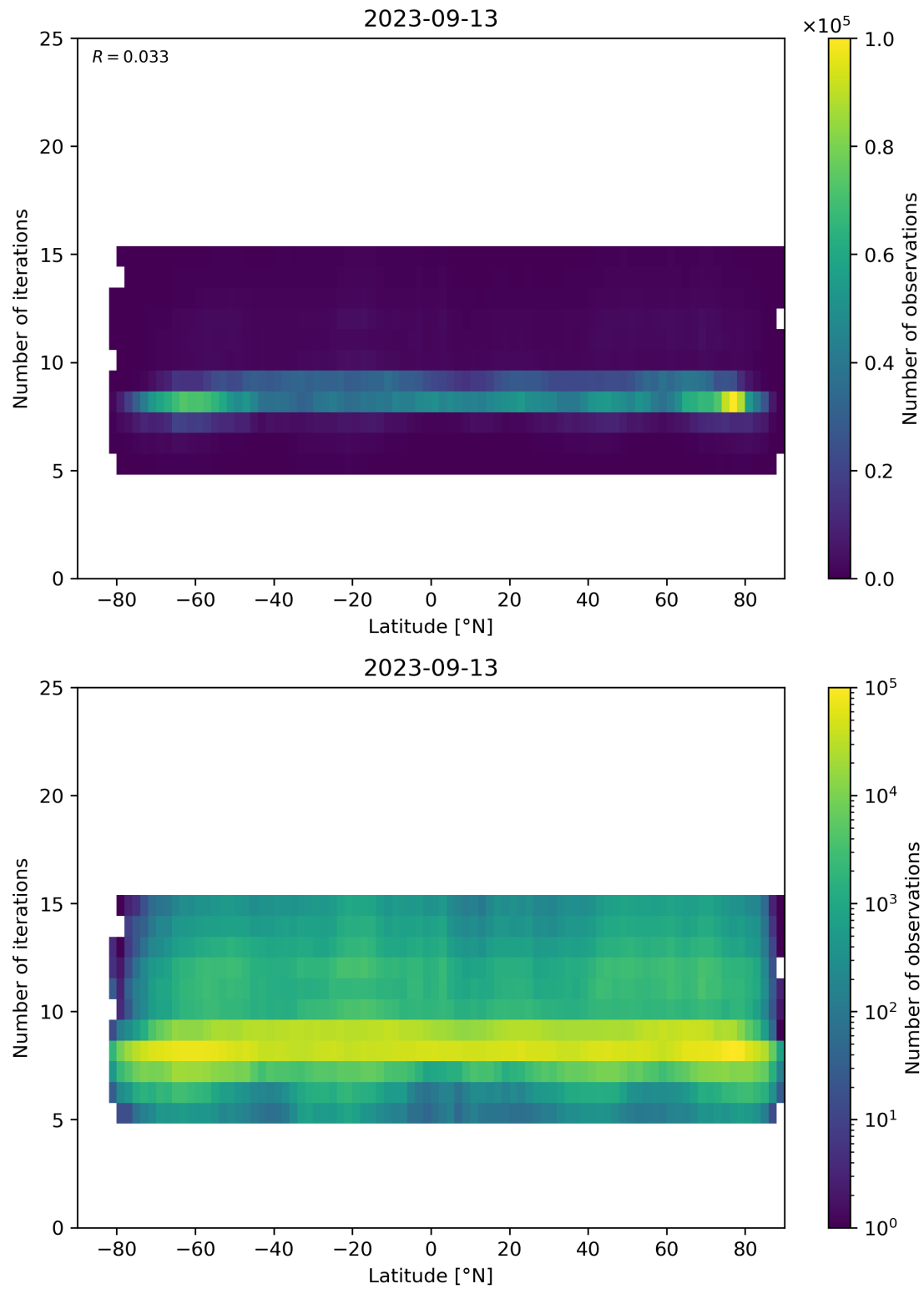
Figure 56: Scatter density plot of “Latitude” against “Number of iterations” for 2023-09-12 to 2023-09-14.
