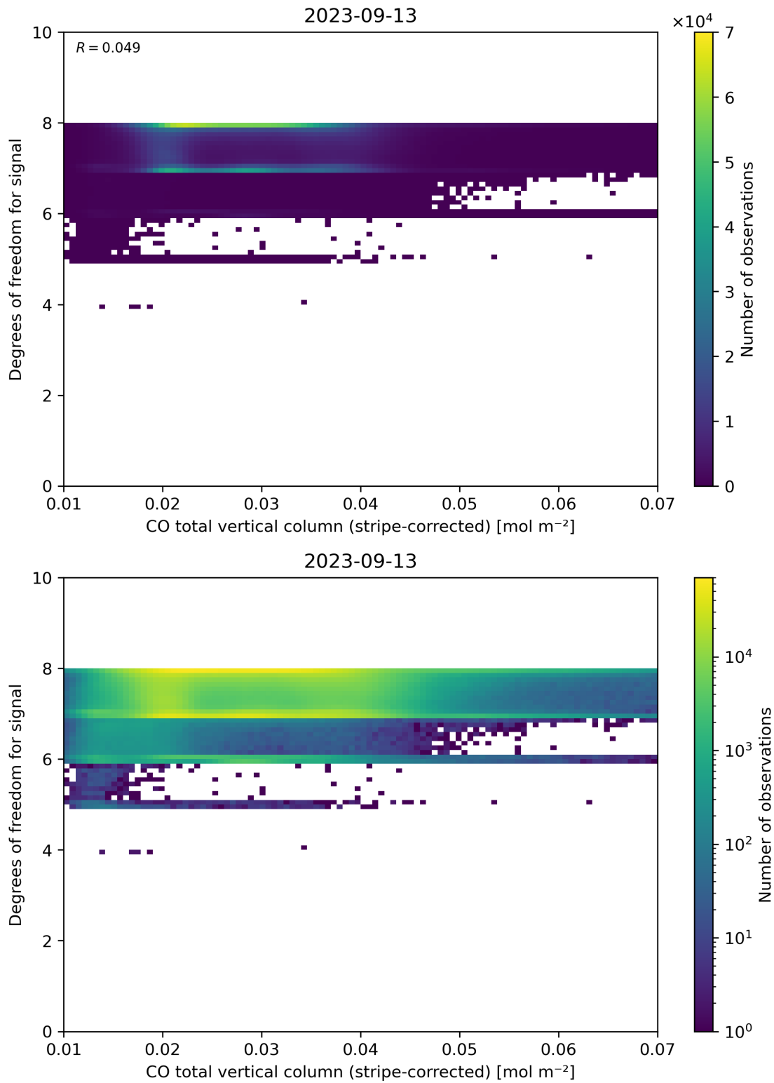
Figure 38: Scatter density plot of “CO total vertical column (stripe-corrected)” against “Degrees of freedom for signal” for 2023-09-12 to 2023-09-14.
