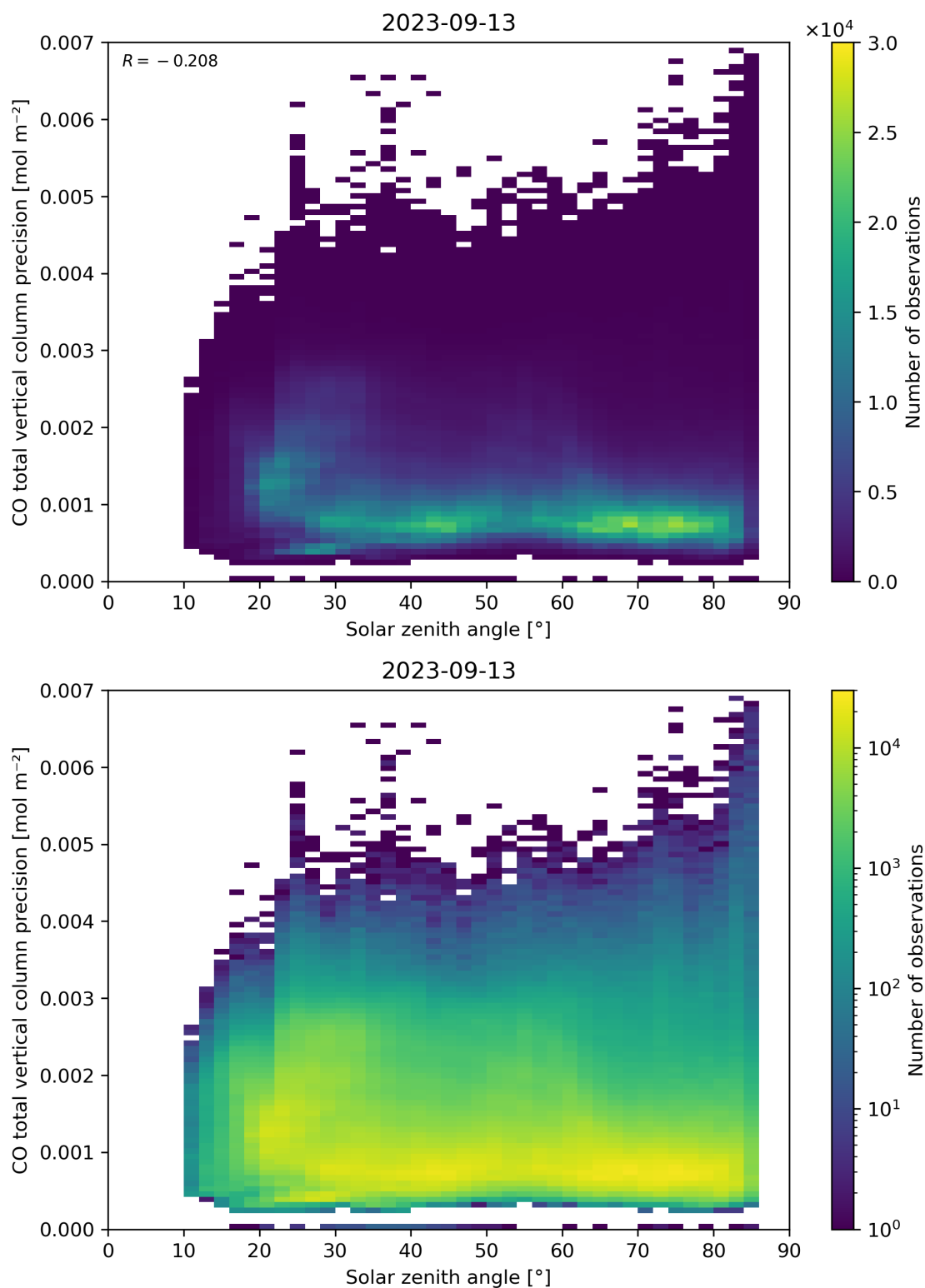
Figure 63: Scatter density plot of “Solar zenith angle” against “CO total vertical column precision” for 2023-09-12 to 2023-09-14.
