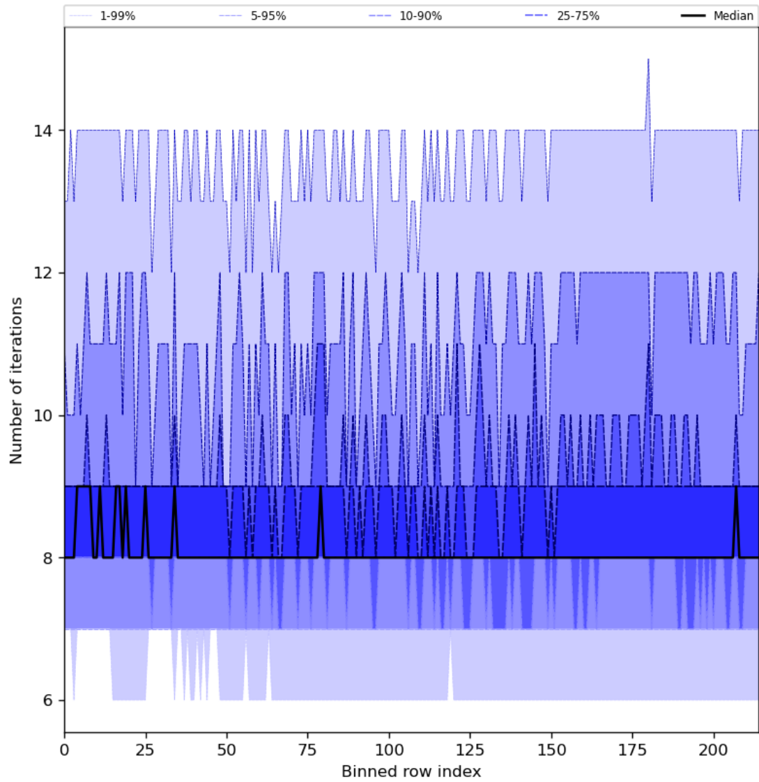
Figure 32: Along track statistics of “Number of iterations” for 2023-09-12 to 2023-09-14
