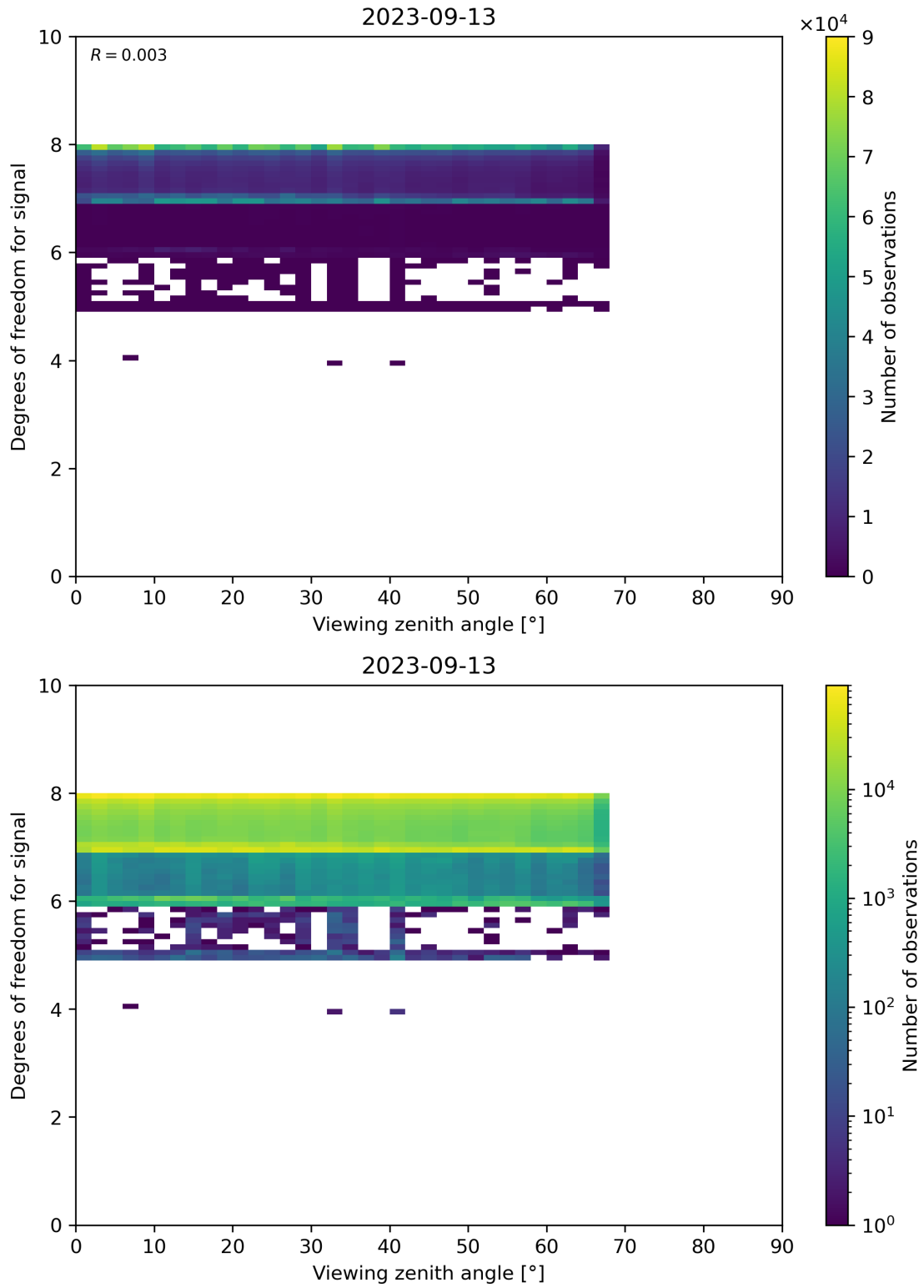
Figure 73: Scatter density plot of “Viewing zenith angle” against “Degrees of freedom for signal” for 2023-09-12 to 2023-09-14.
