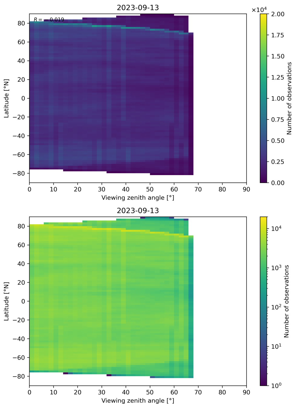
Figure 74: Scatter density plot of “Viewing zenith angle” against “Latitude” for 2023-09-12 to 2023-09-14.
