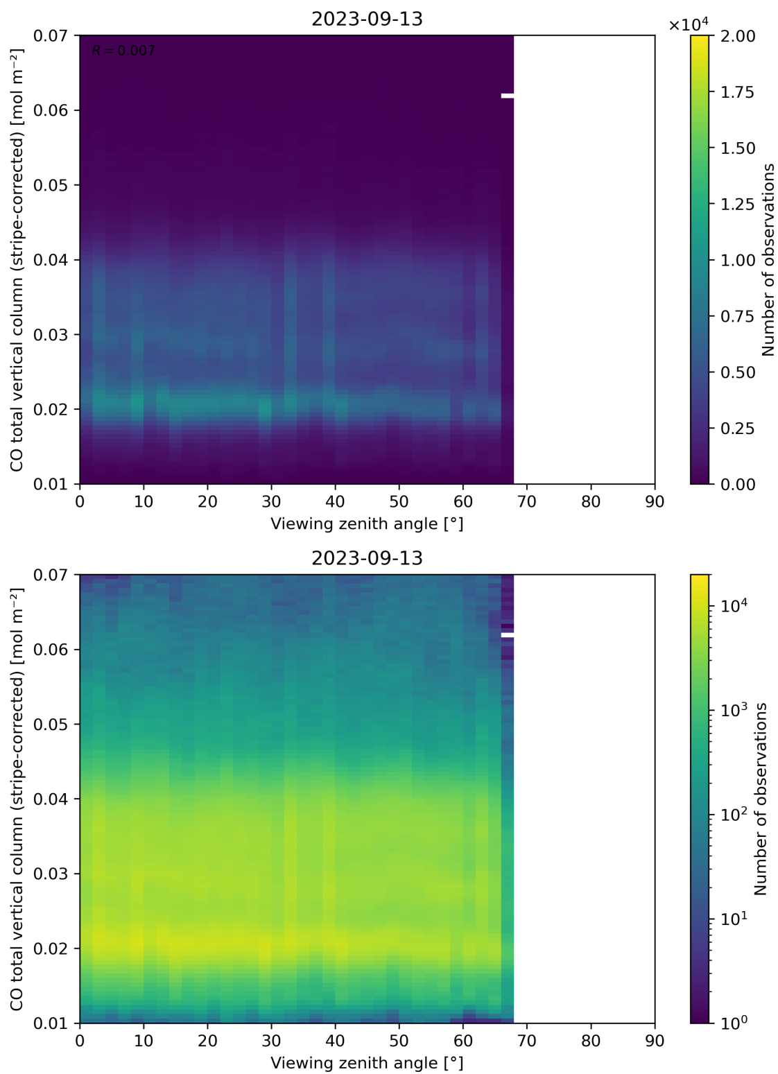
Figure 70: Scatter density plot of “Viewing zenith angle” against “CO total vertical column (stripe-corrected)” for 2023-09-12 to 2023-09-14.
