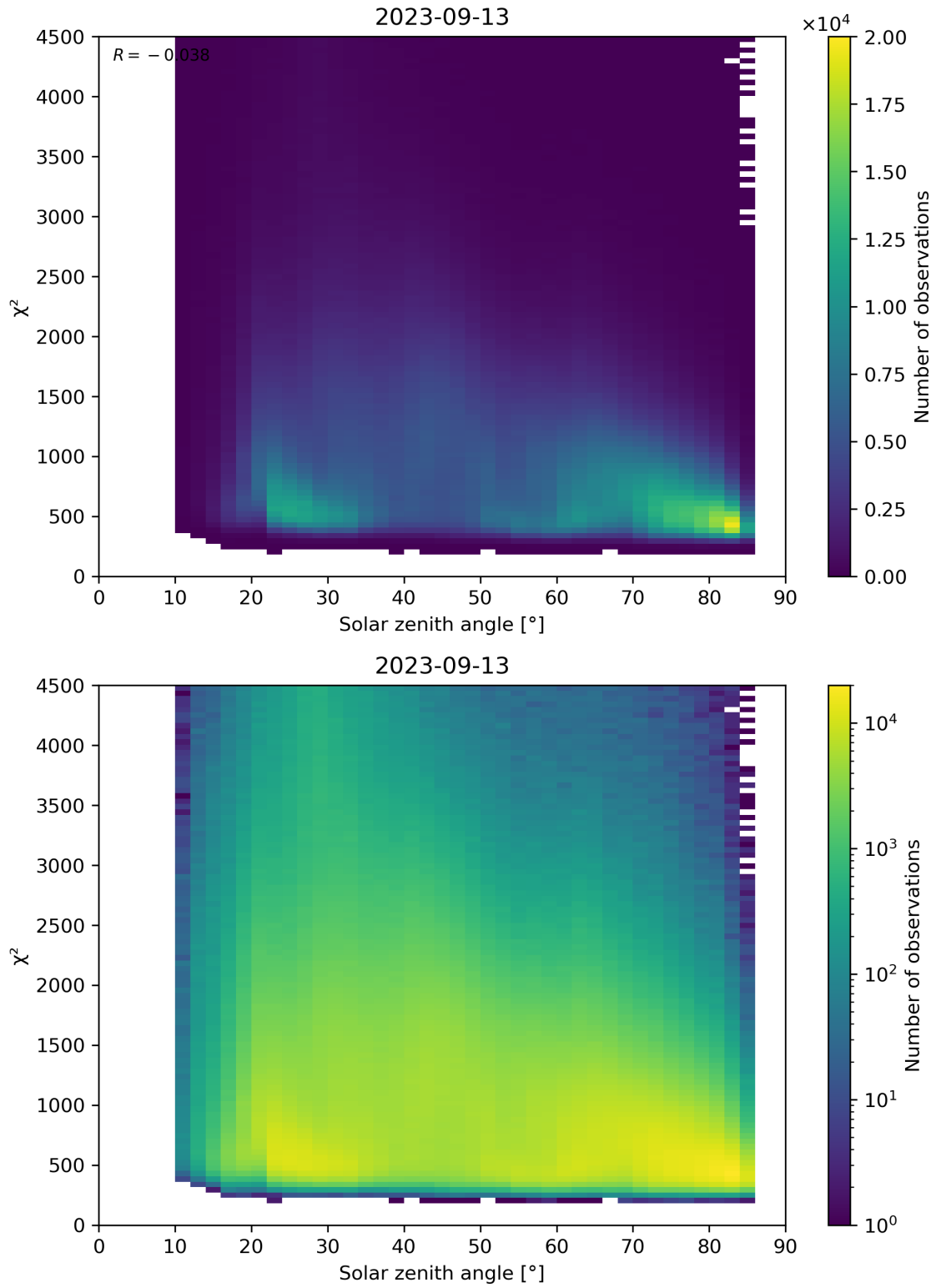
Figure 64: Scatter density plot of “Solar zenith angle” against “ \chi^2 ” for 2023-09-12 to 2023-09-14.
