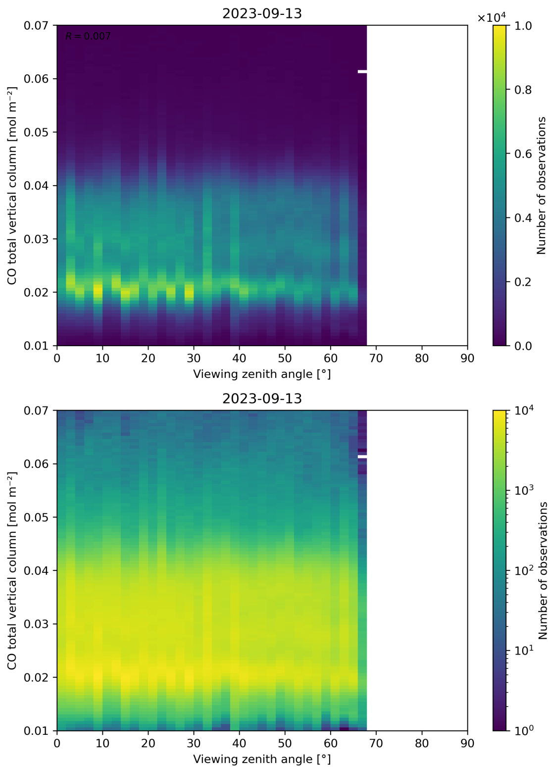
Figure 69: Scatter density plot of “Viewing zenith angle” against “CO total vertical column” for 2023-09-12 to 2023-09-14.
