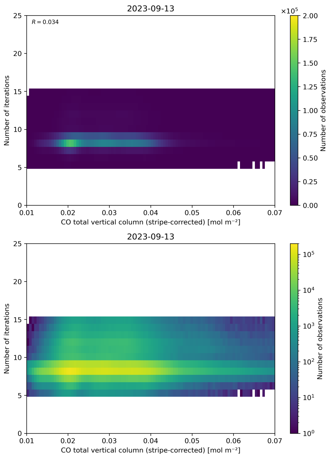
Figure 39: Scatter density plot of “CO total vertical column (stripe-corrected)” against “Number of iterations” for 2023-09-12 to 2023-09-14.
