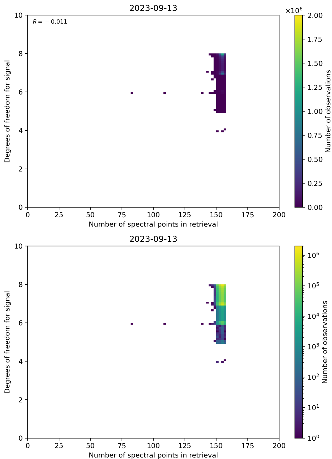
Figure 59: Scatter density plot of “Number of spectral points in retrieval” against “Degrees of freedom for signal” for 2023-09-12 to 2023-09-14.
