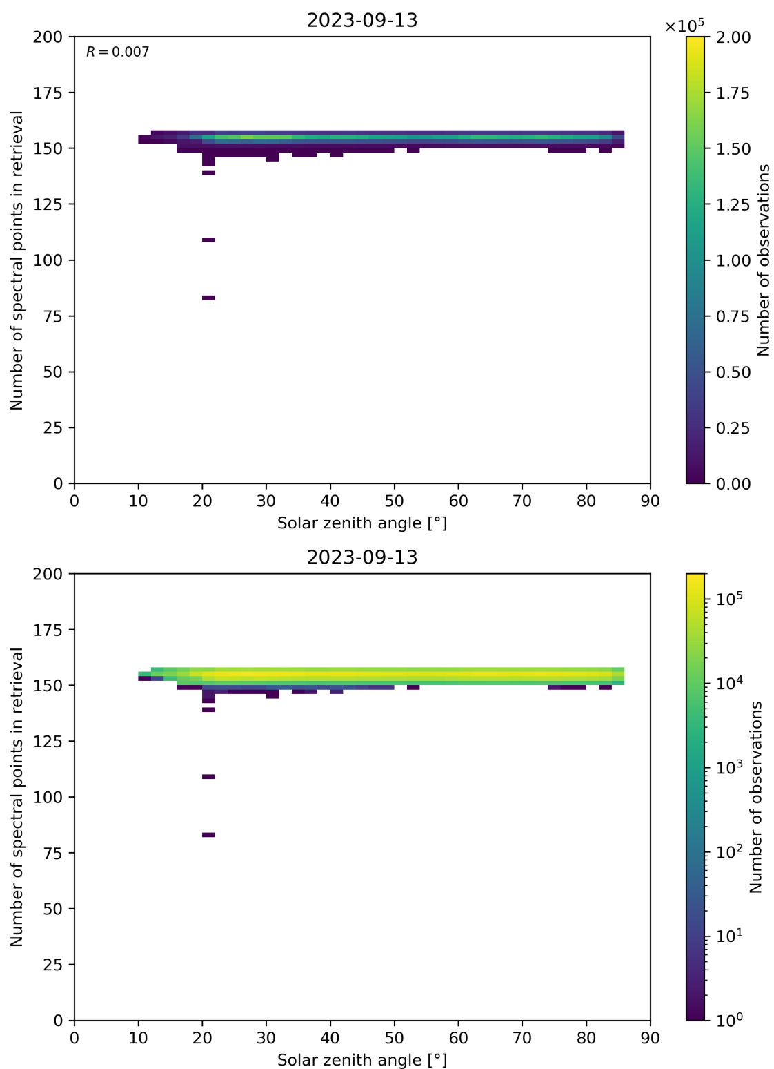
Figure 68: Scatter density plot of “Solar zenith angle” against “Number of spectral points in retrieval” for 2023-09-12 to 2023-09-14.
