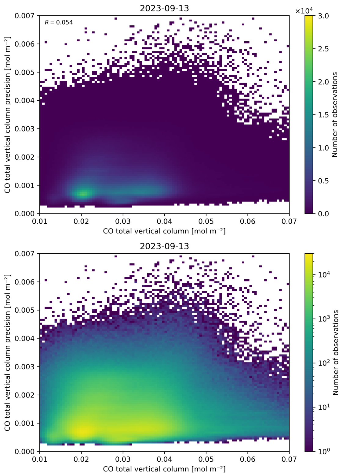
Figure 34: Scatter density plot of “CO total vertical column” against “CO total vertical column precision” for 2023-09-12 to 2023-09-14.
