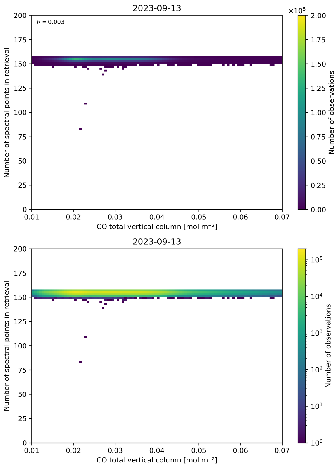
Figure 43: Scatter density plot of “CO total vertical column” against “Number of spectral points in retrieval” for 2023-09-12 to 2023-09-14.
