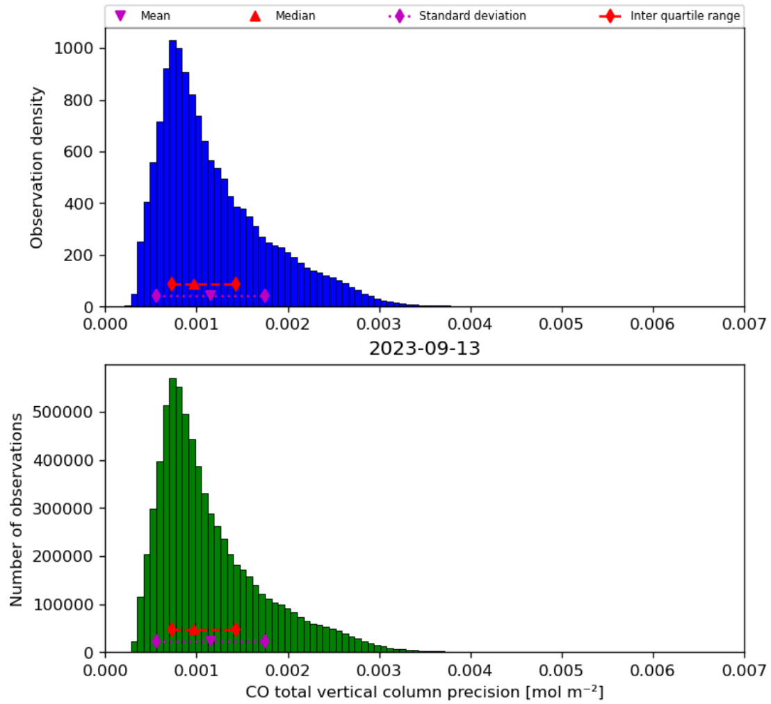
Figure 20: Histogram of “CO total vertical column precision” for 2023-09-12 to 2023-09-14
