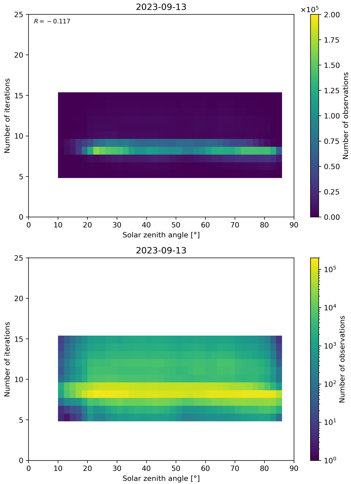
Figure 67: Scatter density plot of “Solar zenith angle” against “Number of iterations” for 2023-09-12 to 2023-09-14.
