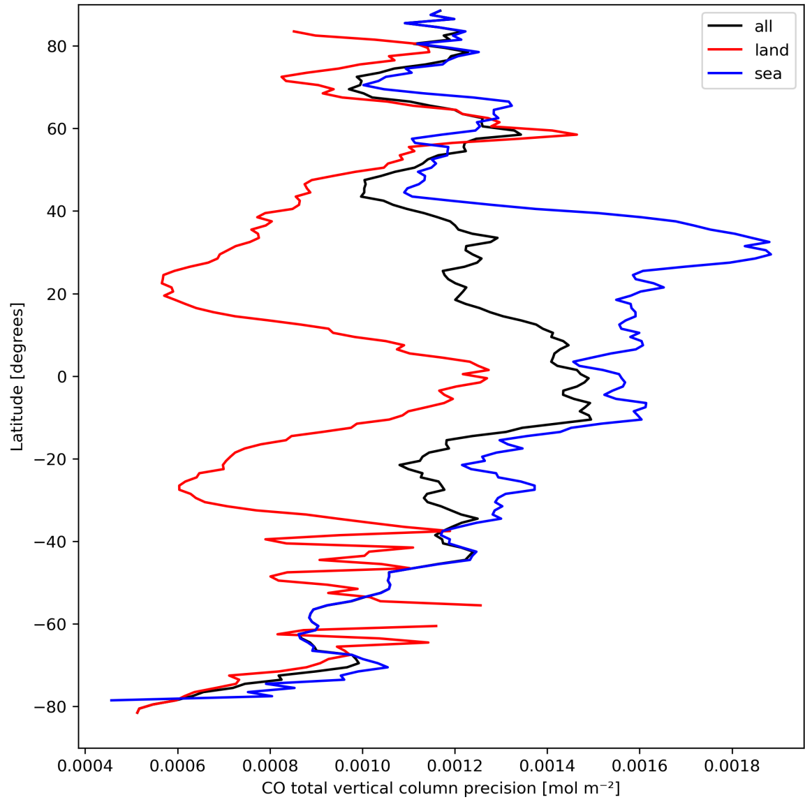
Figure 12: Zonal average of “CO total vertical column precision” for 2023-09-12 to 2023-09-14.
