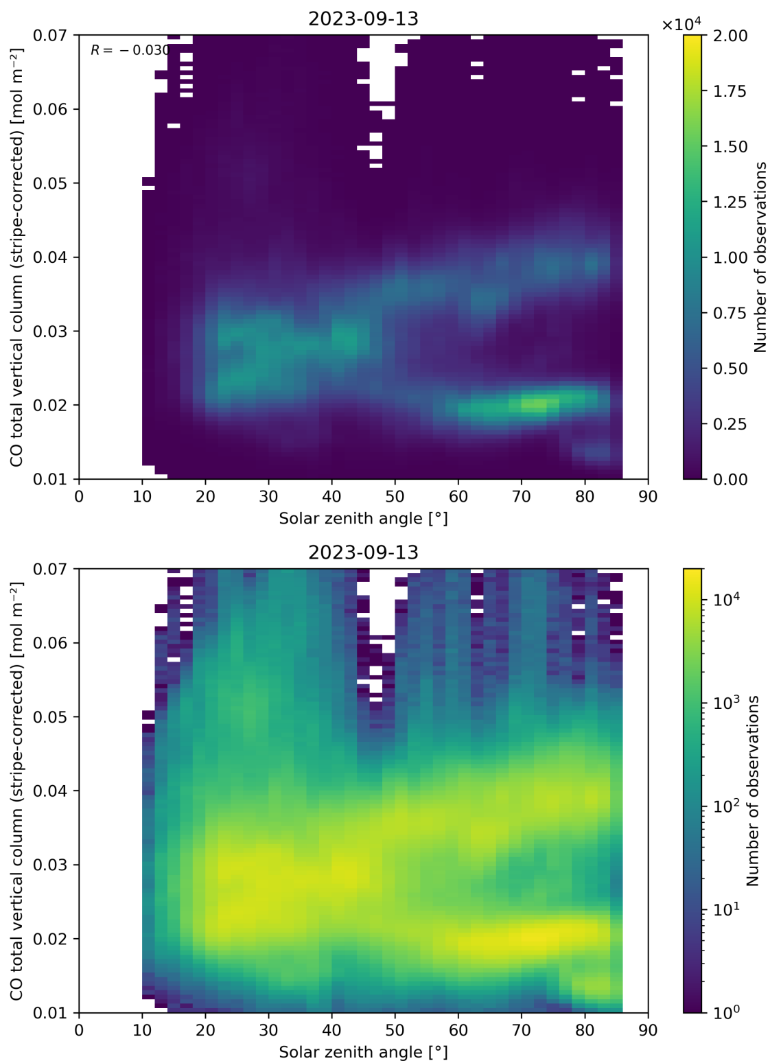
Figure 62: Scatter density plot of “Solar zenith angle” against “CO total vertical column (stripe-corrected)” for 2023-09-12 to 2023-09-14.
