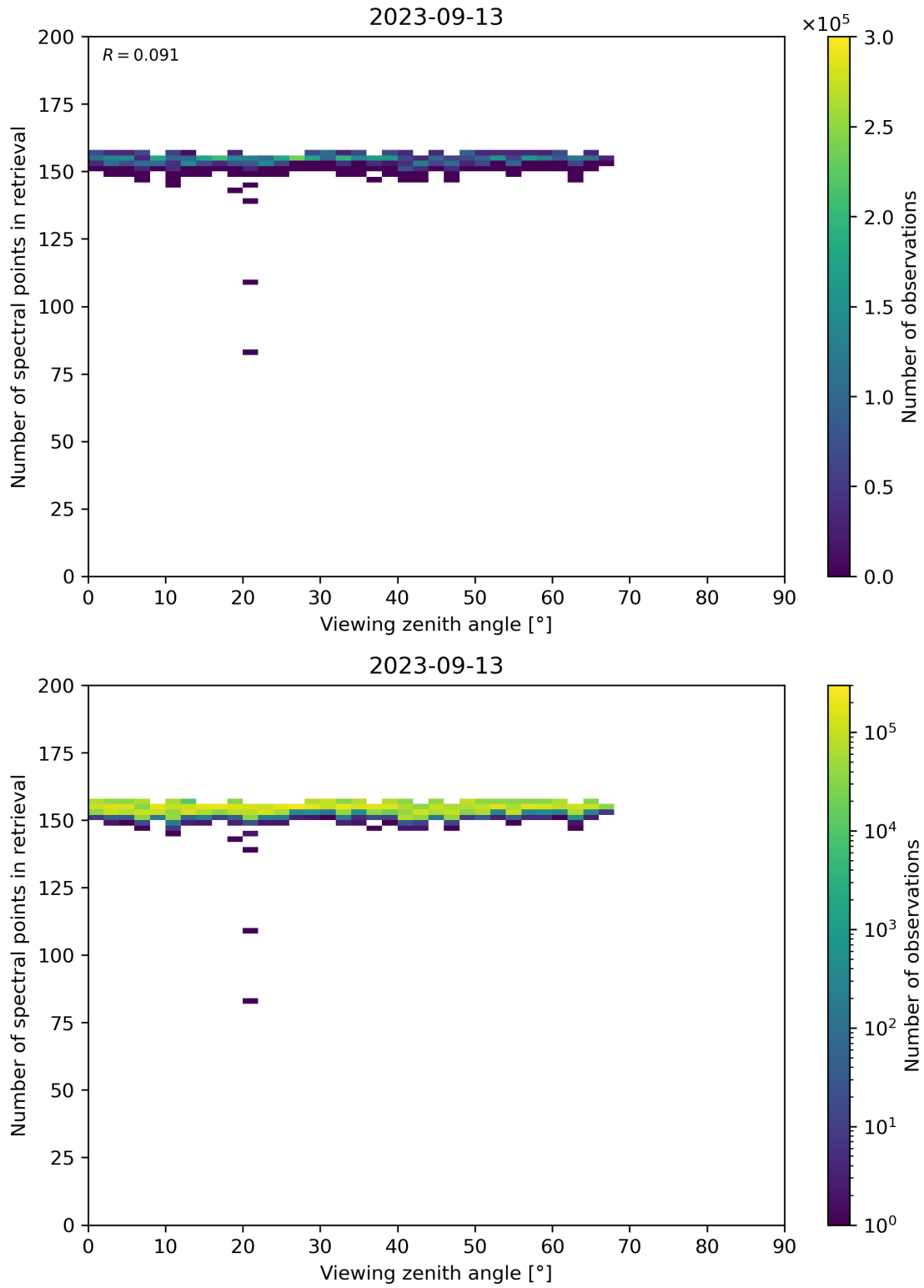
Figure 76: Scatter density plot of “Viewing zenith angle” against “Number of spectral points in retrieval” for 2023-09-12 to 2023-09-14.
