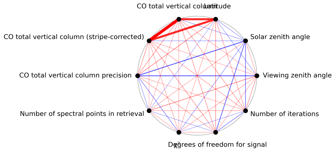
Figure 1: Map of correlation graph for 2023-09-12 to 2023-09-14.
