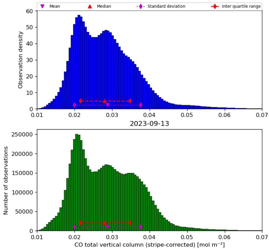
Figure 19: Histogram of “CO total vertical column (stripe-corrected)” for 2023-09-12 to 2023-09-14
