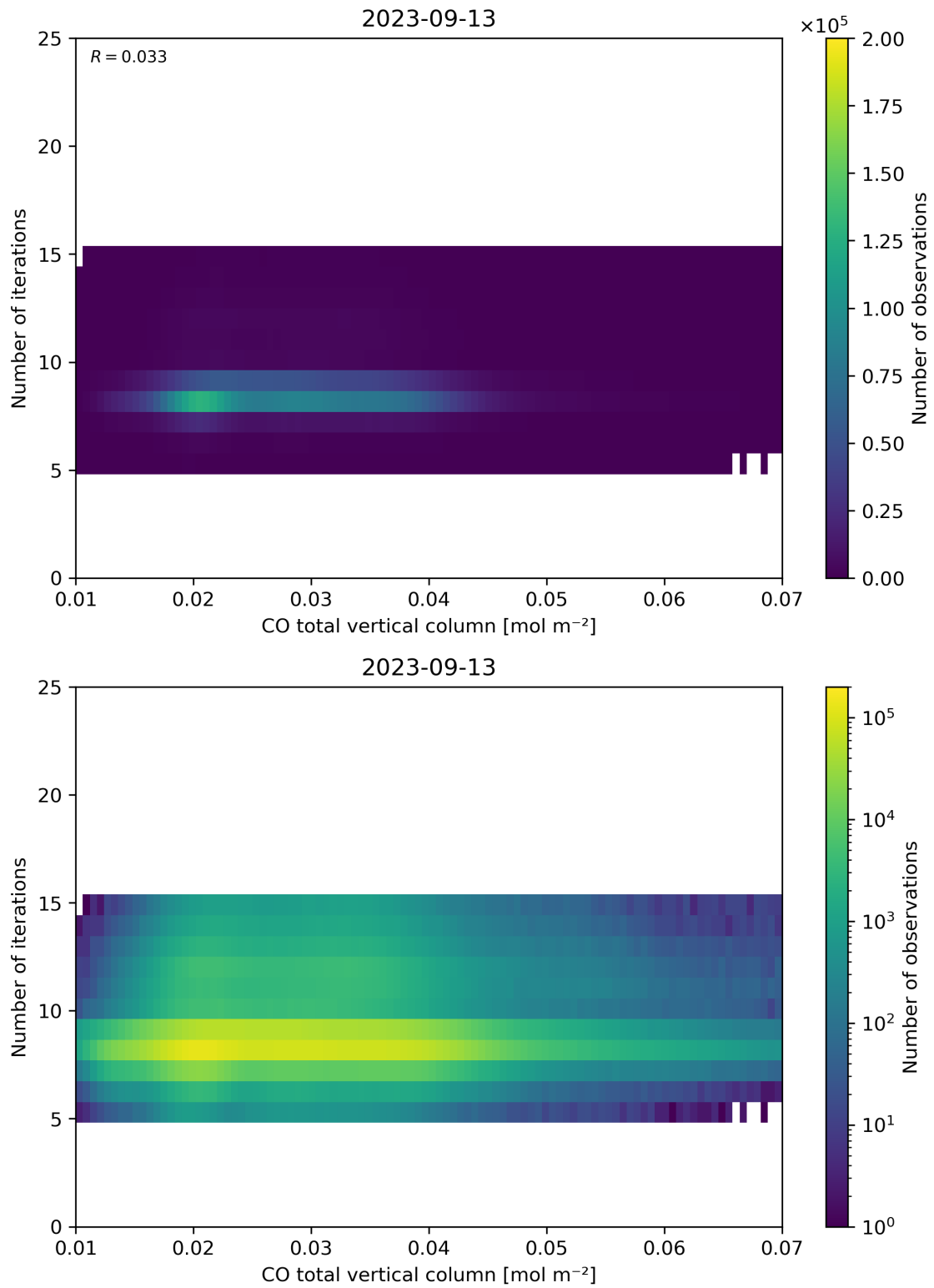
Figure 42: Scatter density plot of “CO total vertical column” against “Number of iterations” for 2023-09-12 to 2023-09-14.
