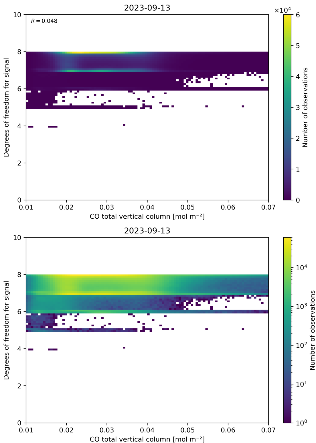
Figure 41: Scatter density plot of “CO total vertical column” against “Degrees of freedom for signal” for 2023-09-12 to 2023-09-14.
