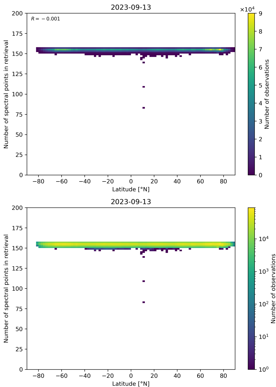
Figure 57: Scatter density plot of “Latitude” against “Number of spectral points in retrieval” for 2023-09-12 to 2023-09-14.
