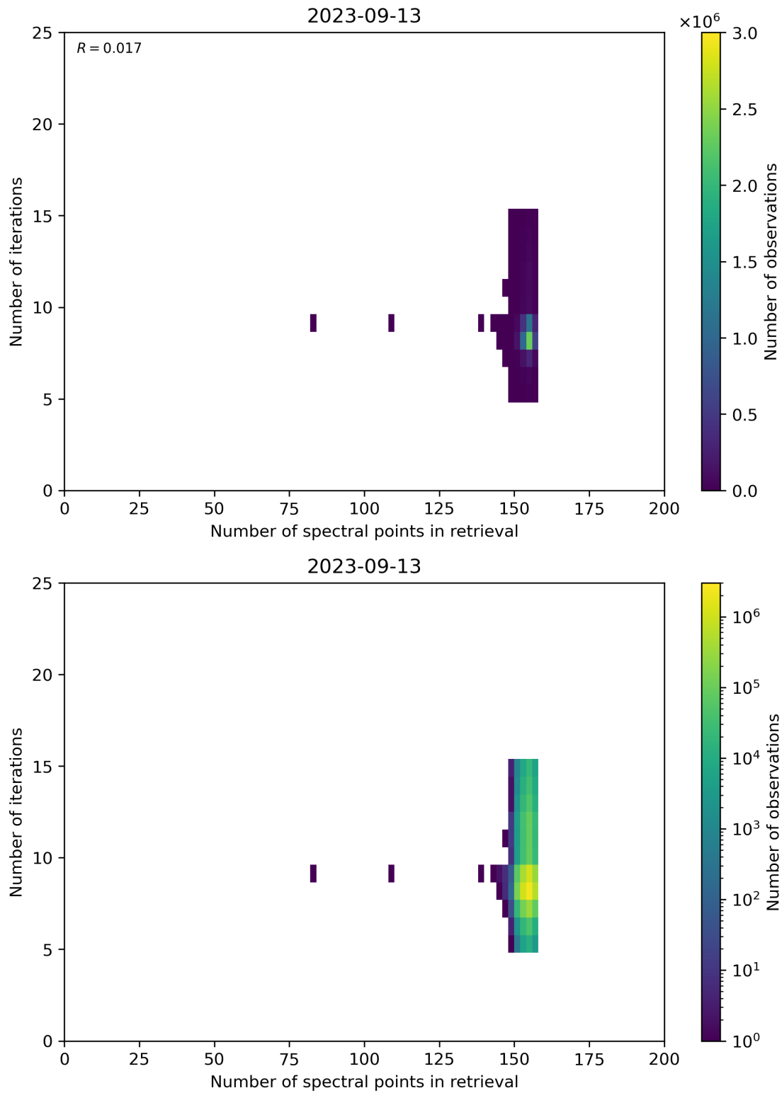
Figure 60: Scatter density plot of “Number of spectral points in retrieval” against “Number of iterations” for 2023-09-12 to 2023-09-14.
