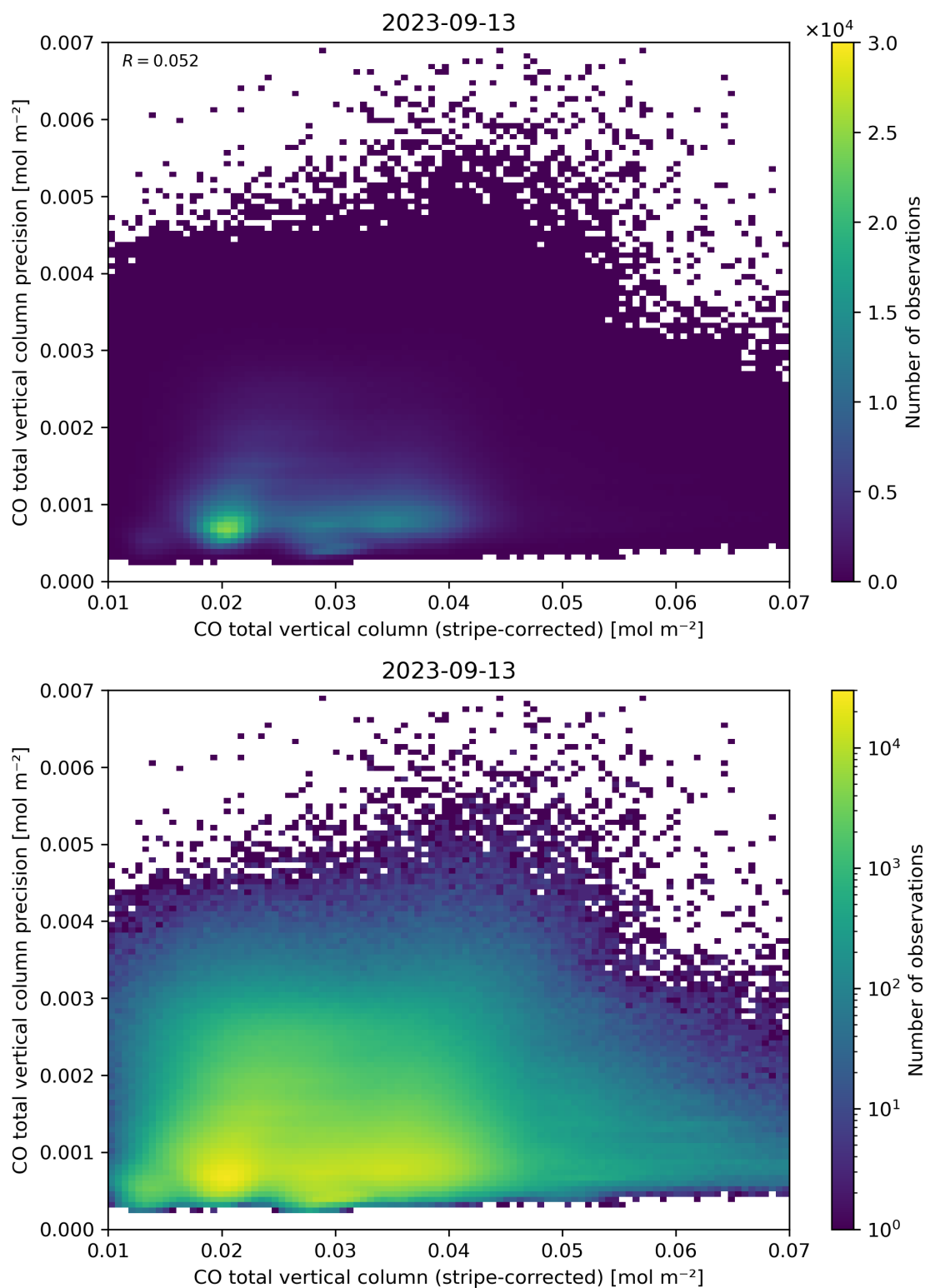
Figure 36: Scatter density plot of “CO total vertical column (stripe-corrected)” against “CO total vertical column precision” for 2023-09-12 to 2023-09-14.
