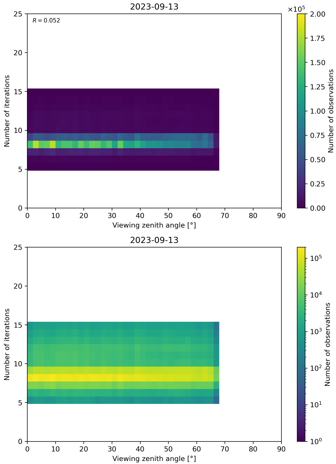
Figure 75: Scatter density plot of “Viewing zenith angle” against “Number of iterations” for 2023-09-12 to 2023-09-14.
