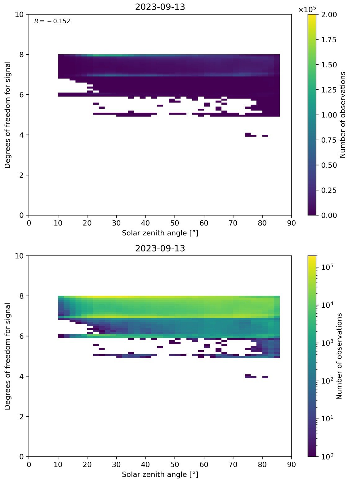
Figure 65: Scatter density plot of “Solar zenith angle” against “Degrees of freedom for signal” for 2023-09-12 to 2023-09-14.
