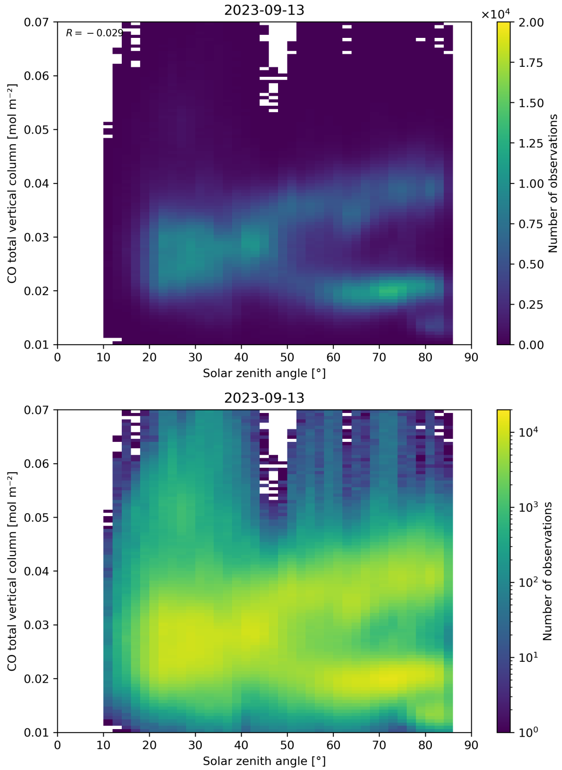
Figure 61: Scatter density plot of “Solar zenith angle” against “CO total vertical column” for 2023-09-12 to 2023-09-14.
