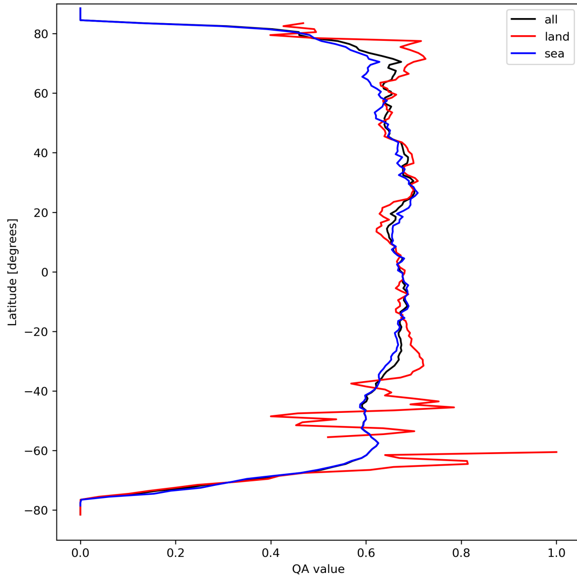
Figure 9: Zonal average of “QA value” for 2023-09-12 to 2023-09-14.
