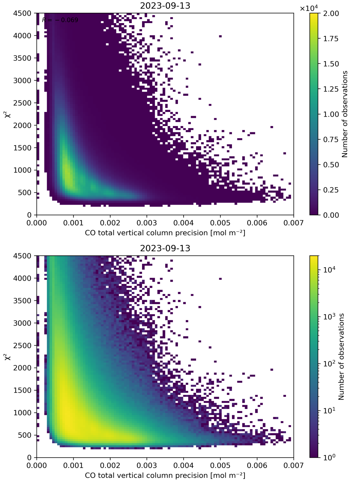
Figure 44: Scatter density plot of “CO total vertical column precision” against “ \chi^2 ” for 2023-09-12 to 2023-09-14.
