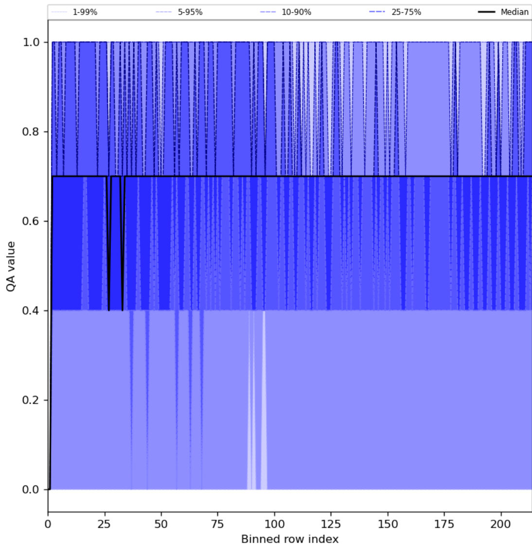
Figure 25: Along track statistics of “QA value” for 2023-09-12 to 2023-09-14
