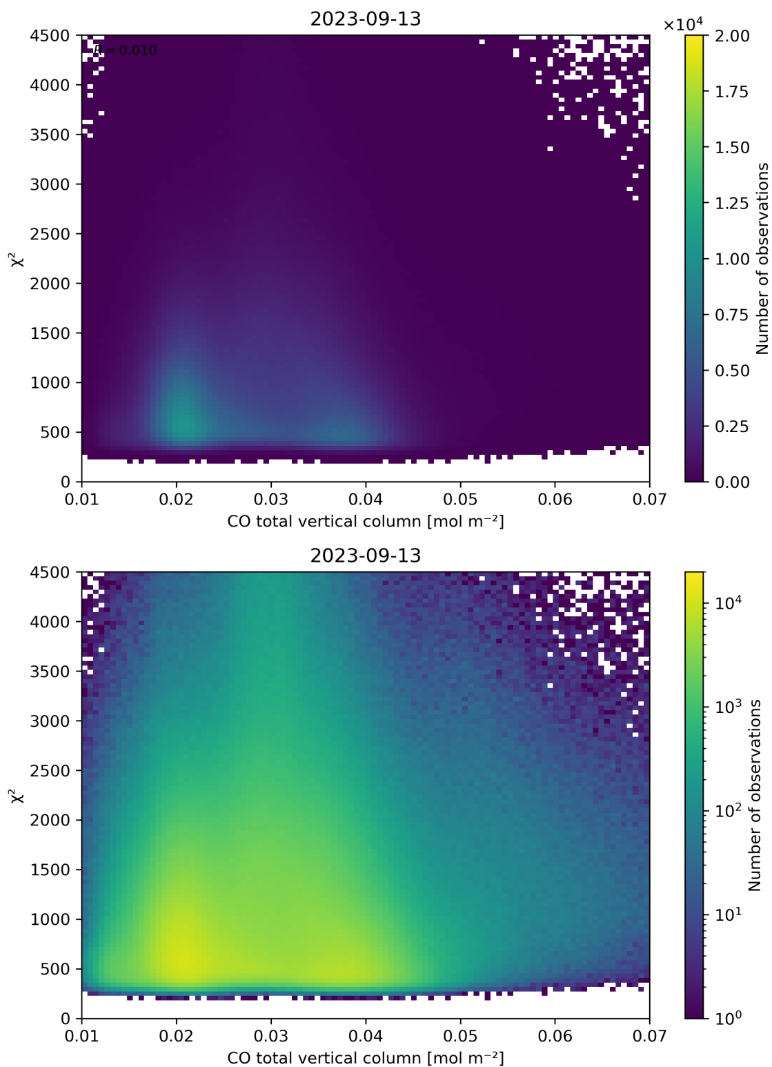
Figure 35: Scatter density plot of “CO total vertical column” against “ \chi^2 ” for 2023-09-12 to 2023-09-14.
