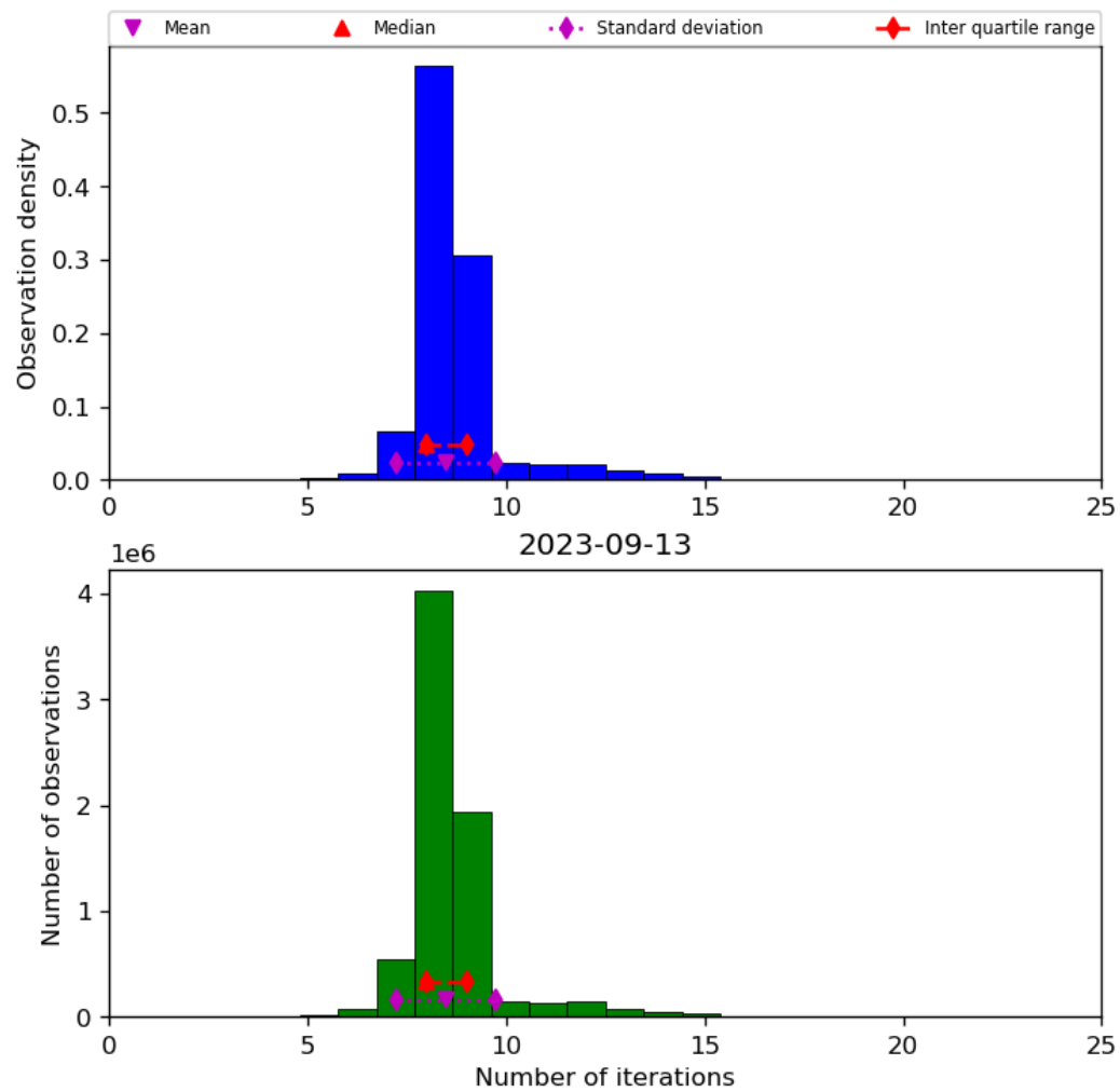
Figure 24: Histogram of “Number of iterations” for 2023-09-12 to 2023-09-14
