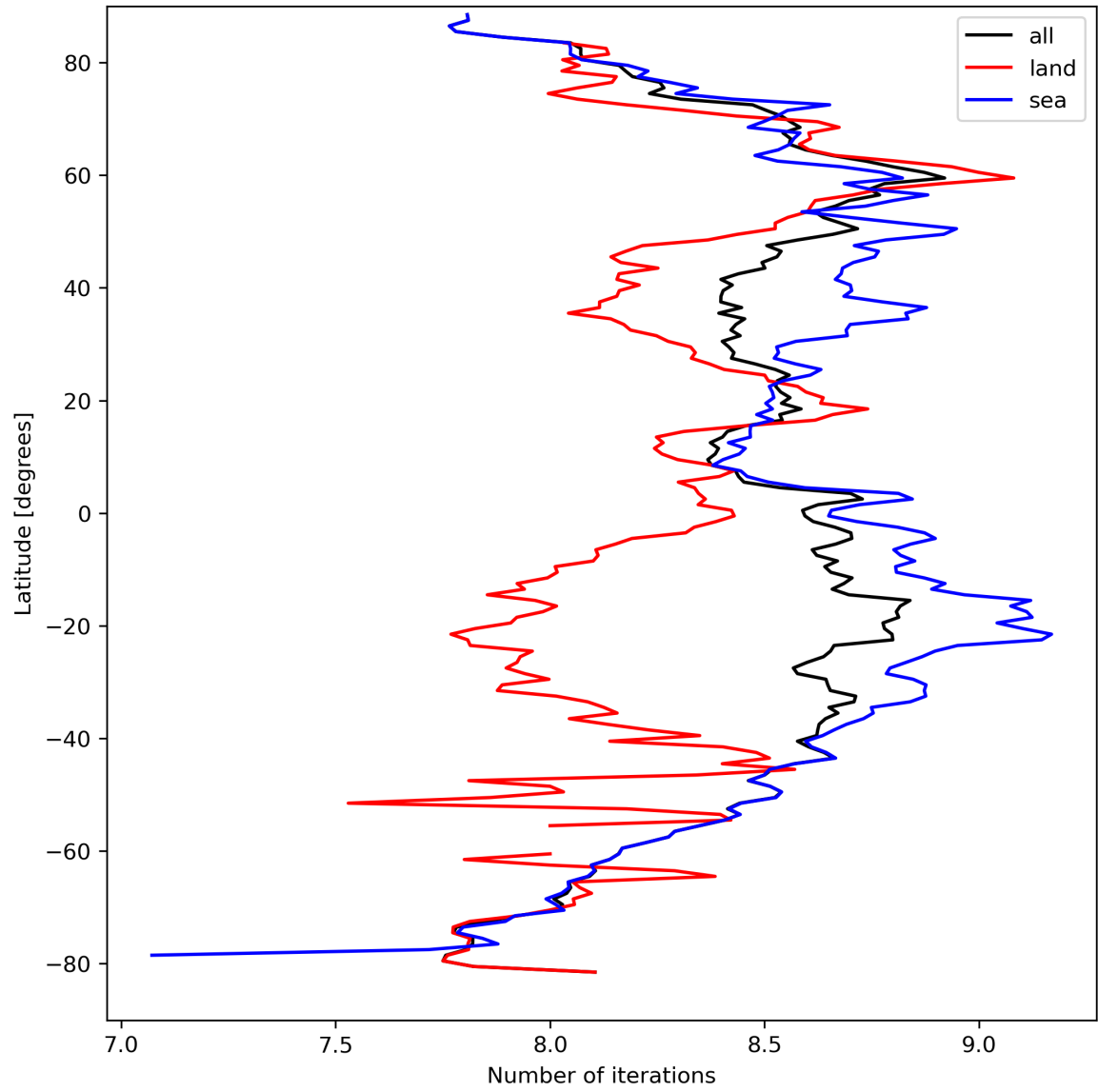
Figure 16: Zonal average of “Number of iterations” for 2023-09-12 to 2023-09-14.
