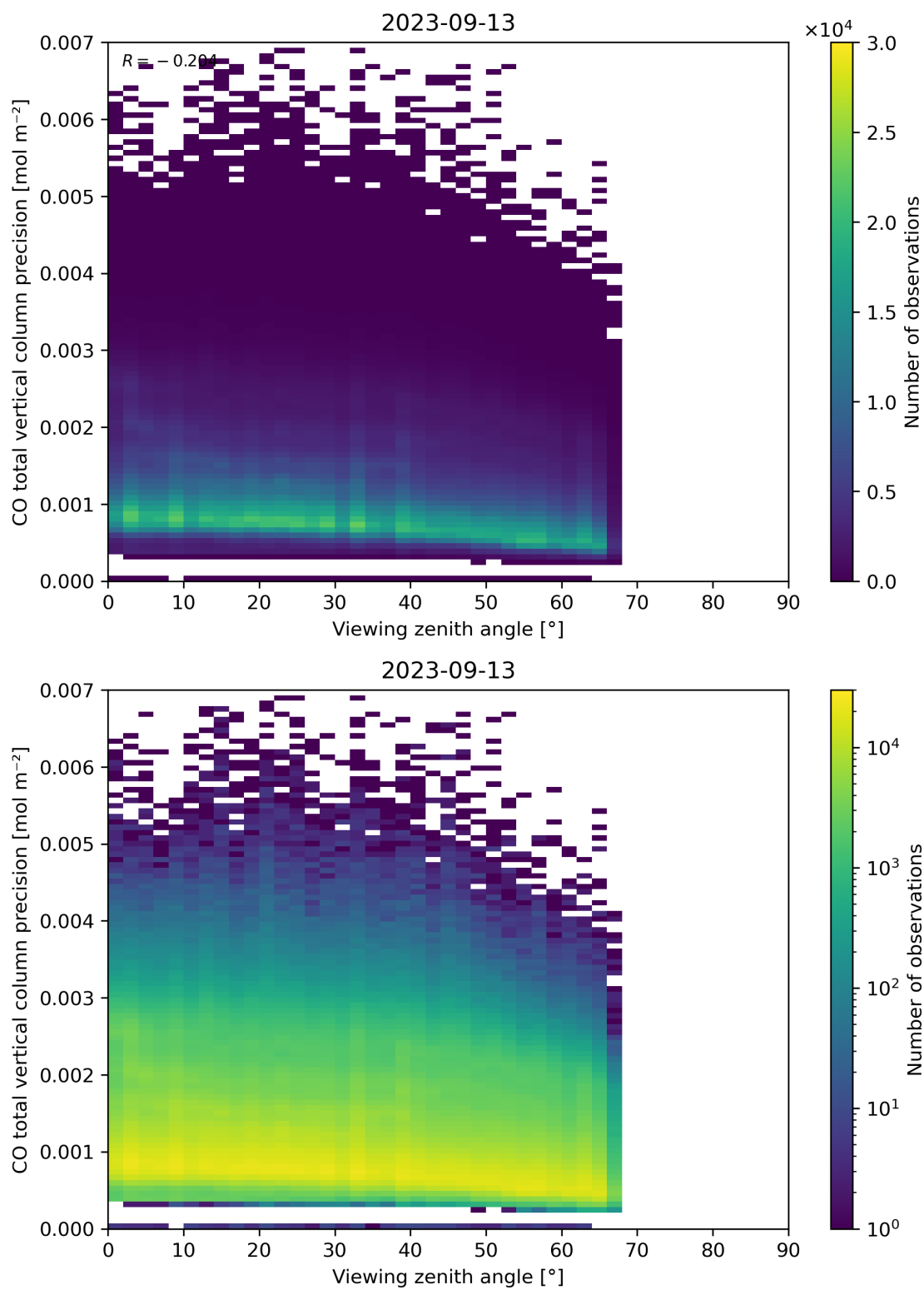
Figure 71: Scatter density plot of “Viewing zenith angle” against “CO total vertical column precision” for 2023-09-12 to 2023-09-14.
