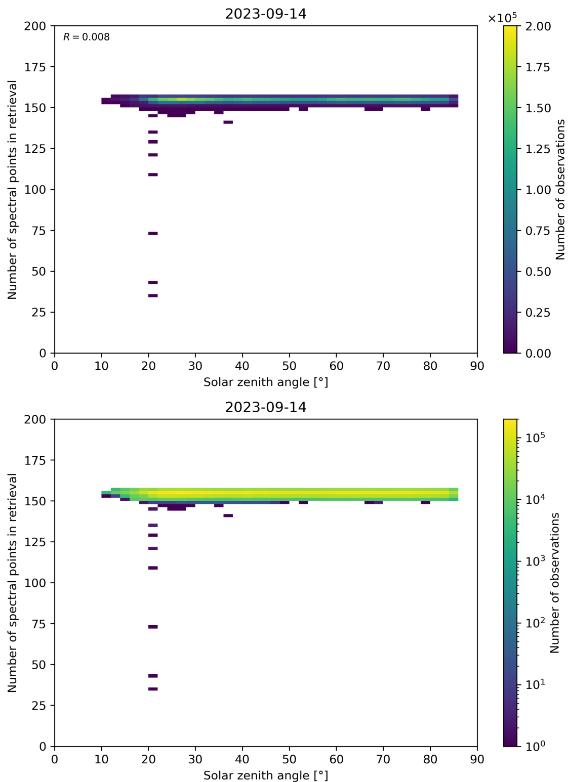
Figure 68: Scatter density plot of “Solar zenith angle” against “Number of spectral points in retrieval” for 2023-09-13 to 2023-09-15.
