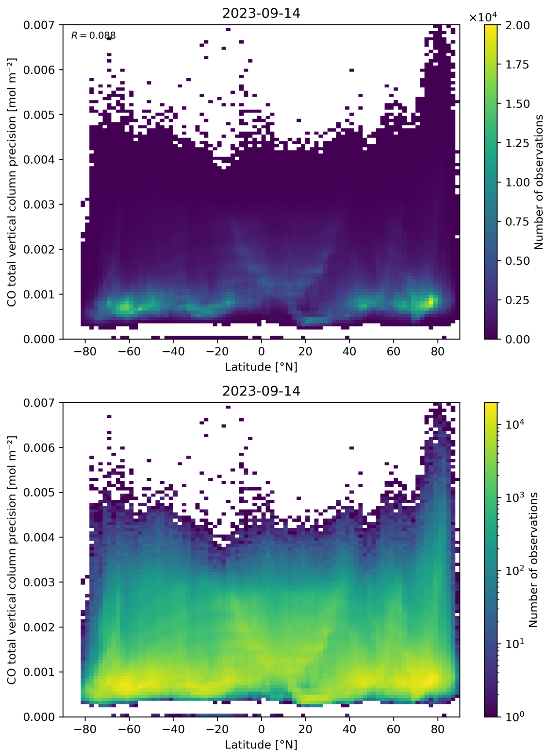
Figure 53: Scatter density plot of “Latitude” against “CO total vertical column precision” for 2023-09-13 to 2023-09-15.
