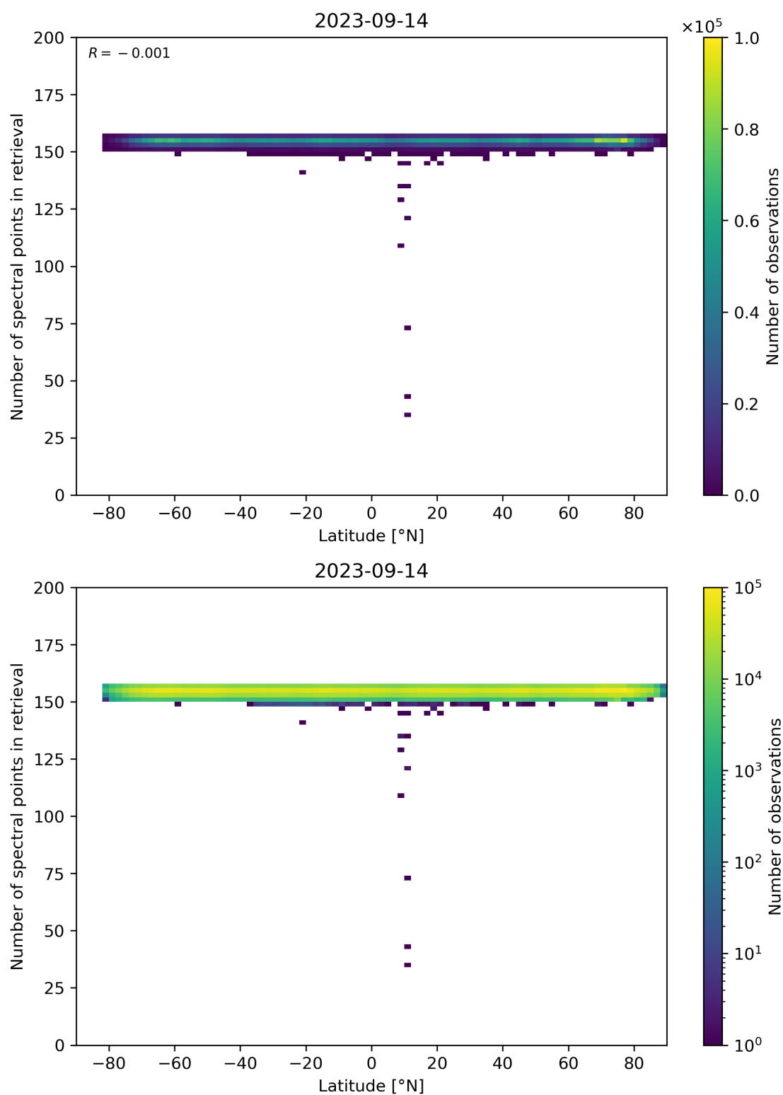
Figure 57: Scatter density plot of “Latitude” against “Number of spectral points in retrieval” for 2023-09-13 to 2023-09-15.
