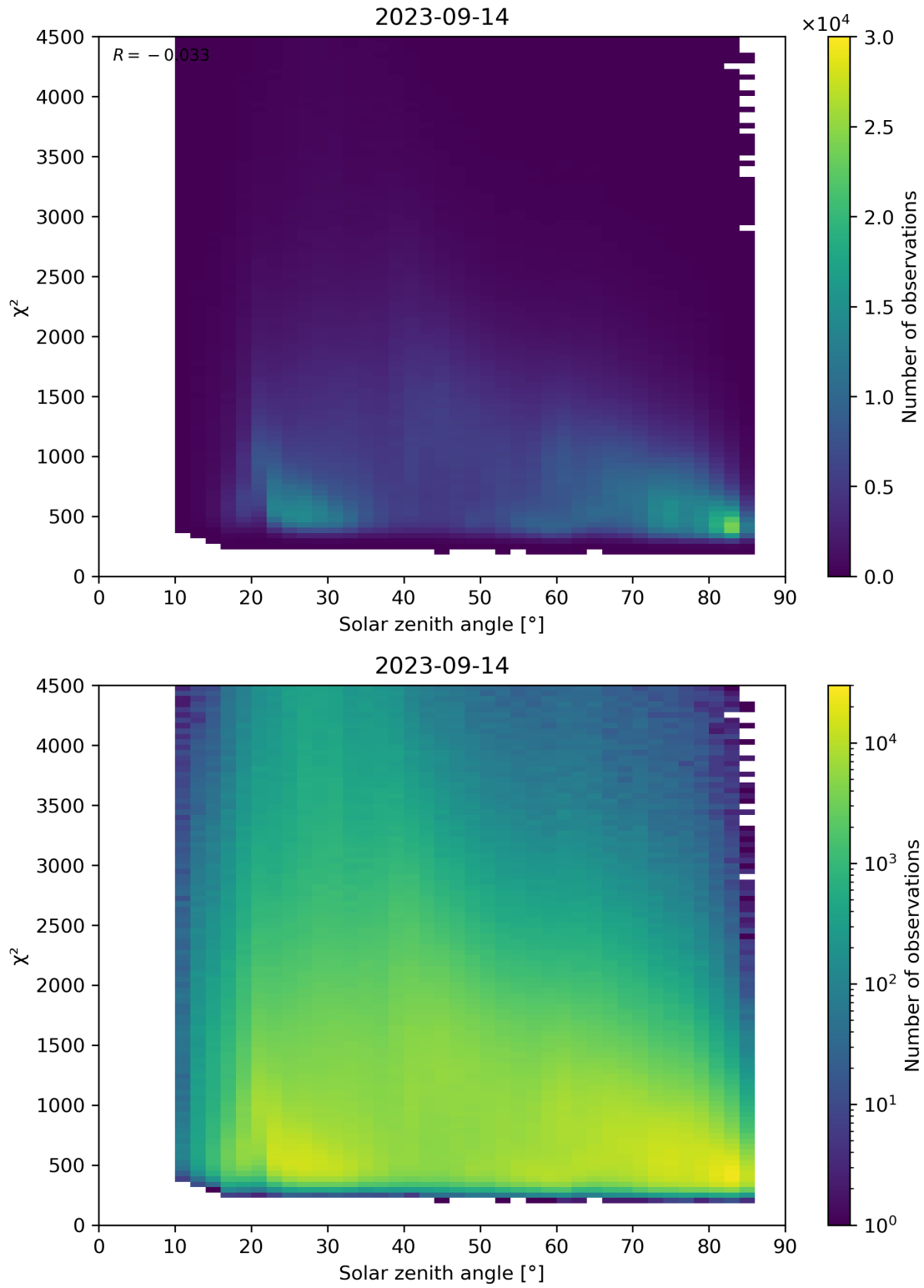
Figure 64: Scatter density plot of “Solar zenith angle” against “ \chi^2 ” for 2023-09-13 to 2023-09-15.
