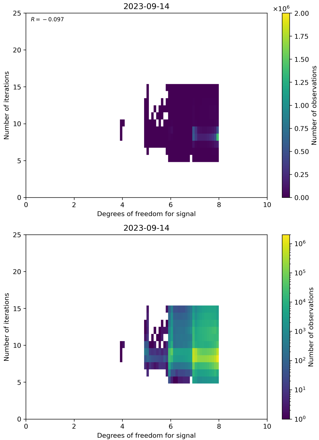
Figure 50: Scatter density plot of “Degrees of freedom for signal” against “Number of iterations” for 2023-09-13 to 2023-09-15.
