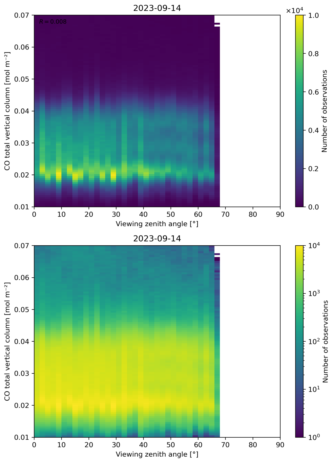
Figure 69: Scatter density plot of “Viewing zenith angle” against “CO total vertical column” for 2023-09-13 to 2023-09-15.
