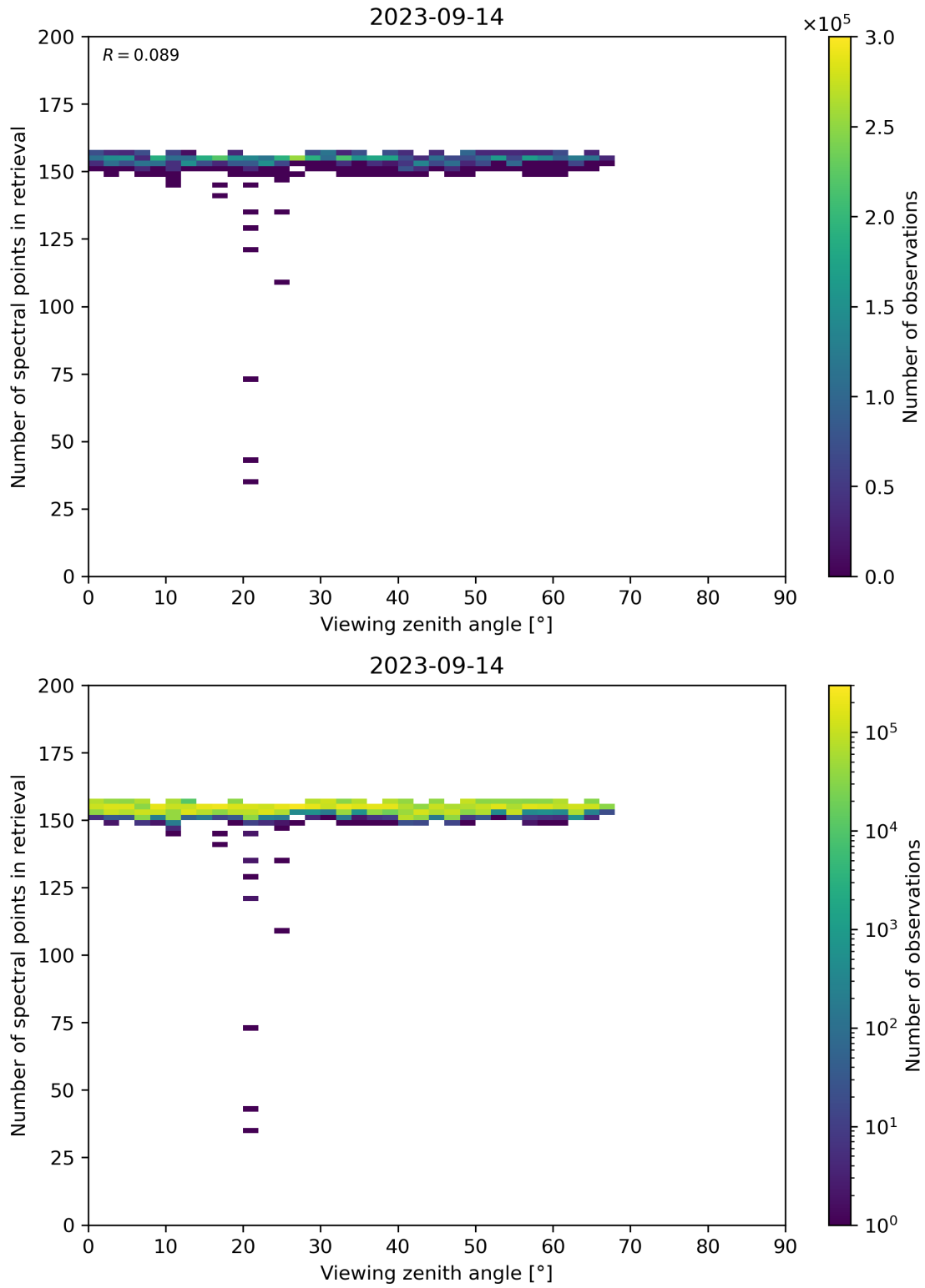
Figure 76: Scatter density plot of “Viewing zenith angle” against “Number of spectral points in retrieval” for 2023-09-13 to 2023-09-15.
