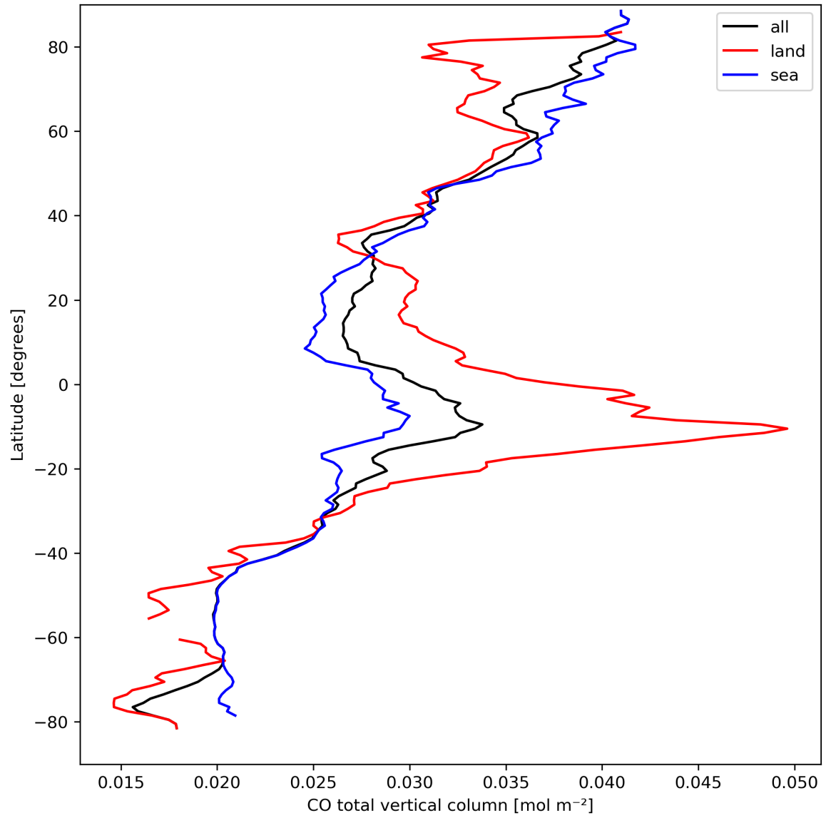
Figure 10: Zonal average of “CO total vertical column” for 2023-09-13 to 2023-09-15.
