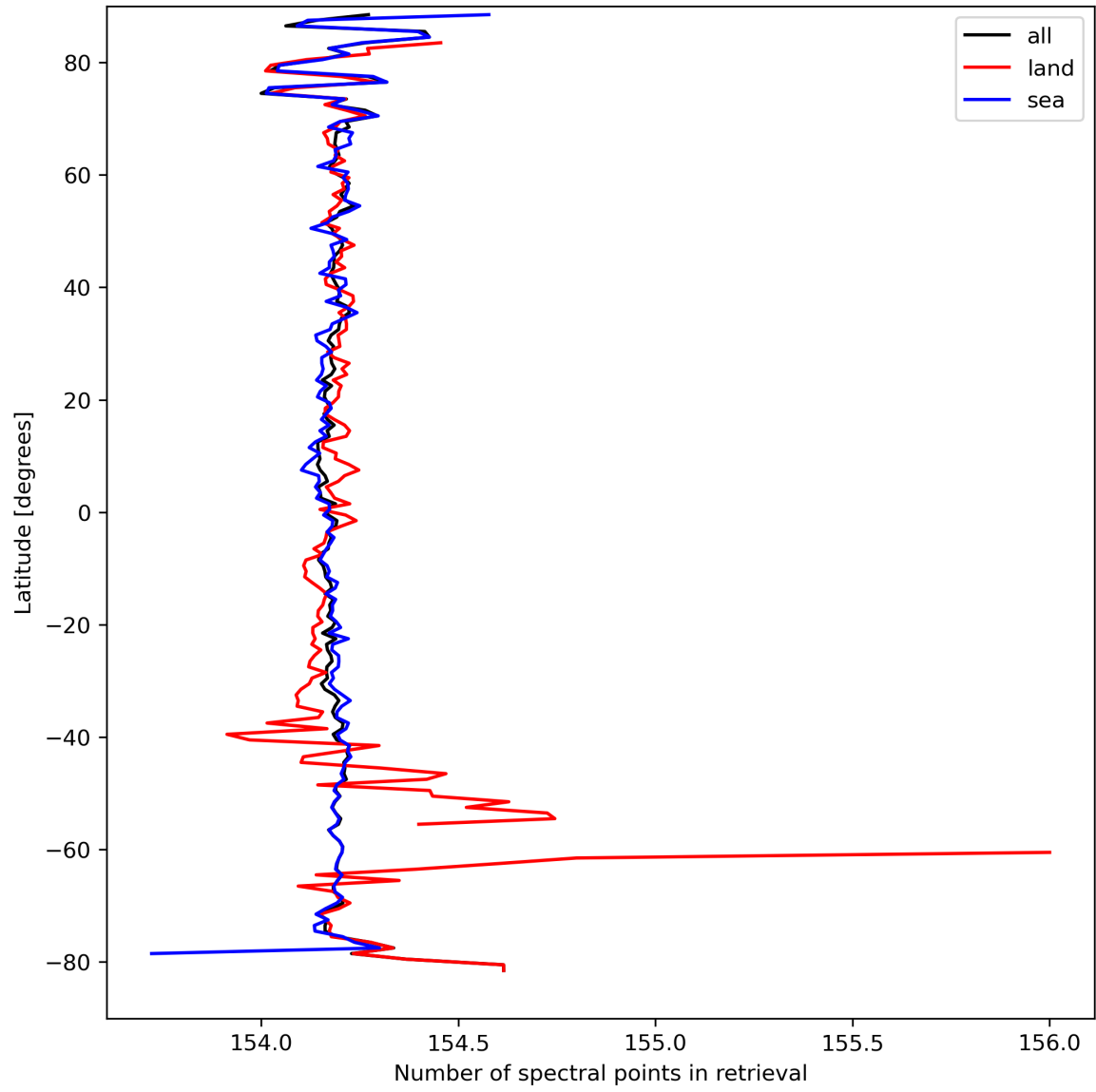
Figure 13: Zonal average of “Number of spectral points in retrieval” for 2023-09-13 to 2023-09-15.
