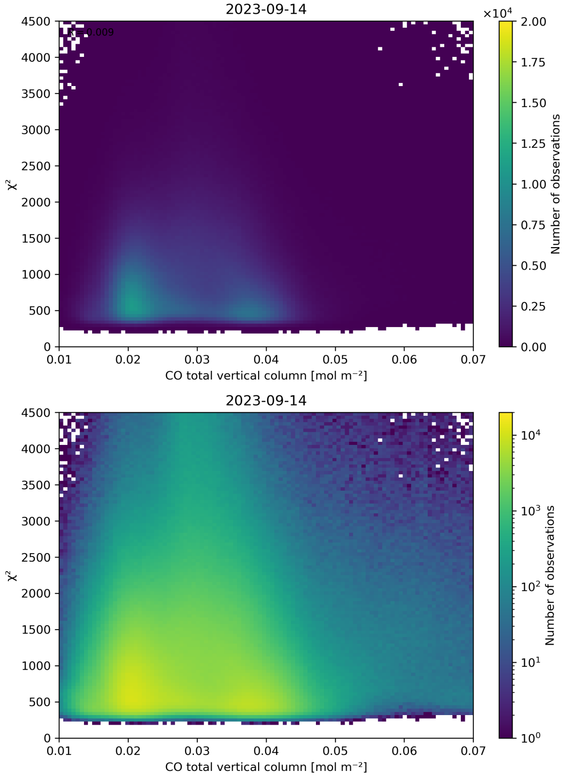
Figure 35: Scatter density plot of “CO total vertical column” against “ \chi^2 ” for 2023-09-13 to 2023-09-15.
