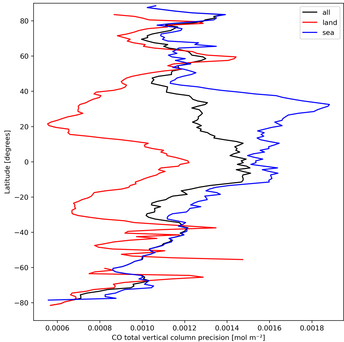
Figure 12: Zonal average of “CO total vertical column precision” for 2023-09-13 to 2023-09-15.
