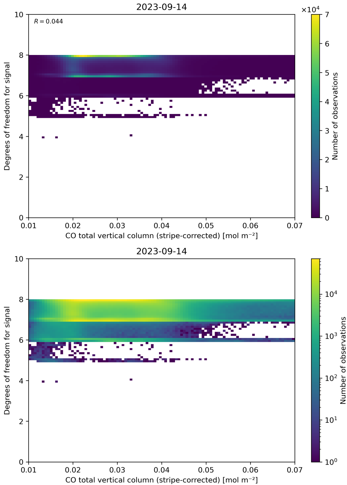
Figure 38: Scatter density plot of “CO total vertical column (stripe-corrected)” against “Degrees of freedom for signal” for 2023-09-13 to 2023-09-15.
