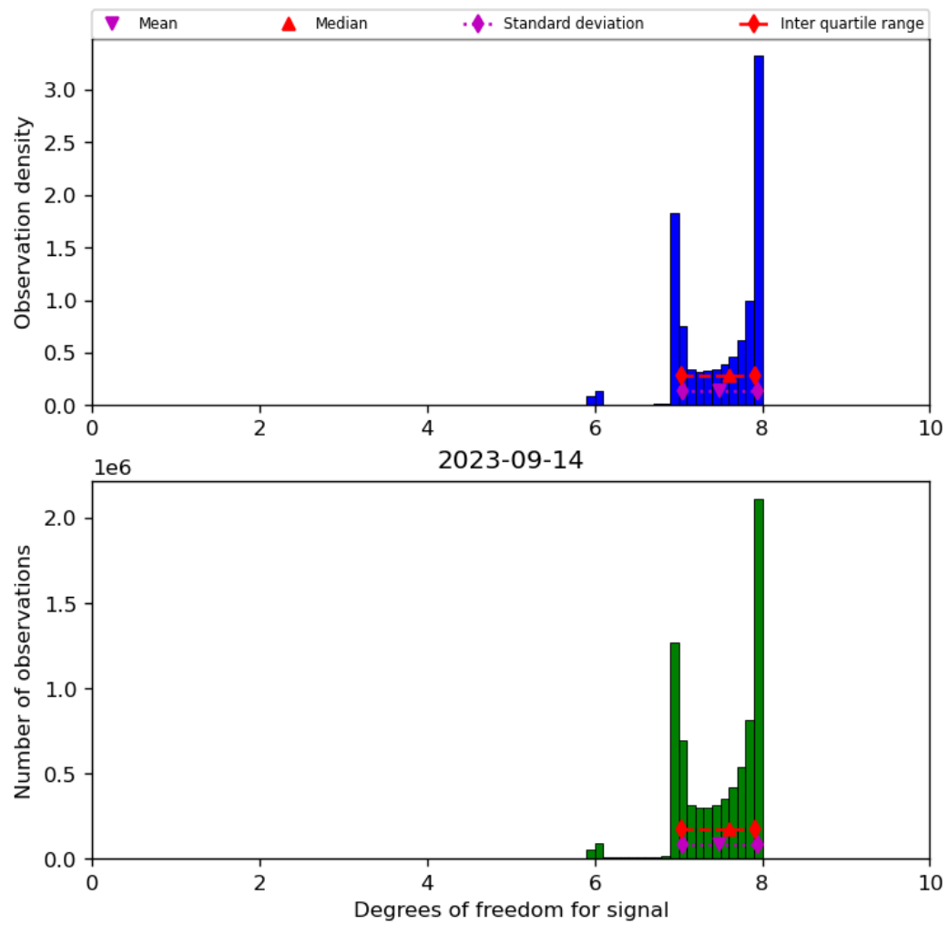
Figure 23: Histogram of “Degrees of freedom for signal” for 2023-09-13 to 2023-09-15
