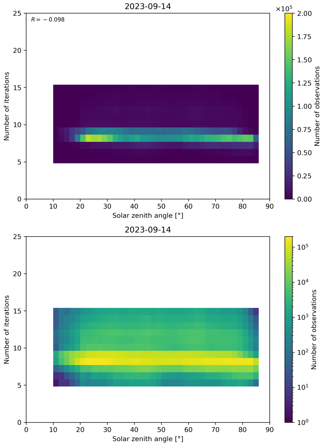
Figure 67: Scatter density plot of “Solar zenith angle” against “Number of iterations” for 2023-09-13 to 2023-09-15.
