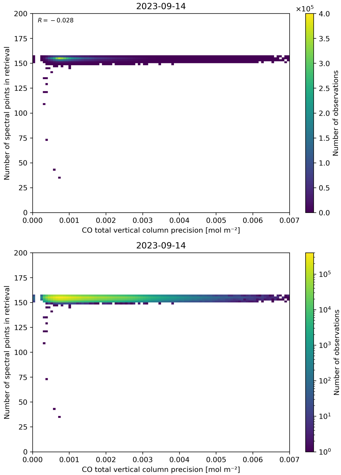
Figure 47: Scatter density plot of “CO total vertical column precision” against “Number of spectral points in retrieval” for 2023-09-13 to 2023-09-15.
