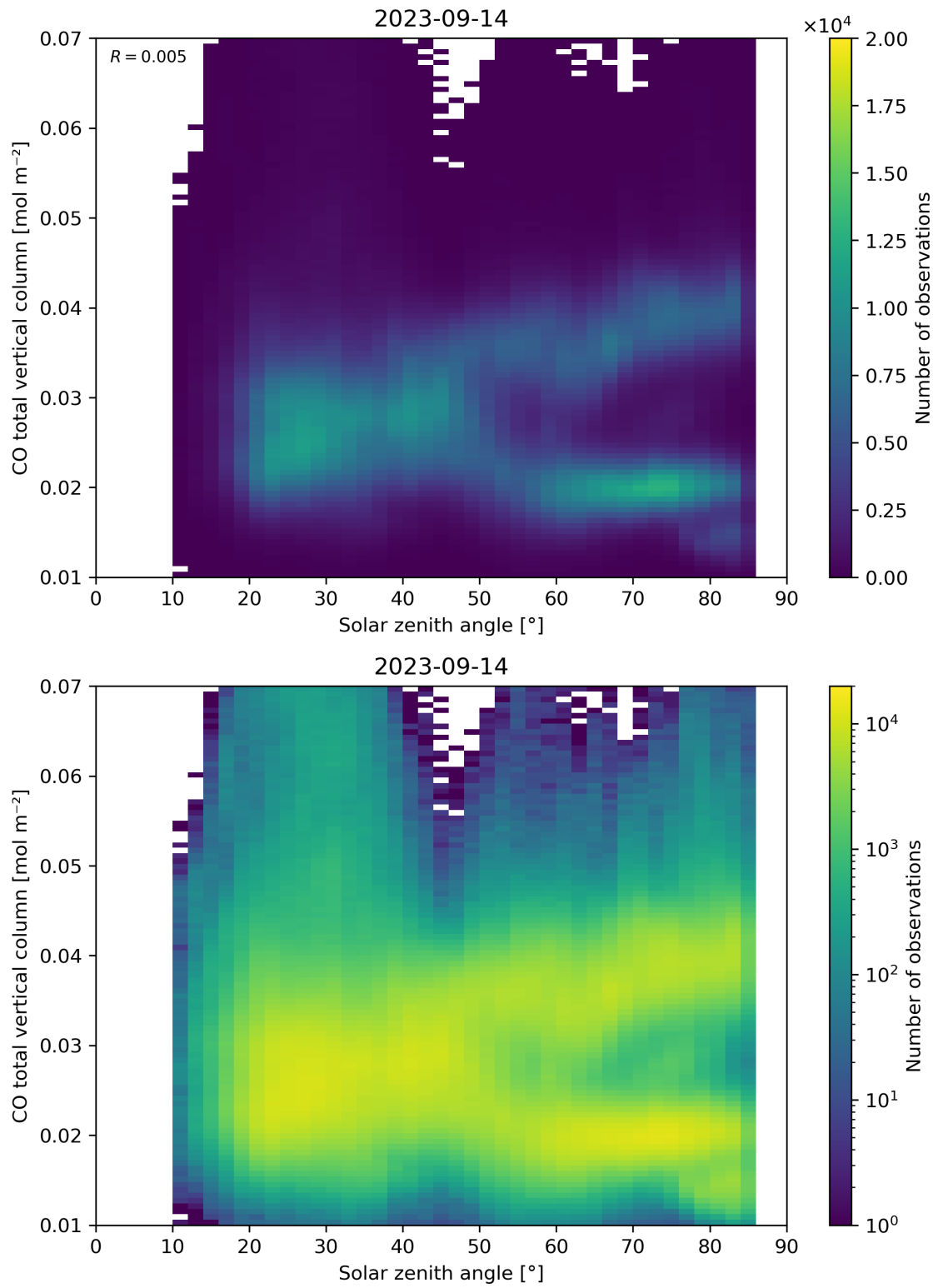
Figure 61: Scatter density plot of “Solar zenith angle” against “CO total vertical column” for 2023-09-13 to 2023-09-15.
