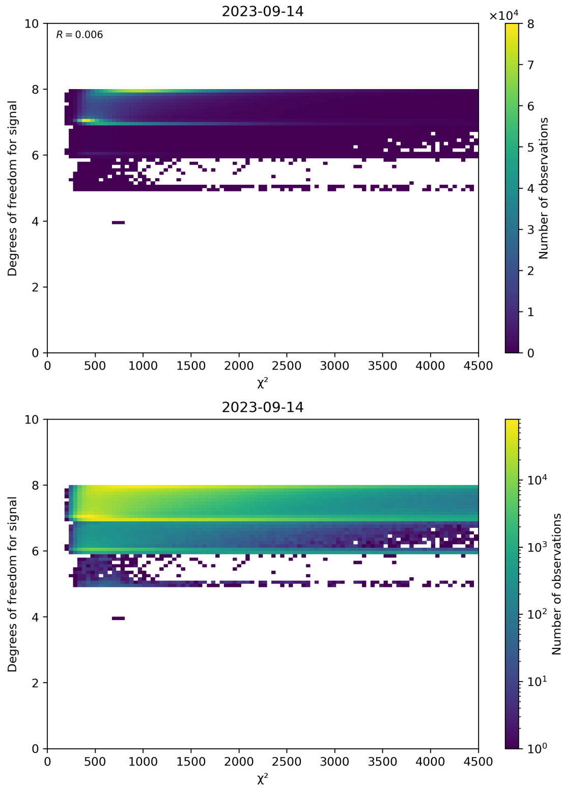
Figure 48: Scatter density plot of " \chi^2 " against "Degrees of freedom for signal" for 2023-09-13 to 2023-09-15.
