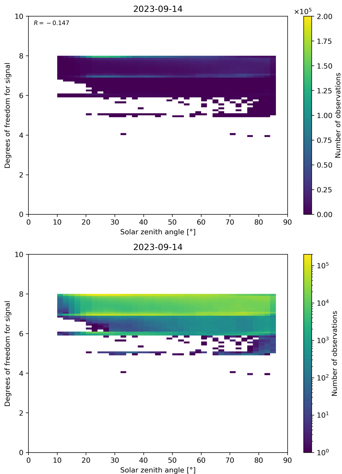
Figure 65: Scatter density plot of “Solar zenith angle” against “Degrees of freedom for signal” for 2023-09-13 to 2023-09-15.
