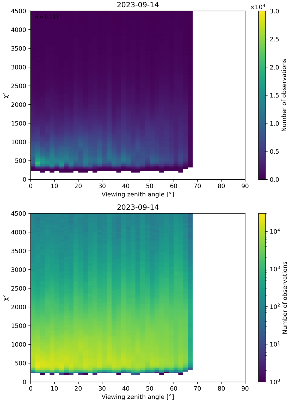
Figure 72: Scatter density plot of “Viewing zenith angle” against “ \chi^2 ” for 2023-09-13 to 2023-09-15.
