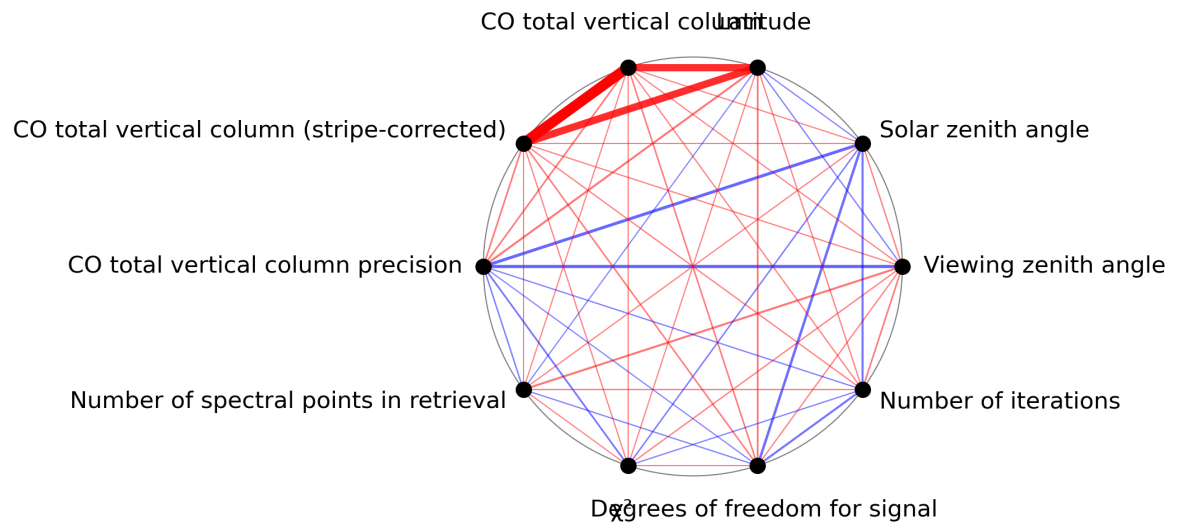
Figure 1: Map of correlation graph for 2023-09-13 to 2023-09-15.
