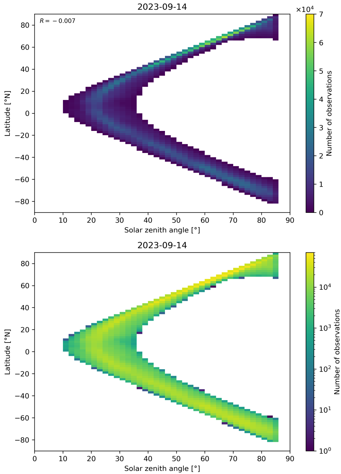
Figure 66: Scatter density plot of “Solar zenith angle” against “Latitude” for 2023-09-13 to 2023-09-15.
