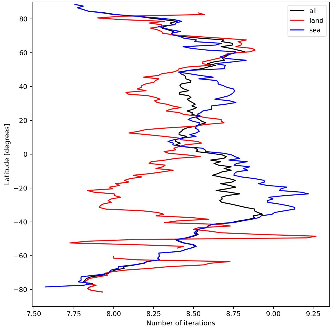
Figure 16: Zonal average of “Number of iterations” for 2023-09-13 to 2023-09-15.
