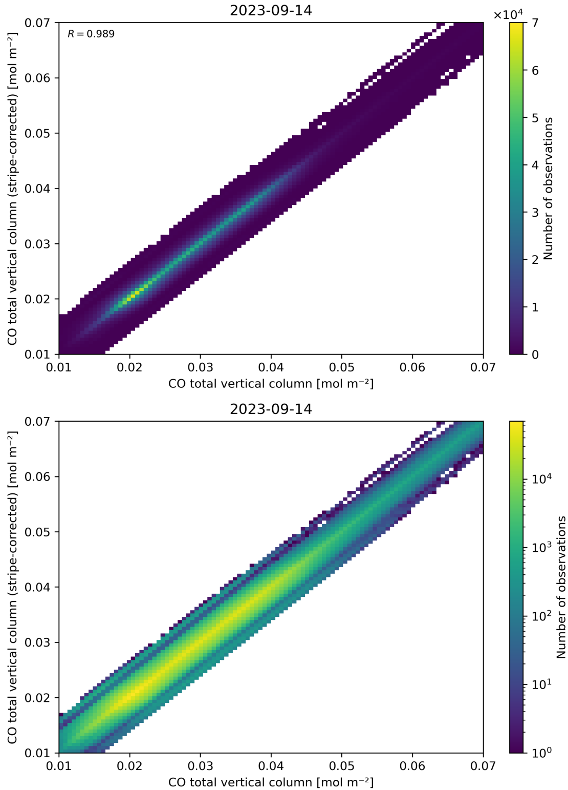
Figure 33: Scatter density plot of “CO total vertical column” against “CO total vertical column (stripe-corrected)” for 2023-09-13 to 2023-09-15.
