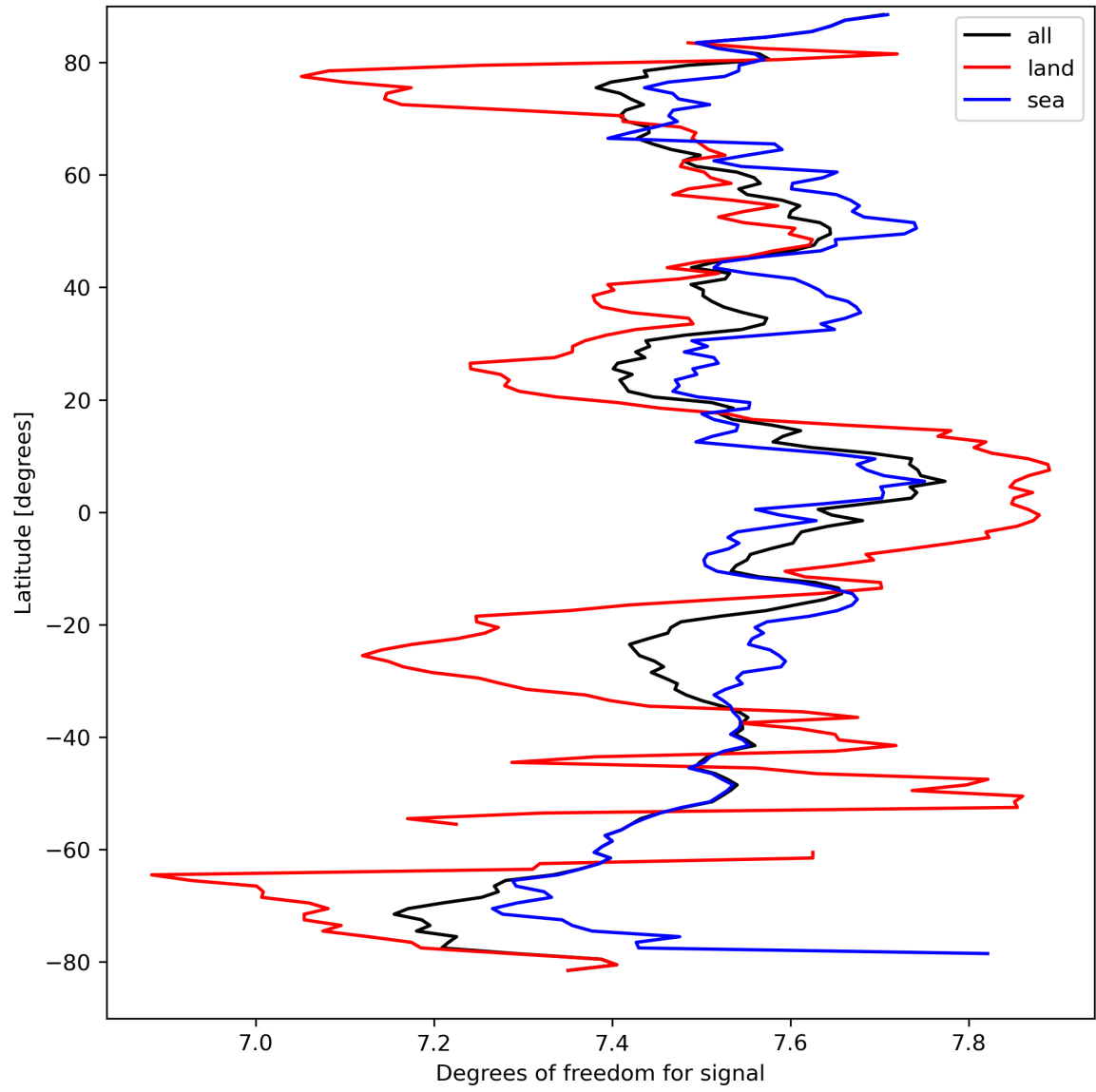
Figure 15: Zonal average of “Degrees of freedom for signal” for 2023-09-13 to 2023-09-15.
