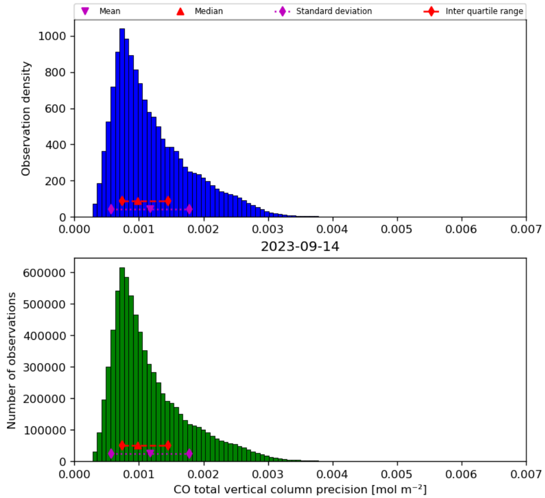
Figure 20: Histogram of “CO total vertical column precision” for 2023-09-13 to 2023-09-15
