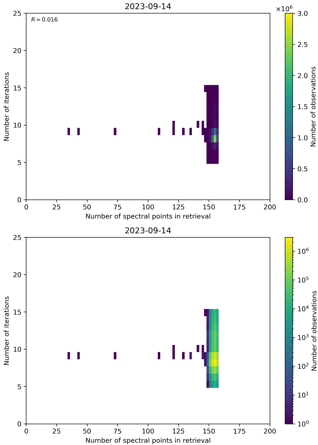
Figure 60: Scatter density plot of “Number of spectral points in retrieval” against “Number of iterations” for 2023-09-13 to 2023-09-15.
