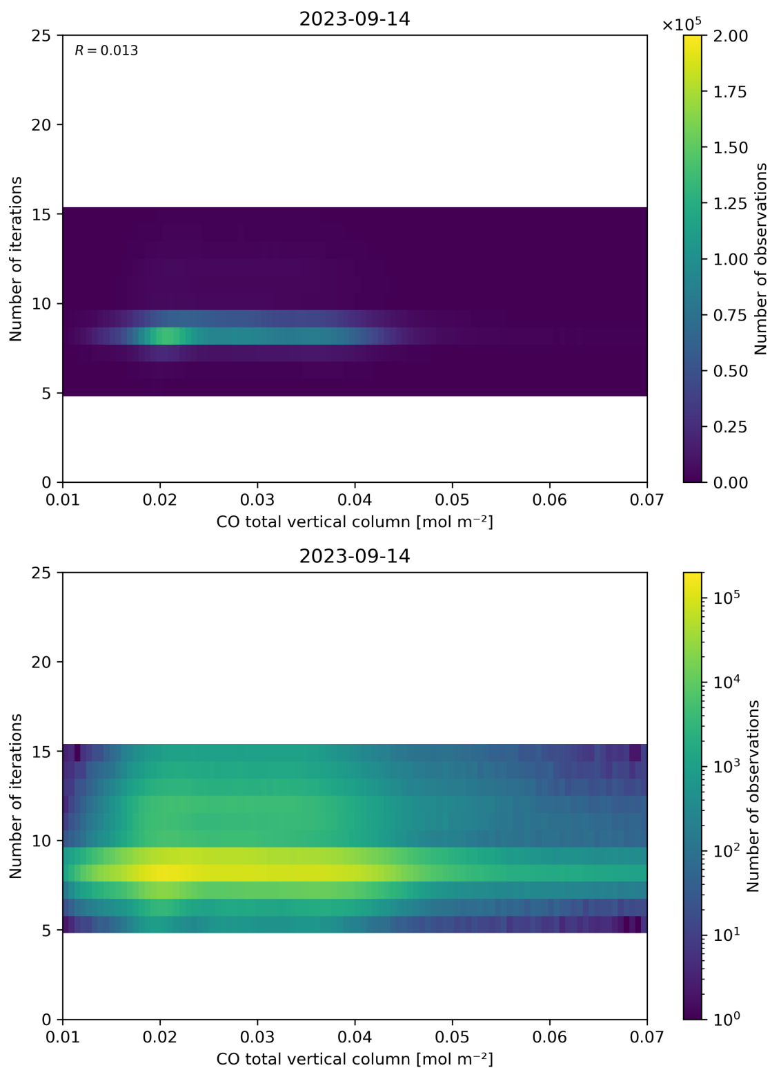
Figure 42: Scatter density plot of “CO total vertical column” against “Number of iterations” for 2023-09-13 to 2023-09-15.
