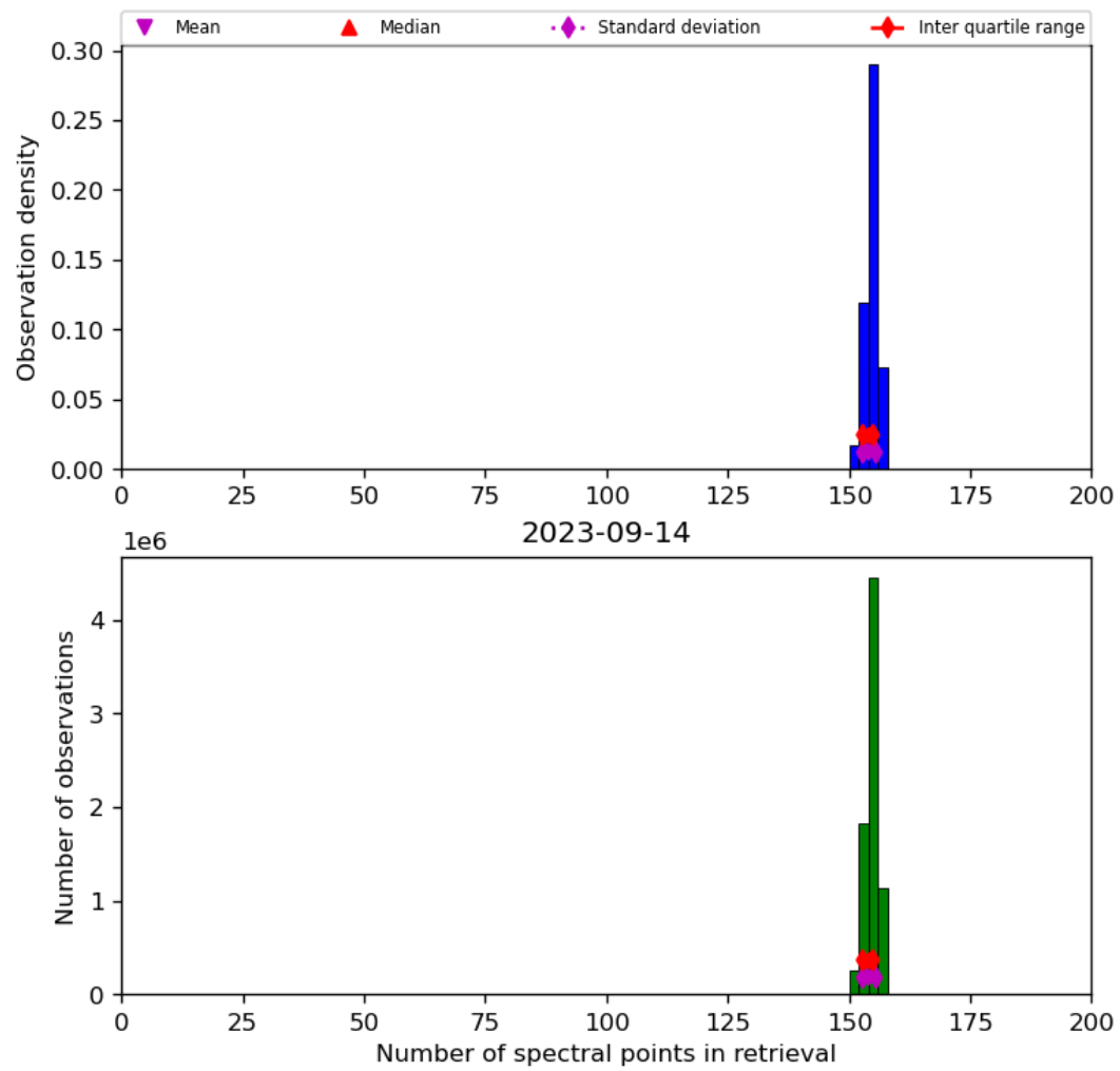
Figure 21: Histogram of “Number of spectral points in retrieval” for 2023-09-13 to 2023-09-15
