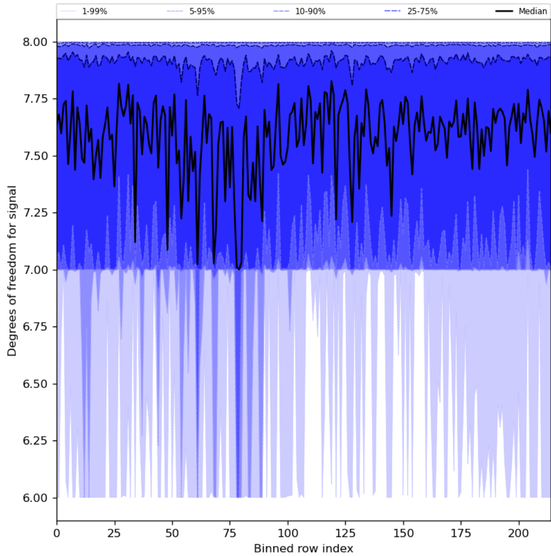
Figure 31: Along track statistics of “Degrees of freedom for signal” for 2023-09-13 to 2023-09-15
