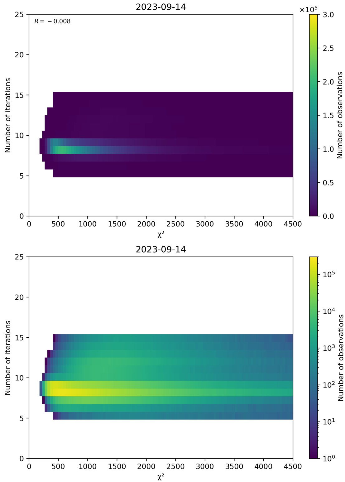
Figure 49: Scatter density plot of “ \chi^2 ” against “Number of iterations” for 2023-09-13 to 2023-09-15.
