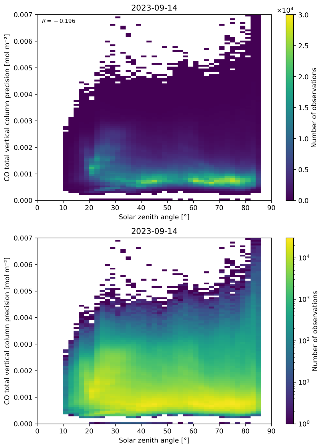
Figure 63: Scatter density plot of “Solar zenith angle” against “CO total vertical column precision” for 2023-09-13 to 2023-09-15.
