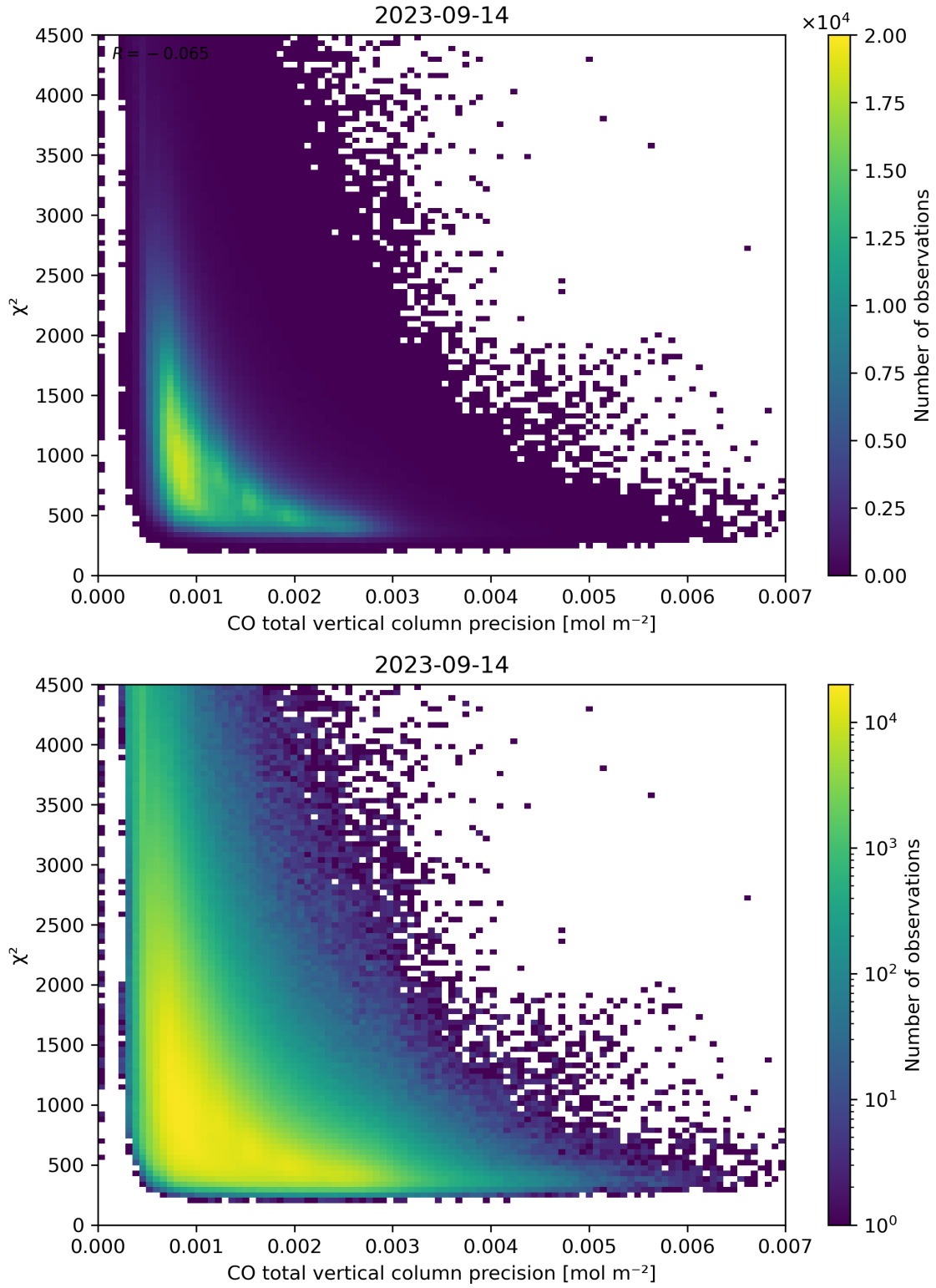
Figure 44: Scatter density plot of “CO total vertical column precision” against “ \chi^2 ” for 2023-09-13 to 2023-09-15.
