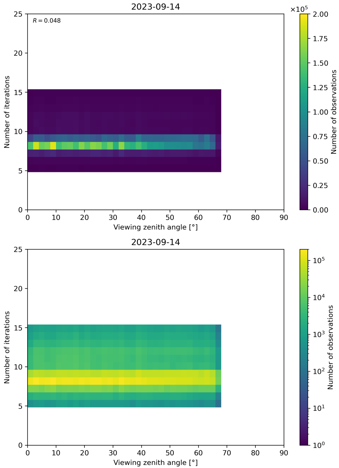
Figure 75: Scatter density plot of “Viewing zenith angle” against “Number of iterations” for 2023-09-13 to 2023-09-15.
