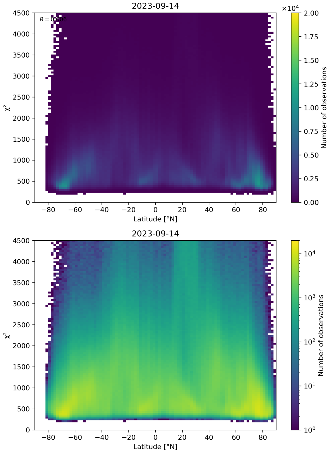
Figure 54: Scatter density plot of “Latitude” against “ \chi^2 ” for 2023-09-13 to 2023-09-15.
