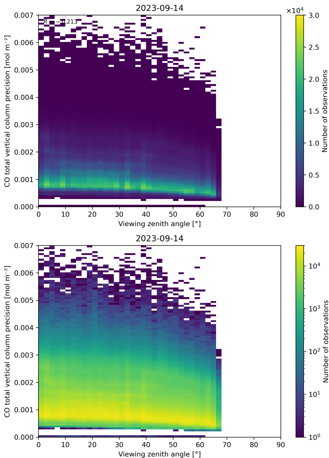
Figure 71: Scatter density plot of “Viewing zenith angle” against “CO total vertical column precision” for 2023-09-13 to 2023-09-15.
