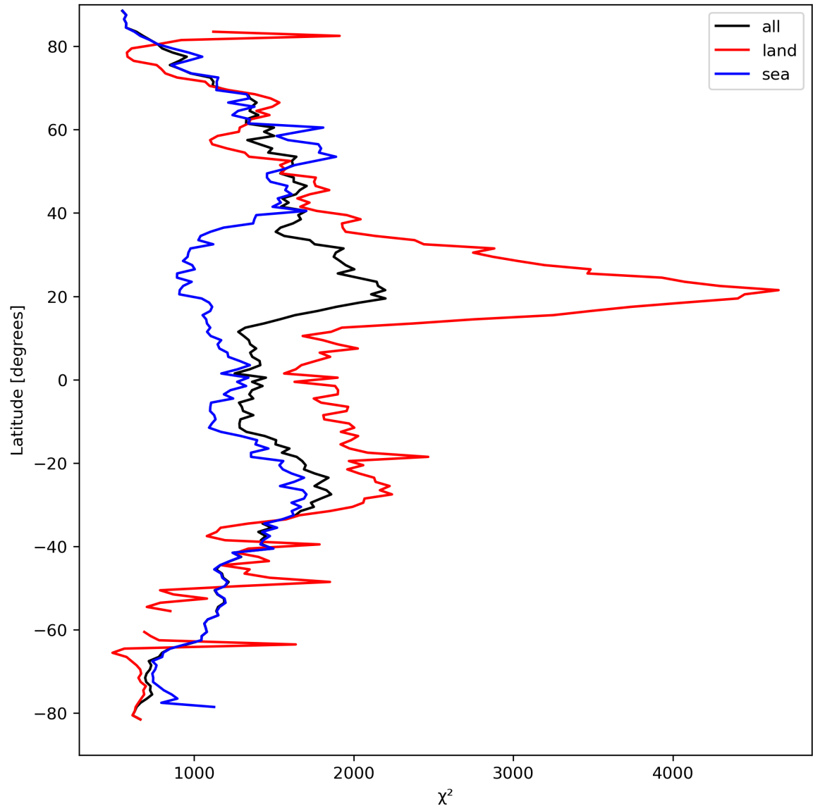
Figure 14: Zonal average of “ \chi^2 ” for 2023-09-13 to 2023-09-15.
