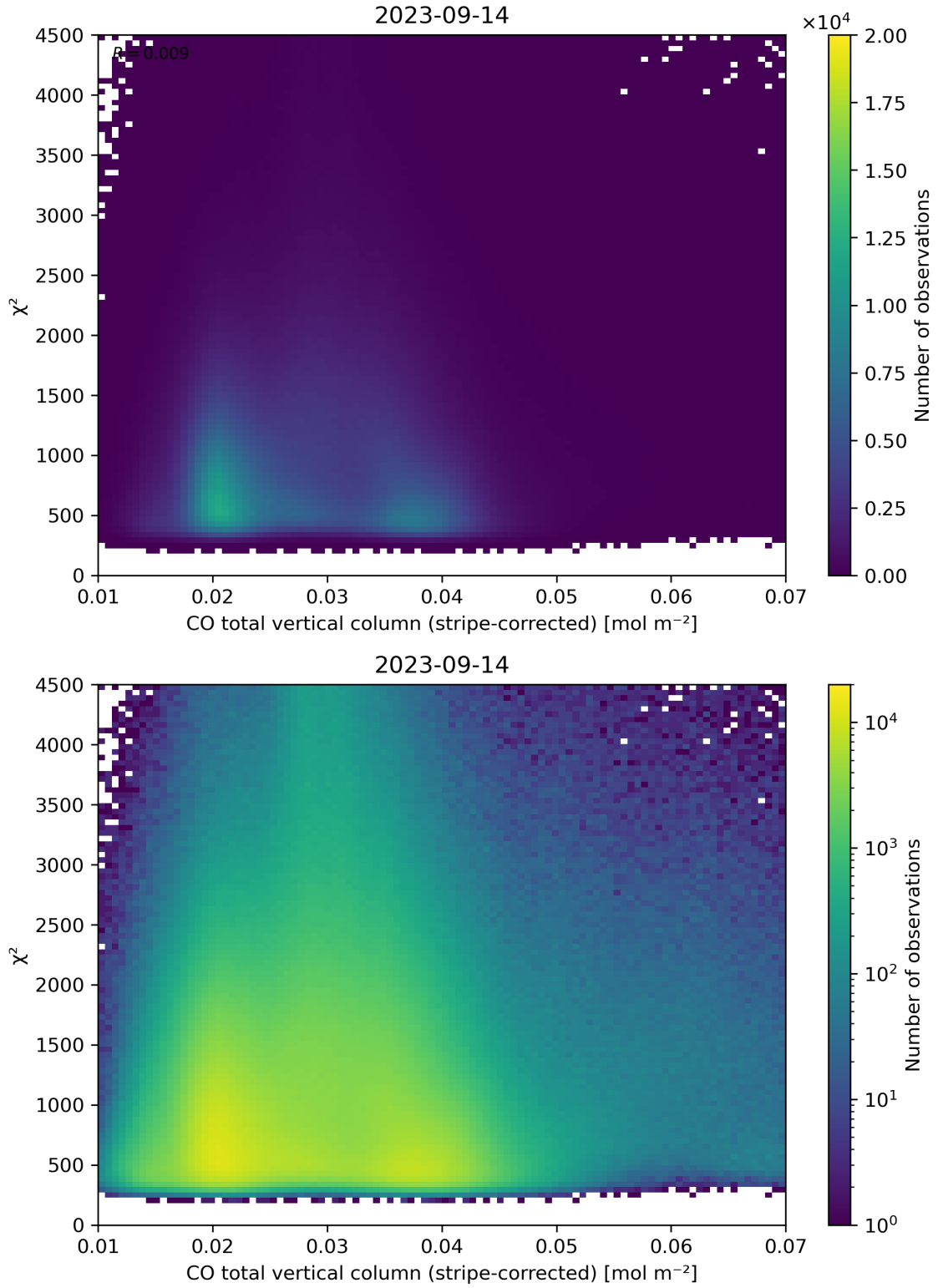
Figure 37: Scatter density plot of “CO total vertical column (stripe-corrected)” against “ \chi^2 ” for 2023-09-13 to 2023-09-15.
