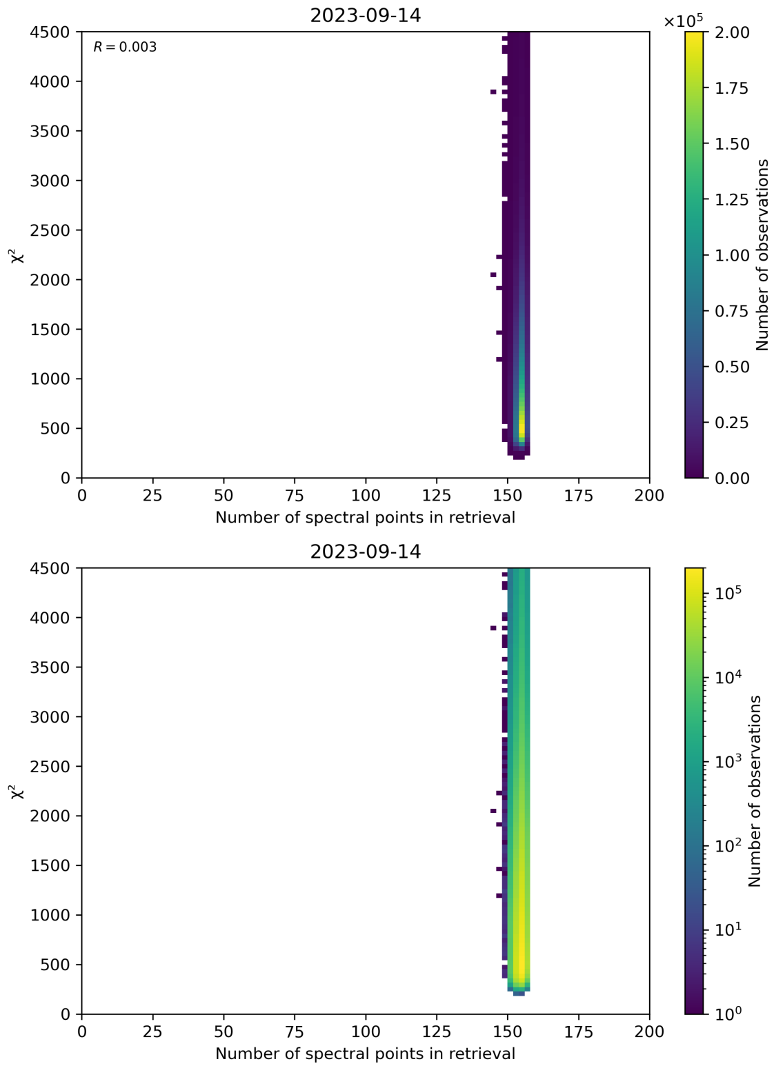
Figure 58: Scatter density plot of “Number of spectral points in retrieval” against “ \chi^2 ” for 2023-09-13 to 2023-09-15.
