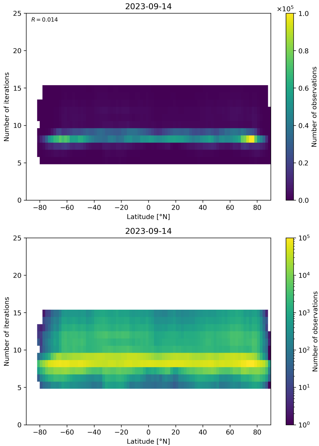
Figure 56: Scatter density plot of “Latitude” against “Number of iterations” for 2023-09-13 to 2023-09-15.
