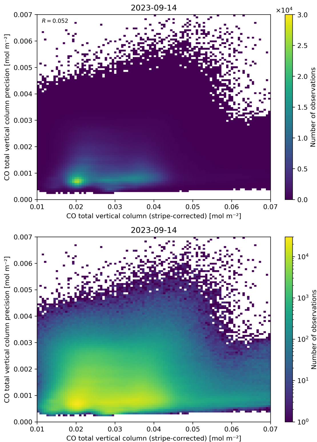
Figure 36: Scatter density plot of “CO total vertical column (stripe-corrected)” against “CO total vertical column precision” for 2023-09-13 to 2023-09-15.
