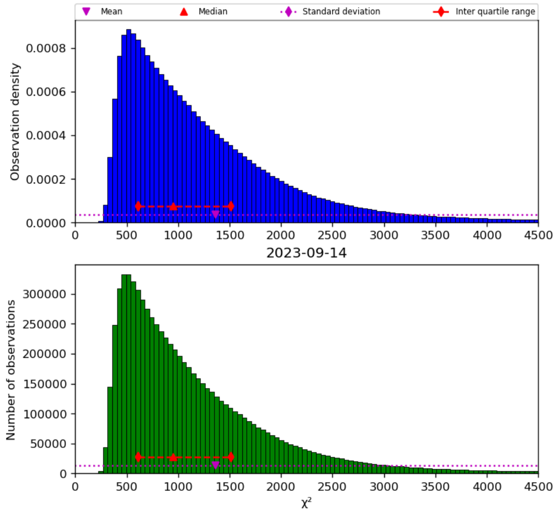
Figure 22: Histogram of " \chi^2 " for 2023-09-13 to 2023-09-15
