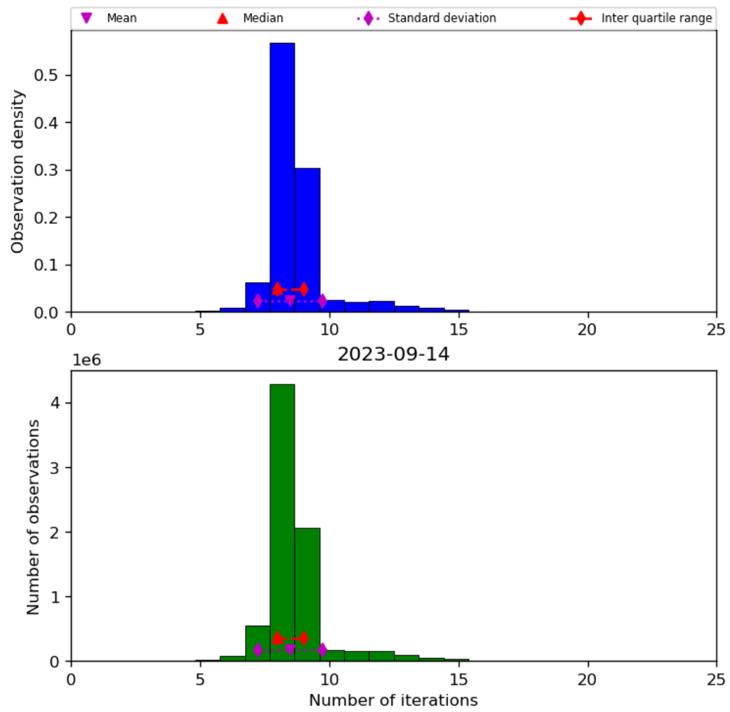
Figure 24: Histogram of “Number of iterations” for 2023-09-13 to 2023-09-15
