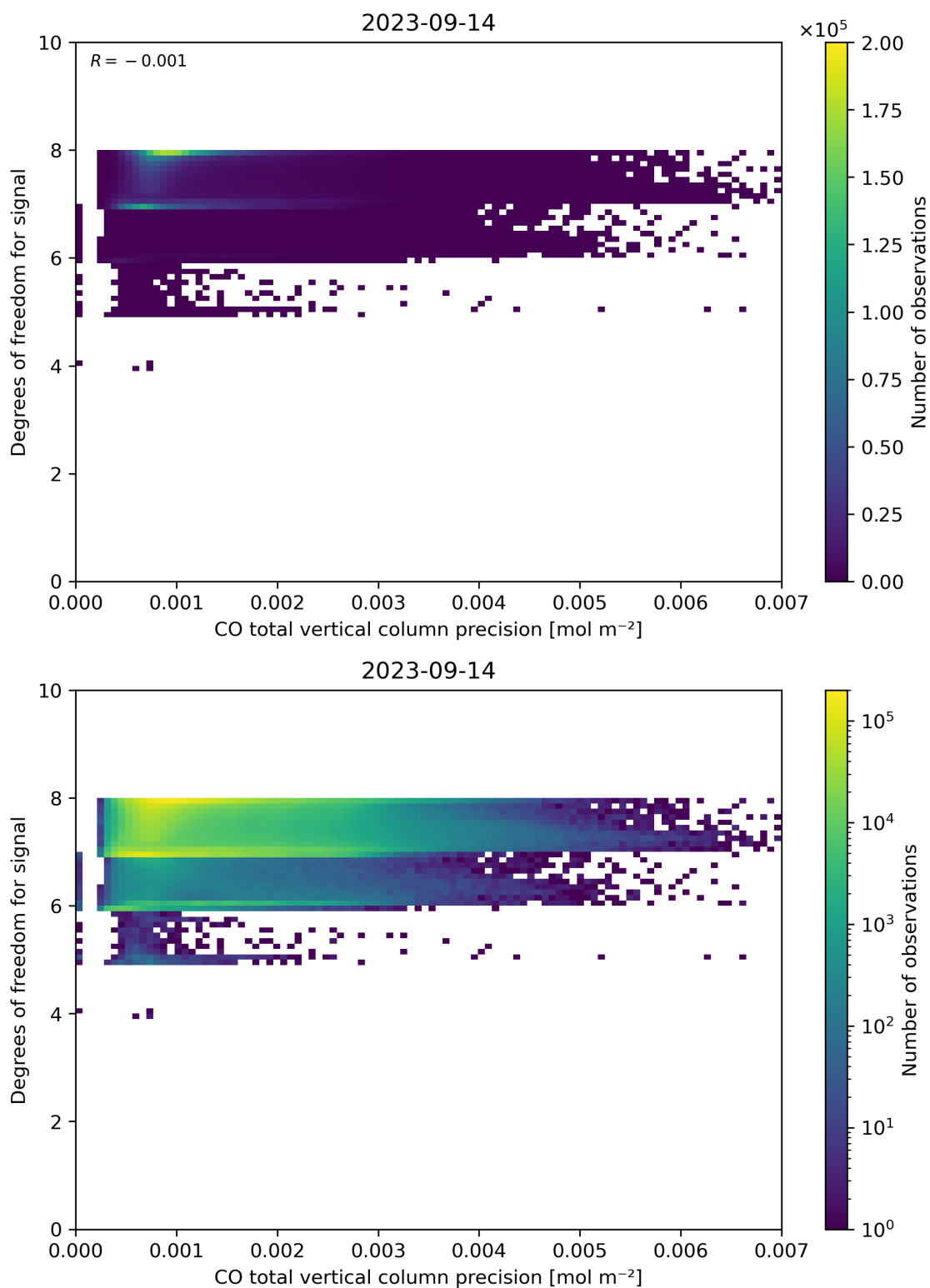
Figure 45: Scatter density plot of “CO total vertical column precision” against “Degrees of freedom for signal” for 2023-09-13 to 2023-09-15.
