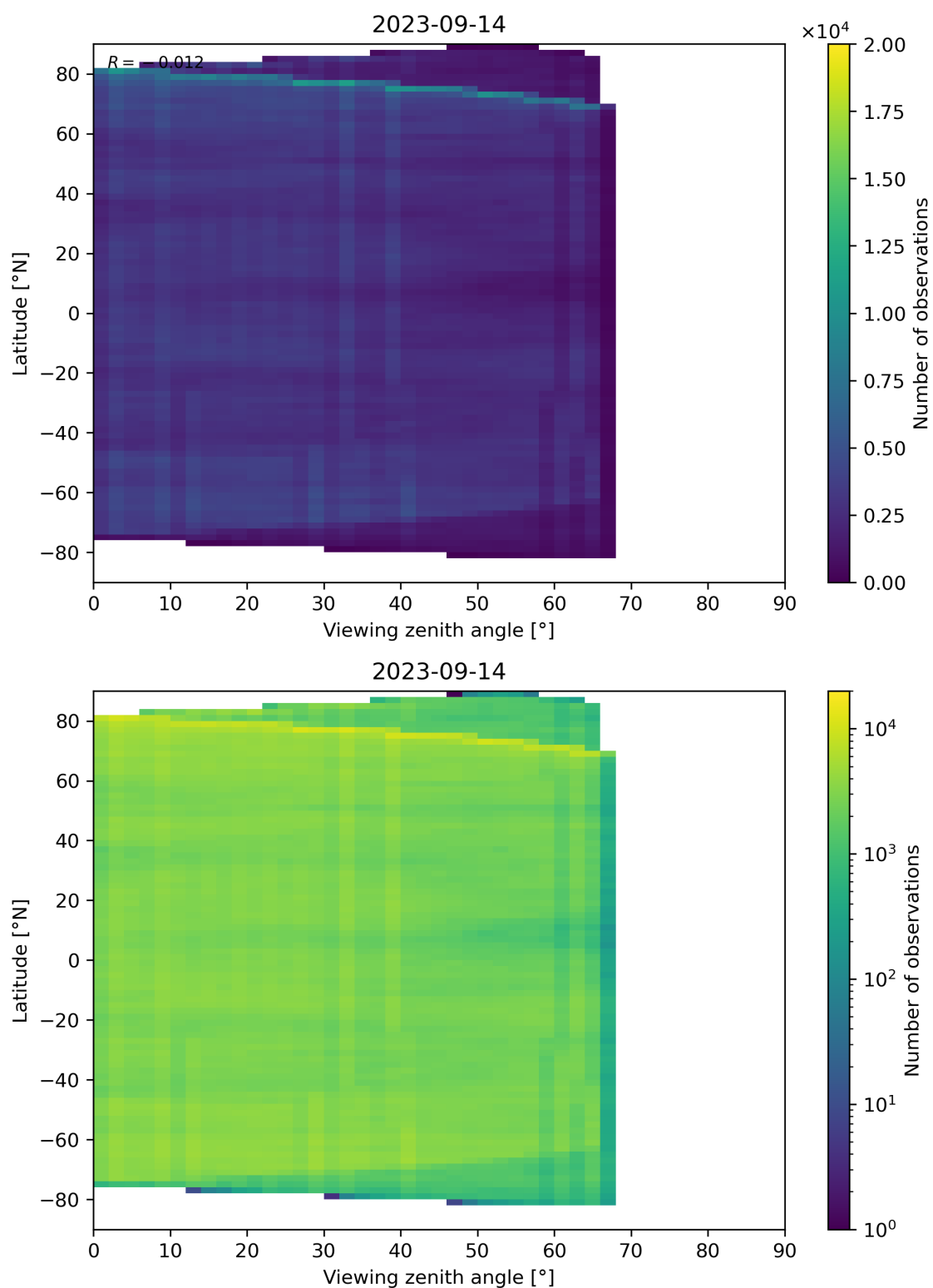
Figure 74: Scatter density plot of “Viewing zenith angle” against “Latitude” for 2023-09-13 to 2023-09-15.
