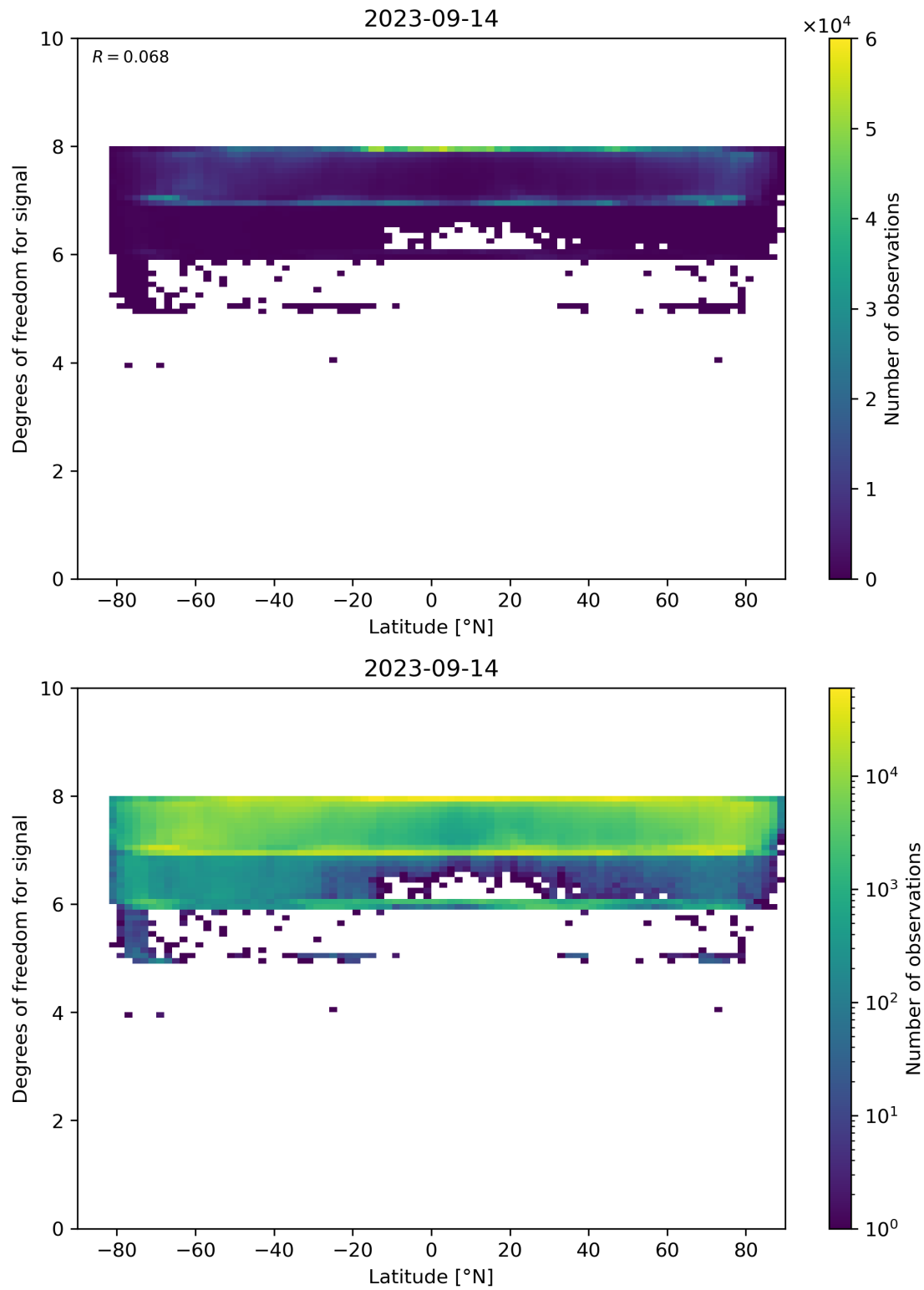
Figure 55: Scatter density plot of “Latitude” against “Degrees of freedom for signal” for 2023-09-13 to 2023-09-15.
