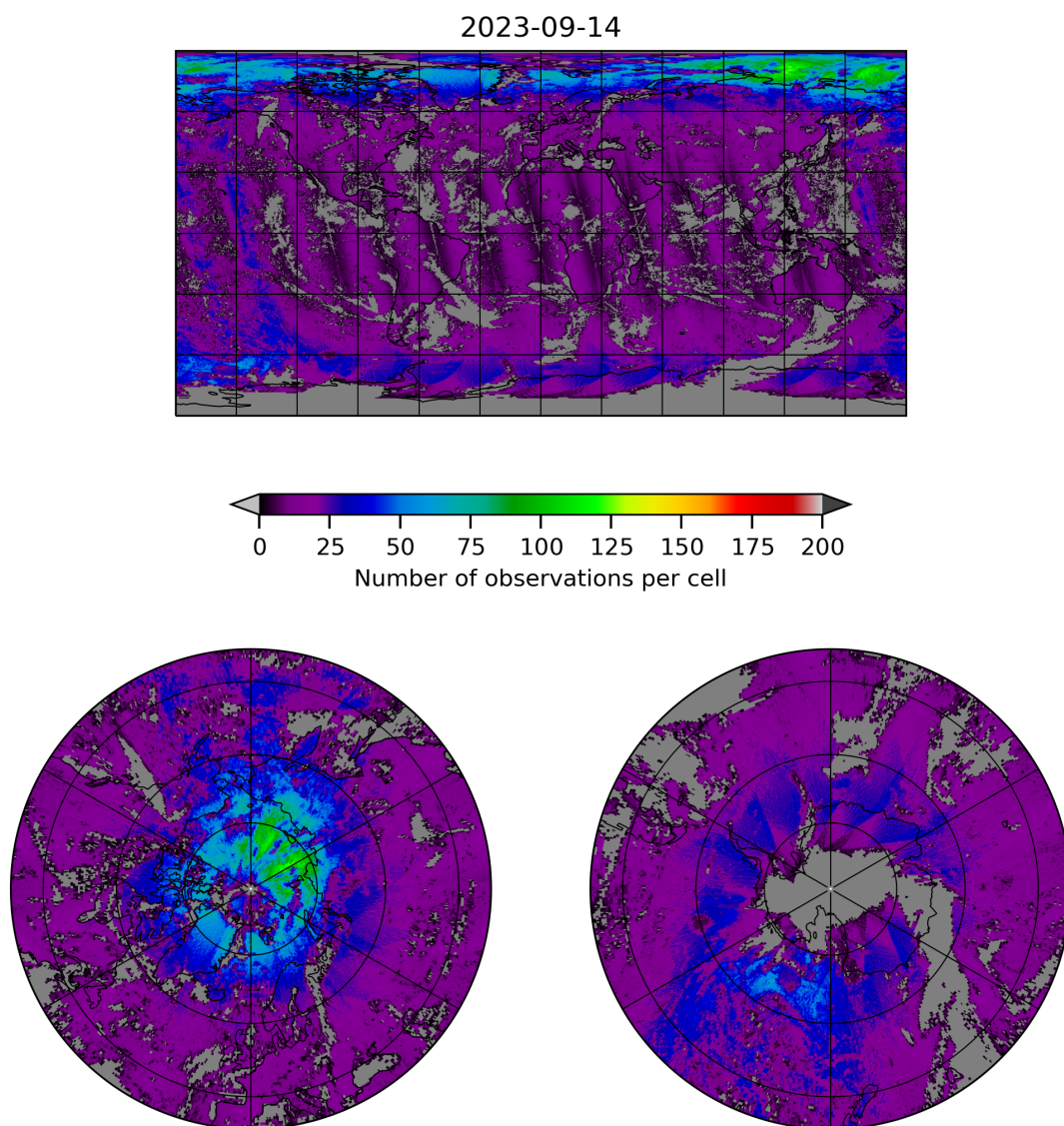
Figure 8: Map of the number of observations for 2023-09-13 to 2023-09-15
