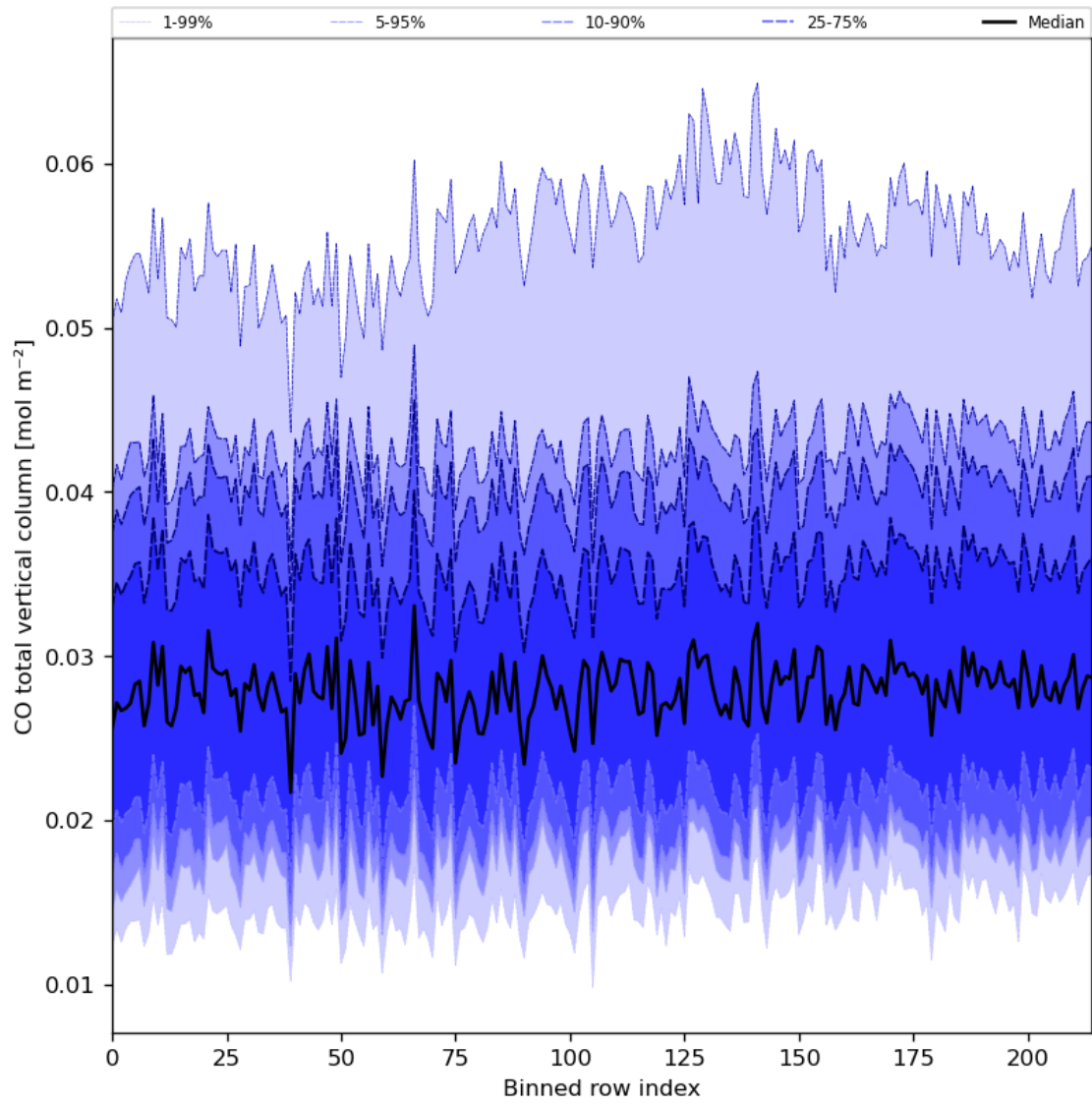
Figure 26: Along track statistics of “CO total vertical column” for 2023-09-13 to 2023-09-15
