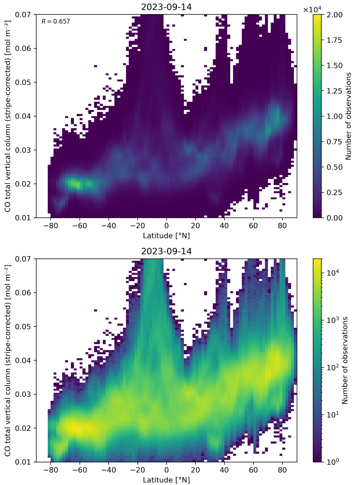
Figure 52: Scatter density plot of “Latitude” against “CO total vertical column (stripe-corrected)” for 2023-09-13 to 2023-09-15.
