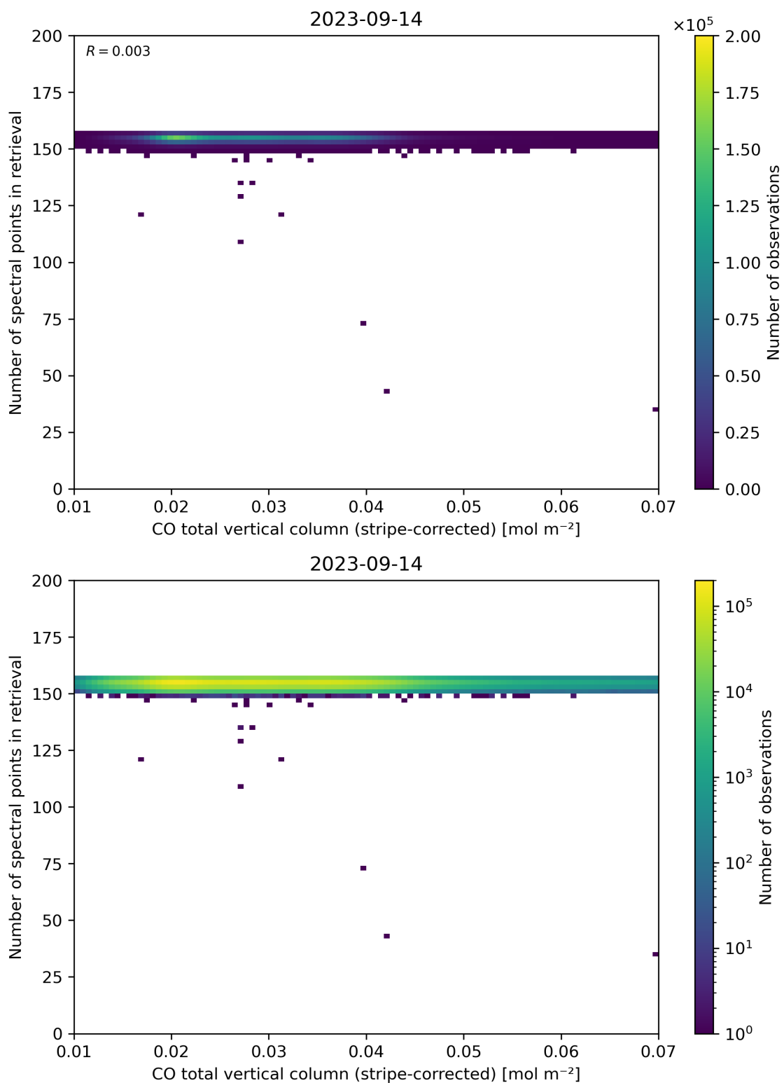
Figure 40: Scatter density plot of “CO total vertical column (stripe-corrected)” against “Number of spectral points in retrieval” for 2023-09-13 to 2023-09-15.
