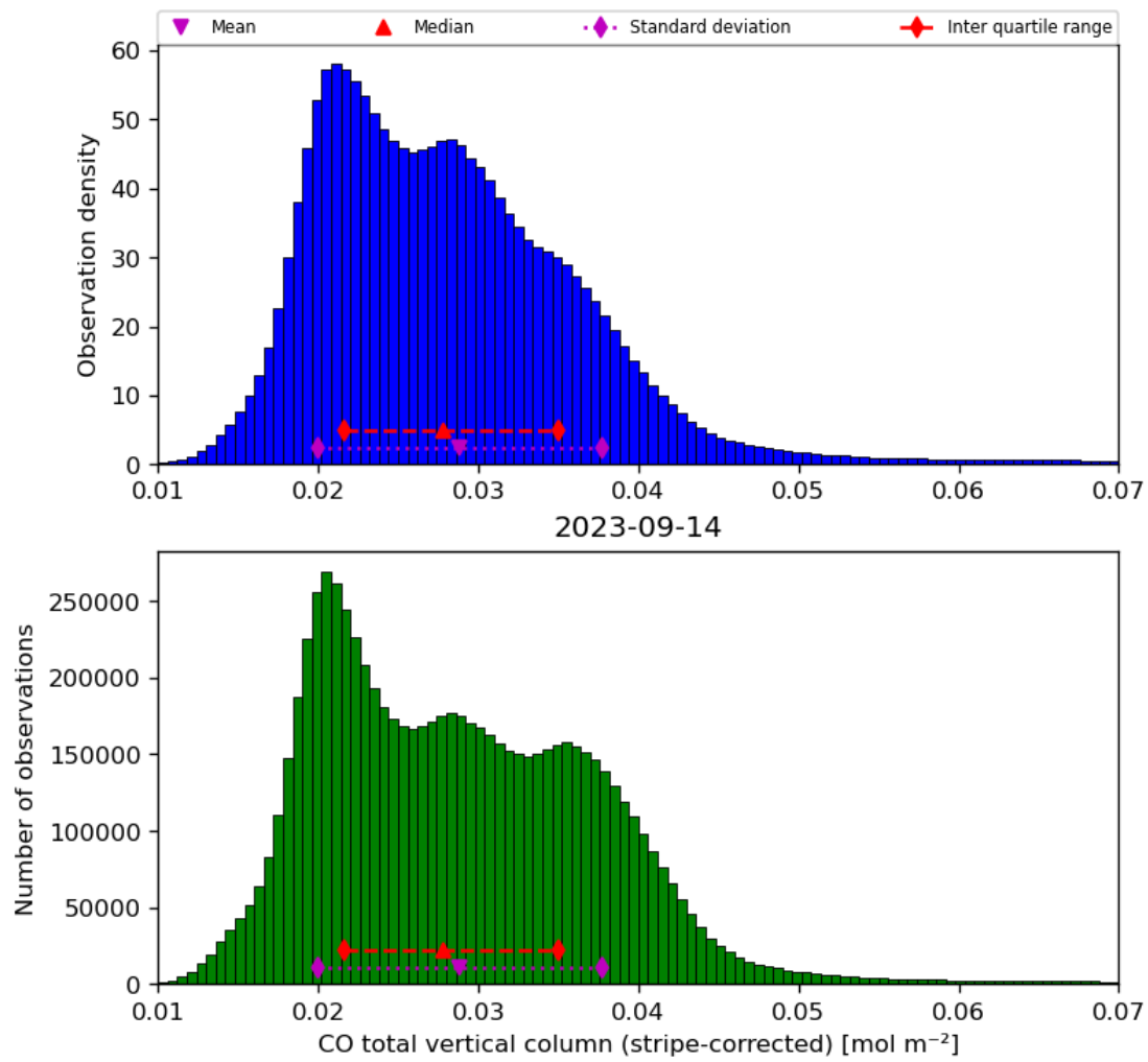
Figure 19: Histogram of “CO total vertical column (stripe-corrected)” for 2023-09-13 to 2023-09-15
