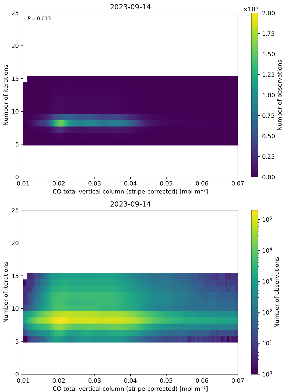
Figure 39: Scatter density plot of “CO total vertical column (stripe-corrected)” against “Number of iterations” for 2023-09-13 to 2023-09-15.
