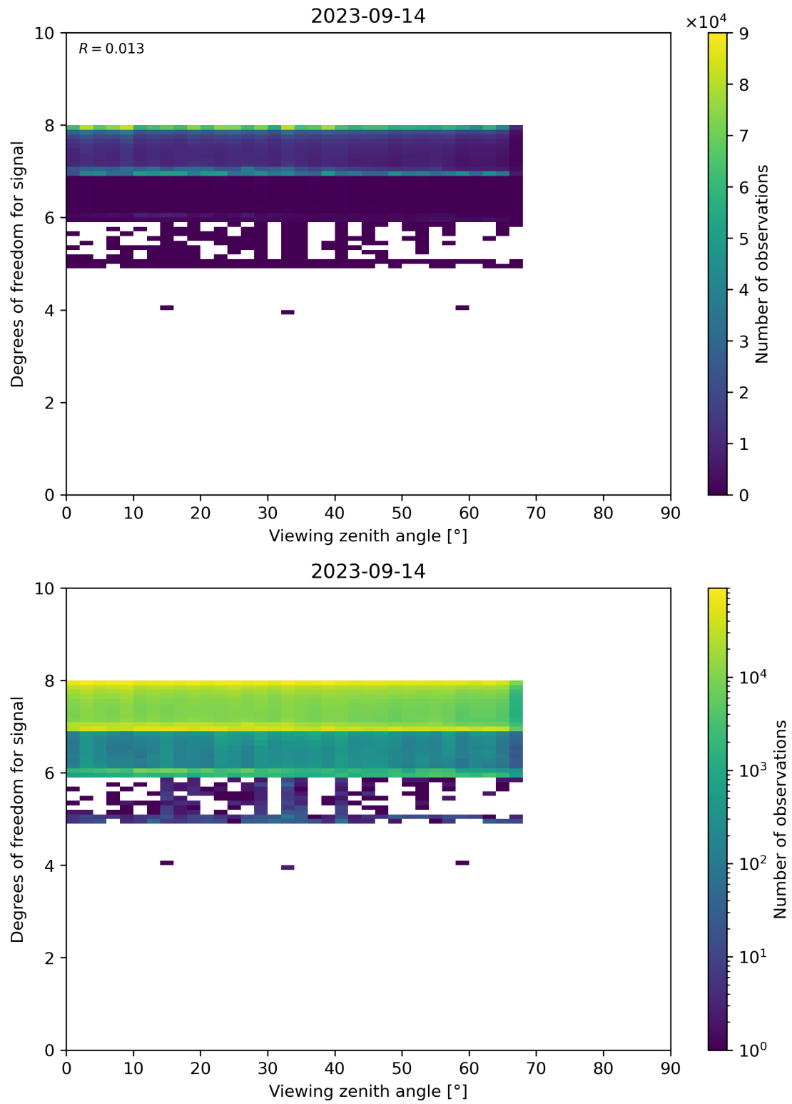
Figure 73: Scatter density plot of “Viewing zenith angle” against “Degrees of freedom for signal” for 2023-09-13 to 2023-09-15.
