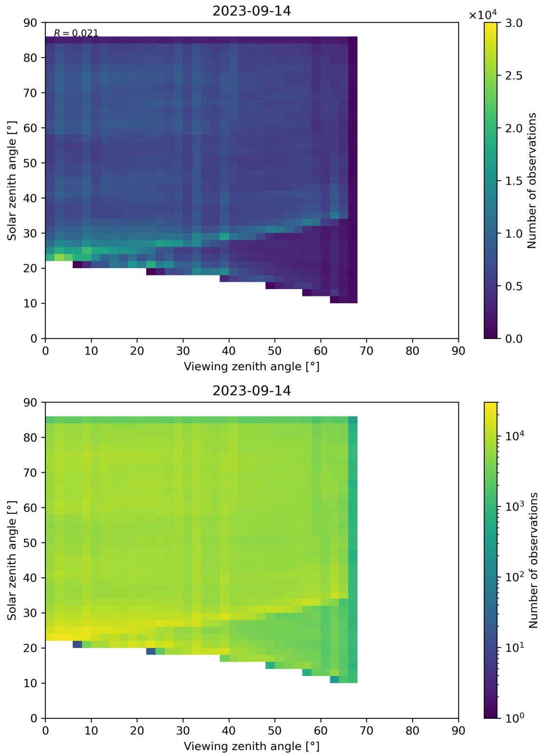
Figure 77: Scatter density plot of “Viewing zenith angle” against “Solar zenith angle” for 2023-09-13 to 2023-09-15.
