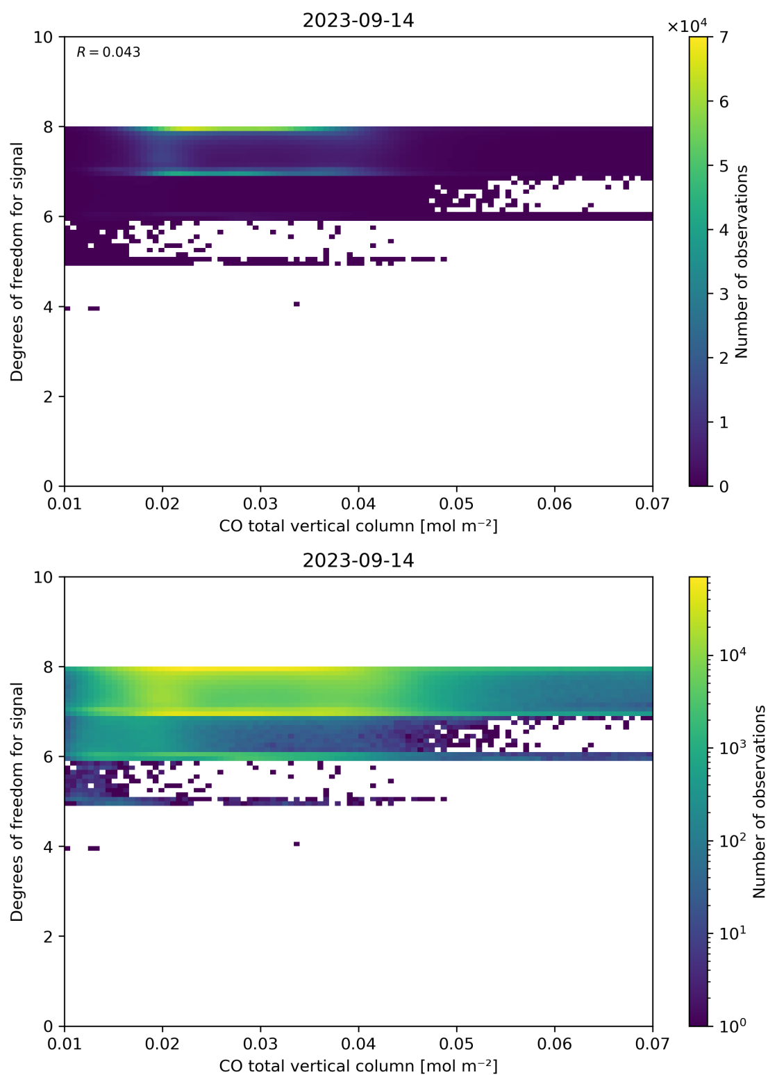
Figure 41: Scatter density plot of “CO total vertical column” against “Degrees of freedom for signal” for 2023-09-13 to 2023-09-15.
