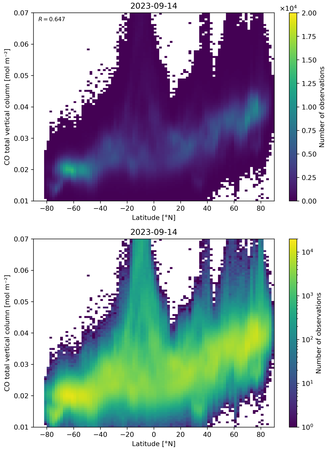
Figure 51: Scatter density plot of “Latitude” against “CO total vertical column” for 2023-09-13 to 2023-09-15.
