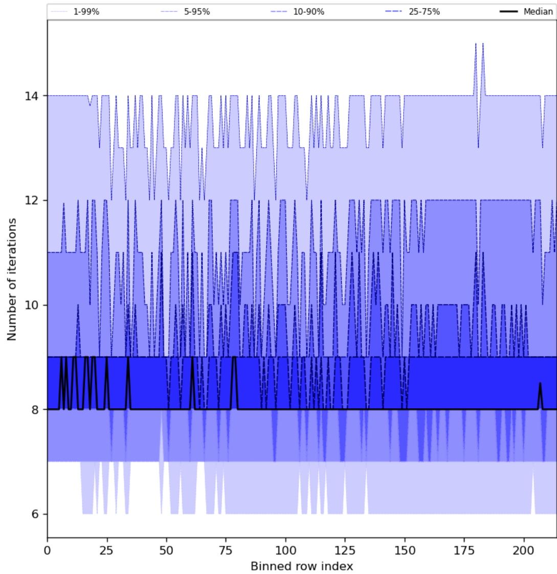
Figure 32: Along track statistics of “Number of iterations” for 2023-09-13 to 2023-09-15
