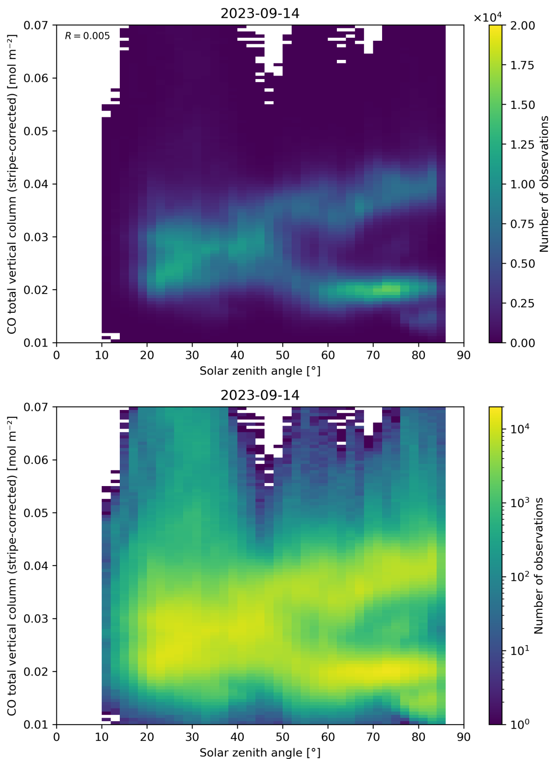
Figure 62: Scatter density plot of “Solar zenith angle” against “CO total vertical column (stripe-corrected)” for 2023-09-13 to 2023-09-15.
