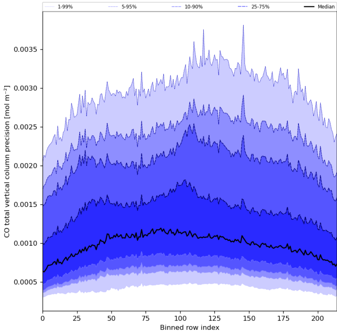
Figure 28: Along track statistics of “CO total vertical column precision” for 2023-09-13 to 2023-09-15
