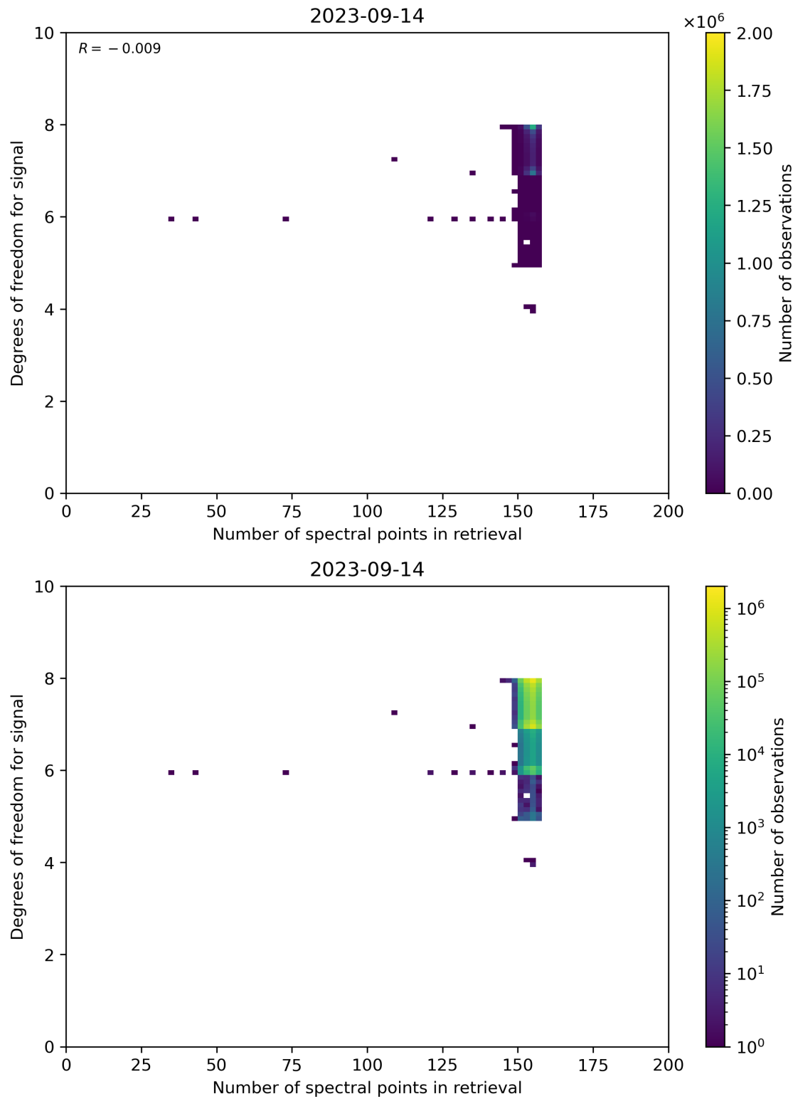
Figure 59: Scatter density plot of “Number of spectral points in retrieval” against “Degrees of freedom for signal” for 2023-09-13 to 2023-09-15.
