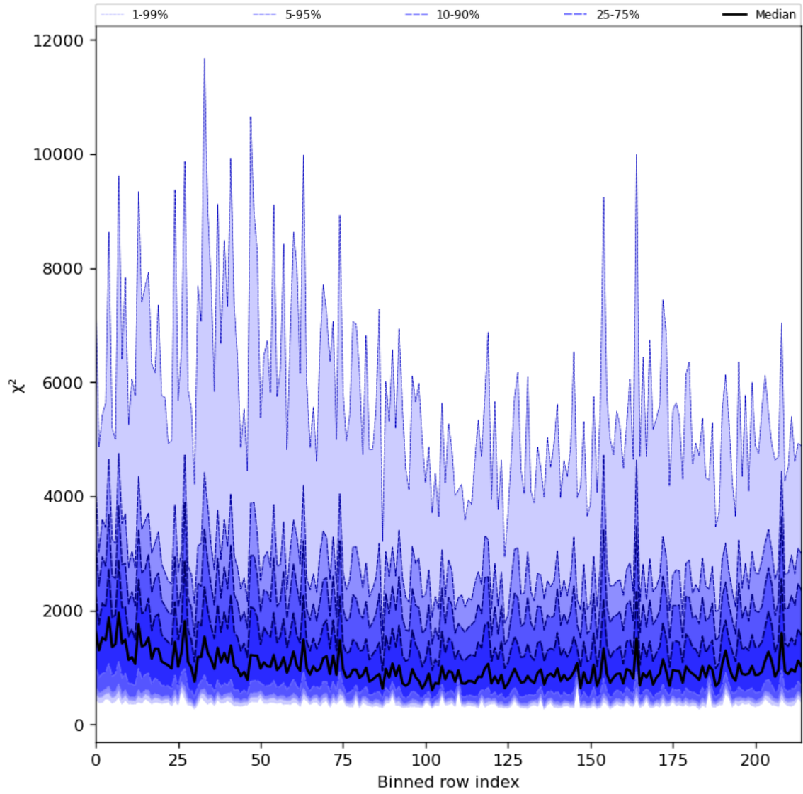
Figure 30: Along track statistics of “ \chi^2 ” for 2023-09-13 to 2023-09-15
