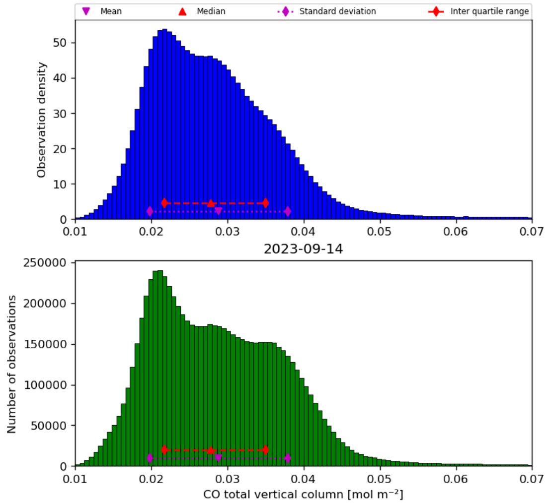
Figure 18: Histogram of “CO total vertical column” for 2023-09-13 to 2023-09-15
