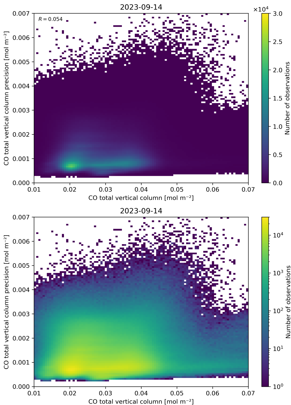
Figure 34: Scatter density plot of “CO total vertical column” against “CO total vertical column precision” for 2023-09-13 to 2023-09-15.
