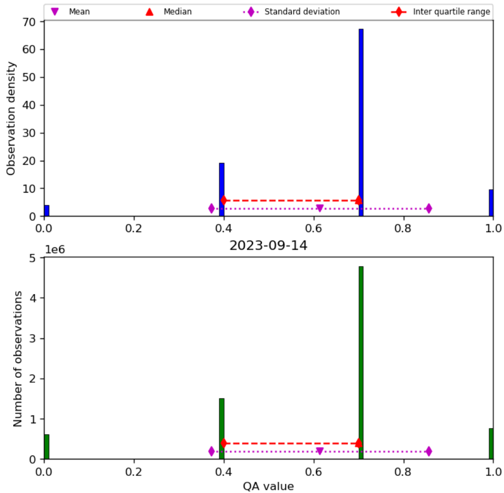
Figure 17: Histogram of “QA value” for 2023-09-13 to 2023-09-15
