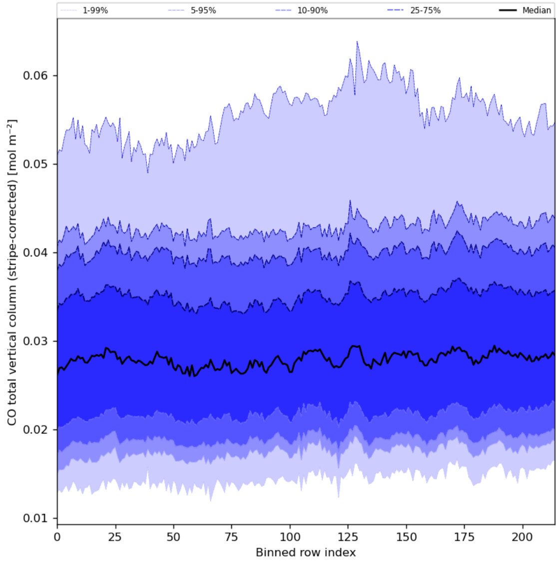
Figure 27: Along track statistics of “CO total vertical column (stripe-corrected)” for 2023-09-13 to 2023-09-15
