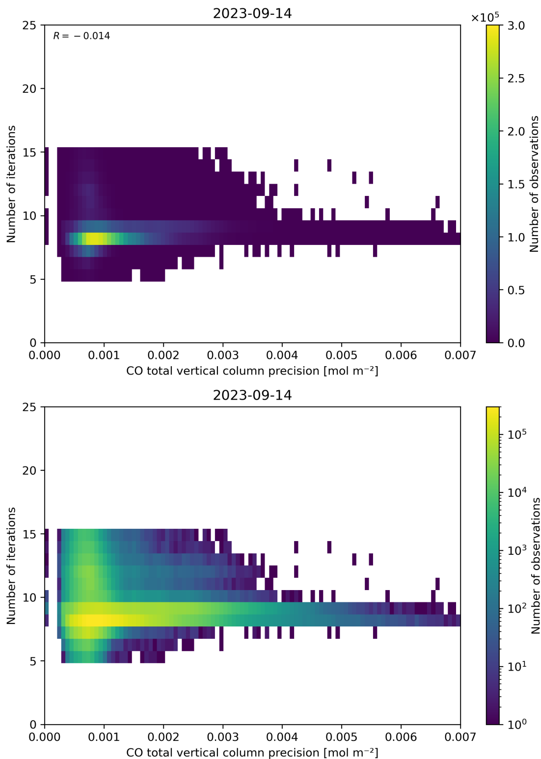
Figure 46: Scatter density plot of “CO total vertical column precision” against “Number of iterations” for 2023-09-13 to 2023-09-15.
