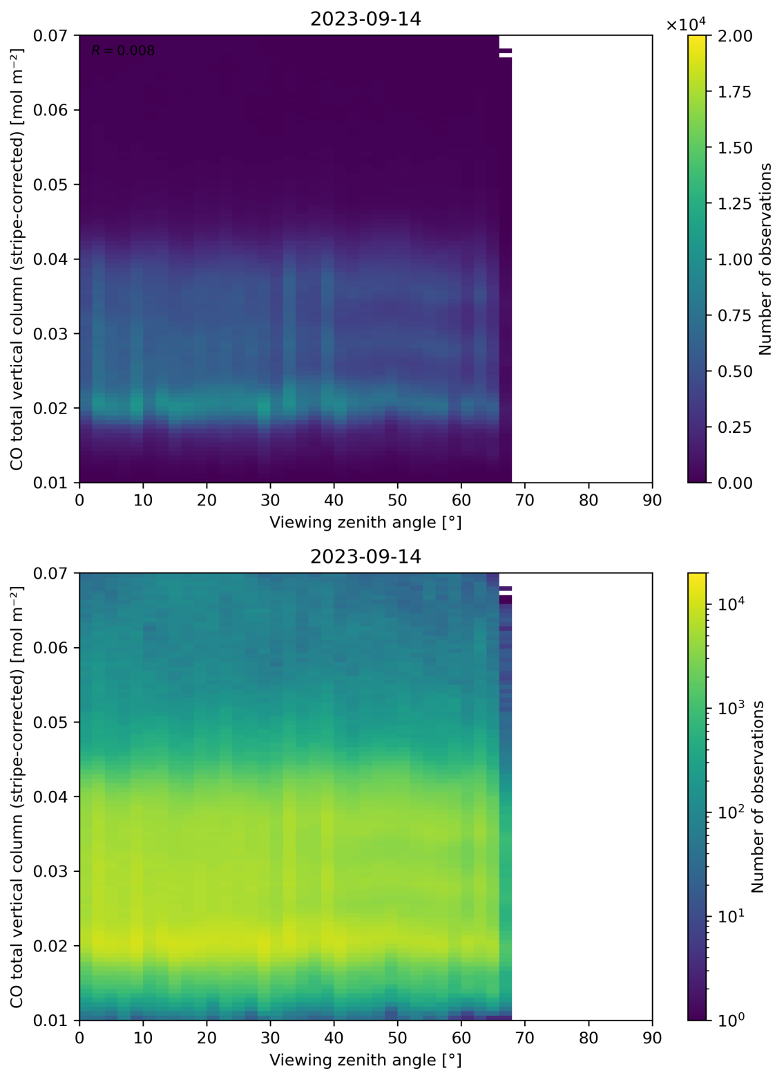
Figure 70: Scatter density plot of “Viewing zenith angle” against “CO total vertical column (stripe-corrected)” for 2023-09-13 to 2023-09-15.
