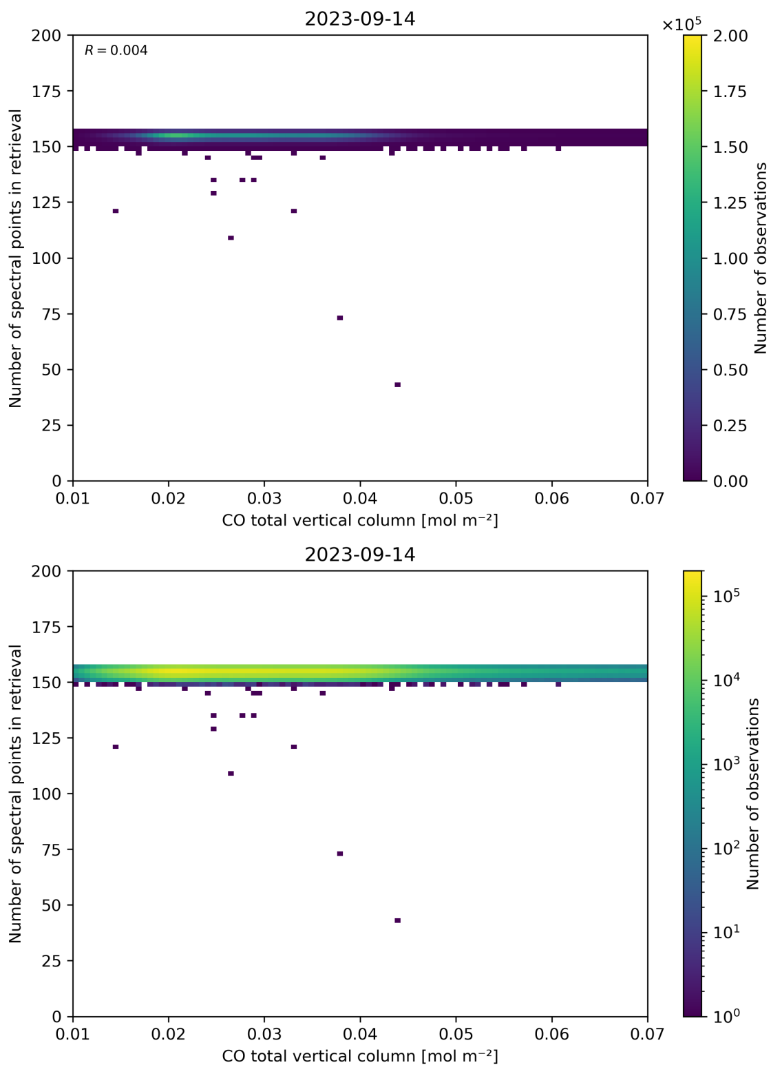
Figure 43: Scatter density plot of “CO total vertical column” against “Number of spectral points in retrieval” for 2023-09-13 to 2023-09-15.
