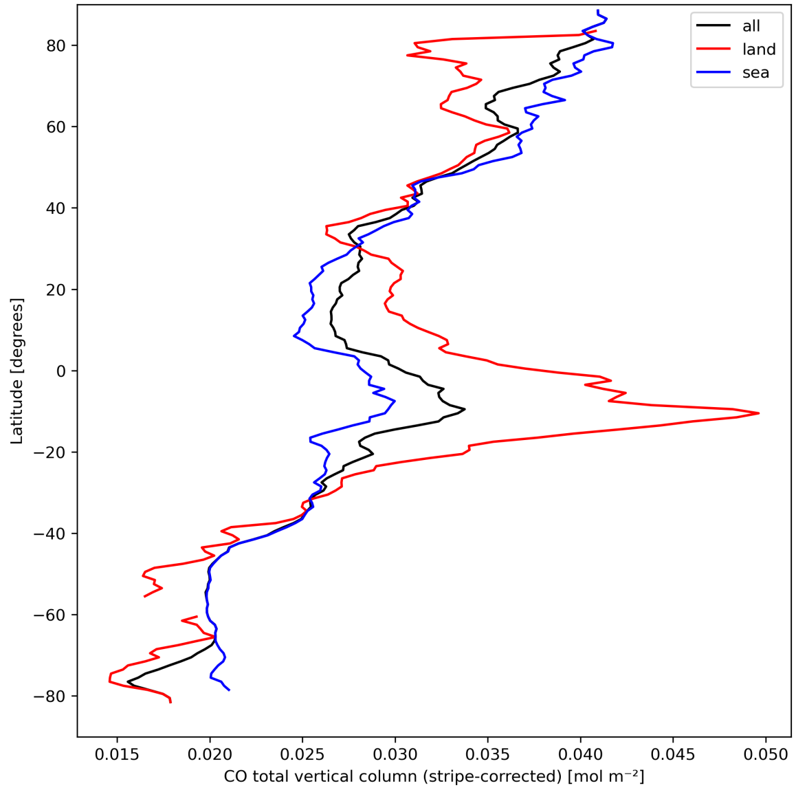
Figure 11: Zonal average of “CO total vertical column (stripe-corrected)” for 2023-09-13 to 2023-09-15.
