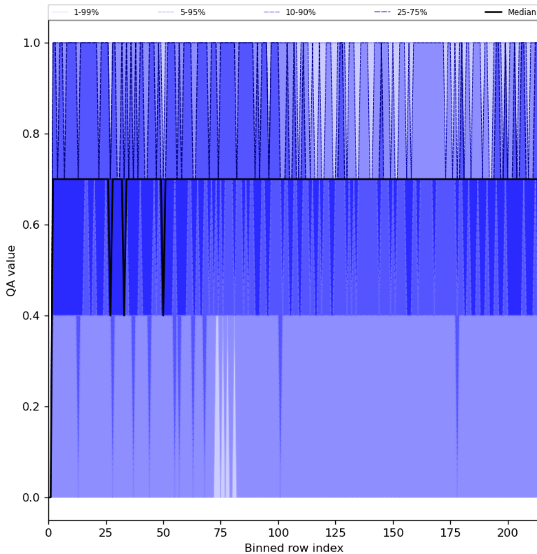
Figure 25: Along track statistics of “QA value” for 2023-09-13 to 2023-09-15
