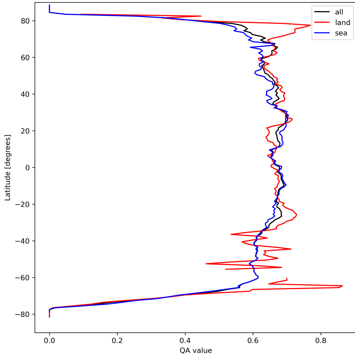
Figure 9: Zonal average of “QA value” for 2023-09-13 to 2023-09-15.
