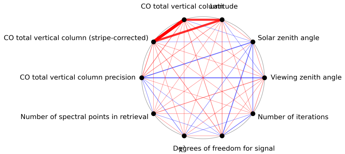
Figure 1: Map of correlation graph for 2023-09-15 to 2023-09-16.
