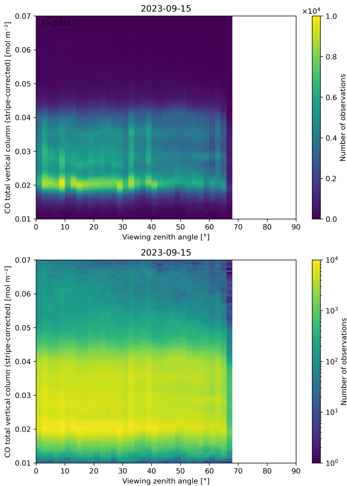
Figure 70: Scatter density plot of “Viewing zenith angle” against “CO total vertical column (stripe-corrected)” for 2023-09-15 to 2023-09-16.
