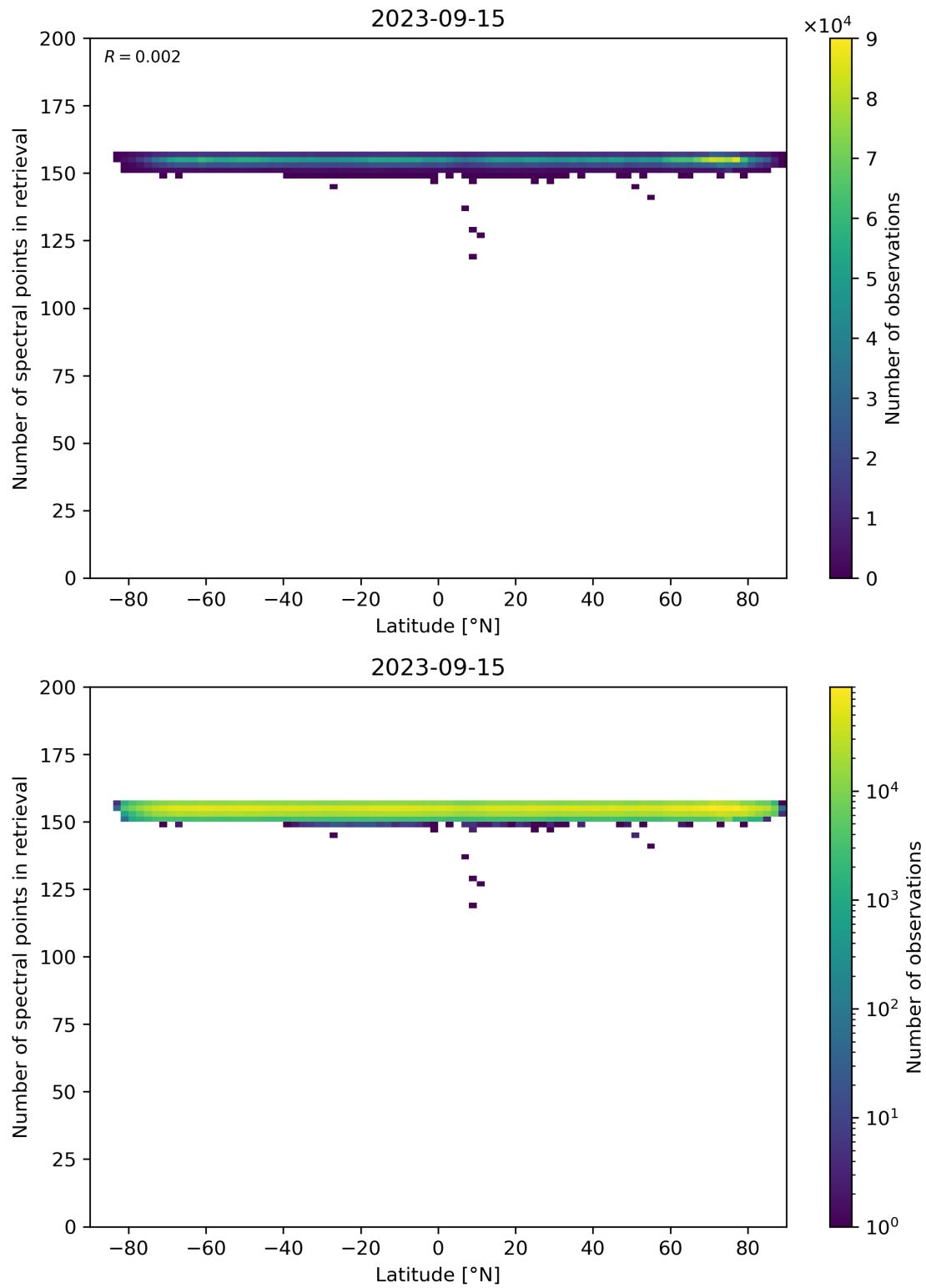
Figure 57: Scatter density plot of “Latitude” against “Number of spectral points in retrieval” for 2023-09-15 to 2023-09-16.
