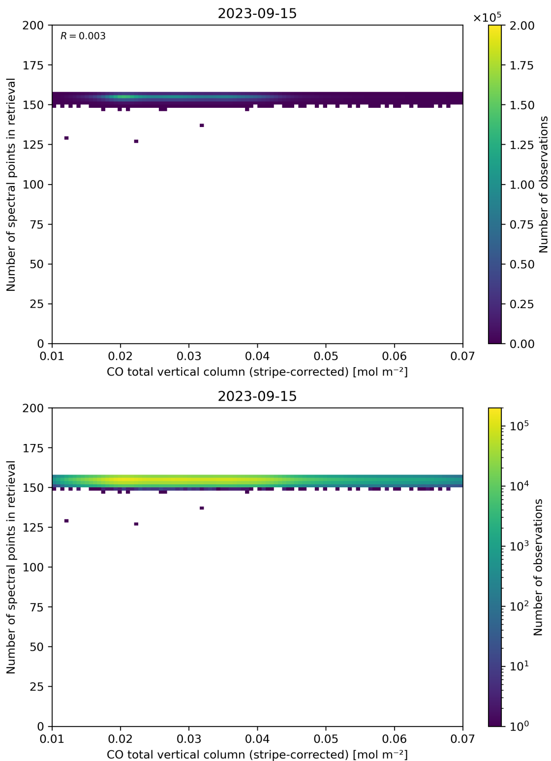
Figure 40: Scatter density plot of “CO total vertical column (stripe-corrected)” against “Number of spectral points in retrieval” for 2023-09-15 to 2023-09-16.
