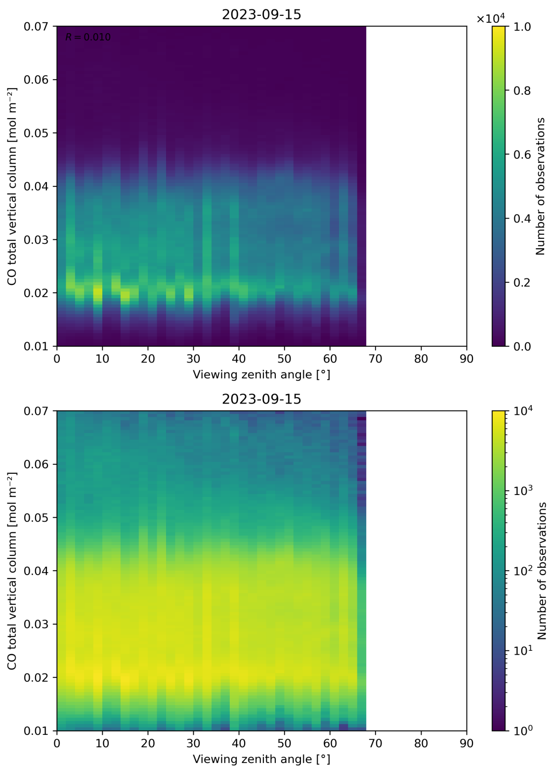
Figure 69: Scatter density plot of “Viewing zenith angle” against “CO total vertical column” for 2023-09-15 to 2023-09-16.
