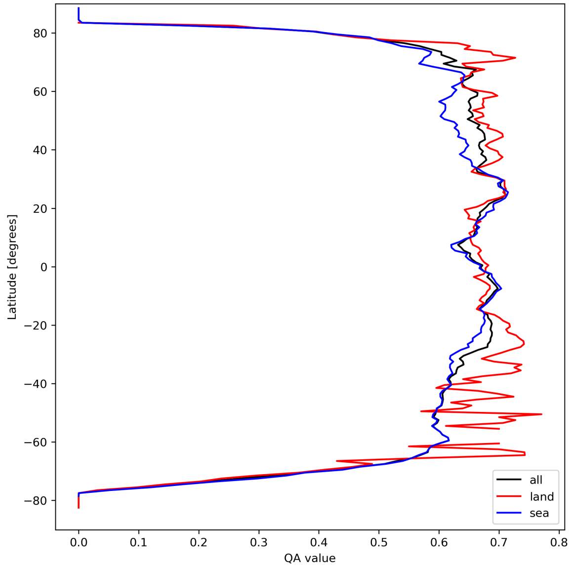
Figure 9: Zonal average of “QA value” for 2023-09-15 to 2023-09-16.
