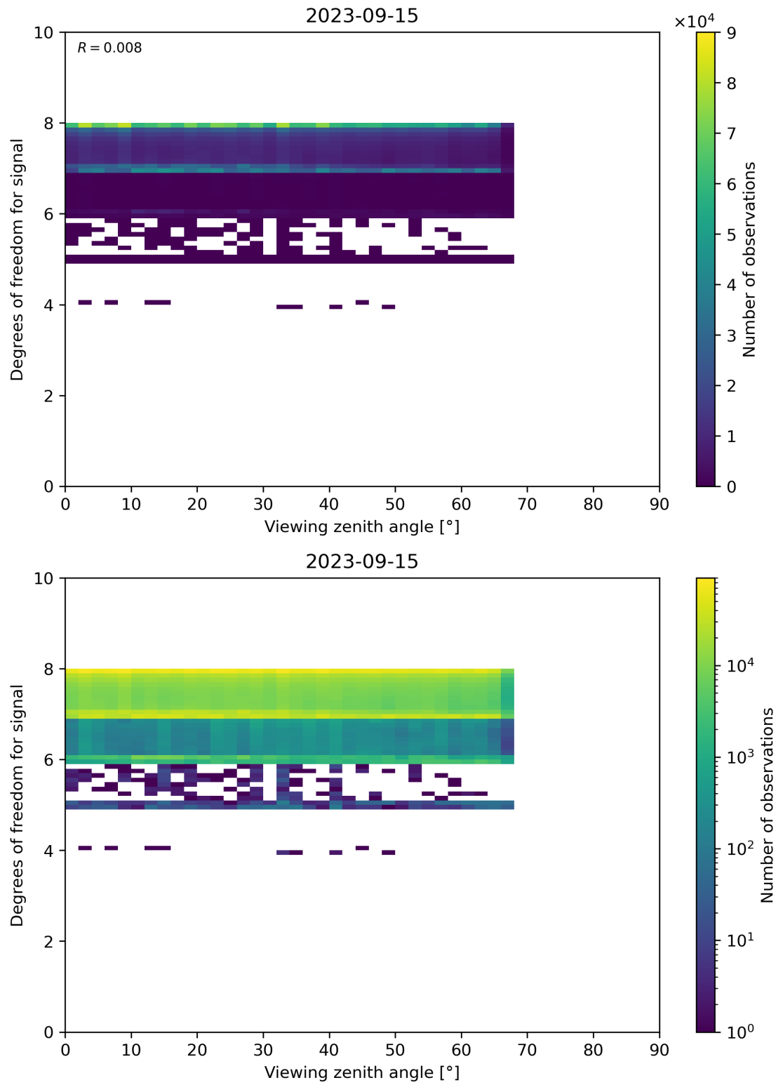
Figure 73: Scatter density plot of “Viewing zenith angle” against “Degrees of freedom for signal” for 2023-09-15 to 2023-09-16.
