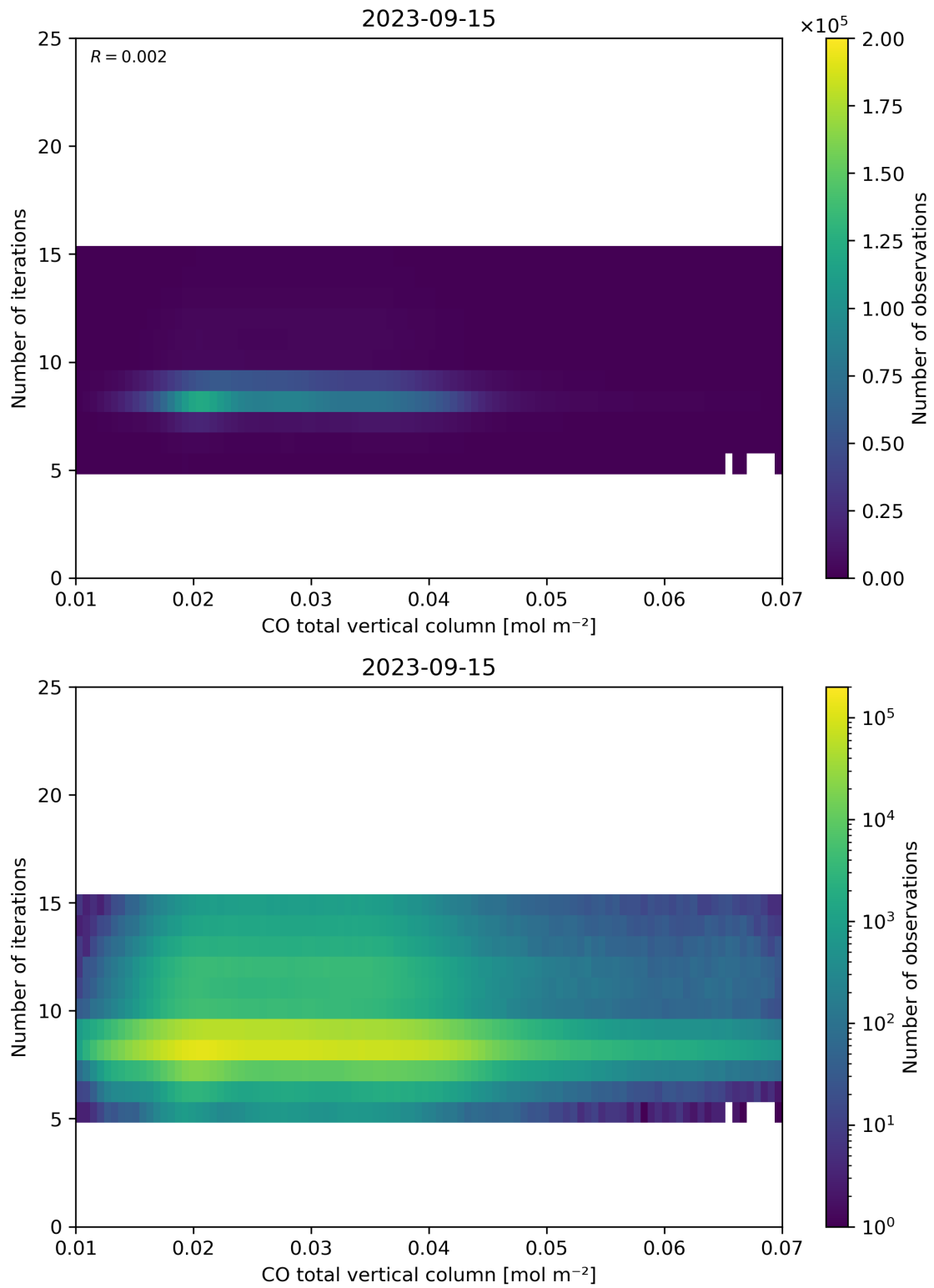
Figure 42: Scatter density plot of “CO total vertical column” against “Number of iterations” for 2023-09-15 to 2023-09-16.
