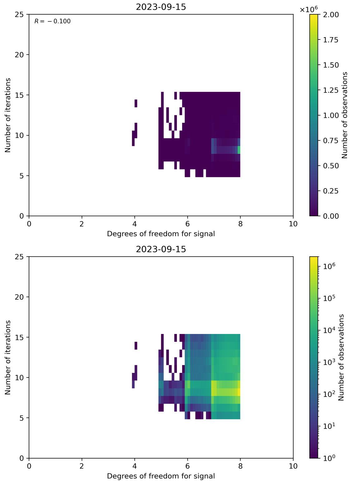
Figure 50: Scatter density plot of “Degrees of freedom for signal” against “Number of iterations” for 2023-09-15 to 2023-09-16.
