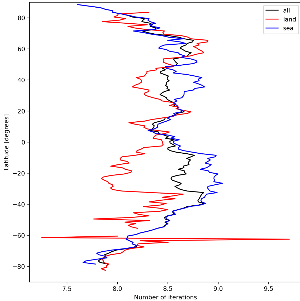
Figure 16: Zonal average of “Number of iterations” for 2023-09-15 to 2023-09-16.
