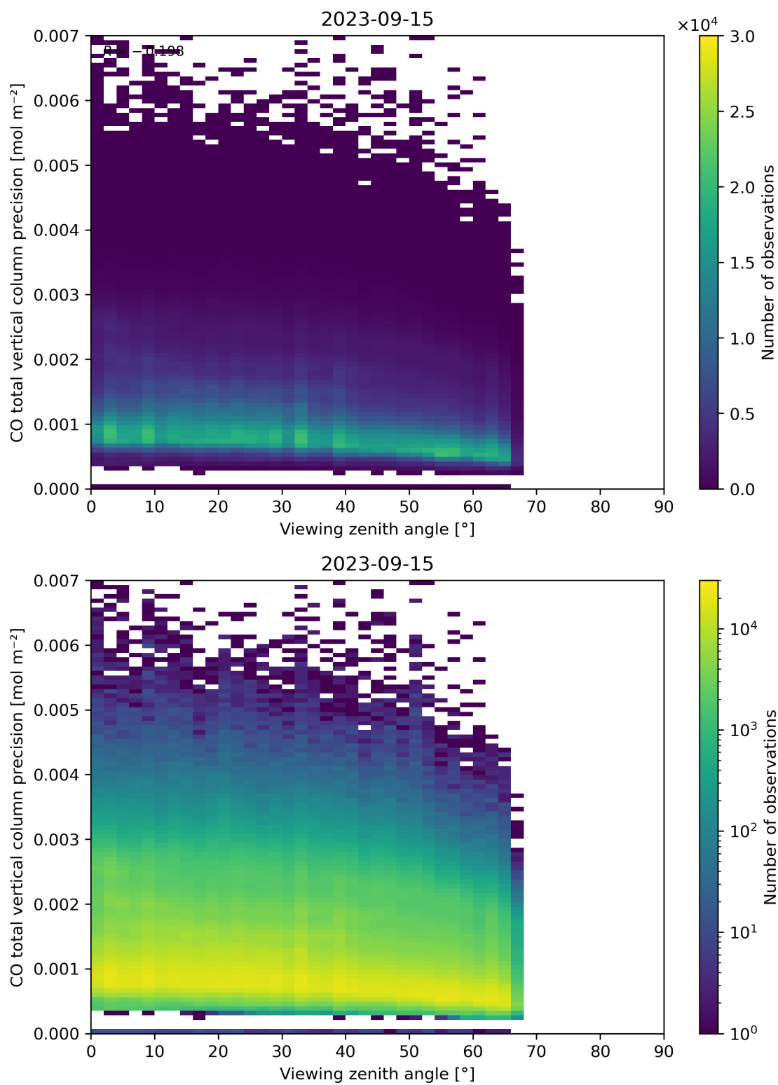
Figure 71: Scatter density plot of “Viewing zenith angle” against “CO total vertical column precision” for 2023-09-15 to 2023-09-16.
