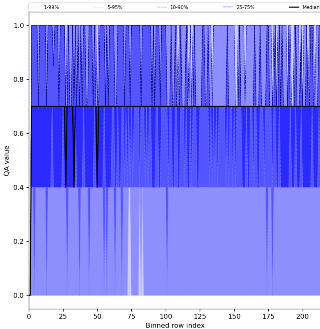
Figure 25: Along track statistics of “QA value” for 2023-09-15 to 2023-09-16
