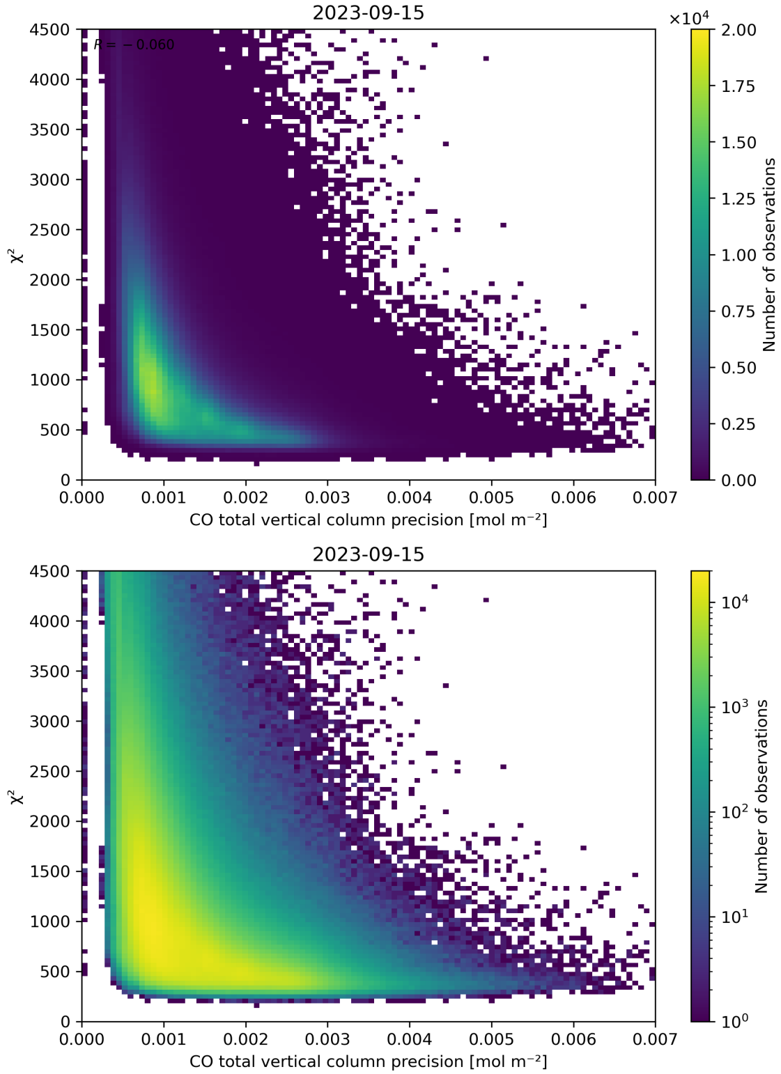
Figure 44: Scatter density plot of “CO total vertical column precision” against “ \chi^2 ” for 2023-09-15 to 2023-09-16.
