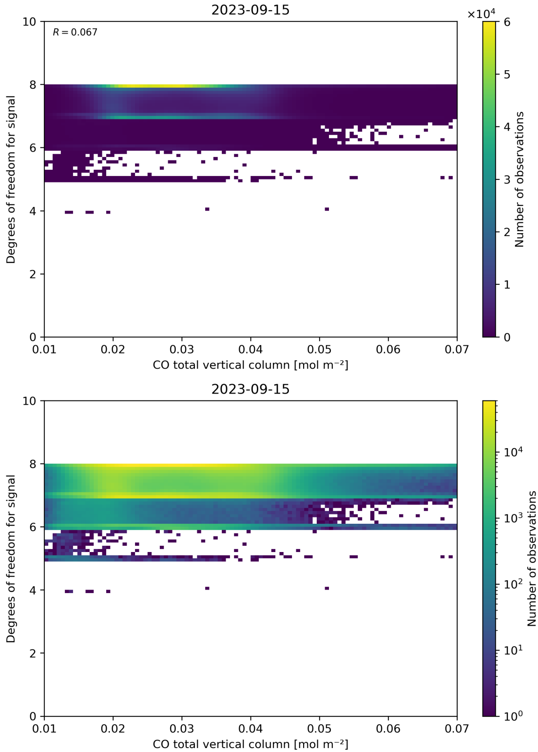
Figure 41: Scatter density plot of “CO total vertical column” against “Degrees of freedom for signal” for 2023-09-15 to 2023-09-16.
