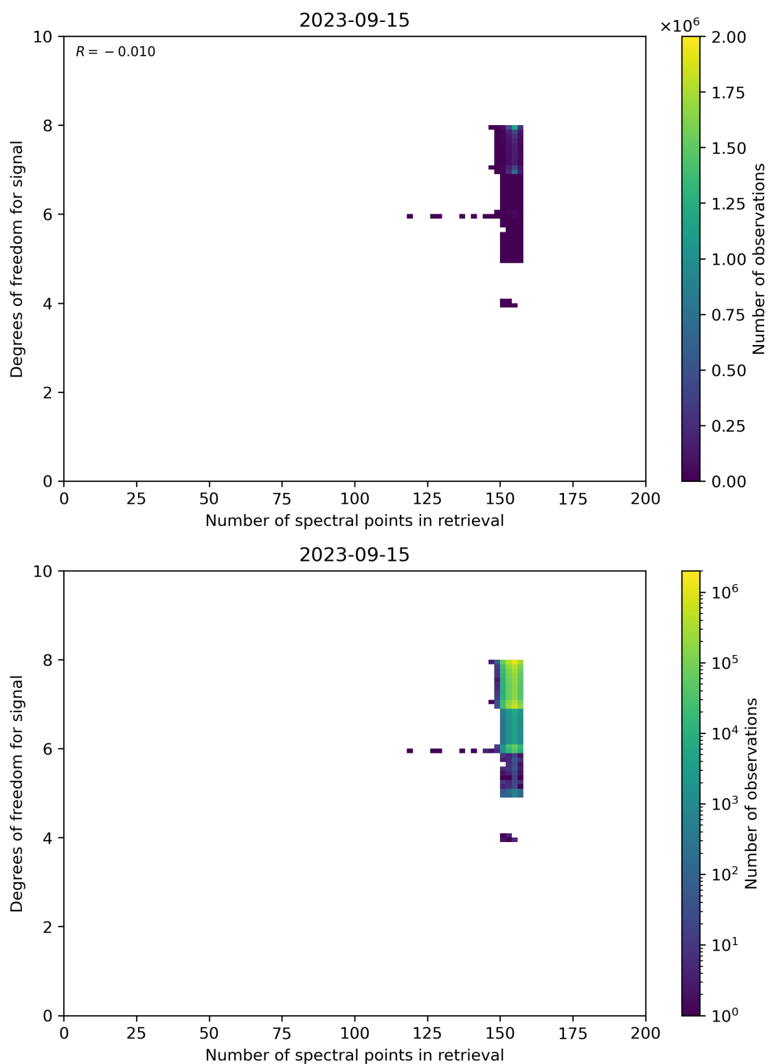
Figure 59: Scatter density plot of “Number of spectral points in retrieval” against “Degrees of freedom for signal” for 2023-09-15 to 2023-09-16.
