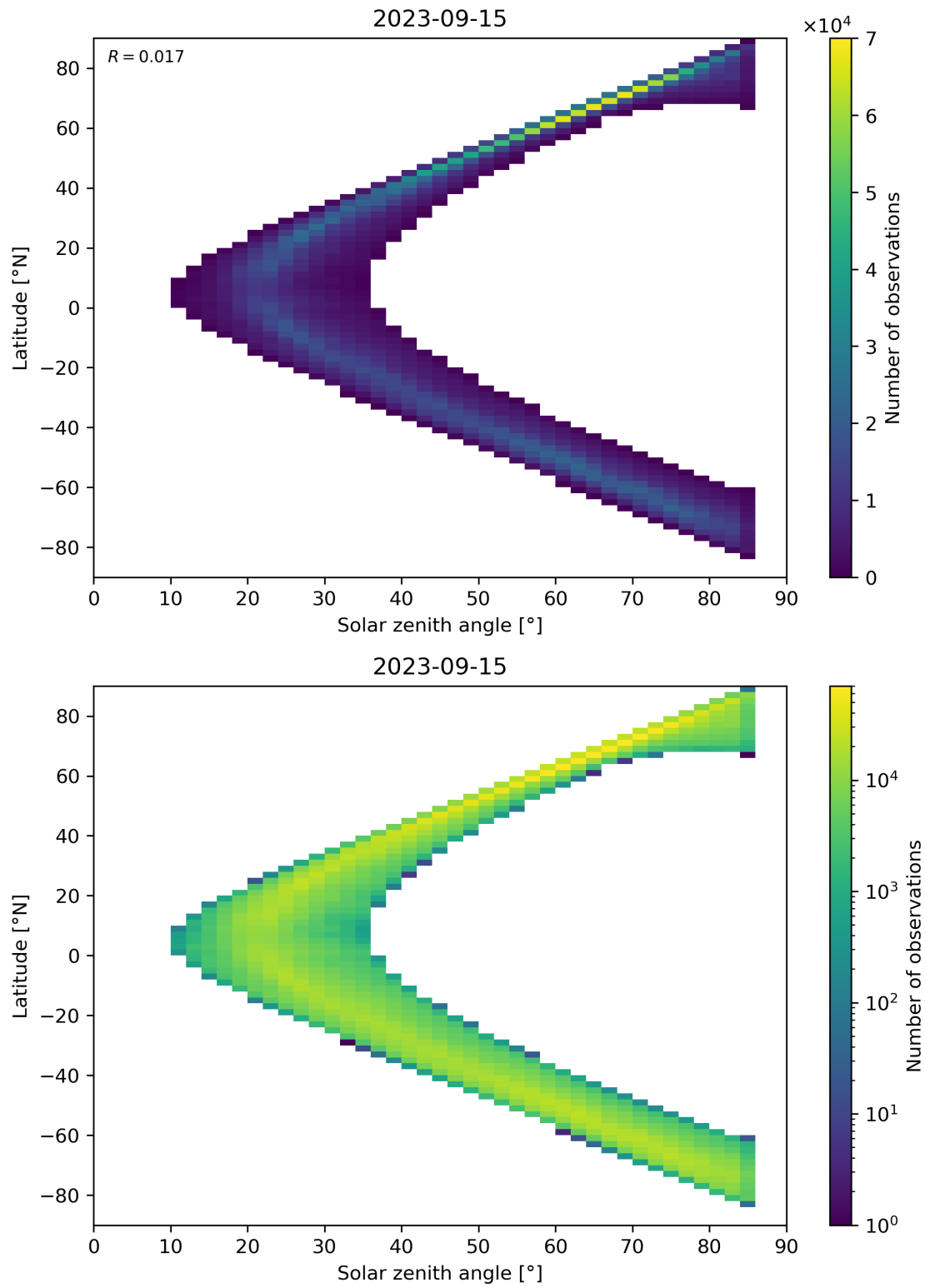
Figure 66: Scatter density plot of “Solar zenith angle” against “Latitude” for 2023-09-15 to 2023-09-16.
