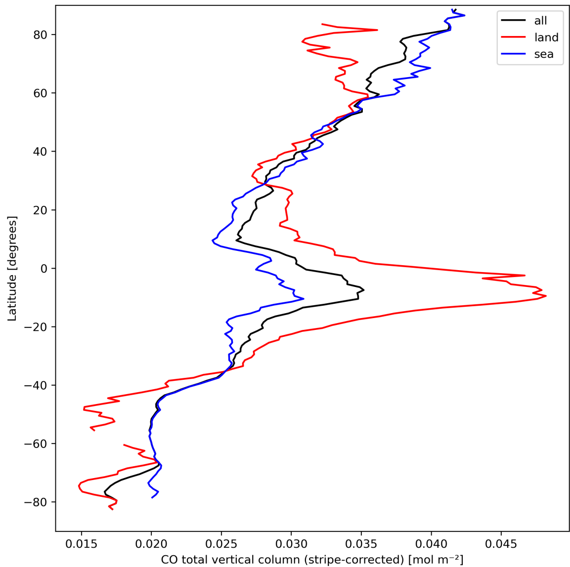
Figure 11: Zonal average of “CO total vertical column (stripe-corrected)” for 2023-09-15 to 2023-09-16.
