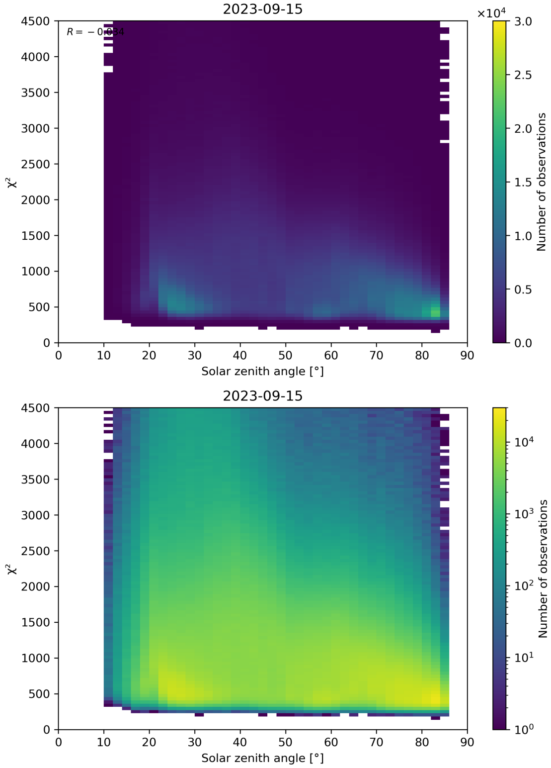
Figure 64: Scatter density plot of “Solar zenith angle” against “ \chi^2 ” for 2023-09-15 to 2023-09-16.
