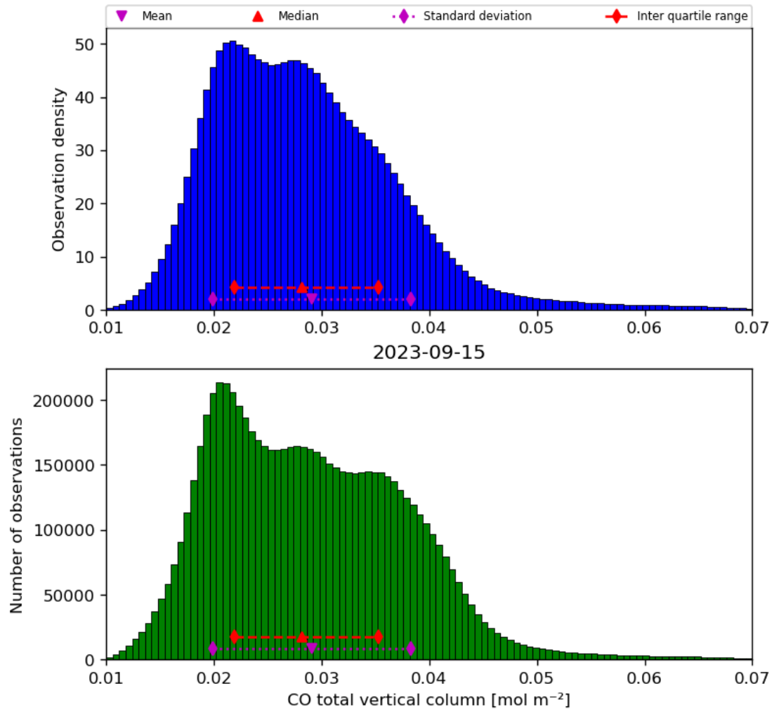
Figure 18: Histogram of “CO total vertical column” for 2023-09-15 to 2023-09-16
