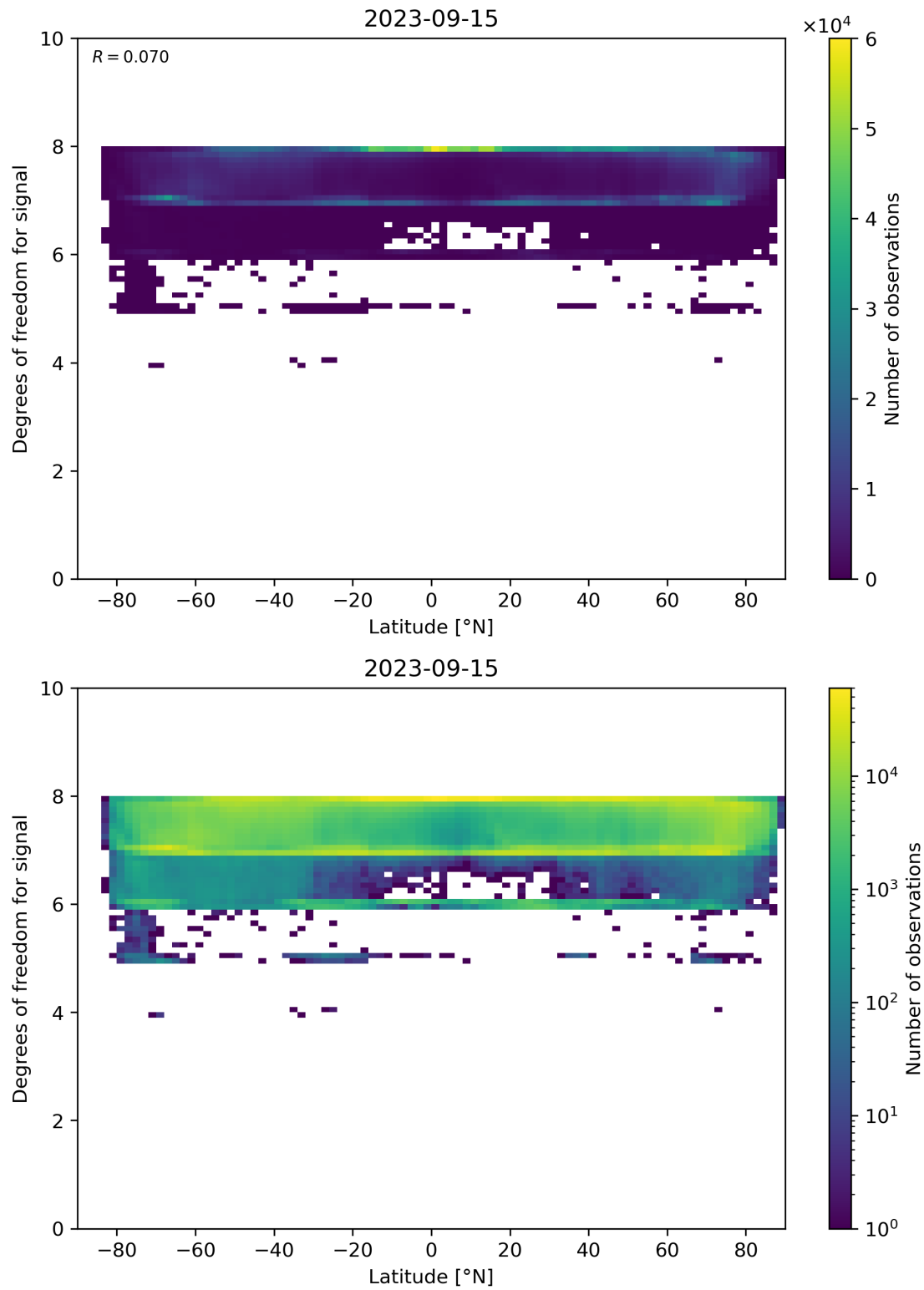
Figure 55: Scatter density plot of “Latitude” against “Degrees of freedom for signal” for 2023-09-15 to 2023-09-16.
