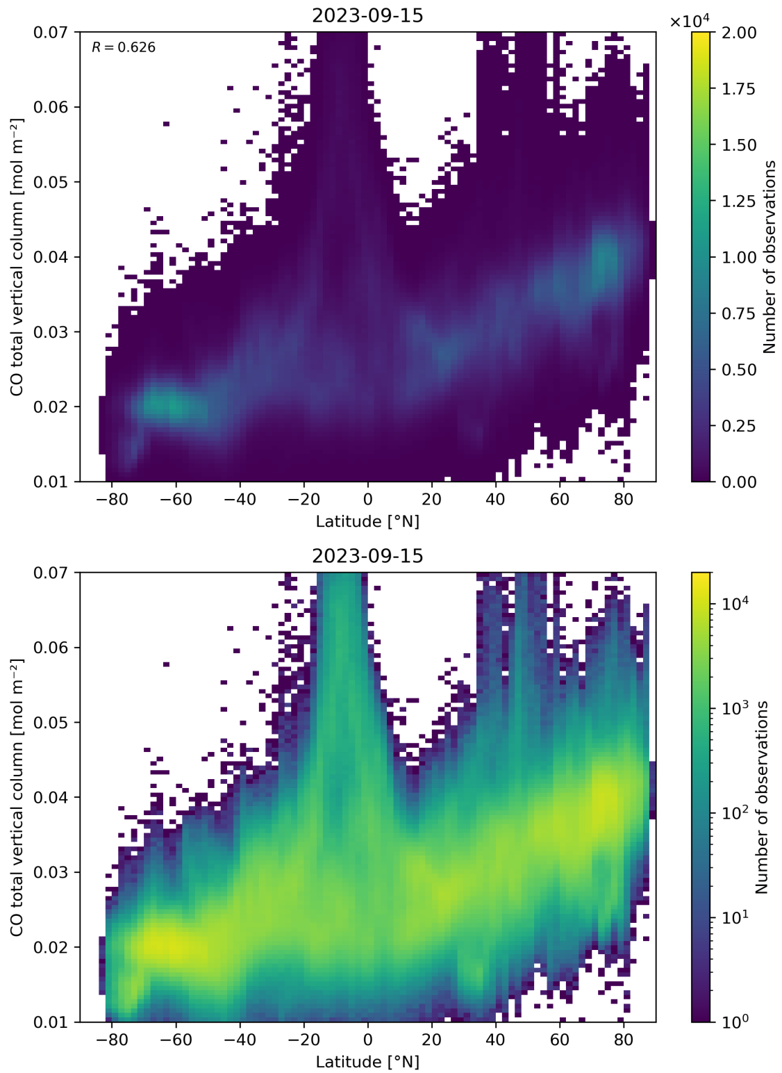
Figure 51: Scatter density plot of “Latitude” against “CO total vertical column” for 2023-09-15 to 2023-09-16.
