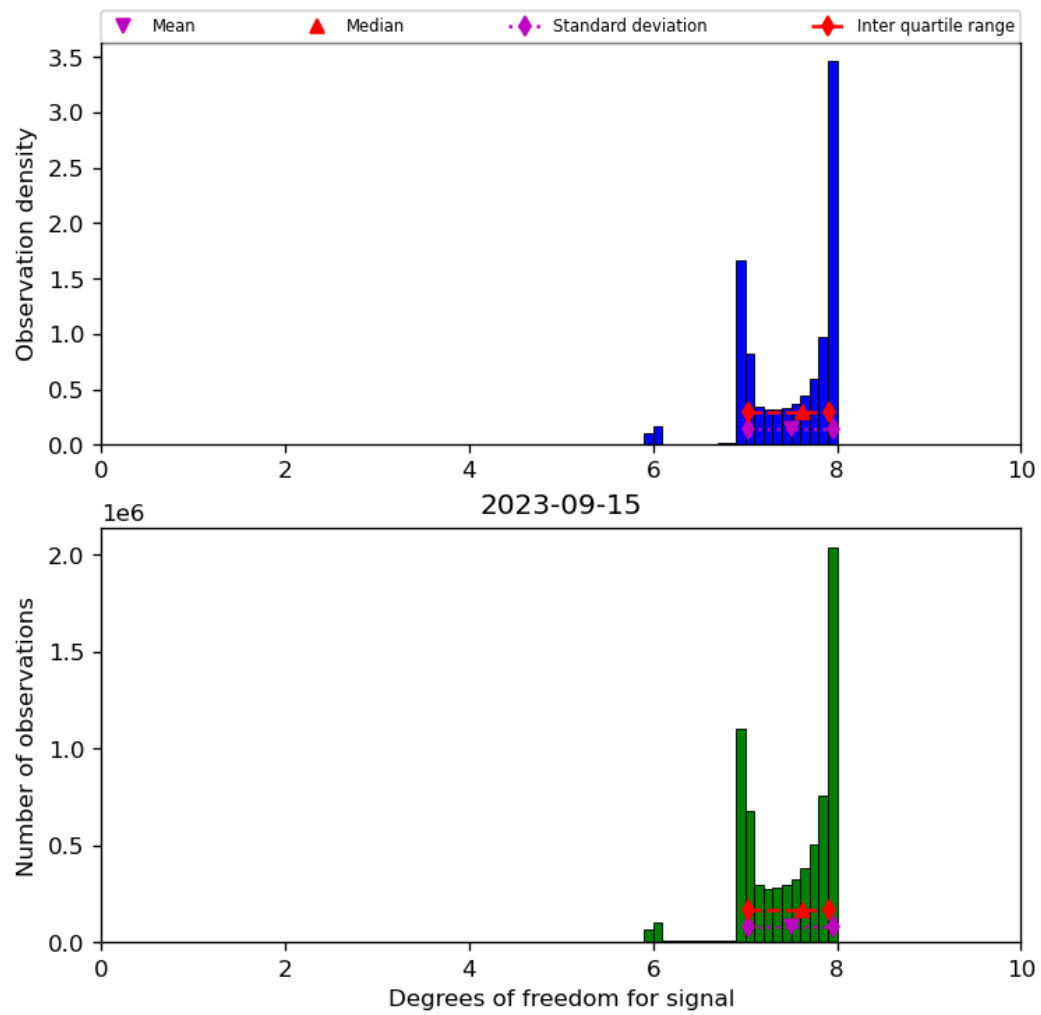
Figure 23: Histogram of “Degrees of freedom for signal” for 2023-09-15 to 2023-09-16
