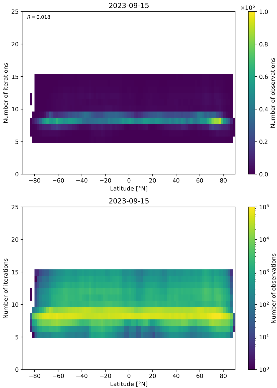
Figure 56: Scatter density plot of “Latitude” against “Number of iterations” for 2023-09-15 to 2023-09-16.
