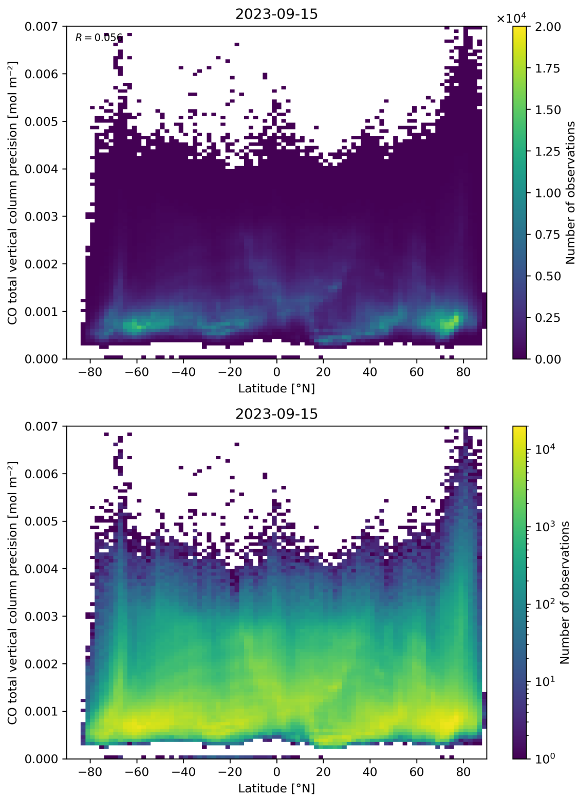
Figure 53: Scatter density plot of “Latitude” against “CO total vertical column precision” for 2023-09-15 to 2023-09-16.
