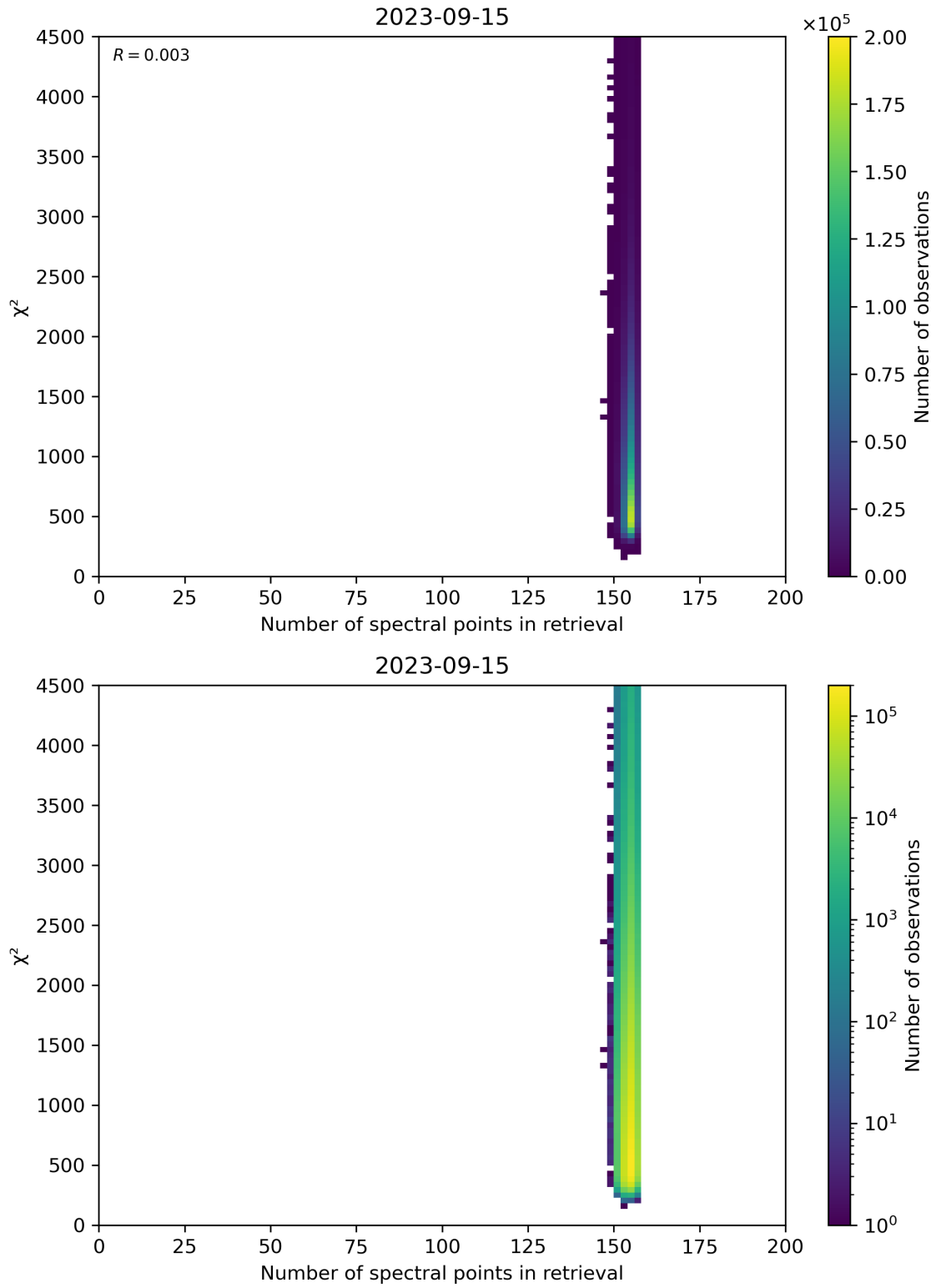
Figure 58: Scatter density plot of “Number of spectral points in retrieval” against “ \chi^2 ” for 2023-09-15 to 2023-09-16.
