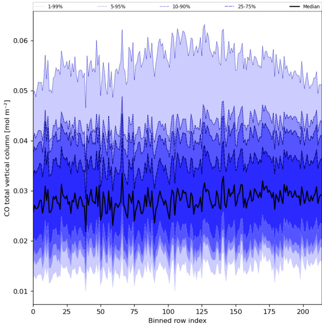
Figure 26: Along track statistics of “CO total vertical column” for 2023-09-15 to 2023-09-16
