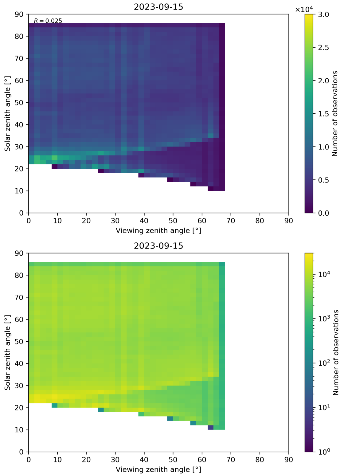
Figure 77: Scatter density plot of “Viewing zenith angle” against “Solar zenith angle” for 2023-09-15 to 2023-09-16.
