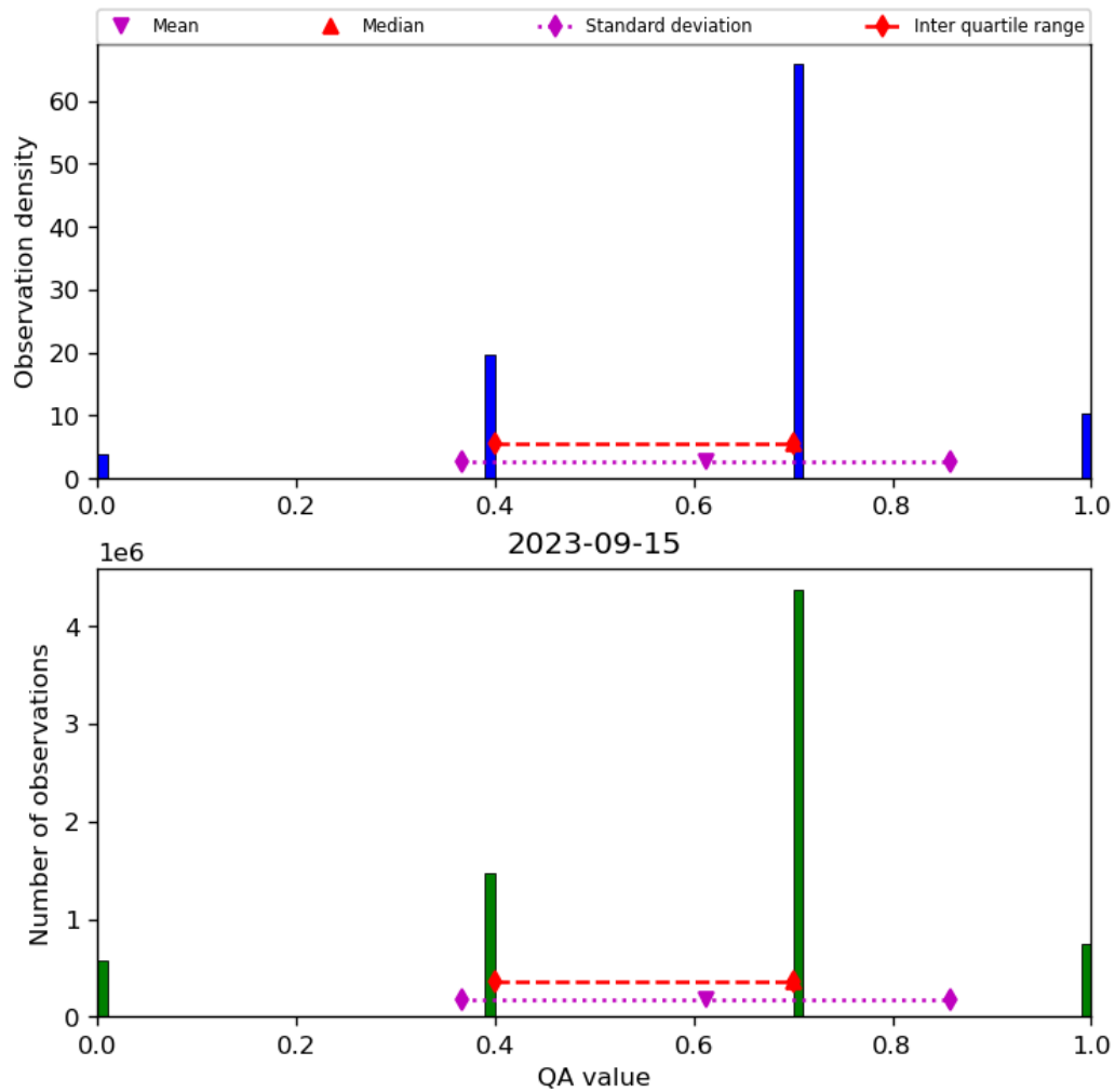
Figure 17: Histogram of “QA value” for 2023-09-15 to 2023-09-16
