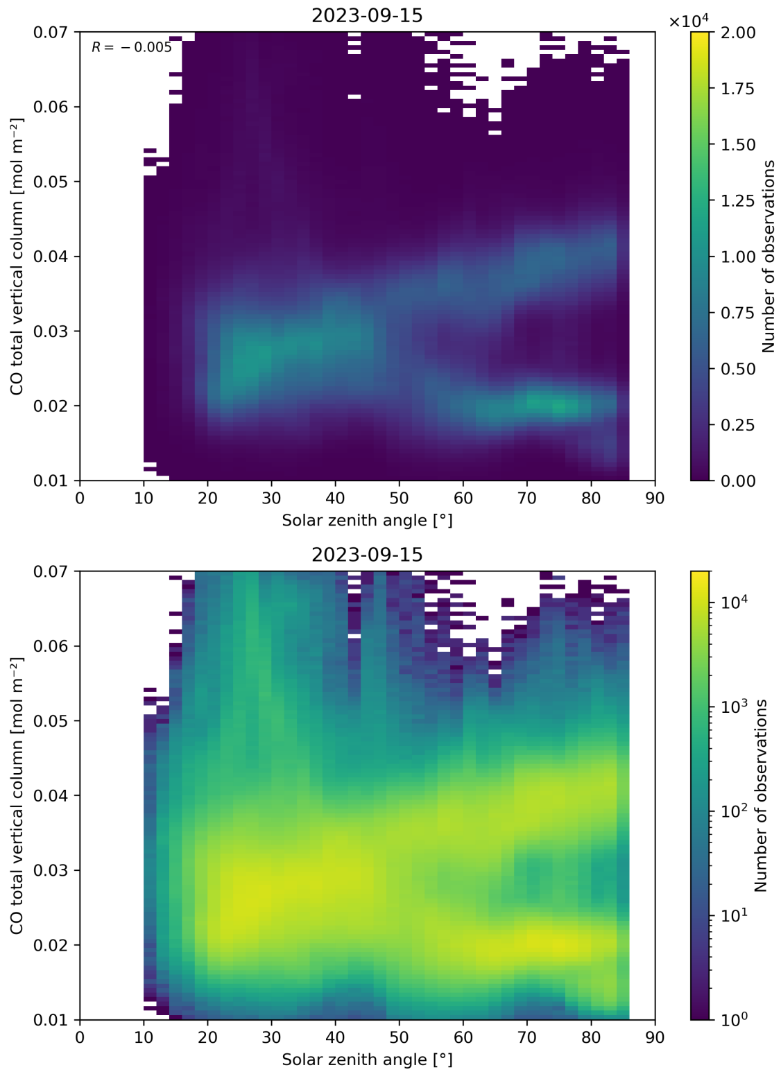
Figure 61: Scatter density plot of “Solar zenith angle” against “CO total vertical column” for 2023-09-15 to 2023-09-16.
