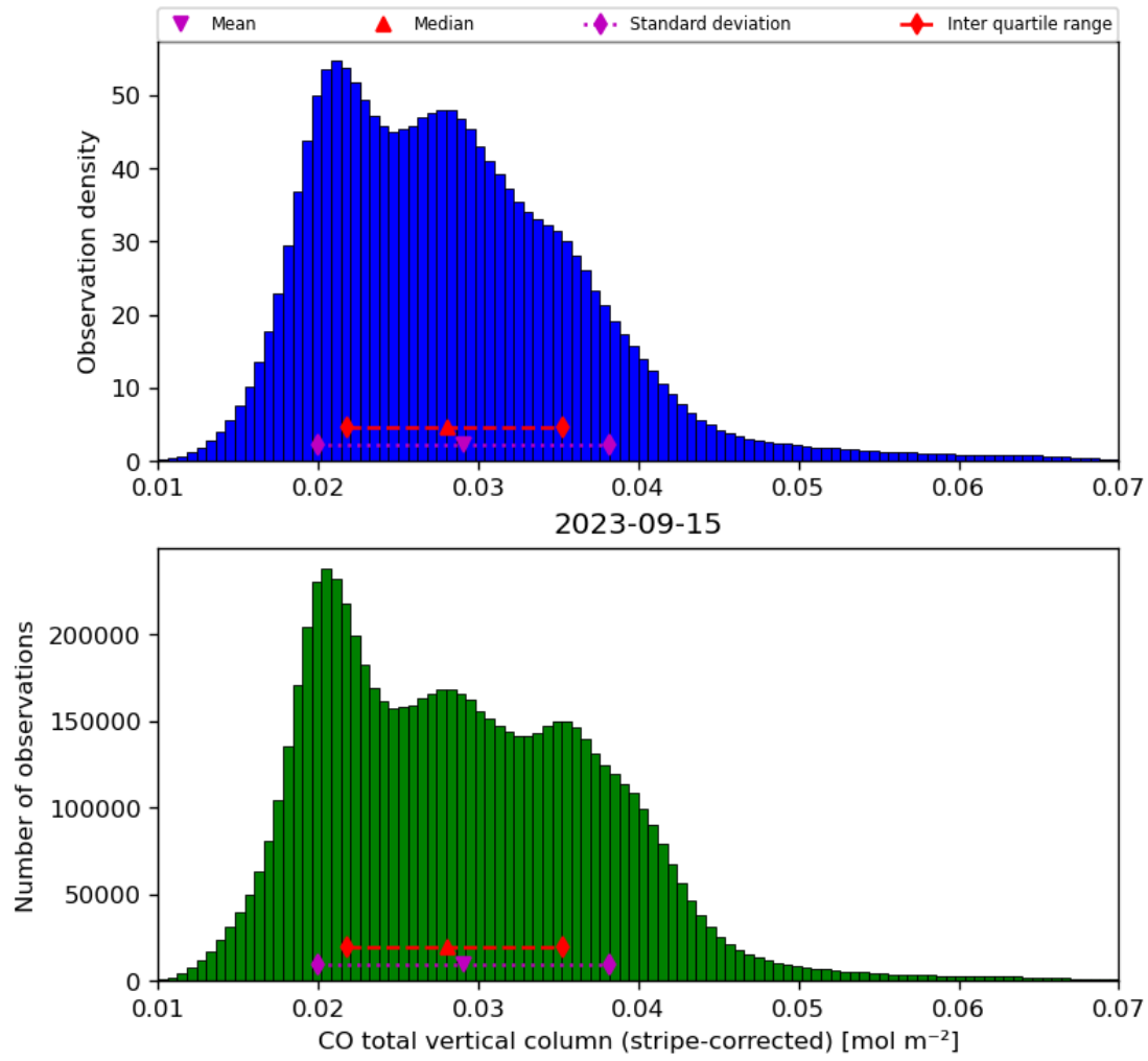
Figure 19: Histogram of “CO total vertical column (stripe-corrected)” for 2023-09-15 to 2023-09-16
