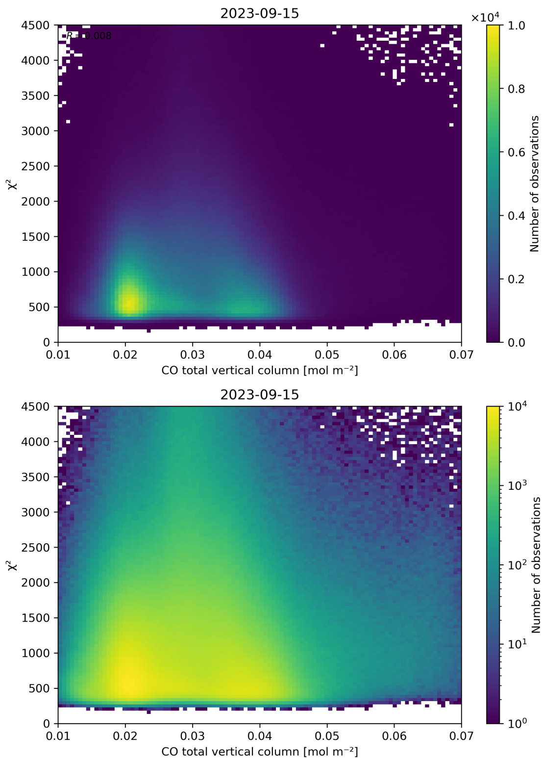
Figure 35: Scatter density plot of “CO total vertical column” against “ \chi^2 ” for 2023-09-15 to 2023-09-16.
