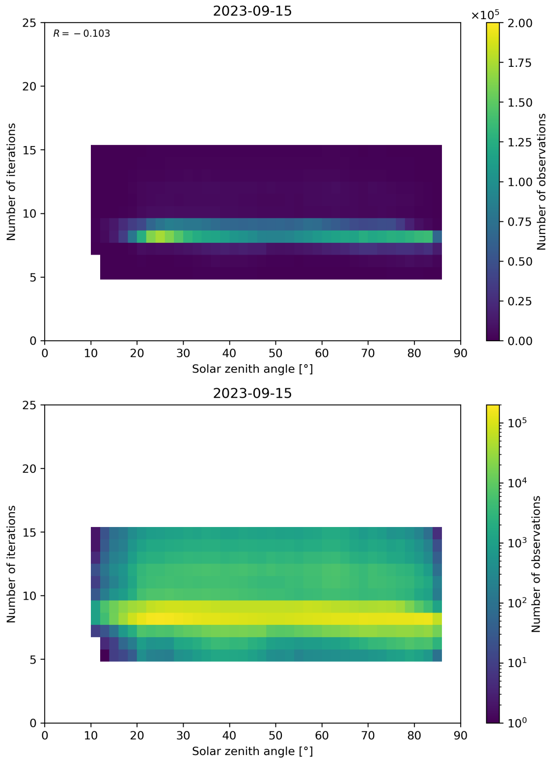
Figure 67: Scatter density plot of “Solar zenith angle” against “Number of iterations” for 2023-09-15 to 2023-09-16.
