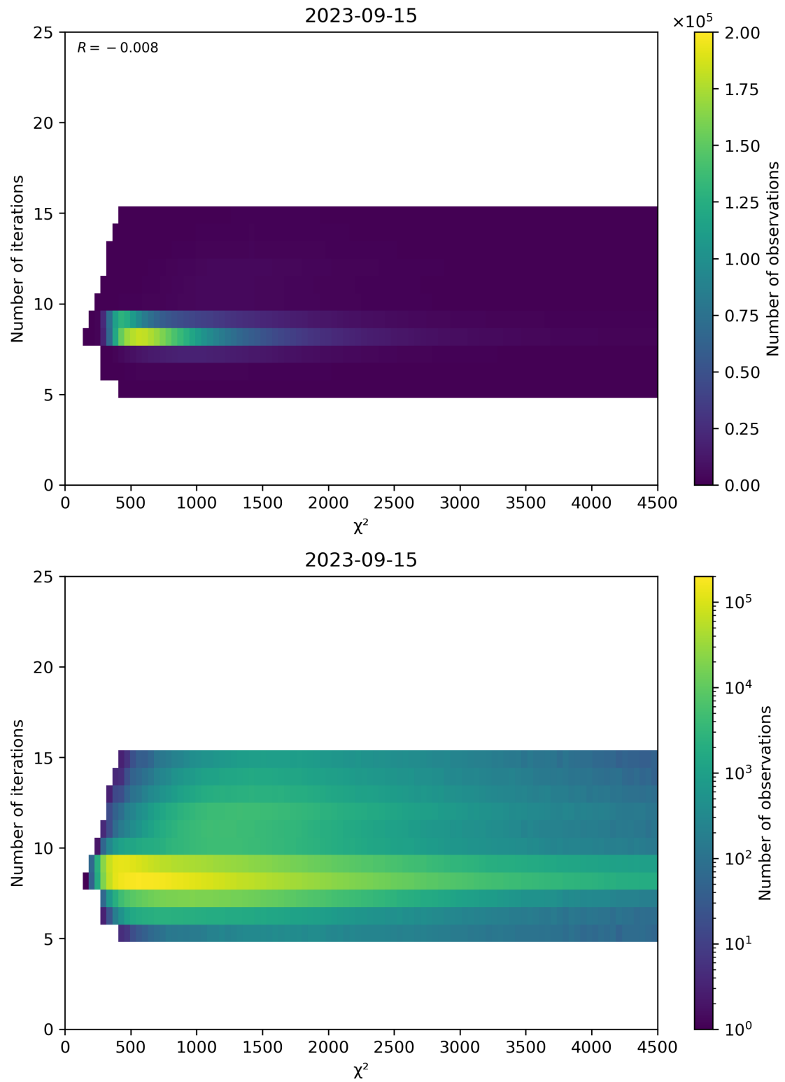
Figure 49: Scatter density plot of “ \chi^2 ” against “Number of iterations” for 2023-09-15 to 2023-09-16.
