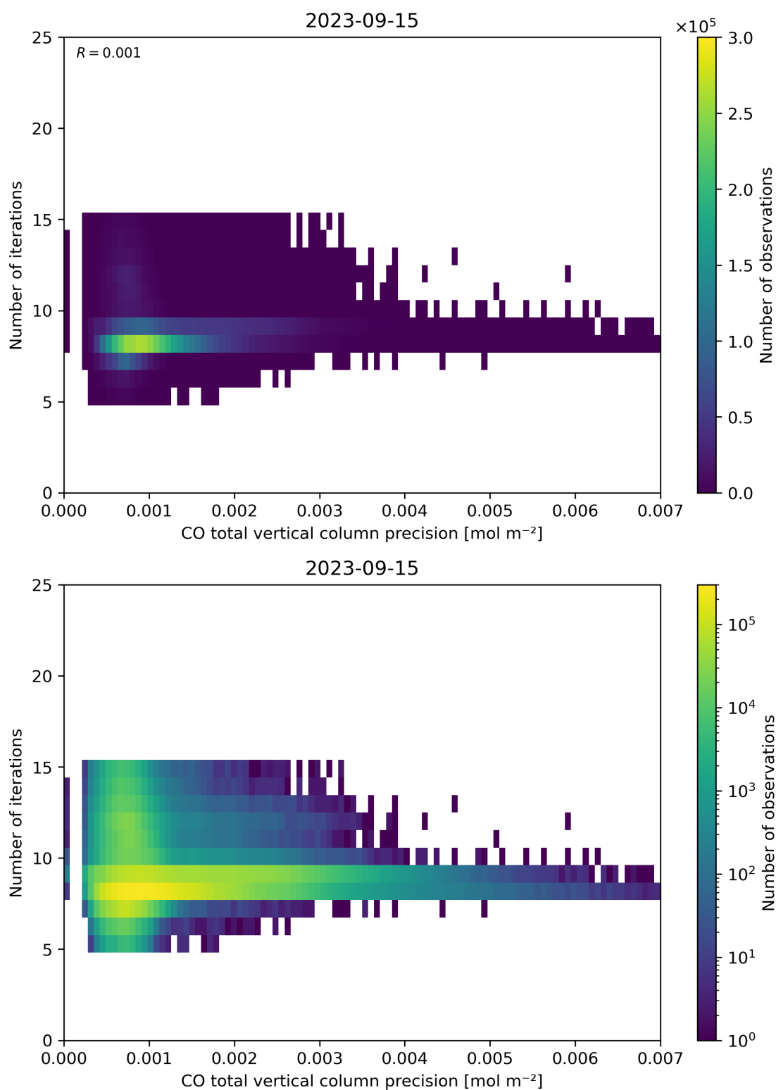
Figure 46: Scatter density plot of “CO total vertical column precision” against “Number of iterations” for 2023-09-15 to 2023-09-16.
