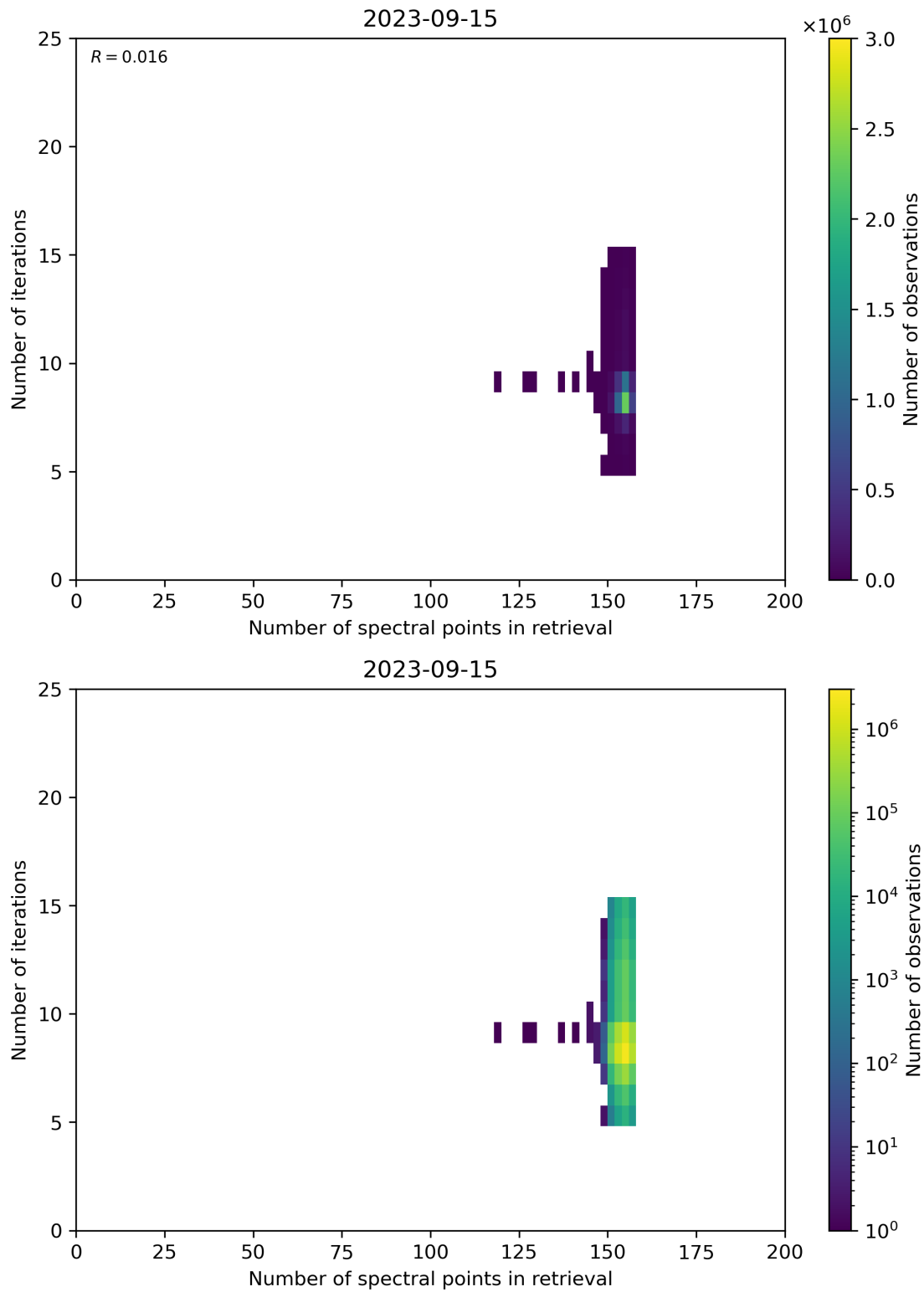
Figure 60: Scatter density plot of “Number of spectral points in retrieval” against “Number of iterations” for 2023-09-15 to 2023-09-16.
