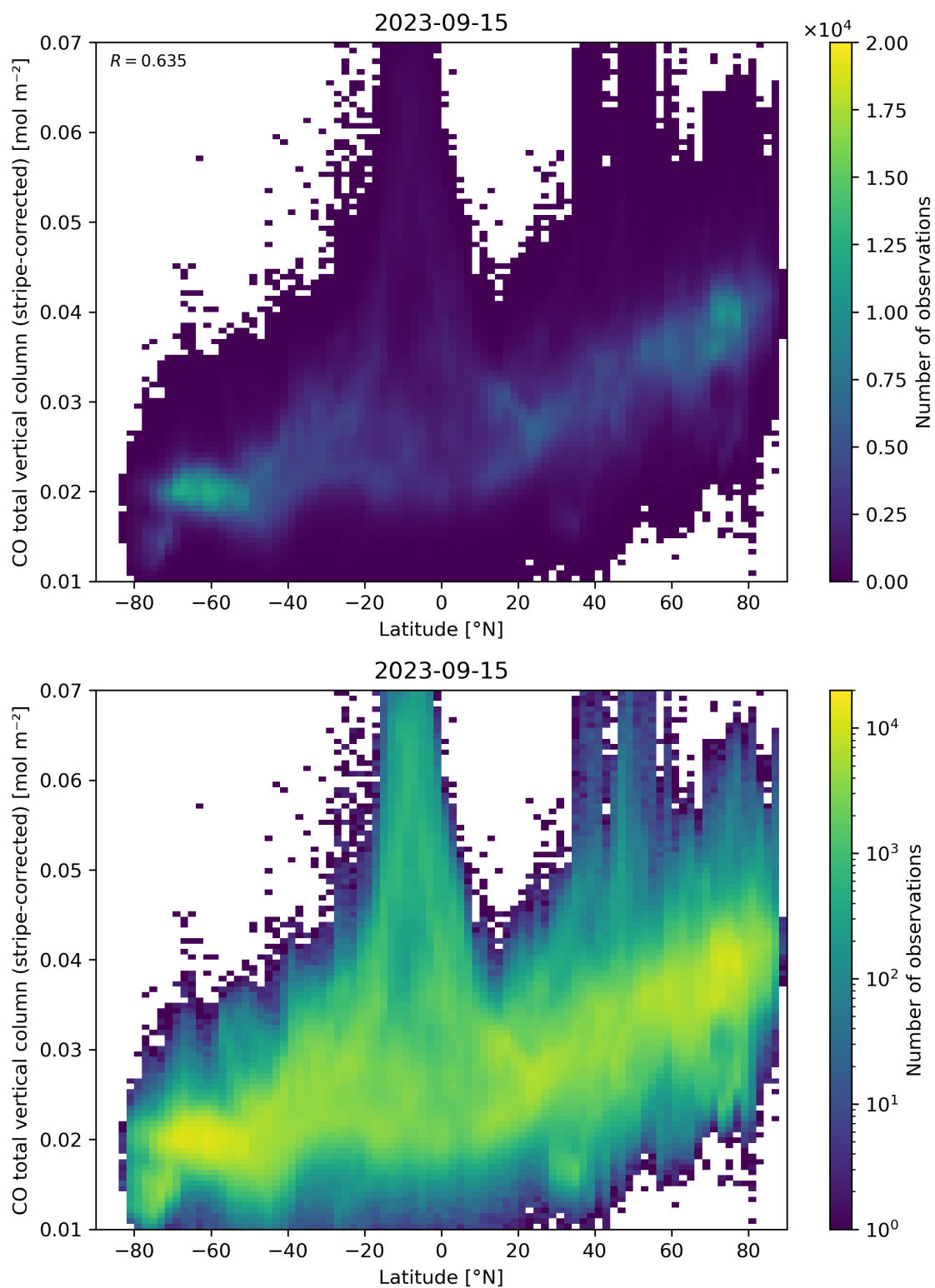
Figure 52: Scatter density plot of “Latitude” against “CO total vertical column (stripe-corrected)” for 2023-09-15 to 2023-09-16.
