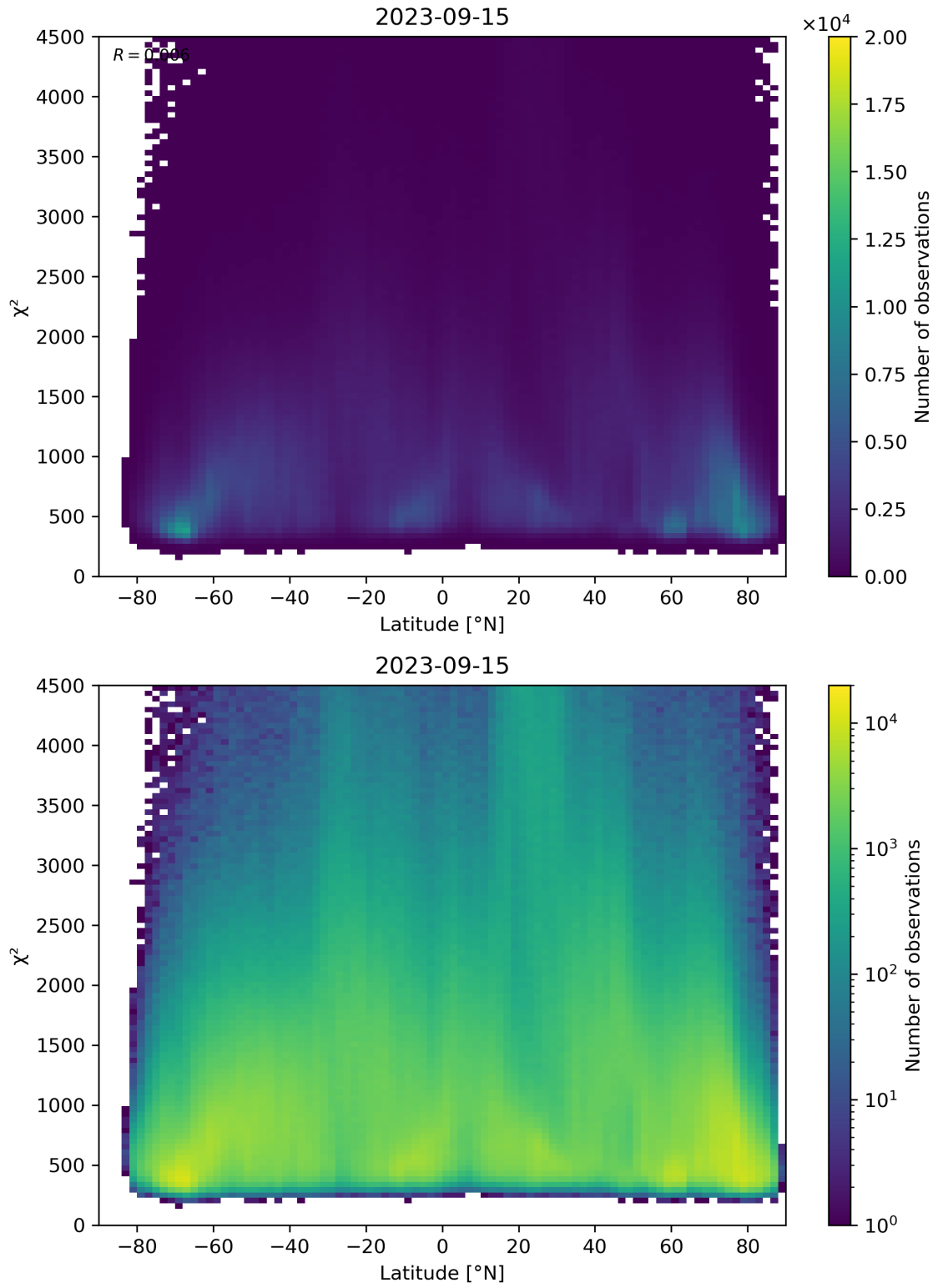
Figure 54: Scatter density plot of “Latitude” against “ \chi^2 ” for 2023-09-15 to 2023-09-16.
