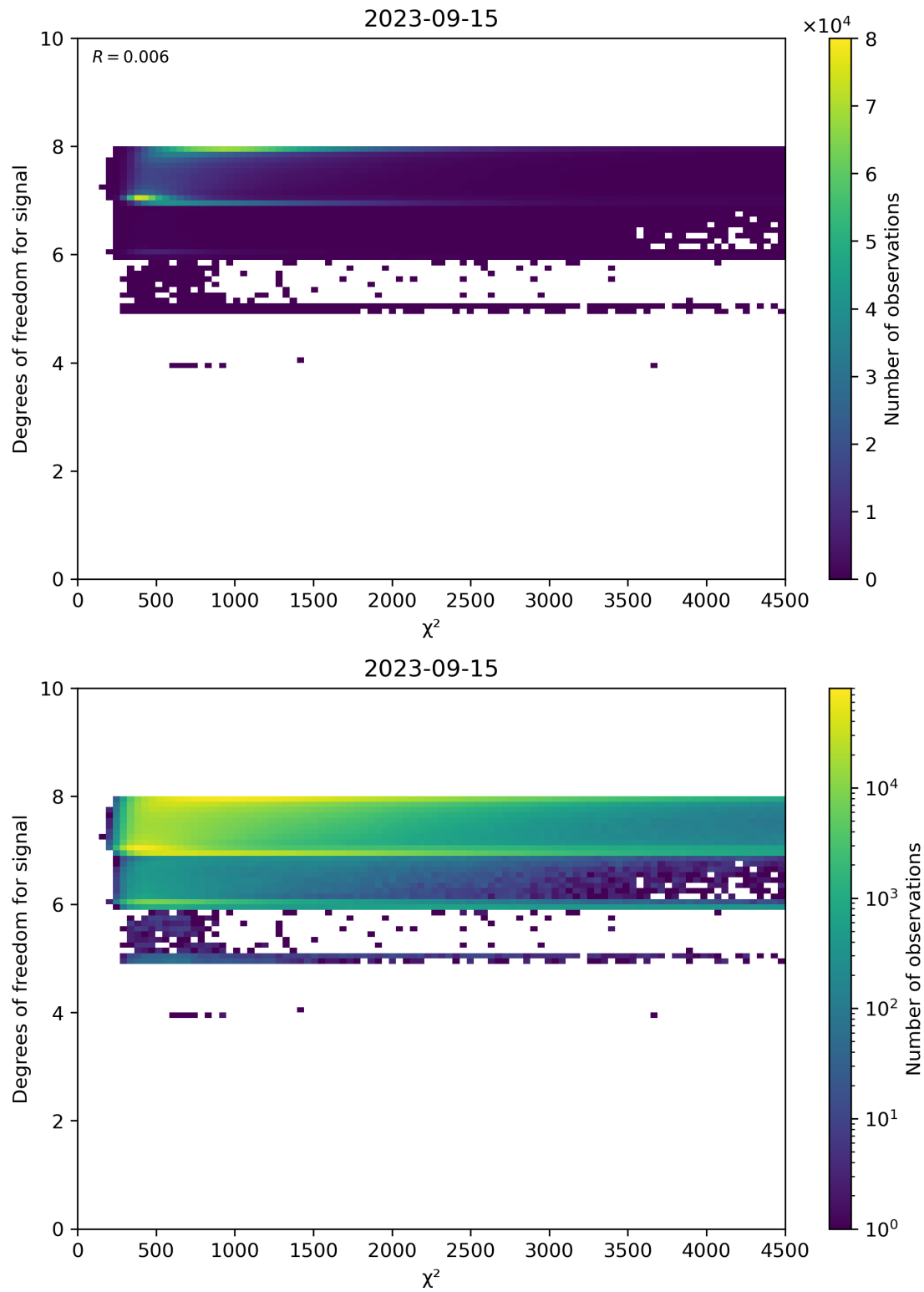
Figure 48: Scatter density plot of “ \chi^2 ” against “Degrees of freedom for signal” for 2023-09-15 to 2023-09-16.
