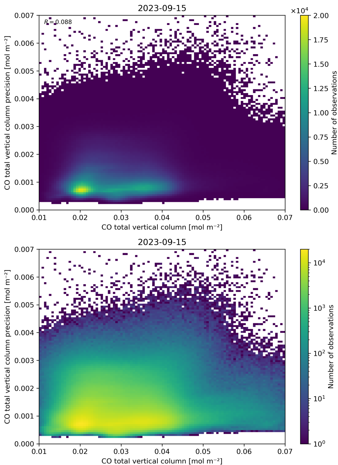
Figure 34: Scatter density plot of “CO total vertical column” against “CO total vertical column precision” for 2023-09-15 to 2023-09-16.
