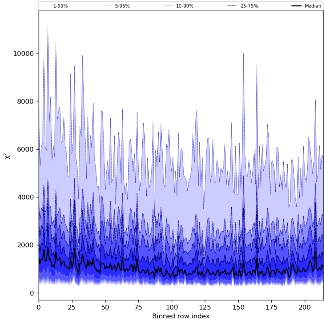
Figure 30: Along track statistics of “ \chi^2 ” for 2023-09-15 to 2023-09-16
