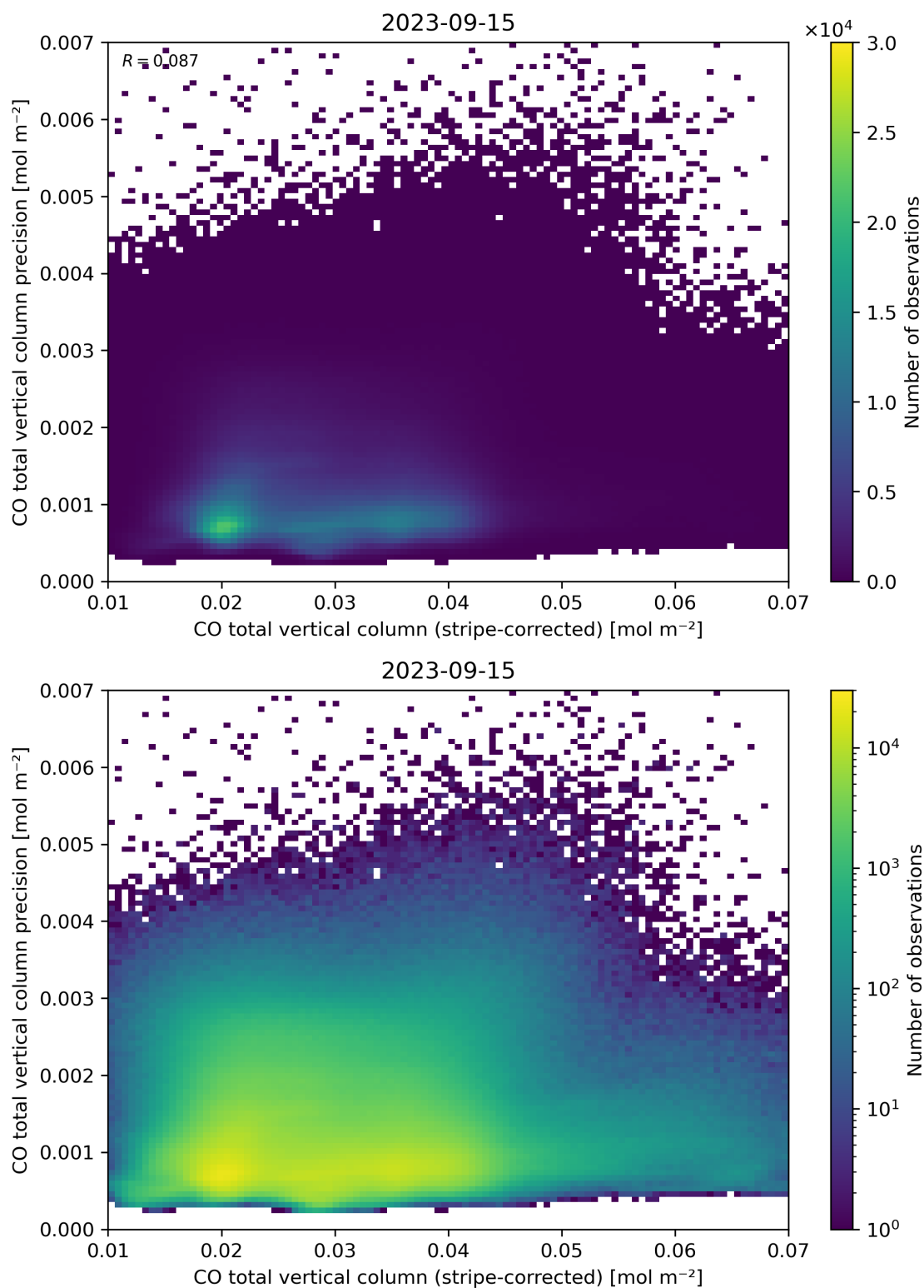
Figure 36: Scatter density plot of “CO total vertical column (stripe-corrected)” against “CO total vertical column precision” for 2023-09-15 to 2023-09-16.
