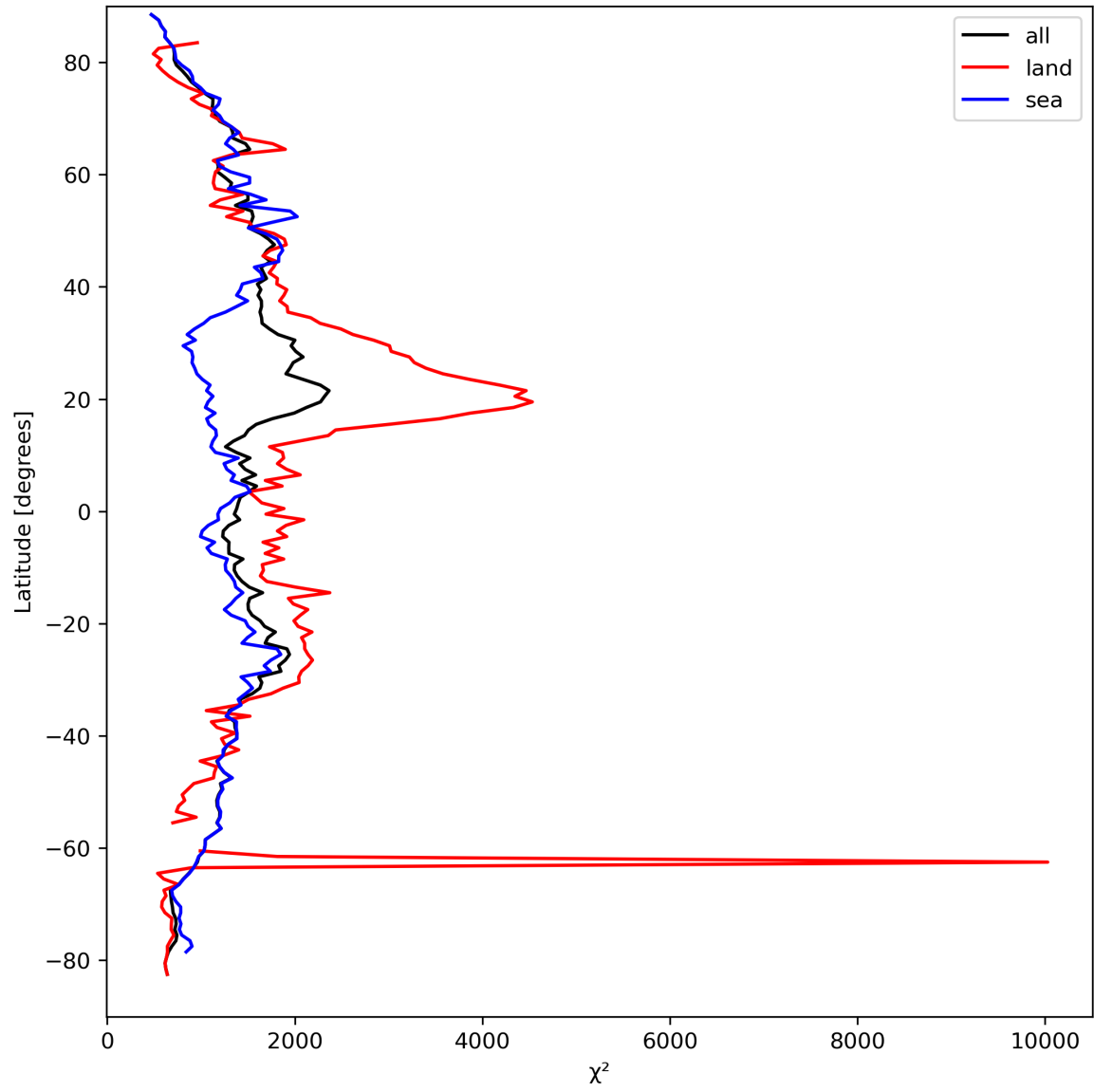
Figure 14: Zonal average of “ \chi^2 ” for 2023-09-15 to 2023-09-16.
