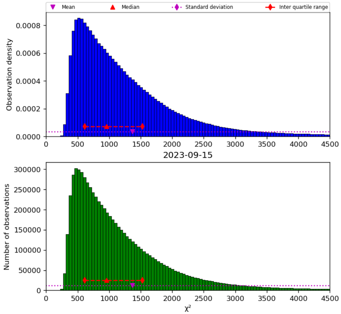
Figure 22: Histogram of " \chi^2 " for 2023-09-15 to 2023-09-16
