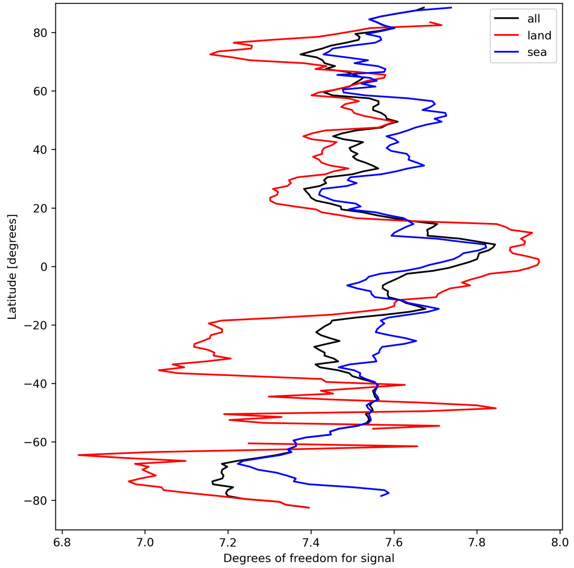
Figure 15: Zonal average of “Degrees of freedom for signal” for 2023-09-15 to 2023-09-16.
