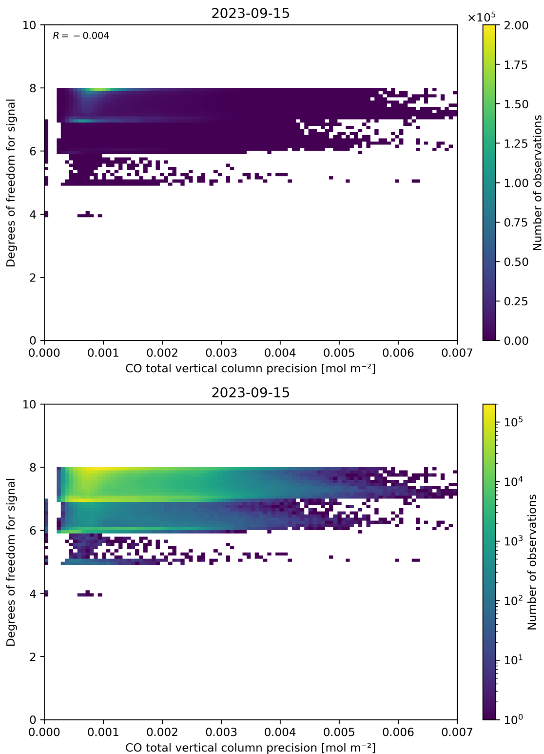
Figure 45: Scatter density plot of “CO total vertical column precision” against “Degrees of freedom for signal” for 2023-09-15 to 2023-09-16.
