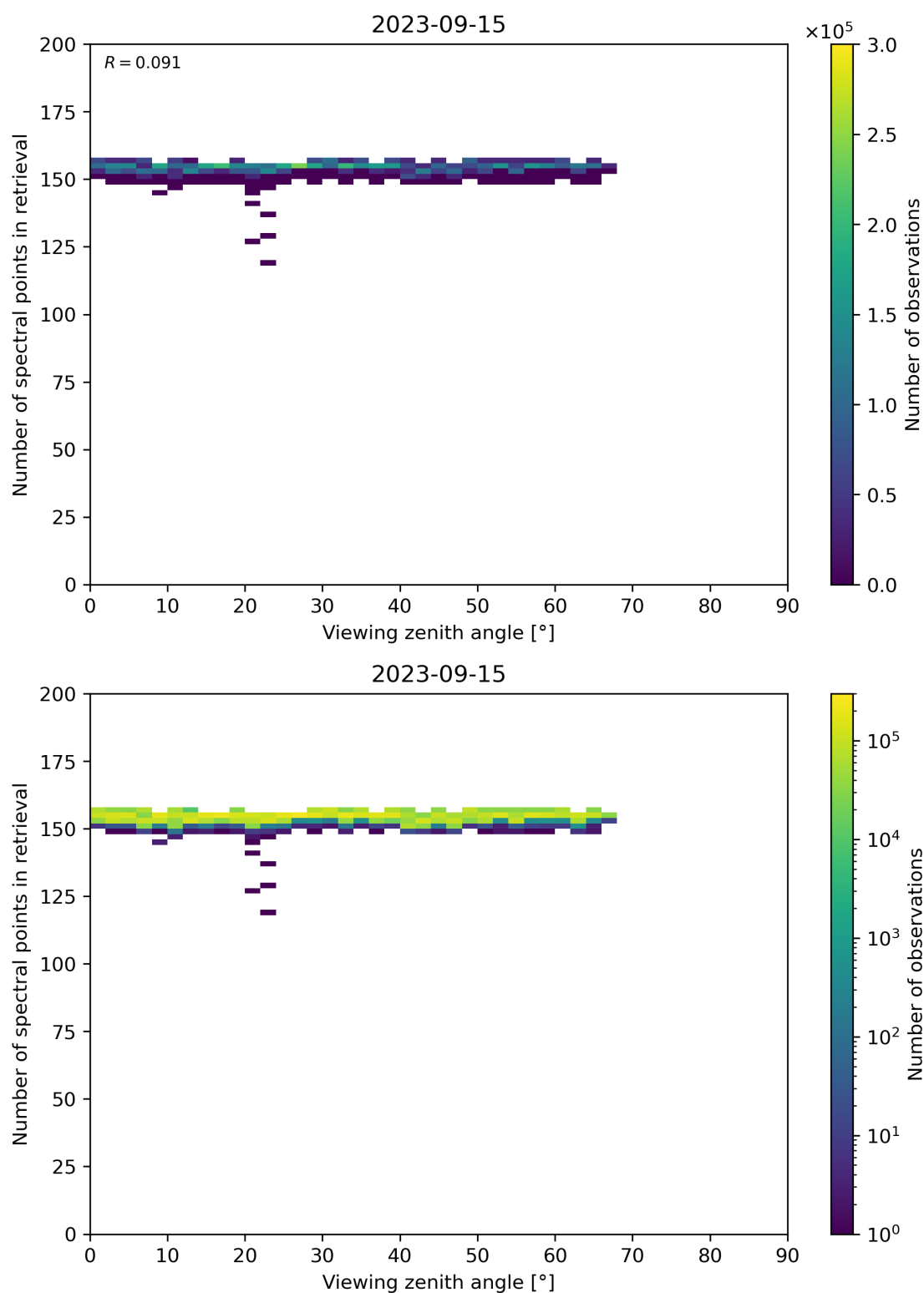
Figure 76: Scatter density plot of “Viewing zenith angle” against “Number of spectral points in retrieval” for 2023-09-15 to 2023-09-16.
