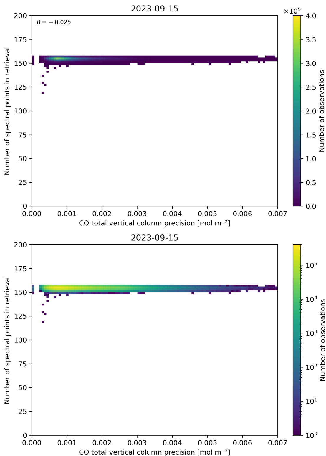
Figure 47: Scatter density plot of “CO total vertical column precision” against “Number of spectral points in retrieval” for 2023-09-15 to 2023-09-16.
