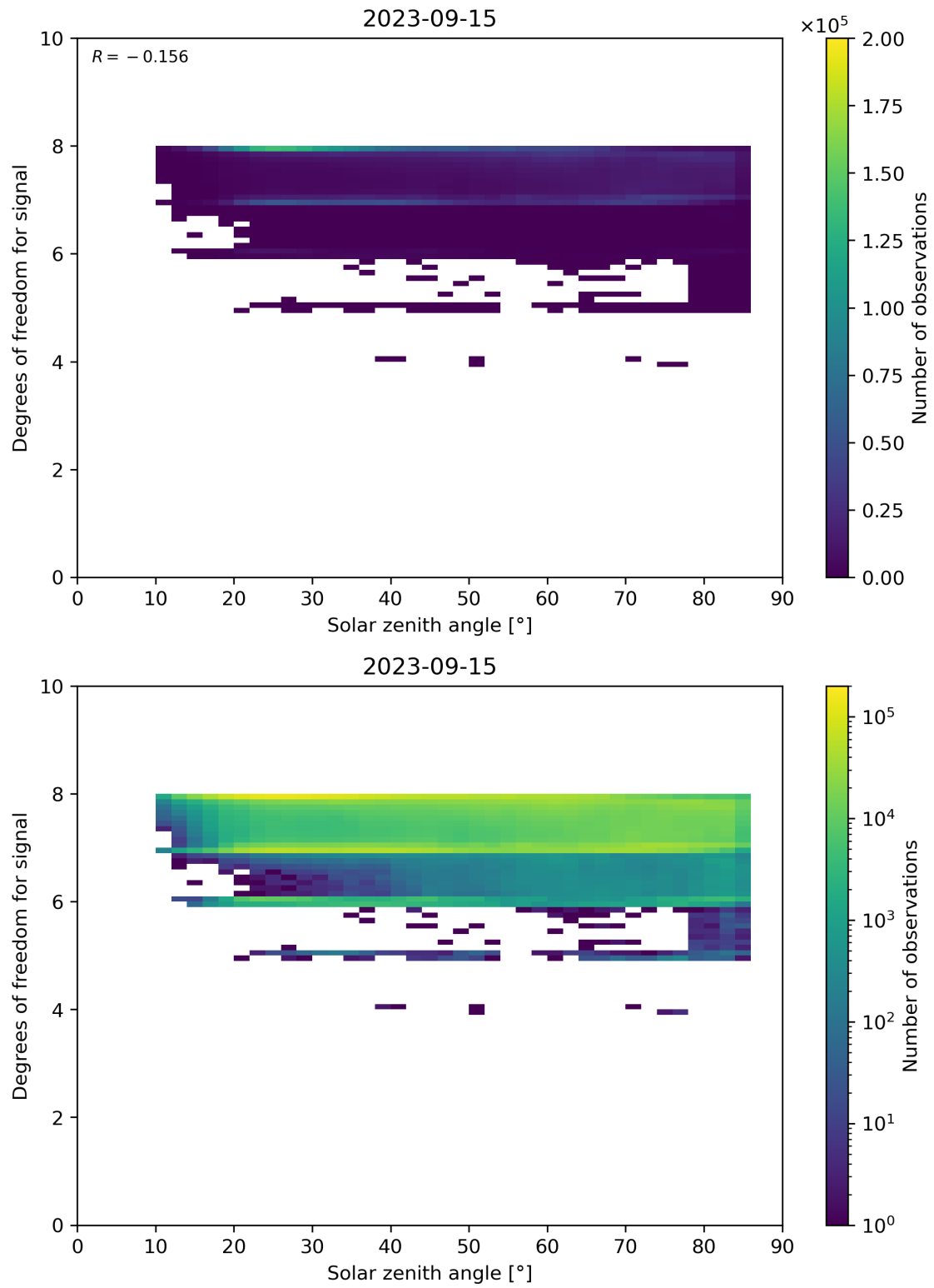
Figure 65: Scatter density plot of “Solar zenith angle” against “Degrees of freedom for signal” for 2023-09-15 to 2023-09-16.
