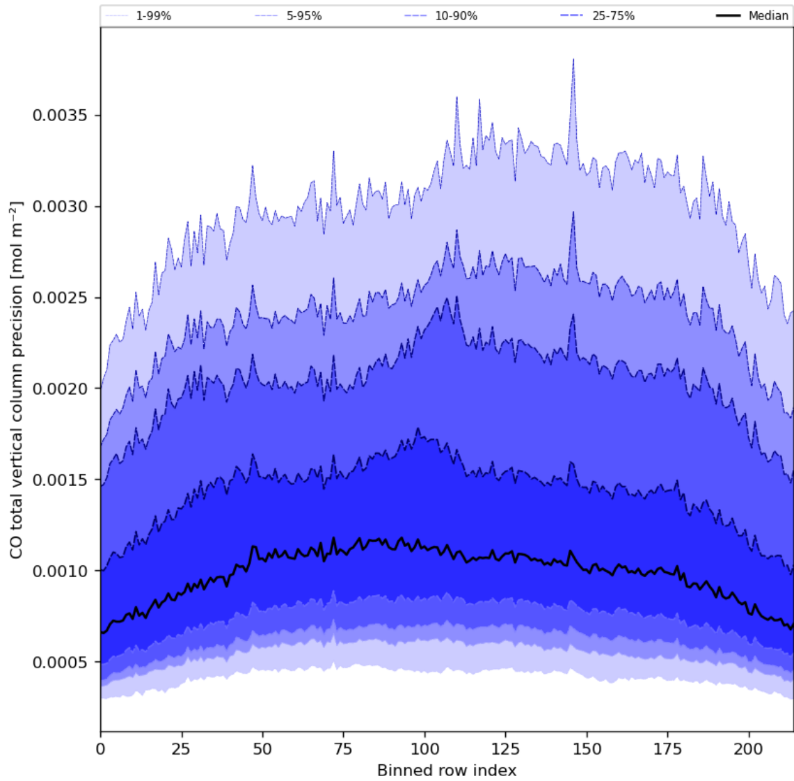
Figure 28: Along track statistics of “CO total vertical column precision” for 2023-09-15 to 2023-09-16
