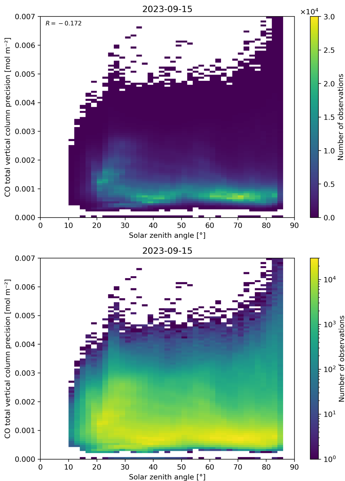
Figure 63: Scatter density plot of “Solar zenith angle” against “CO total vertical column precision” for 2023-09-15 to 2023-09-16.
