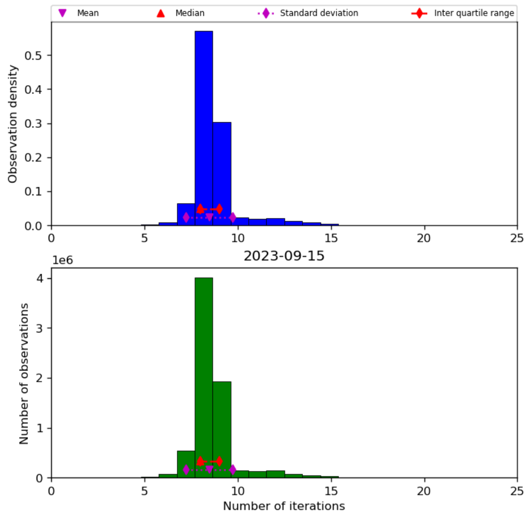
Figure 24: Histogram of “Number of iterations” for 2023-09-15 to 2023-09-16
