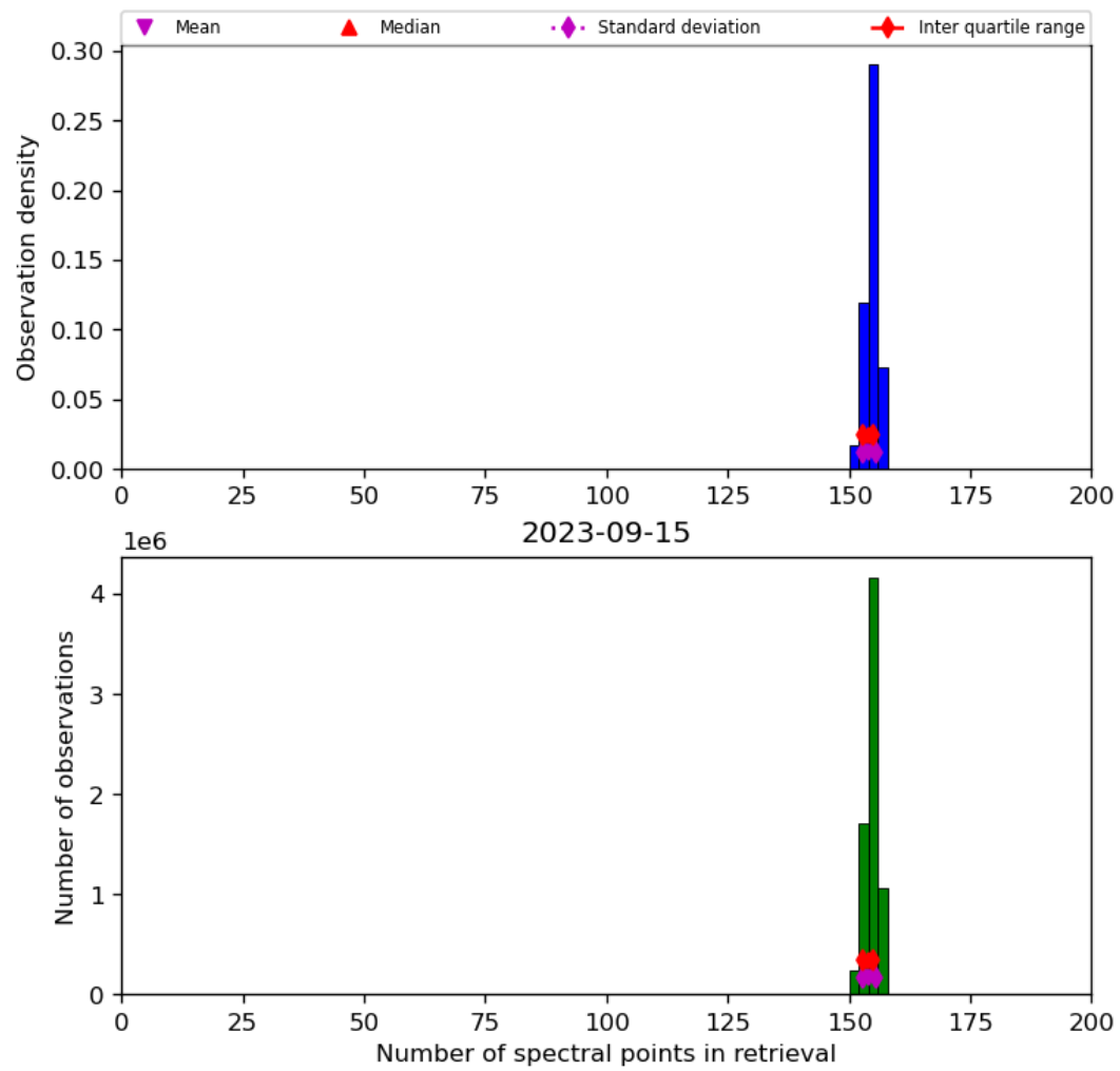
Figure 21: Histogram of “Number of spectral points in retrieval” for 2023-09-15 to 2023-09-16
