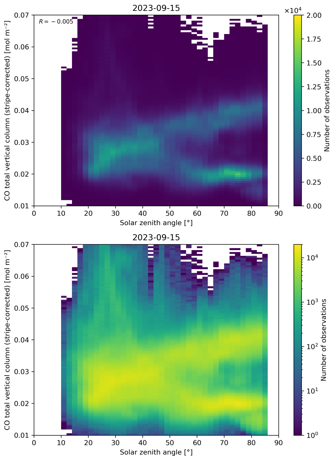
Figure 62: Scatter density plot of “Solar zenith angle” against “CO total vertical column (stripe-corrected)” for 2023-09-15 to 2023-09-16.
