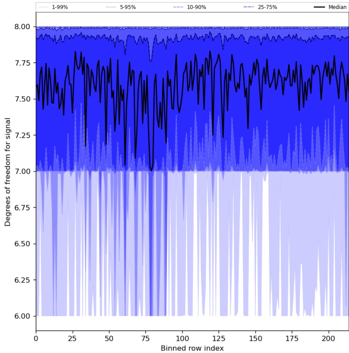
Figure 31: Along track statistics of “Degrees of freedom for signal” for 2023-09-15 to 2023-09-16
