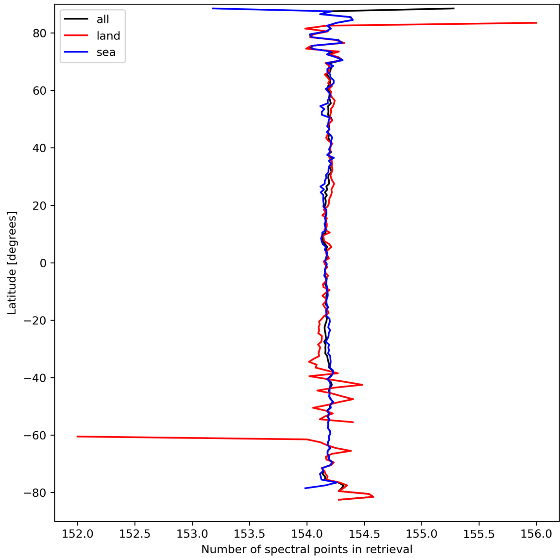
Figure 13: Zonal average of “Number of spectral points in retrieval” for 2023-09-15 to 2023-09-16.
