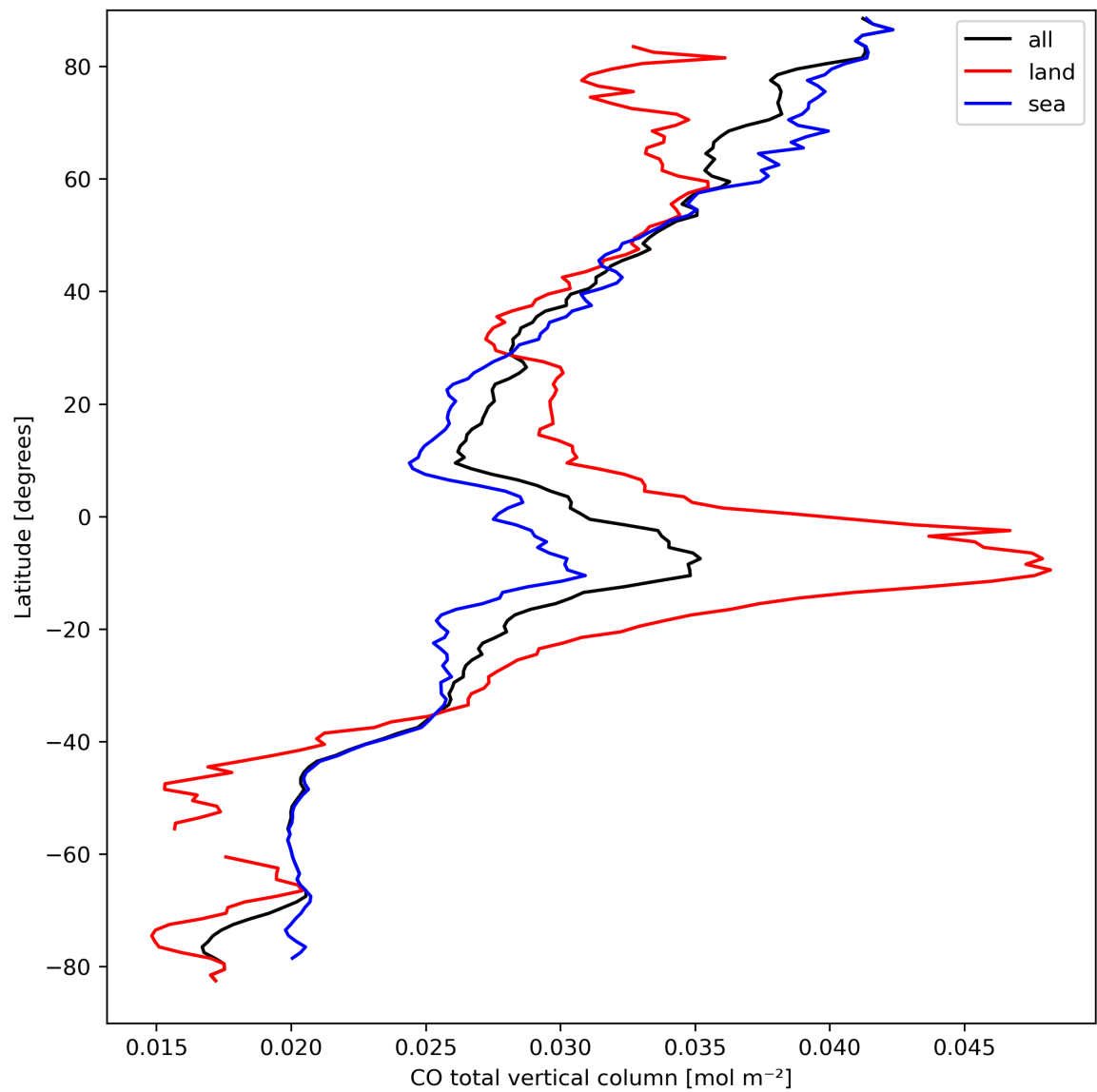
Figure 10: Zonal average of “CO total vertical column” for 2023-09-15 to 2023-09-16.
