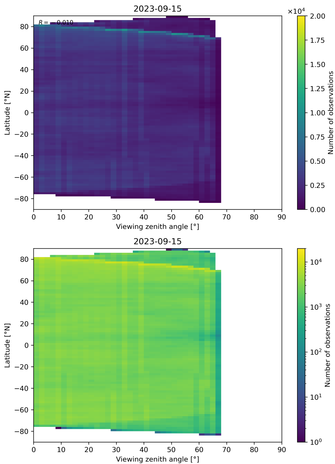
Figure 74: Scatter density plot of “Viewing zenith angle” against “Latitude” for 2023-09-15 to 2023-09-16.
