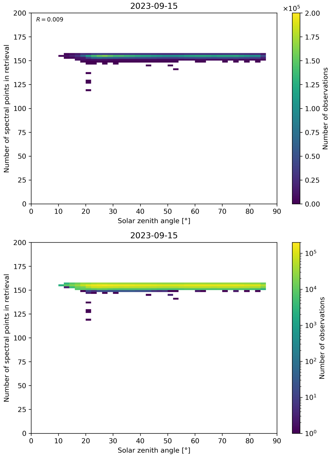
Figure 68: Scatter density plot of “Solar zenith angle” against “Number of spectral points in retrieval” for 2023-09-15 to 2023-09-16.
