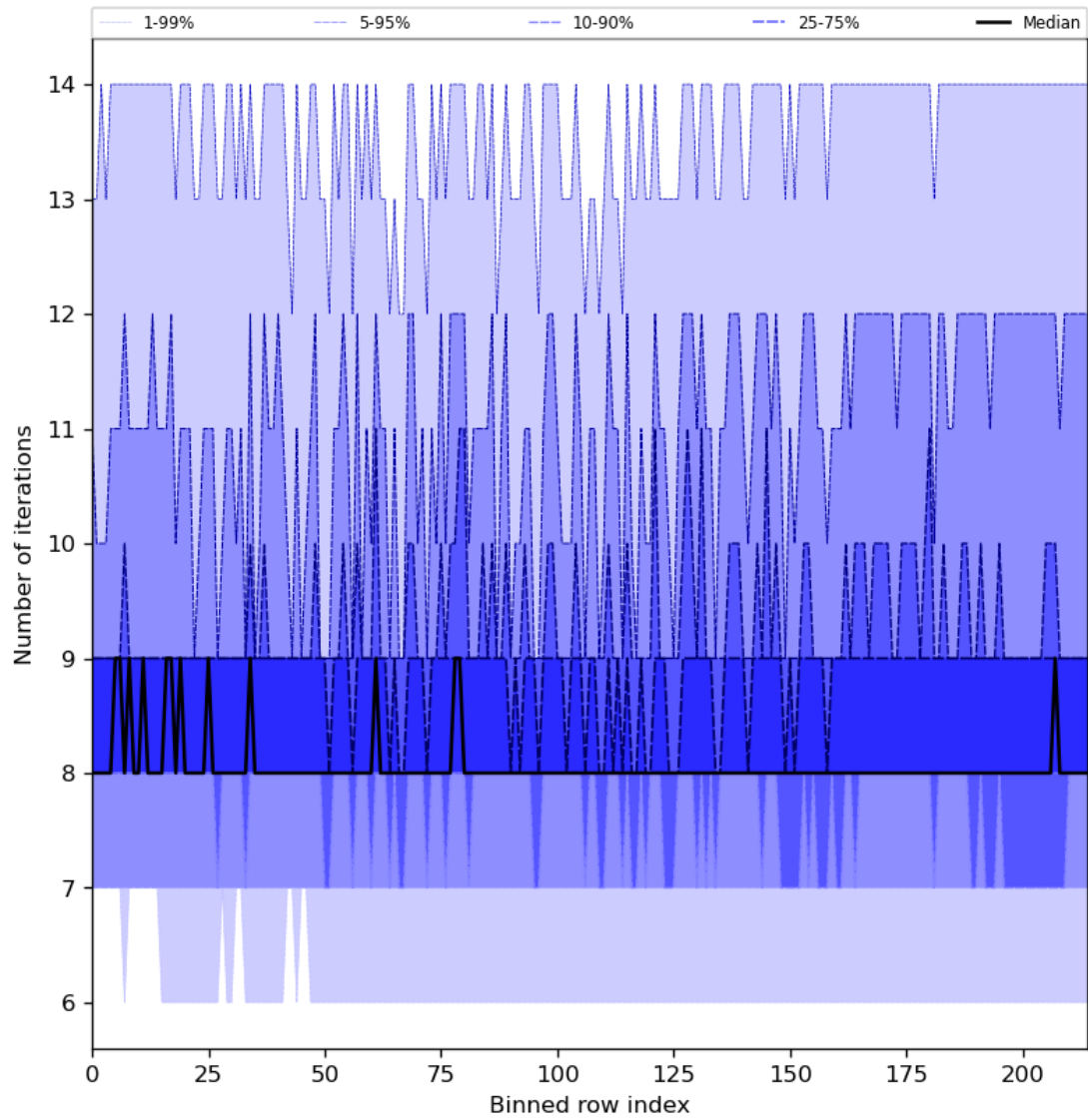
Figure 32: Along track statistics of “Number of iterations” for 2023-09-15 to 2023-09-16
