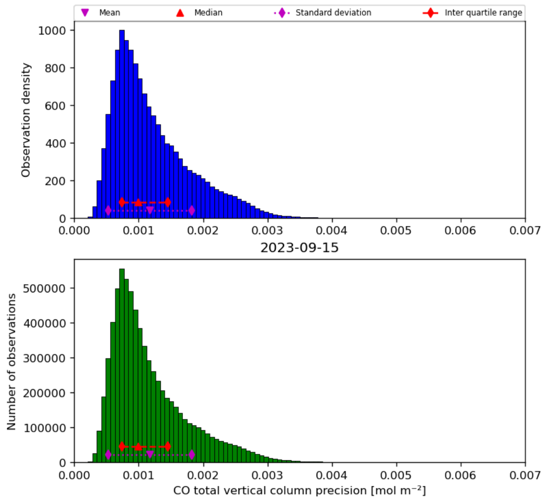
Figure 20: Histogram of “CO total vertical column precision” for 2023-09-15 to 2023-09-16
