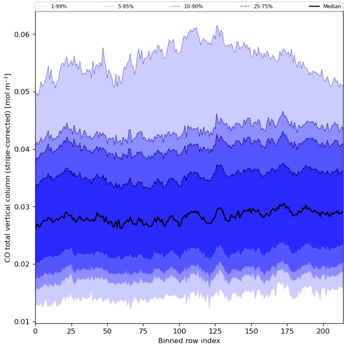
Figure 27: Along track statistics of “CO total vertical column (stripe-corrected)” for 2023-09-15 to 2023-09-16
