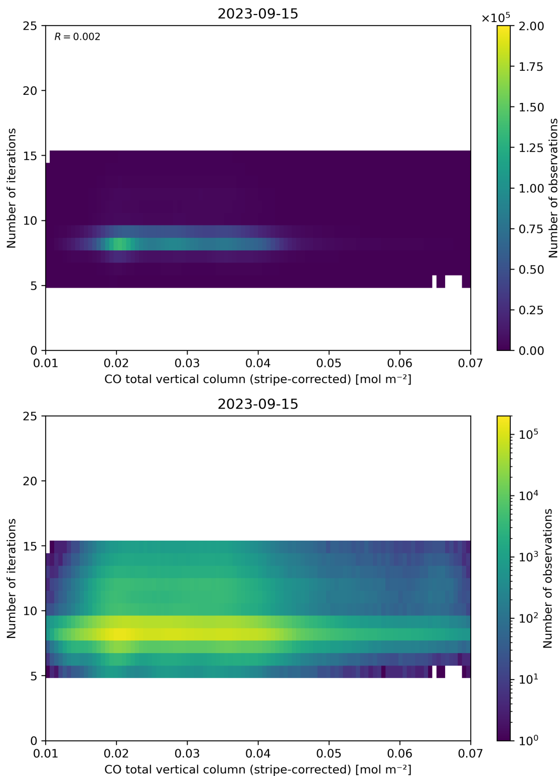
Figure 39: Scatter density plot of “CO total vertical column (stripe-corrected)” against “Number of iterations” for 2023-09-15 to 2023-09-16.
