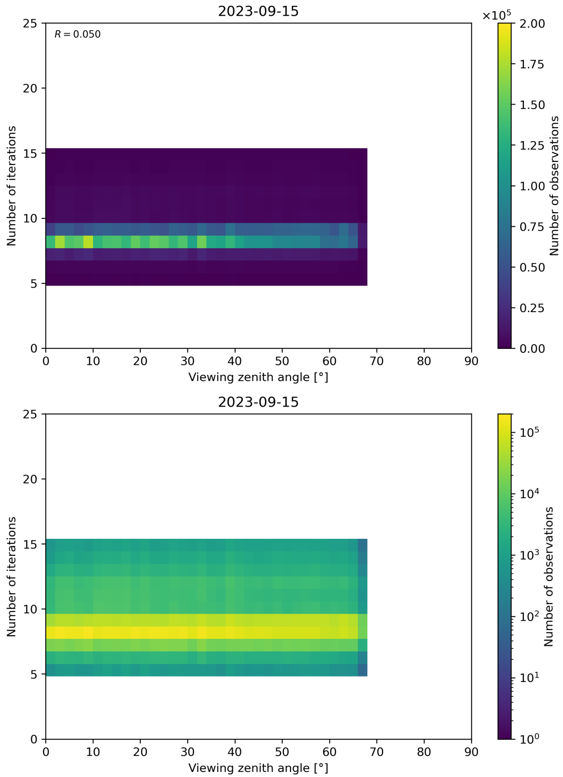
Figure 75: Scatter density plot of “Viewing zenith angle” against “Number of iterations” for 2023-09-15 to 2023-09-16.
