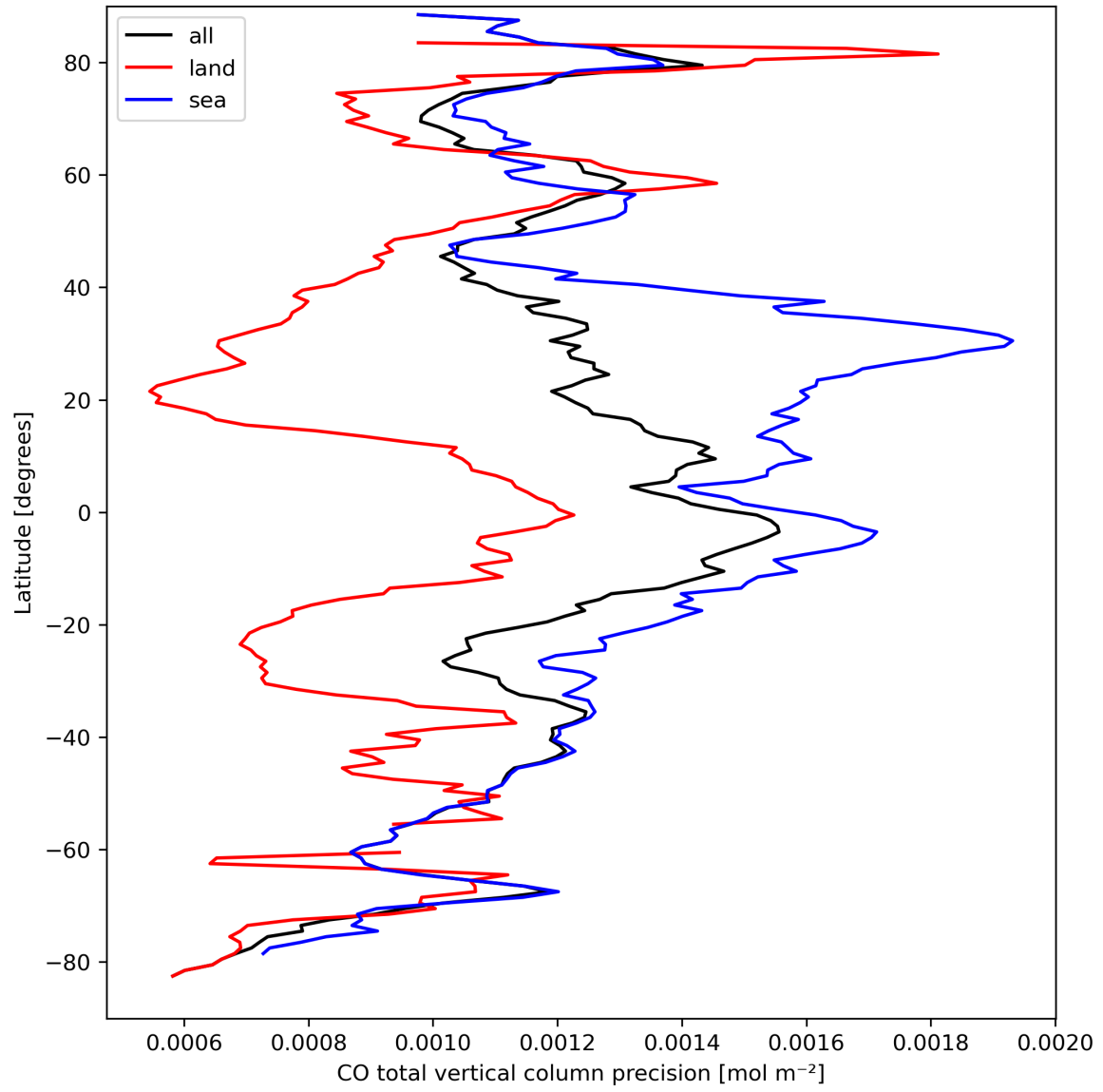
Figure 12: Zonal average of “CO total vertical column precision” for 2023-09-15 to 2023-09-16.
