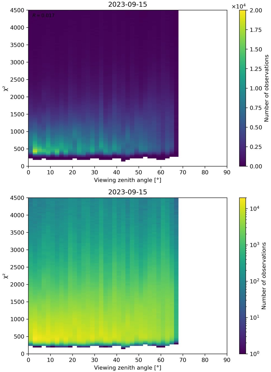
Figure 72: Scatter density plot of “Viewing zenith angle” against “ \chi^2 ” for 2023-09-15 to 2023-09-16.
