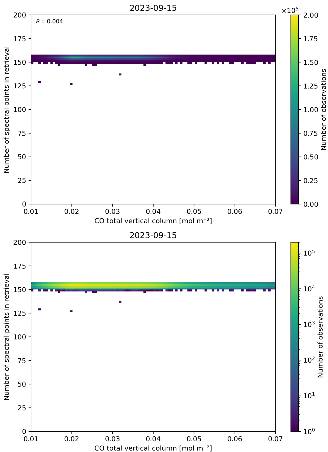
Figure 43: Scatter density plot of “CO total vertical column” against “Number of spectral points in retrieval” for 2023-09-15 to 2023-09-16.
