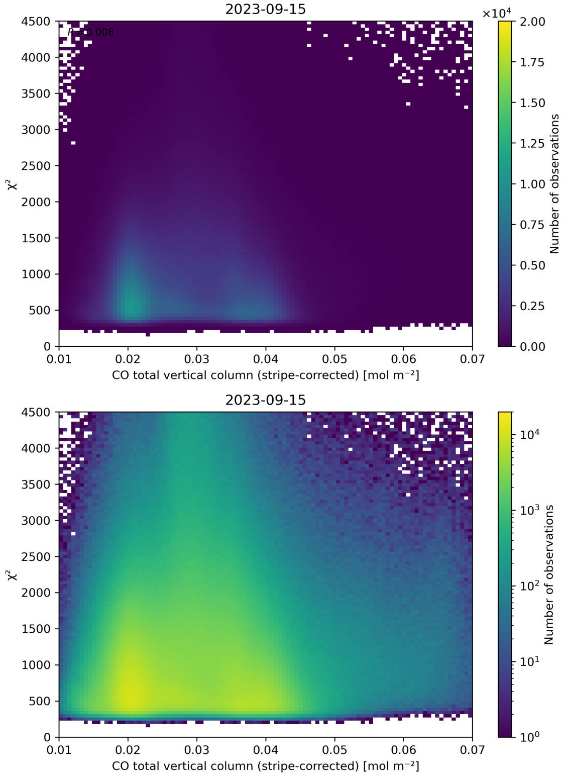
Figure 37: Scatter density plot of “CO total vertical column (stripe-corrected)” against “ \chi^2 ” for 2023-09-15 to 2023-09-16.
