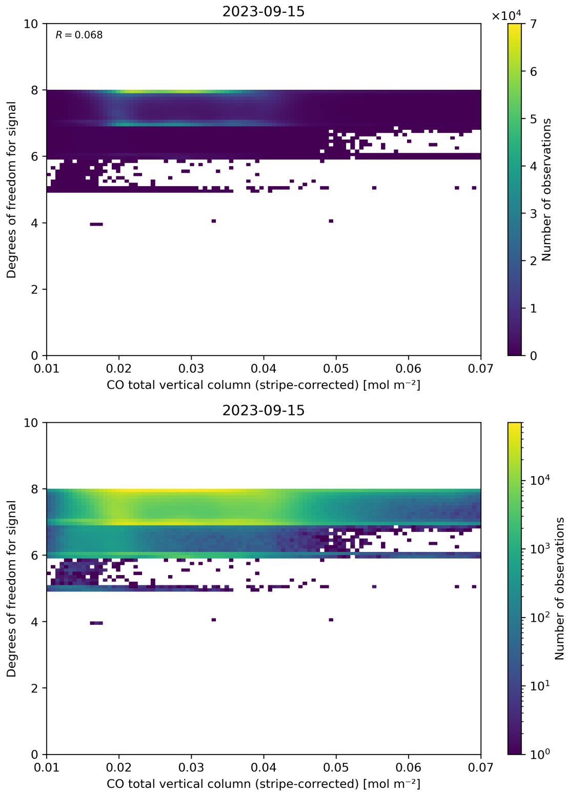
Figure 38: Scatter density plot of “CO total vertical column (stripe-corrected)” against “Degrees of freedom for signal” for 2023-09-15 to 2023-09-16.
