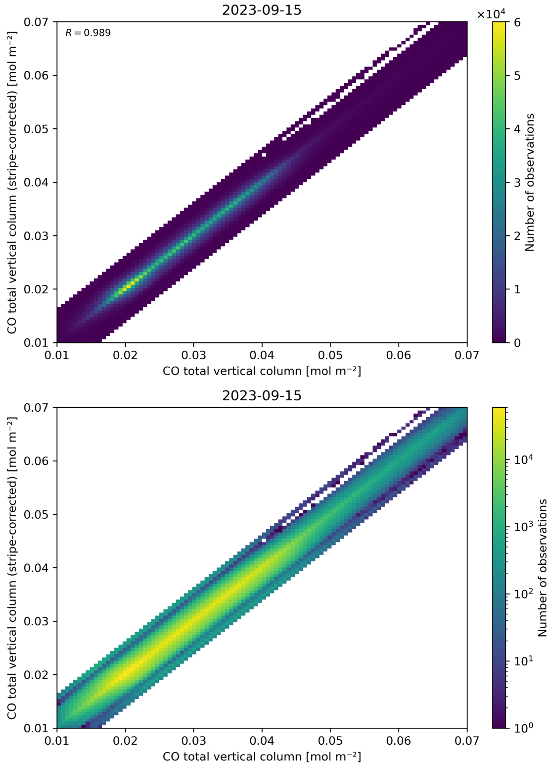
Figure 33: Scatter density plot of “CO total vertical column” against “CO total vertical column (stripe-corrected)” for 2023-09-15 to 2023-09-16.
