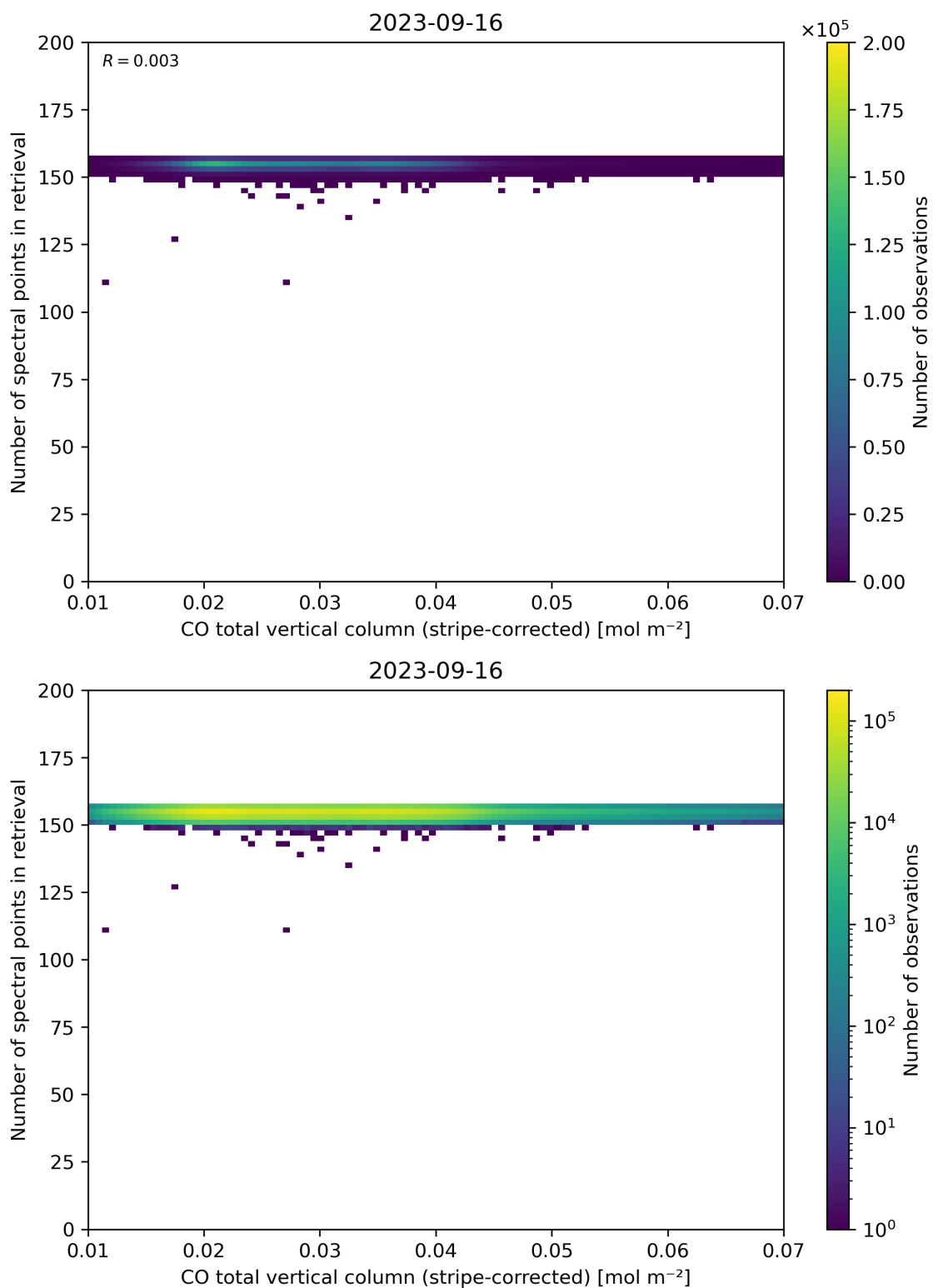
Figure 40: Scatter density plot of “CO total vertical column (stripe-corrected)” against “Number of spectral points in retrieval” for 2023-09-15 to 2023-09-17.
