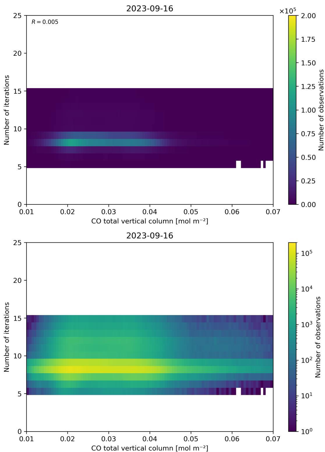
Figure 42: Scatter density plot of “CO total vertical column” against “Number of iterations” for 2023-09-15 to 2023-09-17.
