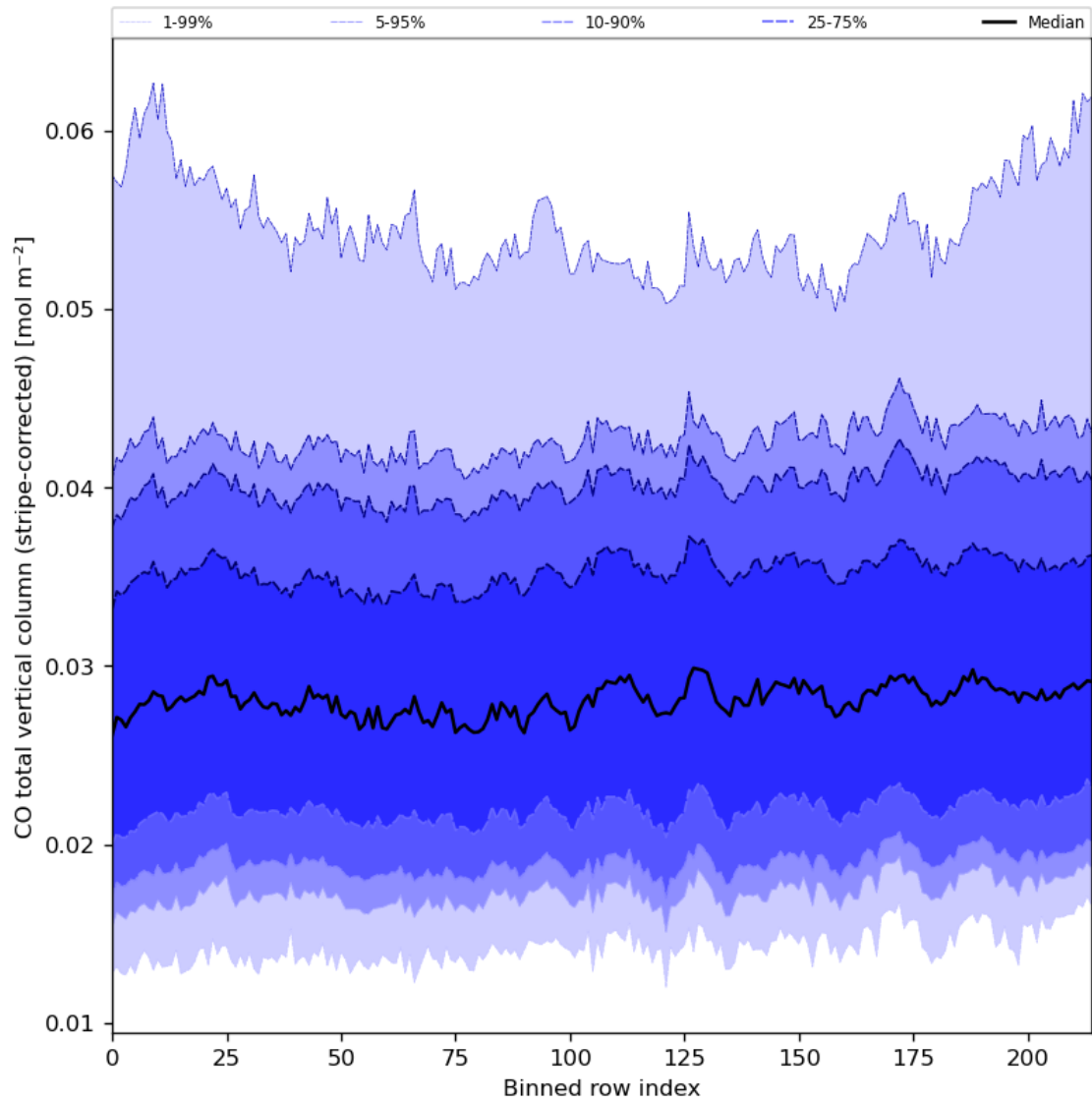
Figure 27: Along track statistics of “CO total vertical column (stripe-corrected)” for 2023-09-15 to 2023-09-17
