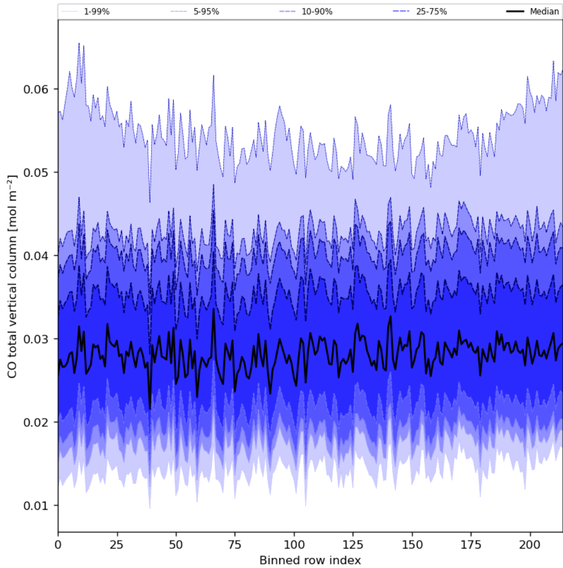
Figure 26: Along track statistics of “CO total vertical column” for 2023-09-15 to 2023-09-17
