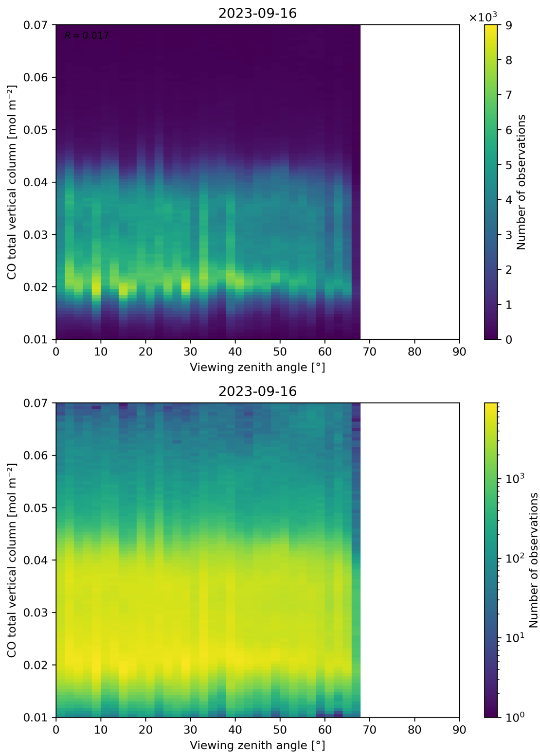
Figure 69: Scatter density plot of “Viewing zenith angle” against “CO total vertical column” for 2023-09-15 to 2023-09-17.
