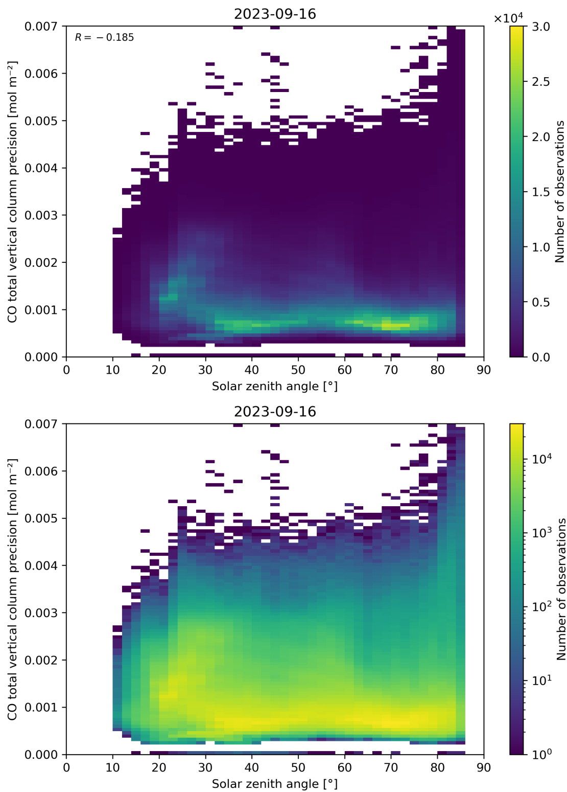
Figure 63: Scatter density plot of “Solar zenith angle” against “CO total vertical column precision” for 2023-09-15 to 2023-09-17.
