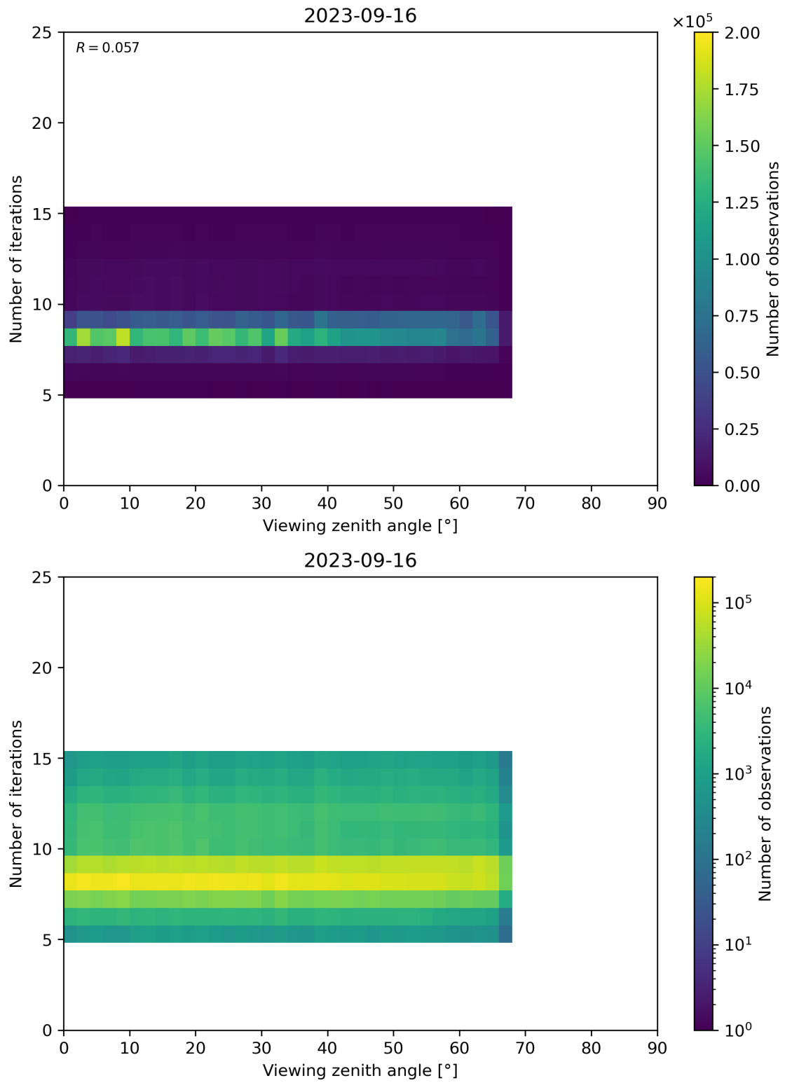
Figure 75: Scatter density plot of “Viewing zenith angle” against “Number of iterations” for 2023-09-15 to 2023-09-17.
