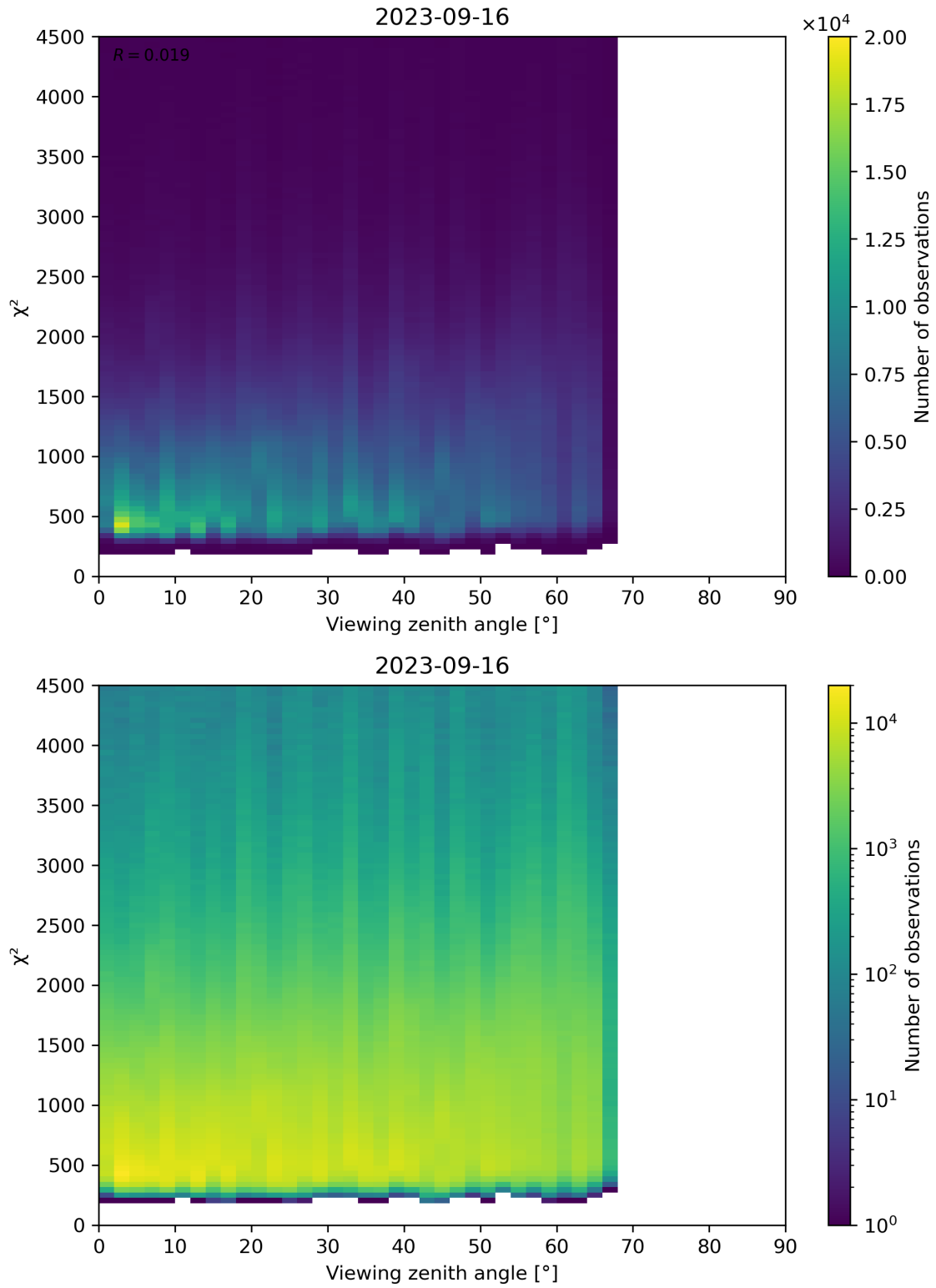
Figure 72: Scatter density plot of “Viewing zenith angle” against “ \chi^2 ” for 2023-09-15 to 2023-09-17.
