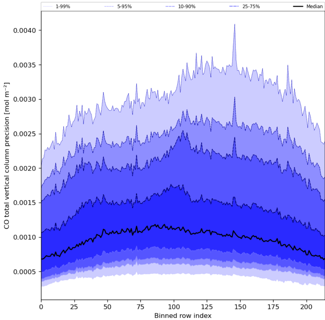
Figure 28: Along track statistics of “CO total vertical column precision” for 2023-09-15 to 2023-09-17
