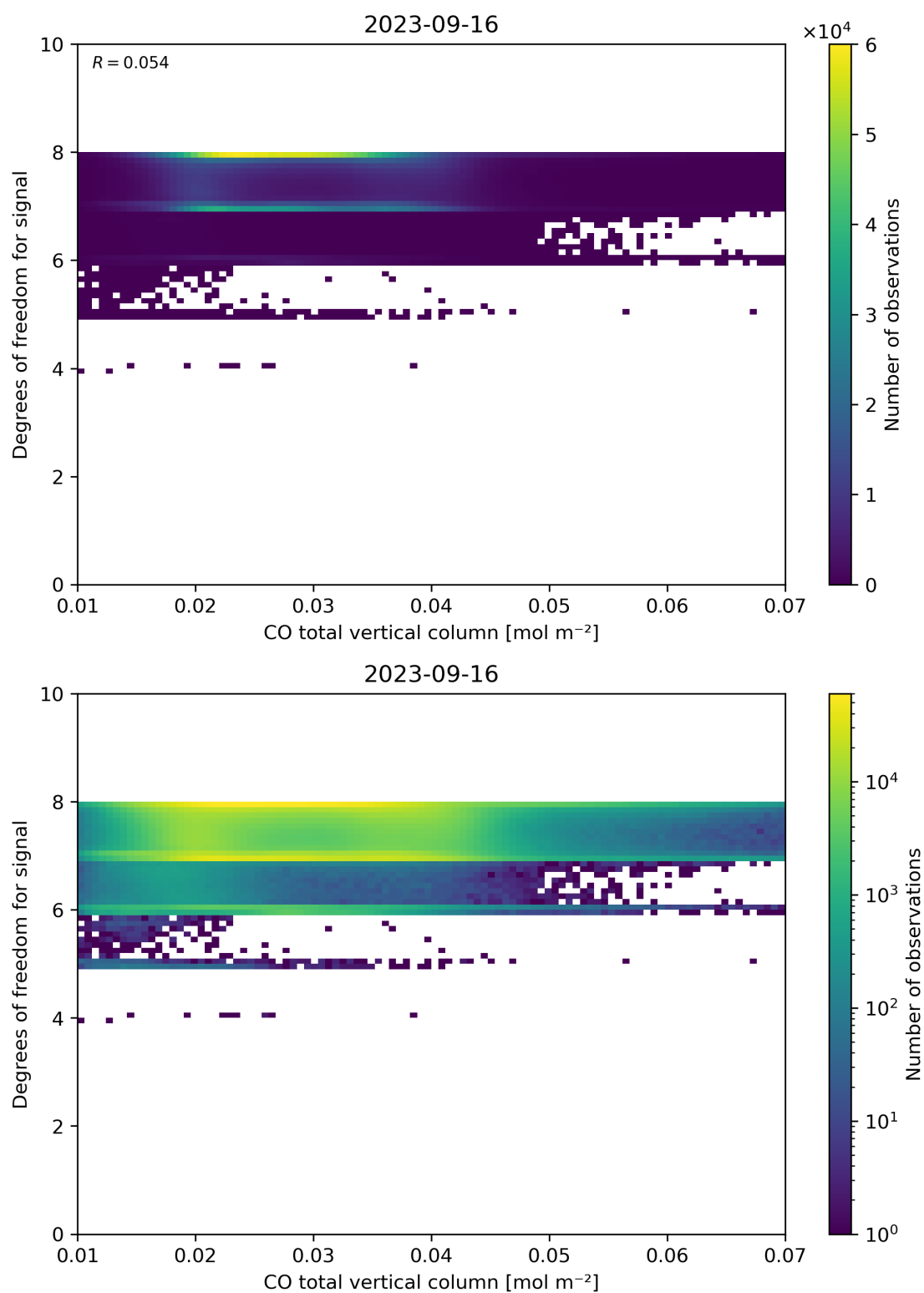
Figure 41: Scatter density plot of “CO total vertical column” against “Degrees of freedom for signal” for 2023-09-15 to 2023-09-17.
