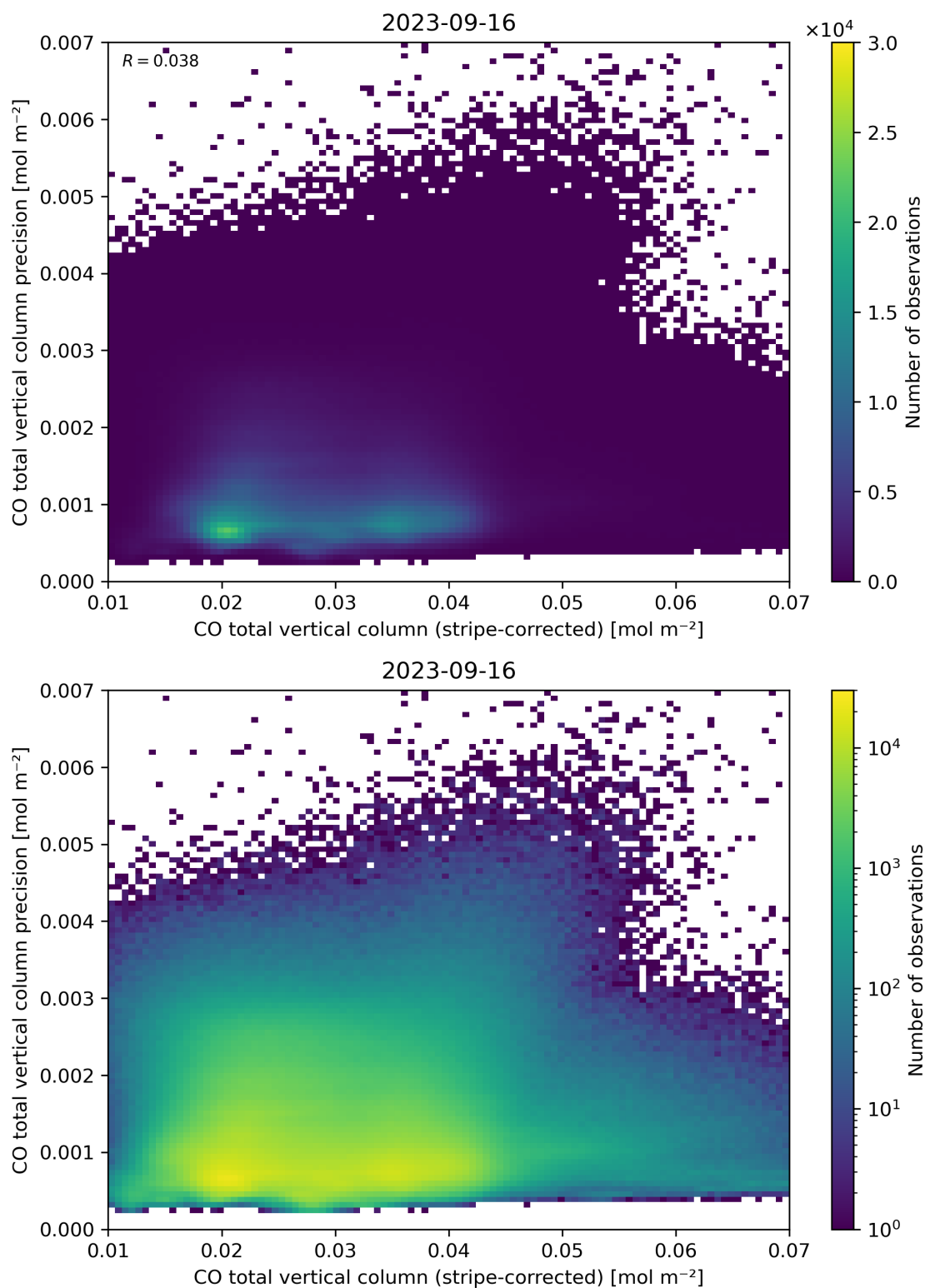
Figure 36: Scatter density plot of “CO total vertical column (stripe-corrected)” against “CO total vertical column precision” for 2023-09-15 to 2023-09-17.
