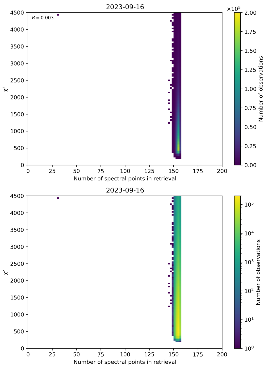
Figure 58: Scatter density plot of “Number of spectral points in retrieval” against “ \chi^2 ” for 2023-09-15 to 2023-09-17.
