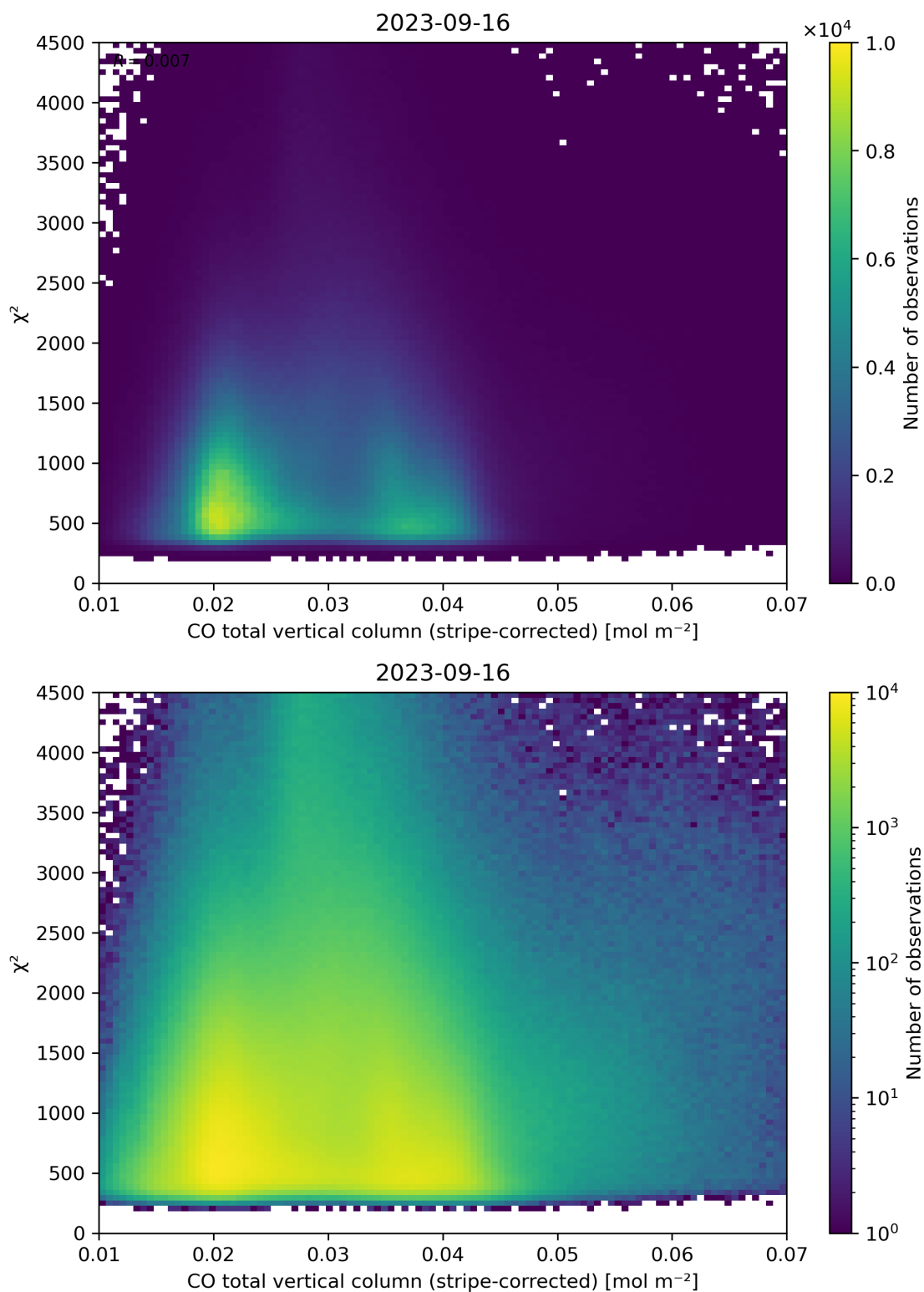
Figure 37: Scatter density plot of “CO total vertical column (stripe-corrected)” against “ \chi^2 ” for 2023-09-15 to 2023-09-17.
