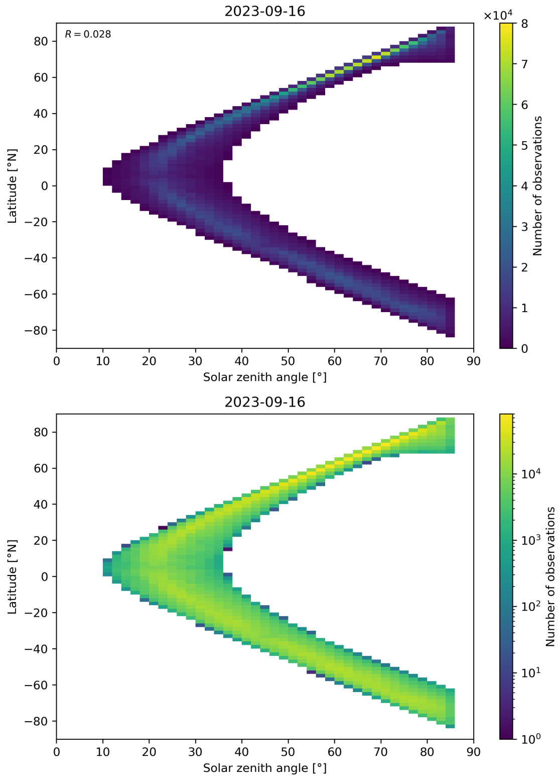
Figure 66: Scatter density plot of “Solar zenith angle” against “Latitude” for 2023-09-15 to 2023-09-17.
