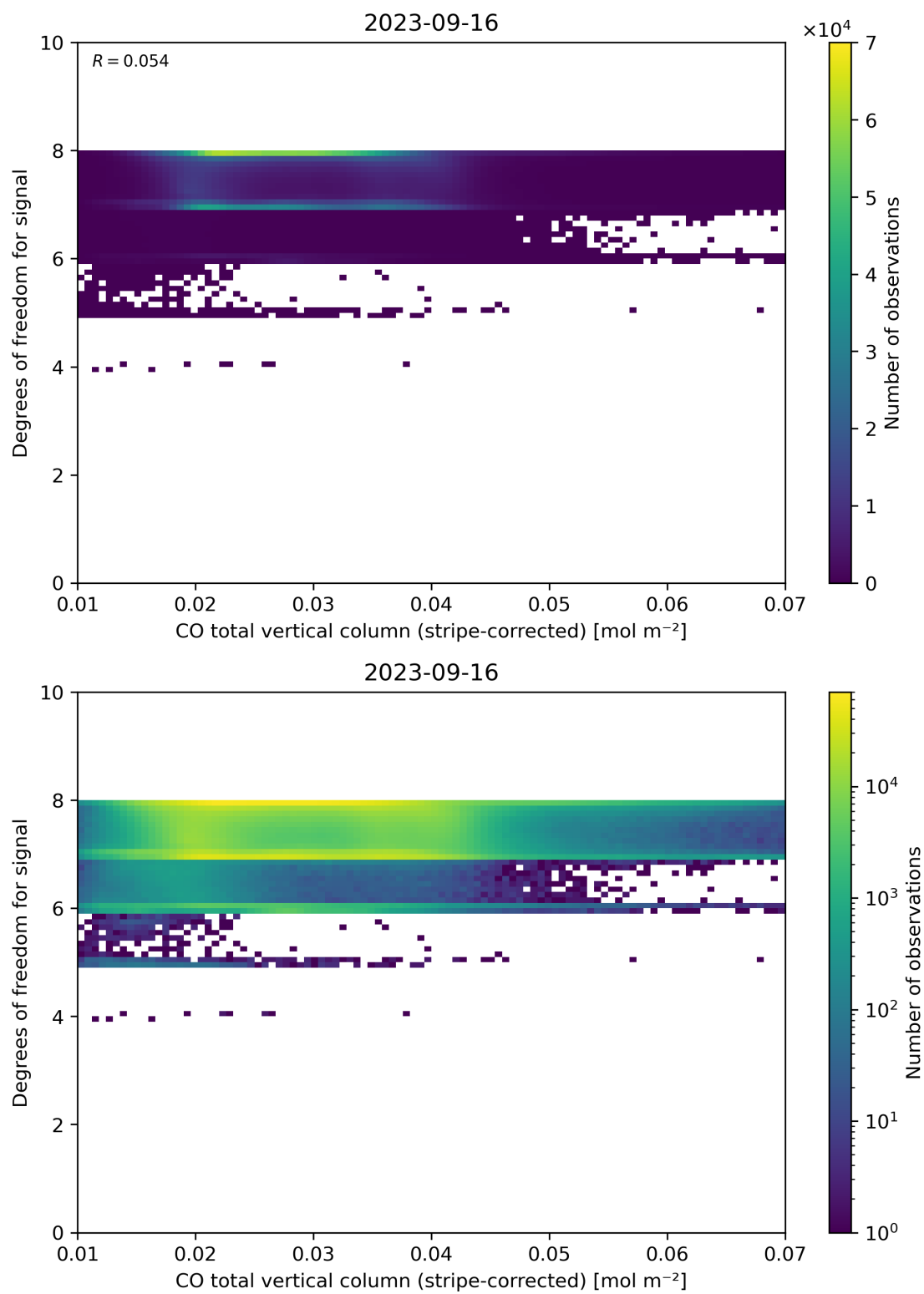
Figure 38: Scatter density plot of “CO total vertical column (stripe-corrected)” against “Degrees of freedom for signal” for 2023-09-15 to 2023-09-17.
