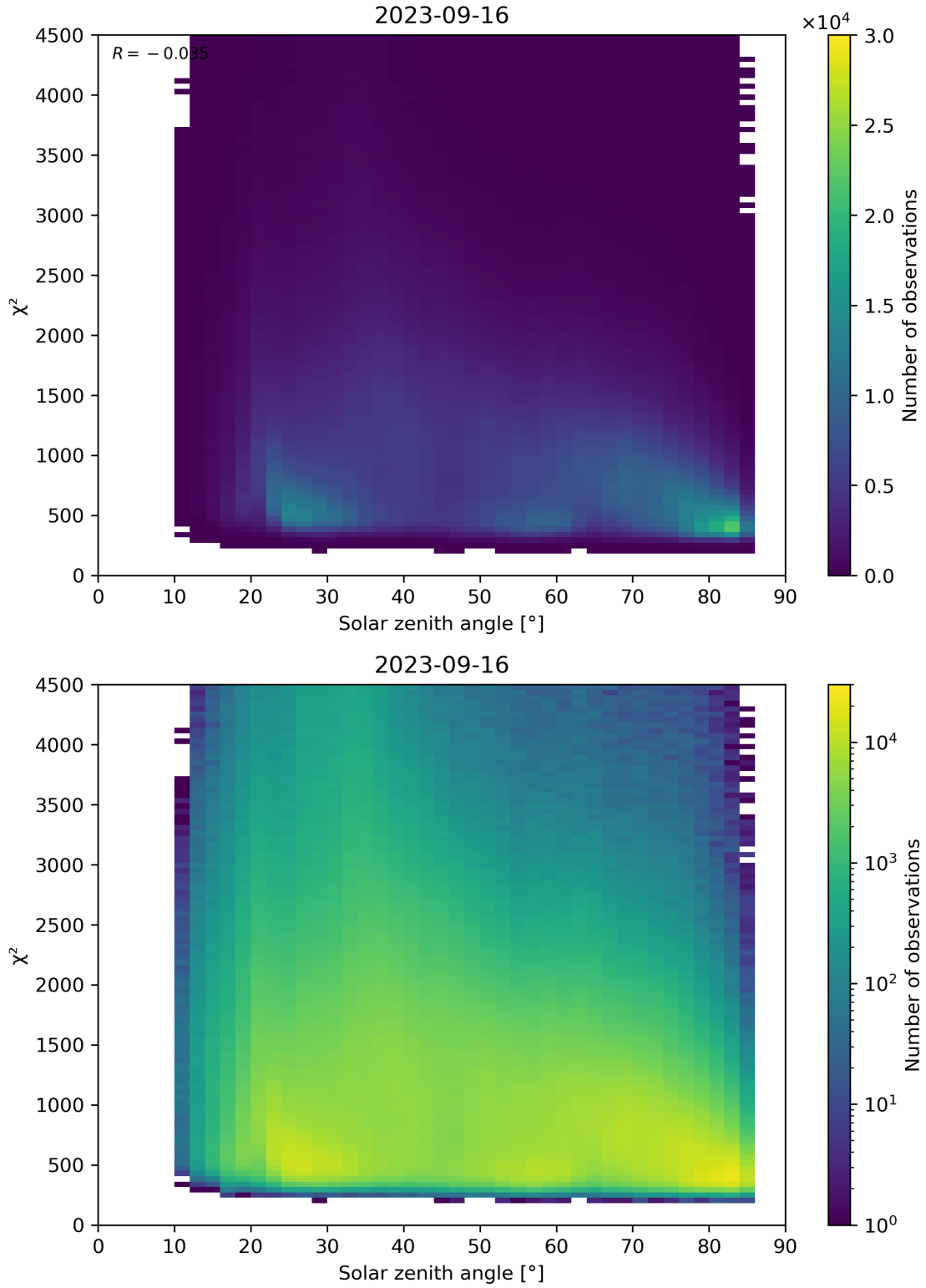
Figure 64: Scatter density plot of “Solar zenith angle” against “ \chi^2 ” for 2023-09-15 to 2023-09-17.
