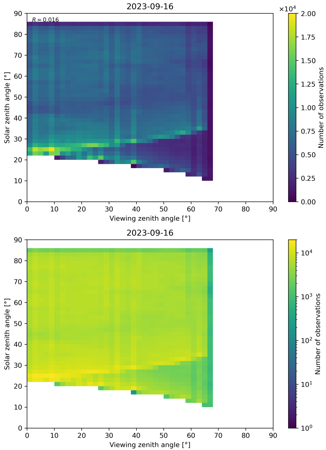
Figure 77: Scatter density plot of “Viewing zenith angle” against “Solar zenith angle” for 2023-09-15 to 2023-09-17.
