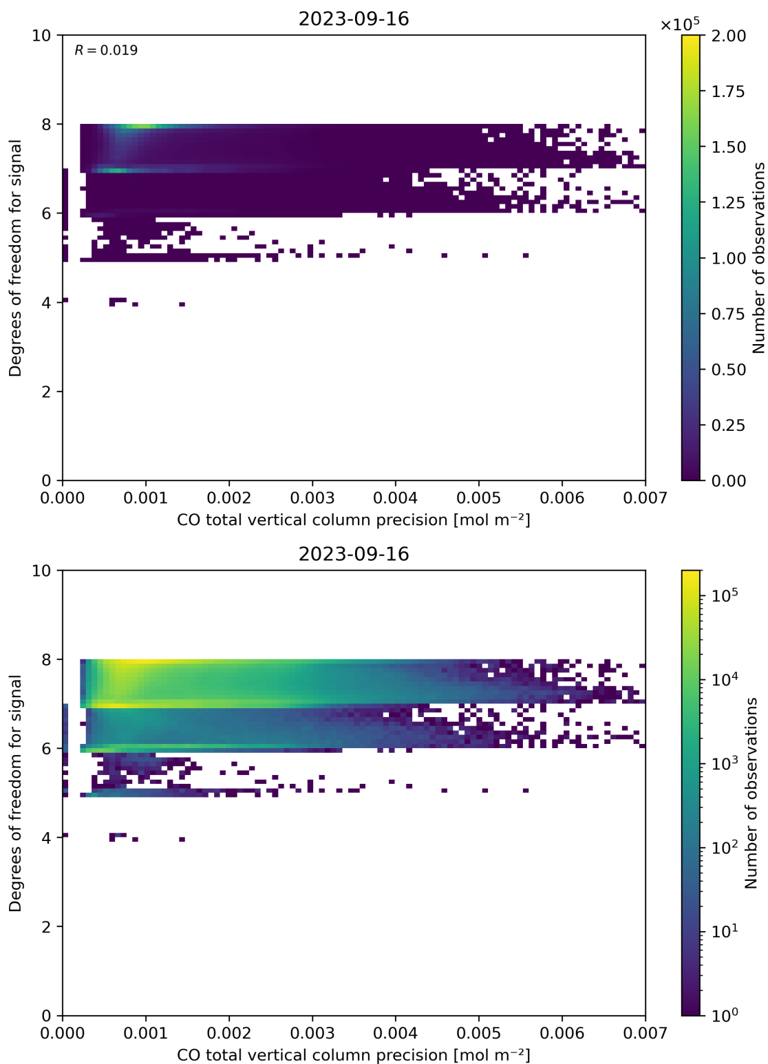
Figure 45: Scatter density plot of “CO total vertical column precision” against “Degrees of freedom for signal” for 2023-09-15 to 2023-09-17.
