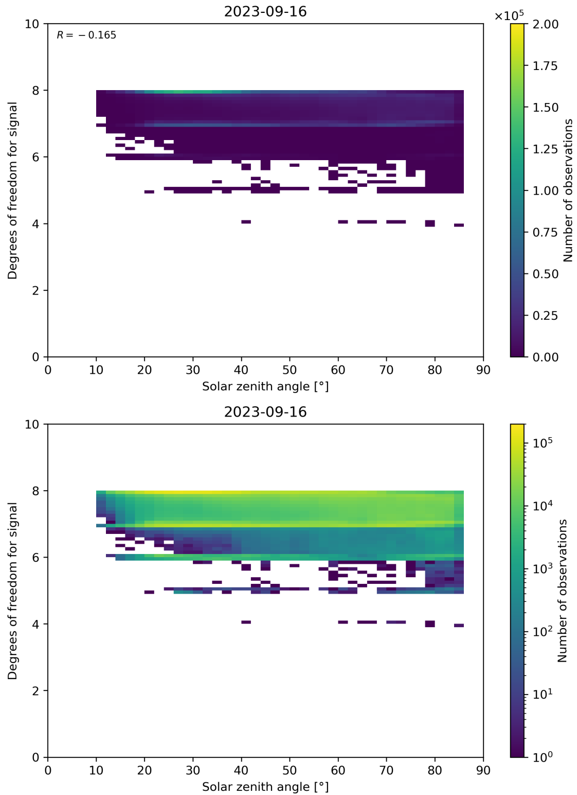
Figure 65: Scatter density plot of “Solar zenith angle” against “Degrees of freedom for signal” for 2023-09-15 to 2023-09-17.
