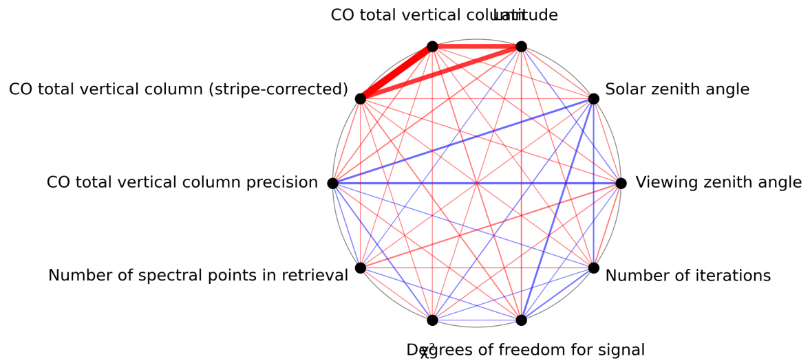
Figure 1: Map of correlation graph for 2023-09-15 to 2023-09-17.
