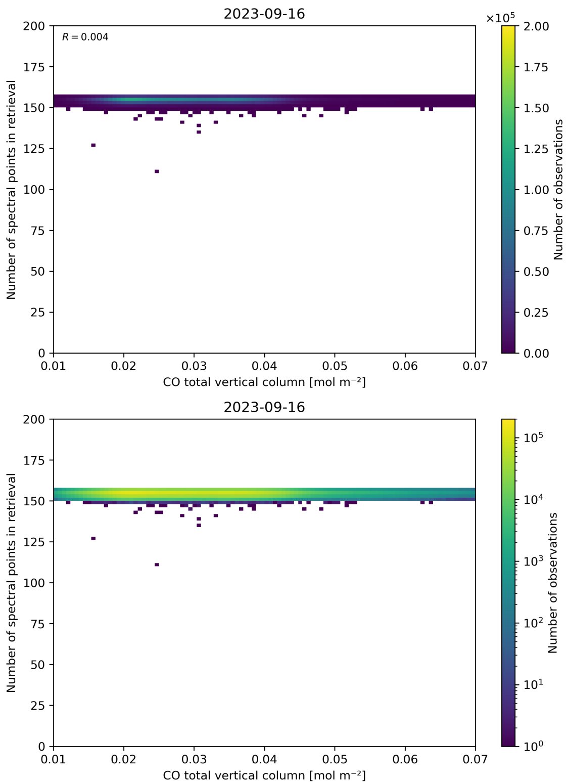
Figure 43: Scatter density plot of “CO total vertical column” against “Number of spectral points in retrieval” for 2023-09-15 to 2023-09-17.
