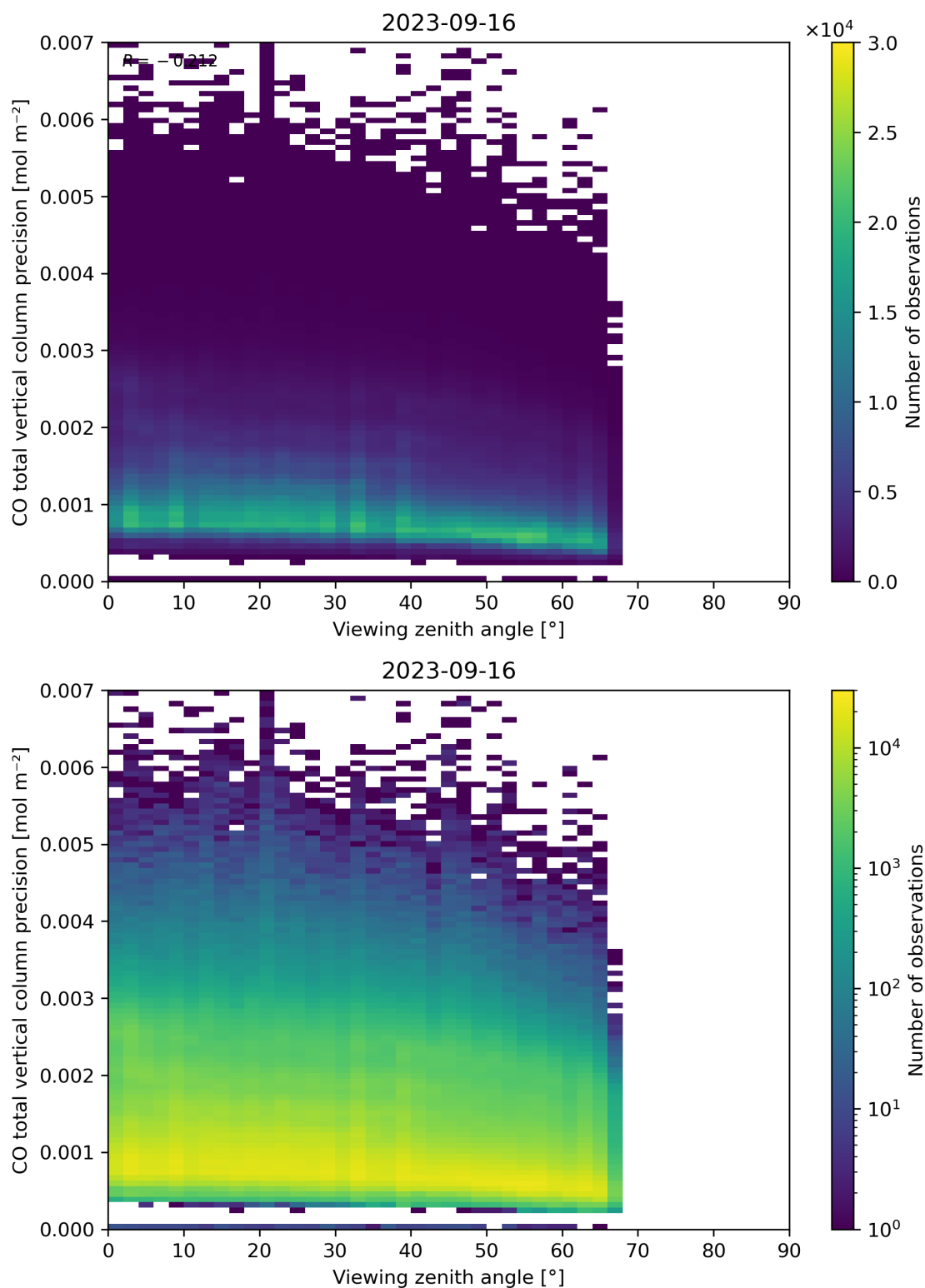
Figure 71: Scatter density plot of “Viewing zenith angle” against “CO total vertical column precision” for 2023-09-15 to 2023-09-17.
