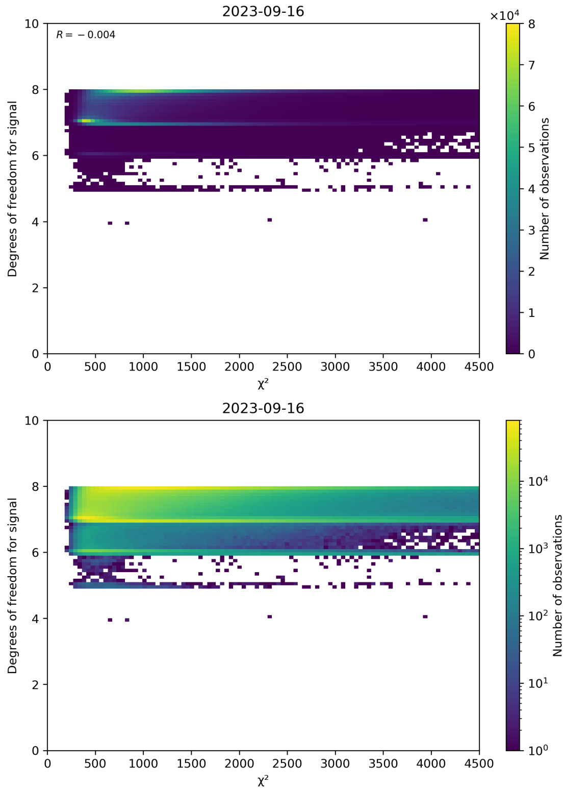
Figure 48: Scatter density plot of “ \chi^2 ” against “Degrees of freedom for signal” for 2023-09-15 to 2023-09-17.
