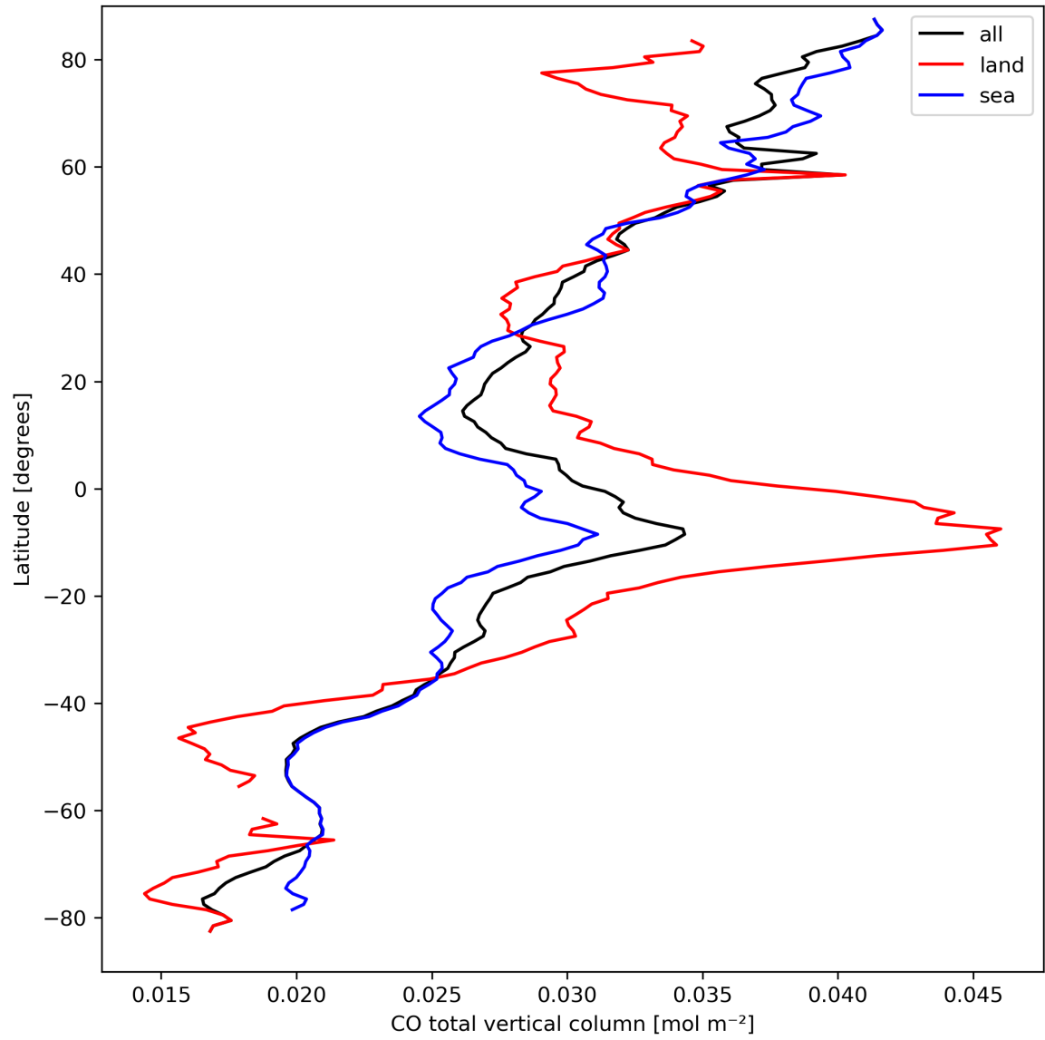
Figure 10: Zonal average of “CO total vertical column” for 2023-09-15 to 2023-09-17.
