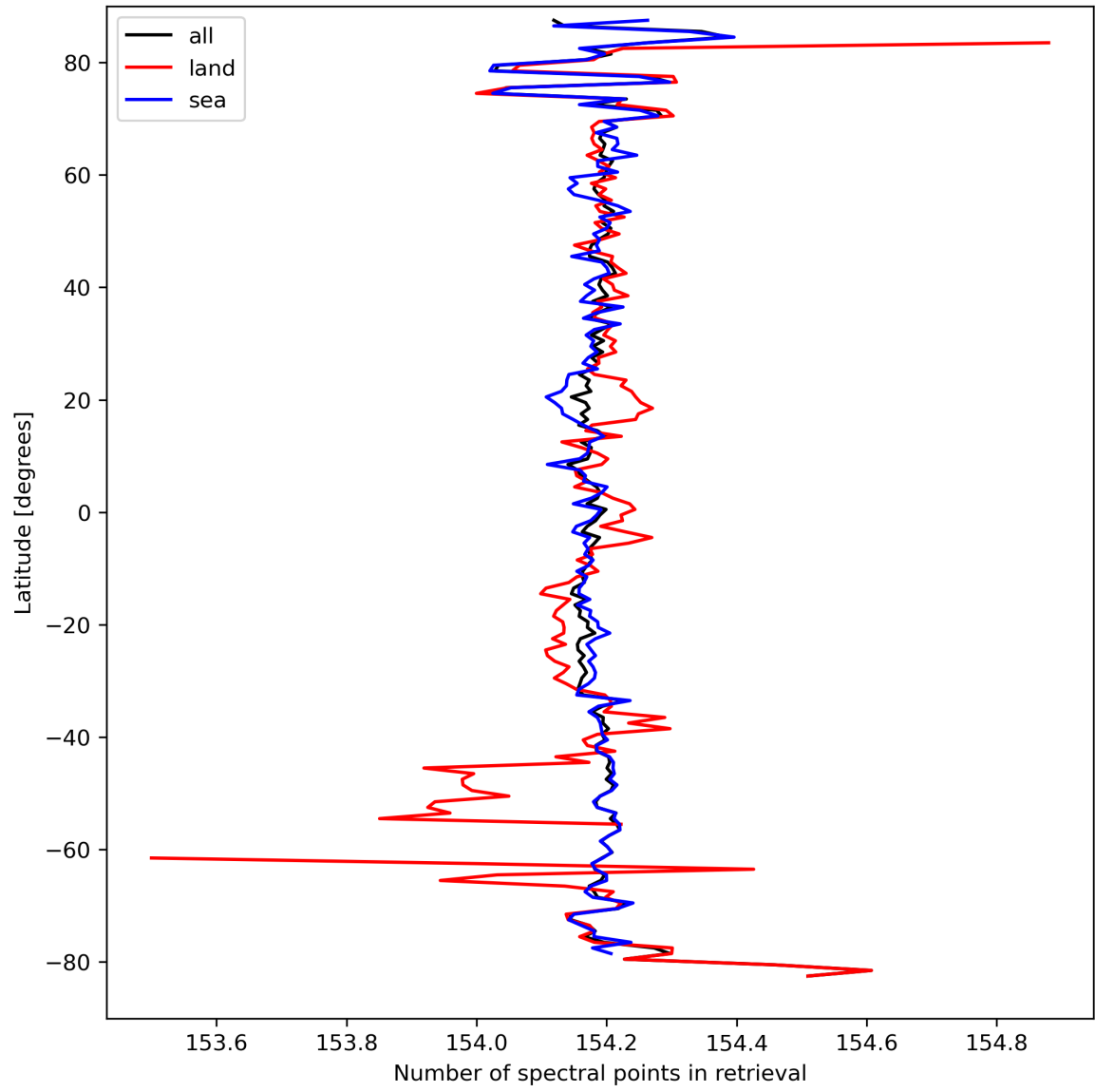
Figure 13: Zonal average of “Number of spectral points in retrieval” for 2023-09-15 to 2023-09-17.
