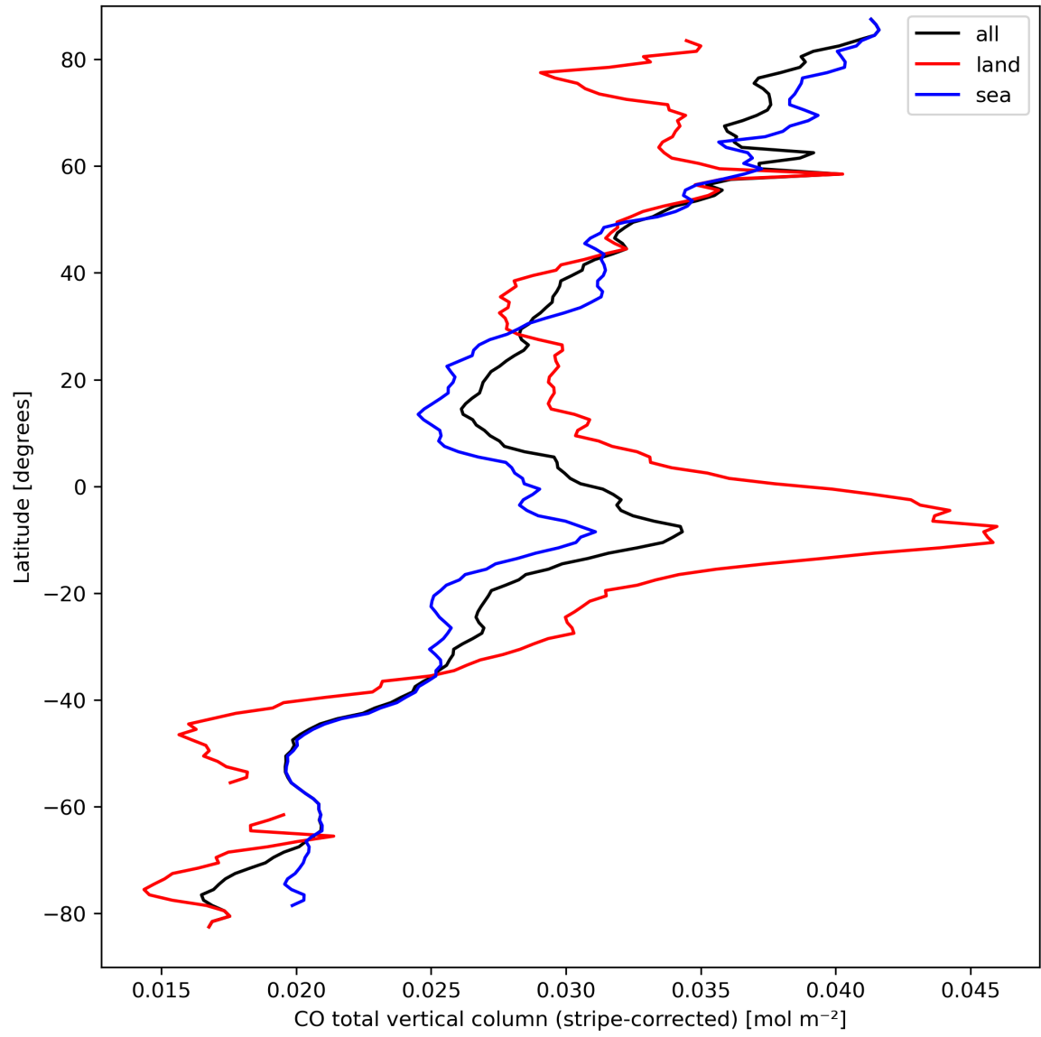
Figure 11: Zonal average of “CO total vertical column (stripe-corrected)” for 2023-09-15 to 2023-09-17.
