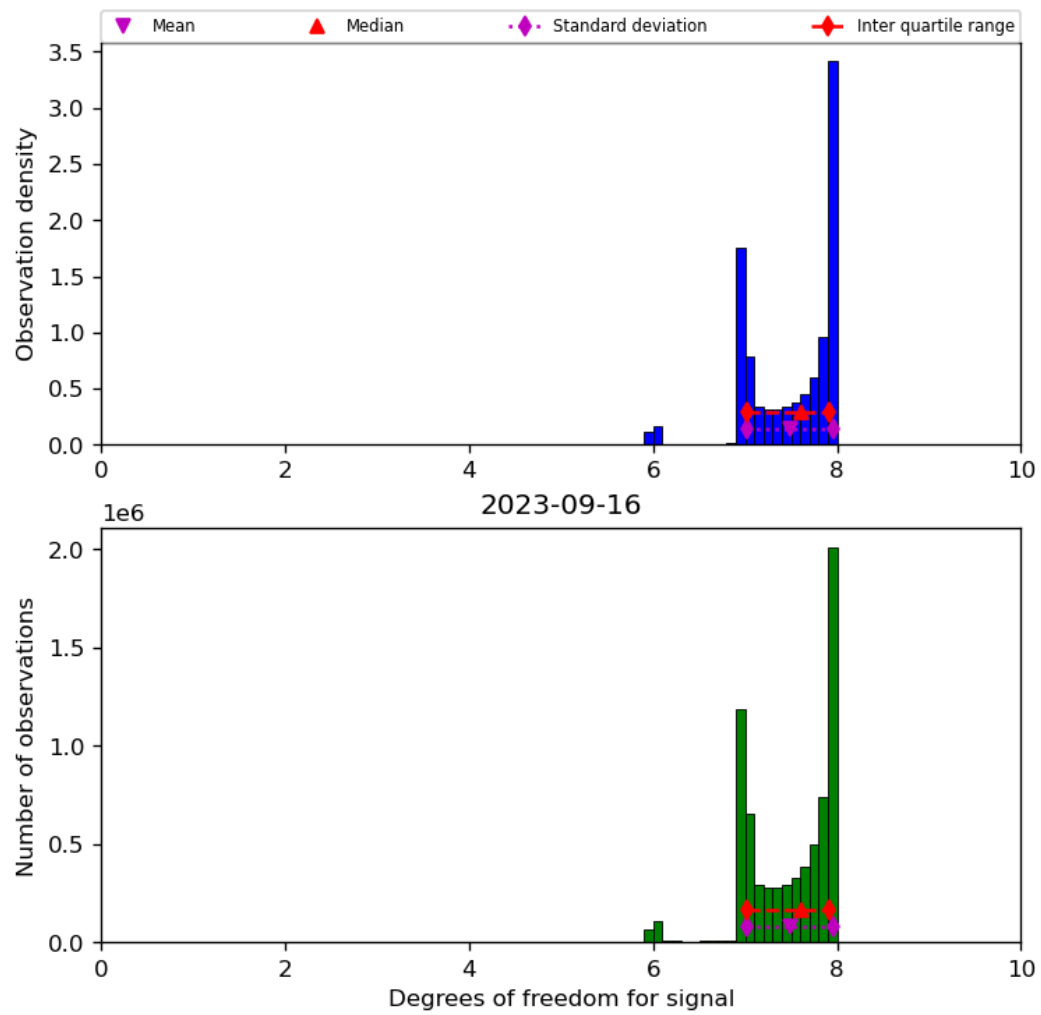
Figure 23: Histogram of “Degrees of freedom for signal” for 2023-09-15 to 2023-09-17
