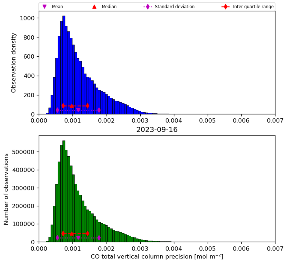
Figure 20: Histogram of “CO total vertical column precision” for 2023-09-15 to 2023-09-17
