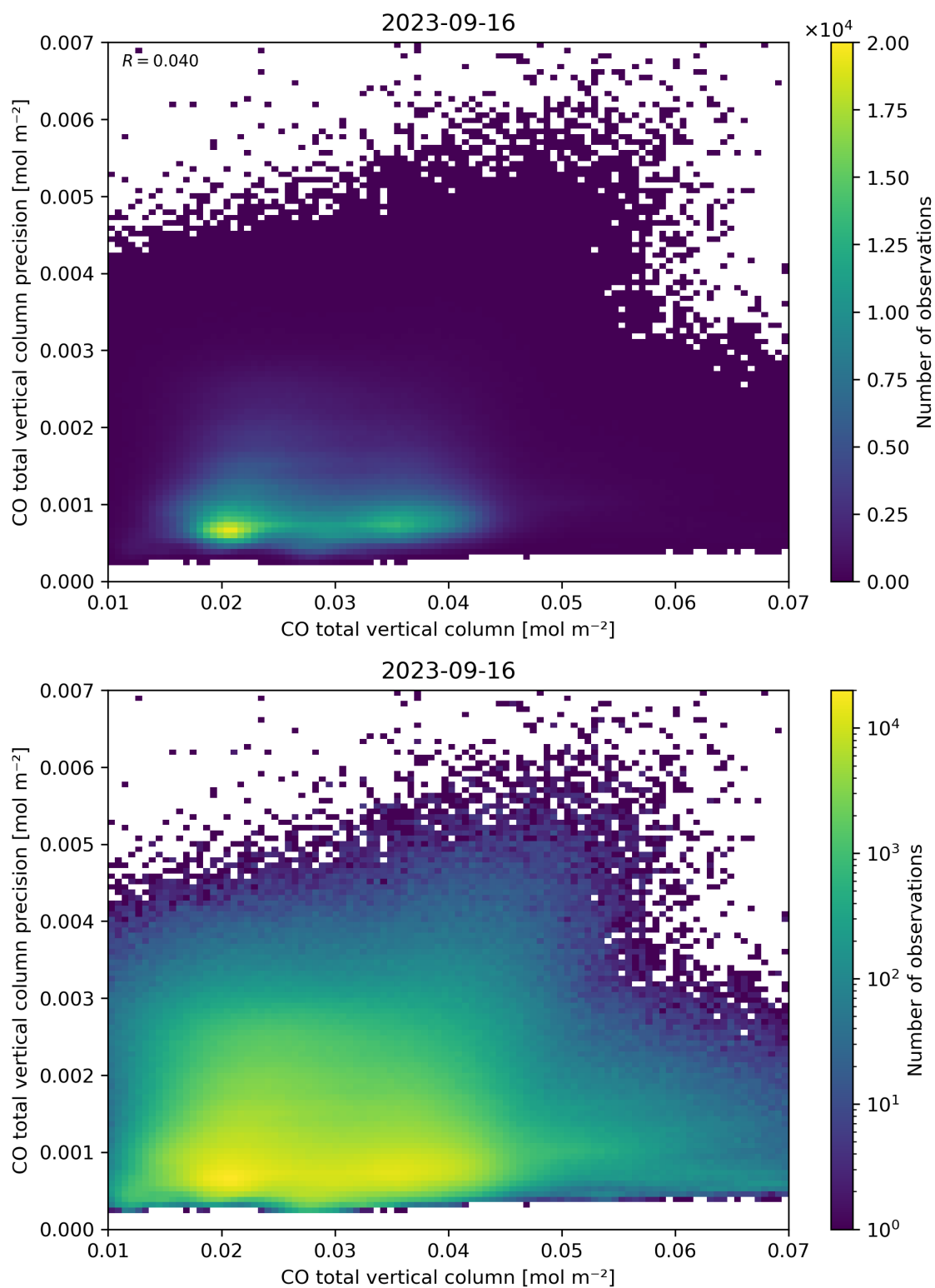
Figure 34: Scatter density plot of “CO total vertical column” against “CO total vertical column precision” for 2023-09-15 to 2023-09-17.
