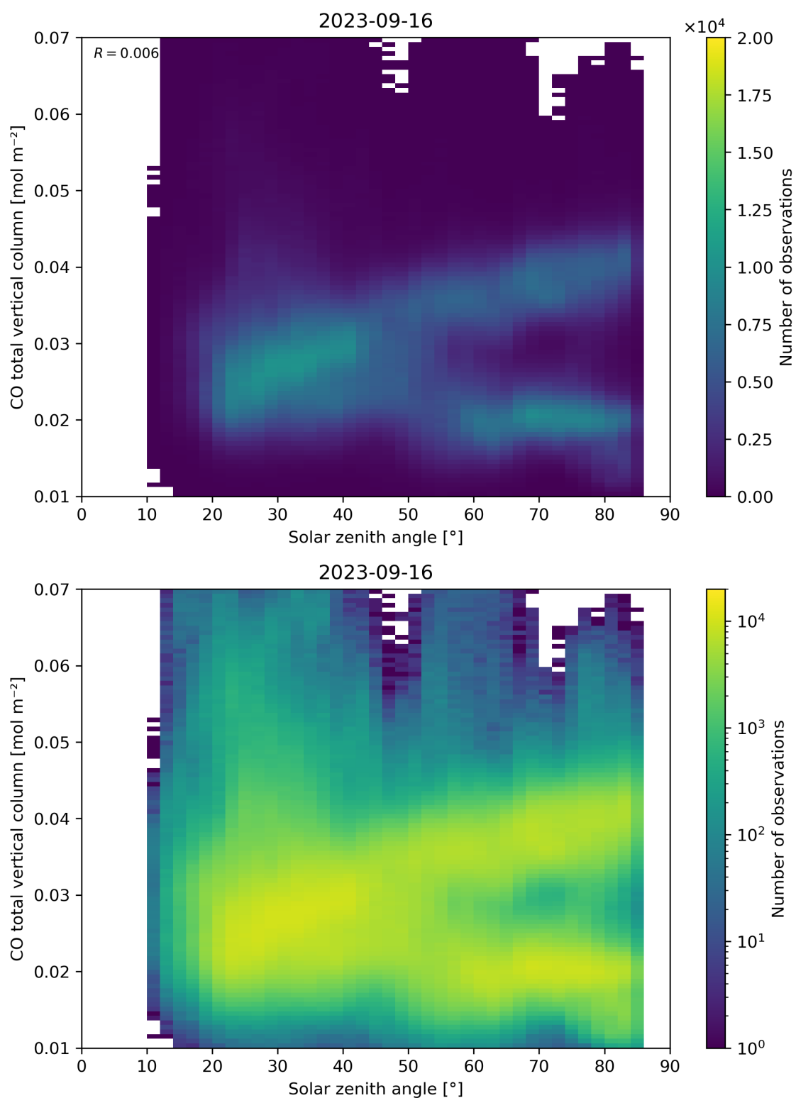
Figure 61: Scatter density plot of “Solar zenith angle” against “CO total vertical column” for 2023-09-15 to 2023-09-17.
