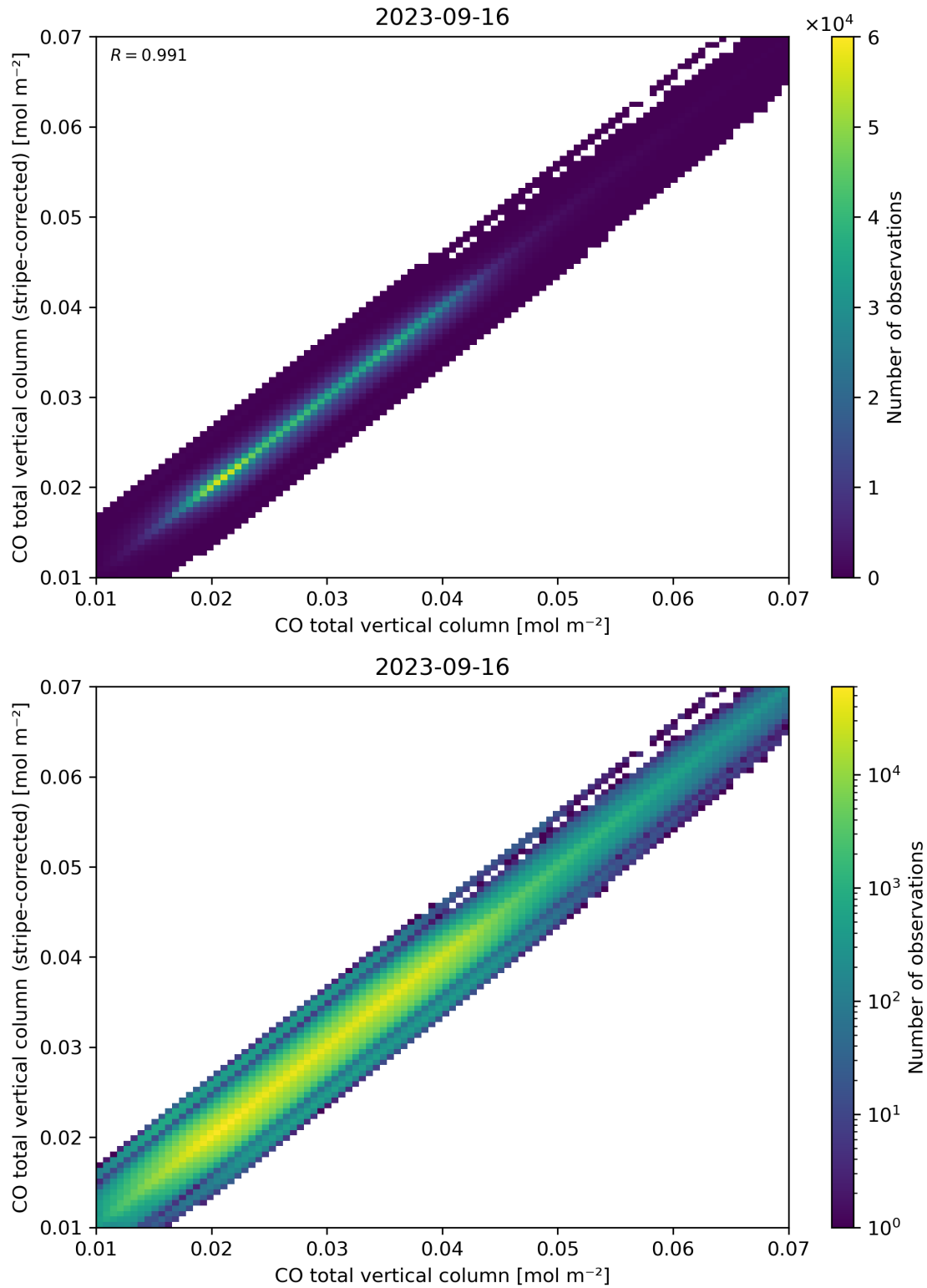
Figure 33: Scatter density plot of “CO total vertical column” against “CO total vertical column (stripe-corrected)” for 2023-09-15 to 2023-09-17.
