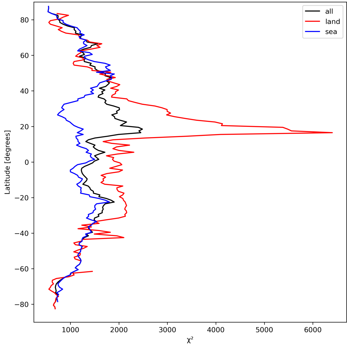
Figure 14: Zonal average of “ \chi^2 ” for 2023-09-15 to 2023-09-17.
