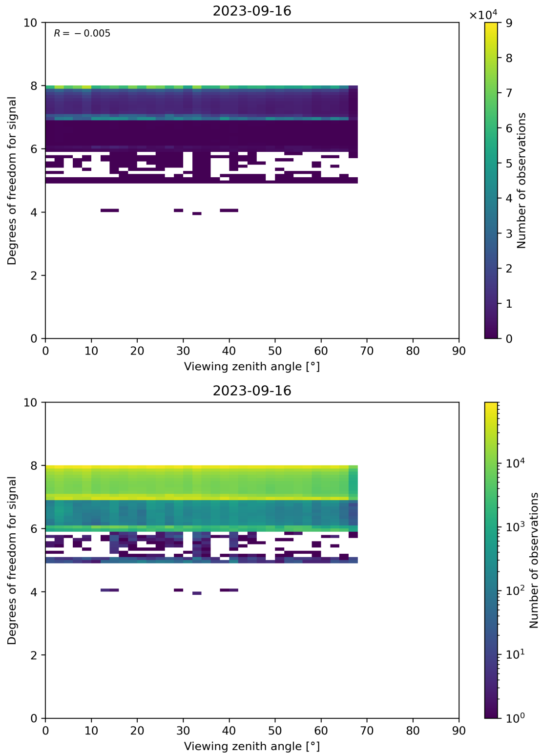
Figure 73: Scatter density plot of “Viewing zenith angle” against “Degrees of freedom for signal” for 2023-09-15 to 2023-09-17.
