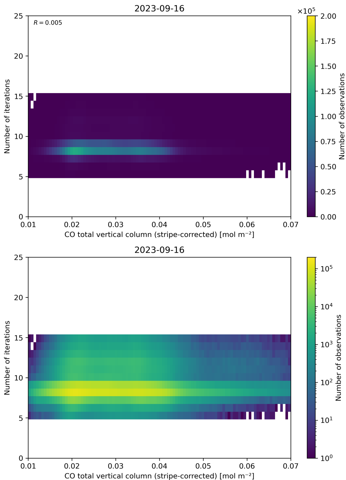
Figure 39: Scatter density plot of “CO total vertical column (stripe-corrected)” against “Number of iterations” for 2023-09-15 to 2023-09-17.
