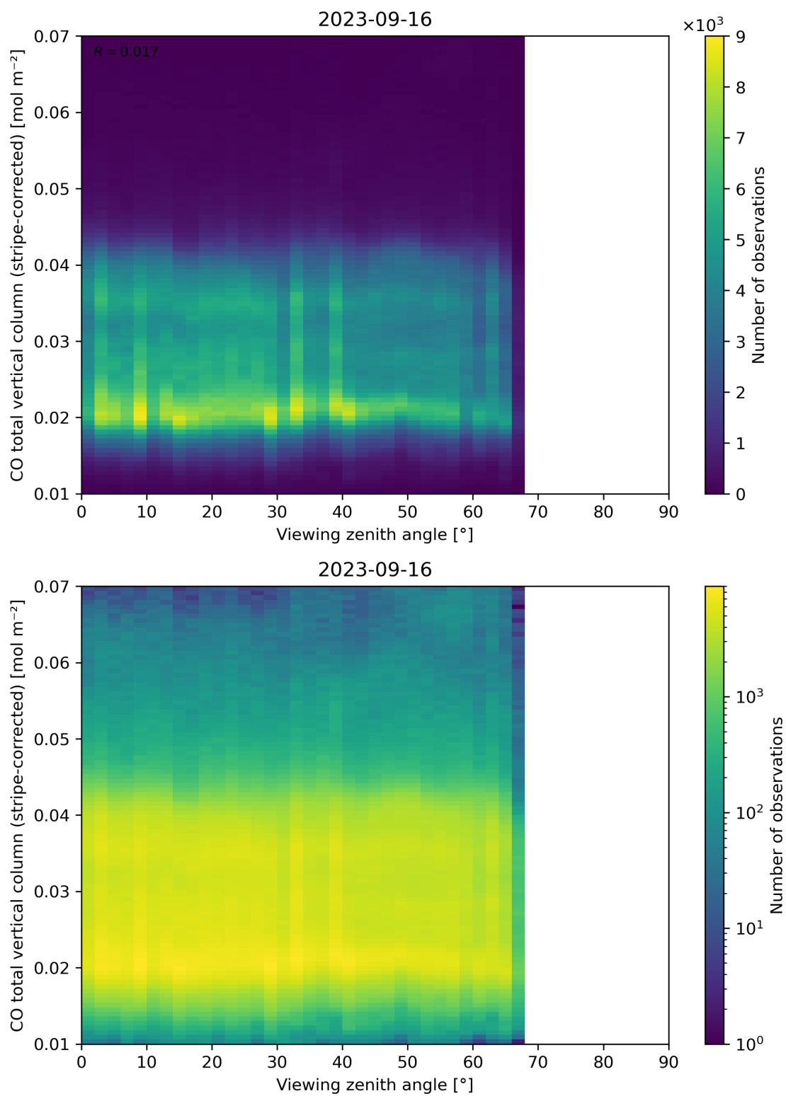
Figure 70: Scatter density plot of “Viewing zenith angle” against “CO total vertical column (stripe-corrected)” for 2023-09-15 to 2023-09-17.
