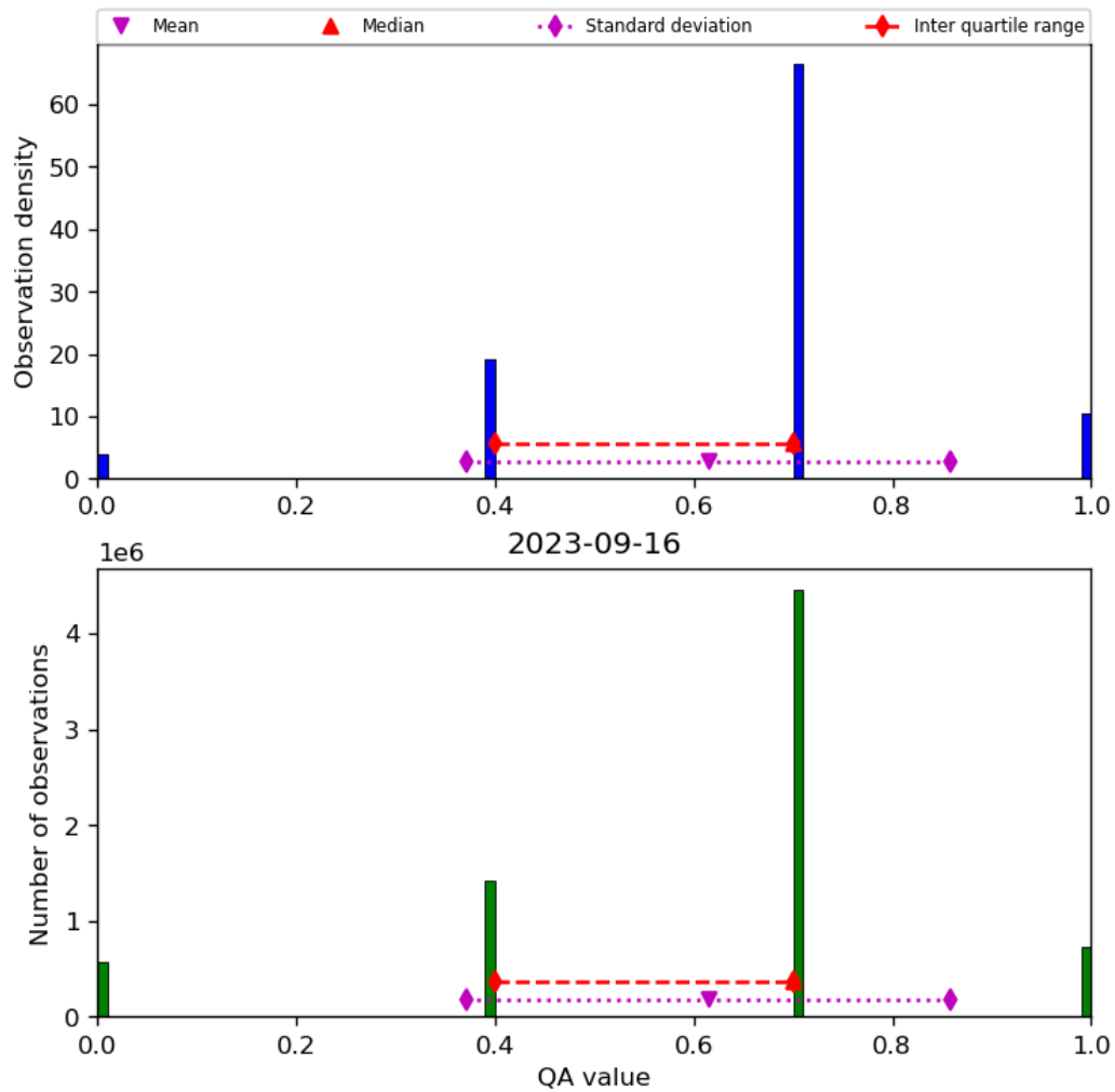
Figure 17: Histogram of “QA value” for 2023-09-15 to 2023-09-17
