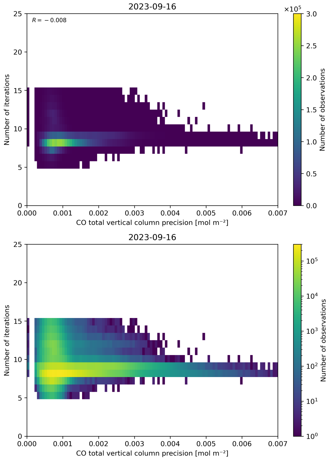
Figure 46: Scatter density plot of “CO total vertical column precision” against “Number of iterations” for 2023-09-15 to 2023-09-17.
