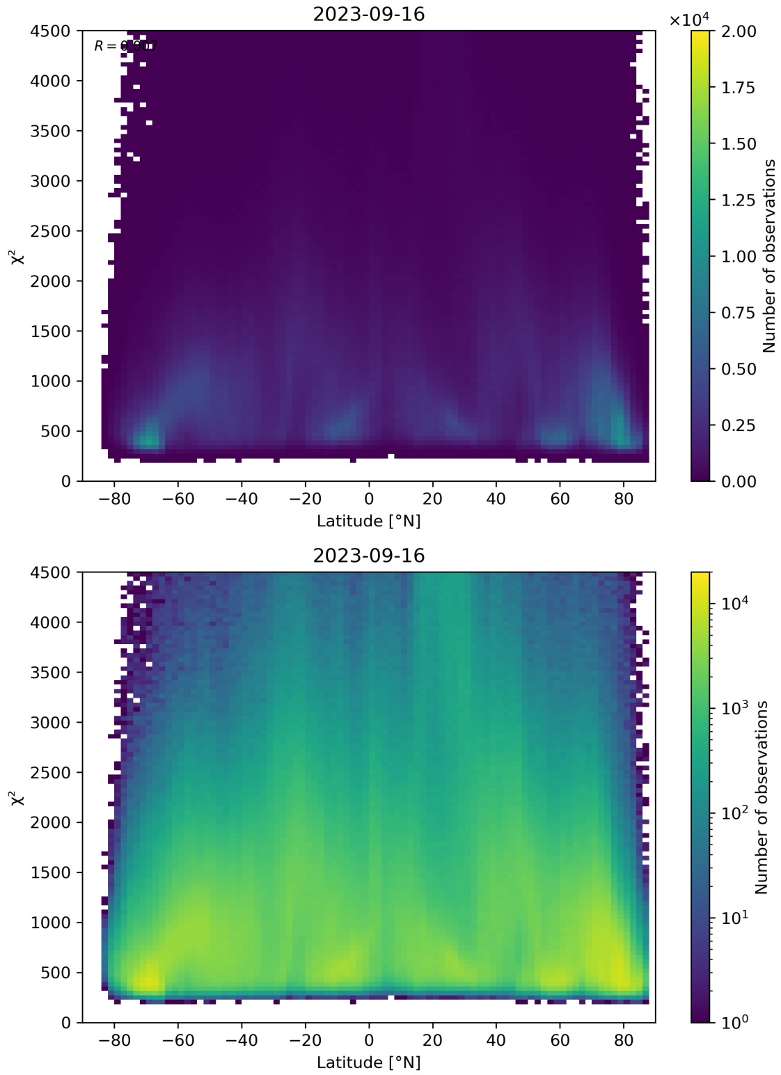
Figure 54: Scatter density plot of “Latitude” against “ \chi^2 ” for 2023-09-15 to 2023-09-17.
