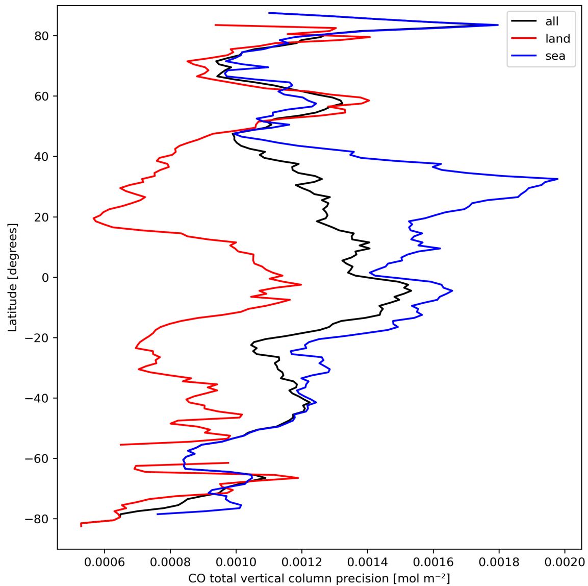
Figure 12: Zonal average of “CO total vertical column precision” for 2023-09-15 to 2023-09-17.
