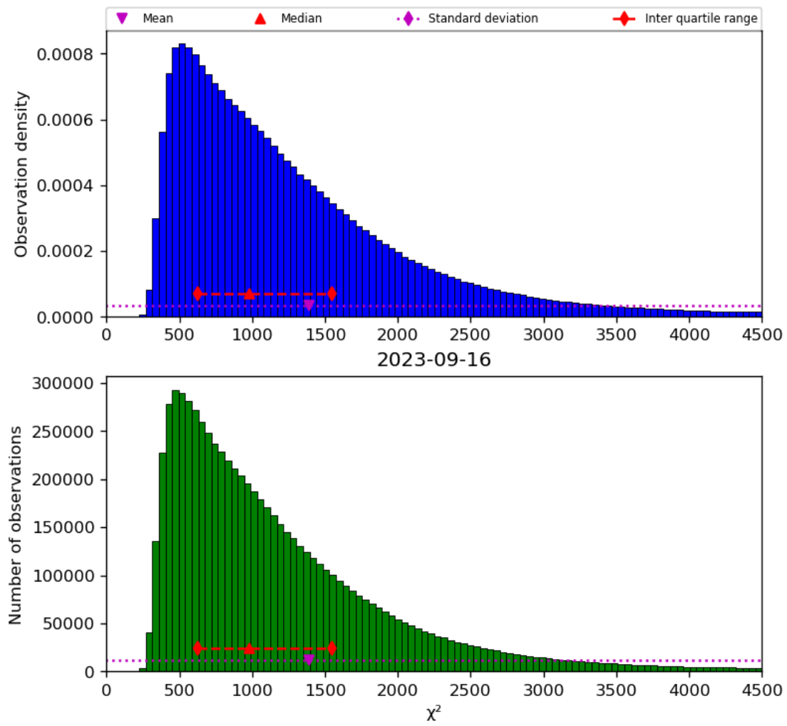
Figure 22: Histogram of “ \chi^2 ” for 2023-09-15 to 2023-09-17
