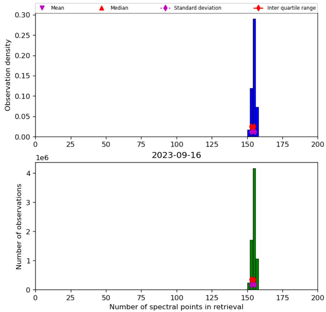
Figure 21: Histogram of “Number of spectral points in retrieval” for 2023-09-15 to 2023-09-17
