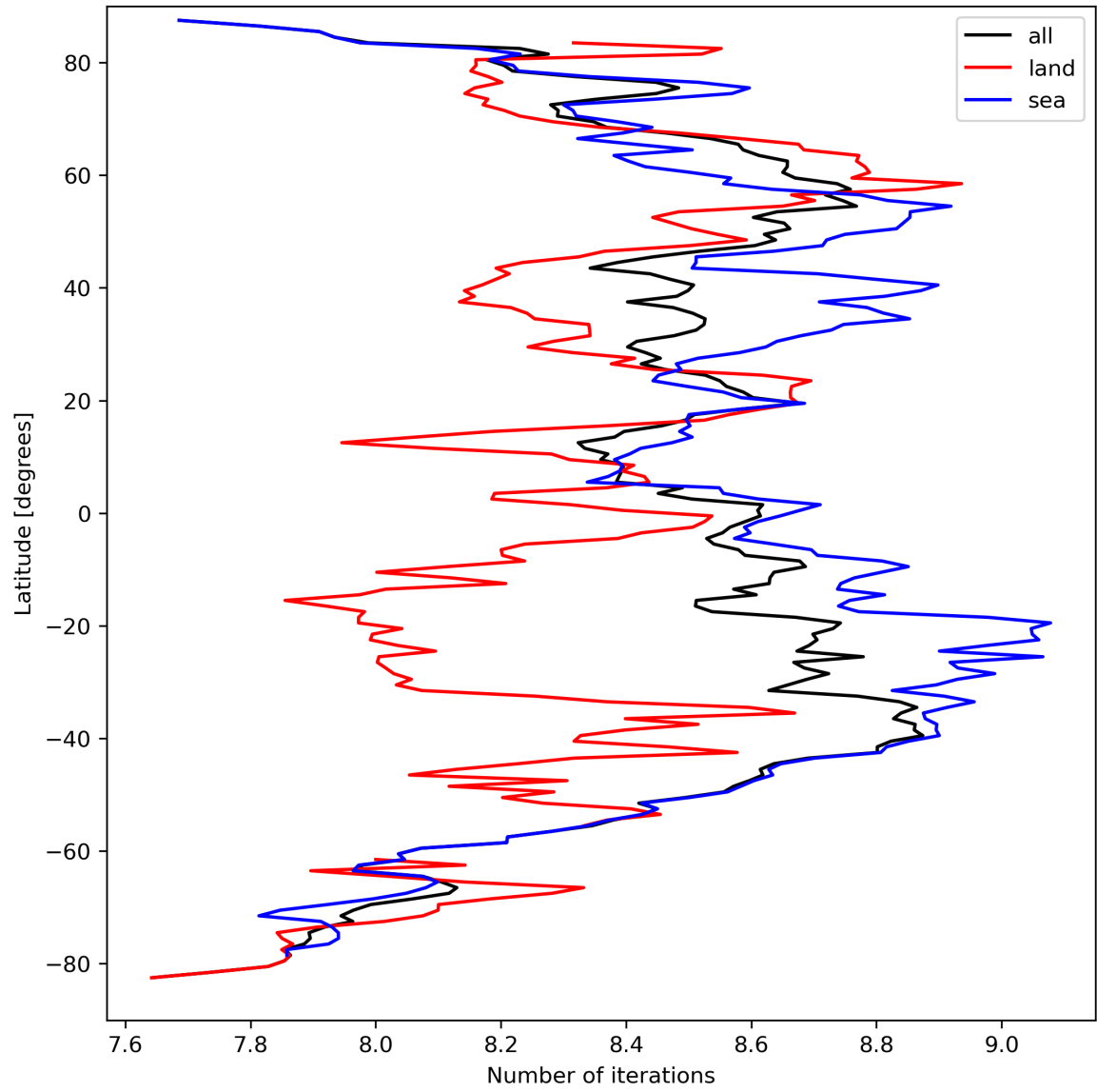
Figure 16: Zonal average of “Number of iterations” for 2023-09-15 to 2023-09-17.
