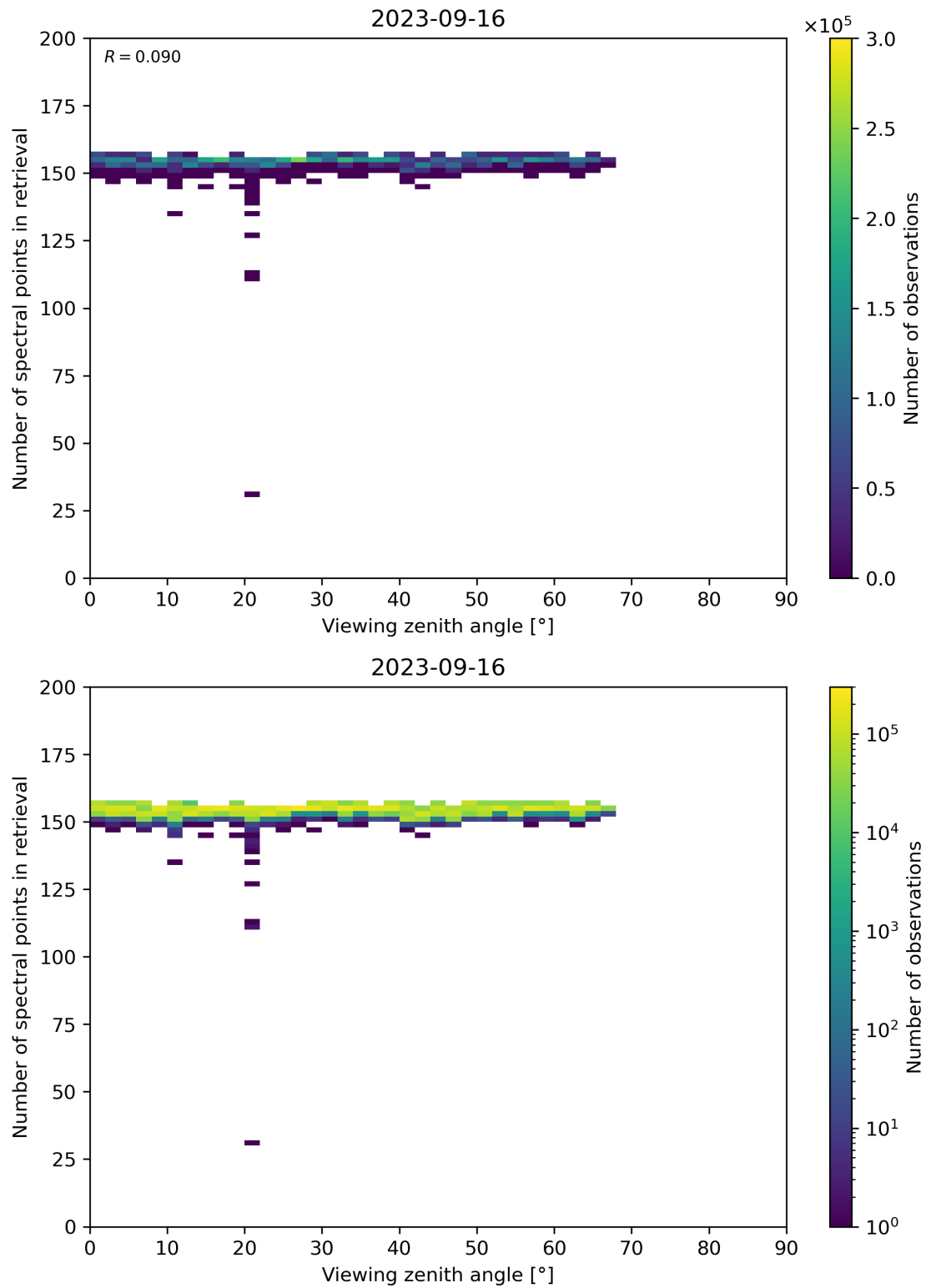
Figure 76: Scatter density plot of “Viewing zenith angle” against “Number of spectral points in retrieval” for 2023-09-15 to 2023-09-17.
