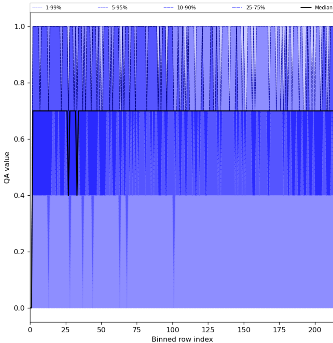
Figure 25: Along track statistics of “QA value” for 2023-09-15 to 2023-09-17
