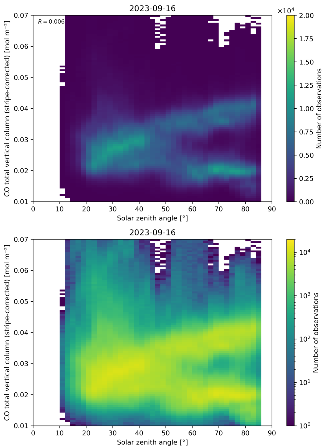
Figure 62: Scatter density plot of “Solar zenith angle” against “CO total vertical column (stripe-corrected)” for 2023-09-15 to 2023-09-17.
