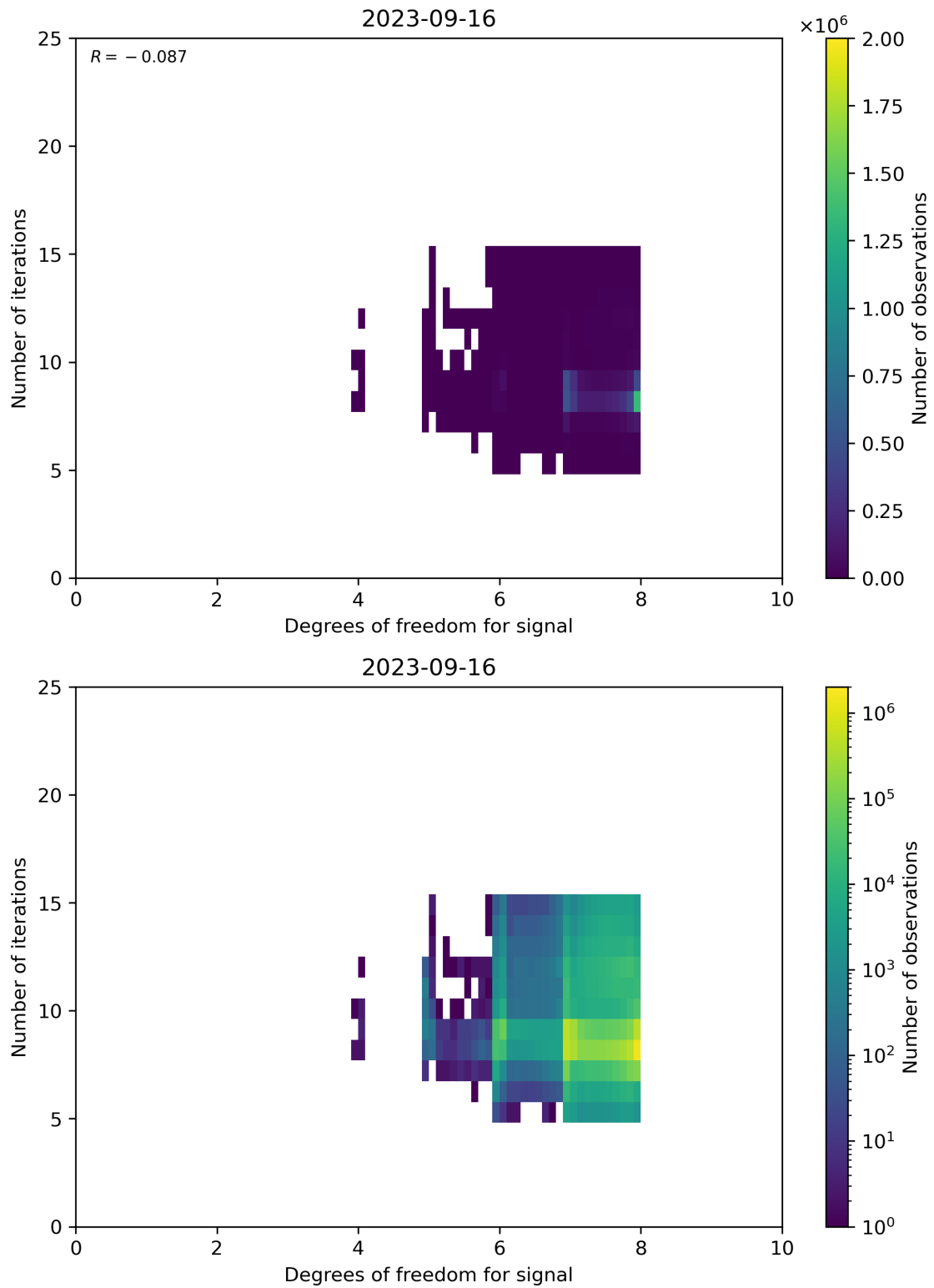
Figure 50: Scatter density plot of “Degrees of freedom for signal” against “Number of iterations” for 2023-09-15 to 2023-09-17.
