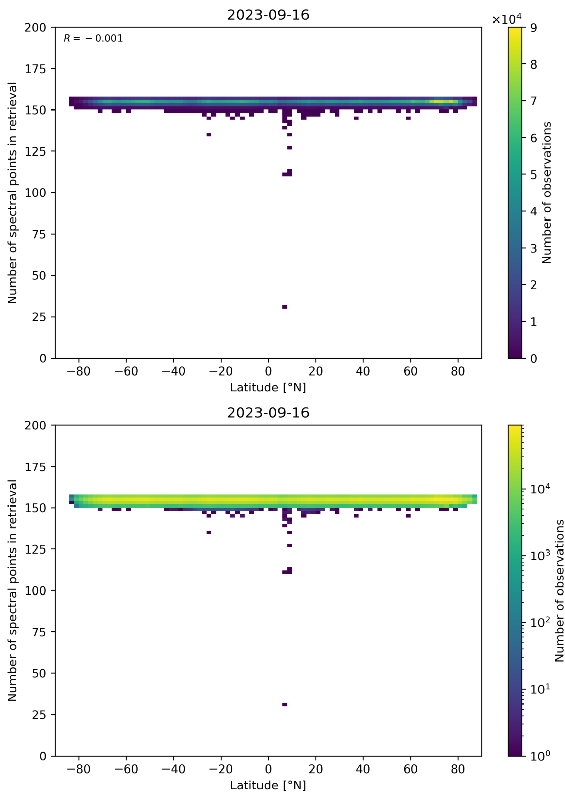
Figure 57: Scatter density plot of “Latitude” against “Number of spectral points in retrieval” for 2023-09-15 to 2023-09-17.
