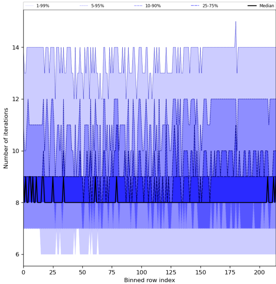
Figure 32: Along track statistics of “Number of iterations” for 2023-09-15 to 2023-09-17
