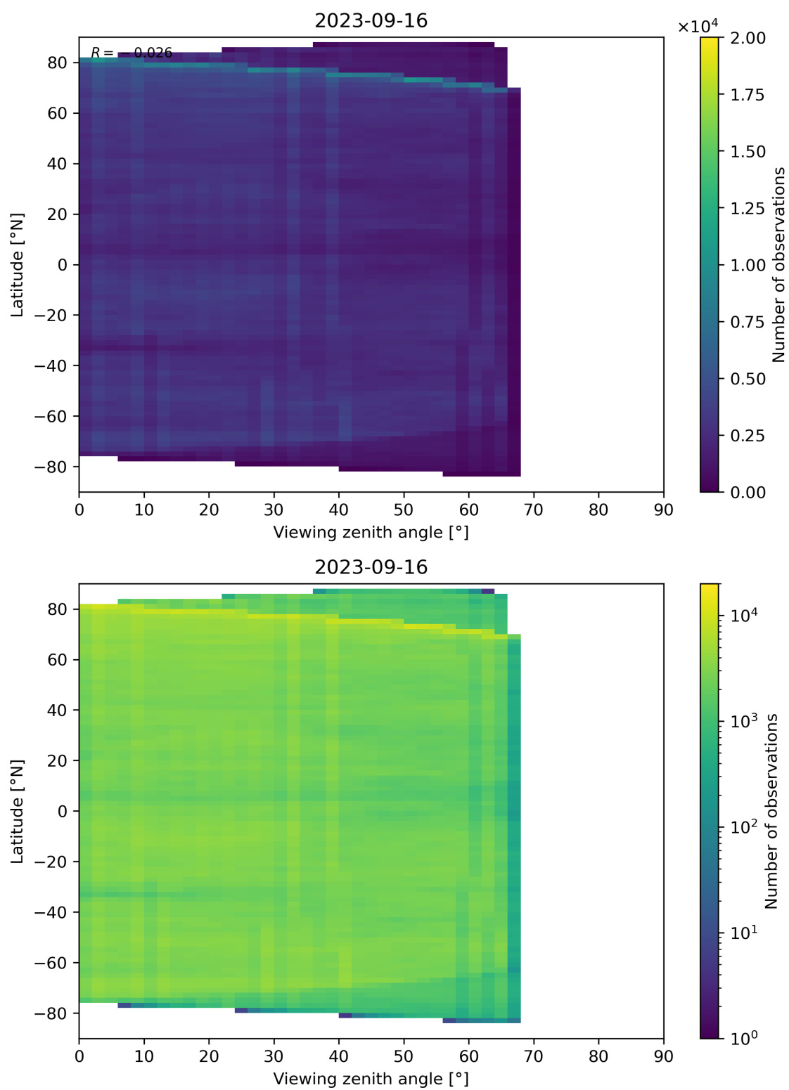
Figure 74: Scatter density plot of “Viewing zenith angle” against “Latitude” for 2023-09-15 to 2023-09-17.
