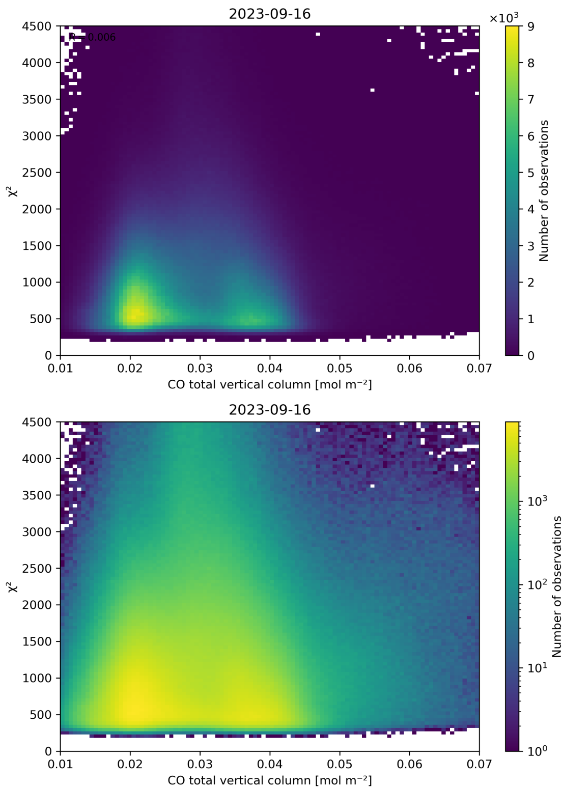
Figure 35: Scatter density plot of “CO total vertical column” against “ \chi^2 ” for 2023-09-15 to 2023-09-17.
