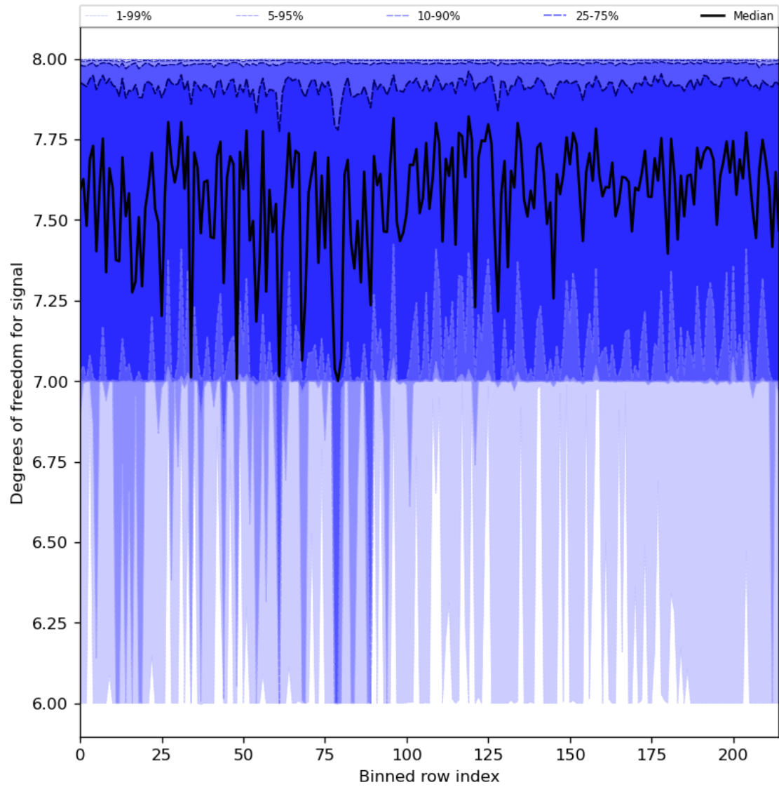
Figure 31: Along track statistics of “Degrees of freedom for signal” for 2023-09-15 to 2023-09-17
