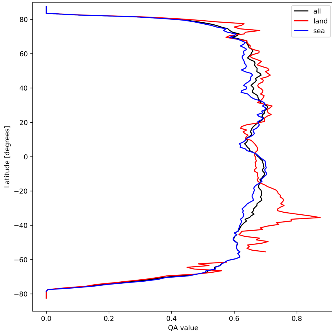
Figure 9: Zonal average of “QA value” for 2023-09-15 to 2023-09-17.
