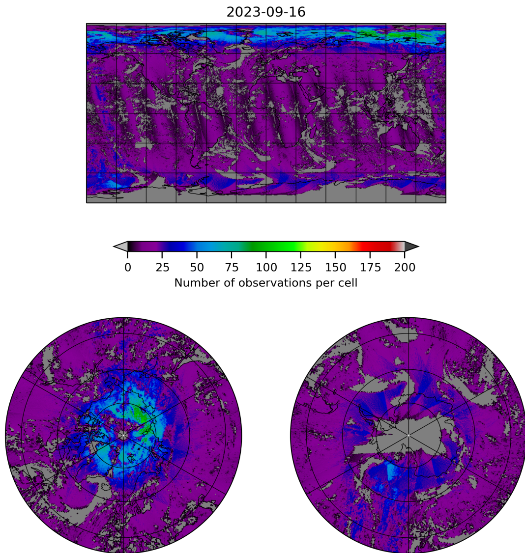
Figure 8: Map of the number of observations for 2023-09-15 to 2023-09-17
