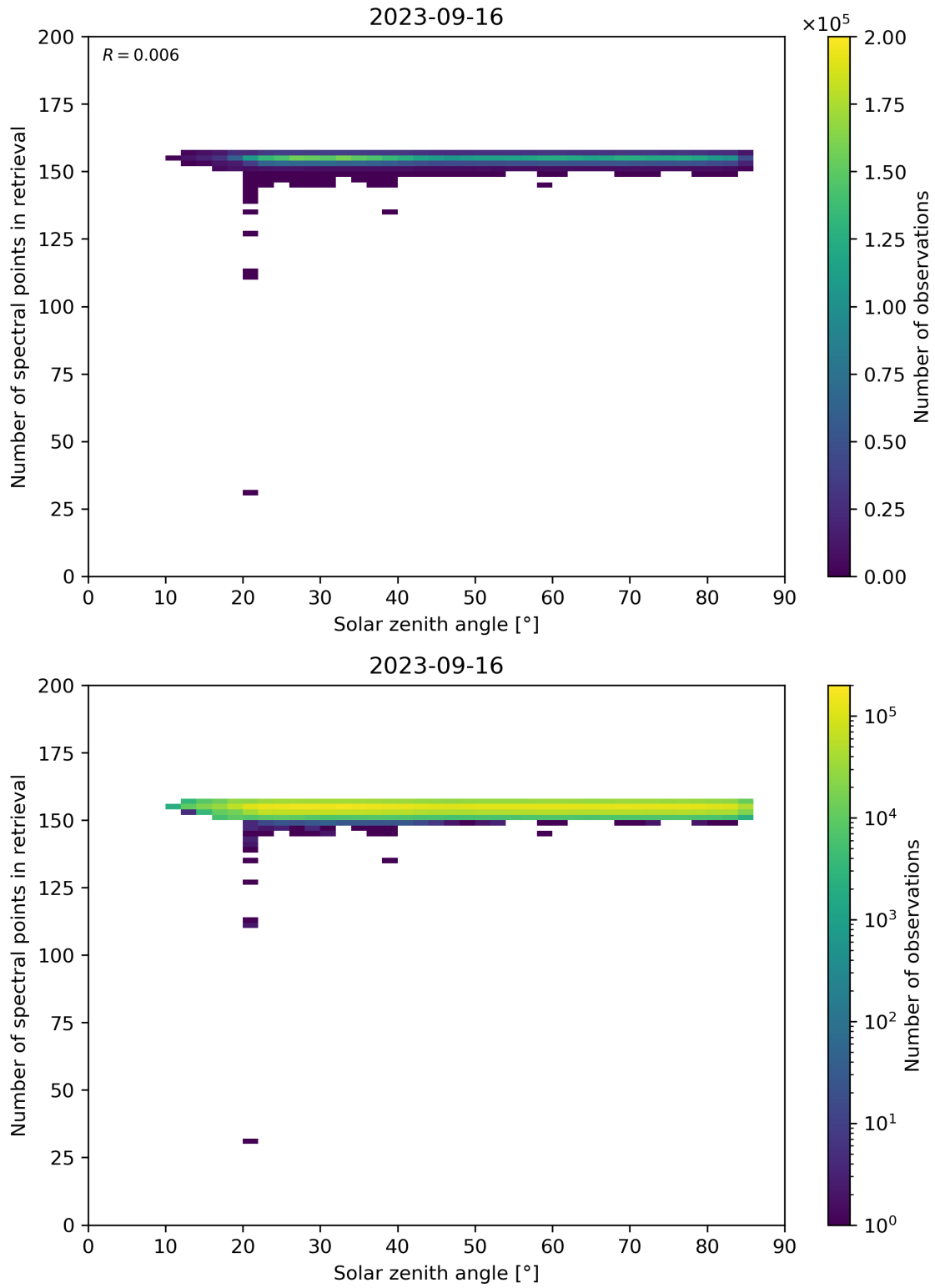
Figure 68: Scatter density plot of “Solar zenith angle” against “Number of spectral points in retrieval” for 2023-09-15 to 2023-09-17.
