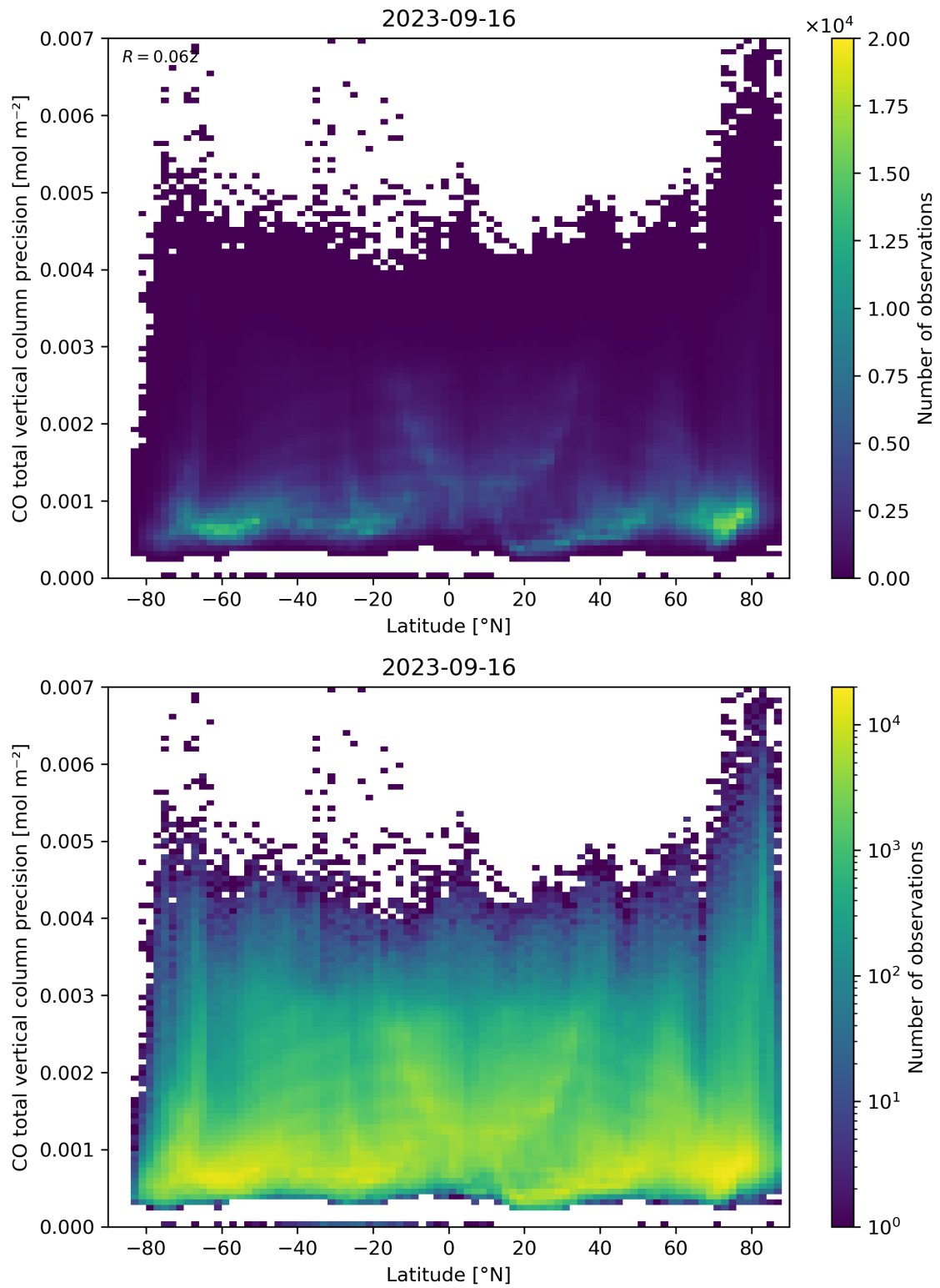
Figure 53: Scatter density plot of “Latitude” against “CO total vertical column precision” for 2023-09-15 to 2023-09-17.
