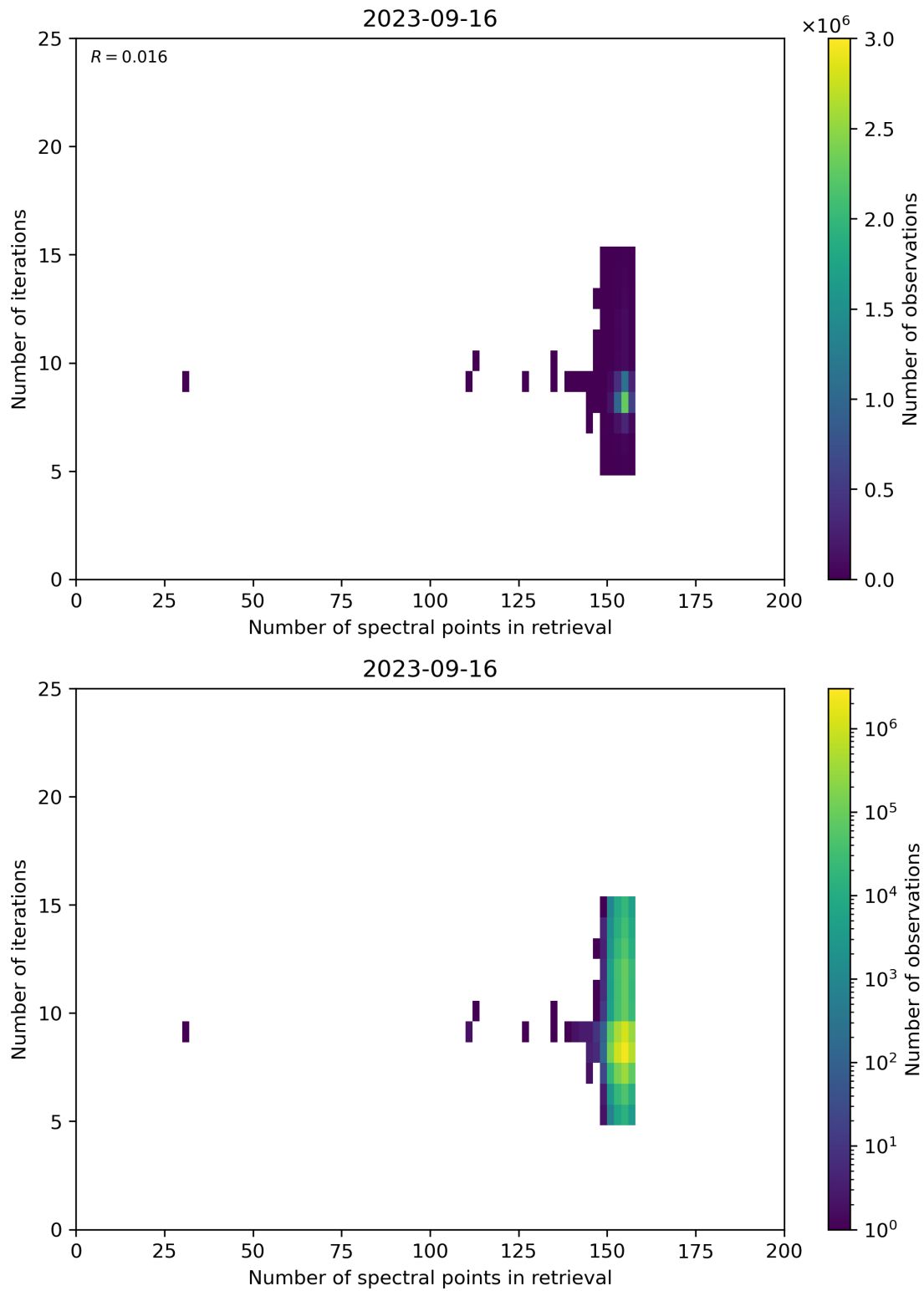
Figure 60: Scatter density plot of “Number of spectral points in retrieval” against “Number of iterations” for 2023-09-15 to 2023-09-17.
