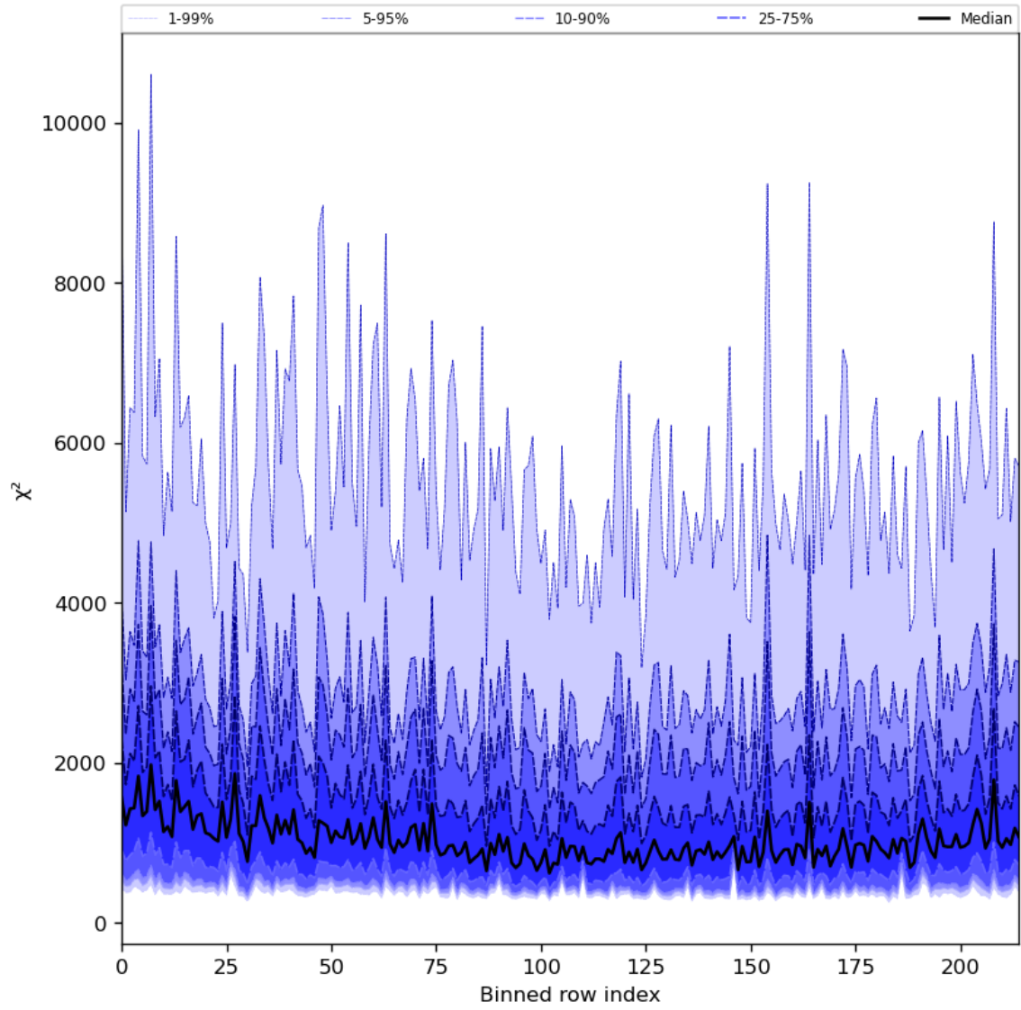
Figure 30: Along track statistics of “ \chi^2 ” for 2023-09-15 to 2023-09-17
