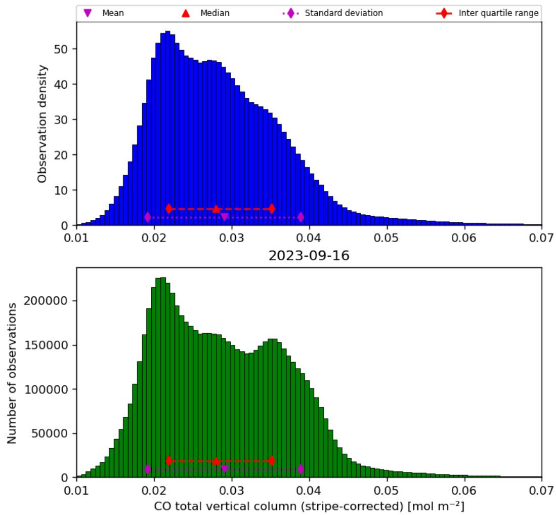
Figure 19: Histogram of “CO total vertical column (stripe-corrected)” for 2023-09-15 to 2023-09-17
