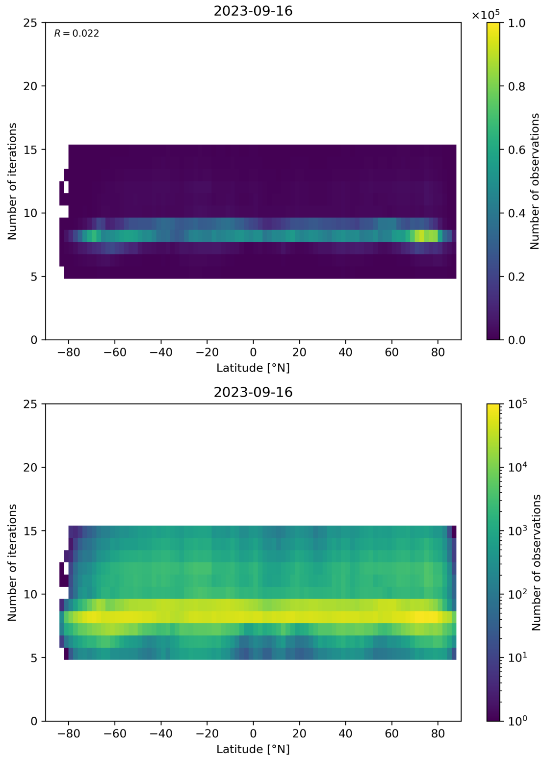
Figure 56: Scatter density plot of “Latitude” against “Number of iterations” for 2023-09-15 to 2023-09-17.
