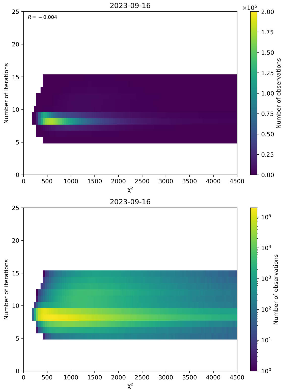
Figure 49: Scatter density plot of “ \chi^2 ” against “Number of iterations” for 2023-09-15 to 2023-09-17.
