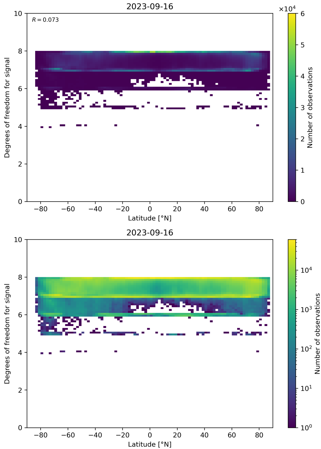
Figure 55: Scatter density plot of “Latitude” against “Degrees of freedom for signal” for 2023-09-15 to 2023-09-17.
