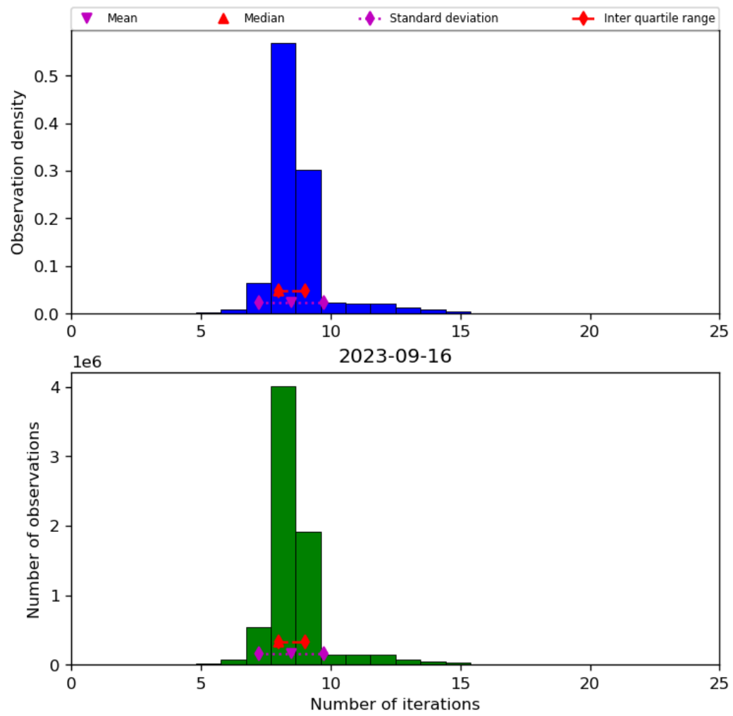
Figure 24: Histogram of “Number of iterations” for 2023-09-15 to 2023-09-17
