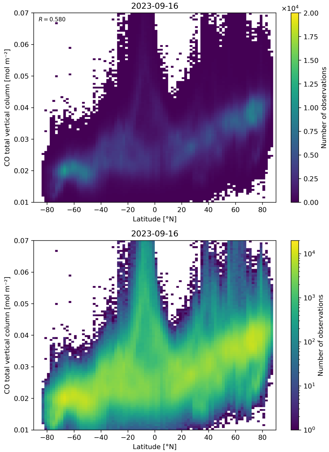
Figure 51: Scatter density plot of “Latitude” against “CO total vertical column” for 2023-09-15 to 2023-09-17.
