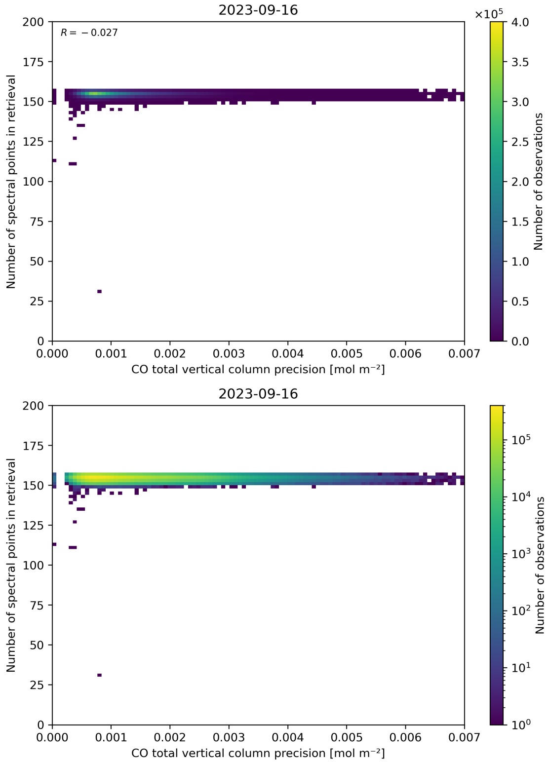
Figure 47: Scatter density plot of “CO total vertical column precision” against “Number of spectral points in retrieval” for 2023-09-15 to 2023-09-17.
