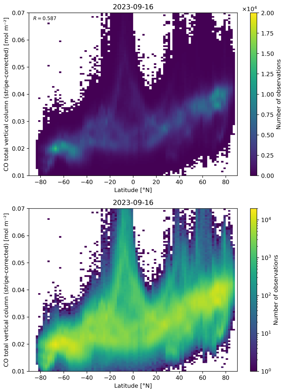
Figure 52: Scatter density plot of “Latitude” against “CO total vertical column (stripe-corrected)” for 2023-09-15 to 2023-09-17.
