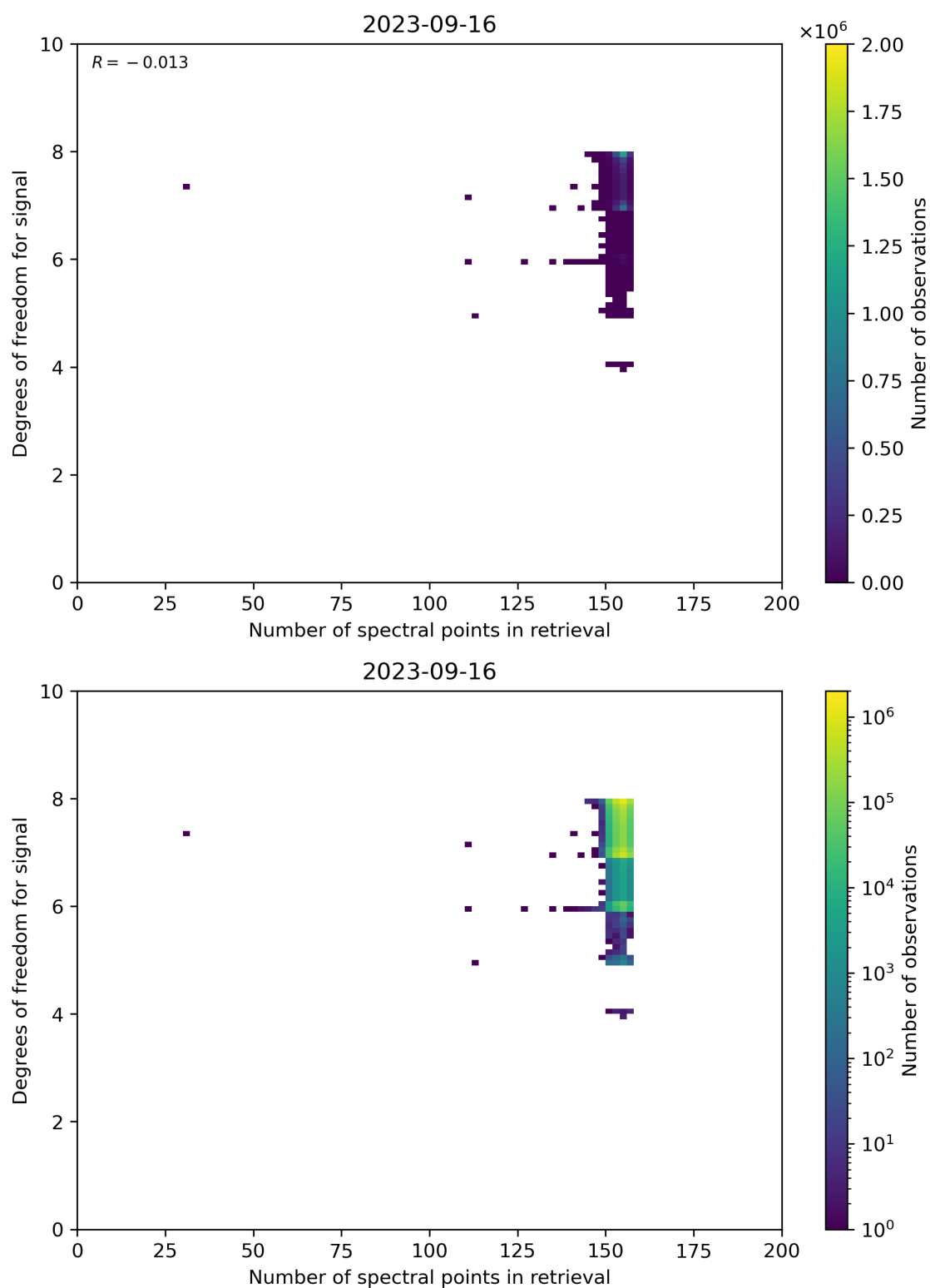
Figure 59: Scatter density plot of “Number of spectral points in retrieval” against “Degrees of freedom for signal” for 2023-09-15 to 2023-09-17.
