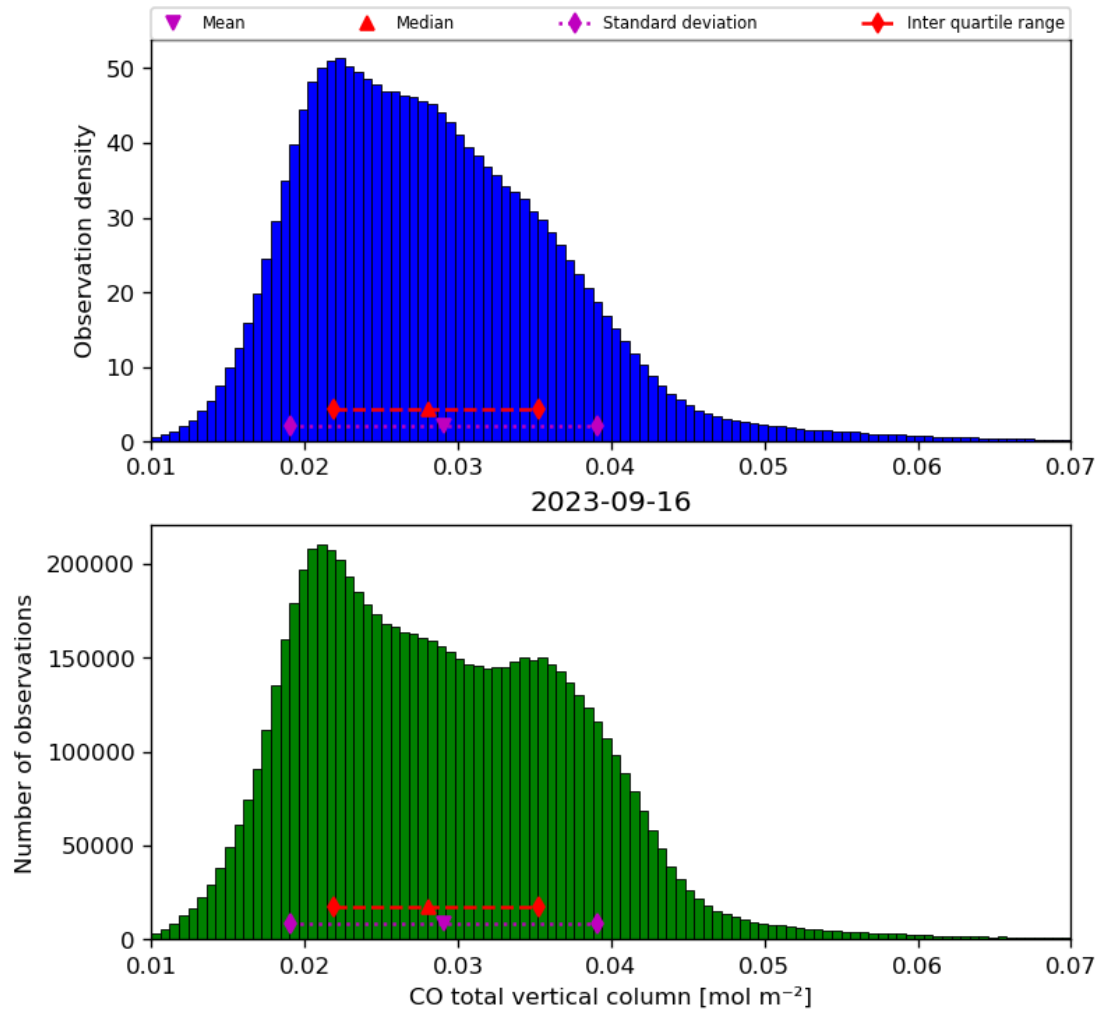
Figure 18: Histogram of “CO total vertical column” for 2023-09-15 to 2023-09-17
