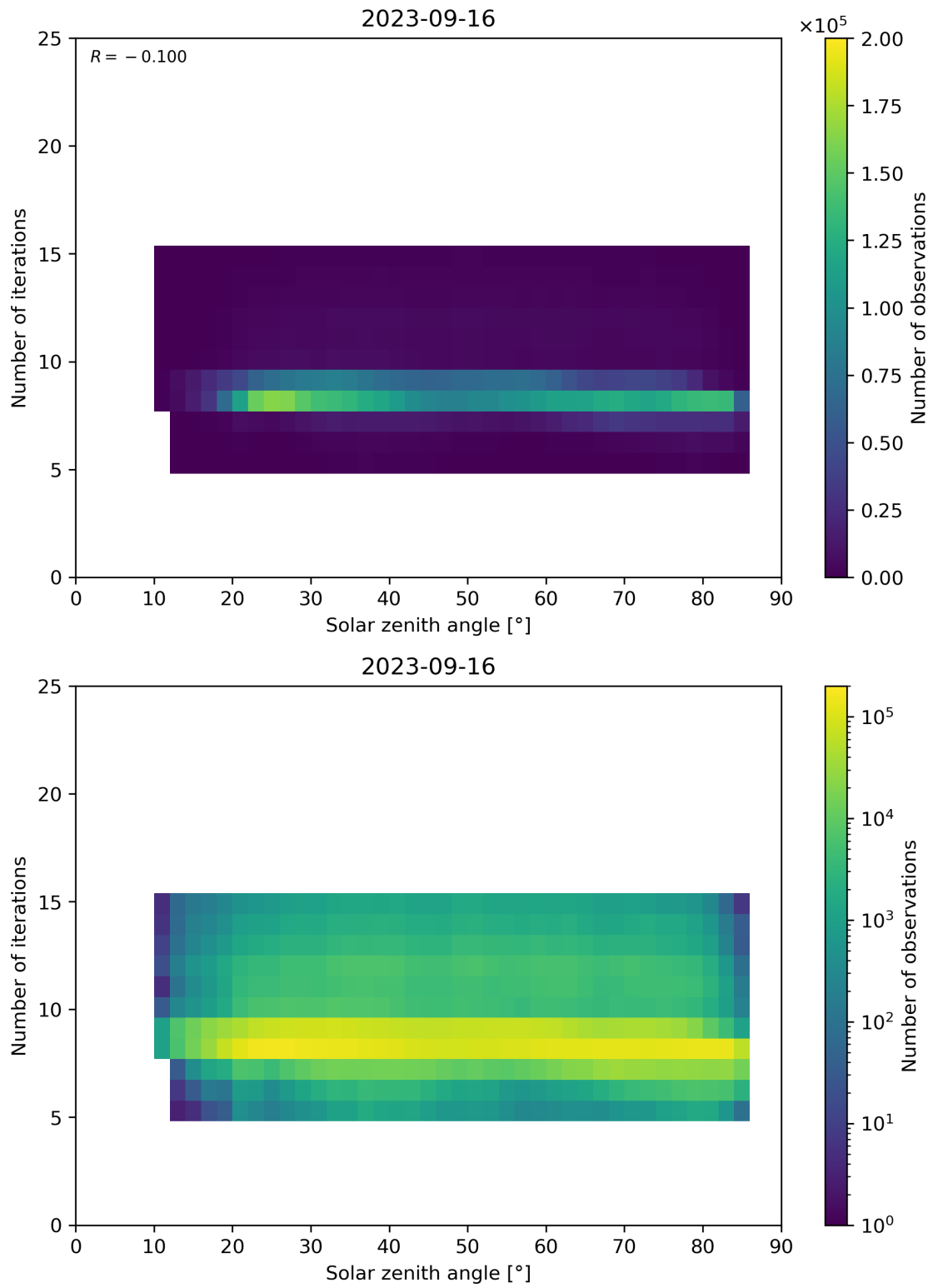
Figure 67: Scatter density plot of “Solar zenith angle” against “Number of iterations” for 2023-09-15 to 2023-09-17.
