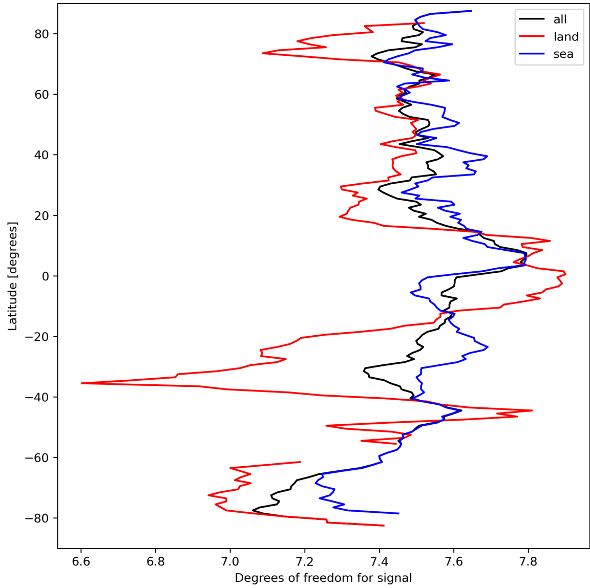
Figure 15: Zonal average of “Degrees of freedom for signal” for 2023-09-15 to 2023-09-17.
