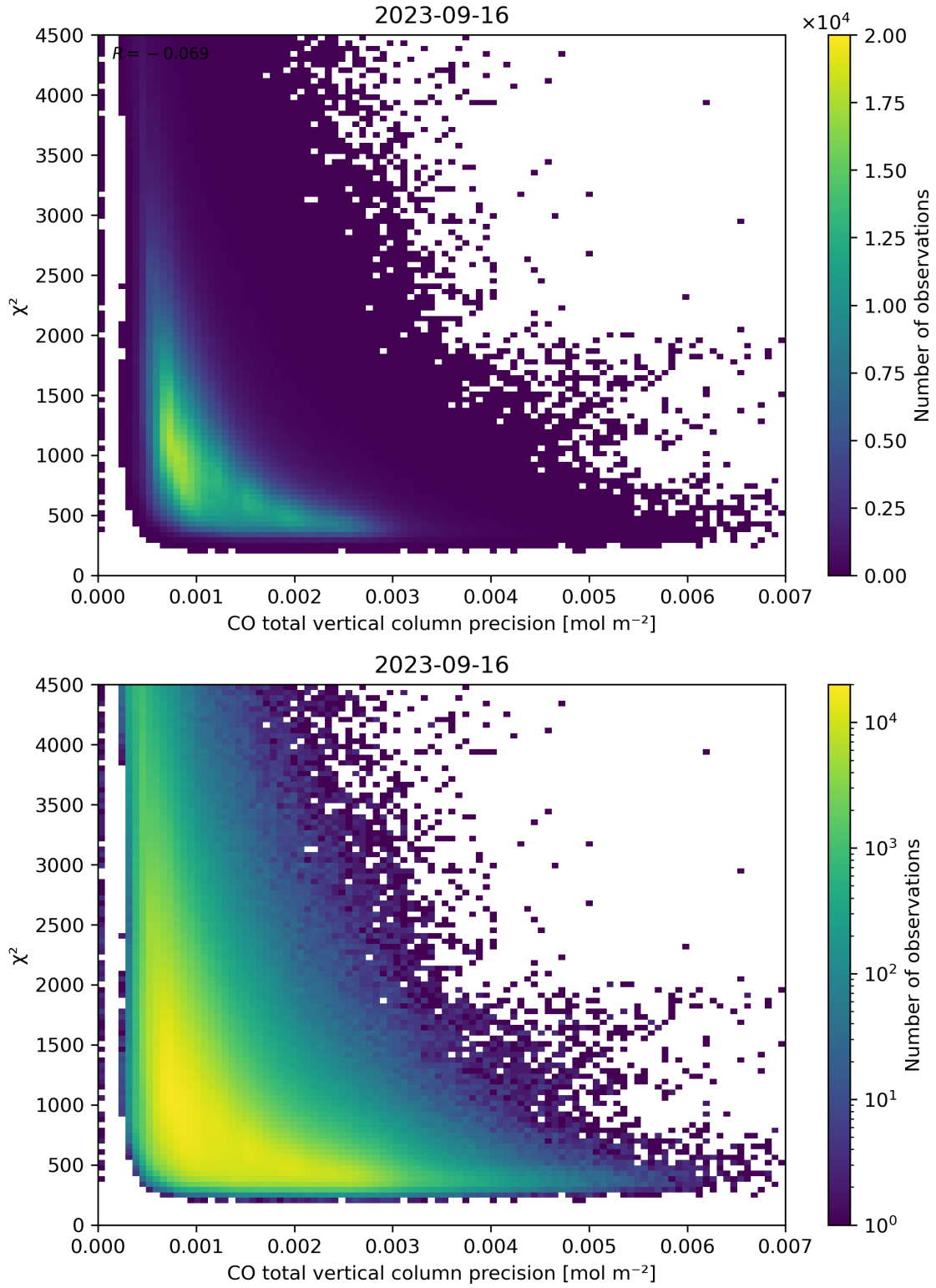
Figure 44: Scatter density plot of “CO total vertical column precision” against “ \chi^2 ” for 2023-09-15 to 2023-09-17.
