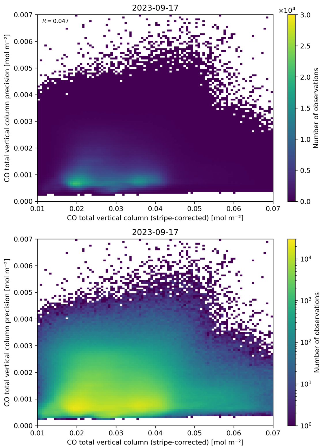
Figure 36: Scatter density plot of “CO total vertical column (stripe-corrected)” against “CO total vertical column precision” for 2023-09-16 to 2023-09-18.
