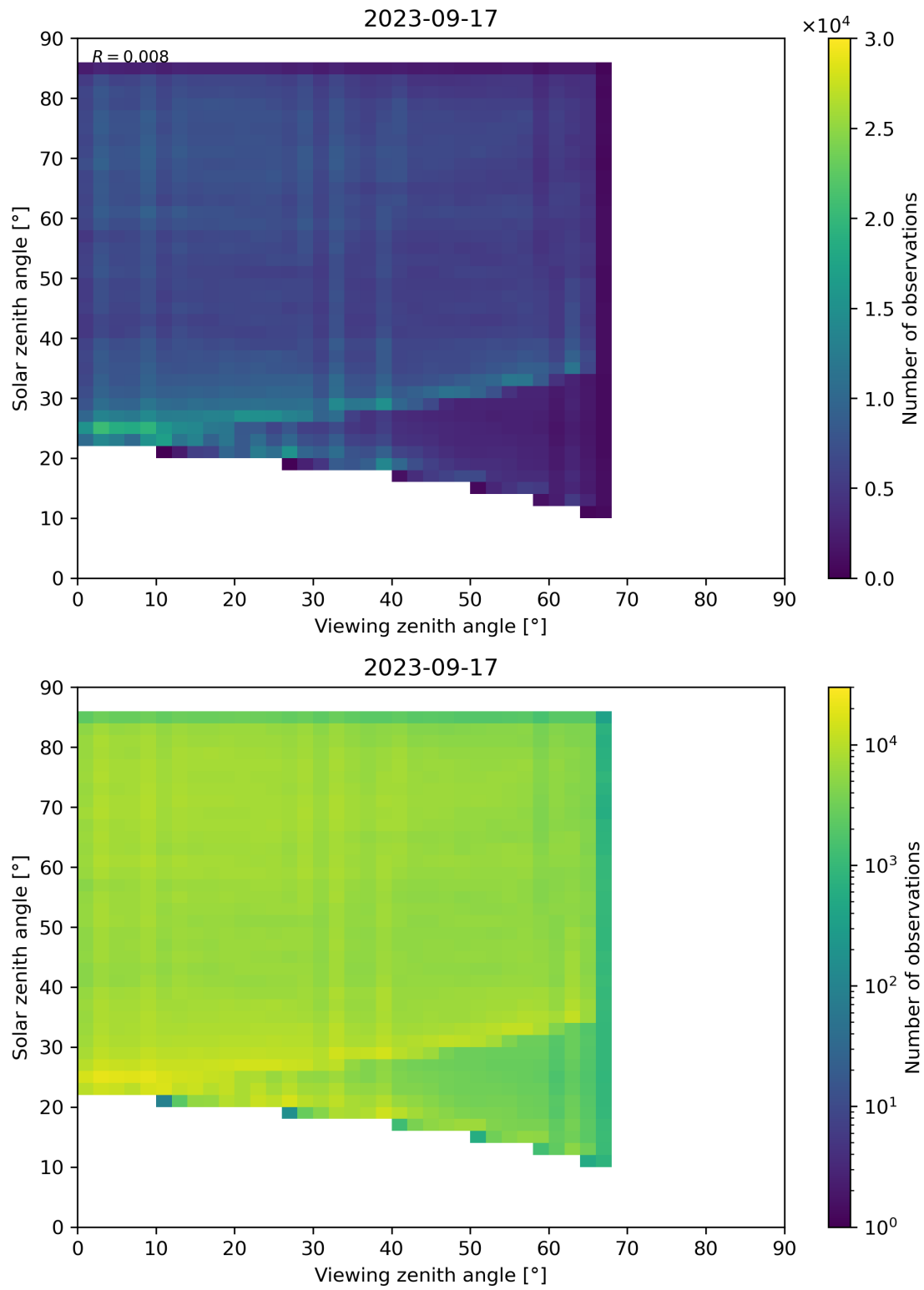
Figure 77: Scatter density plot of “Viewing zenith angle” against “Solar zenith angle” for 2023-09-16 to 2023-09-18.
