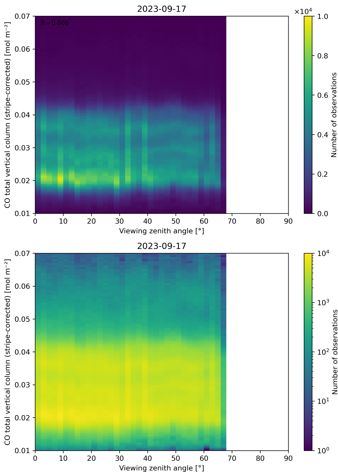
Figure 70: Scatter density plot of “Viewing zenith angle” against “CO total vertical column (stripe-corrected)” for 2023-09-16 to 2023-09-18.
