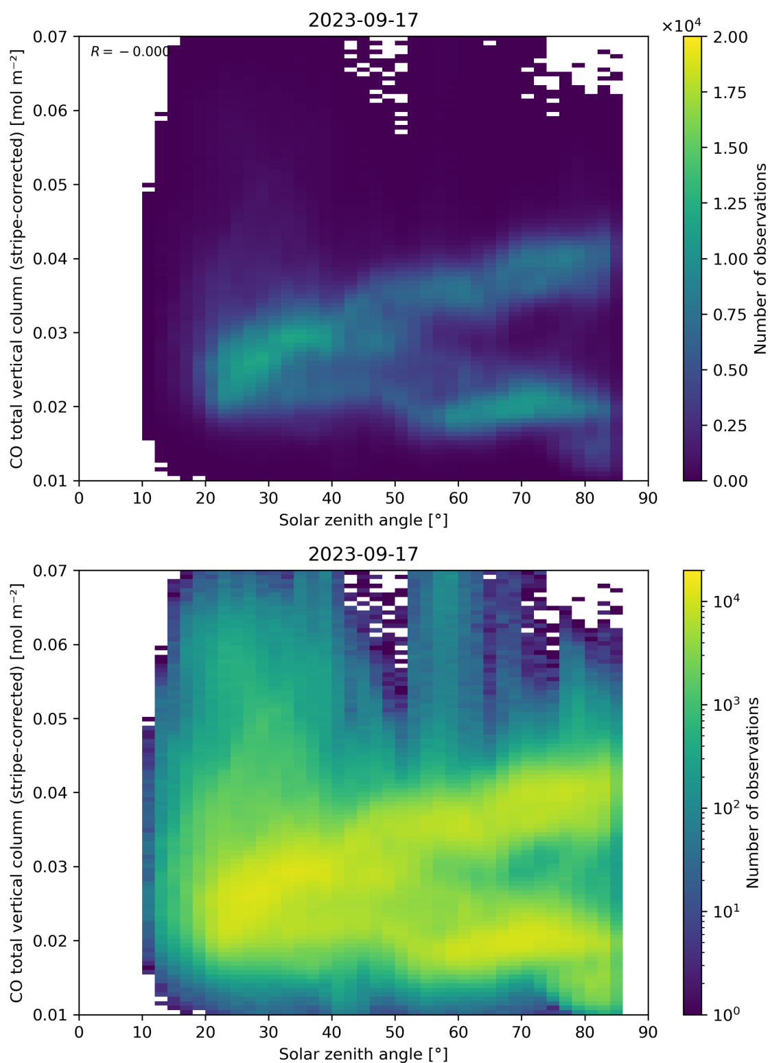
Figure 62: Scatter density plot of “Solar zenith angle” against “CO total vertical column (stripe-corrected)” for 2023-09-16 to 2023-09-18.
