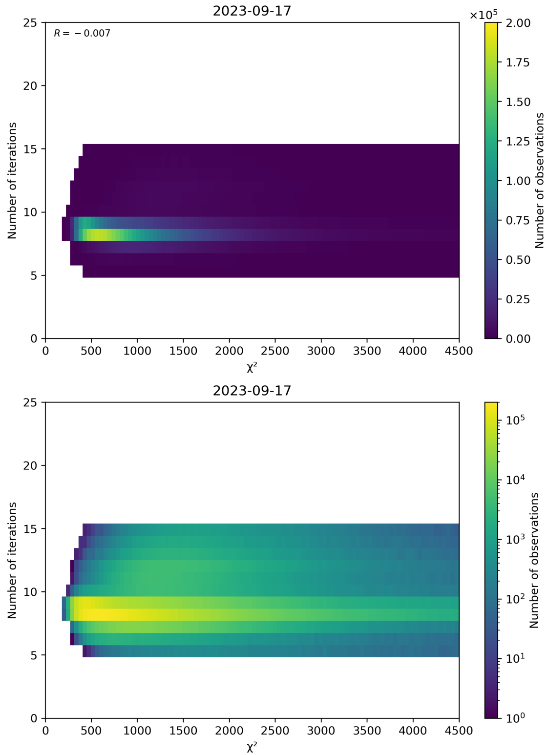
Figure 49: Scatter density plot of “ \chi^2 ” against “Number of iterations” for 2023-09-16 to 2023-09-18.
