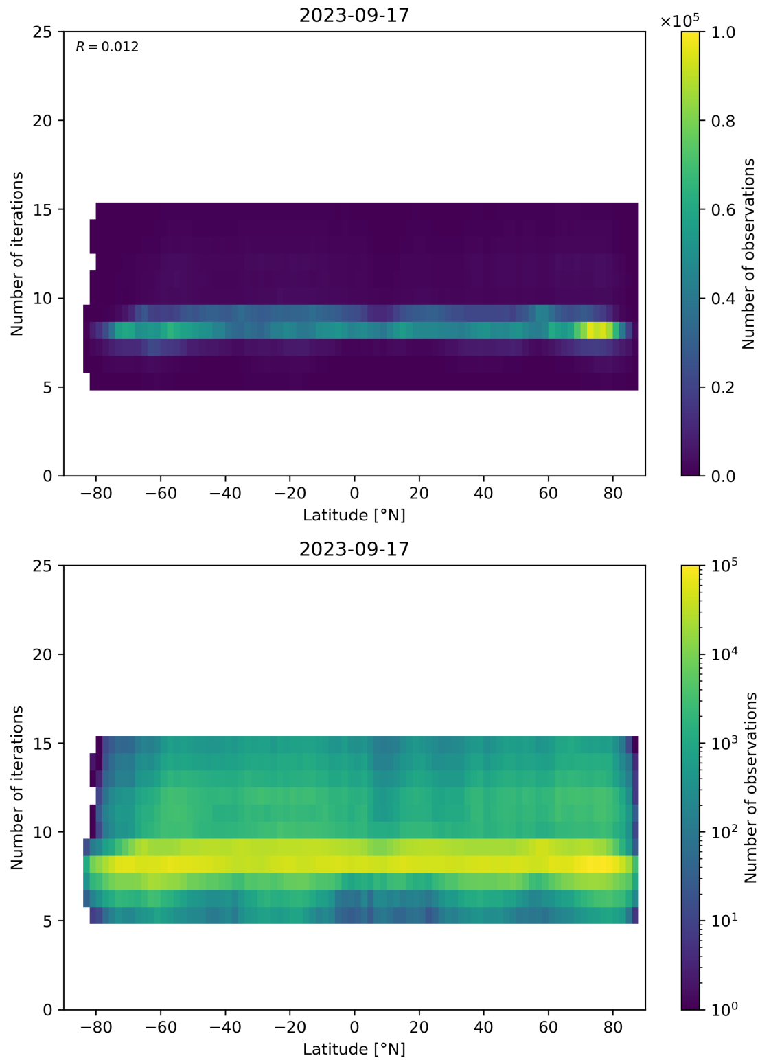
Figure 56: Scatter density plot of “Latitude” against “Number of iterations” for 2023-09-16 to 2023-09-18.
