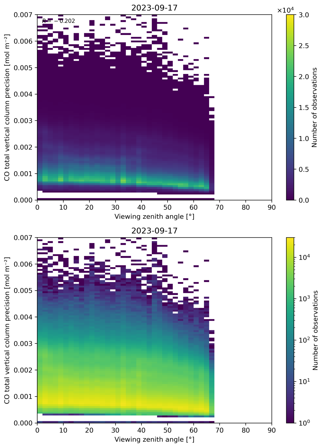
Figure 71: Scatter density plot of “Viewing zenith angle” against “CO total vertical column precision” for 2023-09-16 to 2023-09-18.
