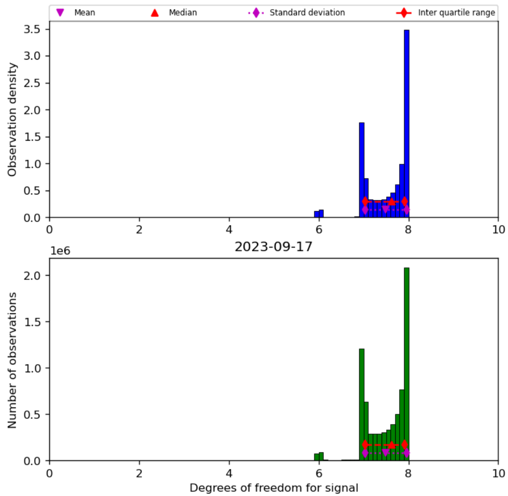
Figure 23: Histogram of “Degrees of freedom for signal” for 2023-09-16 to 2023-09-18
