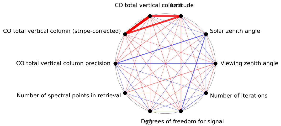
Figure 1: Map of correlation graph for 2023-09-16 to 2023-09-18.
