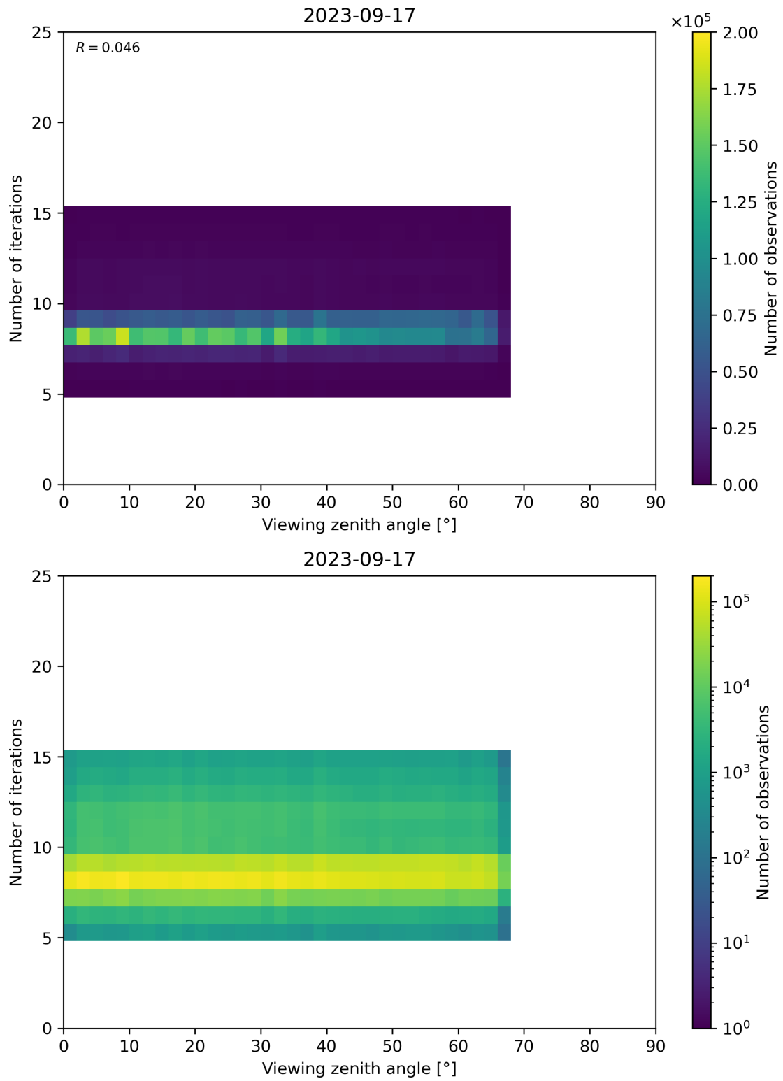
Figure 75: Scatter density plot of “Viewing zenith angle” against “Number of iterations” for 2023-09-16 to 2023-09-18.
