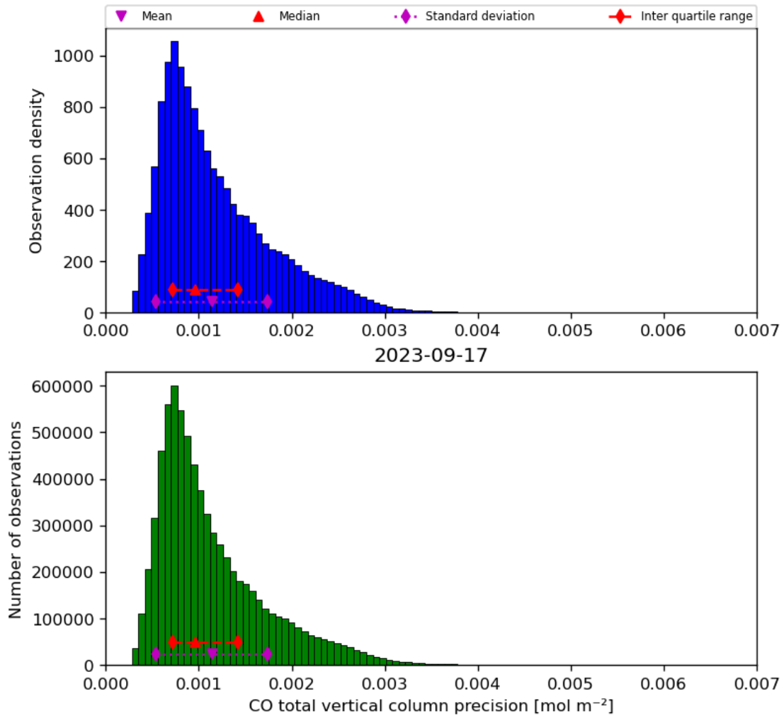
Figure 20: Histogram of “CO total vertical column precision” for 2023-09-16 to 2023-09-18
