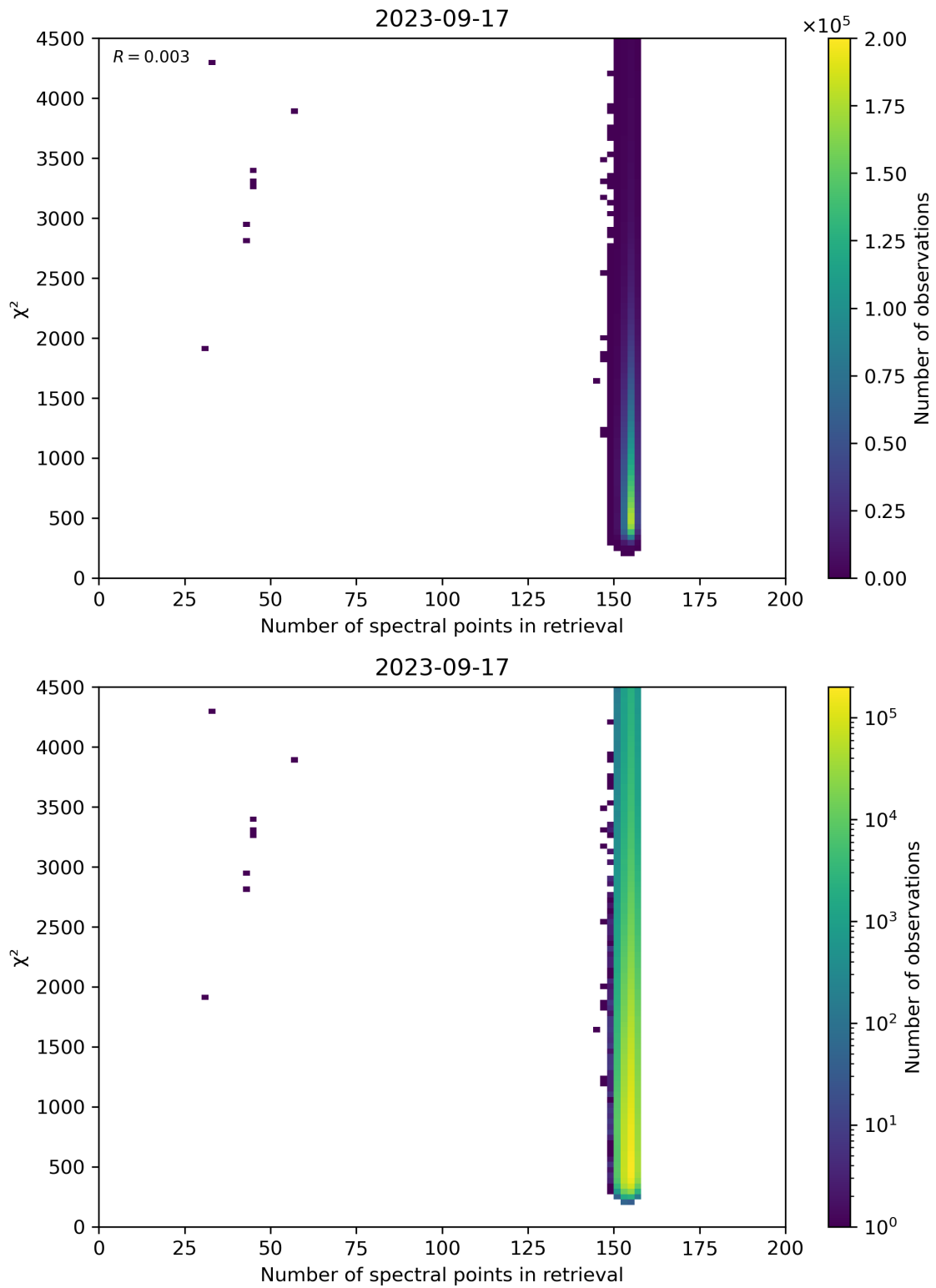
Figure 58: Scatter density plot of “Number of spectral points in retrieval” against “ \chi^2 ” for 2023-09-16 to 2023-09-18.
