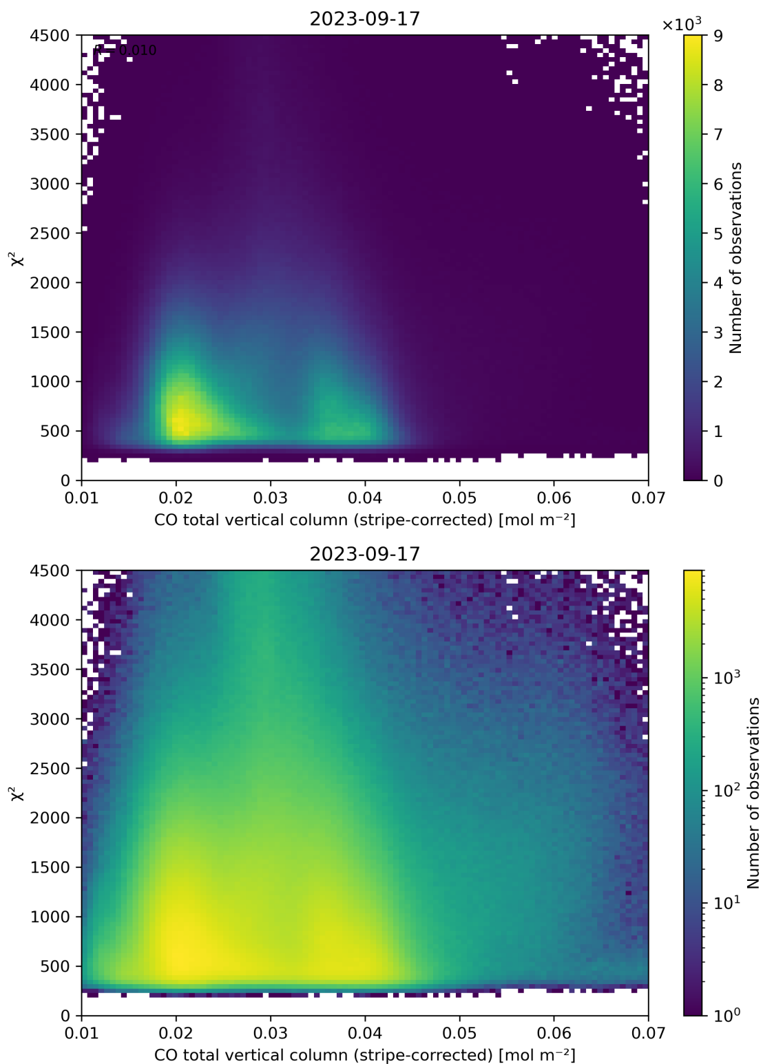
Figure 37: Scatter density plot of “CO total vertical column (stripe-corrected)” against “ \chi^2 ” for 2023-09-16 to 2023-09-18.
