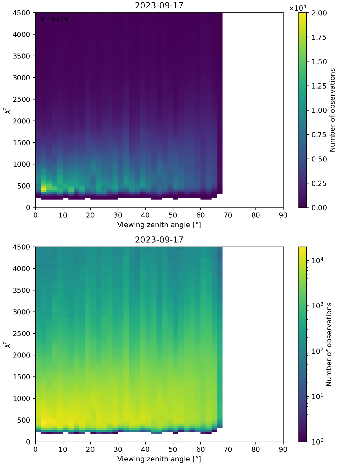
Figure 72: Scatter density plot of “Viewing zenith angle” against “ \chi^2 ” for 2023-09-16 to 2023-09-18.
