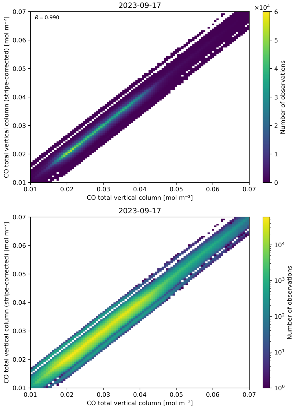
Figure 33: Scatter density plot of “CO total vertical column” against “CO total vertical column (stripe-corrected)” for 2023-09-16 to 2023-09-18.
