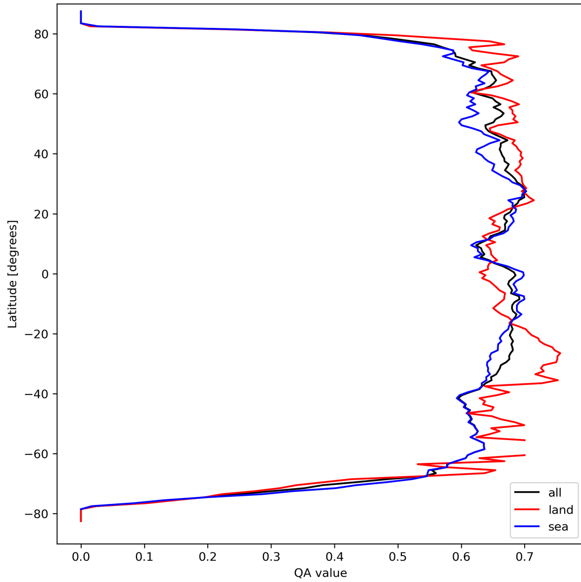
Figure 9: Zonal average of “QA value” for 2023-09-16 to 2023-09-18.
