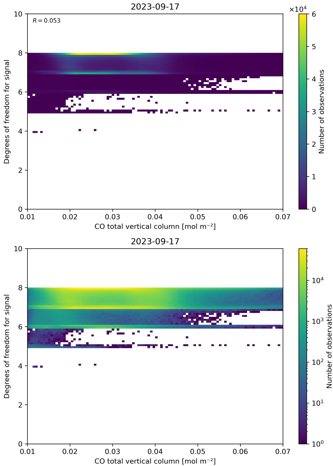
Figure 41: Scatter density plot of “CO total vertical column” against “Degrees of freedom for signal” for 2023-09-16 to 2023-09-18.
