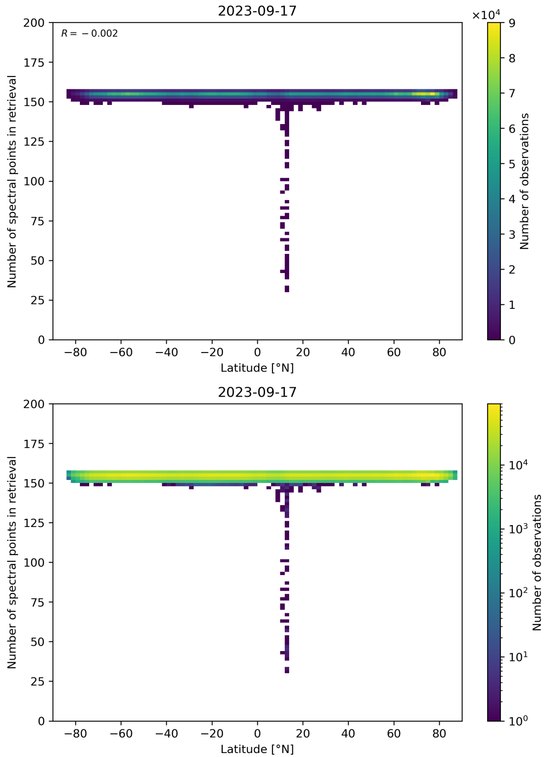
Figure 57: Scatter density plot of “Latitude” against “Number of spectral points in retrieval” for 2023-09-16 to 2023-09-18.
