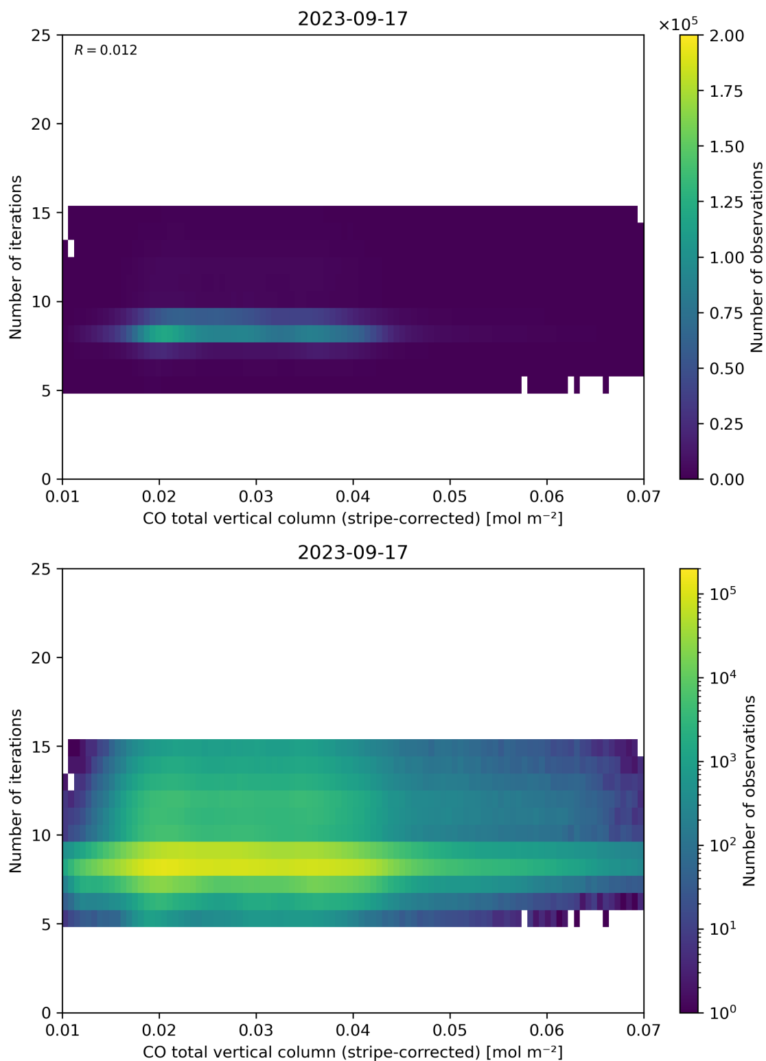
Figure 39: Scatter density plot of “CO total vertical column (stripe-corrected)” against “Number of iterations” for 2023-09-16 to 2023-09-18.
