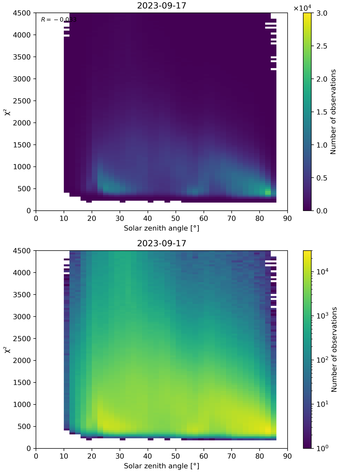
Figure 64: Scatter density plot of “Solar zenith angle” against “ \chi^2 ” for 2023-09-16 to 2023-09-18.
