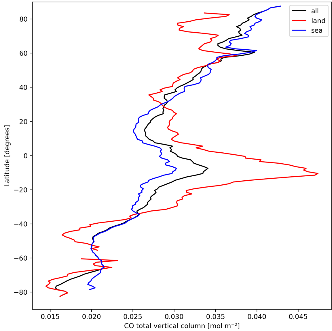
Figure 10: Zonal average of “CO total vertical column” for 2023-09-16 to 2023-09-18.
