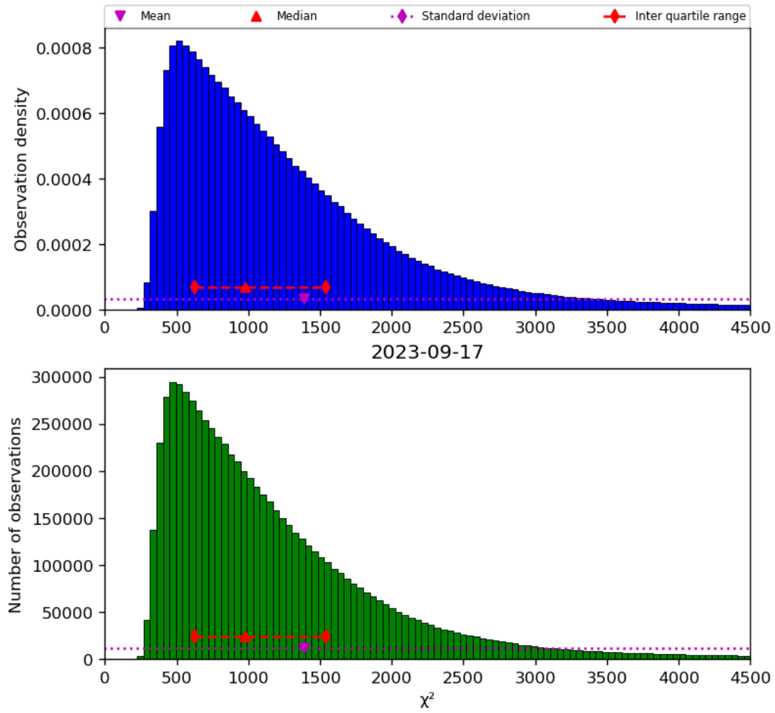
Figure 22: Histogram of “ \chi^2 ” for 2023-09-16 to 2023-09-18
