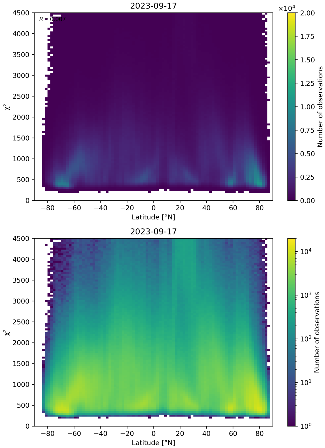
Figure 54: Scatter density plot of “Latitude” against “ \chi^2 ” for 2023-09-16 to 2023-09-18.
