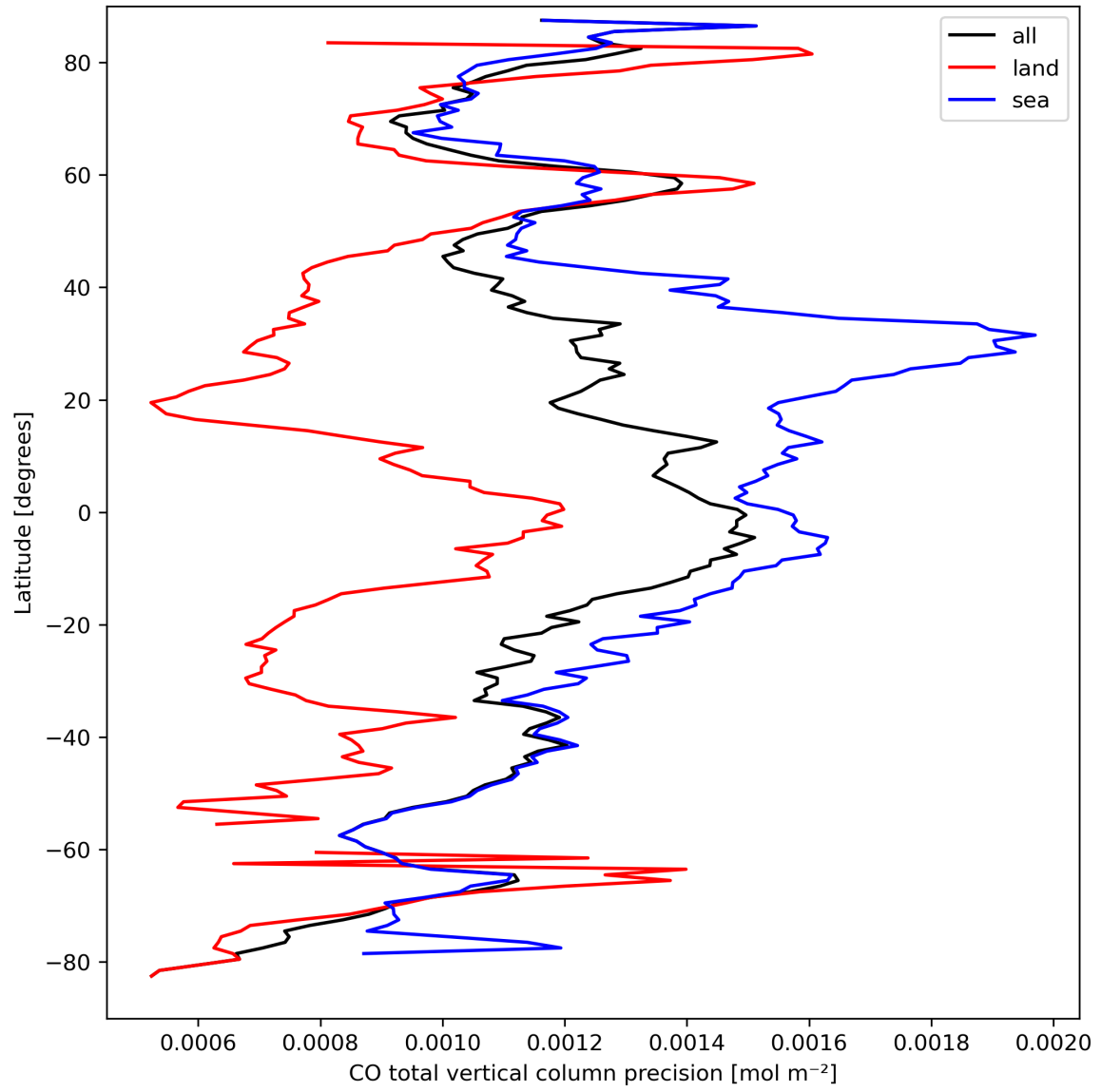
Figure 12: Zonal average of "CO total vertical column precision" for 2023-09-16 to 2023-09-18.
