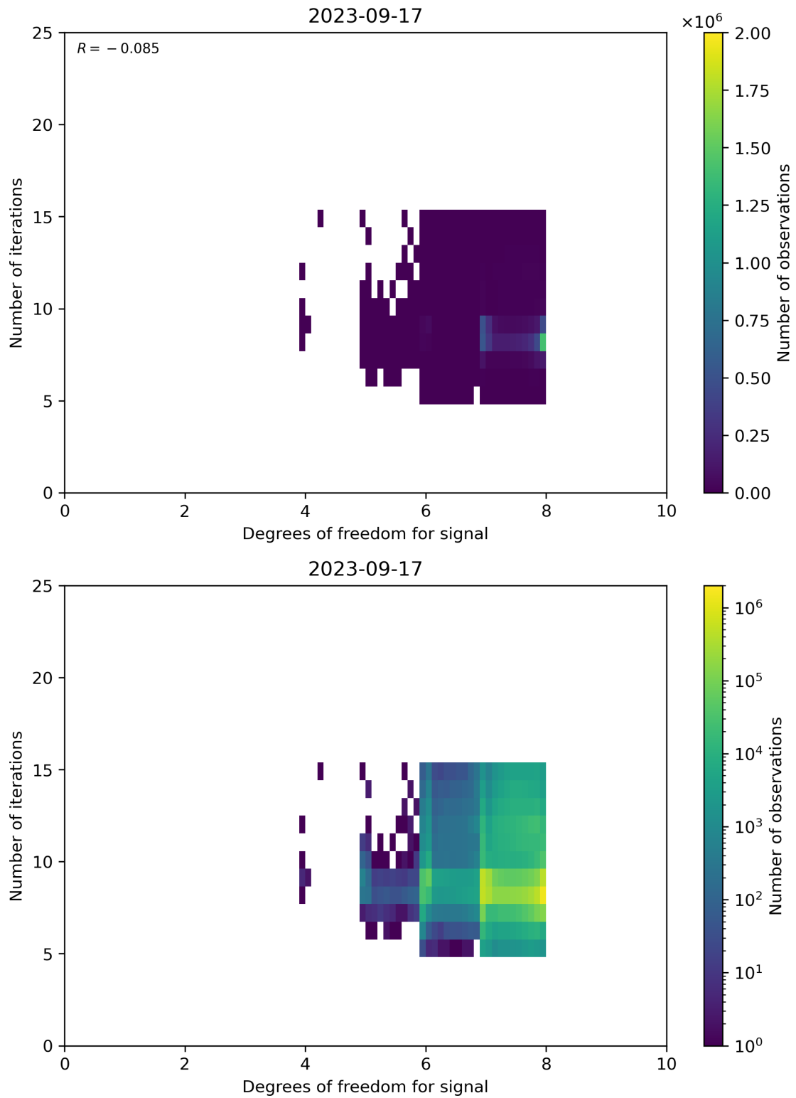
Figure 50: Scatter density plot of “Degrees of freedom for signal” against “Number of iterations” for 2023-09-16 to 2023-09-18.
