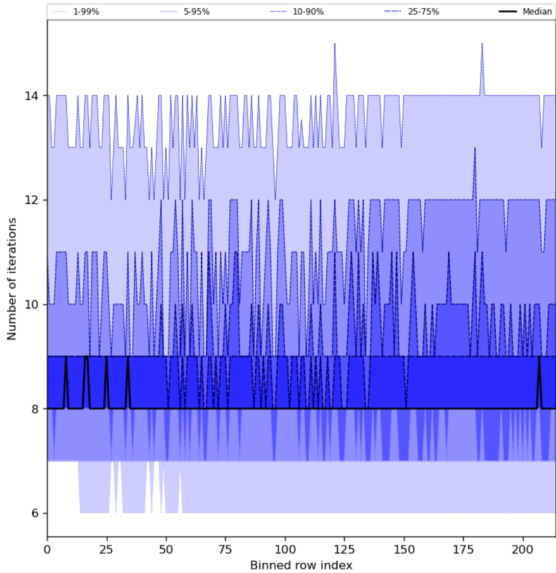
Figure 32: Along track statistics of “Number of iterations” for 2023-09-16 to 2023-09-18
