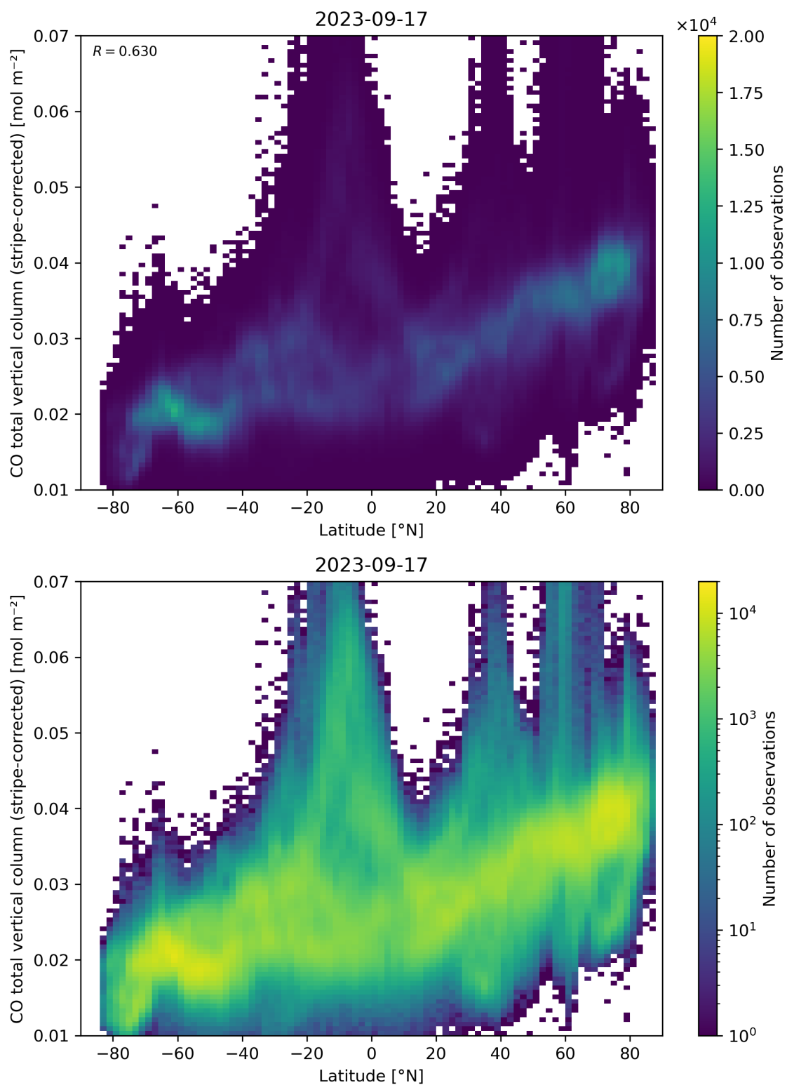
Figure 52: Scatter density plot of “Latitude” against “CO total vertical column (stripe-corrected)” for 2023-09-16 to 2023-09-18.
