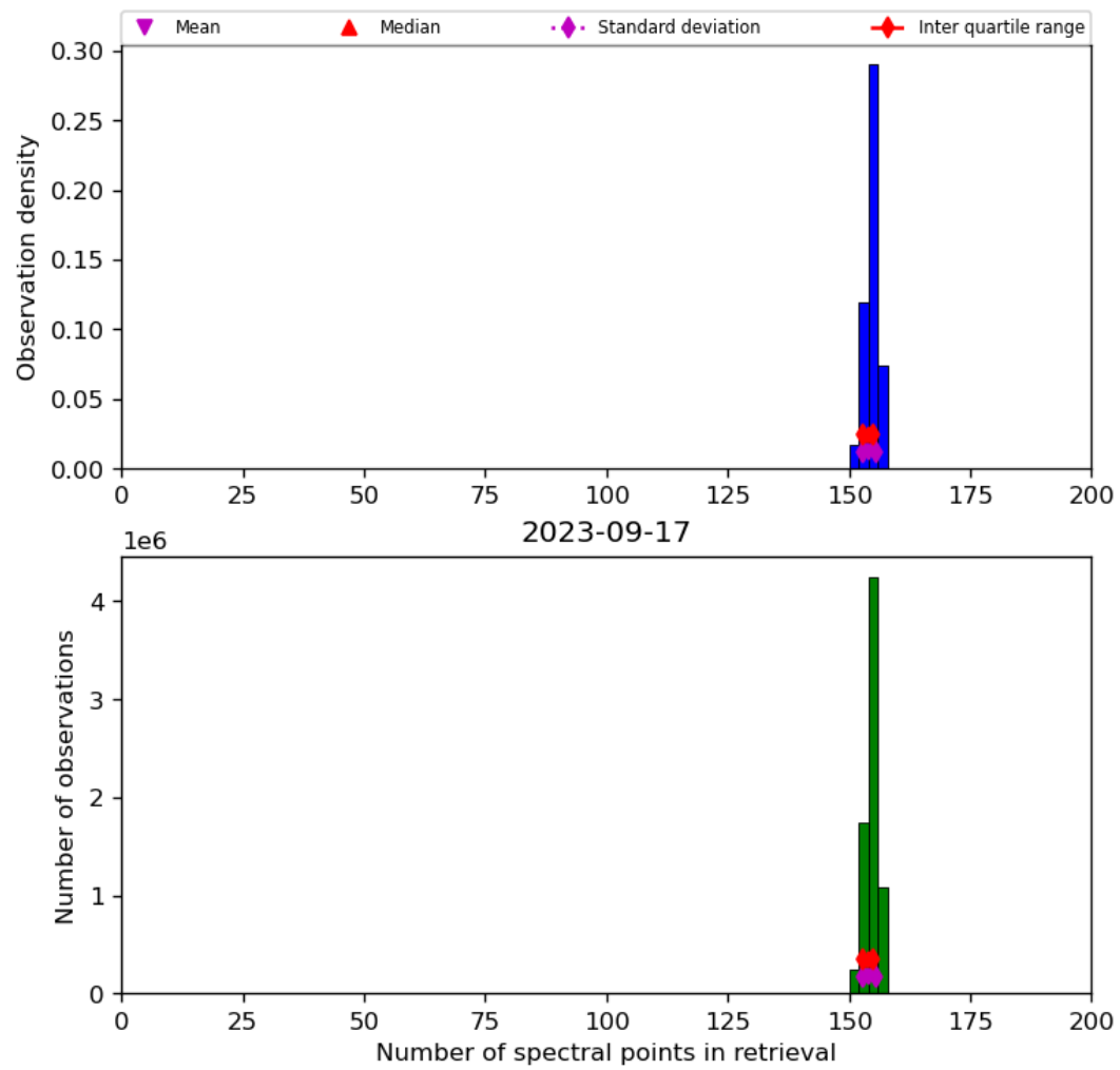
Figure 21: Histogram of “Number of spectral points in retrieval” for 2023-09-16 to 2023-09-18
