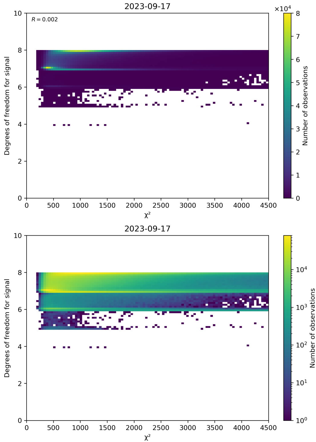
Figure 48: Scatter density plot of “ \chi^2 ” against “Degrees of freedom for signal” for 2023-09-16 to 2023-09-18.
