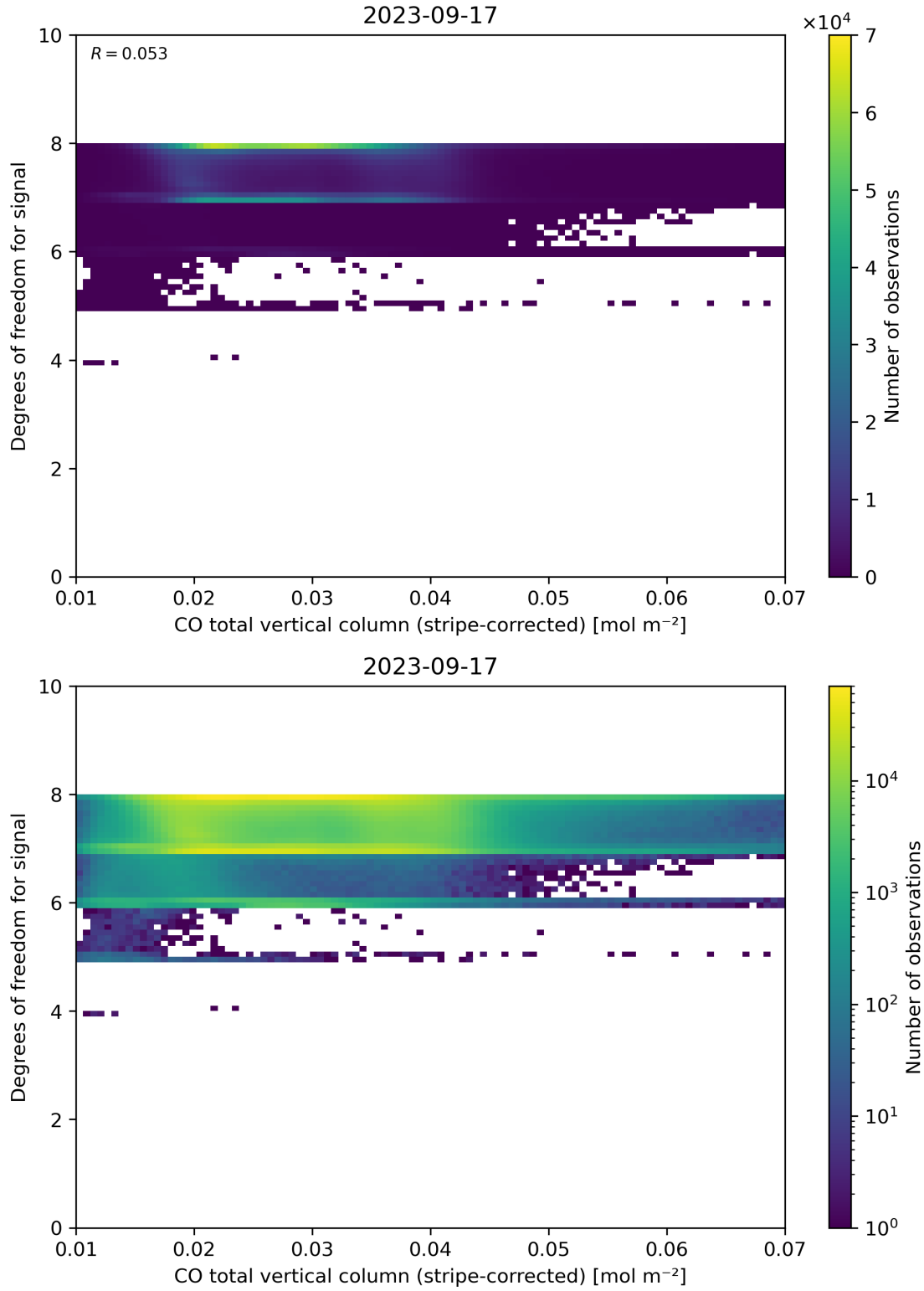
Figure 38: Scatter density plot of “CO total vertical column (stripe-corrected)” against “Degrees of freedom for signal” for 2023-09-16 to 2023-09-18.
