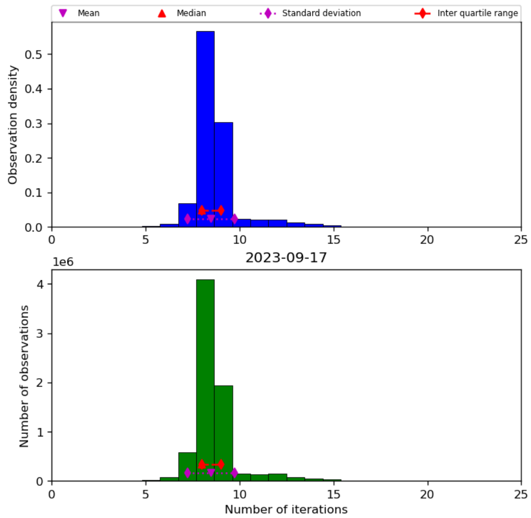
Figure 24: Histogram of “Number of iterations” for 2023-09-16 to 2023-09-18
