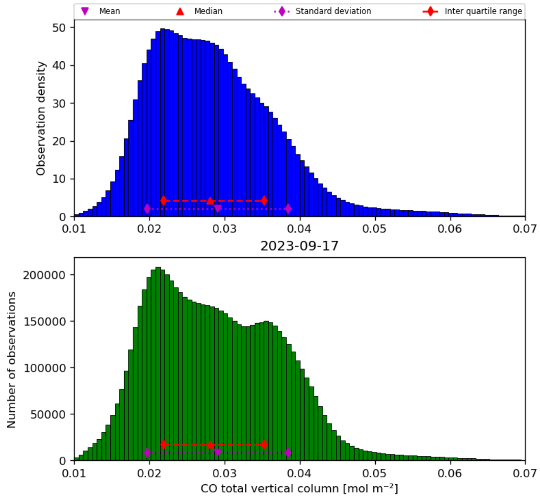
Figure 18: Histogram of “CO total vertical column” for 2023-09-16 to 2023-09-18
