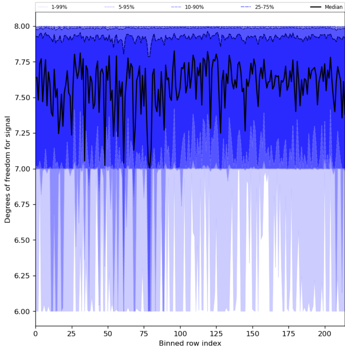
Figure 31: Along track statistics of “Degrees of freedom for signal” for 2023-09-16 to 2023-09-18
