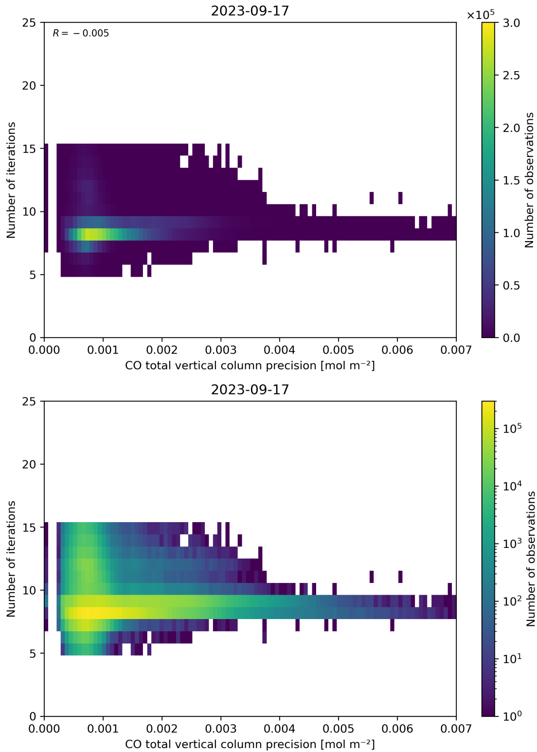
Figure 46: Scatter density plot of “CO total vertical column precision” against “Number of iterations” for 2023-09-16 to 2023-09-18.
