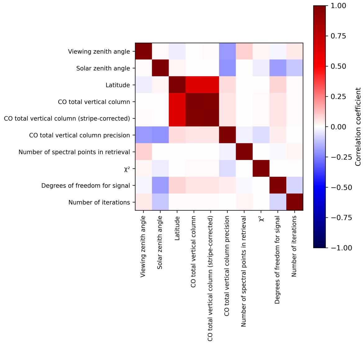
Figure 2: Map of correlation matrix for 2023-09-16 to 2023-09-18.
