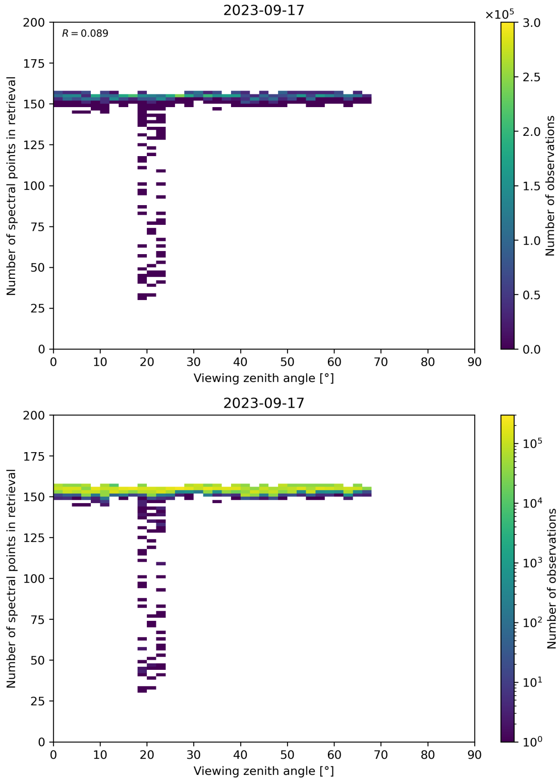
Figure 76: Scatter density plot of “Viewing zenith angle” against “Number of spectral points in retrieval” for 2023-09-16 to 2023-09-18.
