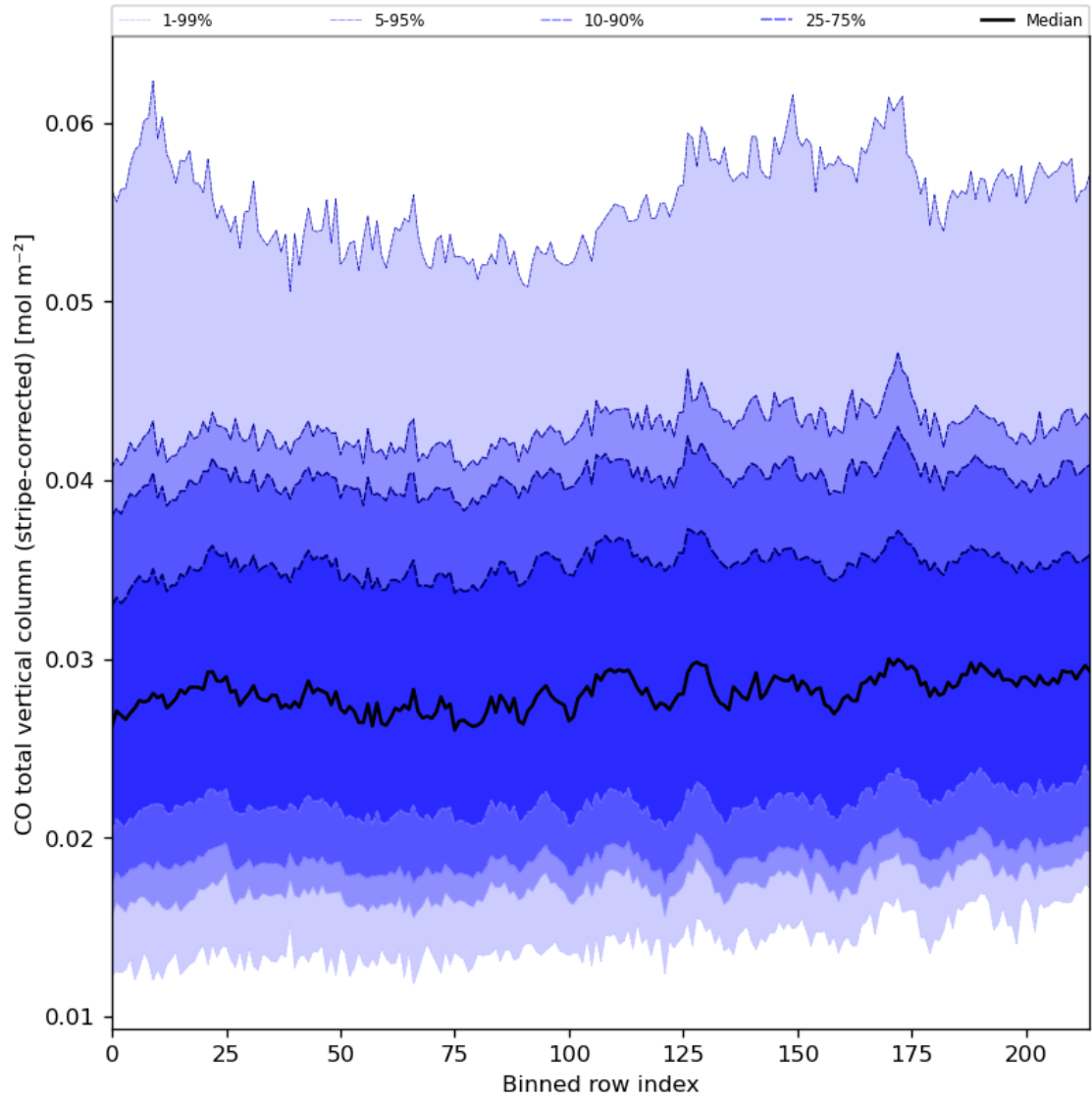
Figure 27: Along track statistics of “CO total vertical column (stripe-corrected)” for 2023-09-16 to 2023-09-18
