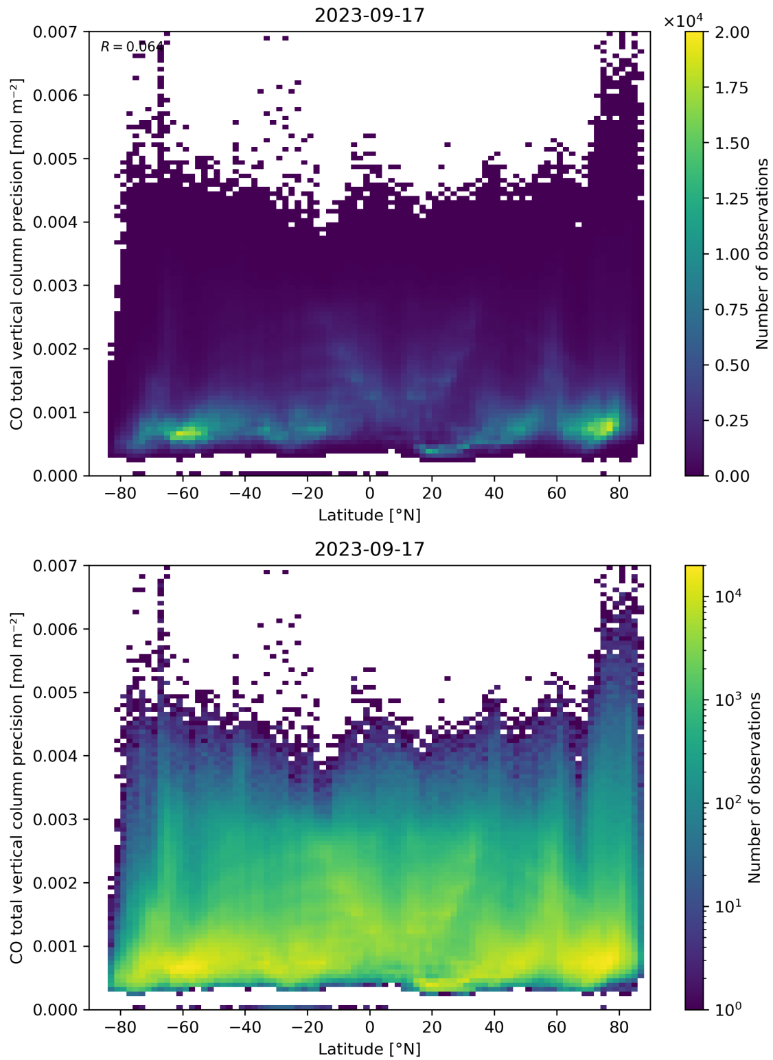
Figure 53: Scatter density plot of “Latitude” against “CO total vertical column precision” for 2023-09-16 to 2023-09-18.
