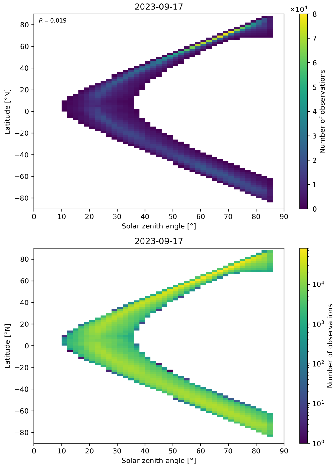
Figure 66: Scatter density plot of “Solar zenith angle” against “Latitude” for 2023-09-16 to 2023-09-18.
