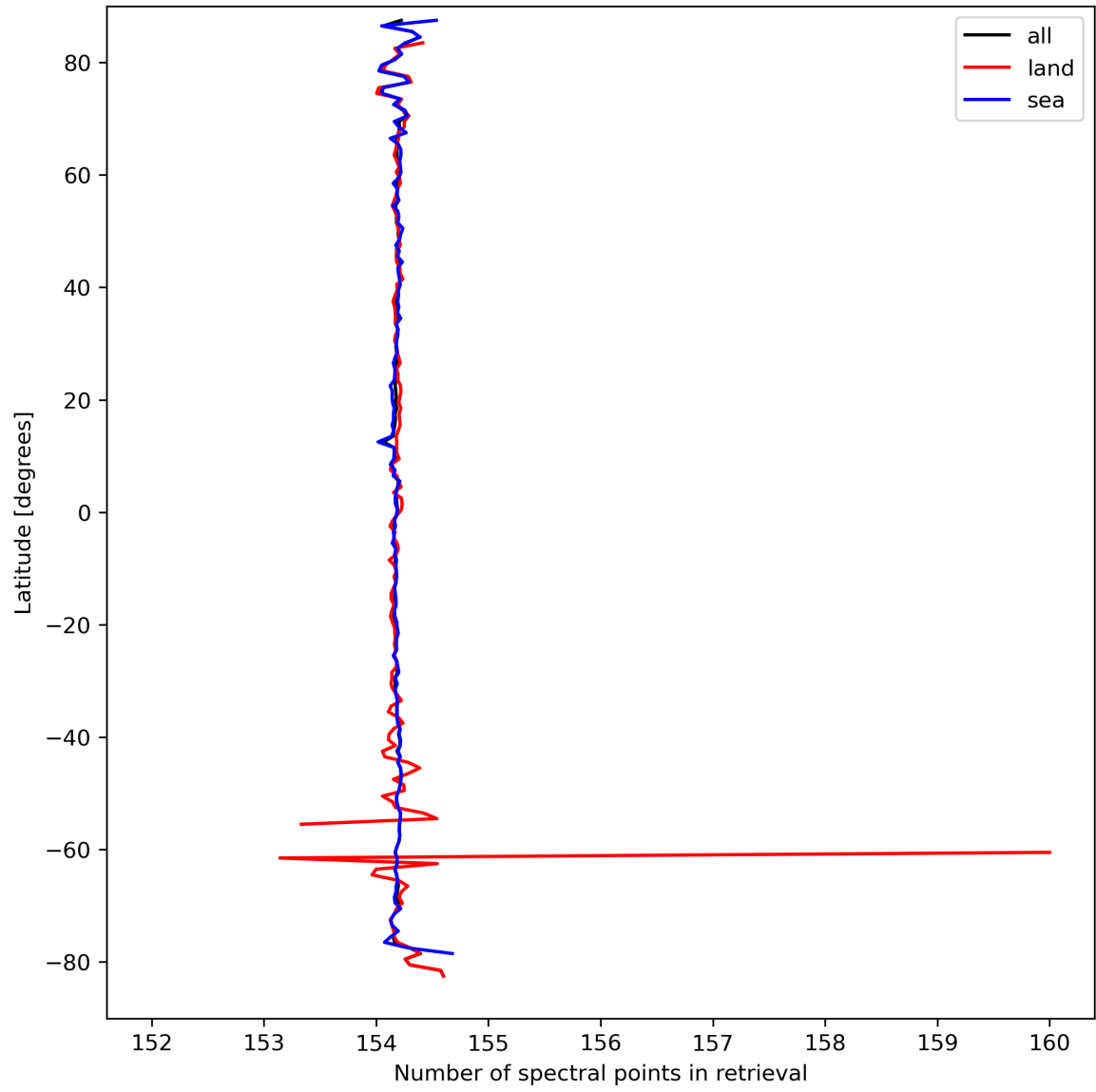
Figure 13: Zonal average of “Number of spectral points in retrieval” for 2023-09-16 to 2023-09-18.
