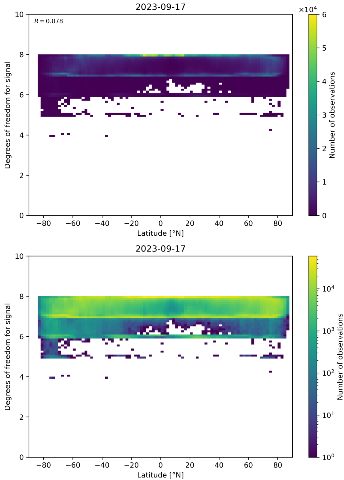
Figure 55: Scatter density plot of “Latitude” against “Degrees of freedom for signal” for 2023-09-16 to 2023-09-18.
