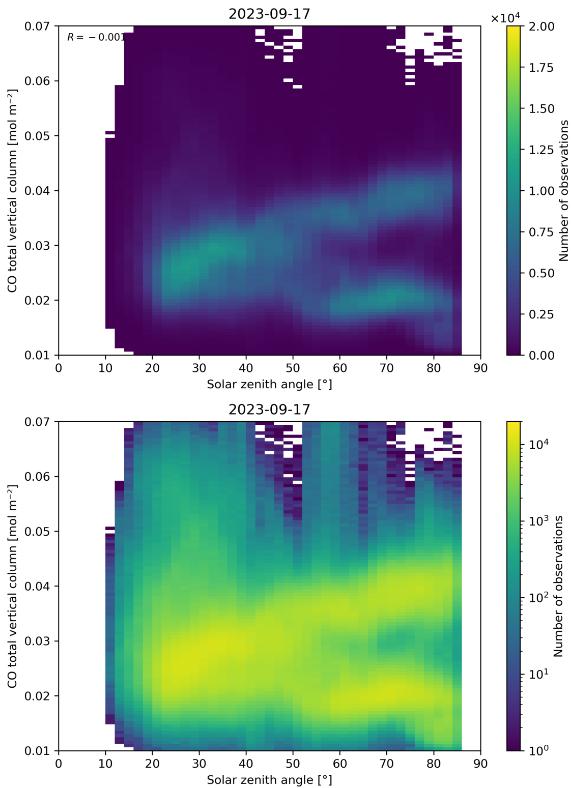
Figure 61: Scatter density plot of “Solar zenith angle” against “CO total vertical column” for 2023-09-16 to 2023-09-18.
