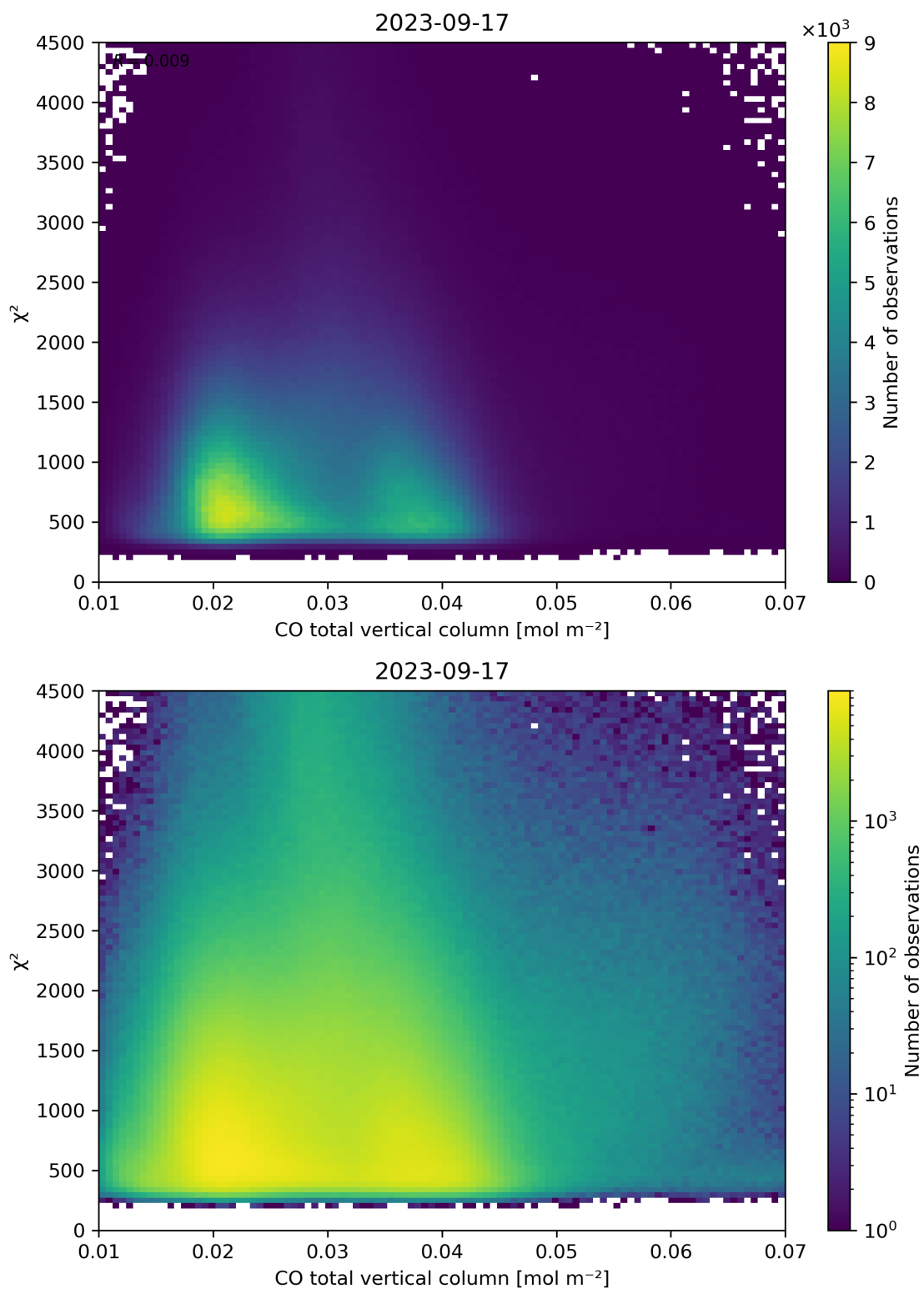
Figure 35: Scatter density plot of “CO total vertical column” against “ \chi^2 ” for 2023-09-16 to 2023-09-18.
