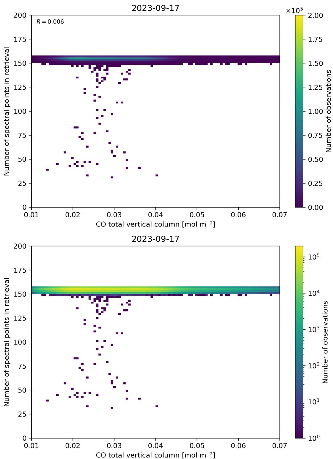
Figure 43: Scatter density plot of “CO total vertical column” against “Number of spectral points in retrieval” for 2023-09-16 to 2023-09-18.
