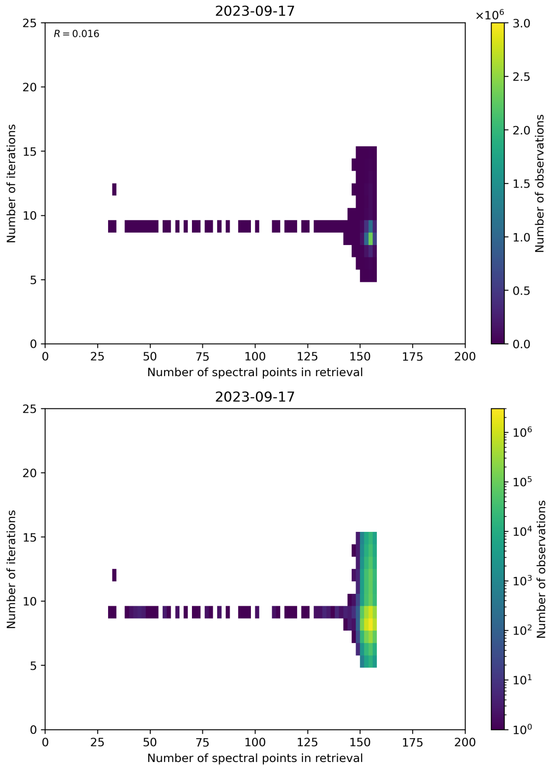
Figure 60: Scatter density plot of “Number of spectral points in retrieval” against “Number of iterations” for 2023-09-16 to 2023-09-18.
