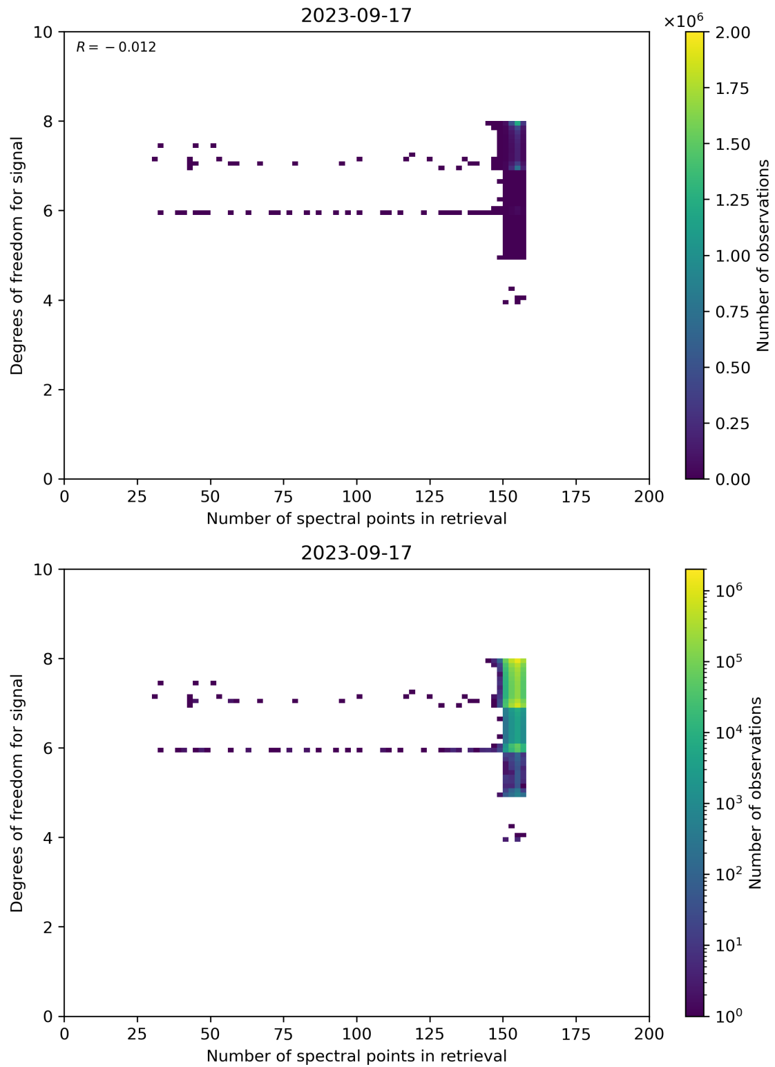
Figure 59: Scatter density plot of “Number of spectral points in retrieval” against “Degrees of freedom for signal” for 2023-09-16 to 2023-09-18.
