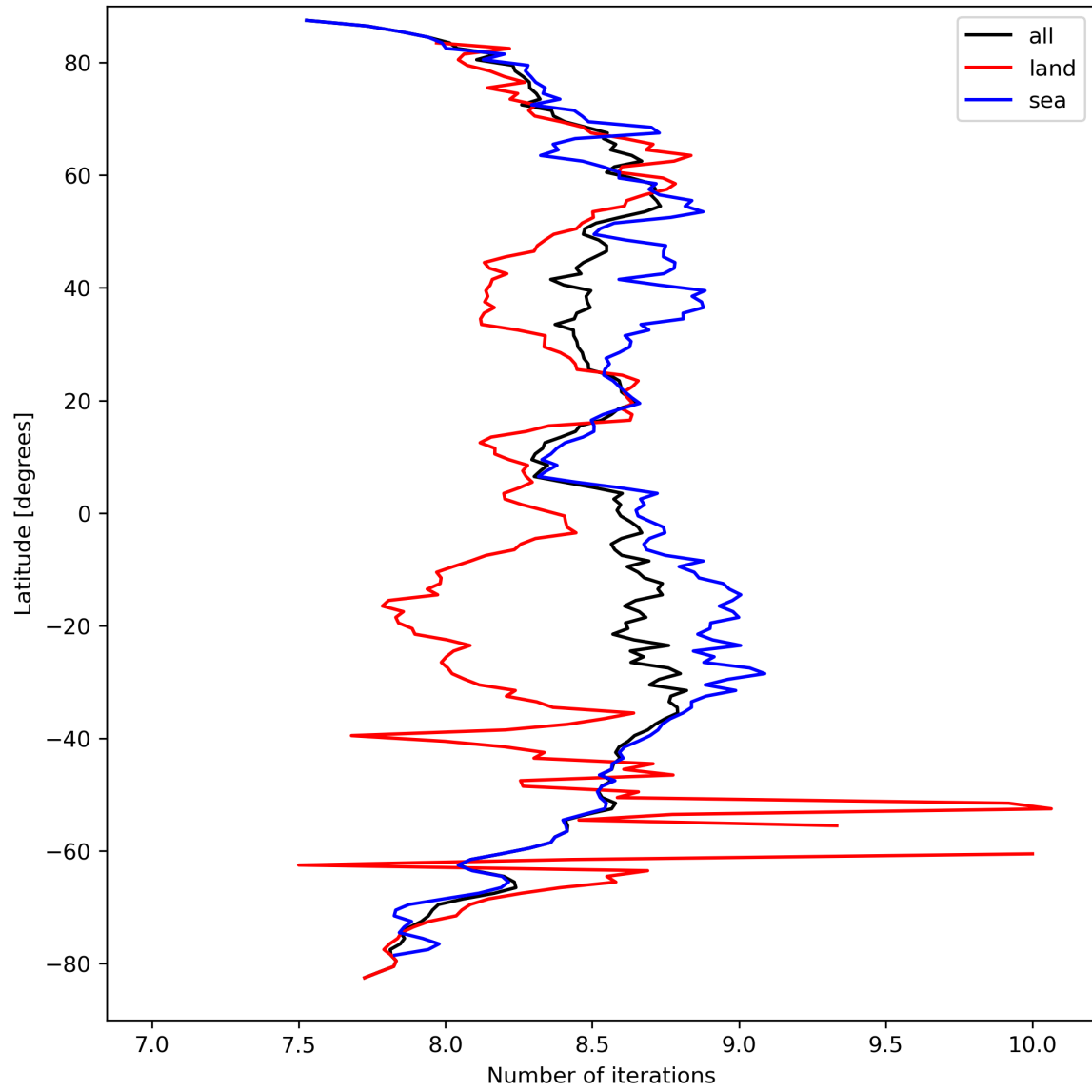
Figure 16: Zonal average of “Number of iterations” for 2023-09-16 to 2023-09-18.
