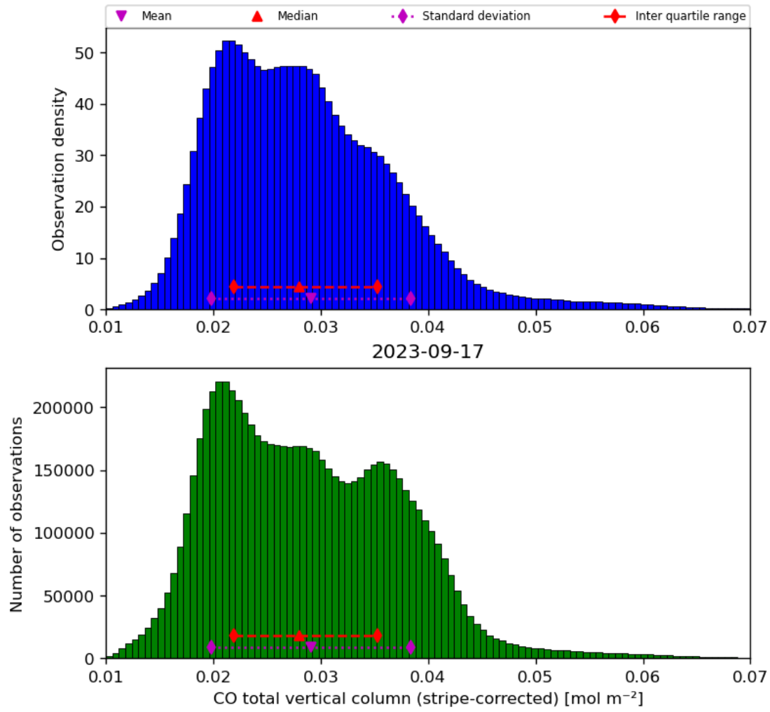
Figure 19: Histogram of “CO total vertical column (stripe-corrected)” for 2023-09-16 to 2023-09-18
