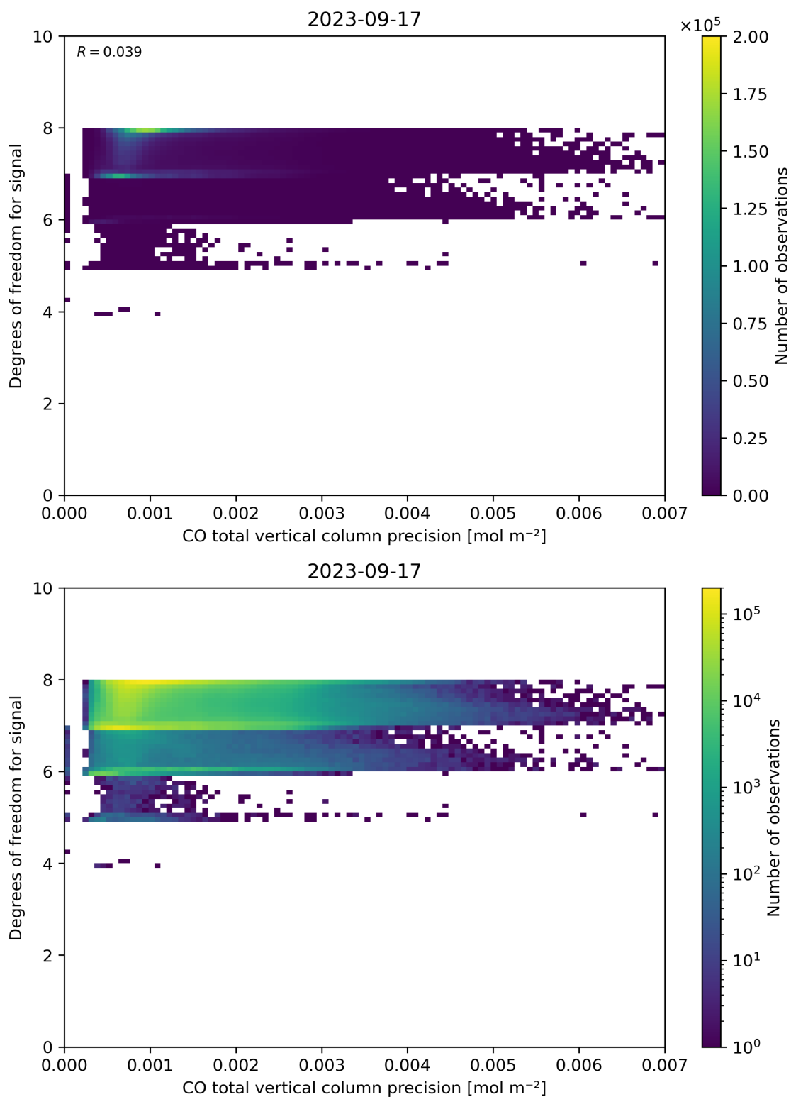
Figure 45: Scatter density plot of “CO total vertical column precision” against “Degrees of freedom for signal” for 2023-09-16 to 2023-09-18.
