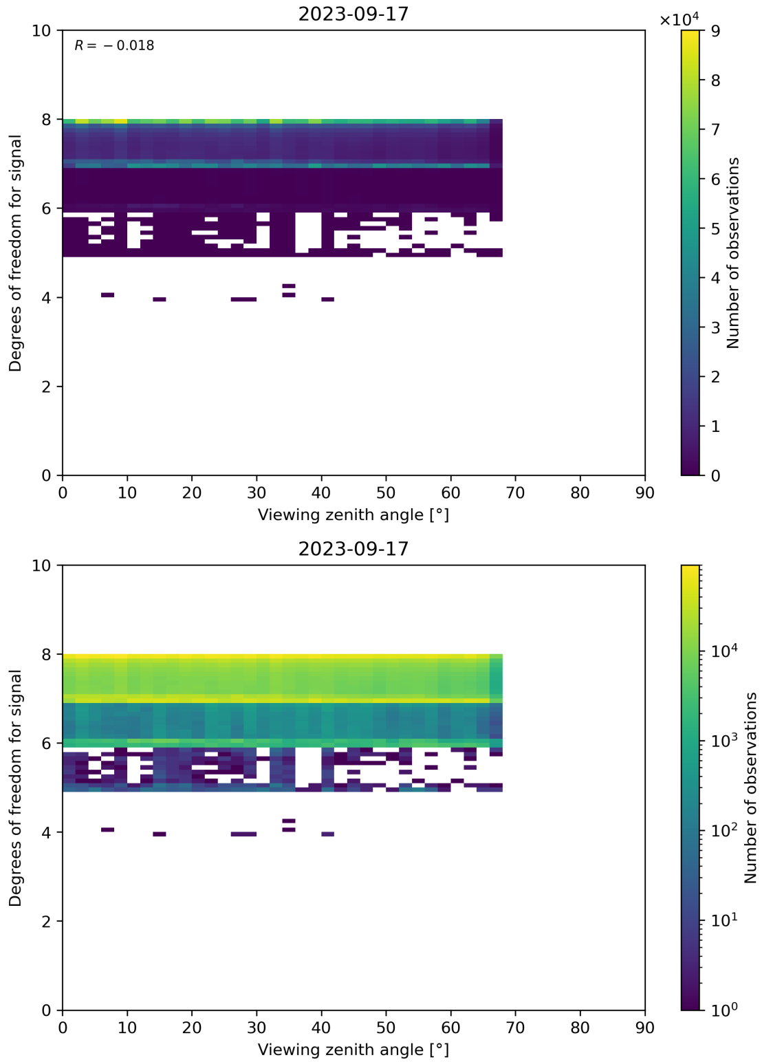
Figure 73: Scatter density plot of “Viewing zenith angle” against “Degrees of freedom for signal” for 2023-09-16 to 2023-09-18.
