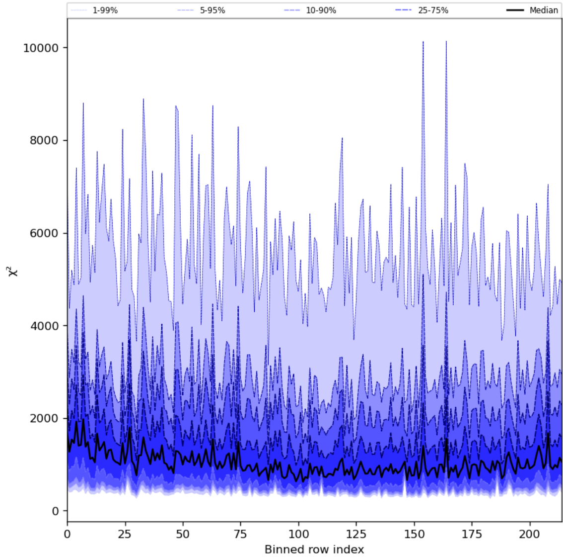
Figure 30: Along track statistics of “ \chi^2 ” for 2023-09-16 to 2023-09-18
