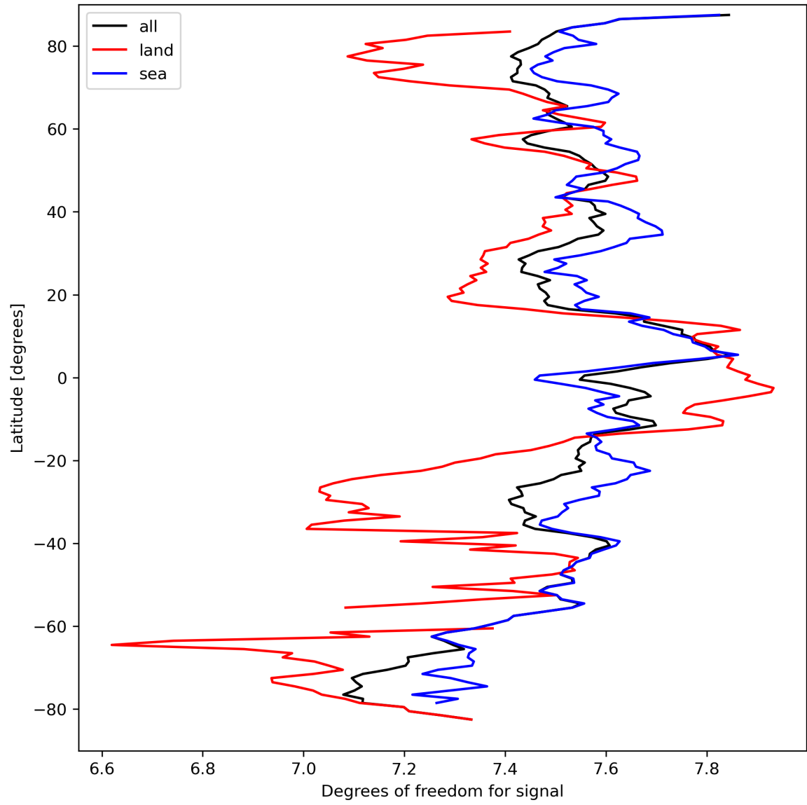
Figure 15: Zonal average of “Degrees of freedom for signal” for 2023-09-16 to 2023-09-18.
