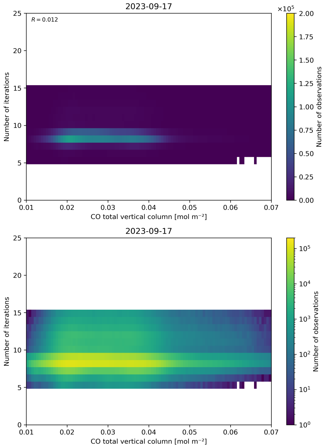
Figure 42: Scatter density plot of “CO total vertical column” against “Number of iterations” for 2023-09-16 to 2023-09-18.
