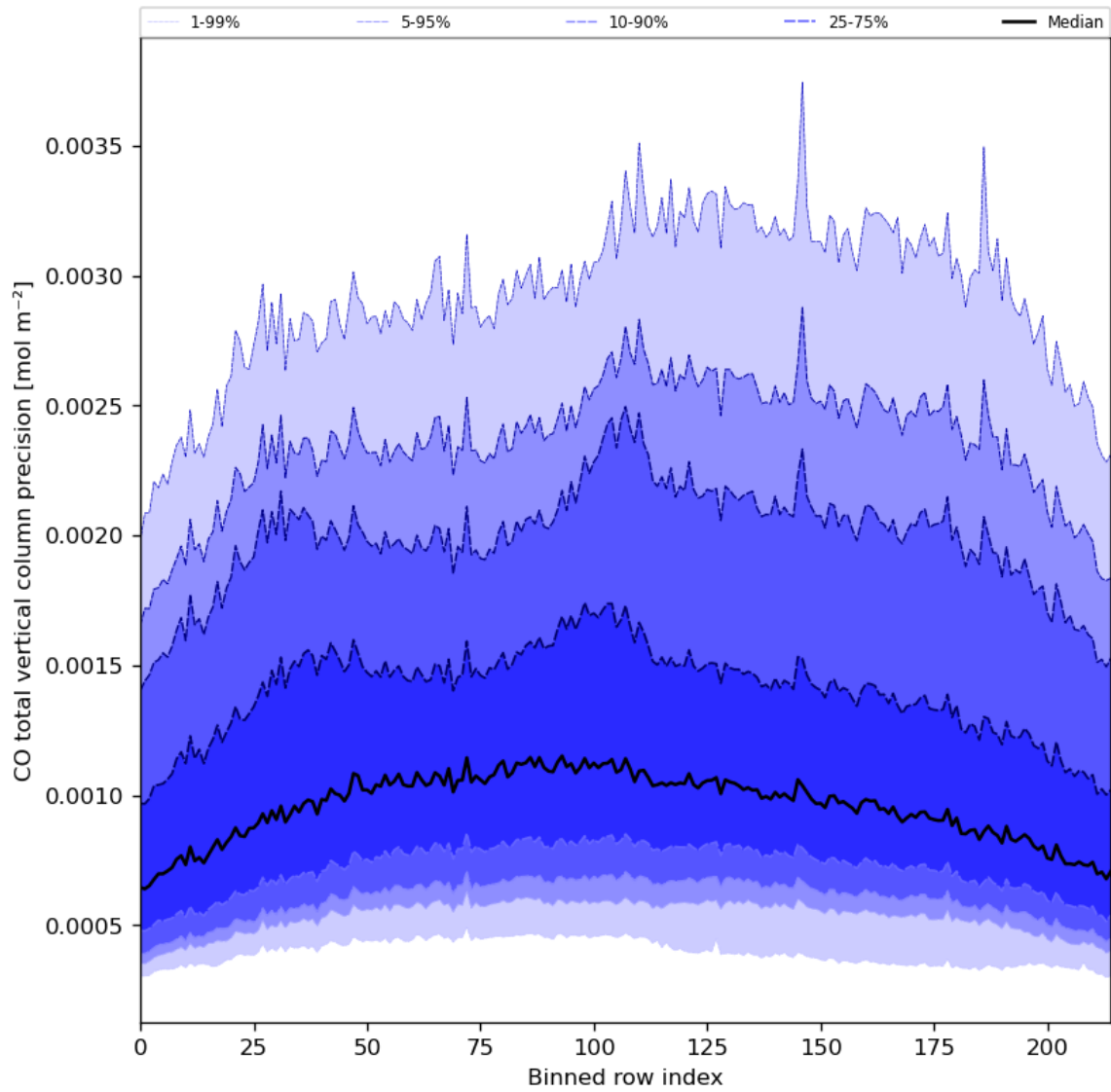
Figure 28: Along track statistics of “CO total vertical column precision” for 2023-09-16 to 2023-09-18
