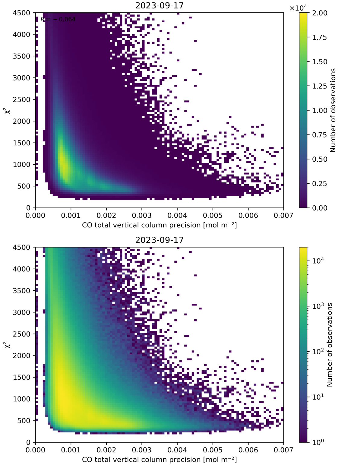
Figure 44: Scatter density plot of “CO total vertical column precision” against “ \chi^2 ” for 2023-09-16 to 2023-09-18.
