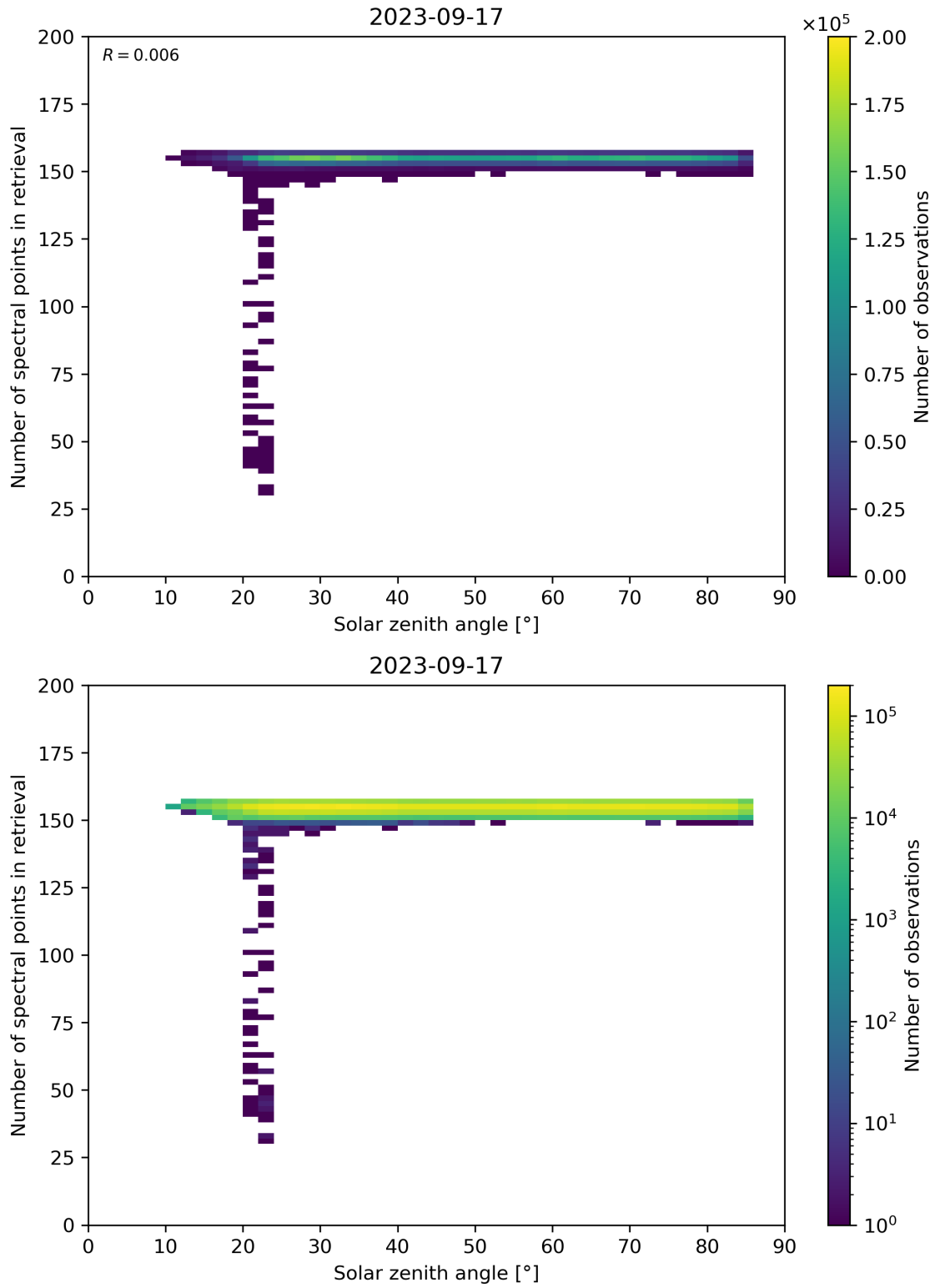
Figure 68: Scatter density plot of “Solar zenith angle” against “Number of spectral points in retrieval” for 2023-09-16 to 2023-09-18.
