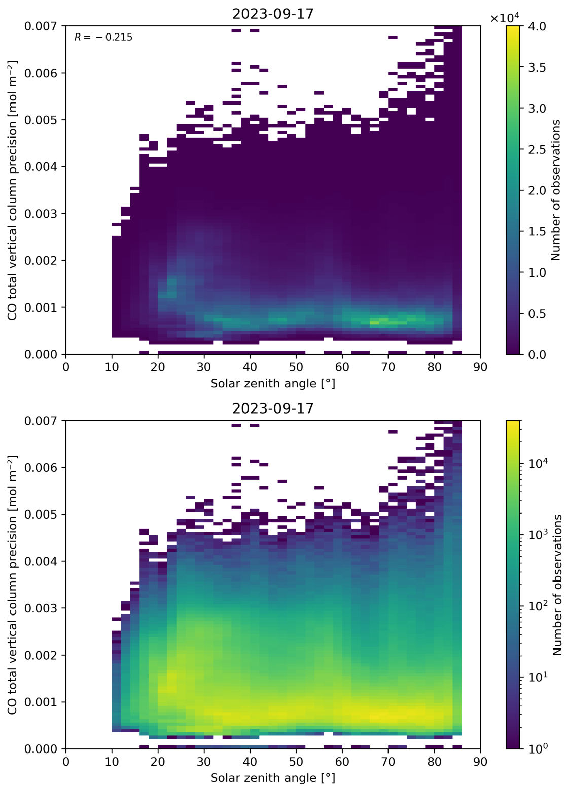
Figure 63: Scatter density plot of “Solar zenith angle” against “CO total vertical column precision” for 2023-09-16 to 2023-09-18.
