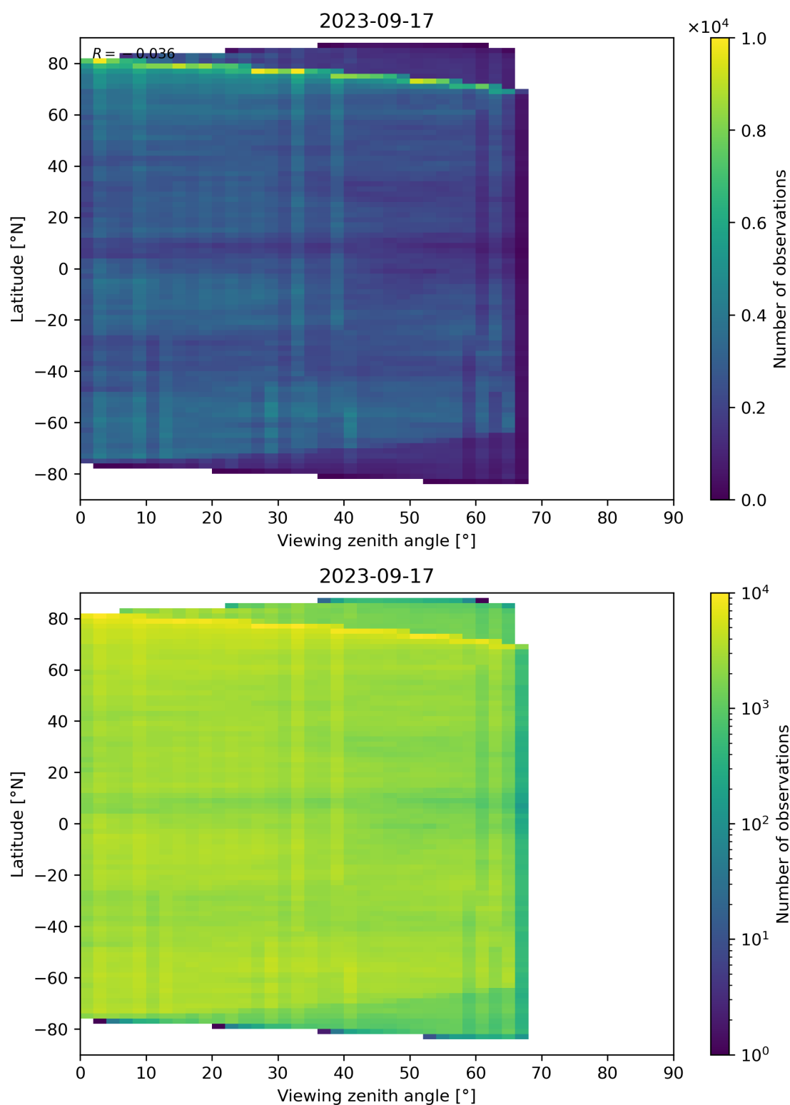
Figure 74: Scatter density plot of “Viewing zenith angle” against “Latitude” for 2023-09-16 to 2023-09-18.
