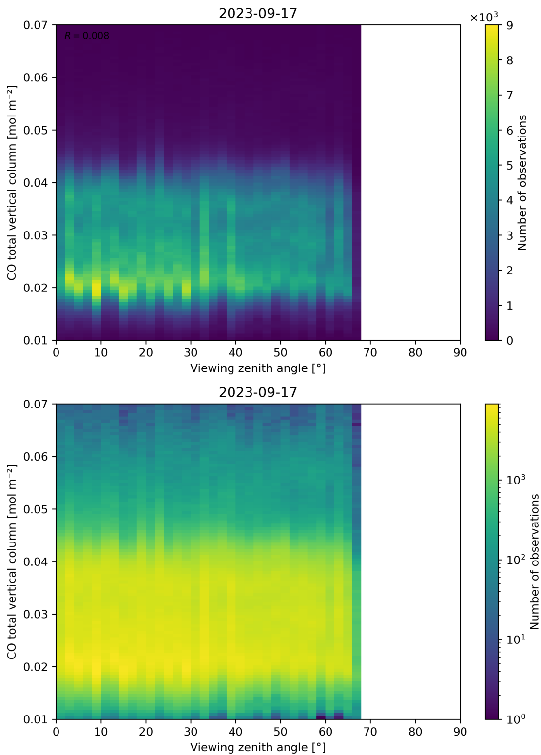
Figure 69: Scatter density plot of “Viewing zenith angle” against “CO total vertical column” for 2023-09-16 to 2023-09-18.
