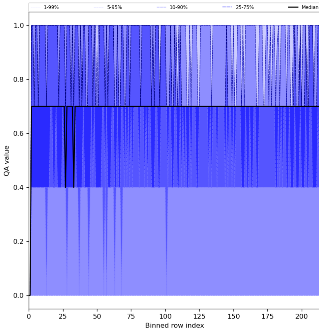
Figure 25: Along track statistics of “QA value” for 2023-09-16 to 2023-09-18
