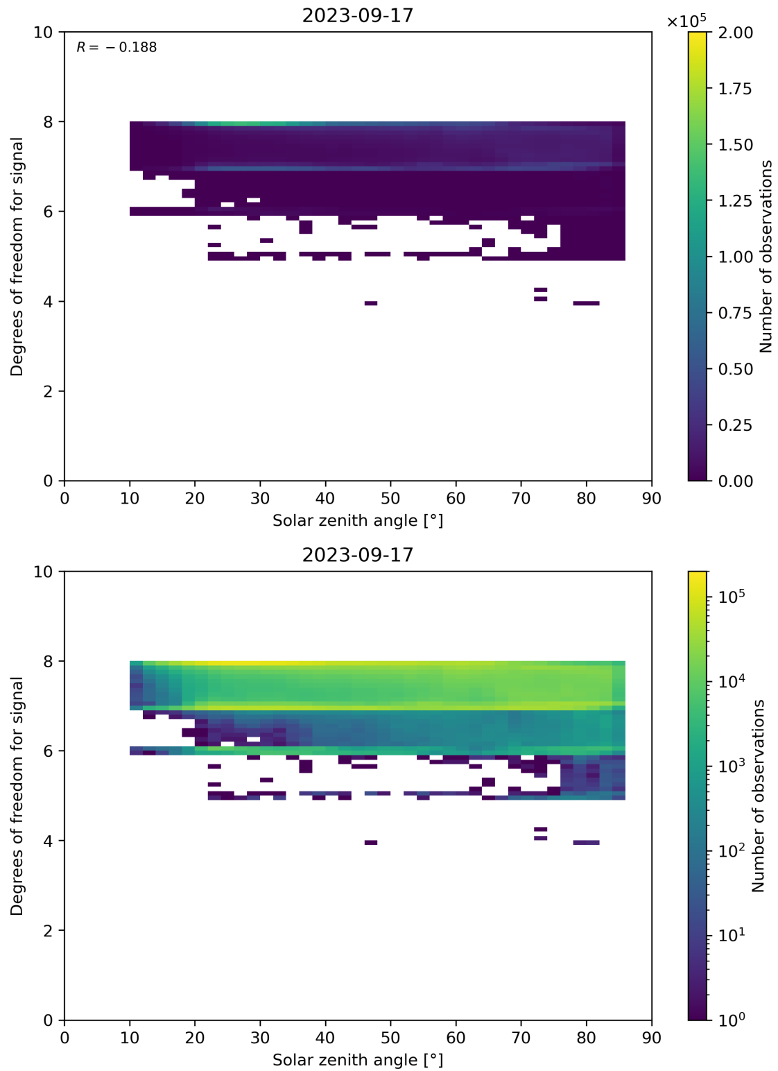
Figure 65: Scatter density plot of “Solar zenith angle” against “Degrees of freedom for signal” for 2023-09-16 to 2023-09-18.
