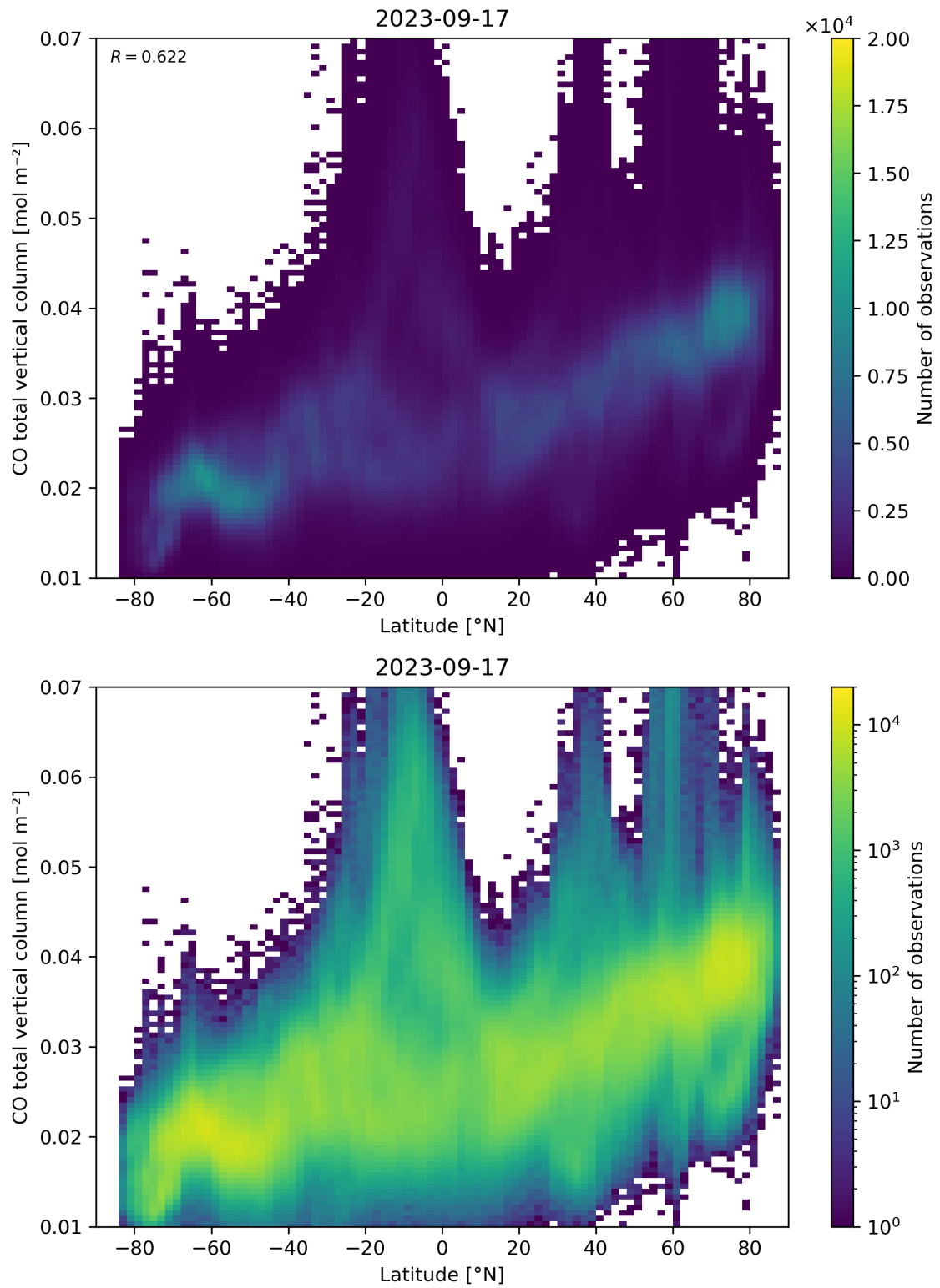
Figure 51: Scatter density plot of “Latitude” against “CO total vertical column” for 2023-09-16 to 2023-09-18.
