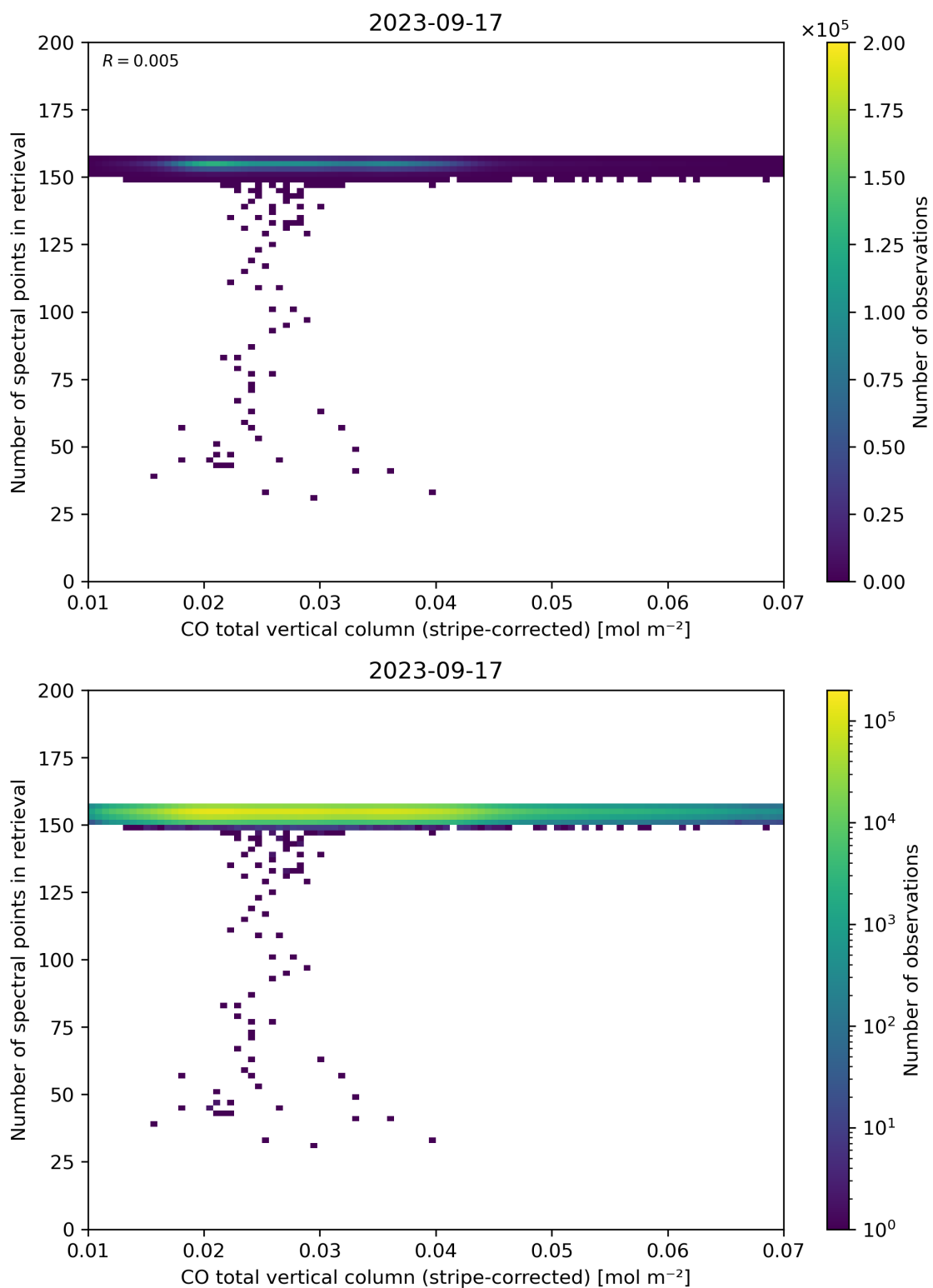
Figure 40: Scatter density plot of “CO total vertical column (stripe-corrected)” against “Number of spectral points in retrieval” for 2023-09-16 to 2023-09-18.
