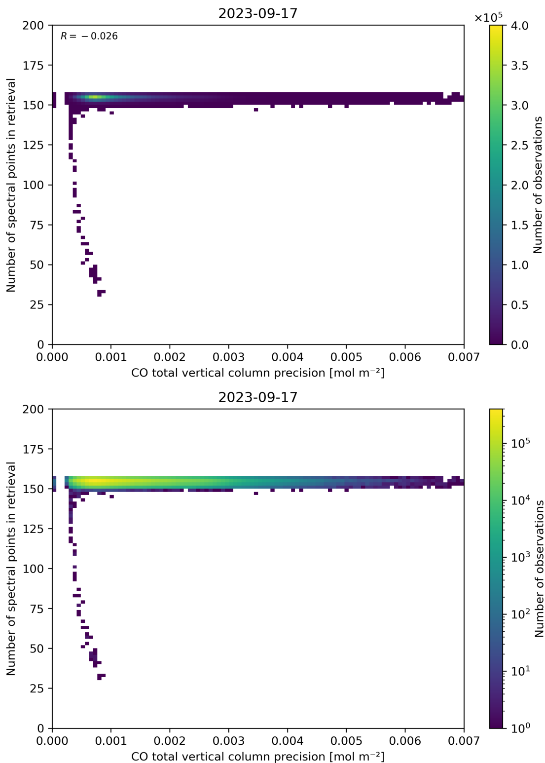
Figure 47: Scatter density plot of “CO total vertical column precision” against “Number of spectral points in retrieval” for 2023-09-16 to 2023-09-18.
