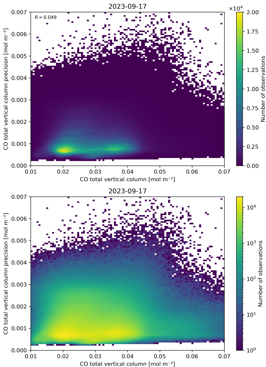
Figure 34: Scatter density plot of “CO total vertical column” against “CO total vertical column precision” for 2023-09-16 to 2023-09-18.
