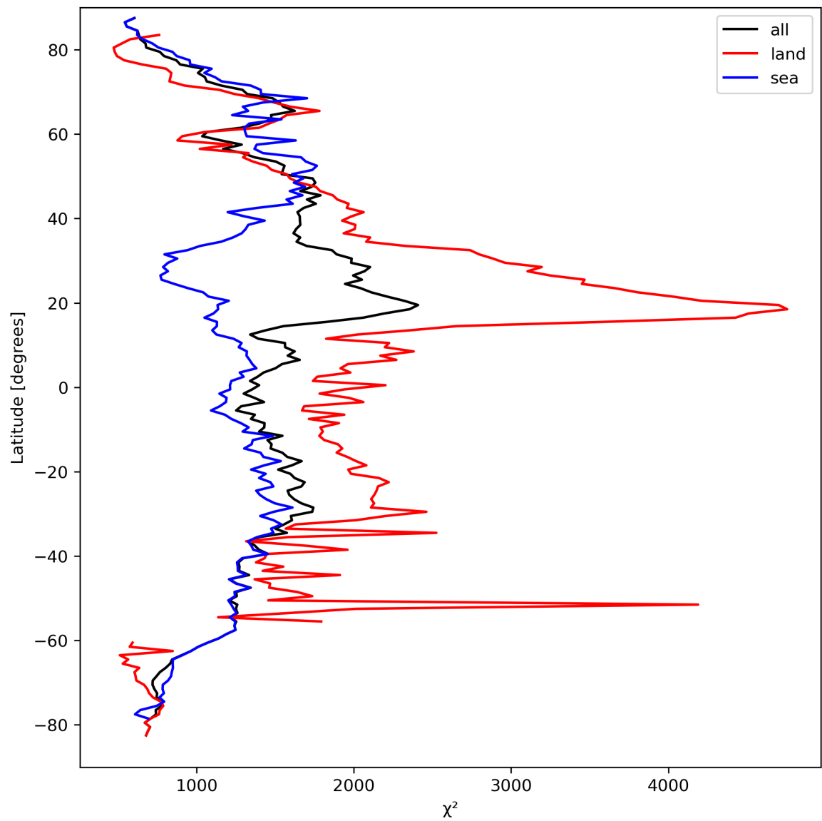
Figure 14: Zonal average of “ \chi^2 ” for 2023-09-16 to 2023-09-18.
