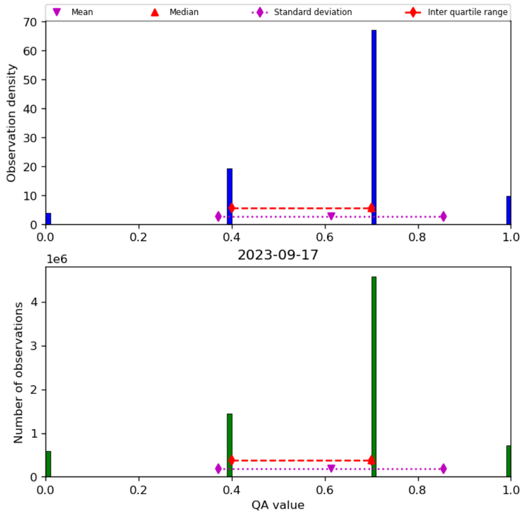
Figure 17: Histogram of “QA value” for 2023-09-16 to 2023-09-18
