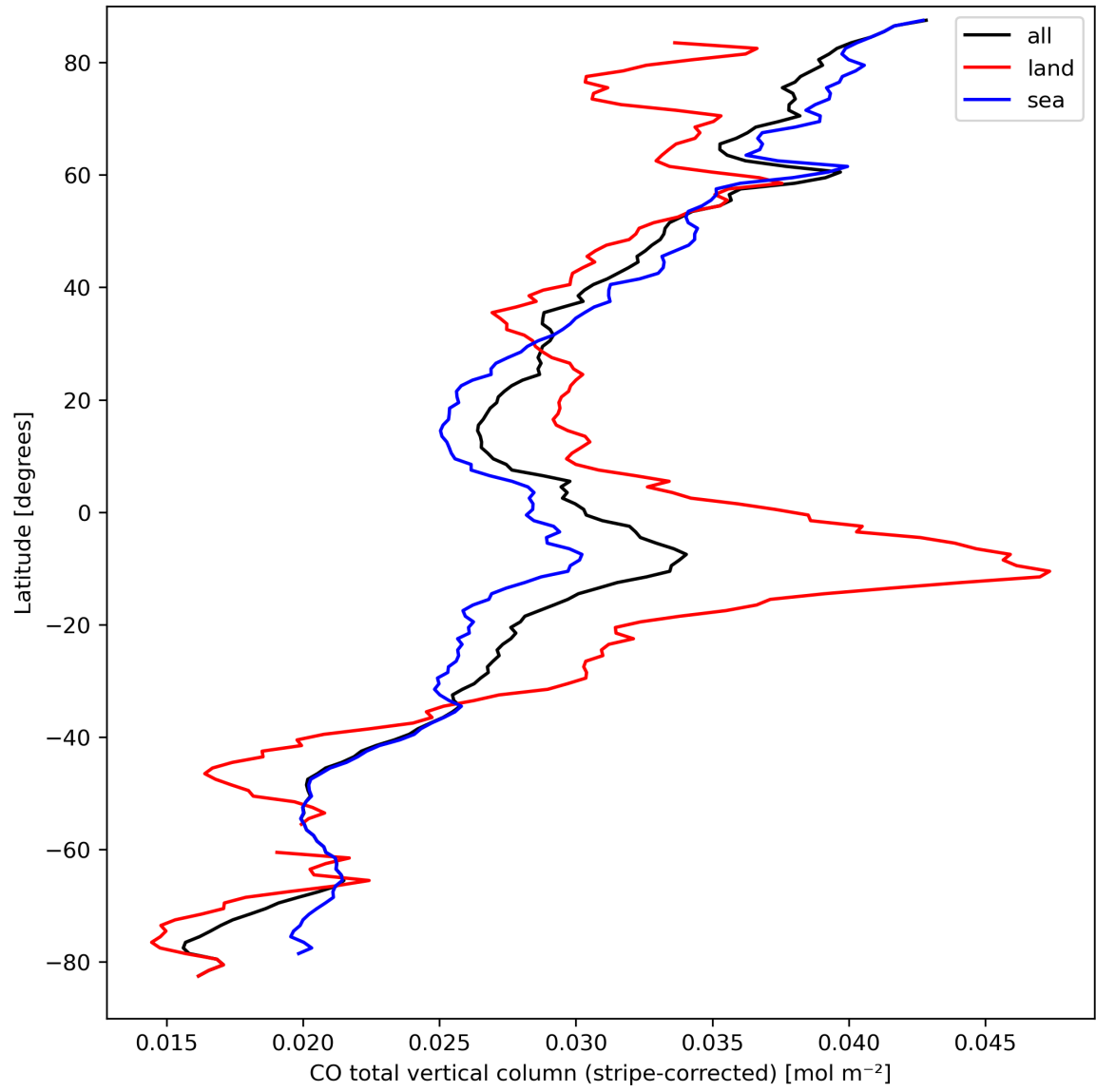
Figure 11: Zonal average of “CO total vertical column (stripe-corrected)” for 2023-09-16 to 2023-09-18.
