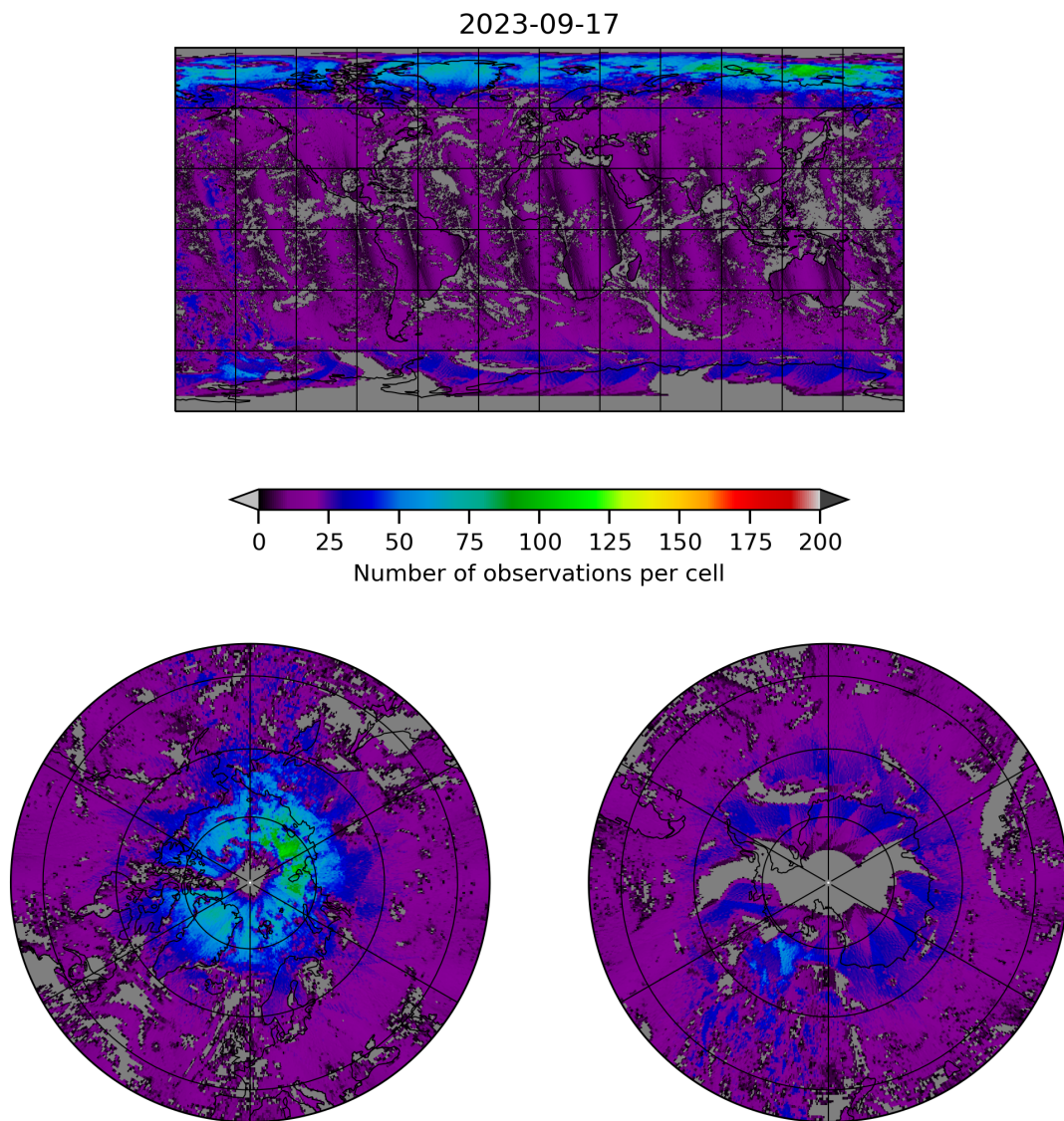
Figure 8: Map of the number of observations for 2023-09-16 to 2023-09-18
