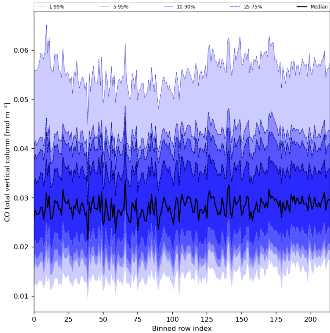
Figure 26: Along track statistics of “CO total vertical column” for 2023-09-16 to 2023-09-18
