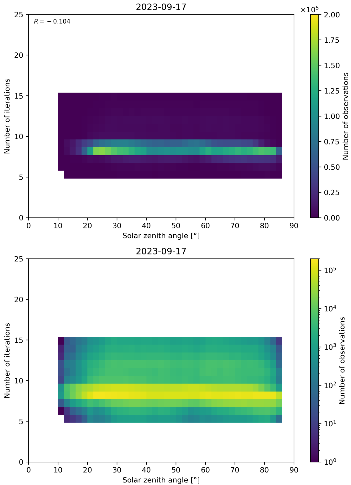
Figure 67: Scatter density plot of “Solar zenith angle” against “Number of iterations” for 2023-09-16 to 2023-09-18.
