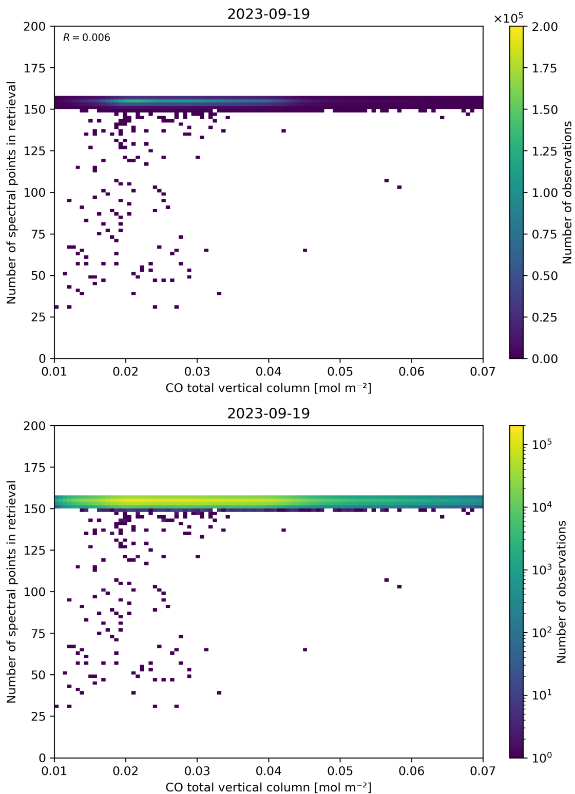
Figure 43: Scatter density plot of “CO total vertical column” against “Number of spectral points in retrieval” for 2023-09-18 to 2023-09-20.
