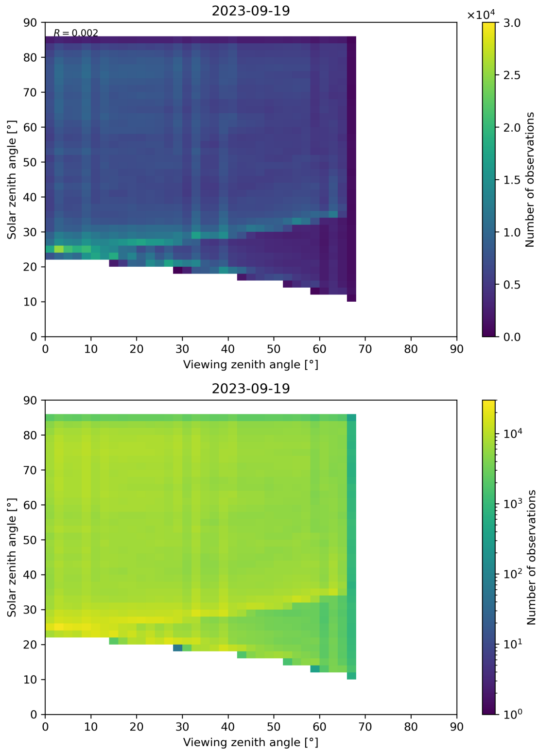
Figure 77: Scatter density plot of “Viewing zenith angle” against “Solar zenith angle” for 2023-09-18 to 2023-09-20.
