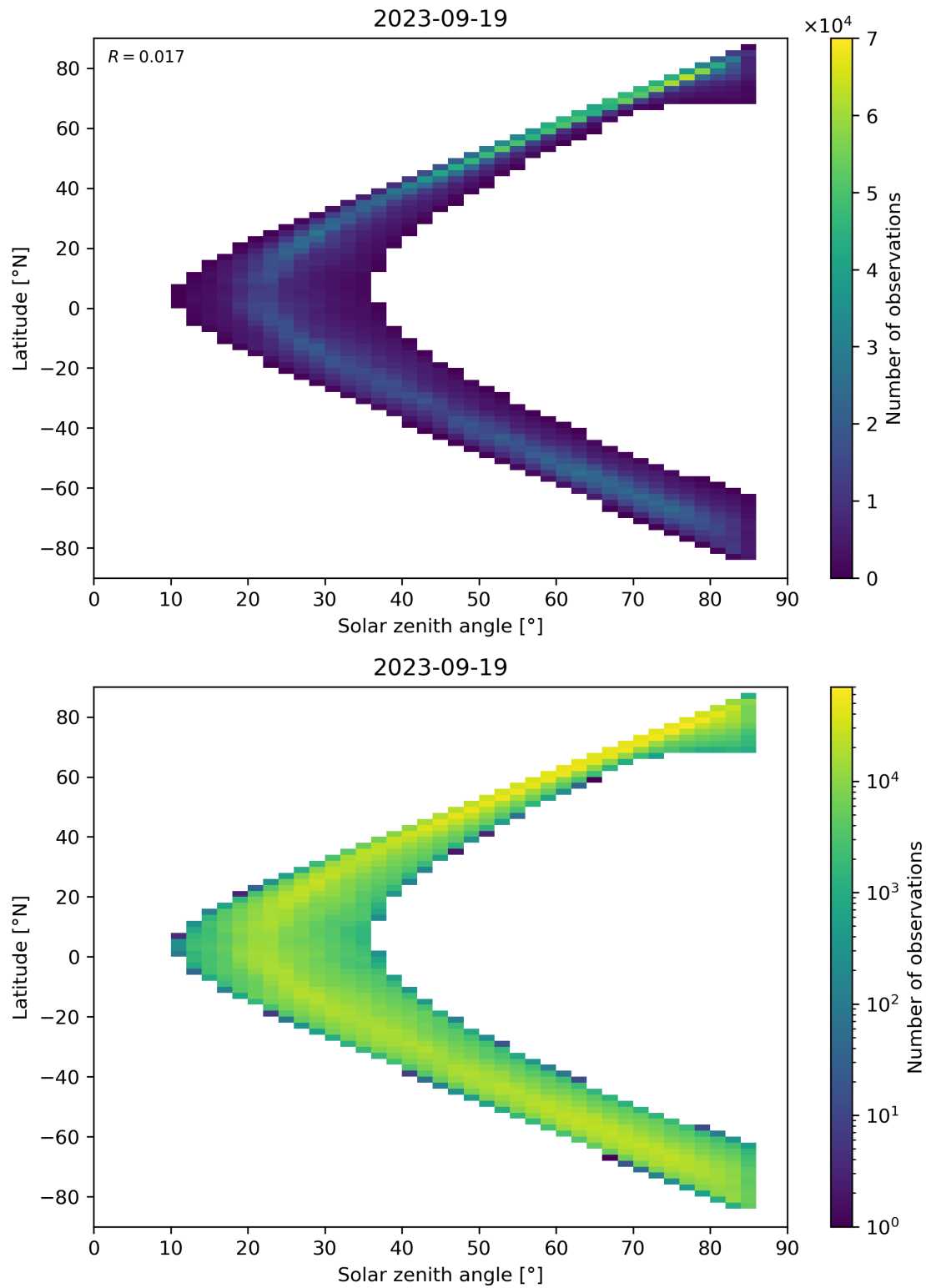
Figure 66: Scatter density plot of “Solar zenith angle” against “Latitude” for 2023-09-18 to 2023-09-20.
