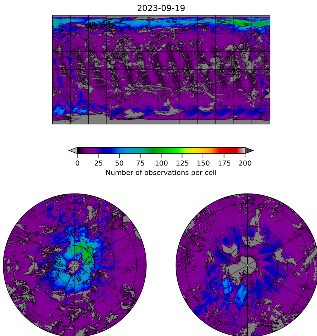
Figure 8: Map of the number of observations for 2023-09-18 to 2023-09-20
