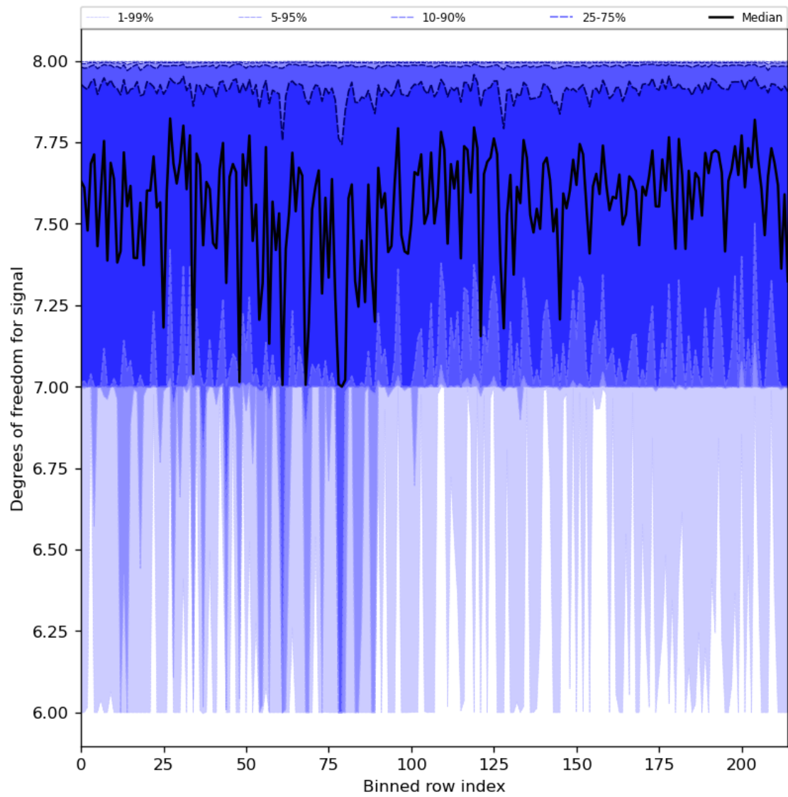
Figure 31: Along track statistics of “Degrees of freedom for signal” for 2023-09-18 to 2023-09-20
