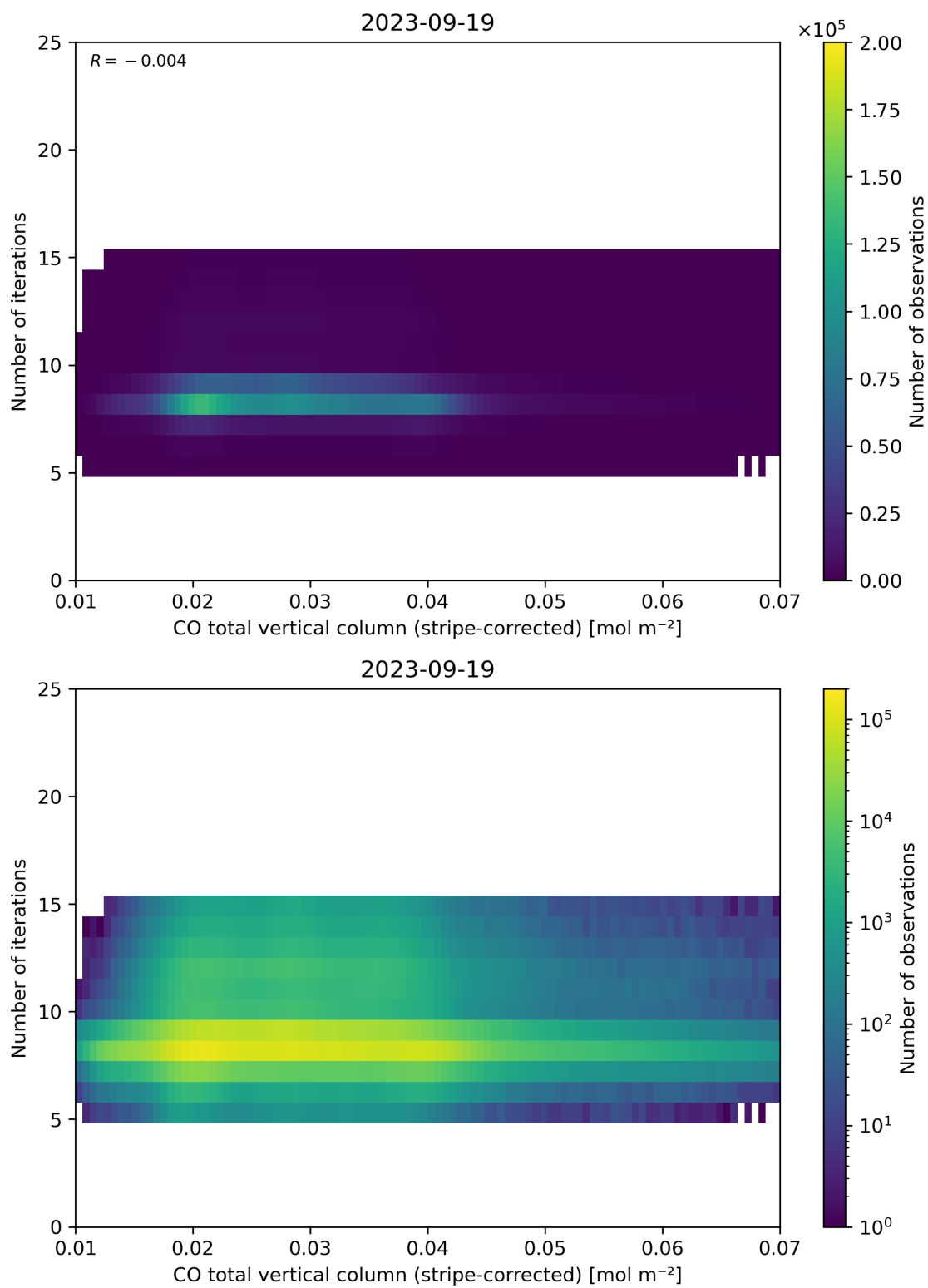
Figure 39: Scatter density plot of “CO total vertical column (stripe-corrected)” against “Number of iterations” for 2023-09-18 to 2023-09-20.
