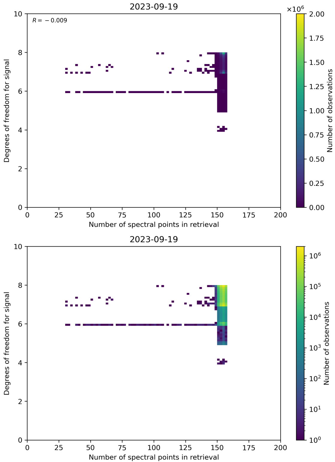
Figure 59: Scatter density plot of “Number of spectral points in retrieval” against “Degrees of freedom for signal” for 2023-09-18 to 2023-09-20.
