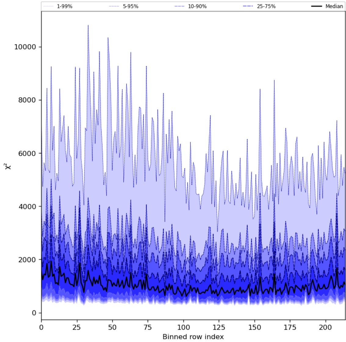
Figure 30: Along track statistics of “ \chi^2 ” for 2023-09-18 to 2023-09-20
