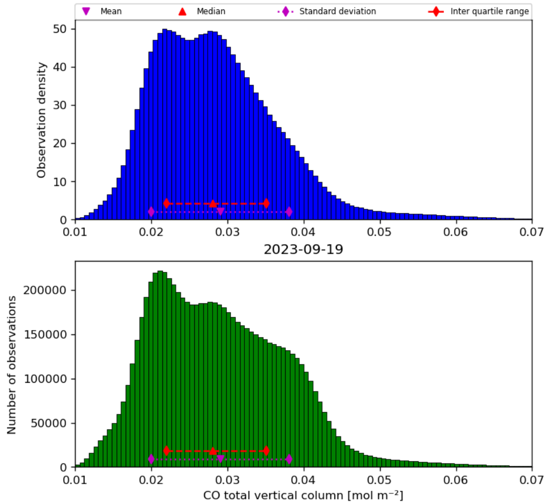
Figure 18: Histogram of “CO total vertical column” for 2023-09-18 to 2023-09-20
