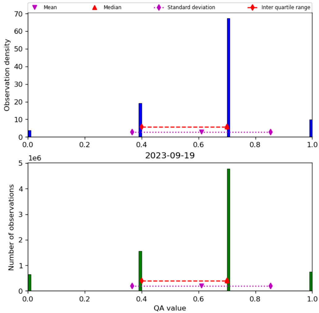
Figure 17: Histogram of “QA value” for 2023-09-18 to 2023-09-20
