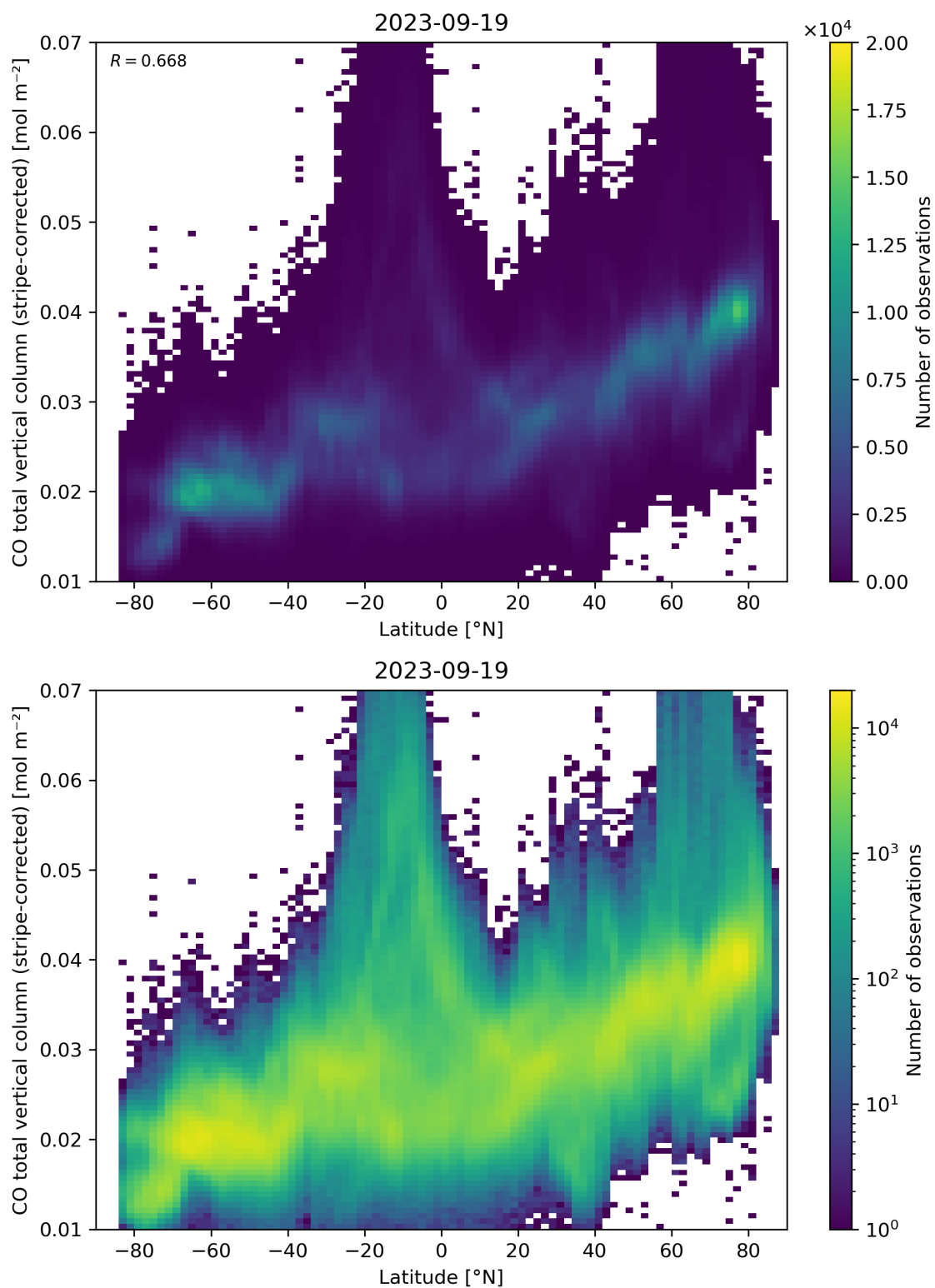
Figure 52: Scatter density plot of “Latitude” against “CO total vertical column (stripe-corrected)” for 2023-09-18 to 2023-09-20.
