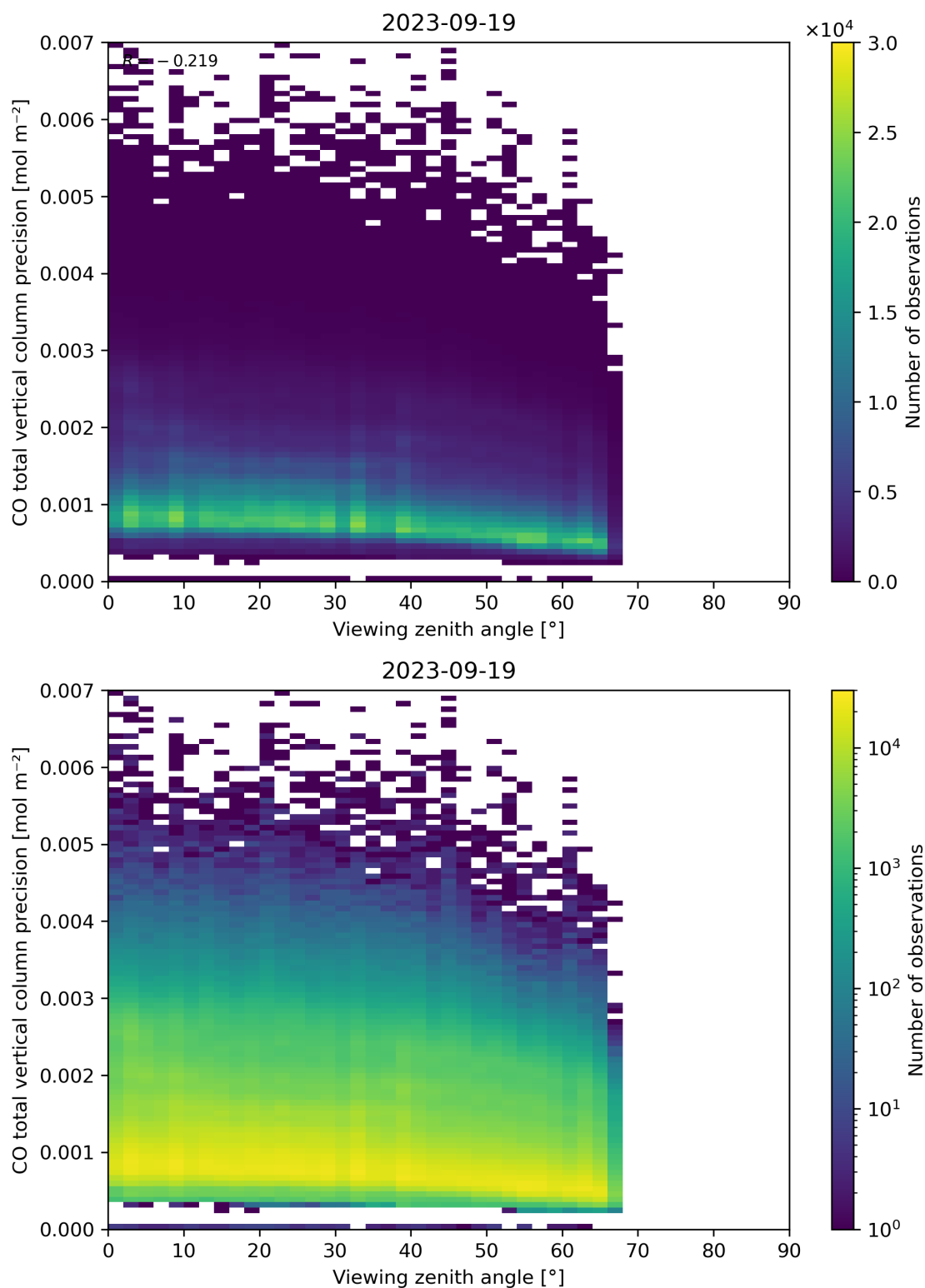
Figure 71: Scatter density plot of “Viewing zenith angle” against “CO total vertical column precision” for 2023-09-18 to 2023-09-20.
