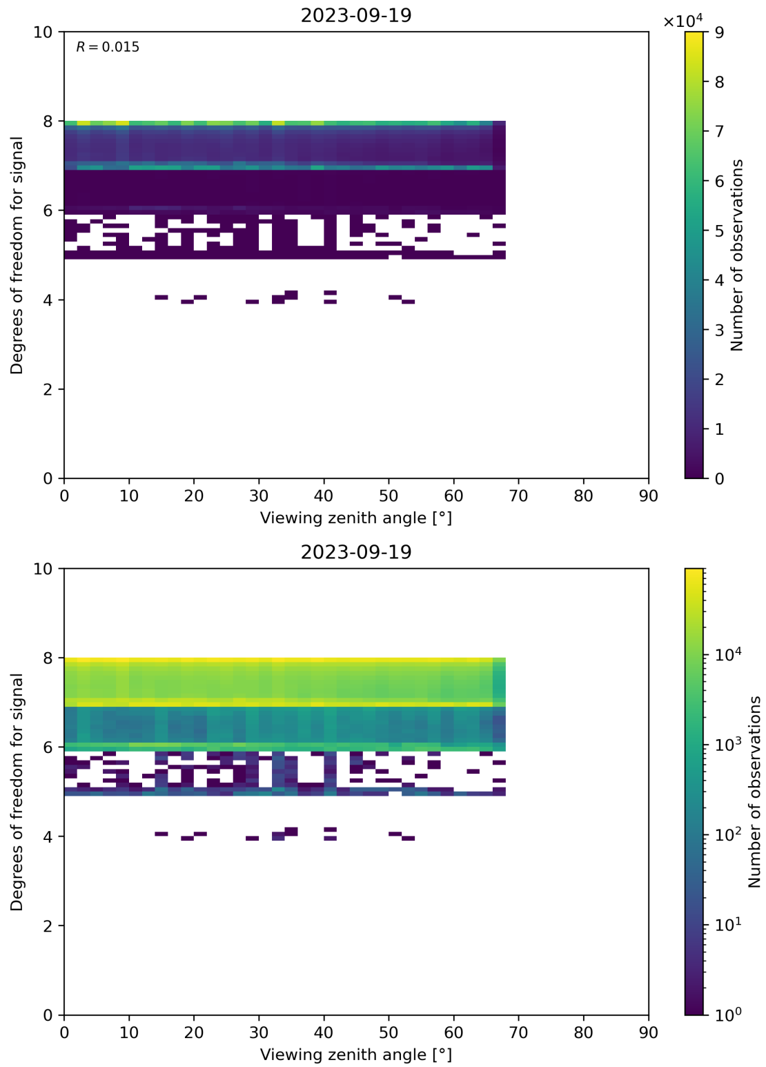
Figure 73: Scatter density plot of “Viewing zenith angle” against “Degrees of freedom for signal” for 2023-09-18 to 2023-09-20.
