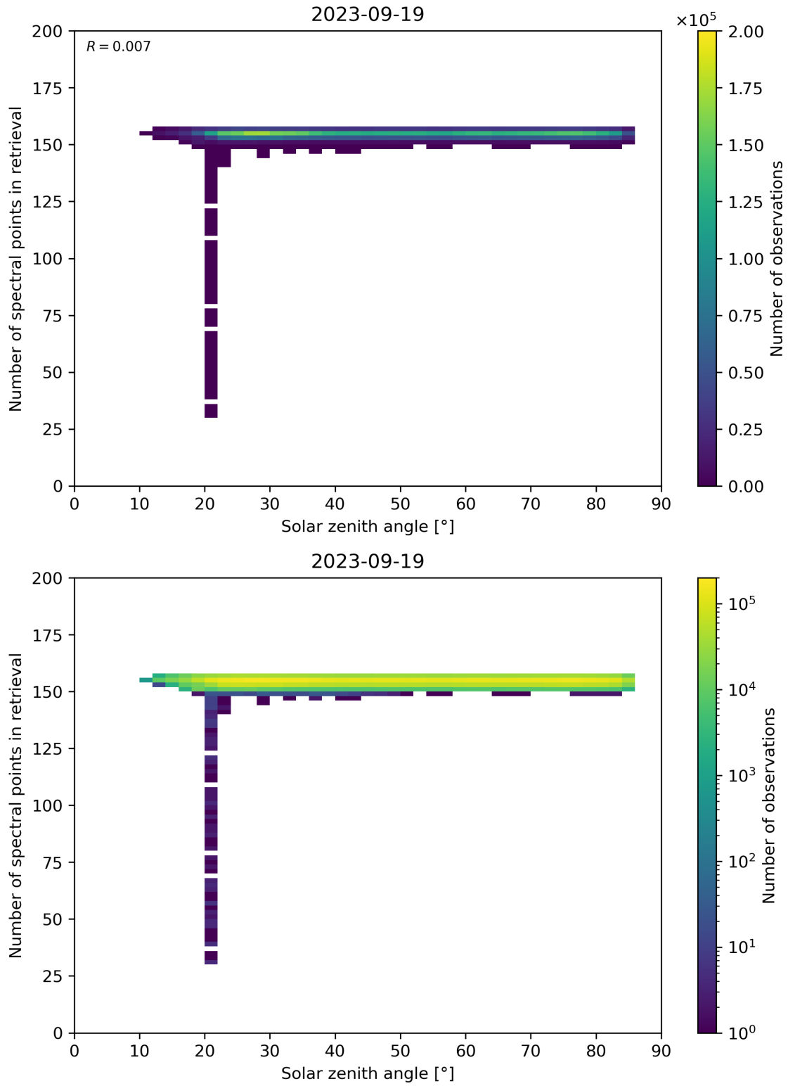
Figure 68: Scatter density plot of “Solar zenith angle” against “Number of spectral points in retrieval” for 2023-09-18 to 2023-09-20.
