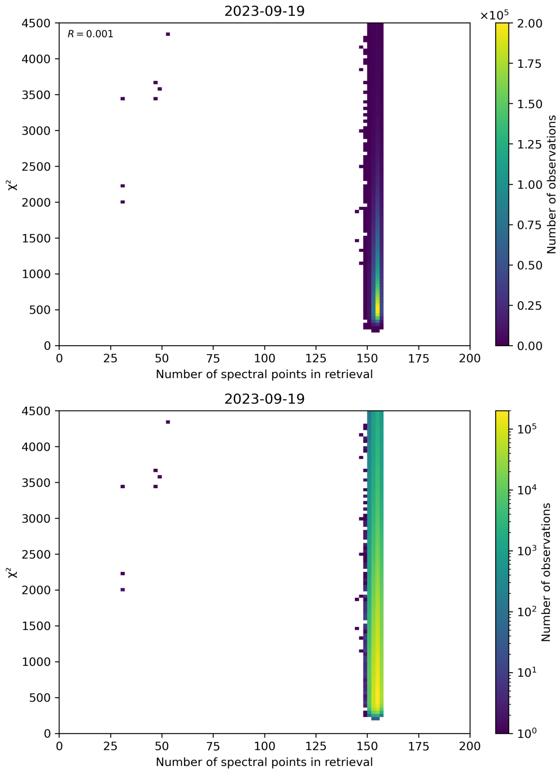
Figure 58: Scatter density plot of “Number of spectral points in retrieval” against “ \chi^2 ” for 2023-09-18 to 2023-09-20.
