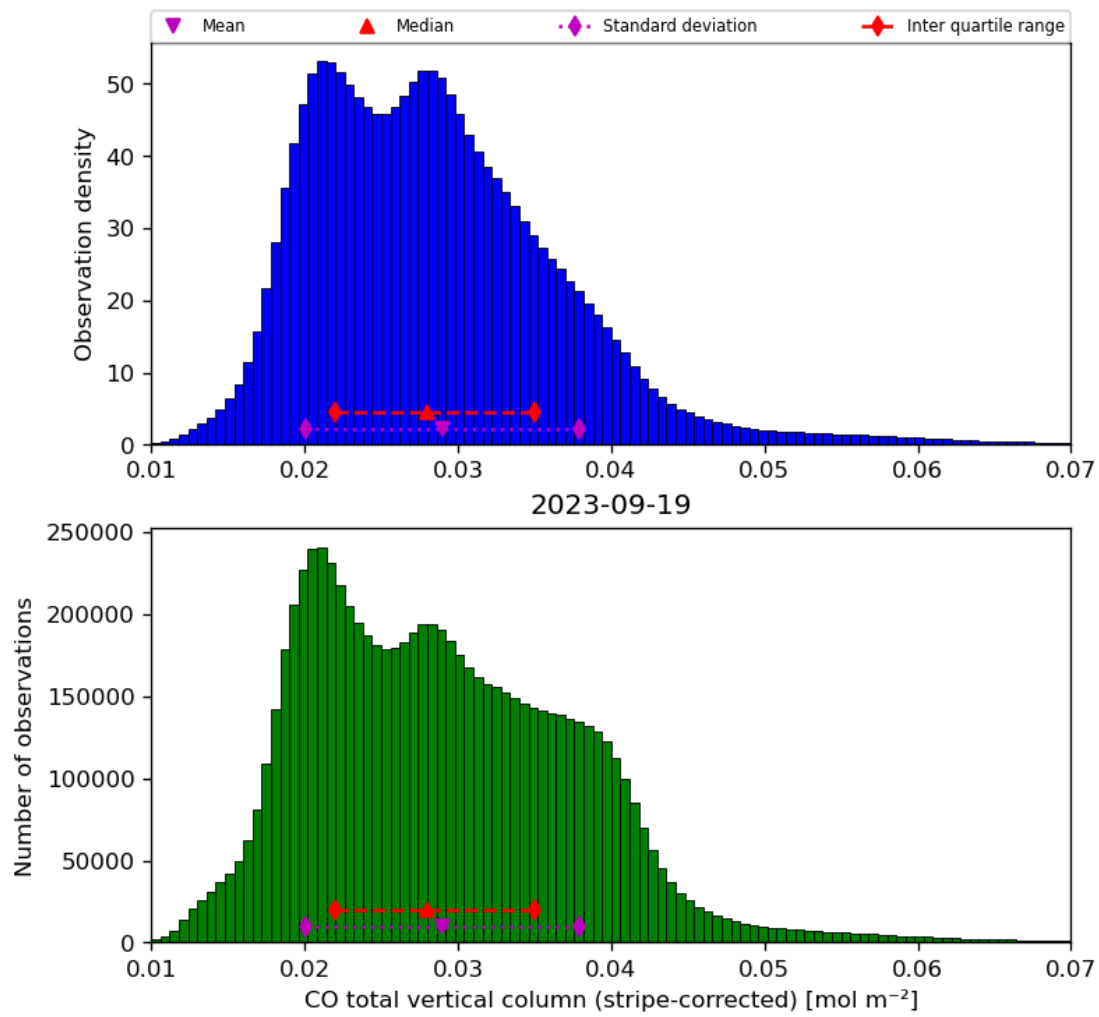
Figure 19: Histogram of “CO total vertical column (stripe-corrected)” for 2023-09-18 to 2023-09-20
