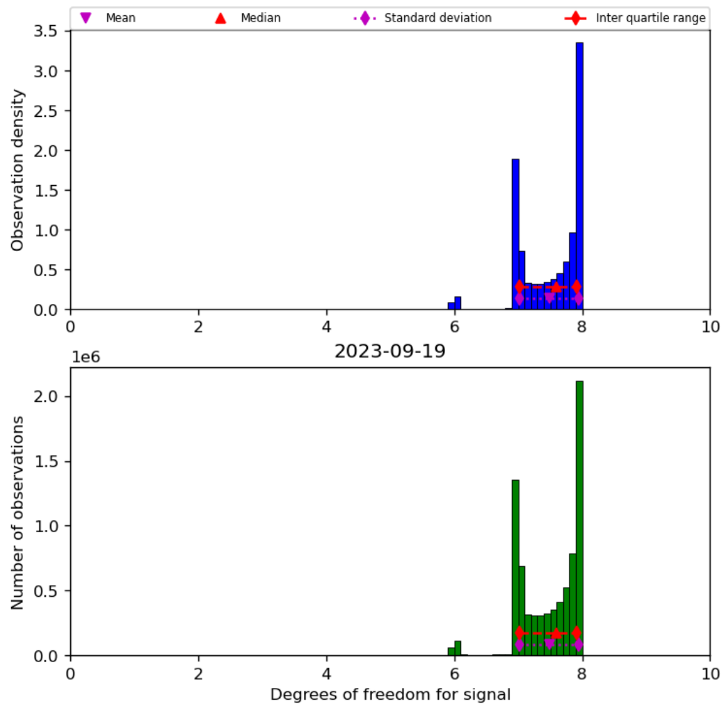
Figure 23: Histogram of “Degrees of freedom for signal” for 2023-09-18 to 2023-09-20
