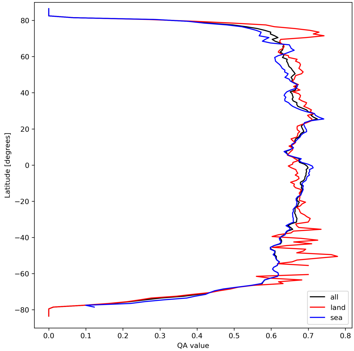
Figure 9: Zonal average of “QA value” for 2023-09-18 to 2023-09-20.
