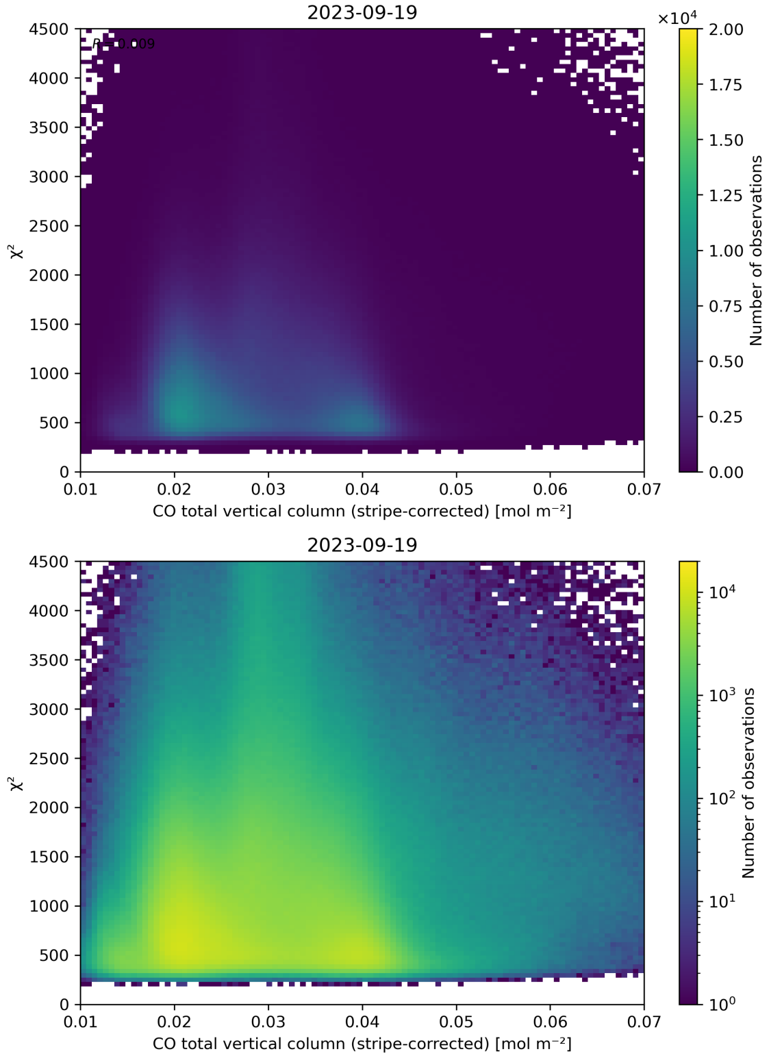
Figure 37: Scatter density plot of “CO total vertical column (stripe-corrected)” against “ \chi^2 ” for 2023-09-18 to 2023-09-20.
