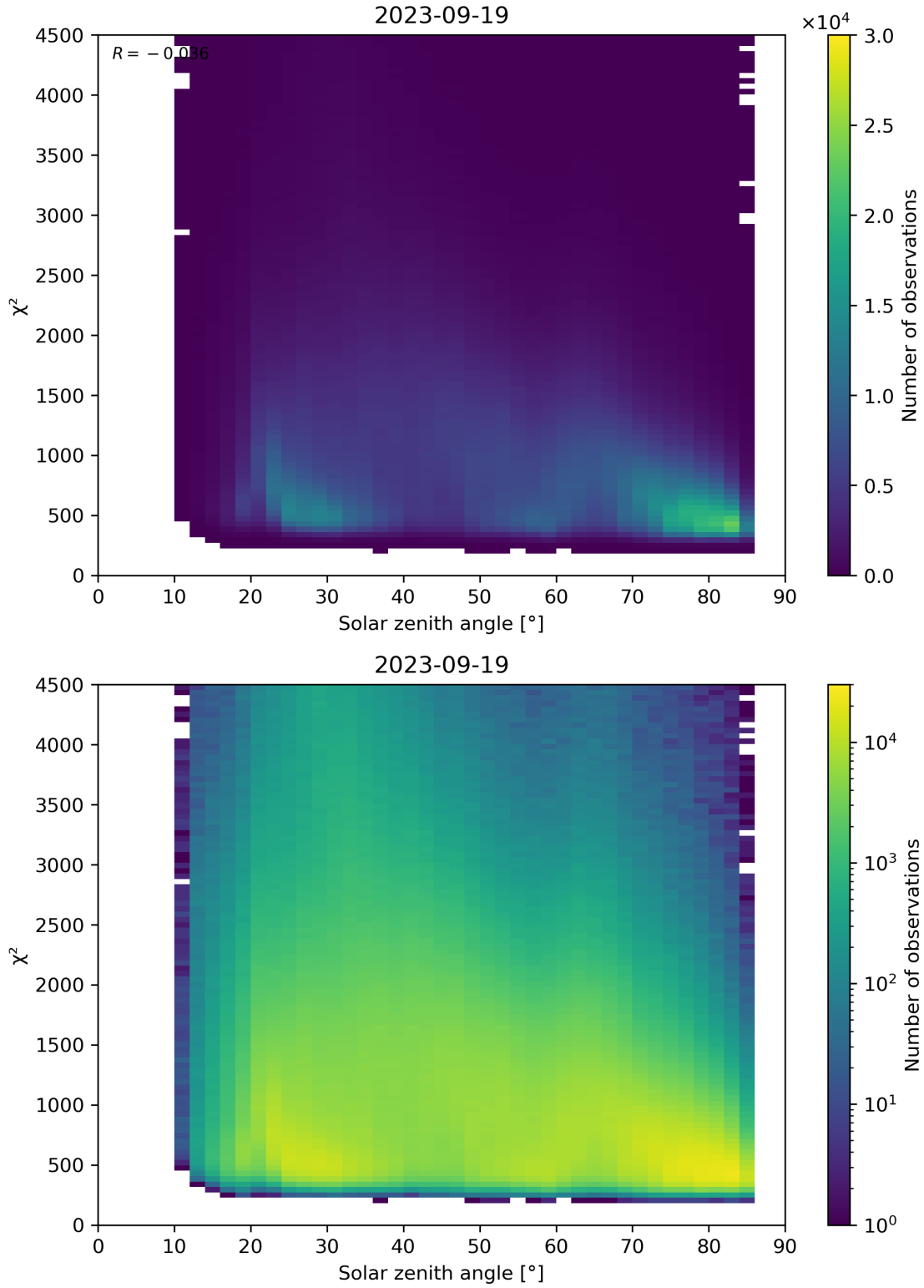
Figure 64: Scatter density plot of “Solar zenith angle” against “ \chi^2 ” for 2023-09-18 to 2023-09-20.
