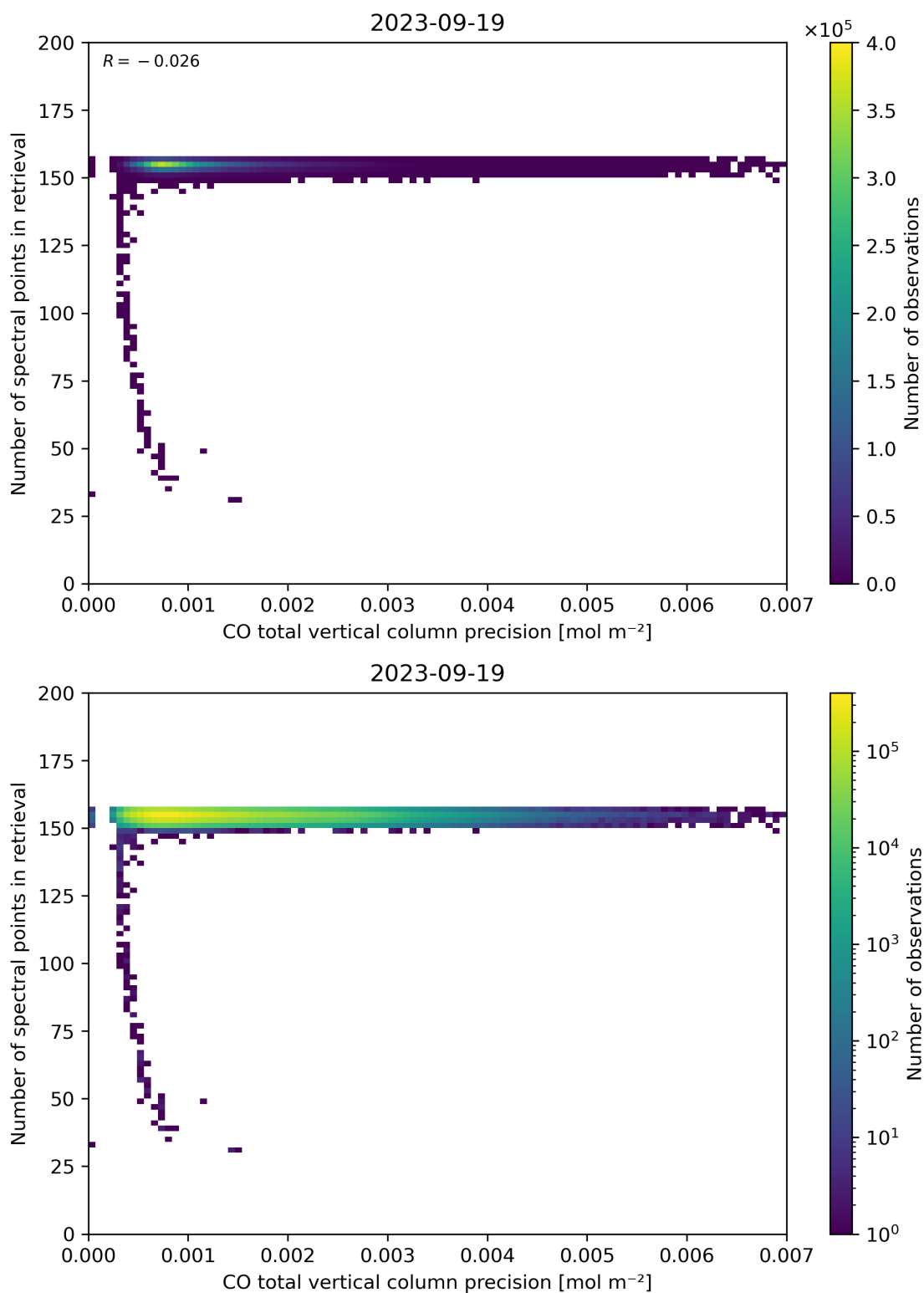
Figure 47: Scatter density plot of “CO total vertical column precision” against “Number of spectral points in retrieval” for 2023-09-18 to 2023-09-20.
