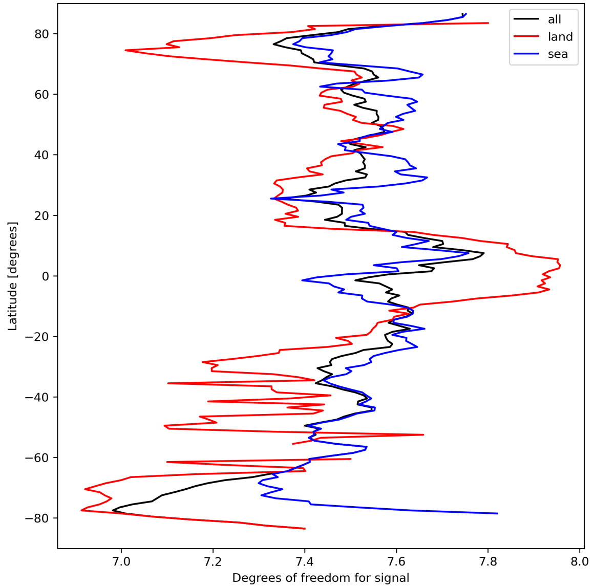
Figure 15: Zonal average of “Degrees of freedom for signal” for 2023-09-18 to 2023-09-20.
