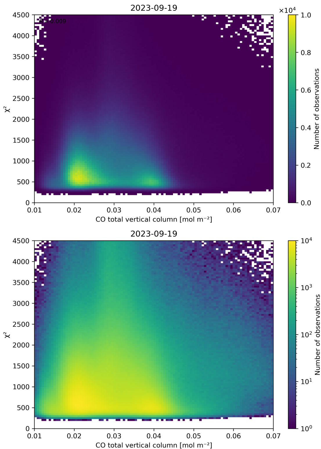
Figure 35: Scatter density plot of “CO total vertical column” against “ \chi^2 ” for 2023-09-18 to 2023-09-20.
