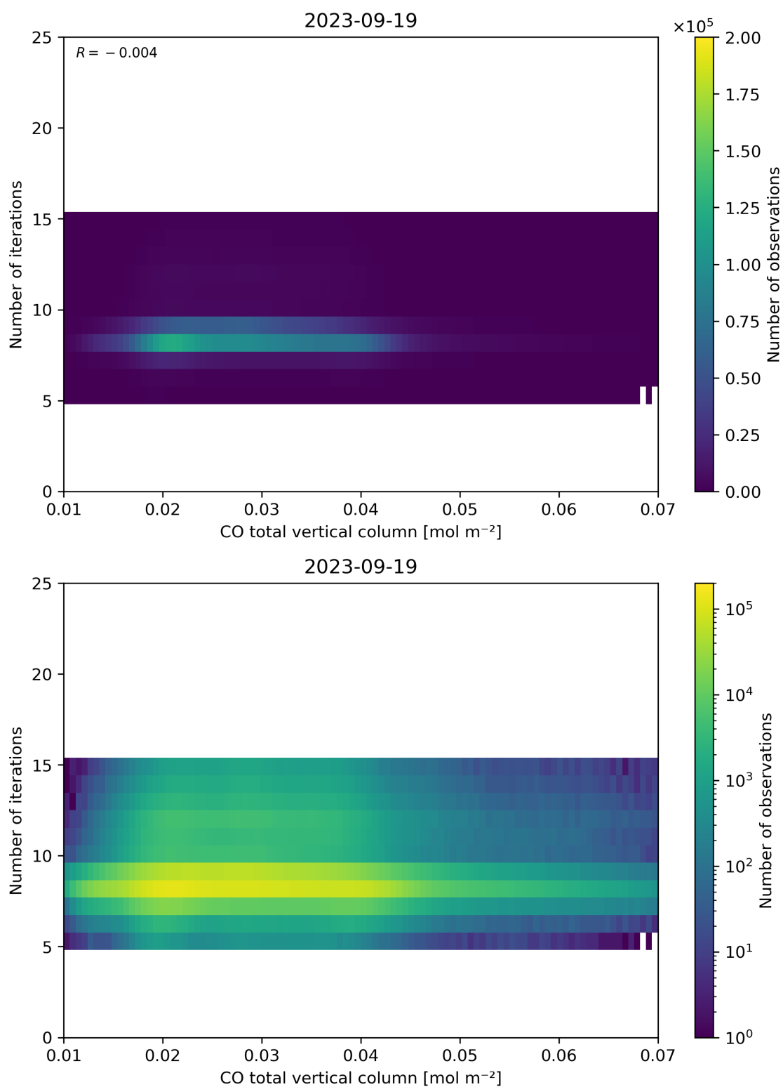
Figure 42: Scatter density plot of “CO total vertical column” against “Number of iterations” for 2023-09-18 to 2023-09-20.
