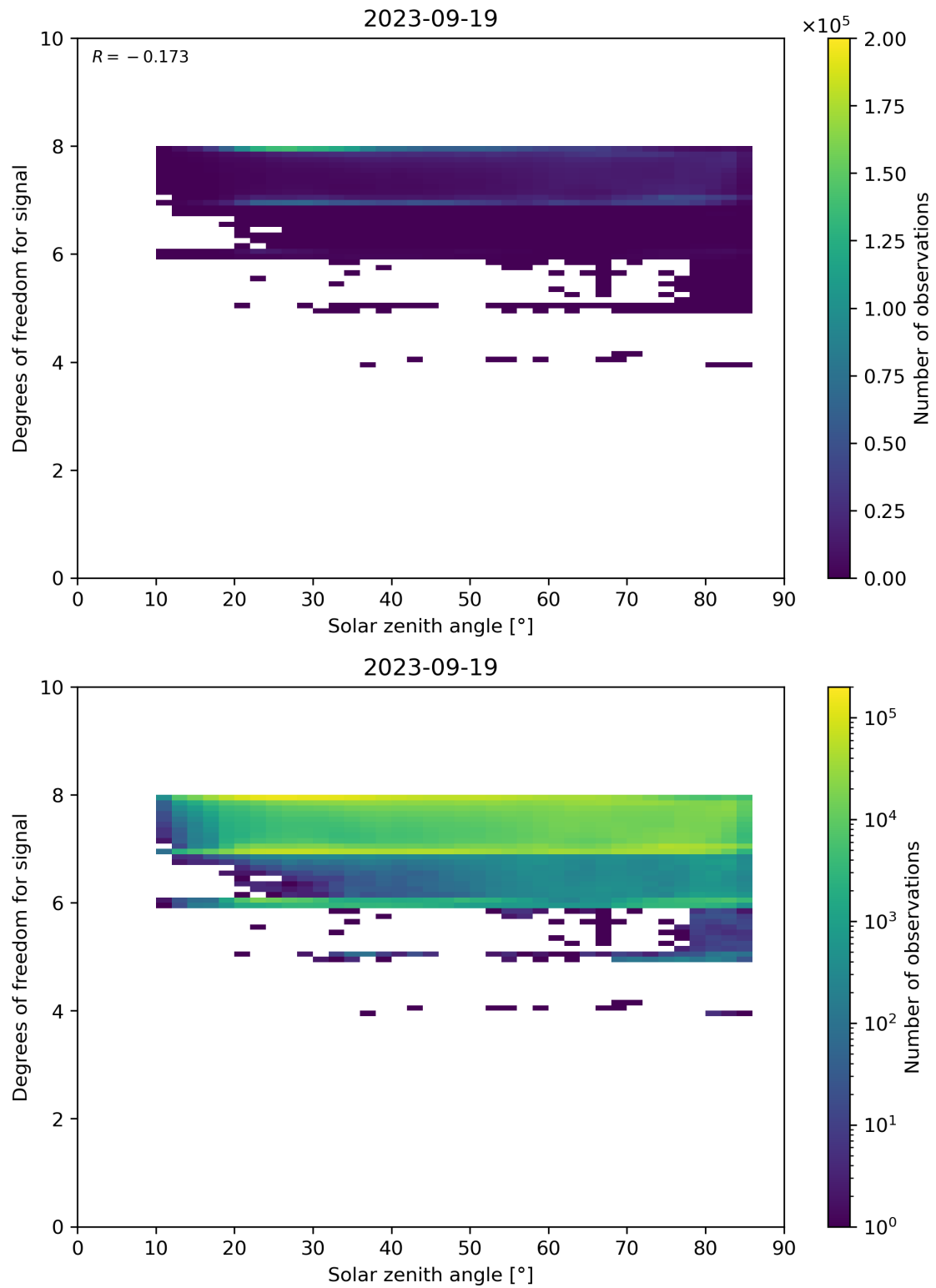
Figure 65: Scatter density plot of “Solar zenith angle” against “Degrees of freedom for signal” for 2023-09-18 to 2023-09-20.
