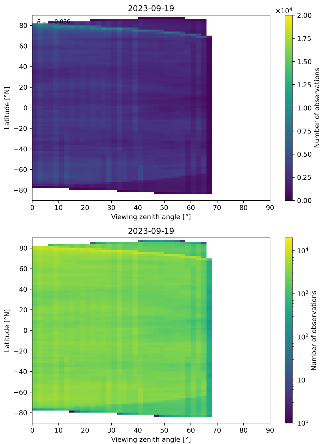
Figure 74: Scatter density plot of “Viewing zenith angle” against “Latitude” for 2023-09-18 to 2023-09-20.
