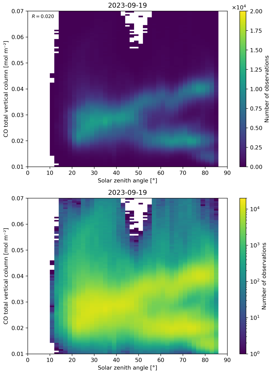
Figure 61: Scatter density plot of “Solar zenith angle” against “CO total vertical column” for 2023-09-18 to 2023-09-20.
