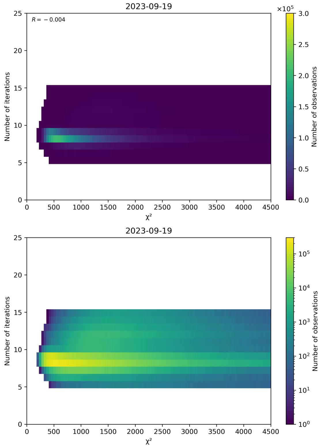
Figure 49: Scatter density plot of “ \chi^2 ” against “Number of iterations” for 2023-09-18 to 2023-09-20.
