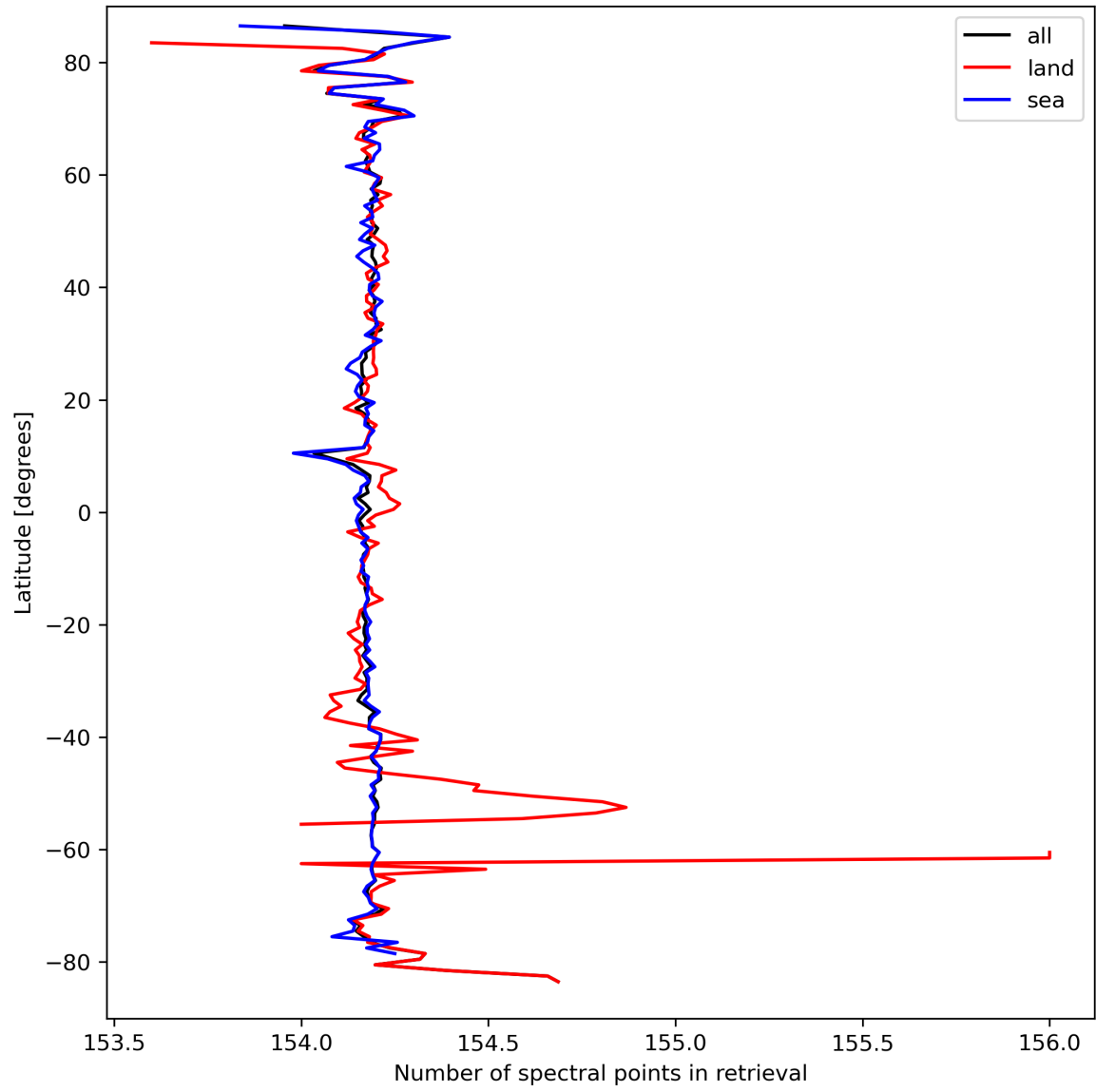
Figure 13: Zonal average of “Number of spectral points in retrieval” for 2023-09-18 to 2023-09-20.
