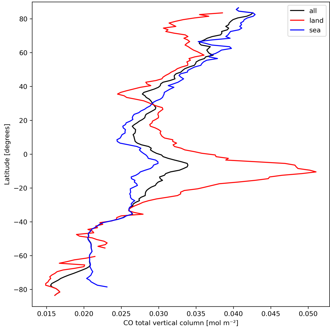
Figure 10: Zonal average of “CO total vertical column” for 2023-09-18 to 2023-09-20.
