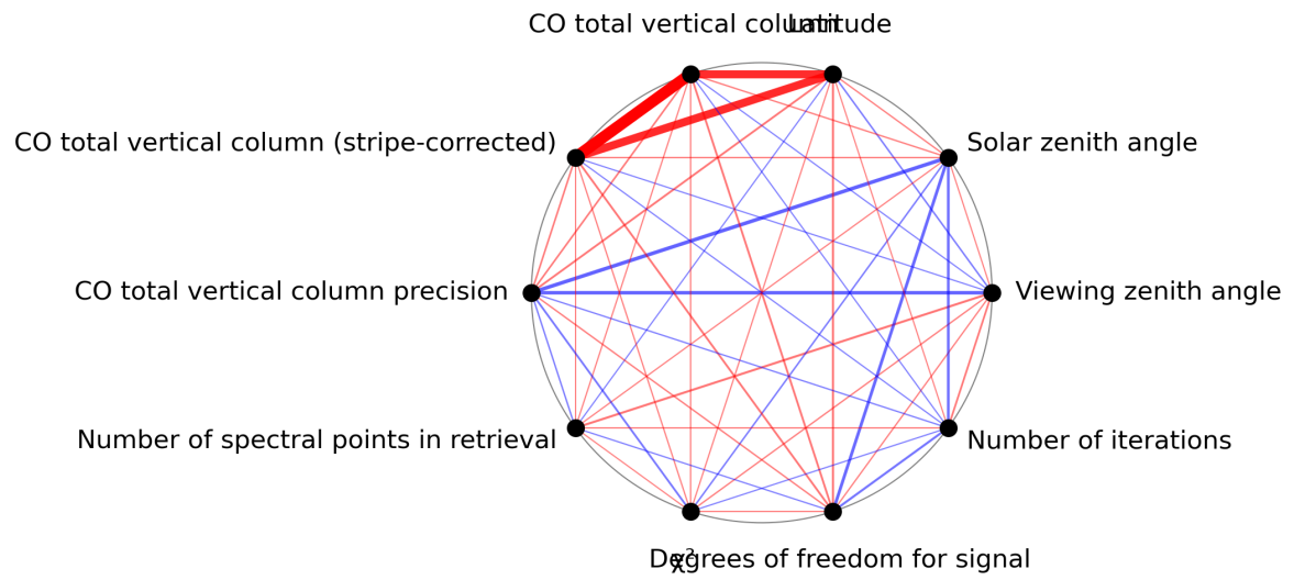
Figure 1: Map of correlation graph for 2023-09-18 to 2023-09-20.
