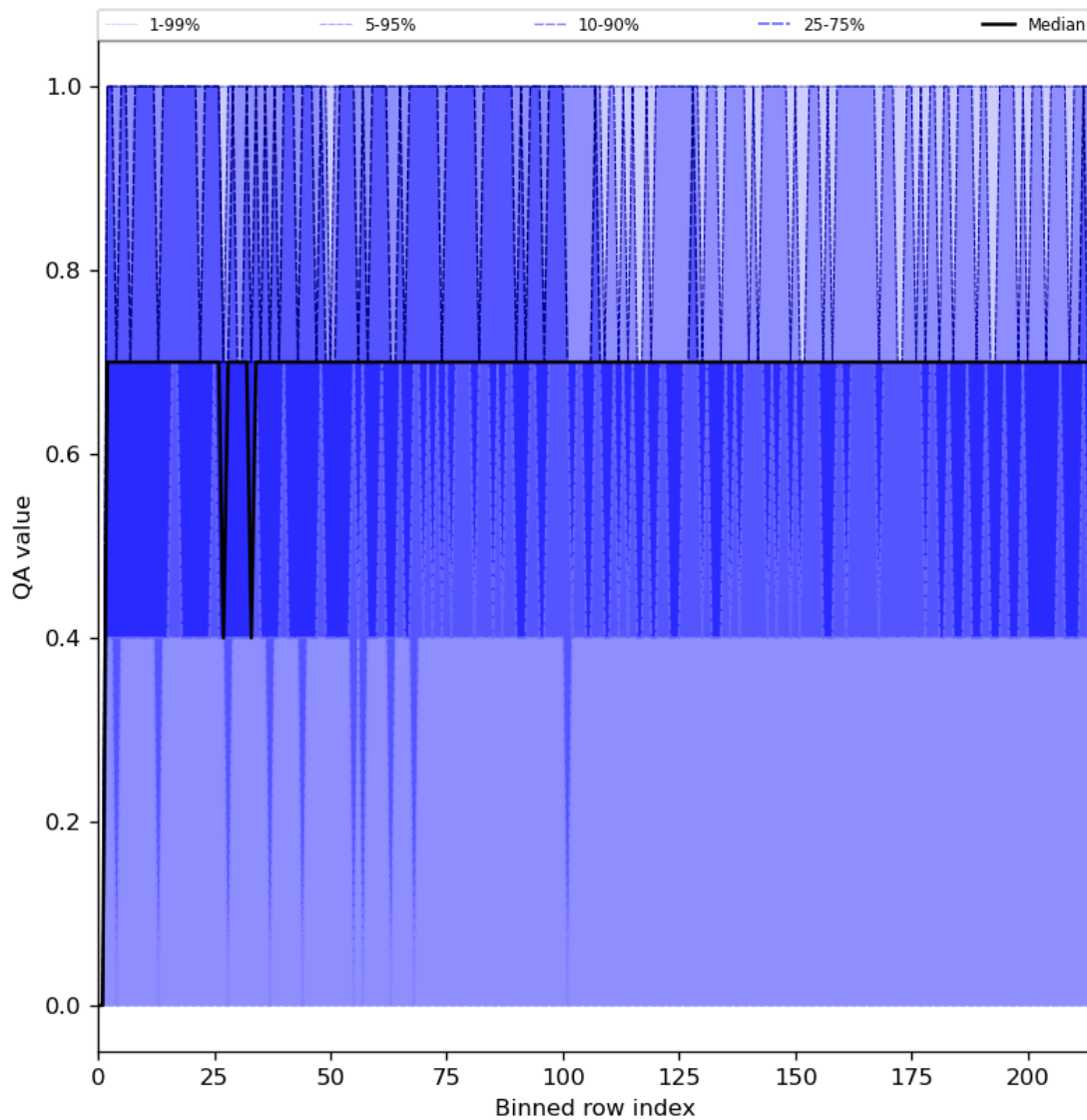
Figure 25: Along track statistics of “QA value” for 2023-09-18 to 2023-09-20
