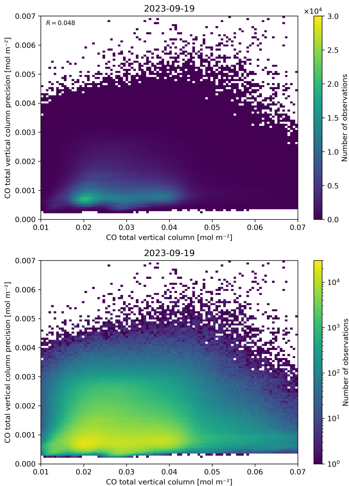
Figure 34: Scatter density plot of “CO total vertical column” against “CO total vertical column precision” for 2023-09-18 to 2023-09-20.
