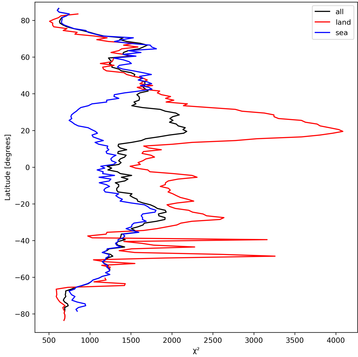
Figure 14: Zonal average of “ \chi^2 ” for 2023-09-18 to 2023-09-20.
