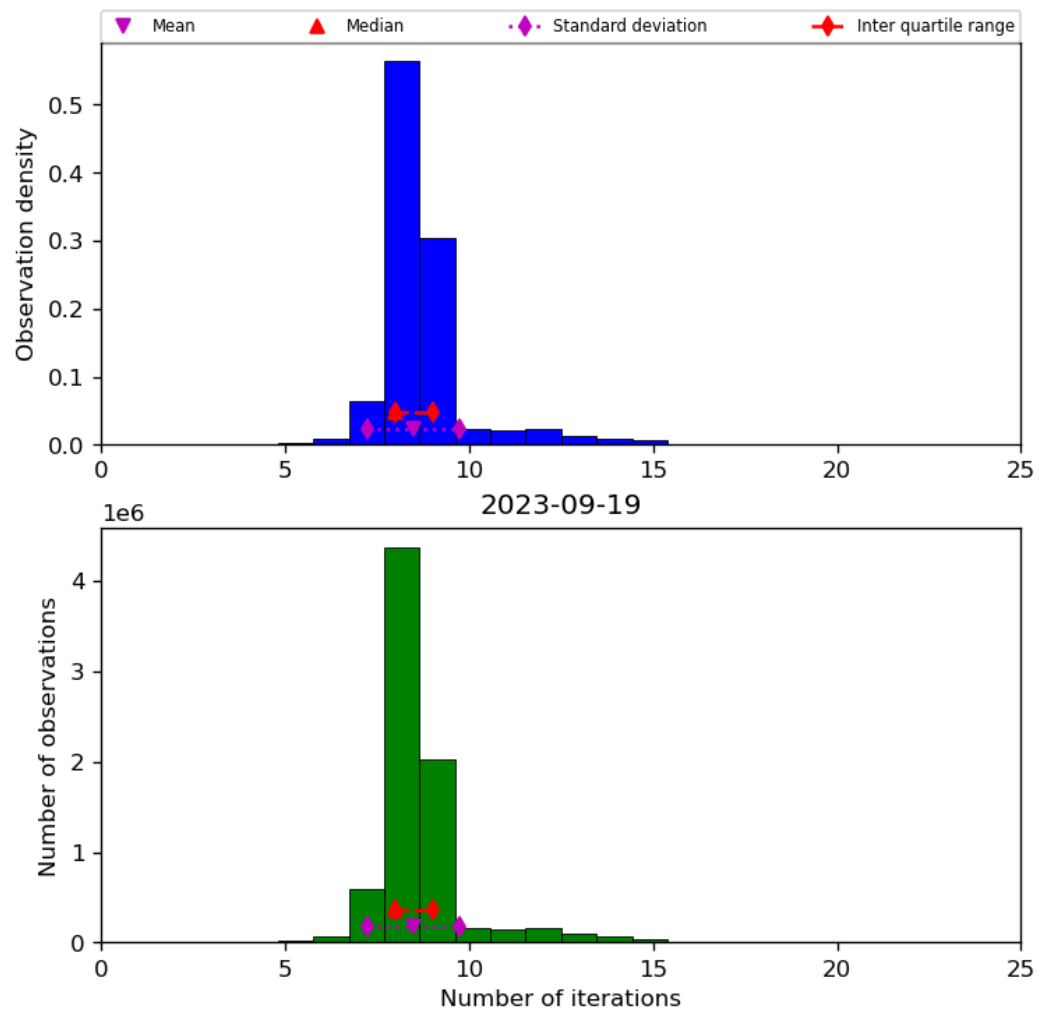
Figure 24: Histogram of “Number of iterations” for 2023-09-18 to 2023-09-20
