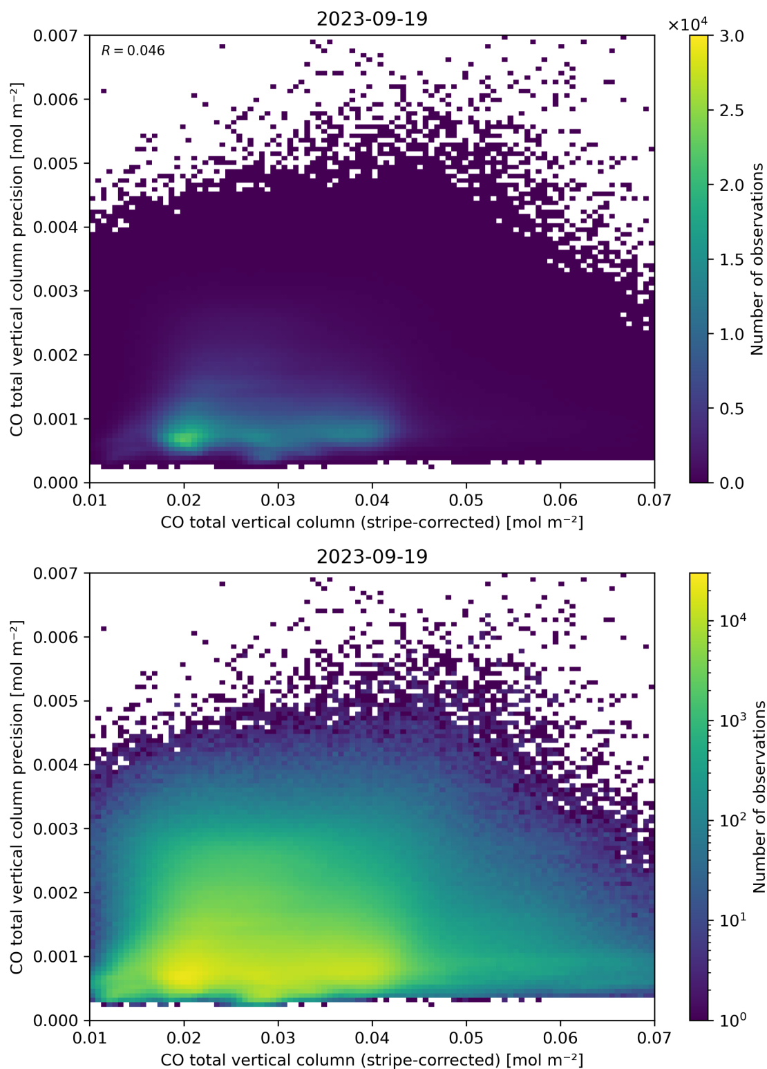
Figure 36: Scatter density plot of “CO total vertical column (stripe-corrected)” against “CO total vertical column precision” for 2023-09-18 to 2023-09-20.
