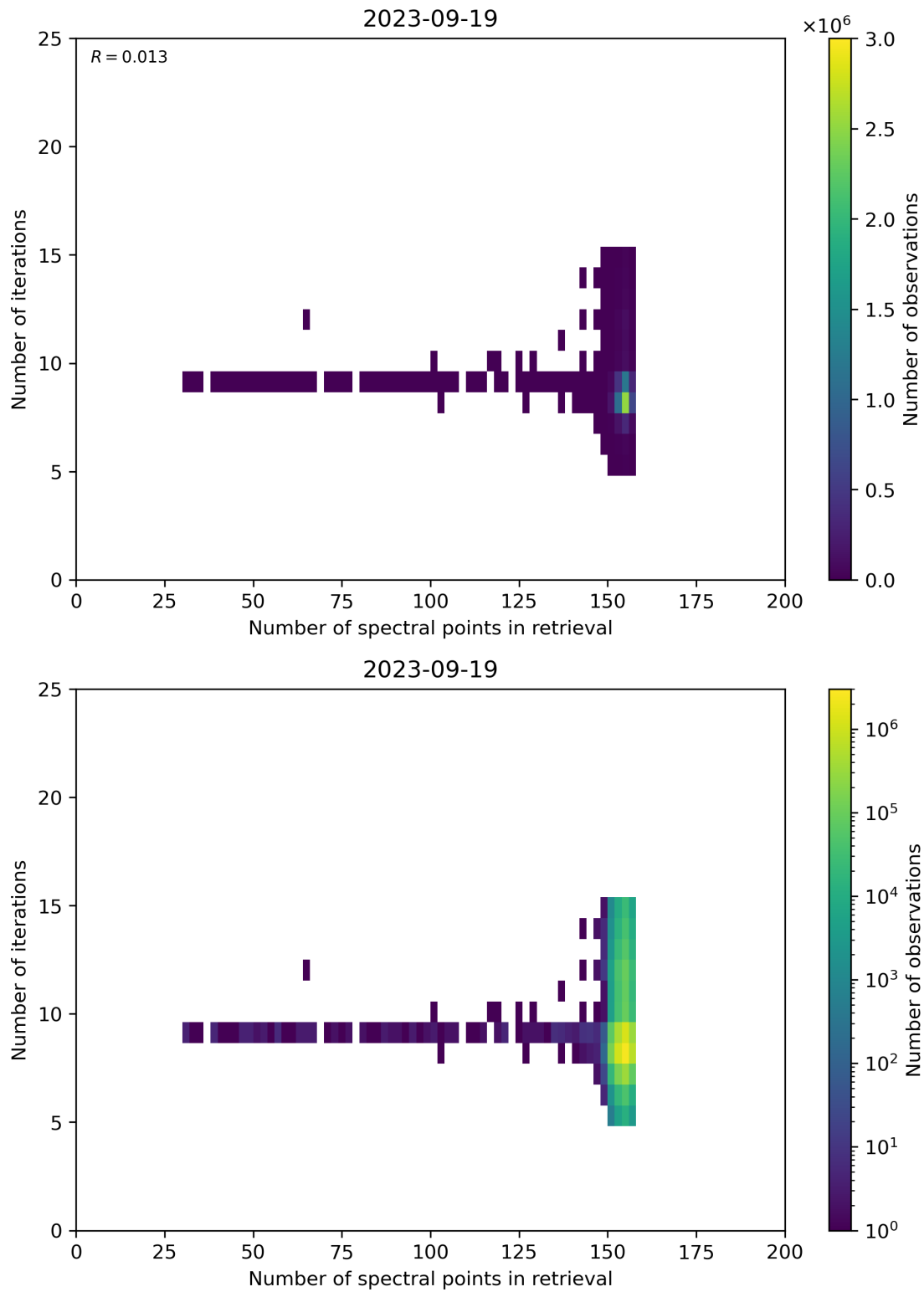
Figure 60: Scatter density plot of “Number of spectral points in retrieval” against “Number of iterations” for 2023-09-18 to 2023-09-20.
