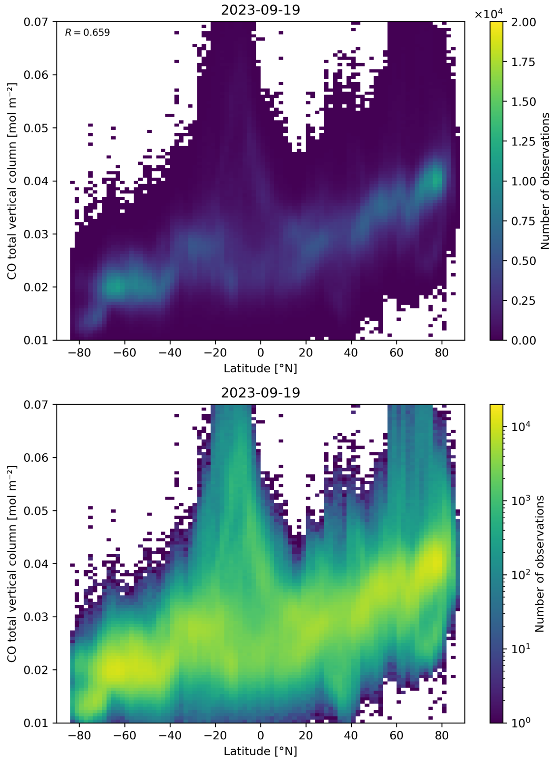
Figure 51: Scatter density plot of “Latitude” against “CO total vertical column” for 2023-09-18 to 2023-09-20.
