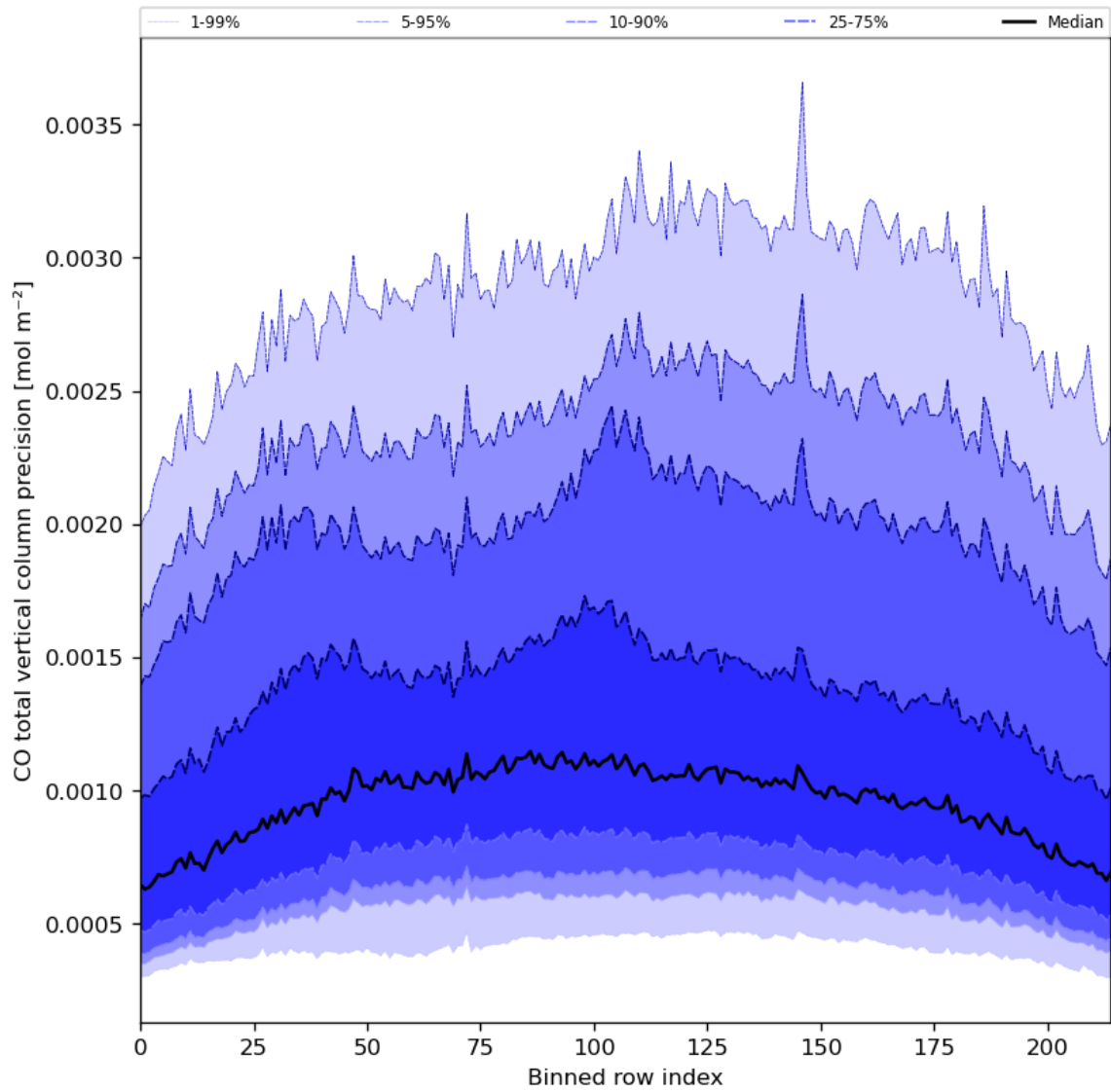
Figure 28: Along track statistics of “CO total vertical column precision” for 2023-09-18 to 2023-09-20
