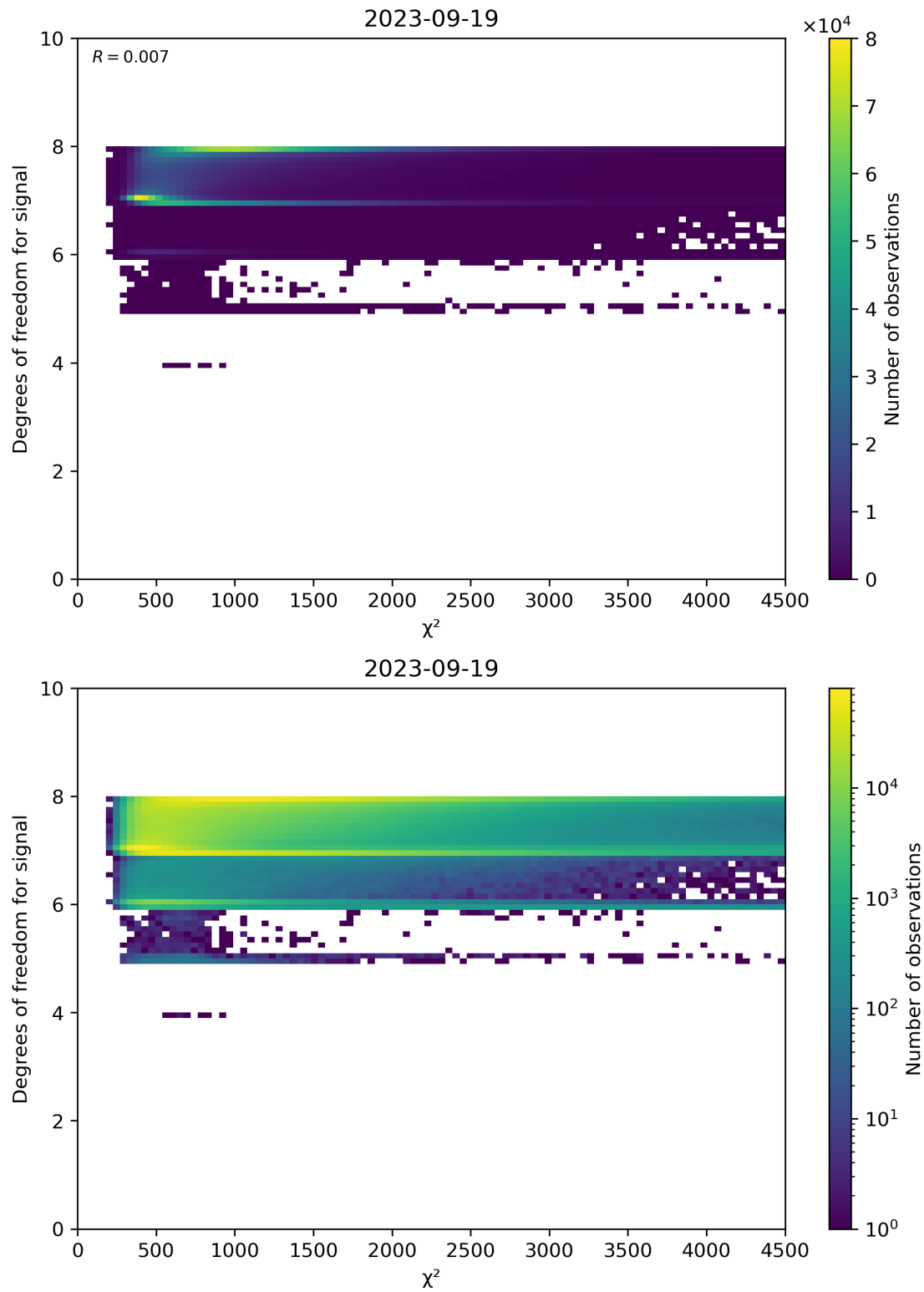
Figure 48: Scatter density plot of “ \chi^2 ” against “Degrees of freedom for signal” for 2023-09-18 to 2023-09-20.
