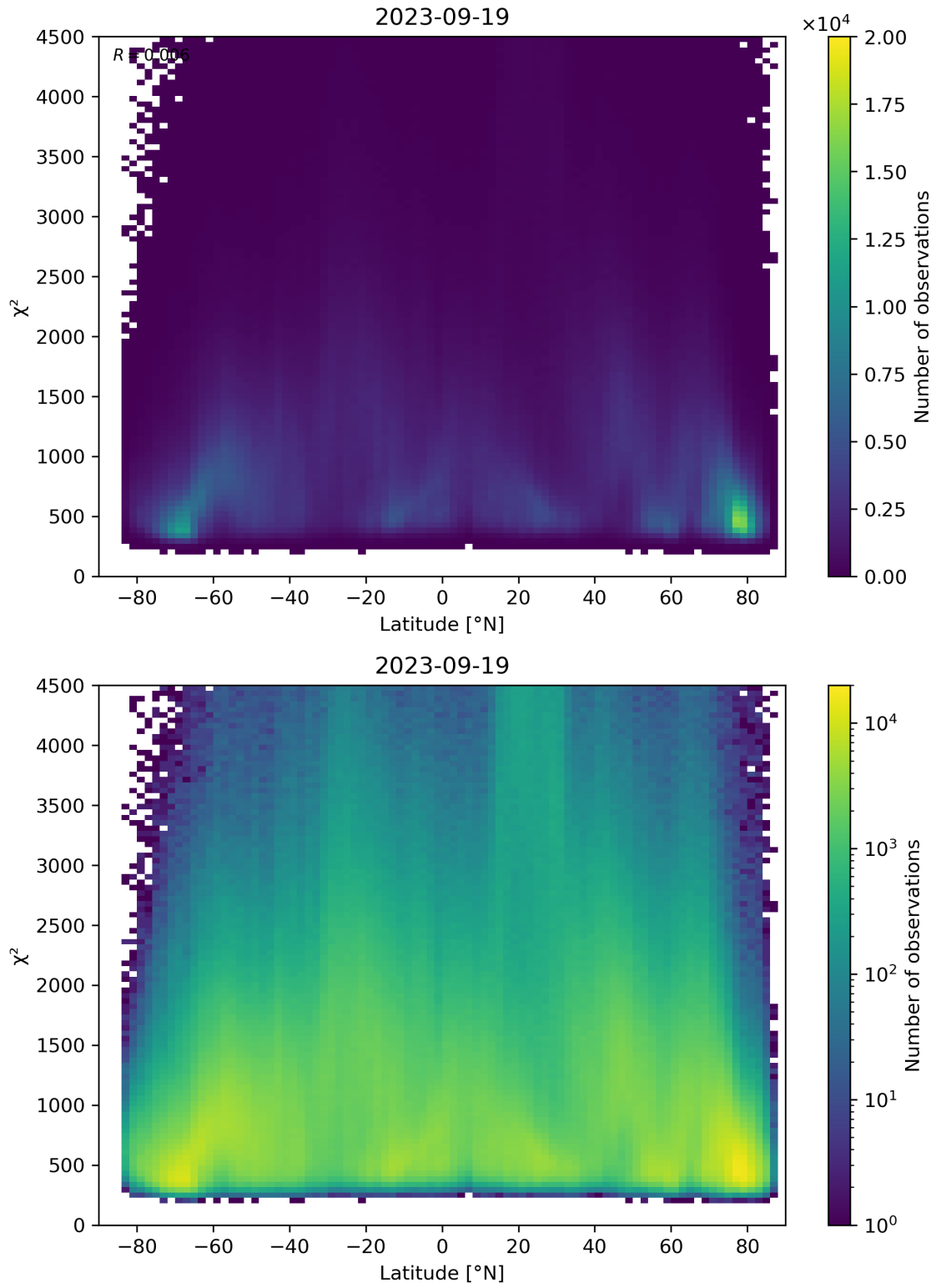
Figure 54: Scatter density plot of “Latitude” against “ \chi^2 ” for 2023-09-18 to 2023-09-20.
