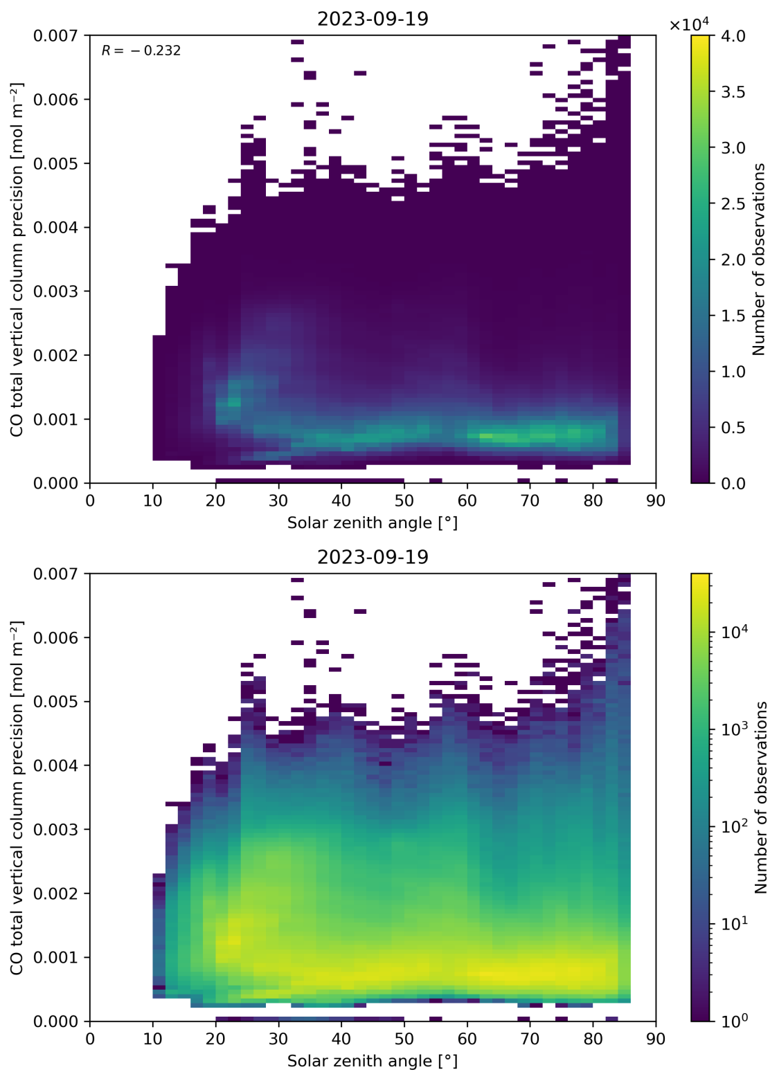
Figure 63: Scatter density plot of “Solar zenith angle” against “CO total vertical column precision” for 2023-09-18 to 2023-09-20.
