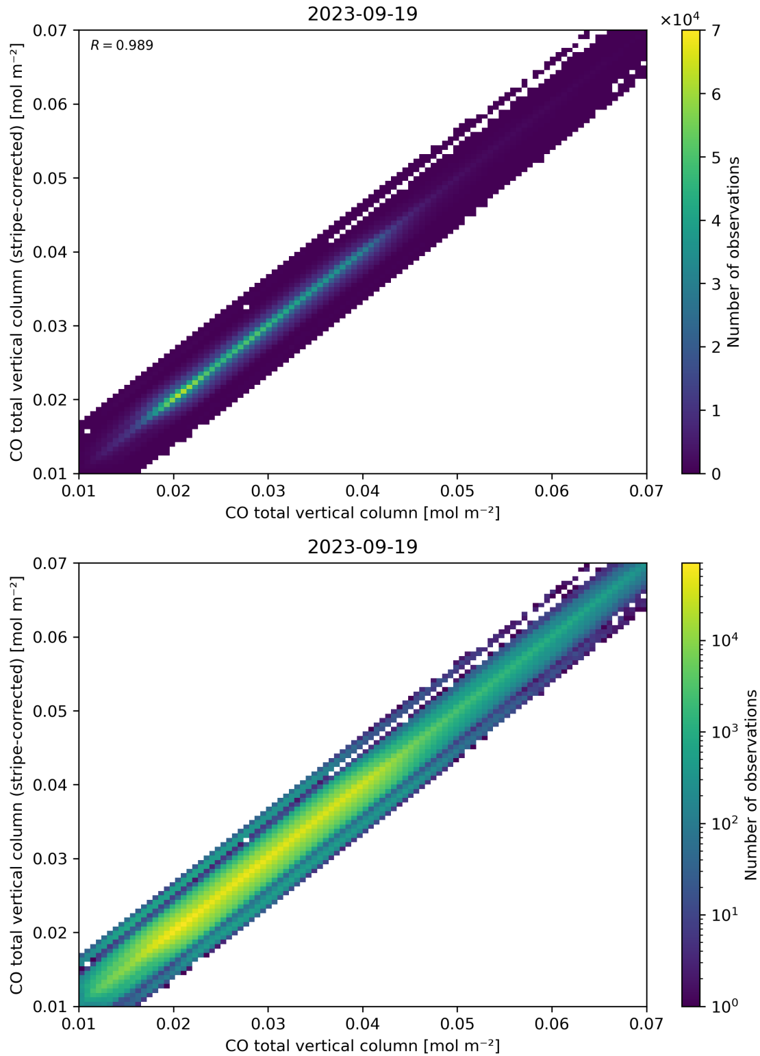
Figure 33: Scatter density plot of “CO total vertical column” against “CO total vertical column (stripe-corrected)” for 2023-09-18 to 2023-09-20.
