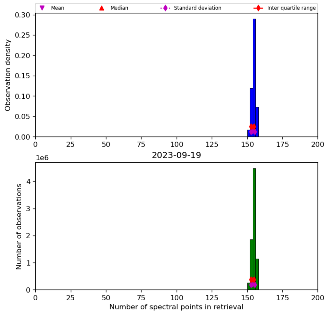
Figure 21: Histogram of “Number of spectral points in retrieval” for 2023-09-18 to 2023-09-20
