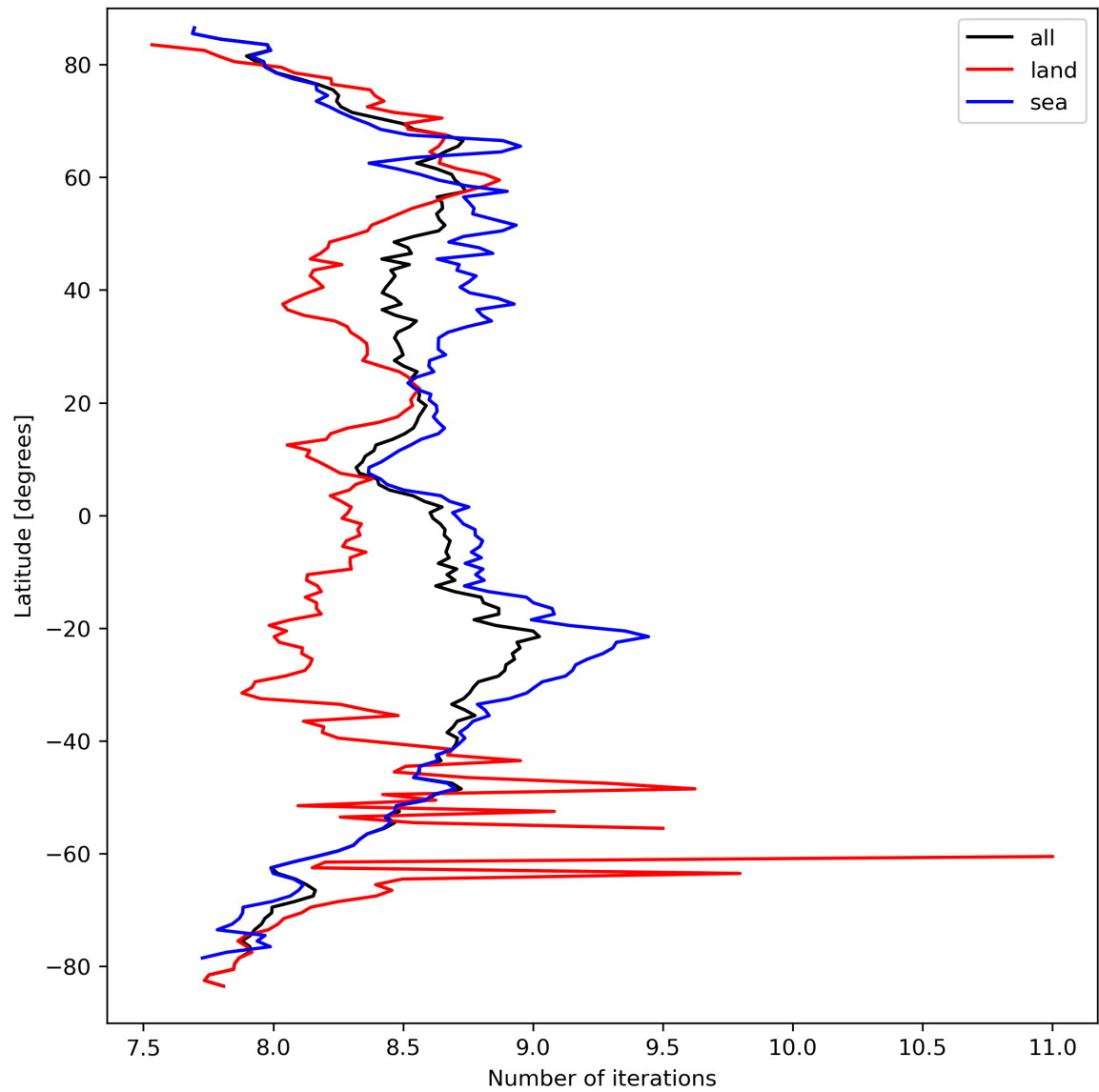
Figure 16: Zonal average of “Number of iterations” for 2023-09-18 to 2023-09-20.
