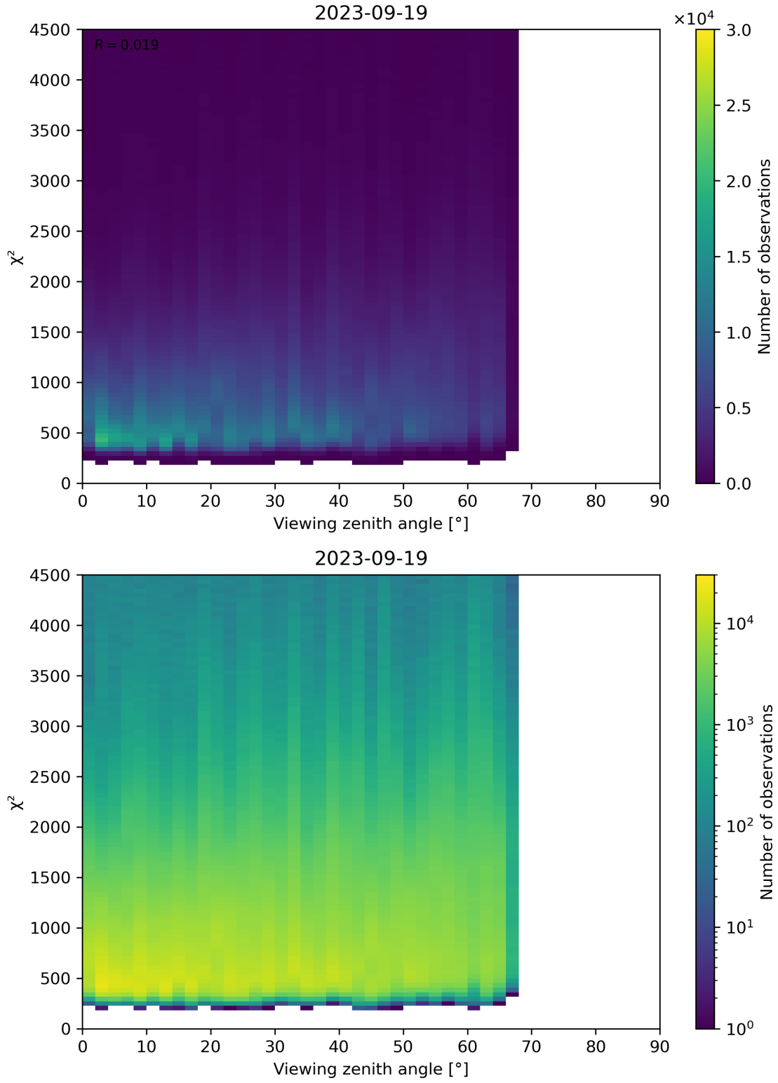
Figure 72: Scatter density plot of “Viewing zenith angle” against “ \chi^2 ” for 2023-09-18 to 2023-09-20.
