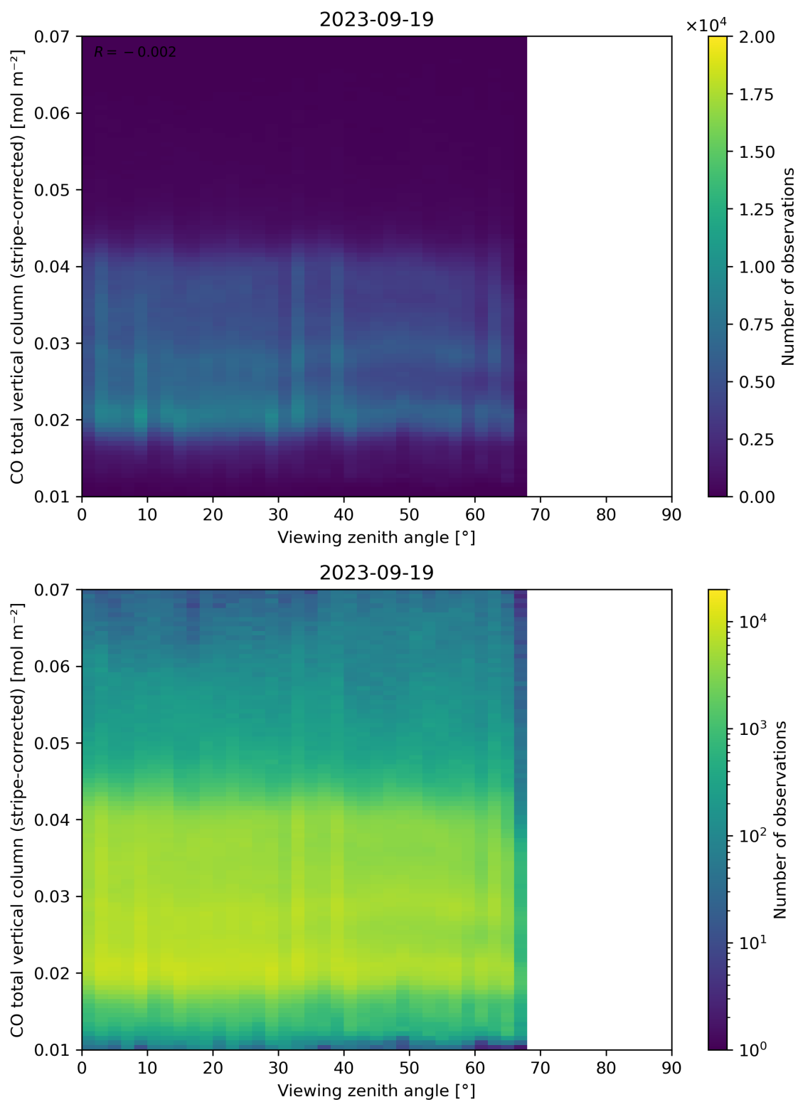
Figure 70: Scatter density plot of “Viewing zenith angle” against “CO total vertical column (stripe-corrected)” for 2023-09-18 to 2023-09-20.
