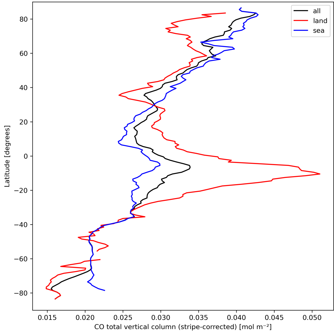
Figure 11: Zonal average of “CO total vertical column (stripe-corrected)” for 2023-09-18 to 2023-09-20.
