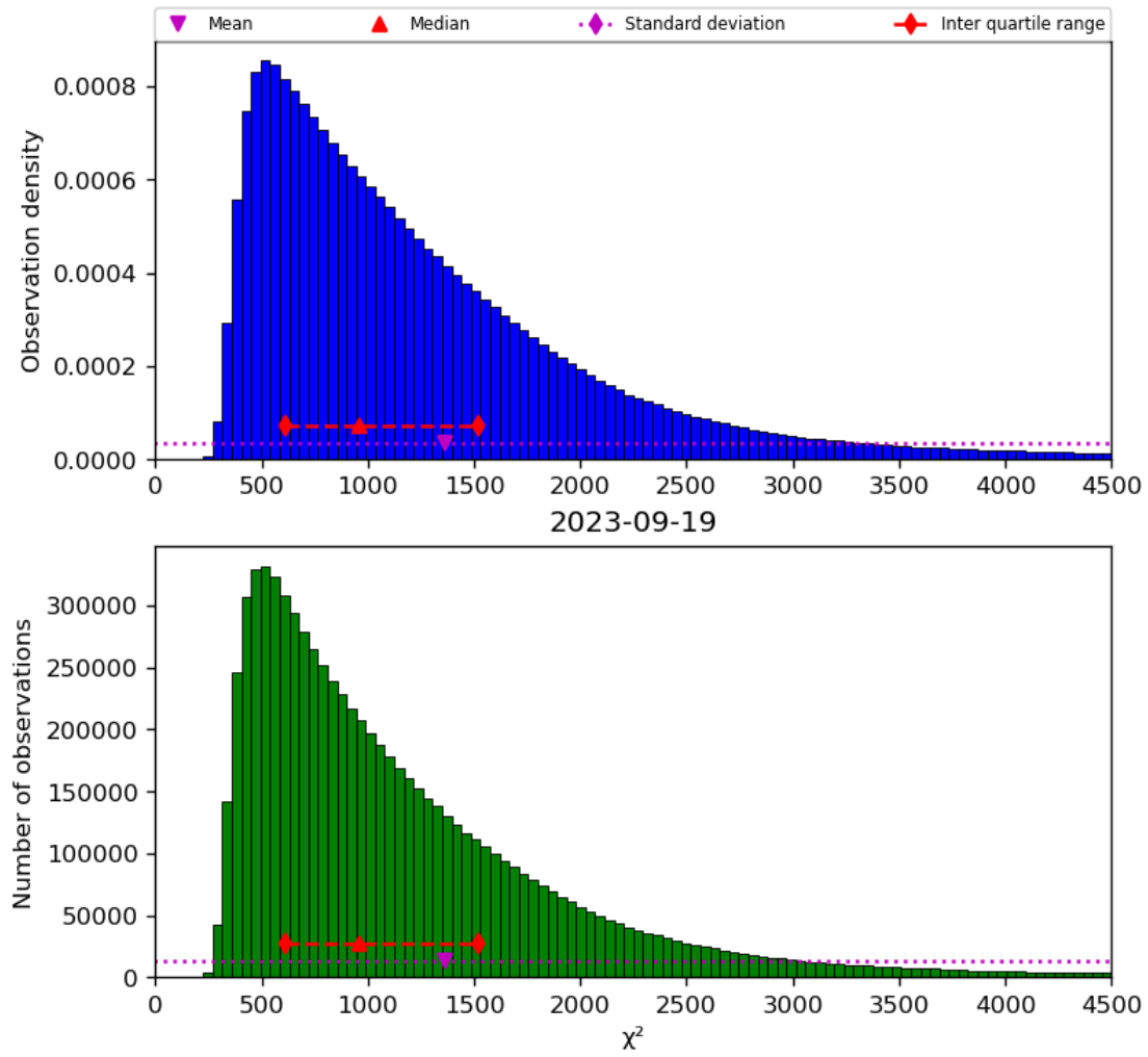
Figure 22: Histogram of “ \chi^2 ” for 2023-09-18 to 2023-09-20
