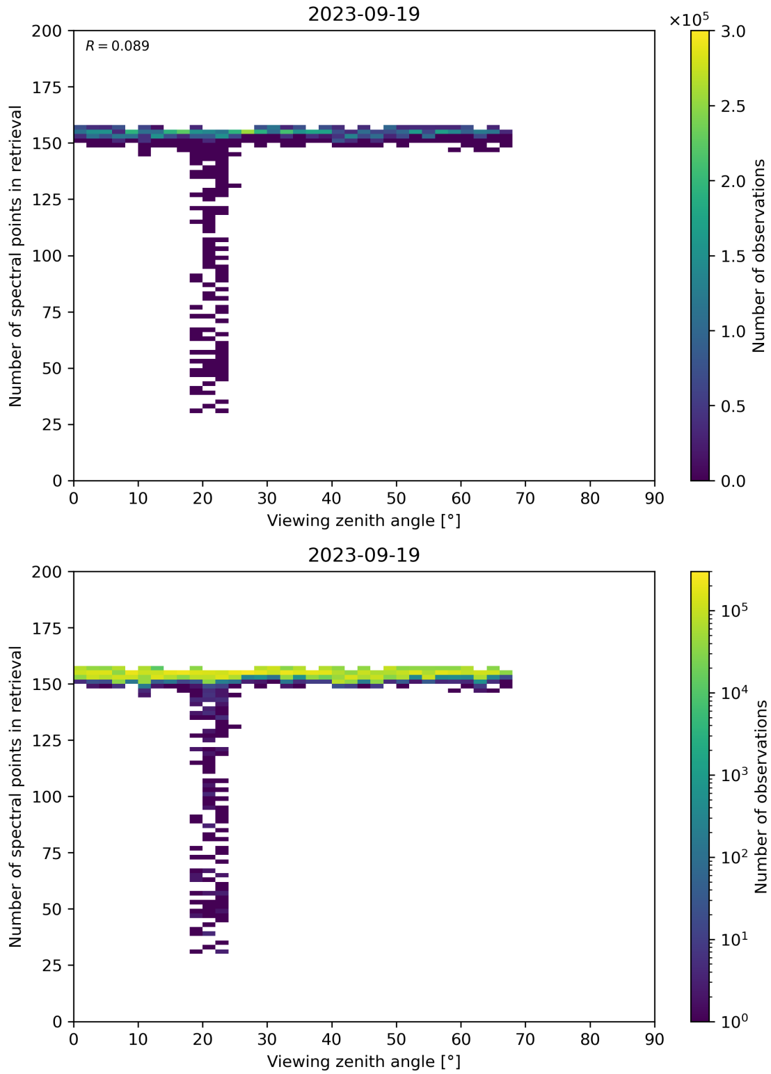
Figure 76: Scatter density plot of “Viewing zenith angle” against “Number of spectral points in retrieval” for 2023-09-18 to 2023-09-20.
