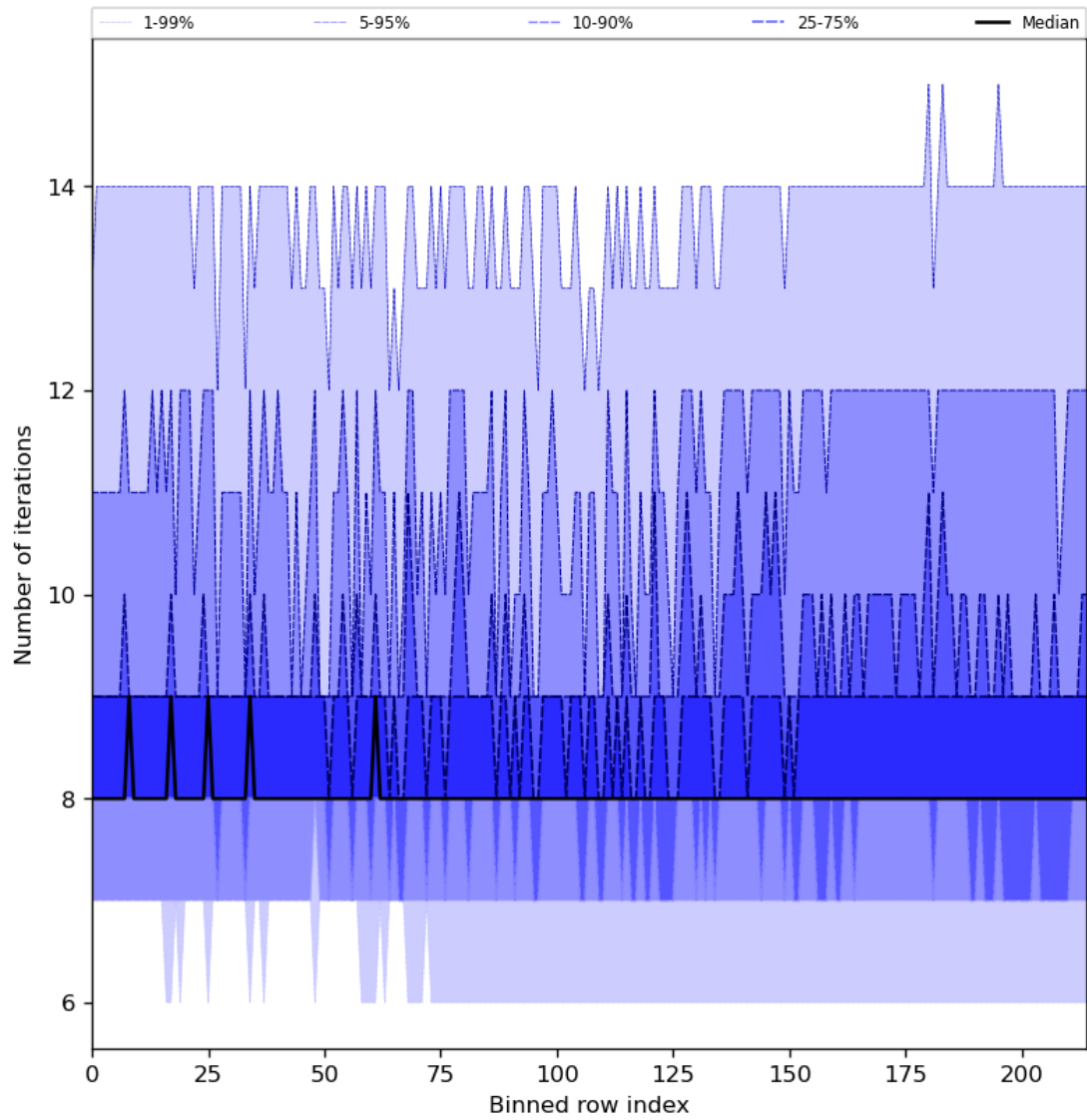
Figure 32: Along track statistics of “Number of iterations” for 2023-09-18 to 2023-09-20
