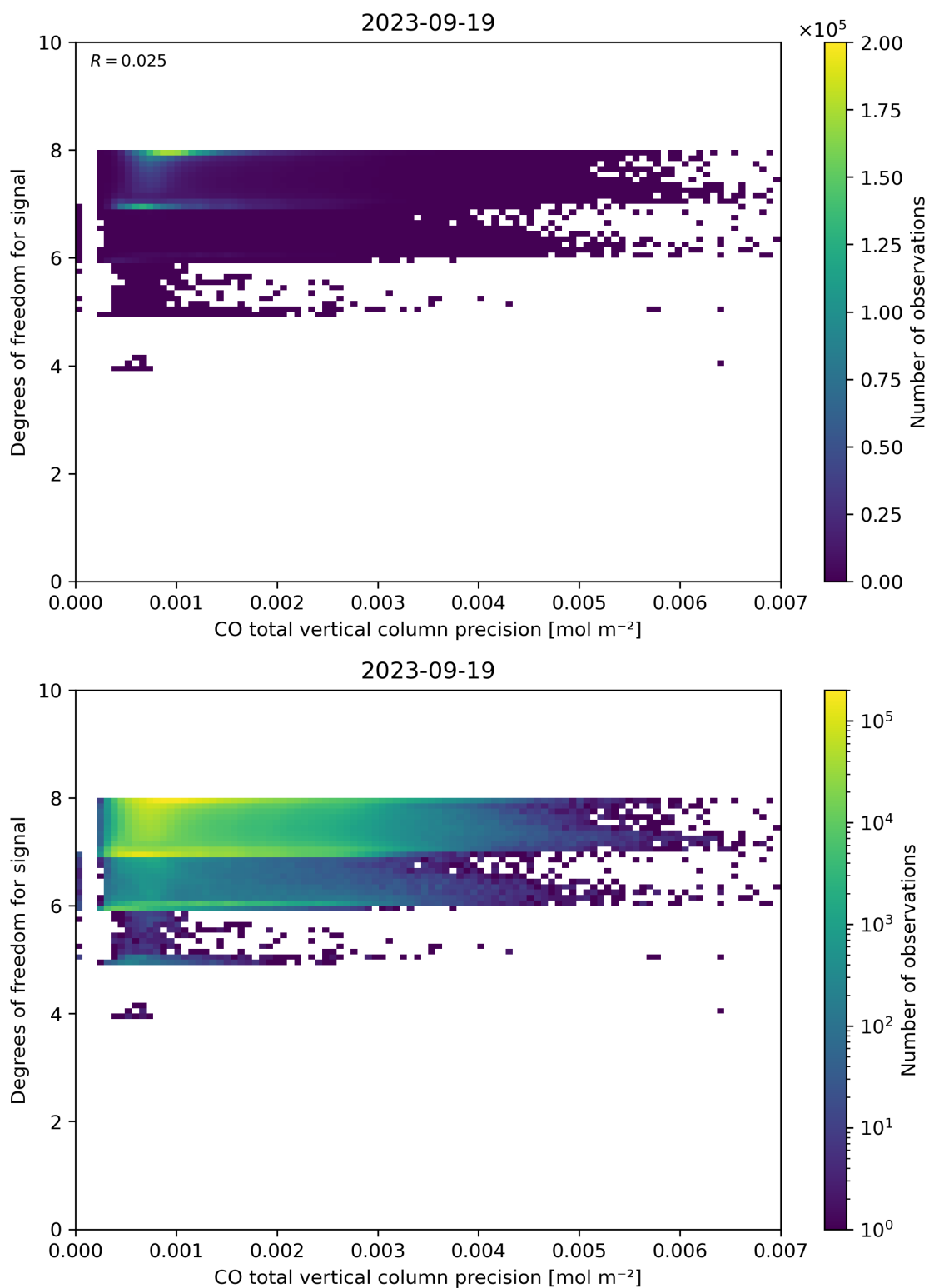
Figure 45: Scatter density plot of “CO total vertical column precision” against “Degrees of freedom for signal” for 2023-09-18 to 2023-09-20.
