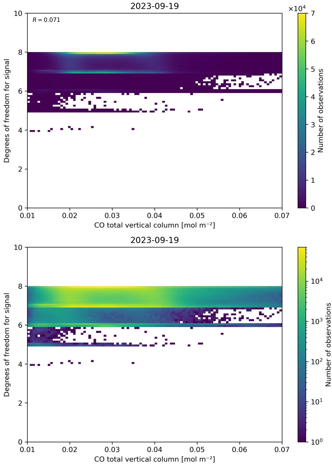
Figure 41: Scatter density plot of “CO total vertical column” against “Degrees of freedom for signal” for 2023-09-18 to 2023-09-20.
