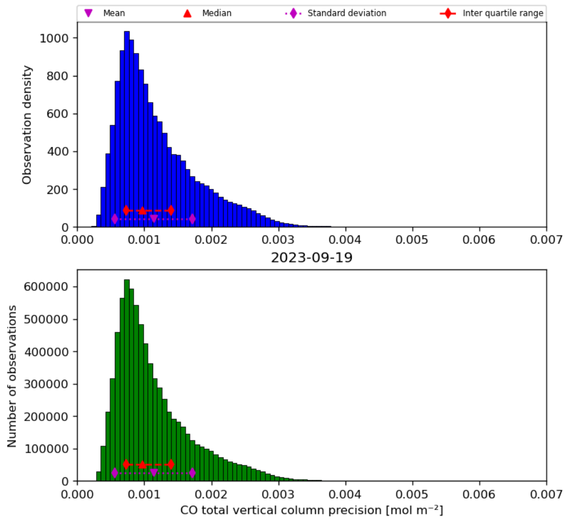
Figure 20: Histogram of “CO total vertical column precision” for 2023-09-18 to 2023-09-20
