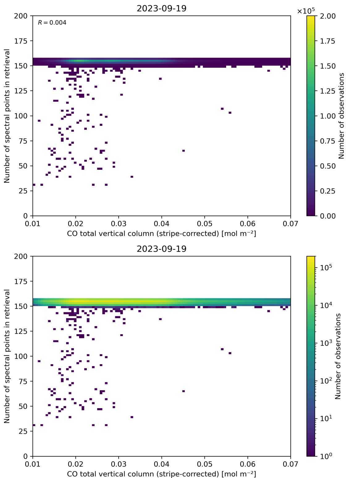
Figure 40: Scatter density plot of “CO total vertical column (stripe-corrected)” against “Number of spectral points in retrieval” for 2023-09-18 to 2023-09-20.
