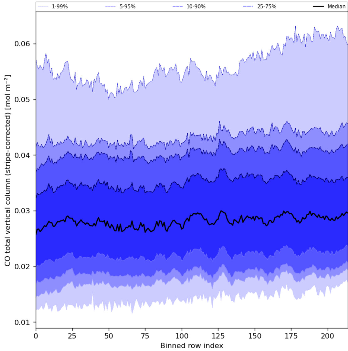
Figure 27: Along track statistics of “CO total vertical column (stripe-corrected)” for 2023-09-18 to 2023-09-20
