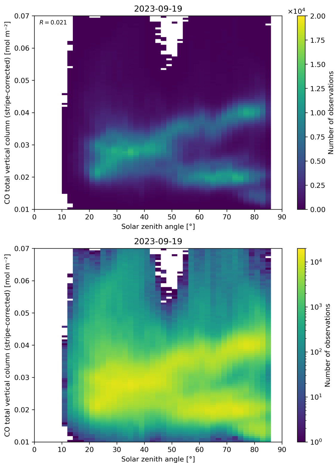
Figure 62: Scatter density plot of “Solar zenith angle” against “CO total vertical column (stripe-corrected)” for 2023-09-18 to 2023-09-20.
