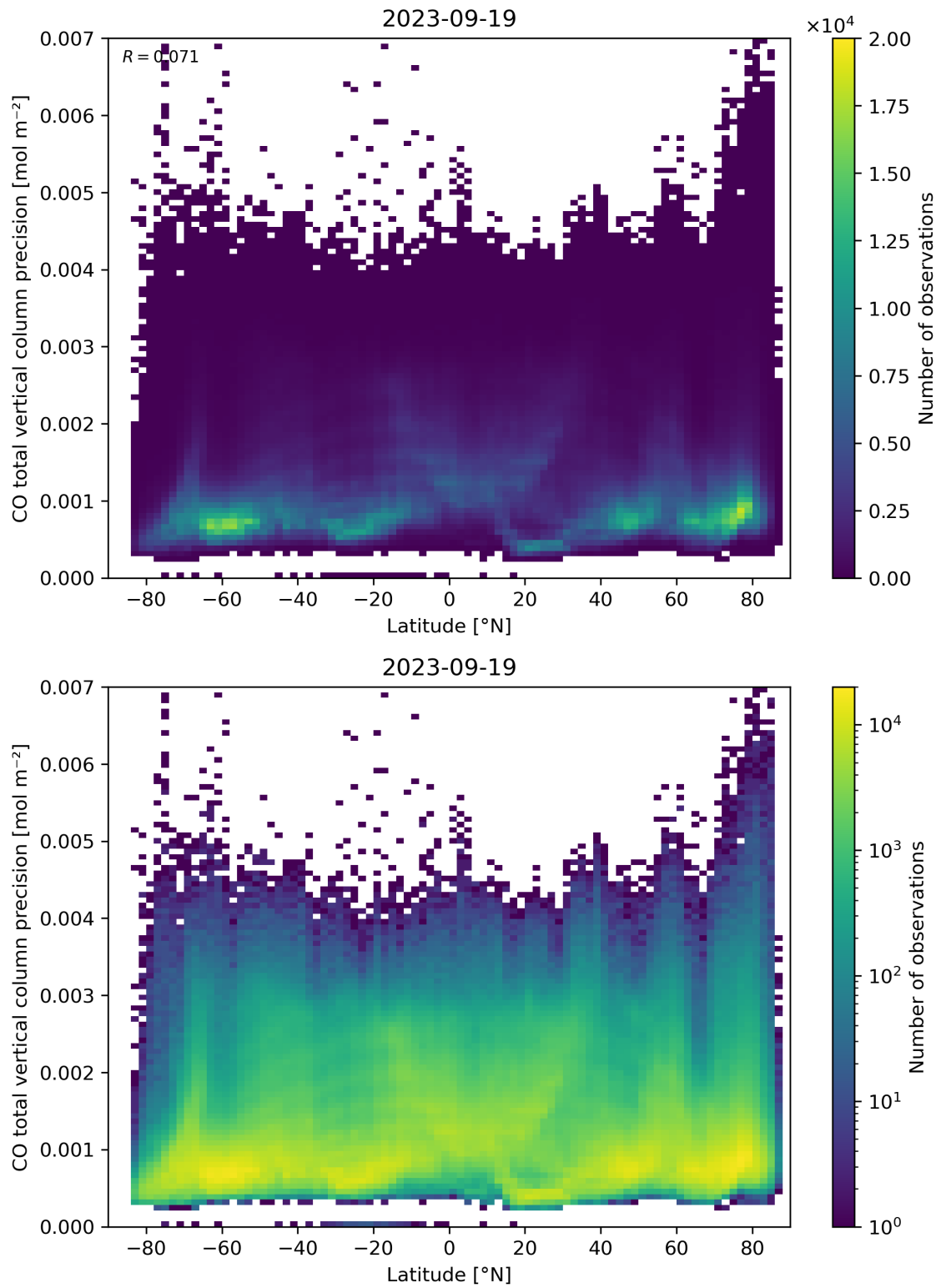
Figure 53: Scatter density plot of “Latitude” against “CO total vertical column precision” for 2023-09-18 to 2023-09-20.
