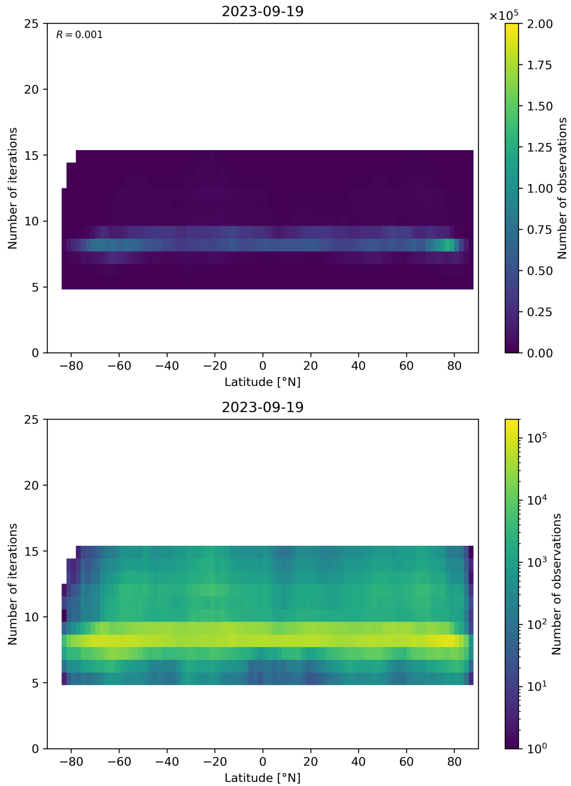
Figure 56: Scatter density plot of “Latitude” against “Number of iterations” for 2023-09-18 to 2023-09-20.
