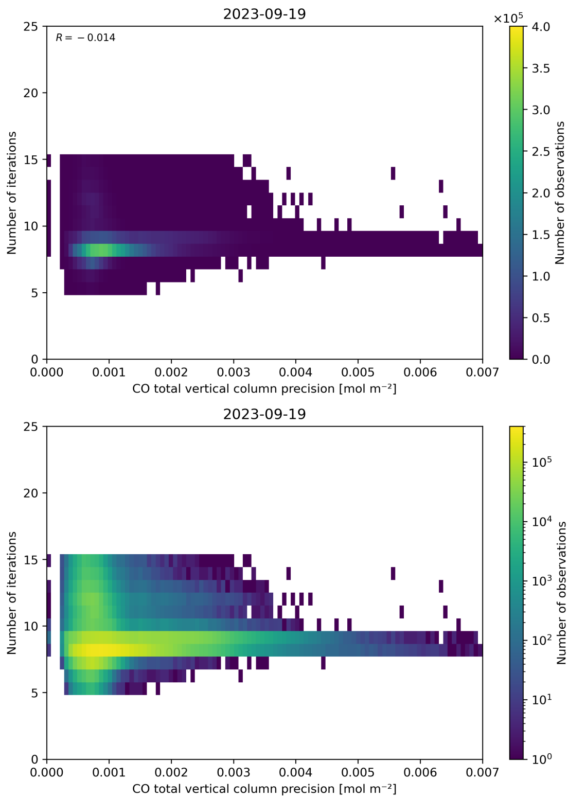
Figure 46: Scatter density plot of “CO total vertical column precision” against “Number of iterations” for 2023-09-18 to 2023-09-20.
