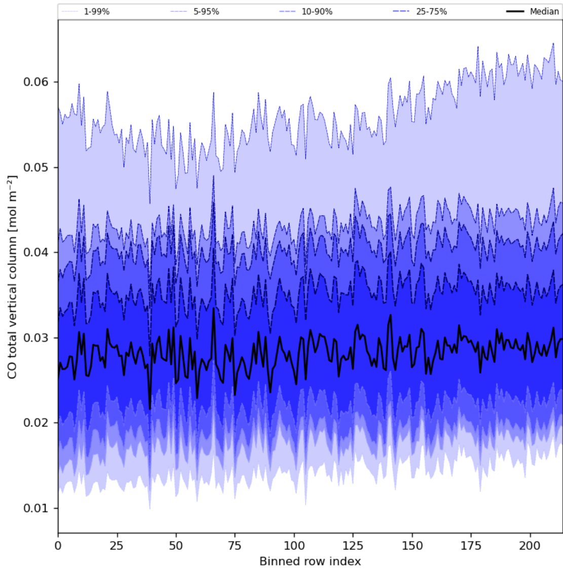
Figure 26: Along track statistics of “CO total vertical column” for 2023-09-18 to 2023-09-20
