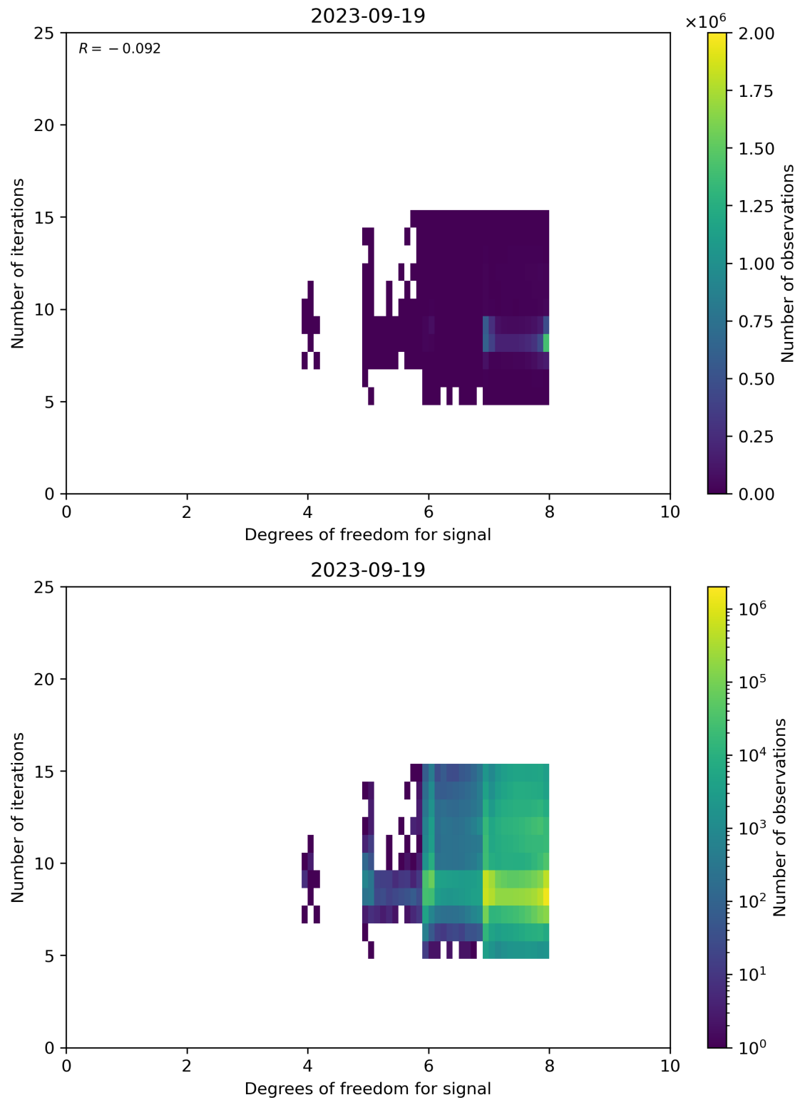
Figure 50: Scatter density plot of “Degrees of freedom for signal” against “Number of iterations” for 2023-09-18 to 2023-09-20.
