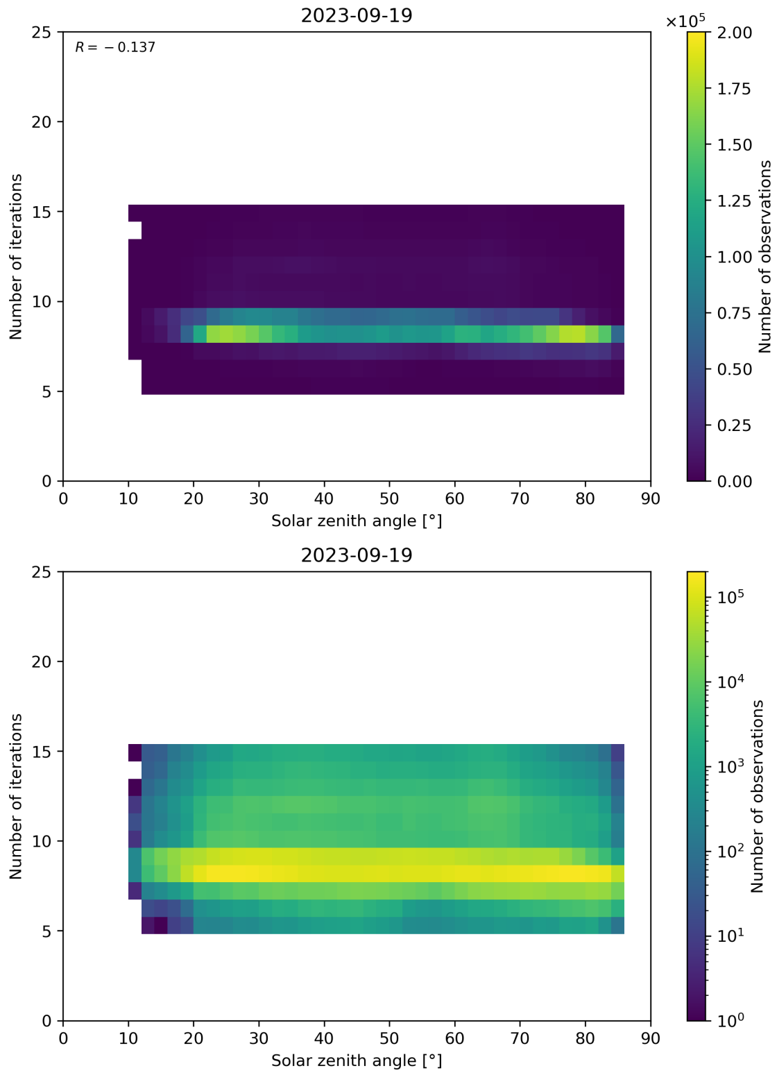
Figure 67: Scatter density plot of “Solar zenith angle” against “Number of iterations” for 2023-09-18 to 2023-09-20.
