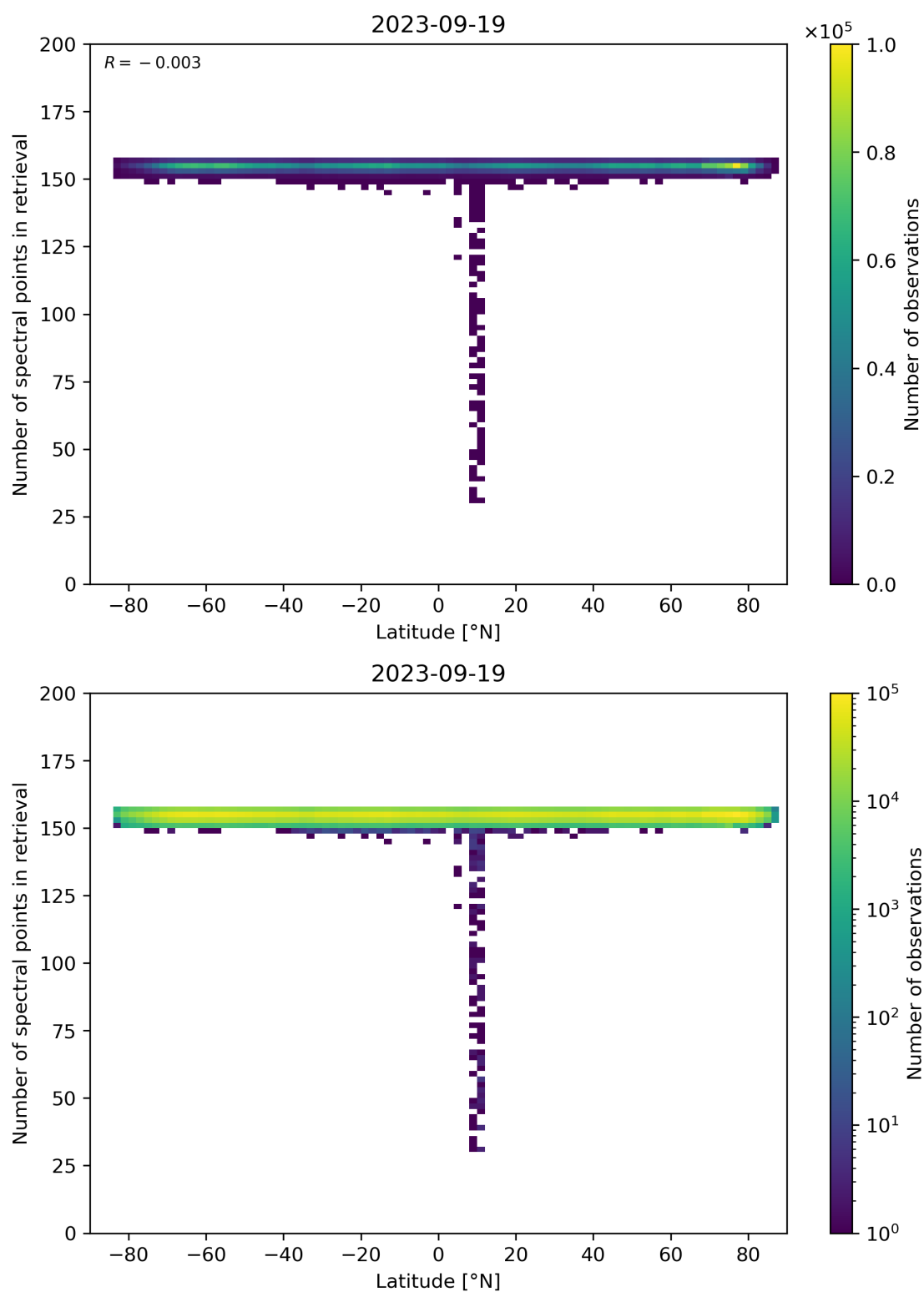
Figure 57: Scatter density plot of “Latitude” against “Number of spectral points in retrieval” for 2023-09-18 to 2023-09-20.
