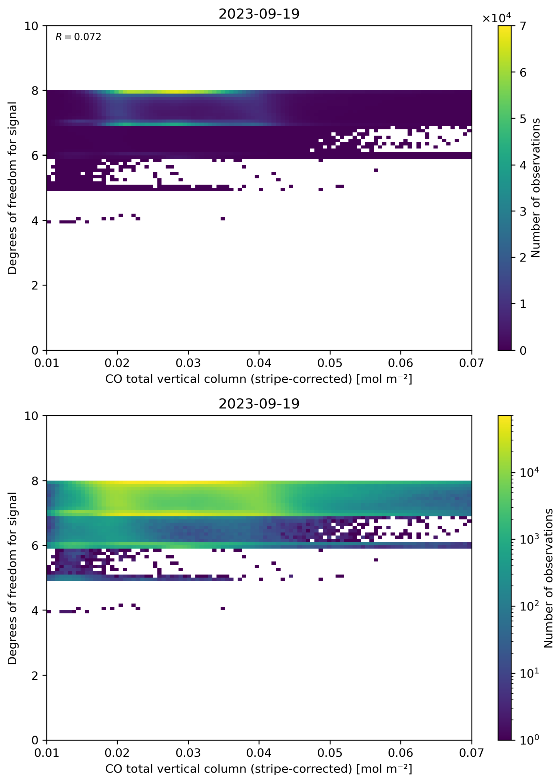
Figure 38: Scatter density plot of “CO total vertical column (stripe-corrected)” against “Degrees of freedom for signal” for 2023-09-18 to 2023-09-20.
