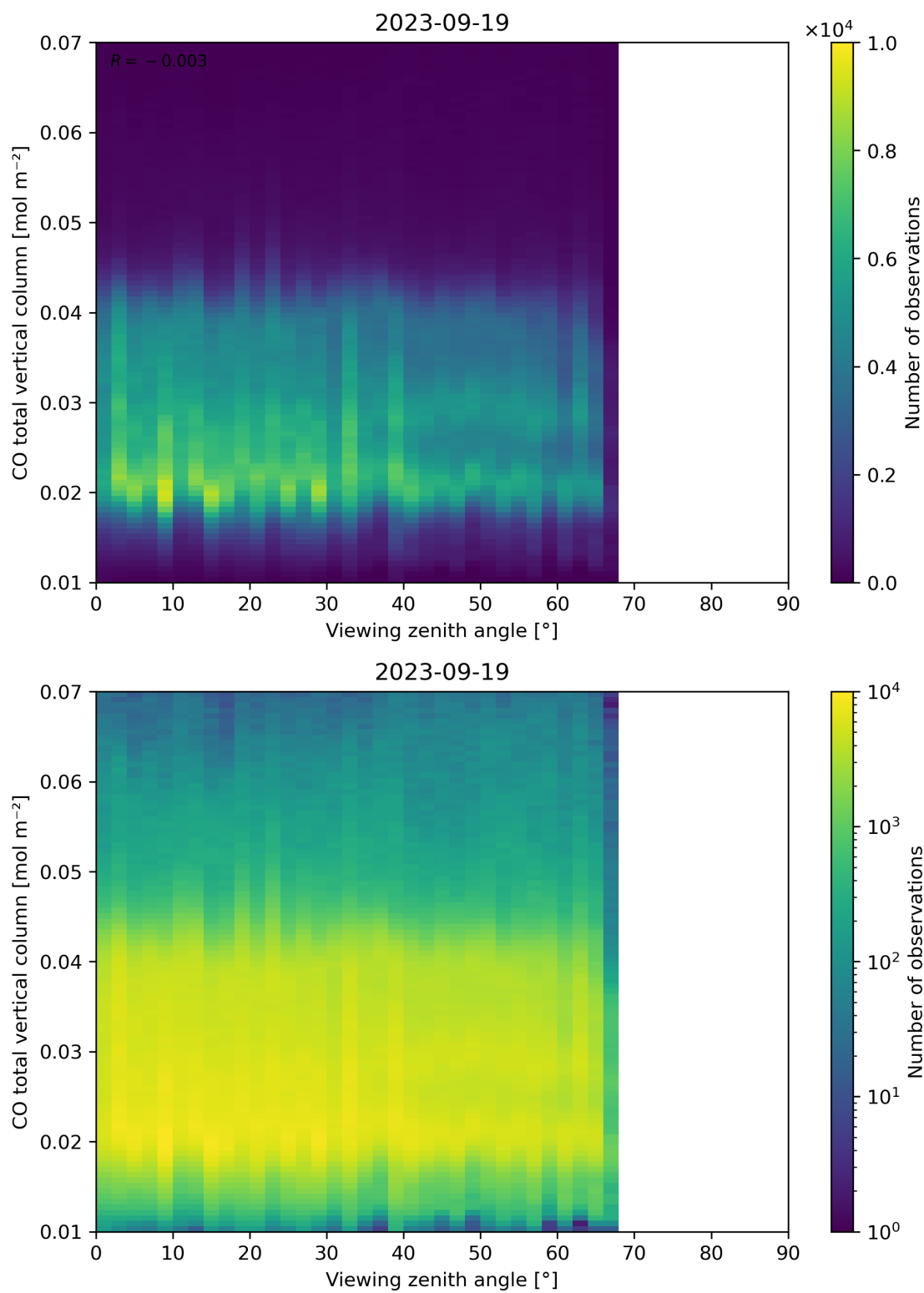
Figure 69: Scatter density plot of “Viewing zenith angle” against “CO total vertical column” for 2023-09-18 to 2023-09-20.
