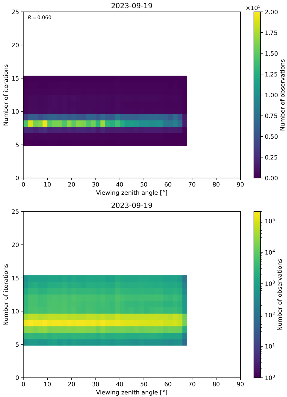
Figure 75: Scatter density plot of “Viewing zenith angle” against “Number of iterations” for 2023-09-18 to 2023-09-20.
