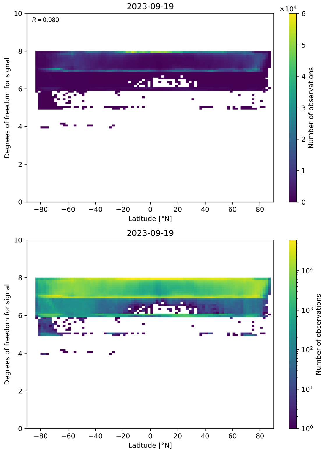
Figure 55: Scatter density plot of “Latitude” against “Degrees of freedom for signal” for 2023-09-18 to 2023-09-20.
