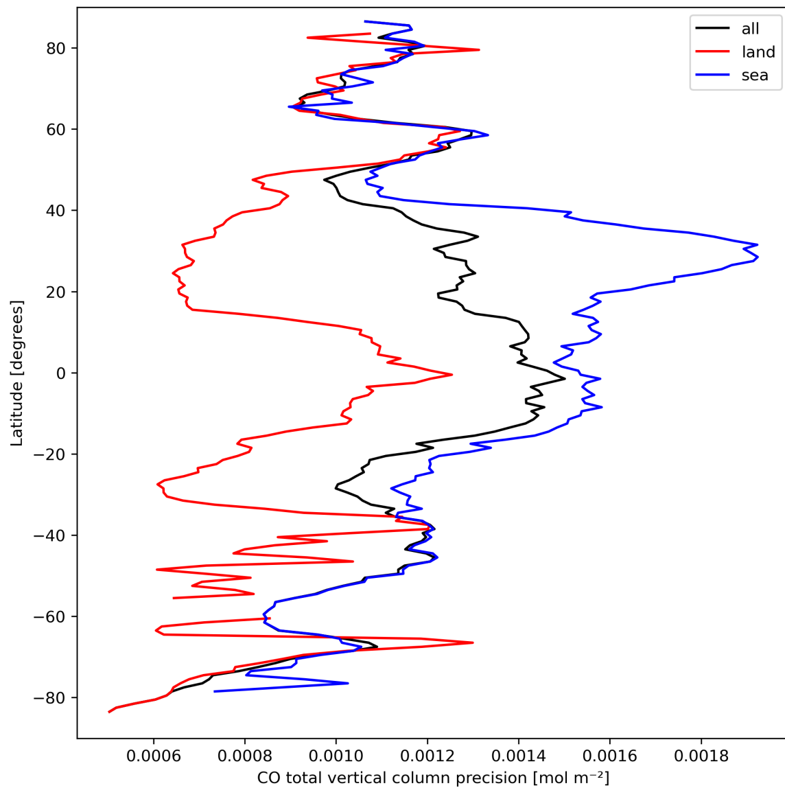
Figure 12: Zonal average of “CO total vertical column precision” for 2023-09-18 to 2023-09-20.
