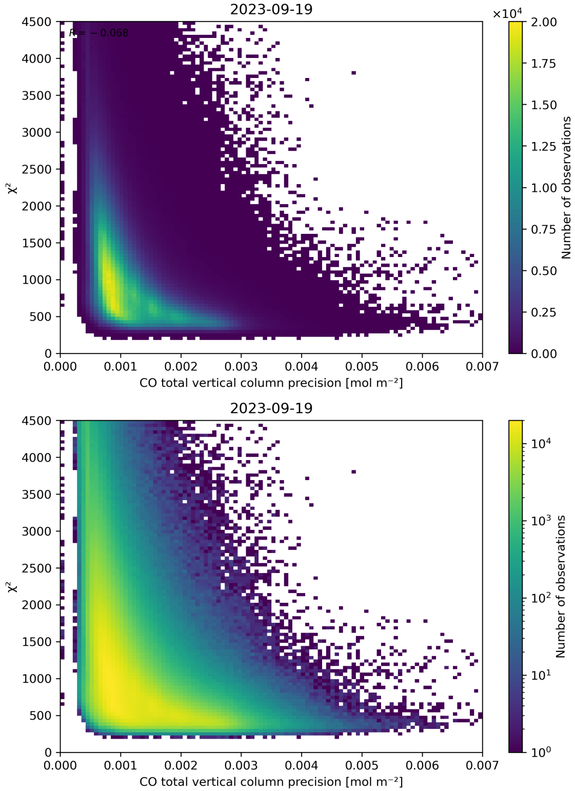
Figure 44: Scatter density plot of “CO total vertical column precision” against “ \chi^2 ” for 2023-09-18 to 2023-09-20.
