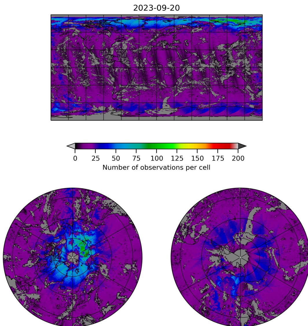
Figure 8: Map of the number of observations for 2023-09-20 to 2023-09-21
