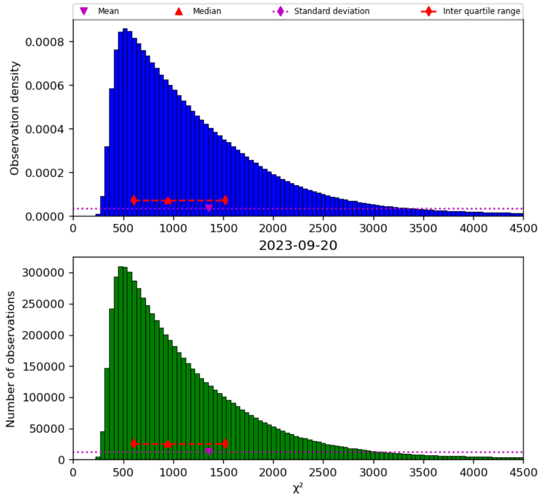
Figure 22: Histogram of “ \chi^2 ” for 2023-09-20 to 2023-09-21
