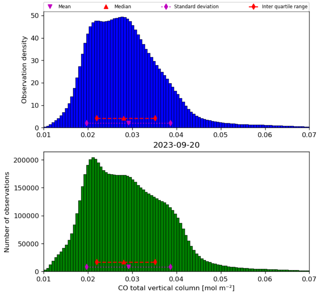
Figure 18: Histogram of “CO total vertical column” for 2023-09-20 to 2023-09-21
