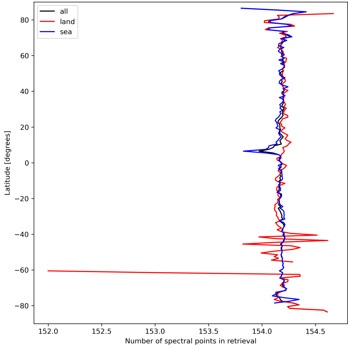
Figure 13: Zonal average of “Number of spectral points in retrieval” for 2023-09-20 to 2023-09-21.
