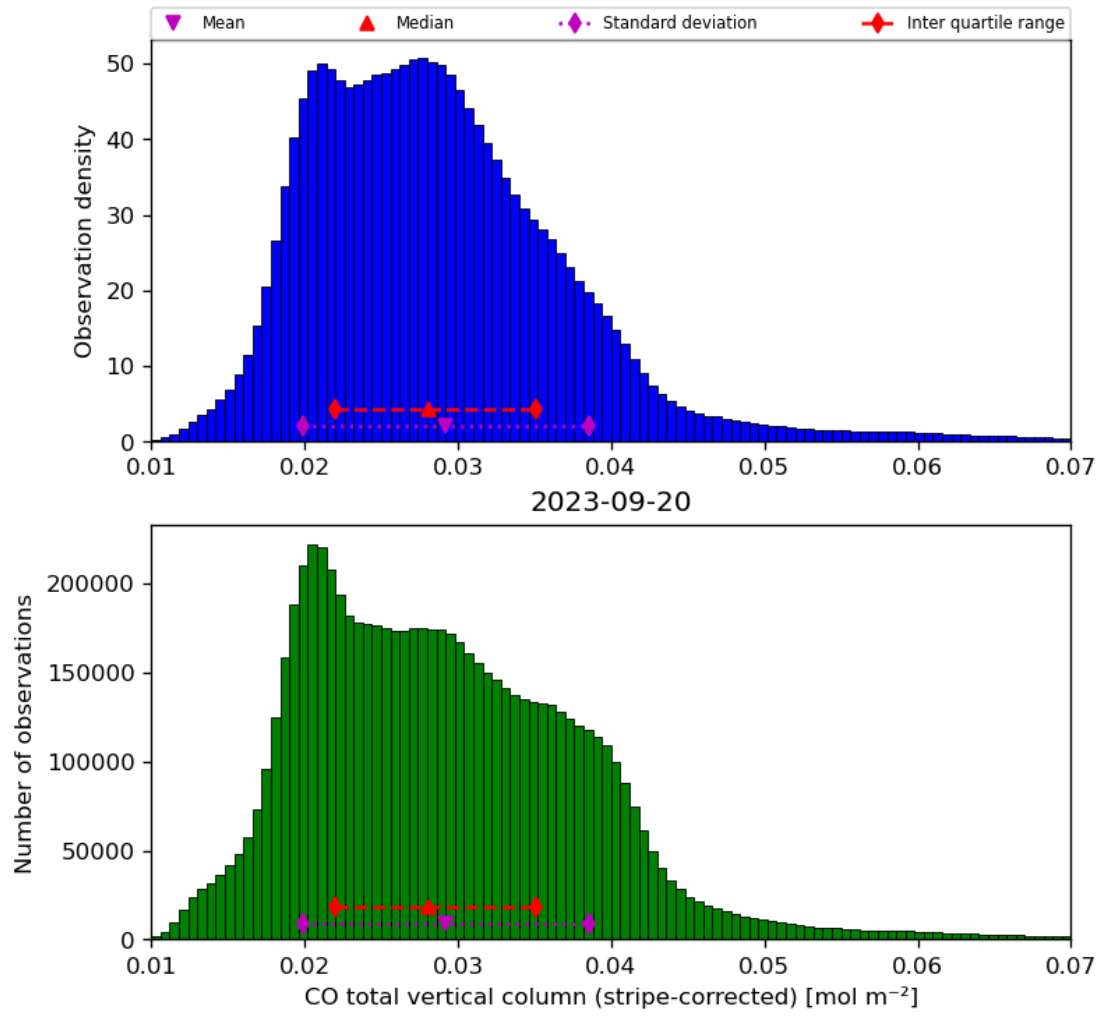
Figure 19: Histogram of “CO total vertical column (stripe-corrected)” for 2023-09-20 to 2023-09-21
