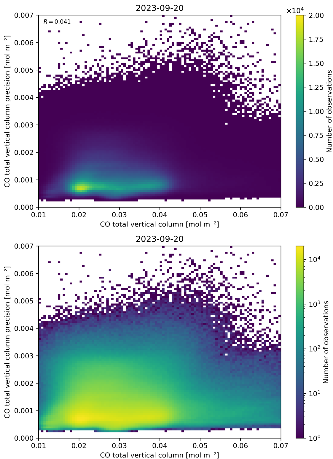
Figure 34: Scatter density plot of “CO total vertical column” against “CO total vertical column precision” for 2023-09-20 to 2023-09-21.
