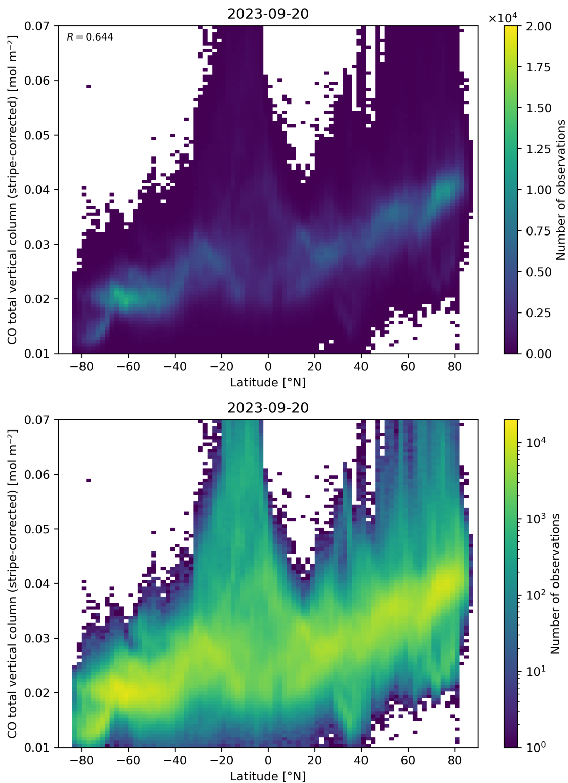
Figure 52: Scatter density plot of “Latitude” against “CO total vertical column (stripe-corrected)” for 2023-09-20 to 2023-09-21.
