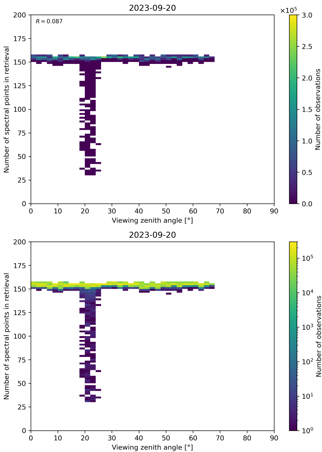
Figure 76: Scatter density plot of “Viewing zenith angle” against “Number of spectral points in retrieval” for 2023-09-20 to 2023-09-21.
