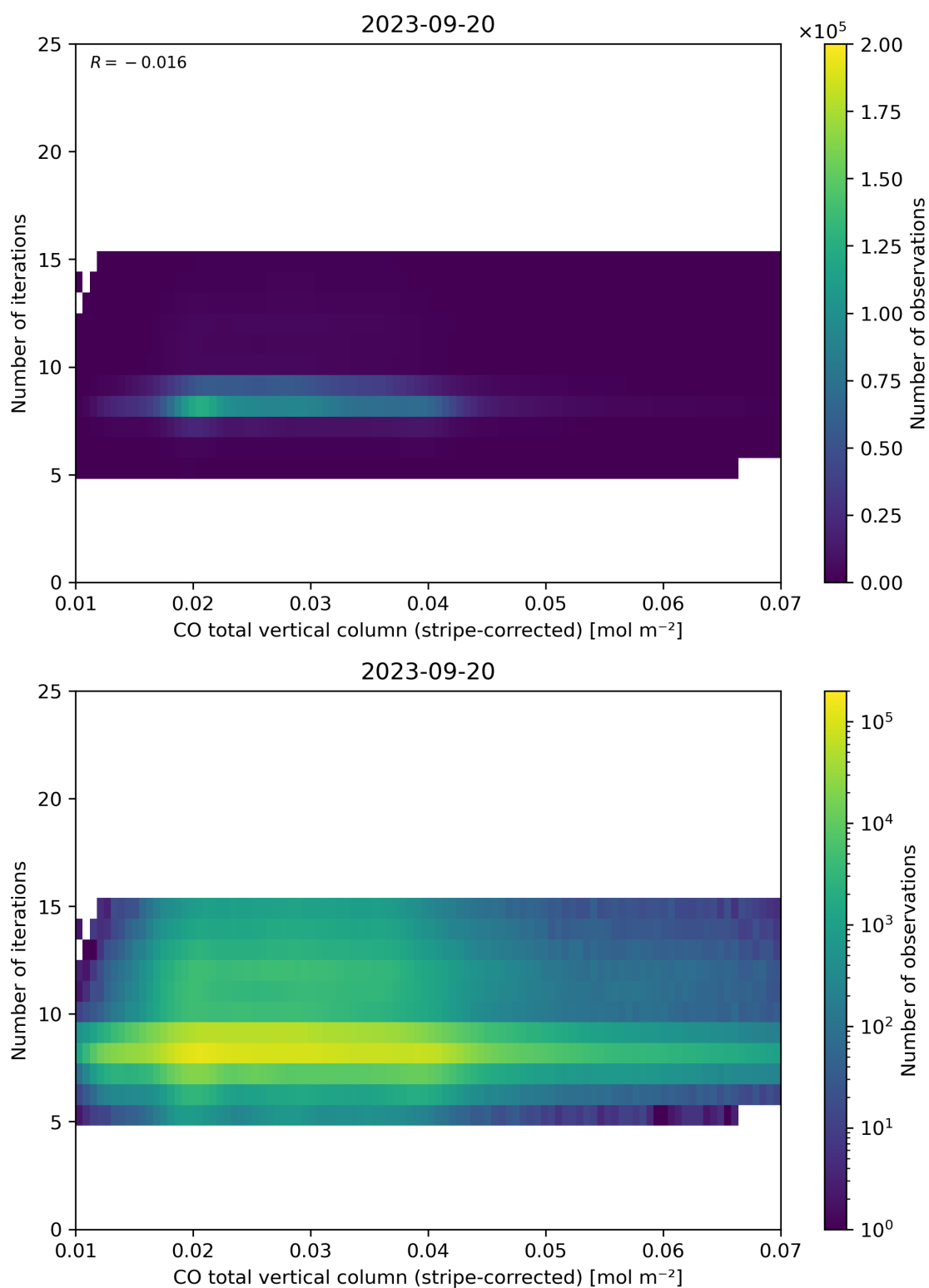
Figure 39: Scatter density plot of “CO total vertical column (stripe-corrected)” against “Number of iterations” for 2023-09-20 to 2023-09-21.
