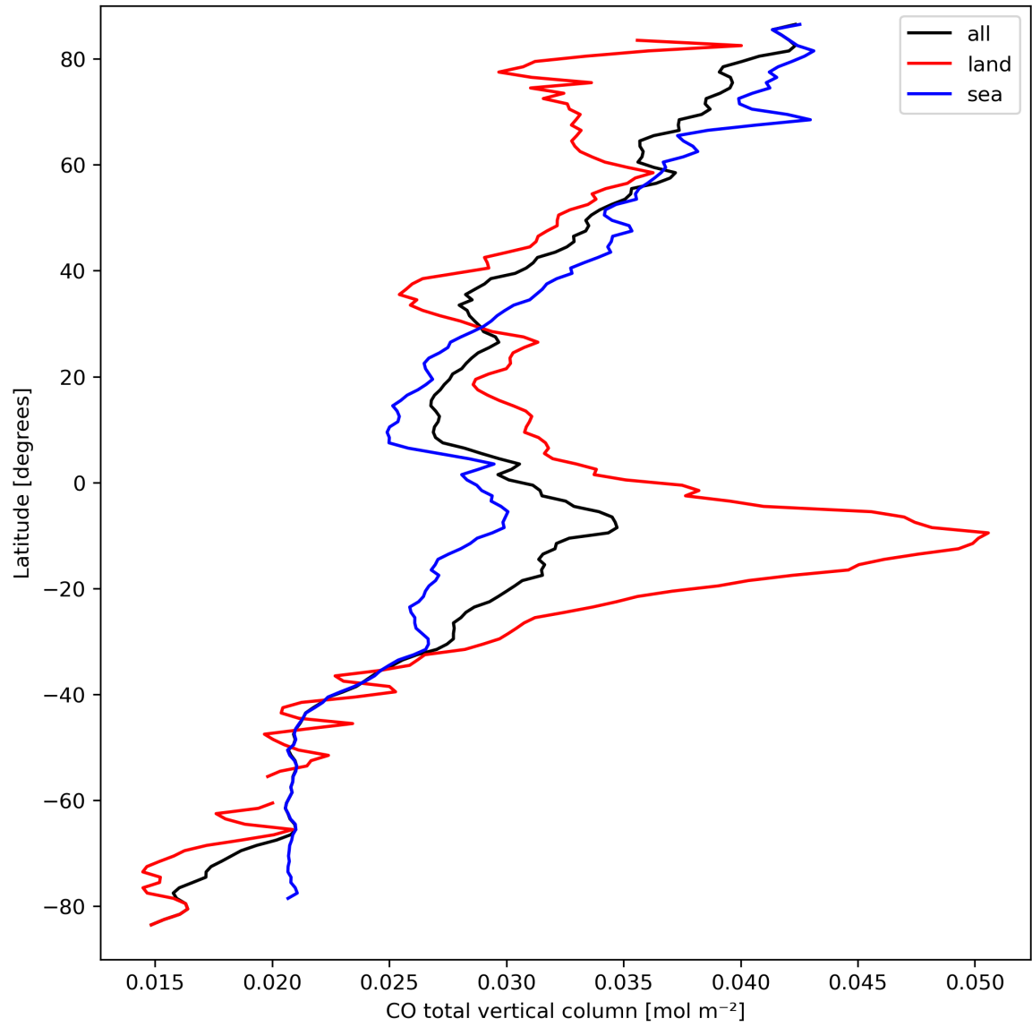
Figure 10: Zonal average of “CO total vertical column” for 2023-09-20 to 2023-09-21.
