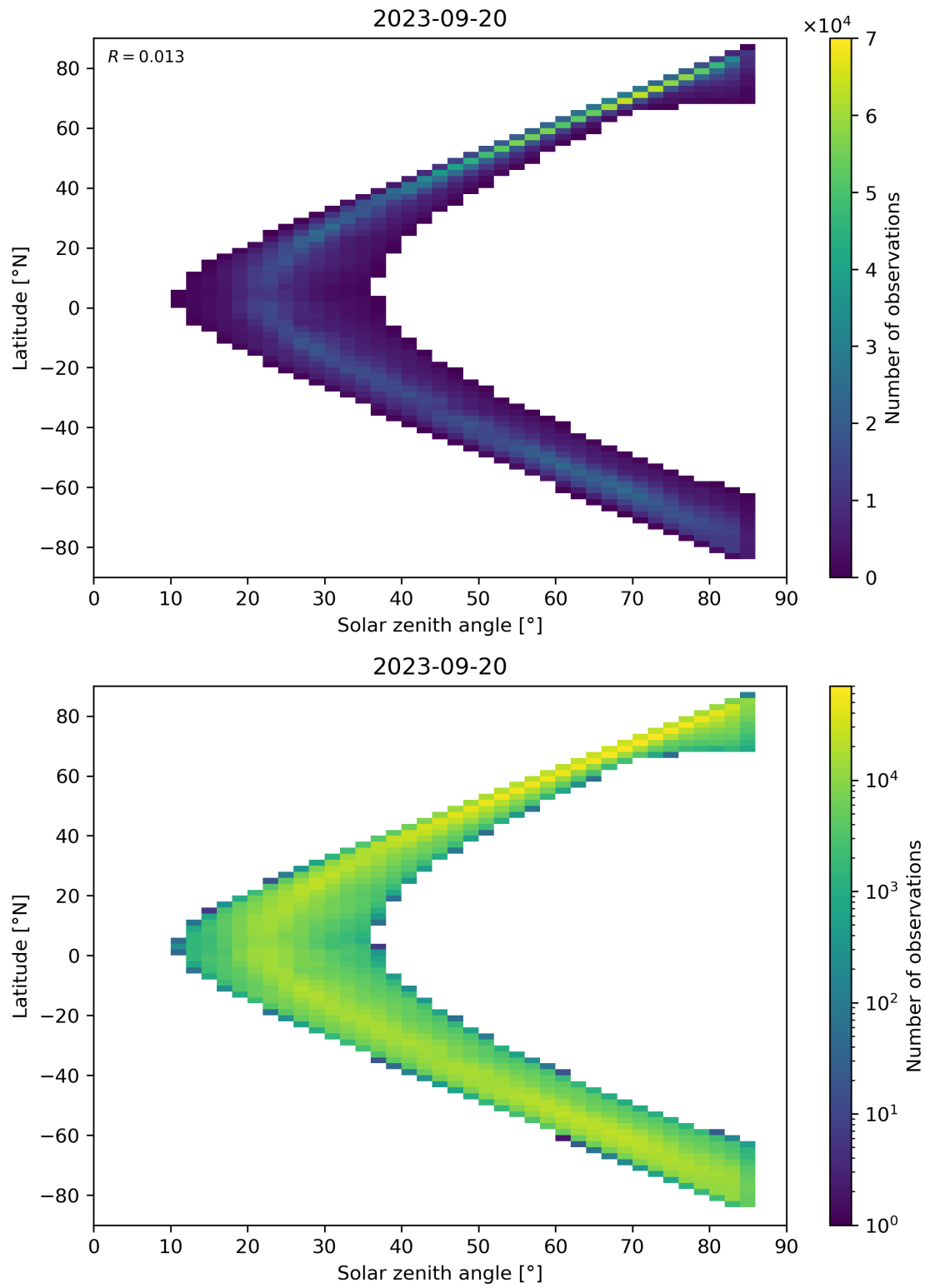
Figure 66: Scatter density plot of “Solar zenith angle” against “Latitude” for 2023-09-20 to 2023-09-21.
