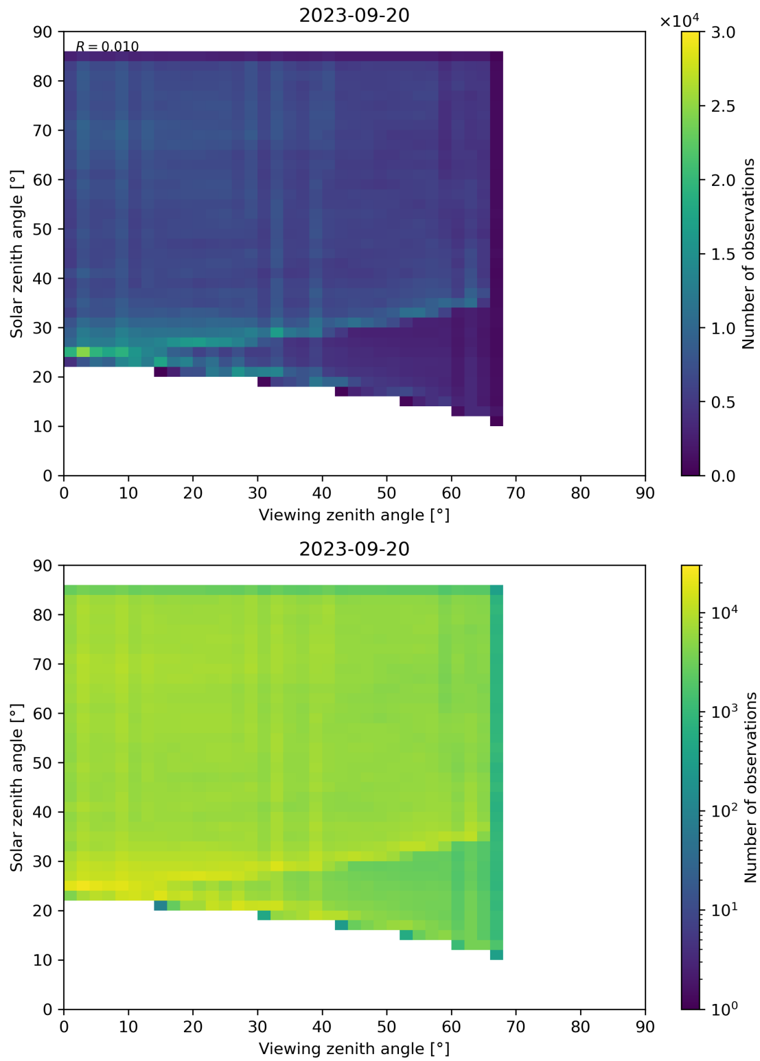
Figure 77: Scatter density plot of “Viewing zenith angle” against “Solar zenith angle” for 2023-09-20 to 2023-09-21.
