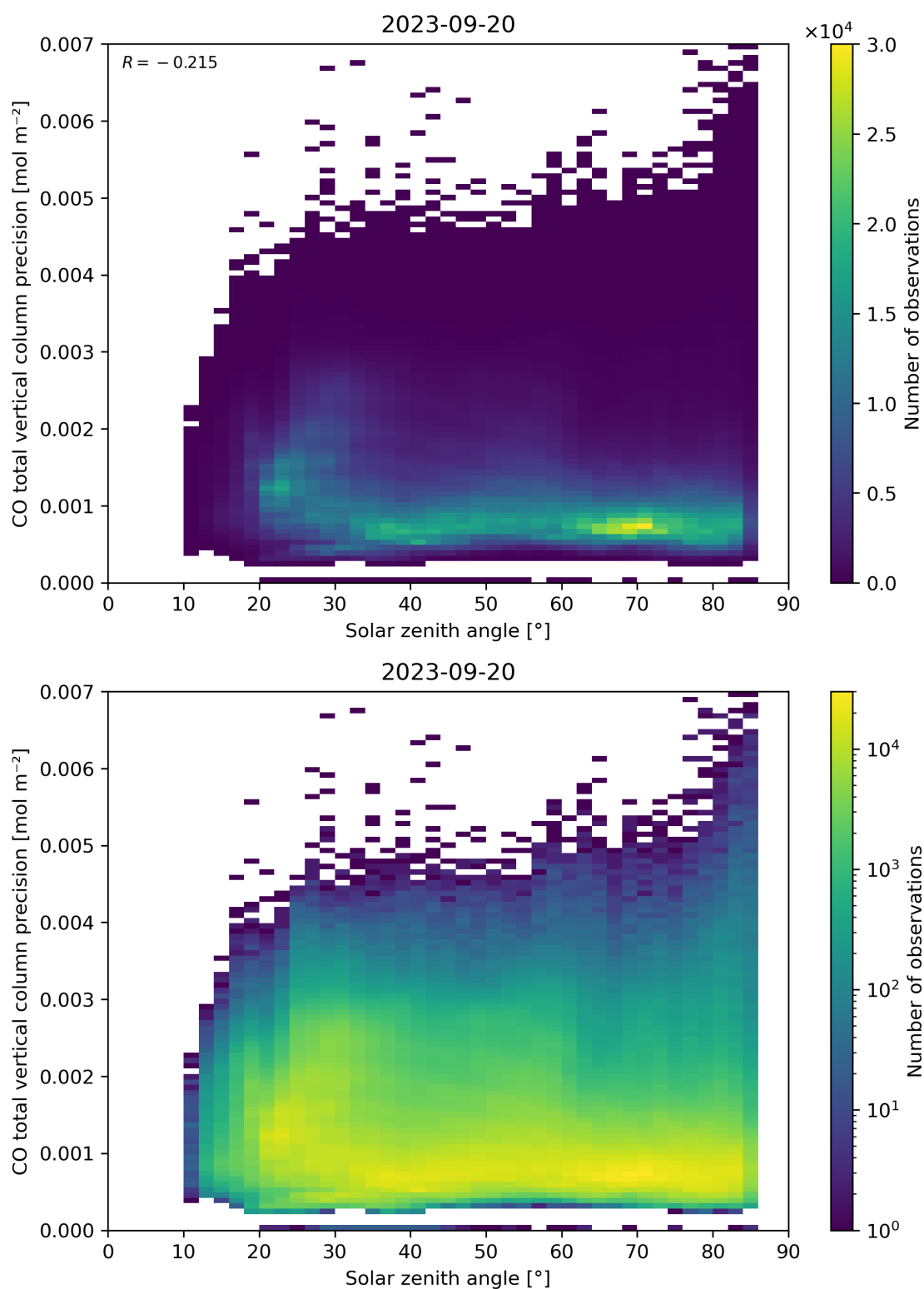
Figure 63: Scatter density plot of “Solar zenith angle” against “CO total vertical column precision” for 2023-09-20 to 2023-09-21.
