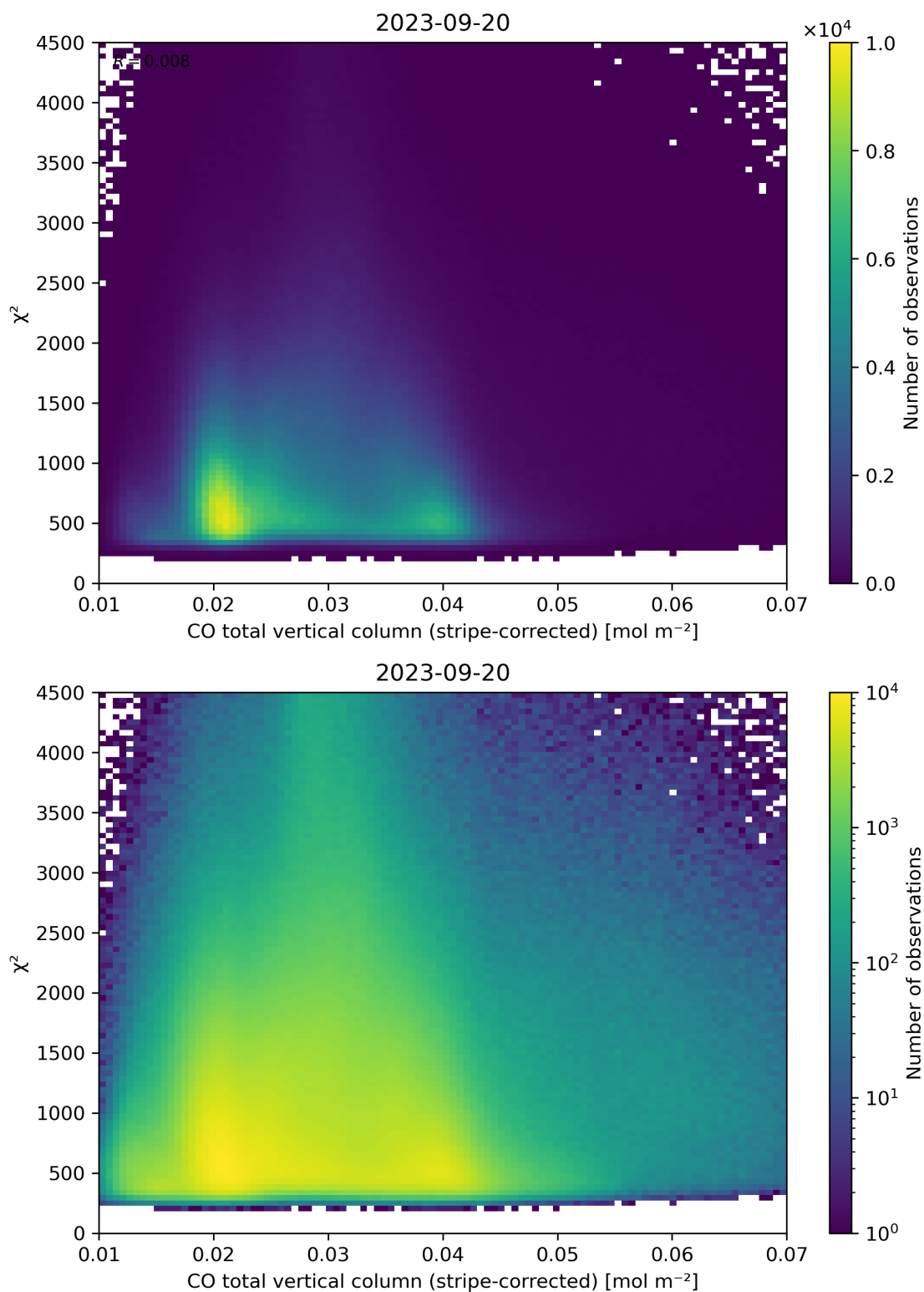
Figure 37: Scatter density plot of “CO total vertical column (stripe-corrected)” against “ \chi^2 ” for 2023-09-20 to 2023-09-21.
