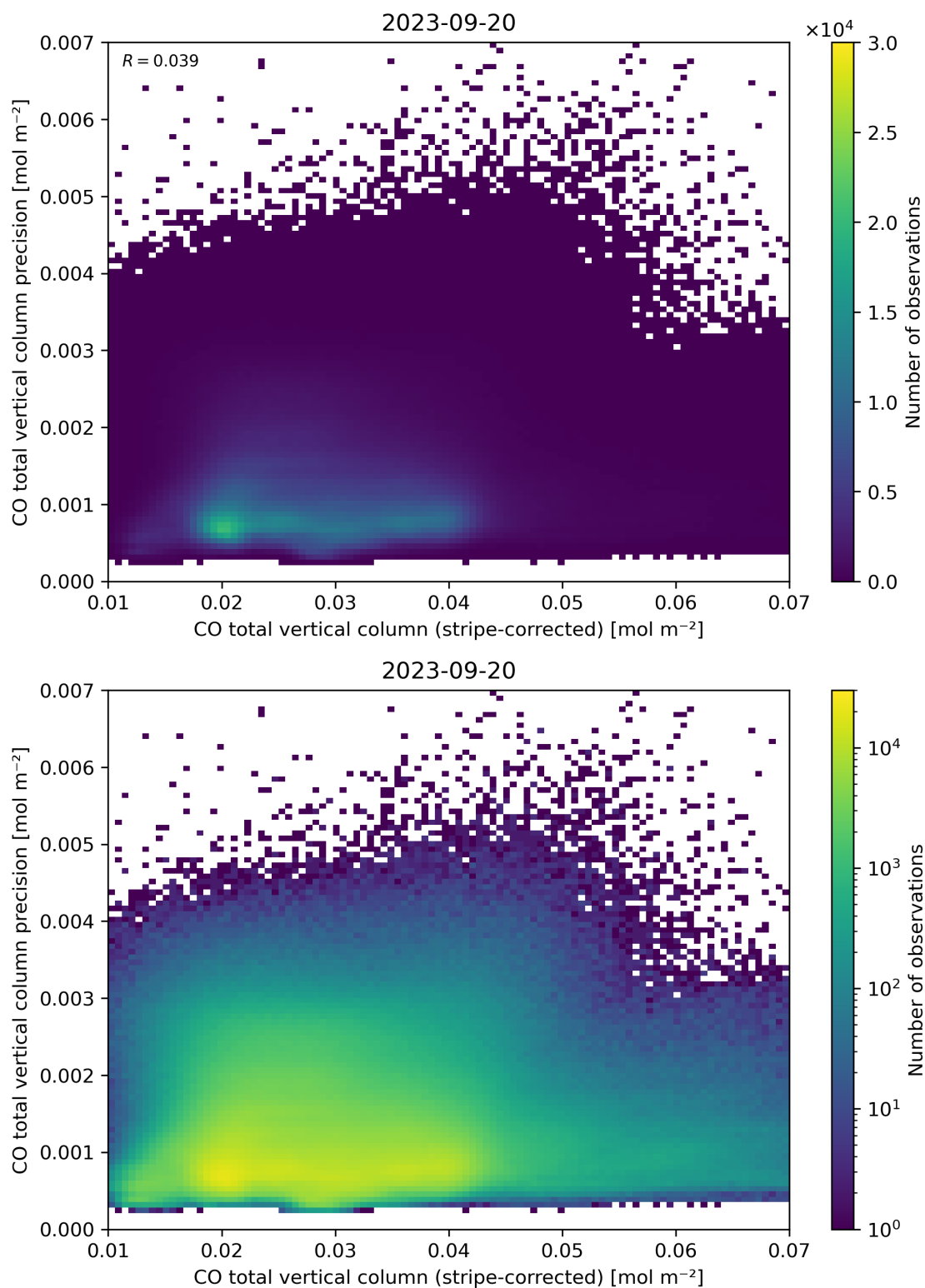
Figure 36: Scatter density plot of “CO total vertical column (stripe-corrected)” against “CO total vertical column precision” for 2023-09-20 to 2023-09-21.
