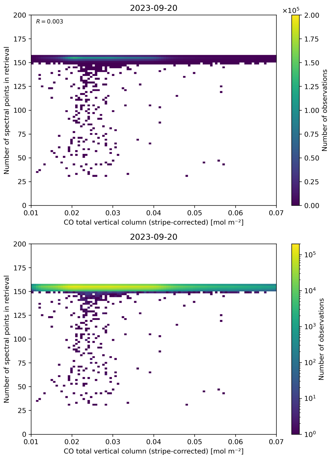
Figure 40: Scatter density plot of “CO total vertical column (stripe-corrected)” against “Number of spectral points in retrieval” for 2023-09-20 to 2023-09-21.
