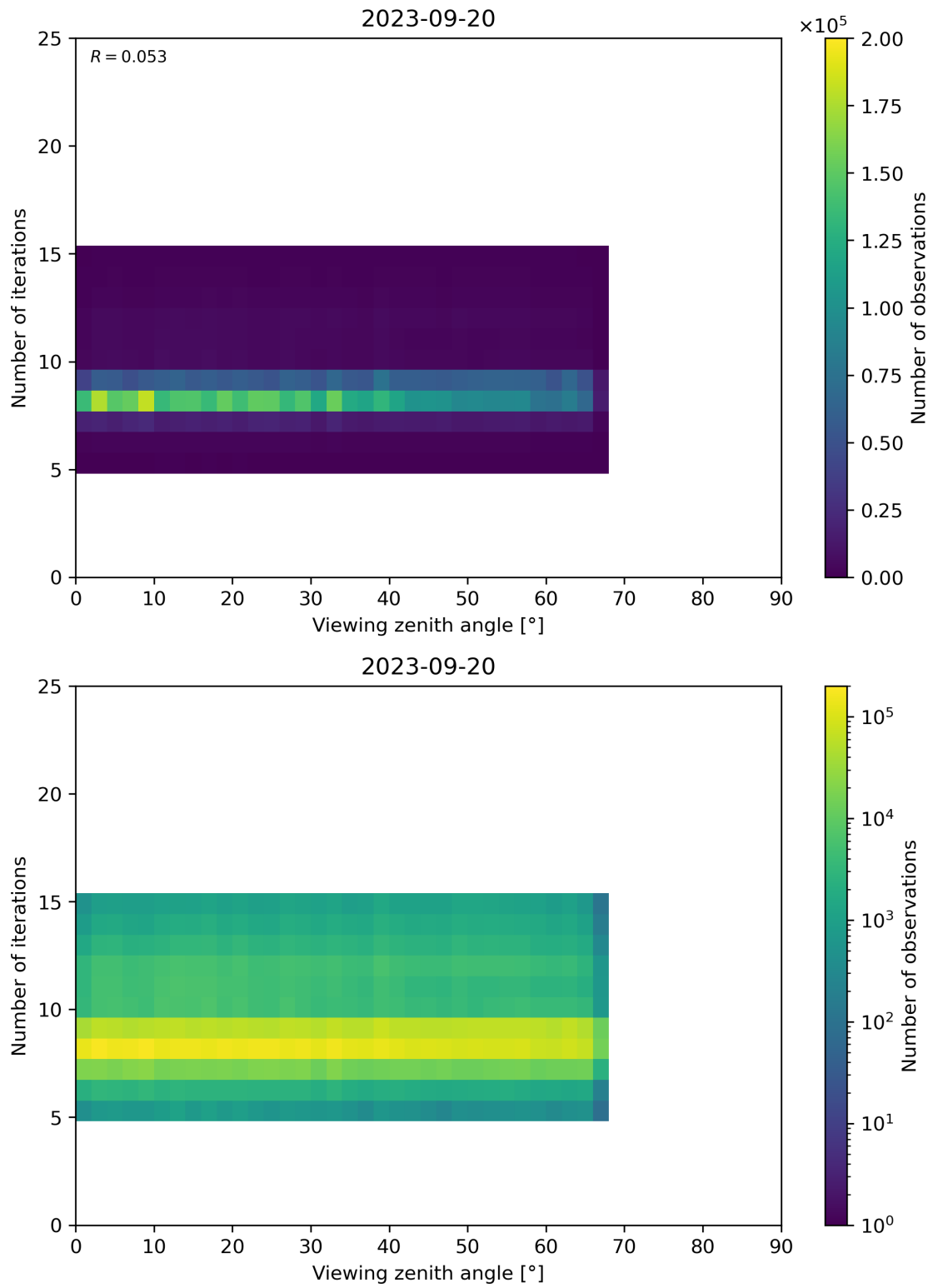
Figure 75: Scatter density plot of “Viewing zenith angle” against “Number of iterations” for 2023-09-20 to 2023-09-21.
