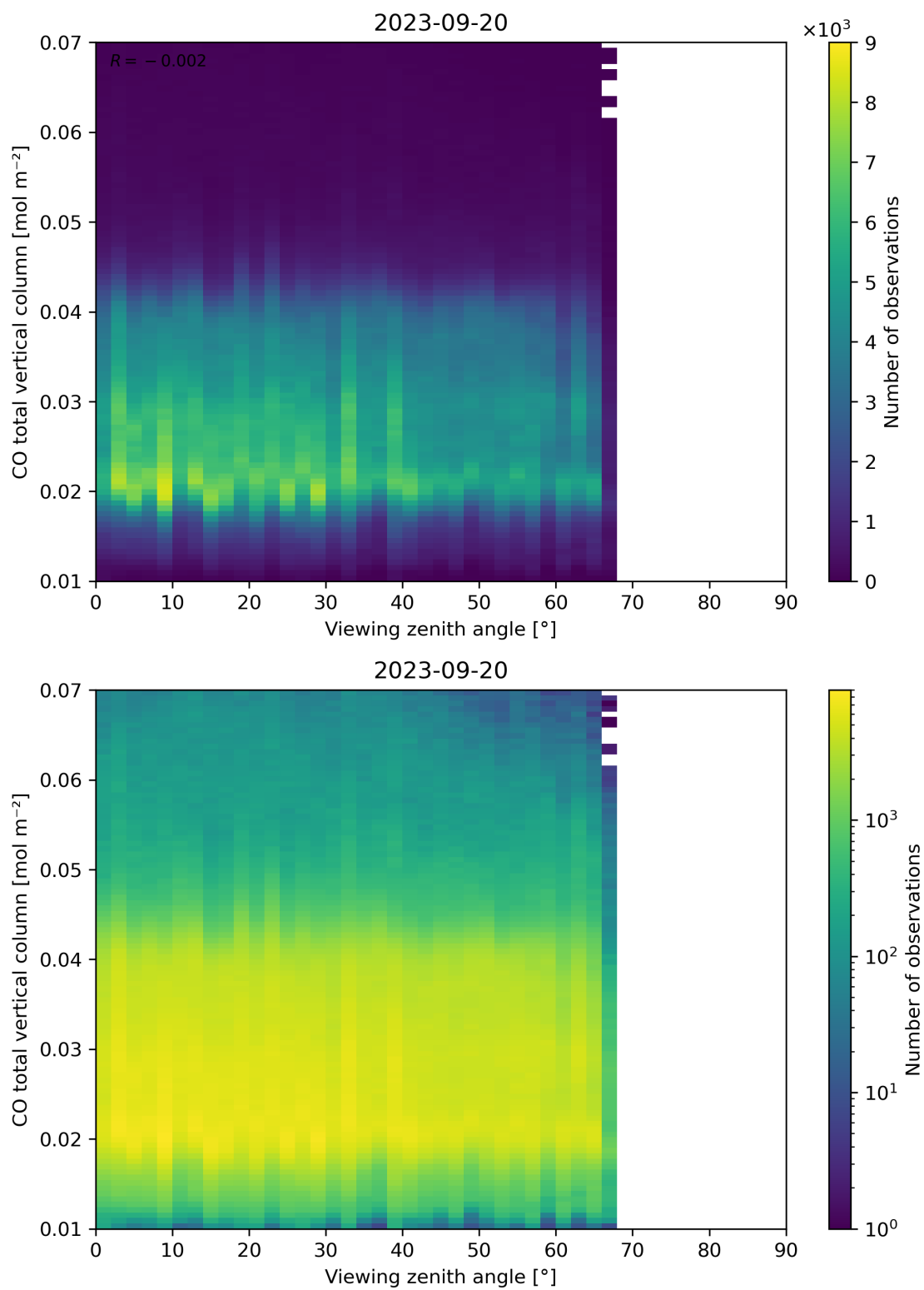
Figure 69: Scatter density plot of “Viewing zenith angle” against “CO total vertical column” for 2023-09-20 to 2023-09-21.
