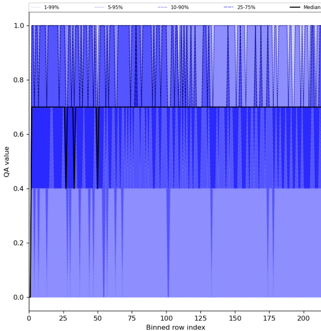
Figure 25: Along track statistics of “QA value” for 2023-09-20 to 2023-09-21
