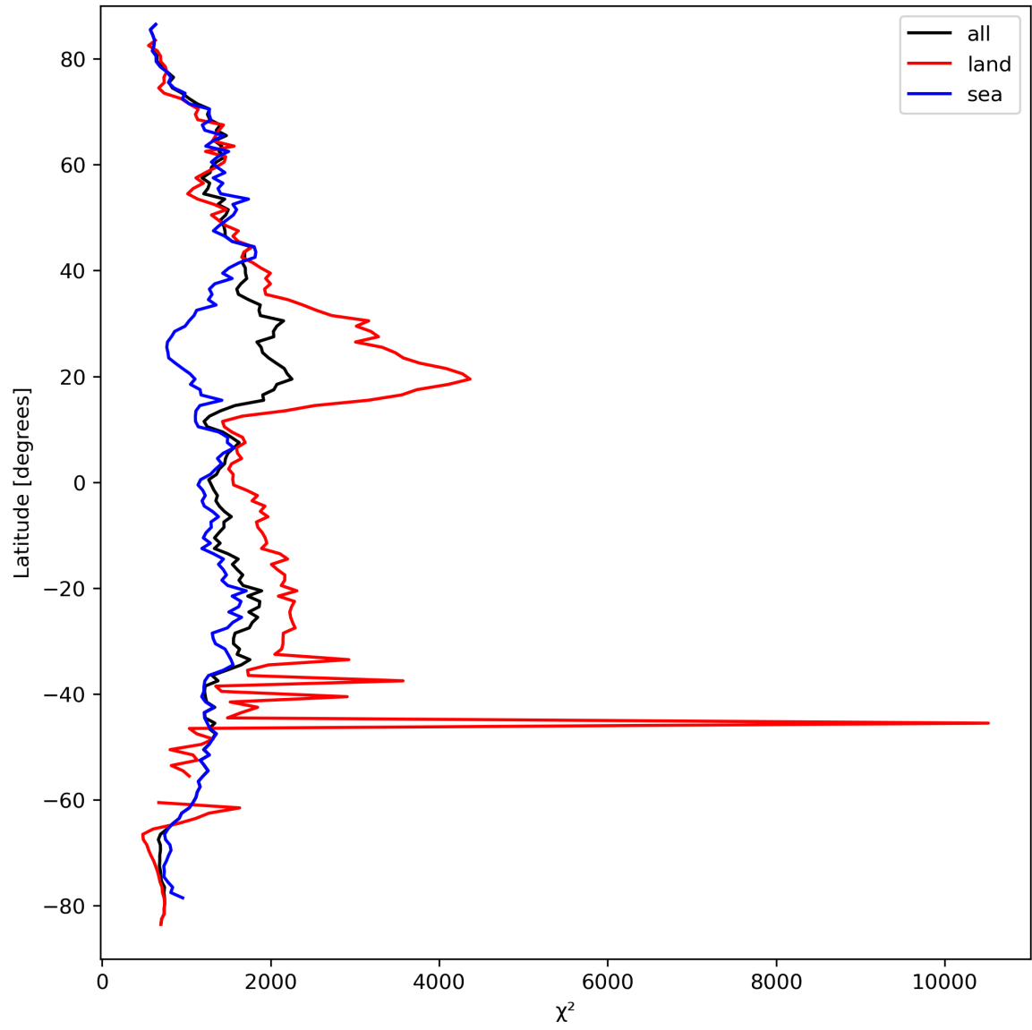
Figure 14: Zonal average of “ \chi^2 ” for 2023-09-20 to 2023-09-21.
