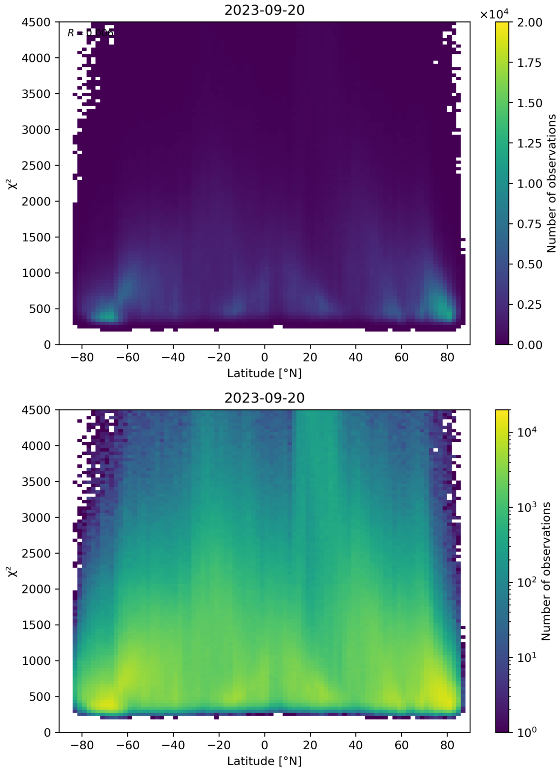
Figure 54: Scatter density plot of “Latitude” against “ \chi^2 ” for 2023-09-20 to 2023-09-21.
