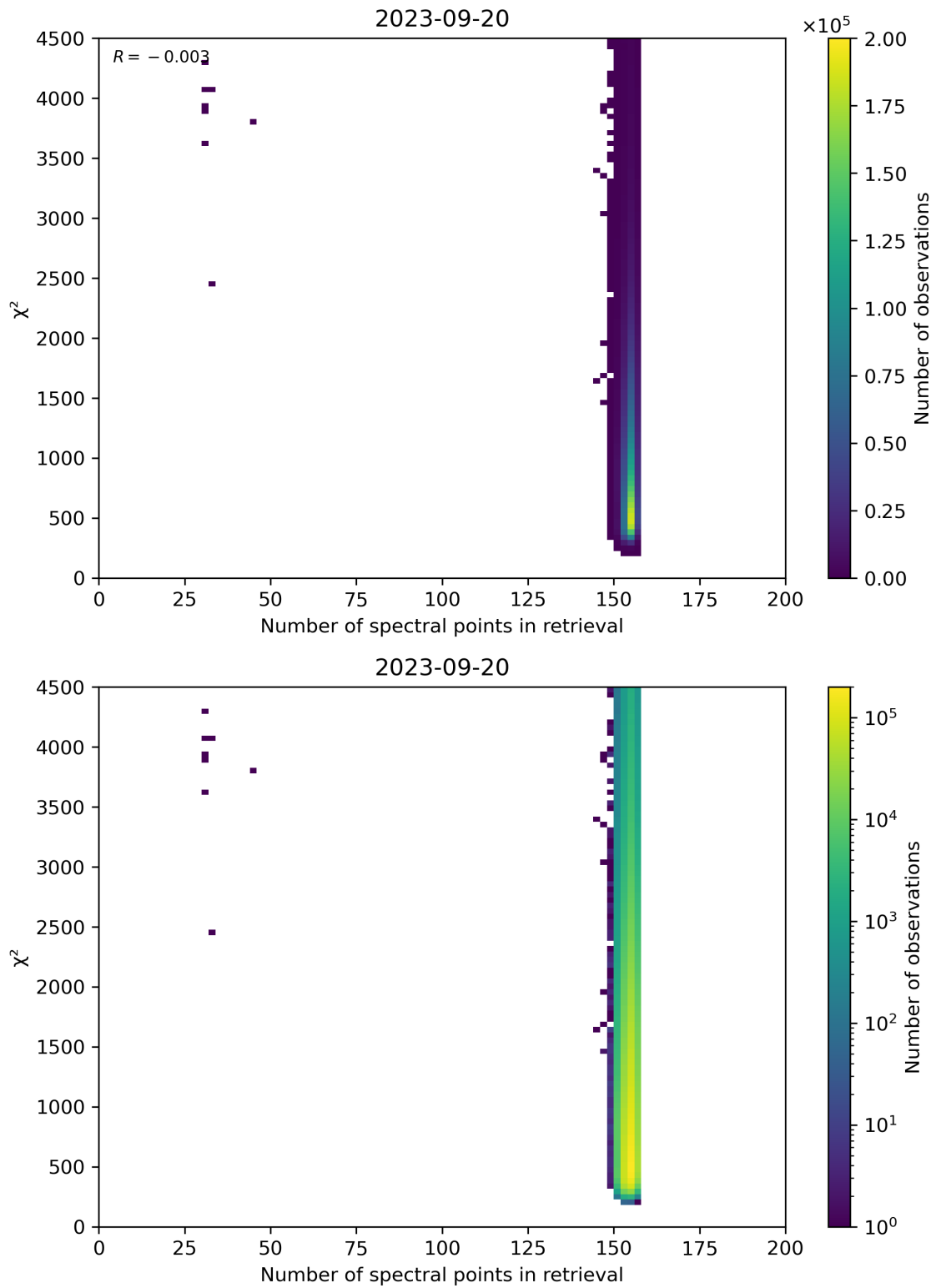
Figure 58: Scatter density plot of “Number of spectral points in retrieval” against “ \chi^2 ” for 2023-09-20 to 2023-09-21.
