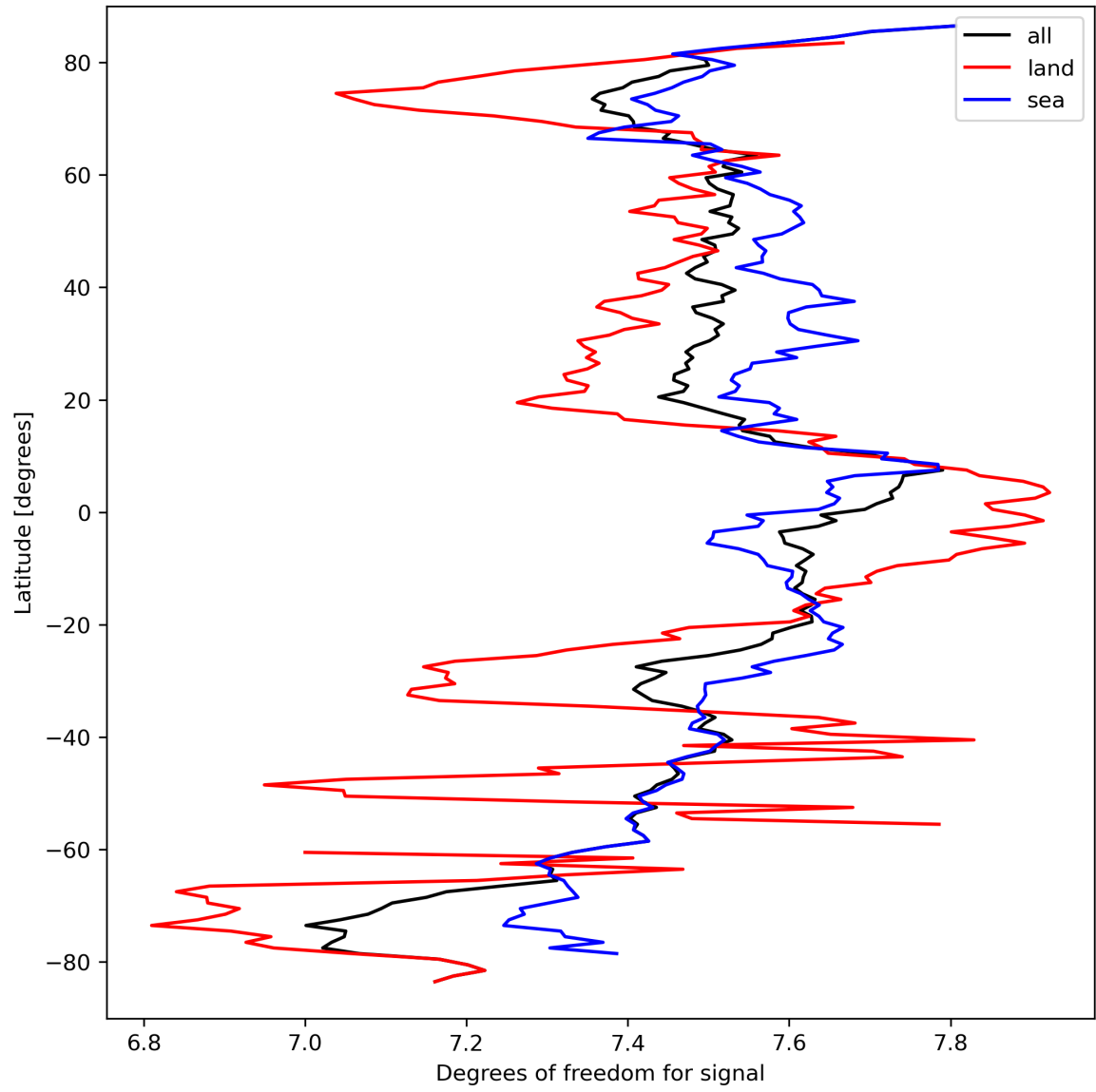
Figure 15: Zonal average of “Degrees of freedom for signal” for 2023-09-20 to 2023-09-21.
