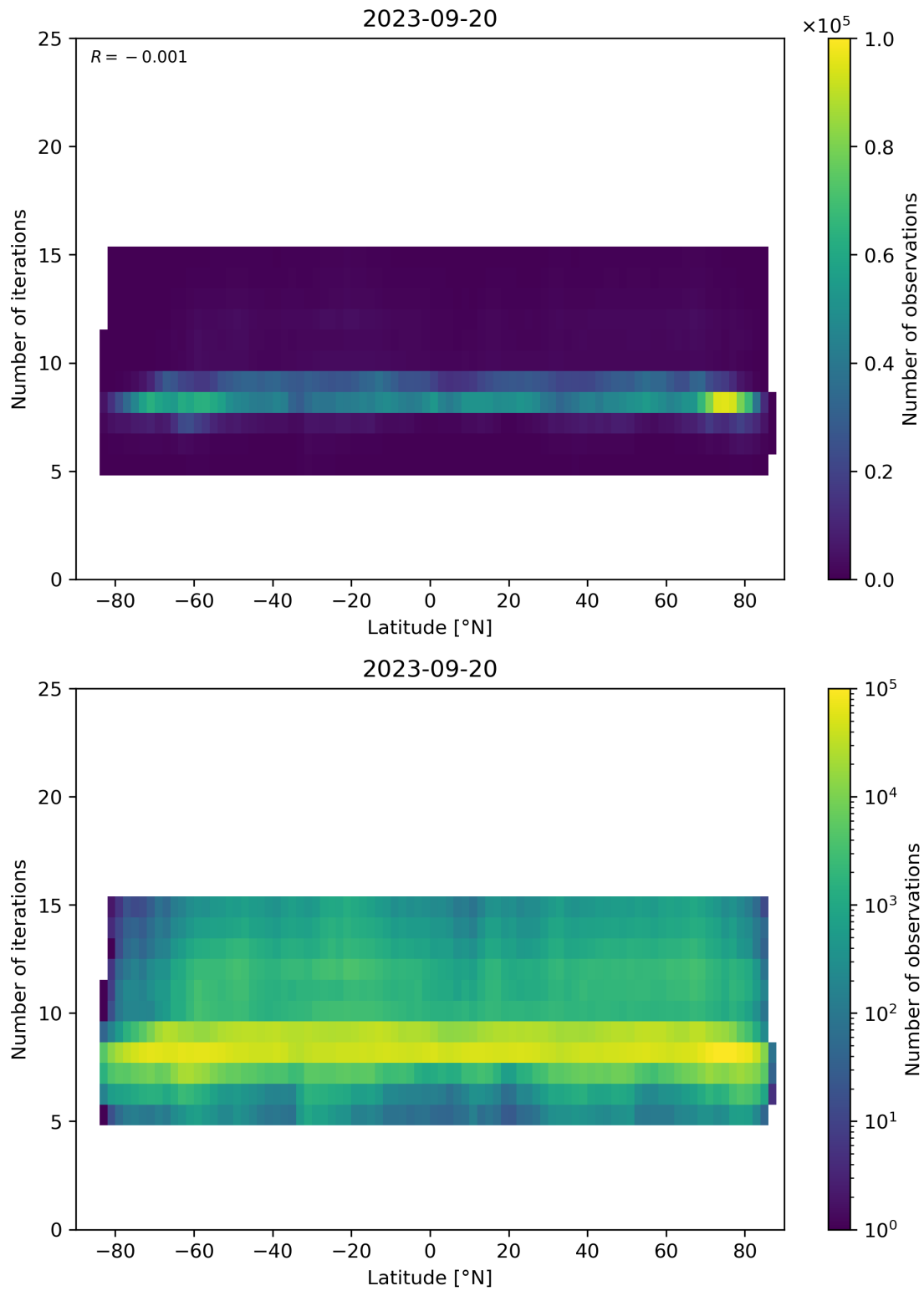
Figure 56: Scatter density plot of “Latitude” against “Number of iterations” for 2023-09-20 to 2023-09-21.
