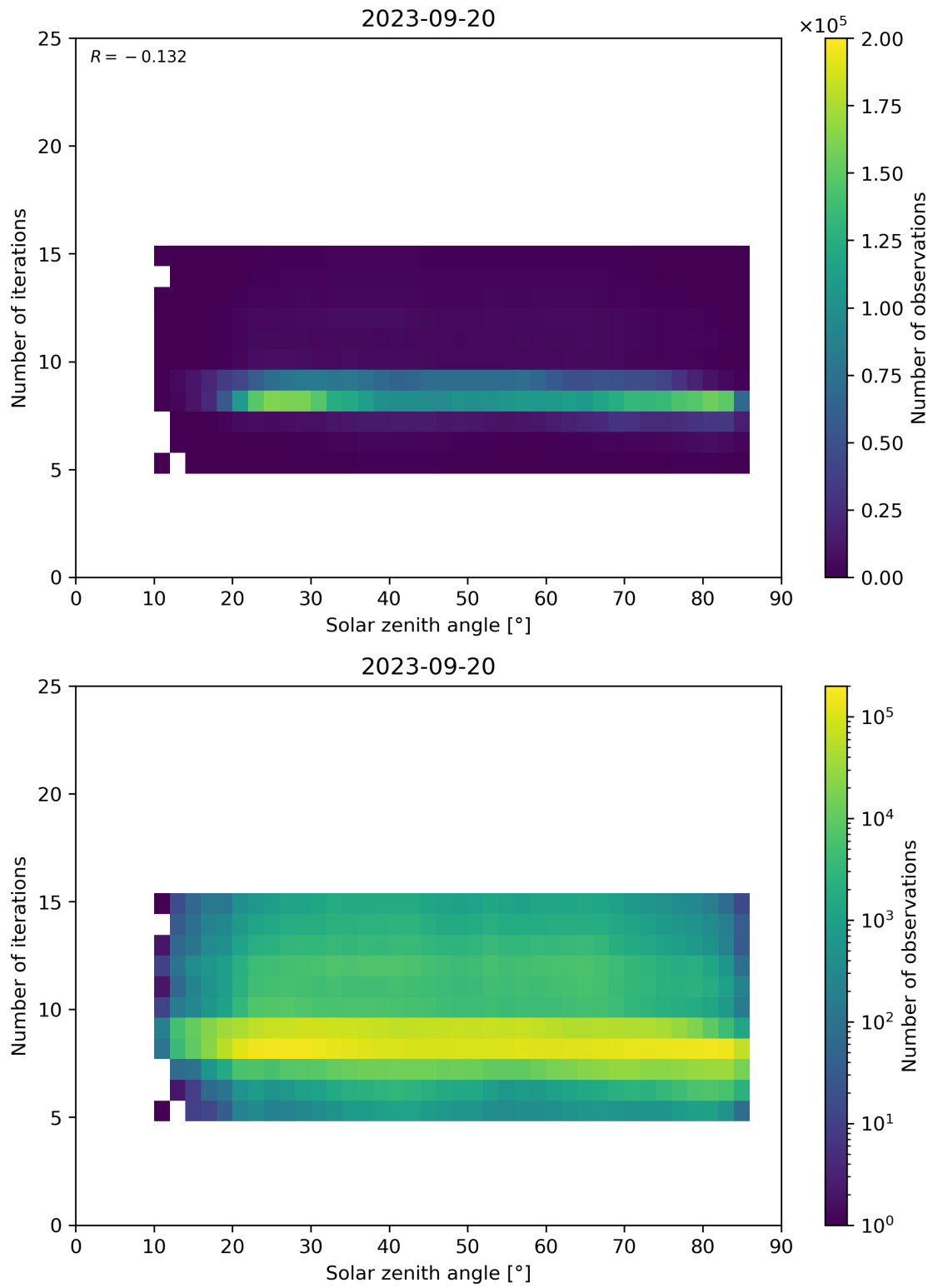
Figure 67: Scatter density plot of “Solar zenith angle” against “Number of iterations” for 2023-09-20 to 2023-09-21.
