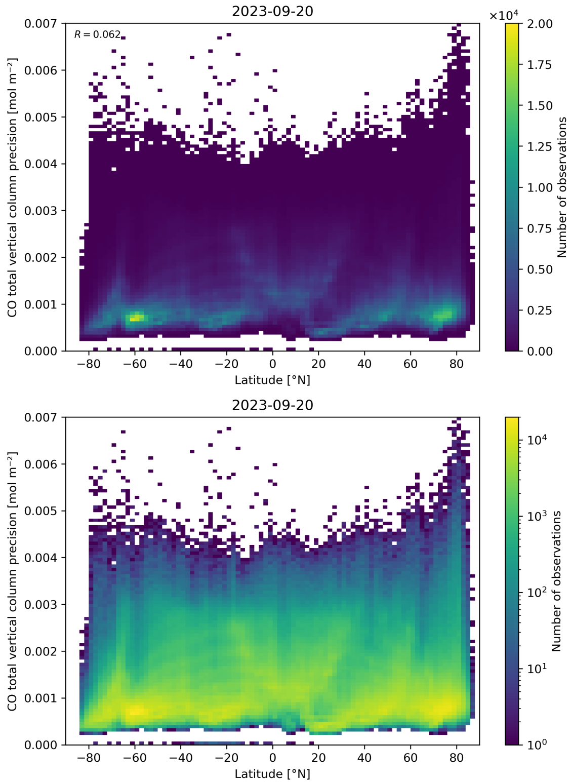
Figure 53: Scatter density plot of “Latitude” against “CO total vertical column precision” for 2023-09-20 to 2023-09-21.
