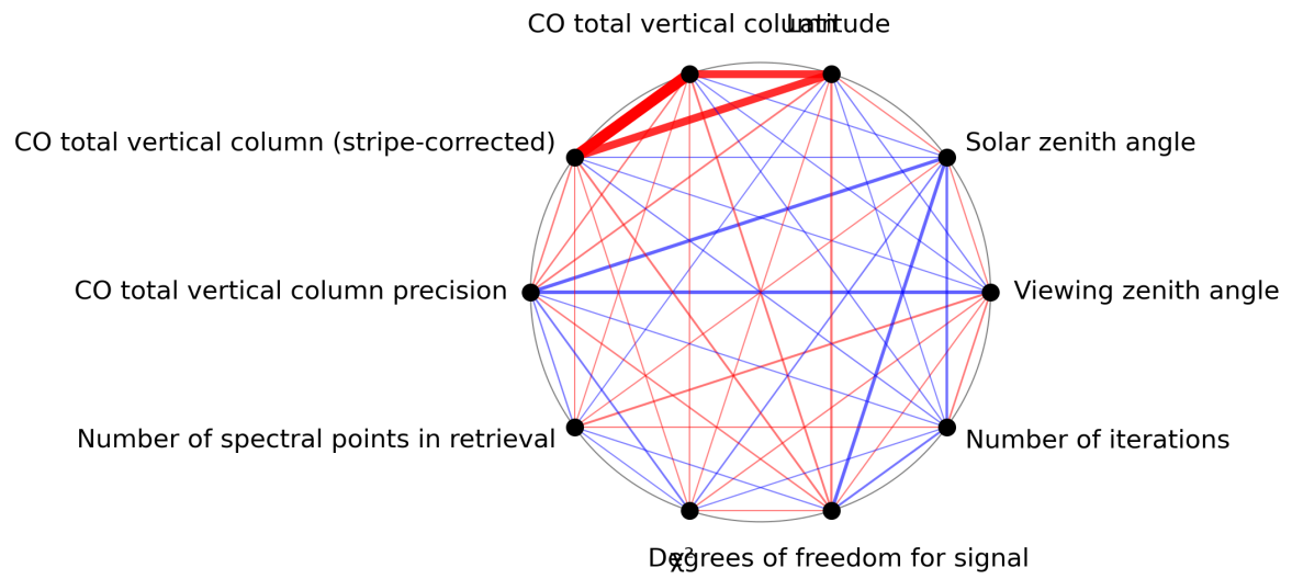
Figure 1: Map of correlation graph for 2023-09-20 to 2023-09-21.
