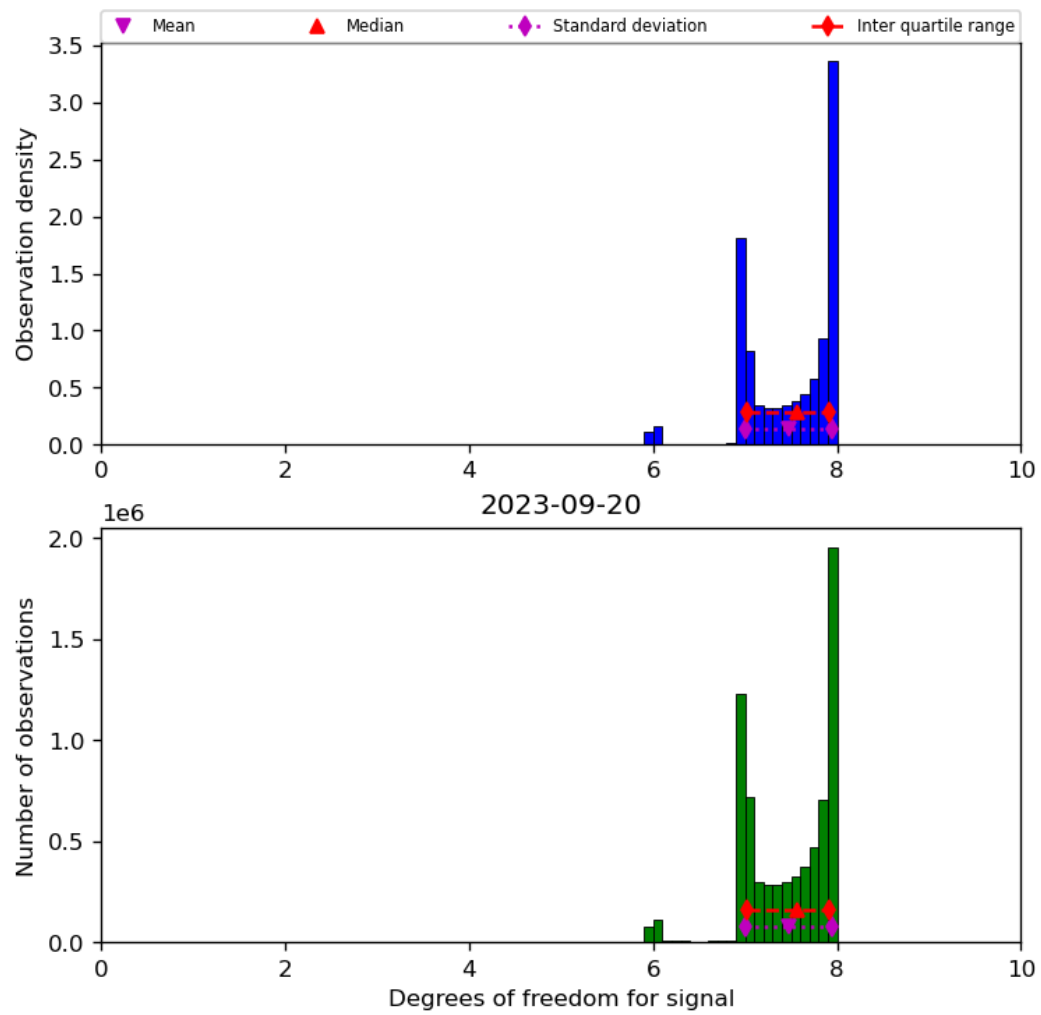
Figure 23: Histogram of “Degrees of freedom for signal” for 2023-09-20 to 2023-09-21
