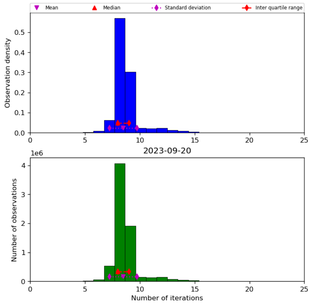
Figure 24: Histogram of “Number of iterations” for 2023-09-20 to 2023-09-21
