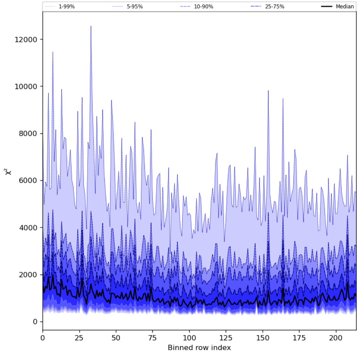
Figure 30: Along track statistics of “ \chi^2 ” for 2023-09-20 to 2023-09-21
