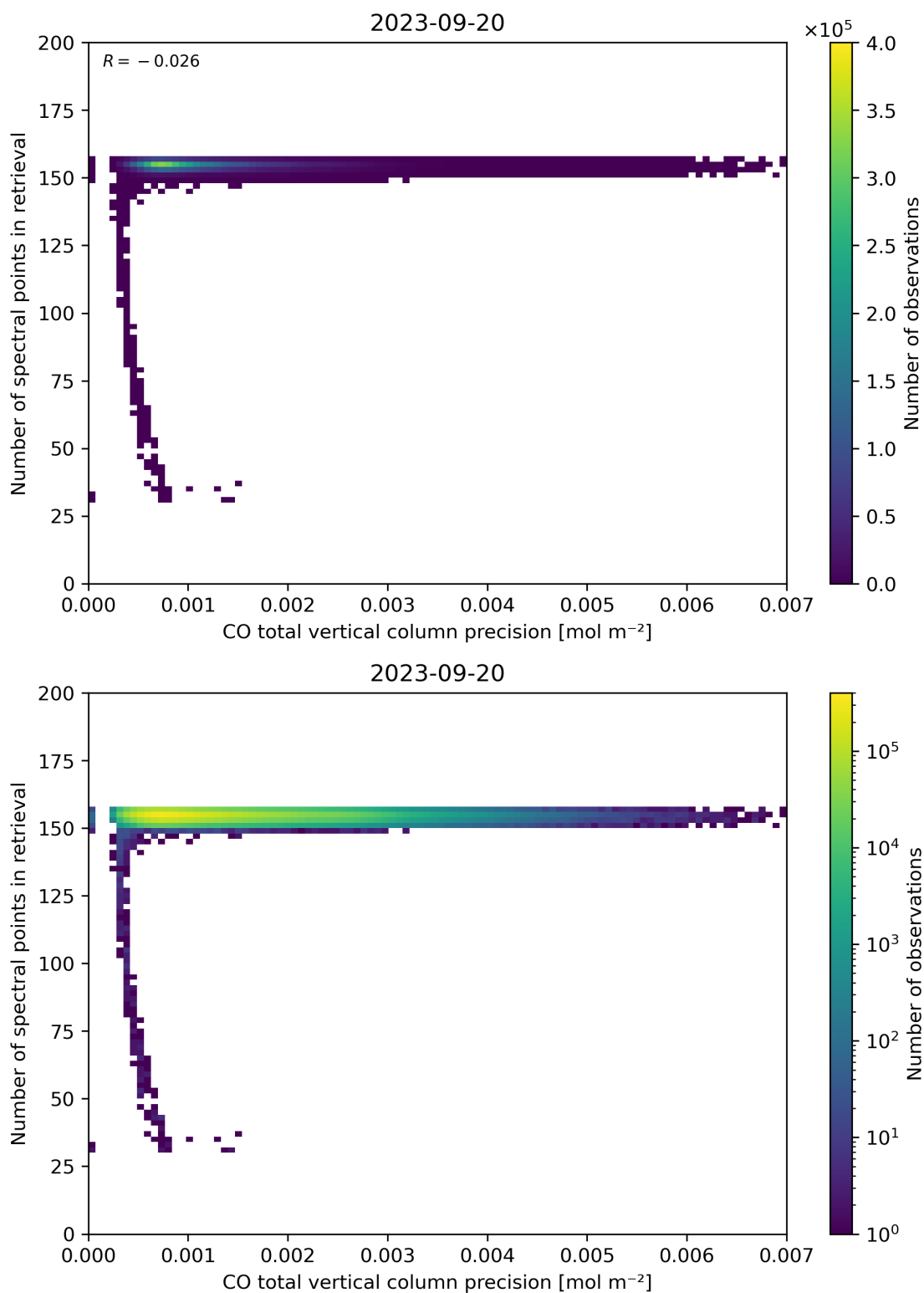
Figure 47: Scatter density plot of “CO total vertical column precision” against “Number of spectral points in retrieval” for 2023-09-20 to 2023-09-21.
