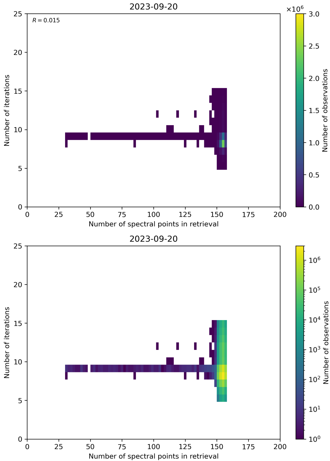
Figure 60: Scatter density plot of “Number of spectral points in retrieval” against “Number of iterations” for 2023-09-20 to 2023-09-21.
