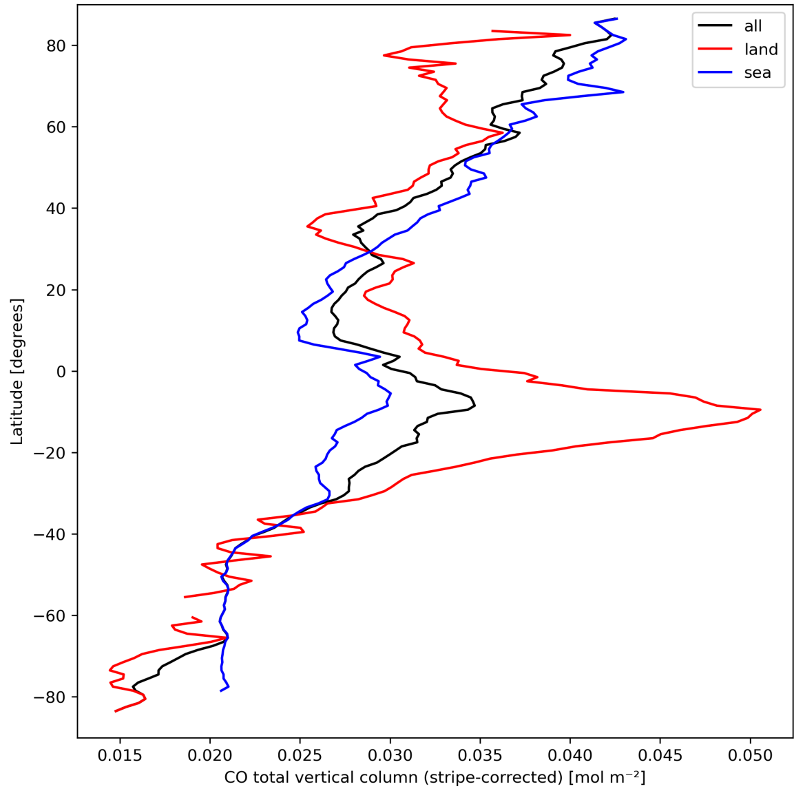
Figure 11: Zonal average of “CO total vertical column (stripe-corrected)” for 2023-09-20 to 2023-09-21.
