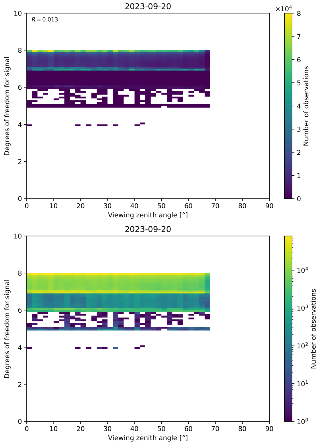
Figure 73: Scatter density plot of “Viewing zenith angle” against “Degrees of freedom for signal” for 2023-09-20 to 2023-09-21.
