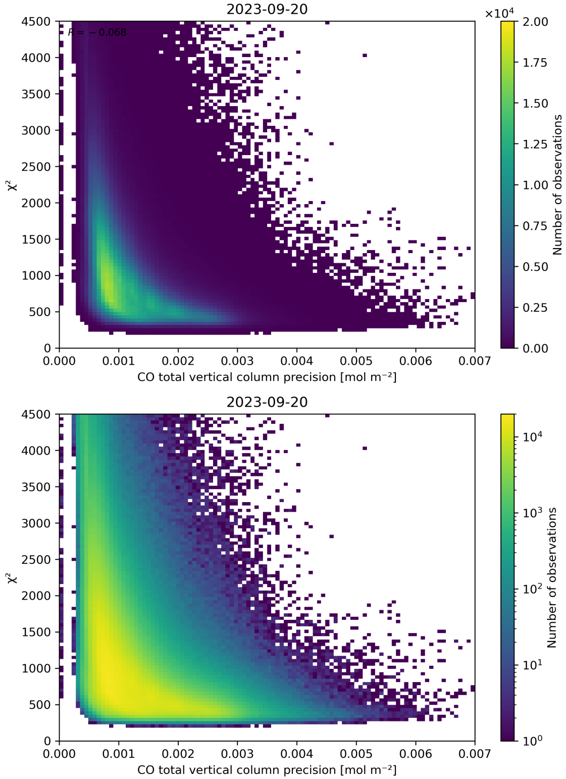
Figure 44: Scatter density plot of “CO total vertical column precision” against “ \chi^2 ” for 2023-09-20 to 2023-09-21.
