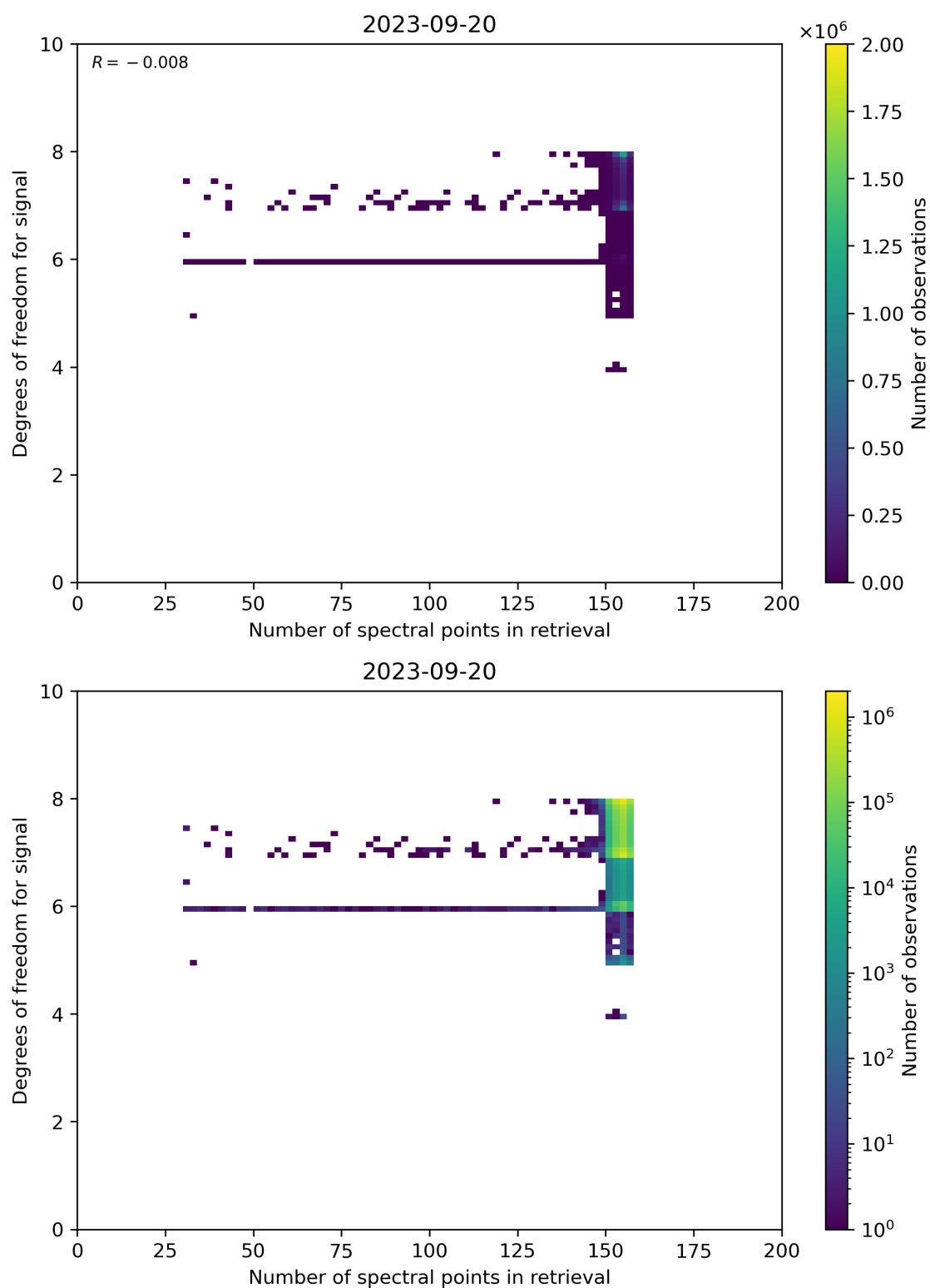
Figure 59: Scatter density plot of “Number of spectral points in retrieval” against “Degrees of freedom for signal” for 2023-09-20 to 2023-09-21.
