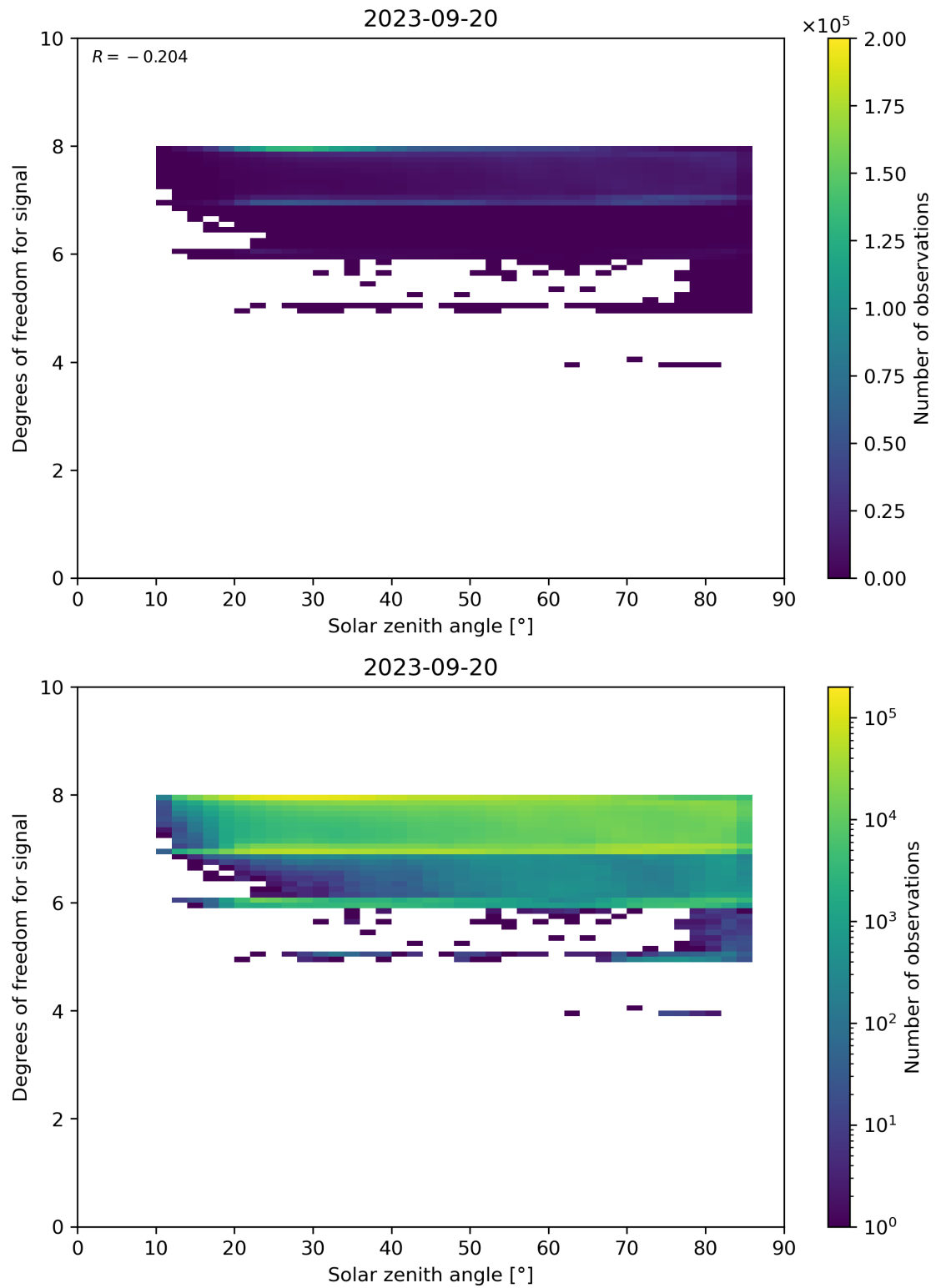
Figure 65: Scatter density plot of “Solar zenith angle” against “Degrees of freedom for signal” for 2023-09-20 to 2023-09-21.
