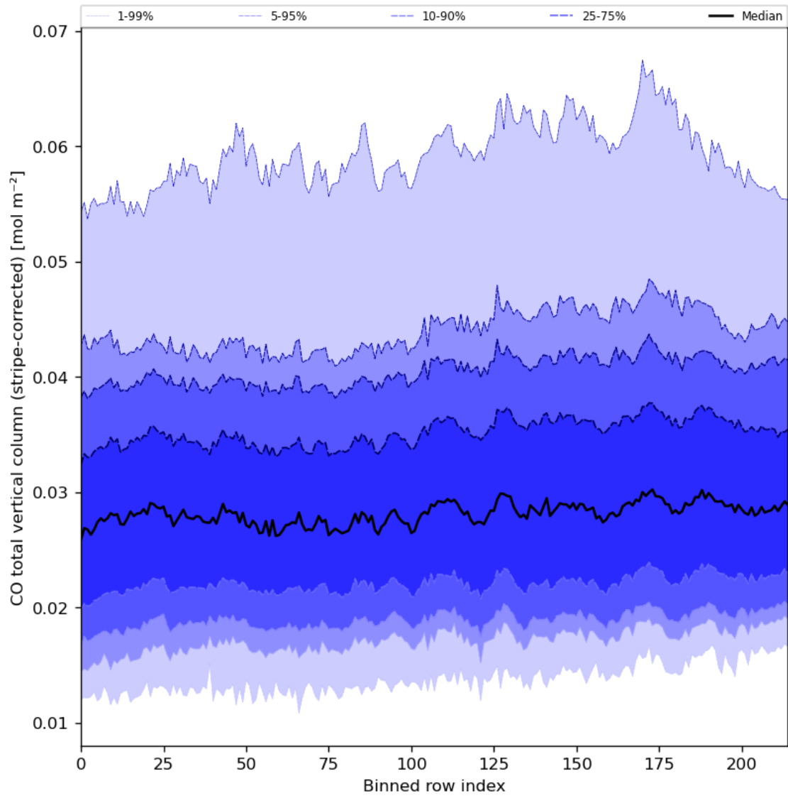
Figure 27: Along track statistics of “CO total vertical column (stripe-corrected)” for 2023-09-20 to 2023-09-21
