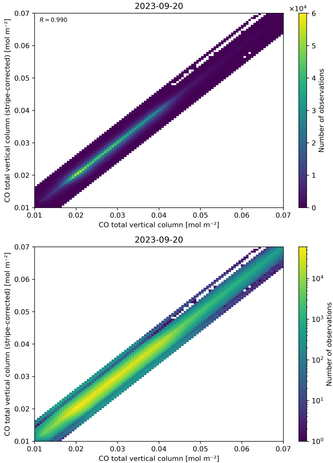
Figure 33: Scatter density plot of “CO total vertical column” against “CO total vertical column (stripe-corrected)” for 2023-09-20 to 2023-09-21.
