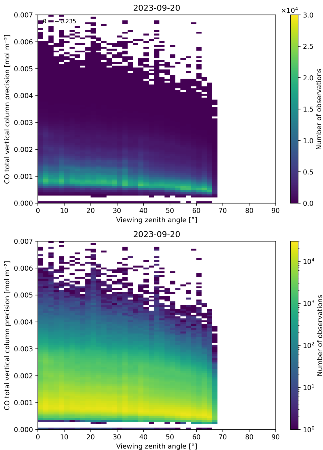
Figure 71: Scatter density plot of “Viewing zenith angle” against “CO total vertical column precision” for 2023-09-20 to 2023-09-21.
