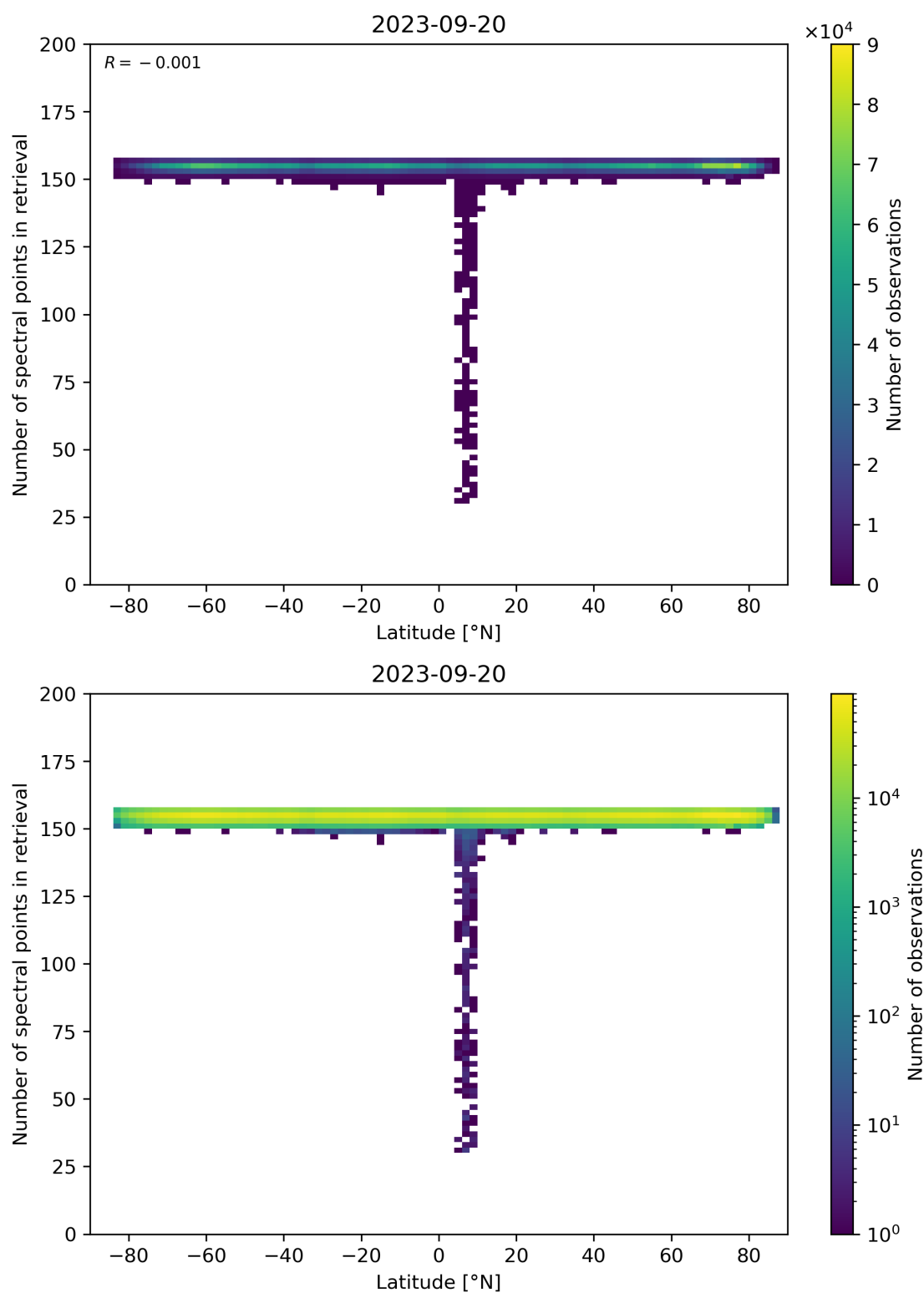
Figure 57: Scatter density plot of “Latitude” against “Number of spectral points in retrieval” for 2023-09-20 to 2023-09-21.
