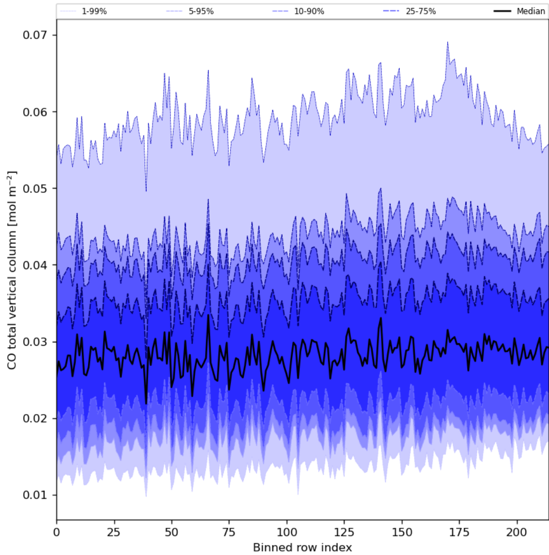
Figure 26: Along track statistics of “CO total vertical column” for 2023-09-20 to 2023-09-21
