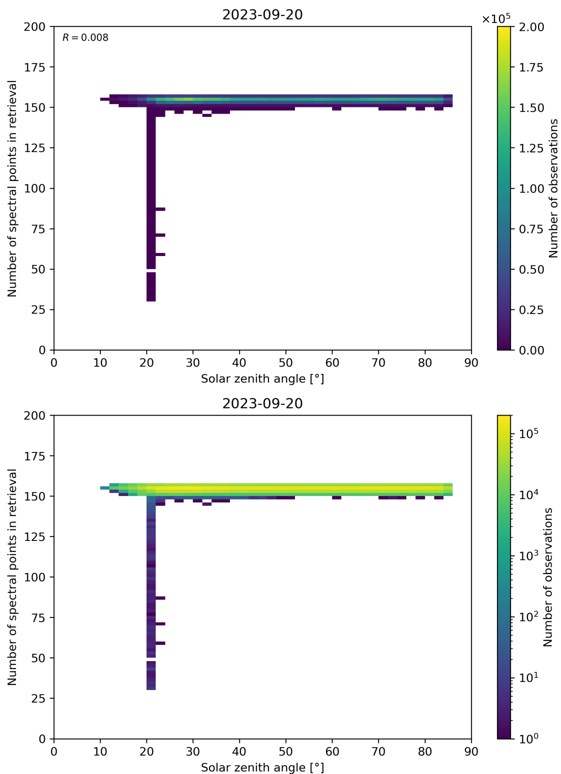
Figure 68: Scatter density plot of “Solar zenith angle” against “Number of spectral points in retrieval” for 2023-09-20 to 2023-09-21.
