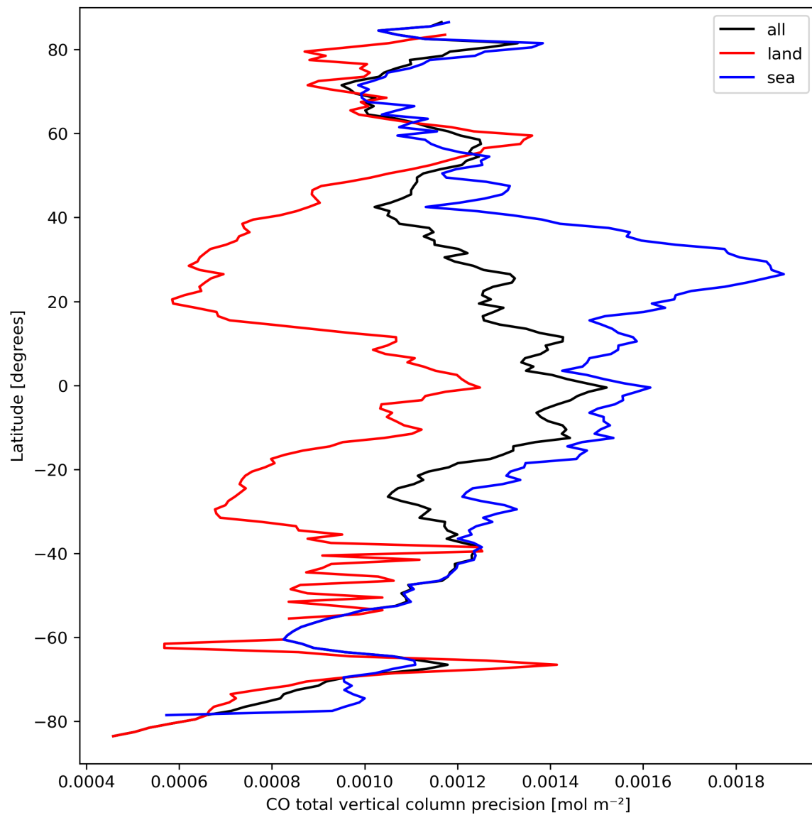
Figure 12: Zonal average of “CO total vertical column precision” for 2023-09-20 to 2023-09-21.
