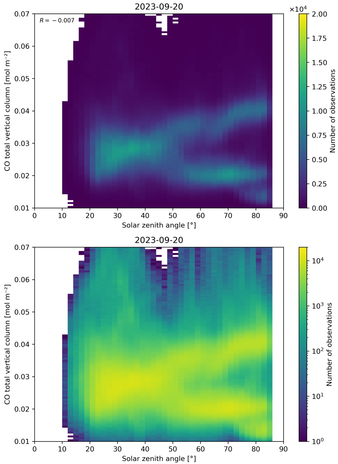
Figure 61: Scatter density plot of “Solar zenith angle” against “CO total vertical column” for 2023-09-20 to 2023-09-21.
