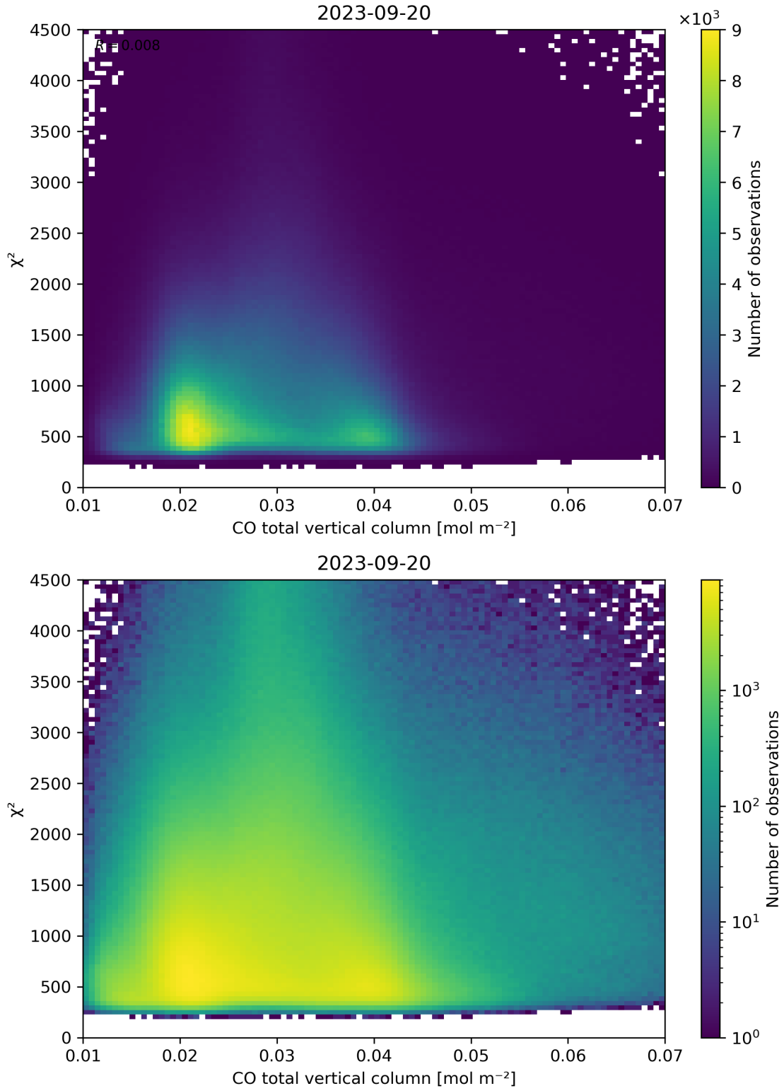
Figure 35: Scatter density plot of “CO total vertical column” against “ \chi^2 ” for 2023-09-20 to 2023-09-21.
