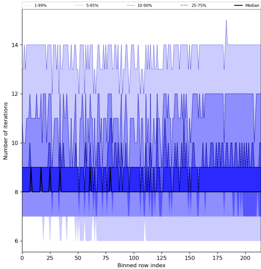
Figure 32: Along track statistics of “Number of iterations” for 2023-09-20 to 2023-09-21
