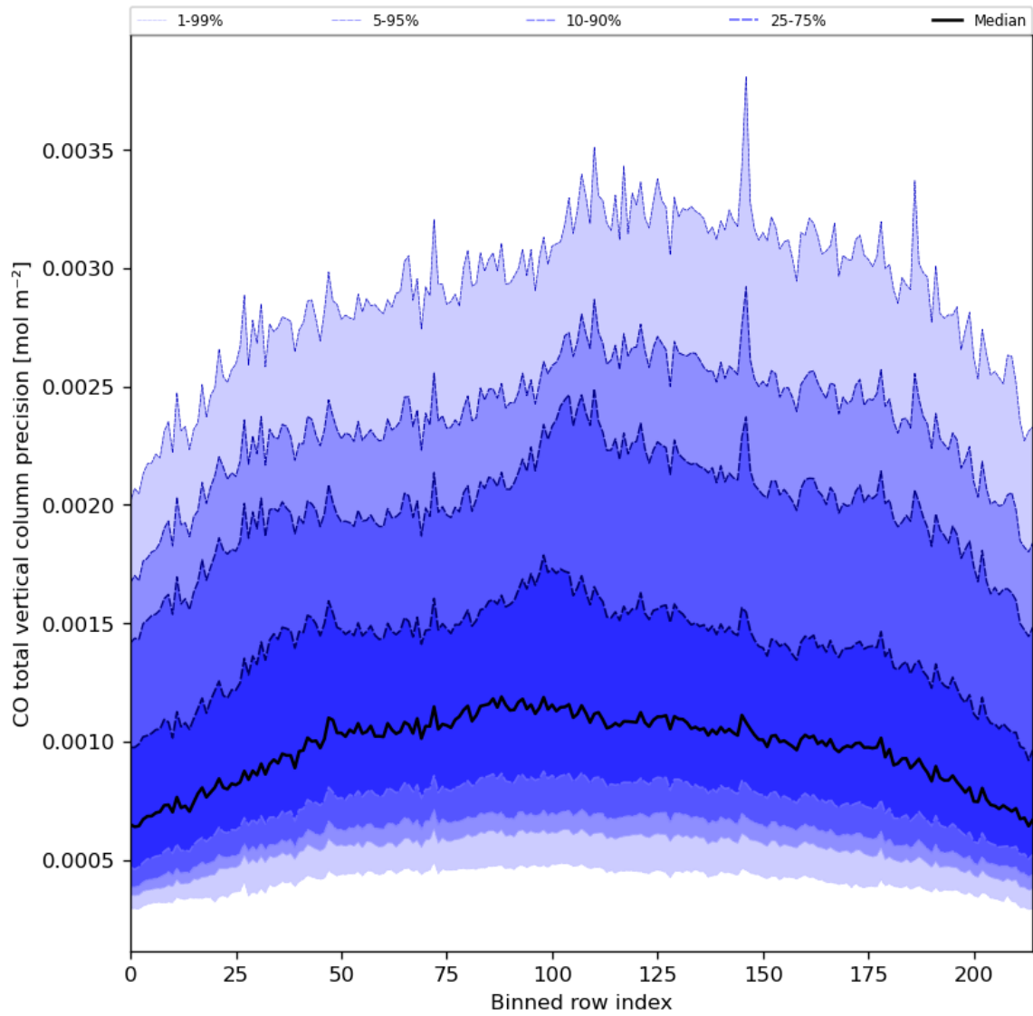
Figure 28: Along track statistics of “CO total vertical column precision” for 2023-09-20 to 2023-09-21
