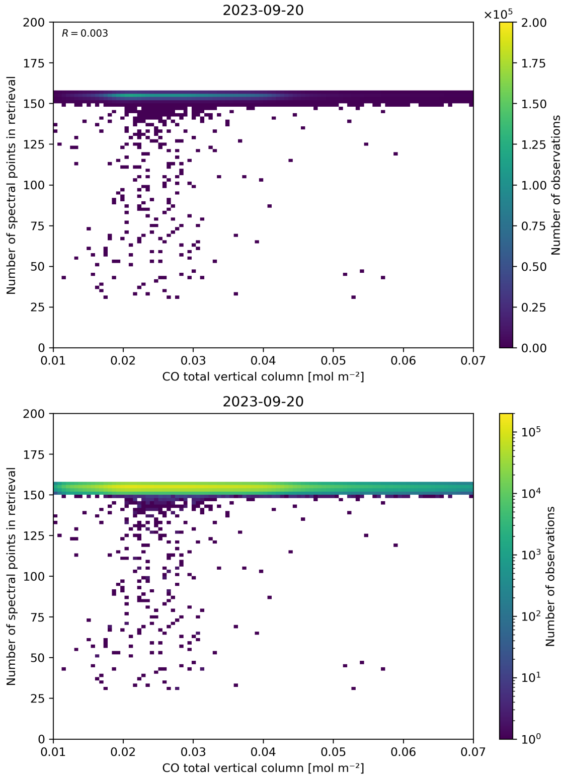
Figure 43: Scatter density plot of “CO total vertical column” against “Number of spectral points in retrieval” for 2023-09-20 to 2023-09-21.
