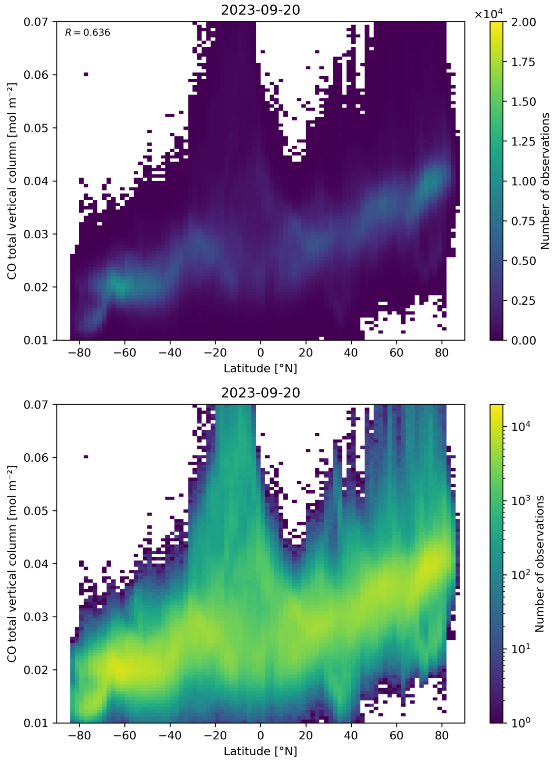
Figure 51: Scatter density plot of “Latitude” against “CO total vertical column” for 2023-09-20 to 2023-09-21.
