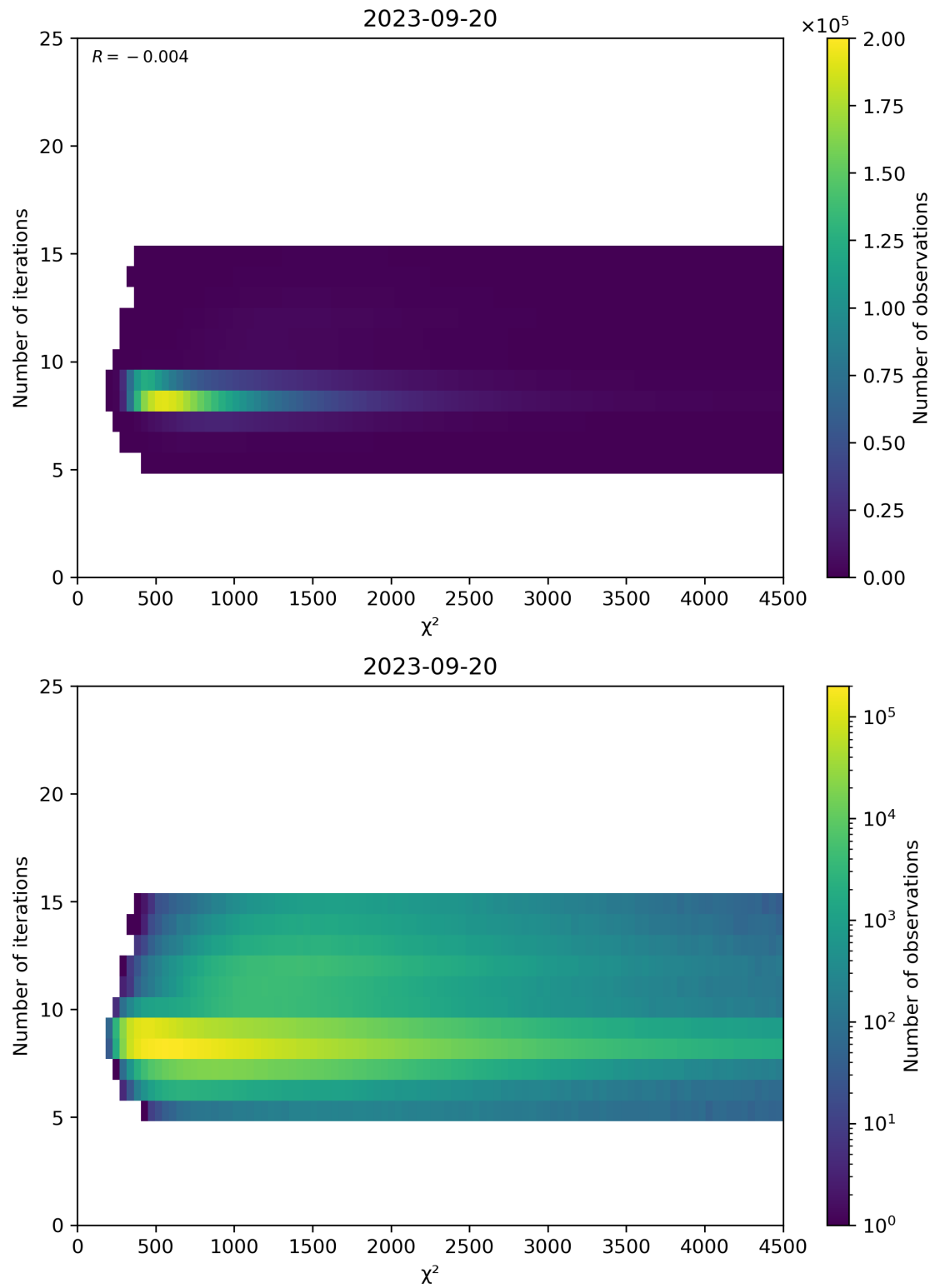
Figure 49: Scatter density plot of “ \chi^2 ” against “Number of iterations” for 2023-09-20 to 2023-09-21.
