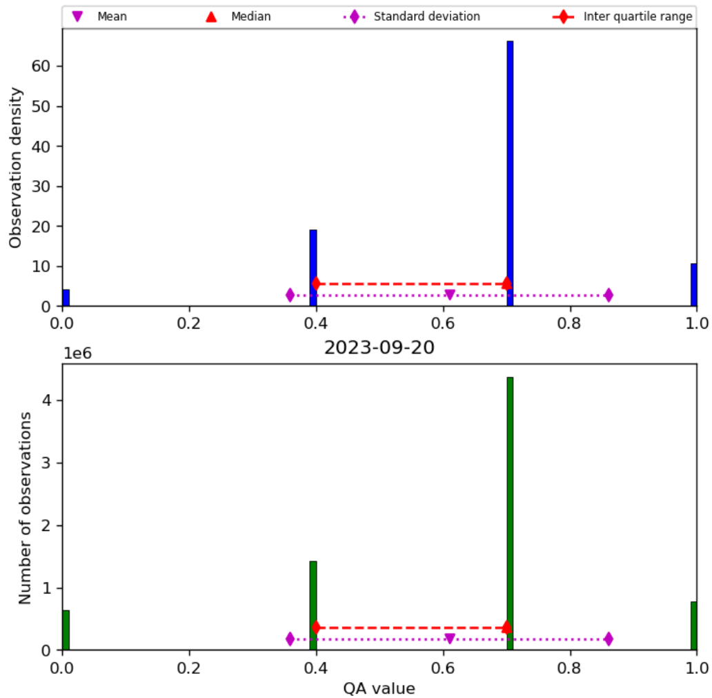
Figure 17: Histogram of “QA value” for 2023-09-20 to 2023-09-21
