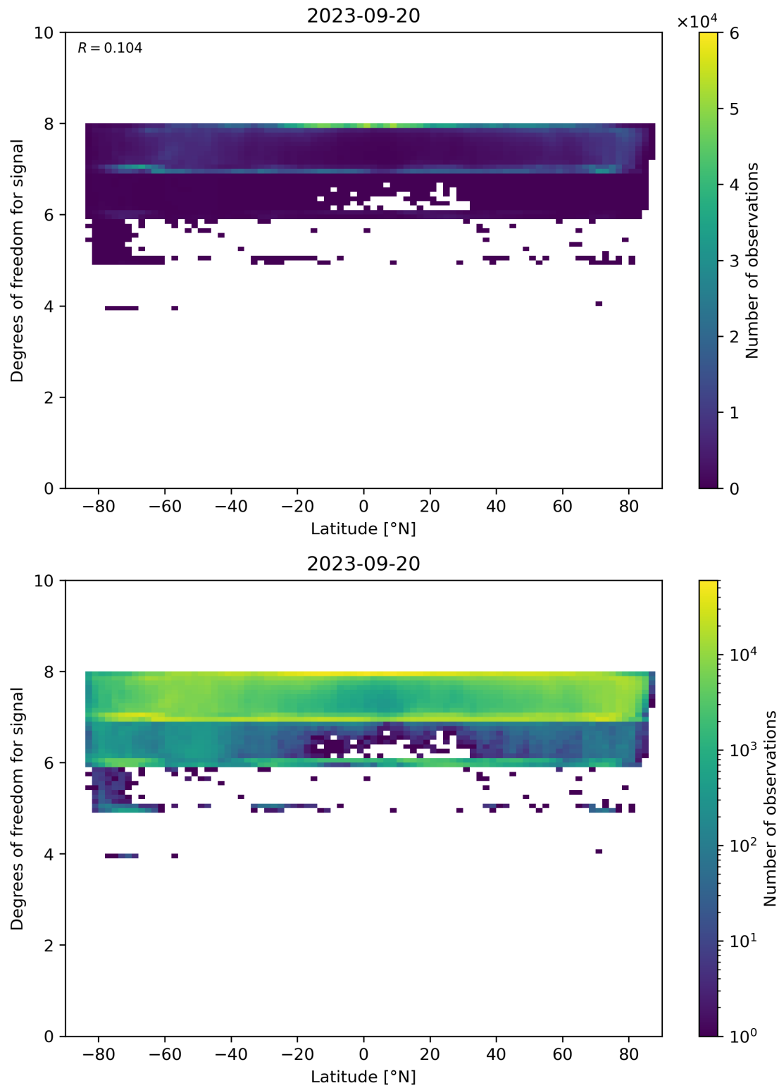
Figure 55: Scatter density plot of “Latitude” against “Degrees of freedom for signal” for 2023-09-20 to 2023-09-21.
