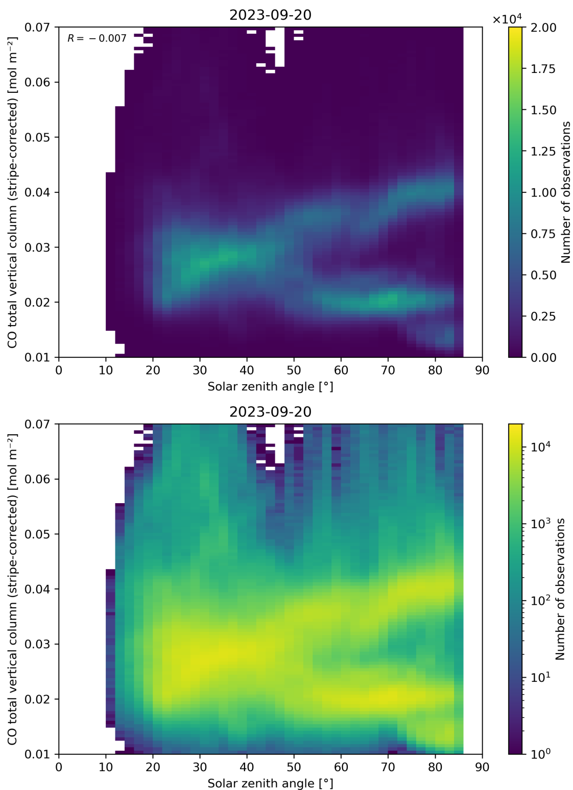
Figure 62: Scatter density plot of “Solar zenith angle” against “CO total vertical column (stripe-corrected)” for 2023-09-20 to 2023-09-21.
