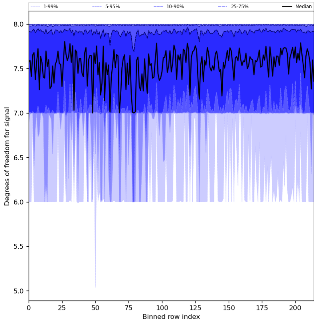
Figure 31: Along track statistics of “Degrees of freedom for signal” for 2023-09-20 to 2023-09-21
