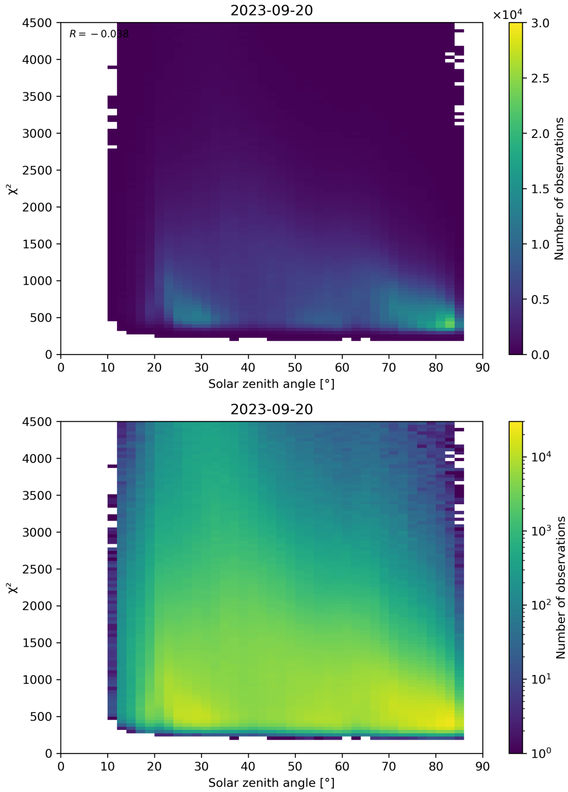
Figure 64: Scatter density plot of “Solar zenith angle” against “ \chi^2 ” for 2023-09-20 to 2023-09-21.
