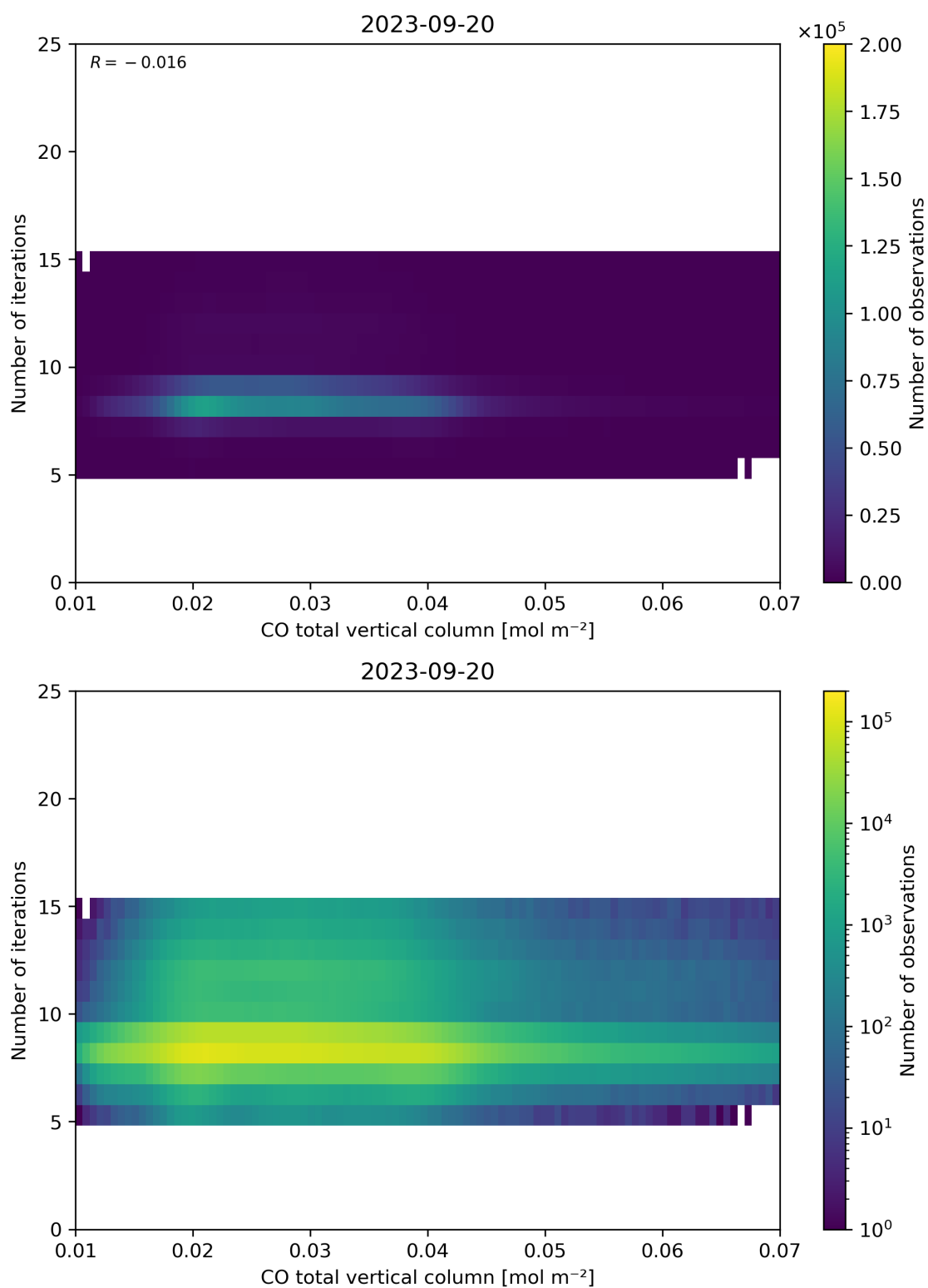
Figure 42: Scatter density plot of “CO total vertical column” against “Number of iterations” for 2023-09-20 to 2023-09-21.
