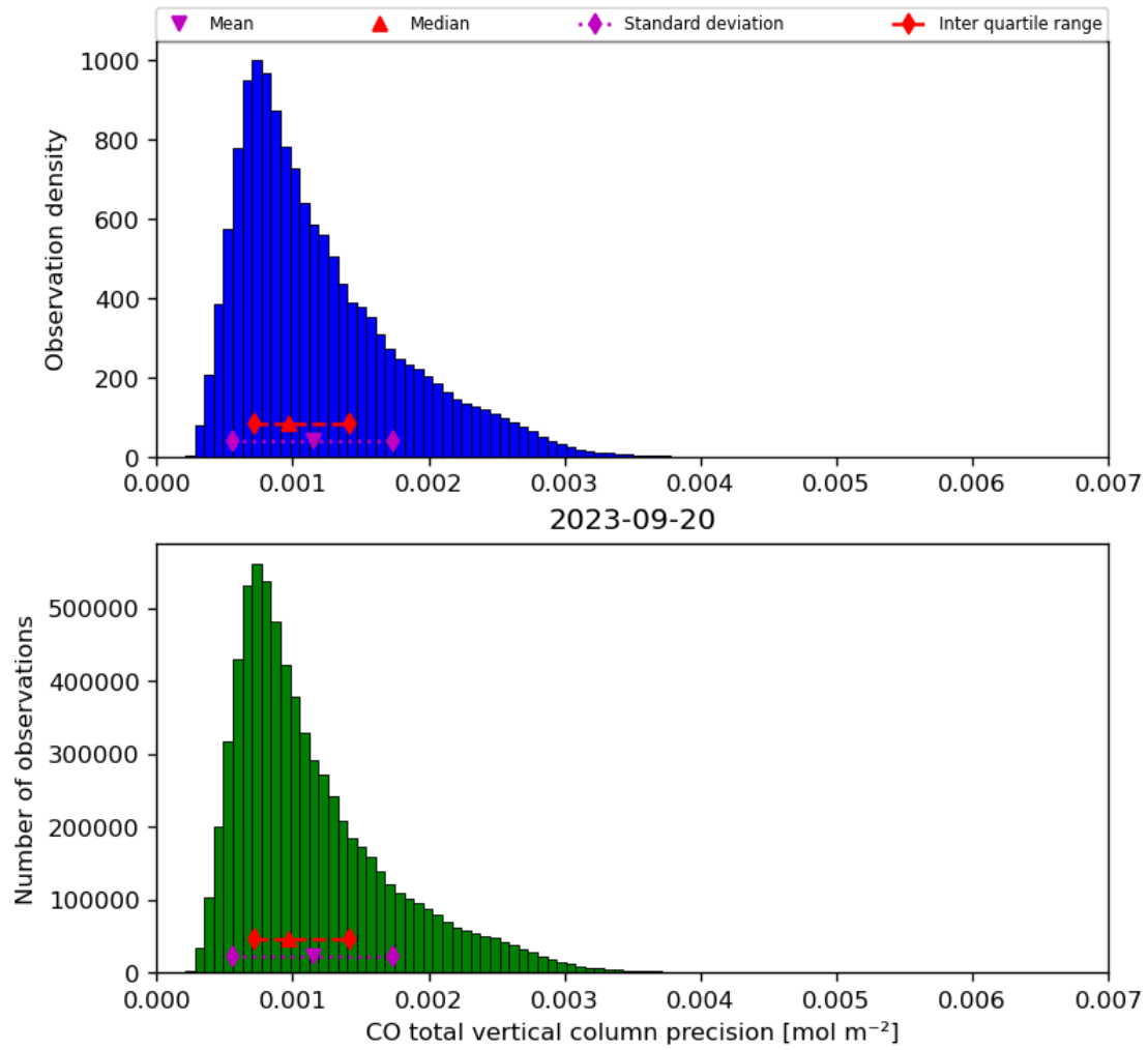
Figure 20: Histogram of “CO total vertical column precision” for 2023-09-20 to 2023-09-21
