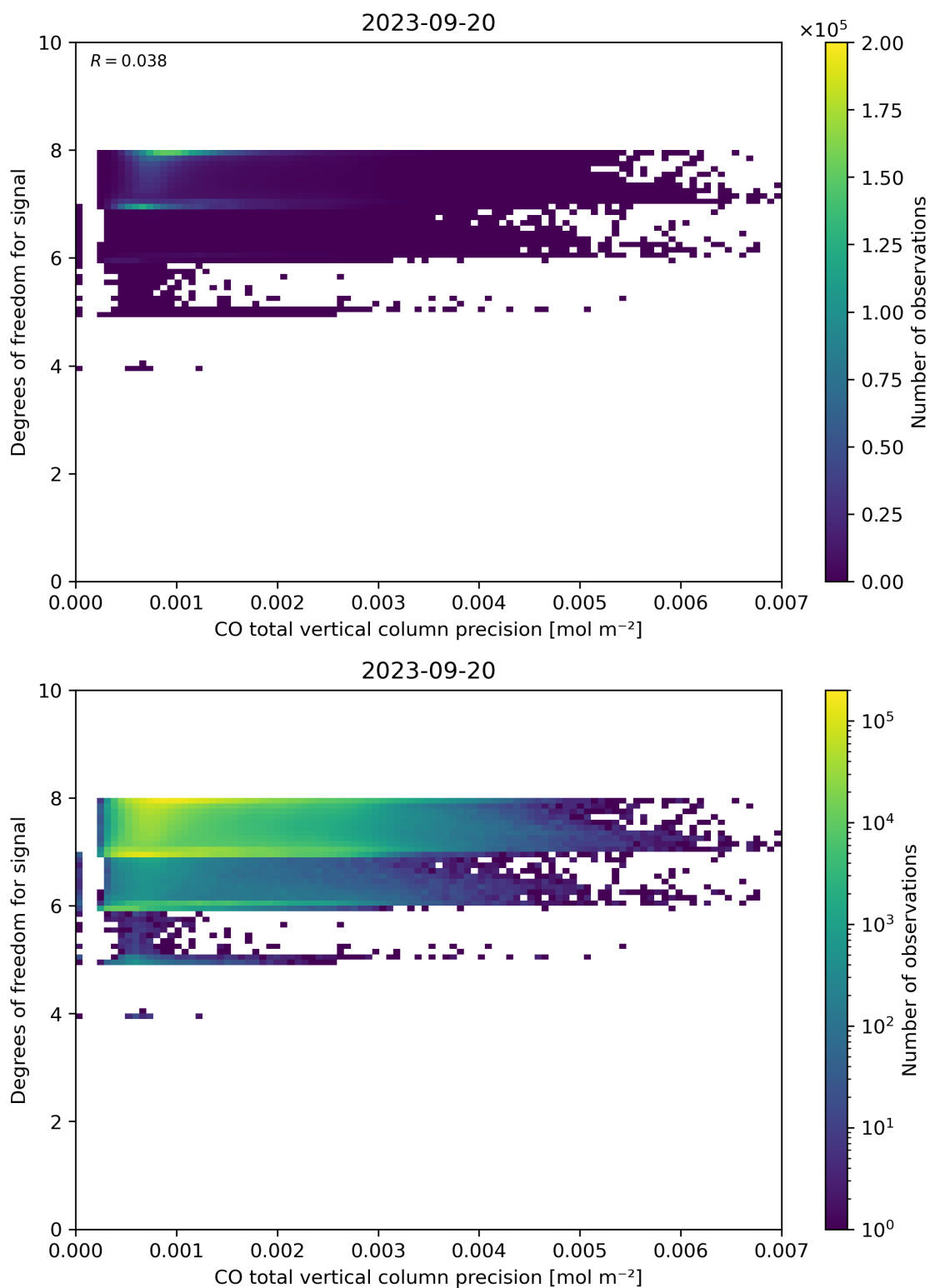
Figure 45: Scatter density plot of “CO total vertical column precision” against “Degrees of freedom for signal” for 2023-09-20 to 2023-09-21.
