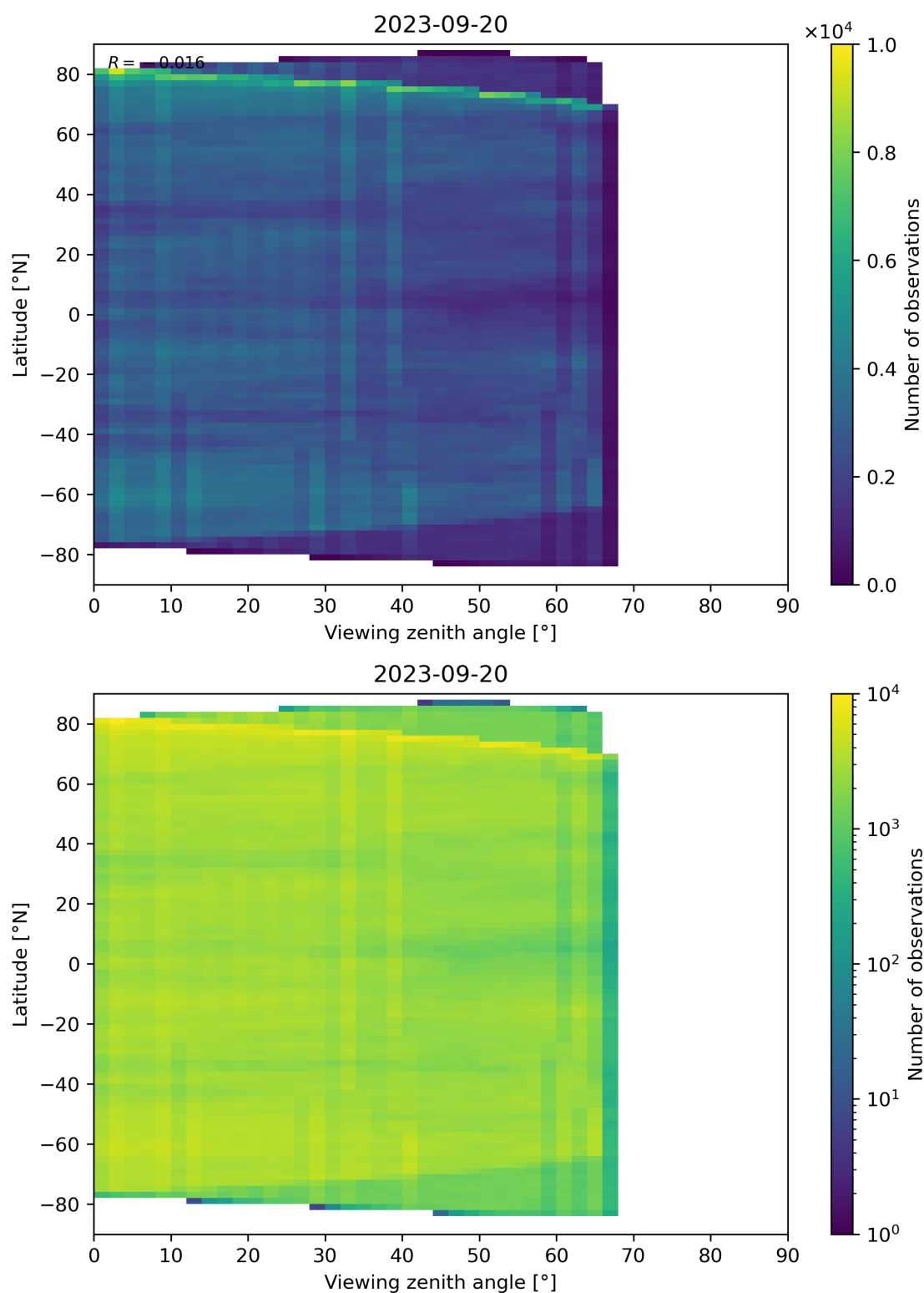
Figure 74: Scatter density plot of “Viewing zenith angle” against “Latitude” for 2023-09-20 to 2023-09-21.
