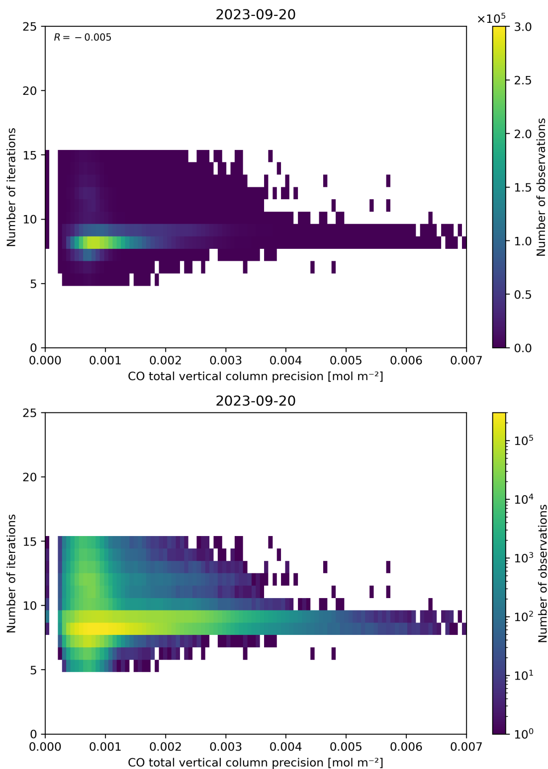
Figure 46: Scatter density plot of “CO total vertical column precision” against “Number of iterations” for 2023-09-20 to 2023-09-21.
