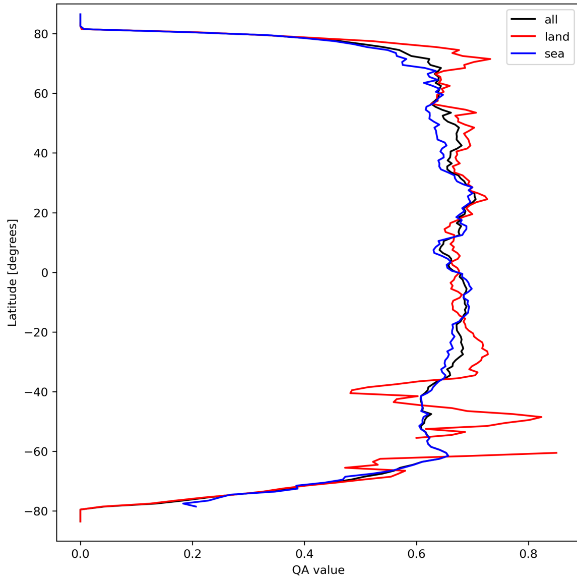
Figure 9: Zonal average of “QA value” for 2023-09-20 to 2023-09-21.
