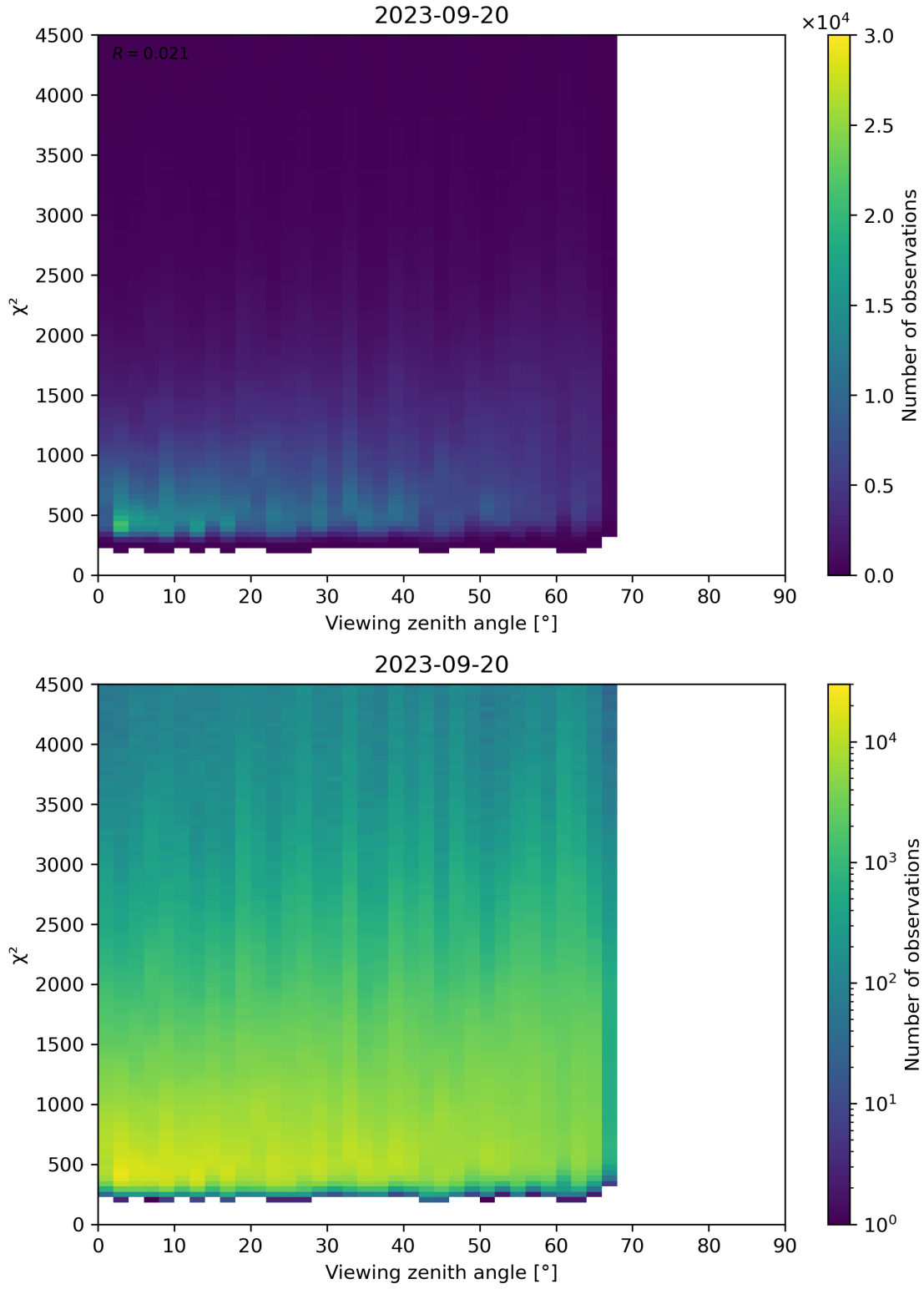
Figure 72: Scatter density plot of “Viewing zenith angle” against “ \chi^2 ” for 2023-09-20 to 2023-09-21.
