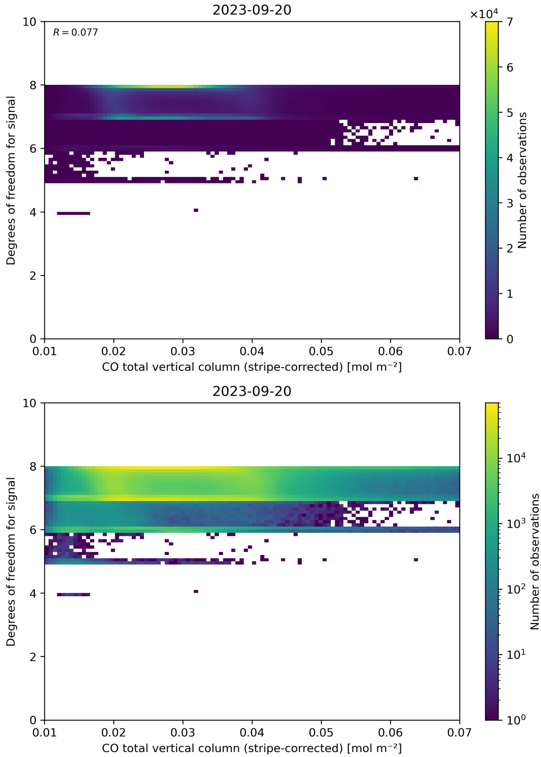
Figure 38: Scatter density plot of “CO total vertical column (stripe-corrected)” against “Degrees of freedom for signal” for 2023-09-20 to 2023-09-21.
