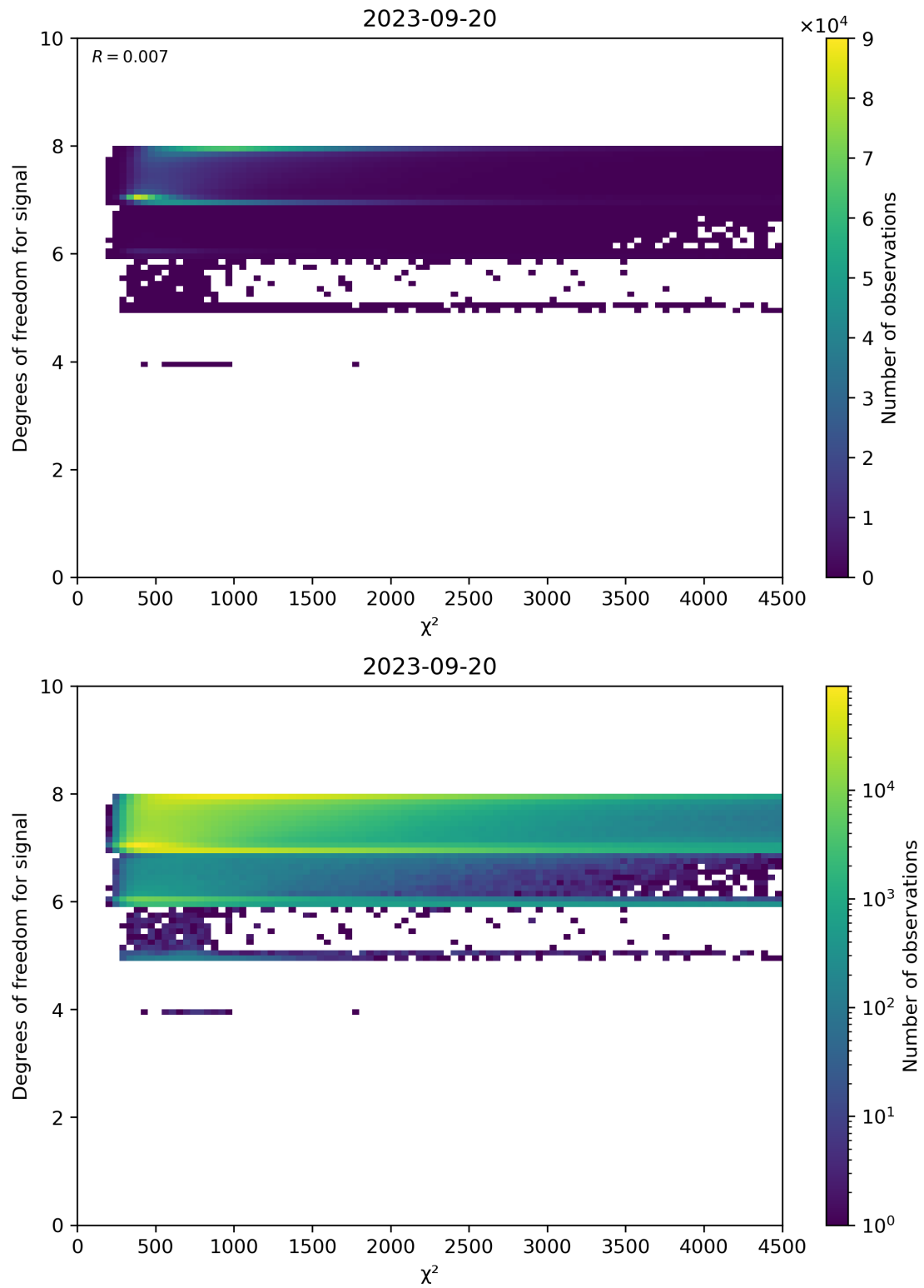
Figure 48: Scatter density plot of “ \chi^2 ” against “Degrees of freedom for signal” for 2023-09-20 to 2023-09-21.
