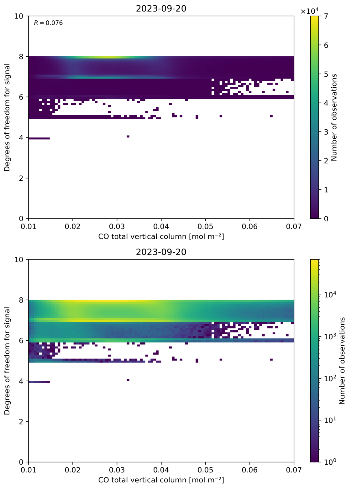
Figure 41: Scatter density plot of “CO total vertical column” against “Degrees of freedom for signal” for 2023-09-20 to 2023-09-21.
