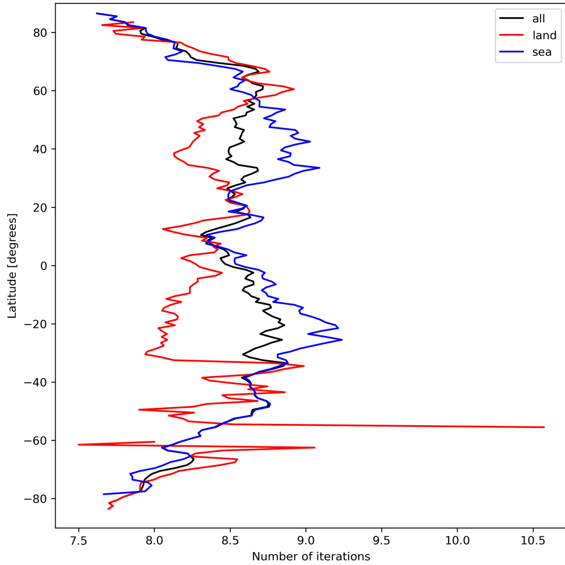
Figure 16: Zonal average of “Number of iterations” for 2023-09-20 to 2023-09-21.
