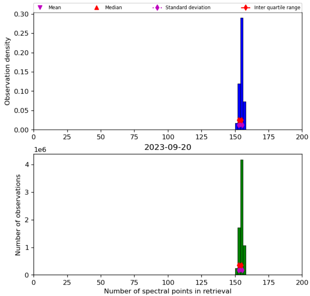
Figure 21: Histogram of “Number of spectral points in retrieval” for 2023-09-20 to 2023-09-21
