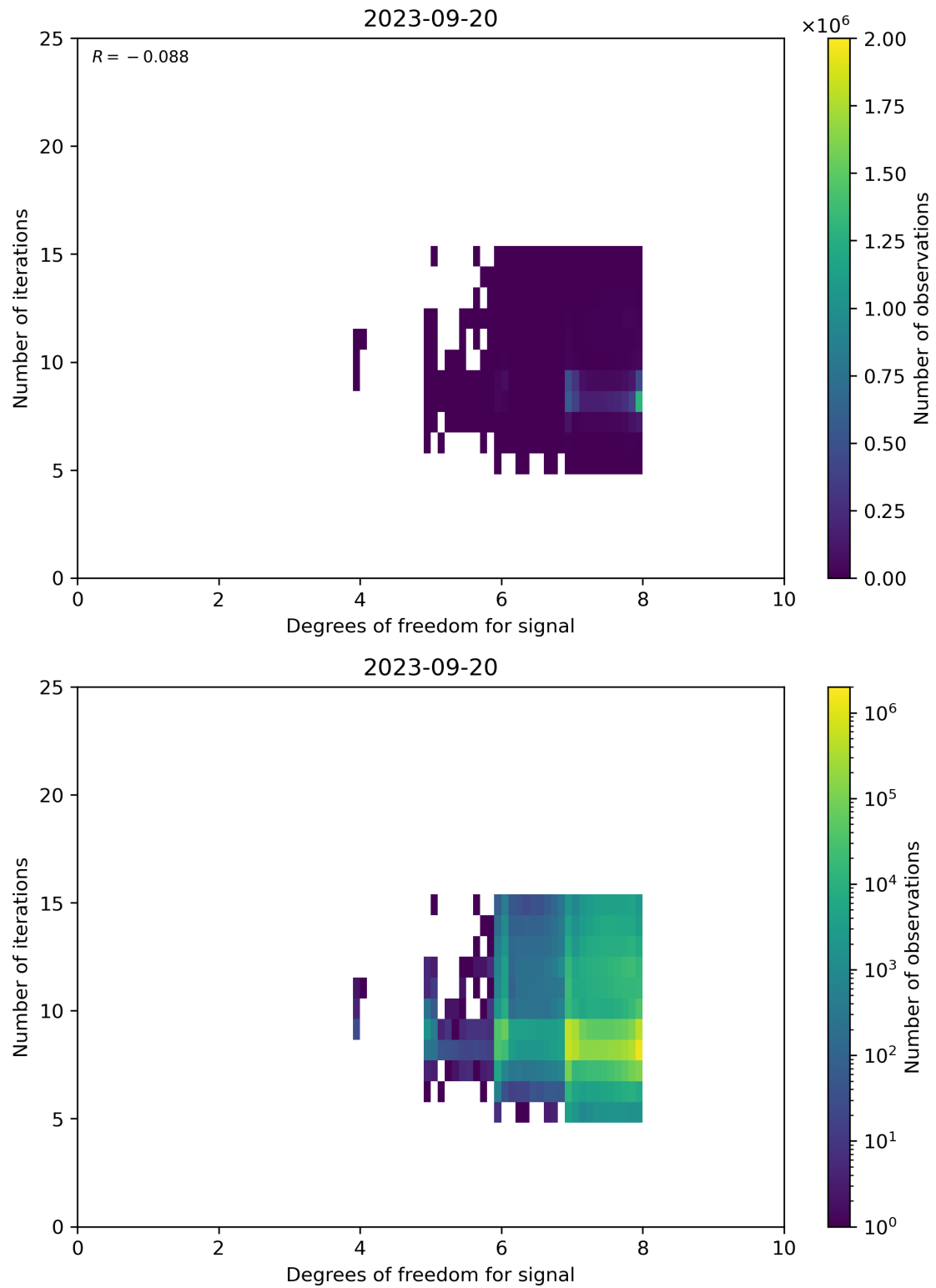
Figure 50: Scatter density plot of “Degrees of freedom for signal” against “Number of iterations” for 2023-09-20 to 2023-09-21.
