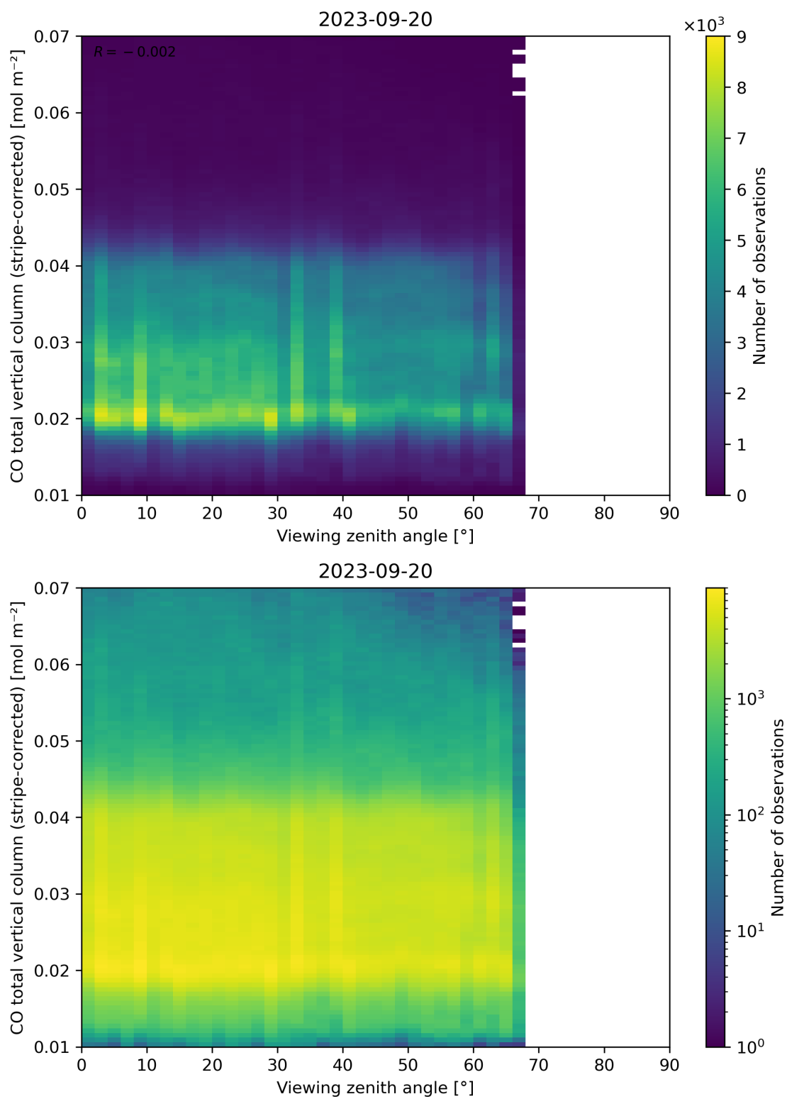
Figure 70: Scatter density plot of “Viewing zenith angle” against “CO total vertical column (stripe-corrected)” for 2023-09-20 to 2023-09-21.
