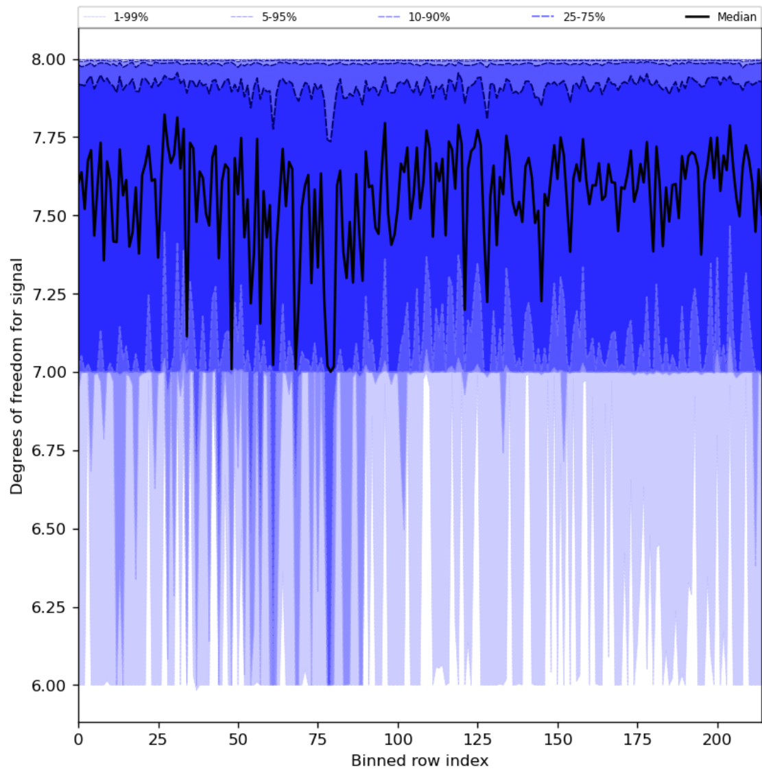
Figure 31: Along track statistics of “Degrees of freedom for signal” for 2023-09-20 to 2023-09-22
