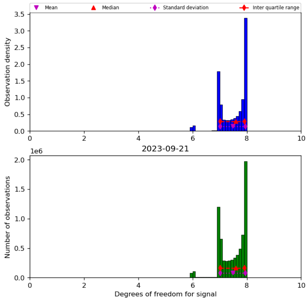
Figure 23: Histogram of “Degrees of freedom for signal” for 2023-09-20 to 2023-09-22
