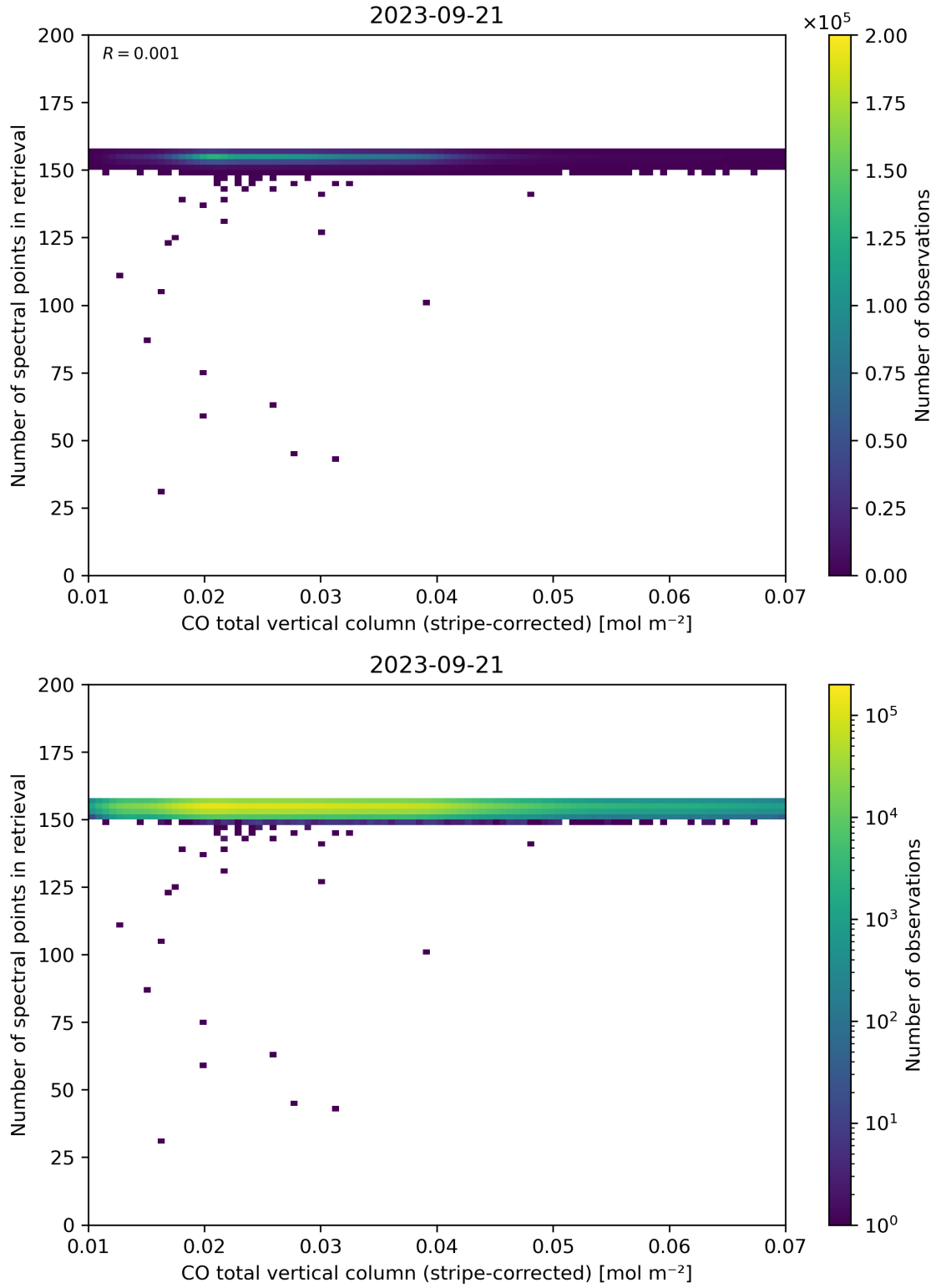
Figure 40: Scatter density plot of “CO total vertical column (stripe-corrected)” against “Number of spectral points in retrieval” for 2023-09-20 to 2023-09-22.
