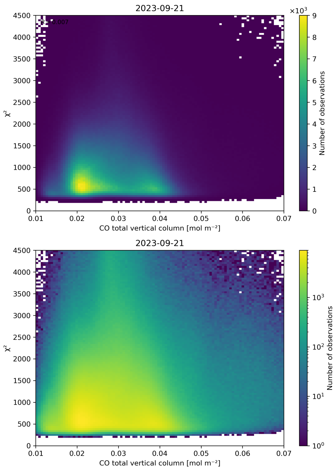
Figure 35: Scatter density plot of “CO total vertical column” against “ \chi^2 ” for 2023-09-20 to 2023-09-22.
