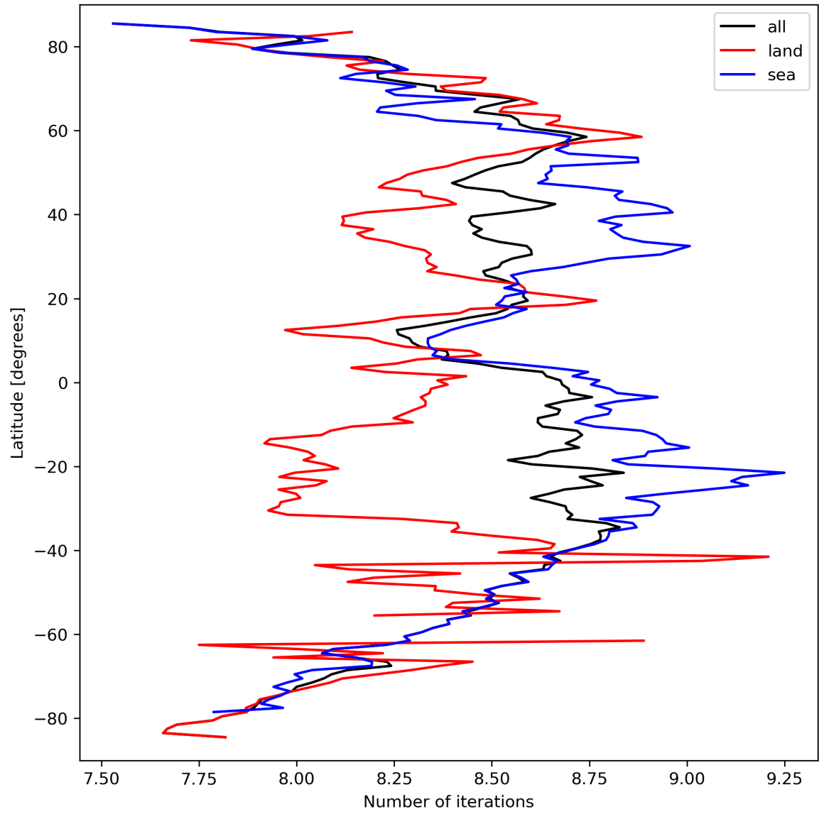
Figure 16: Zonal average of “Number of iterations” for 2023-09-20 to 2023-09-22.
