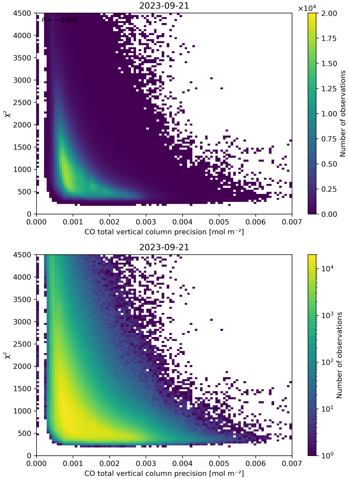
Figure 44: Scatter density plot of “CO total vertical column precision” against “ \chi^2 ” for 2023-09-20 to 2023-09-22.
