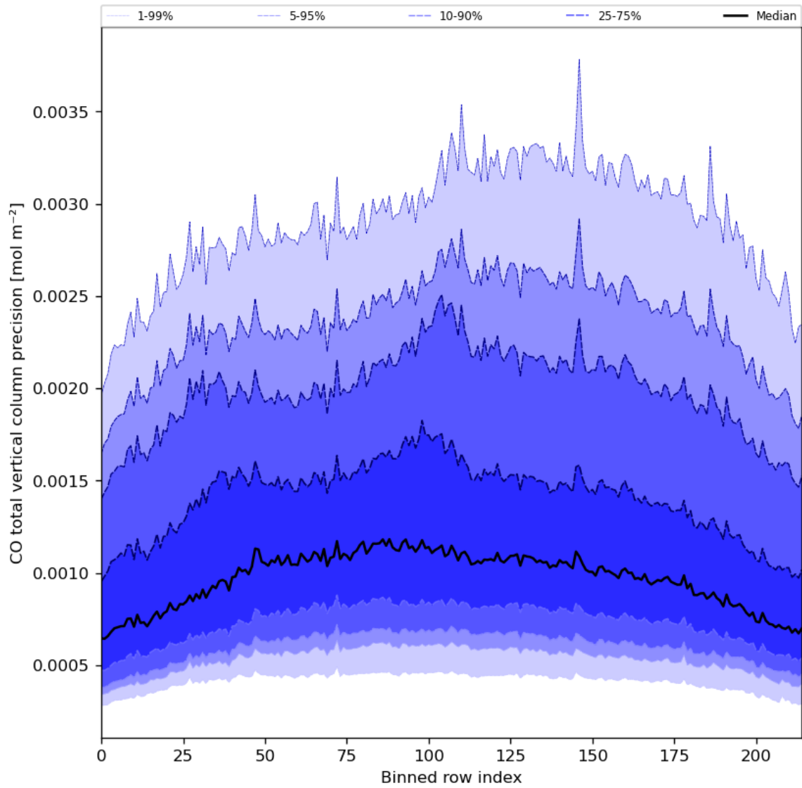
Figure 28: Along track statistics of “CO total vertical column precision” for 2023-09-20 to 2023-09-22
