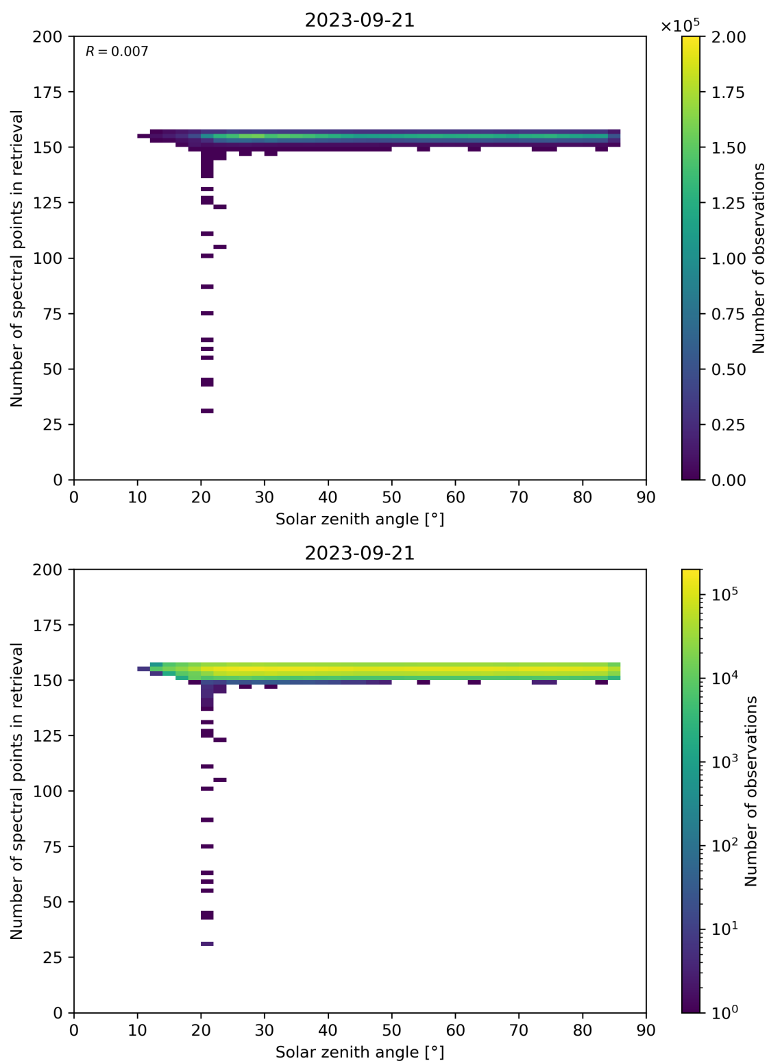
Figure 68: Scatter density plot of “Solar zenith angle” against “Number of spectral points in retrieval” for 2023-09-20 to 2023-09-22.
