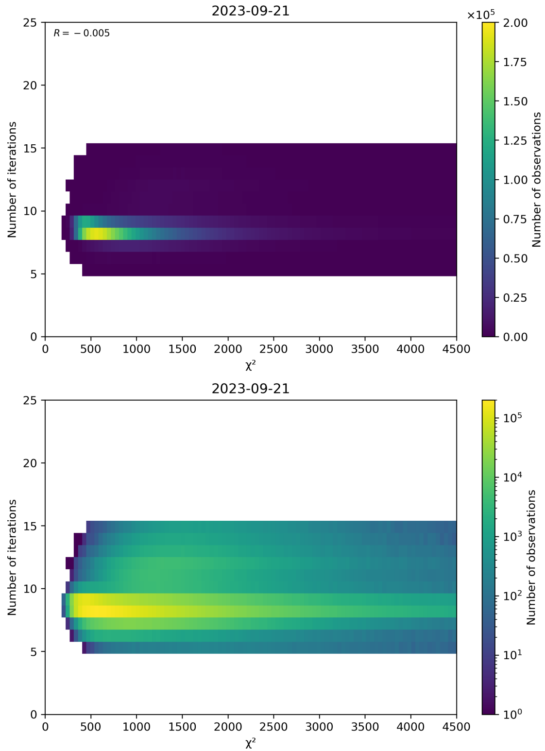
Figure 49: Scatter density plot of “ \chi^2 ” against “Number of iterations” for 2023-09-20 to 2023-09-22.
