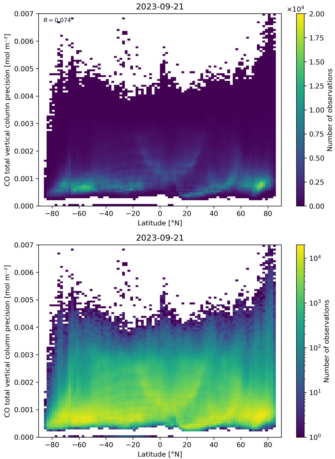
Figure 53: Scatter density plot of “Latitude” against “CO total vertical column precision” for 2023-09-20 to 2023-09-22.
