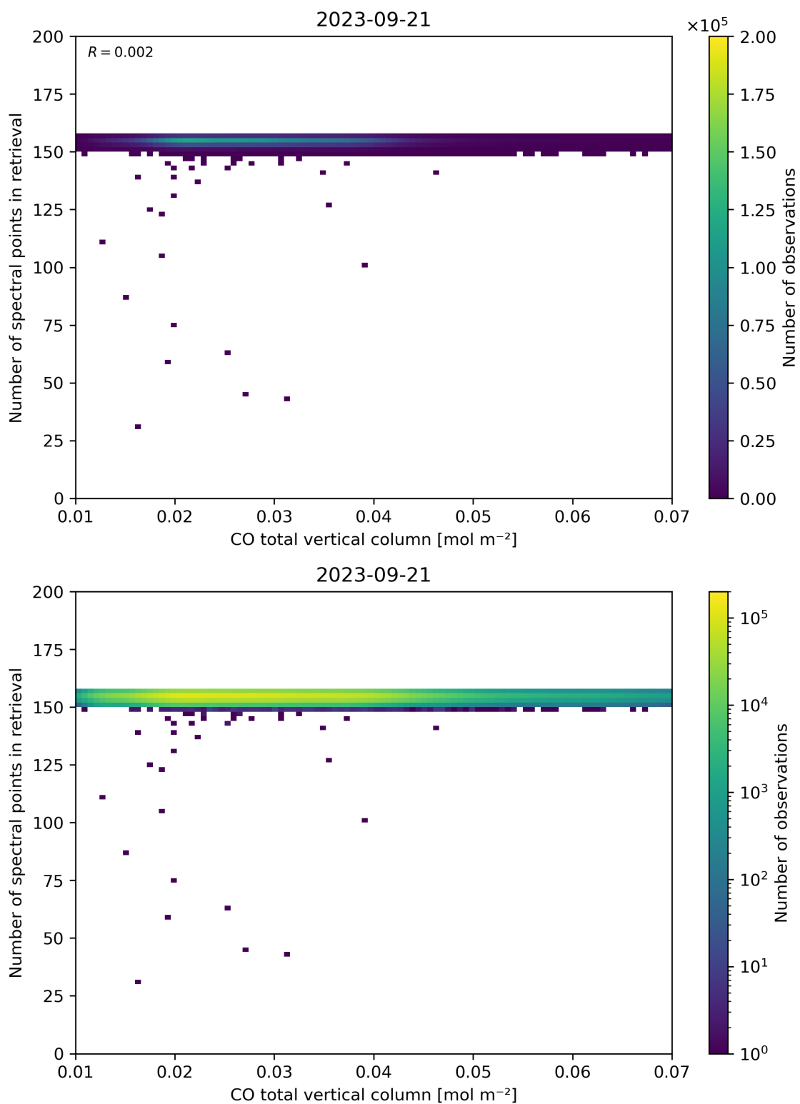
Figure 43: Scatter density plot of “CO total vertical column” against “Number of spectral points in retrieval” for 2023-09-20 to 2023-09-22.
