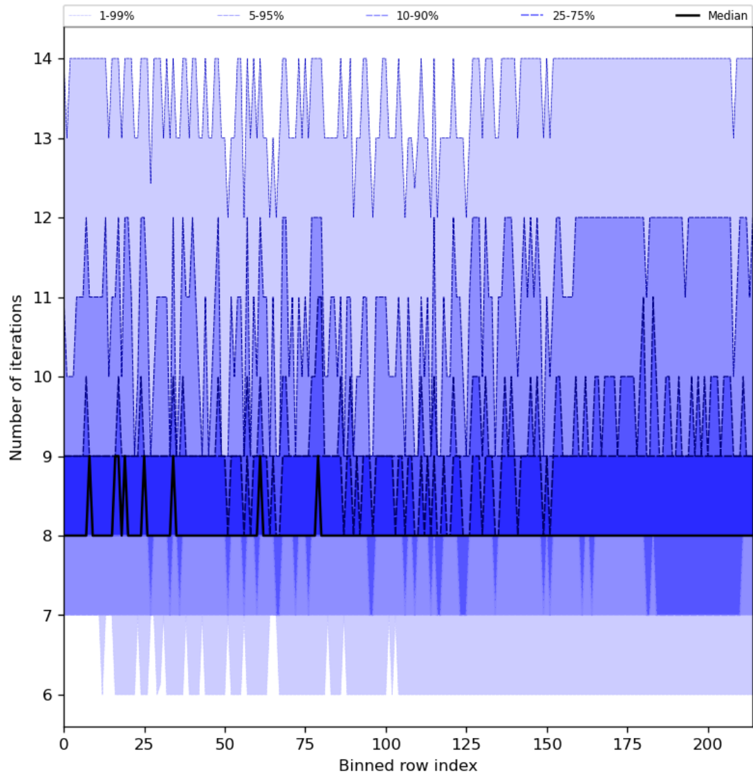
Figure 32: Along track statistics of “Number of iterations” for 2023-09-20 to 2023-09-22
