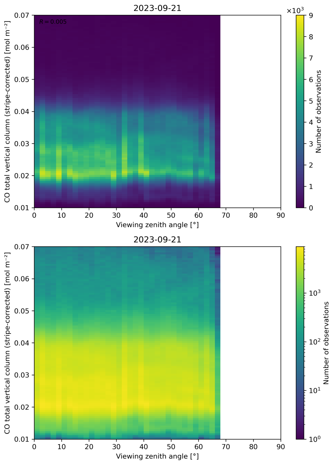
Figure 70: Scatter density plot of “Viewing zenith angle” against “CO total vertical column (stripe-corrected)” for 2023-09-20 to 2023-09-22.
