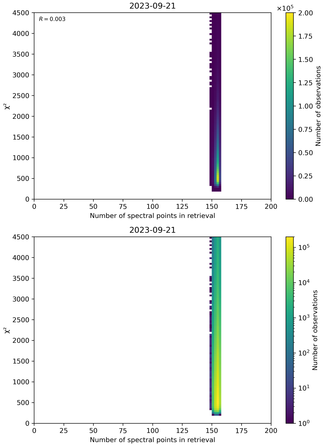
Figure 58: Scatter density plot of “Number of spectral points in retrieval” against “ \chi^2 ” for 2023-09-20 to 2023-09-22.
