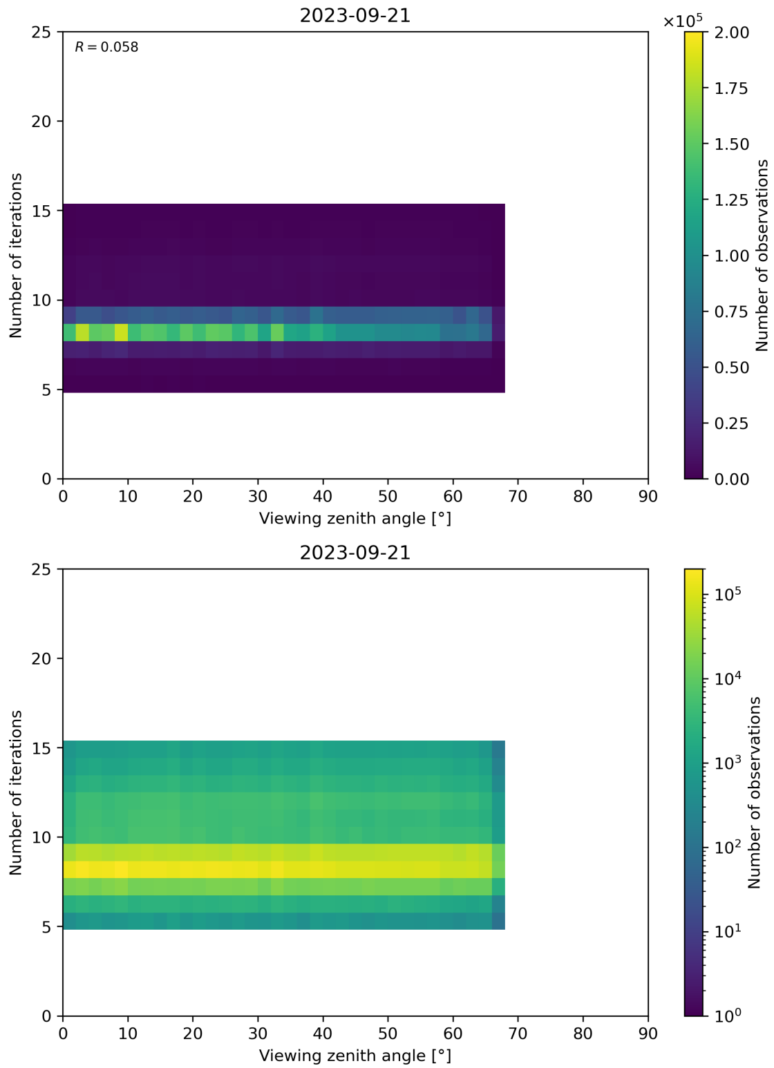
Figure 75: Scatter density plot of “Viewing zenith angle” against “Number of iterations” for 2023-09-20 to 2023-09-22.
