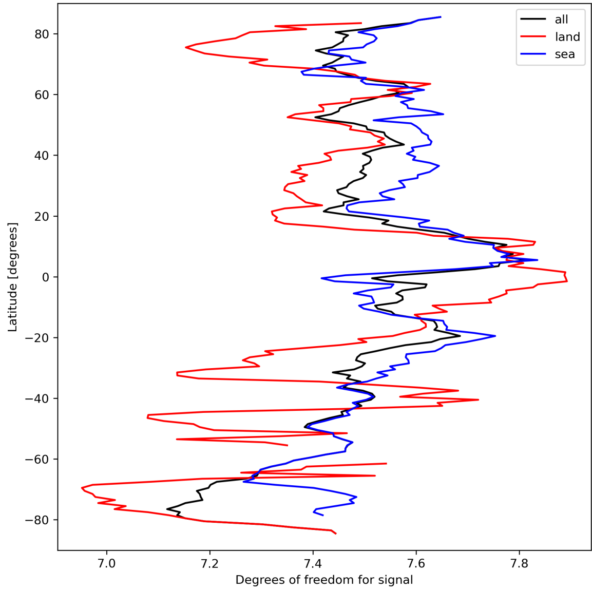
Figure 15: Zonal average of “Degrees of freedom for signal” for 2023-09-20 to 2023-09-22.
