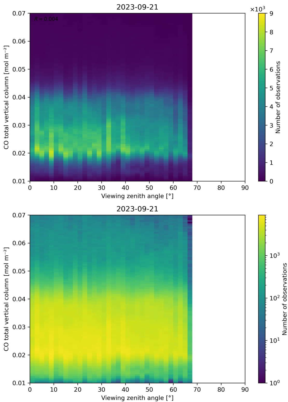
Figure 69: Scatter density plot of “Viewing zenith angle” against “CO total vertical column” for 2023-09-20 to 2023-09-22.
