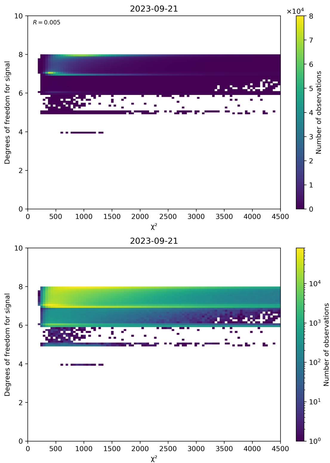
Figure 48: Scatter density plot of “ \chi^2 ” against “Degrees of freedom for signal” for 2023-09-20 to 2023-09-22.
