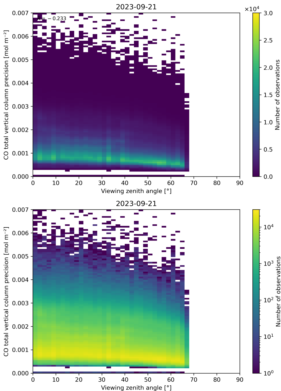
Figure 71: Scatter density plot of “Viewing zenith angle” against “CO total vertical column precision” for 2023-09-20 to 2023-09-22.
