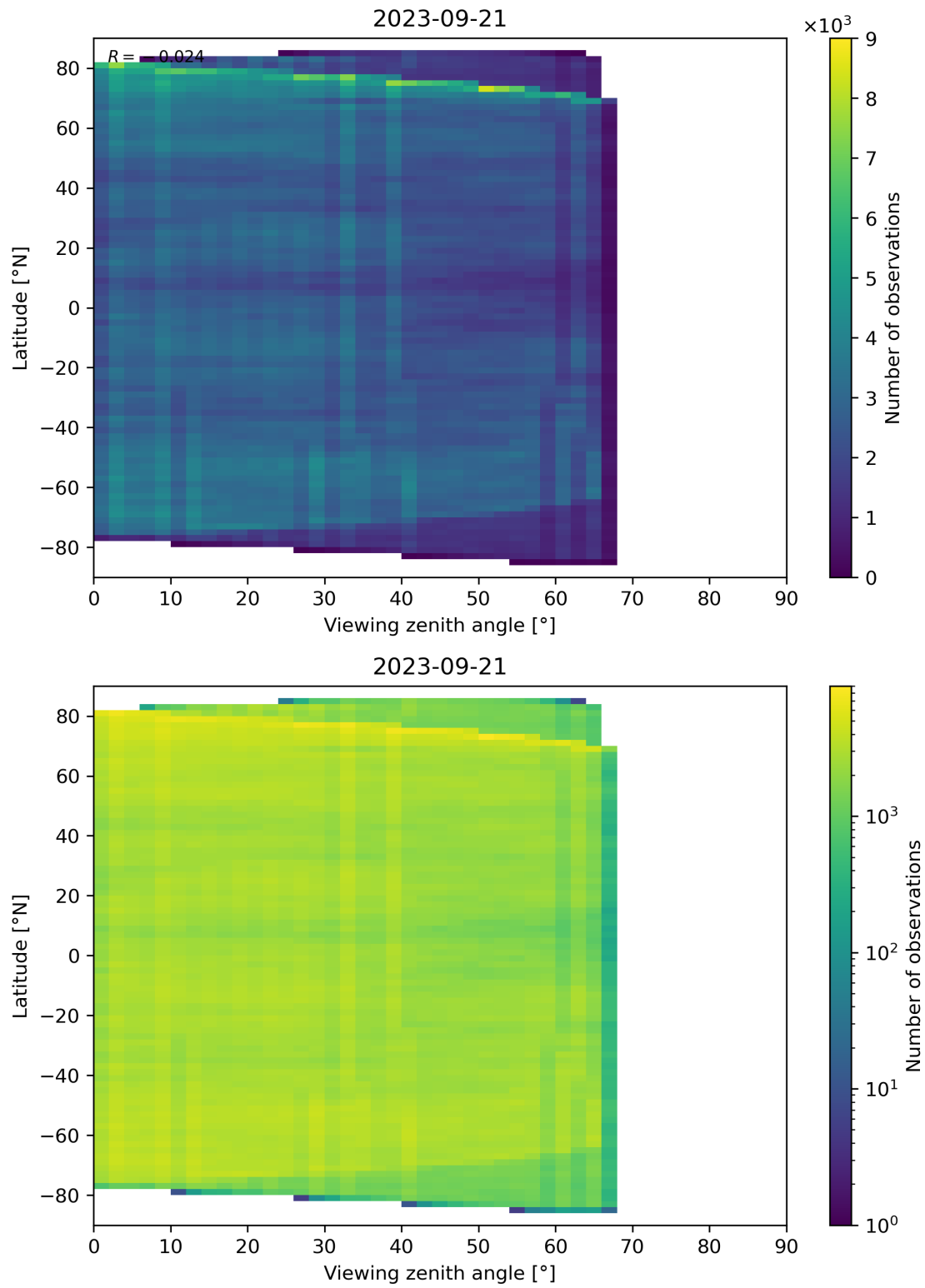
Figure 74: Scatter density plot of “Viewing zenith angle” against “Latitude” for 2023-09-20 to 2023-09-22.
