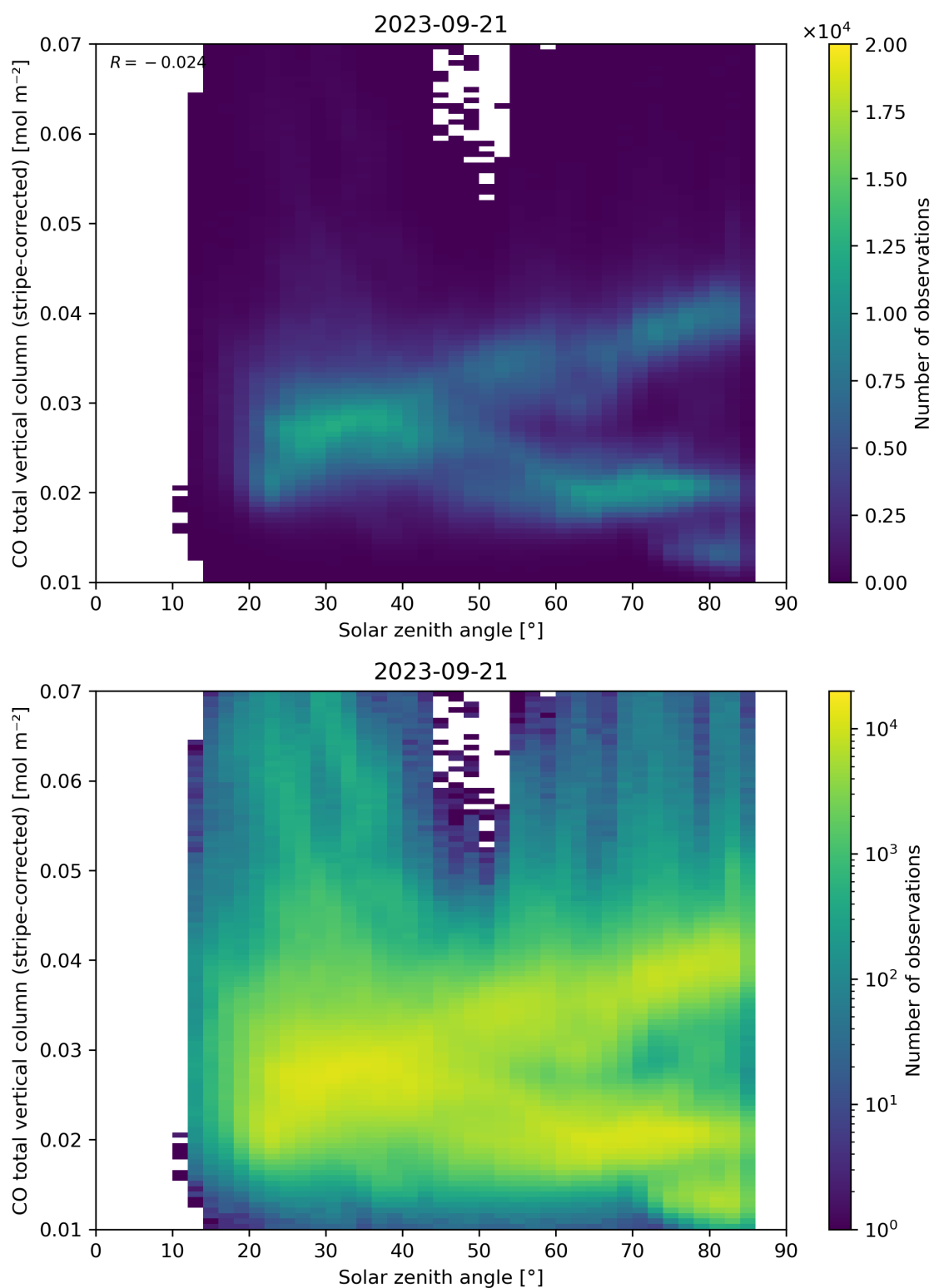
Figure 62: Scatter density plot of “Solar zenith angle” against “CO total vertical column (stripe-corrected)” for 2023-09-20 to 2023-09-22.
