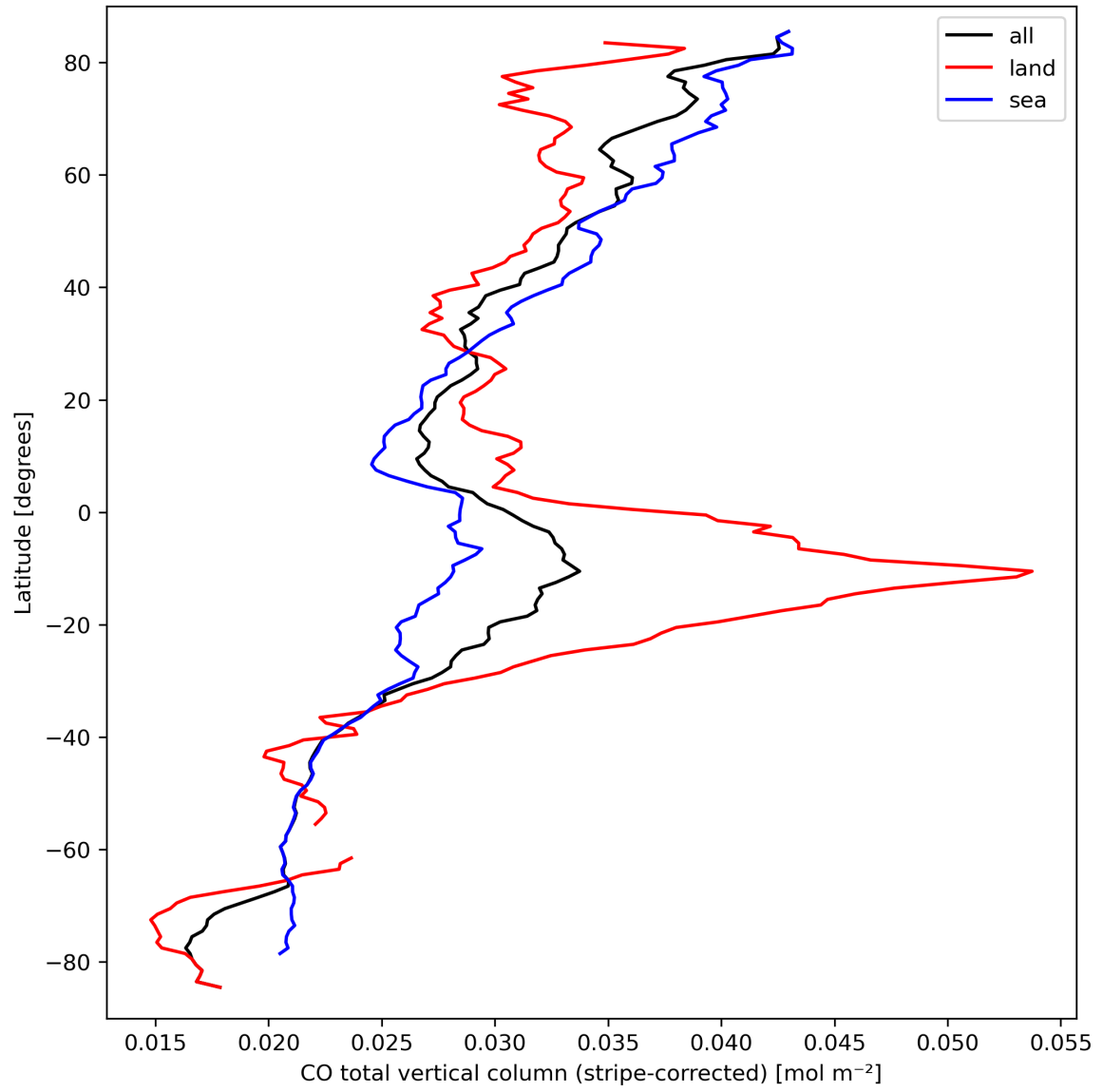
Figure 11: Zonal average of “CO total vertical column (stripe-corrected)” for 2023-09-20 to 2023-09-22.
