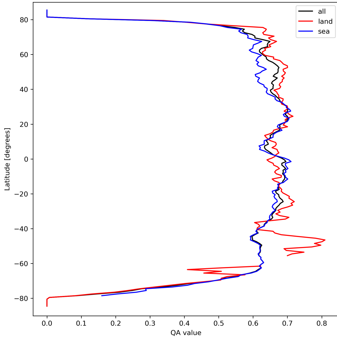
Figure 9: Zonal average of “QA value” for 2023-09-20 to 2023-09-22.
