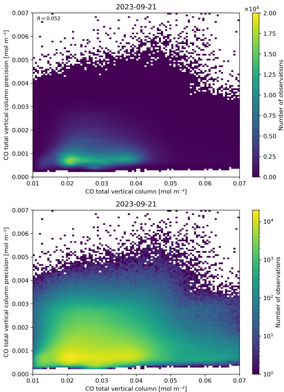
Figure 34: Scatter density plot of “CO total vertical column” against “CO total vertical column precision” for 2023-09-20 to 2023-09-22.
