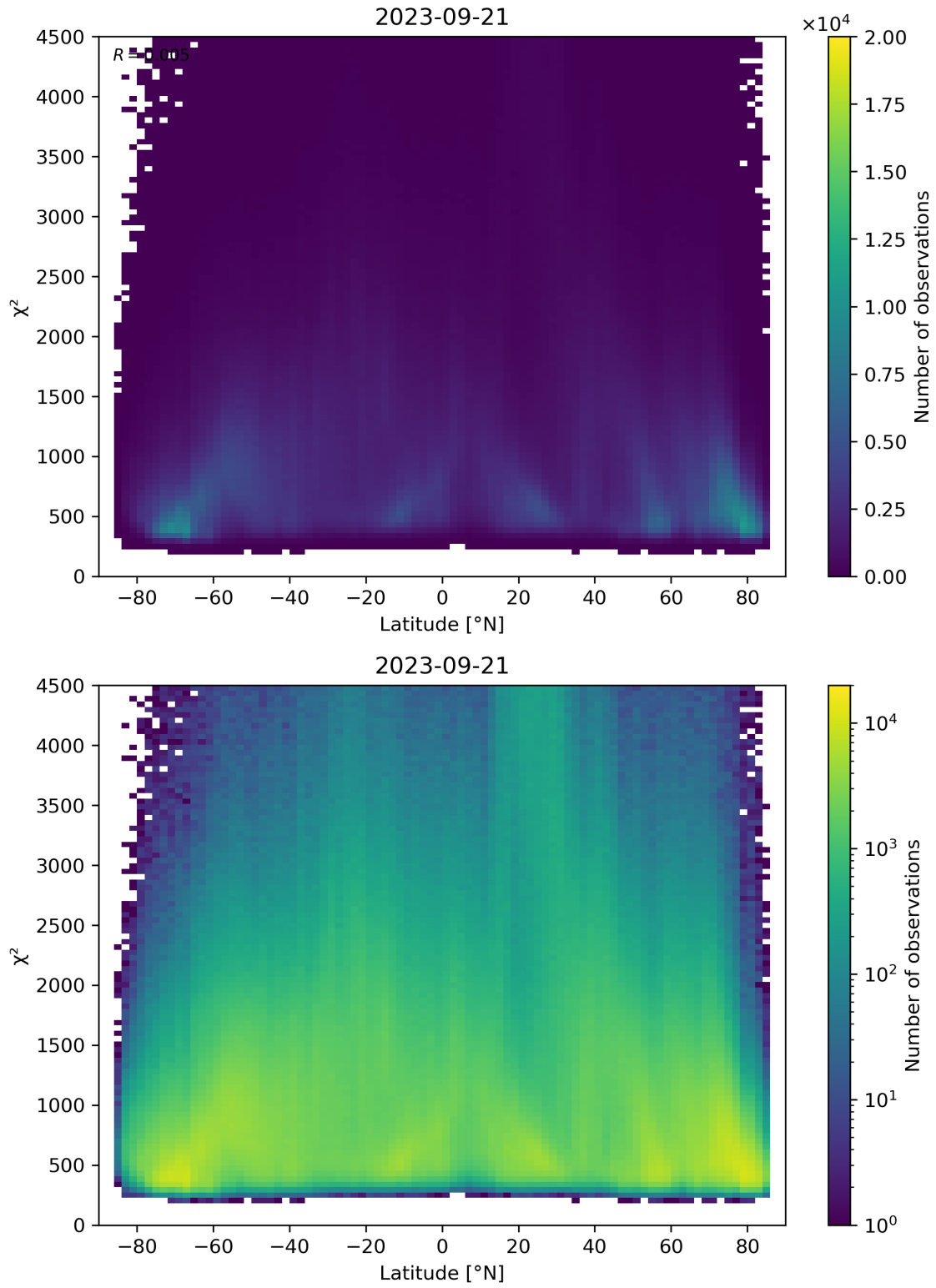
Figure 54: Scatter density plot of “Latitude” against “ \chi^2 ” for 2023-09-20 to 2023-09-22.
