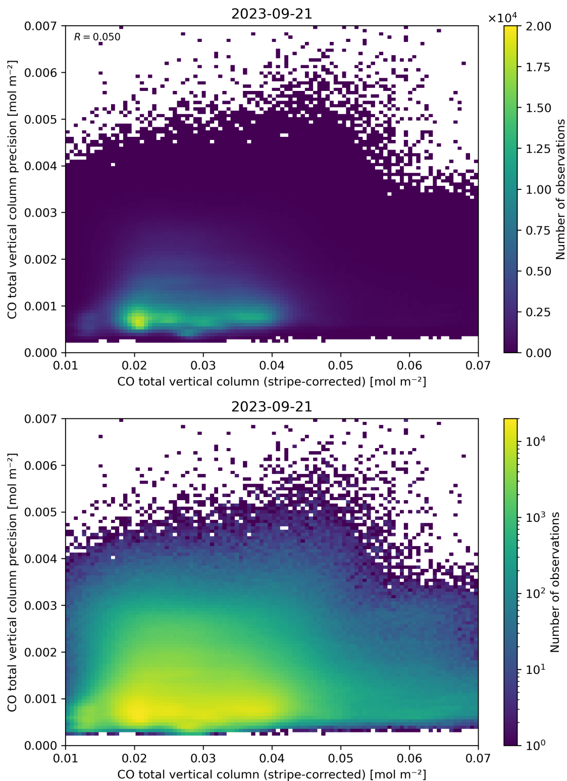
Figure 36: Scatter density plot of “CO total vertical column (stripe-corrected)” against “CO total vertical column precision” for 2023-09-20 to 2023-09-22.
