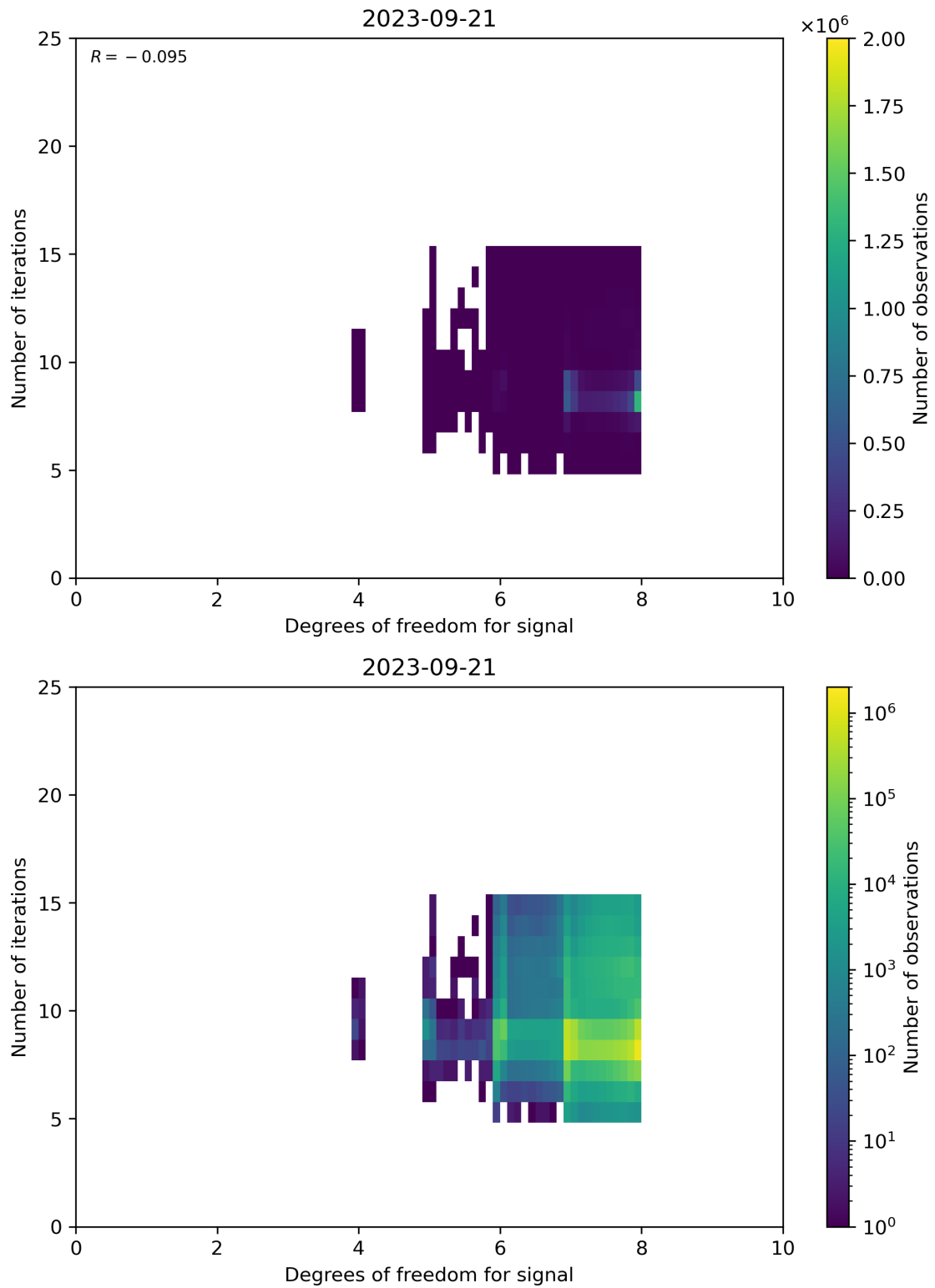
Figure 50: Scatter density plot of “Degrees of freedom for signal” against “Number of iterations” for 2023-09-20 to 2023-09-22.
