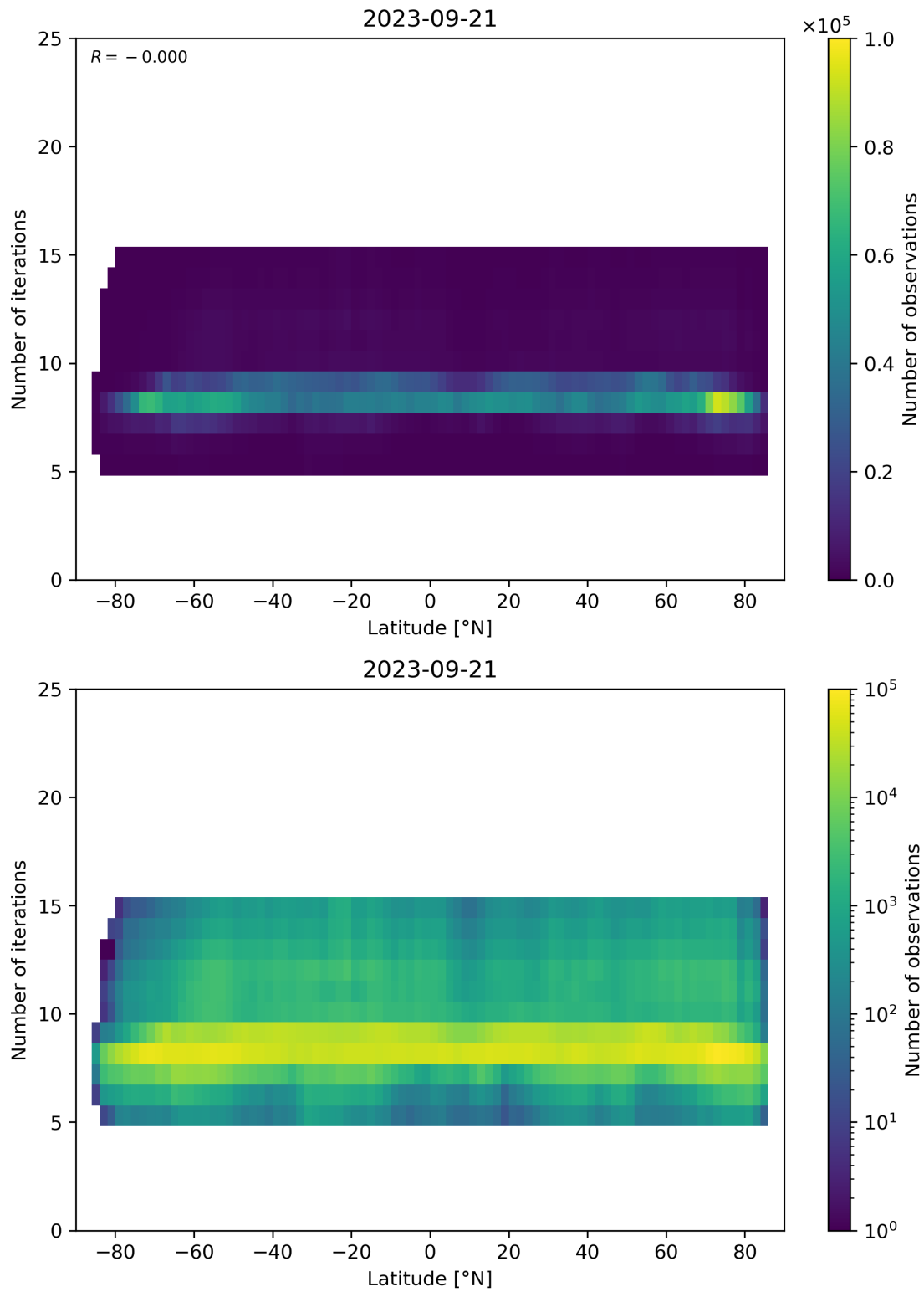
Figure 56: Scatter density plot of “Latitude” against “Number of iterations” for 2023-09-20 to 2023-09-22.
