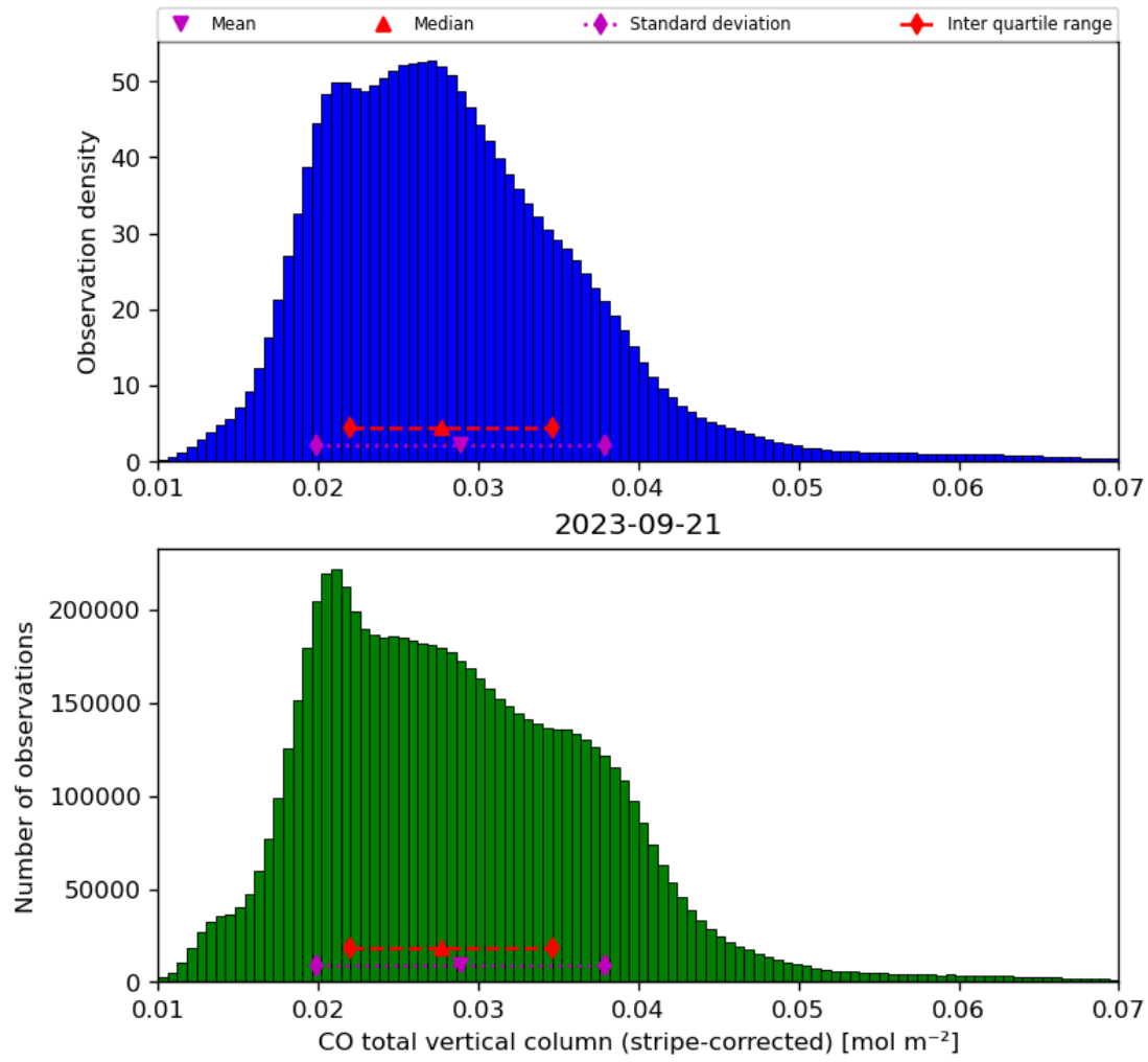
Figure 19: Histogram of “CO total vertical column (stripe-corrected)” for 2023-09-20 to 2023-09-22
