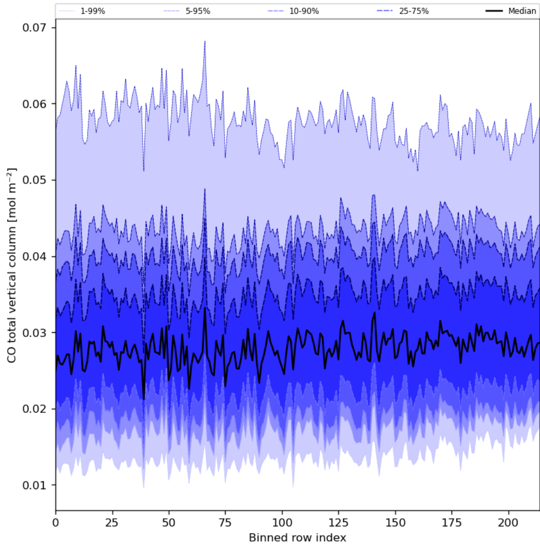
Figure 26: Along track statistics of “CO total vertical column” for 2023-09-20 to 2023-09-22
