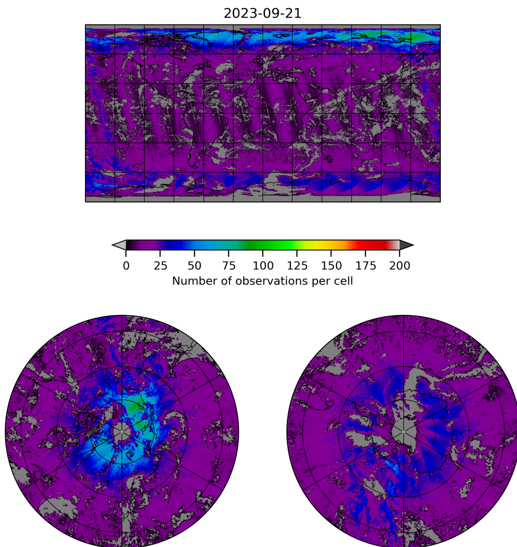
Figure 8: Map of the number of observations for 2023-09-20 to 2023-09-22
