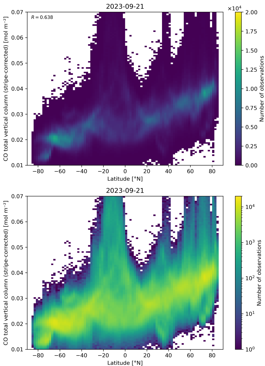
Figure 52: Scatter density plot of “Latitude” against “CO total vertical column (stripe-corrected)” for 2023-09-20 to 2023-09-22.
