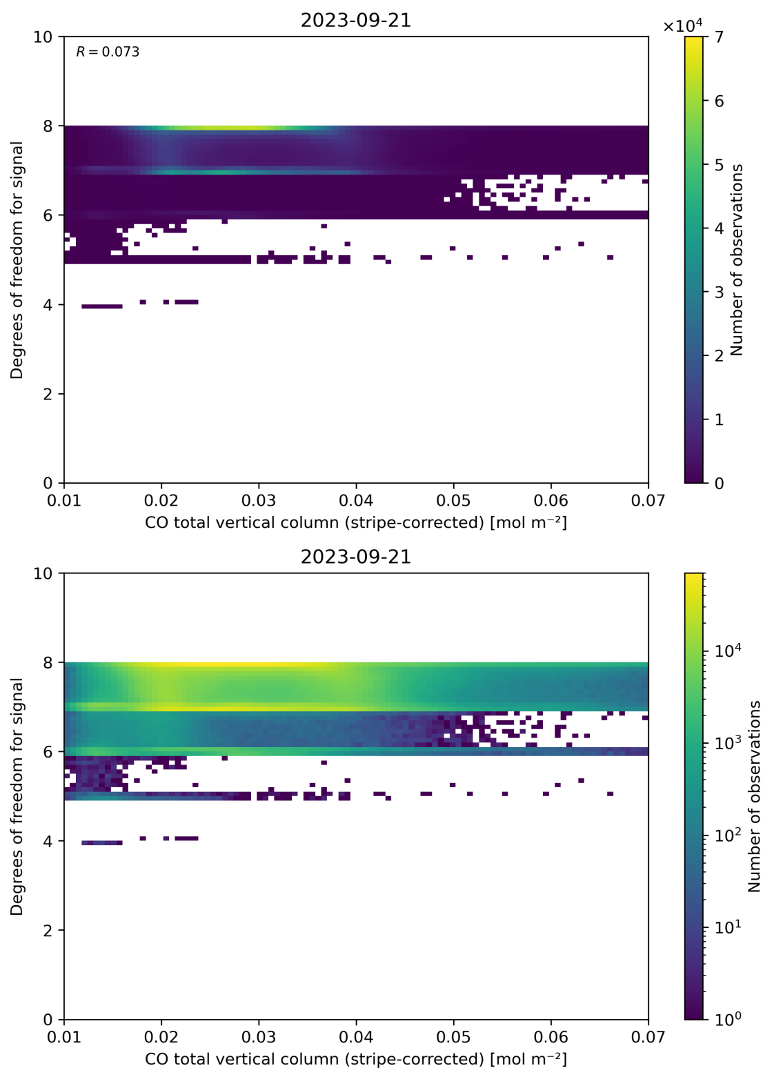
Figure 38: Scatter density plot of “CO total vertical column (stripe-corrected)” against “Degrees of freedom for signal” for 2023-09-20 to 2023-09-22.
