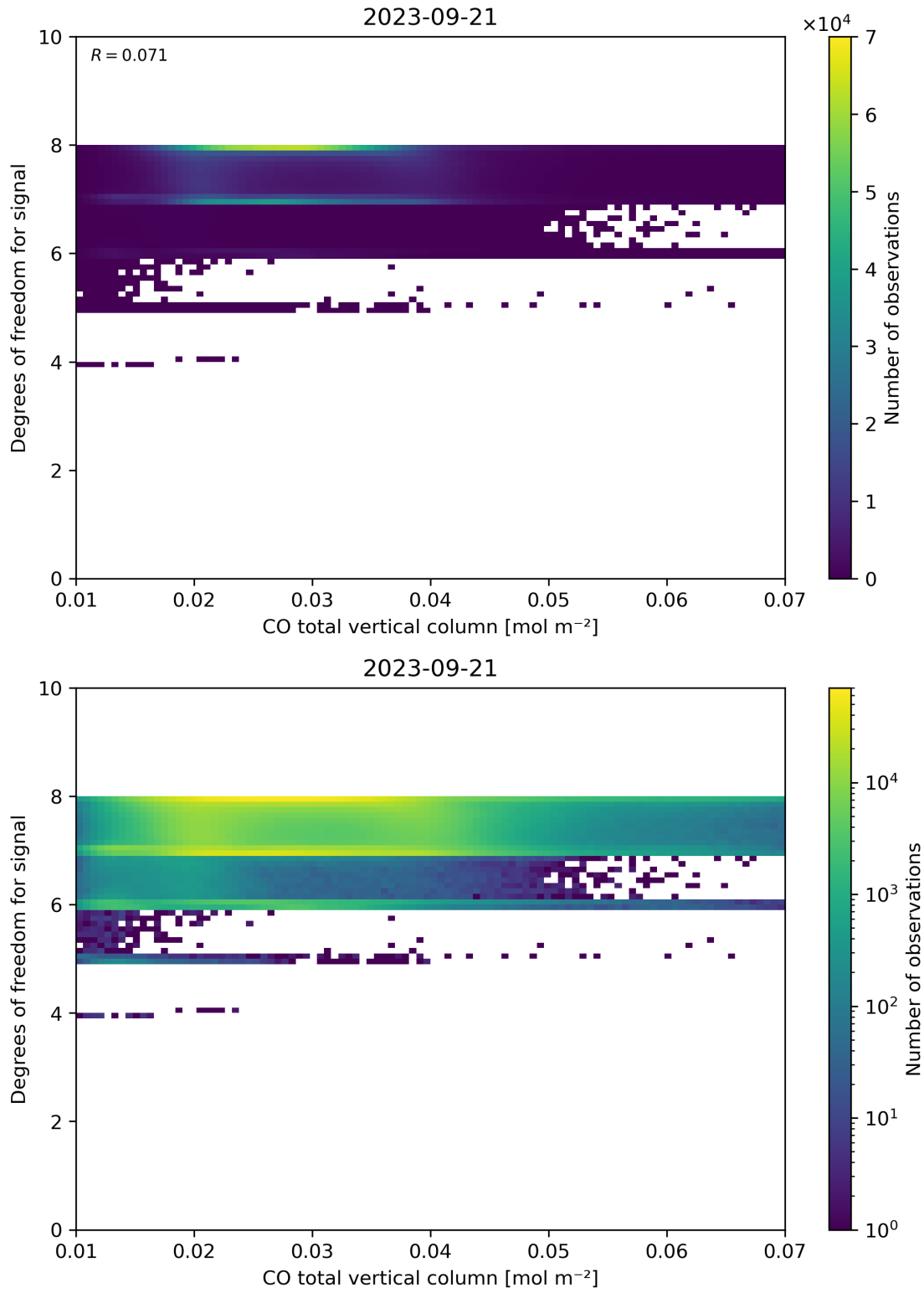
Figure 41: Scatter density plot of “CO total vertical column” against “Degrees of freedom for signal” for 2023-09-20 to 2023-09-22.
