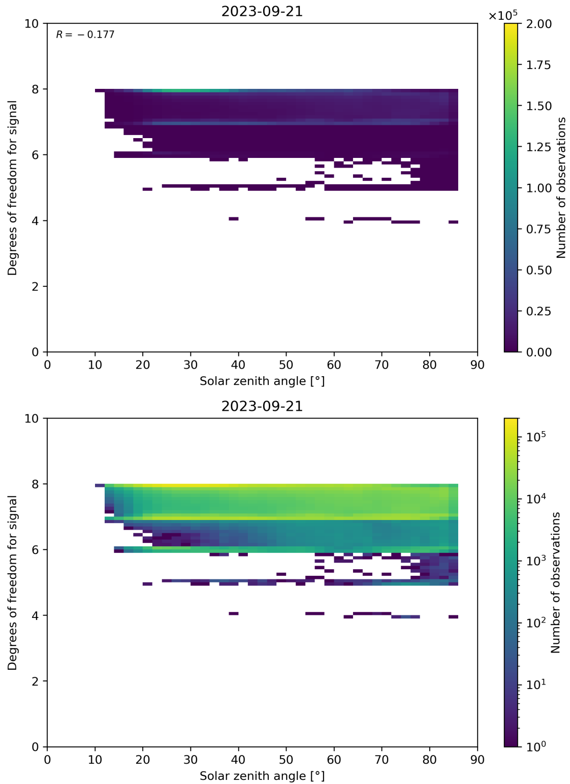
Figure 65: Scatter density plot of “Solar zenith angle” against “Degrees of freedom for signal” for 2023-09-20 to 2023-09-22.
