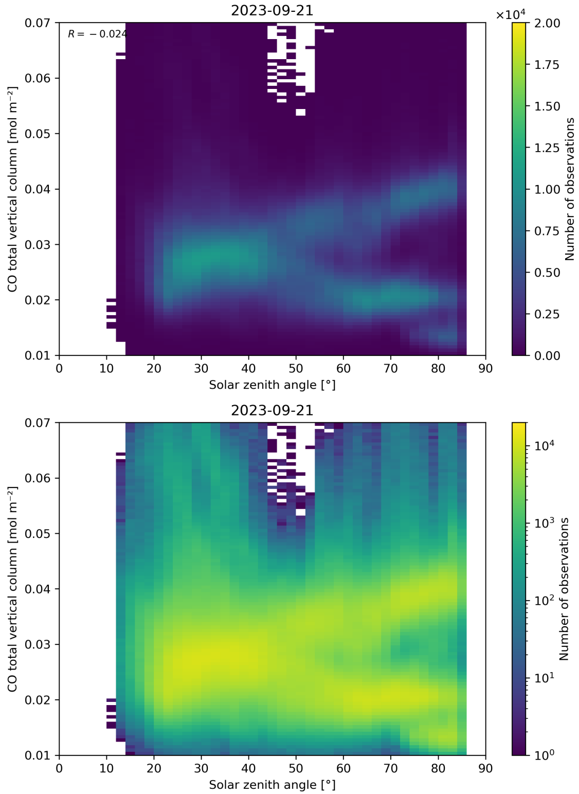
Figure 61: Scatter density plot of “Solar zenith angle” against “CO total vertical column” for 2023-09-20 to 2023-09-22.
