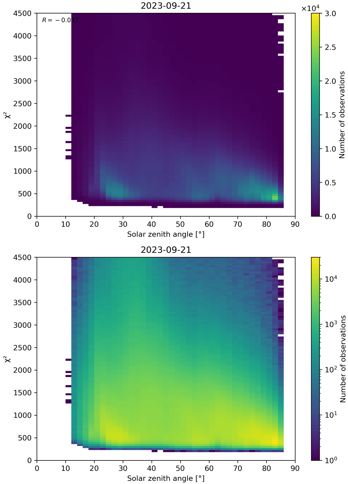
Figure 64: Scatter density plot of “Solar zenith angle” against “ \chi^2 ” for 2023-09-20 to 2023-09-22.
