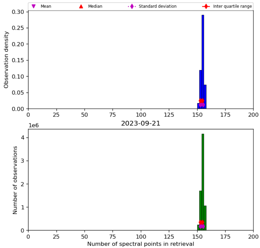
Figure 21: Histogram of “Number of spectral points in retrieval” for 2023-09-20 to 2023-09-22
