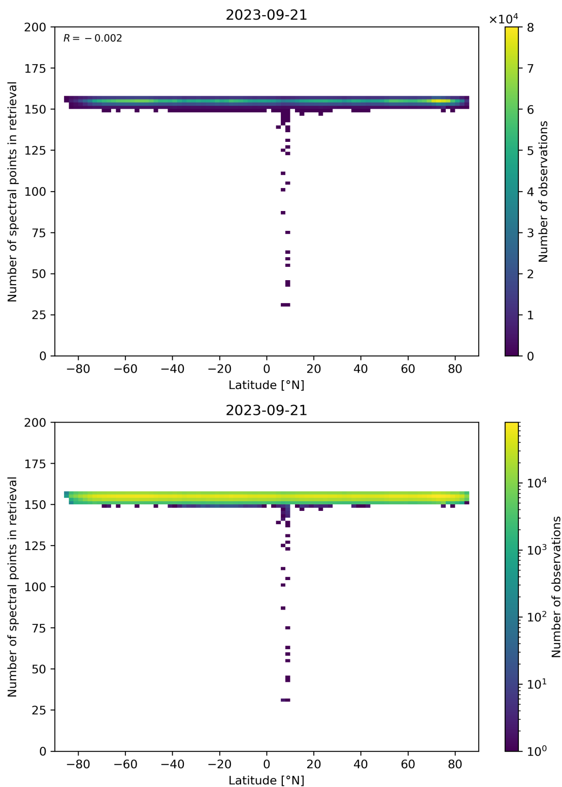
Figure 57: Scatter density plot of “Latitude” against “Number of spectral points in retrieval” for 2023-09-20 to 2023-09-22.
