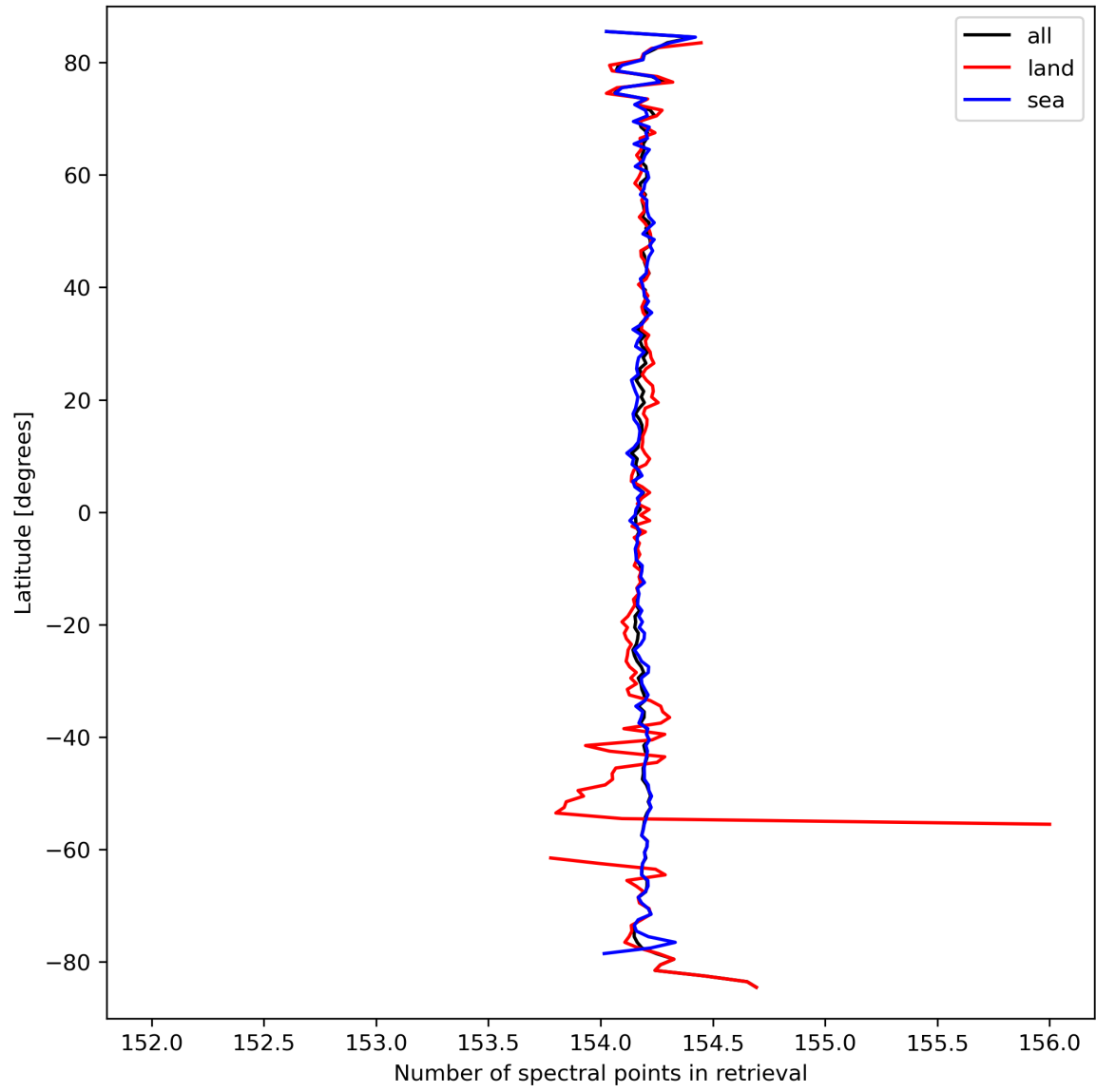
Figure 13: Zonal average of “Number of spectral points in retrieval” for 2023-09-20 to 2023-09-22.
