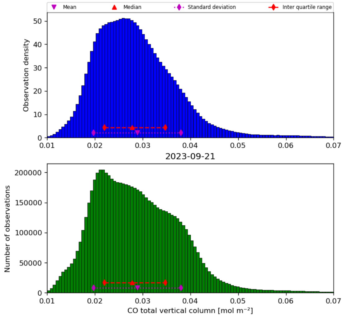
Figure 18: Histogram of “CO total vertical column” for 2023-09-20 to 2023-09-22
