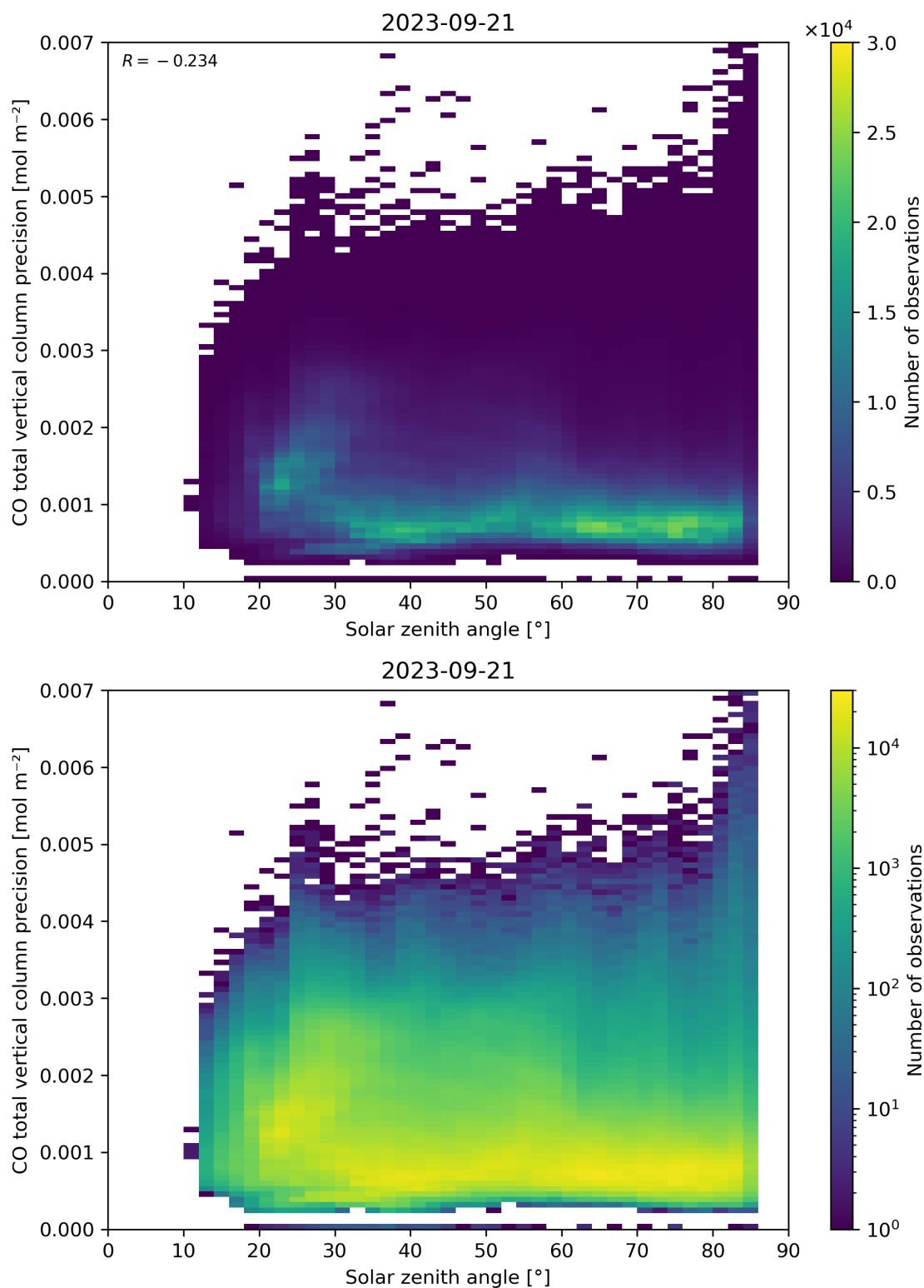
Figure 63: Scatter density plot of “Solar zenith angle” against “CO total vertical column precision” for 2023-09-20 to 2023-09-22.
