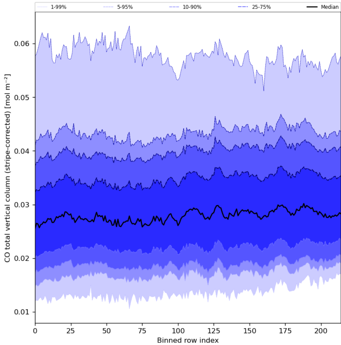
Figure 27: Along track statistics of “CO total vertical column (stripe-corrected)” for 2023-09-20 to 2023-09-22
