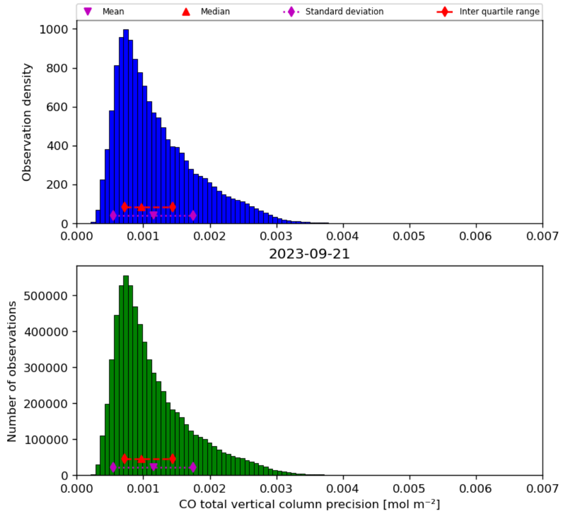
Figure 20: Histogram of “CO total vertical column precision” for 2023-09-20 to 2023-09-22
