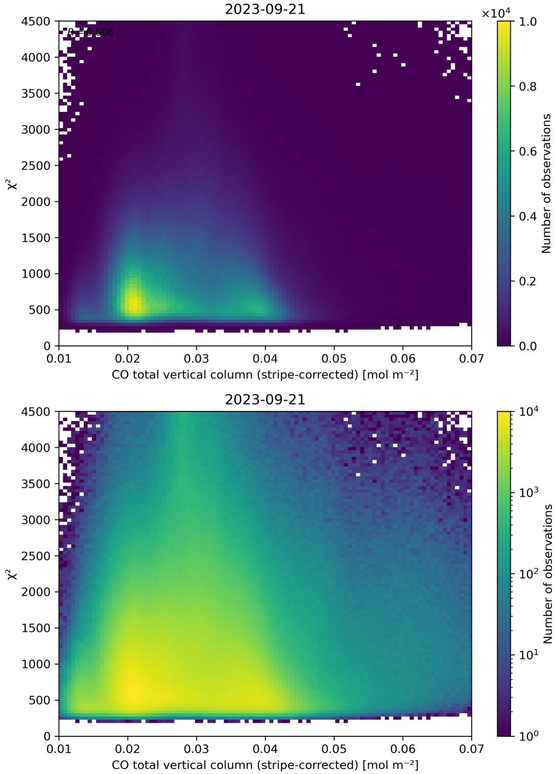
Figure 37: Scatter density plot of “CO total vertical column (stripe-corrected)” against “ \chi^2 ” for 2023-09-20 to 2023-09-22.
