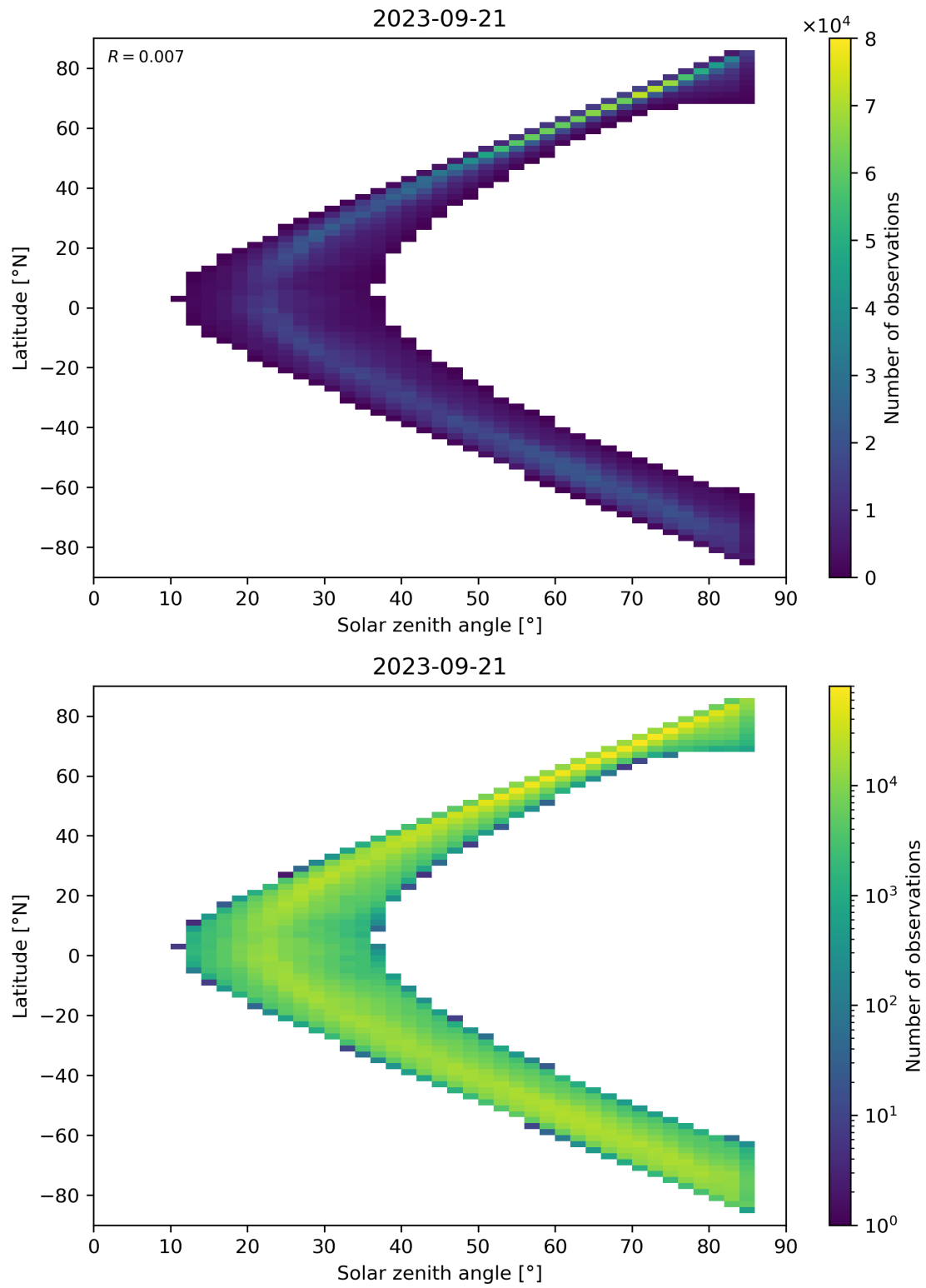
Figure 66: Scatter density plot of “Solar zenith angle” against “Latitude” for 2023-09-20 to 2023-09-22.
