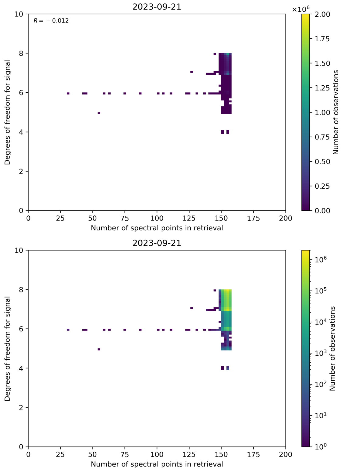
Figure 59: Scatter density plot of “Number of spectral points in retrieval” against “Degrees of freedom for signal” for 2023-09-20 to 2023-09-22.
