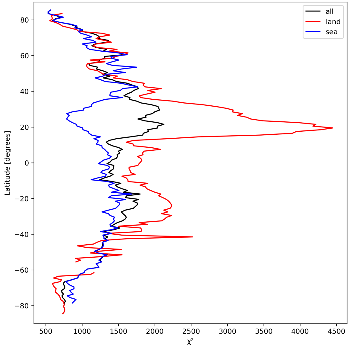
Figure 14: Zonal average of “ \chi^2 ” for 2023-09-20 to 2023-09-22.
