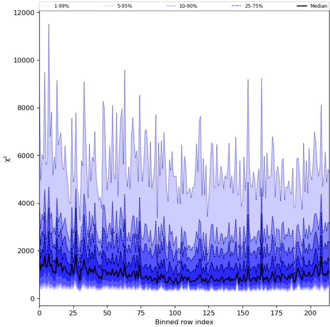
Figure 30: Along track statistics of “ \chi^2 ” for 2023-09-20 to 2023-09-22
