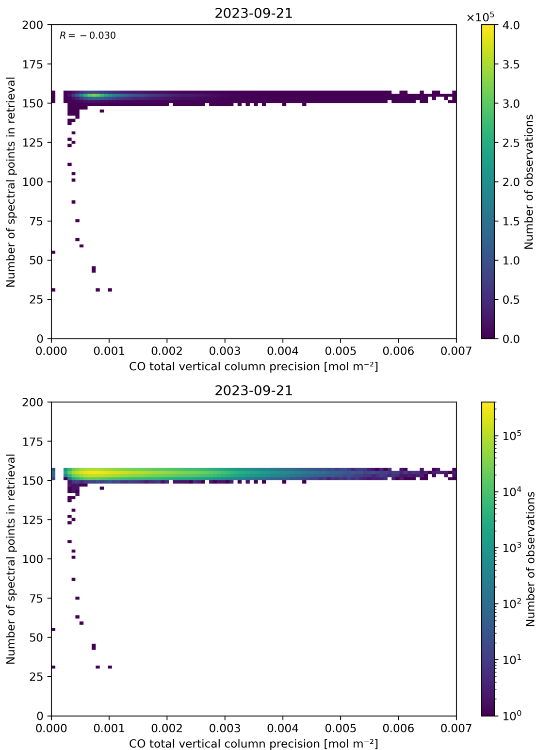
Figure 47: Scatter density plot of “CO total vertical column precision” against “Number of spectral points in retrieval” for 2023-09-20 to 2023-09-22.
