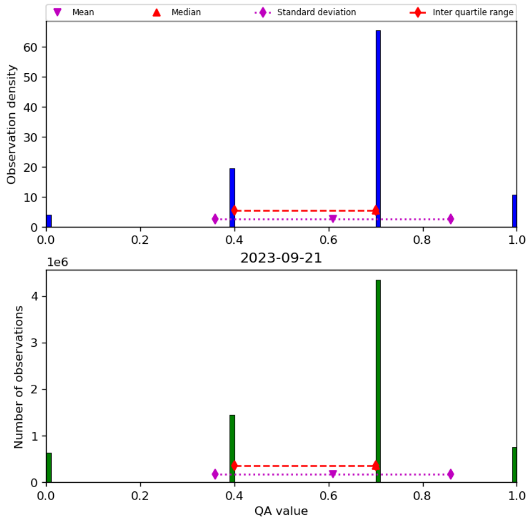
Figure 17: Histogram of “QA value” for 2023-09-20 to 2023-09-22
