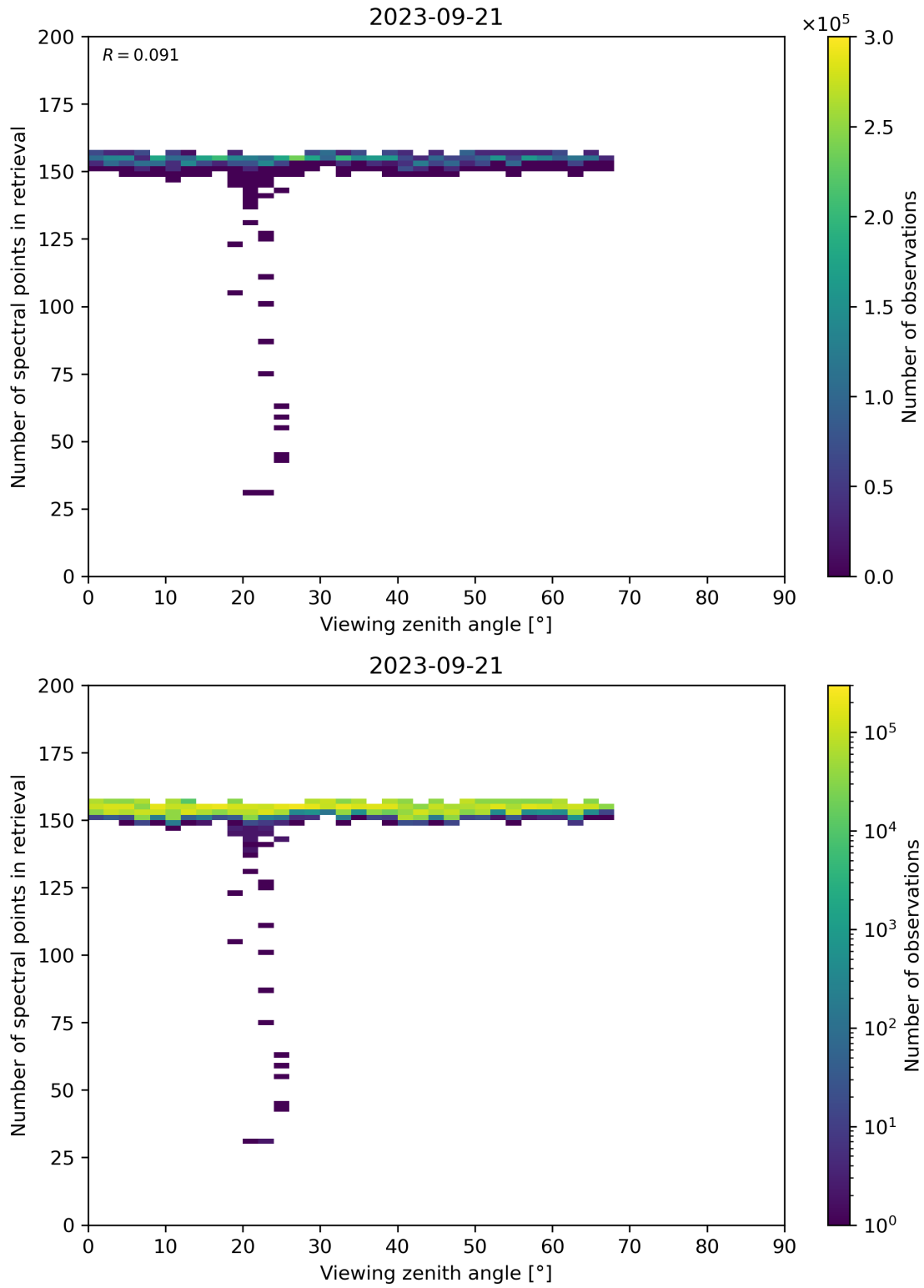
Figure 76: Scatter density plot of “Viewing zenith angle” against “Number of spectral points in retrieval” for 2023-09-20 to 2023-09-22.
