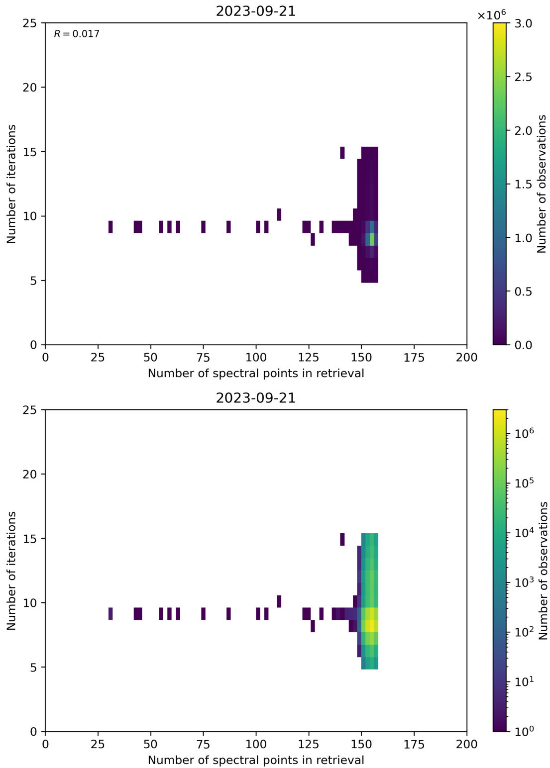
Figure 60: Scatter density plot of “Number of spectral points in retrieval” against “Number of iterations” for 2023-09-20 to 2023-09-22.
