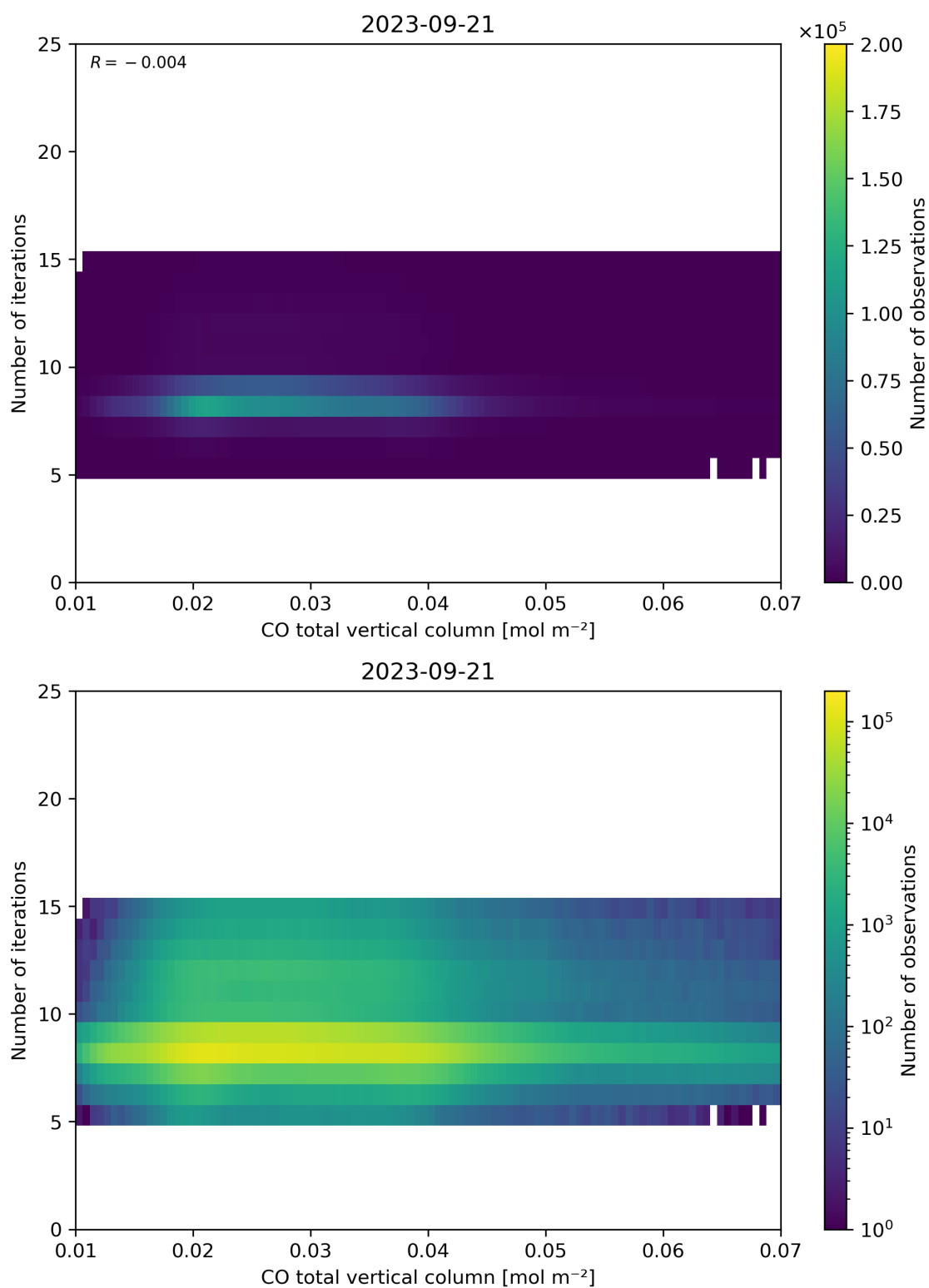
Figure 42: Scatter density plot of “CO total vertical column” against “Number of iterations” for 2023-09-20 to 2023-09-22.
