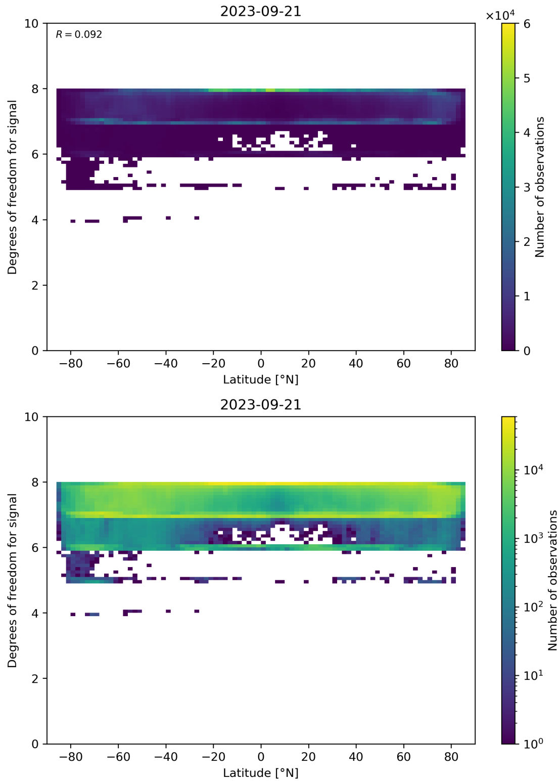
Figure 55: Scatter density plot of “Latitude” against “Degrees of freedom for signal” for 2023-09-20 to 2023-09-22.
