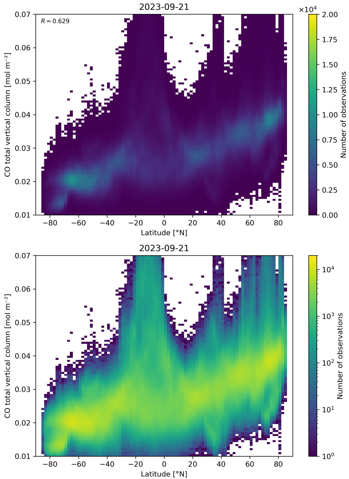
Figure 51: Scatter density plot of “Latitude” against “CO total vertical column” for 2023-09-20 to 2023-09-22.
