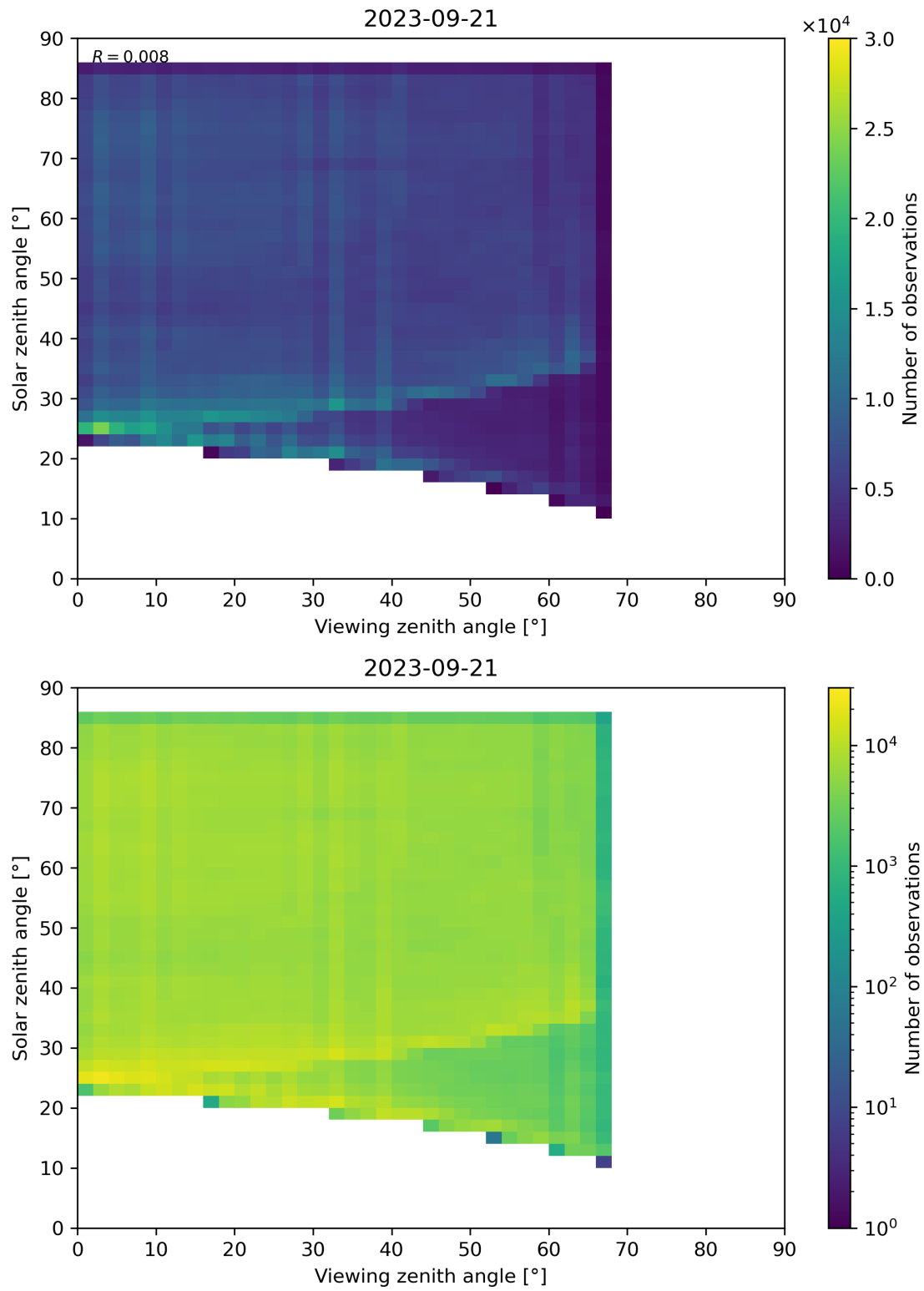
Figure 77: Scatter density plot of “Viewing zenith angle” against “Solar zenith angle” for 2023-09-20 to 2023-09-22.
