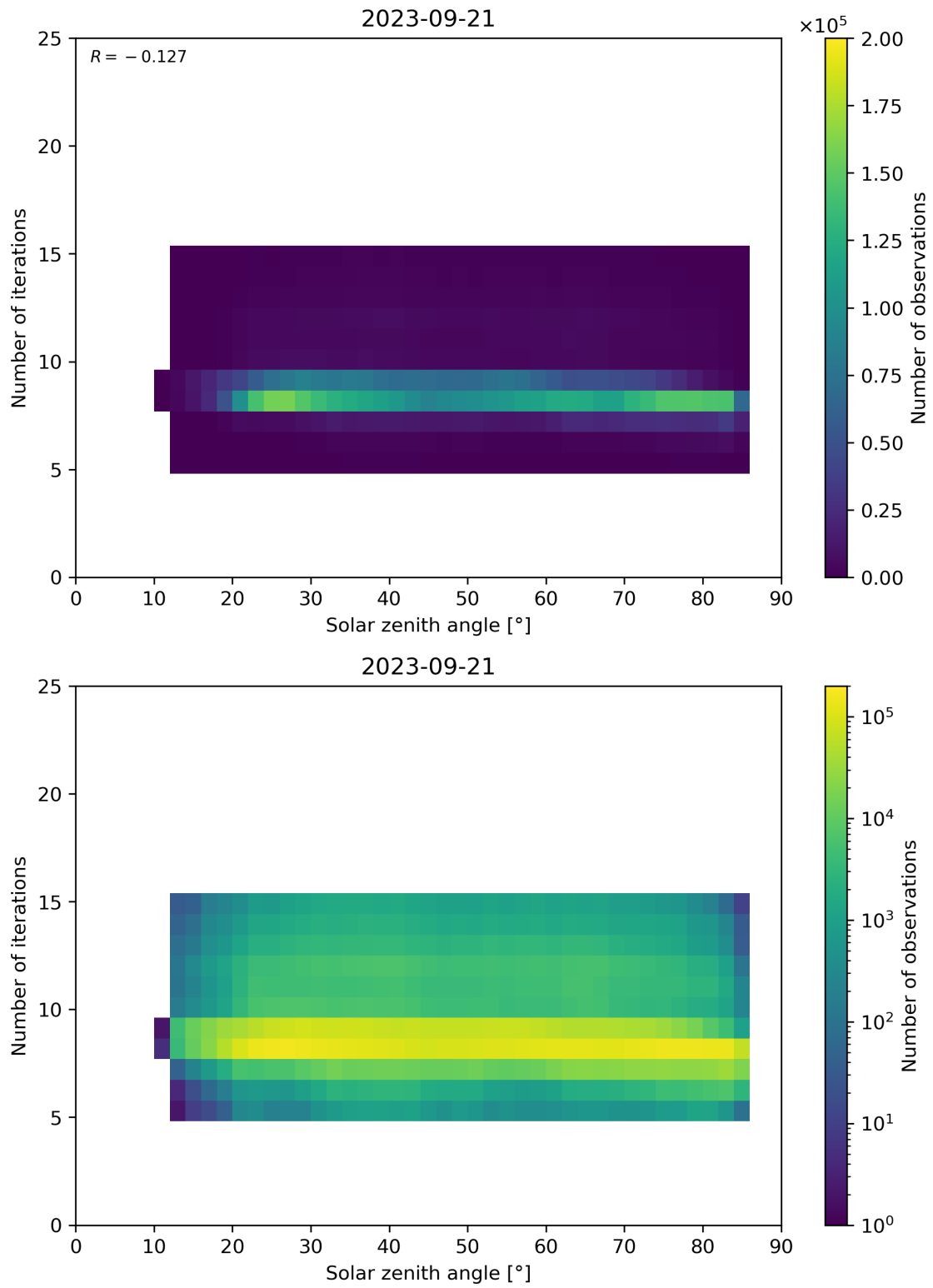
Figure 67: Scatter density plot of “Solar zenith angle” against “Number of iterations” for 2023-09-20 to 2023-09-22.
