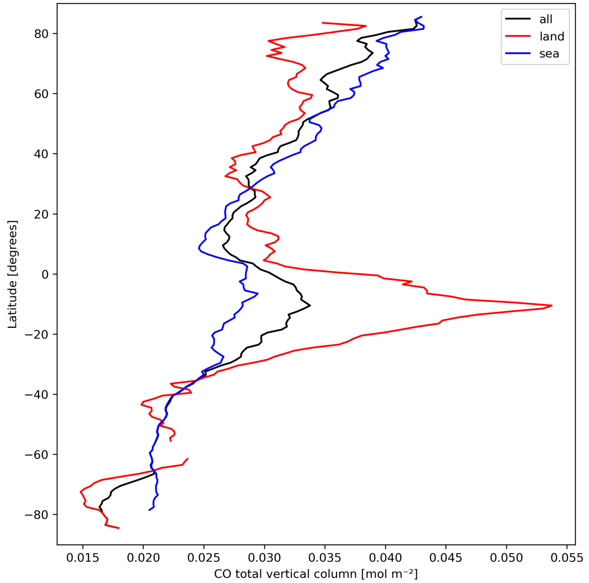
Figure 10: Zonal average of “CO total vertical column” for 2023-09-20 to 2023-09-22.
