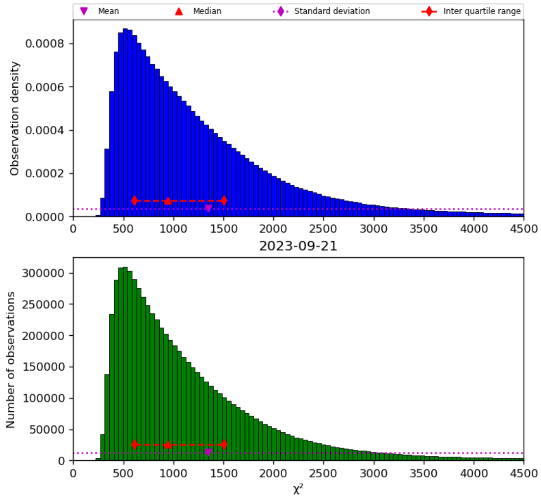
Figure 22: Histogram of “ \chi^2 ” for 2023-09-20 to 2023-09-22
