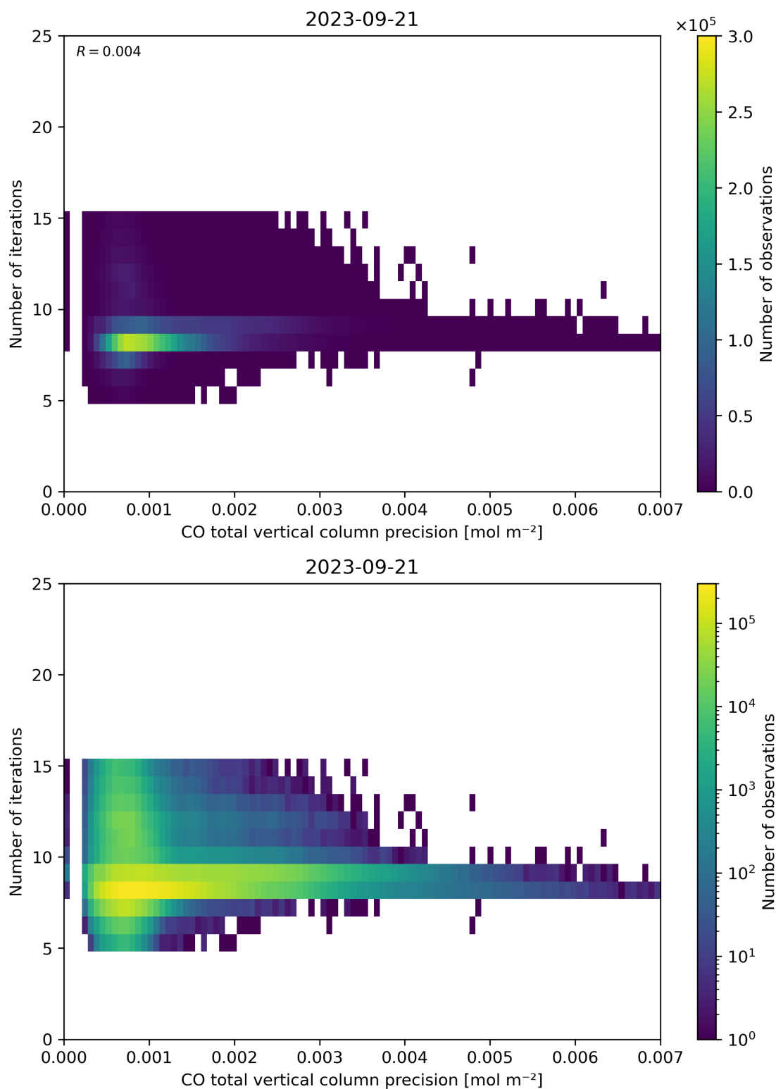
Figure 46: Scatter density plot of “CO total vertical column precision” against “Number of iterations” for 2023-09-20 to 2023-09-22.
