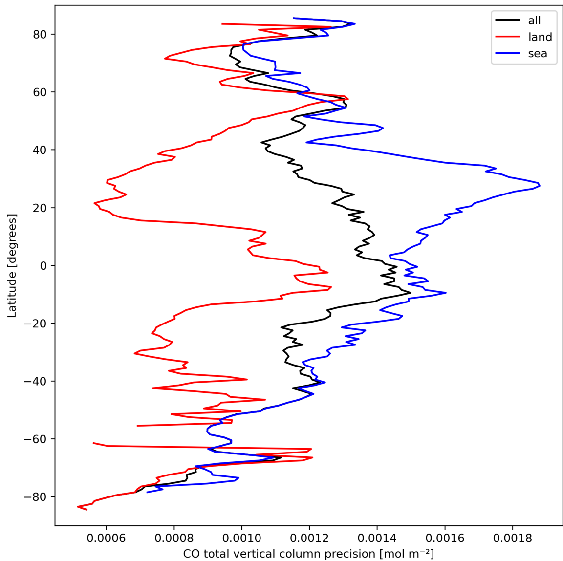
Figure 12: Zonal average of “CO total vertical column precision” for 2023-09-20 to 2023-09-22.
