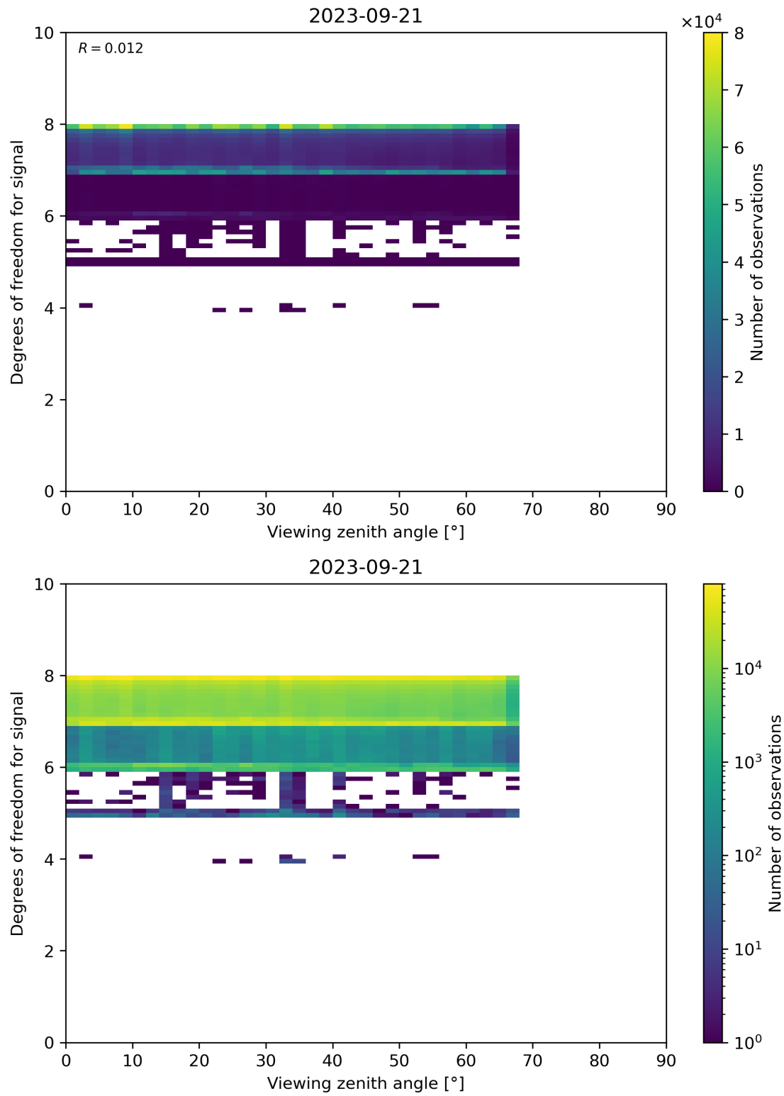
Figure 73: Scatter density plot of “Viewing zenith angle” against “Degrees of freedom for signal” for 2023-09-20 to 2023-09-22.
