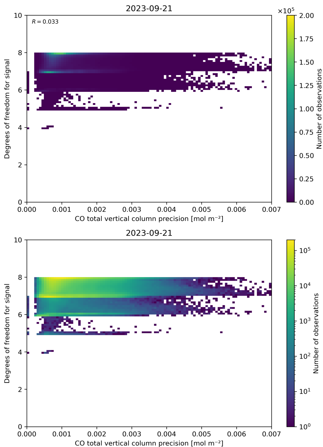
Figure 45: Scatter density plot of “CO total vertical column precision” against “Degrees of freedom for signal” for 2023-09-20 to 2023-09-22.
