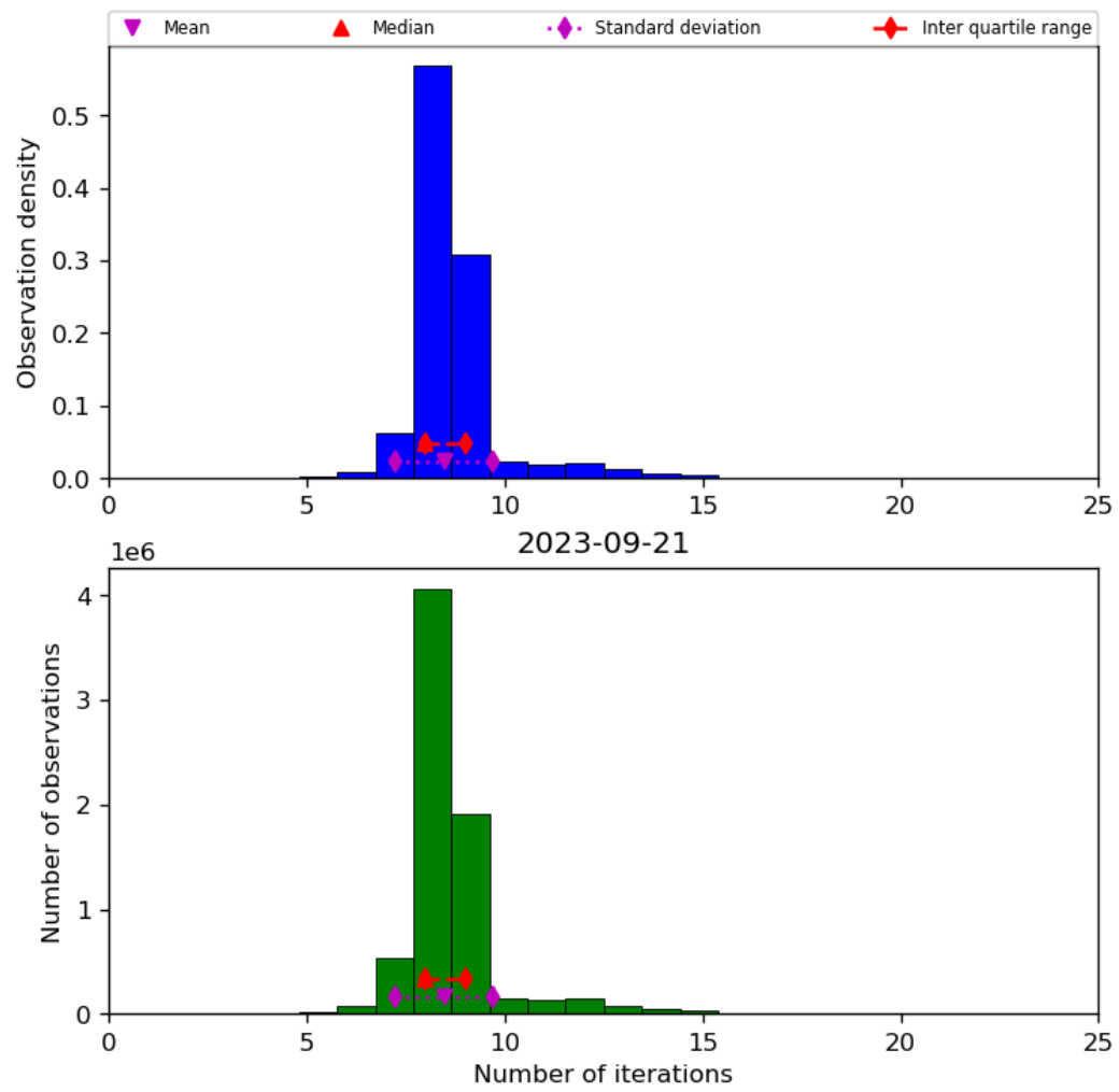
Figure 24: Histogram of “Number of iterations” for 2023-09-20 to 2023-09-22
