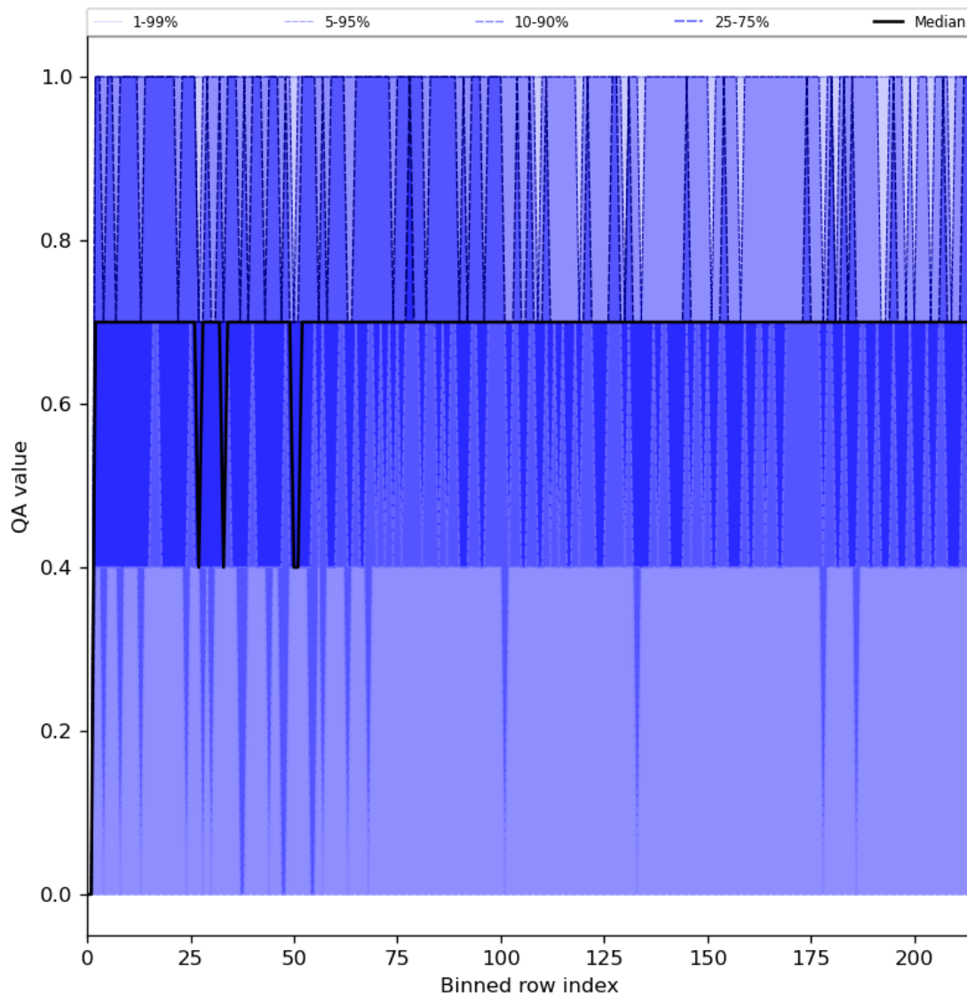
Figure 25: Along track statistics of “QA value” for 2023-09-20 to 2023-09-22
