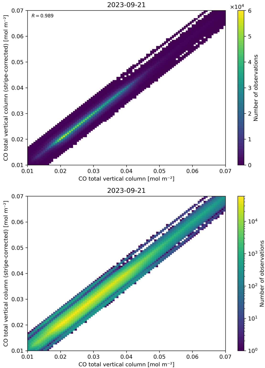
Figure 33: Scatter density plot of “CO total vertical column” against “CO total vertical column (stripe-corrected)” for 2023-09-20 to 2023-09-22.
