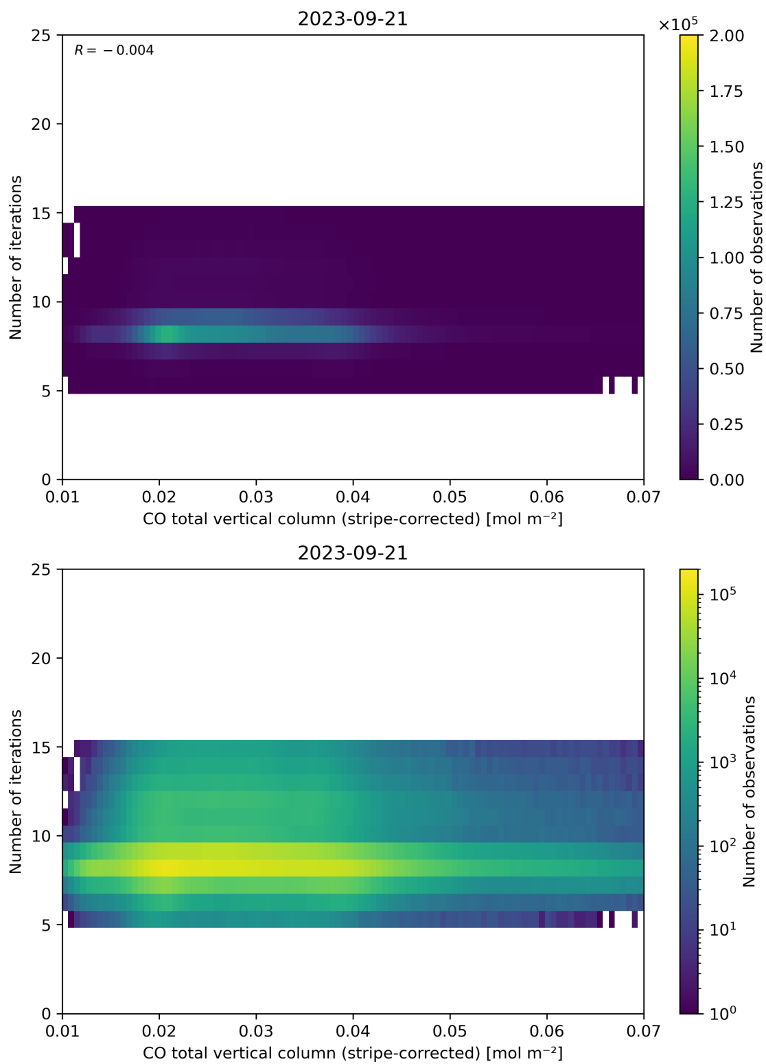
Figure 39: Scatter density plot of “CO total vertical column (stripe-corrected)” against “Number of iterations” for 2023-09-20 to 2023-09-22.
