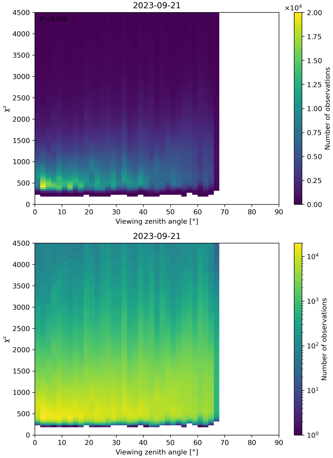
Figure 72: Scatter density plot of “Viewing zenith angle” against “ \chi^2 ” for 2023-09-20 to 2023-09-22.
