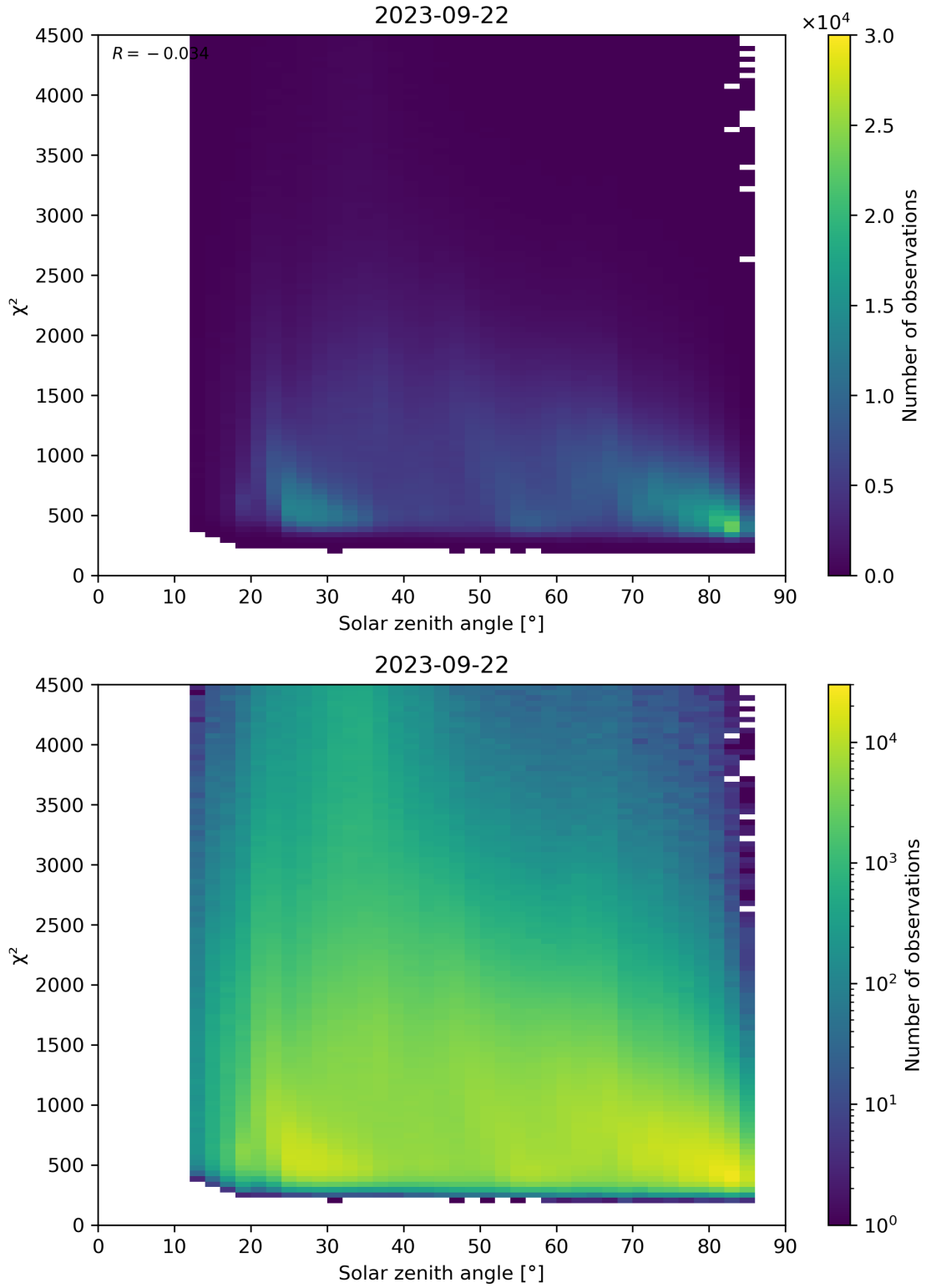
Figure 64: Scatter density plot of “Solar zenith angle” against “ \chi^2 ” for 2023-09-21 to 2023-09-23.
