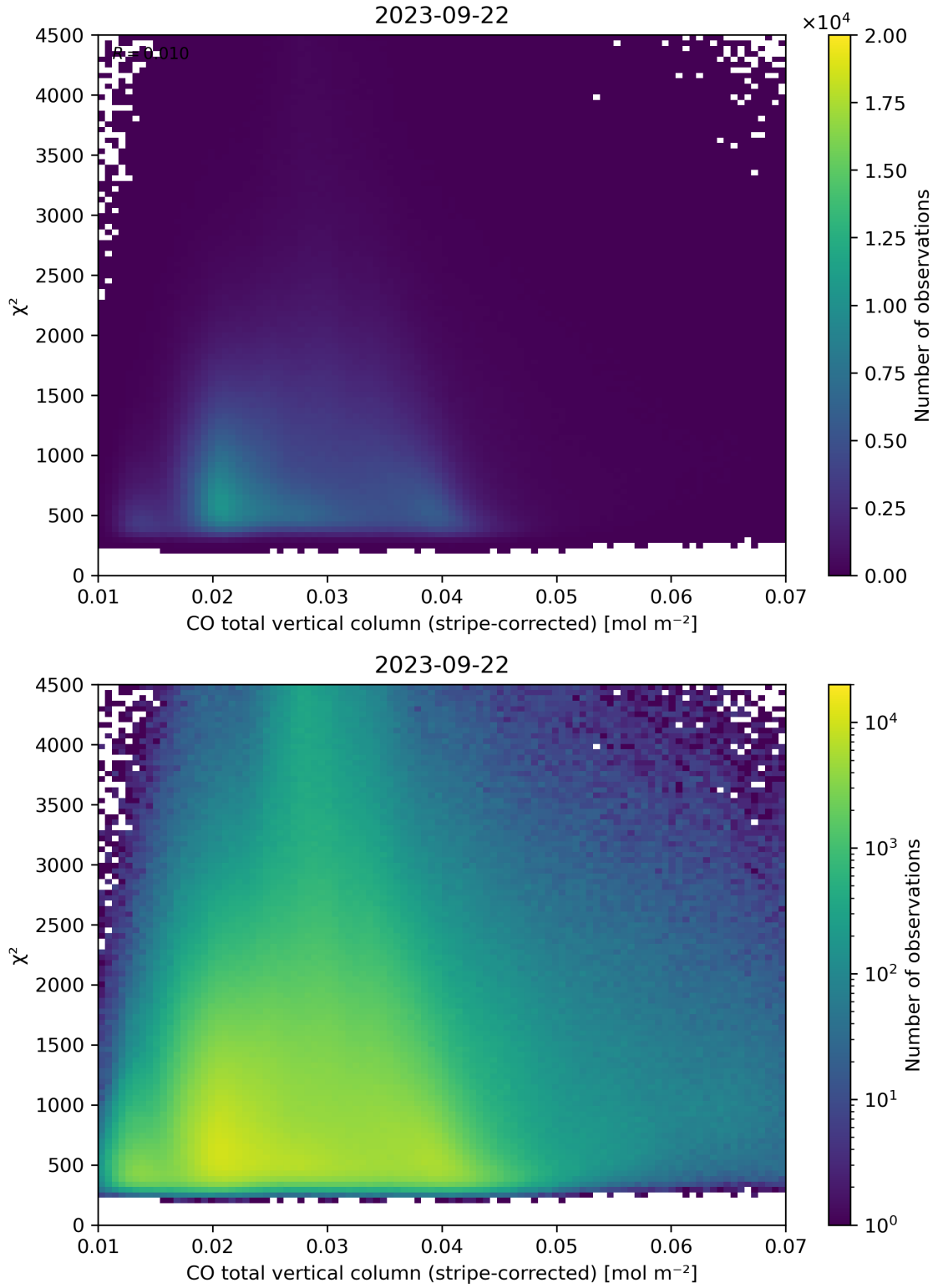
Figure 37: Scatter density plot of “CO total vertical column (stripe-corrected)” against “ \chi^2 ” for 2023-09-21 to 2023-09-23.
