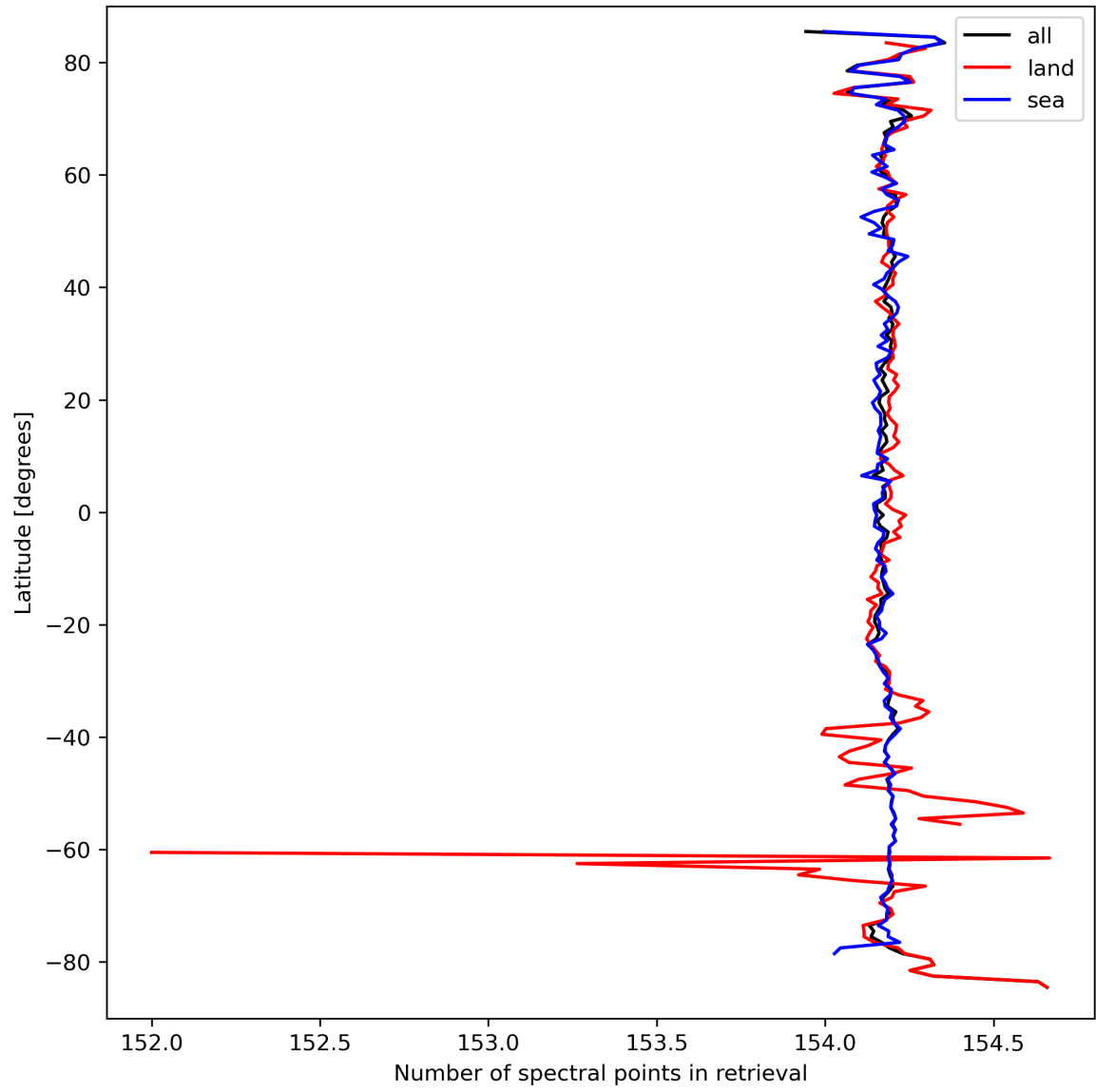
Figure 13: Zonal average of “Number of spectral points in retrieval” for 2023-09-21 to 2023-09-23.
