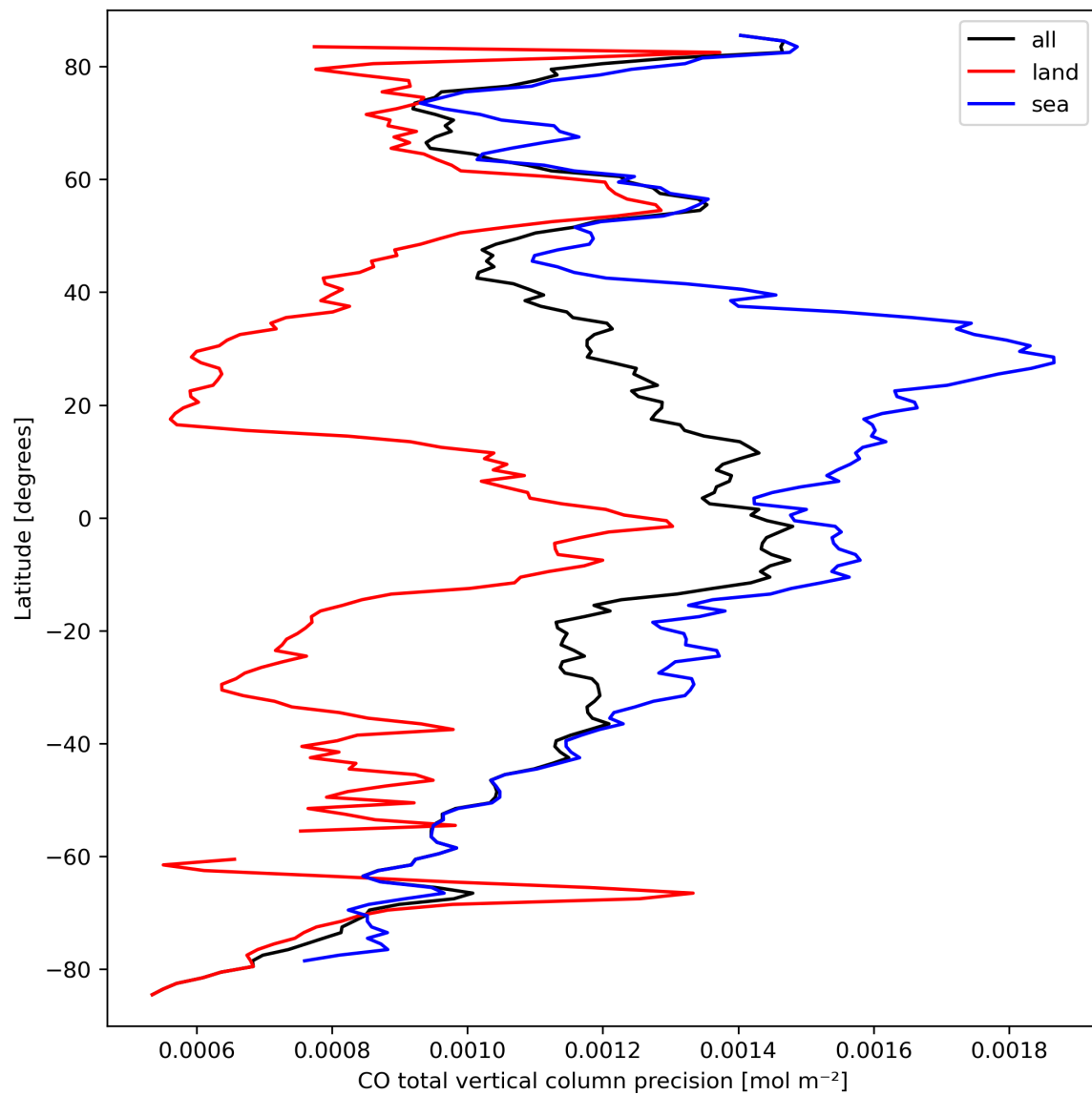
Figure 12: Zonal average of “CO total vertical column precision” for 2023-09-21 to 2023-09-23.
