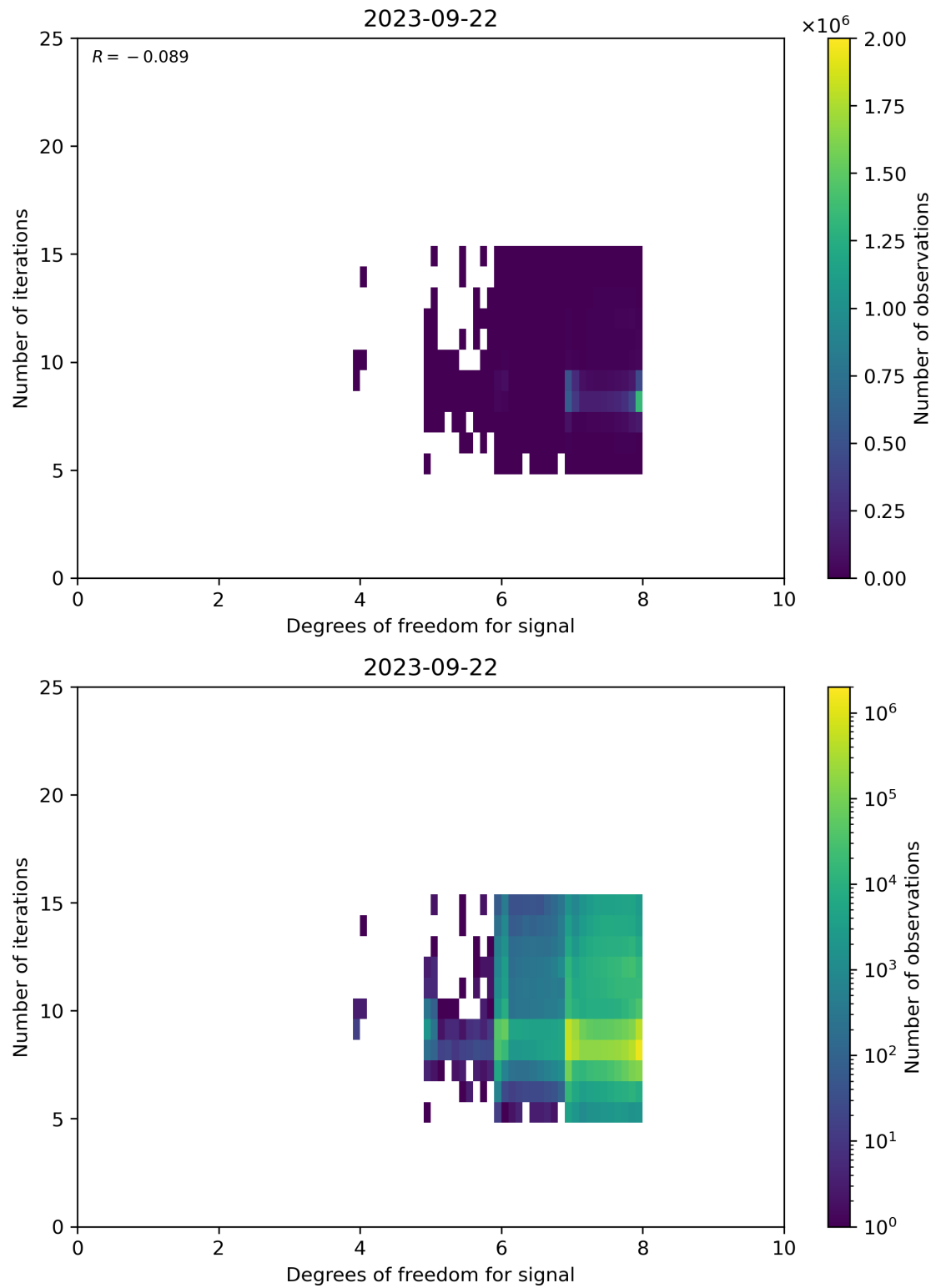
Figure 50: Scatter density plot of “Degrees of freedom for signal” against “Number of iterations” for 2023-09-21 to 2023-09-23.
