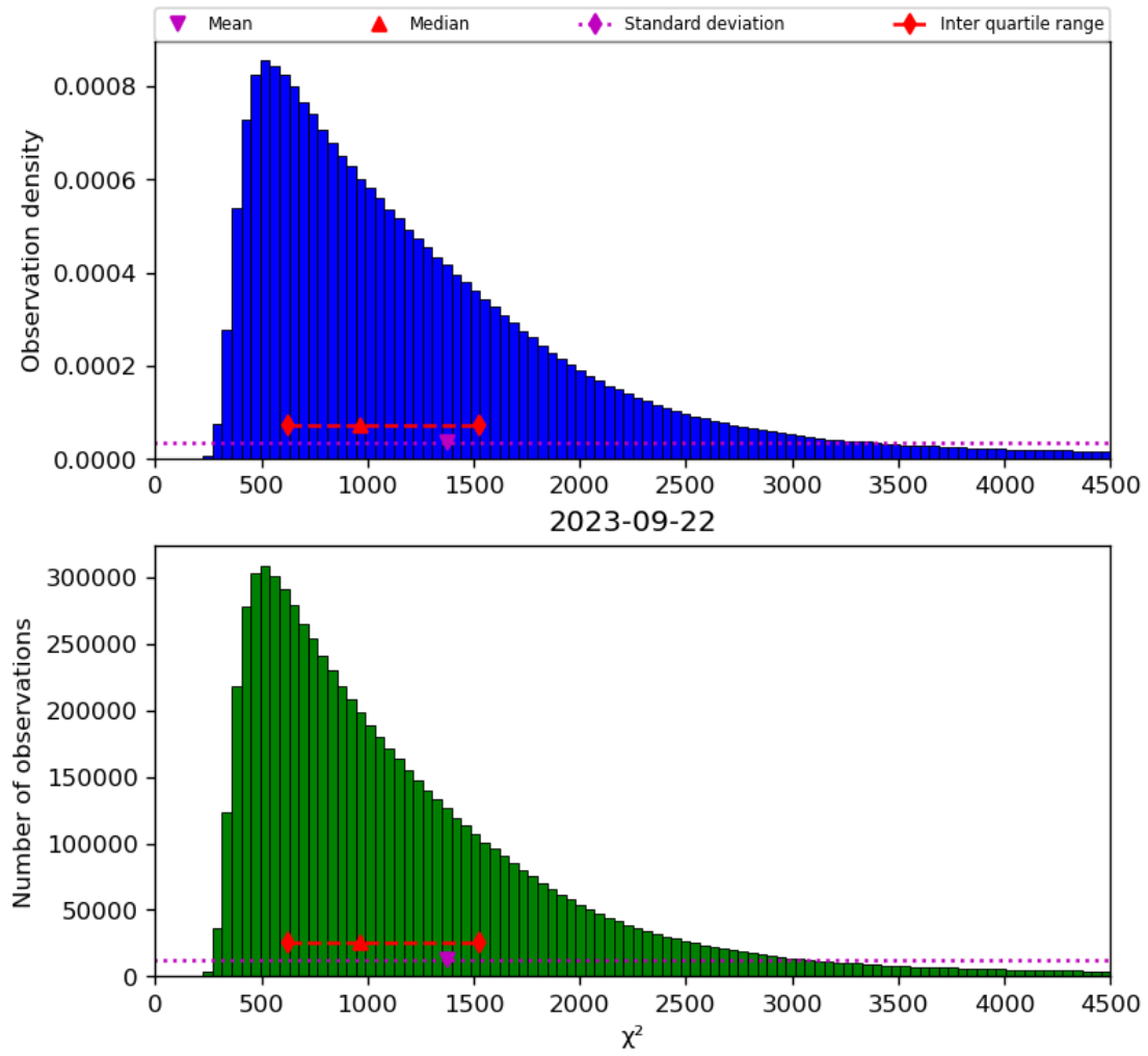
Figure 22: Histogram of “ \chi^2 ” for 2023-09-21 to 2023-09-23
