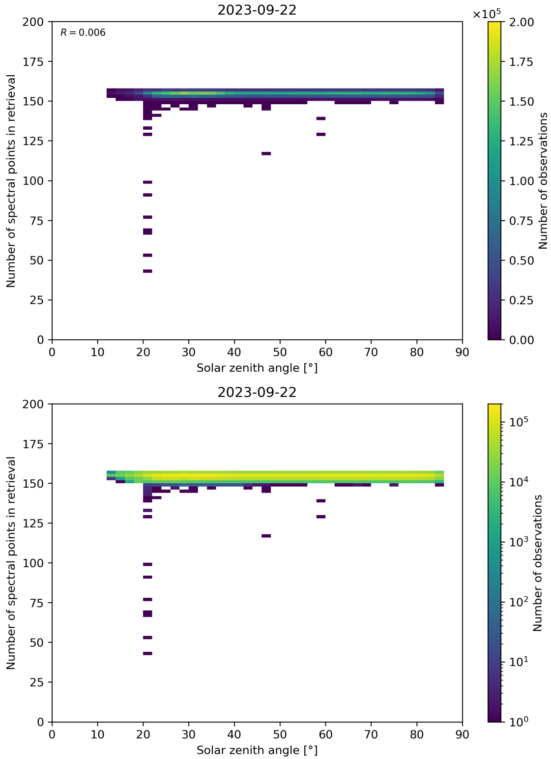
Figure 68: Scatter density plot of “Solar zenith angle” against “Number of spectral points in retrieval” for 2023-09-21 to 2023-09-23.
