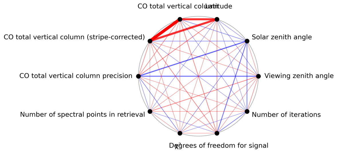
Figure 1: Map of correlation graph for 2023-09-21 to 2023-09-23.
