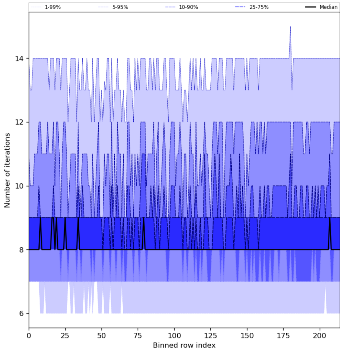
Figure 32: Along track statistics of “Number of iterations” for 2023-09-21 to 2023-09-23
