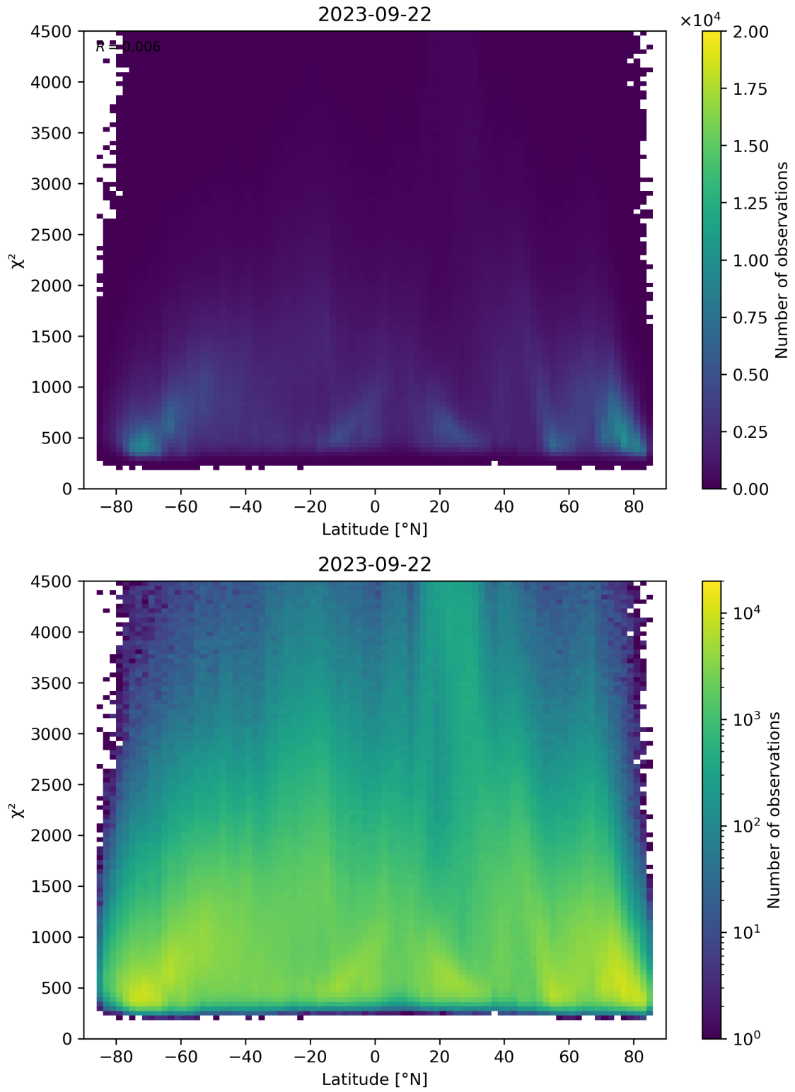
Figure 54: Scatter density plot of “Latitude” against “ \chi^2 ” for 2023-09-21 to 2023-09-23.
