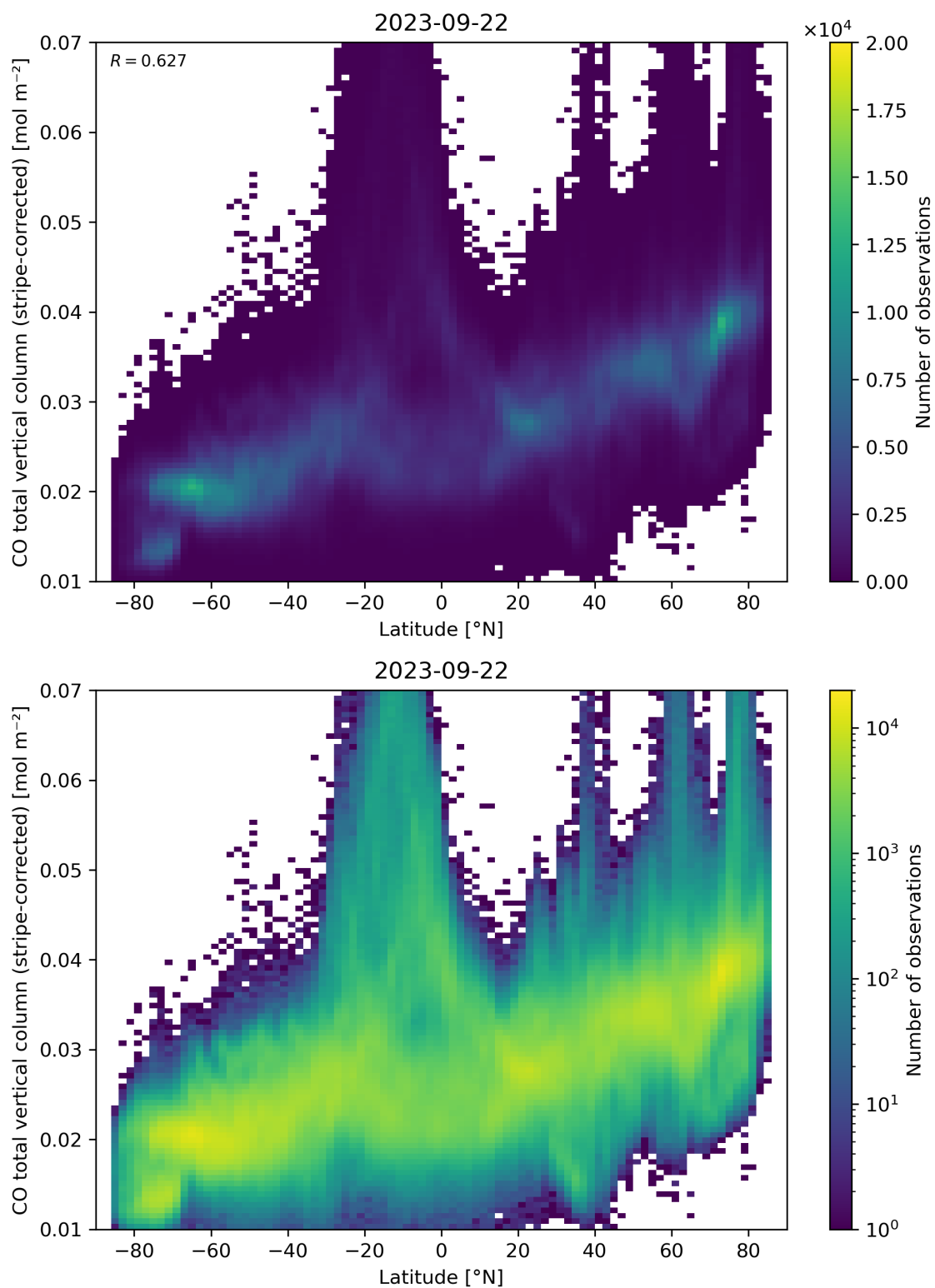
Figure 52: Scatter density plot of “Latitude” against “CO total vertical column (stripe-corrected)” for 2023-09-21 to 2023-09-23.
