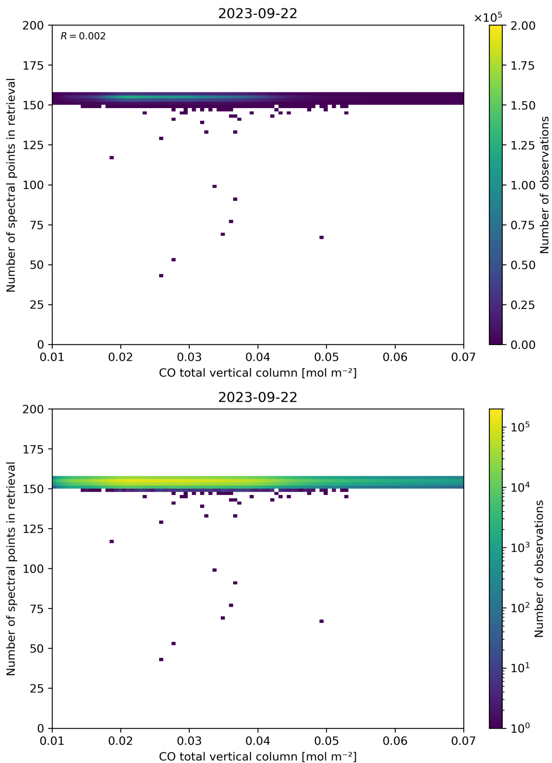
Figure 43: Scatter density plot of “CO total vertical column” against “Number of spectral points in retrieval” for 2023-09-21 to 2023-09-23.
