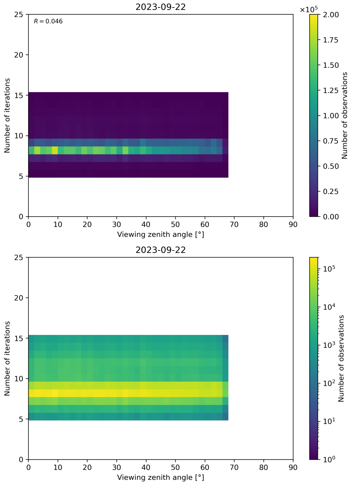
Figure 75: Scatter density plot of “Viewing zenith angle” against “Number of iterations” for 2023-09-21 to 2023-09-23.
