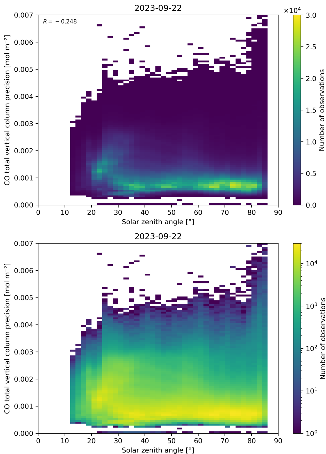
Figure 63: Scatter density plot of “Solar zenith angle” against “CO total vertical column precision” for 2023-09-21 to 2023-09-23.
