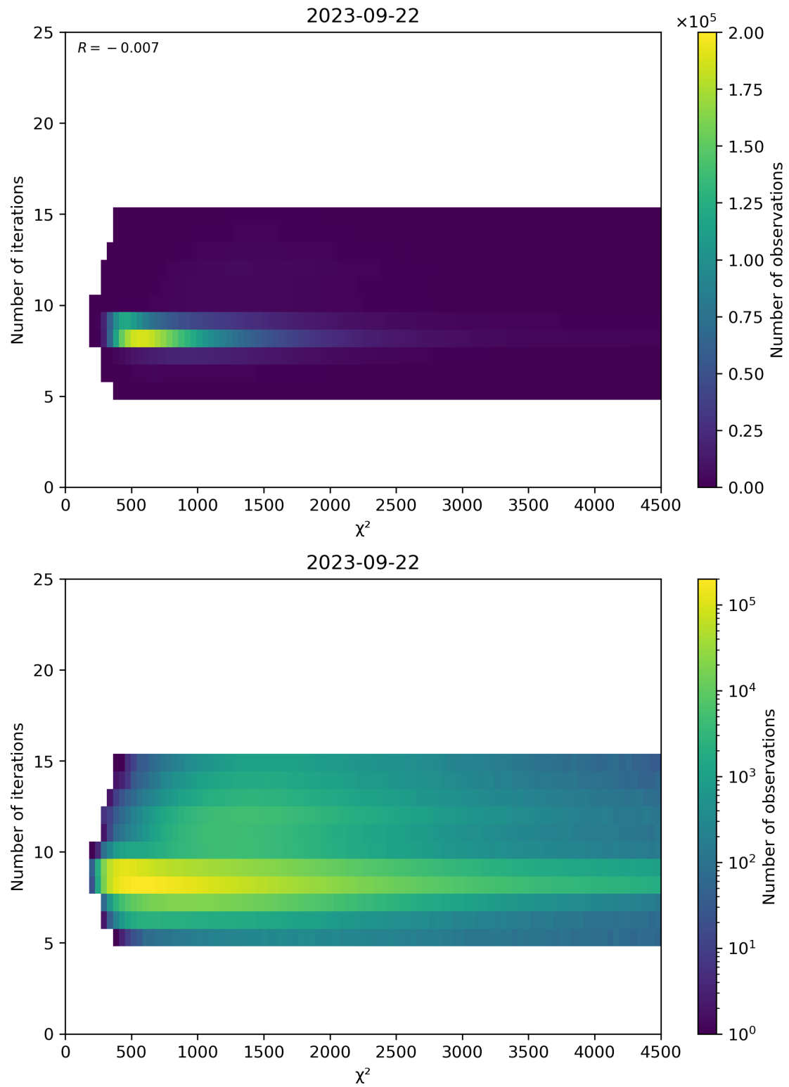
Figure 49: Scatter density plot of “ \chi^2 ” against “Number of iterations” for 2023-09-21 to 2023-09-23.
