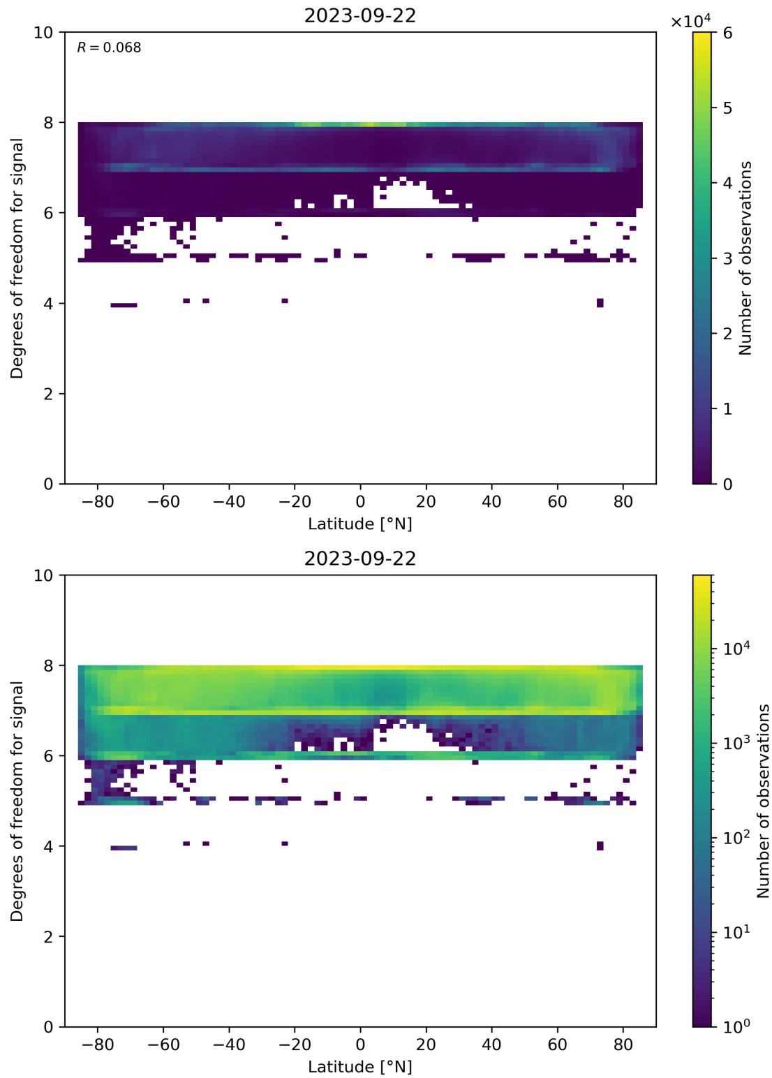
Figure 55: Scatter density plot of “Latitude” against “Degrees of freedom for signal” for 2023-09-21 to 2023-09-23.
