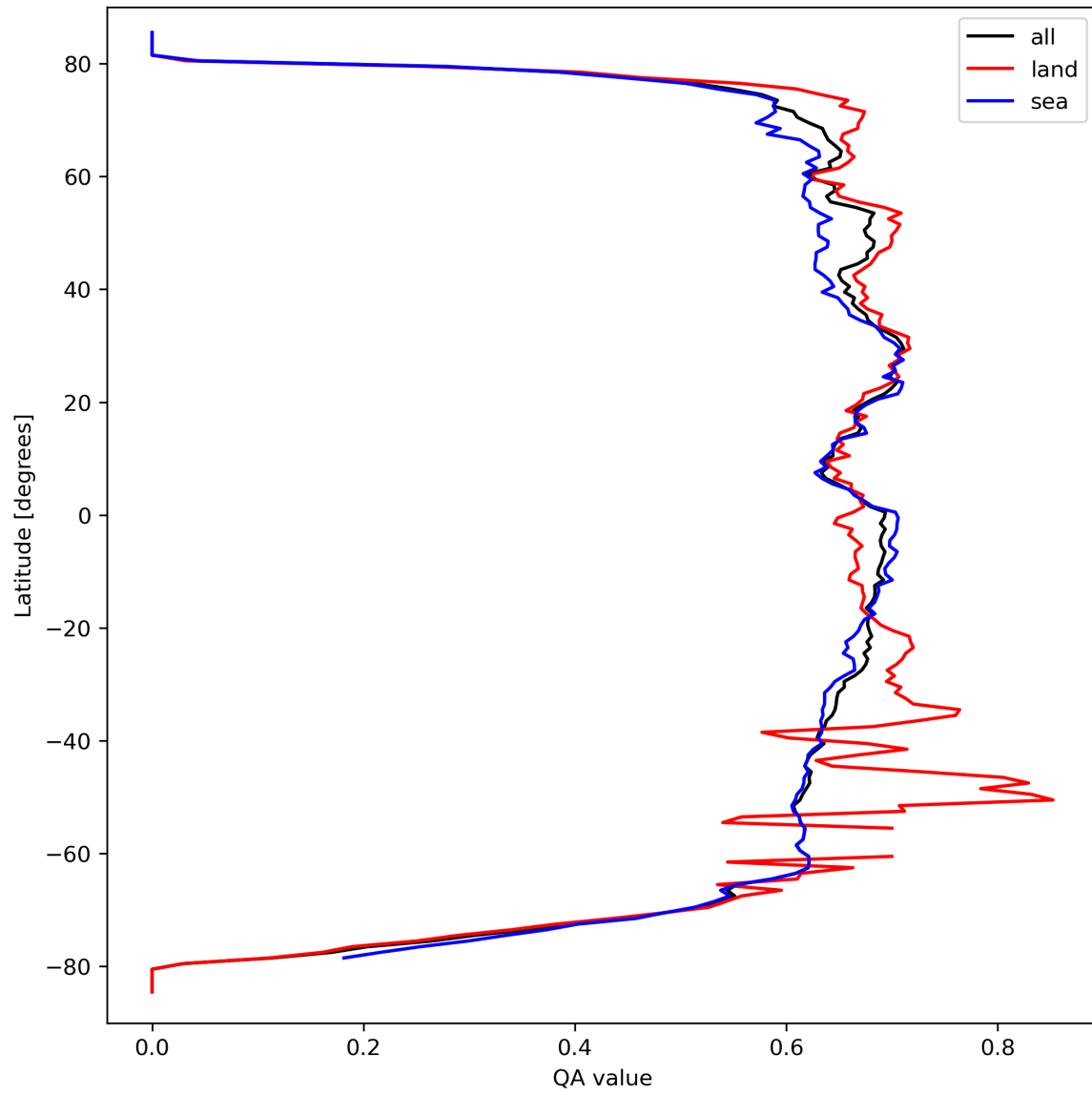
Figure 9: Zonal average of “QA value” for 2023-09-21 to 2023-09-23.
