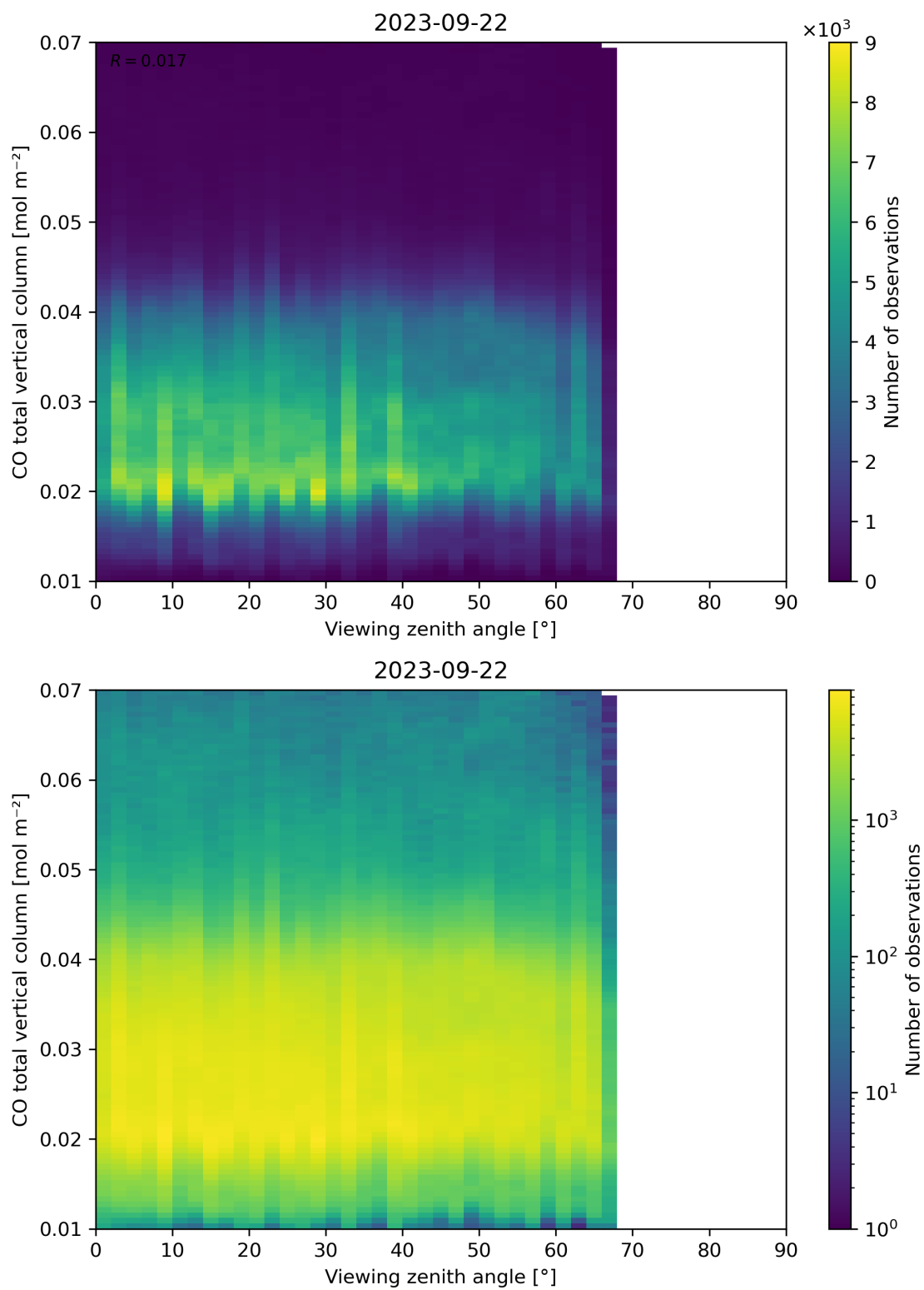
Figure 69: Scatter density plot of “Viewing zenith angle” against “CO total vertical column” for 2023-09-21 to 2023-09-23.
