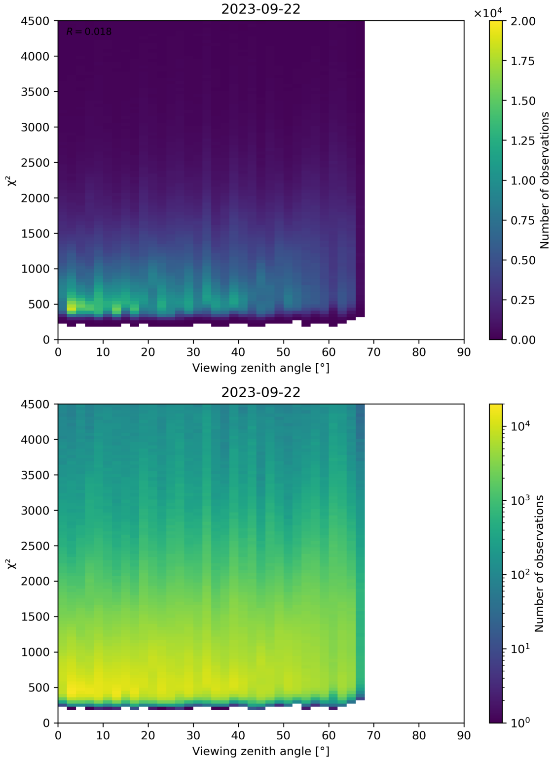
Figure 72: Scatter density plot of “Viewing zenith angle” against “ \chi^2 ” for 2023-09-21 to 2023-09-23.
