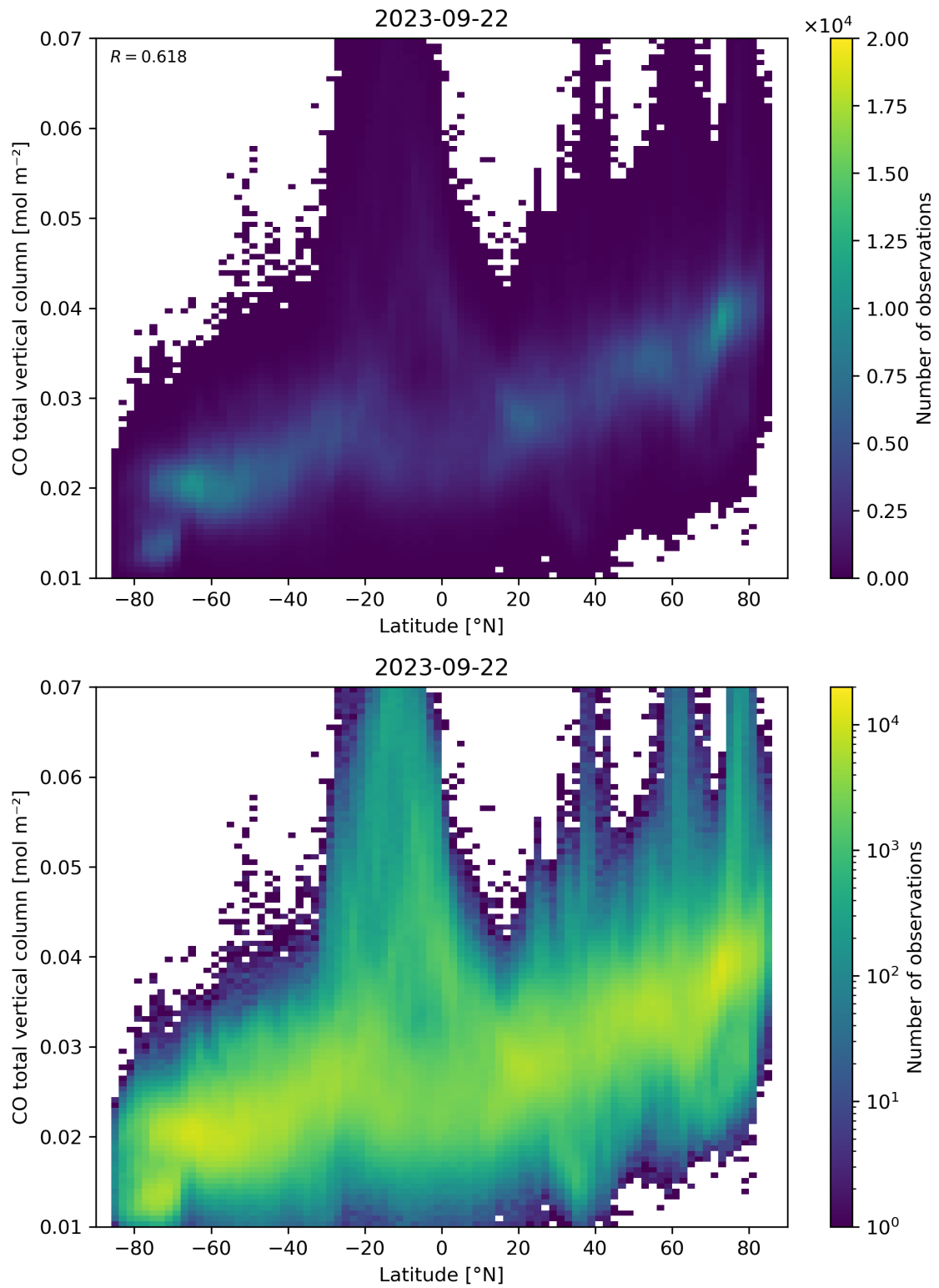
Figure 51: Scatter density plot of “Latitude” against “CO total vertical column” for 2023-09-21 to 2023-09-23.
