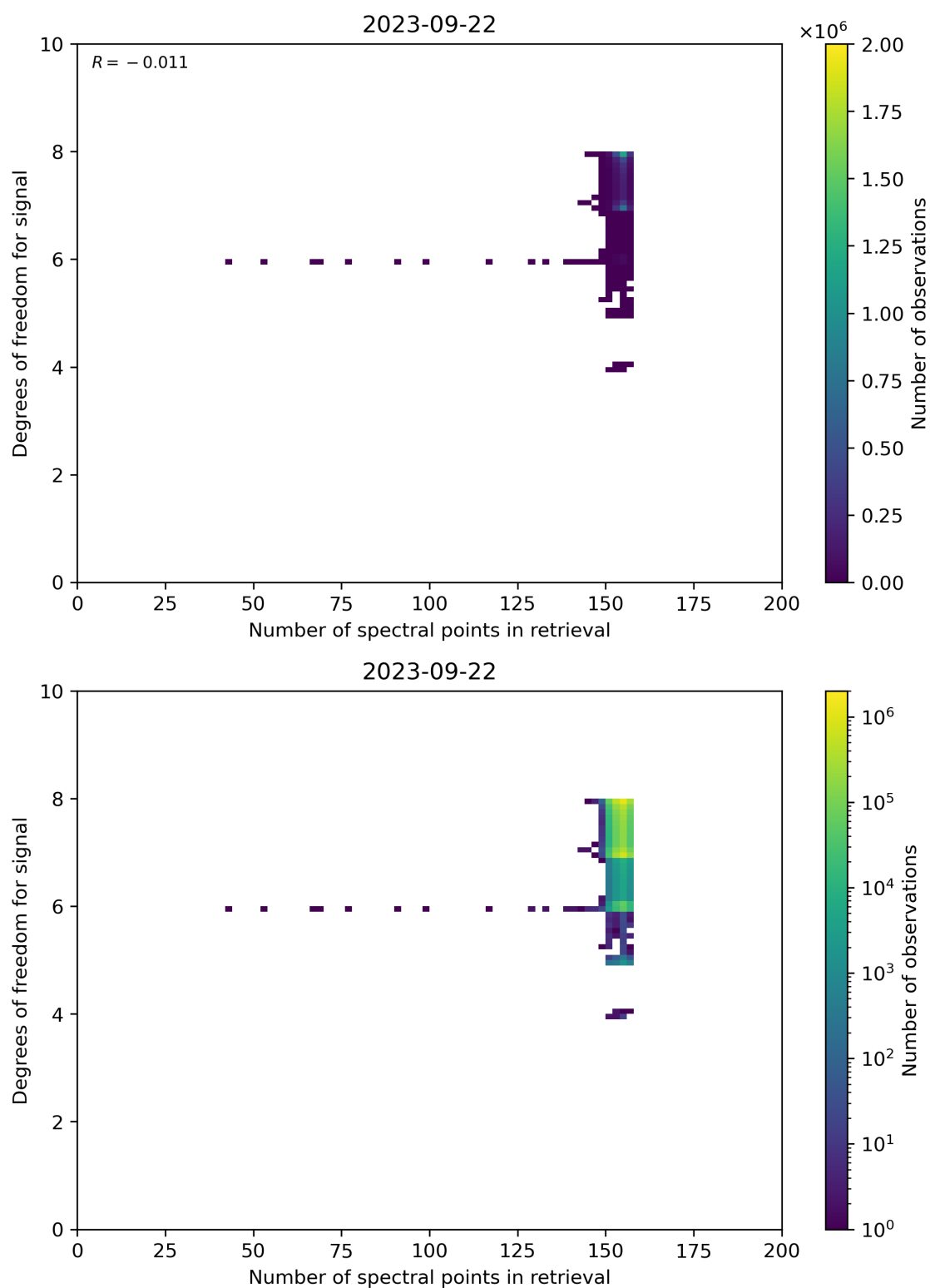
Figure 59: Scatter density plot of “Number of spectral points in retrieval” against “Degrees of freedom for signal” for 2023-09-21 to 2023-09-23.
