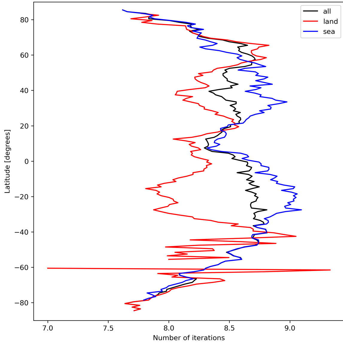
Figure 16: Zonal average of “Number of iterations” for 2023-09-21 to 2023-09-23.
