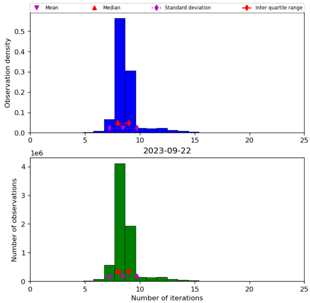
Figure 24: Histogram of “Number of iterations” for 2023-09-21 to 2023-09-23
