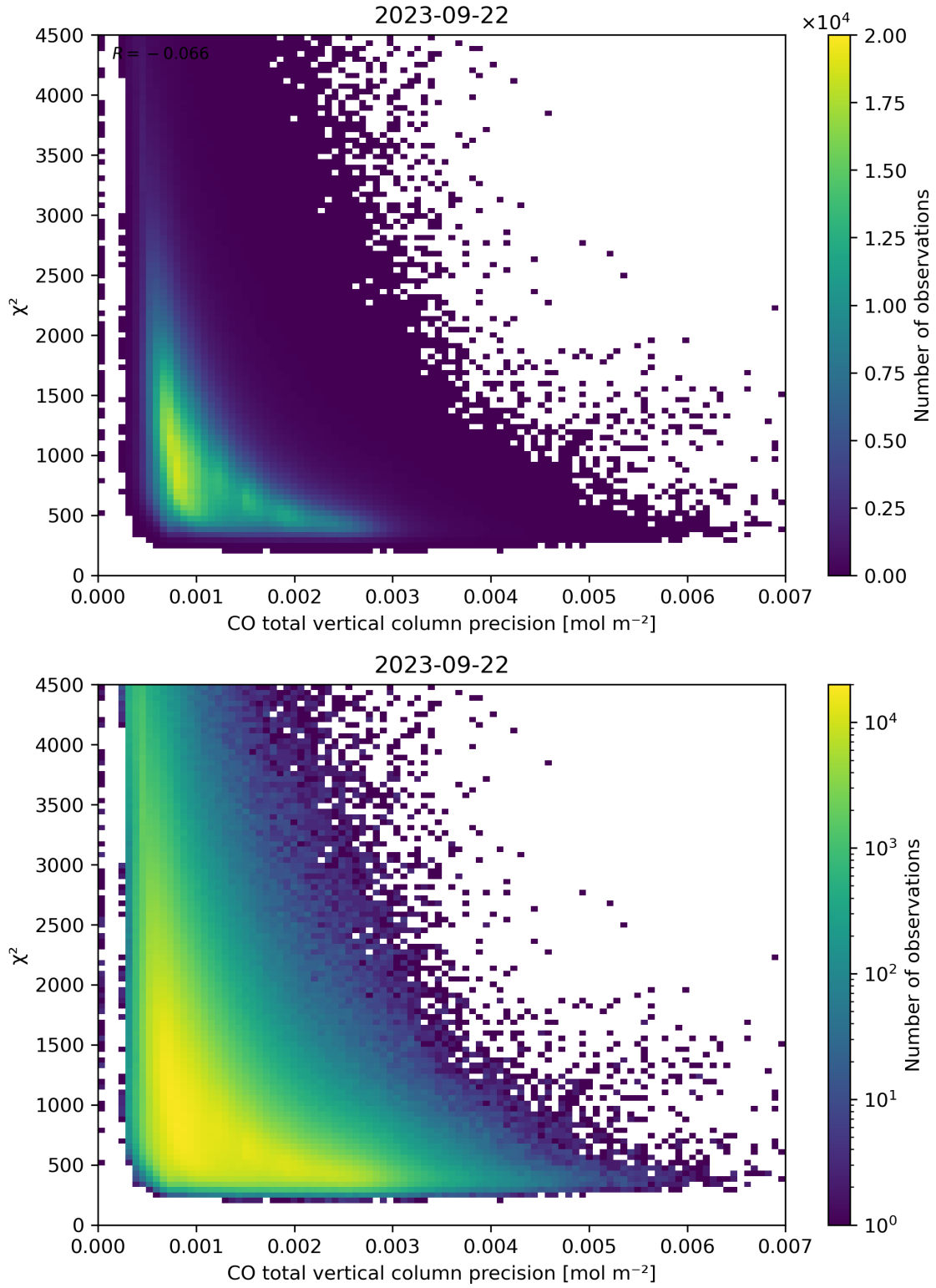
Figure 44: Scatter density plot of “CO total vertical column precision” against “ \chi^2 ” for 2023-09-21 to 2023-09-23.
