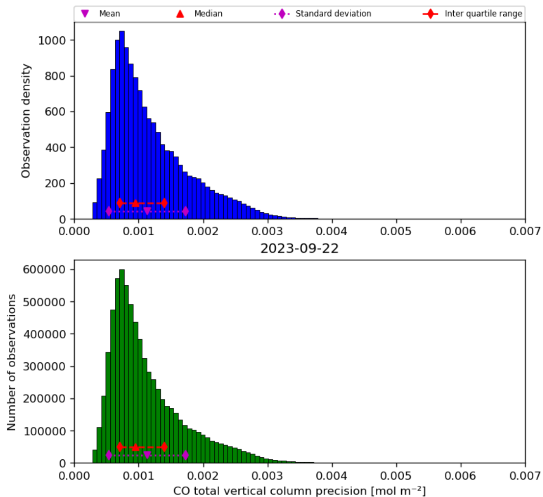
Figure 20: Histogram of “CO total vertical column precision” for 2023-09-21 to 2023-09-23
