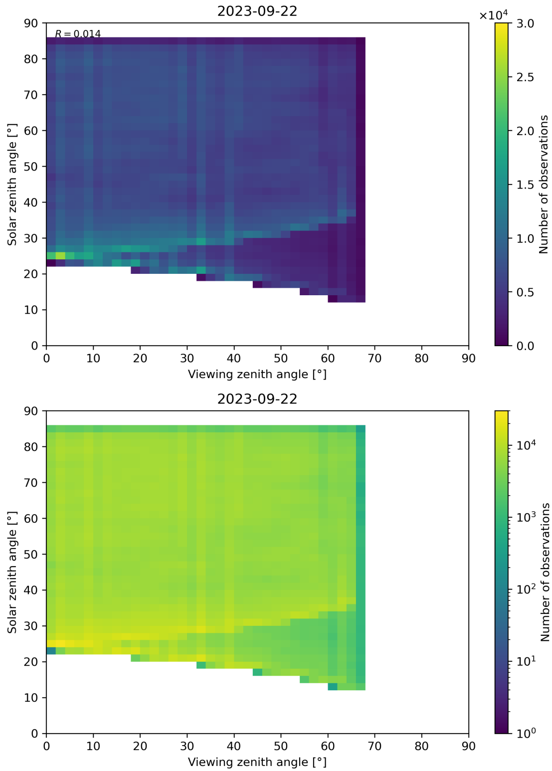
Figure 77: Scatter density plot of “Viewing zenith angle” against “Solar zenith angle” for 2023-09-21 to 2023-09-23.
