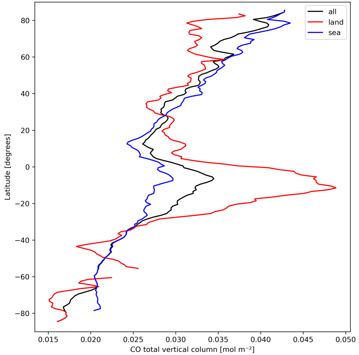
Figure 10: Zonal average of “CO total vertical column” for 2023-09-21 to 2023-09-23.
