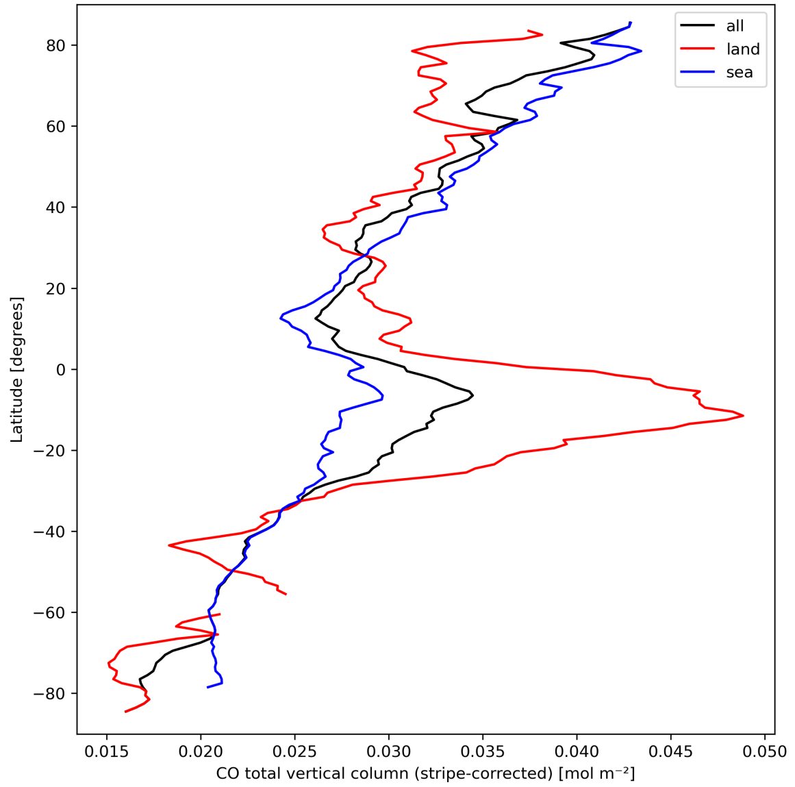
Figure 11: Zonal average of “CO total vertical column (stripe-corrected)” for 2023-09-21 to 2023-09-23.
