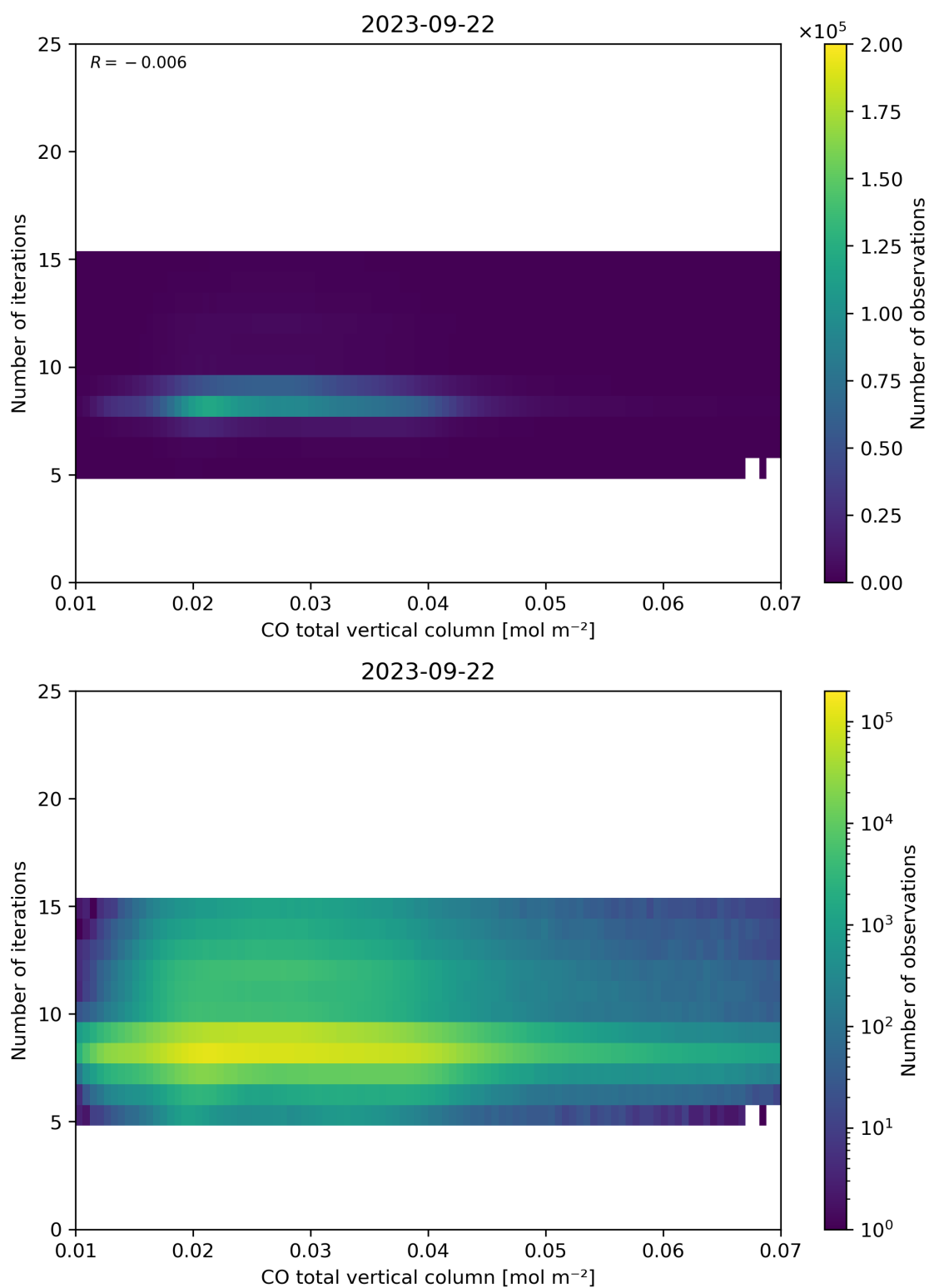
Figure 42: Scatter density plot of “CO total vertical column” against “Number of iterations” for 2023-09-21 to 2023-09-23.
