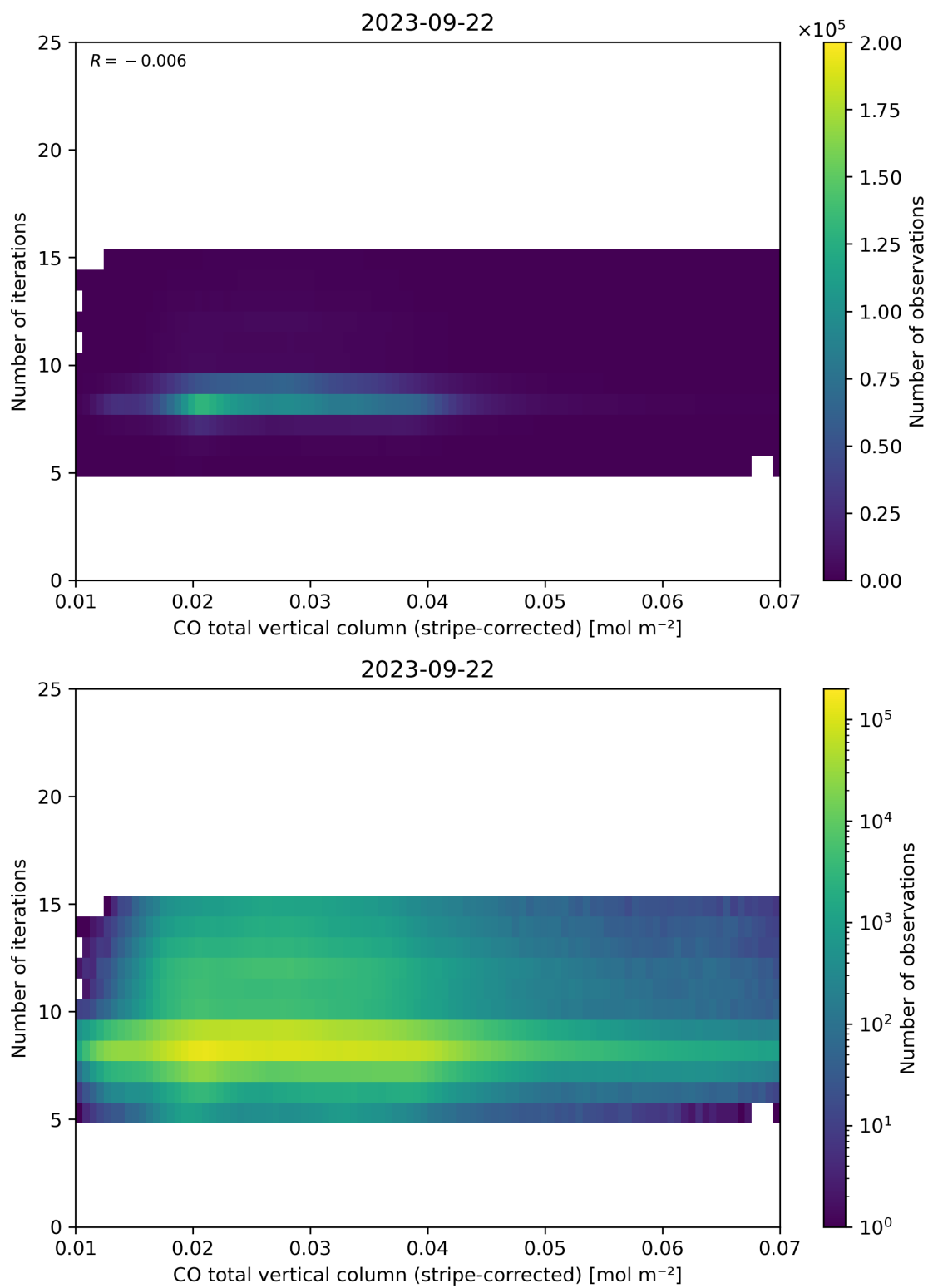
Figure 39: Scatter density plot of “CO total vertical column (stripe-corrected)” against “Number of iterations” for 2023-09-21 to 2023-09-23.
