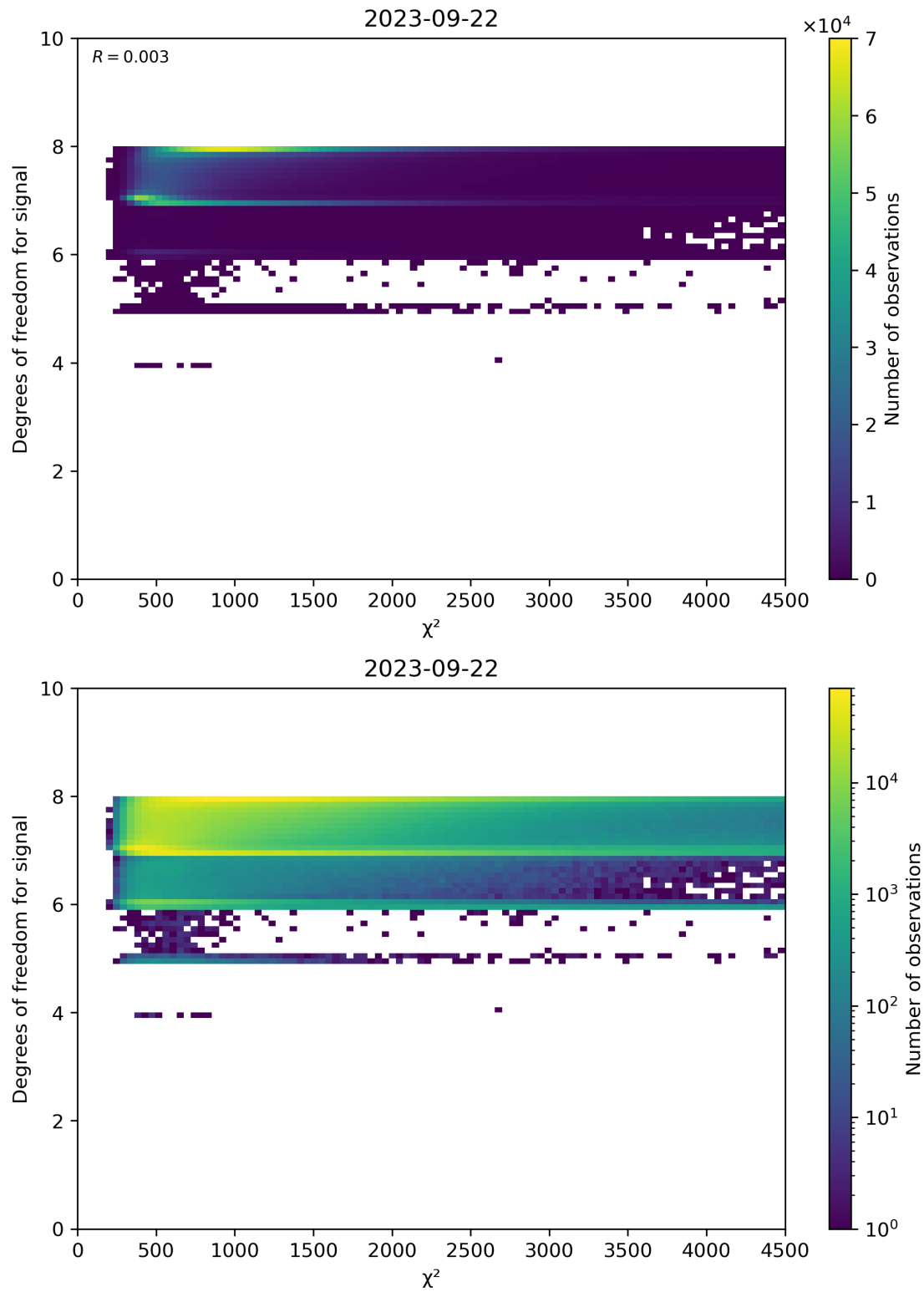
Figure 48: Scatter density plot of “ \chi^2 ” against “Degrees of freedom for signal” for 2023-09-21 to 2023-09-23.
