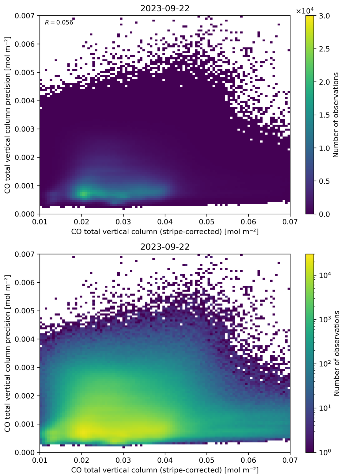
Figure 36: Scatter density plot of “CO total vertical column (stripe-corrected)” against “CO total vertical column precision” for 2023-09-21 to 2023-09-23.
