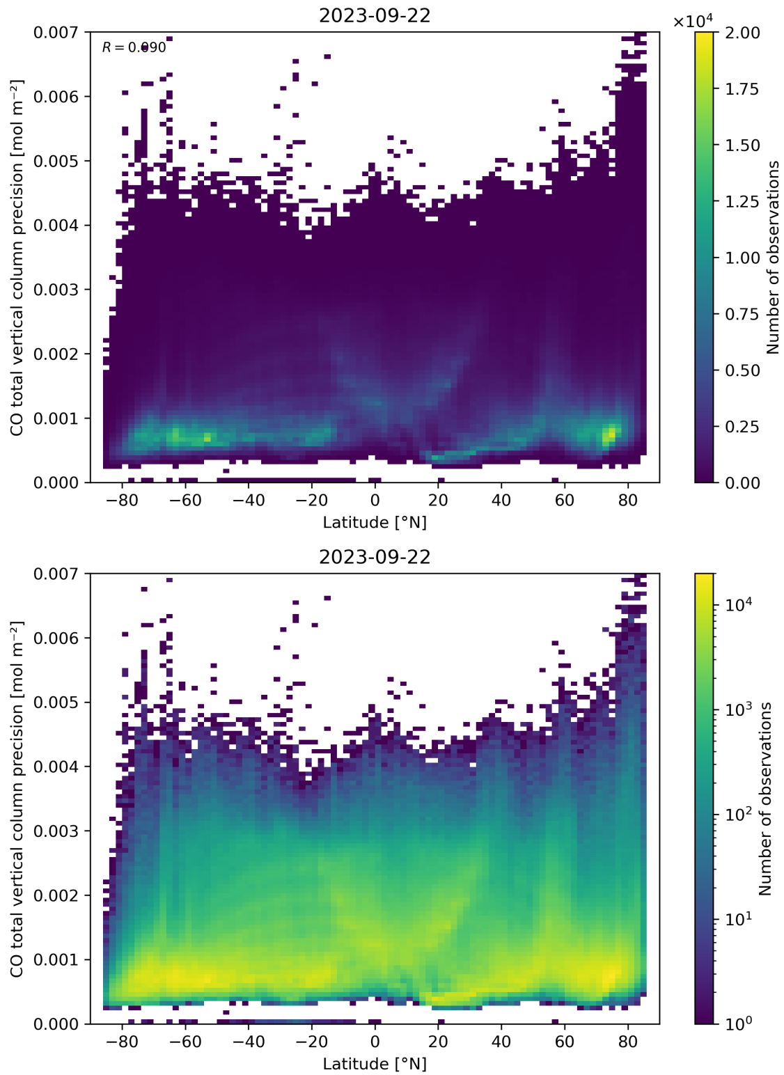
Figure 53: Scatter density plot of “Latitude” against “CO total vertical column precision” for 2023-09-21 to 2023-09-23.
