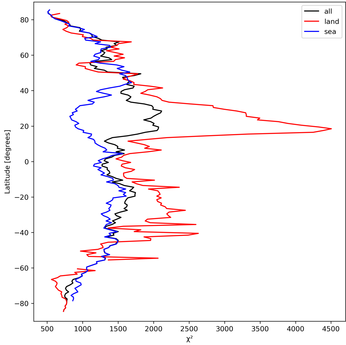
Figure 14: Zonal average of “ \chi^2 ” for 2023-09-21 to 2023-09-23.
