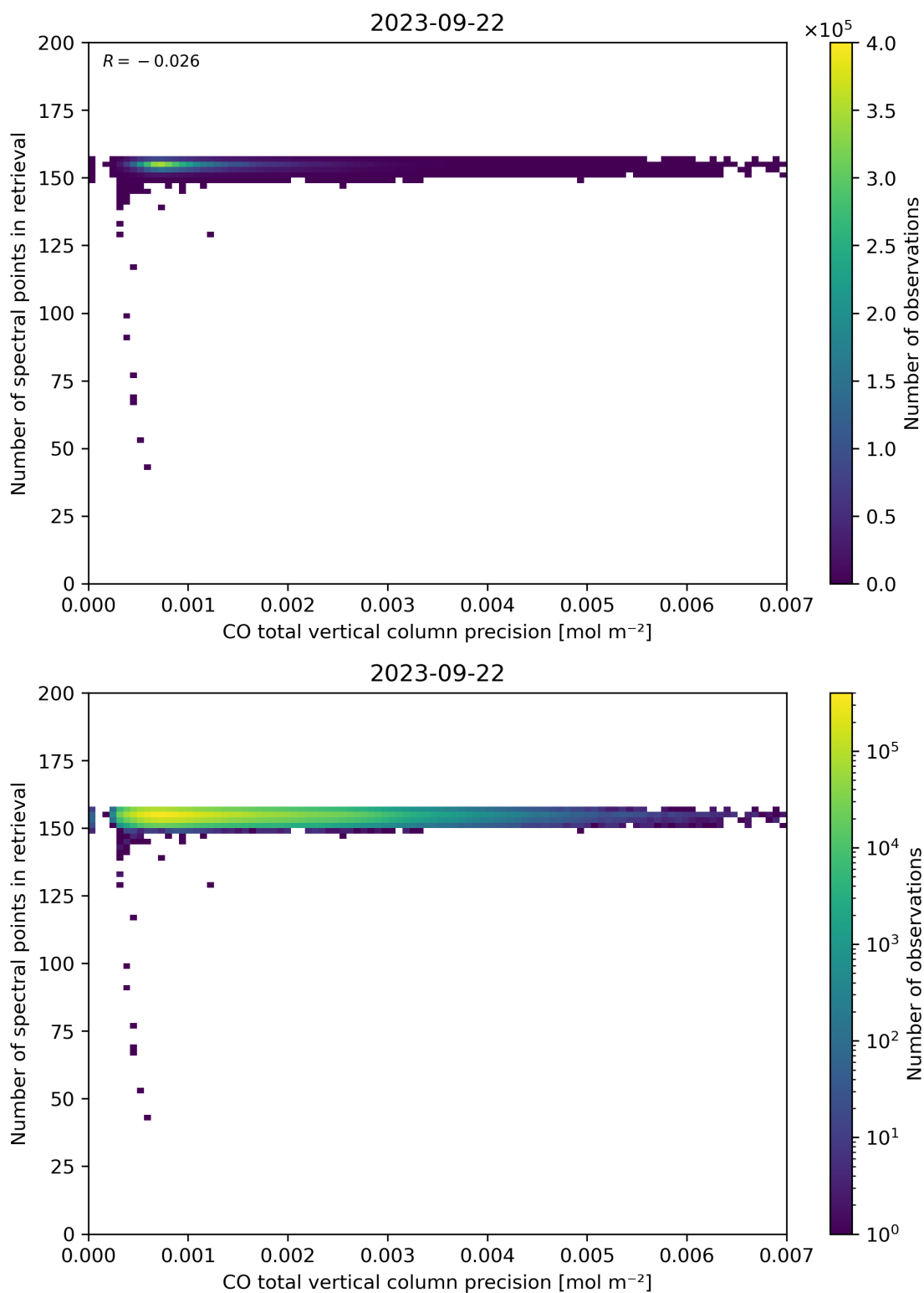
Figure 47: Scatter density plot of “CO total vertical column precision” against “Number of spectral points in retrieval” for 2023-09-21 to 2023-09-23.
