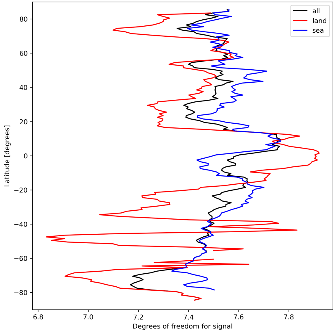
Figure 15: Zonal average of “Degrees of freedom for signal” for 2023-09-21 to 2023-09-23.
