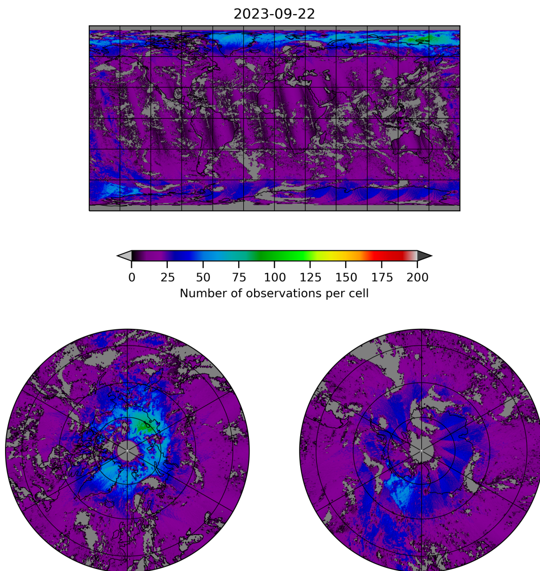
Figure 8: Map of the number of observations for 2023-09-21 to 2023-09-23
