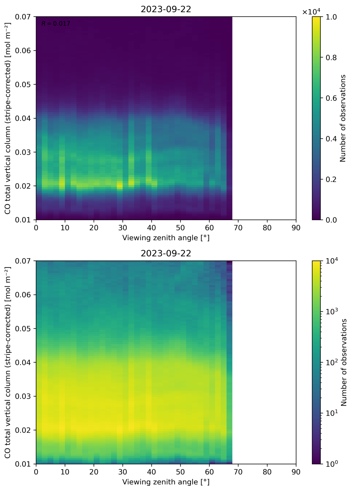
Figure 70: Scatter density plot of “Viewing zenith angle” against “CO total vertical column (stripe-corrected)” for 2023-09-21 to 2023-09-23.
