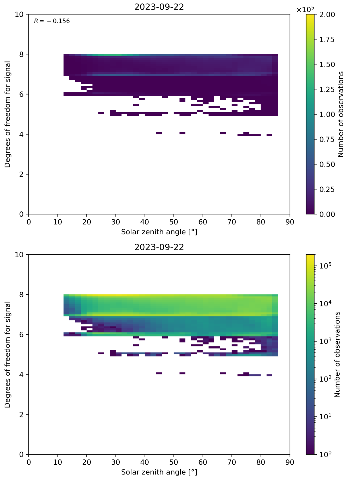
Figure 65: Scatter density plot of “Solar zenith angle” against “Degrees of freedom for signal” for 2023-09-21 to 2023-09-23.
