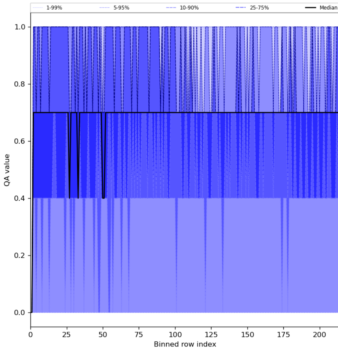
Figure 25: Along track statistics of “QA value” for 2023-09-21 to 2023-09-23
