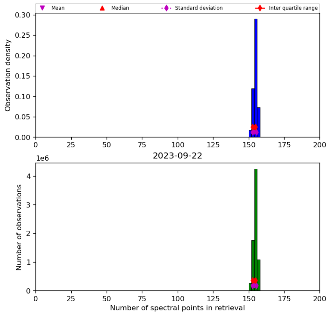
Figure 21: Histogram of “Number of spectral points in retrieval” for 2023-09-21 to 2023-09-23
