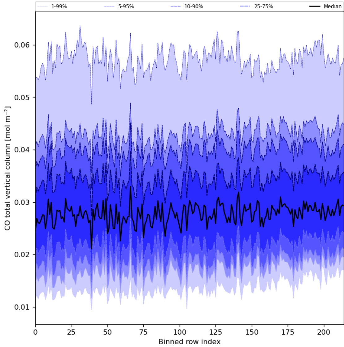
Figure 26: Along track statistics of “CO total vertical column” for 2023-09-21 to 2023-09-23
