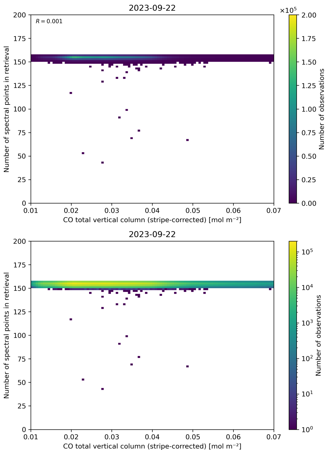
Figure 40: Scatter density plot of “CO total vertical column (stripe-corrected)” against “Number of spectral points in retrieval” for 2023-09-21 to 2023-09-23.
