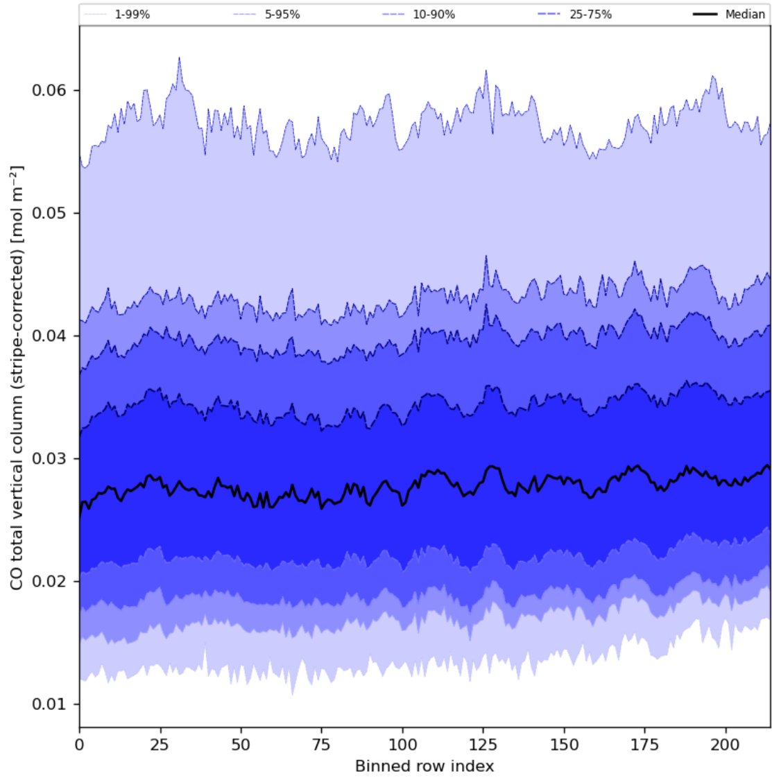
Figure 27: Along track statistics of “CO total vertical column (stripe-corrected)” for 2023-09-21 to 2023-09-23
