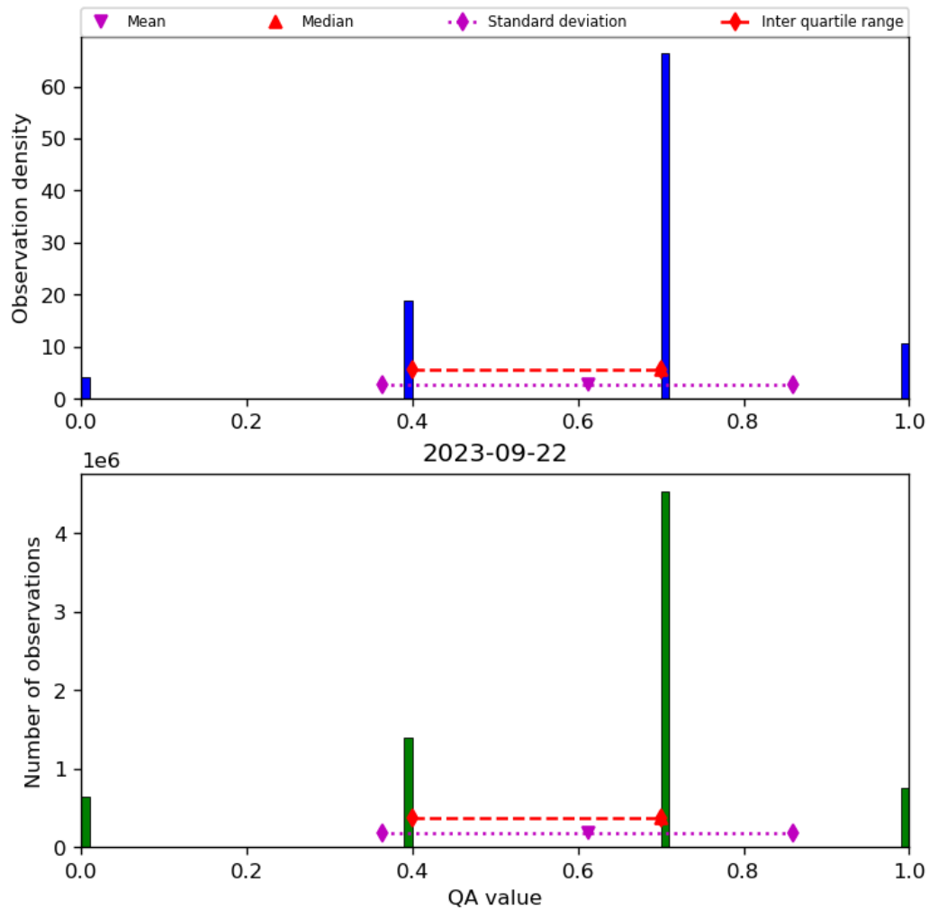
Figure 17: Histogram of “QA value” for 2023-09-21 to 2023-09-23
