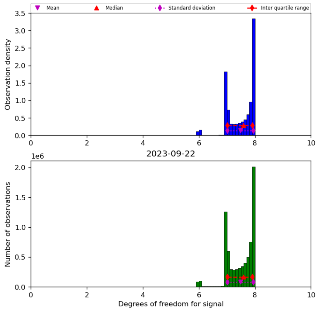
Figure 23: Histogram of “Degrees of freedom for signal” for 2023-09-21 to 2023-09-23
