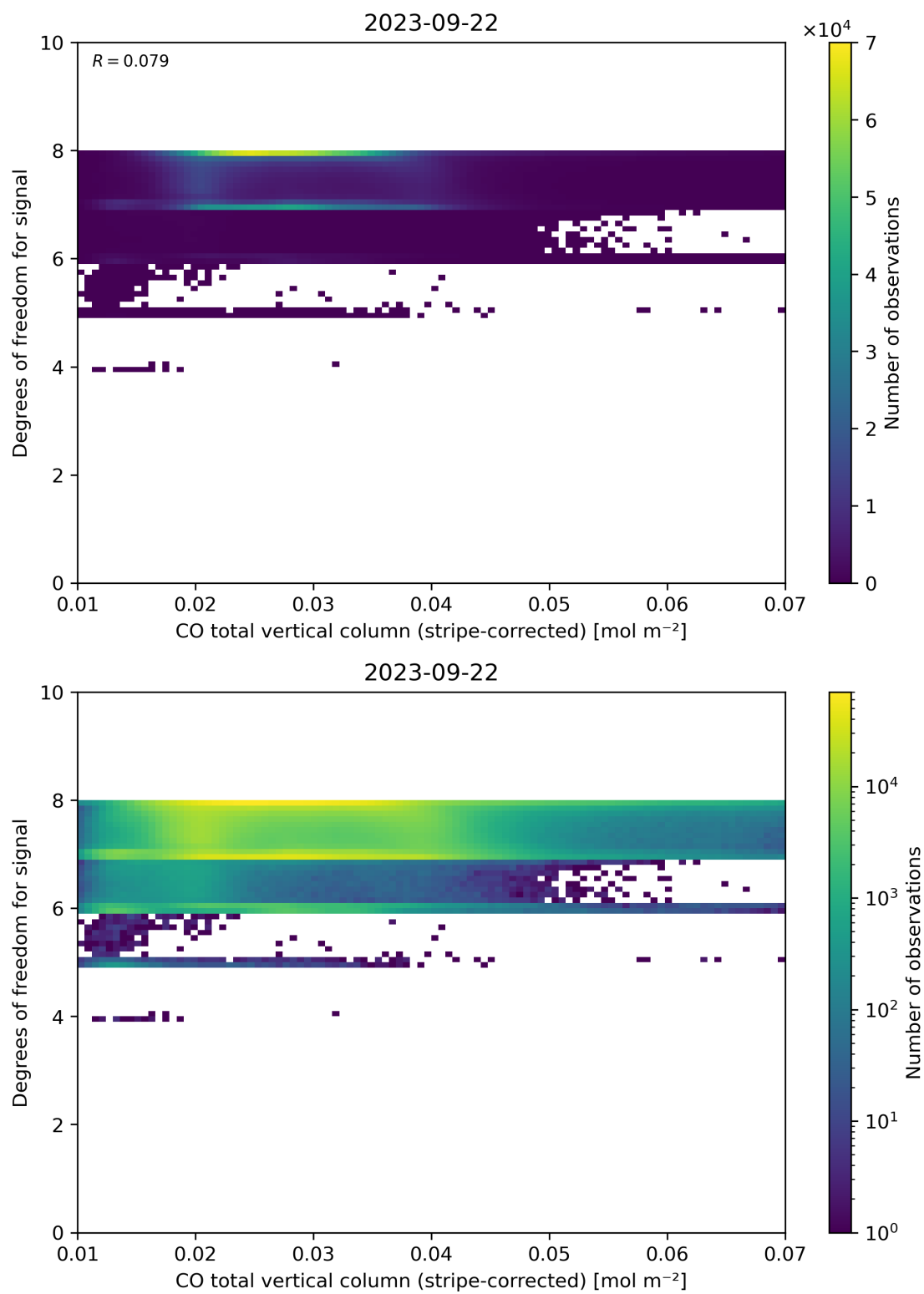
Figure 38: Scatter density plot of “CO total vertical column (stripe-corrected)” against “Degrees of freedom for signal” for 2023-09-21 to 2023-09-23.
