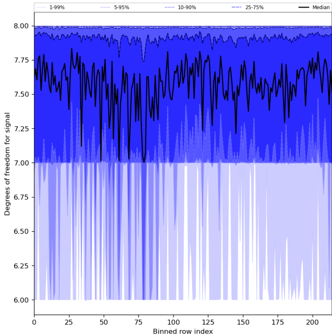
Figure 31: Along track statistics of “Degrees of freedom for signal” for 2023-09-21 to 2023-09-23
