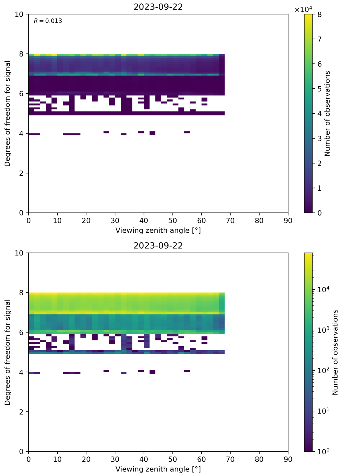
Figure 73: Scatter density plot of “Viewing zenith angle” against “Degrees of freedom for signal” for 2023-09-21 to 2023-09-23.
