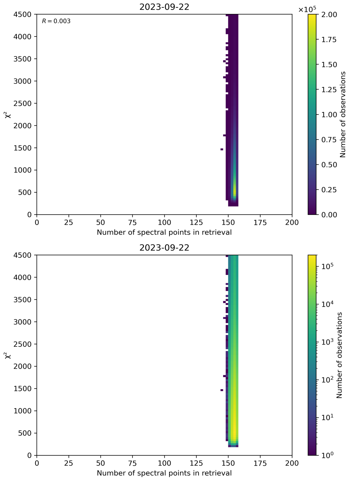
Figure 58: Scatter density plot of “Number of spectral points in retrieval” against “ \chi^2 ” for 2023-09-21 to 2023-09-23.
