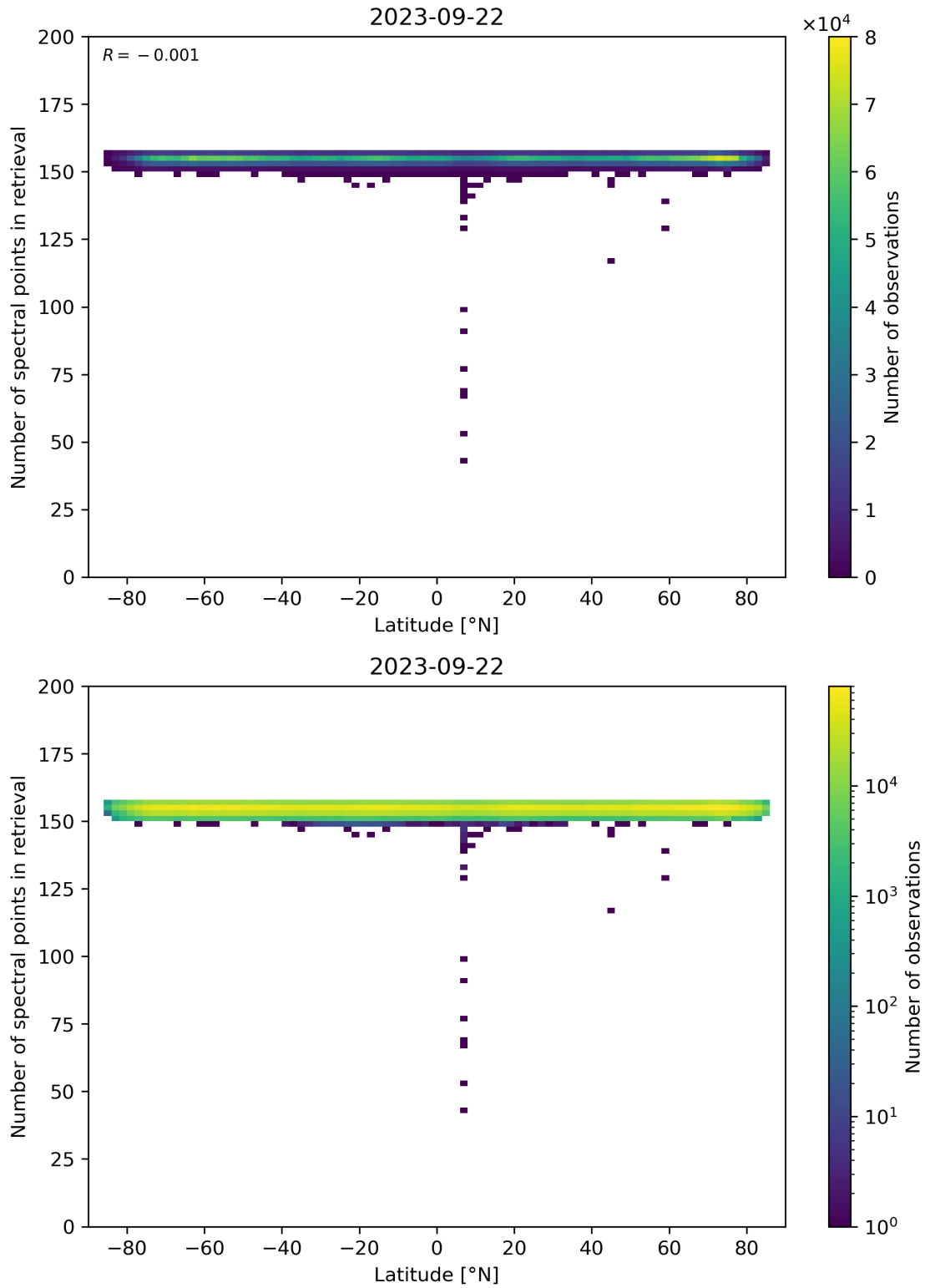
Figure 57: Scatter density plot of “Latitude” against “Number of spectral points in retrieval” for 2023-09-21 to 2023-09-23.
