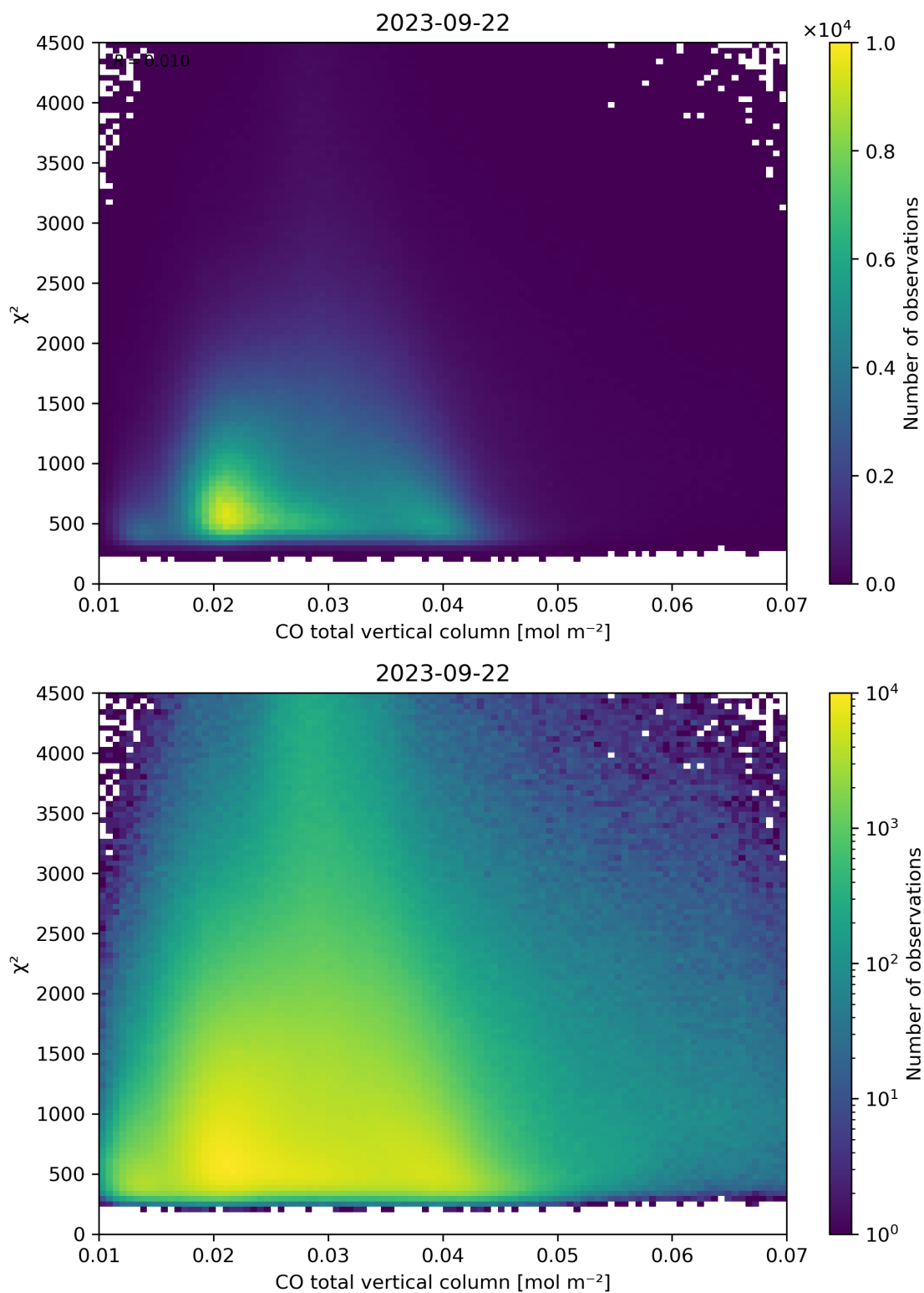
Figure 35: Scatter density plot of “CO total vertical column” against “ \chi^2 ” for 2023-09-21 to 2023-09-23.
