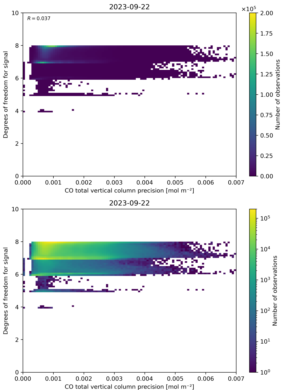
Figure 45: Scatter density plot of “CO total vertical column precision” against “Degrees of freedom for signal” for 2023-09-21 to 2023-09-23.
