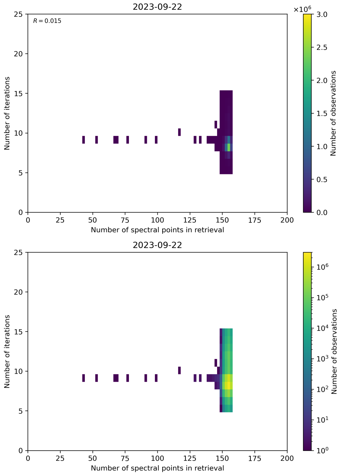
Figure 60: Scatter density plot of “Number of spectral points in retrieval” against “Number of iterations” for 2023-09-21 to 2023-09-23.
