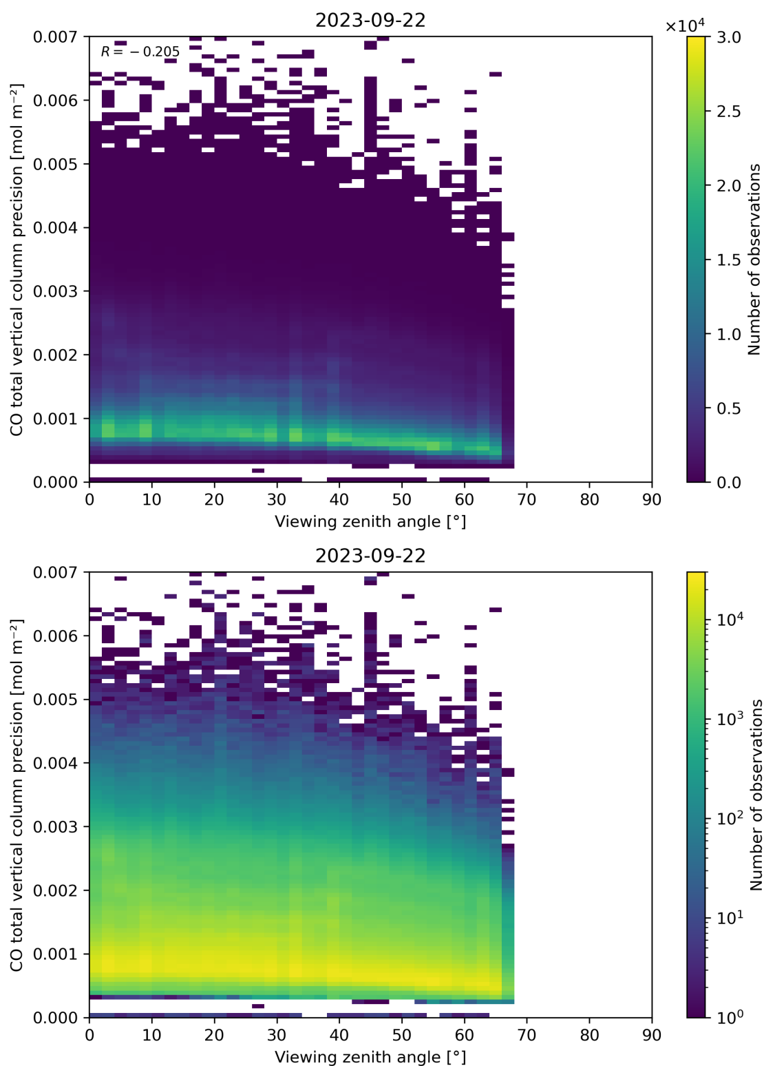
Figure 71: Scatter density plot of “Viewing zenith angle” against “CO total vertical column precision” for 2023-09-21 to 2023-09-23.
