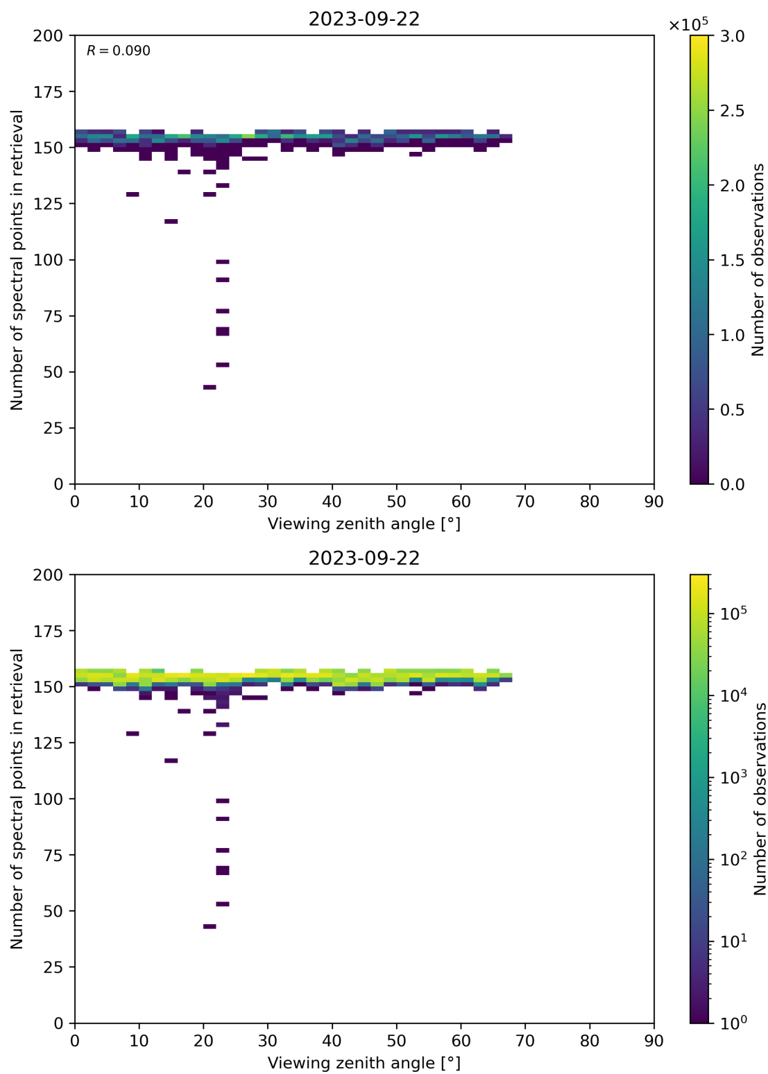
Figure 76: Scatter density plot of “Viewing zenith angle” against “Number of spectral points in retrieval” for 2023-09-21 to 2023-09-23.
