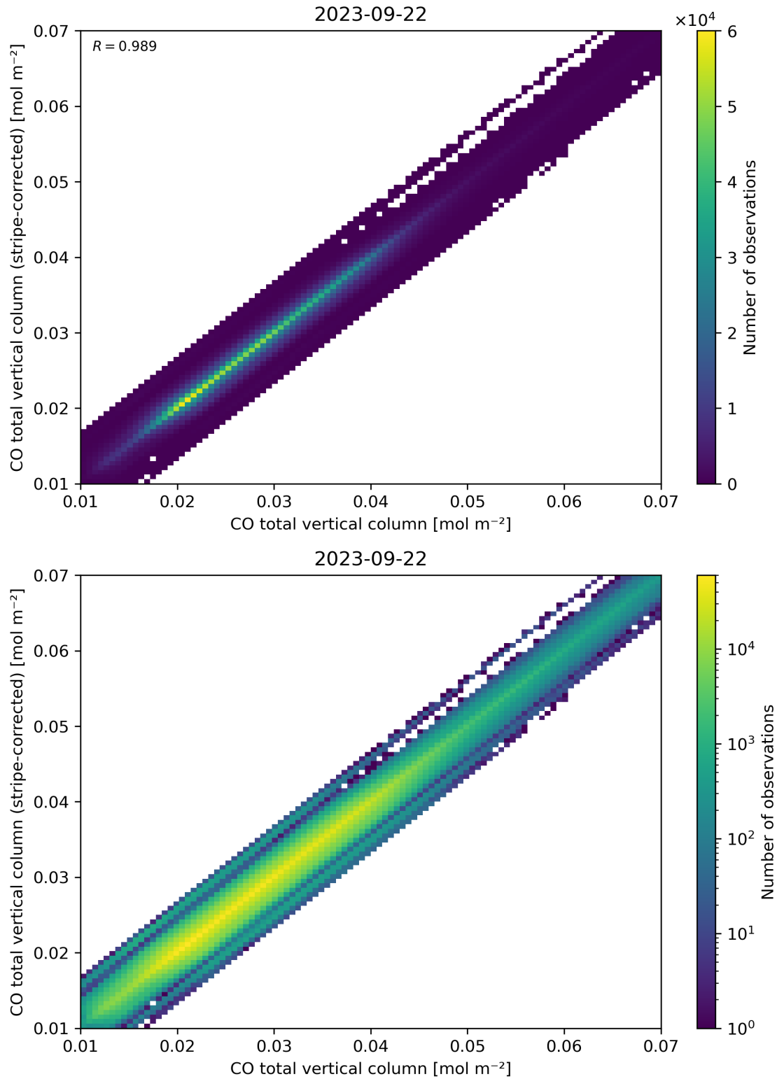
Figure 33: Scatter density plot of “CO total vertical column” against “CO total vertical column (stripe-corrected)” for 2023-09-21 to 2023-09-23.
