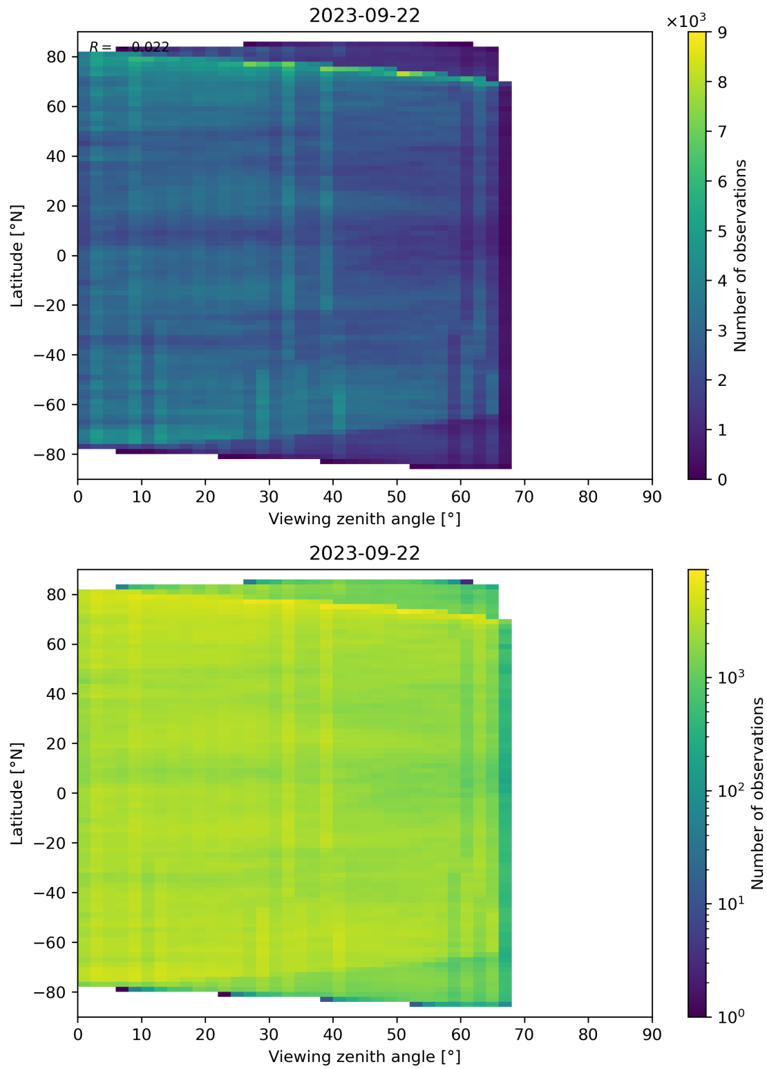
Figure 74: Scatter density plot of “Viewing zenith angle” against “Latitude” for 2023-09-21 to 2023-09-23.
