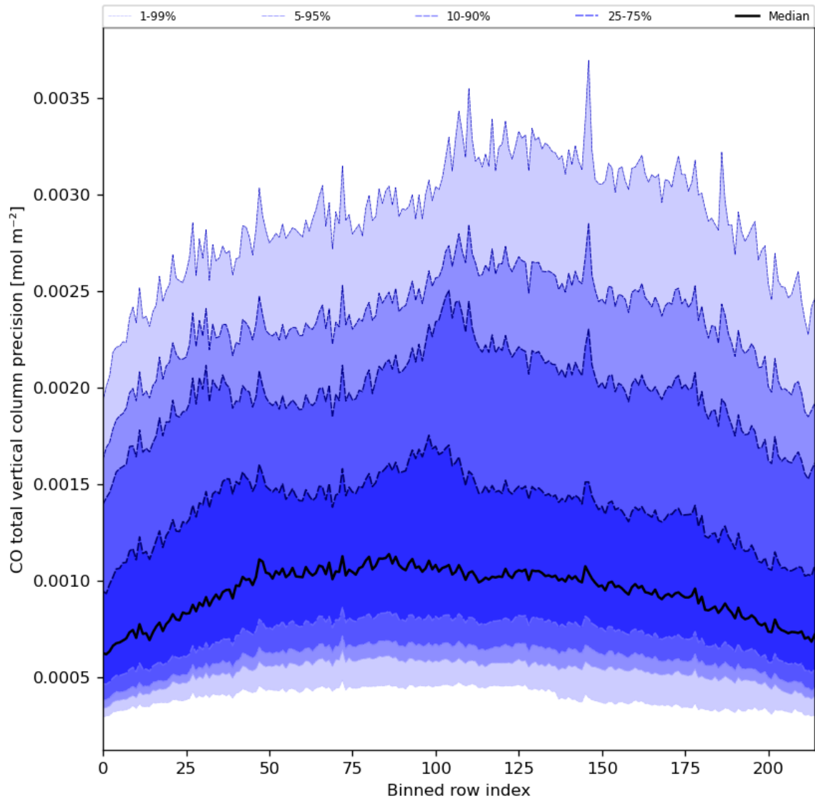
Figure 28: Along track statistics of “CO total vertical column precision” for 2023-09-21 to 2023-09-23
