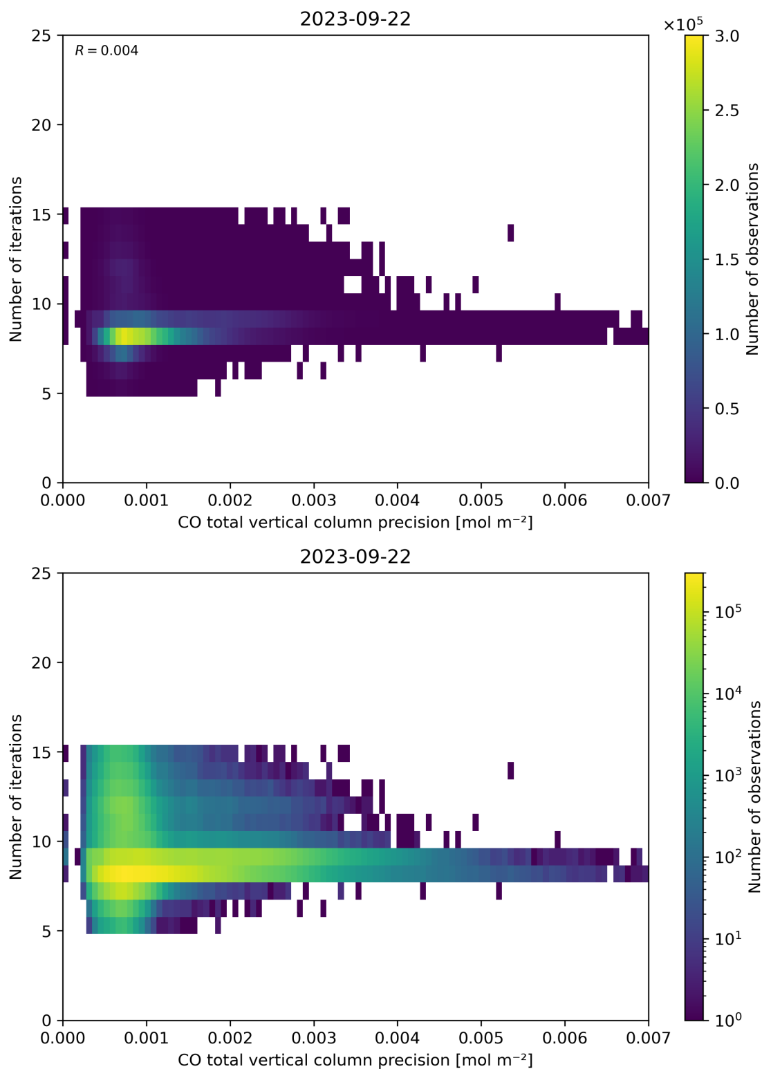
Figure 46: Scatter density plot of “CO total vertical column precision” against “Number of iterations” for 2023-09-21 to 2023-09-23.
