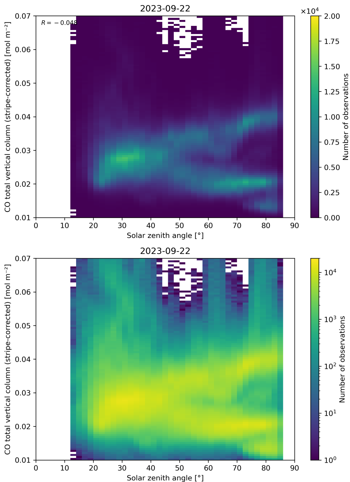
Figure 62: Scatter density plot of “Solar zenith angle” against “CO total vertical column (stripe-corrected)” for 2023-09-21 to 2023-09-23.
