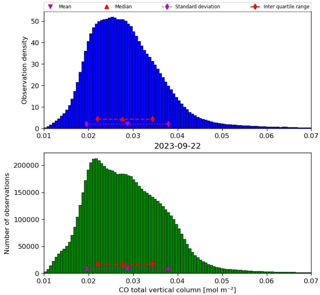
Figure 18: Histogram of “CO total vertical column” for 2023-09-21 to 2023-09-23
