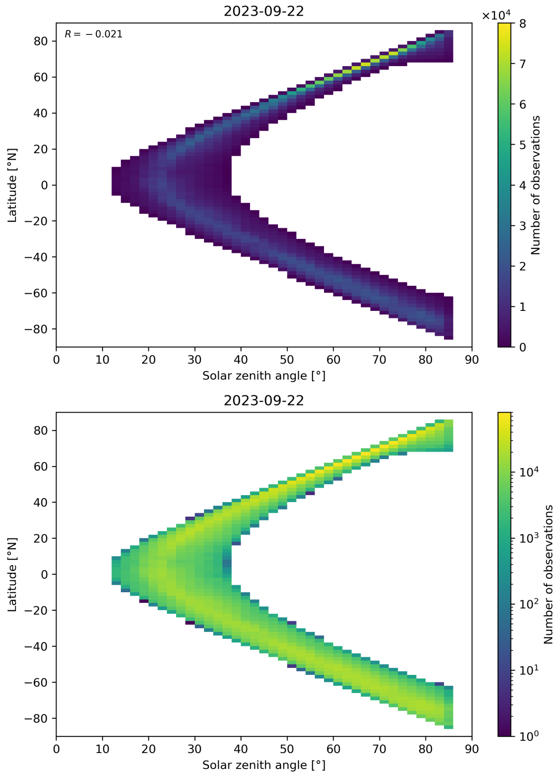
Figure 66: Scatter density plot of “Solar zenith angle” against “Latitude” for 2023-09-21 to 2023-09-23.
