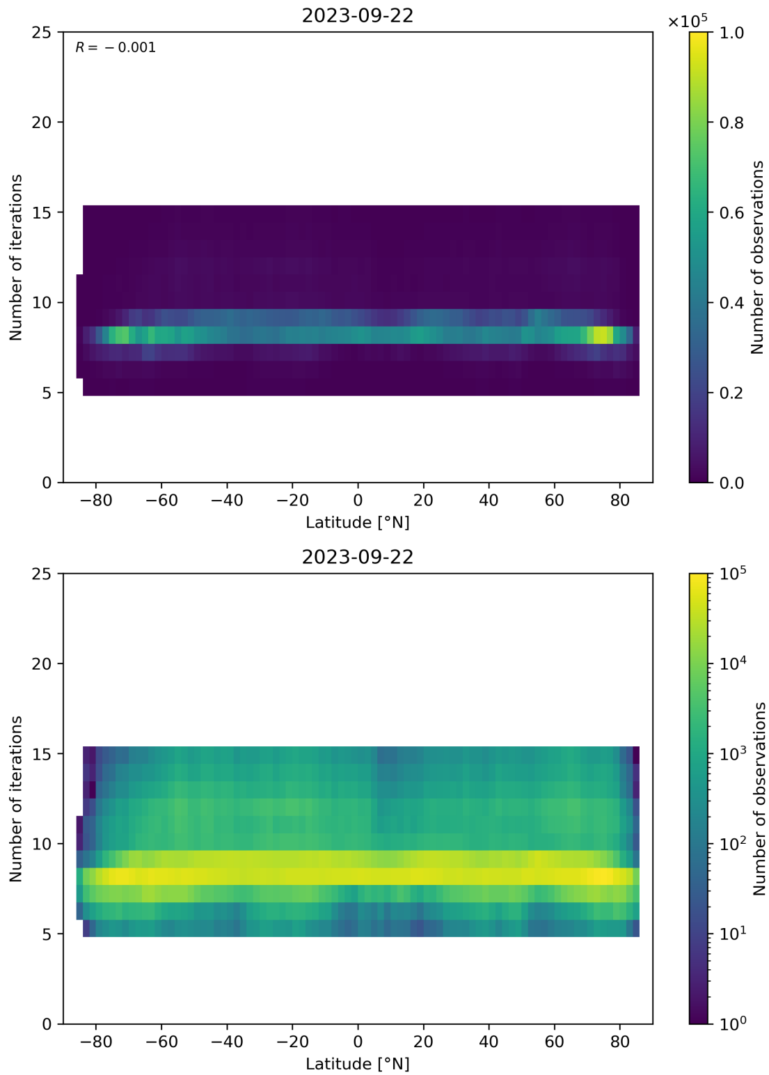
Figure 56: Scatter density plot of “Latitude” against “Number of iterations” for 2023-09-21 to 2023-09-23.
