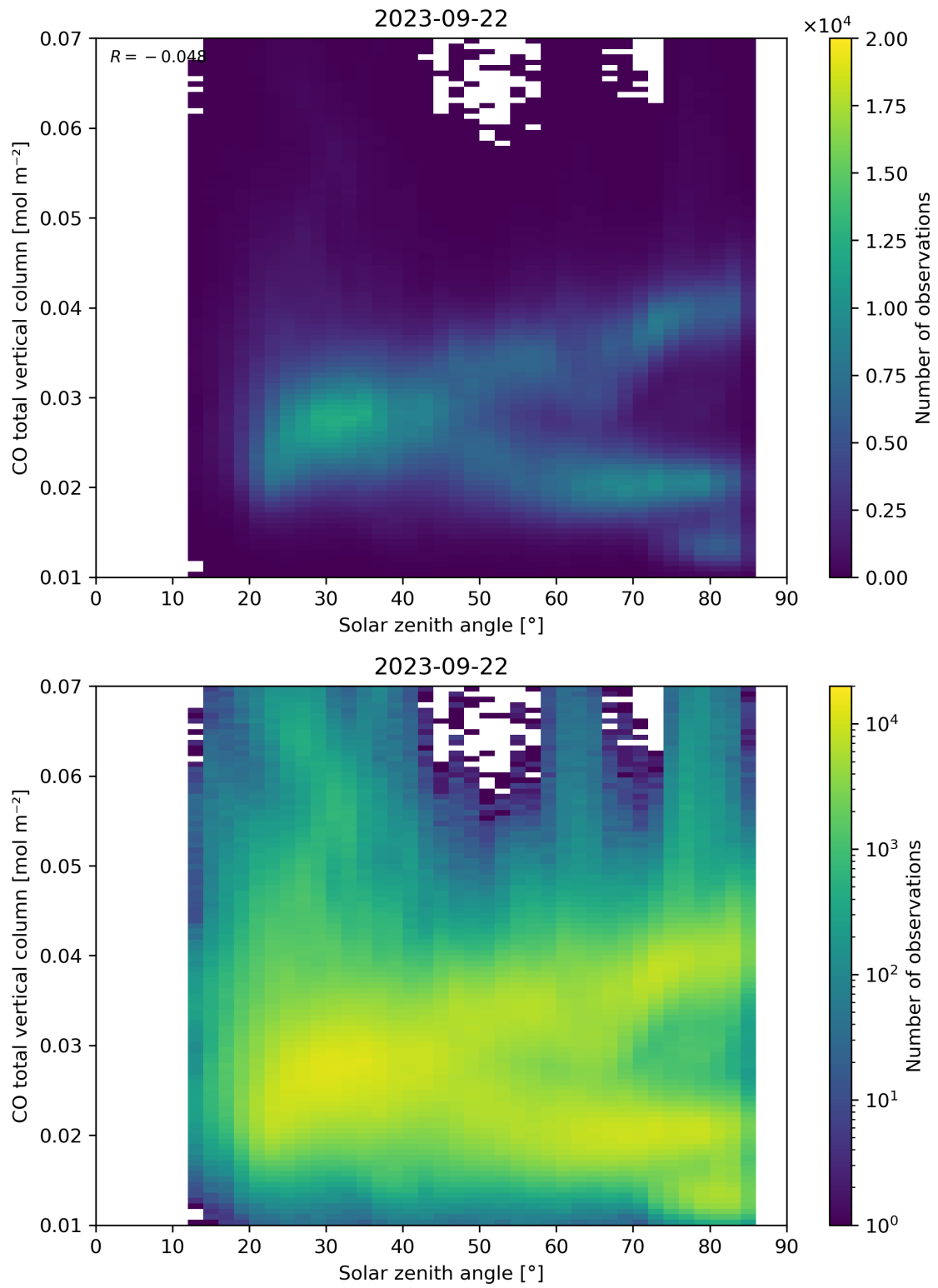
Figure 61: Scatter density plot of “Solar zenith angle” against “CO total vertical column” for 2023-09-21 to 2023-09-23.
