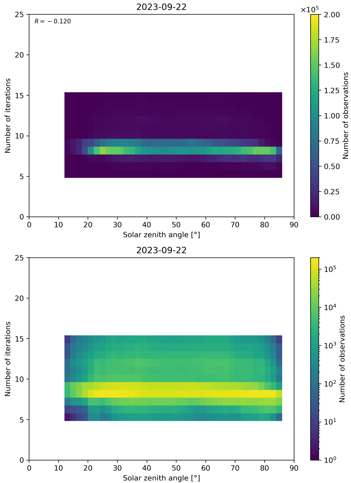
Figure 67: Scatter density plot of “Solar zenith angle” against “Number of iterations” for 2023-09-21 to 2023-09-23.
