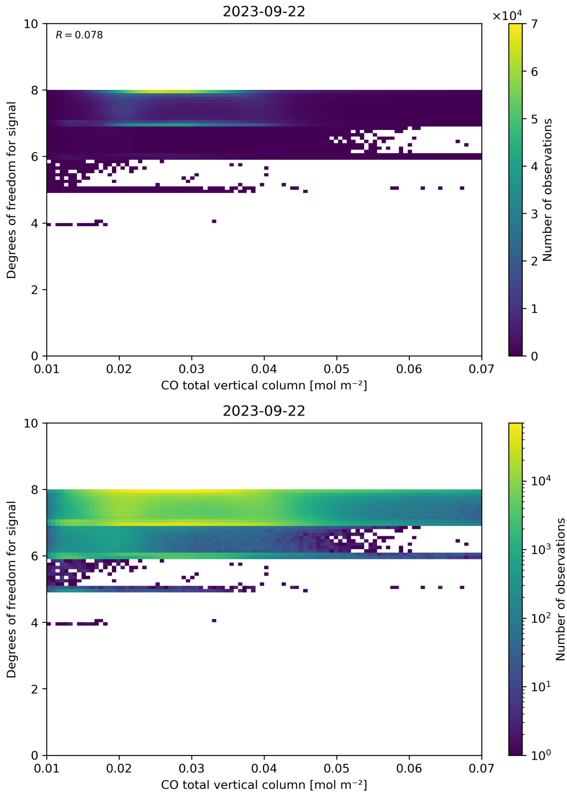
Figure 41: Scatter density plot of “CO total vertical column” against “Degrees of freedom for signal” for 2023-09-21 to 2023-09-23.
