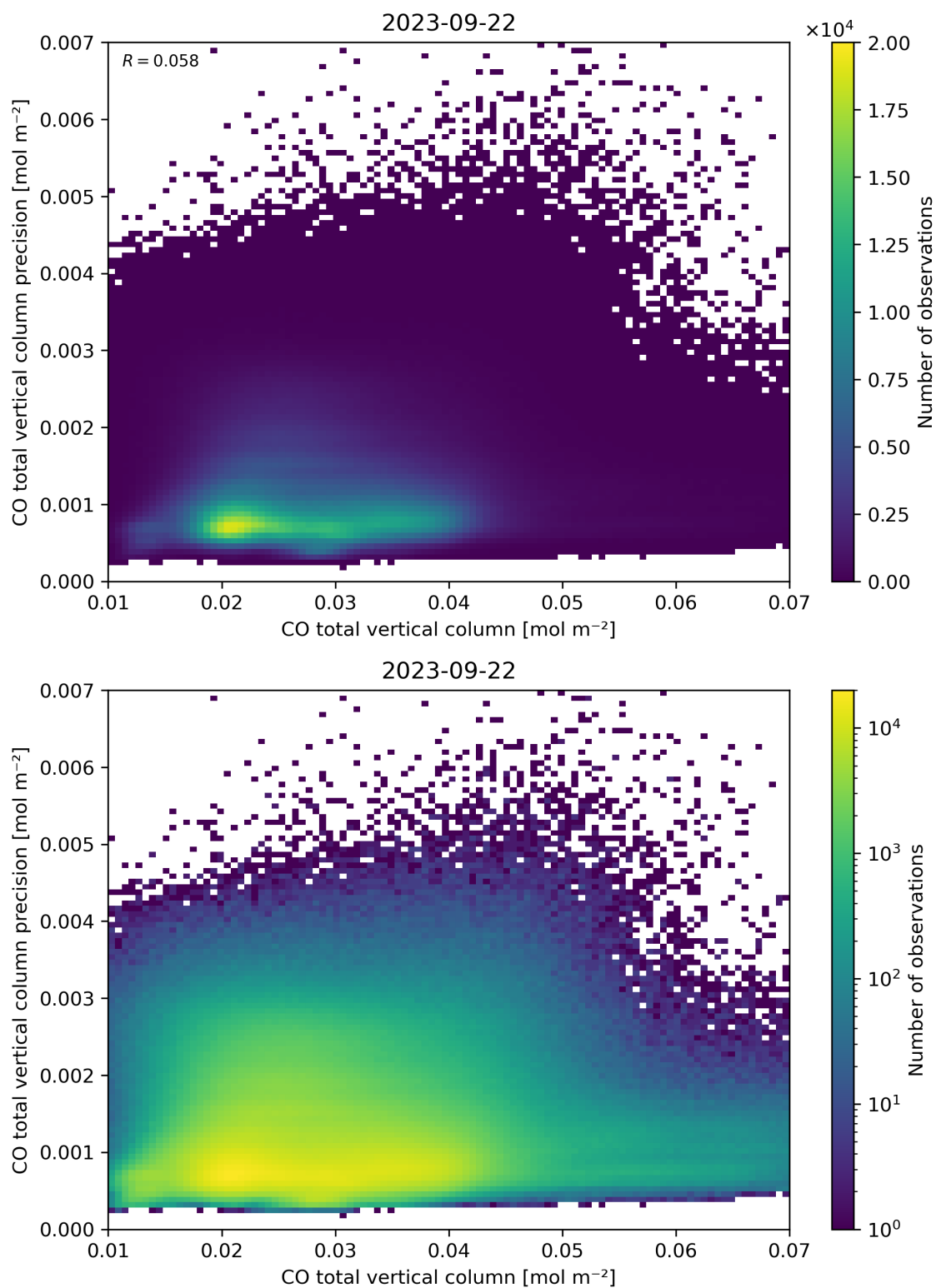
Figure 34: Scatter density plot of “CO total vertical column” against “CO total vertical column precision” for 2023-09-21 to 2023-09-23.
