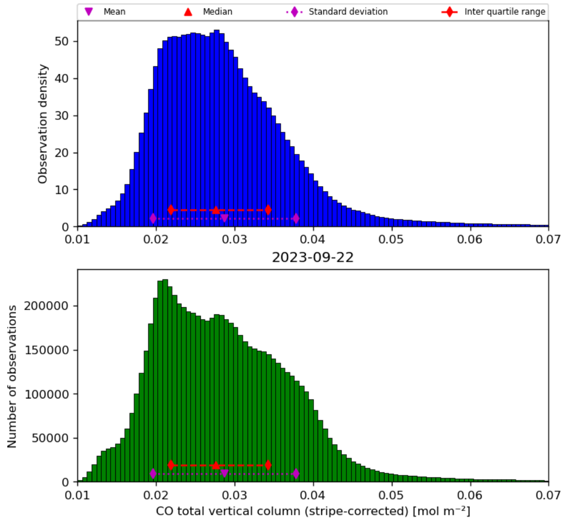
Figure 19: Histogram of “CO total vertical column (stripe-corrected)” for 2023-09-21 to 2023-09-23
