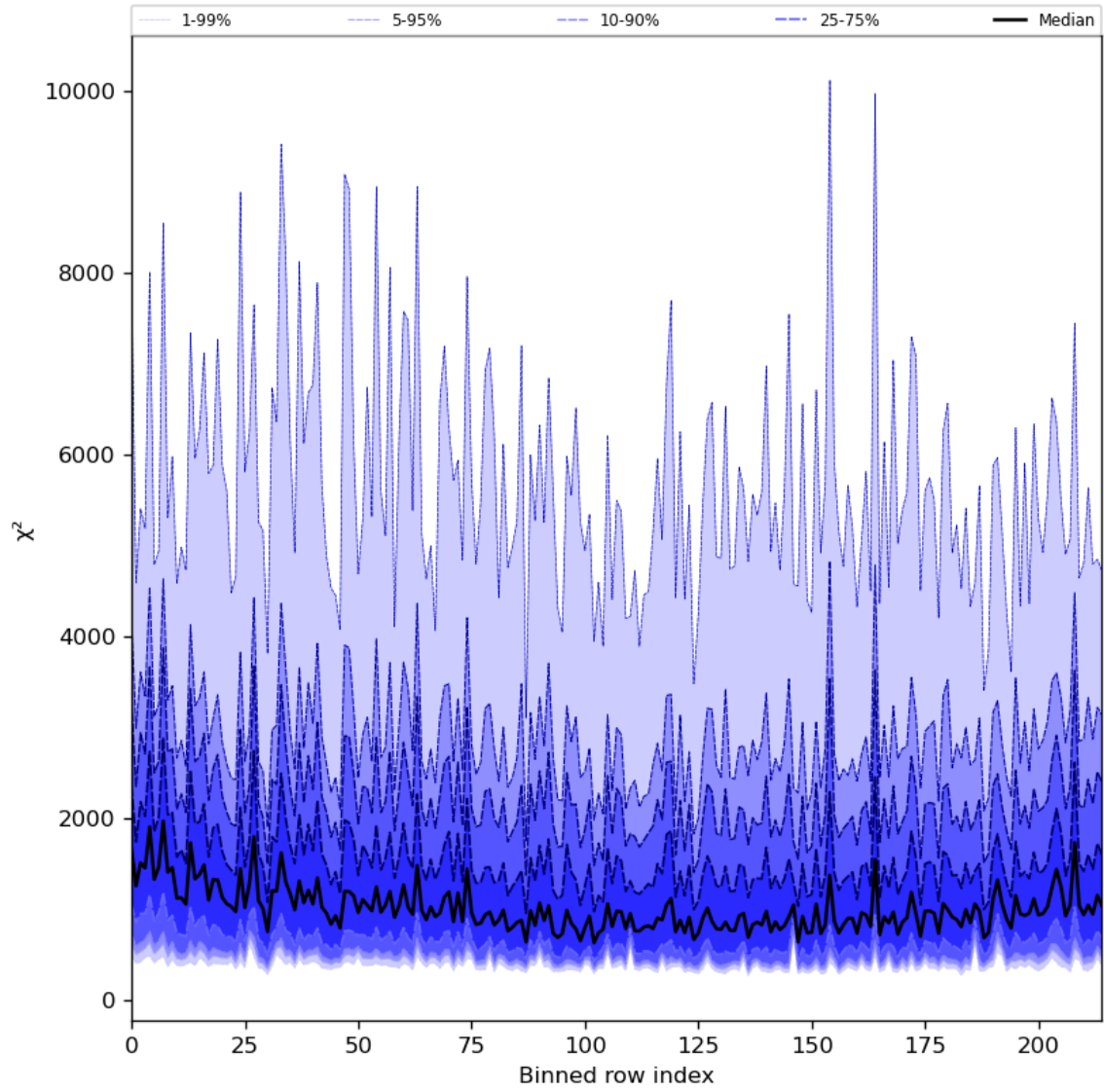
Figure 30: Along track statistics of “ \chi^2 ” for 2023-09-21 to 2023-09-23
