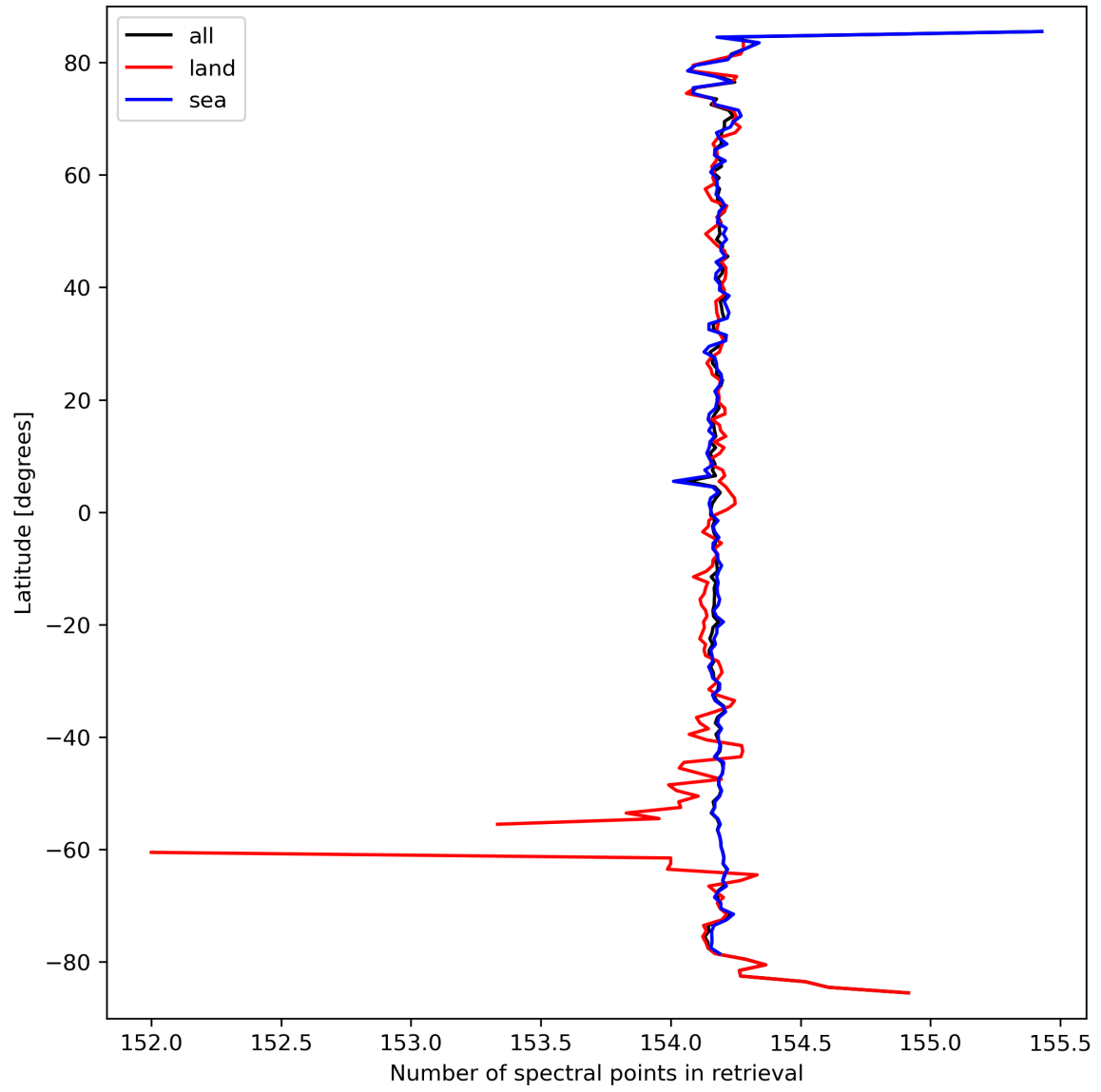
Figure 13: Zonal average of “Number of spectral points in retrieval” for 2023-09-22 to 2023-09-24.
