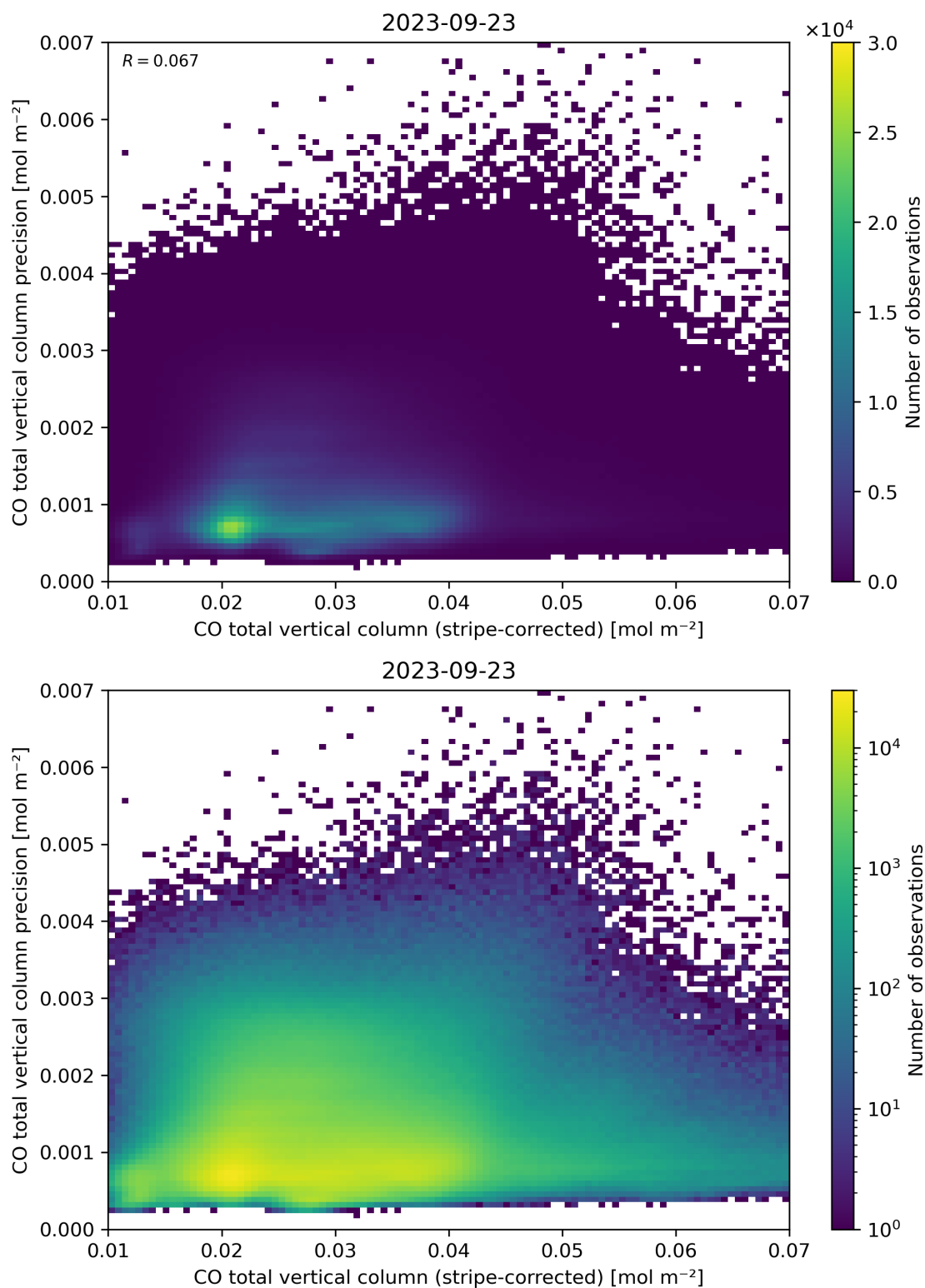
Figure 36: Scatter density plot of “CO total vertical column (stripe-corrected)” against “CO total vertical column precision” for 2023-09-22 to 2023-09-24.
