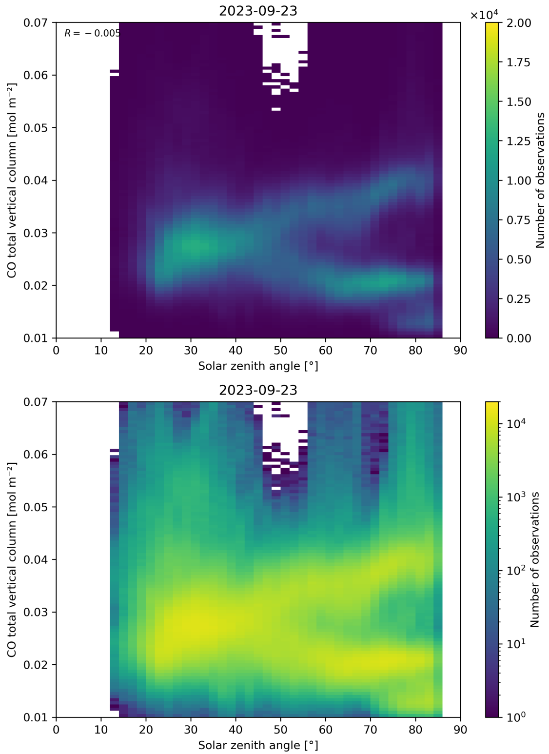
Figure 61: Scatter density plot of “Solar zenith angle” against “CO total vertical column” for 2023-09-22 to 2023-09-24.
