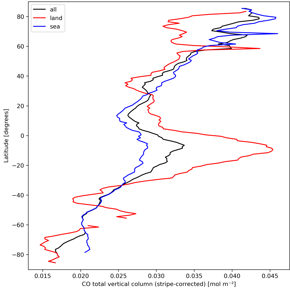
Figure 11: Zonal average of “CO total vertical column (stripe-corrected)” for 2023-09-22 to 2023-09-24.
