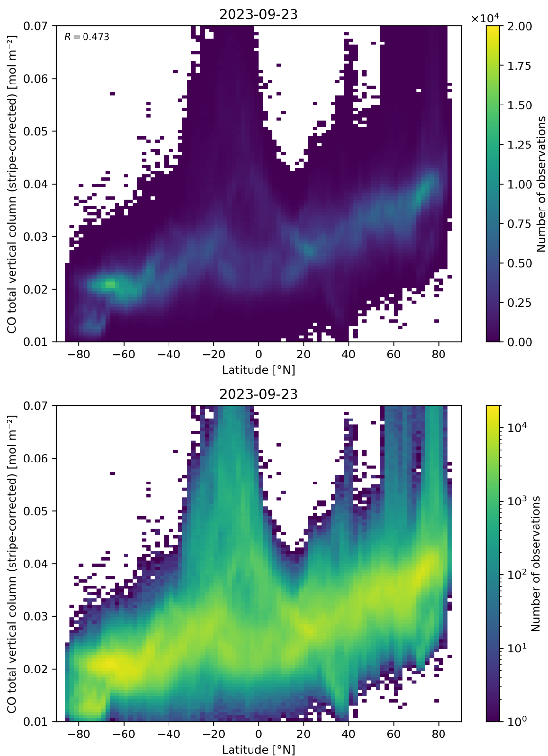
Figure 52: Scatter density plot of “Latitude” against “CO total vertical column (stripe-corrected)” for 2023-09-22 to 2023-09-24.
