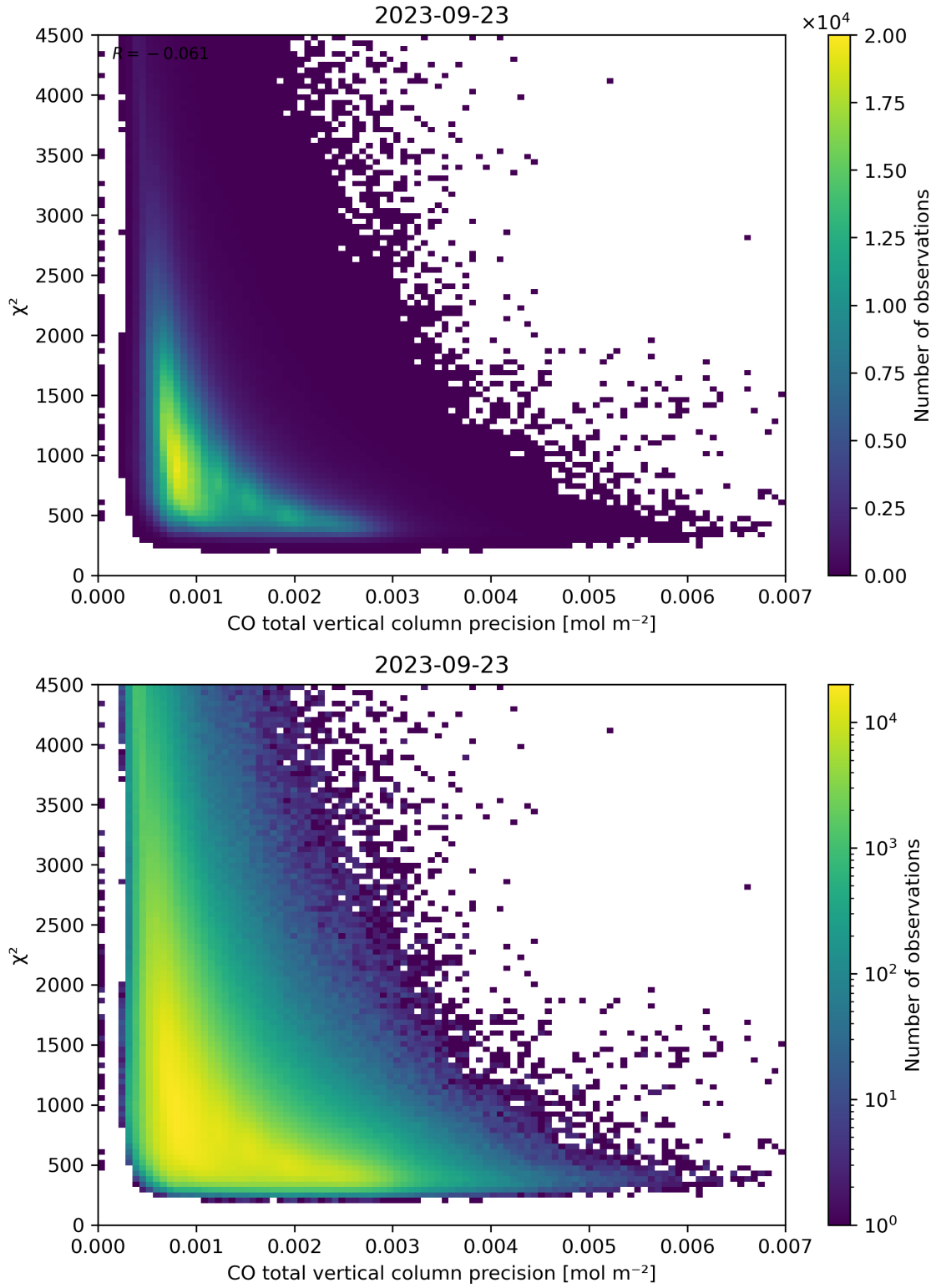
Figure 44: Scatter density plot of “CO total vertical column precision” against “ \chi^2 ” for 2023-09-22 to 2023-09-24.
