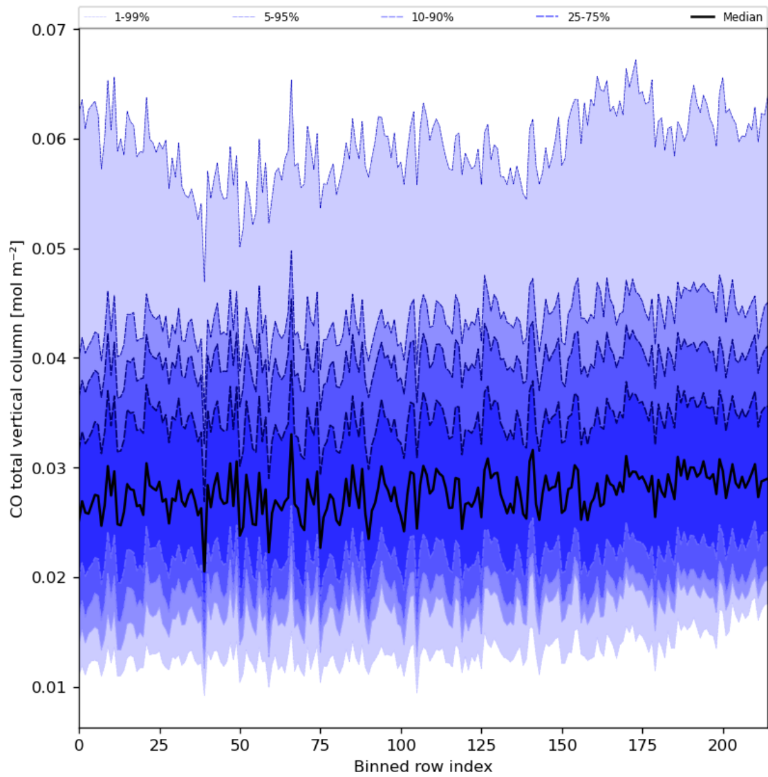
Figure 26: Along track statistics of “CO total vertical column” for 2023-09-22 to 2023-09-24
