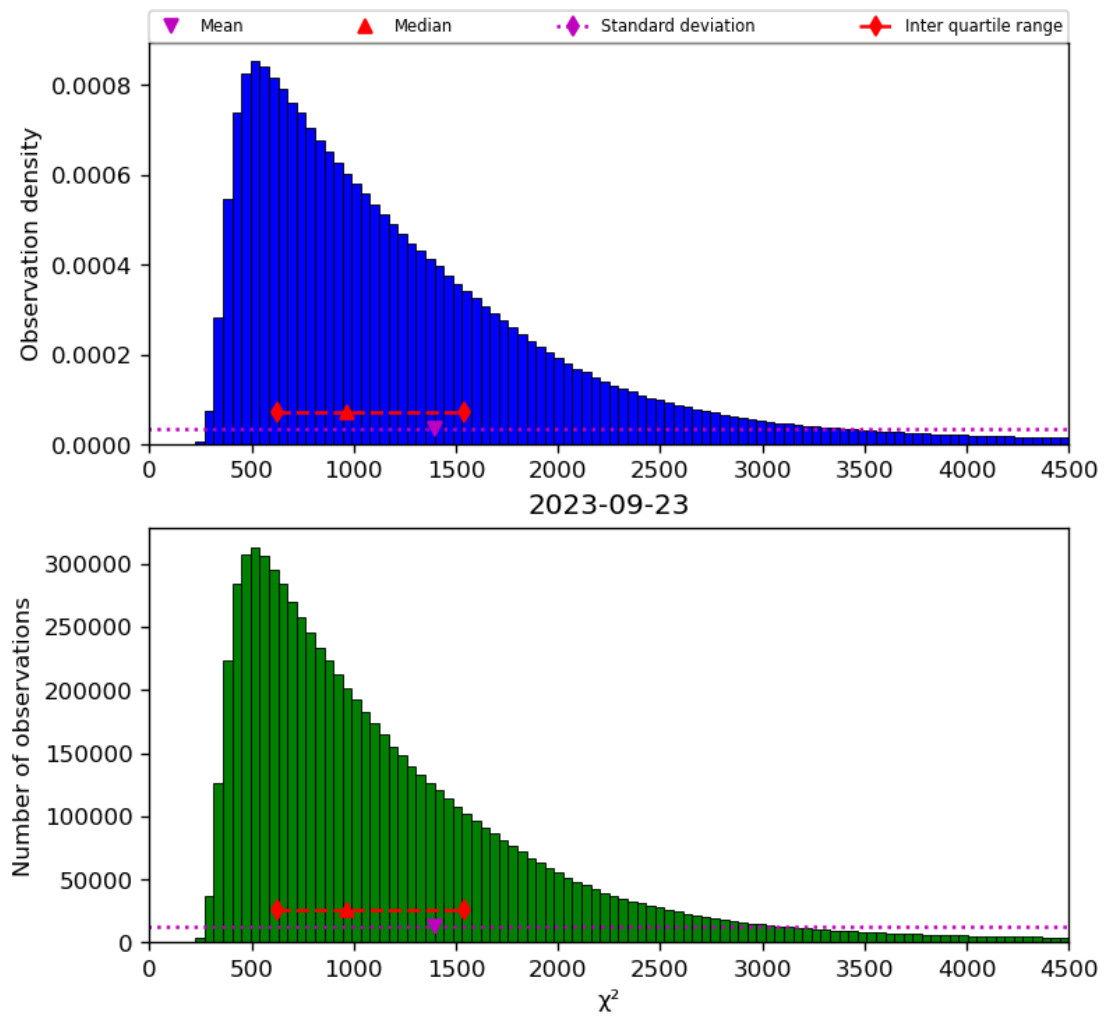
Figure 22: Histogram of “ \chi^2 ” for 2023-09-22 to 2023-09-24
