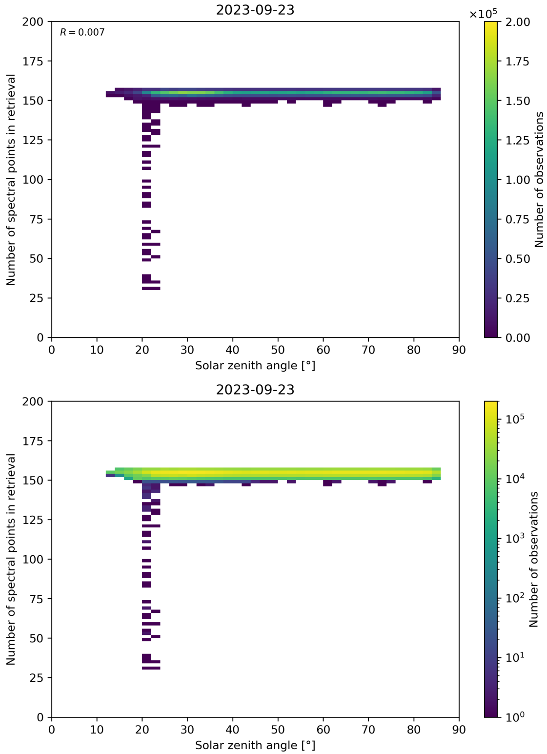
Figure 68: Scatter density plot of “Solar zenith angle” against “Number of spectral points in retrieval” for 2023-09-22 to 2023-09-24.
