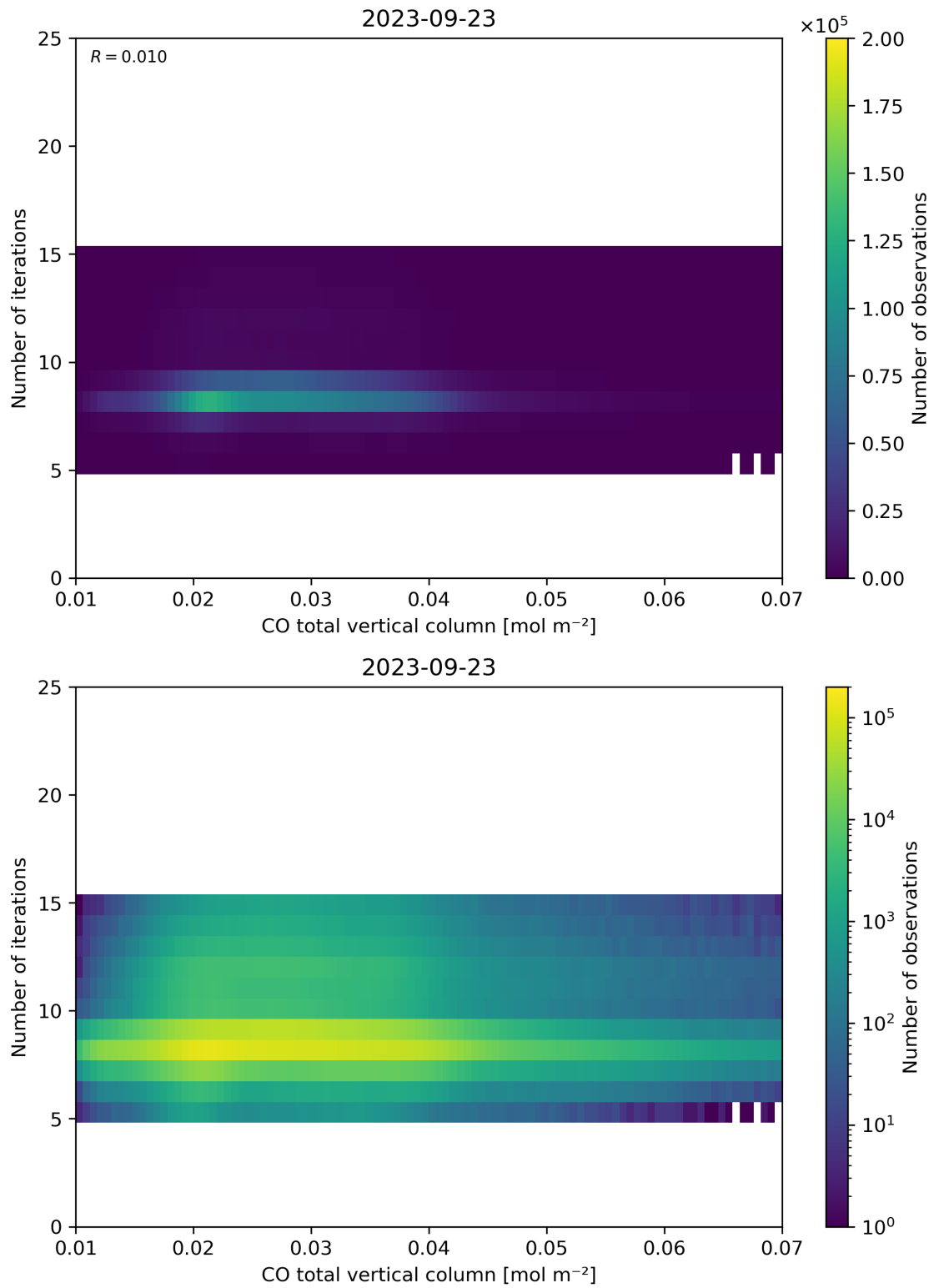
Figure 42: Scatter density plot of “CO total vertical column” against “Number of iterations” for 2023-09-22 to 2023-09-24.
