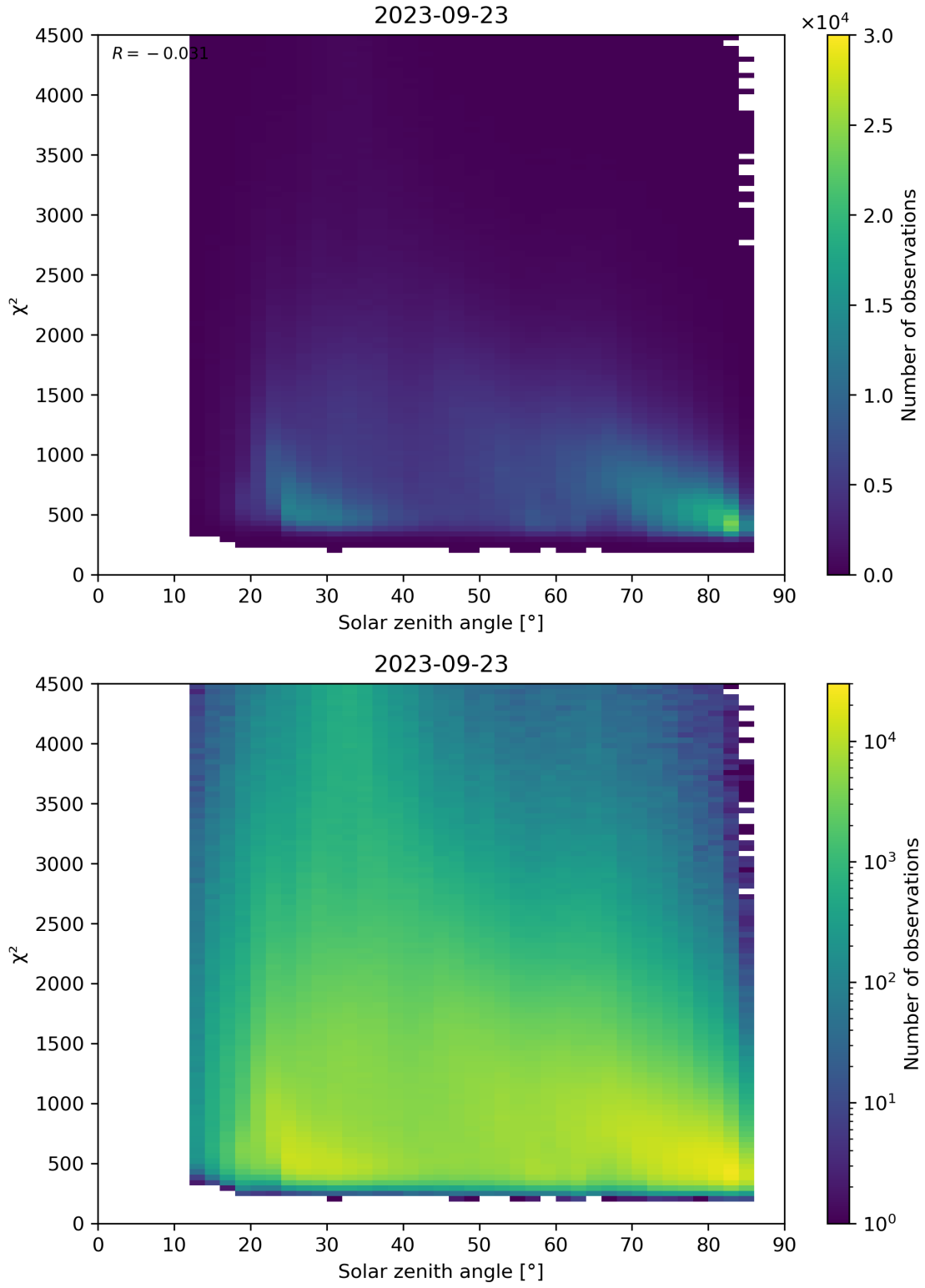
Figure 64: Scatter density plot of “Solar zenith angle” against “ \chi^2 ” for 2023-09-22 to 2023-09-24.
