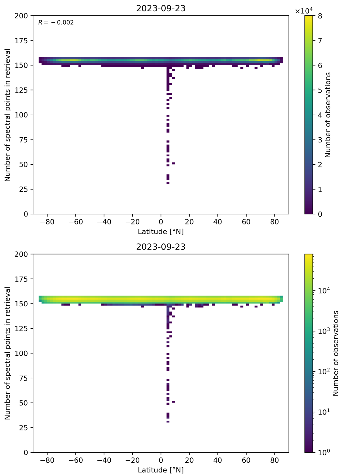
Figure 57: Scatter density plot of “Latitude” against “Number of spectral points in retrieval” for 2023-09-22 to 2023-09-24.
