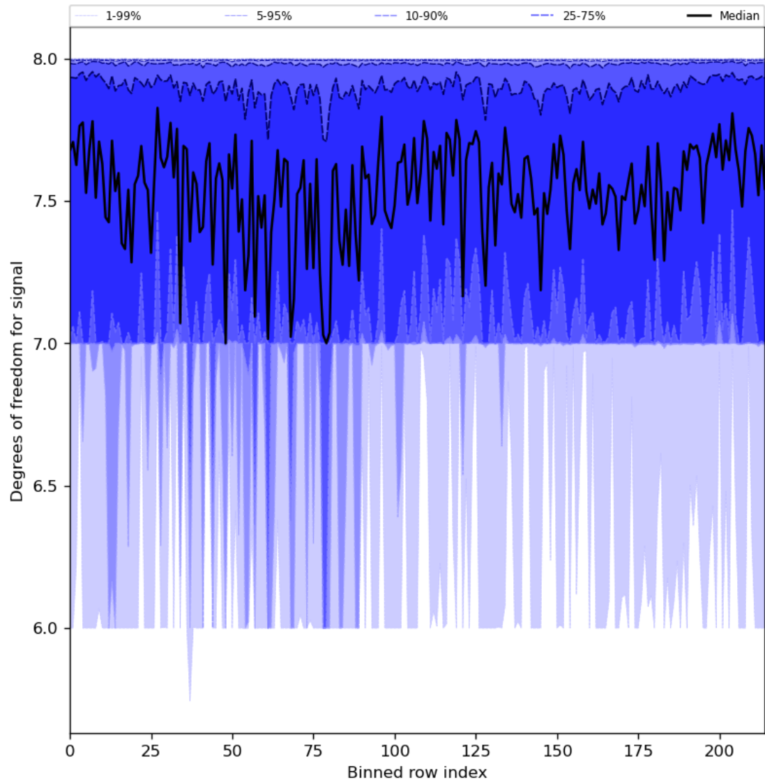
Figure 31: Along track statistics of “Degrees of freedom for signal” for 2023-09-22 to 2023-09-24
