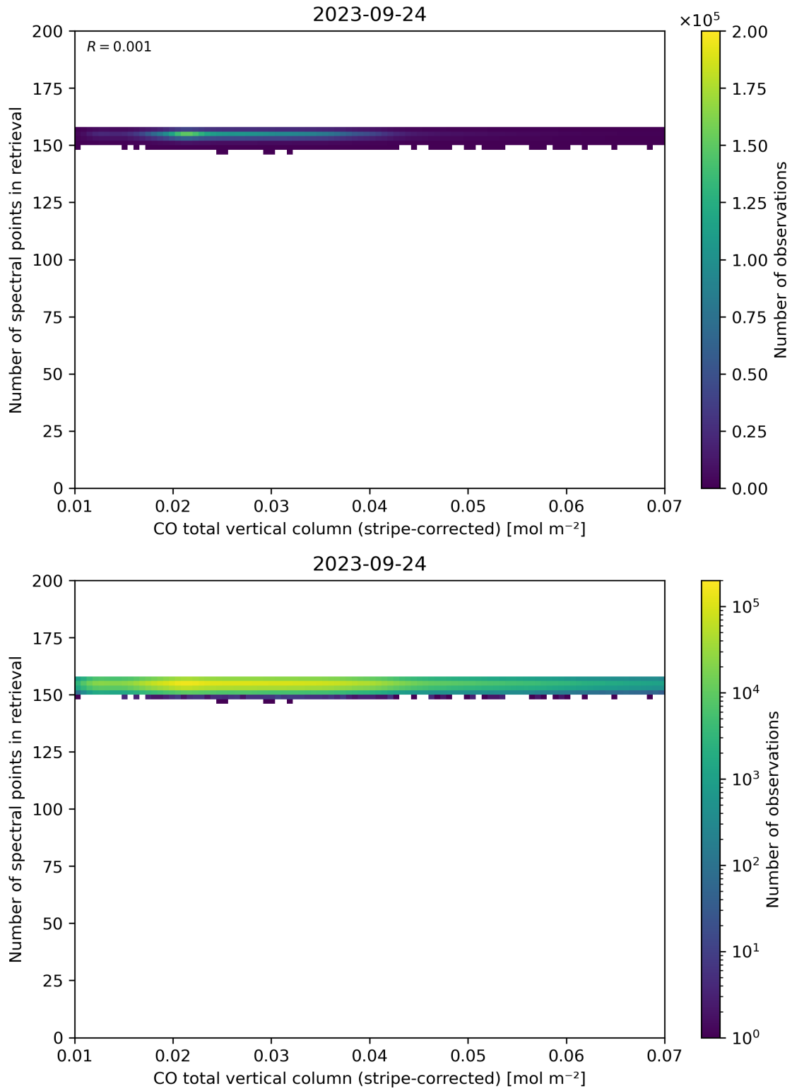
Figure 40: Scatter density plot of “CO total vertical column (stripe-corrected)” against “Number of spectral points in retrieval” for 2023-09-23 to 2023-09-25.
