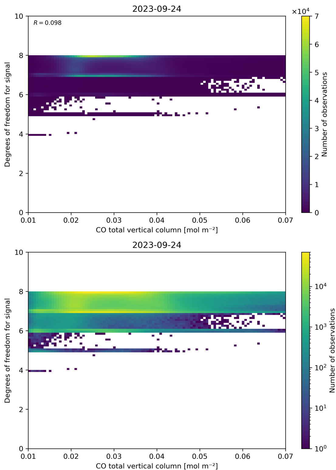
Figure 41: Scatter density plot of “CO total vertical column” against “Degrees of freedom for signal” for 2023-09-23 to 2023-09-25.
