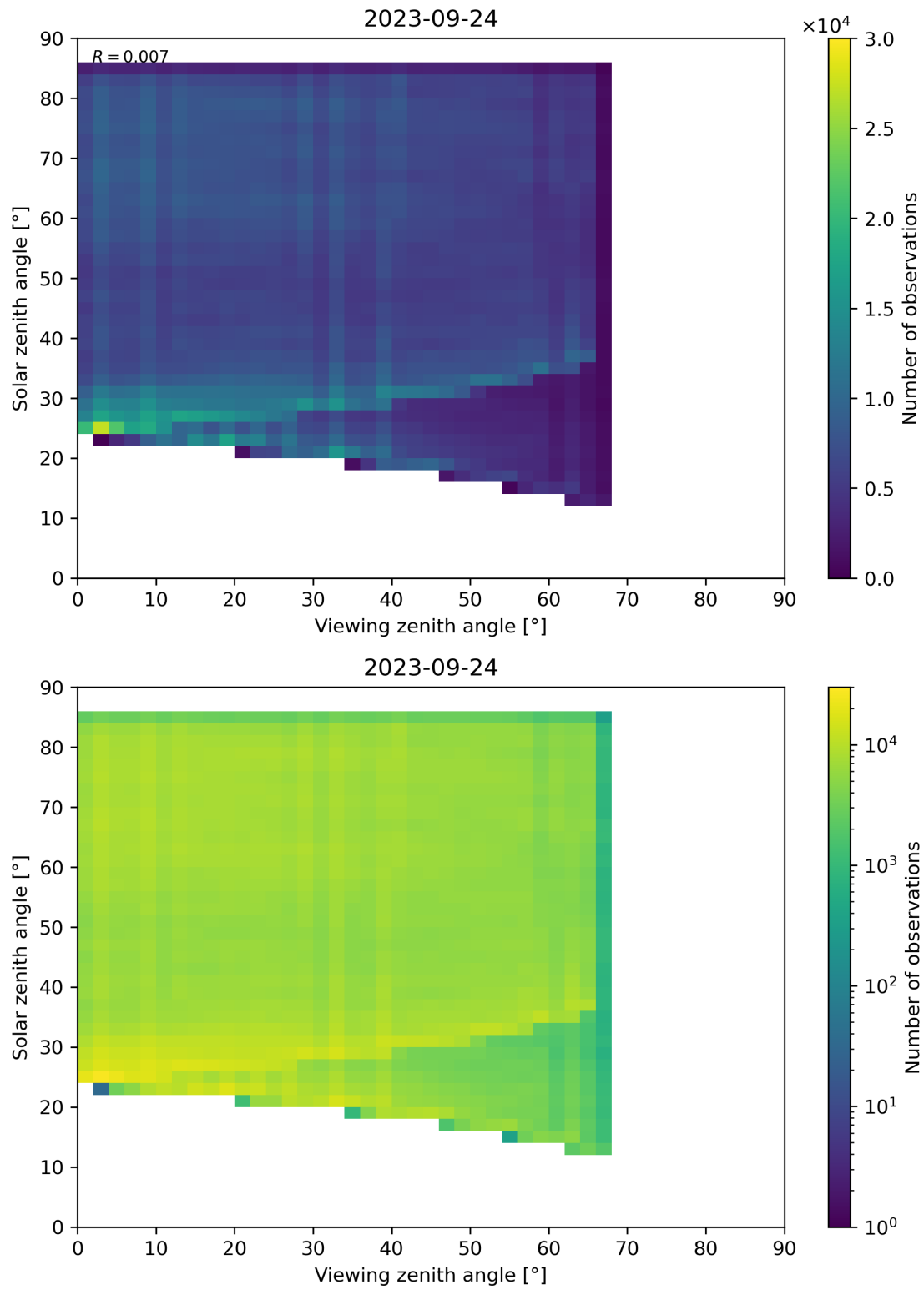
Figure 77: Scatter density plot of “Viewing zenith angle” against “Solar zenith angle” for 2023-09-23 to 2023-09-25.
