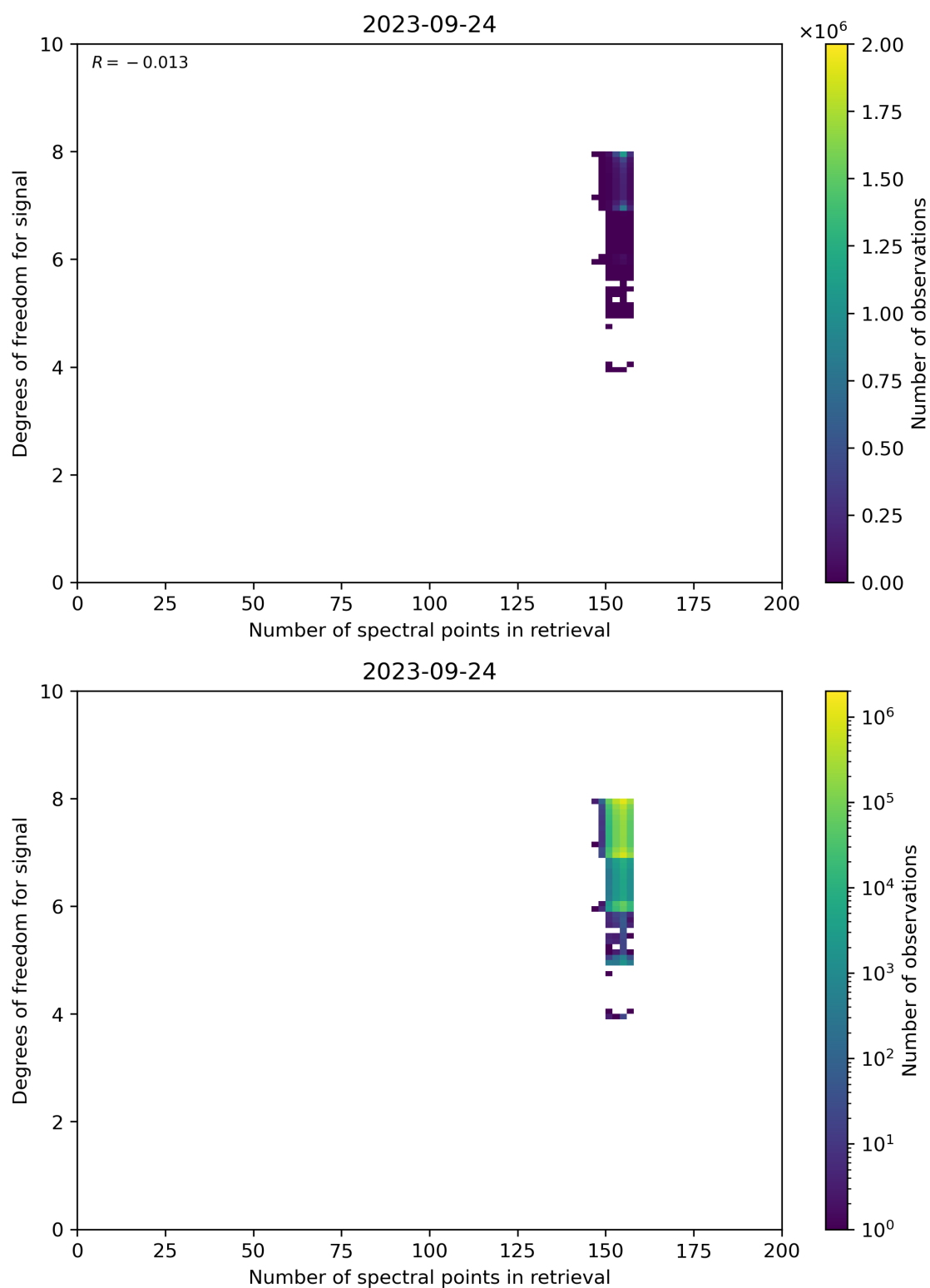
Figure 59: Scatter density plot of “Number of spectral points in retrieval” against “Degrees of freedom for signal” for 2023-09-23 to 2023-09-25.
