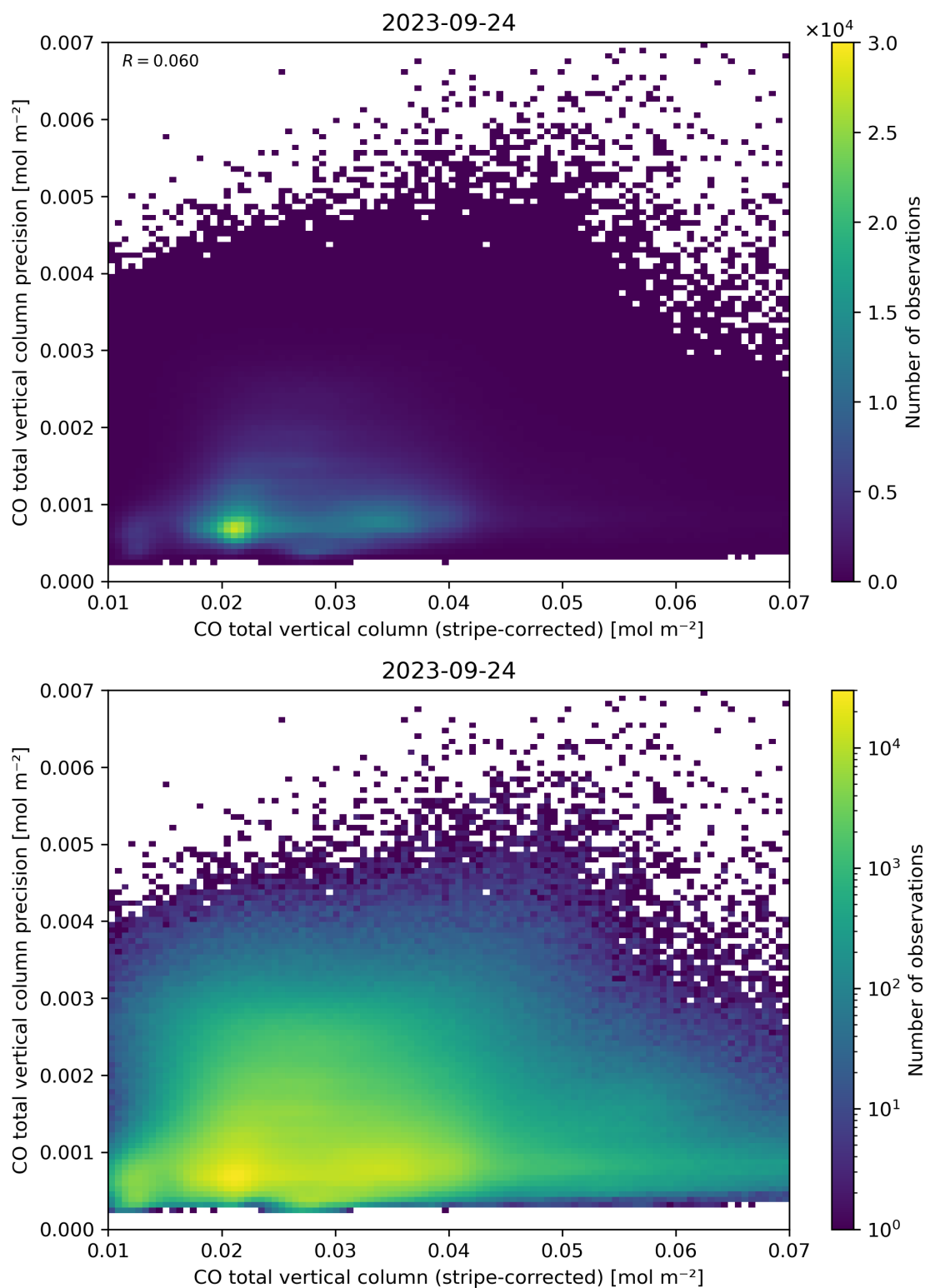
Figure 36: Scatter density plot of “CO total vertical column (stripe-corrected)” against “CO total vertical column precision” for 2023-09-23 to 2023-09-25.
