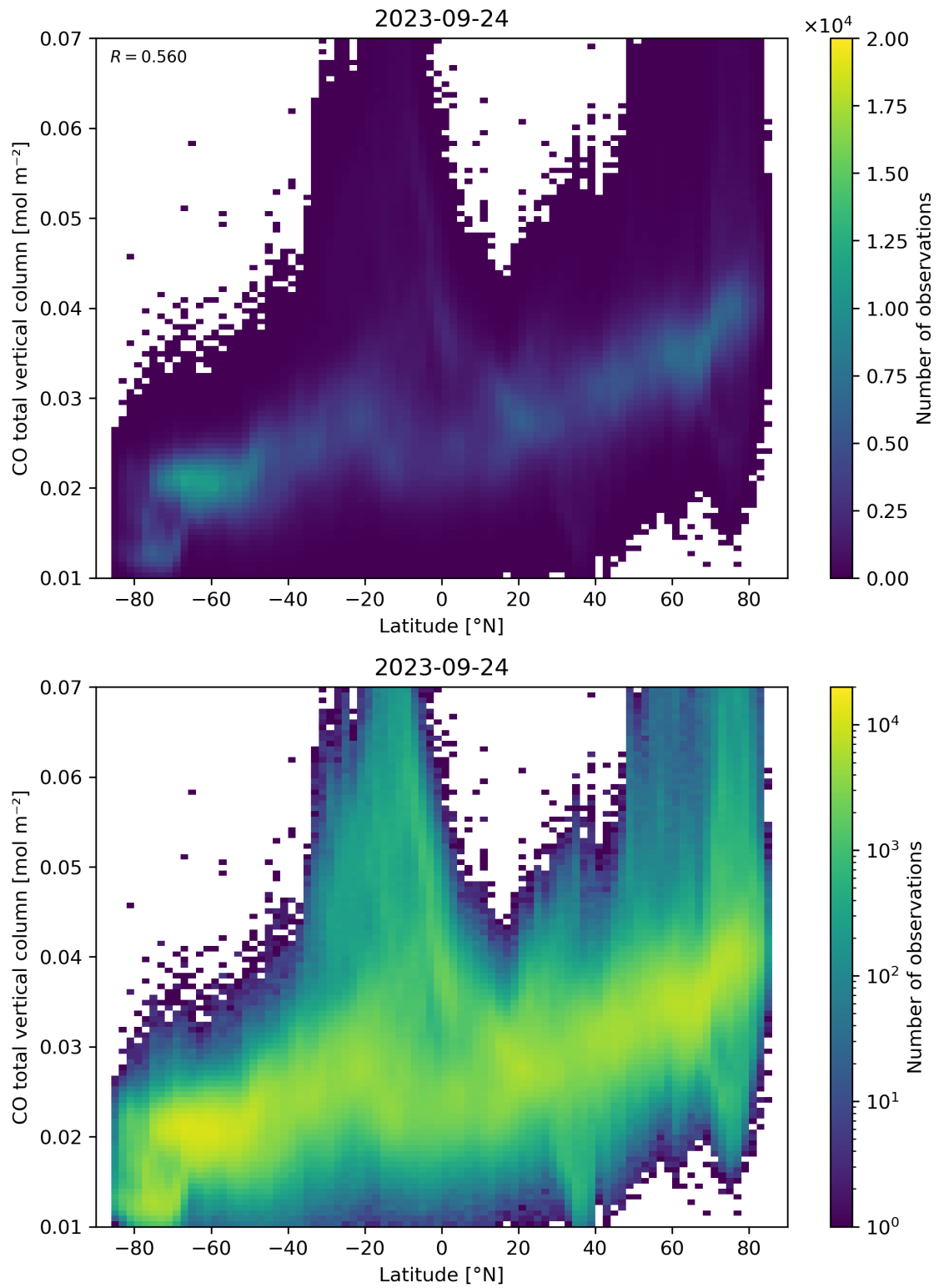
Figure 51: Scatter density plot of “Latitude” against “CO total vertical column” for 2023-09-23 to 2023-09-25.
