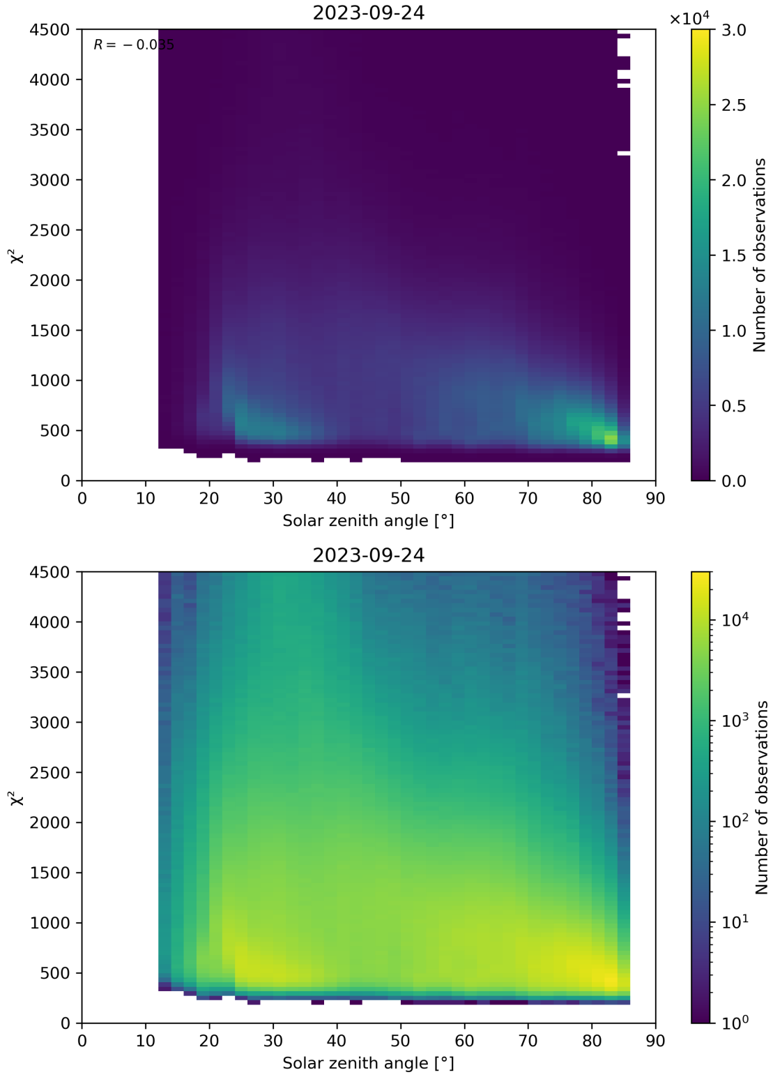
Figure 64: Scatter density plot of “Solar zenith angle” against “ \chi^2 ” for 2023-09-23 to 2023-09-25.
