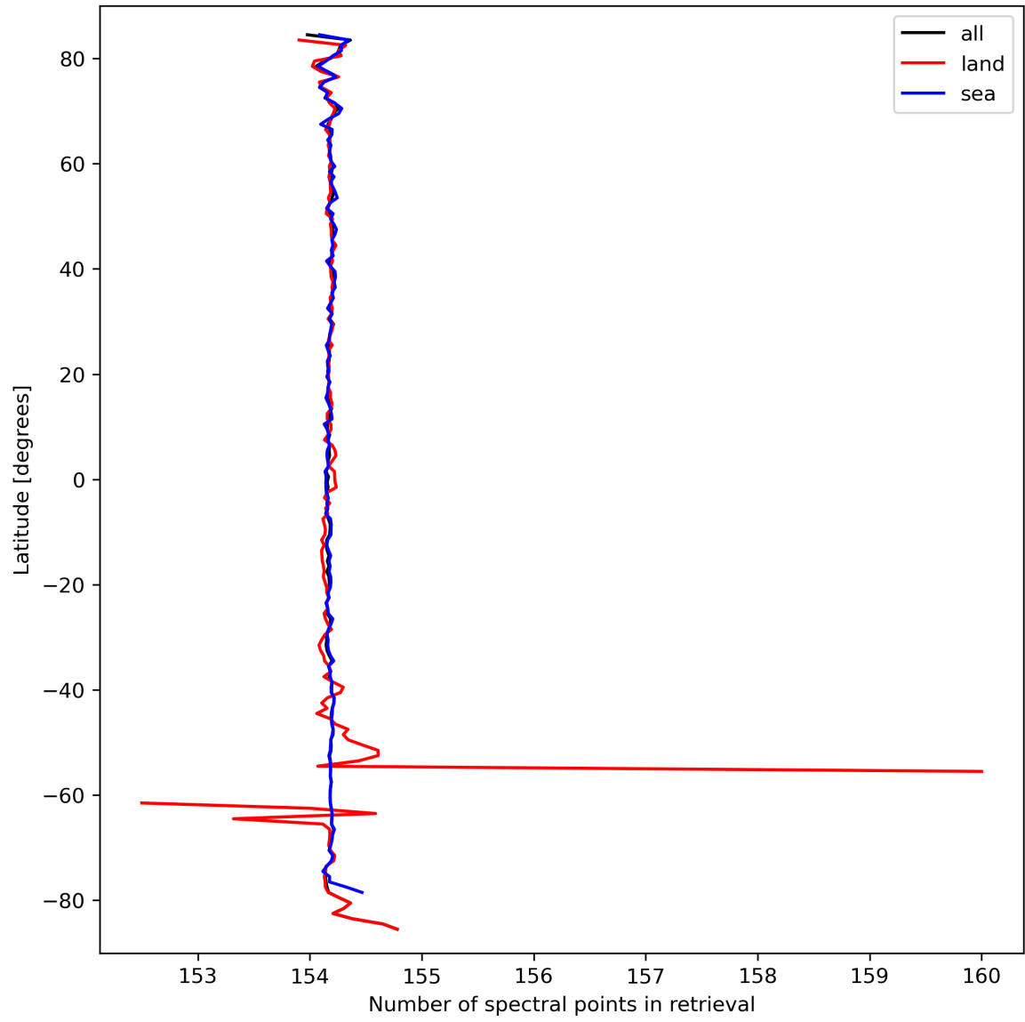
Figure 13: Zonal average of “Number of spectral points in retrieval” for 2023-09-23 to 2023-09-25.
