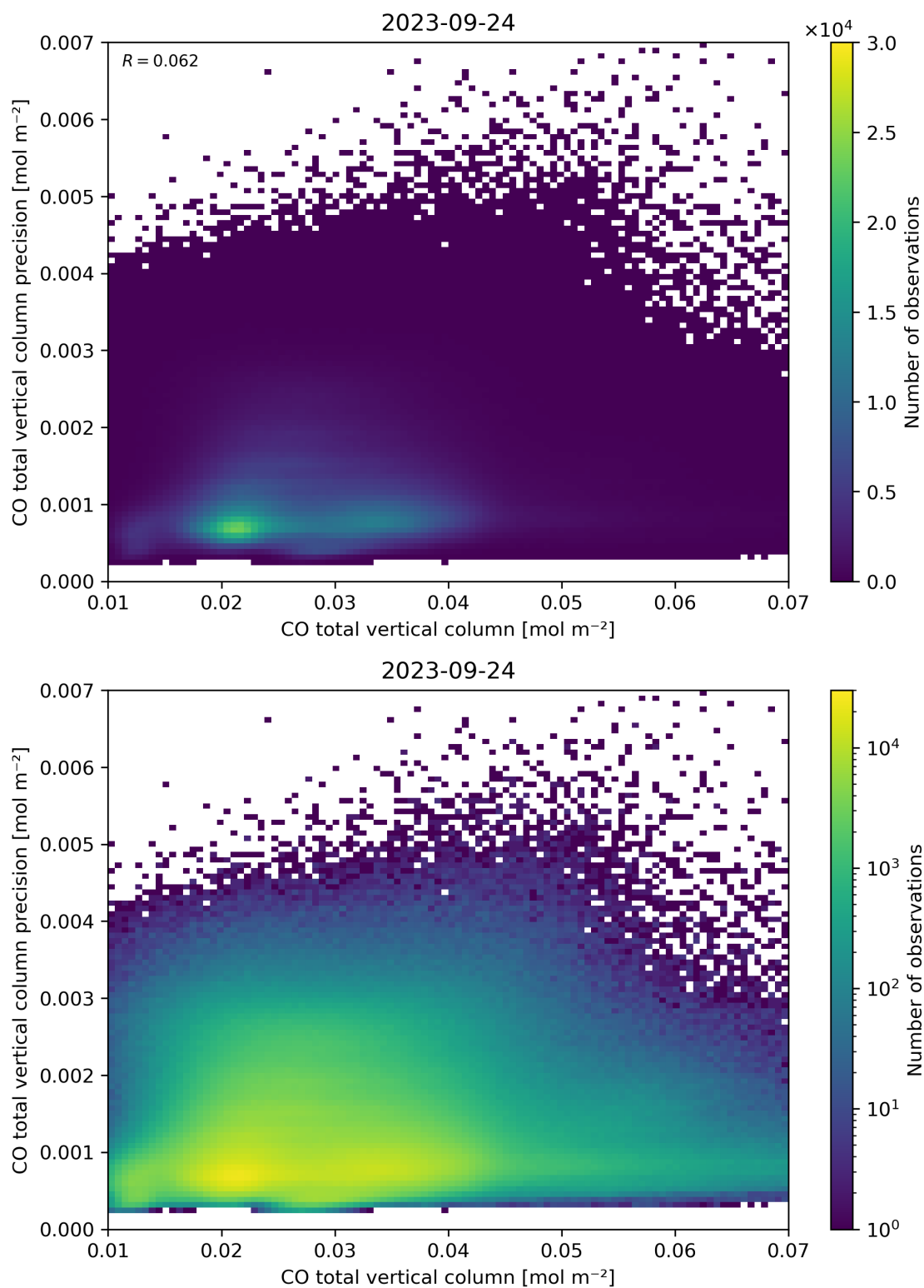
Figure 34: Scatter density plot of “CO total vertical column” against “CO total vertical column precision” for 2023-09-23 to 2023-09-25.
