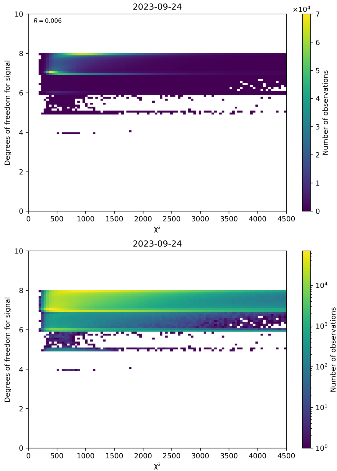
Figure 48: Scatter density plot of “ \chi^2 ” against “Degrees of freedom for signal” for 2023-09-23 to 2023-09-25.
