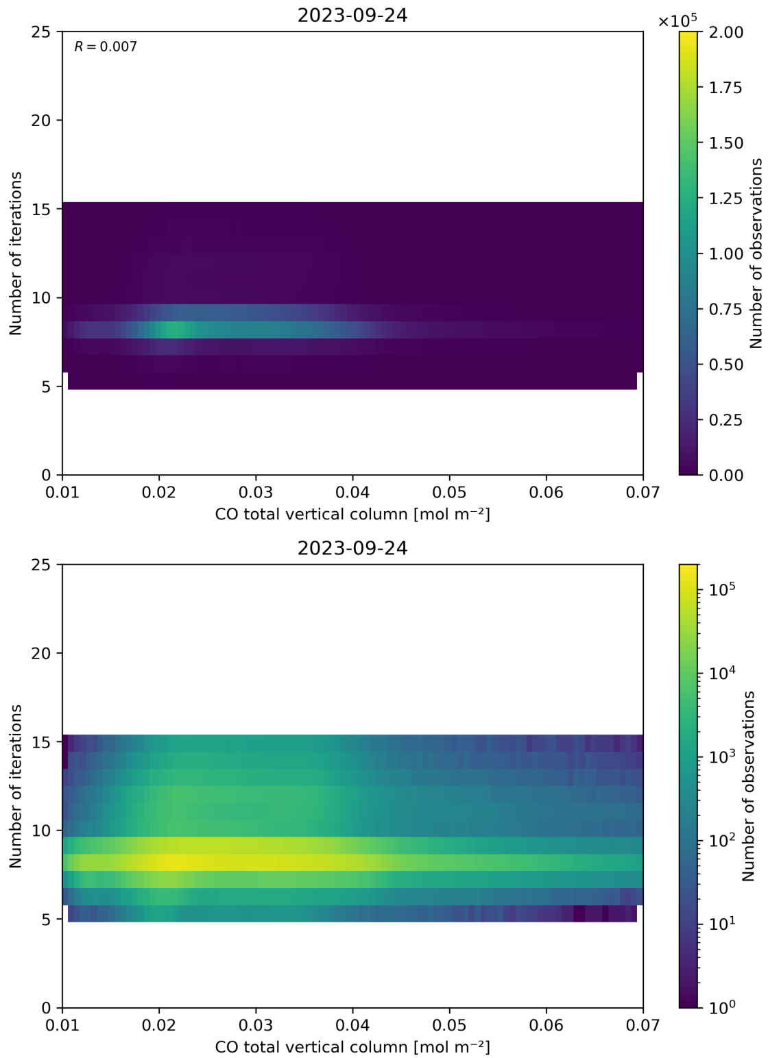
Figure 42: Scatter density plot of “CO total vertical column” against “Number of iterations” for 2023-09-23 to 2023-09-25.
