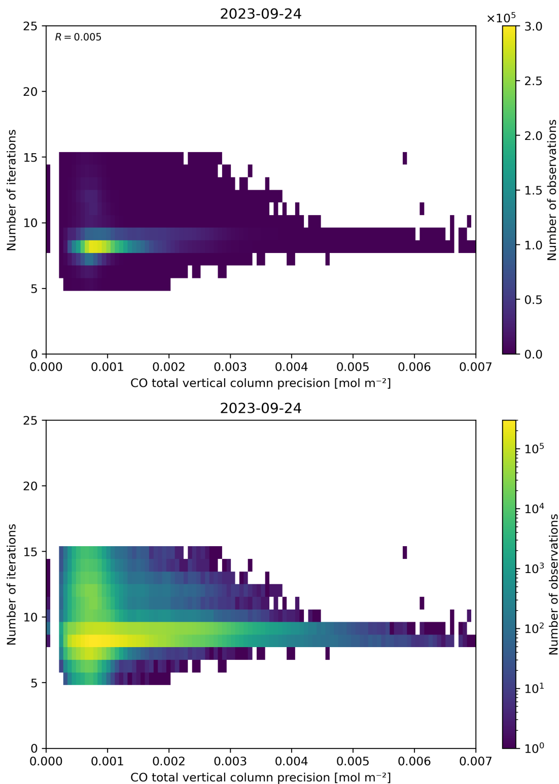
Figure 46: Scatter density plot of “CO total vertical column precision” against “Number of iterations” for 2023-09-23 to 2023-09-25.
