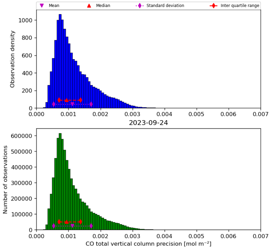
Figure 20: Histogram of “CO total vertical column precision” for 2023-09-23 to 2023-09-25
