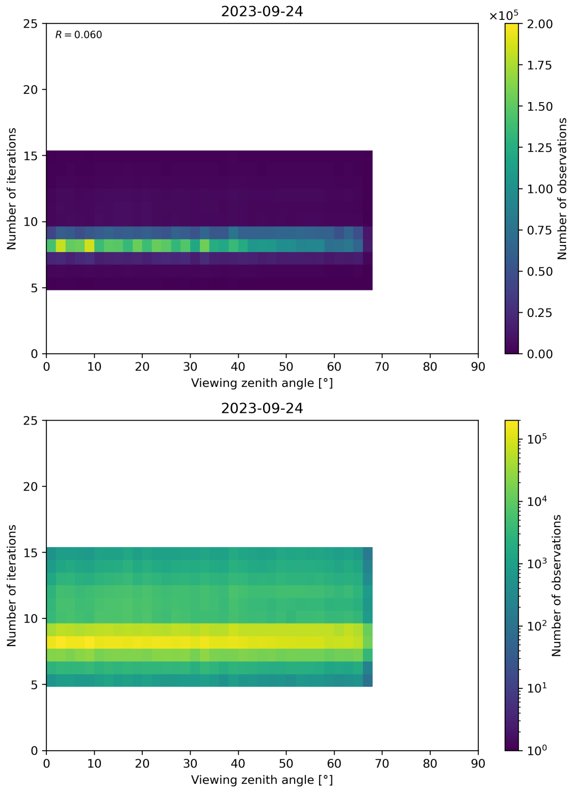
Figure 75: Scatter density plot of “Viewing zenith angle” against “Number of iterations” for 2023-09-23 to 2023-09-25.
