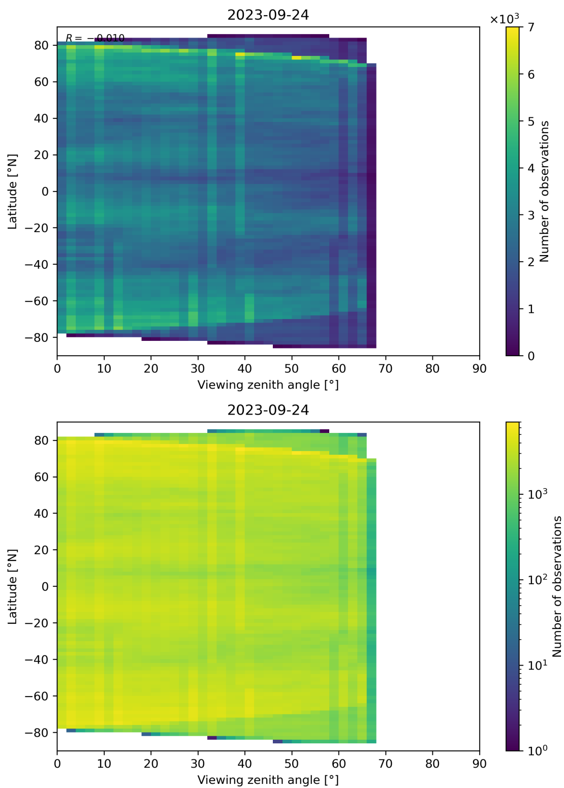
Figure 74: Scatter density plot of “Viewing zenith angle” against “Latitude” for 2023-09-23 to 2023-09-25.
