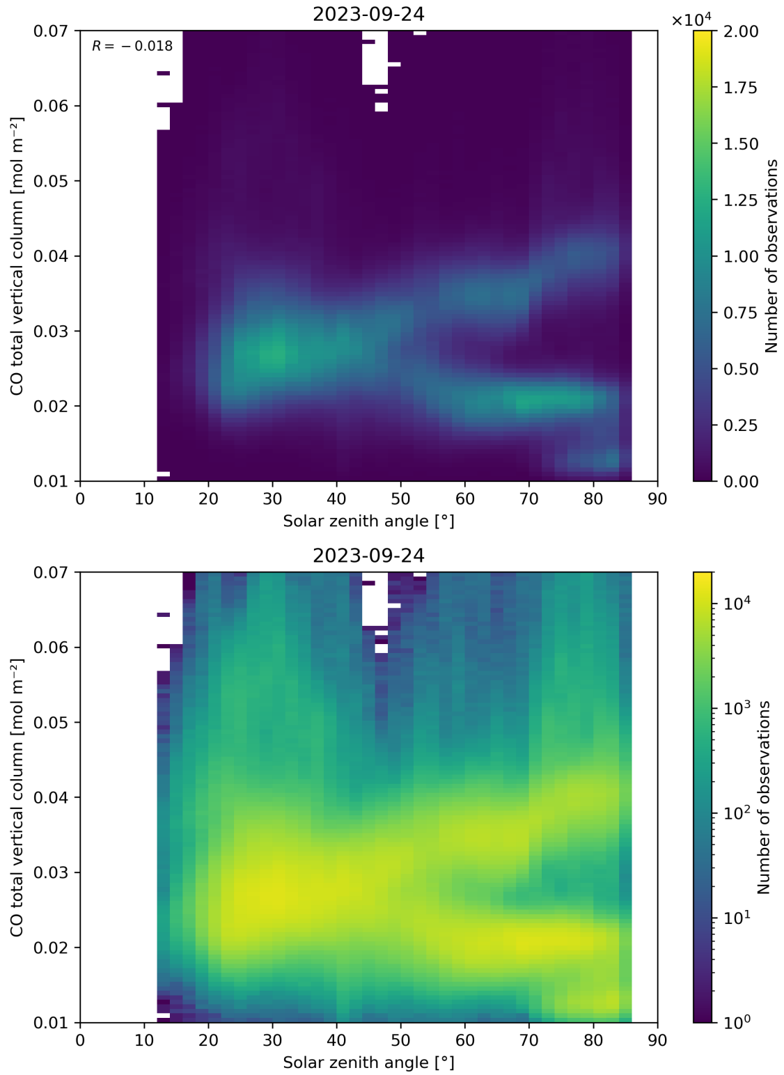
Figure 61: Scatter density plot of “Solar zenith angle” against “CO total vertical column” for 2023-09-23 to 2023-09-25.
