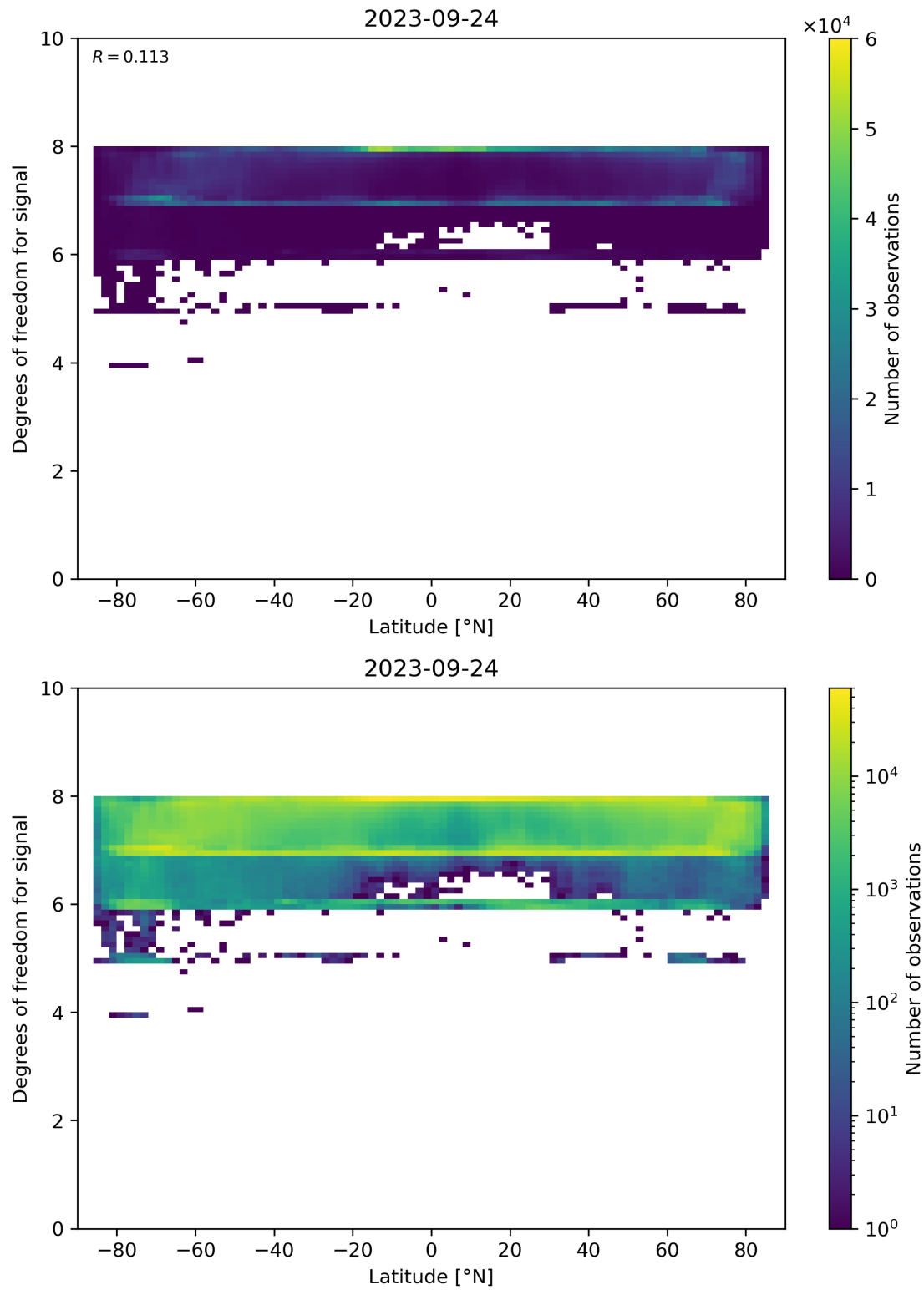
Figure 55: Scatter density plot of “Latitude” against “Degrees of freedom for signal” for 2023-09-23 to 2023-09-25.
