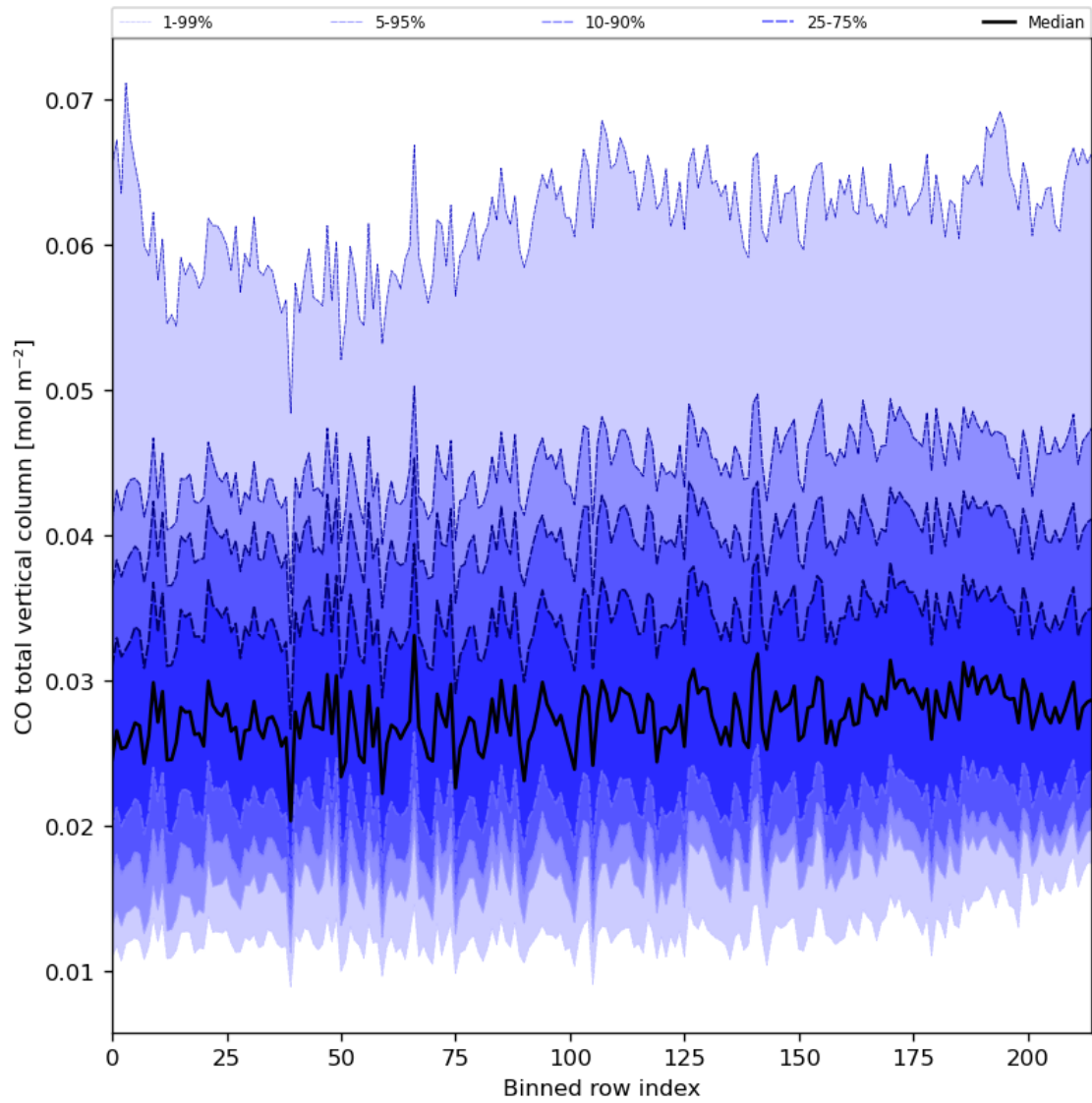
Figure 26: Along track statistics of “CO total vertical column” for 2023-09-23 to 2023-09-25
