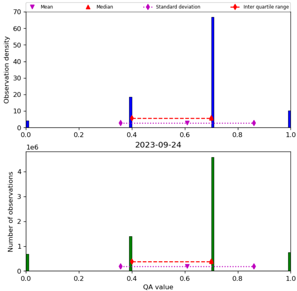
Figure 17: Histogram of “QA value” for 2023-09-23 to 2023-09-25
