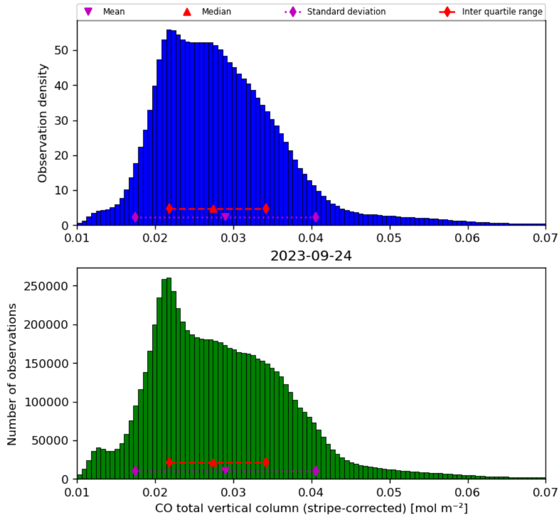
Figure 19: Histogram of “CO total vertical column (stripe-corrected)” for 2023-09-23 to 2023-09-25
