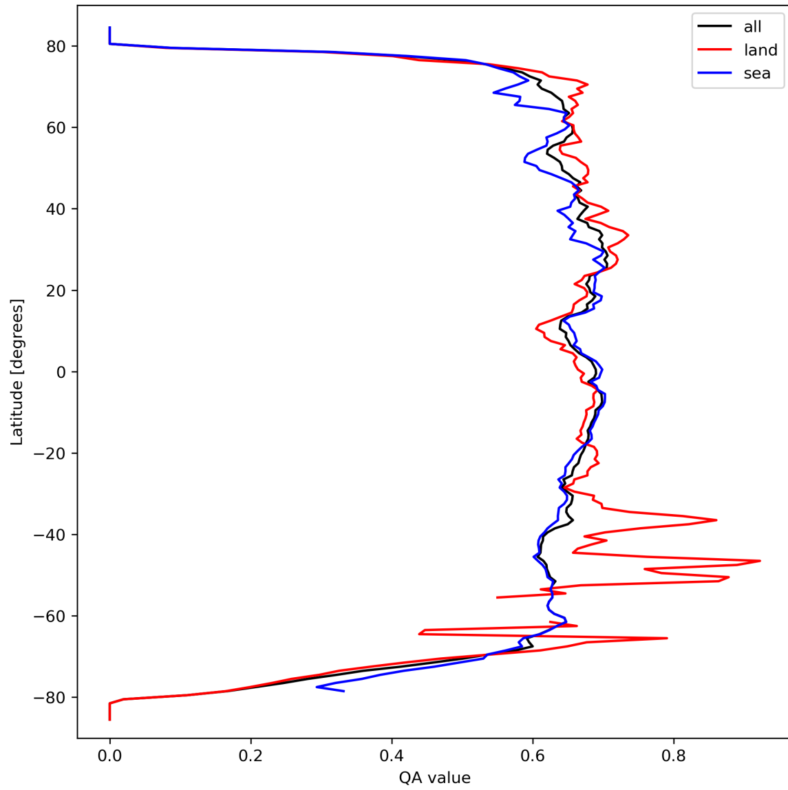
Figure 9: Zonal average of “QA value” for 2023-09-23 to 2023-09-25.
