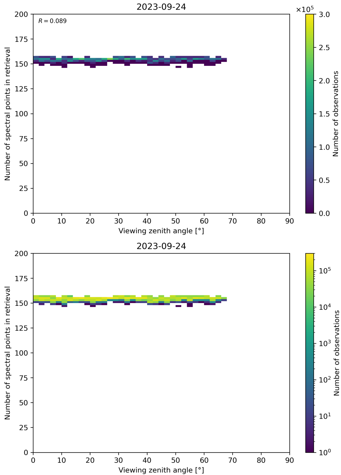
Figure 76: Scatter density plot of “Viewing zenith angle” against “Number of spectral points in retrieval” for 2023-09-23 to 2023-09-25.
