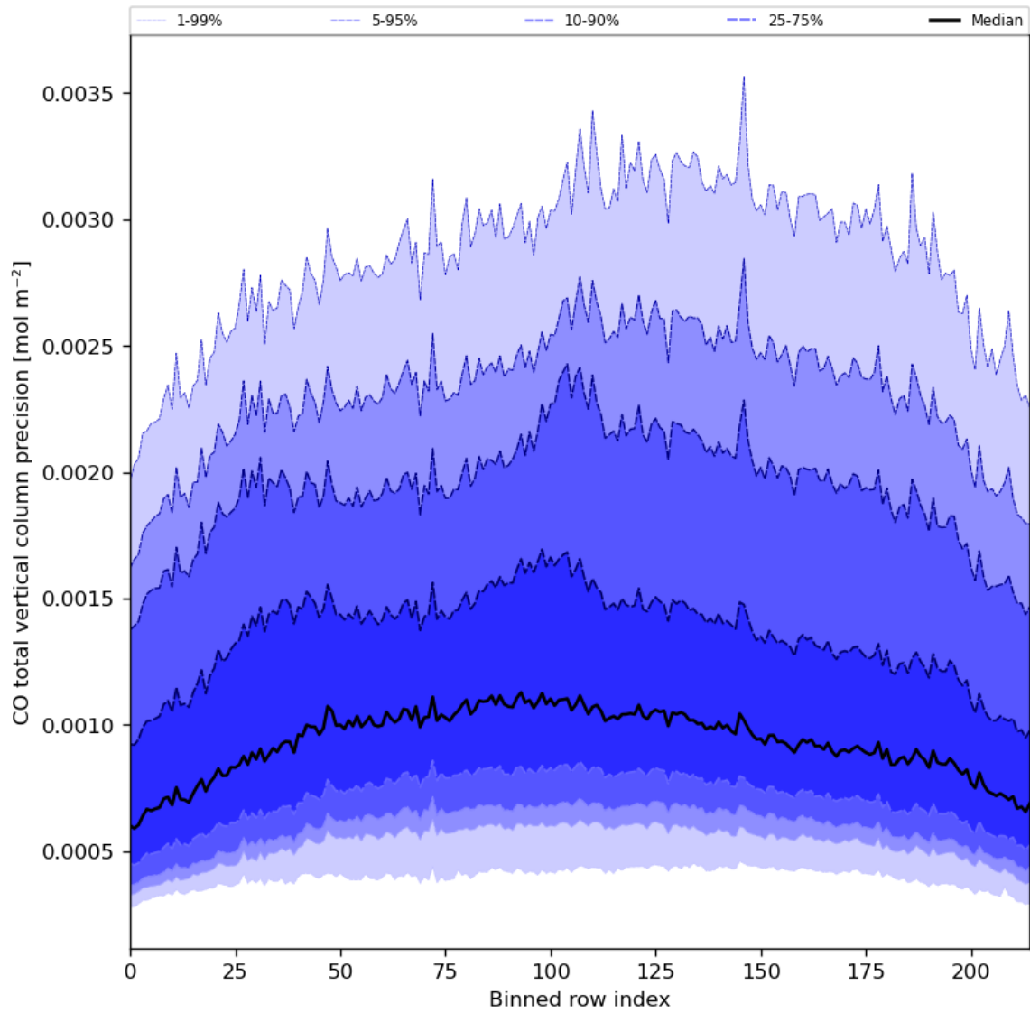
Figure 28: Along track statistics of “CO total vertical column precision” for 2023-09-23 to 2023-09-25
