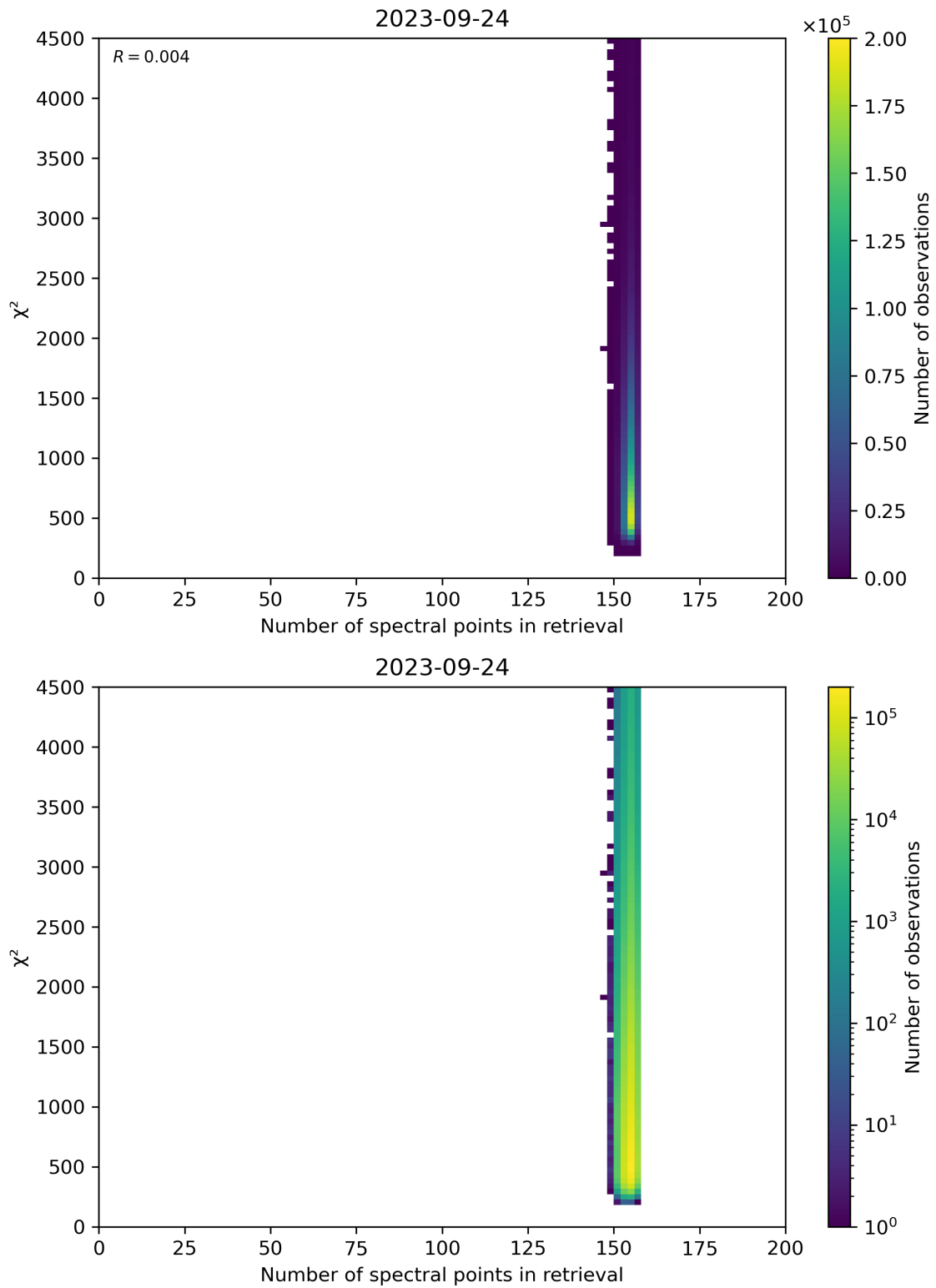
Figure 58: Scatter density plot of “Number of spectral points in retrieval” against “ \chi^2 ” for 2023-09-23 to 2023-09-25.
