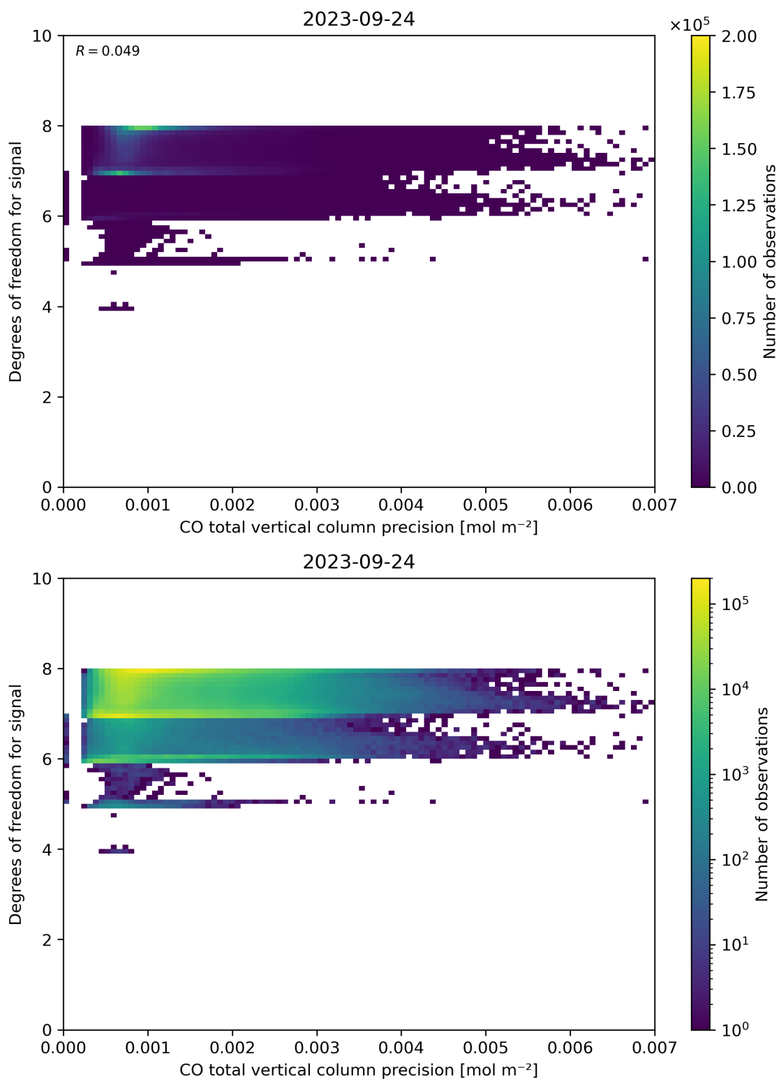
Figure 45: Scatter density plot of “CO total vertical column precision” against “Degrees of freedom for signal” for 2023-09-23 to 2023-09-25.
