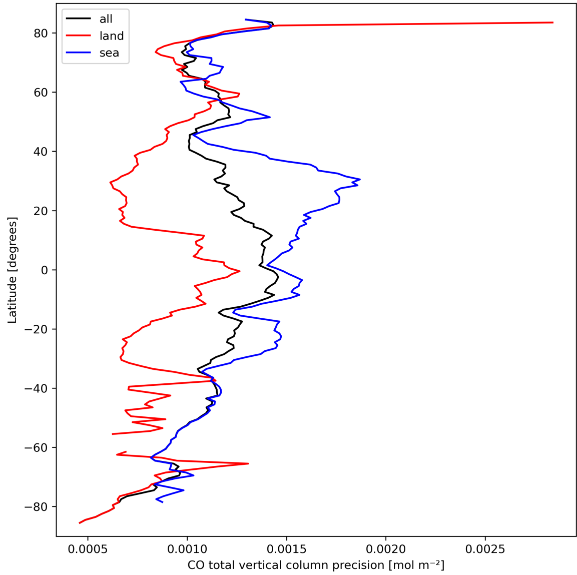
Figure 12: Zonal average of “CO total vertical column precision” for 2023-09-23 to 2023-09-25.
