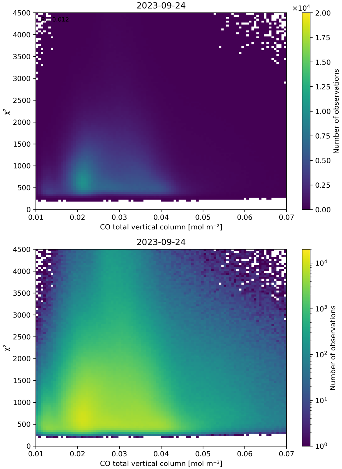
Figure 35: Scatter density plot of “CO total vertical column” against “ \chi^2 ” for 2023-09-23 to 2023-09-25.
