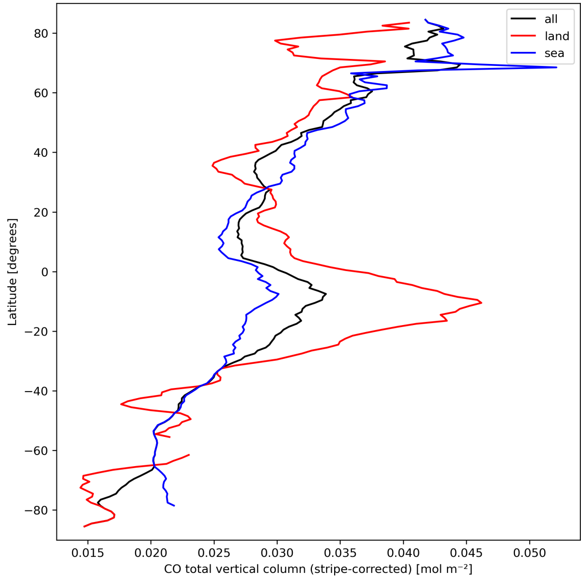
Figure 11: Zonal average of “CO total vertical column (stripe-corrected)” for 2023-09-23 to 2023-09-25.
