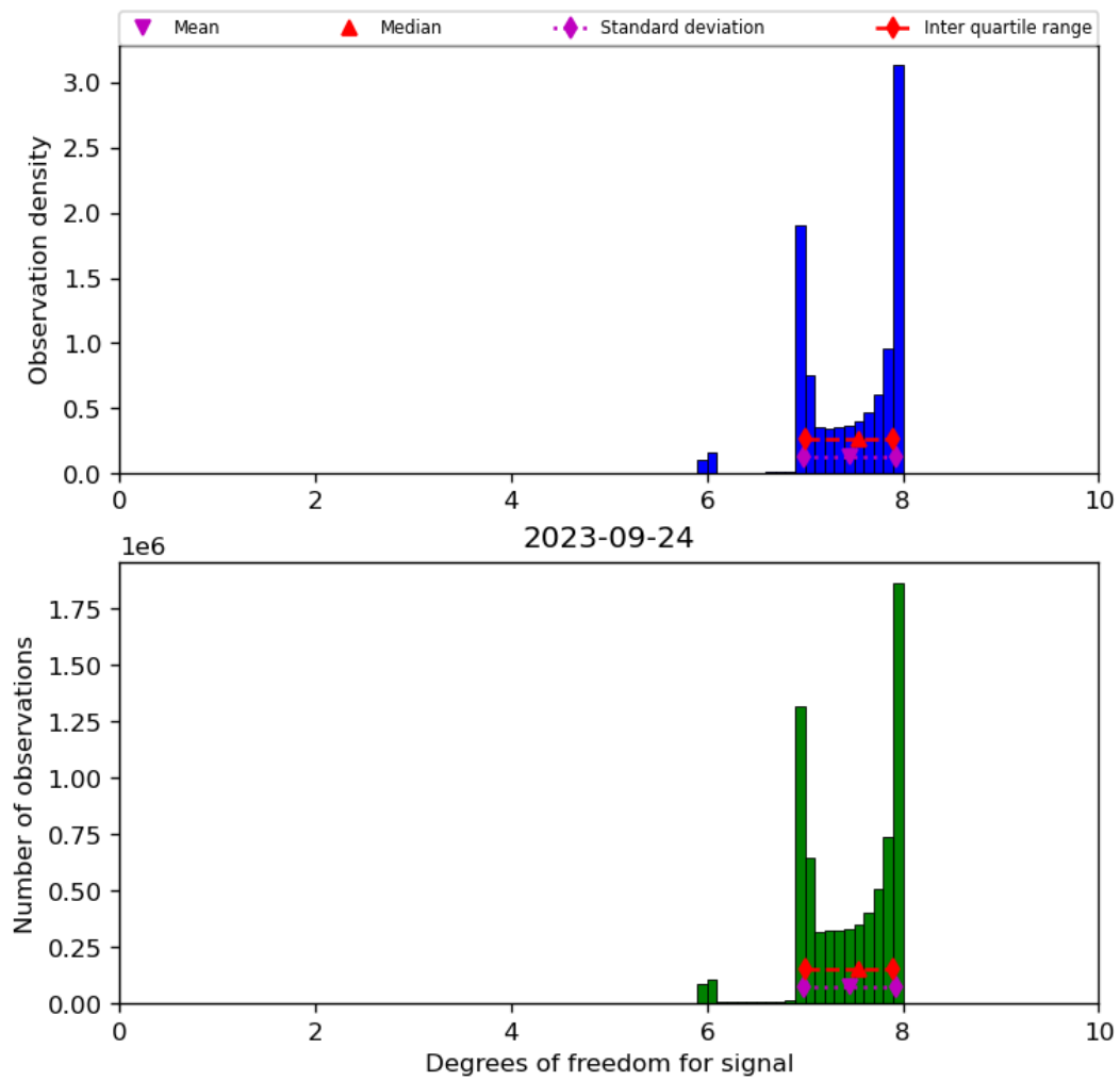
Figure 23: Histogram of “Degrees of freedom for signal” for 2023-09-23 to 2023-09-25
