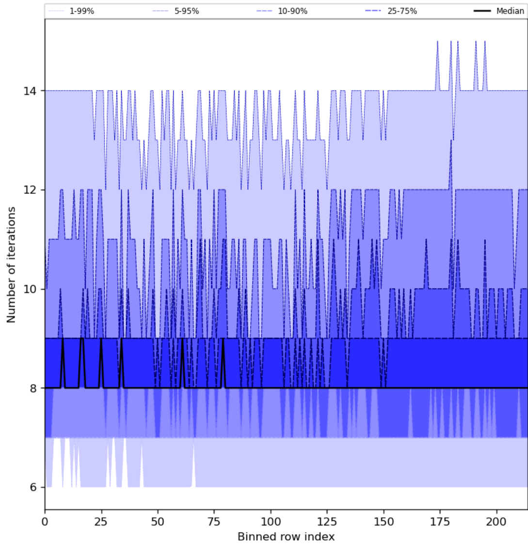
Figure 32: Along track statistics of “Number of iterations” for 2023-09-23 to 2023-09-25
