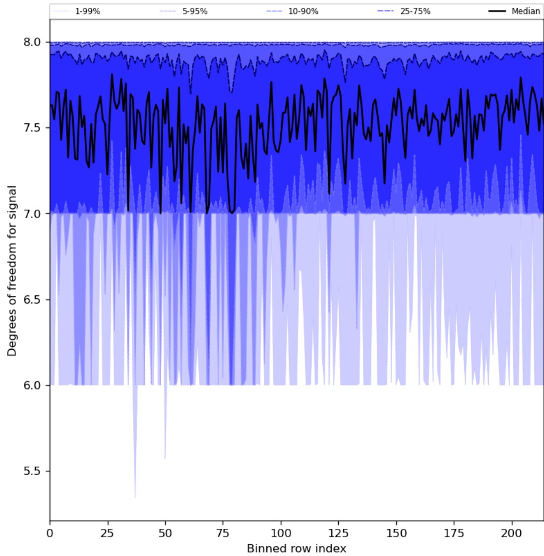
Figure 31: Along track statistics of “Degrees of freedom for signal” for 2023-09-23 to 2023-09-25
