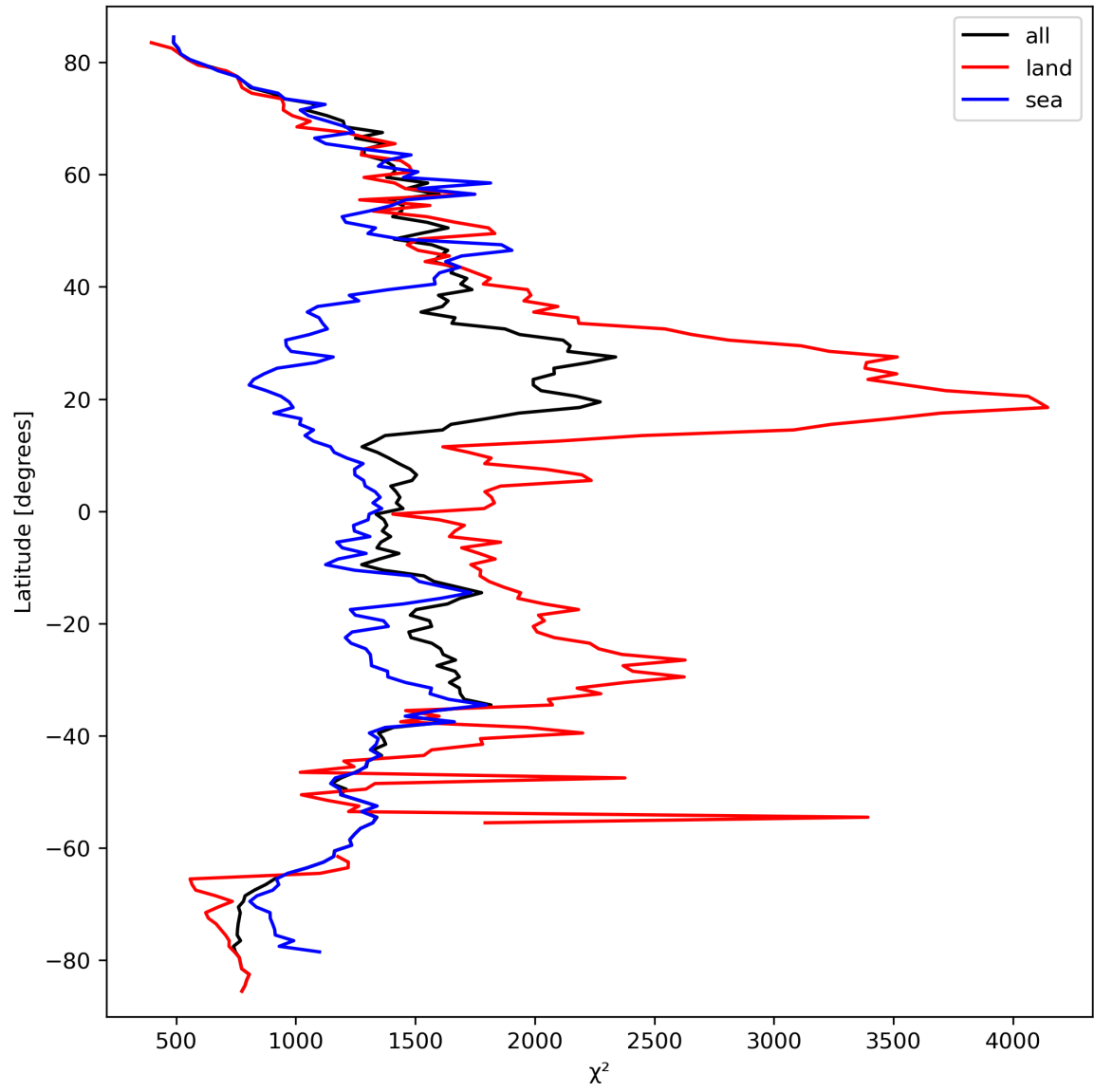
Figure 14: Zonal average of “ \chi^2 ” for 2023-09-23 to 2023-09-25.
