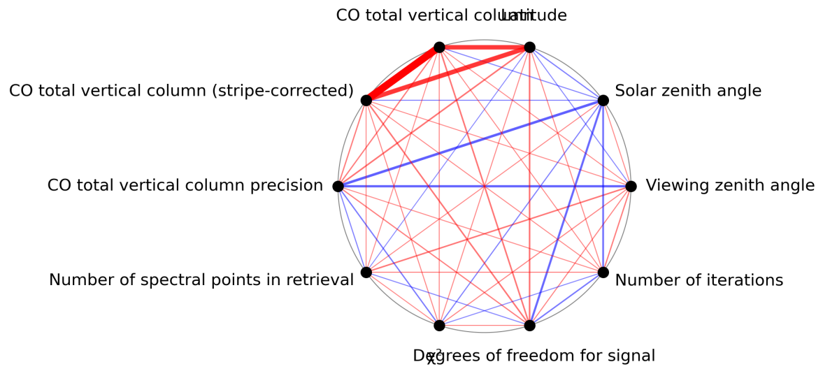
Figure 1: Map of correlation graph for 2023-09-23 to 2023-09-25.
