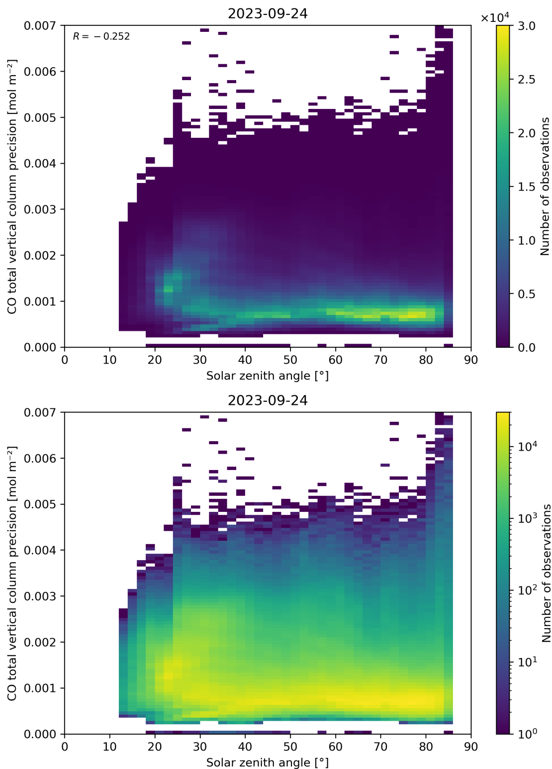
Figure 63: Scatter density plot of “Solar zenith angle” against “CO total vertical column precision” for 2023-09-23 to 2023-09-25.
