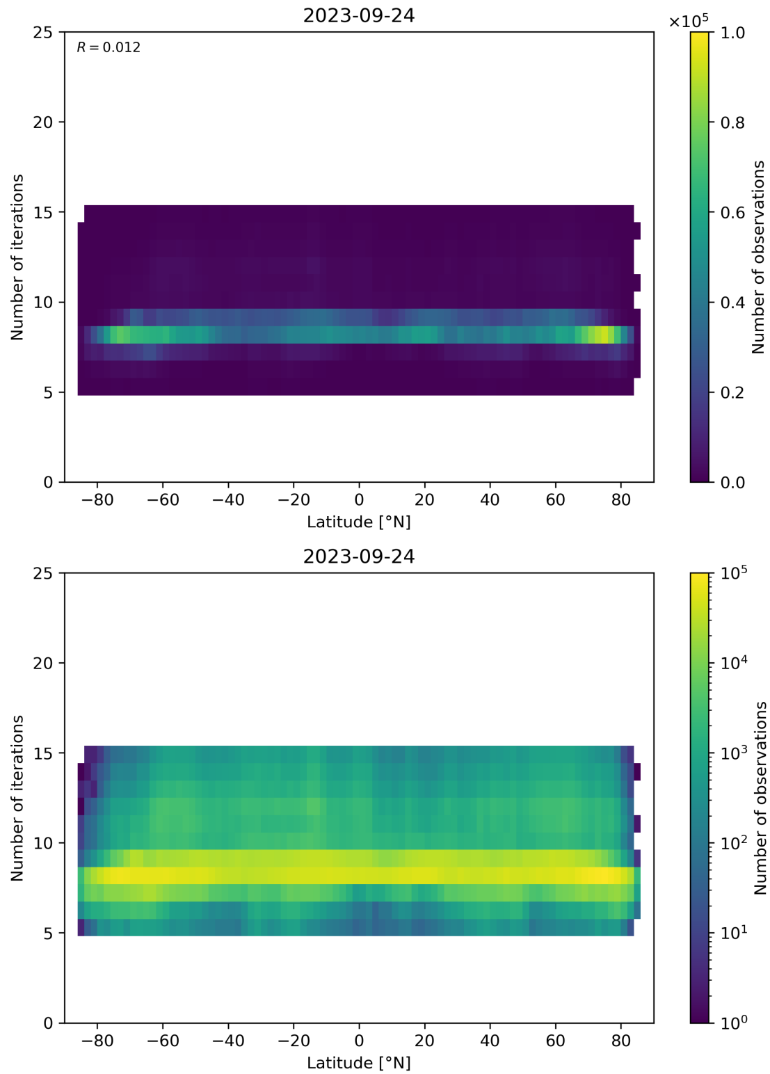
Figure 56: Scatter density plot of “Latitude” against “Number of iterations” for 2023-09-23 to 2023-09-25.
