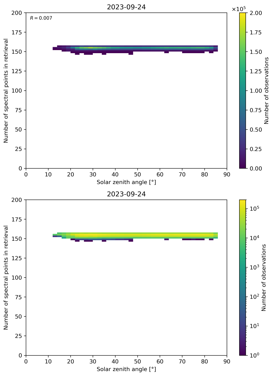
Figure 68: Scatter density plot of “Solar zenith angle” against “Number of spectral points in retrieval” for 2023-09-23 to 2023-09-25.
