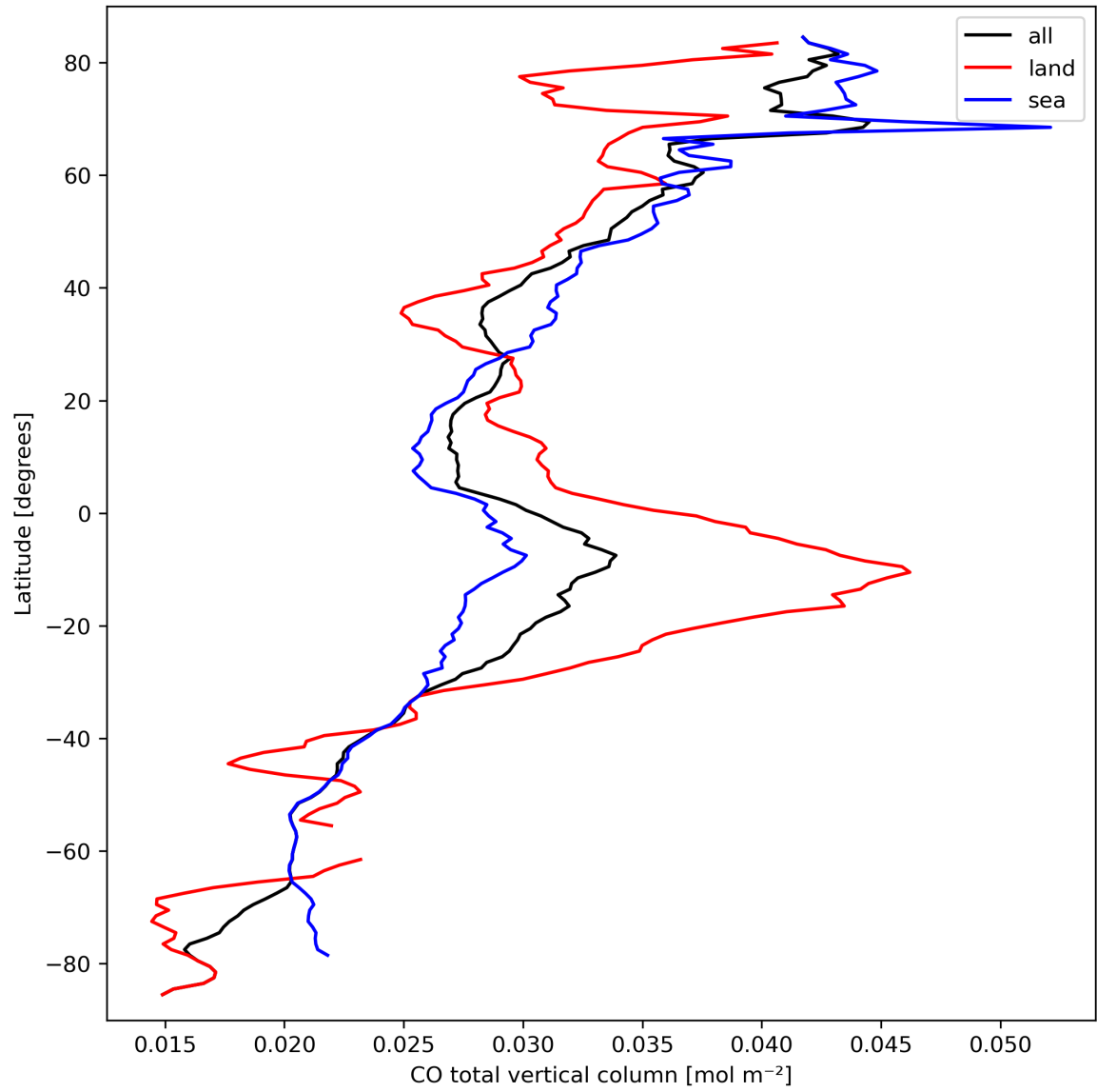
Figure 10: Zonal average of “CO total vertical column” for 2023-09-23 to 2023-09-25.
