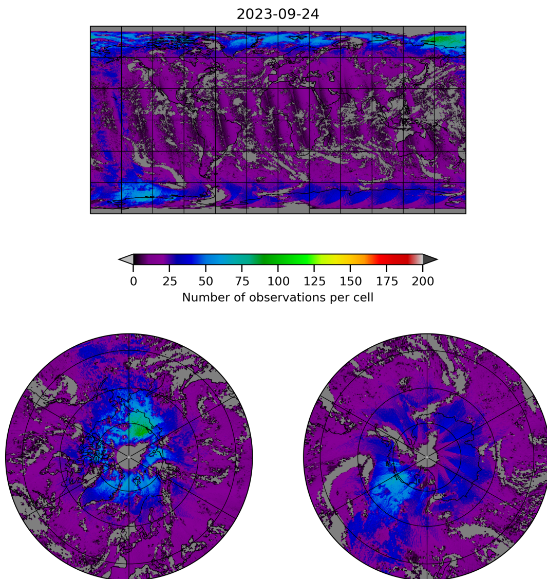
Figure 8: Map of the number of observations for 2023-09-23 to 2023-09-25
