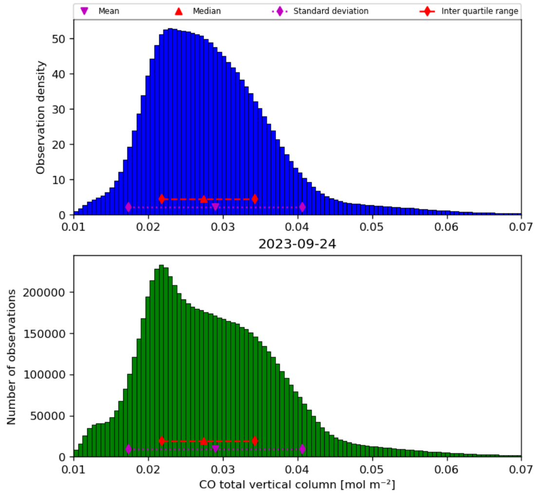
Figure 18: Histogram of “CO total vertical column” for 2023-09-23 to 2023-09-25
