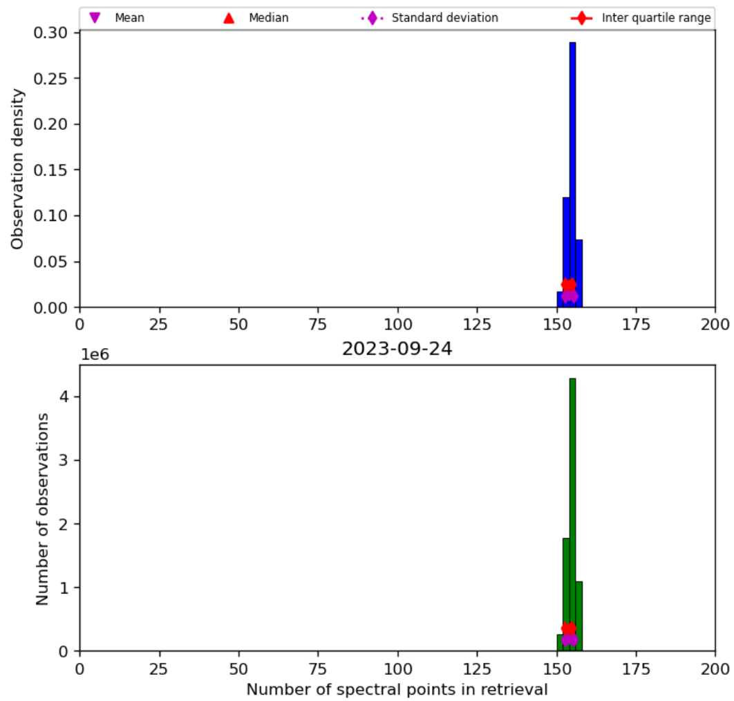
Figure 21: Histogram of “Number of spectral points in retrieval” for 2023-09-23 to 2023-09-25
