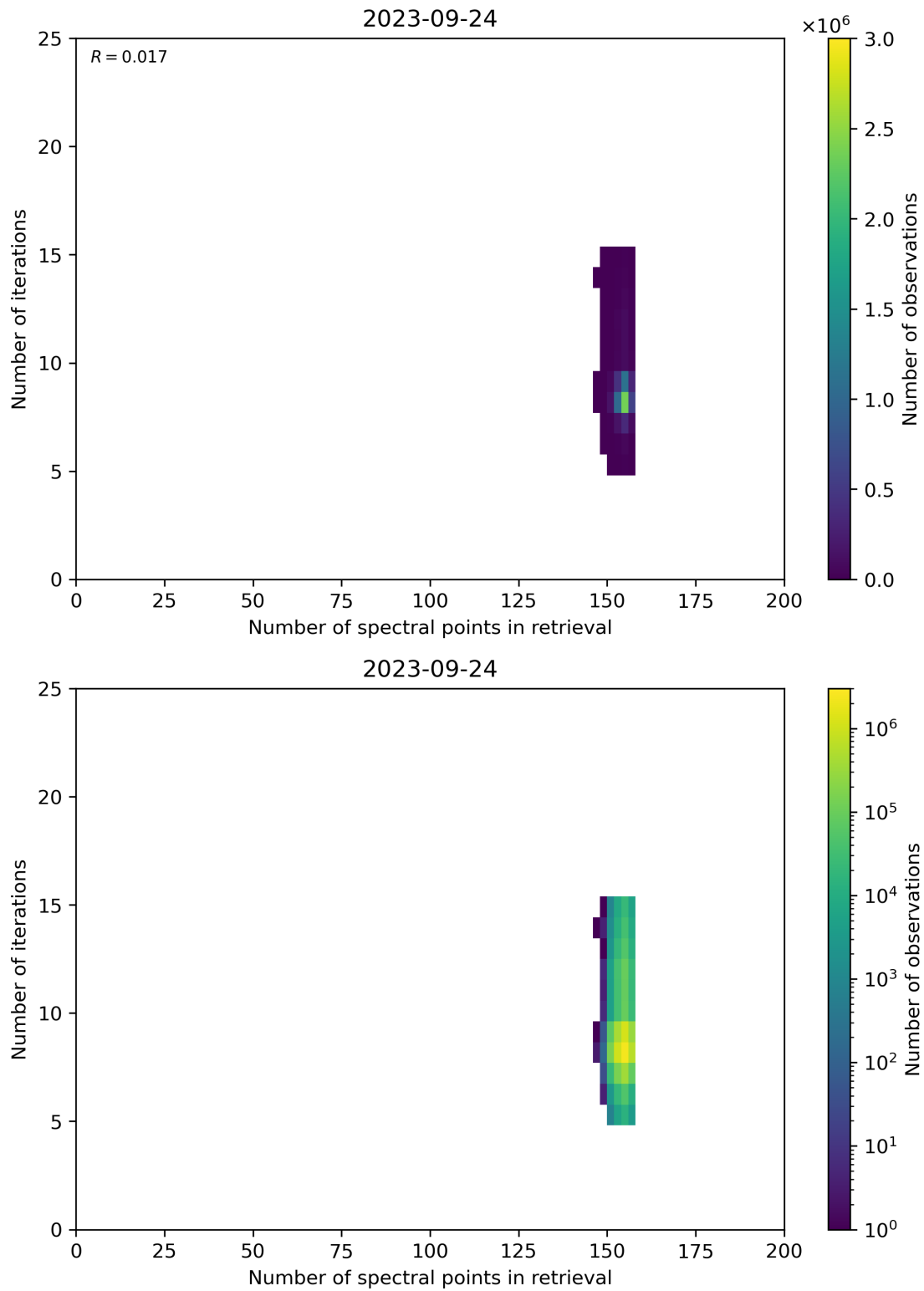
Figure 60: Scatter density plot of “Number of spectral points in retrieval” against “Number of iterations” for 2023-09-23 to 2023-09-25.
