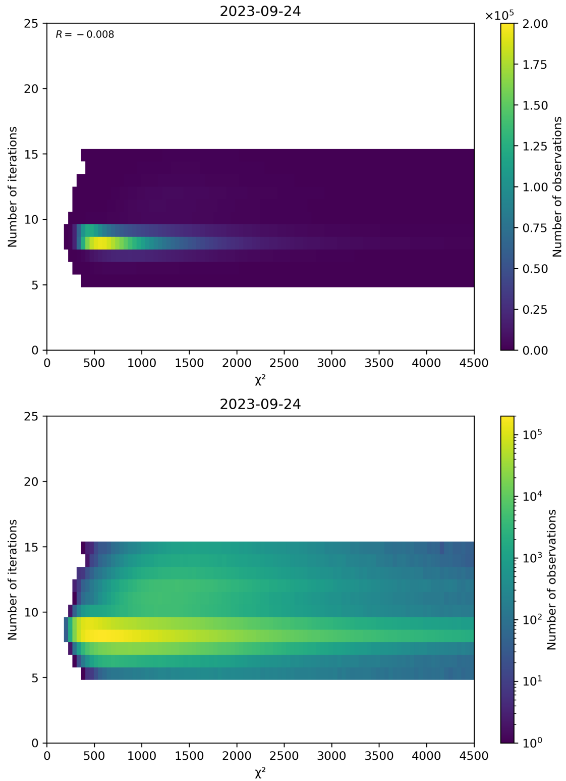
Figure 49: Scatter density plot of “ \chi^2 ” against “Number of iterations” for 2023-09-23 to 2023-09-25.
