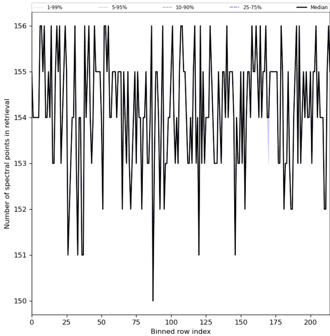
Figure 29: Along track statistics of “Number of spectral points in retrieval” for 2023-09-23 to 2023-09-25
