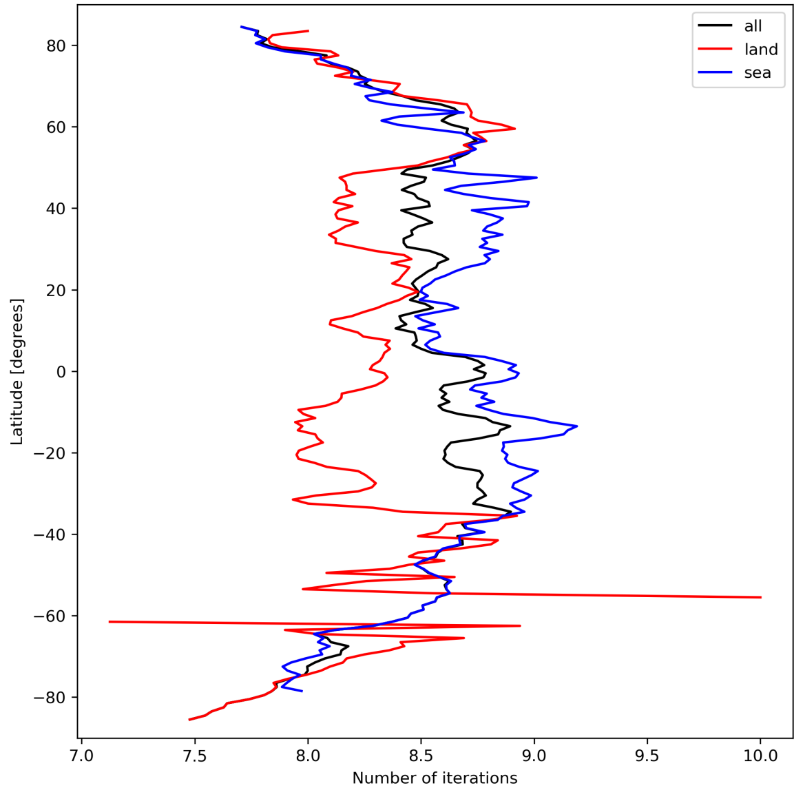
Figure 16: Zonal average of “Number of iterations” for 2023-09-23 to 2023-09-25.
