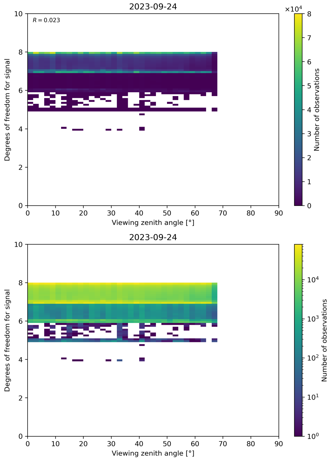
Figure 73: Scatter density plot of “Viewing zenith angle” against “Degrees of freedom for signal” for 2023-09-23 to 2023-09-25.
