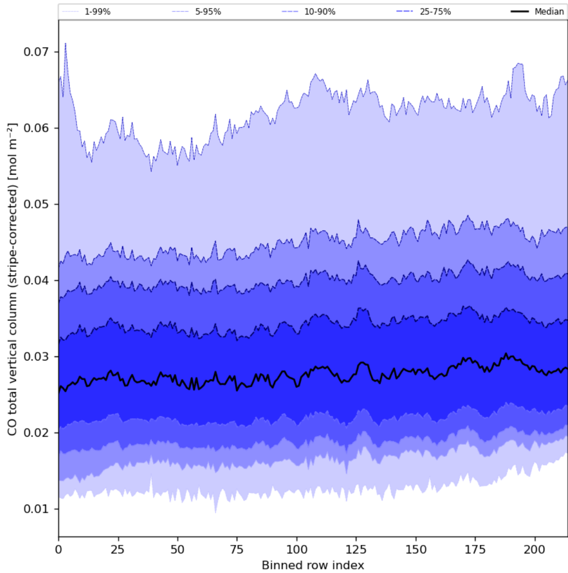
Figure 27: Along track statistics of “CO total vertical column (stripe-corrected)” for 2023-09-23 to 2023-09-25
