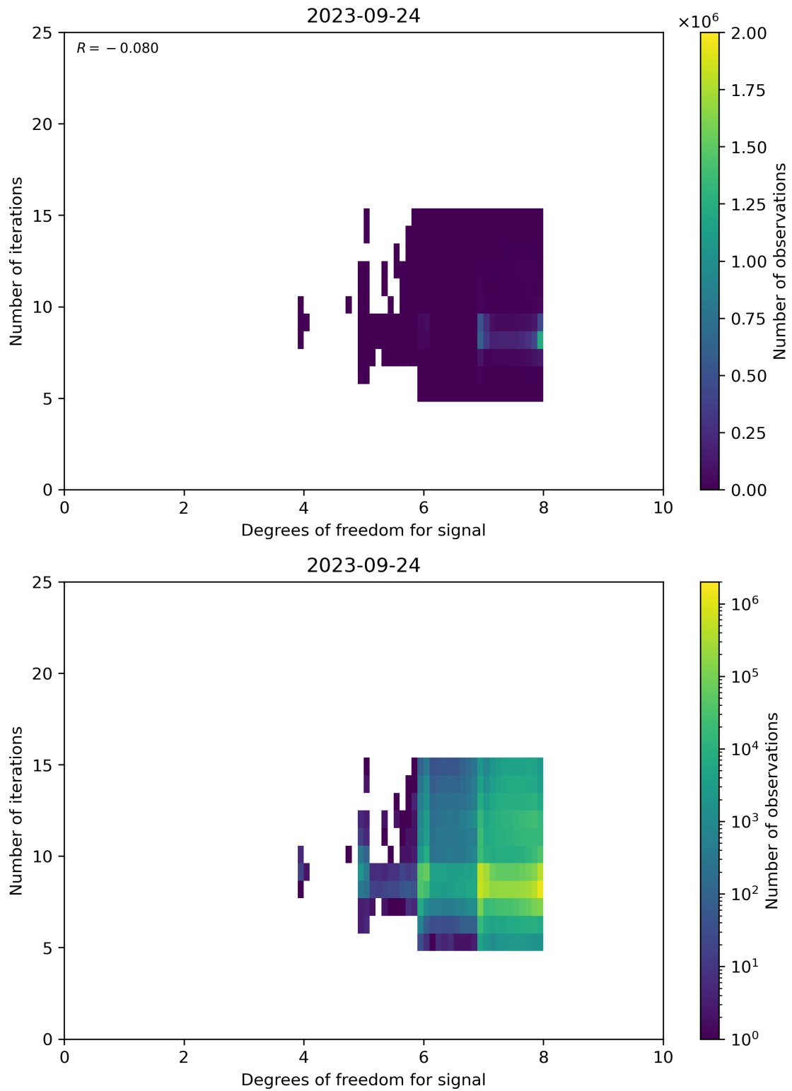
Figure 50: Scatter density plot of “Degrees of freedom for signal” against “Number of iterations” for 2023-09-23 to 2023-09-25.
