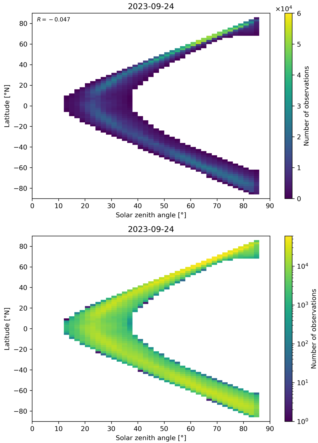
Figure 66: Scatter density plot of “Solar zenith angle” against “Latitude” for 2023-09-23 to 2023-09-25.
