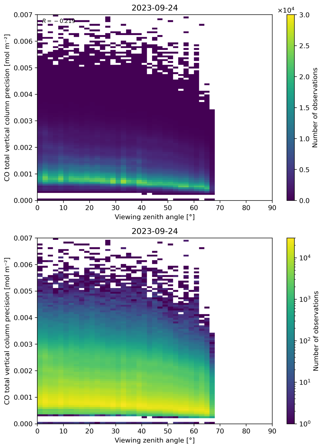
Figure 71: Scatter density plot of “Viewing zenith angle” against “CO total vertical column precision” for 2023-09-23 to 2023-09-25.
