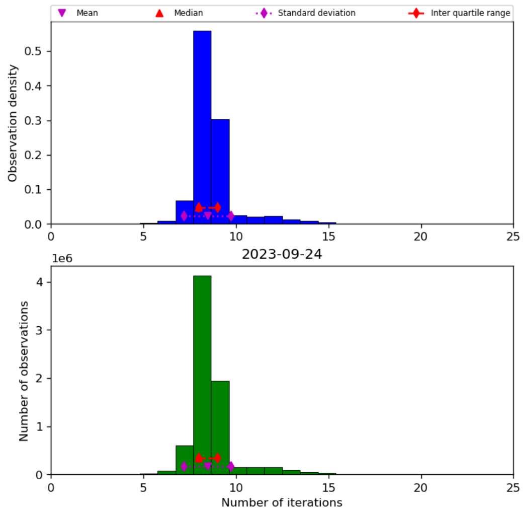
Figure 24: Histogram of “Number of iterations” for 2023-09-23 to 2023-09-25
