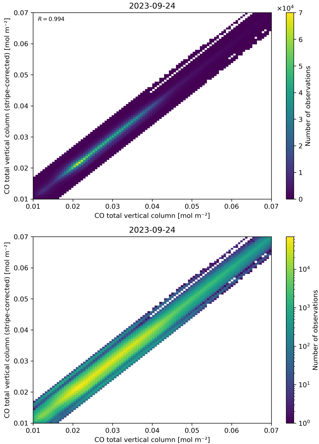
Figure 33: Scatter density plot of “CO total vertical column” against “CO total vertical column (stripe-corrected)” for 2023-09-23 to 2023-09-25.
