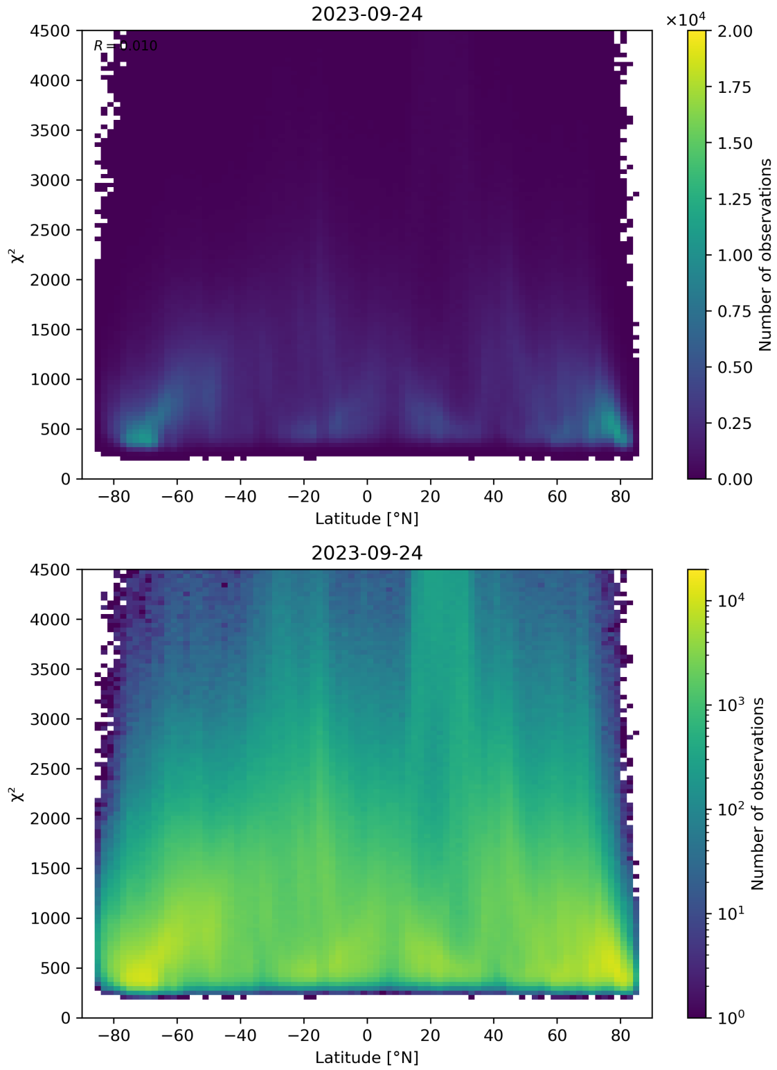
Figure 54: Scatter density plot of “Latitude” against “ \chi^2 ” for 2023-09-23 to 2023-09-25.
