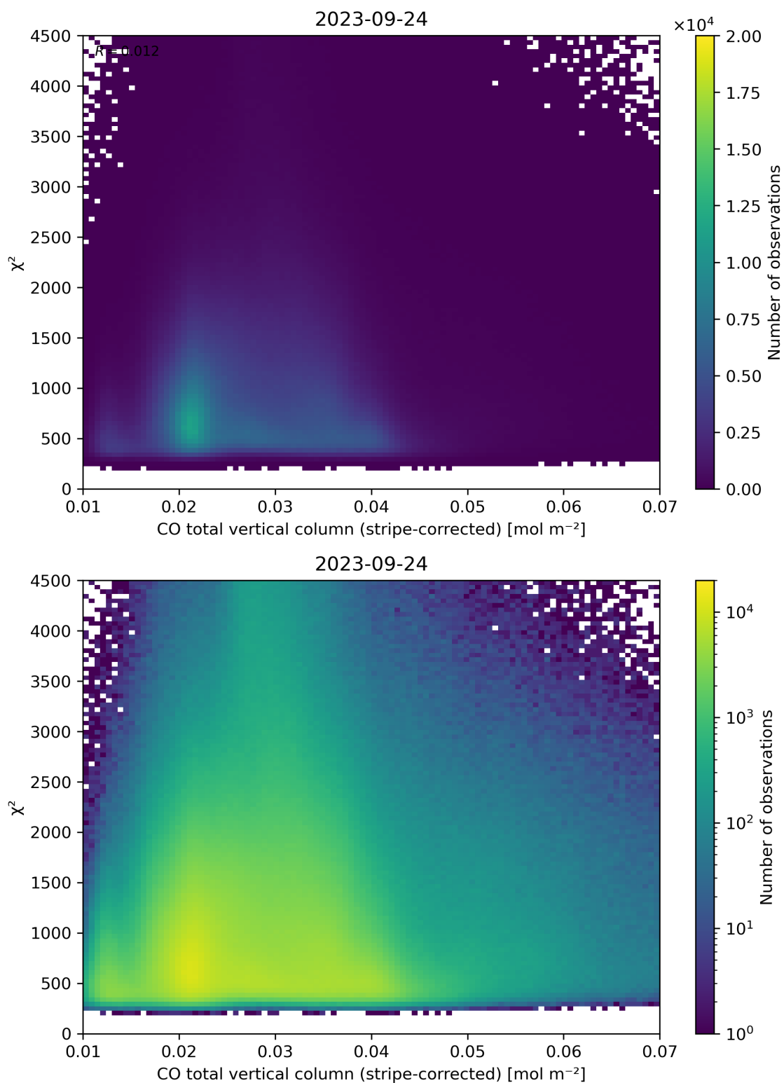
Figure 37: Scatter density plot of “CO total vertical column (stripe-corrected)” against “ \chi^2 ” for 2023-09-23 to 2023-09-25.
