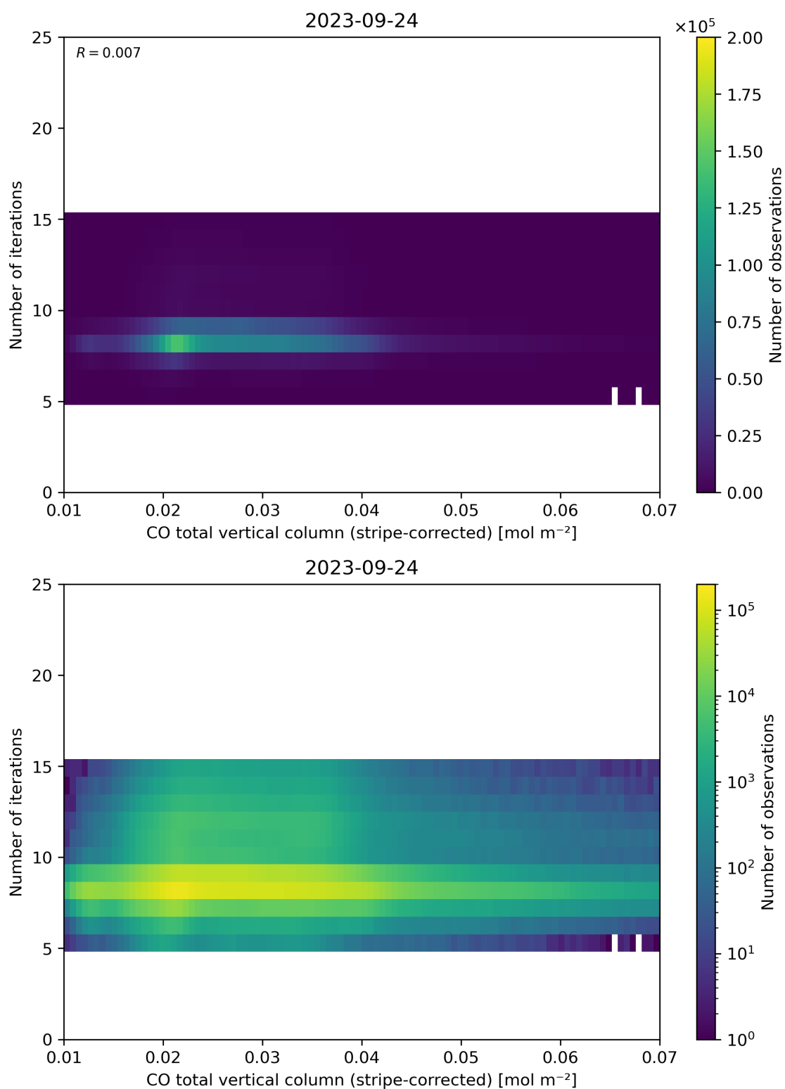
Figure 39: Scatter density plot of “CO total vertical column (stripe-corrected)” against “Number of iterations” for 2023-09-23 to 2023-09-25.
