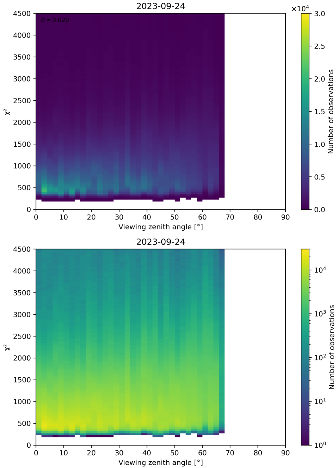
Figure 72: Scatter density plot of “Viewing zenith angle” against “ \chi^2 ” for 2023-09-23 to 2023-09-25.
