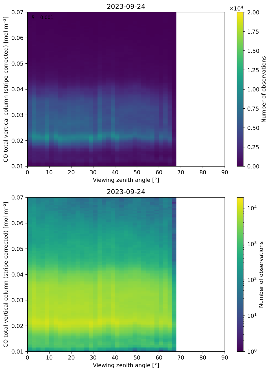
Figure 70: Scatter density plot of “Viewing zenith angle” against “CO total vertical column (stripe-corrected)” for 2023-09-23 to 2023-09-25.
