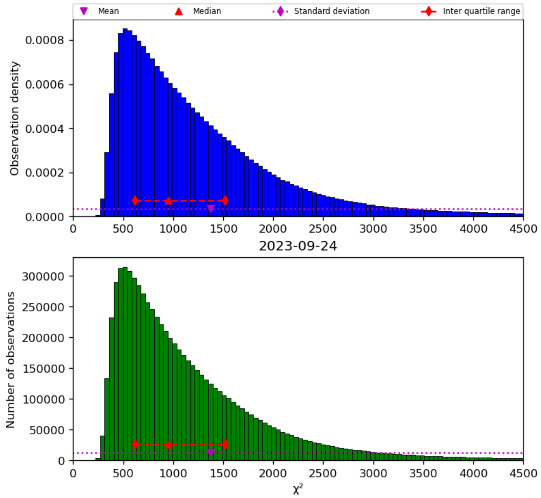
Figure 22: Histogram of “ \chi^2 ” for 2023-09-23 to 2023-09-25
