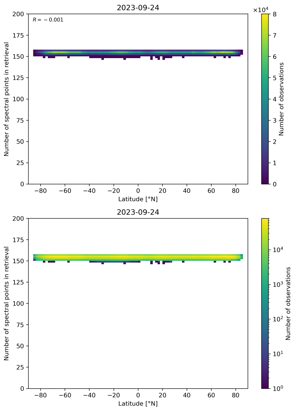
Figure 57: Scatter density plot of “Latitude” against “Number of spectral points in retrieval” for 2023-09-23 to 2023-09-25.
