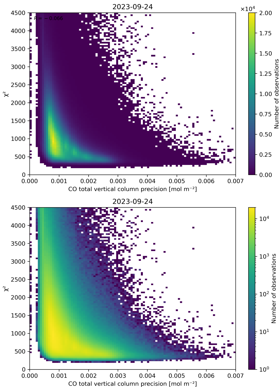
Figure 44: Scatter density plot of “CO total vertical column precision” against “ \chi^2 ” for 2023-09-23 to 2023-09-25.
