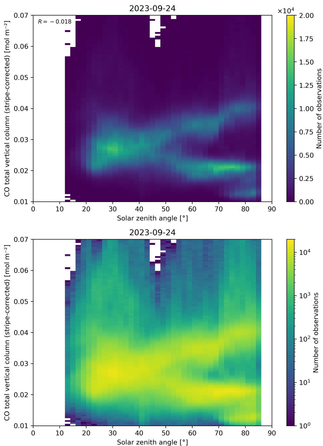
Figure 62: Scatter density plot of “Solar zenith angle” against “CO total vertical column (stripe-corrected)” for 2023-09-23 to 2023-09-25.
