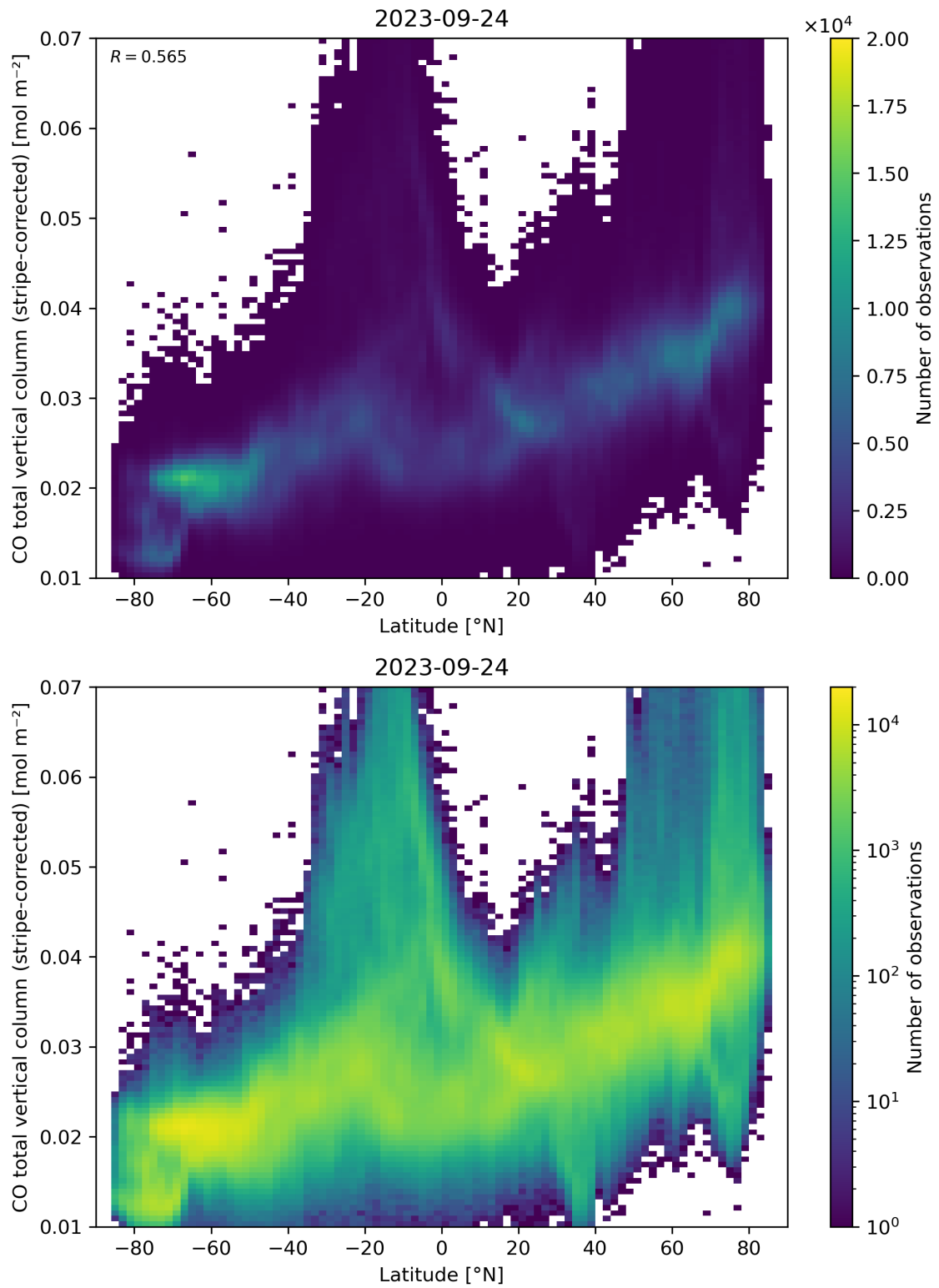
Figure 52: Scatter density plot of “Latitude” against “CO total vertical column (stripe-corrected)” for 2023-09-23 to 2023-09-25.
