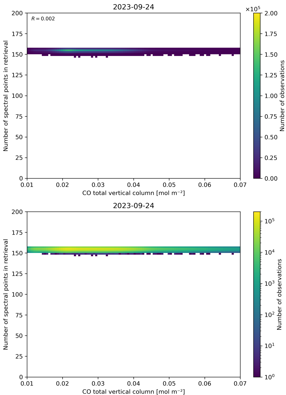
Figure 43: Scatter density plot of “CO total vertical column” against “Number of spectral points in retrieval” for 2023-09-23 to 2023-09-25.
