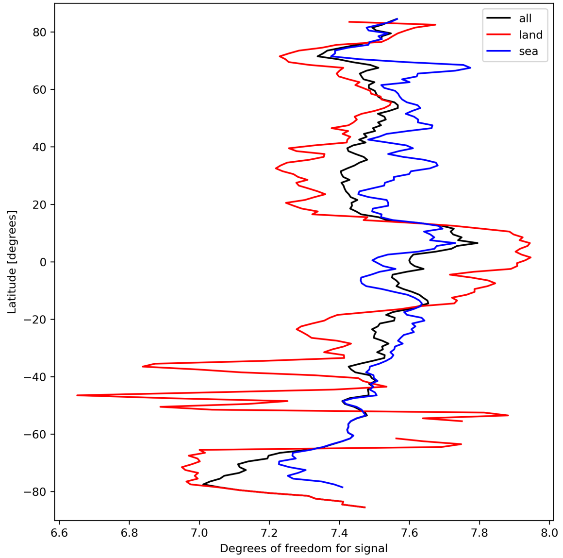
Figure 15: Zonal average of “Degrees of freedom for signal” for 2023-09-23 to 2023-09-25.
