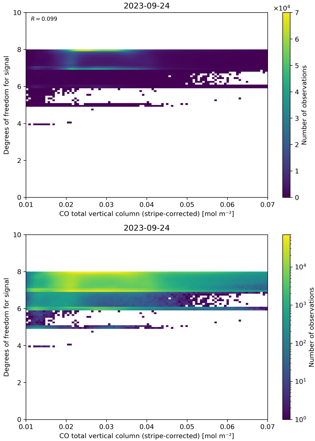
Figure 38: Scatter density plot of “CO total vertical column (stripe-corrected)” against “Degrees of freedom for signal” for 2023-09-23 to 2023-09-25.
