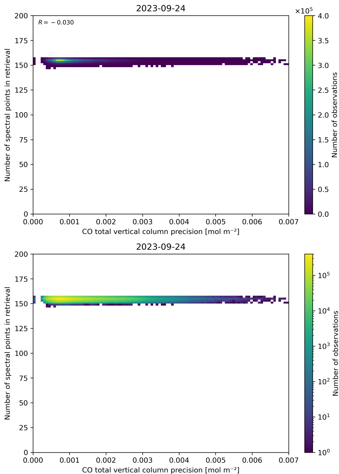
Figure 47: Scatter density plot of “CO total vertical column precision” against “Number of spectral points in retrieval” for 2023-09-23 to 2023-09-25.
