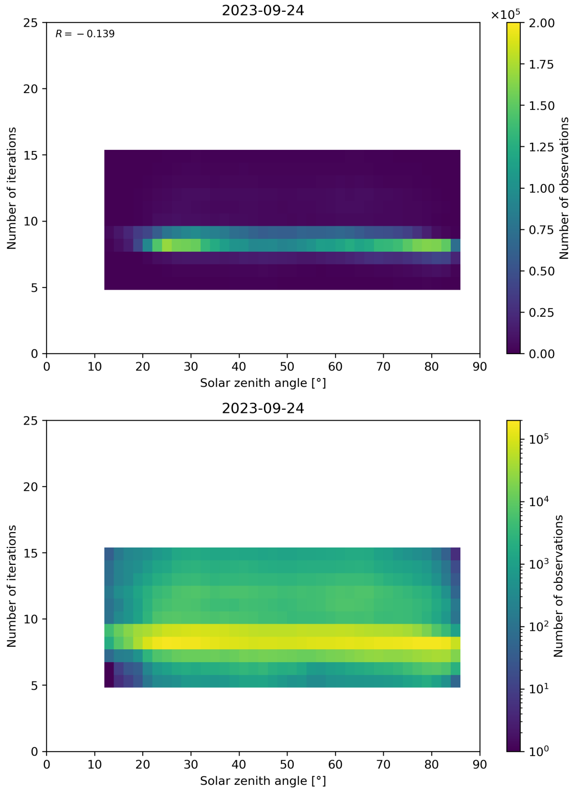
Figure 67: Scatter density plot of “Solar zenith angle” against “Number of iterations” for 2023-09-23 to 2023-09-25.
