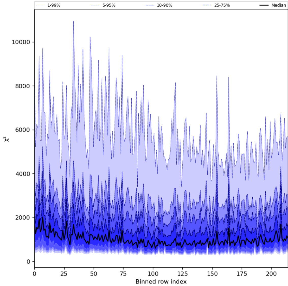
Figure 30: Along track statistics of “ \chi^2 ” for 2023-09-23 to 2023-09-25
