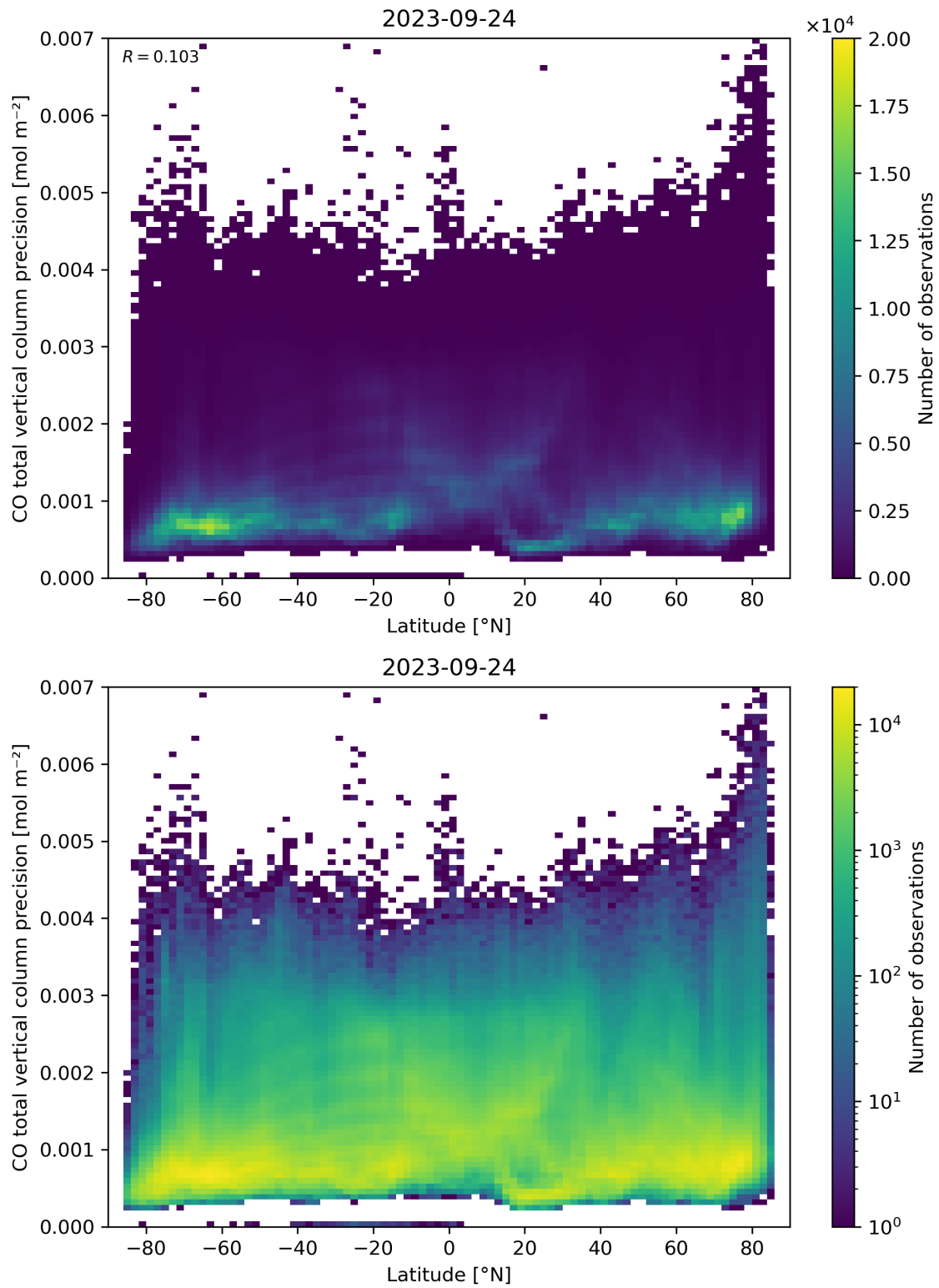
Figure 53: Scatter density plot of “Latitude” against “CO total vertical column precision” for 2023-09-23 to 2023-09-25.
