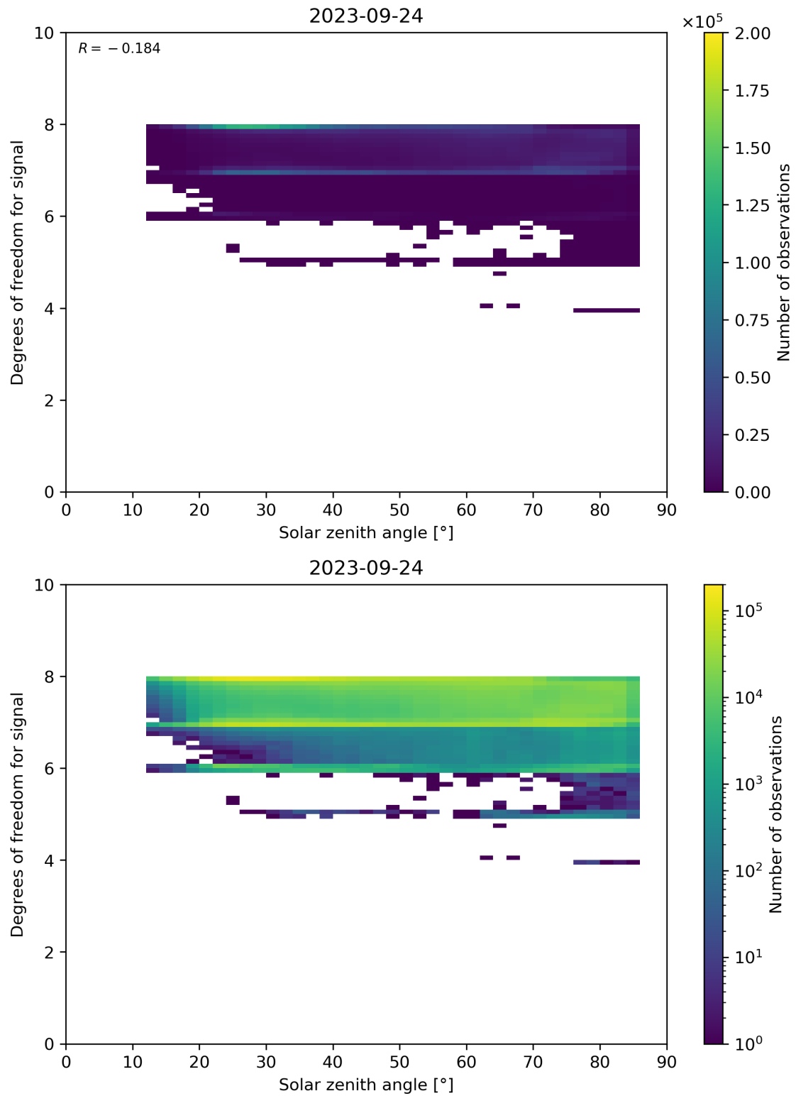
Figure 65: Scatter density plot of “Solar zenith angle” against “Degrees of freedom for signal” for 2023-09-23 to 2023-09-25.
