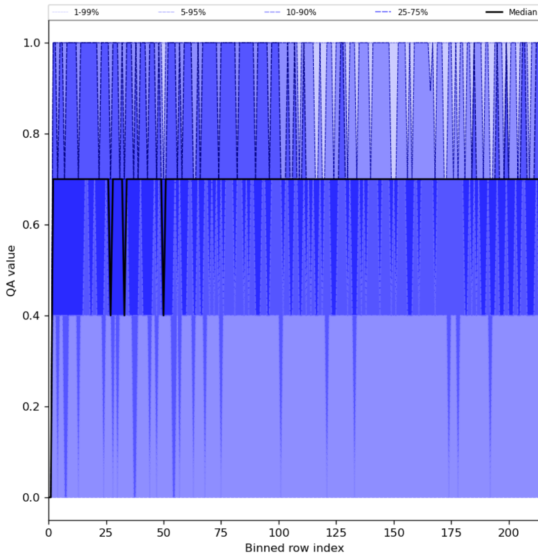
Figure 25: Along track statistics of “QA value” for 2023-09-23 to 2023-09-25
