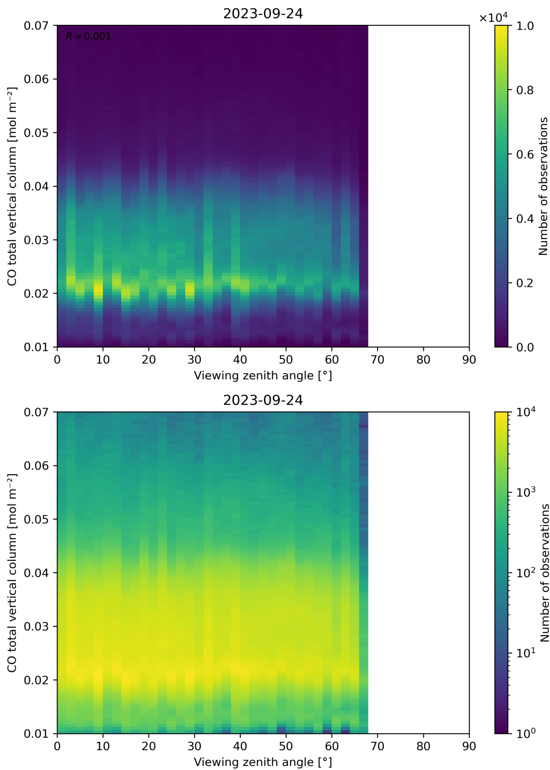
Figure 69: Scatter density plot of “Viewing zenith angle” against “CO total vertical column” for 2023-09-23 to 2023-09-25.
