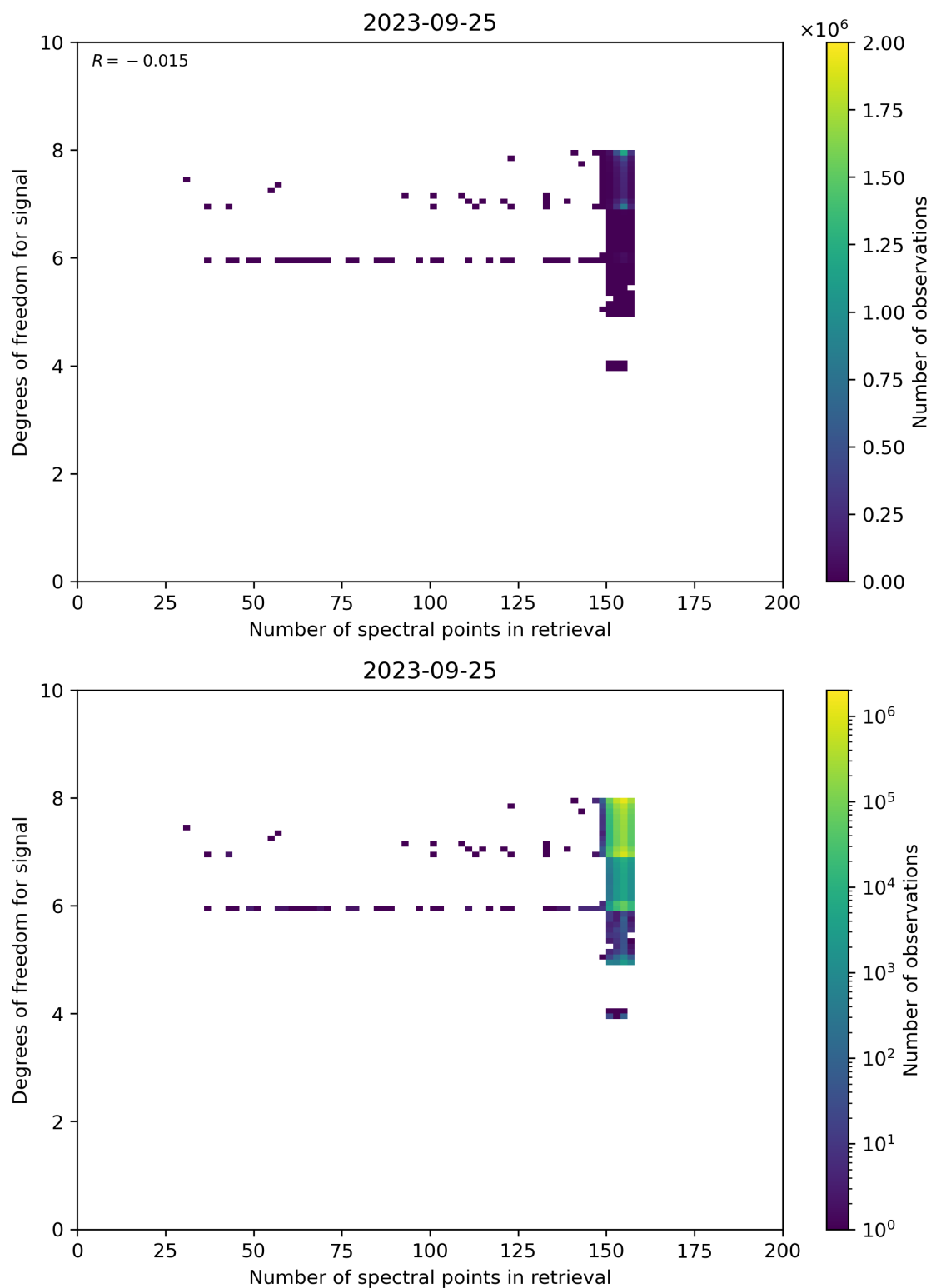
Figure 59: Scatter density plot of “Number of spectral points in retrieval” against “Degrees of freedom for signal” for 2023-09-24 to 2023-09-26.
