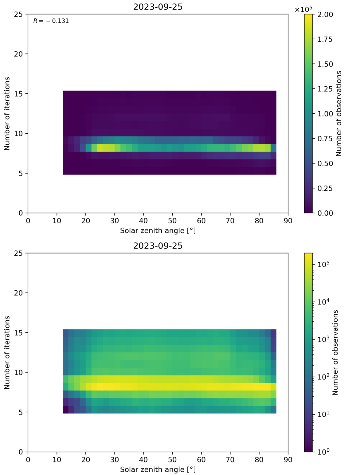
Figure 67: Scatter density plot of “Solar zenith angle” against “Number of iterations” for 2023-09-24 to 2023-09-26.
