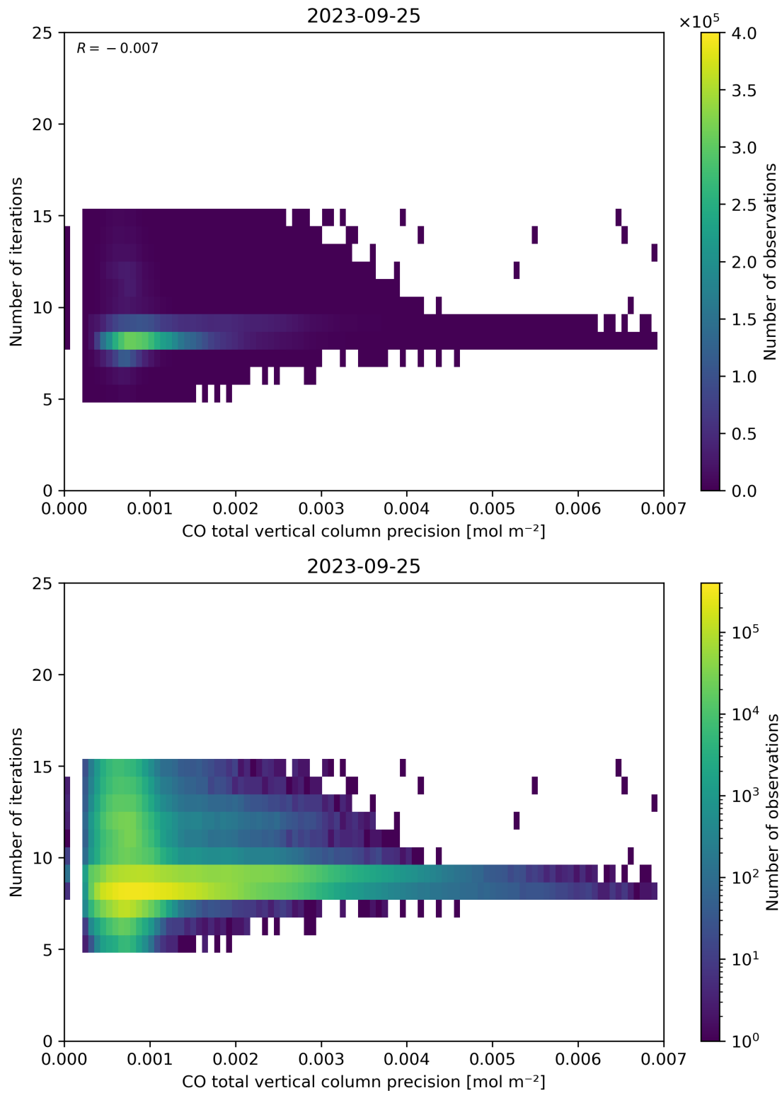
Figure 46: Scatter density plot of “CO total vertical column precision” against “Number of iterations” for 2023-09-24 to 2023-09-26.
