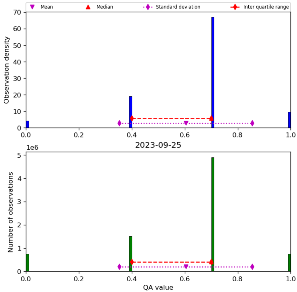
Figure 17: Histogram of “QA value” for 2023-09-24 to 2023-09-26
