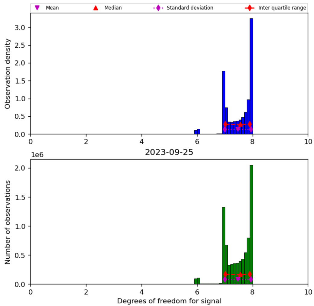
Figure 23: Histogram of “Degrees of freedom for signal” for 2023-09-24 to 2023-09-26
