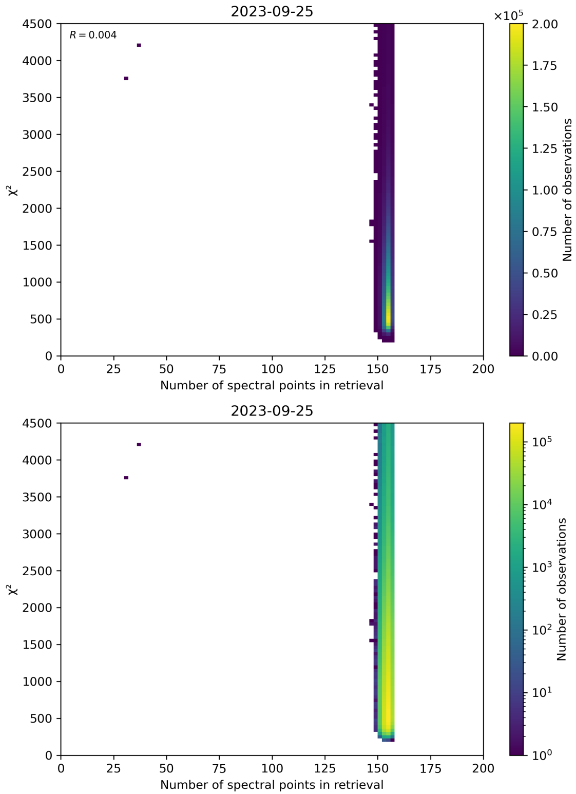
Figure 58: Scatter density plot of “Number of spectral points in retrieval” against “ \chi^2 ” for 2023-09-24 to 2023-09-26.
