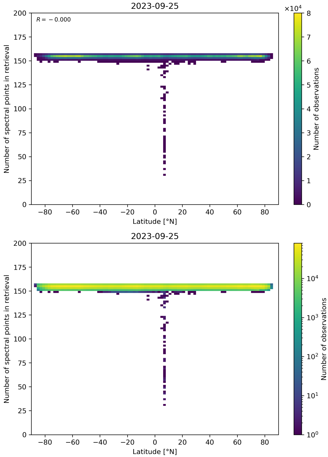
Figure 57: Scatter density plot of “Latitude” against “Number of spectral points in retrieval” for 2023-09-24 to 2023-09-26.
