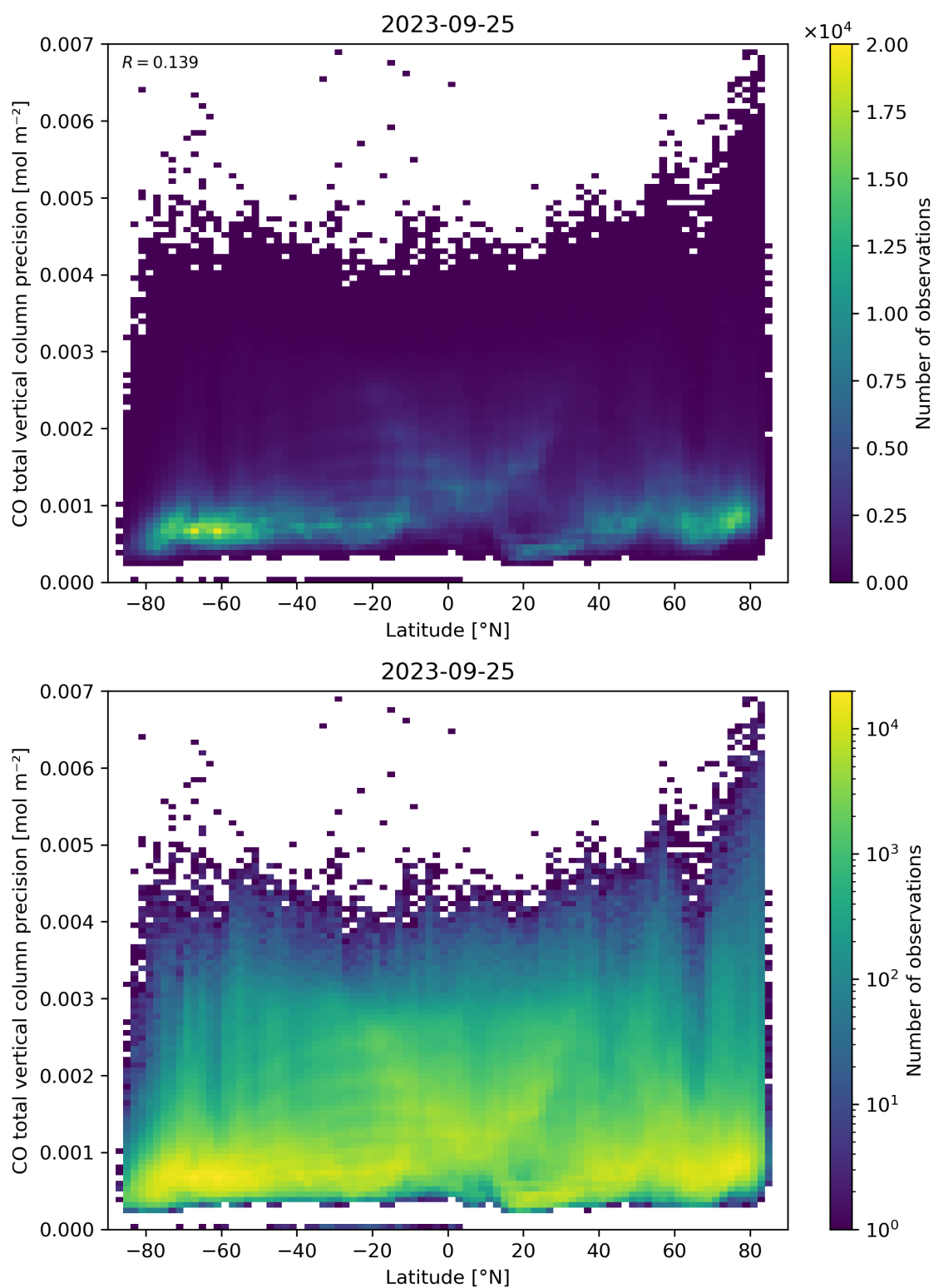
Figure 53: Scatter density plot of “Latitude” against “CO total vertical column precision” for 2023-09-24 to 2023-09-26.
