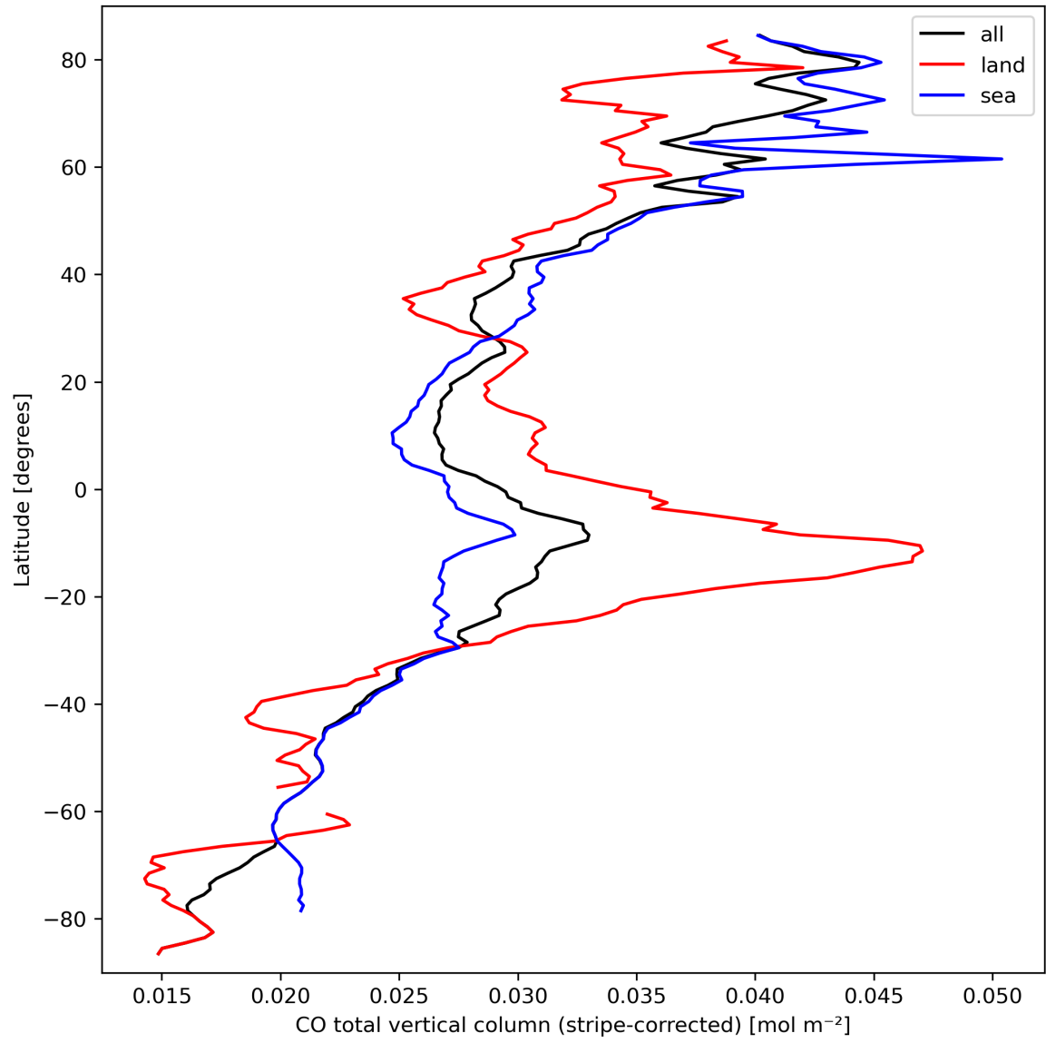
Figure 11: Zonal average of “CO total vertical column (stripe-corrected)” for 2023-09-24 to 2023-09-26.
