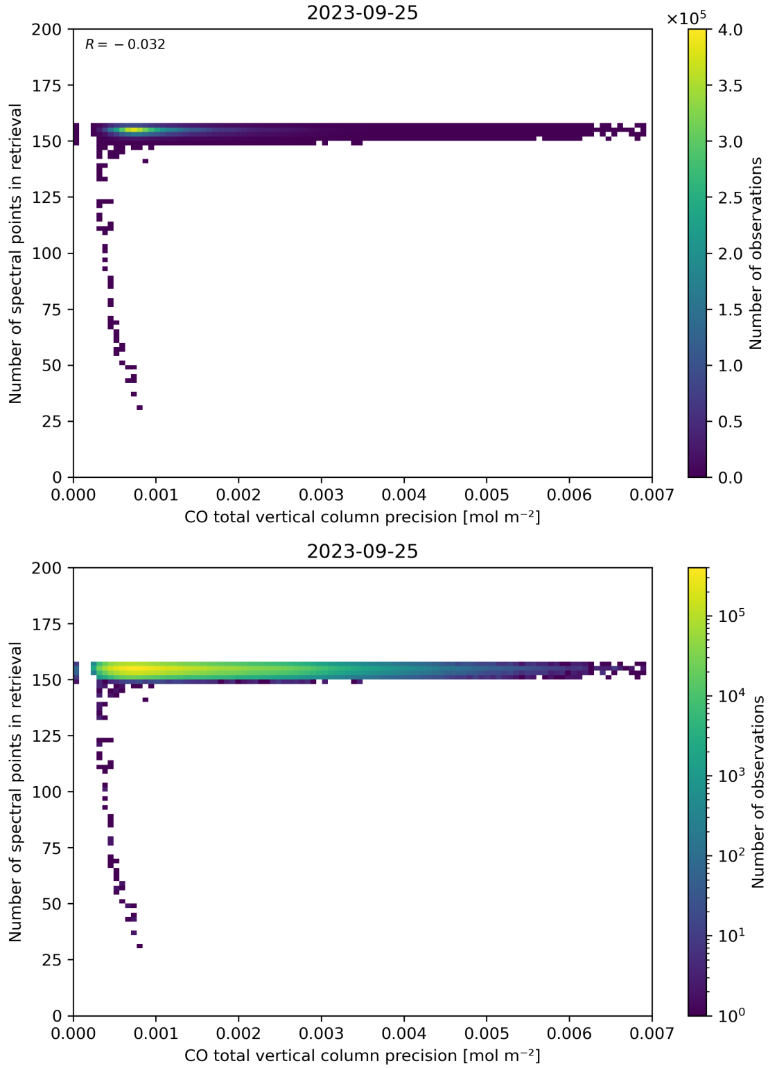
Figure 47: Scatter density plot of “CO total vertical column precision” against “Number of spectral points in retrieval” for 2023-09-24 to 2023-09-26.
