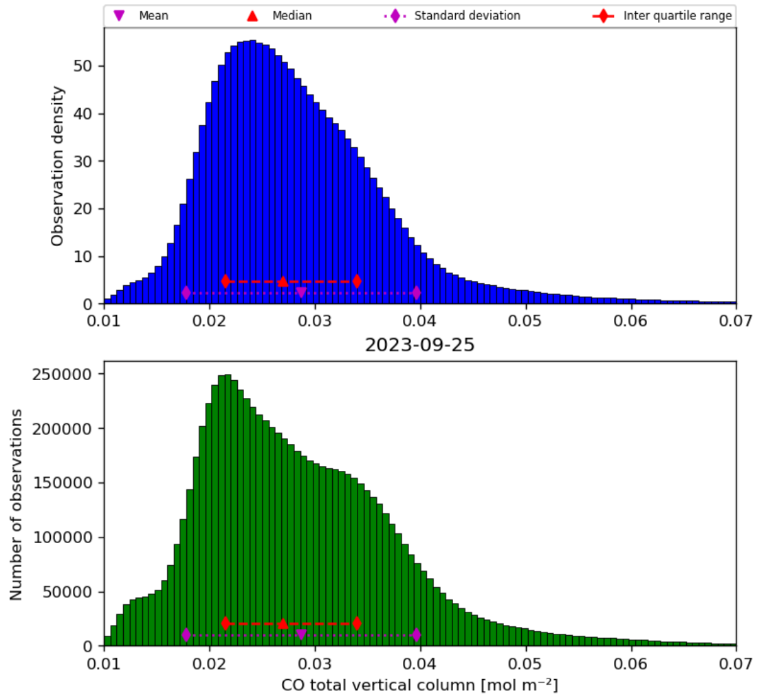
Figure 18: Histogram of “CO total vertical column” for 2023-09-24 to 2023-09-26
