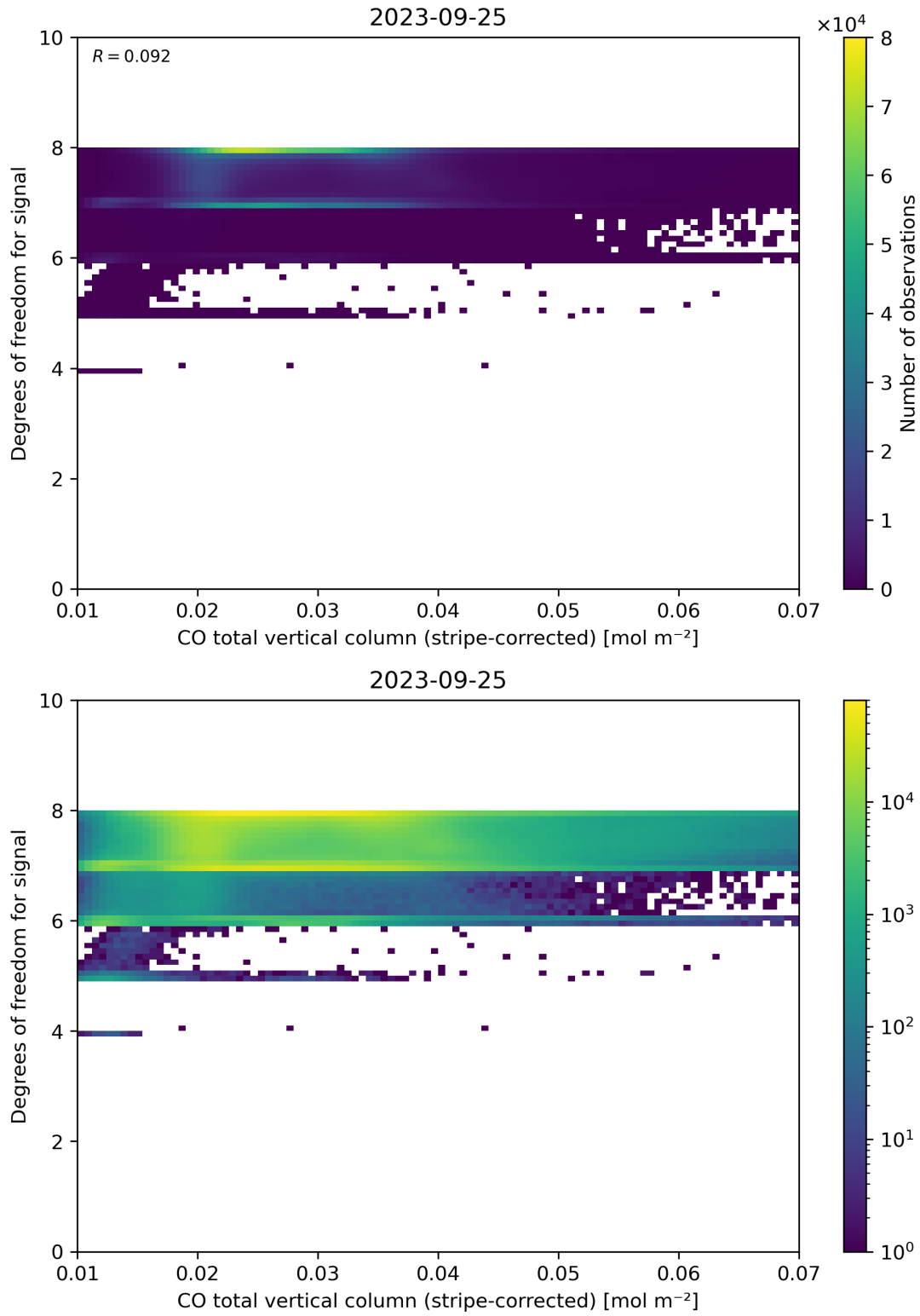
Figure 38: Scatter density plot of “CO total vertical column (stripe-corrected)” against “Degrees of freedom for signal” for 2023-09-24 to 2023-09-26.
