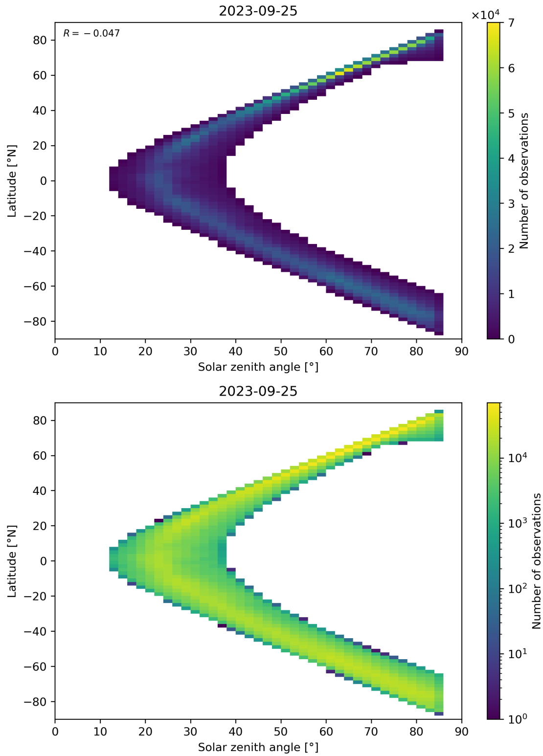
Figure 66: Scatter density plot of “Solar zenith angle” against “Latitude” for 2023-09-24 to 2023-09-26.
