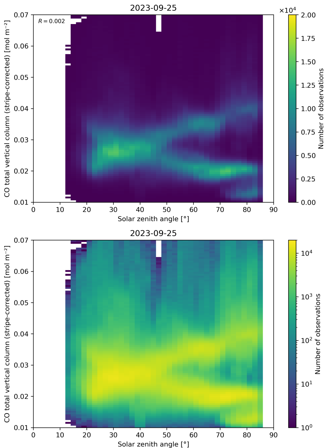
Figure 62: Scatter density plot of “Solar zenith angle” against “CO total vertical column (stripe-corrected)” for 2023-09-24 to 2023-09-26.
