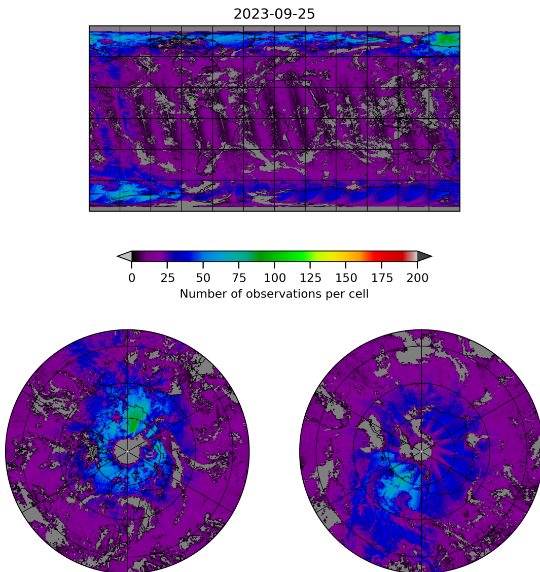
Figure 8: Map of the number of observations for 2023-09-24 to 2023-09-26
