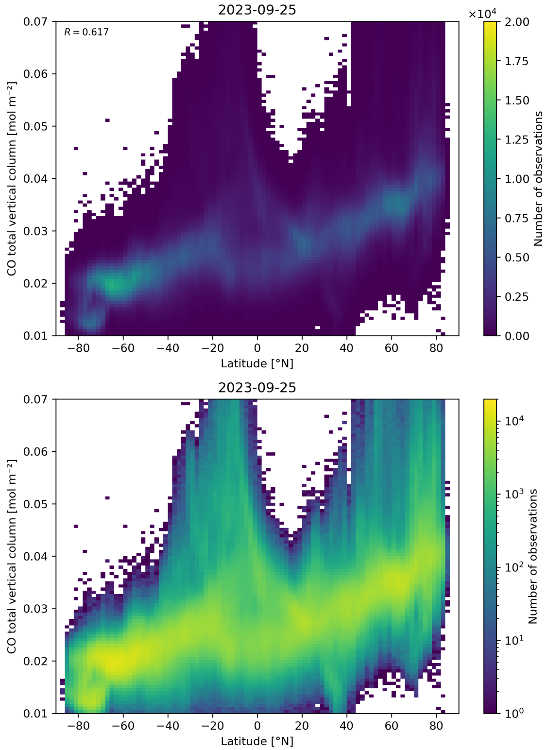
Figure 51: Scatter density plot of “Latitude” against “CO total vertical column” for 2023-09-24 to 2023-09-26.
