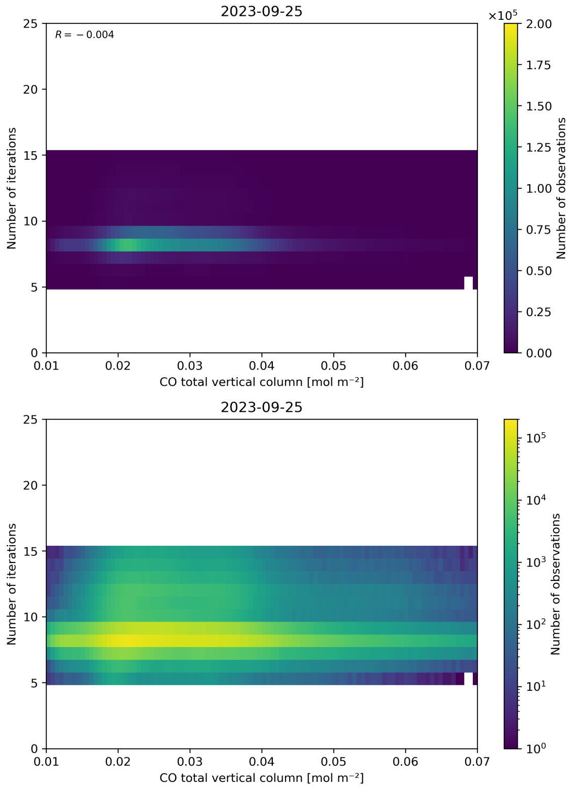
Figure 42: Scatter density plot of “CO total vertical column” against “Number of iterations” for 2023-09-24 to 2023-09-26.
