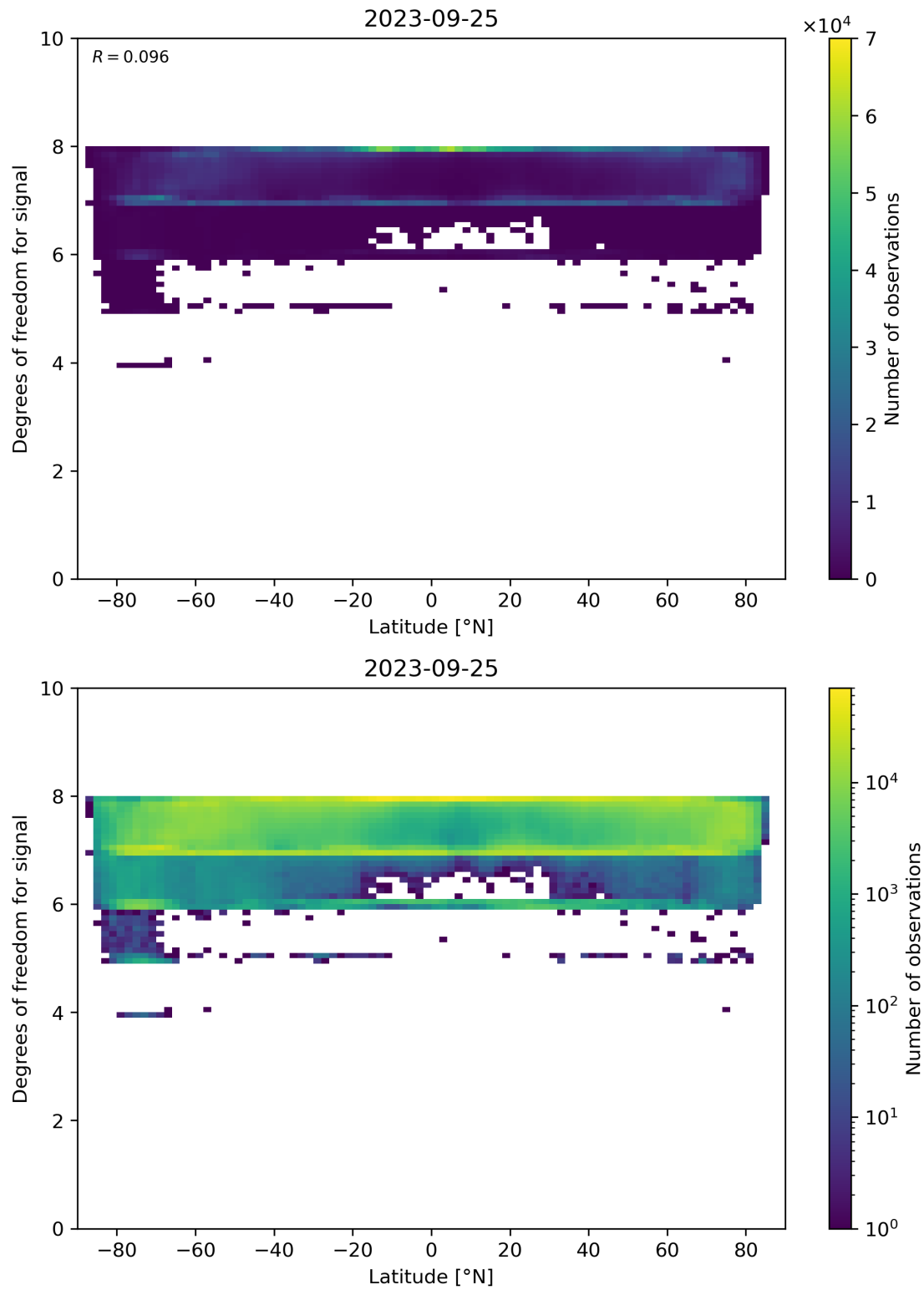
Figure 55: Scatter density plot of “Latitude” against “Degrees of freedom for signal” for 2023-09-24 to 2023-09-26.
