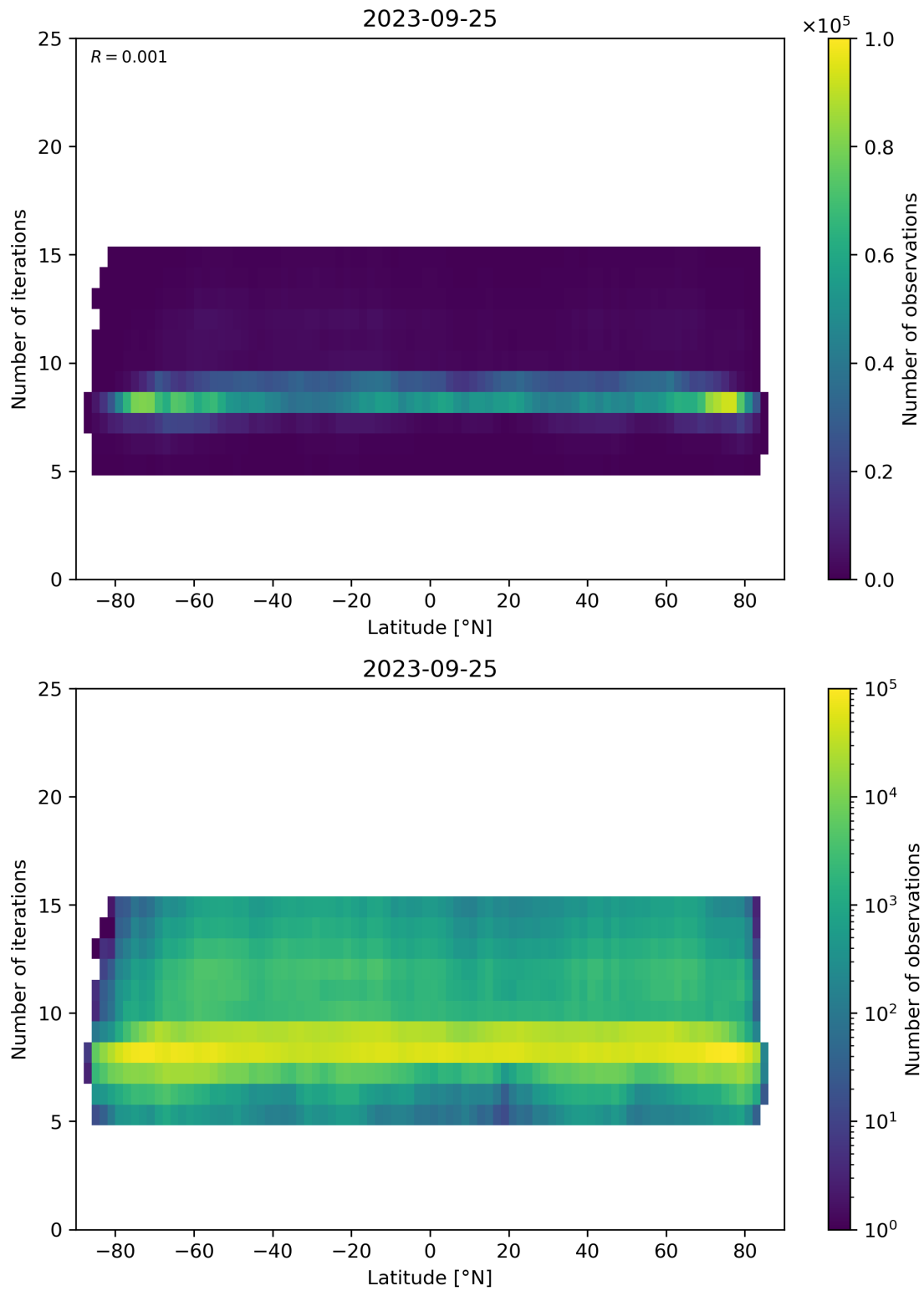
Figure 56: Scatter density plot of “Latitude” against “Number of iterations” for 2023-09-24 to 2023-09-26.
