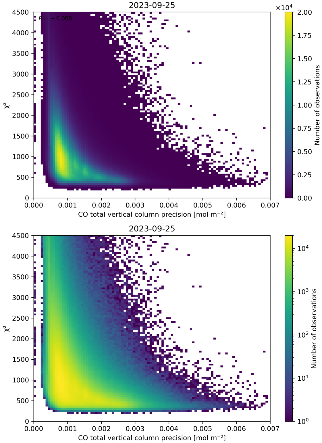
Figure 44: Scatter density plot of “CO total vertical column precision” against “ \chi^2 ” for 2023-09-24 to 2023-09-26.
