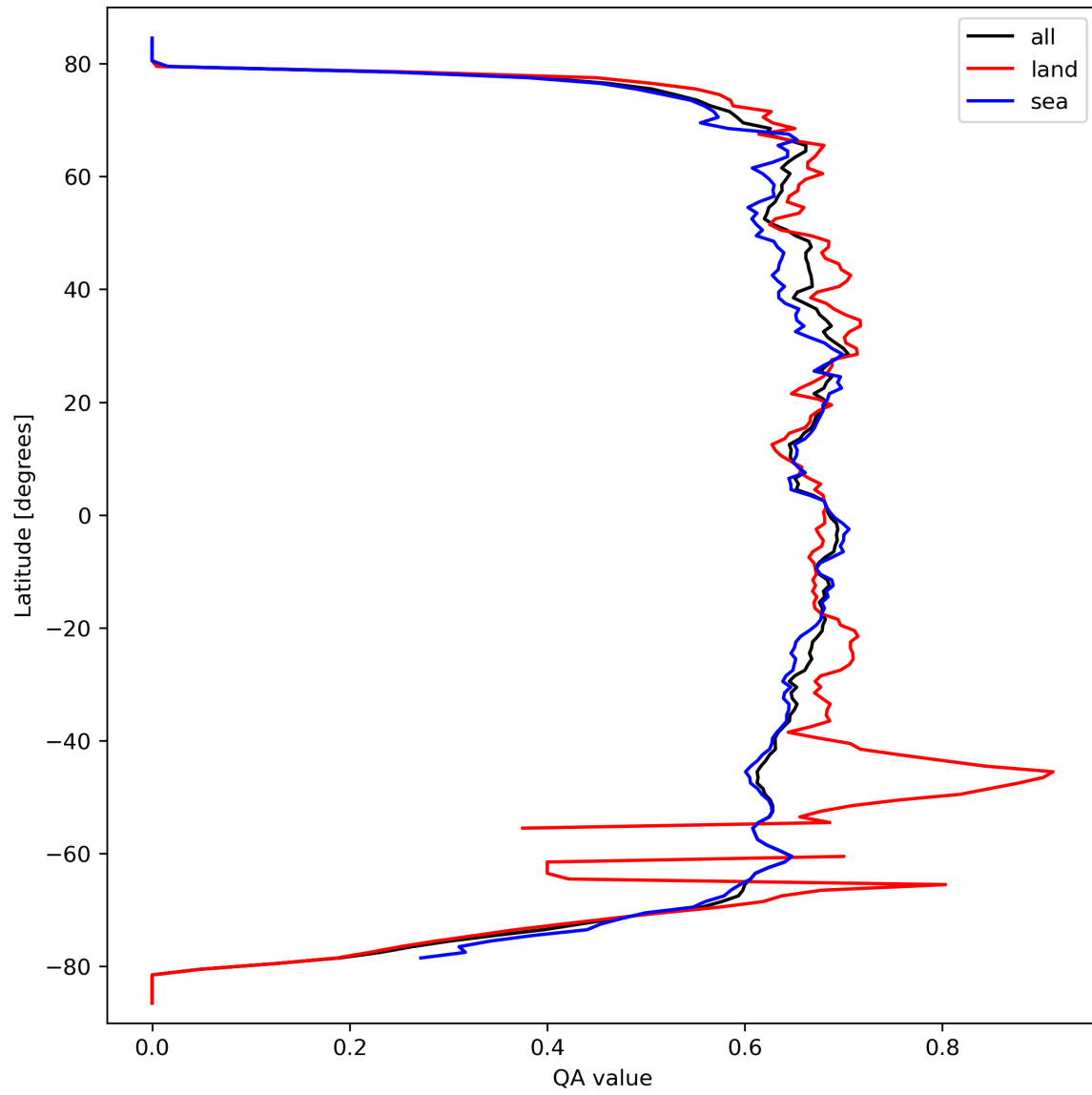
Figure 9: Zonal average of “QA value” for 2023-09-24 to 2023-09-26.
