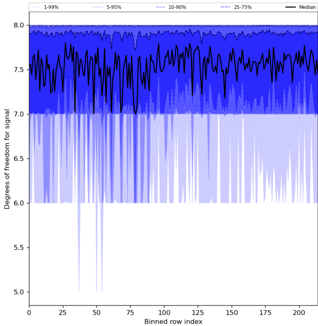
Figure 31: Along track statistics of “Degrees of freedom for signal” for 2023-09-24 to 2023-09-26
