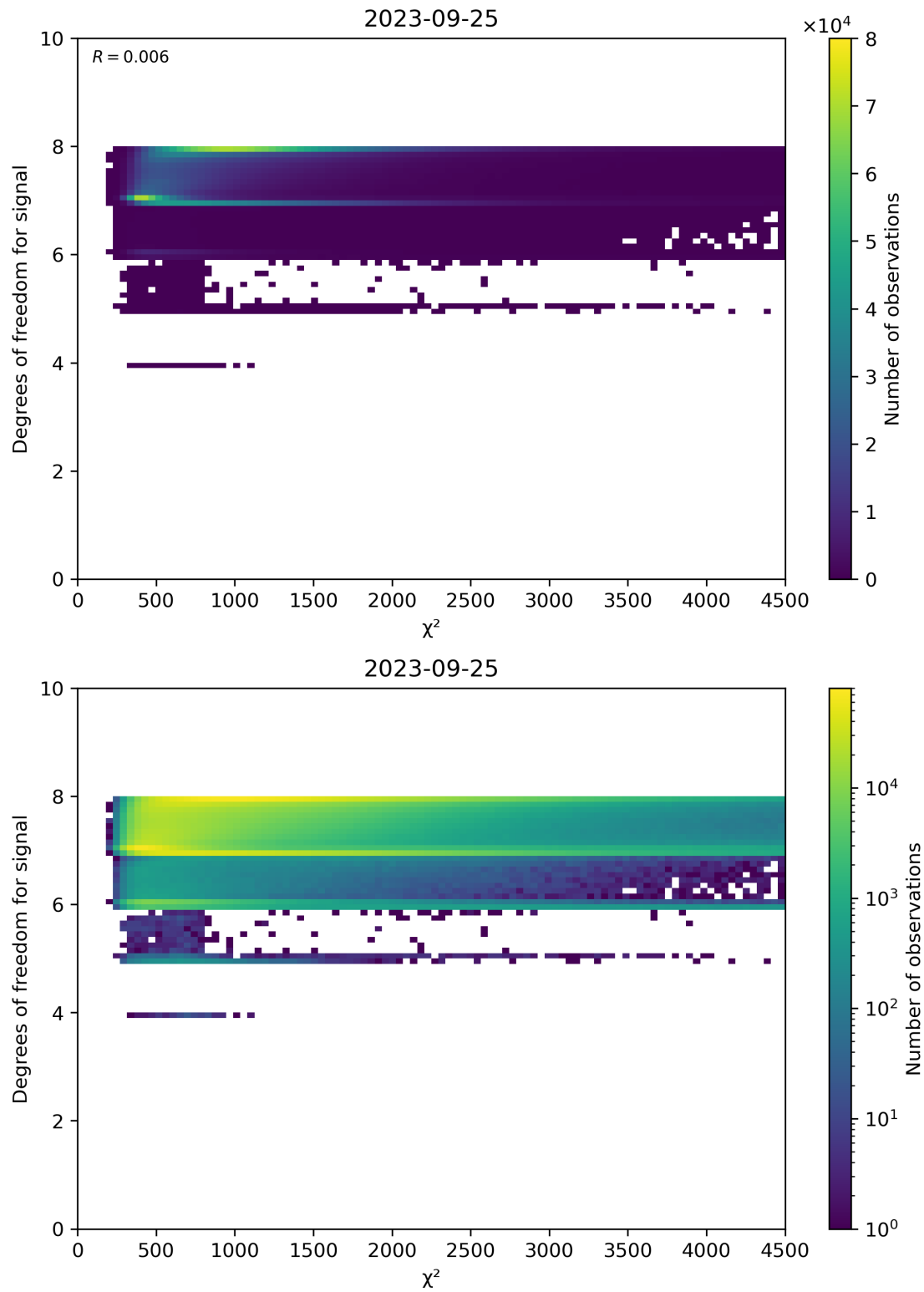
Figure 48: Scatter density plot of “ \chi^2 ” against “Degrees of freedom for signal” for 2023-09-24 to 2023-09-26.
