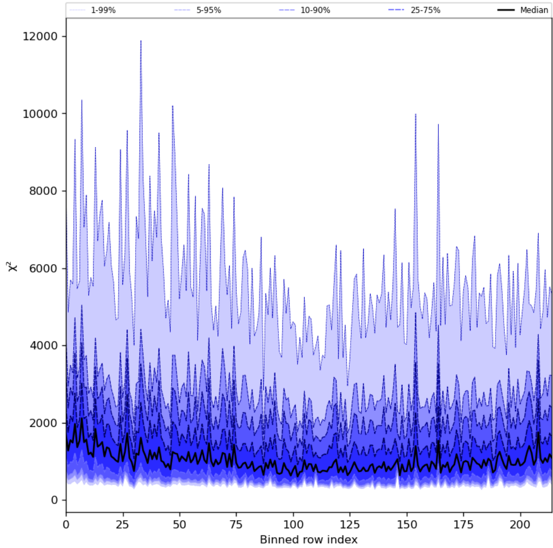
Figure 30: Along track statistics of “ \chi^2 ” for 2023-09-24 to 2023-09-26
