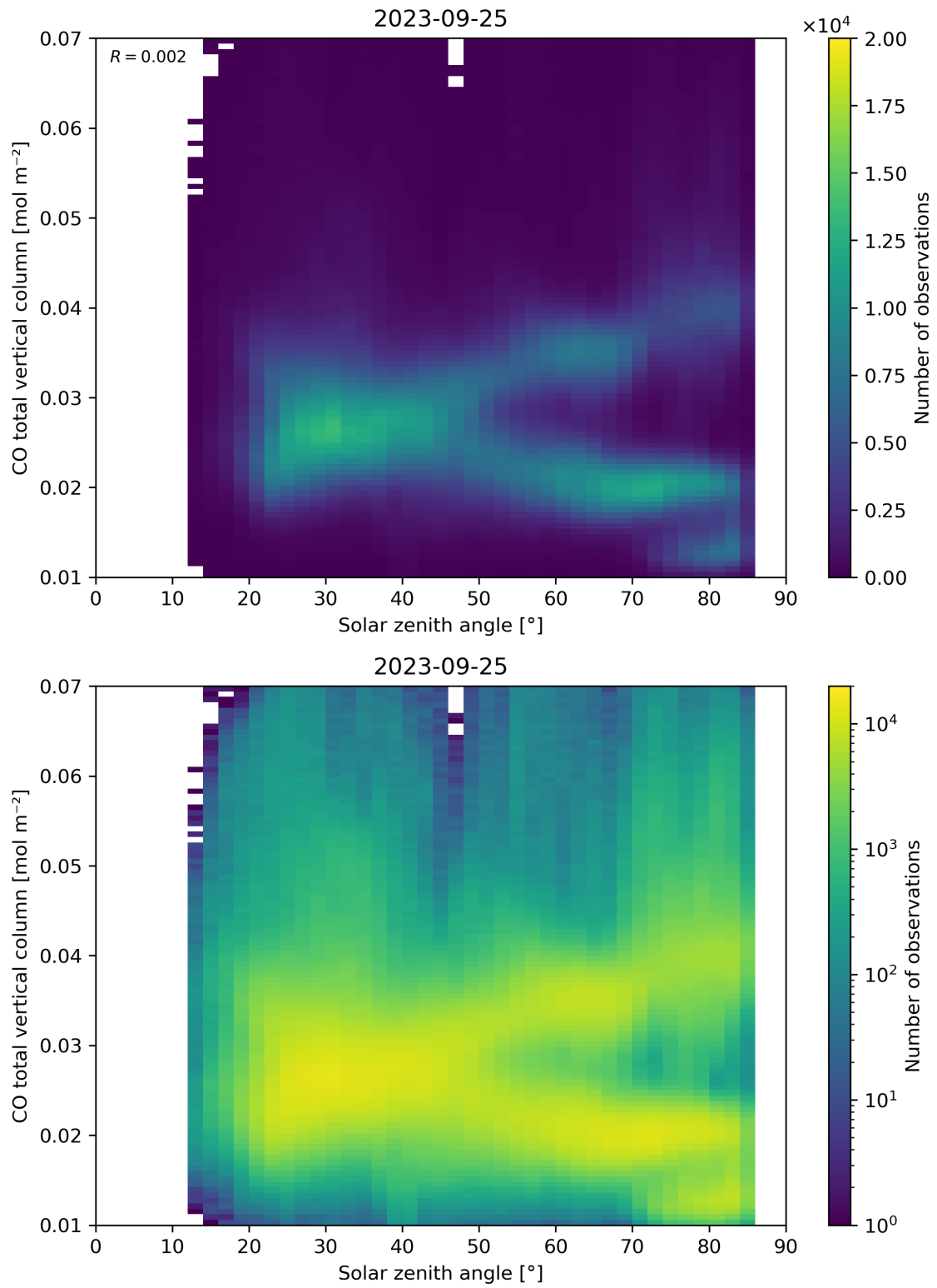
Figure 61: Scatter density plot of “Solar zenith angle” against “CO total vertical column” for 2023-09-24 to 2023-09-26.
