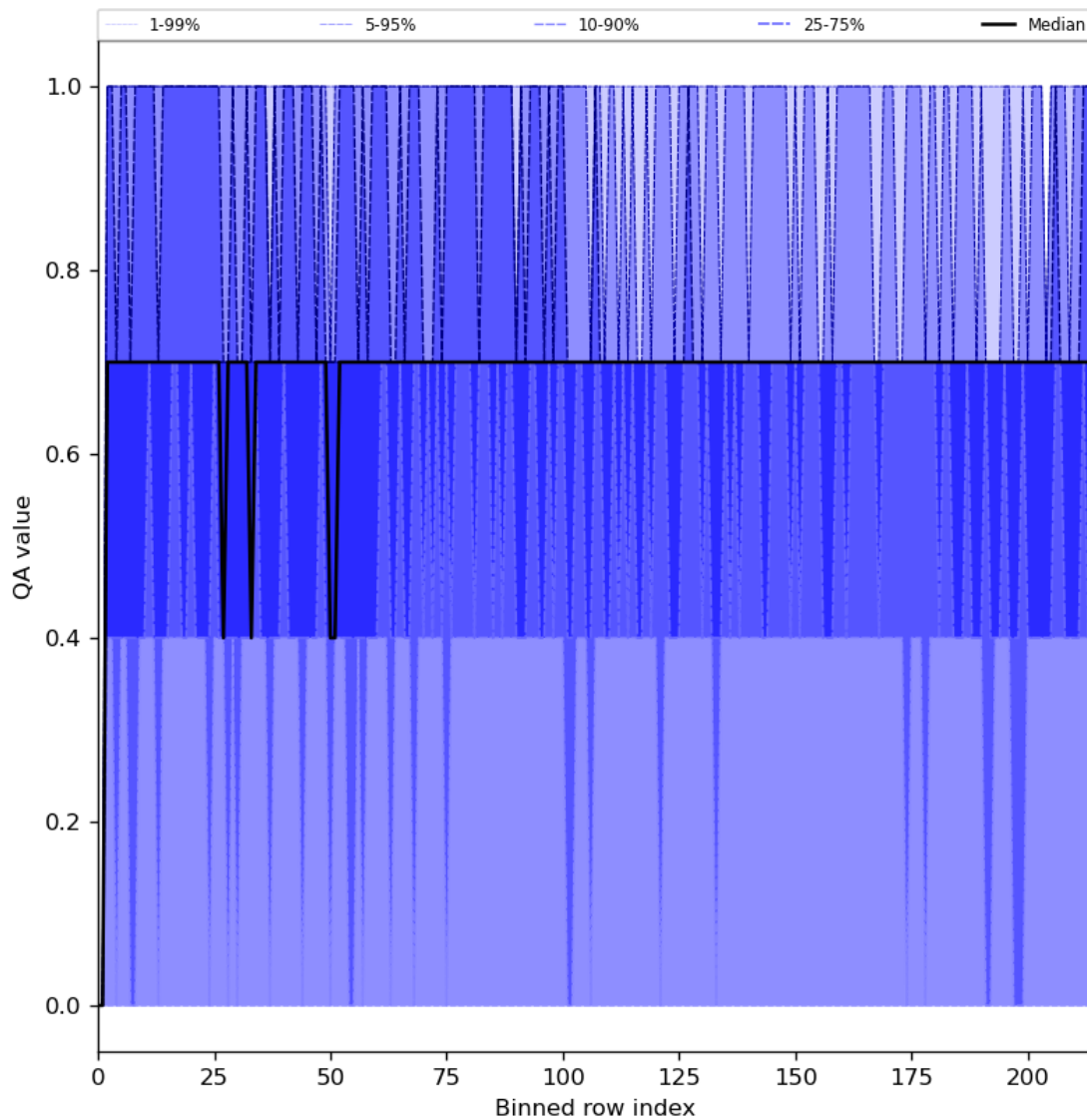
Figure 25: Along track statistics of “QA value” for 2023-09-24 to 2023-09-26
