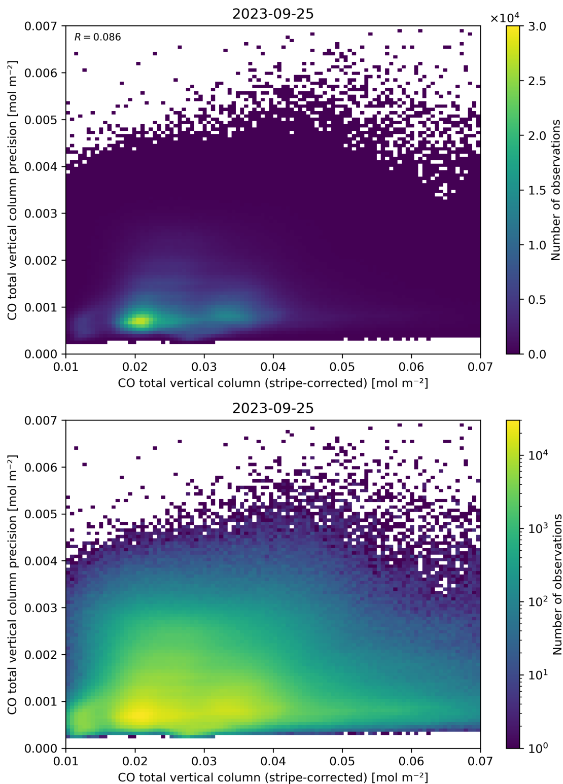
Figure 36: Scatter density plot of “CO total vertical column (stripe-corrected)” against “CO total vertical column precision” for 2023-09-24 to 2023-09-26.
