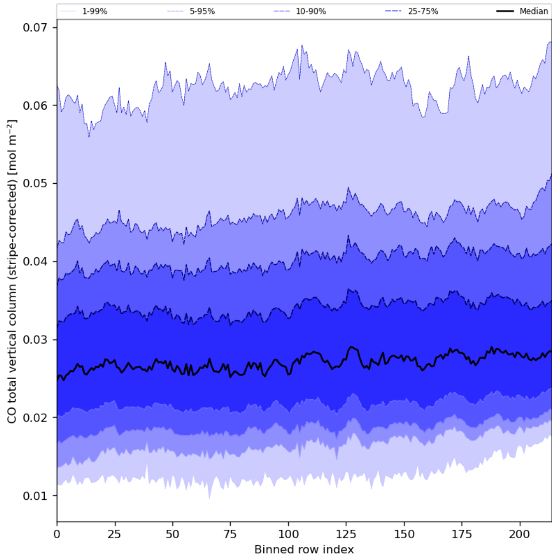
Figure 27: Along track statistics of “CO total vertical column (stripe-corrected)” for 2023-09-24 to 2023-09-26
