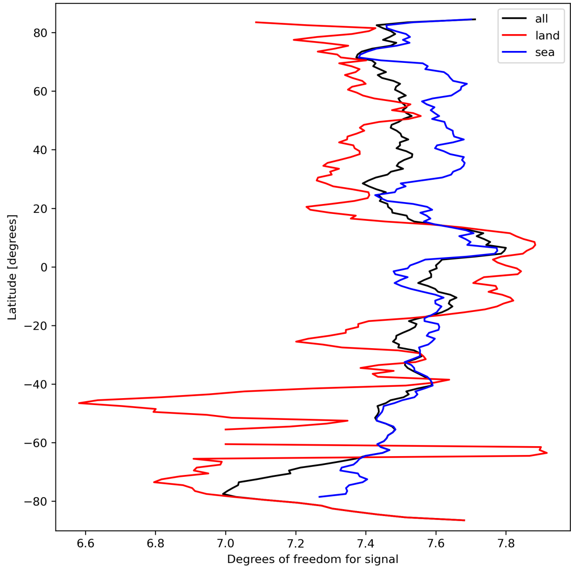
Figure 15: Zonal average of “Degrees of freedom for signal” for 2023-09-24 to 2023-09-26.
