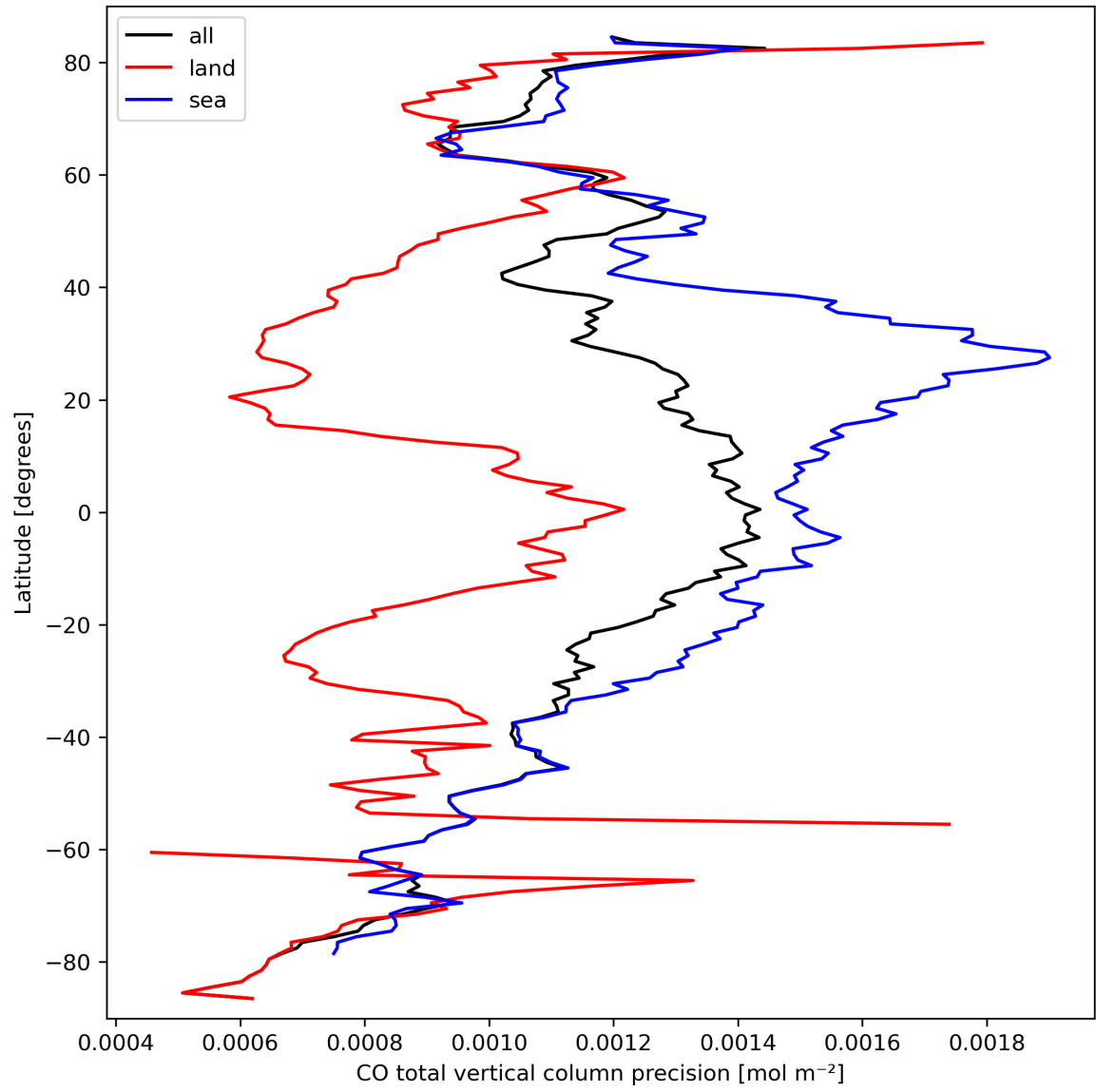
Figure 12: Zonal average of “CO total vertical column precision” for 2023-09-24 to 2023-09-26.
