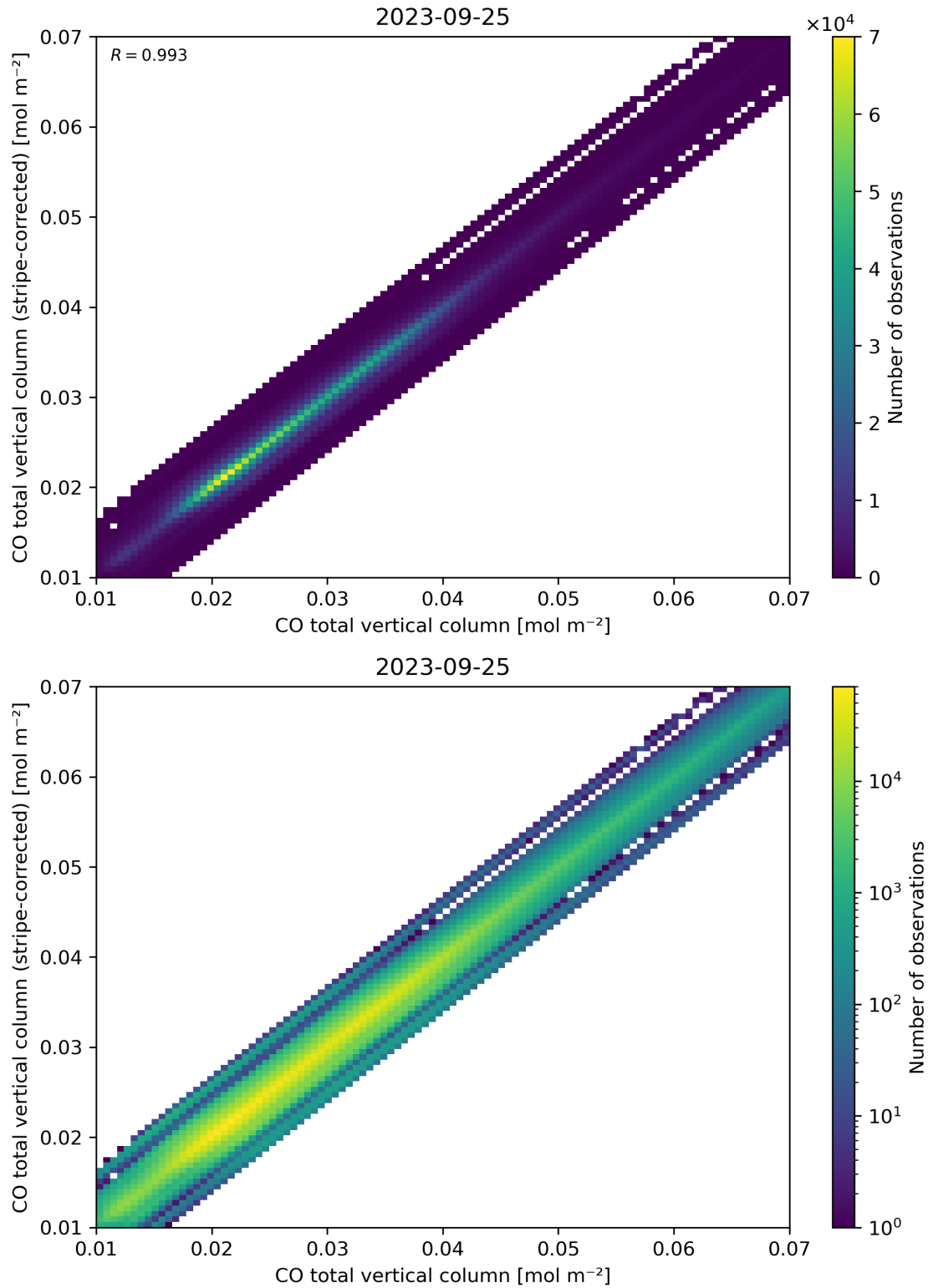
Figure 33: Scatter density plot of “CO total vertical column” against “CO total vertical column (stripe-corrected)” for 2023-09-24 to 2023-09-26.
