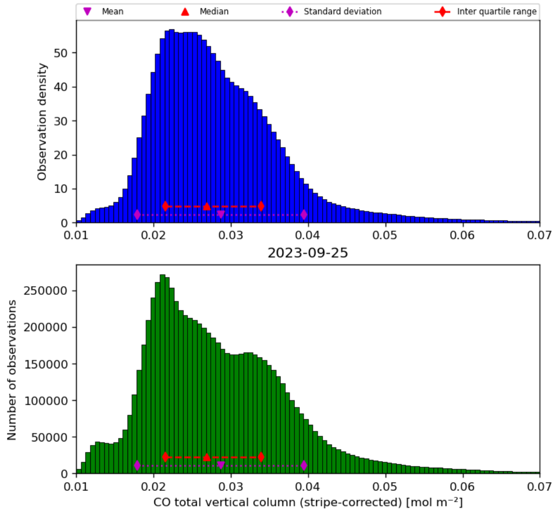
Figure 19: Histogram of “CO total vertical column (stripe-corrected)” for 2023-09-24 to 2023-09-26
