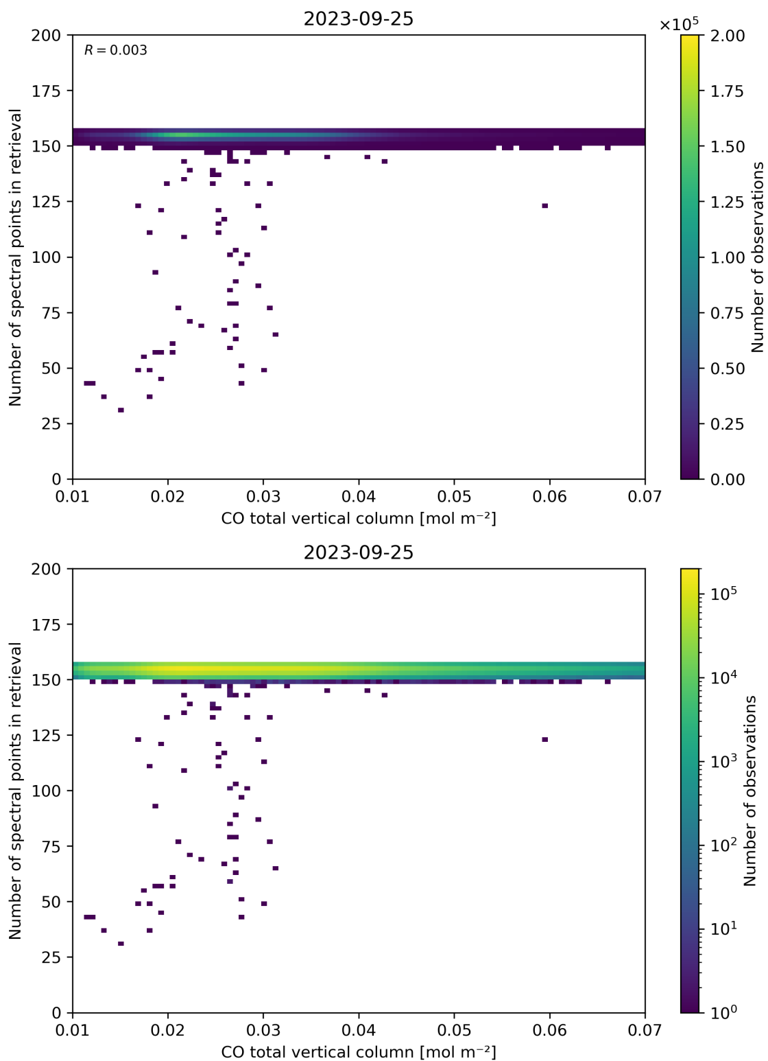
Figure 43: Scatter density plot of “CO total vertical column” against “Number of spectral points in retrieval” for 2023-09-24 to 2023-09-26.
