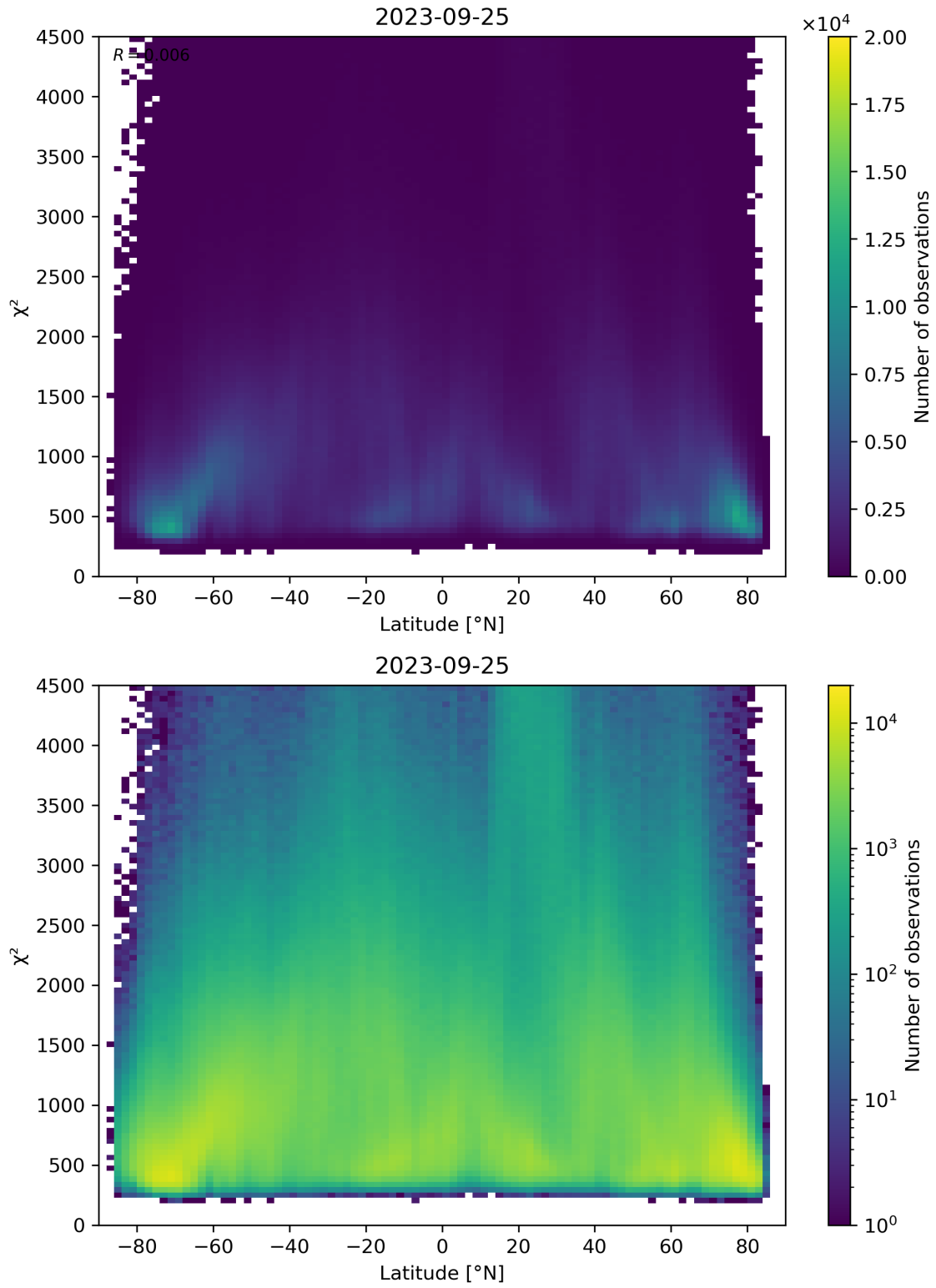
Figure 54: Scatter density plot of “Latitude” against “ \chi^2 ” for 2023-09-24 to 2023-09-26.
