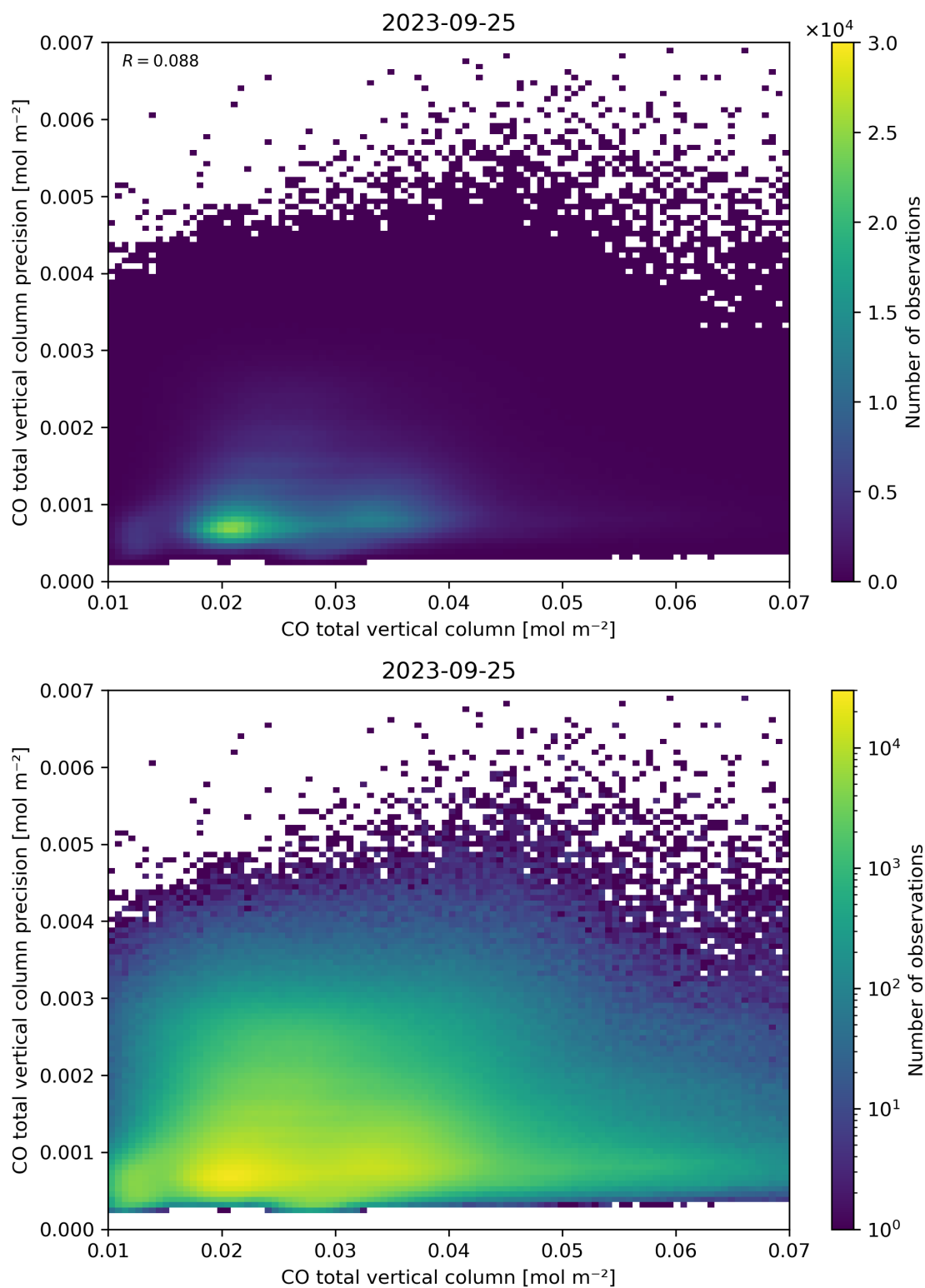
Figure 34: Scatter density plot of “CO total vertical column” against “CO total vertical column precision” for 2023-09-24 to 2023-09-26.
