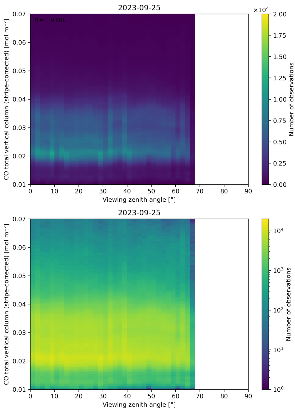
Figure 70: Scatter density plot of “Viewing zenith angle” against “CO total vertical column (stripe-corrected)” for 2023-09-24 to 2023-09-26.
