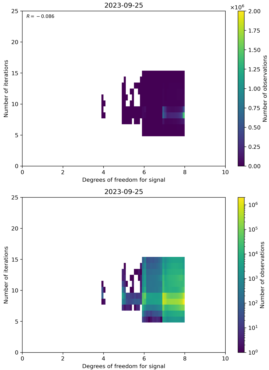
Figure 50: Scatter density plot of “Degrees of freedom for signal” against “Number of iterations” for 2023-09-24 to 2023-09-26.
