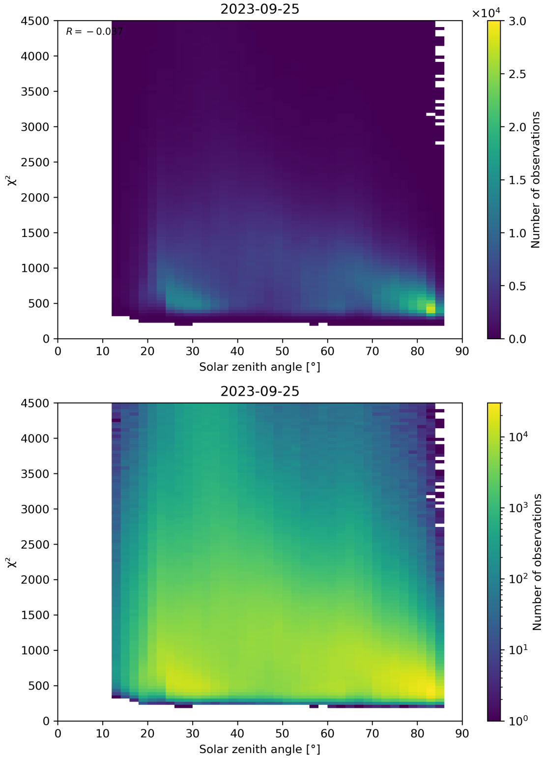
Figure 64: Scatter density plot of “Solar zenith angle” against “ \chi^2 ” for 2023-09-24 to 2023-09-26.
