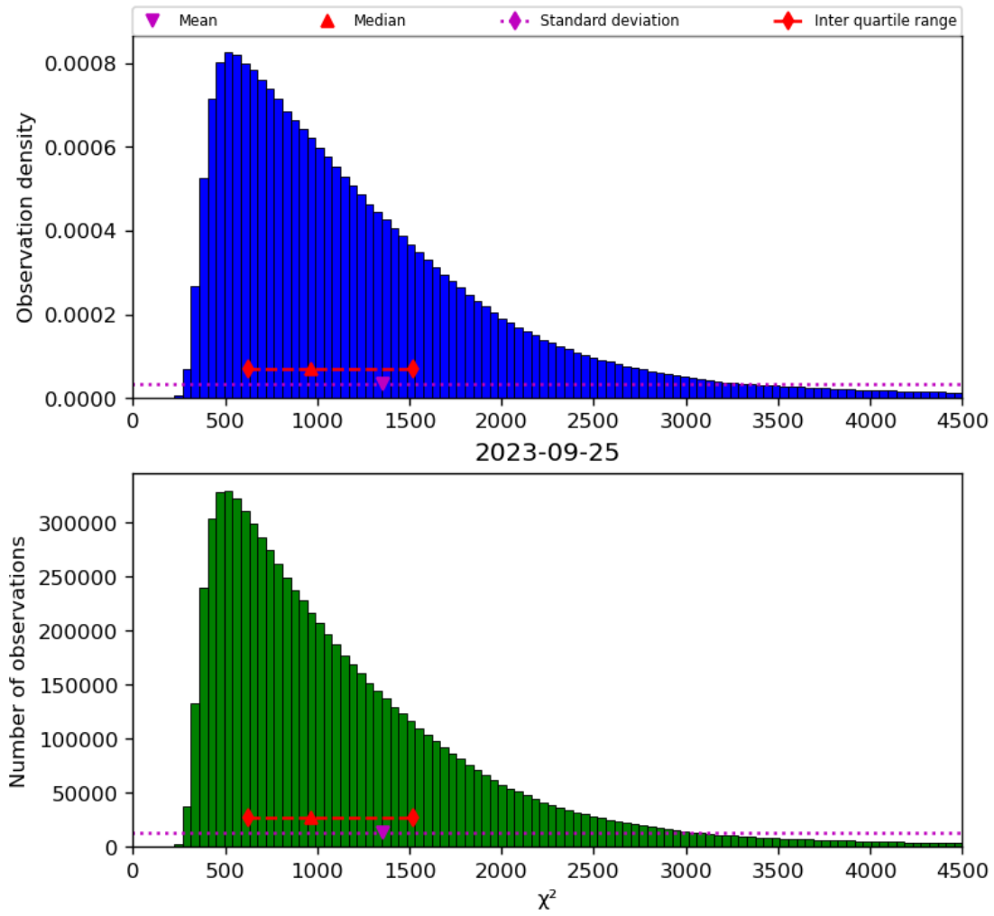
Figure 22: Histogram of “ \chi^2 ” for 2023-09-24 to 2023-09-26
