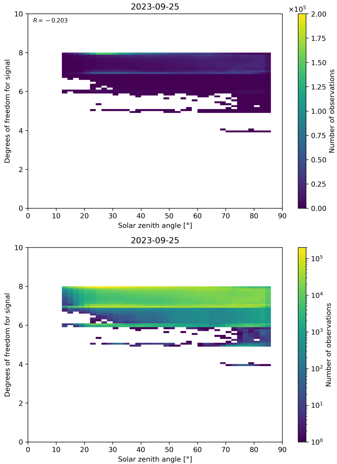
Figure 65: Scatter density plot of “Solar zenith angle” against “Degrees of freedom for signal” for 2023-09-24 to 2023-09-26.
