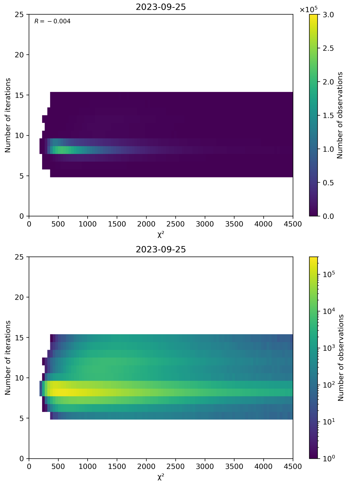
Figure 49: Scatter density plot of “ \chi^2 ” against “Number of iterations” for 2023-09-24 to 2023-09-26.
