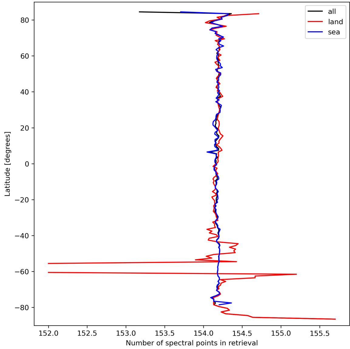
Figure 13: Zonal average of “Number of spectral points in retrieval” for 2023-09-24 to 2023-09-26.
