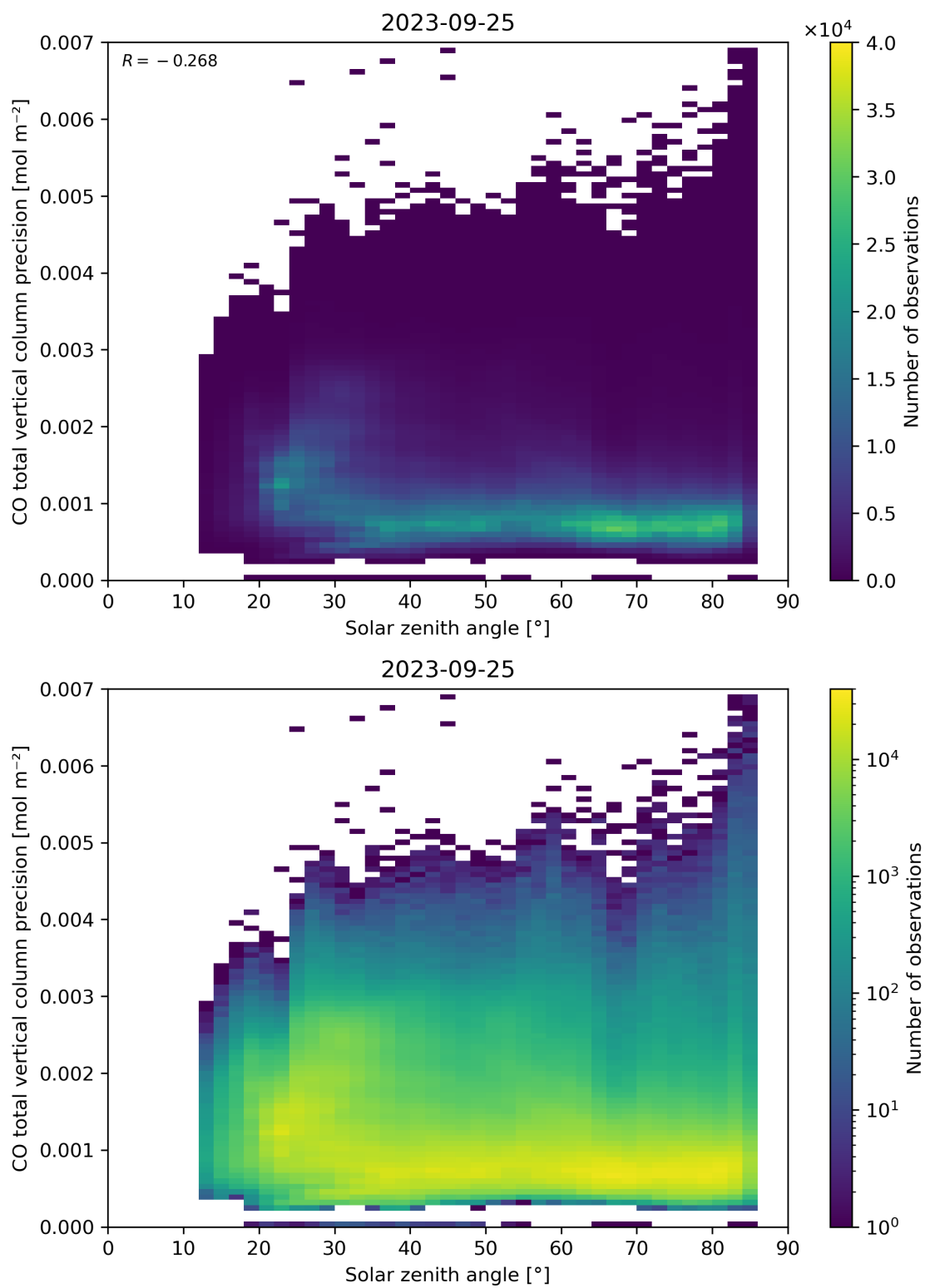
Figure 63: Scatter density plot of “Solar zenith angle” against “CO total vertical column precision” for 2023-09-24 to 2023-09-26.
