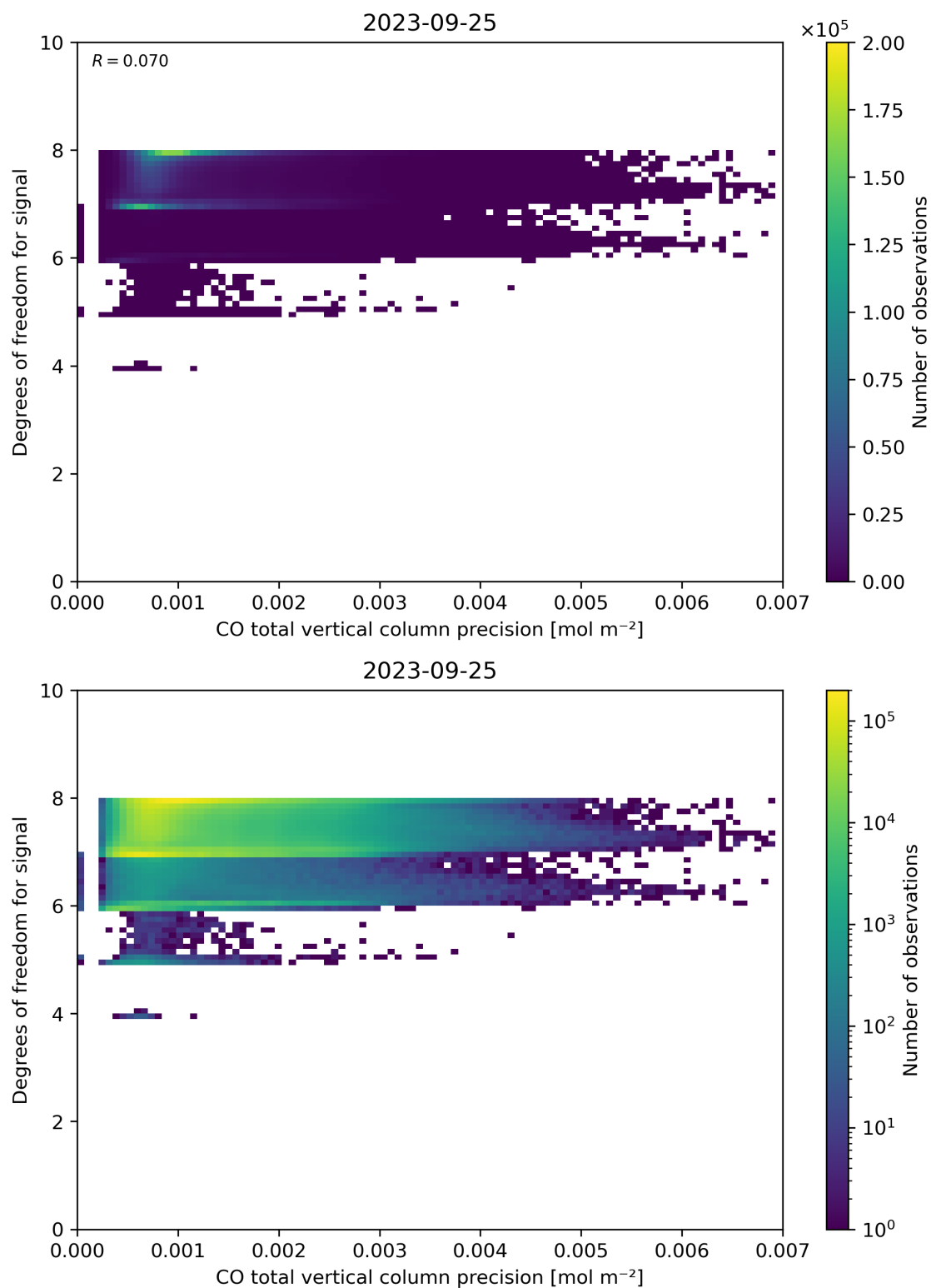
Figure 45: Scatter density plot of “CO total vertical column precision” against “Degrees of freedom for signal” for 2023-09-24 to 2023-09-26.
