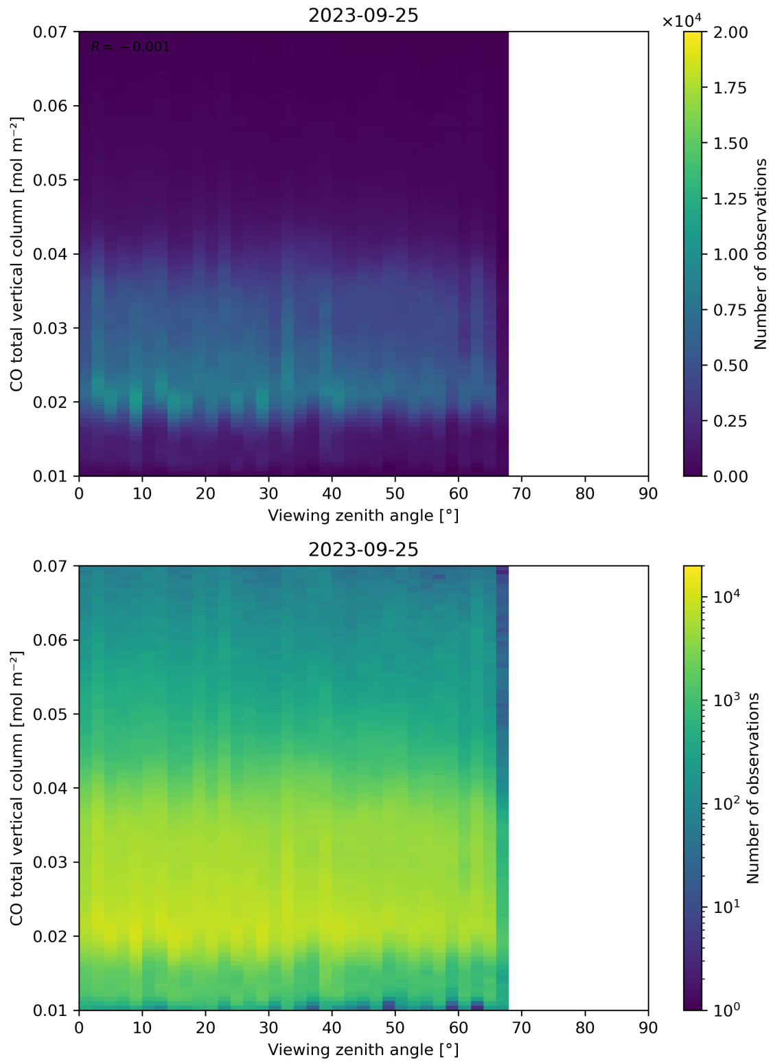
Figure 69: Scatter density plot of “Viewing zenith angle” against “CO total vertical column” for 2023-09-24 to 2023-09-26.
