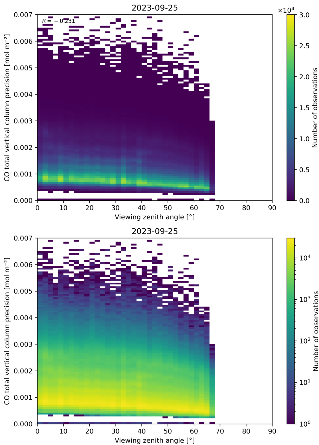
Figure 71: Scatter density plot of “Viewing zenith angle” against “CO total vertical column precision” for 2023-09-24 to 2023-09-26.
