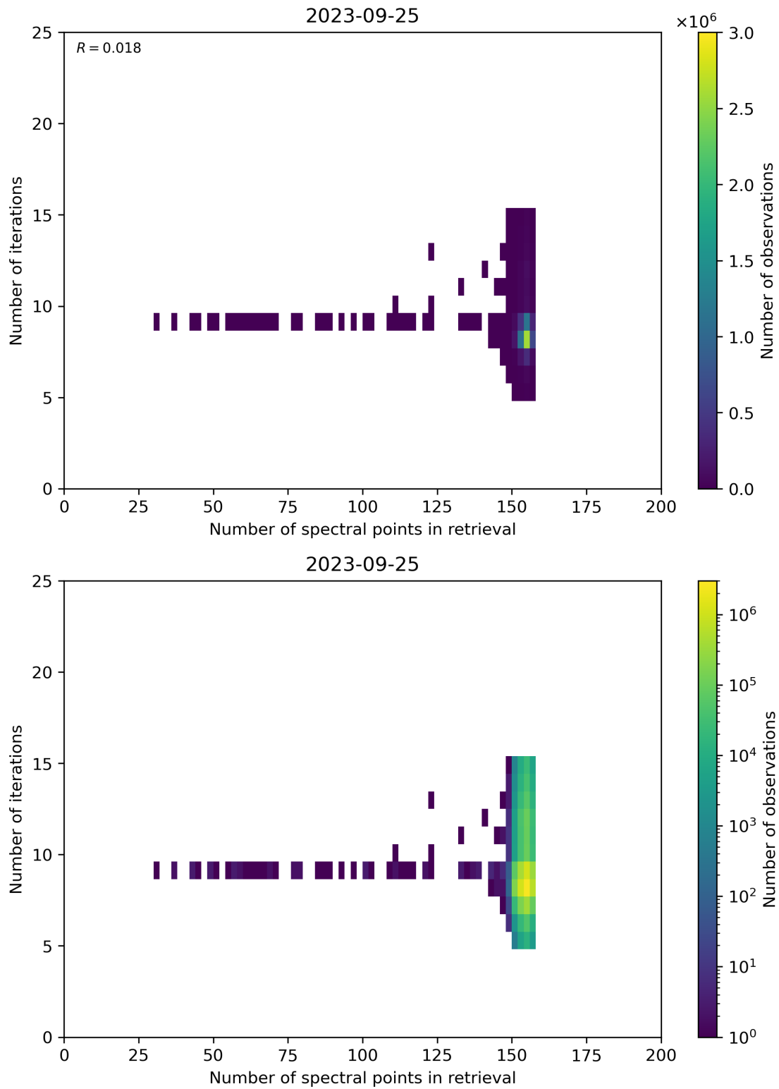
Figure 60: Scatter density plot of “Number of spectral points in retrieval” against “Number of iterations” for 2023-09-24 to 2023-09-26.
