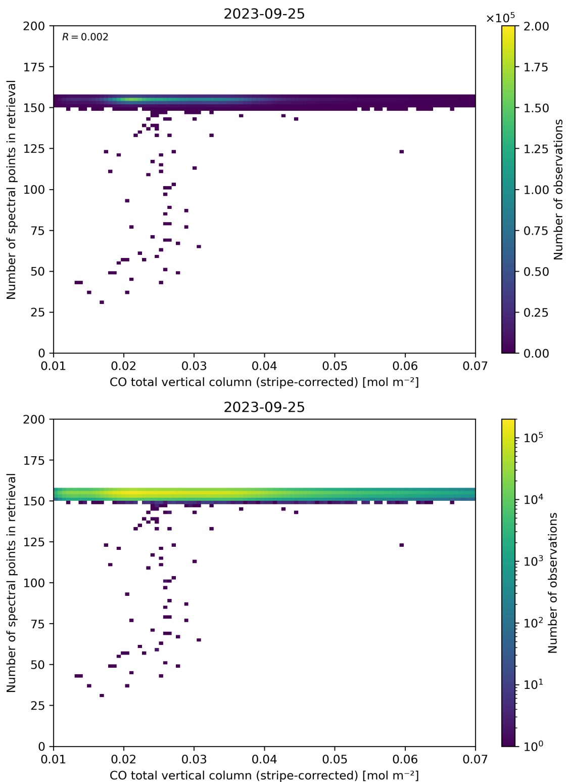
Figure 40: Scatter density plot of “CO total vertical column (stripe-corrected)” against “Number of spectral points in retrieval” for 2023-09-24 to 2023-09-26.
