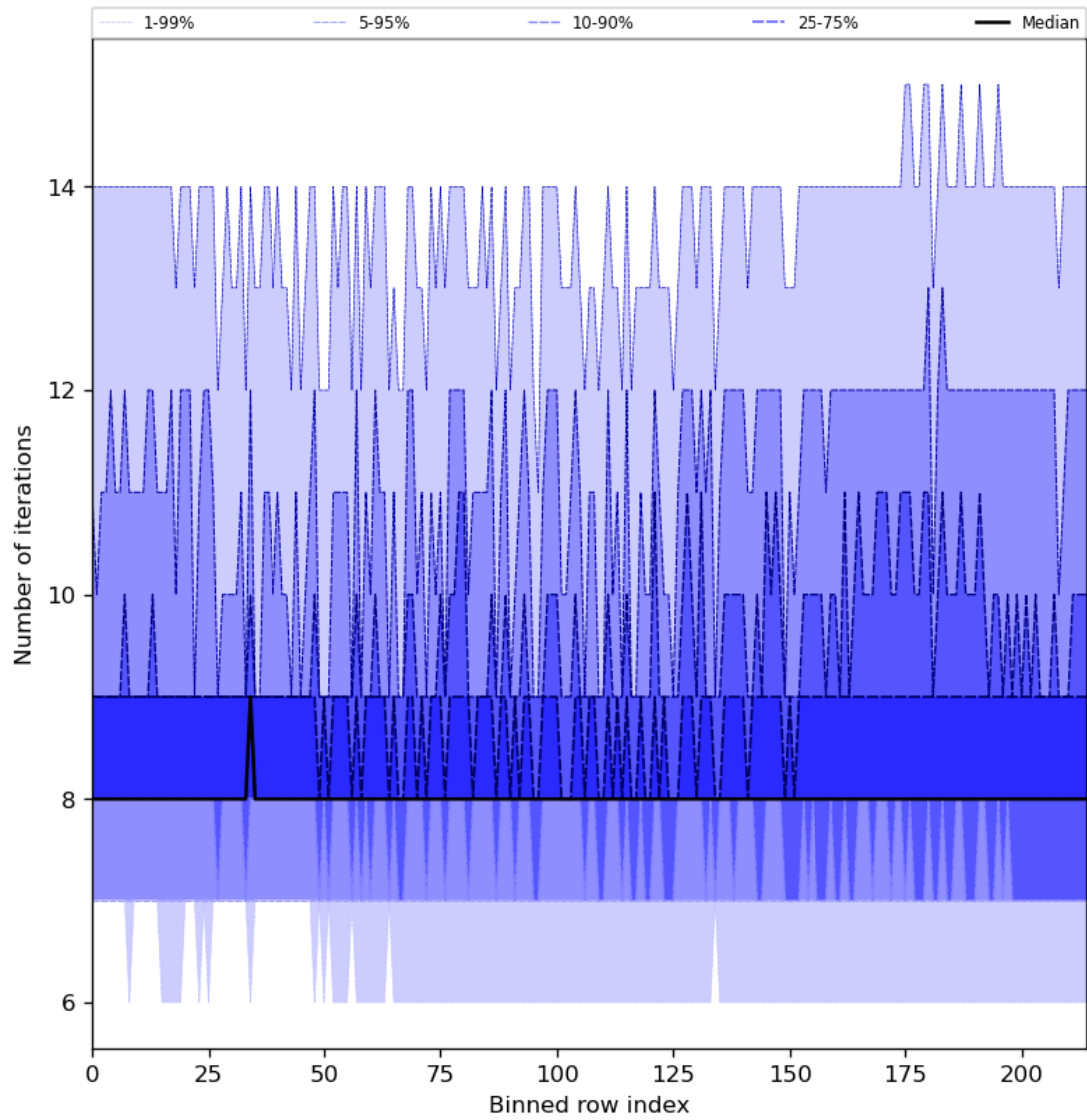
Figure 32: Along track statistics of “Number of iterations” for 2023-09-24 to 2023-09-26
