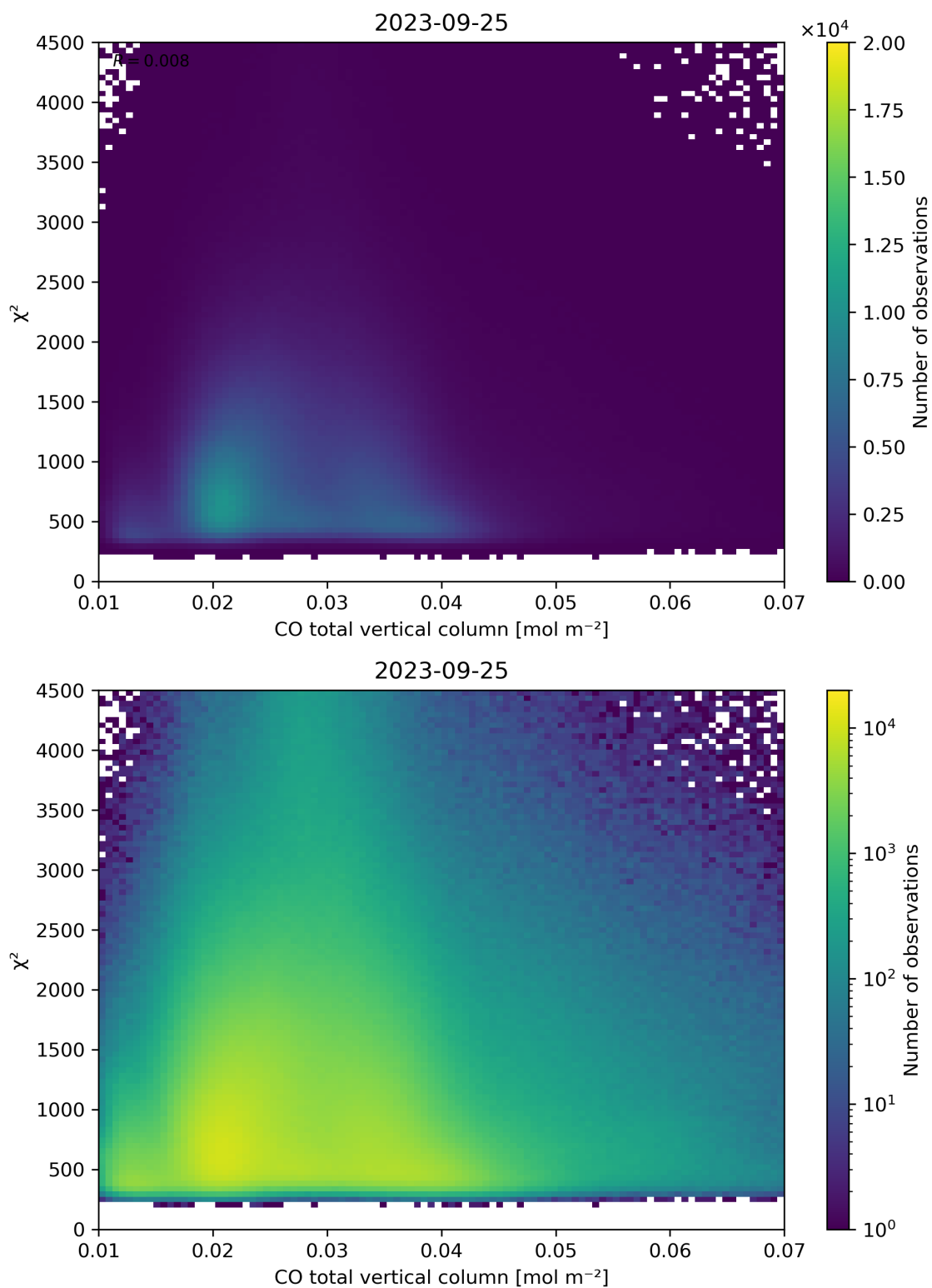
Figure 35: Scatter density plot of “CO total vertical column” against “ \chi^2 ” for 2023-09-24 to 2023-09-26.
