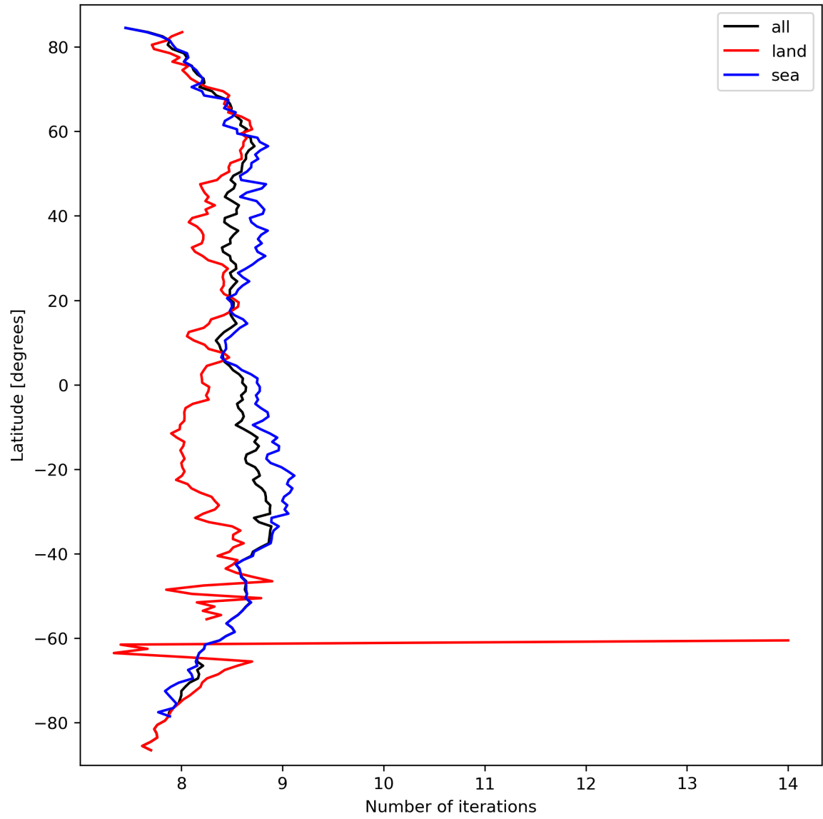
Figure 16: Zonal average of “Number of iterations” for 2023-09-24 to 2023-09-26.
