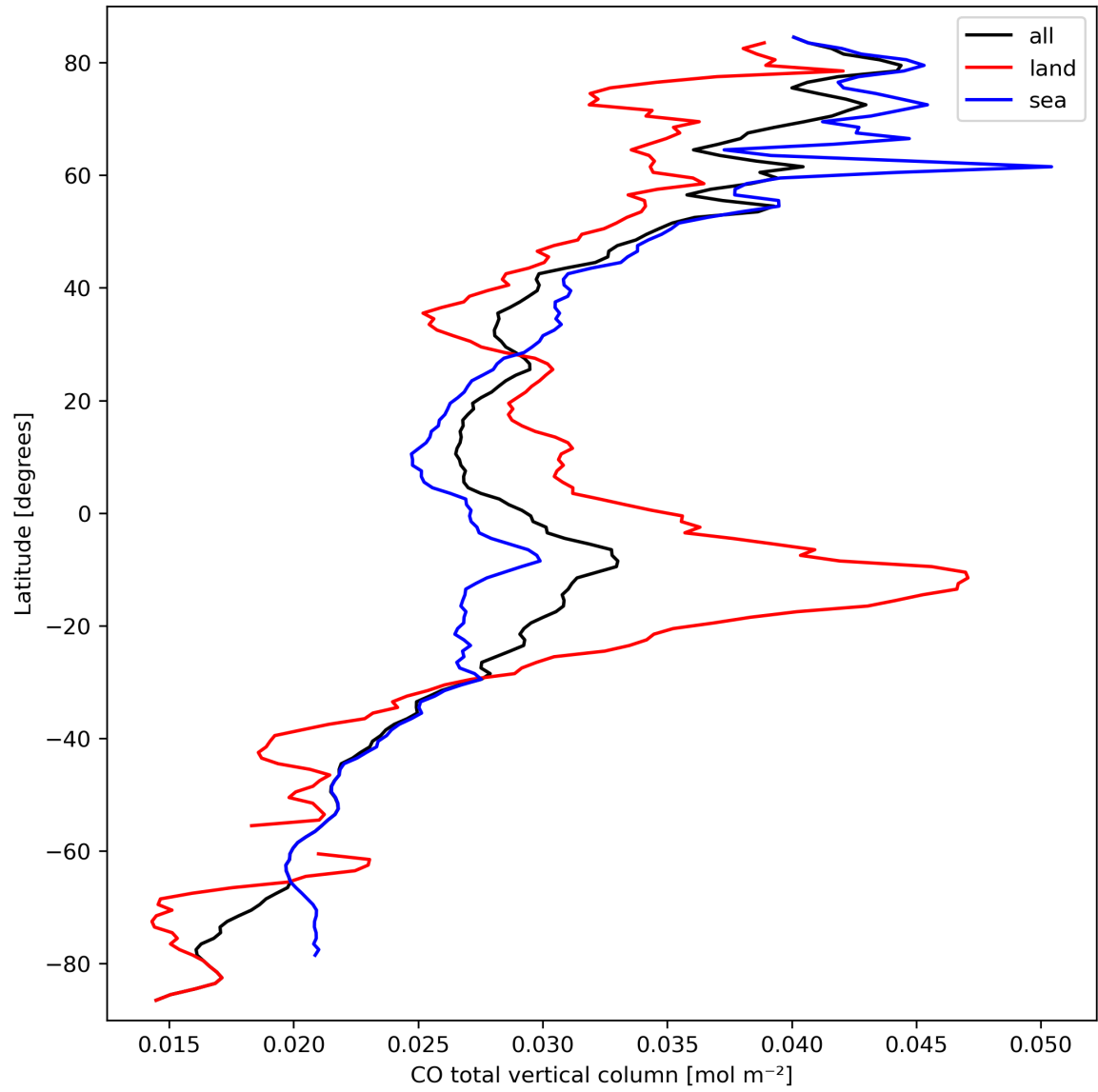
Figure 10: Zonal average of “CO total vertical column” for 2023-09-24 to 2023-09-26.
