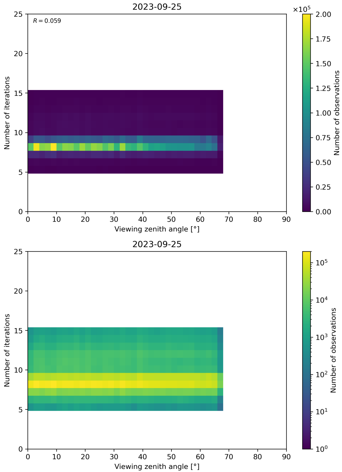
Figure 75: Scatter density plot of “Viewing zenith angle” against “Number of iterations” for 2023-09-24 to 2023-09-26.
