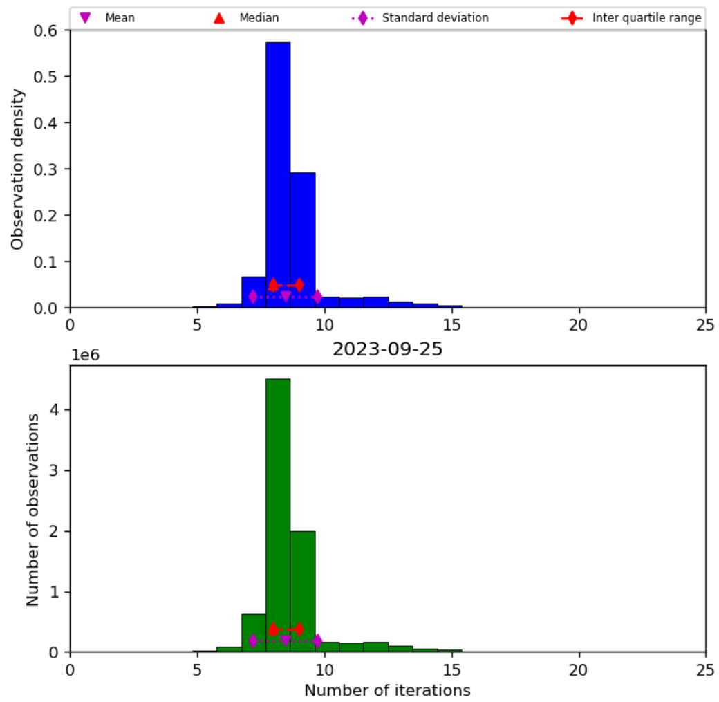
Figure 24: Histogram of “Number of iterations” for 2023-09-24 to 2023-09-26
