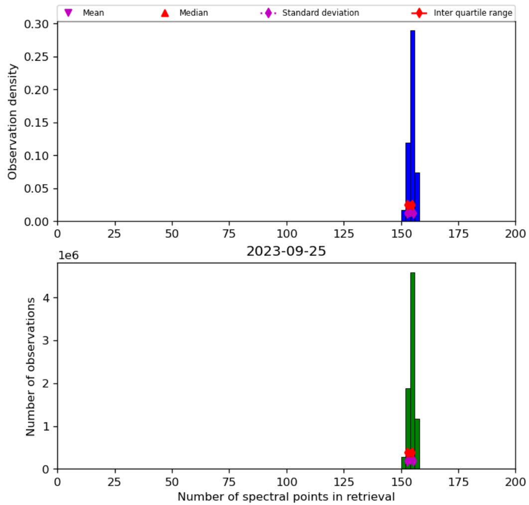
Figure 21: Histogram of “Number of spectral points in retrieval” for 2023-09-24 to 2023-09-26
