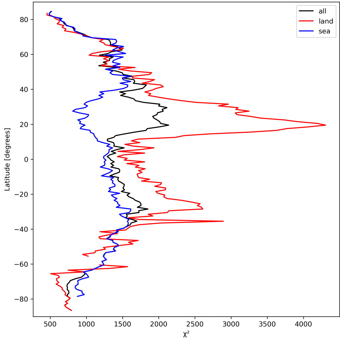
Figure 14: Zonal average of “ \chi^2 ” for 2023-09-24 to 2023-09-26.
