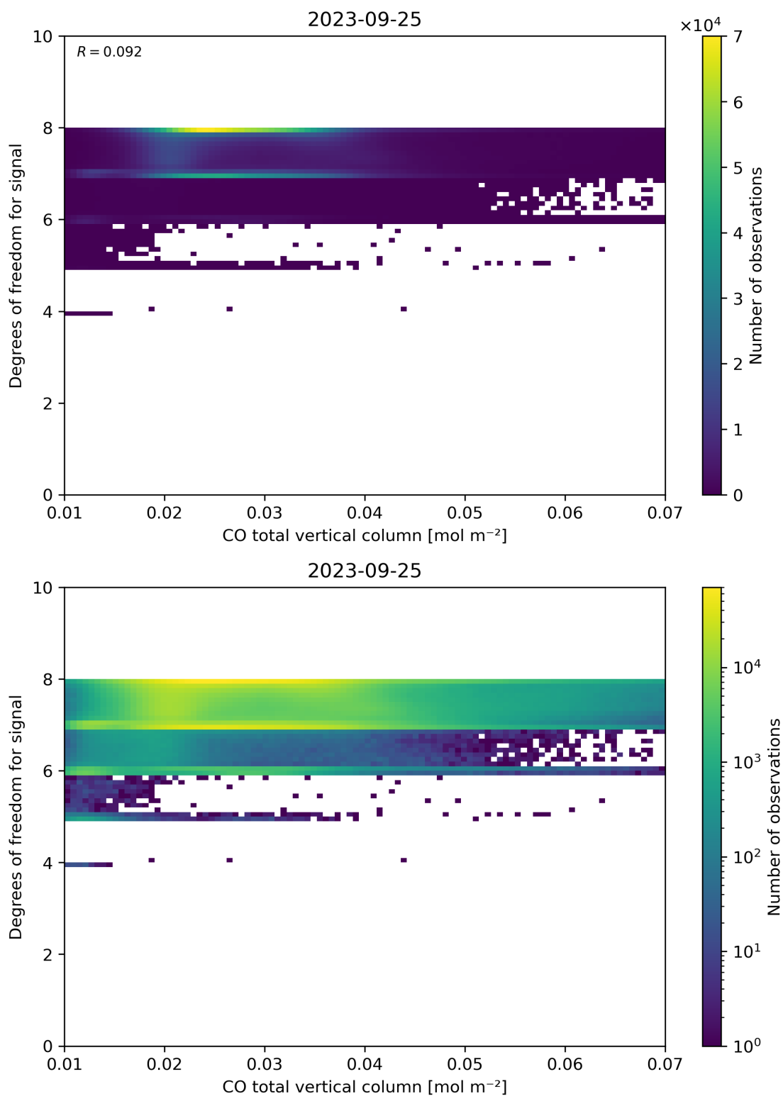
Figure 41: Scatter density plot of “CO total vertical column” against “Degrees of freedom for signal” for 2023-09-24 to 2023-09-26.
