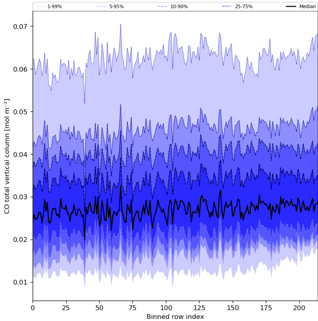
Figure 26: Along track statistics of “CO total vertical column” for 2023-09-24 to 2023-09-26
