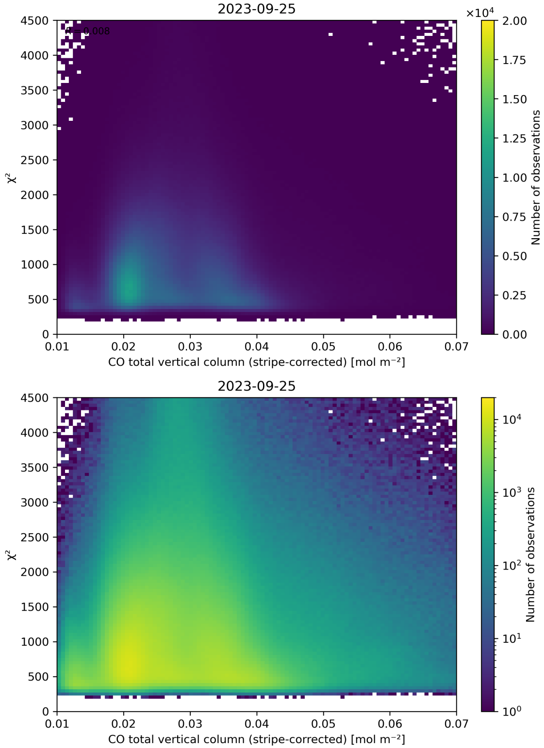
Figure 37: Scatter density plot of “CO total vertical column (stripe-corrected)” against “ \chi^2 ” for 2023-09-24 to 2023-09-26.
