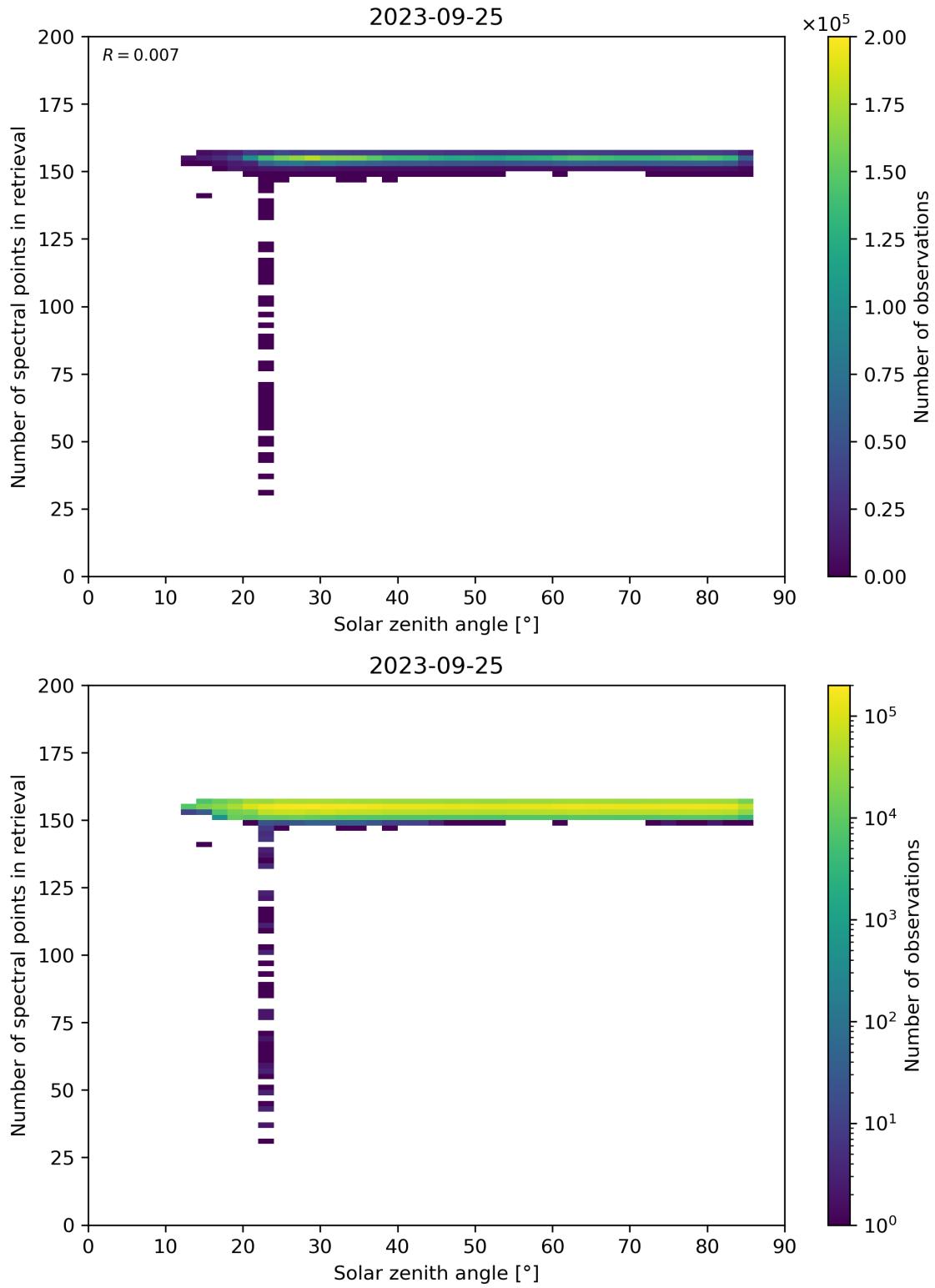
Figure 68: Scatter density plot of “Solar zenith angle” against “Number of spectral points in retrieval” for 2023-09-24 to 2023-09-26.
