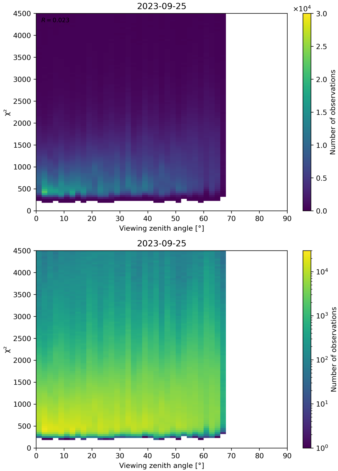
Figure 72: Scatter density plot of “Viewing zenith angle” against “ \chi^2 ” for 2023-09-24 to 2023-09-26.
