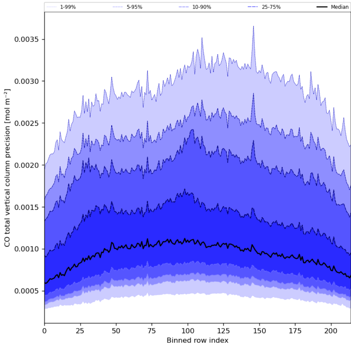
Figure 28: Along track statistics of “CO total vertical column precision” for 2023-09-24 to 2023-09-26
