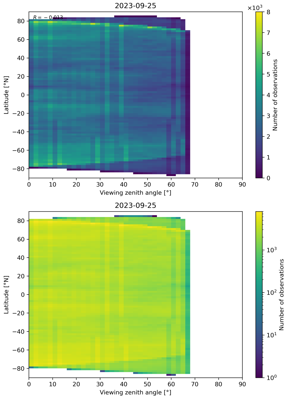
Figure 74: Scatter density plot of “Viewing zenith angle” against “Latitude” for 2023-09-24 to 2023-09-26.
