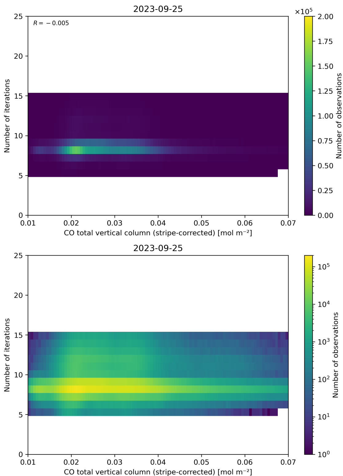
Figure 39: Scatter density plot of “CO total vertical column (stripe-corrected)” against “Number of iterations” for 2023-09-24 to 2023-09-26.
