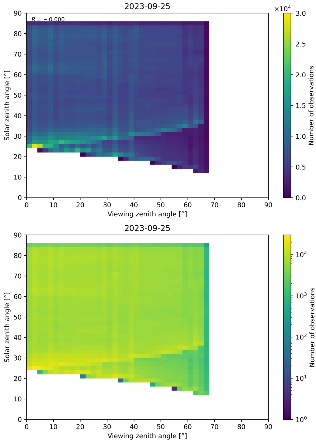
Figure 77: Scatter density plot of “Viewing zenith angle” against “Solar zenith angle” for 2023-09-24 to 2023-09-26.
