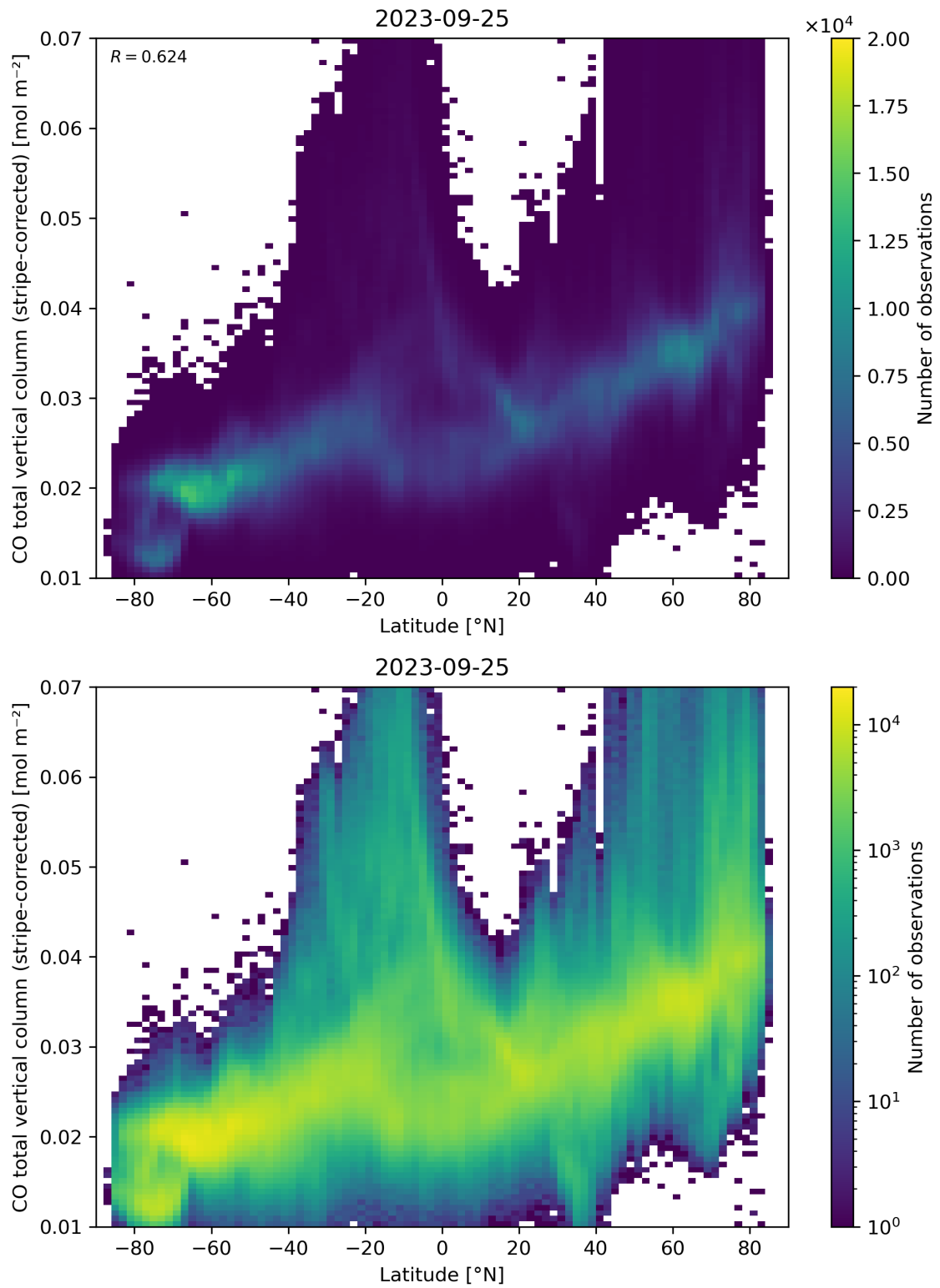
Figure 52: Scatter density plot of “Latitude” against “CO total vertical column (stripe-corrected)” for 2023-09-24 to 2023-09-26.
