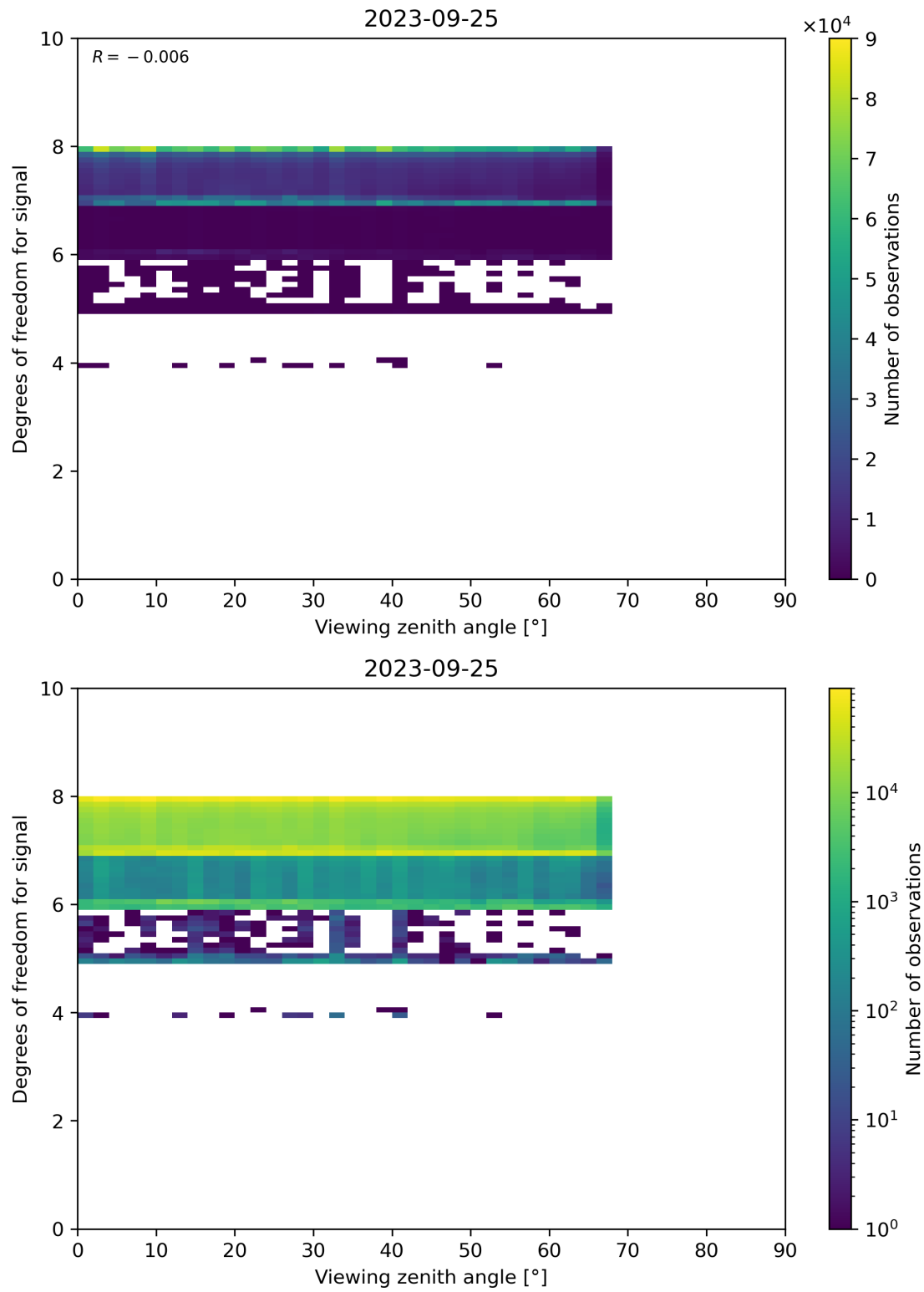
Figure 73: Scatter density plot of “Viewing zenith angle” against “Degrees of freedom for signal” for 2023-09-24 to 2023-09-26.
