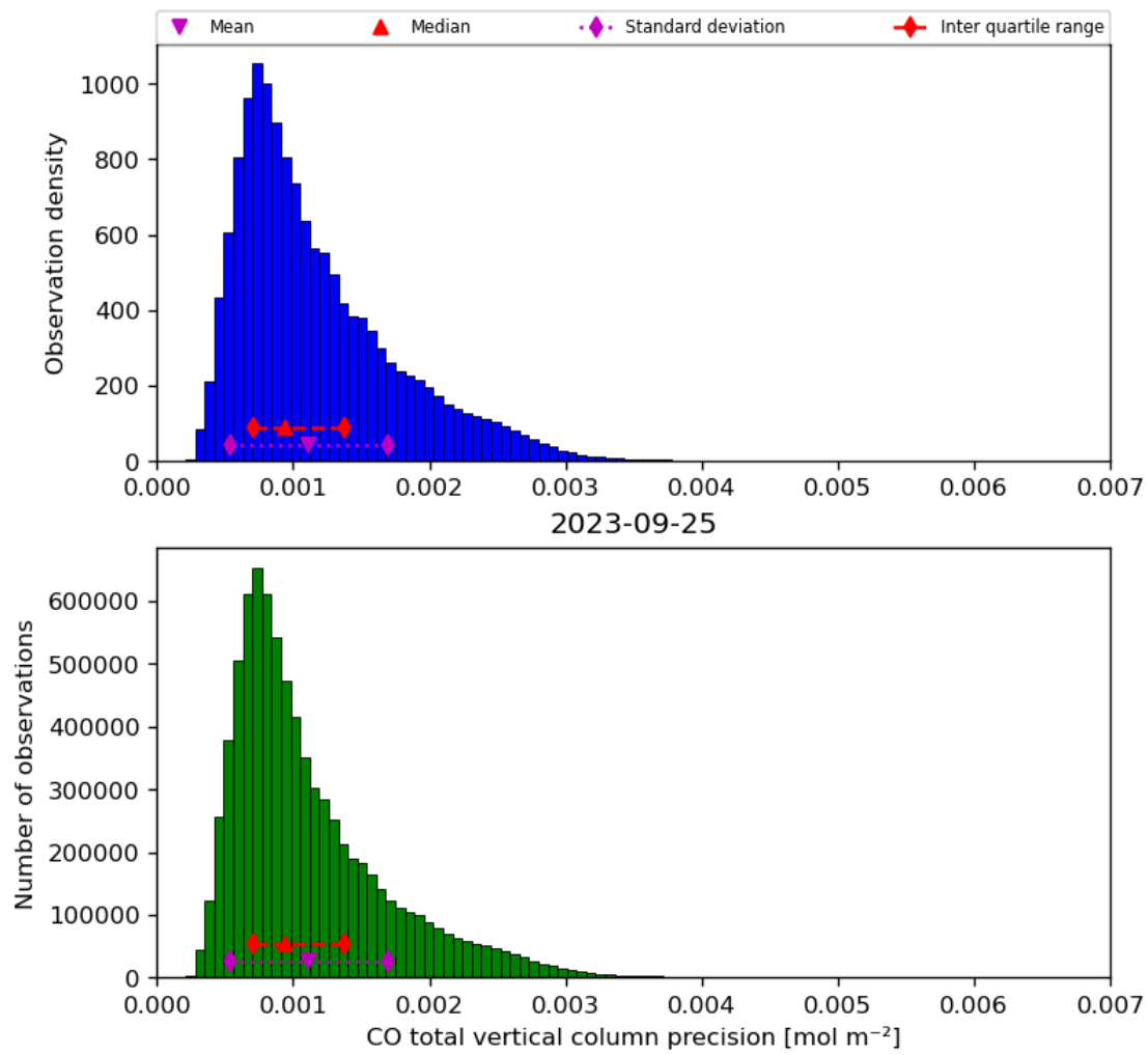
Figure 20: Histogram of “CO total vertical column precision” for 2023-09-24 to 2023-09-26
