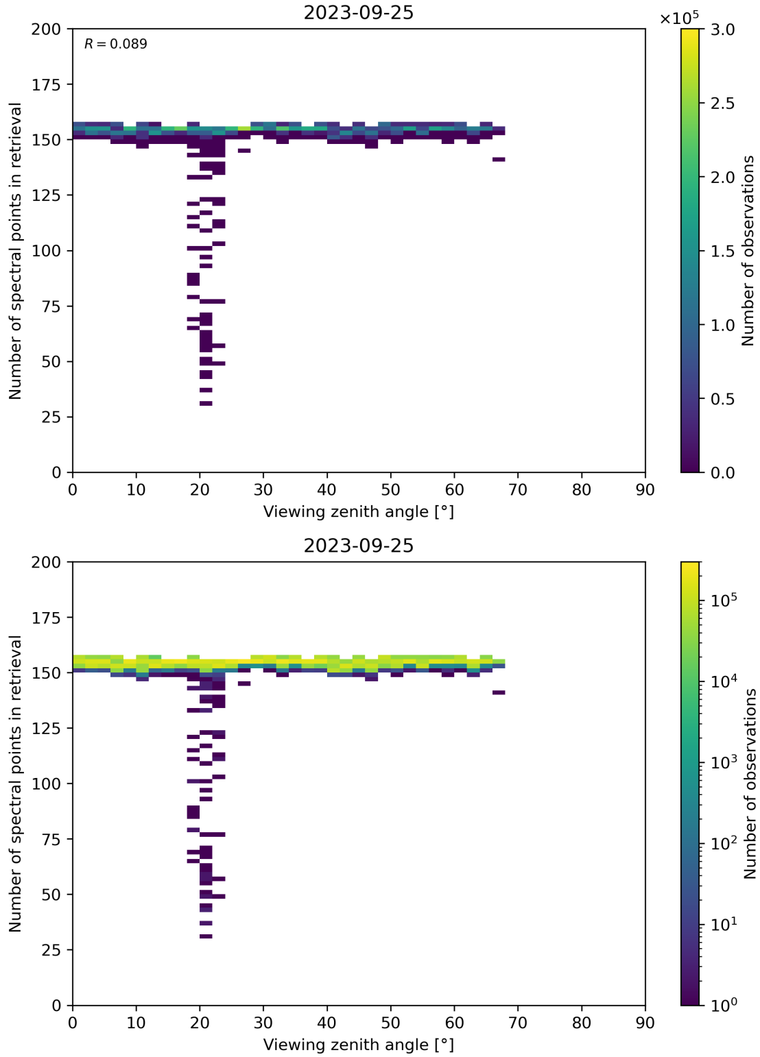
Figure 76: Scatter density plot of “Viewing zenith angle” against “Number of spectral points in retrieval” for 2023-09-24 to 2023-09-26.
