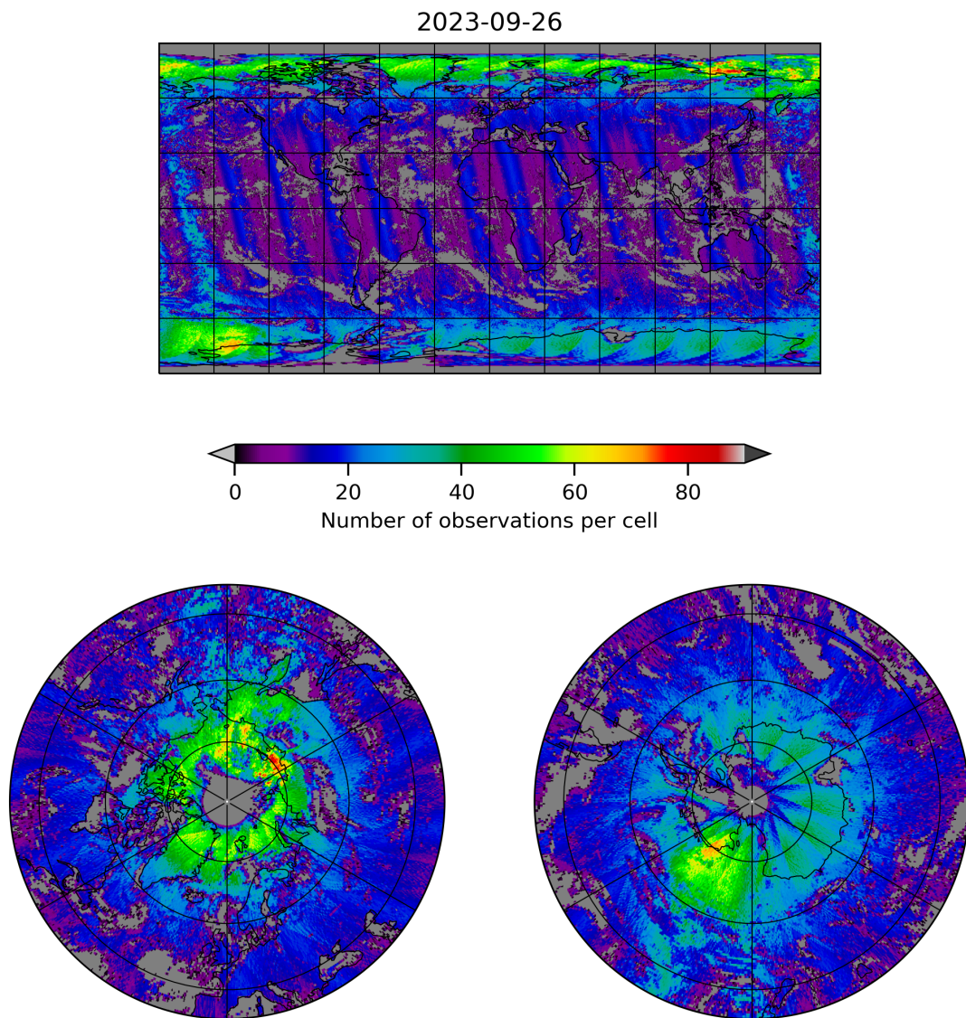
Figure 8: Map of the number of observations for 2023-09-26 to 2023-09-27
