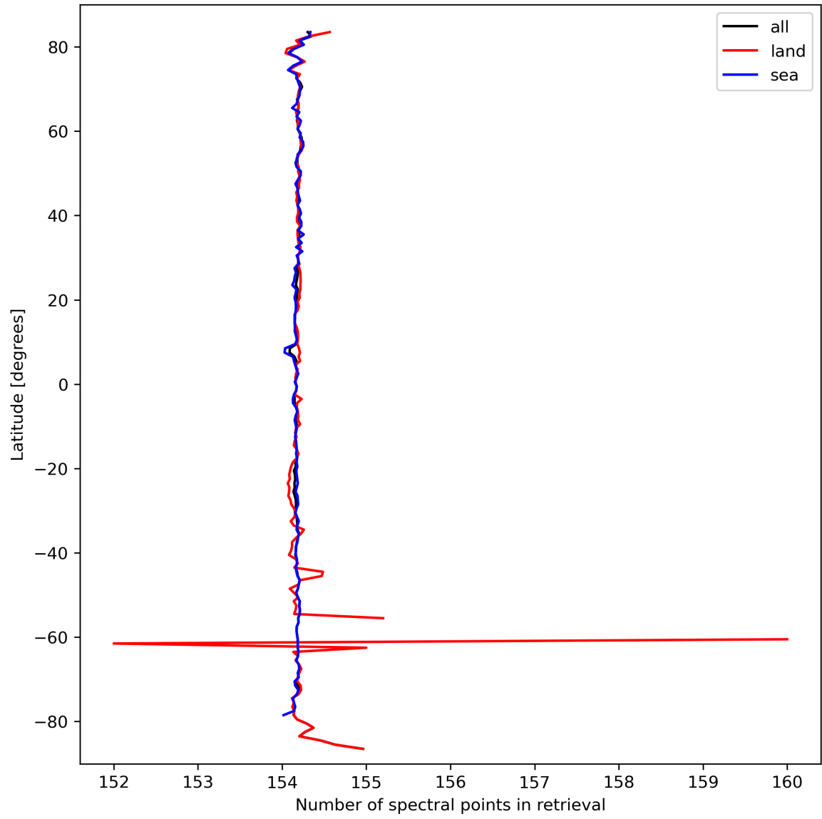
Figure 13: Zonal average of “Number of spectral points in retrieval” for 2023-09-26 to 2023-09-27.
