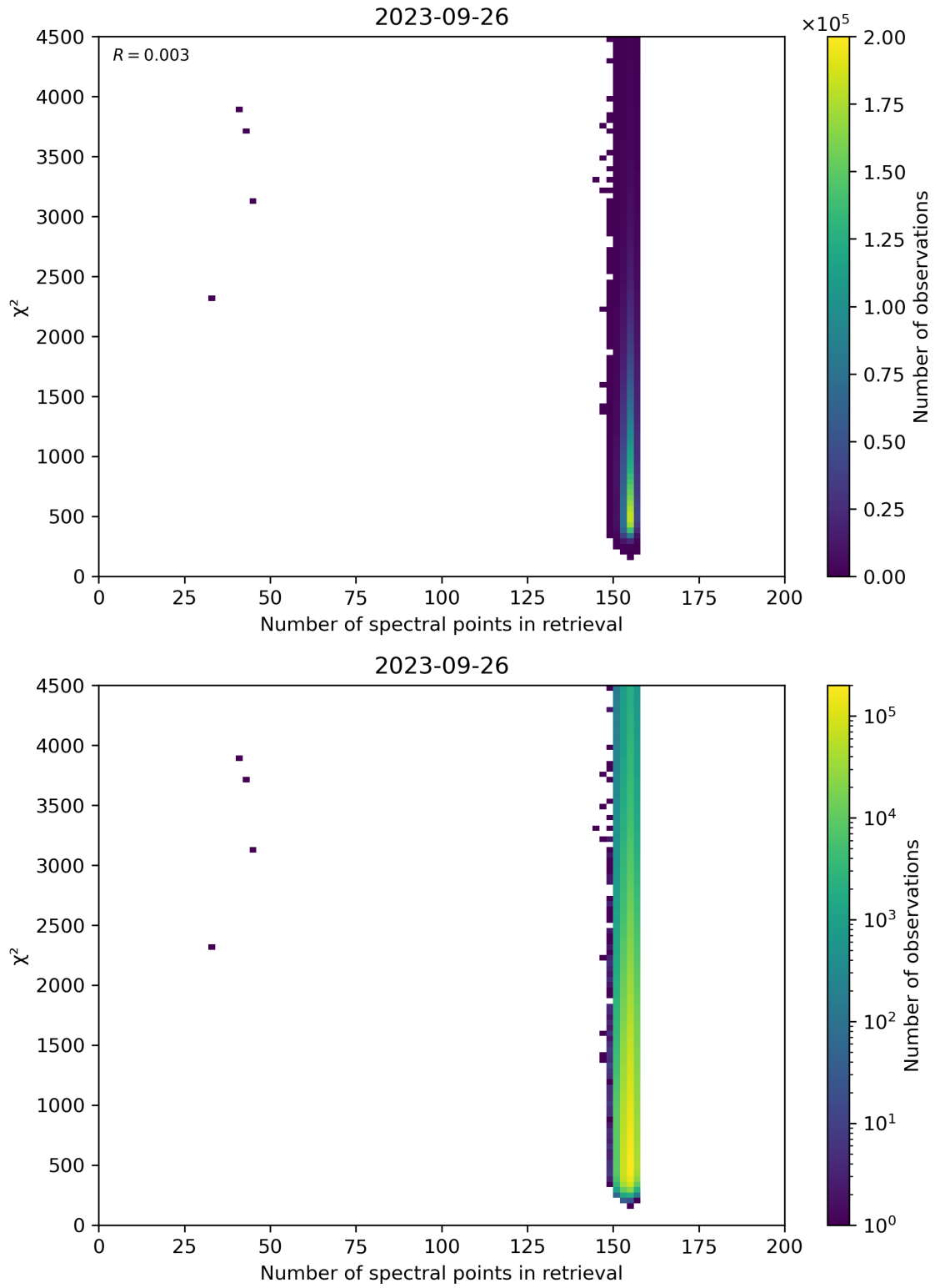
Figure 58: Scatter density plot of “Number of spectral points in retrieval” against “ \chi^2 ” for 2023-09-26 to 2023-09-27.
