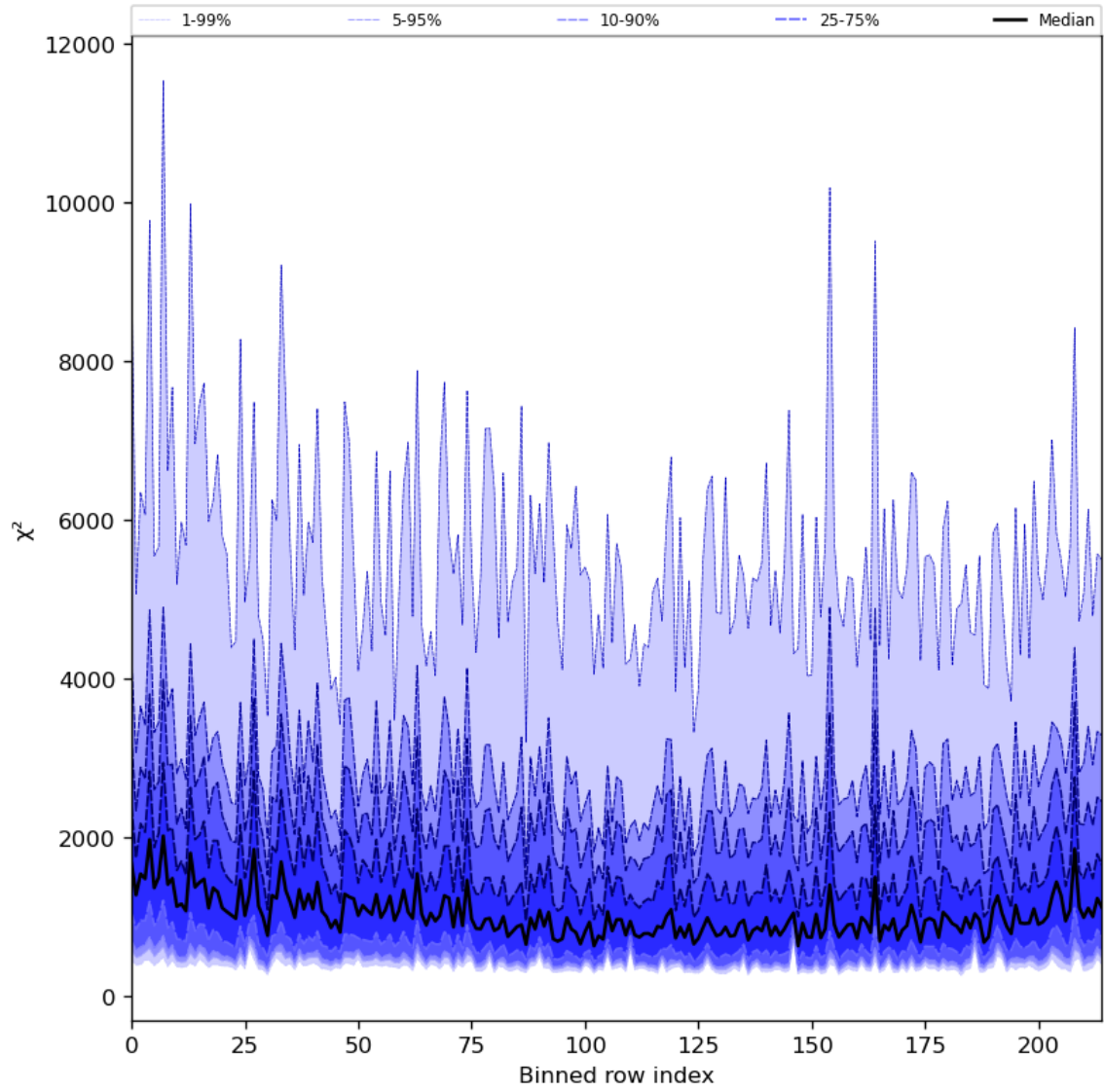
Figure 30: Along track statistics of “ \chi^2 ” for 2023-09-26 to 2023-09-27
