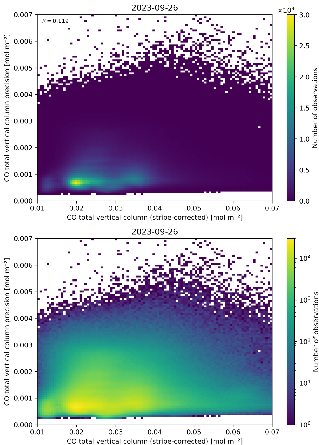
Figure 36: Scatter density plot of “CO total vertical column (stripe-corrected)” against “CO total vertical column precision” for 2023-09-26 to 2023-09-27.
