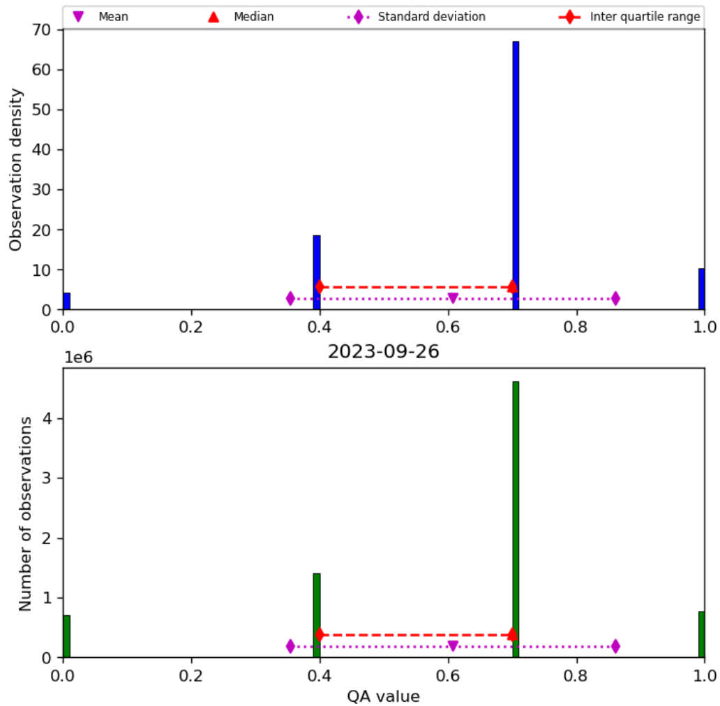
Figure 17: Histogram of “QA value” for 2023-09-26 to 2023-09-27
