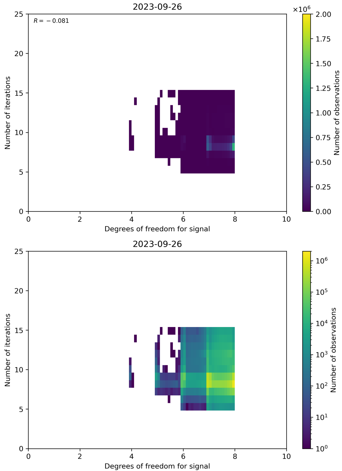
Figure 50: Scatter density plot of “Degrees of freedom for signal” against “Number of iterations” for 2023-09-26 to 2023-09-27.
