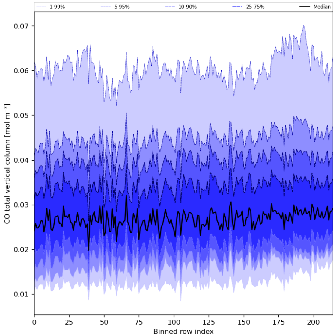
Figure 26: Along track statistics of “CO total vertical column” for 2023-09-26 to 2023-09-27
