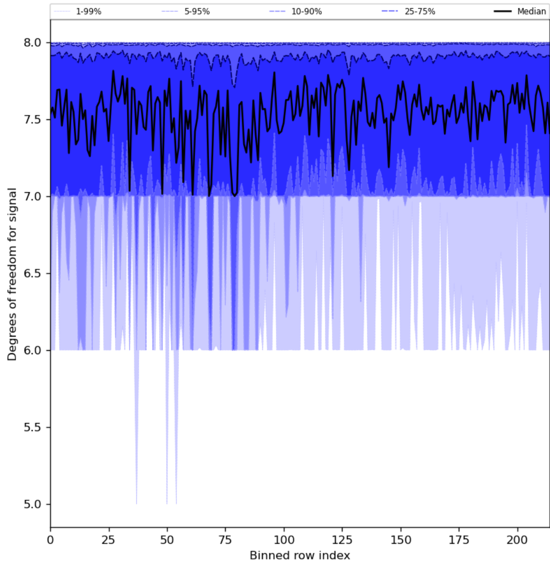
Figure 31: Along track statistics of “Degrees of freedom for signal” for 2023-09-26 to 2023-09-27
