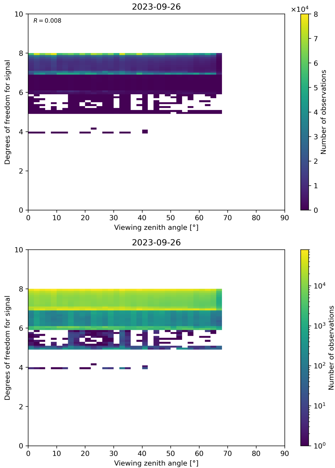
Figure 73: Scatter density plot of “Viewing zenith angle” against “Degrees of freedom for signal” for 2023-09-26 to 2023-09-27.
