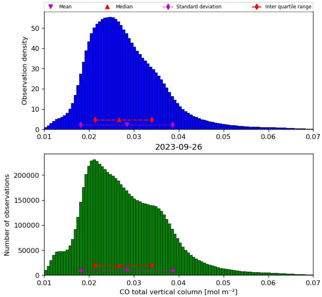
Figure 18: Histogram of “CO total vertical column” for 2023-09-26 to 2023-09-27
