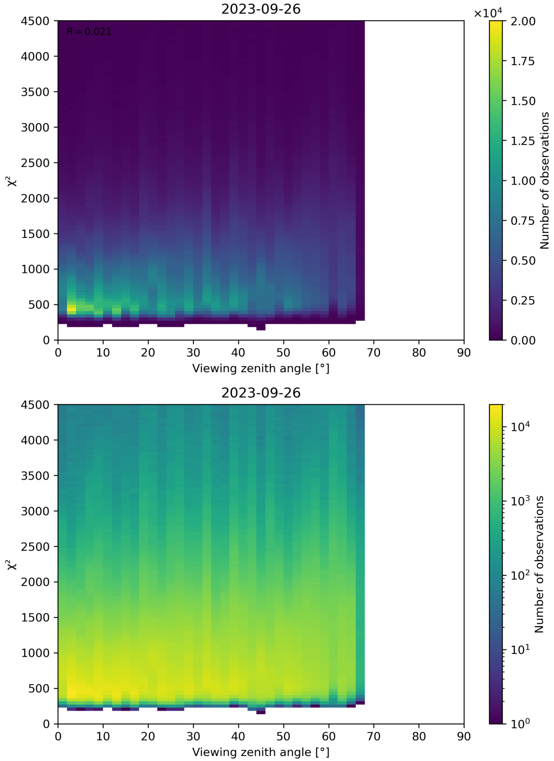
Figure 72: Scatter density plot of “Viewing zenith angle” against “ \chi^2 ” for 2023-09-26 to 2023-09-27.
