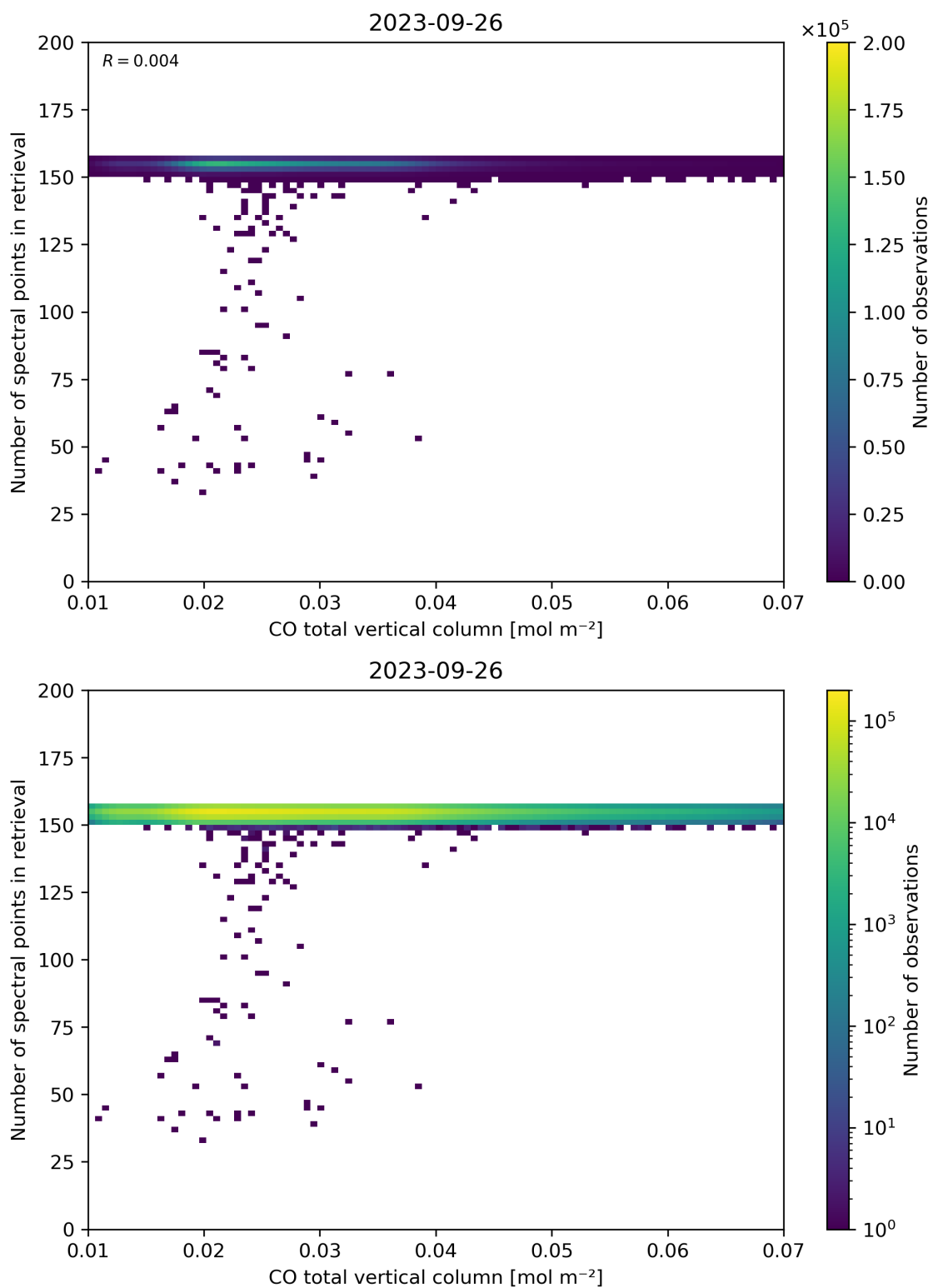
Figure 43: Scatter density plot of “CO total vertical column” against “Number of spectral points in retrieval” for 2023-09-26 to 2023-09-27.
