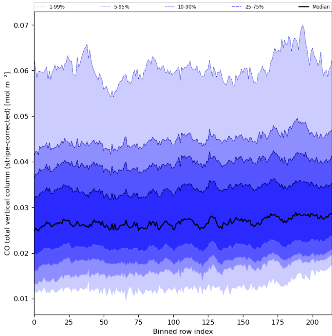
Figure 27: Along track statistics of “CO total vertical column (stripe-corrected)” for 2023-09-26 to 2023-09-27
