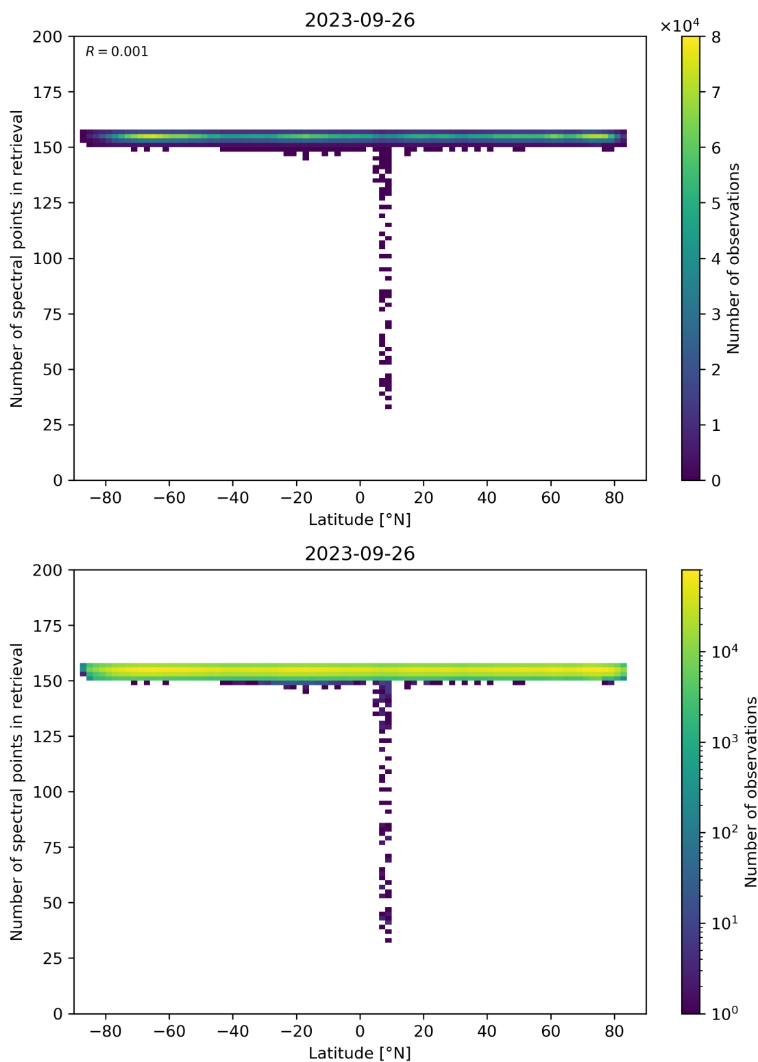
Figure 57: Scatter density plot of “Latitude” against “Number of spectral points in retrieval” for 2023-09-26 to 2023-09-27.
