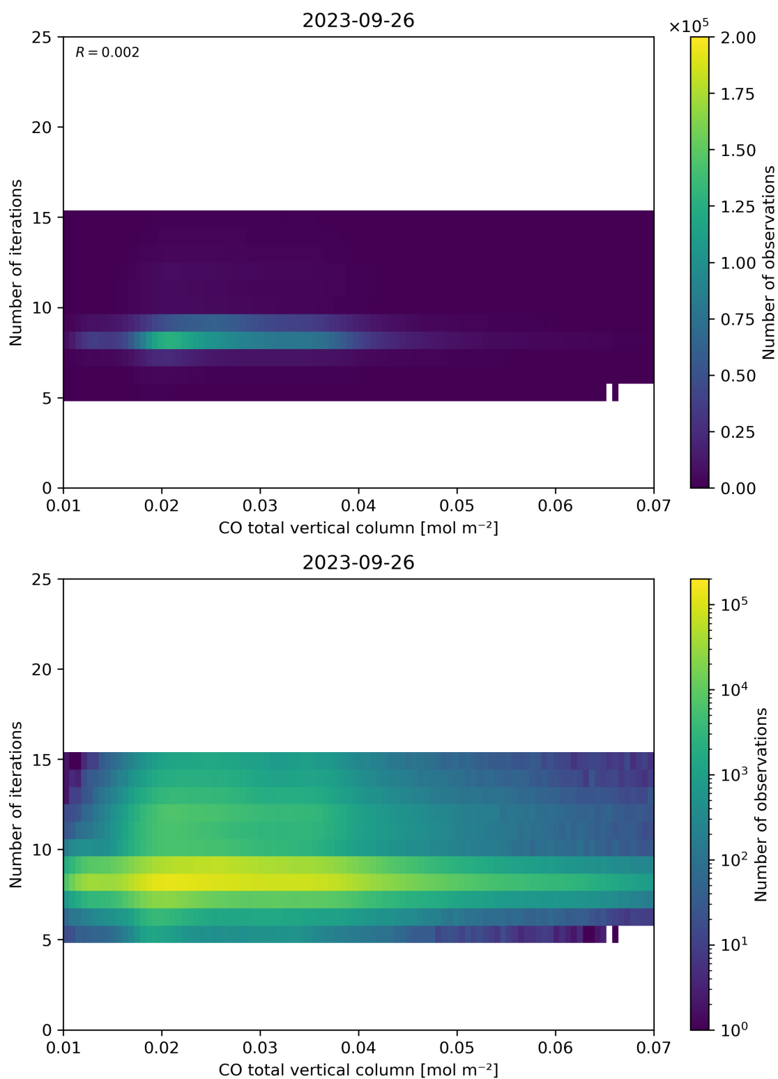
Figure 42: Scatter density plot of “CO total vertical column” against “Number of iterations” for 2023-09-26 to 2023-09-27.
