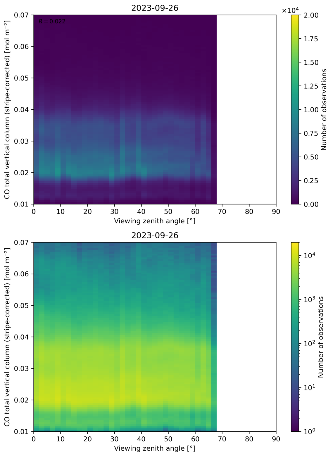
Figure 70: Scatter density plot of “Viewing zenith angle” against “CO total vertical column (stripe-corrected)” for 2023-09-26 to 2023-09-27.
