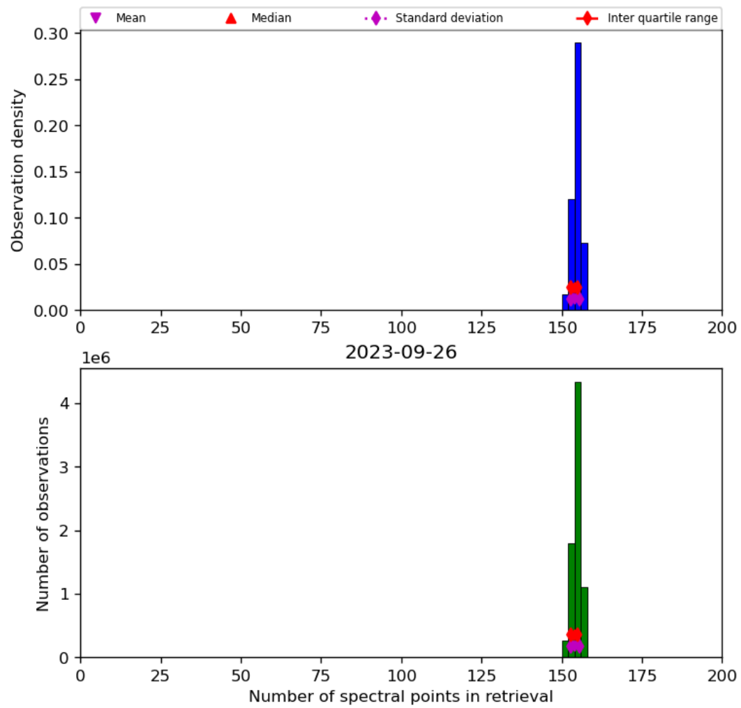
Figure 21: Histogram of “Number of spectral points in retrieval” for 2023-09-26 to 2023-09-27
