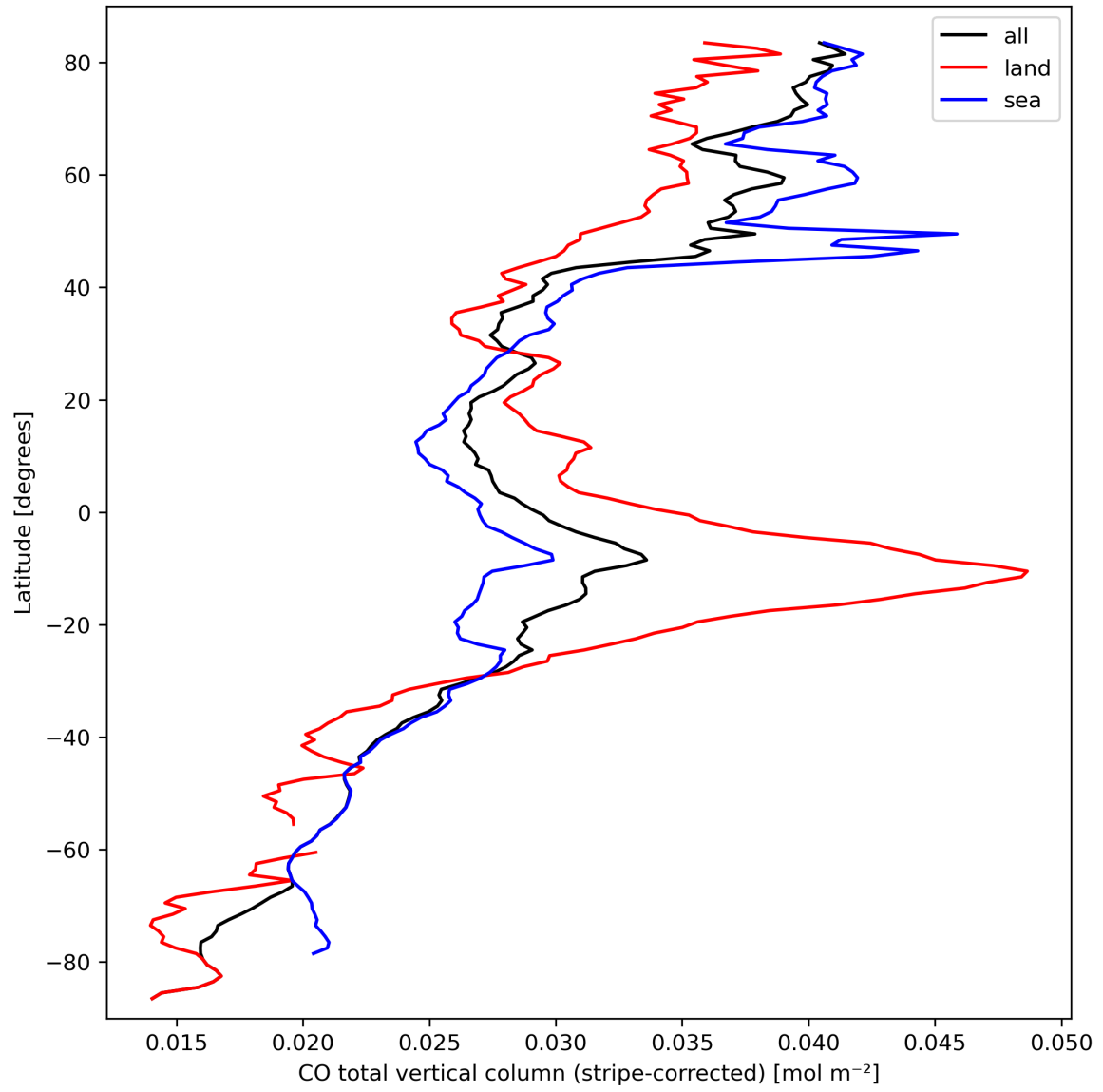
Figure 11: Zonal average of “CO total vertical column (stripe-corrected)” for 2023-09-26 to 2023-09-27.
