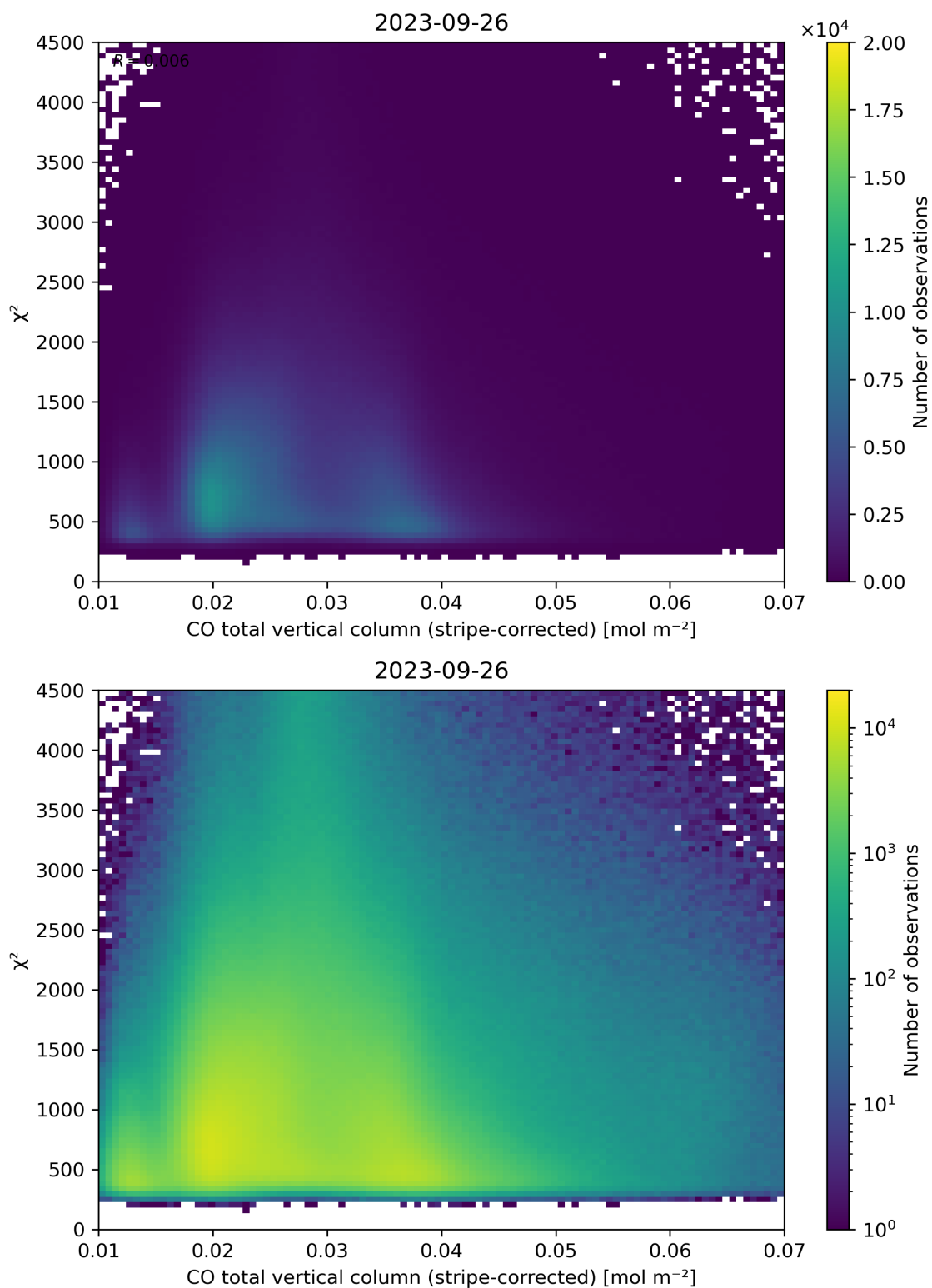
Figure 37: Scatter density plot of “CO total vertical column (stripe-corrected)” against “ \chi^2 ” for 2023-09-26 to 2023-09-27.
