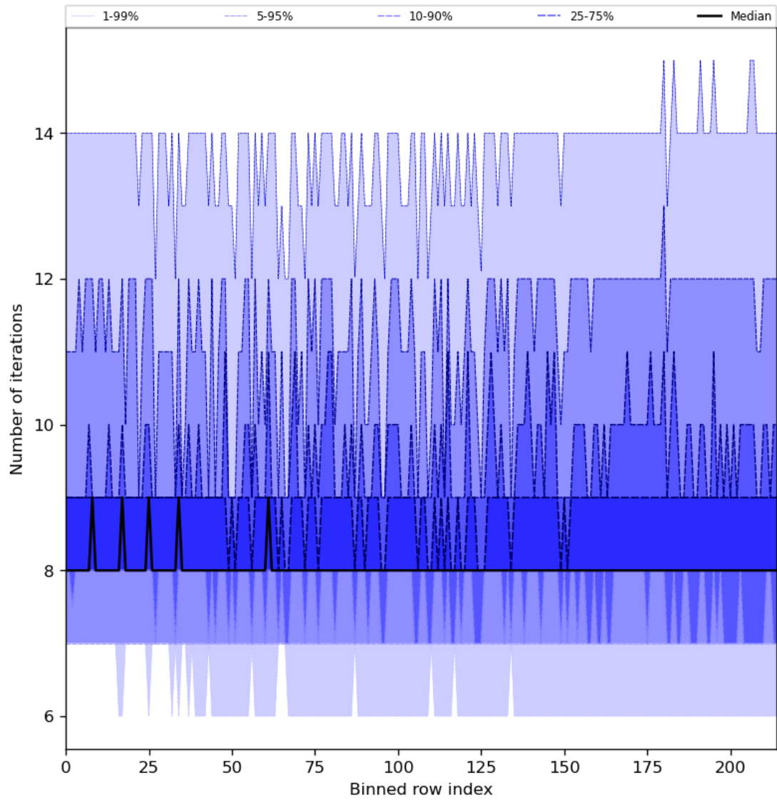
Figure 32: Along track statistics of “Number of iterations” for 2023-09-26 to 2023-09-27
