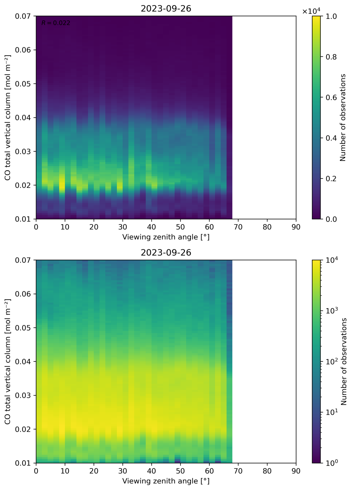
Figure 69: Scatter density plot of “Viewing zenith angle” against “CO total vertical column” for 2023-09-26 to 2023-09-27.
