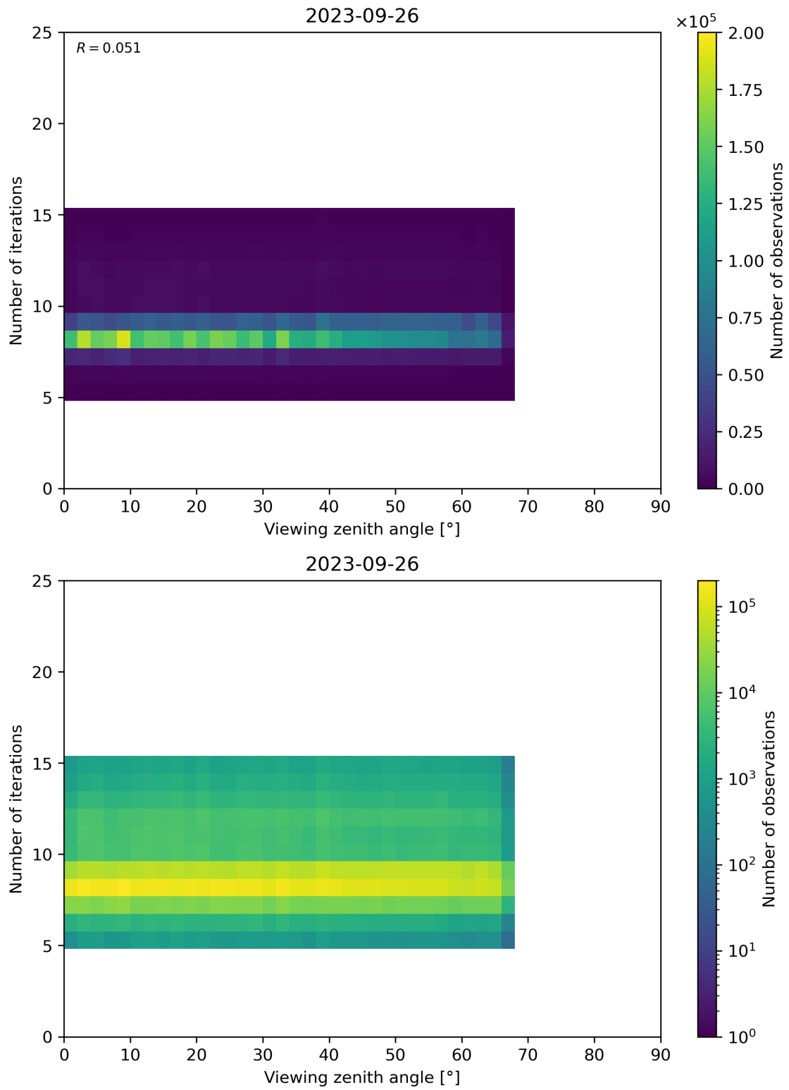
Figure 75: Scatter density plot of “Viewing zenith angle” against “Number of iterations” for 2023-09-26 to 2023-09-27.
