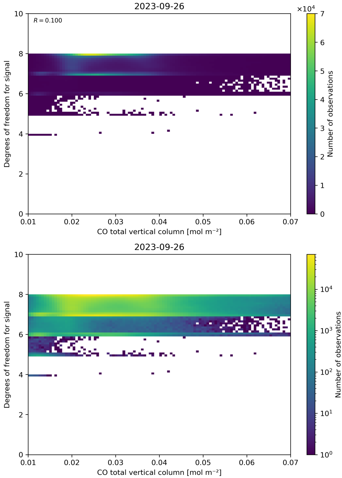
Figure 41: Scatter density plot of “CO total vertical column” against “Degrees of freedom for signal” for 2023-09-26 to 2023-09-27.
