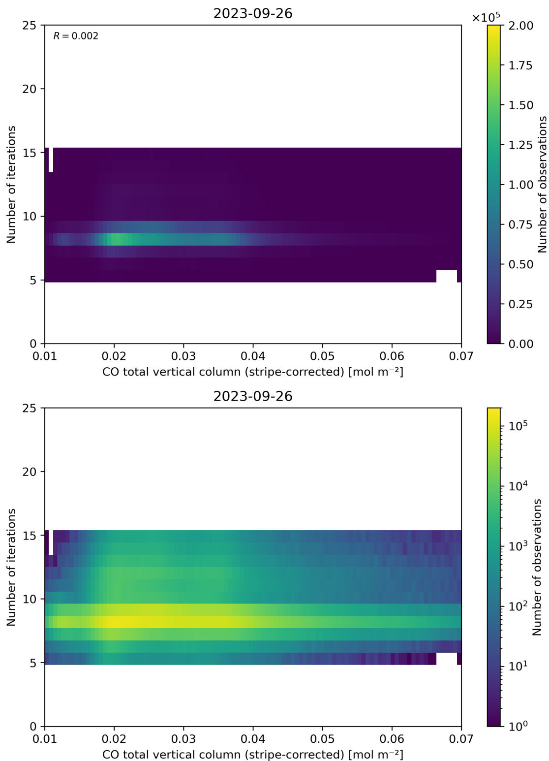
Figure 39: Scatter density plot of “CO total vertical column (stripe-corrected)” against “Number of iterations” for 2023-09-26 to 2023-09-27.
