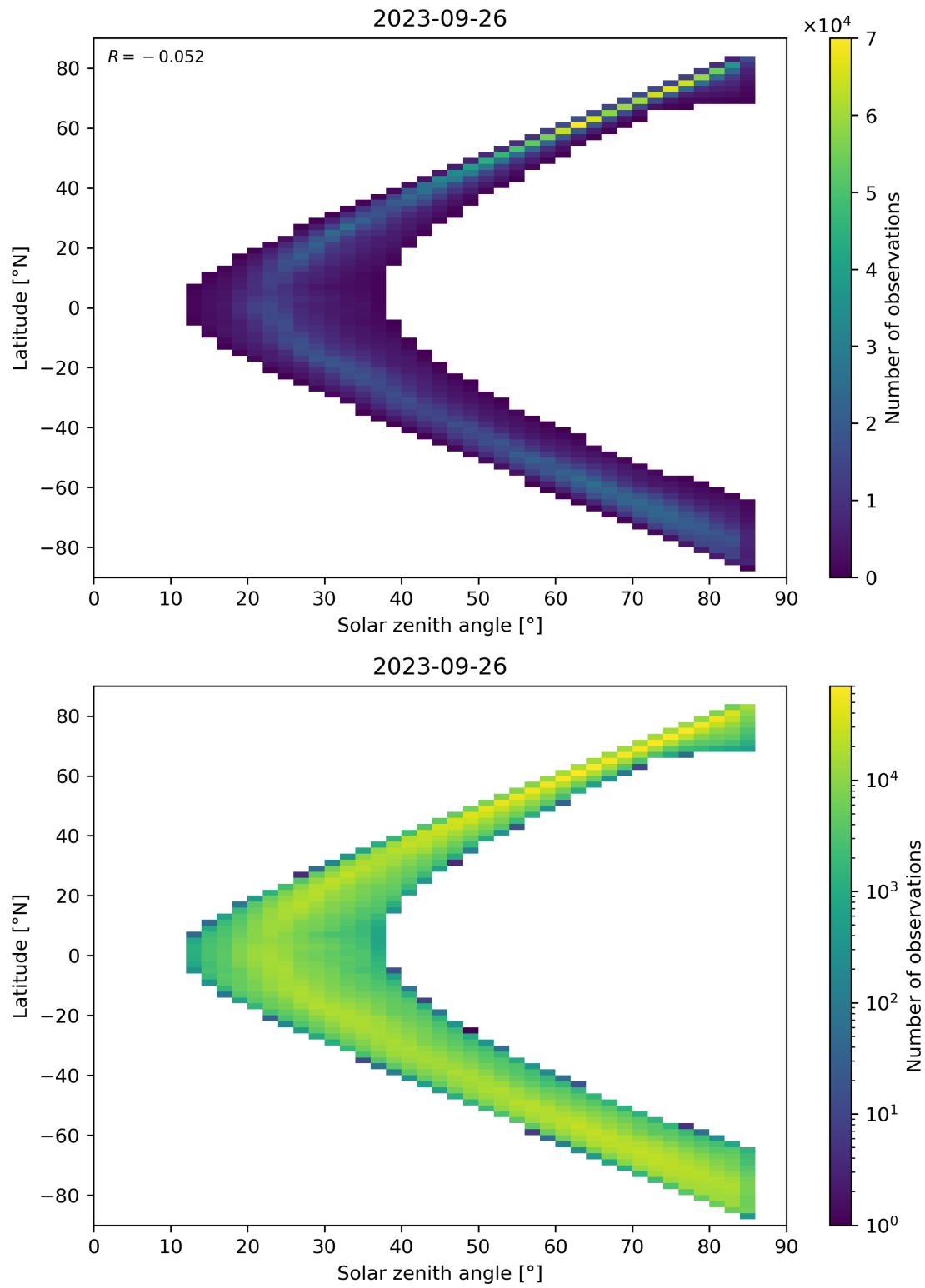
Figure 66: Scatter density plot of “Solar zenith angle” against “Latitude” for 2023-09-26 to 2023-09-27.
