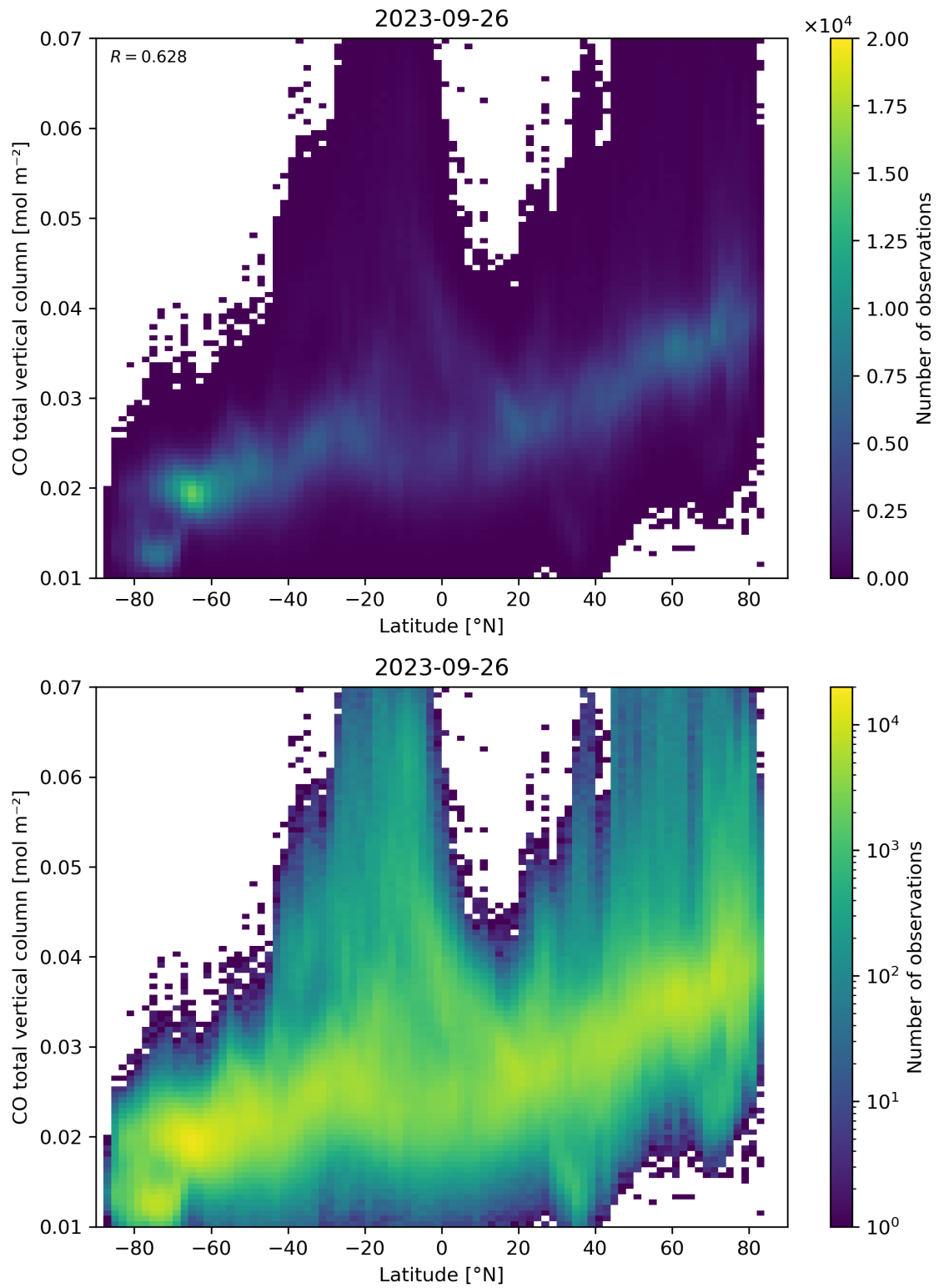
Figure 51: Scatter density plot of “Latitude” against “CO total vertical column” for 2023-09-26 to 2023-09-27.
