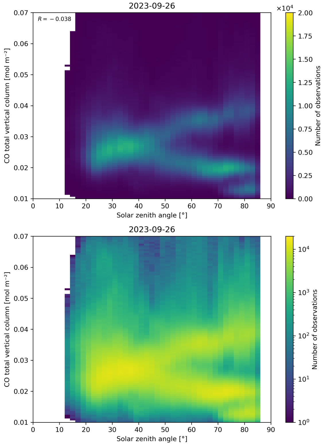
Figure 61: Scatter density plot of “Solar zenith angle” against “CO total vertical column” for 2023-09-26 to 2023-09-27.
