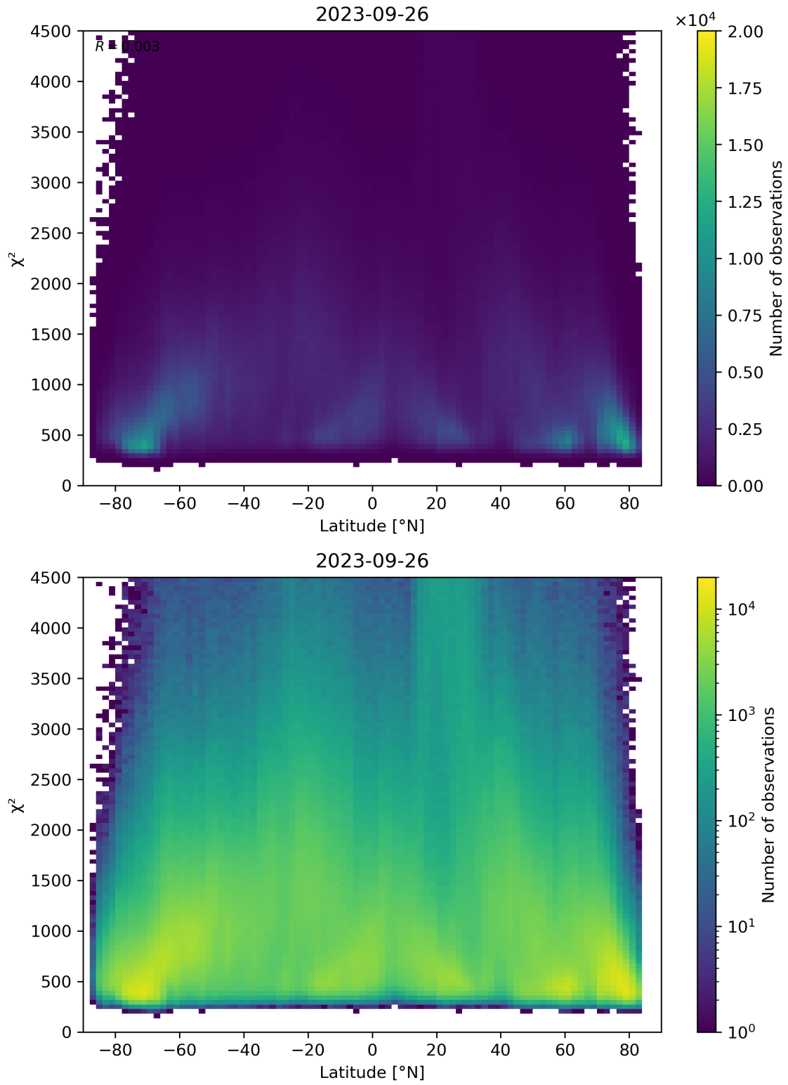
Figure 54: Scatter density plot of “Latitude” against “ \chi^2 ” for 2023-09-26 to 2023-09-27.
