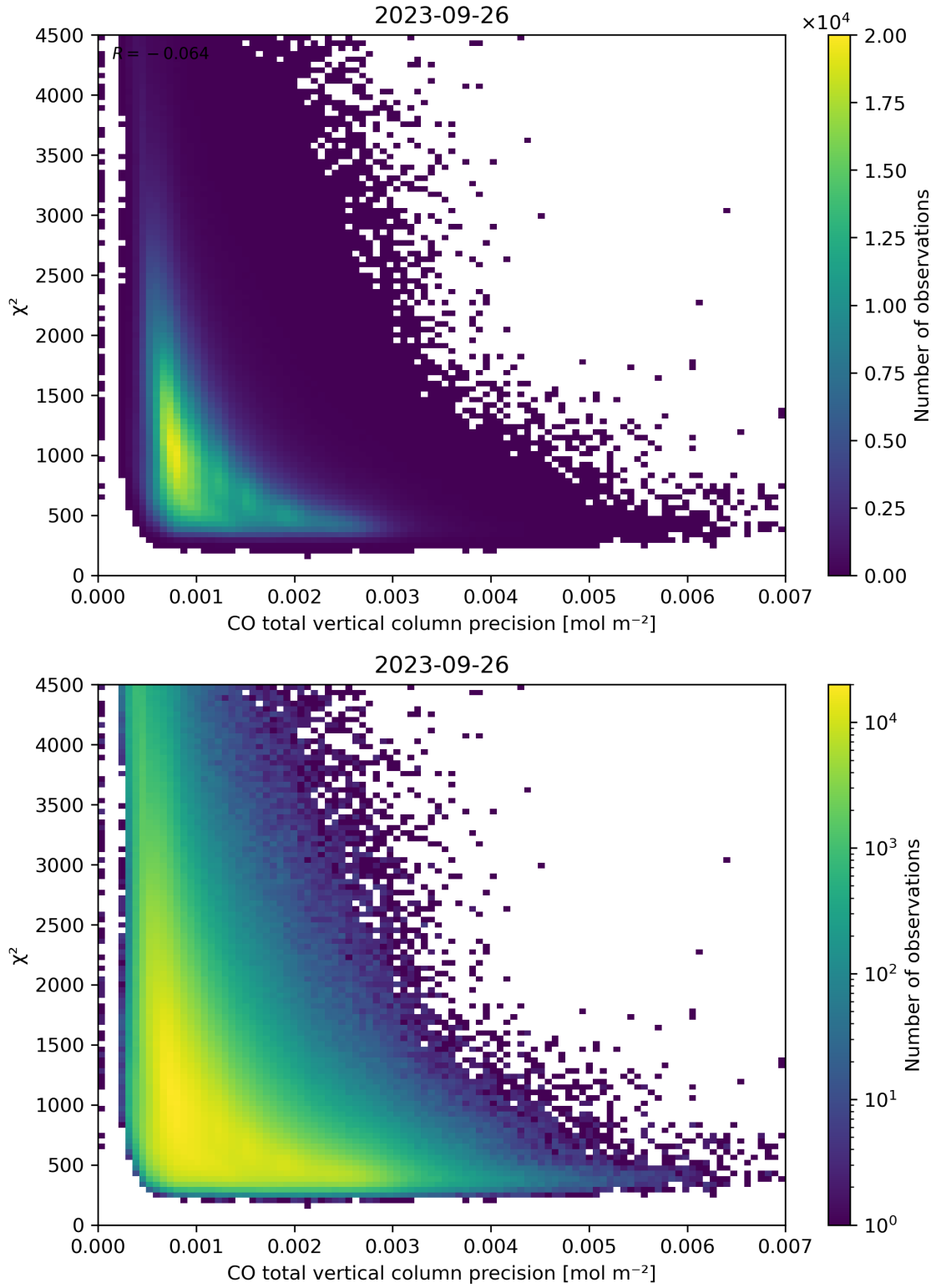
Figure 44: Scatter density plot of “CO total vertical column precision” against “ \chi^2 ” for 2023-09-26 to 2023-09-27.
