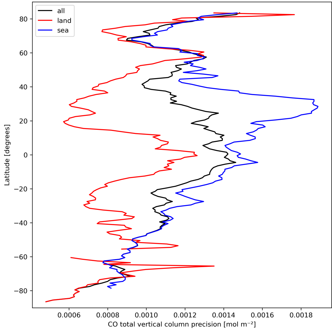
Figure 12: Zonal average of “CO total vertical column precision” for 2023-09-26 to 2023-09-27.
