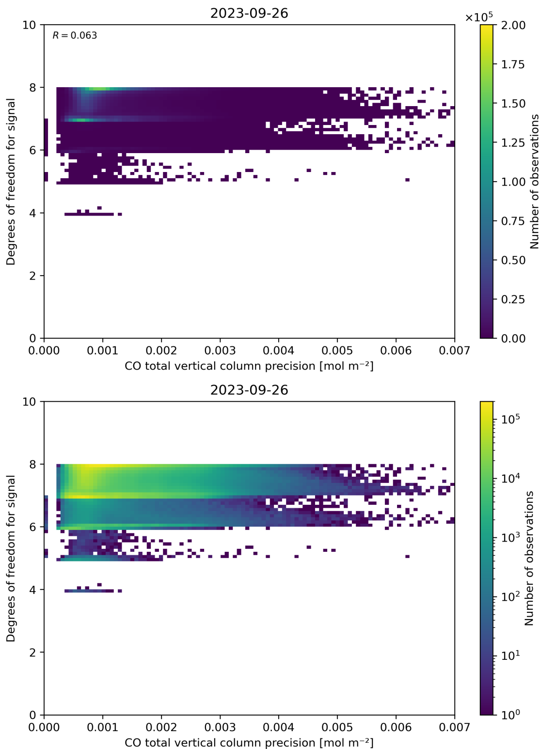
Figure 45: Scatter density plot of “CO total vertical column precision” against “Degrees of freedom for signal” for 2023-09-26 to 2023-09-27.
