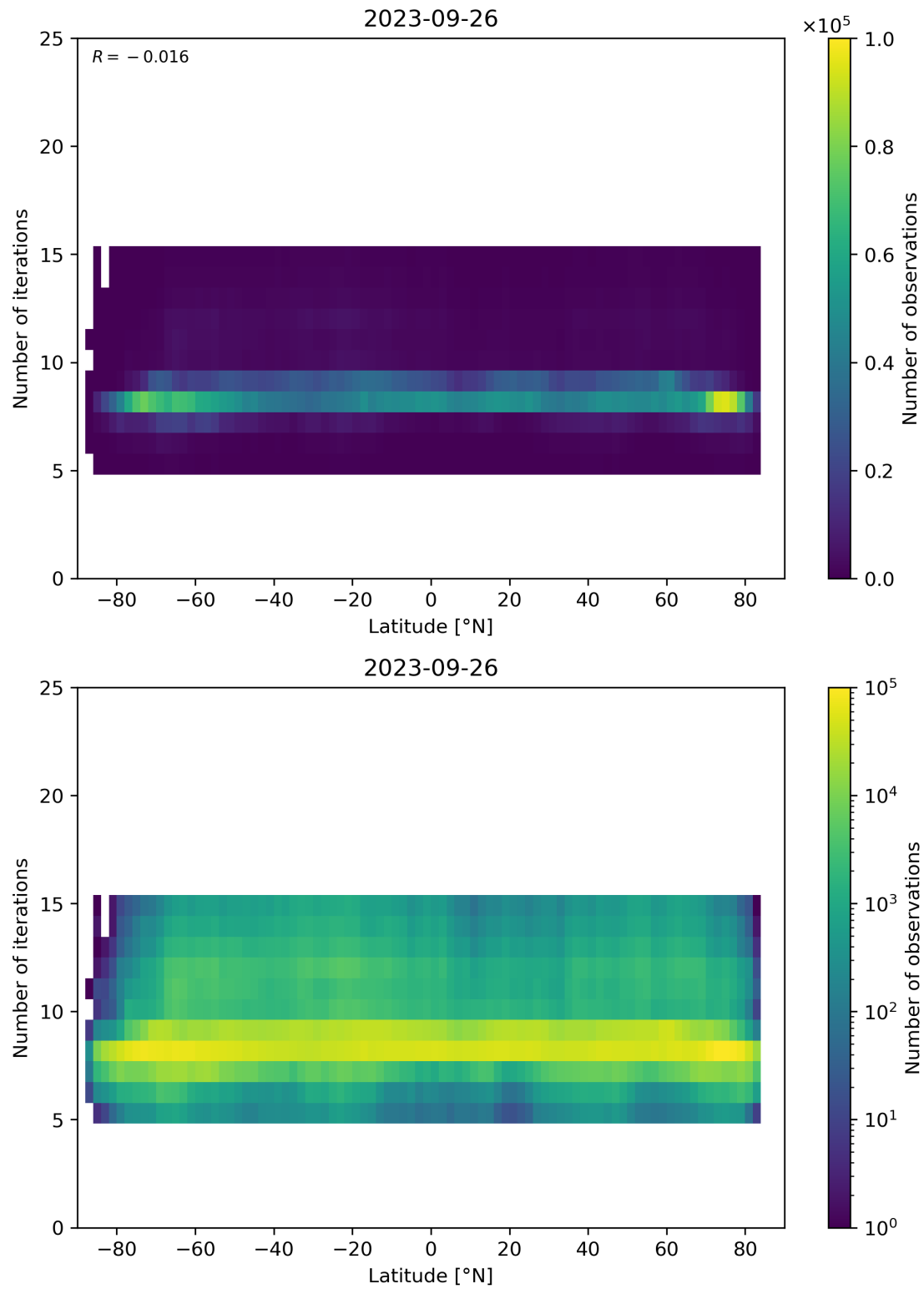
Figure 56: Scatter density plot of “Latitude” against “Number of iterations” for 2023-09-26 to 2023-09-27.
