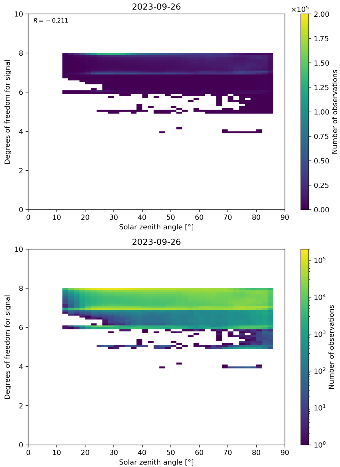
Figure 65: Scatter density plot of “Solar zenith angle” against “Degrees of freedom for signal” for 2023-09-26 to 2023-09-27.
