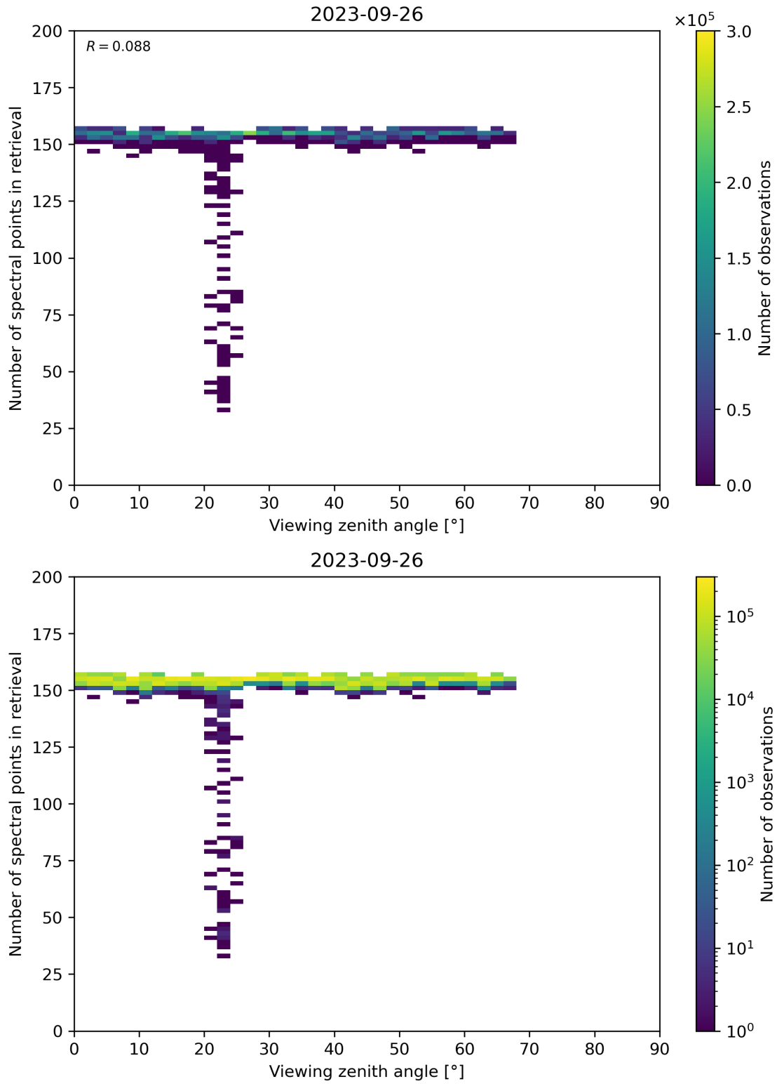
Figure 76: Scatter density plot of “Viewing zenith angle” against “Number of spectral points in retrieval” for 2023-09-26 to 2023-09-27.
