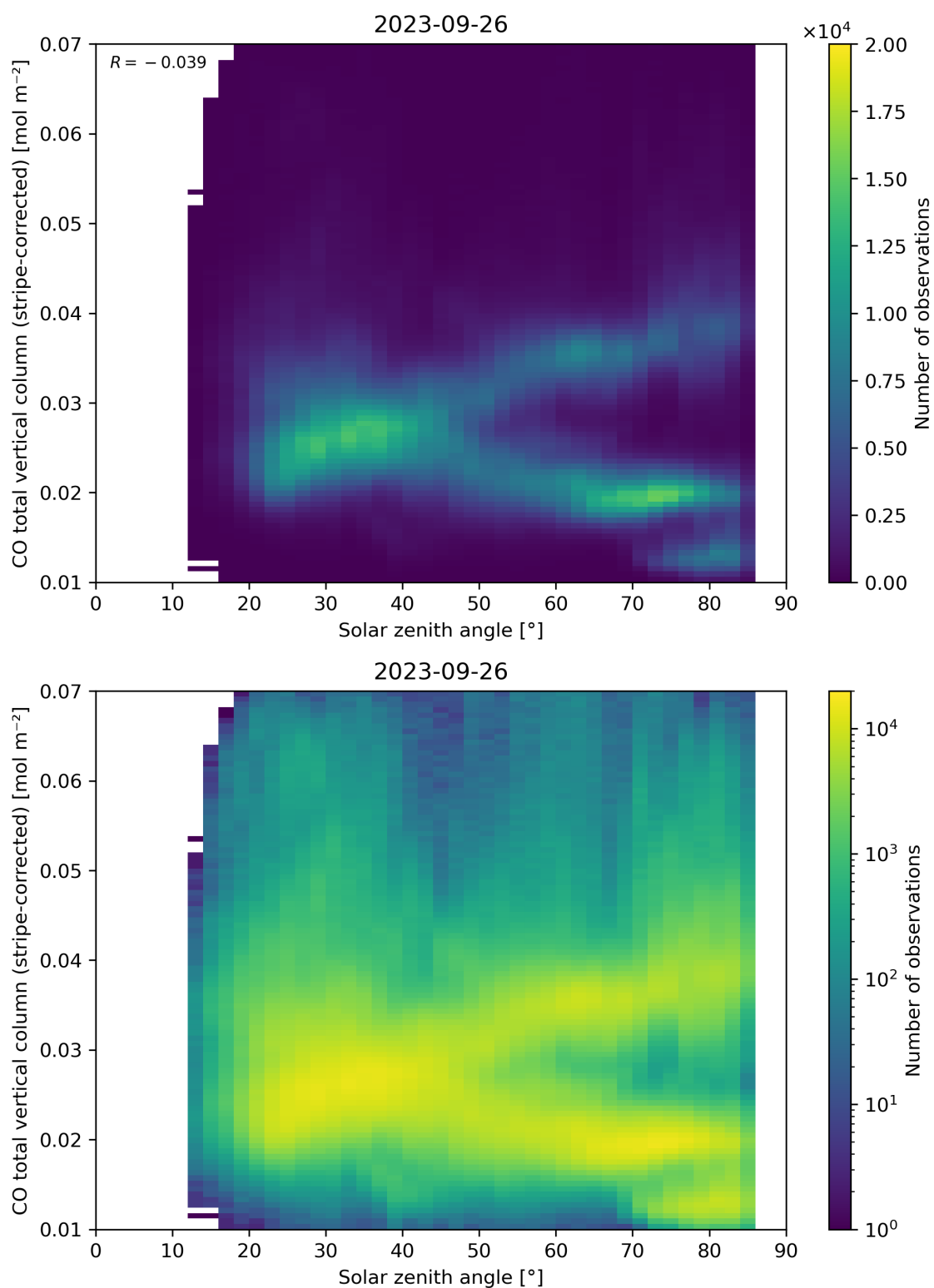
Figure 62: Scatter density plot of “Solar zenith angle” against “CO total vertical column (stripe-corrected)” for 2023-09-26 to 2023-09-27.
