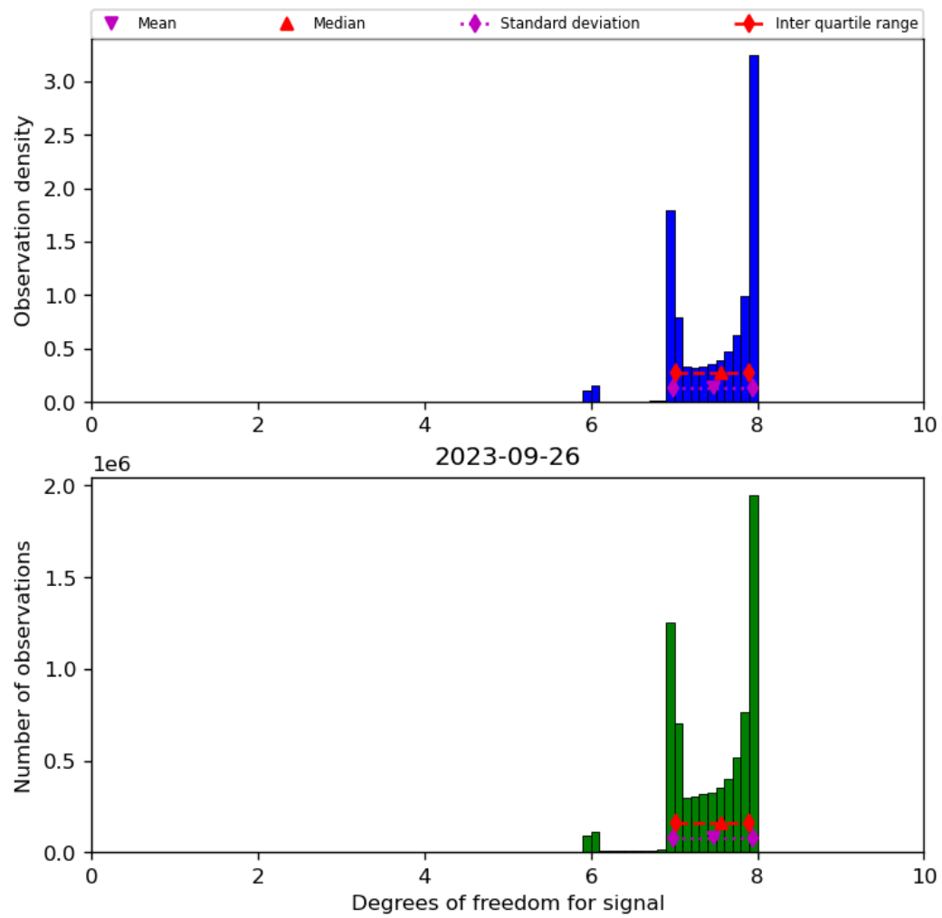
Figure 23: Histogram of “Degrees of freedom for signal” for 2023-09-26 to 2023-09-27
