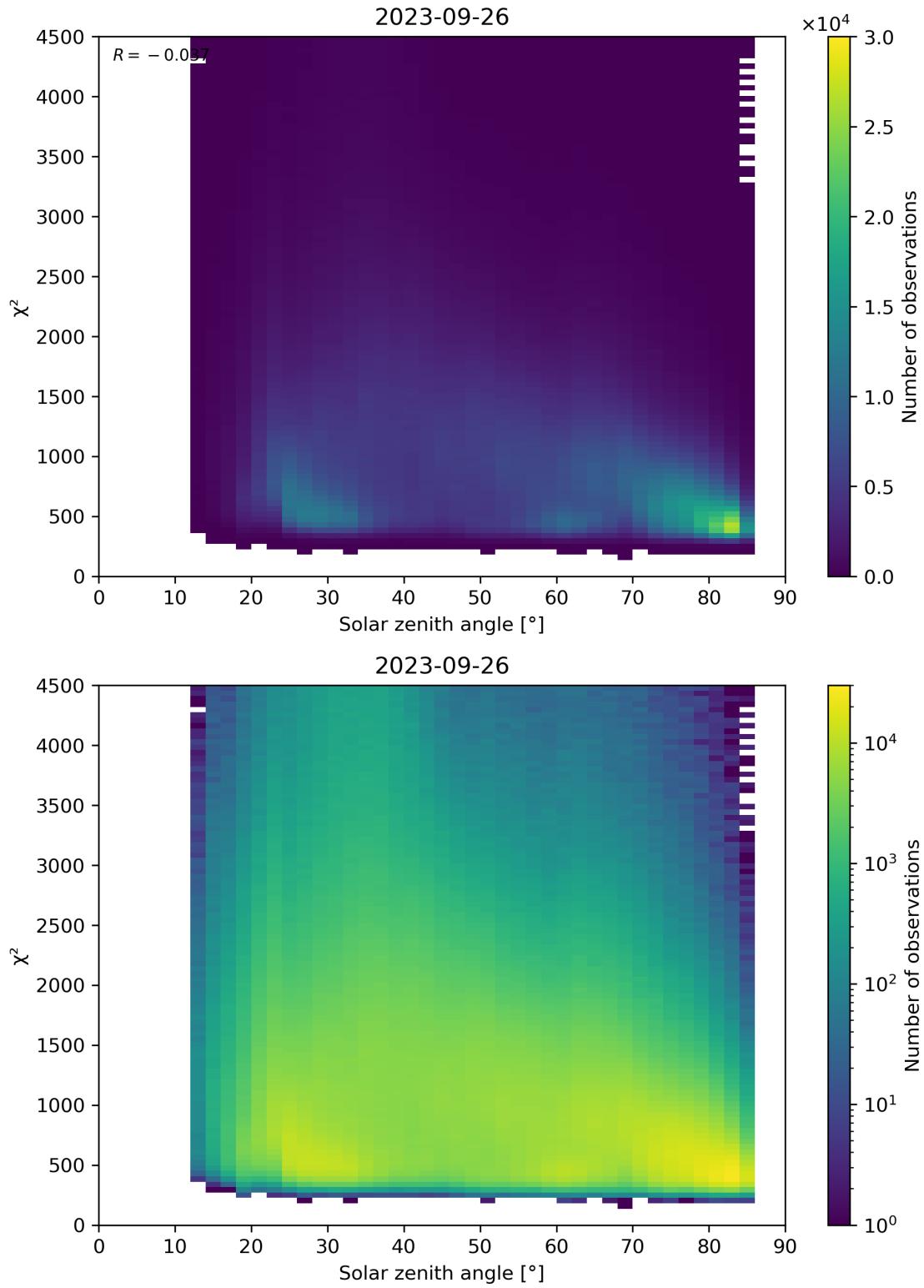
Figure 64: Scatter density plot of “Solar zenith angle” against “ \chi^2 ” for 2023-09-26 to 2023-09-27.
