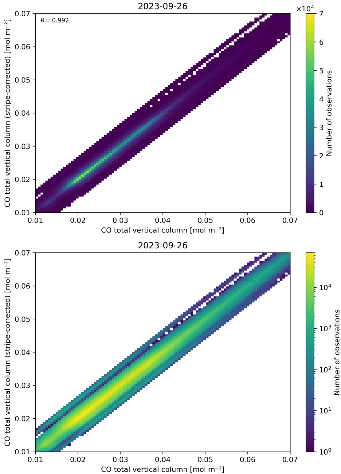
Figure 33: Scatter density plot of “CO total vertical column” against “CO total vertical column (stripe-corrected)” for 2023-09-26 to 2023-09-27.
