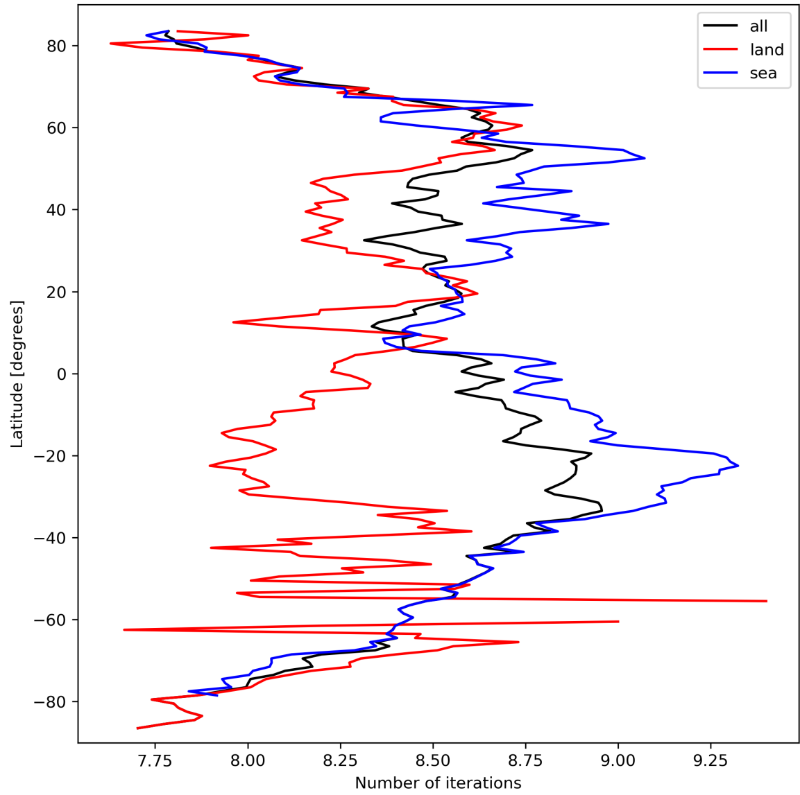
Figure 16: Zonal average of “Number of iterations” for 2023-09-26 to 2023-09-27.
