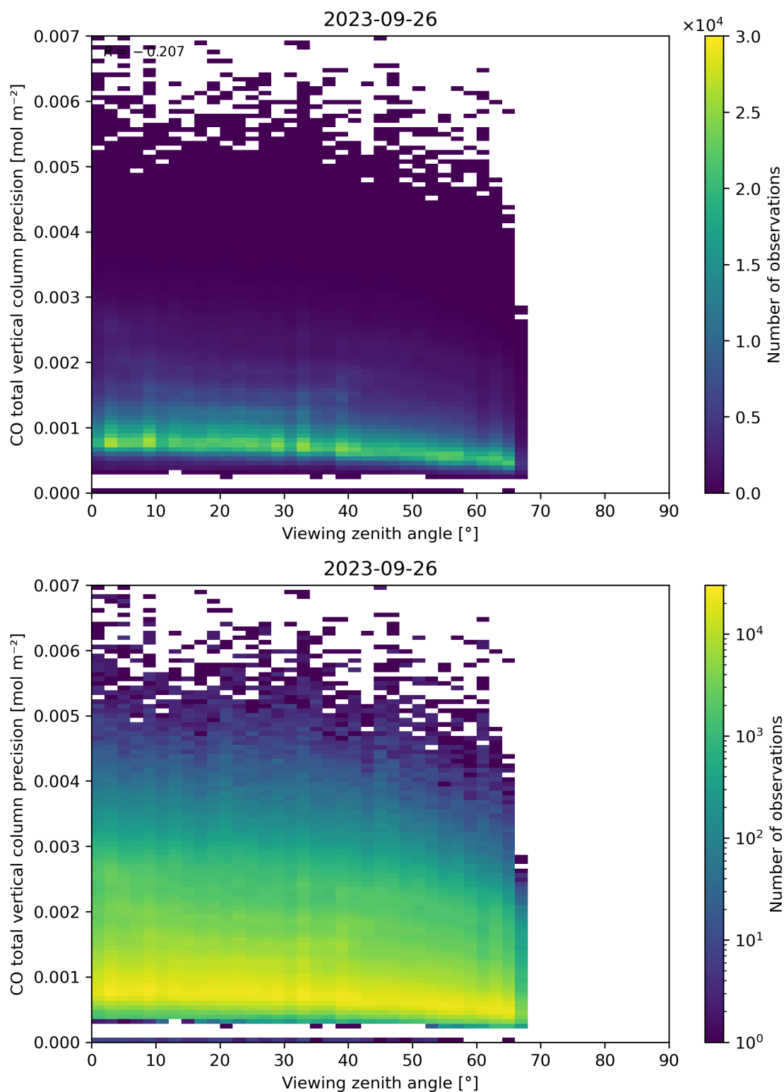
Figure 71: Scatter density plot of “Viewing zenith angle” against “CO total vertical column precision” for 2023-09-26 to 2023-09-27.
