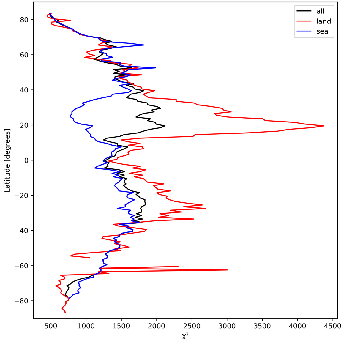
Figure 14: Zonal average of “ \chi^2 ” for 2023-09-26 to 2023-09-27.
