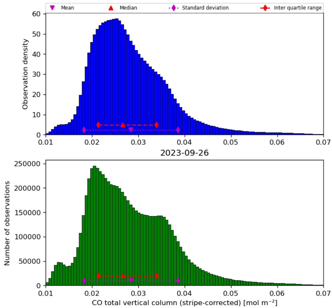
Figure 19: Histogram of “CO total vertical column (stripe-corrected)” for 2023-09-26 to 2023-09-27
