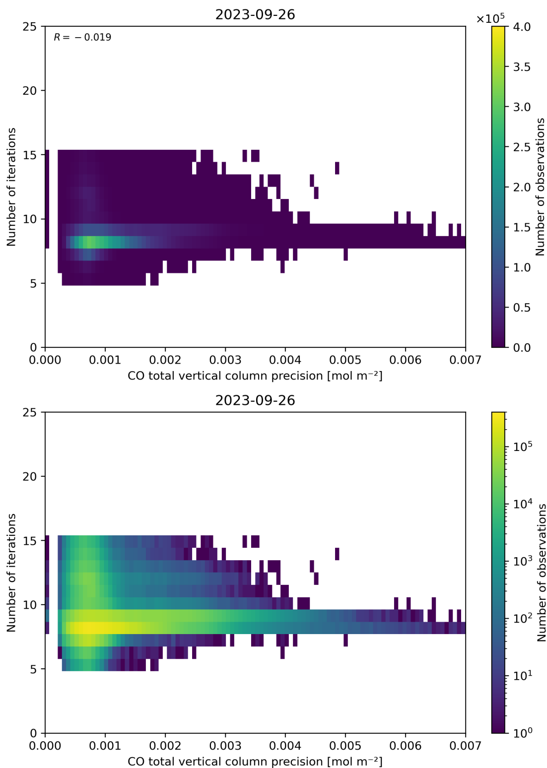
Figure 46: Scatter density plot of “CO total vertical column precision” against “Number of iterations” for 2023-09-26 to 2023-09-27.
