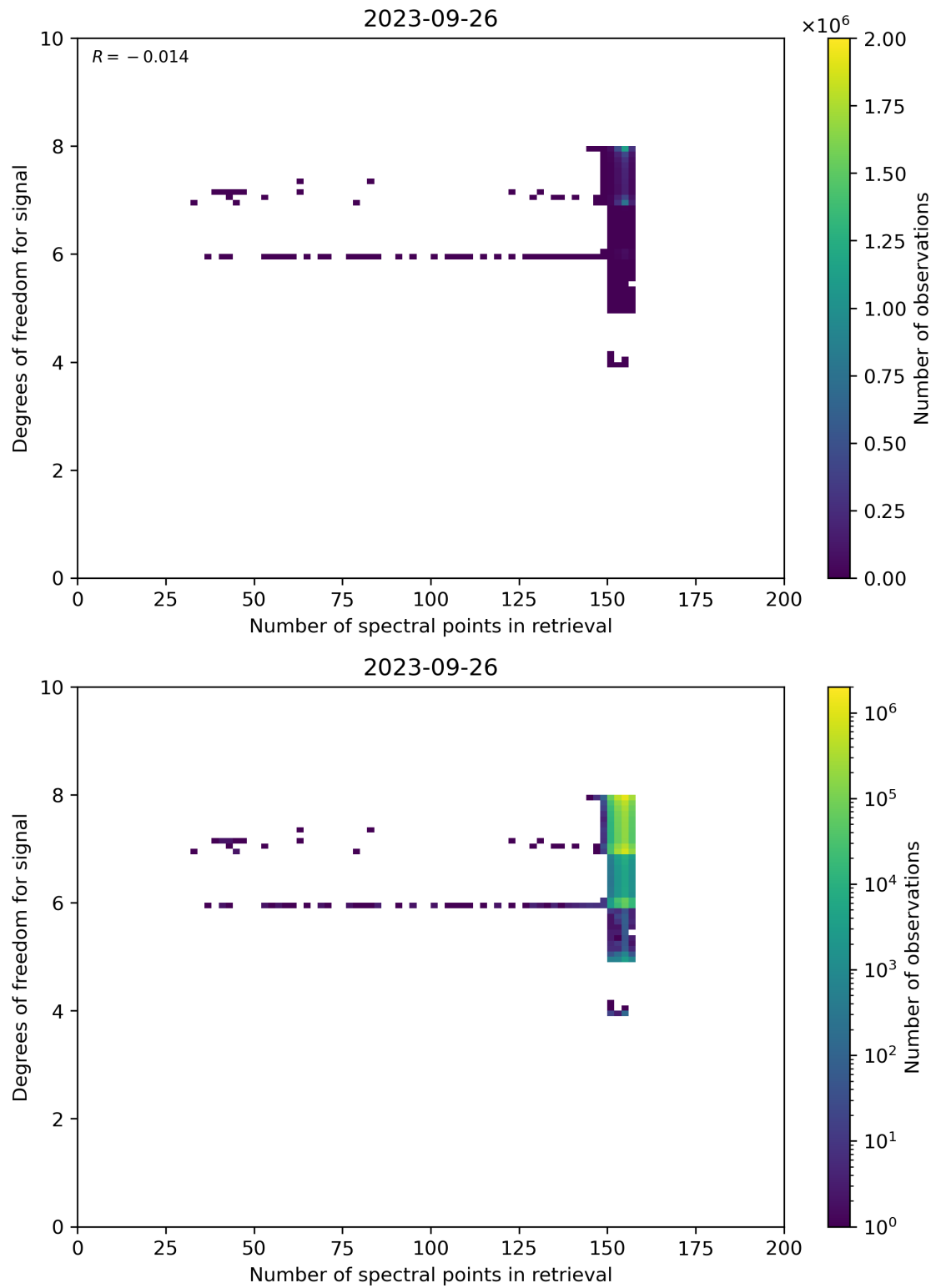
Figure 59: Scatter density plot of “Number of spectral points in retrieval” against “Degrees of freedom for signal” for 2023-09-26 to 2023-09-27.
