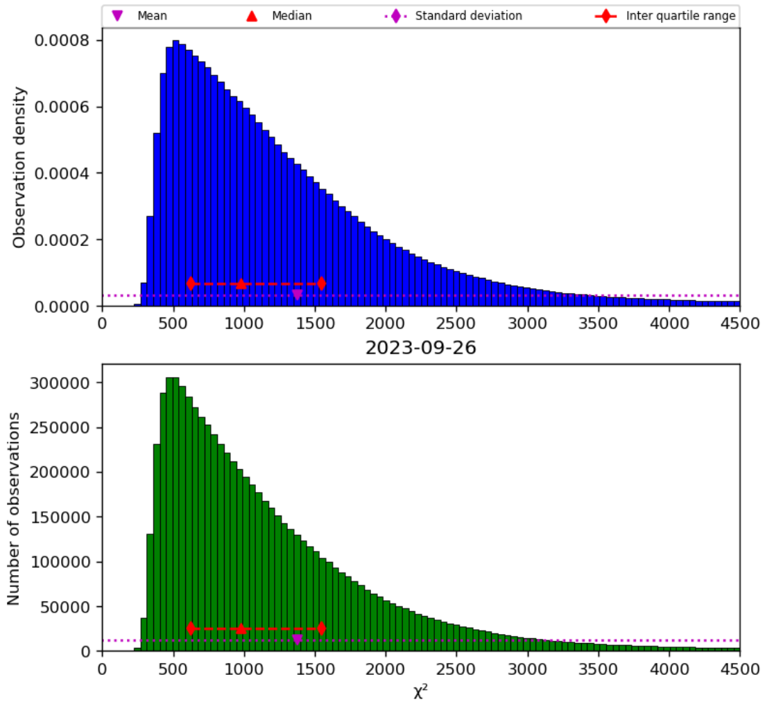
Figure 22: Histogram of “ \chi^2 ” for 2023-09-26 to 2023-09-27
