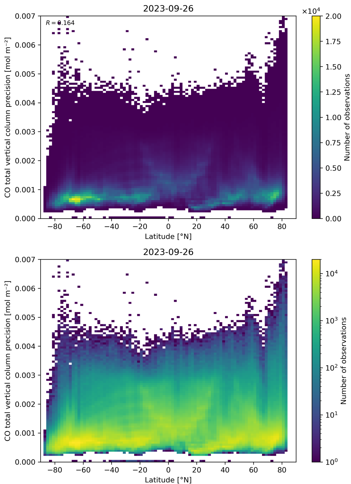
Figure 53: Scatter density plot of “Latitude” against “CO total vertical column precision” for 2023-09-26 to 2023-09-27.
