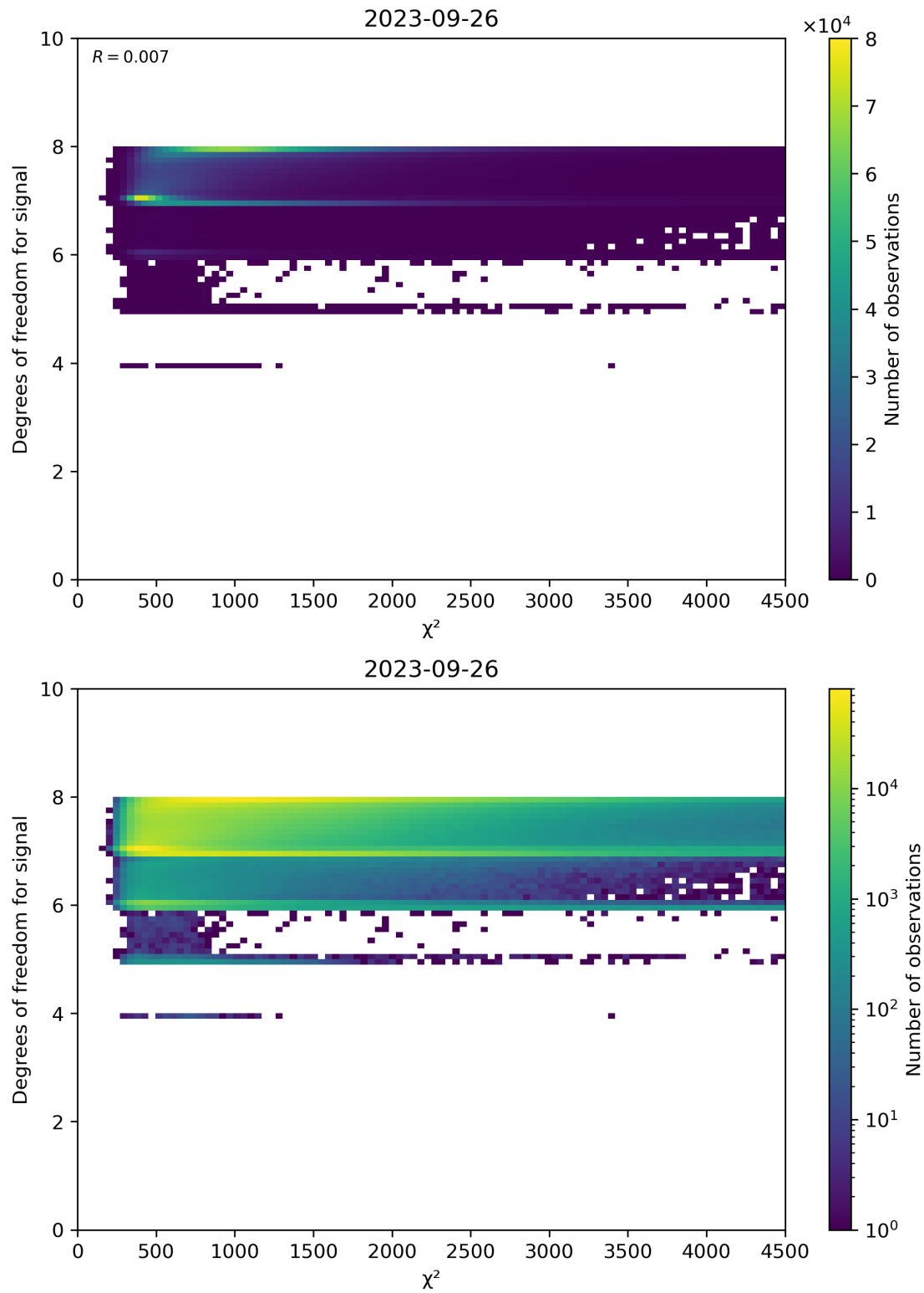
Figure 48: Scatter density plot of “ \chi^2 ” against “Degrees of freedom for signal” for 2023-09-26 to 2023-09-27.
