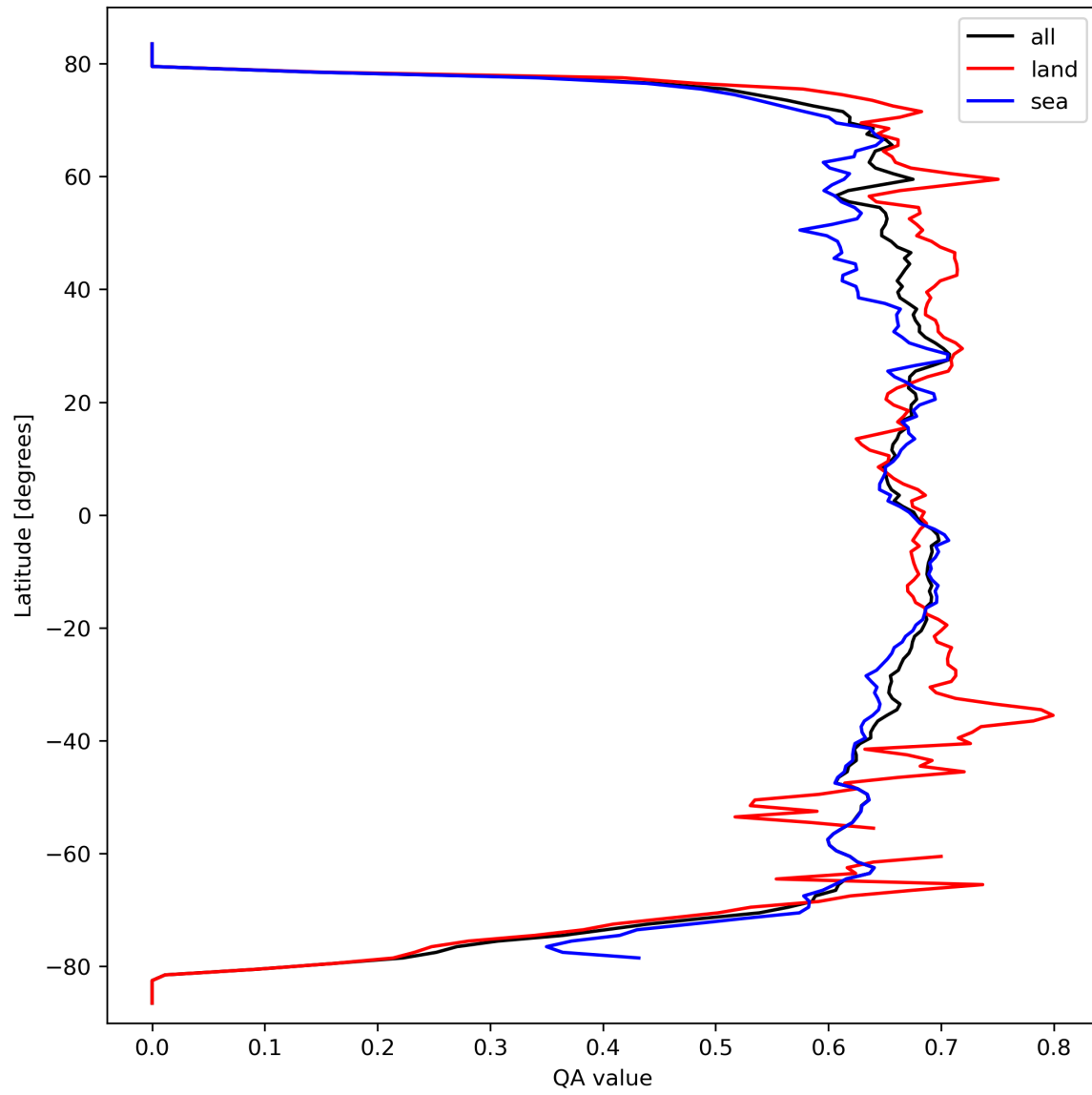
Figure 9: Zonal average of “QA value” for 2023-09-26 to 2023-09-27.
