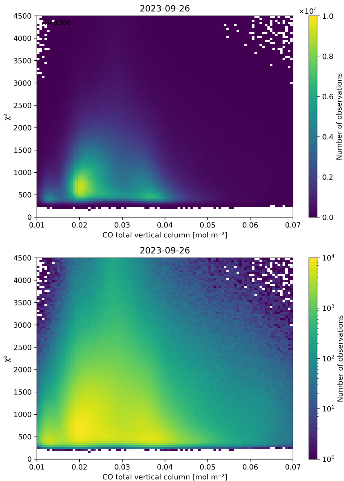
Figure 35: Scatter density plot of “CO total vertical column” against “ \chi^2 ” for 2023-09-26 to 2023-09-27.
