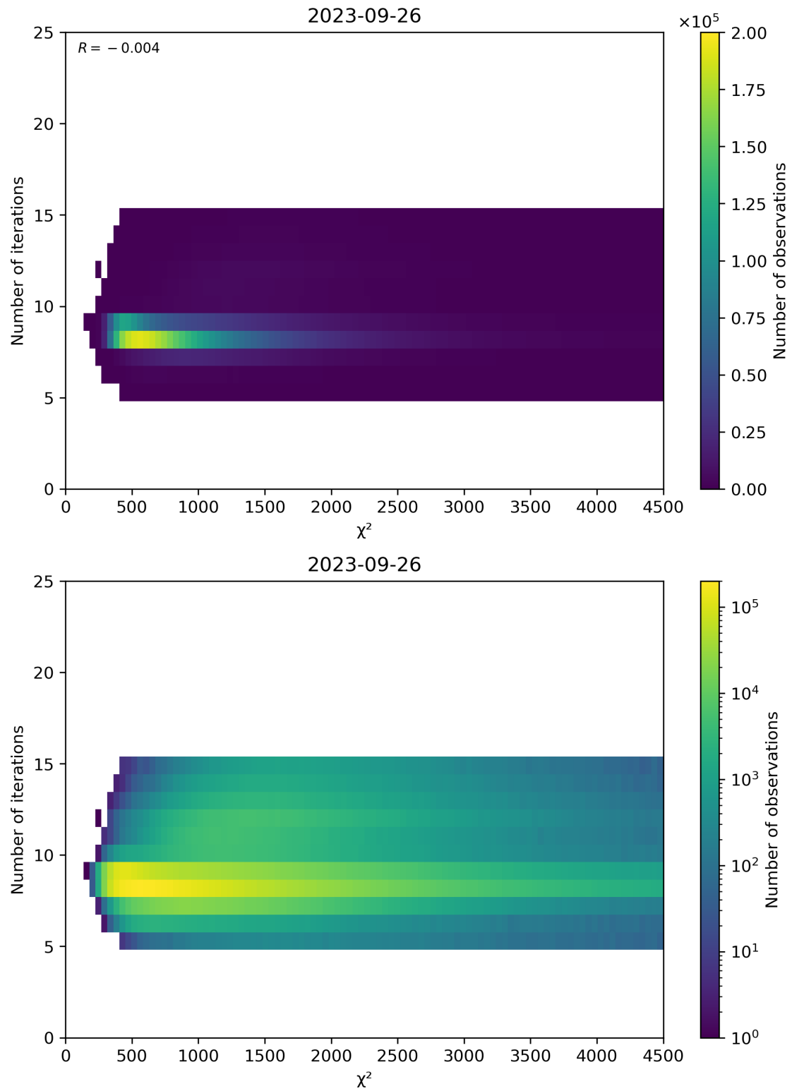
Figure 49: Scatter density plot of “ \chi^2 ” against “Number of iterations” for 2023-09-26 to 2023-09-27.
