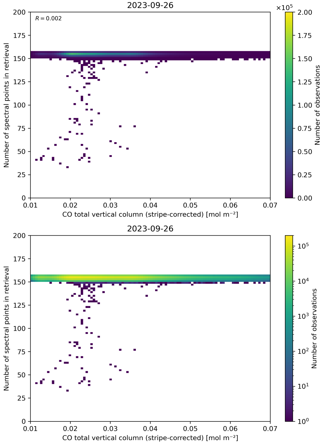
Figure 40: Scatter density plot of “CO total vertical column (stripe-corrected)” against “Number of spectral points in retrieval” for 2023-09-26 to 2023-09-27.
