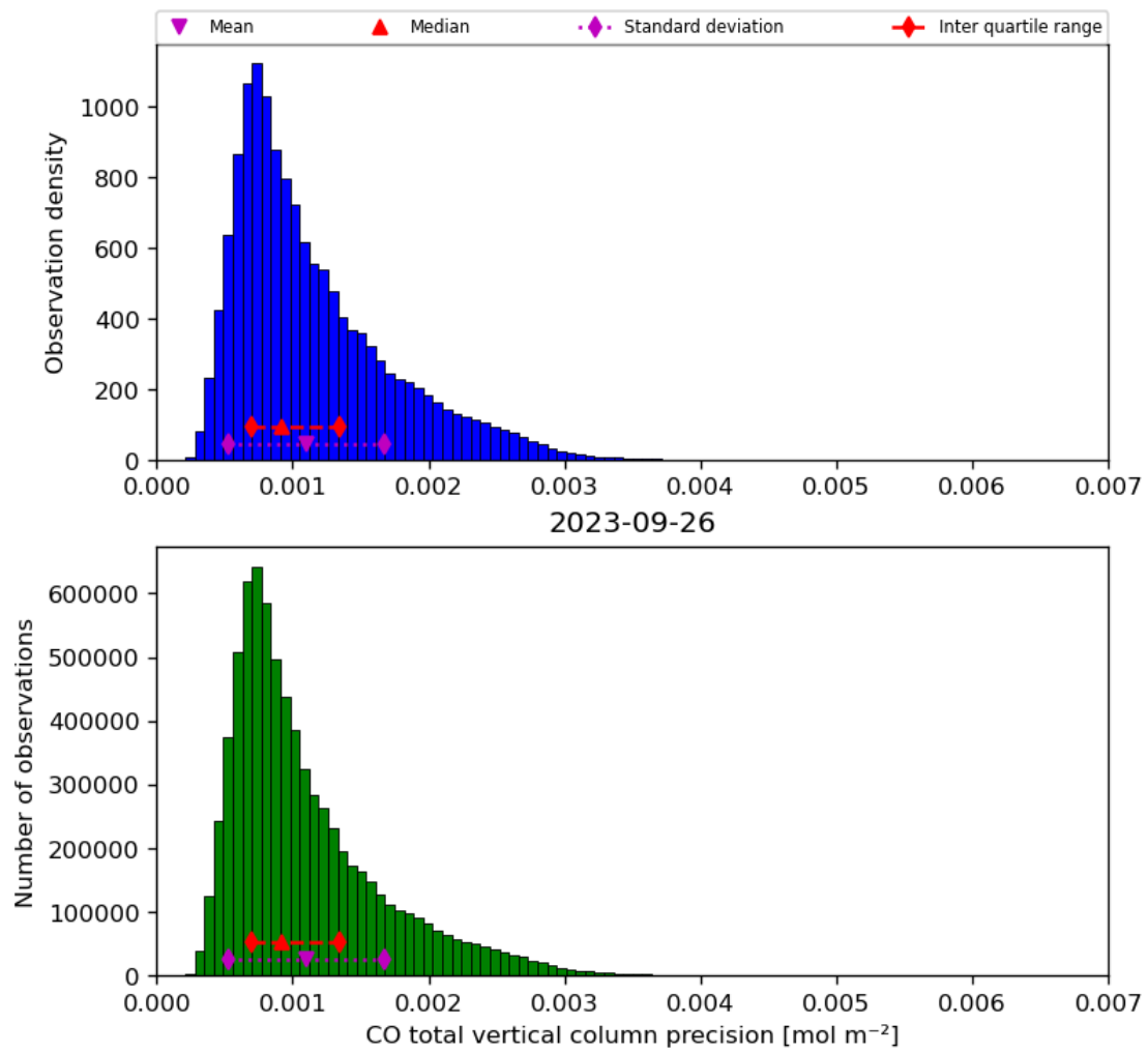
Figure 20: Histogram of “CO total vertical column precision” for 2023-09-26 to 2023-09-27
