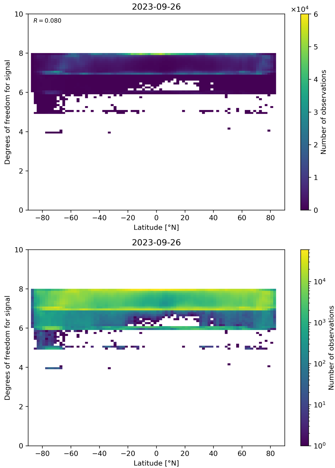
Figure 55: Scatter density plot of “Latitude” against “Degrees of freedom for signal” for 2023-09-26 to 2023-09-27.
