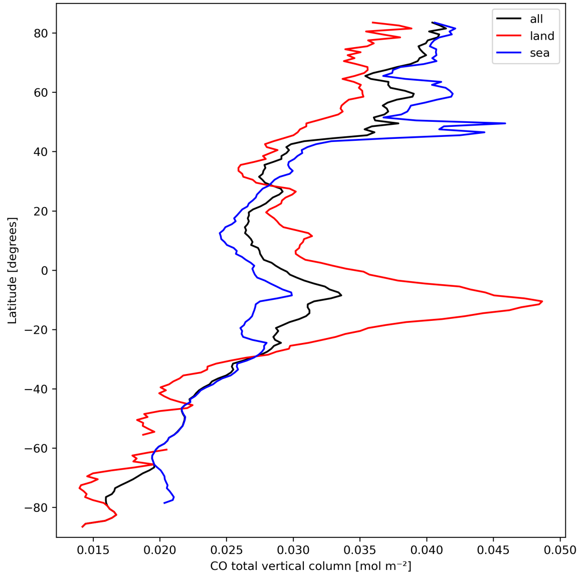
Figure 10: Zonal average of “CO total vertical column” for 2023-09-26 to 2023-09-27.
