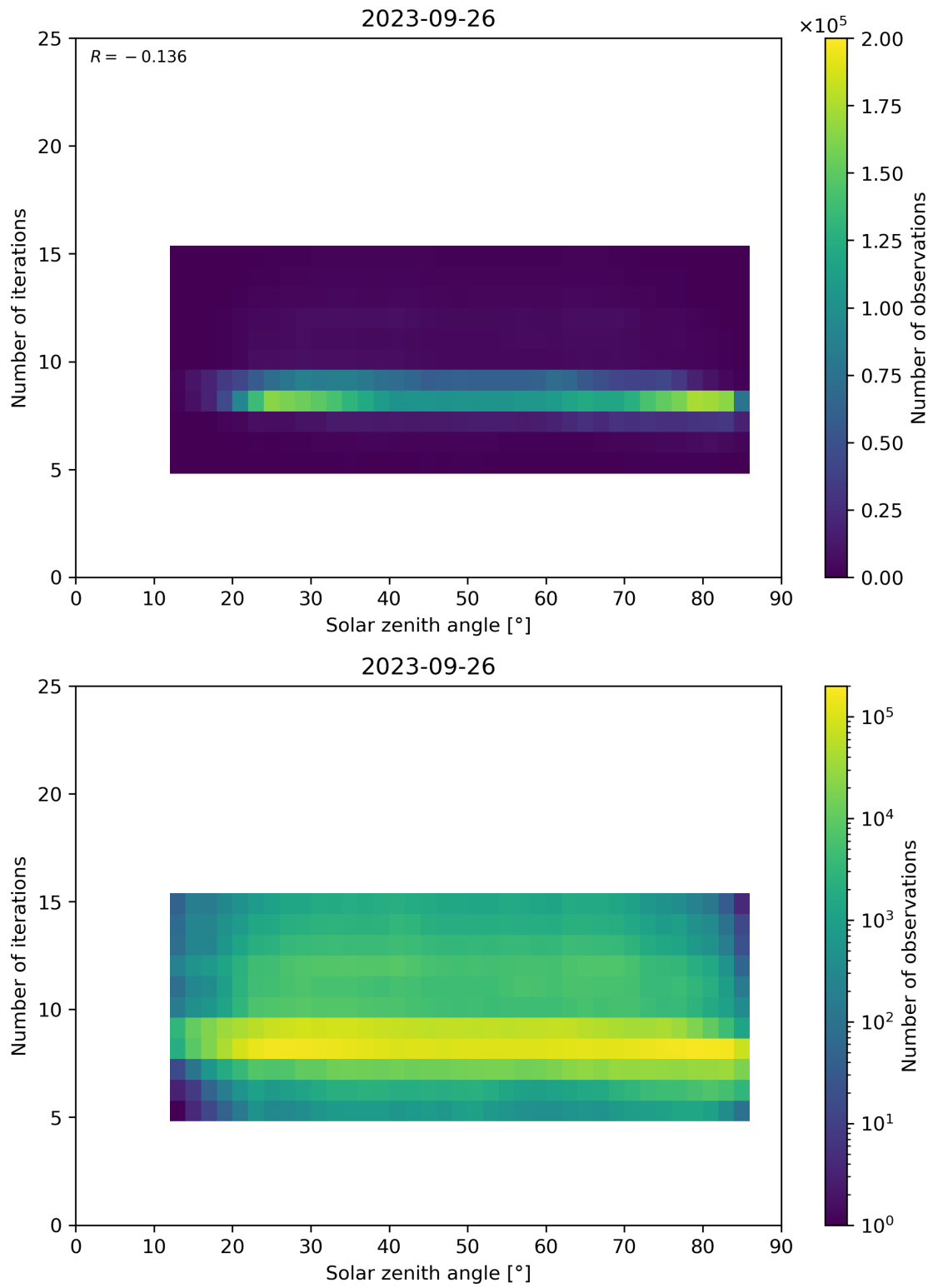
Figure 67: Scatter density plot of “Solar zenith angle” against “Number of iterations” for 2023-09-26 to 2023-09-27.
