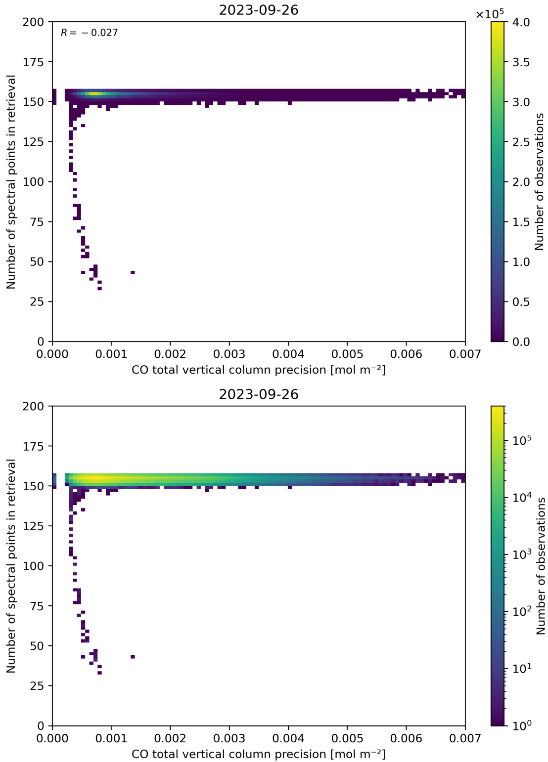
Figure 47: Scatter density plot of “CO total vertical column precision” against “Number of spectral points in retrieval” for 2023-09-26 to 2023-09-27.
