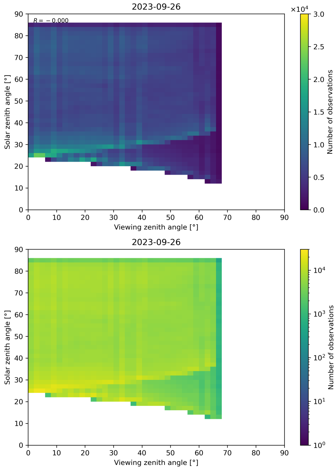
Figure 77: Scatter density plot of “Viewing zenith angle” against “Solar zenith angle” for 2023-09-26 to 2023-09-27.
