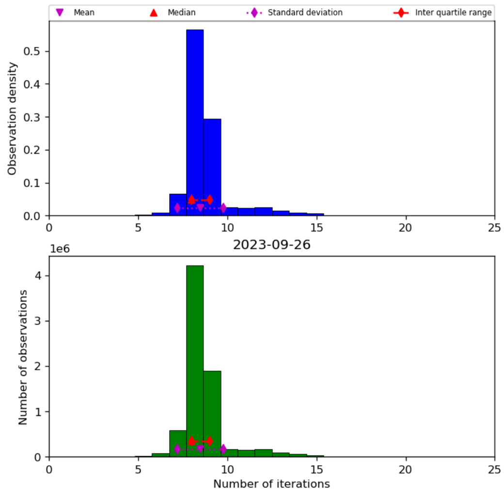
Figure 24: Histogram of “Number of iterations” for 2023-09-26 to 2023-09-27
