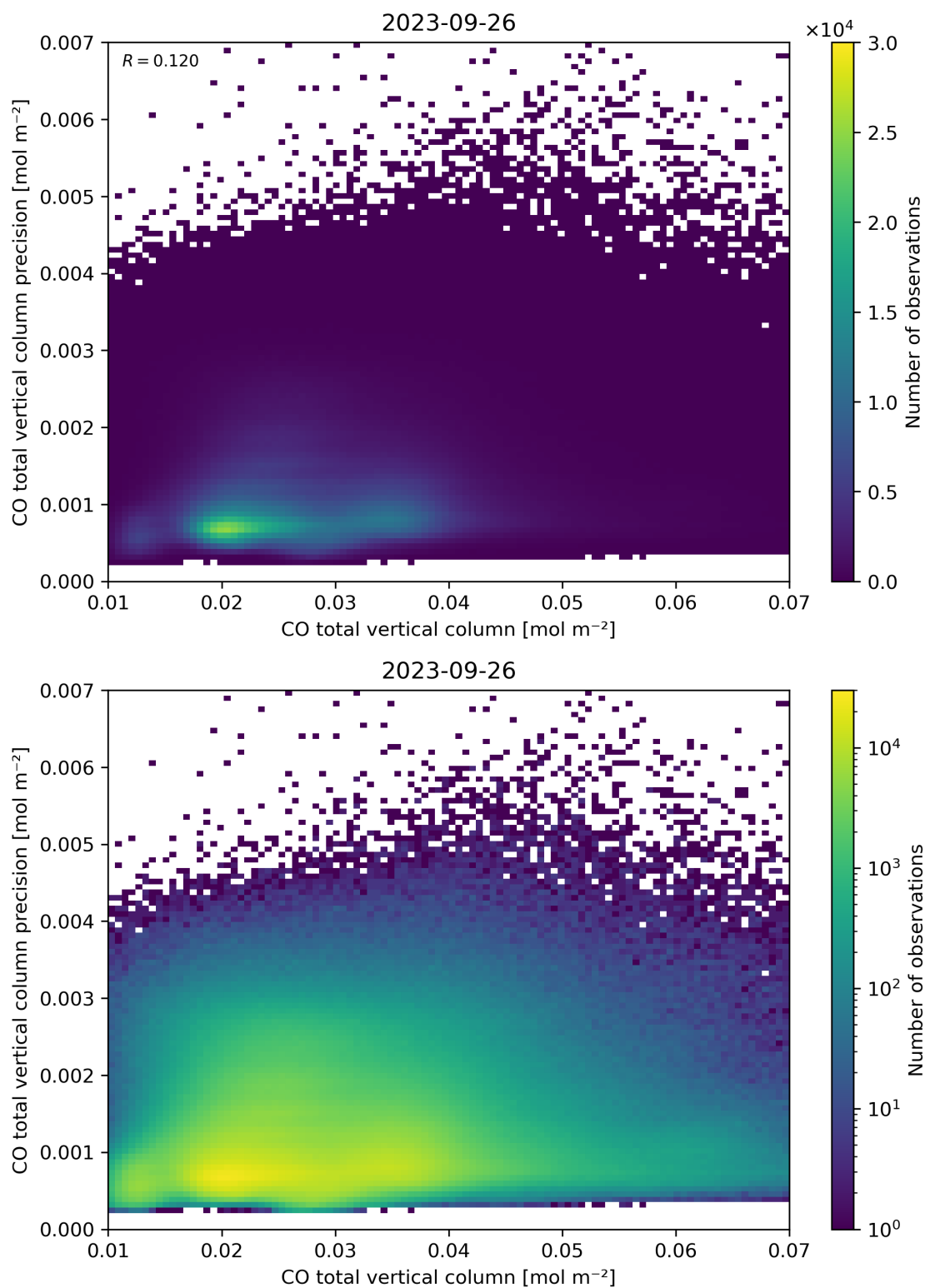
Figure 34: Scatter density plot of “CO total vertical column” against “CO total vertical column precision” for 2023-09-26 to 2023-09-27.
