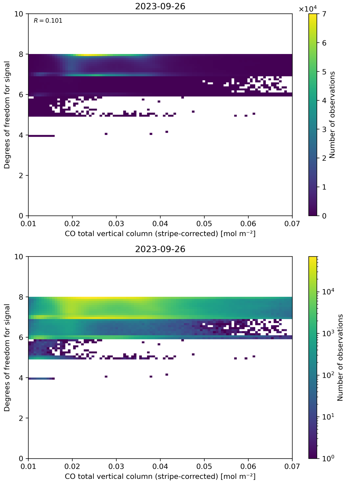
Figure 38: Scatter density plot of “CO total vertical column (stripe-corrected)” against “Degrees of freedom for signal” for 2023-09-26 to 2023-09-27.
