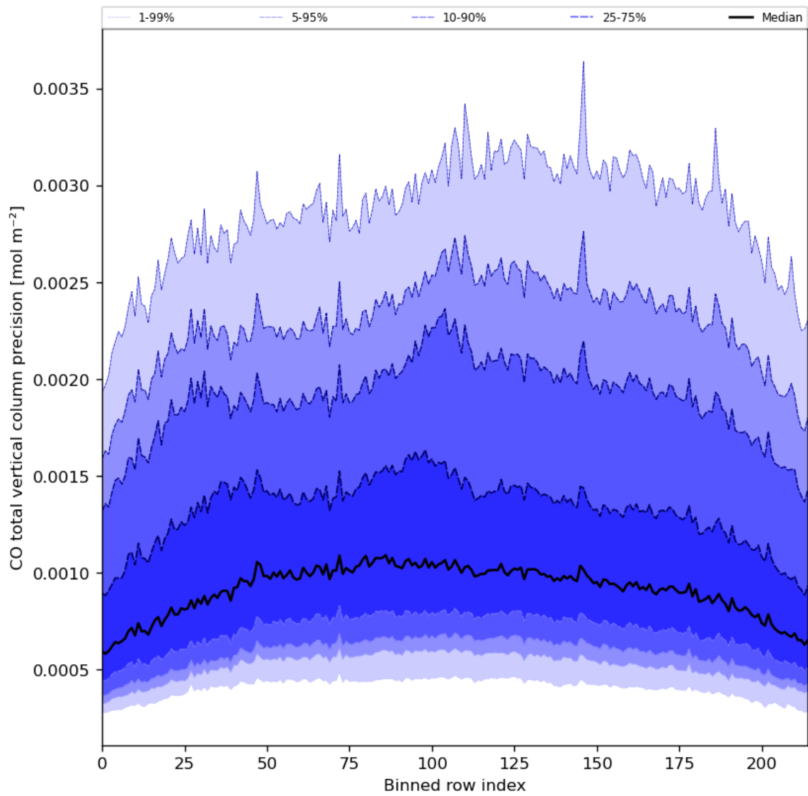
Figure 28: Along track statistics of “CO total vertical column precision” for 2023-09-26 to 2023-09-27
