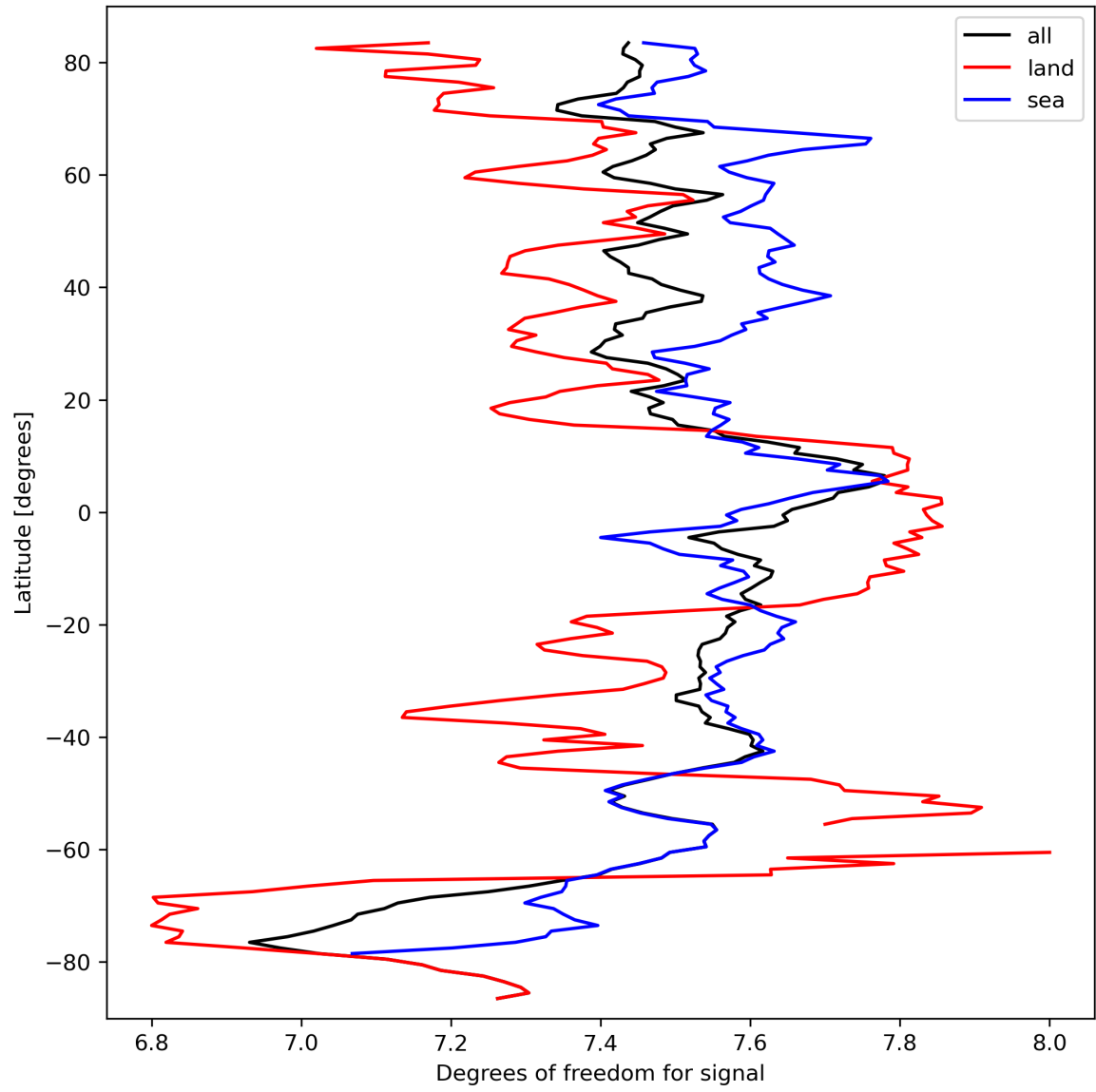
Figure 15: Zonal average of “Degrees of freedom for signal” for 2023-09-26 to 2023-09-27.
