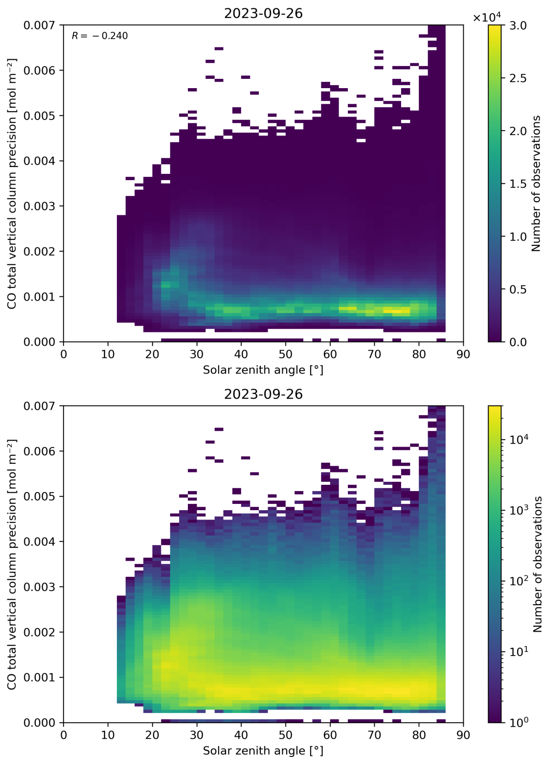
Figure 63: Scatter density plot of “Solar zenith angle” against “CO total vertical column precision” for 2023-09-26 to 2023-09-27.
