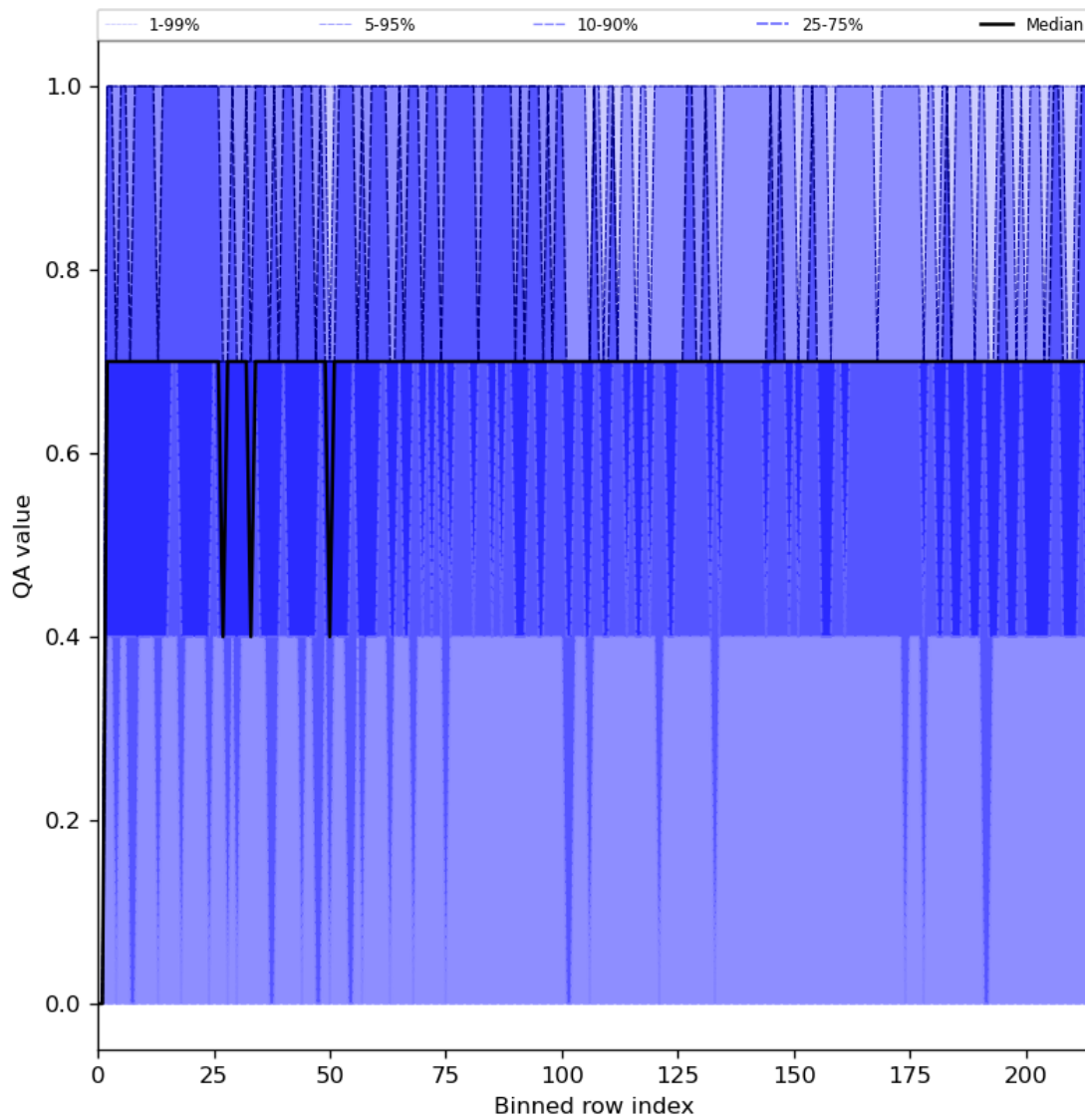
Figure 25: Along track statistics of “QA value” for 2023-09-26 to 2023-09-27
