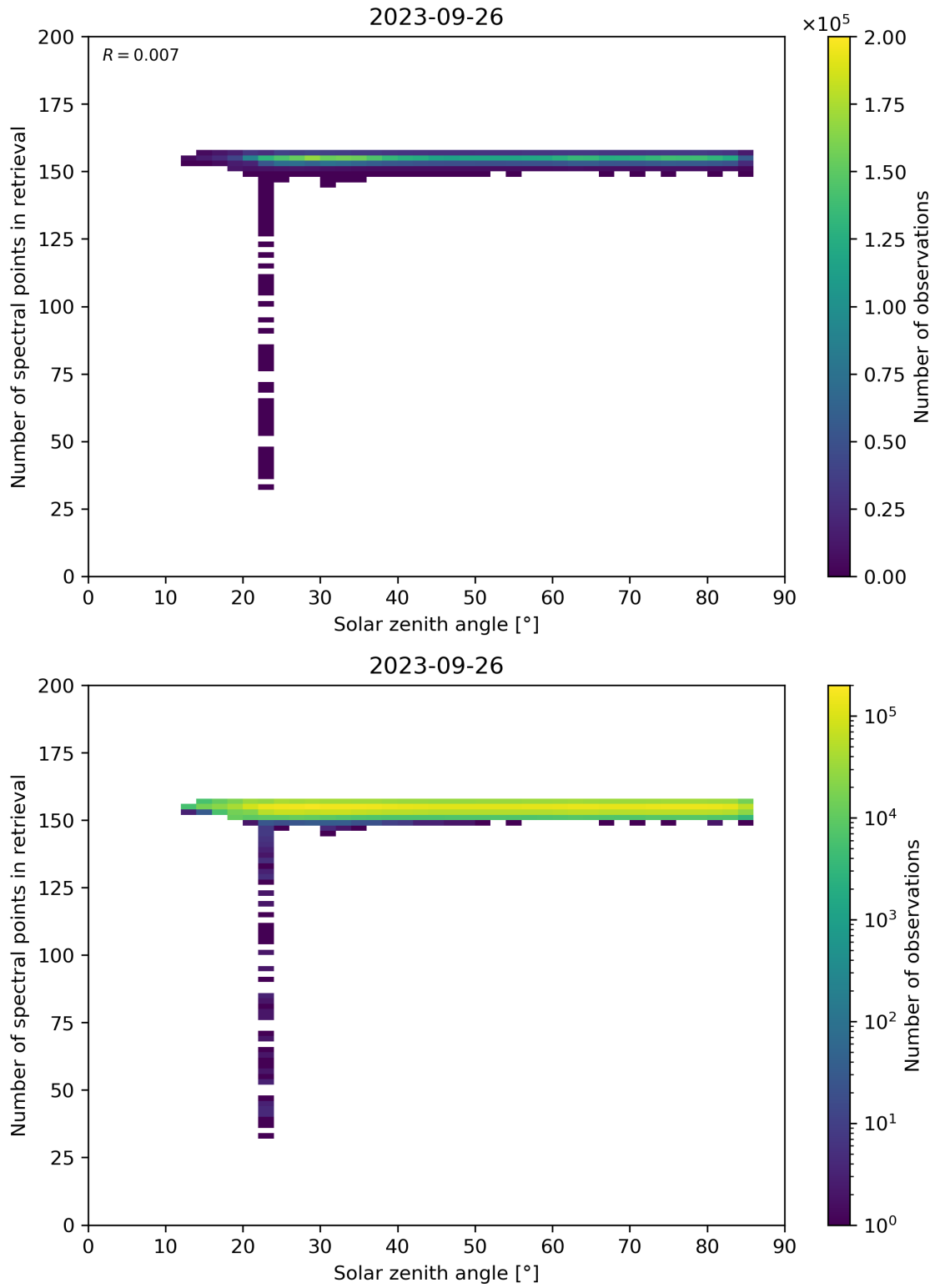
Figure 68: Scatter density plot of “Solar zenith angle” against “Number of spectral points in retrieval” for 2023-09-26 to 2023-09-27.
