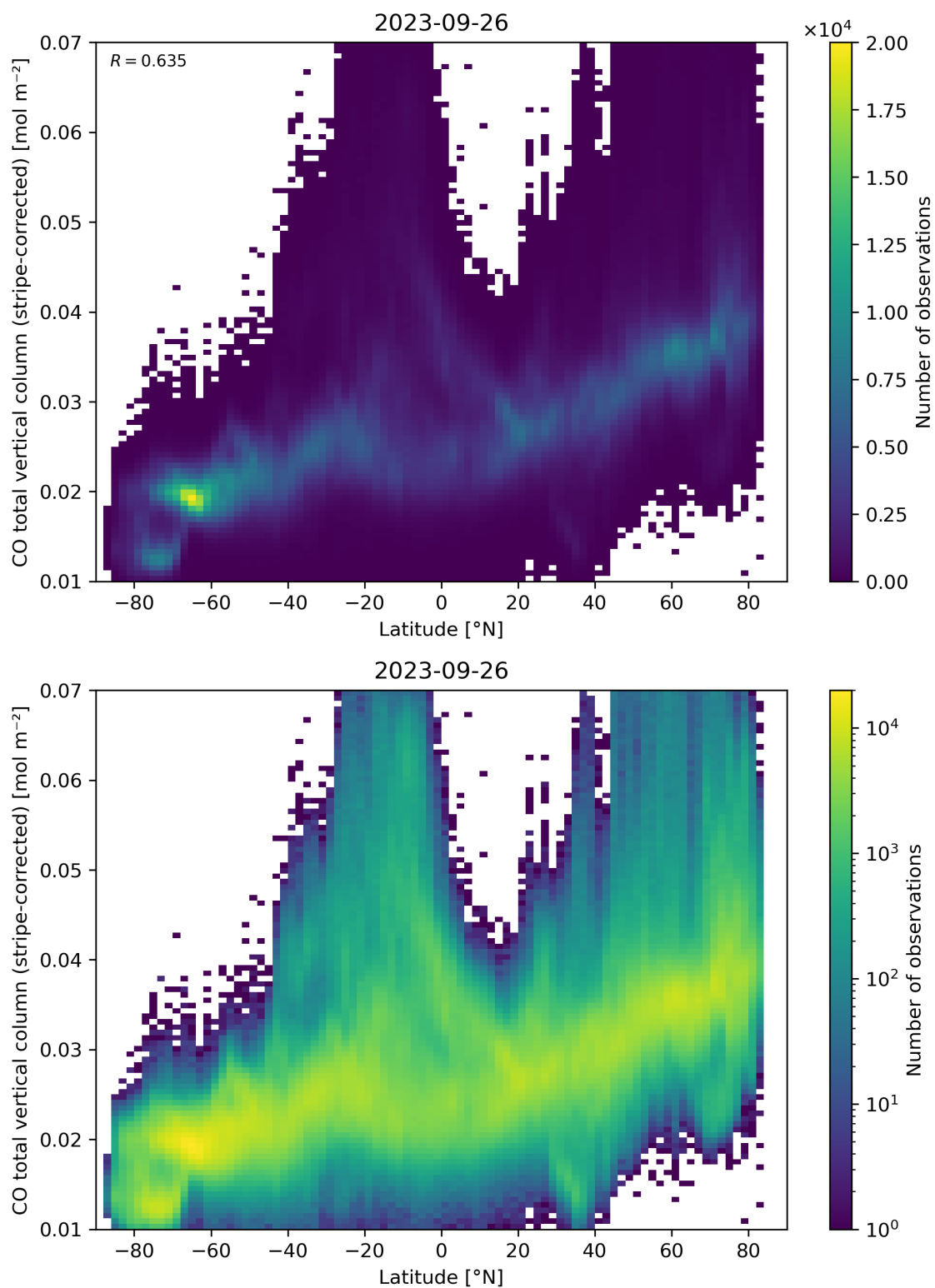
Figure 52: Scatter density plot of “Latitude” against “CO total vertical column (stripe-corrected)” for 2023-09-26 to 2023-09-27.
