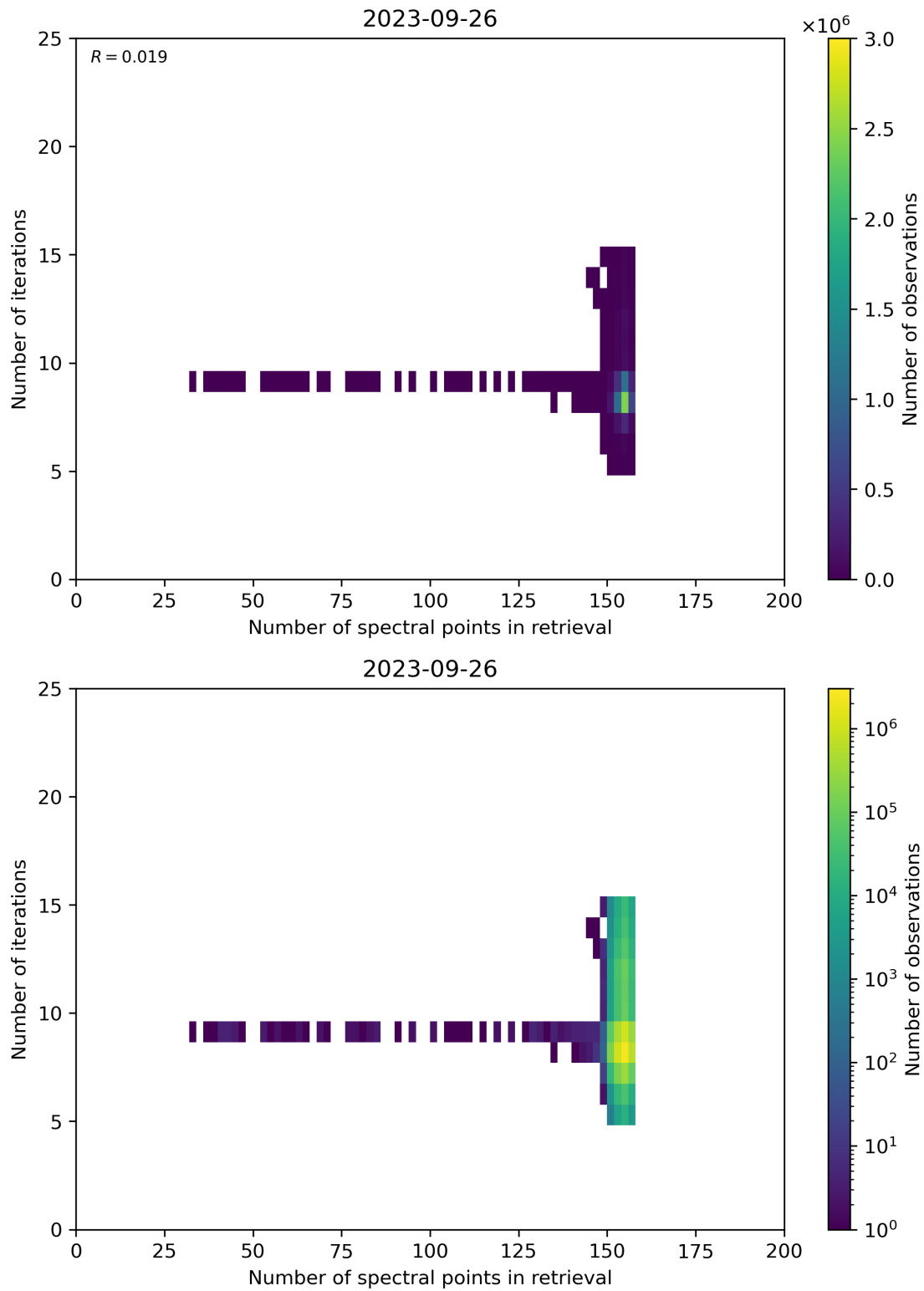
Figure 60: Scatter density plot of “Number of spectral points in retrieval” against “Number of iterations” for 2023-09-26 to 2023-09-27.
