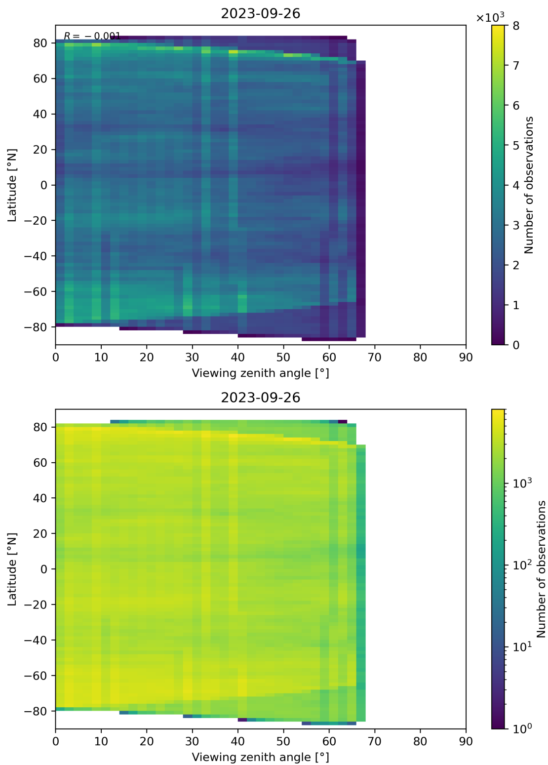
Figure 74: Scatter density plot of “Viewing zenith angle” against “Latitude” for 2023-09-26 to 2023-09-27.
