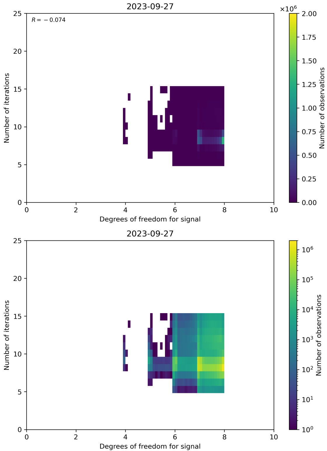
Figure 50: Scatter density plot of “Degrees of freedom for signal” against “Number of iterations” for 2023-09-26 to 2023-09-28.
