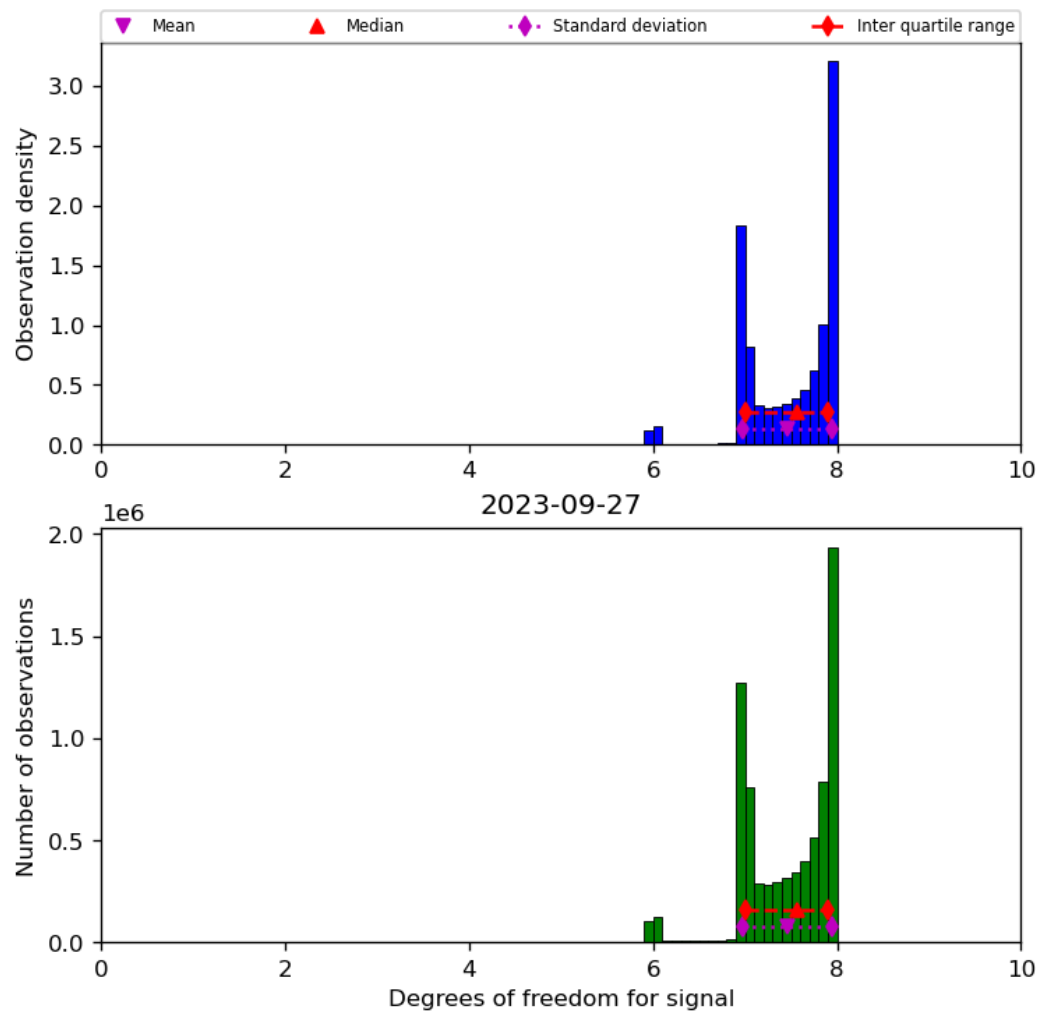
Figure 23: Histogram of “Degrees of freedom for signal” for 2023-09-26 to 2023-09-28
