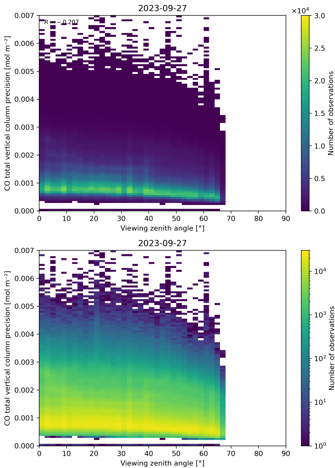
Figure 71: Scatter density plot of “Viewing zenith angle” against “CO total vertical column precision” for 2023-09-26 to 2023-09-28.
