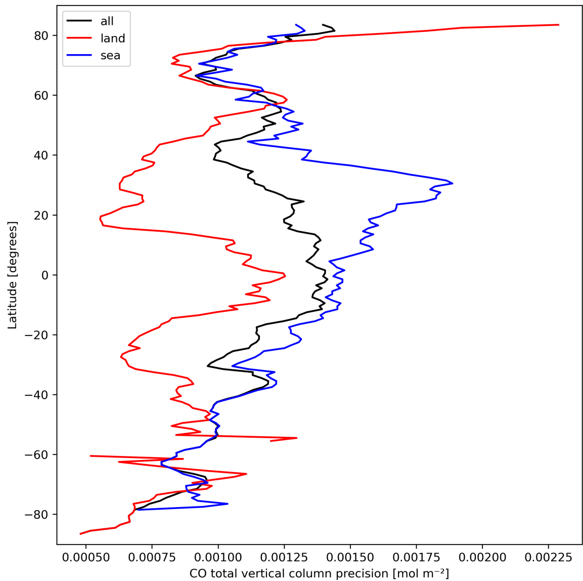
Figure 12: Zonal average of “CO total vertical column precision” for 2023-09-26 to 2023-09-28.
