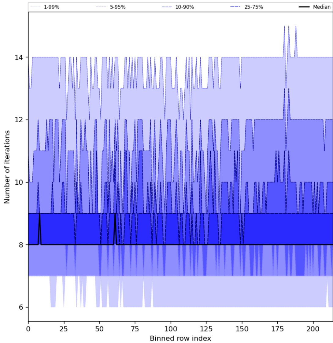
Figure 32: Along track statistics of “Number of iterations” for 2023-09-26 to 2023-09-28
