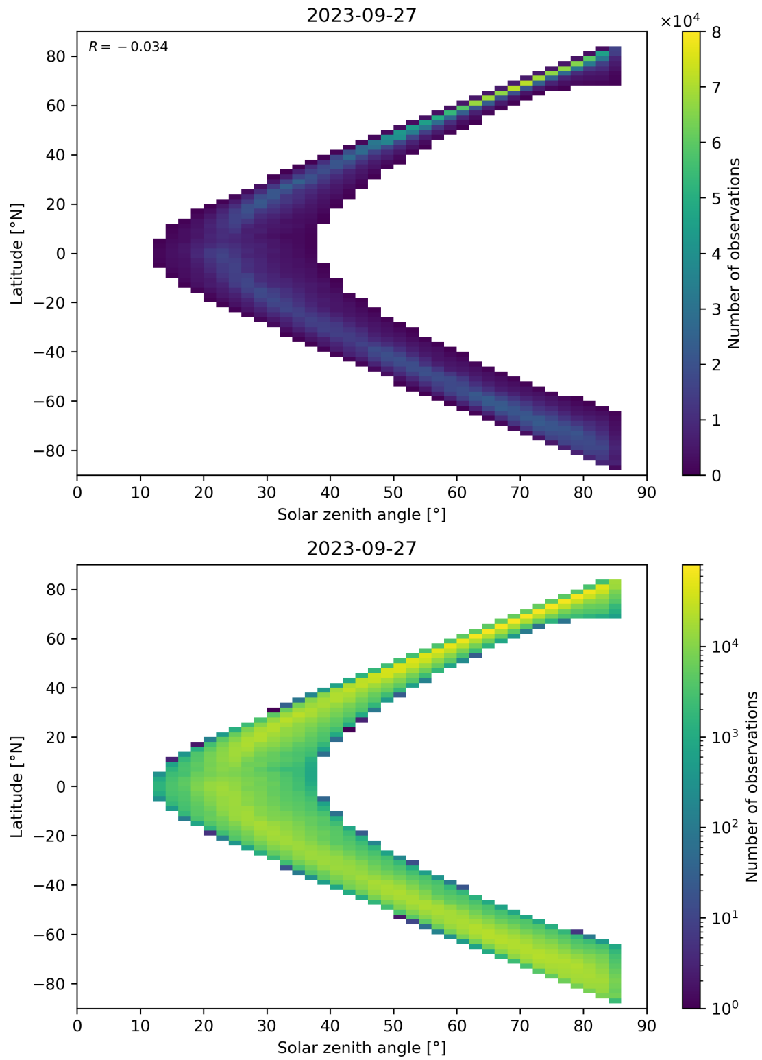
Figure 66: Scatter density plot of “Solar zenith angle” against “Latitude” for 2023-09-26 to 2023-09-28.
