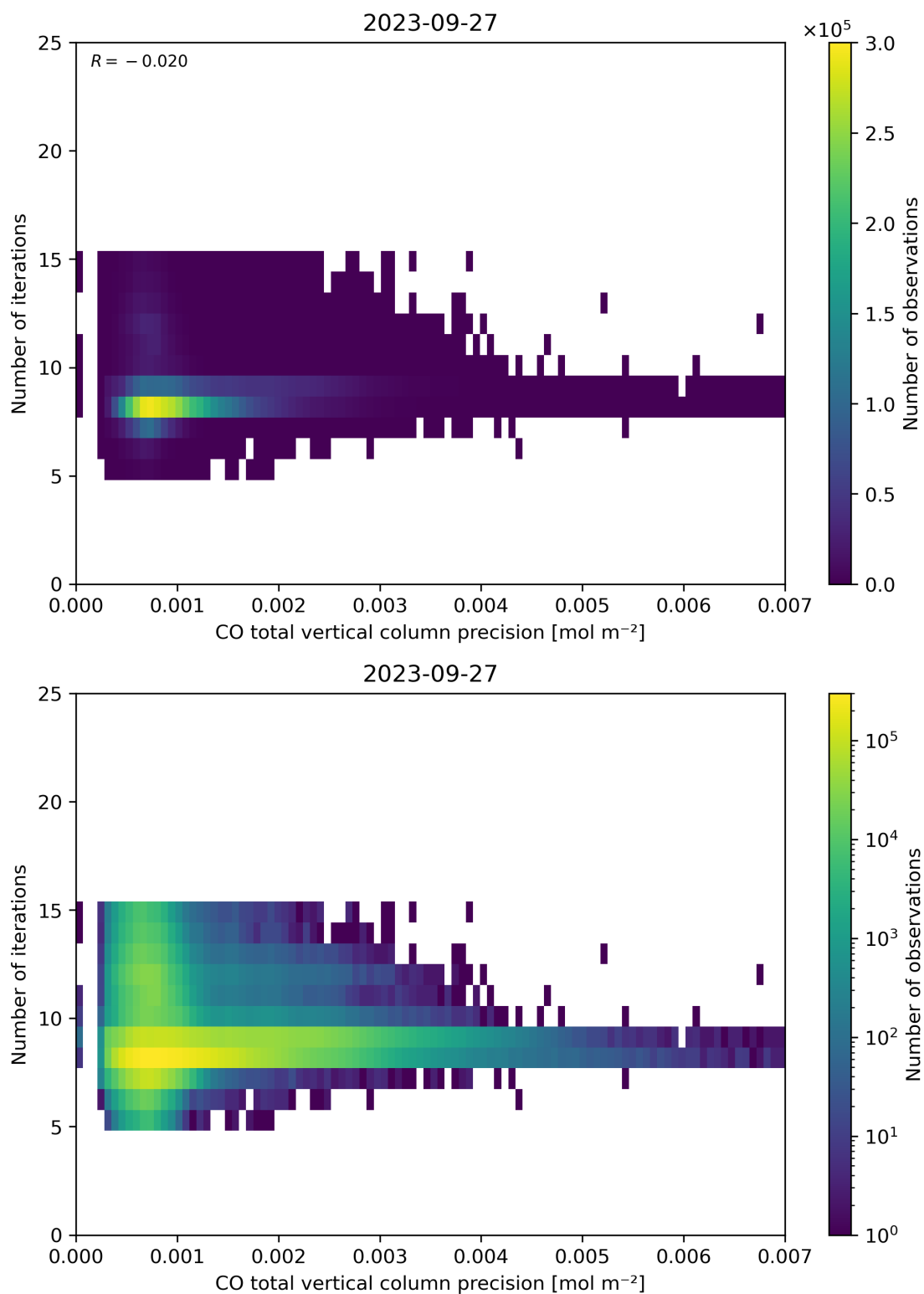
Figure 46: Scatter density plot of “CO total vertical column precision” against “Number of iterations” for 2023-09-26 to 2023-09-28.
