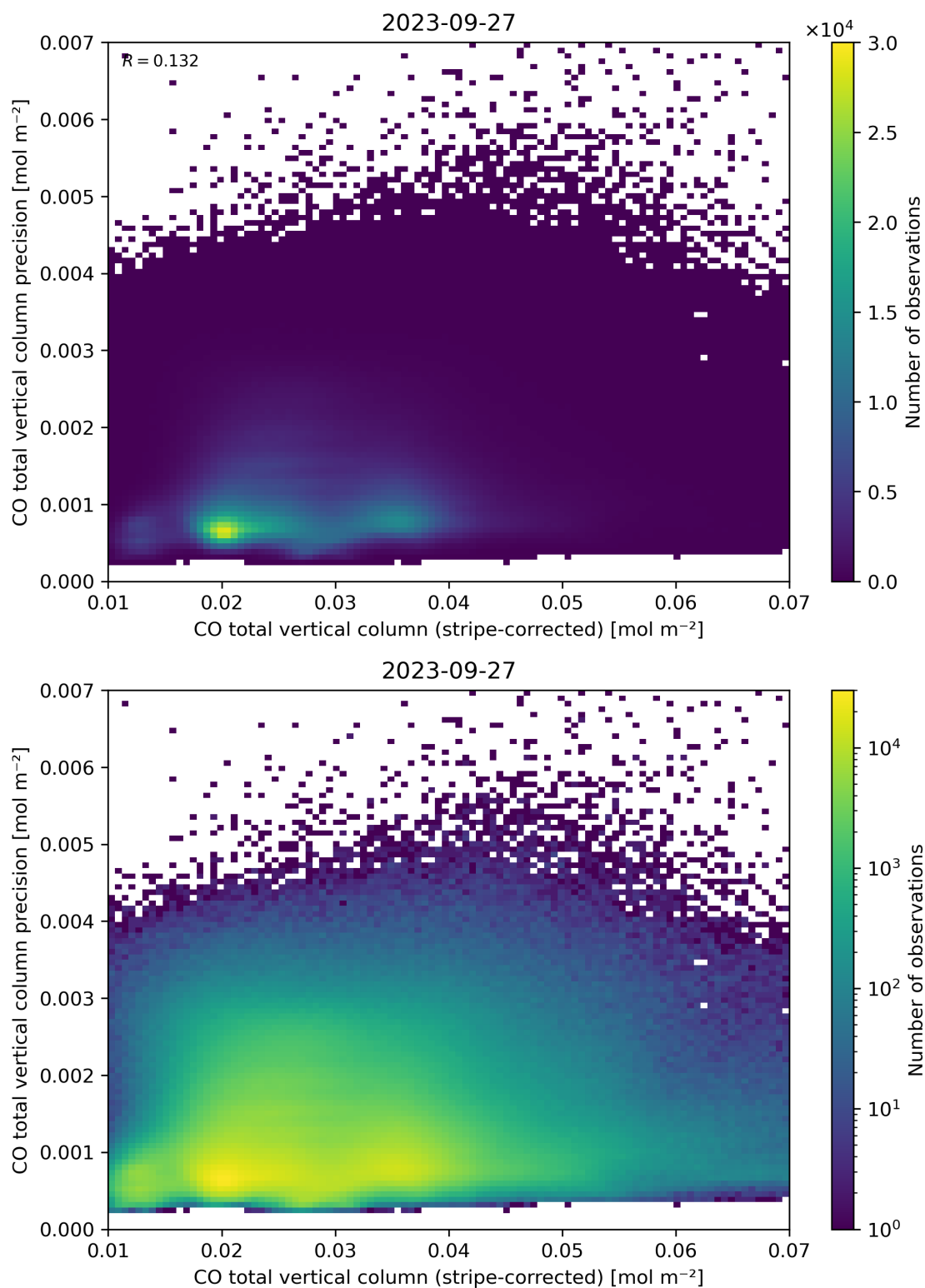
Figure 36: Scatter density plot of “CO total vertical column (stripe-corrected)” against “CO total vertical column precision” for 2023-09-26 to 2023-09-28.
