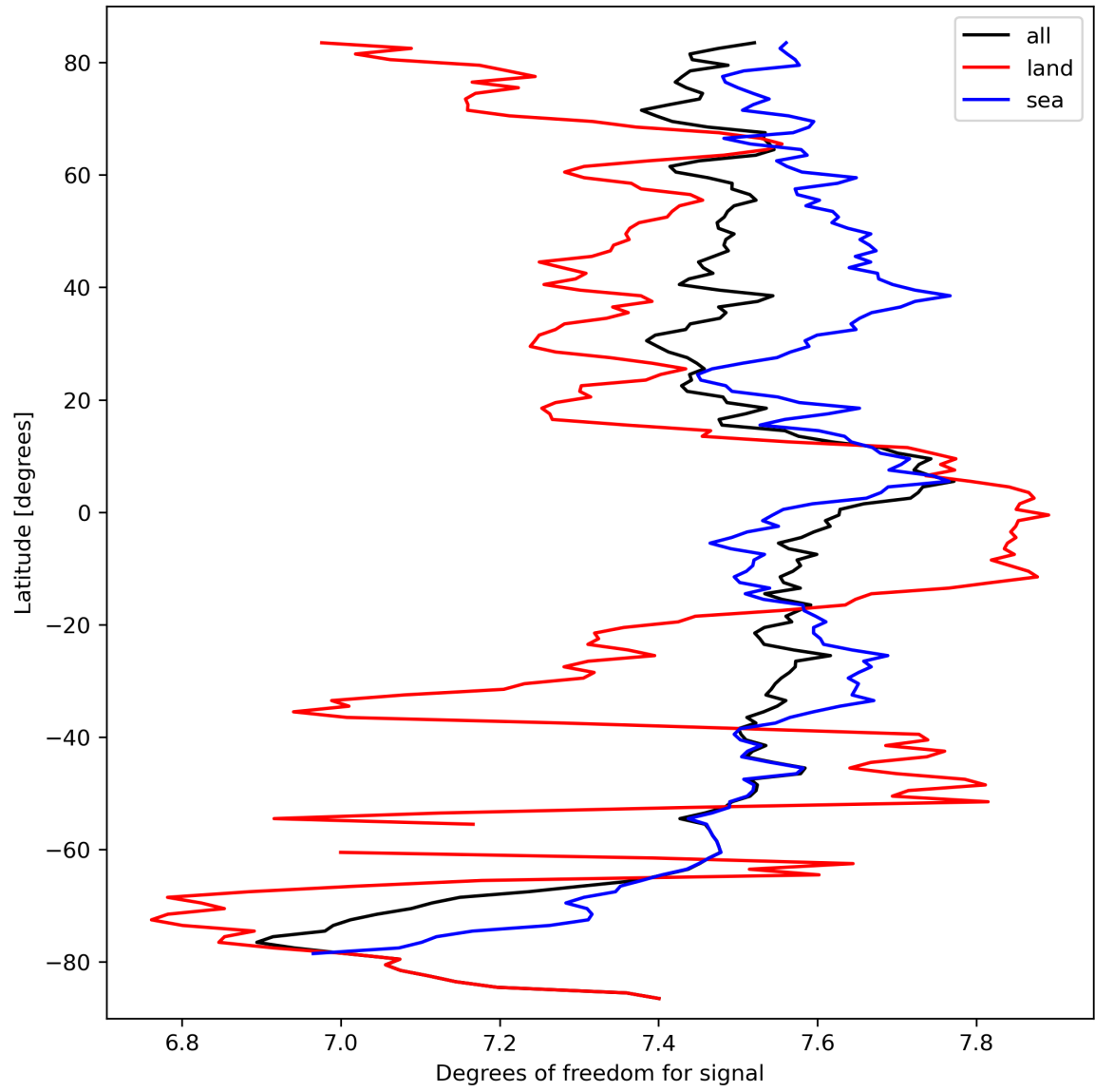
Figure 15: Zonal average of “Degrees of freedom for signal” for 2023-09-26 to 2023-09-28.
