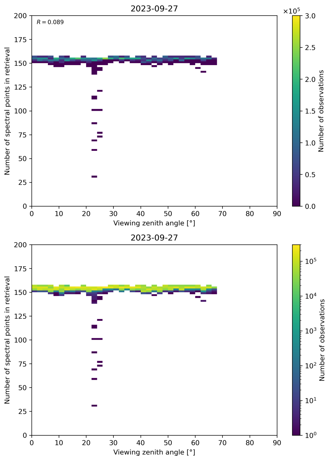
Figure 76: Scatter density plot of “Viewing zenith angle” against “Number of spectral points in retrieval” for 2023-09-26 to 2023-09-28.
