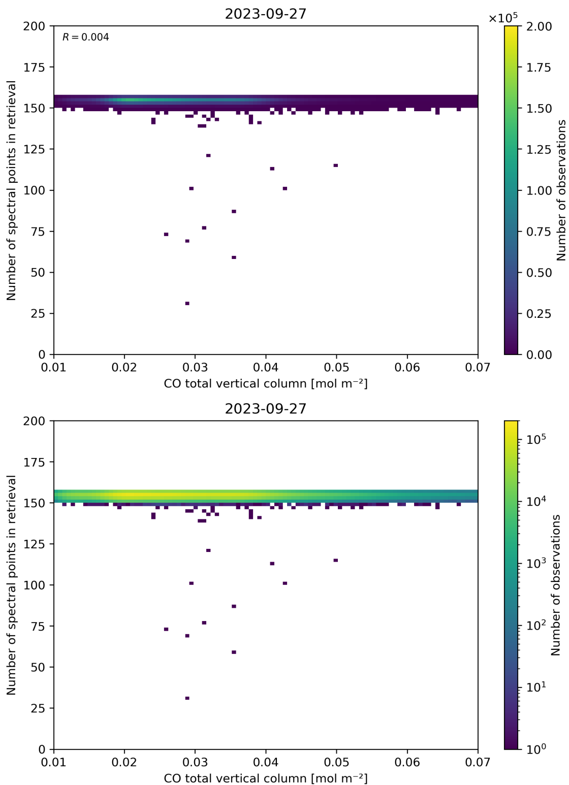
Figure 43: Scatter density plot of “CO total vertical column” against “Number of spectral points in retrieval” for 2023-09-26 to 2023-09-28.
