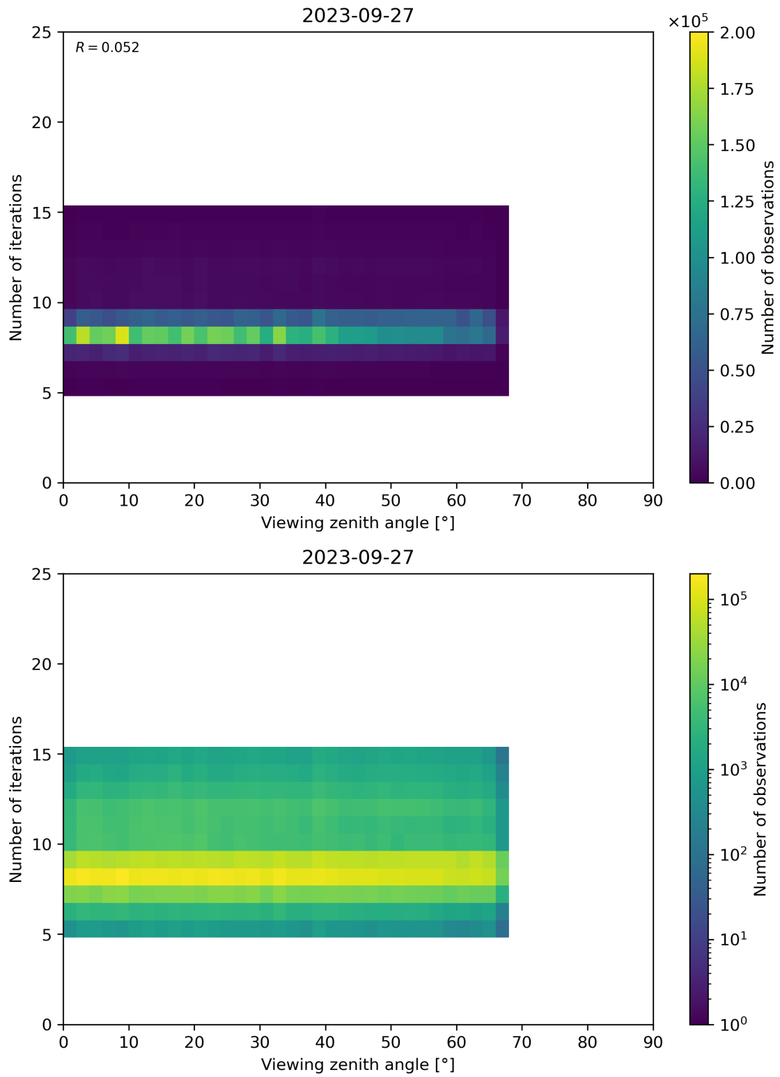
Figure 75: Scatter density plot of “Viewing zenith angle” against “Number of iterations” for 2023-09-26 to 2023-09-28.
