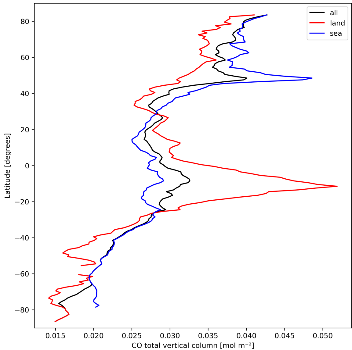
Figure 10: Zonal average of “CO total vertical column” for 2023-09-26 to 2023-09-28.
