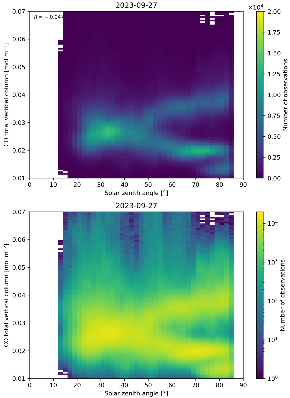
Figure 61: Scatter density plot of “Solar zenith angle” against “CO total vertical column” for 2023-09-26 to 2023-09-28.
