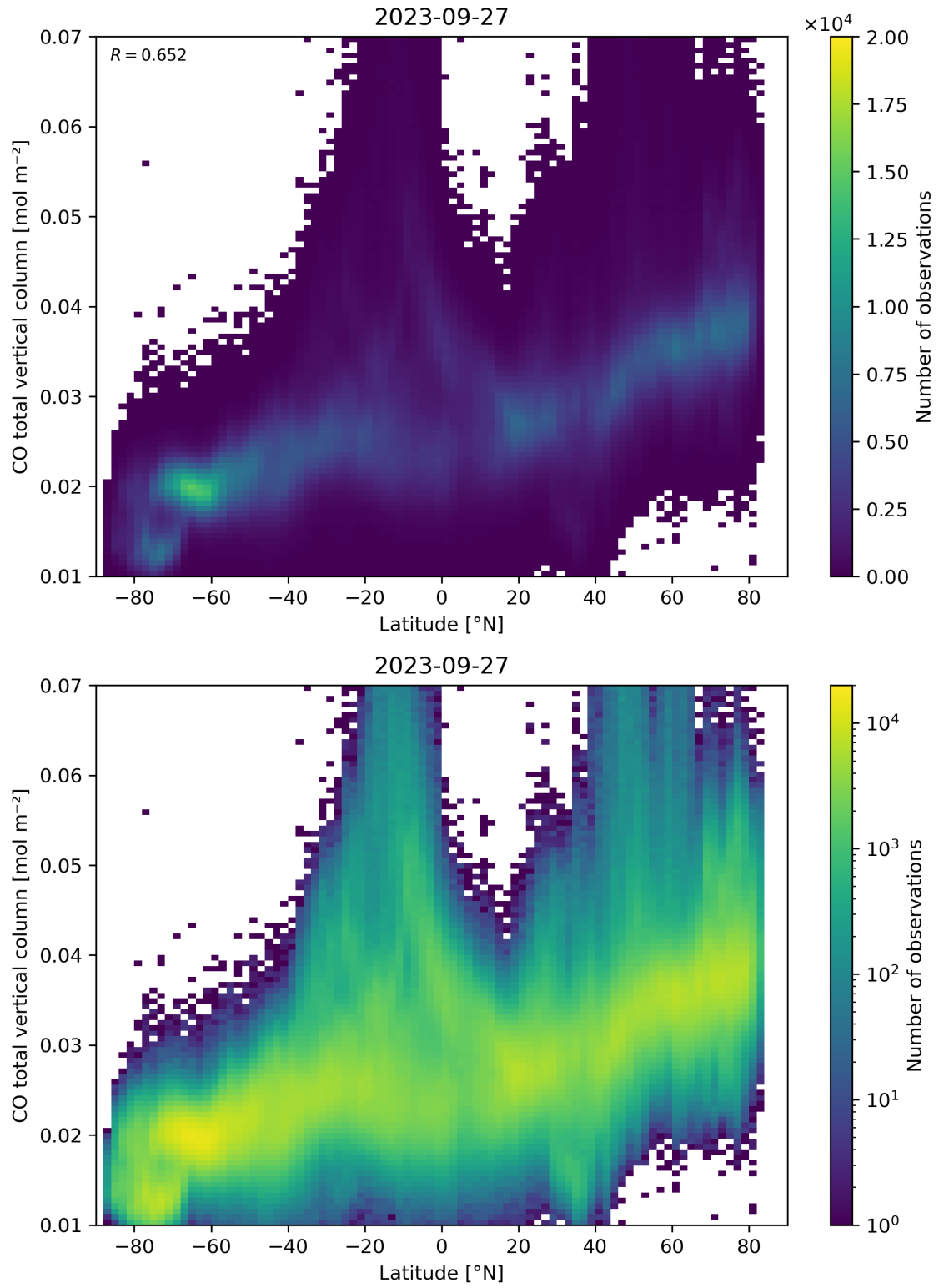
Figure 51: Scatter density plot of “Latitude” against “CO total vertical column” for 2023-09-26 to 2023-09-28.
