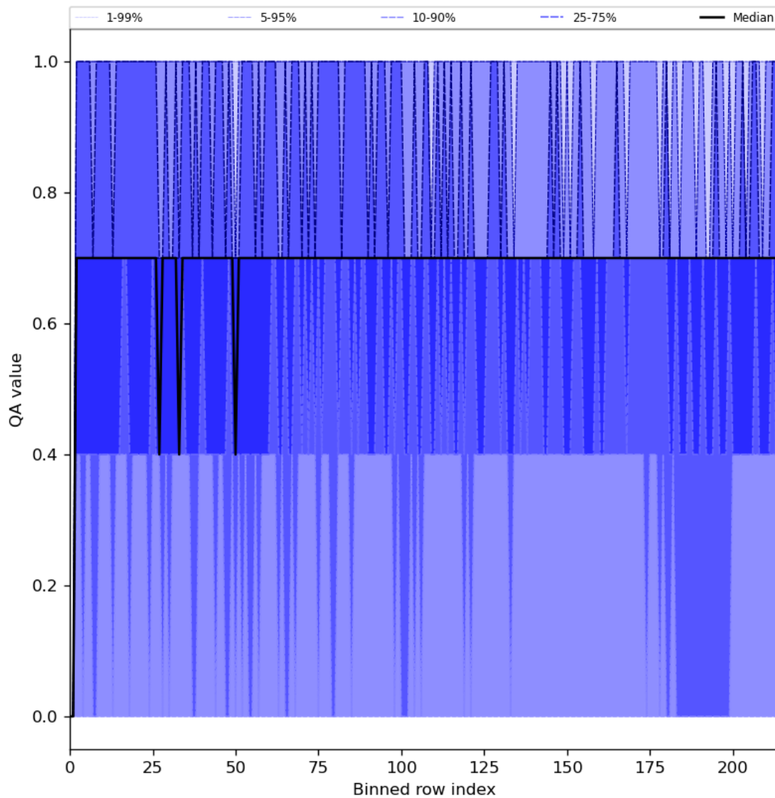
Figure 25: Along track statistics of “QA value” for 2023-09-26 to 2023-09-28
