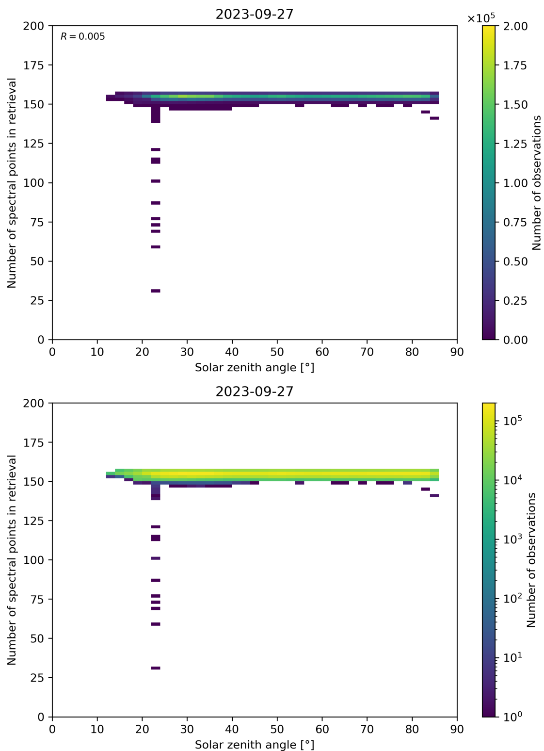
Figure 68: Scatter density plot of “Solar zenith angle” against “Number of spectral points in retrieval” for 2023-09-26 to 2023-09-28.
