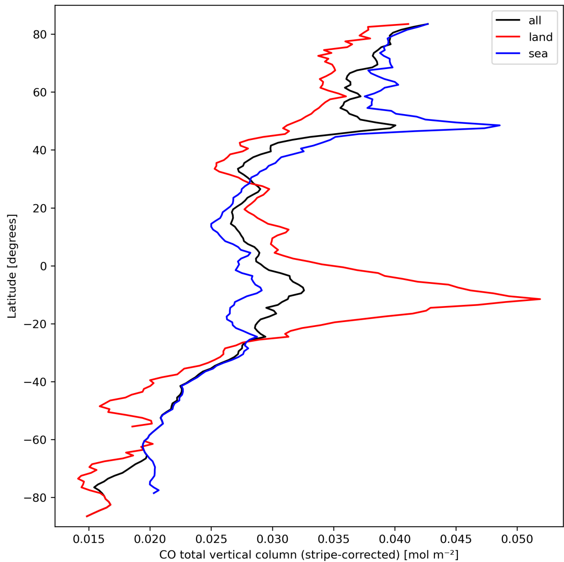
Figure 11: Zonal average of “CO total vertical column (stripe-corrected)” for 2023-09-26 to 2023-09-28.
