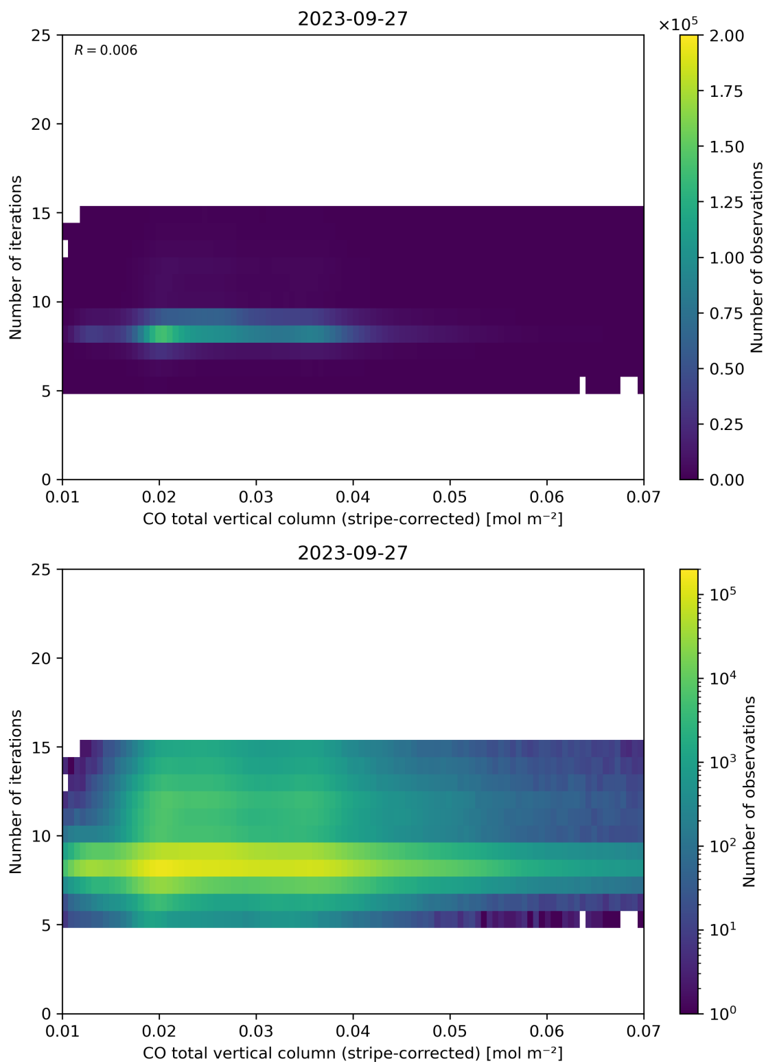
Figure 39: Scatter density plot of “CO total vertical column (stripe-corrected)” against “Number of iterations” for 2023-09-26 to 2023-09-28.
