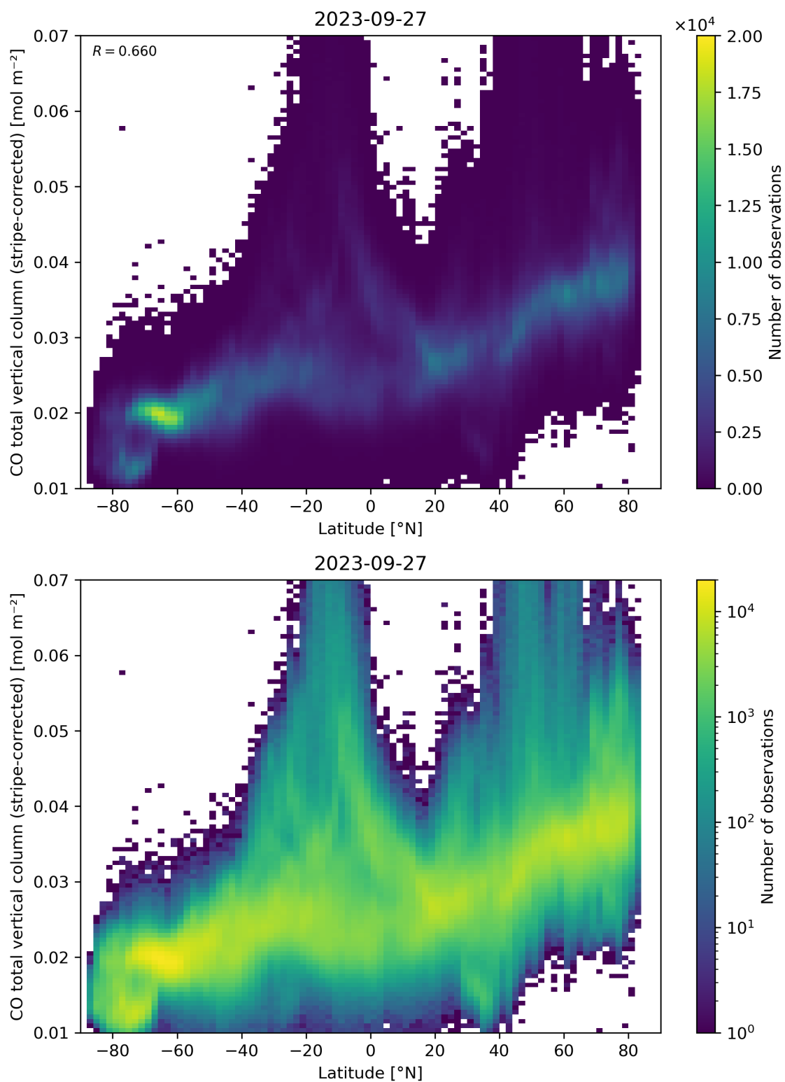
Figure 52: Scatter density plot of “Latitude” against “CO total vertical column (stripe-corrected)” for 2023-09-26 to 2023-09-28.
