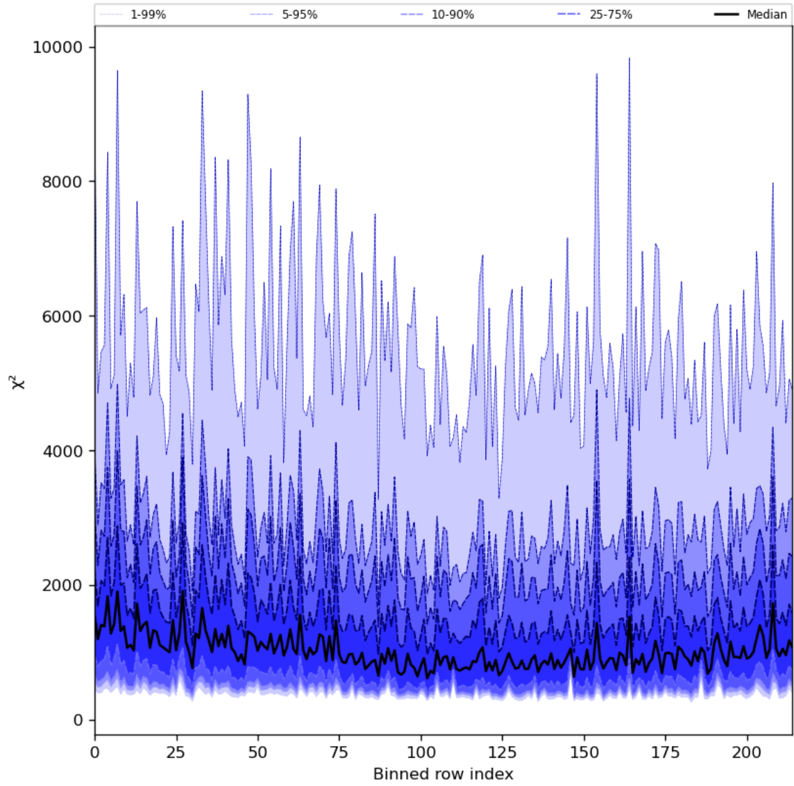
Figure 30: Along track statistics of “ \chi^2 ” for 2023-09-26 to 2023-09-28
