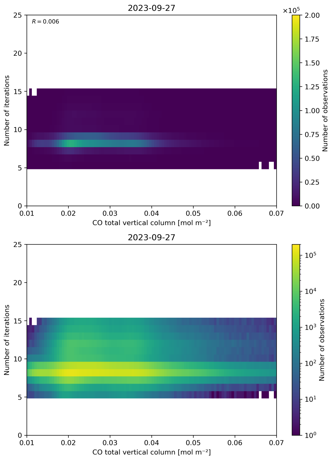
Figure 42: Scatter density plot of “CO total vertical column” against “Number of iterations” for 2023-09-26 to 2023-09-28.
