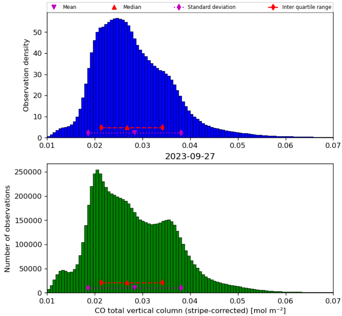
Figure 19: Histogram of “CO total vertical column (stripe-corrected)” for 2023-09-26 to 2023-09-28
