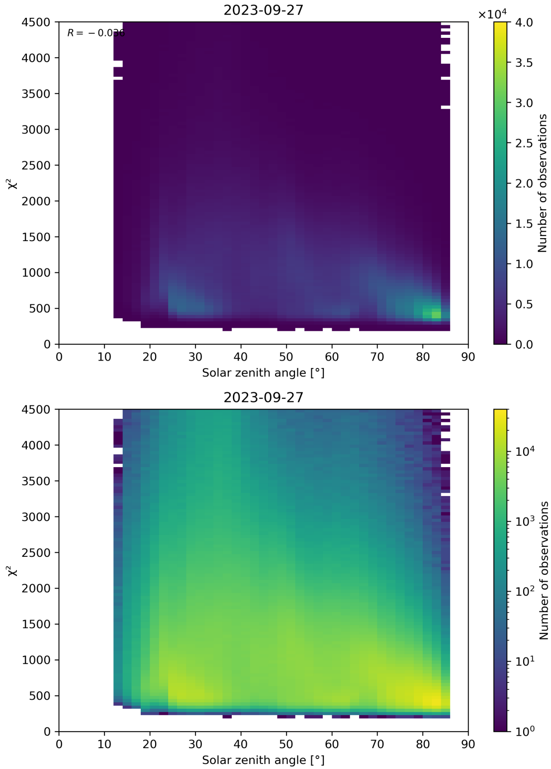
Figure 64: Scatter density plot of “Solar zenith angle” against “ \chi^2 ” for 2023-09-26 to 2023-09-28.
