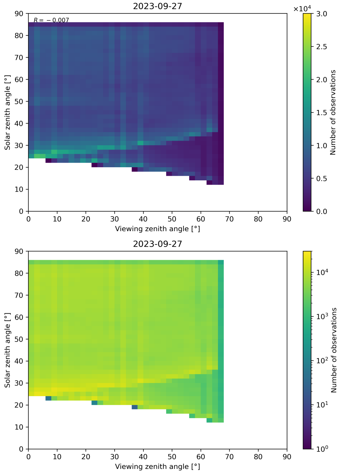
Figure 77: Scatter density plot of “Viewing zenith angle” against “Solar zenith angle” for 2023-09-26 to 2023-09-28.
