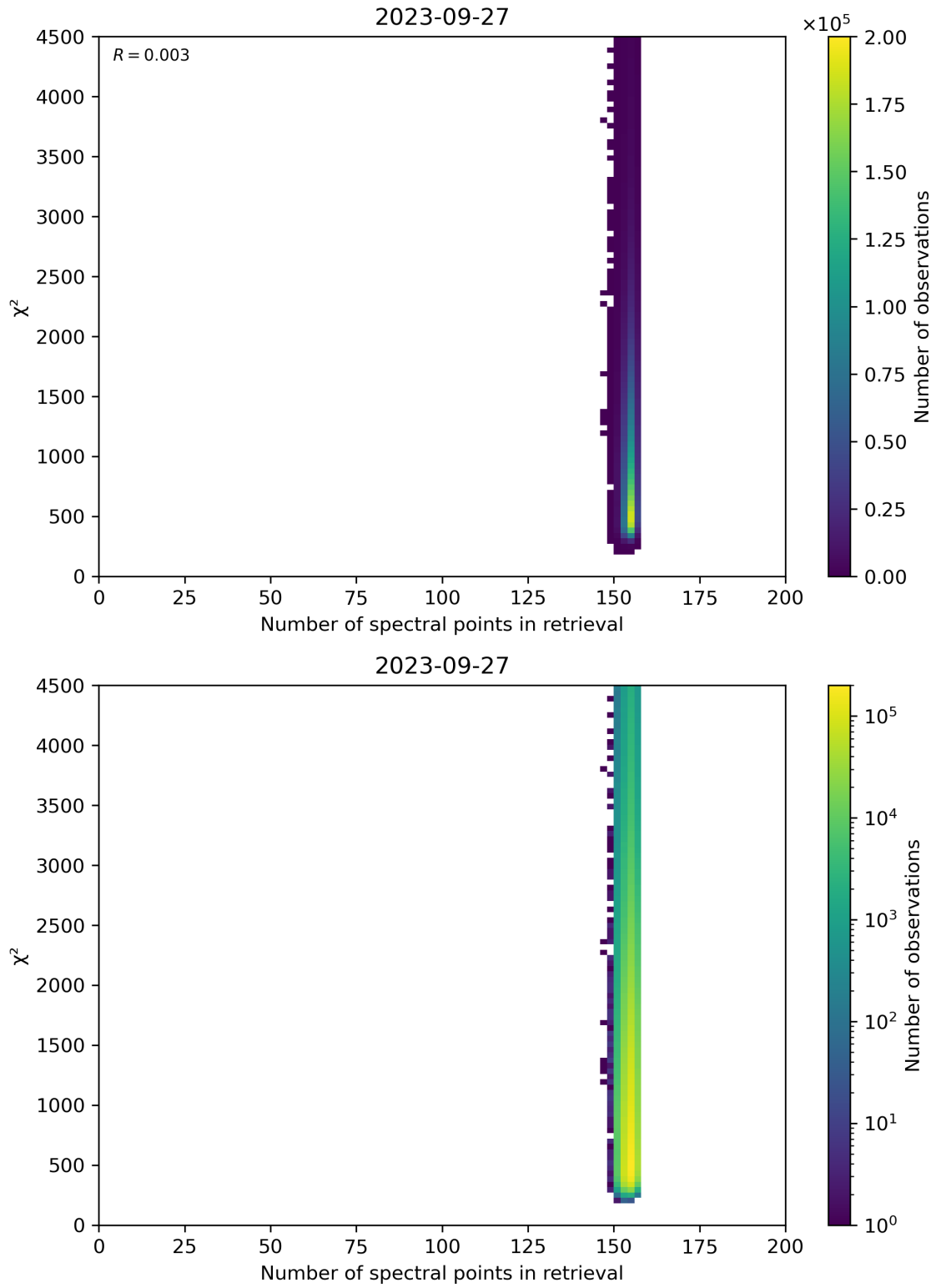
Figure 58: Scatter density plot of “Number of spectral points in retrieval” against “ \chi^2 ” for 2023-09-26 to 2023-09-28.
