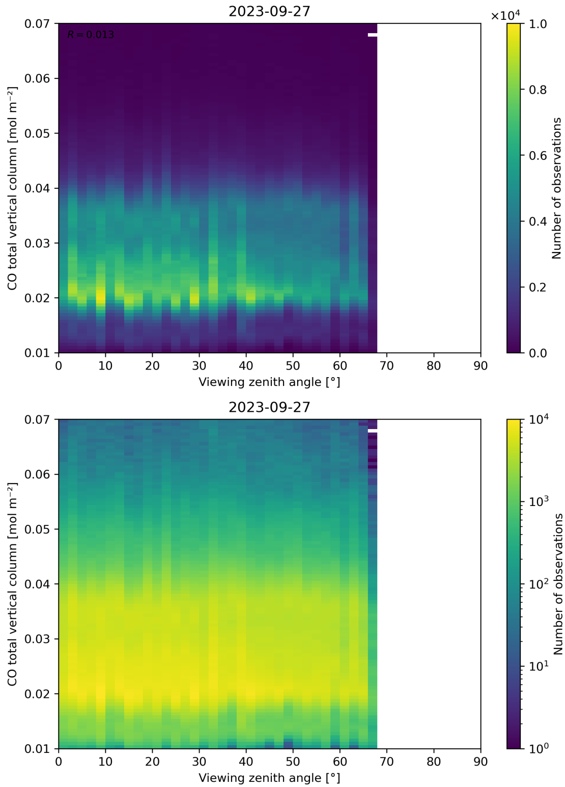
Figure 69: Scatter density plot of “Viewing zenith angle” against “CO total vertical column” for 2023-09-26 to 2023-09-28.
