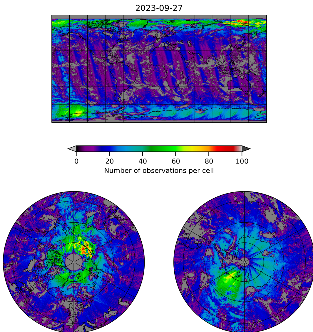
Figure 8: Map of the number of observations for 2023-09-26 to 2023-09-28
