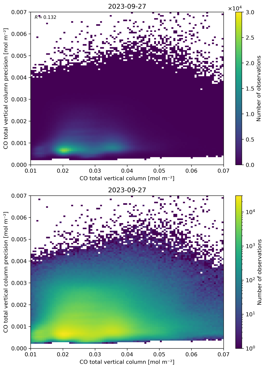
Figure 34: Scatter density plot of “CO total vertical column” against “CO total vertical column precision” for 2023-09-26 to 2023-09-28.
