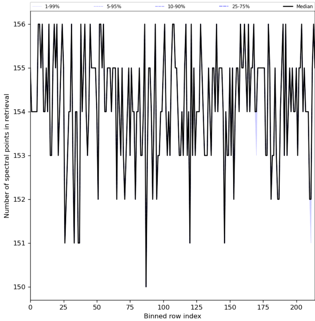
Figure 29: Along track statistics of “Number of spectral points in retrieval” for 2023-09-26 to 2023-09-28
