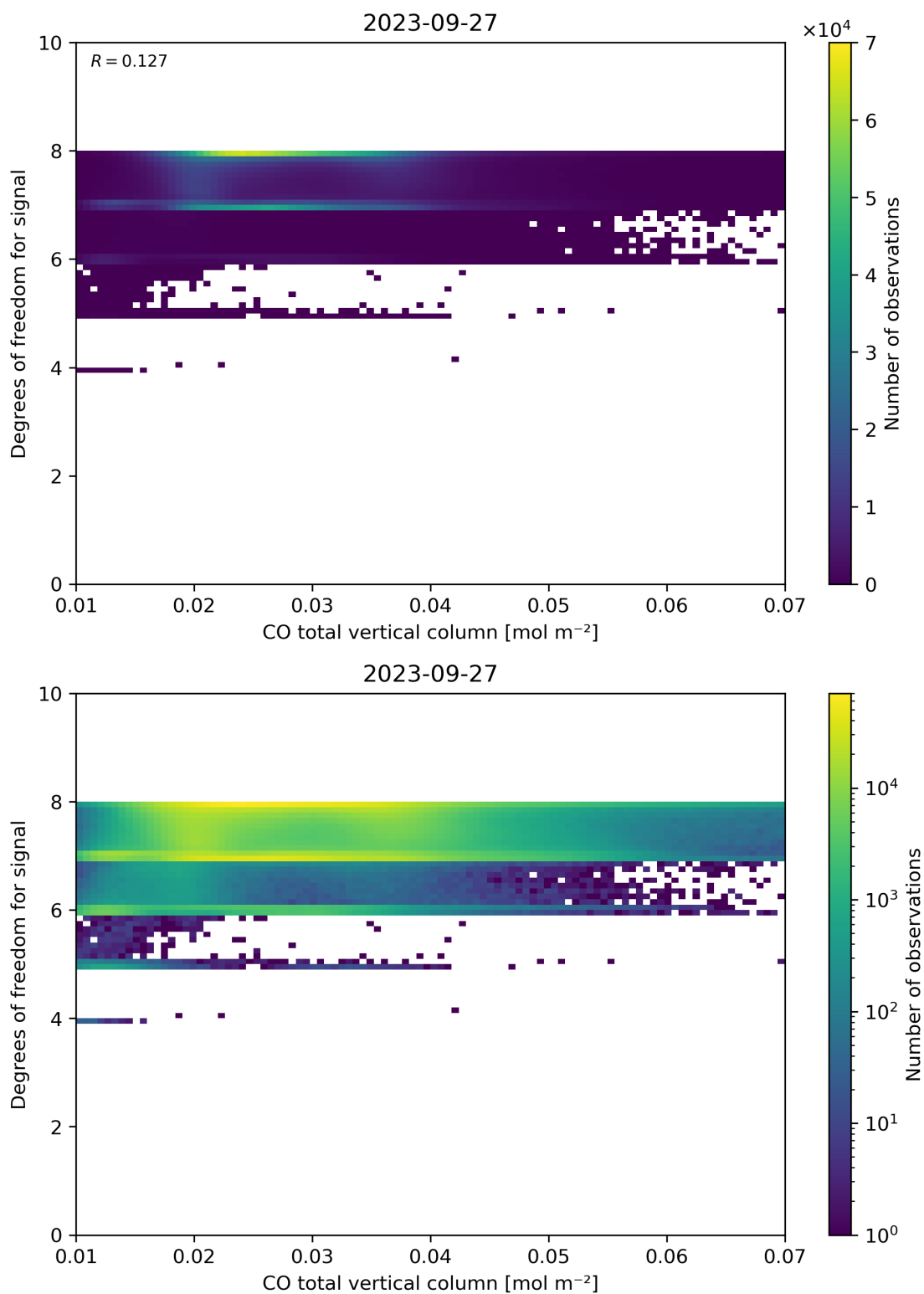
Figure 41: Scatter density plot of “CO total vertical column” against “Degrees of freedom for signal” for 2023-09-26 to 2023-09-28.
