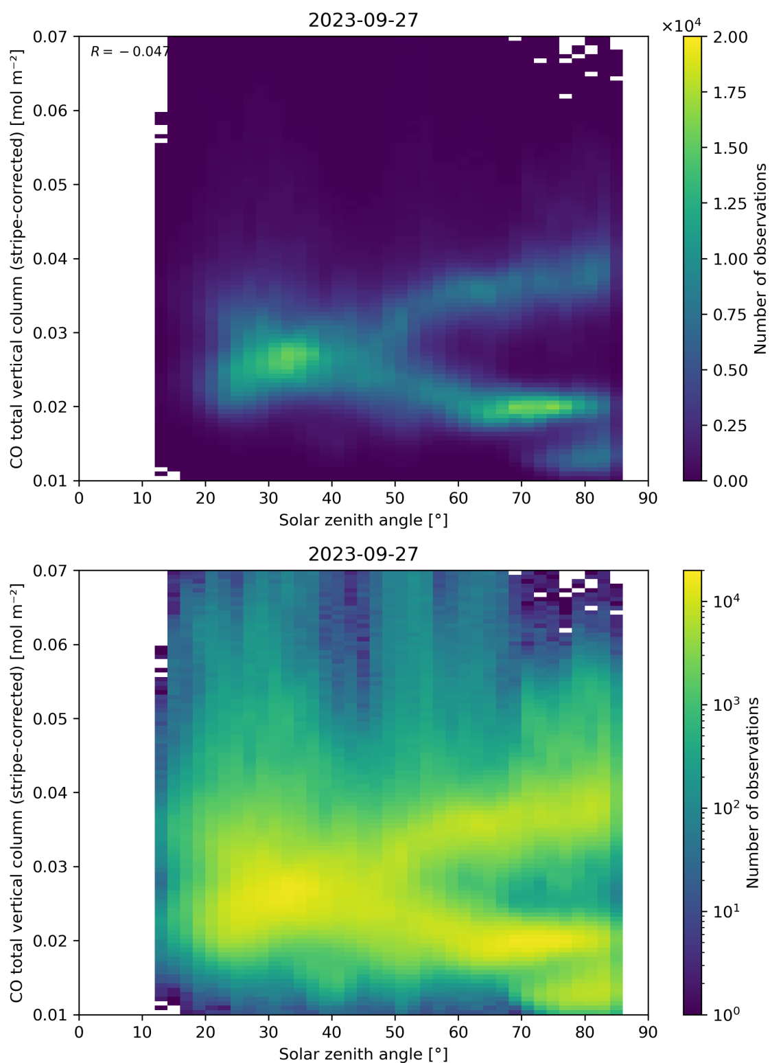
Figure 62: Scatter density plot of “Solar zenith angle” against “CO total vertical column (stripe-corrected)” for 2023-09-26 to 2023-09-28.
