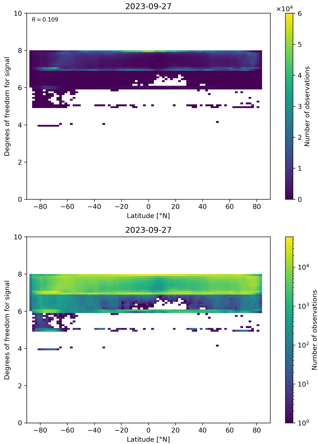
Figure 55: Scatter density plot of “Latitude” against “Degrees of freedom for signal” for 2023-09-26 to 2023-09-28.
