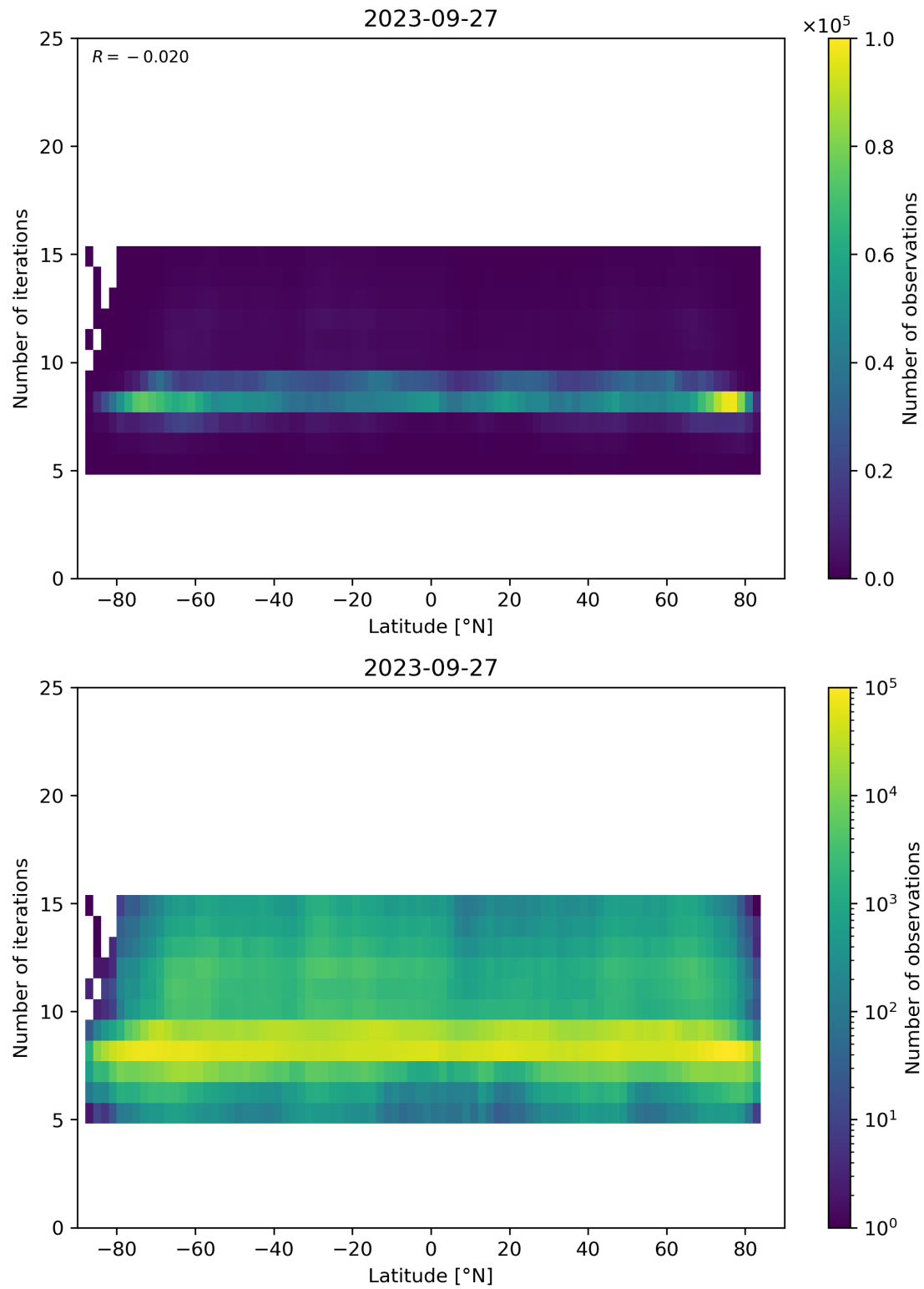
Figure 56: Scatter density plot of “Latitude” against “Number of iterations” for 2023-09-26 to 2023-09-28.
