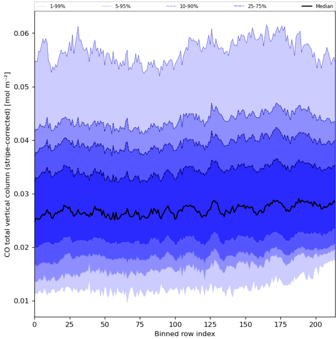
Figure 27: Along track statistics of “CO total vertical column (stripe-corrected)” for 2023-09-26 to 2023-09-28
