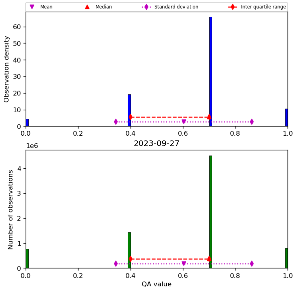
Figure 17: Histogram of “QA value” for 2023-09-26 to 2023-09-28
