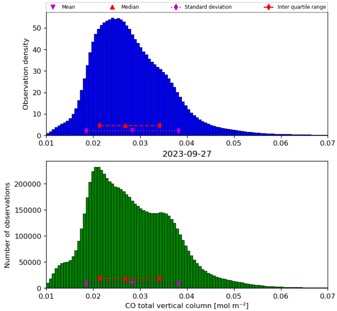
Figure 18: Histogram of “CO total vertical column” for 2023-09-26 to 2023-09-28
