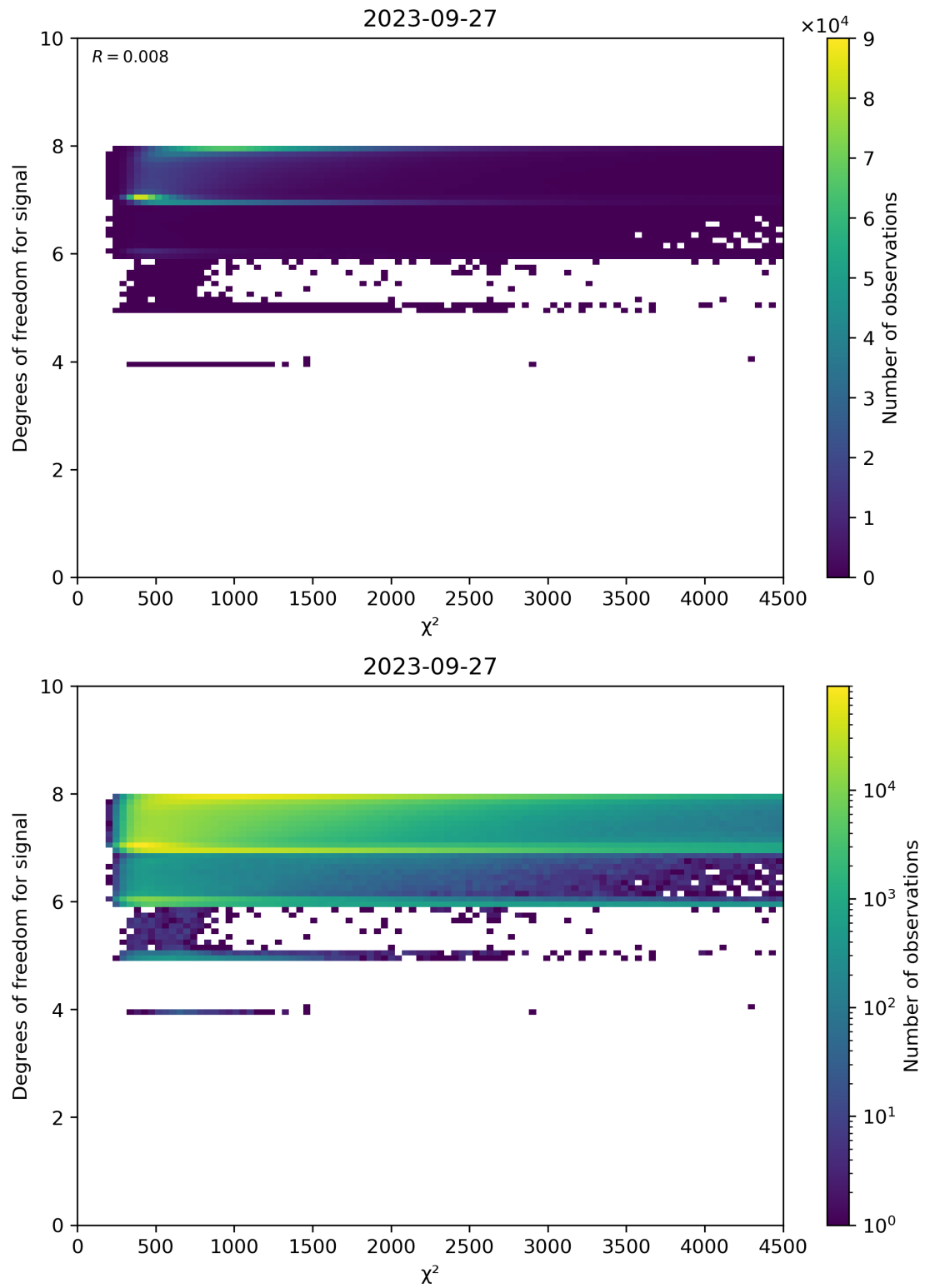
Figure 48: Scatter density plot of “ \chi^2 ” against “Degrees of freedom for signal” for 2023-09-26 to 2023-09-28.
