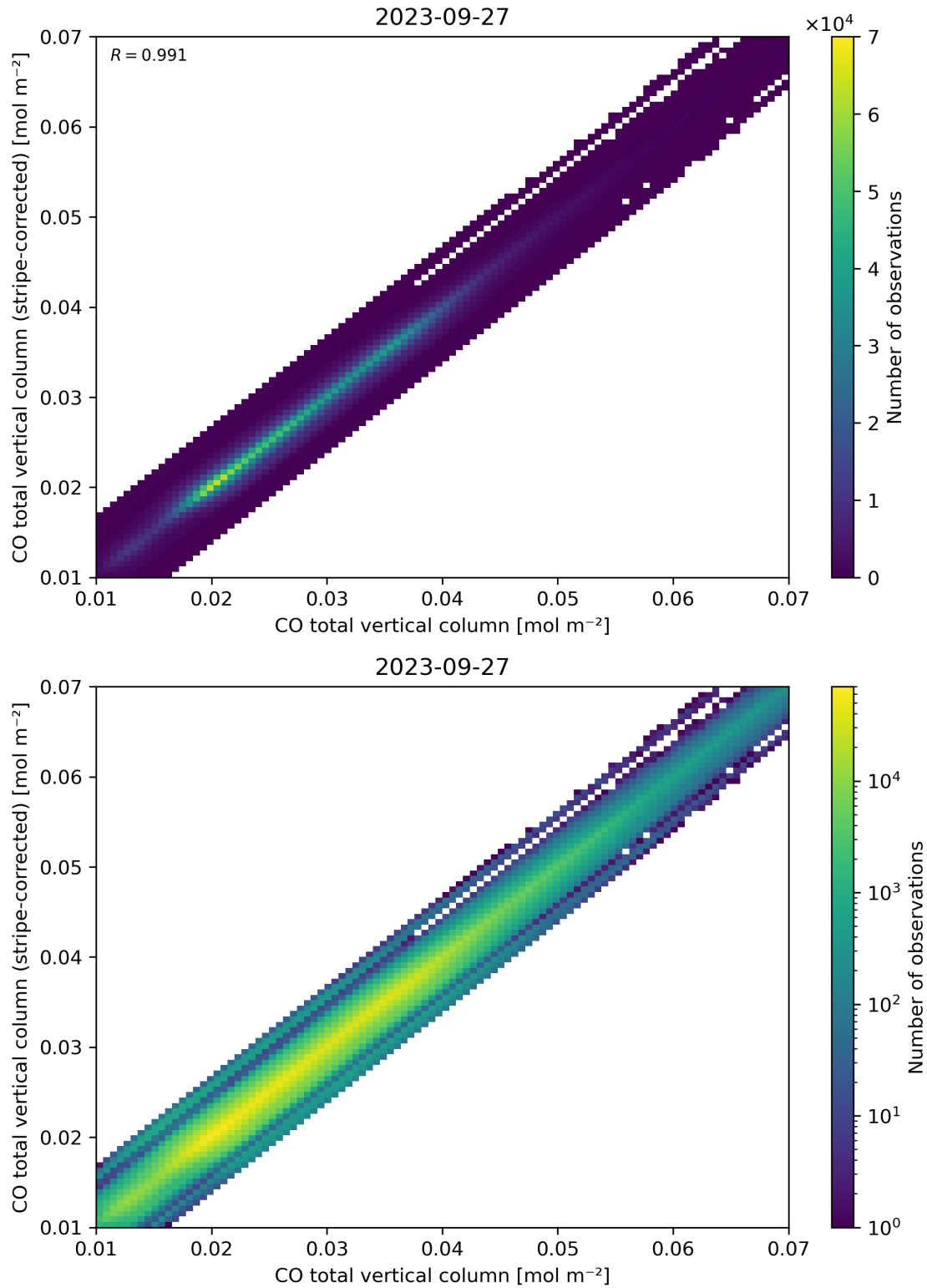
Figure 33: Scatter density plot of “CO total vertical column” against “CO total vertical column (stripe-corrected)” for 2023-09-26 to 2023-09-28.
