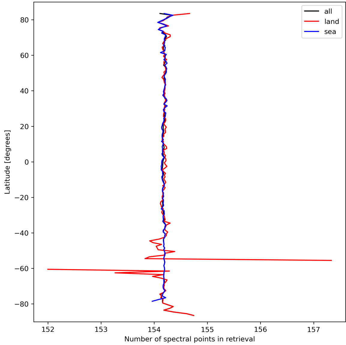
Figure 13: Zonal average of “Number of spectral points in retrieval” for 2023-09-26 to 2023-09-28.
