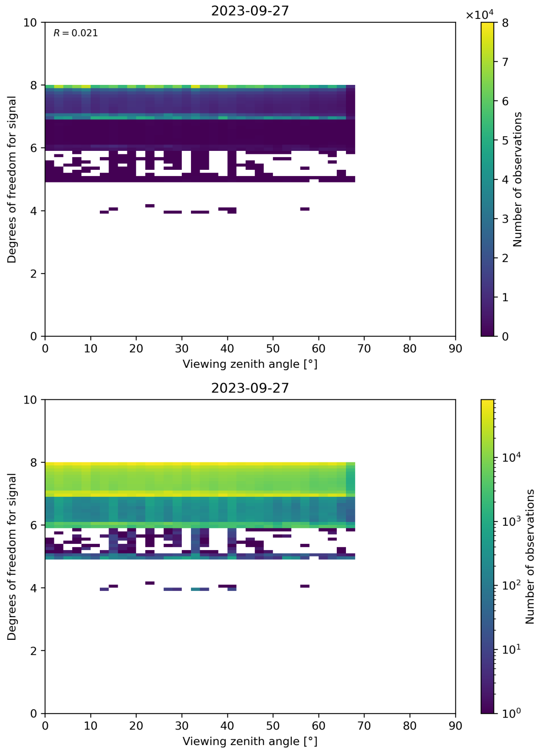
Figure 73: Scatter density plot of “Viewing zenith angle” against “Degrees of freedom for signal” for 2023-09-26 to 2023-09-28.
