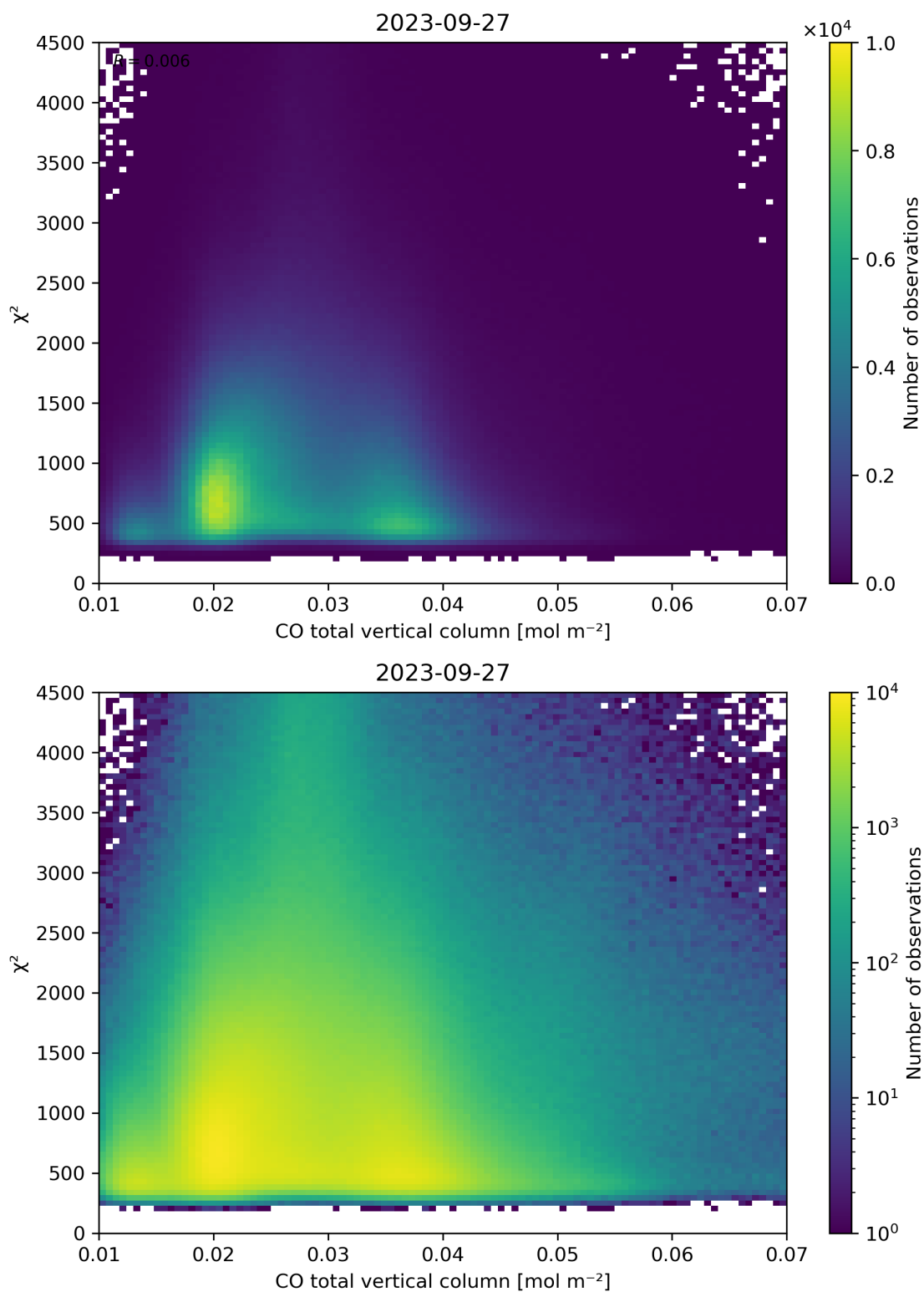
Figure 35: Scatter density plot of “CO total vertical column” against “ \chi^2 ” for 2023-09-26 to 2023-09-28.
