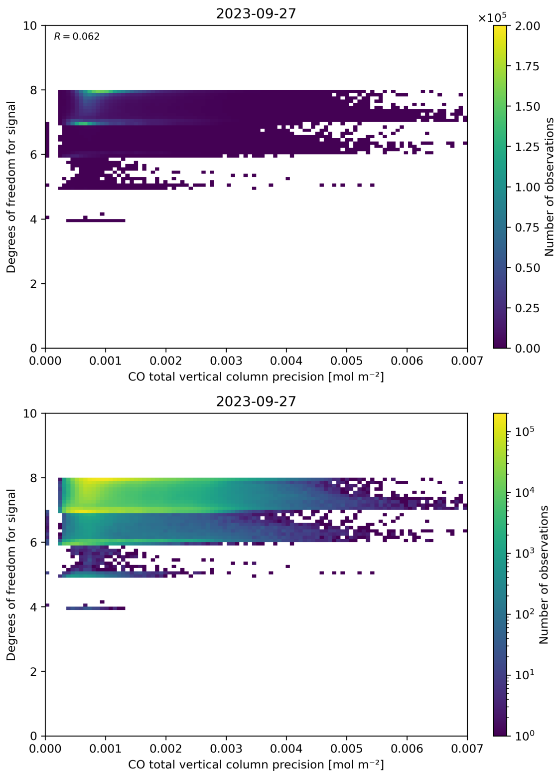
Figure 45: Scatter density plot of “CO total vertical column precision” against “Degrees of freedom for signal” for 2023-09-26 to 2023-09-28.
