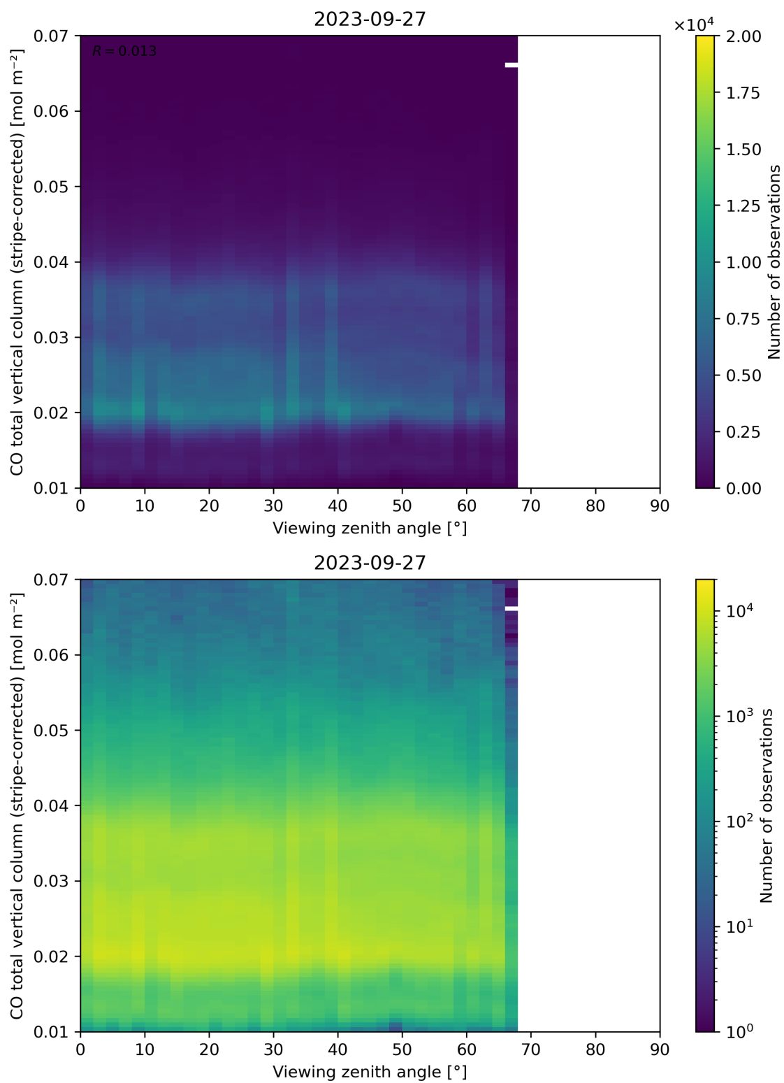
Figure 70: Scatter density plot of “Viewing zenith angle” against “CO total vertical column (stripe-corrected)” for 2023-09-26 to 2023-09-28.
