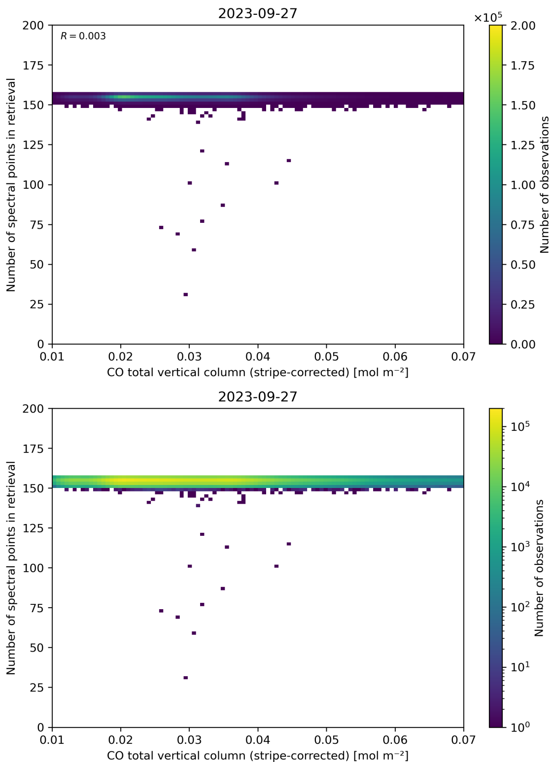
Figure 40: Scatter density plot of “CO total vertical column (stripe-corrected)” against “Number of spectral points in retrieval” for 2023-09-26 to 2023-09-28.
