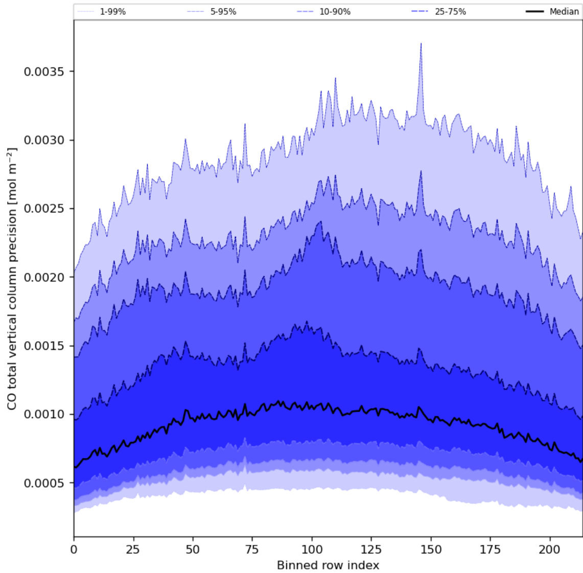
Figure 28: Along track statistics of “CO total vertical column precision” for 2023-09-26 to 2023-09-28
