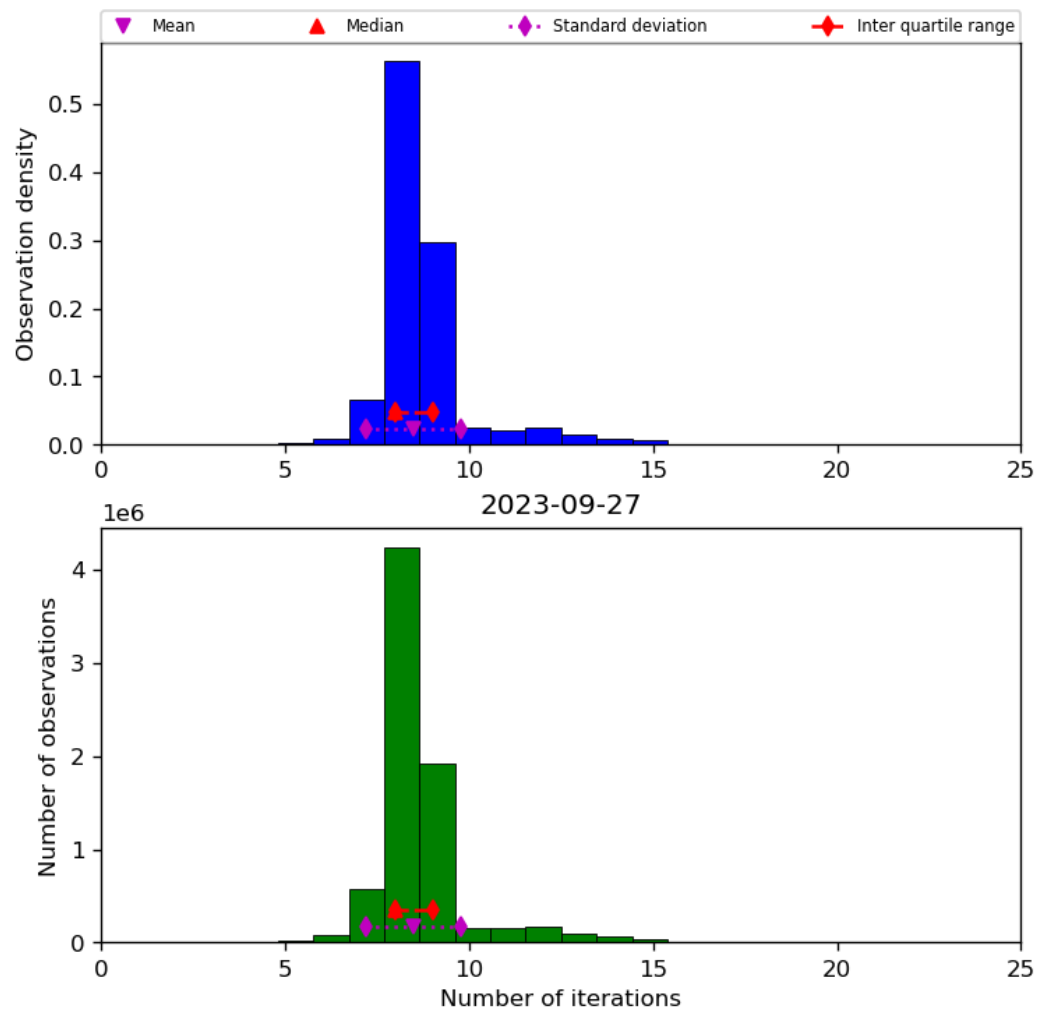
Figure 24: Histogram of “Number of iterations” for 2023-09-26 to 2023-09-28
