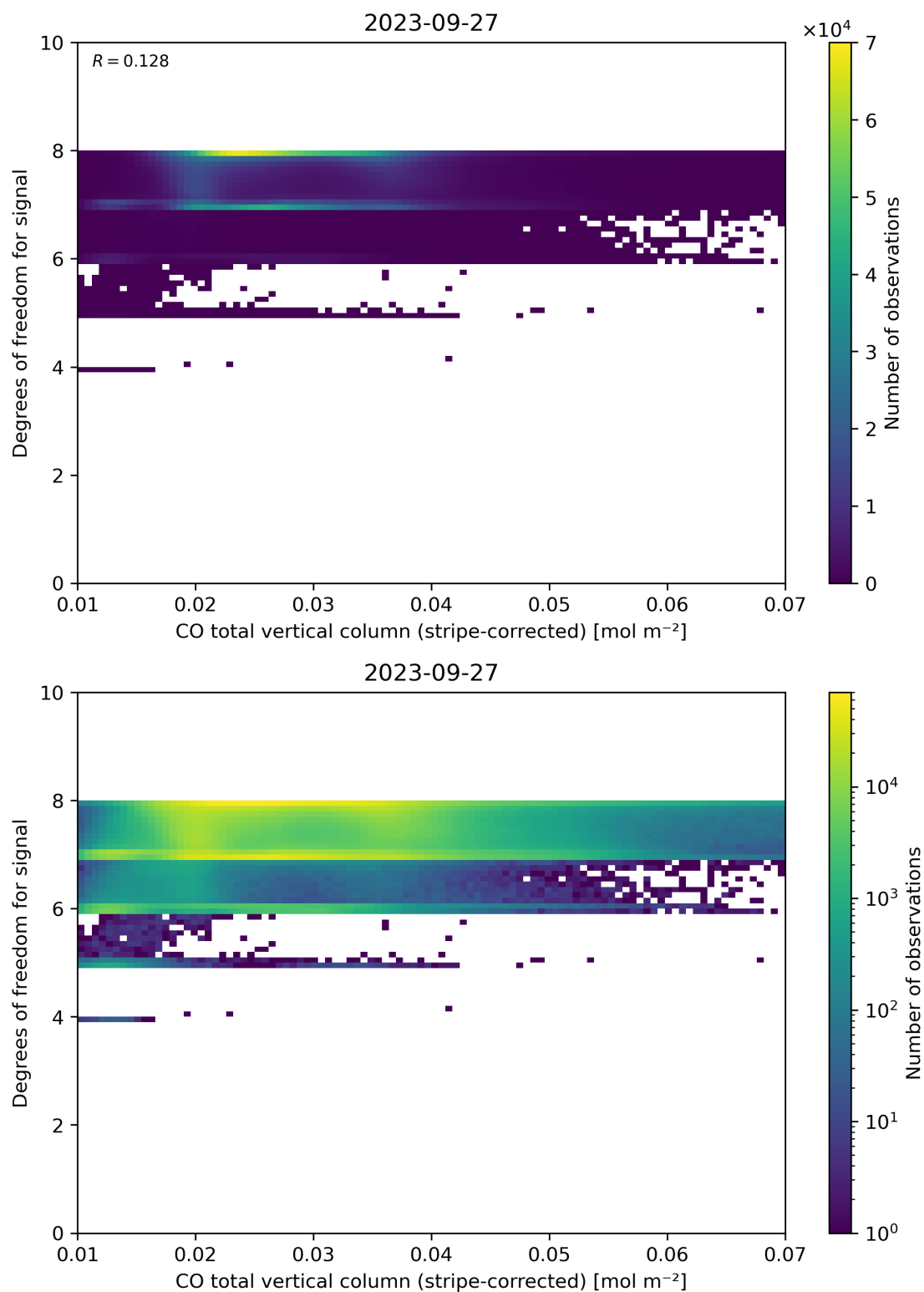
Figure 38: Scatter density plot of “CO total vertical column (stripe-corrected)” against “Degrees of freedom for signal” for 2023-09-26 to 2023-09-28.
