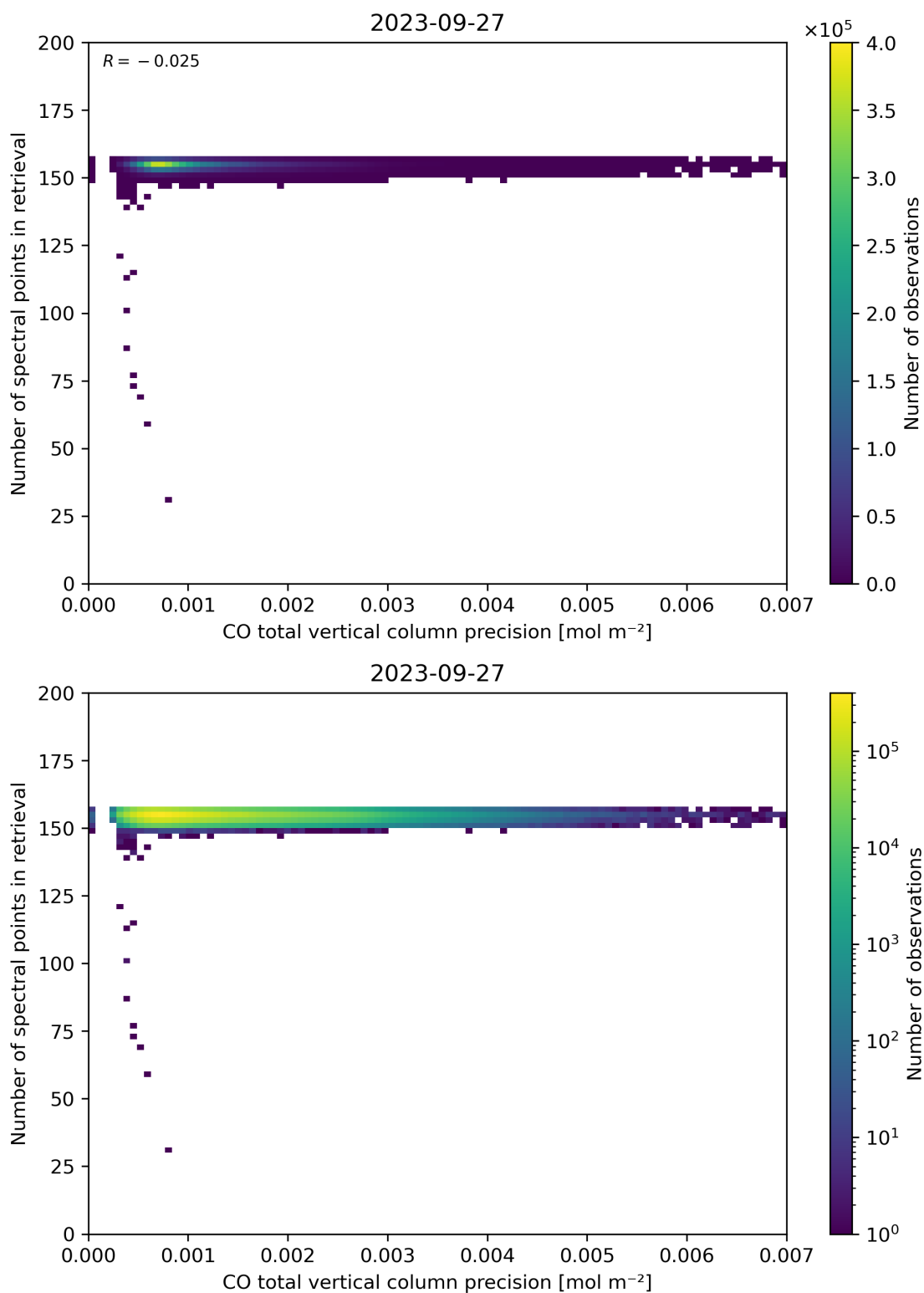
Figure 47: Scatter density plot of “CO total vertical column precision” against “Number of spectral points in retrieval” for 2023-09-26 to 2023-09-28.
