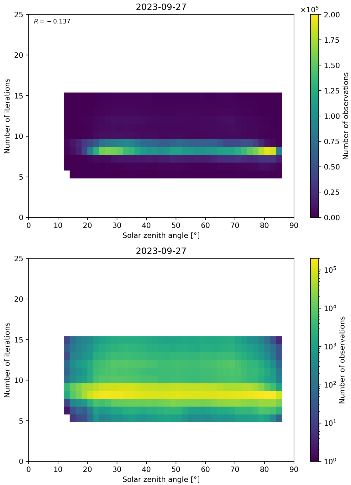
Figure 67: Scatter density plot of “Solar zenith angle” against “Number of iterations” for 2023-09-26 to 2023-09-28.
