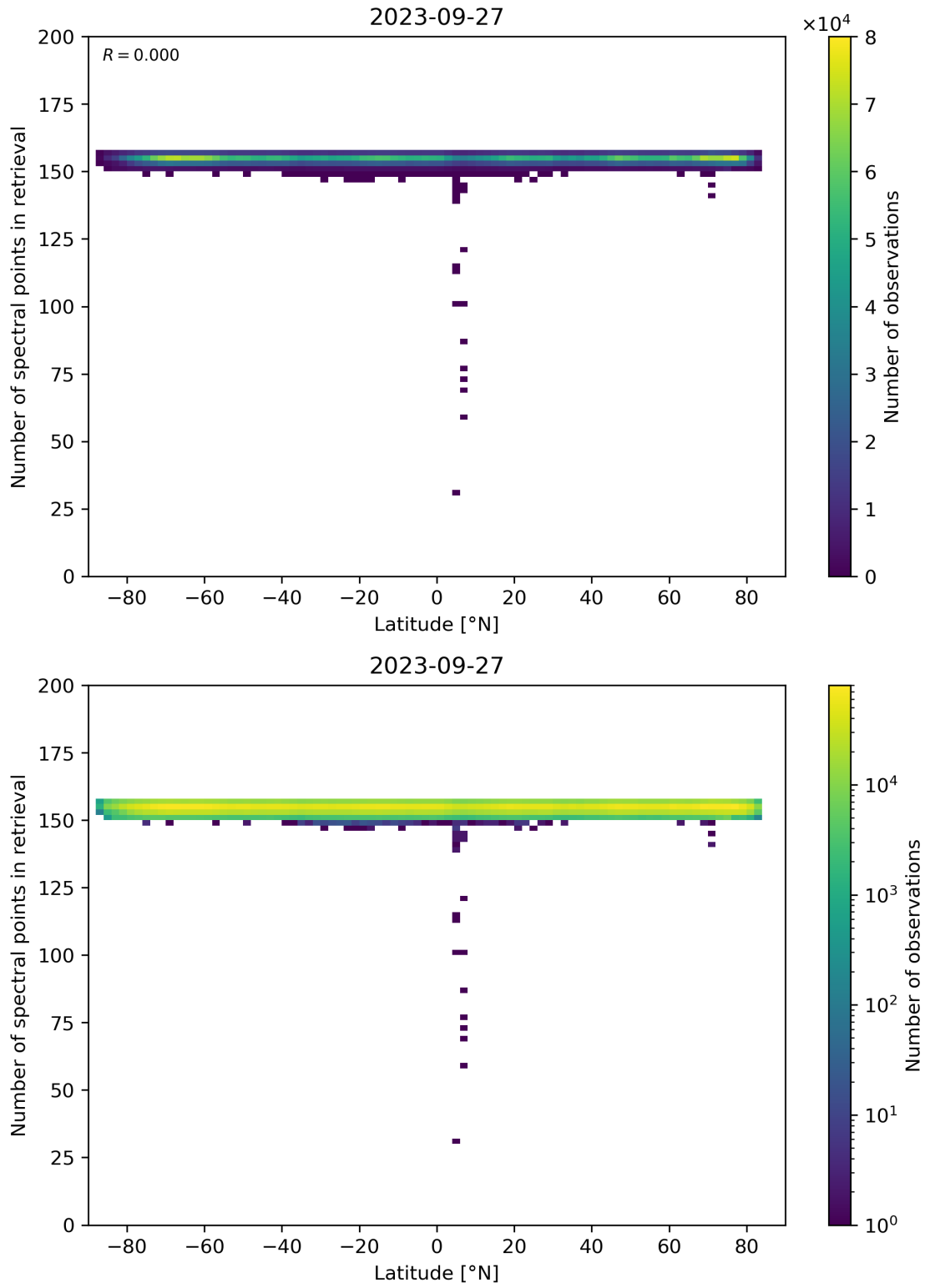
Figure 57: Scatter density plot of “Latitude” against “Number of spectral points in retrieval” for 2023-09-26 to 2023-09-28.
