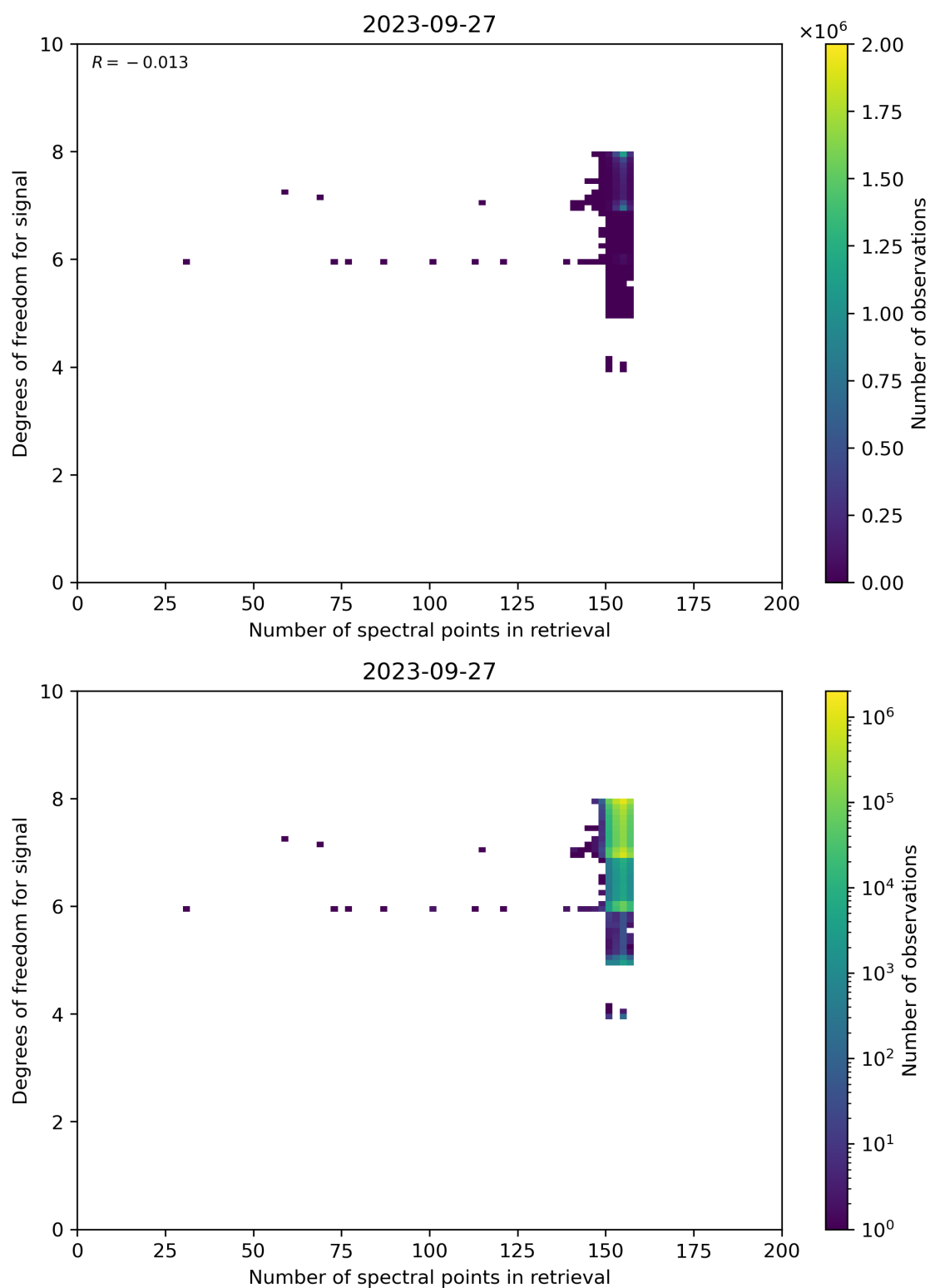
Figure 59: Scatter density plot of “Number of spectral points in retrieval” against “Degrees of freedom for signal” for 2023-09-26 to 2023-09-28.
