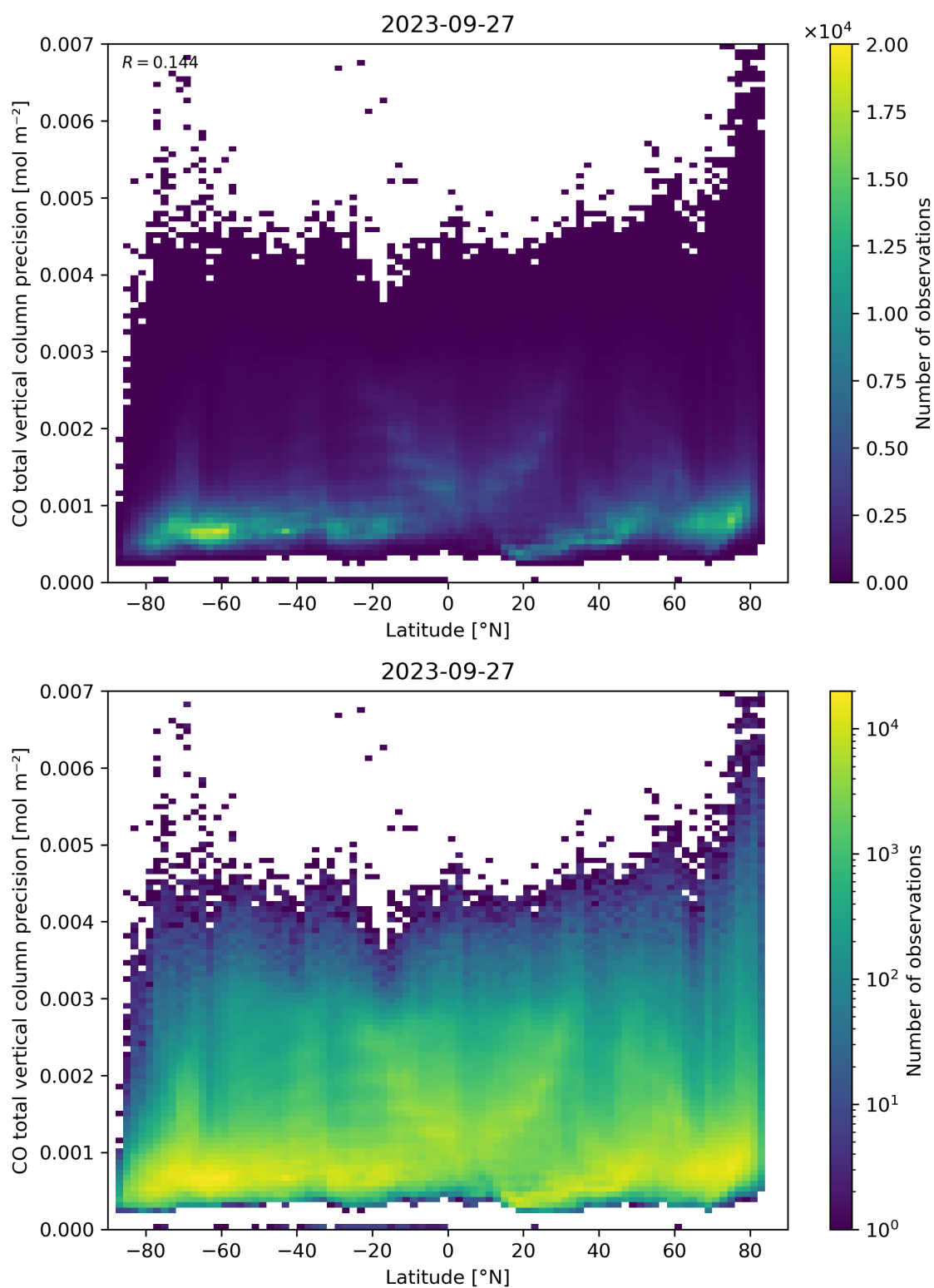
Figure 53: Scatter density plot of “Latitude” against “CO total vertical column precision” for 2023-09-26 to 2023-09-28.
