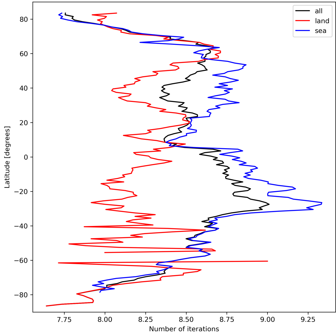
Figure 16: Zonal average of “Number of iterations” for 2023-09-26 to 2023-09-28.
