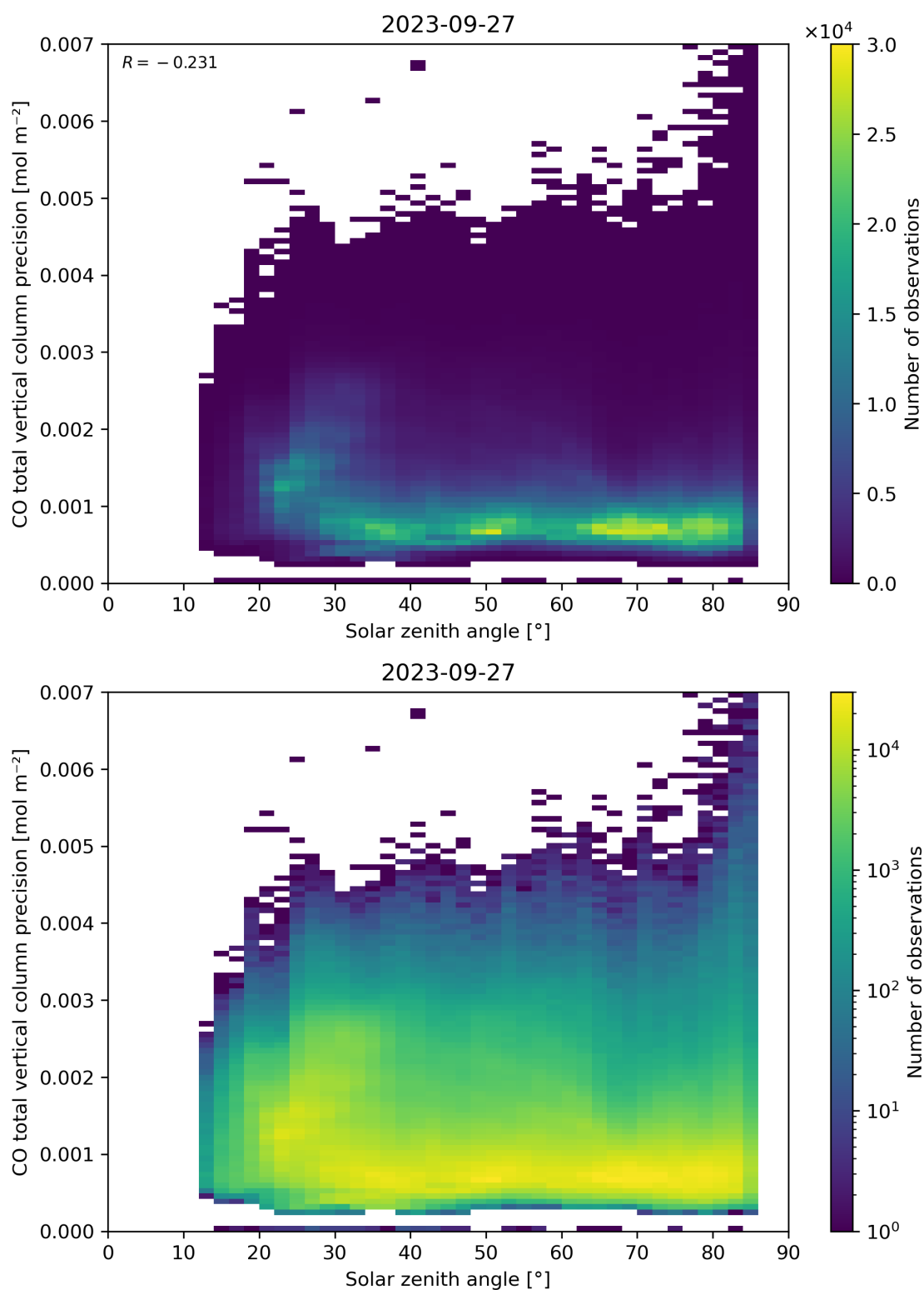
Figure 63: Scatter density plot of “Solar zenith angle” against “CO total vertical column precision” for 2023-09-26 to 2023-09-28.
