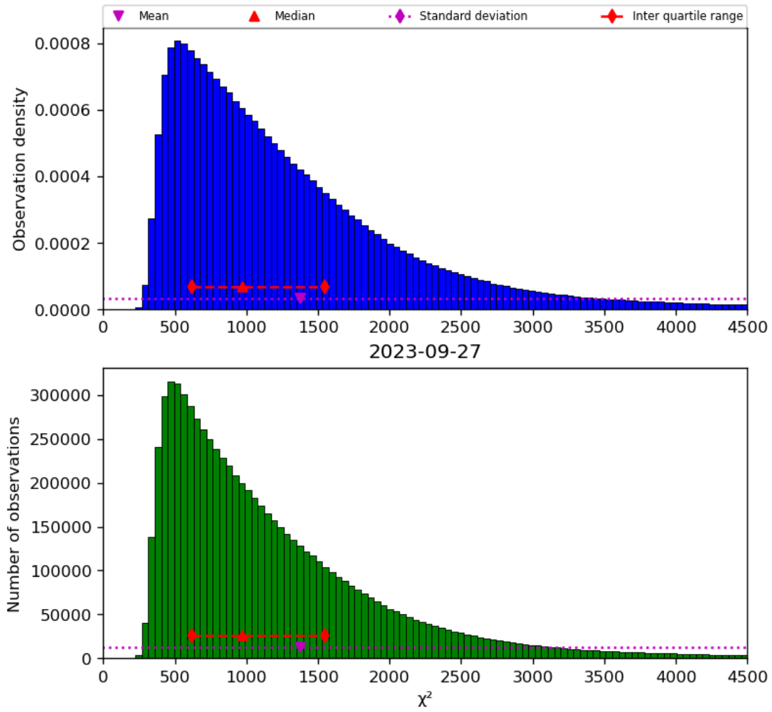
Figure 22: Histogram of “ \chi^2 ” for 2023-09-26 to 2023-09-28
