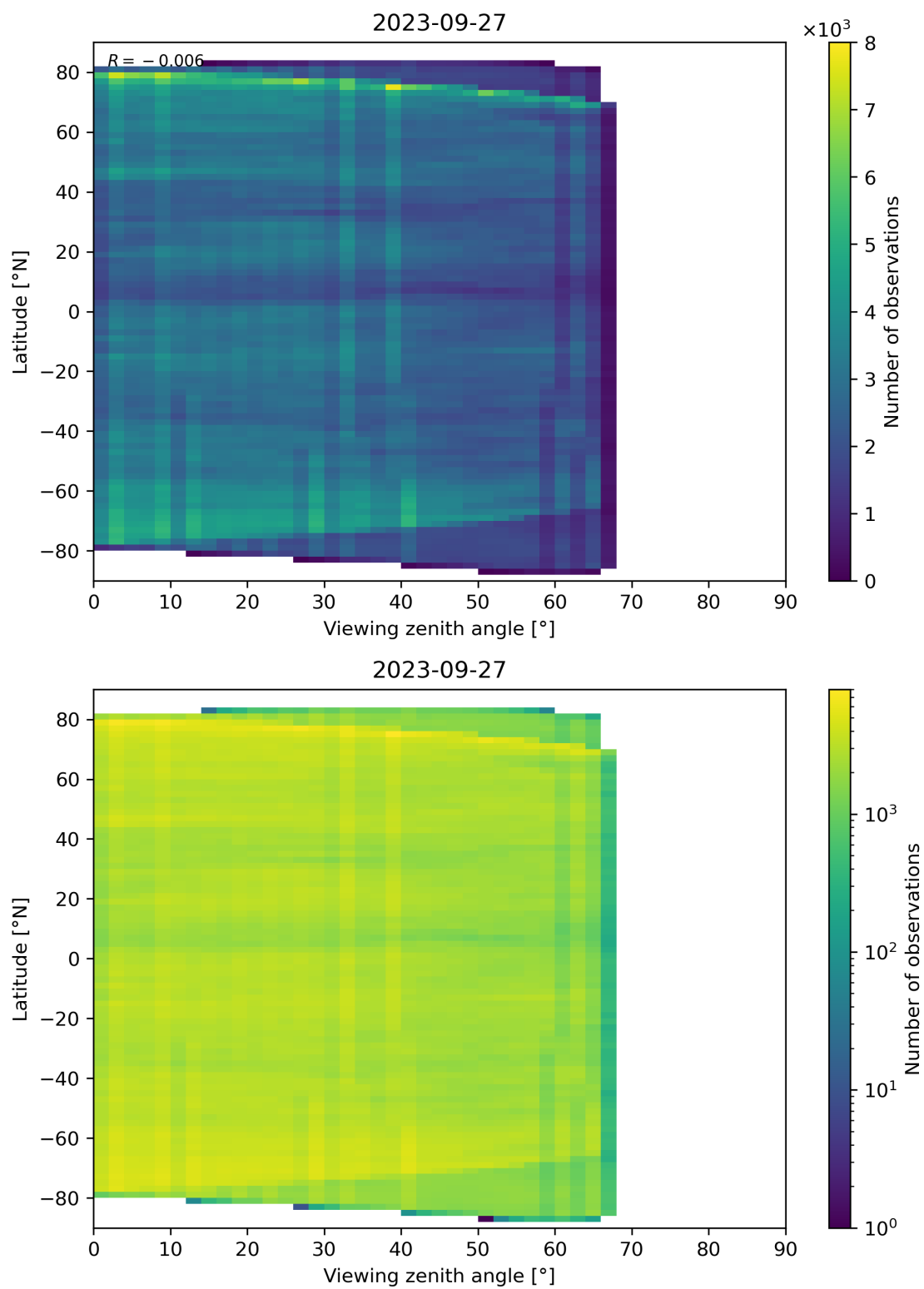
Figure 74: Scatter density plot of “Viewing zenith angle” against “Latitude” for 2023-09-26 to 2023-09-28.
