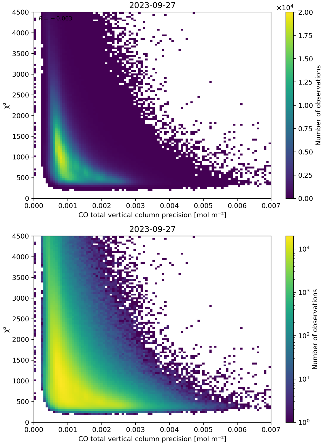
Figure 44: Scatter density plot of “CO total vertical column precision” against “ \chi^2 ” for 2023-09-26 to 2023-09-28.
