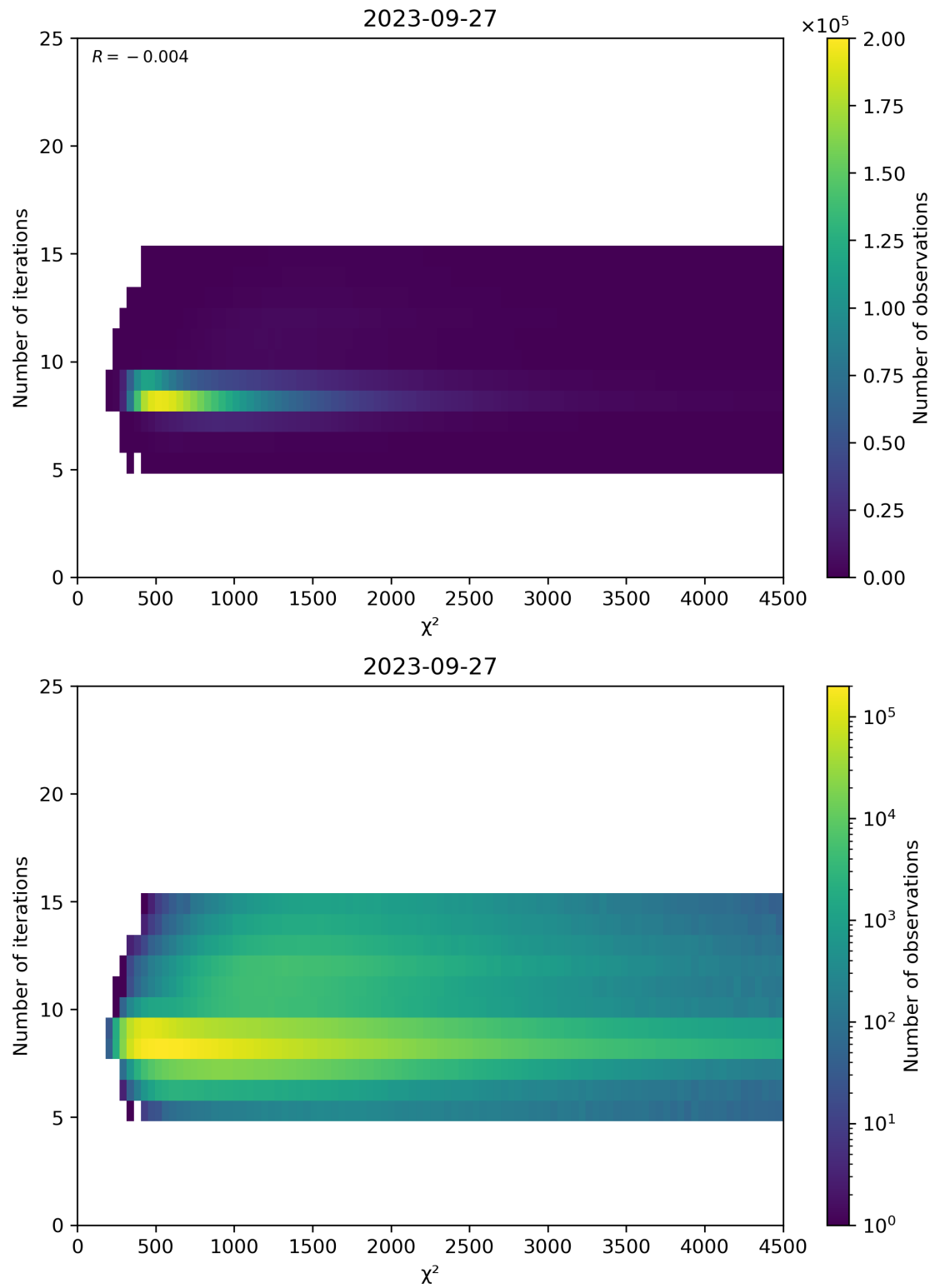
Figure 49: Scatter density plot of “ \chi^2 ” against “Number of iterations” for 2023-09-26 to 2023-09-28.
