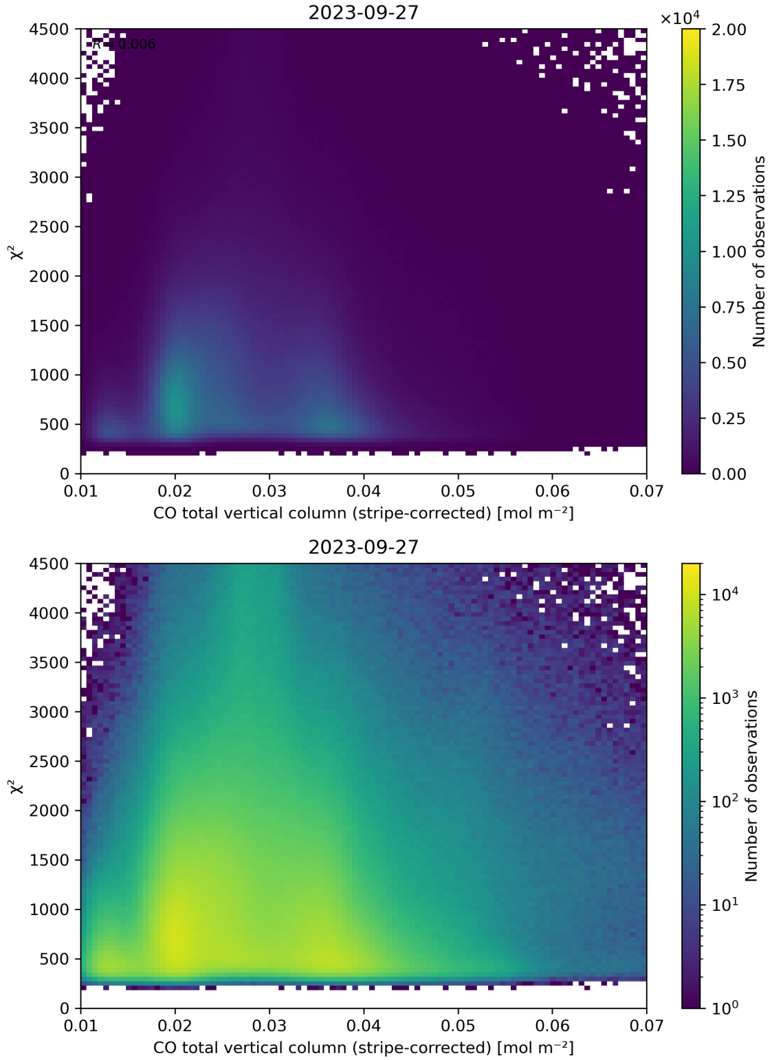
Figure 37: Scatter density plot of “CO total vertical column (stripe-corrected)” against “ \chi^2 ” for 2023-09-26 to 2023-09-28.
