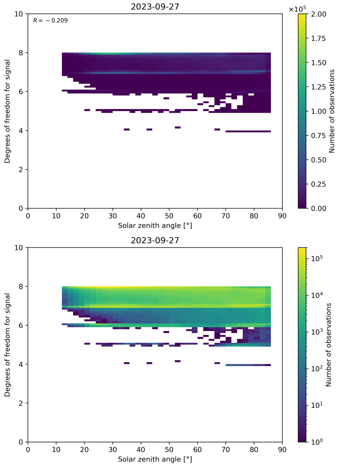
Figure 65: Scatter density plot of “Solar zenith angle” against “Degrees of freedom for signal” for 2023-09-26 to 2023-09-28.
