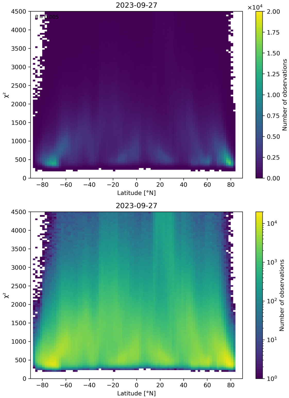
Figure 54: Scatter density plot of “Latitude” against “ \chi^2 ” for 2023-09-26 to 2023-09-28.
