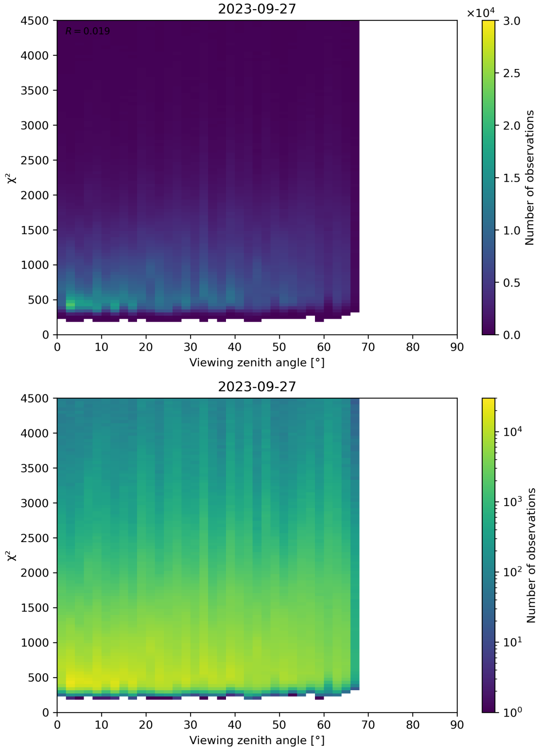
Figure 72: Scatter density plot of “Viewing zenith angle” against “ \chi^2 ” for 2023-09-26 to 2023-09-28.
