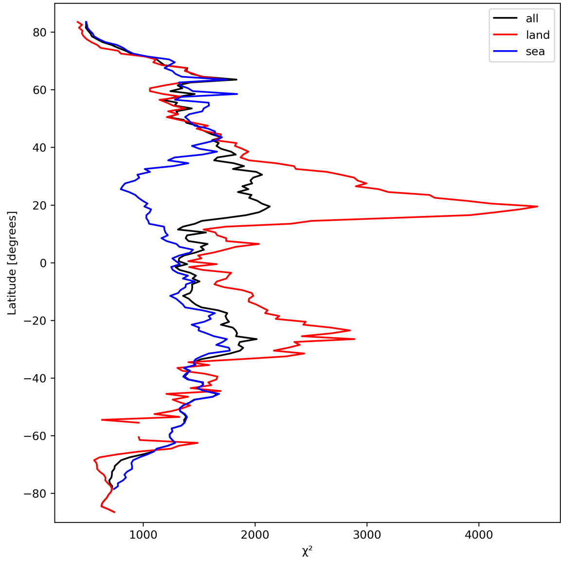
Figure 14: Zonal average of “ \chi^2 ” for 2023-09-26 to 2023-09-28.
