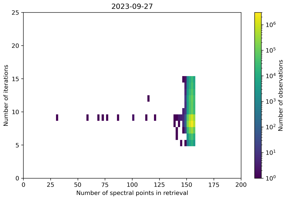
Figure 60: Scatter density plot of “Number of spectral points in retrieval” against “Number of iterations” for 2023-09-26 to 2023-09-28.
