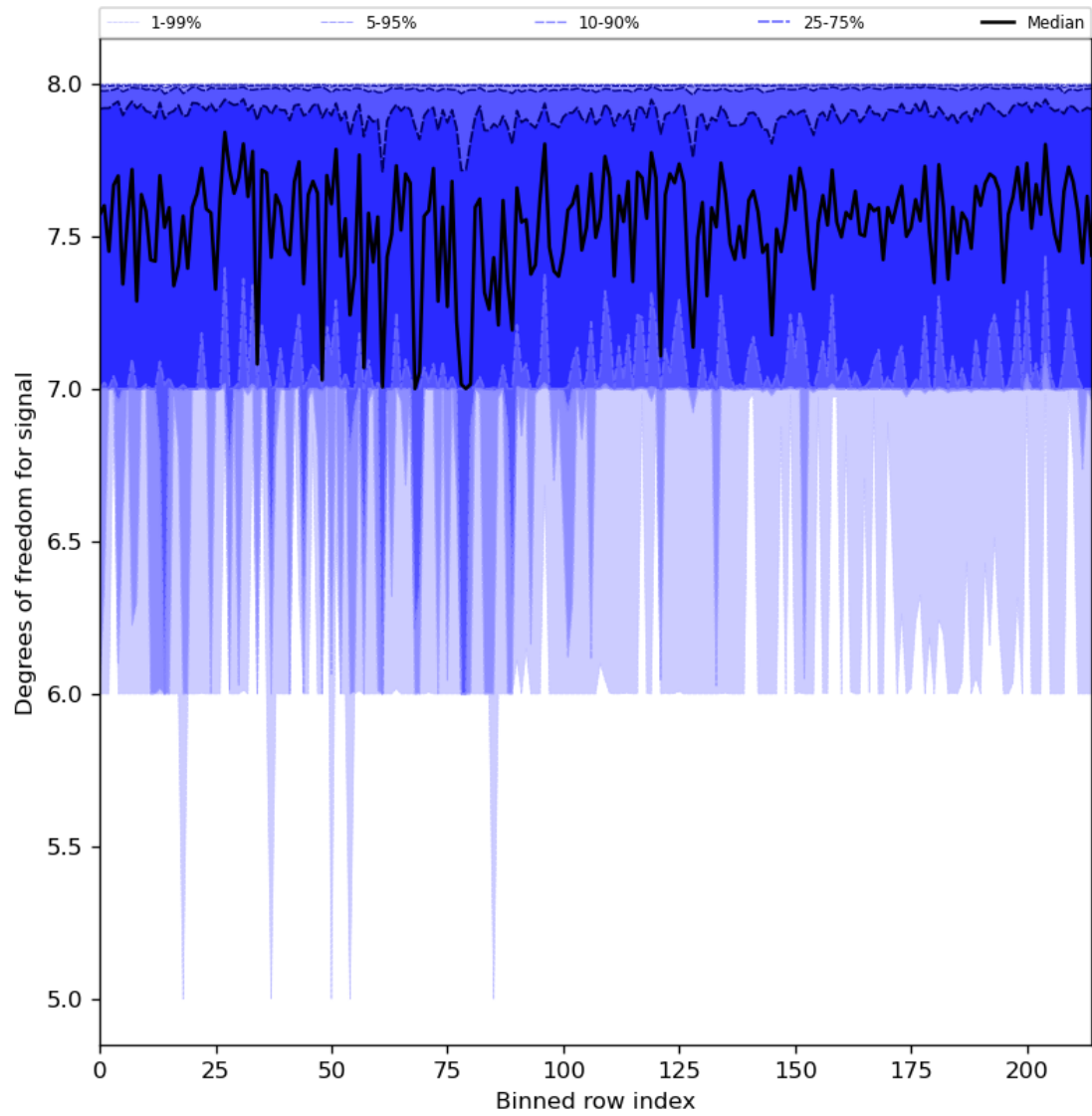
Figure 31: Along track statistics of “Degrees of freedom for signal” for 2023-09-26 to 2023-09-28
