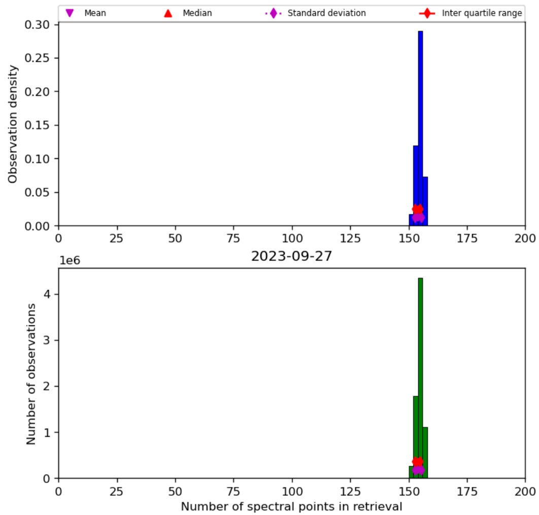
Figure 21: Histogram of “Number of spectral points in retrieval” for 2023-09-26 to 2023-09-28
