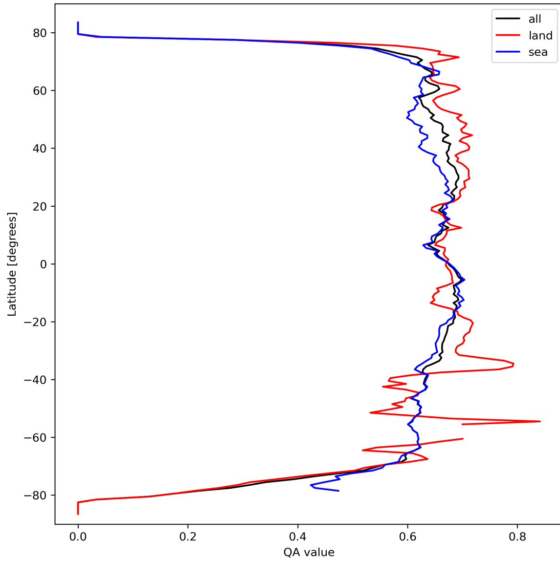
Figure 9: Zonal average of “QA value” for 2023-09-26 to 2023-09-28.
