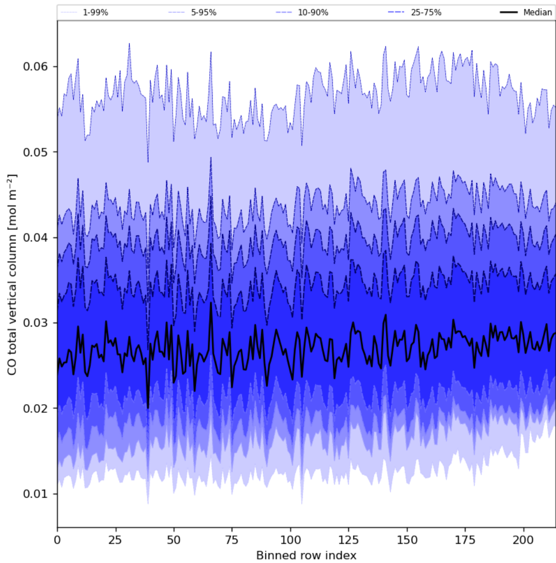
Figure 26: Along track statistics of “CO total vertical column” for 2023-09-26 to 2023-09-28
