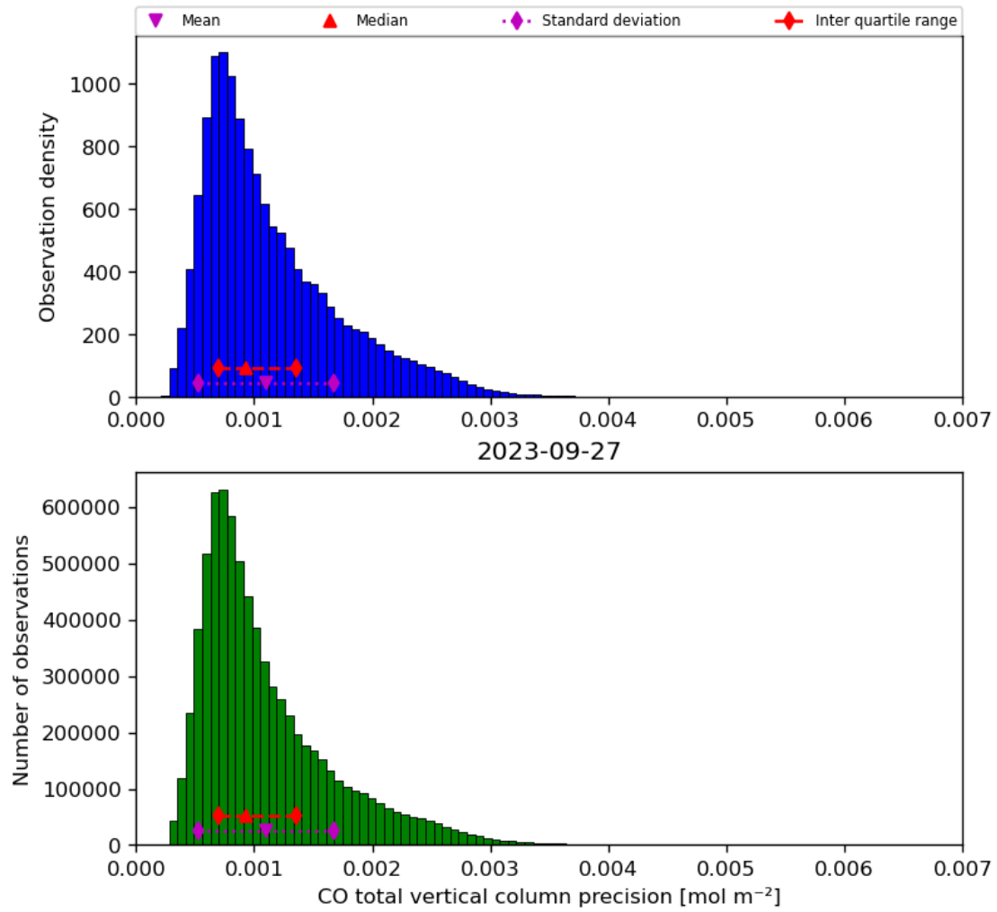
Figure 20: Histogram of “CO total vertical column precision” for 2023-09-26 to 2023-09-28
