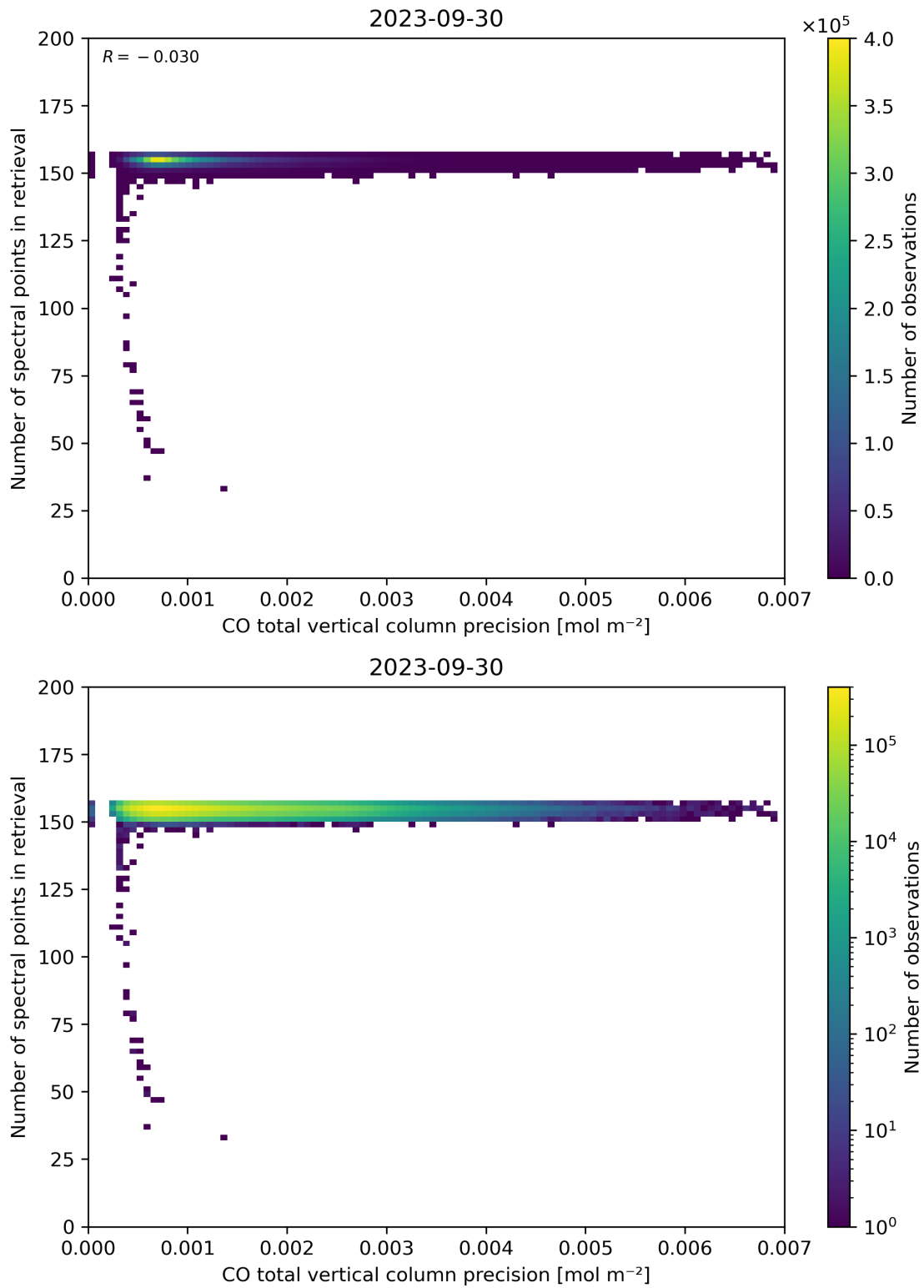
Figure 47: Scatter density plot of “CO total vertical column precision” against “Number of spectral points in retrieval” for 2023-09-29 to 2023-10-01.
