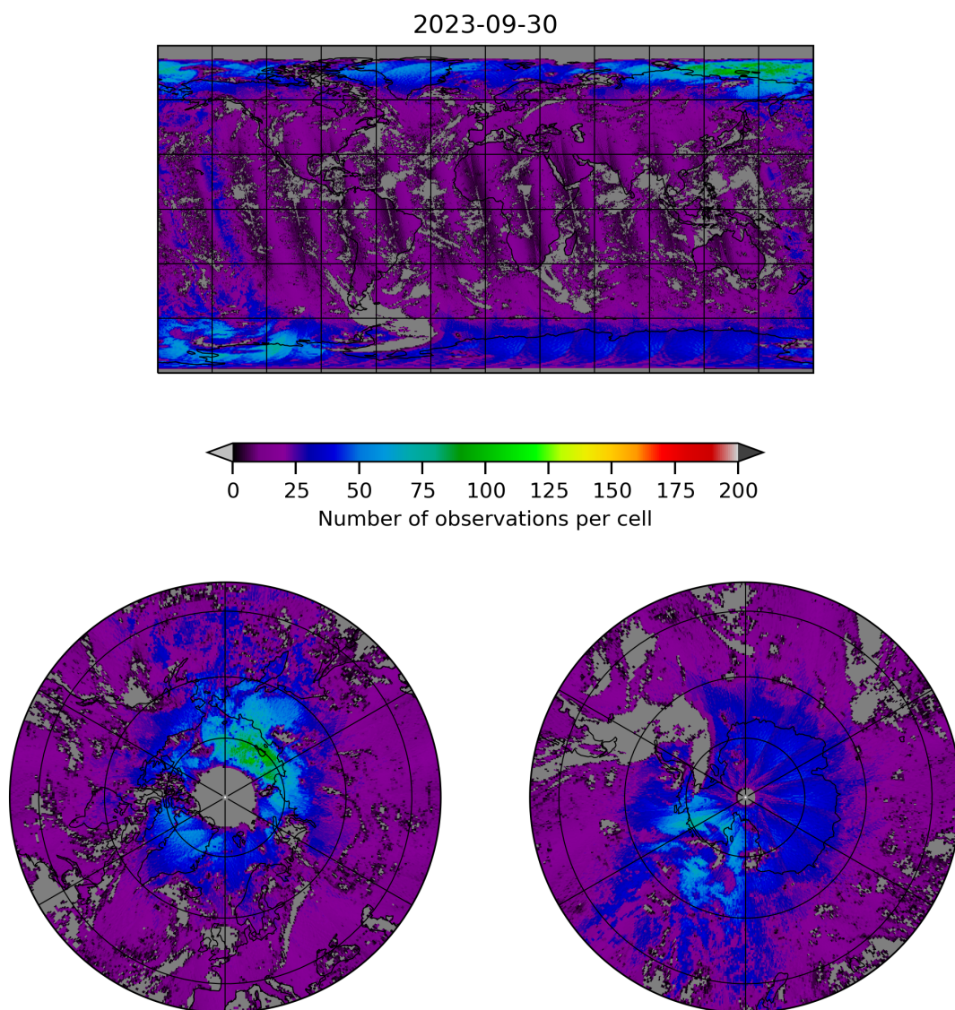
Figure 8: Map of the number of observations for 2023-09-29 to 2023-10-01
