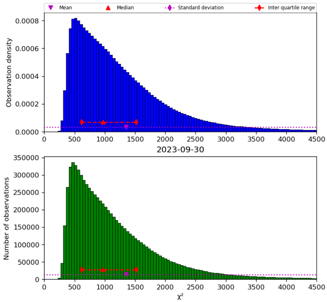
Figure 22: Histogram of “ \chi^2 ” for 2023-09-29 to 2023-10-01
