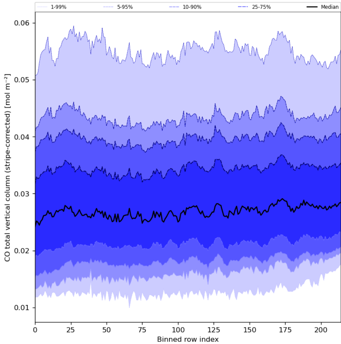
Figure 27: Along track statistics of “CO total vertical column (stripe-corrected)” for 2023-09-29 to 2023-10-01
