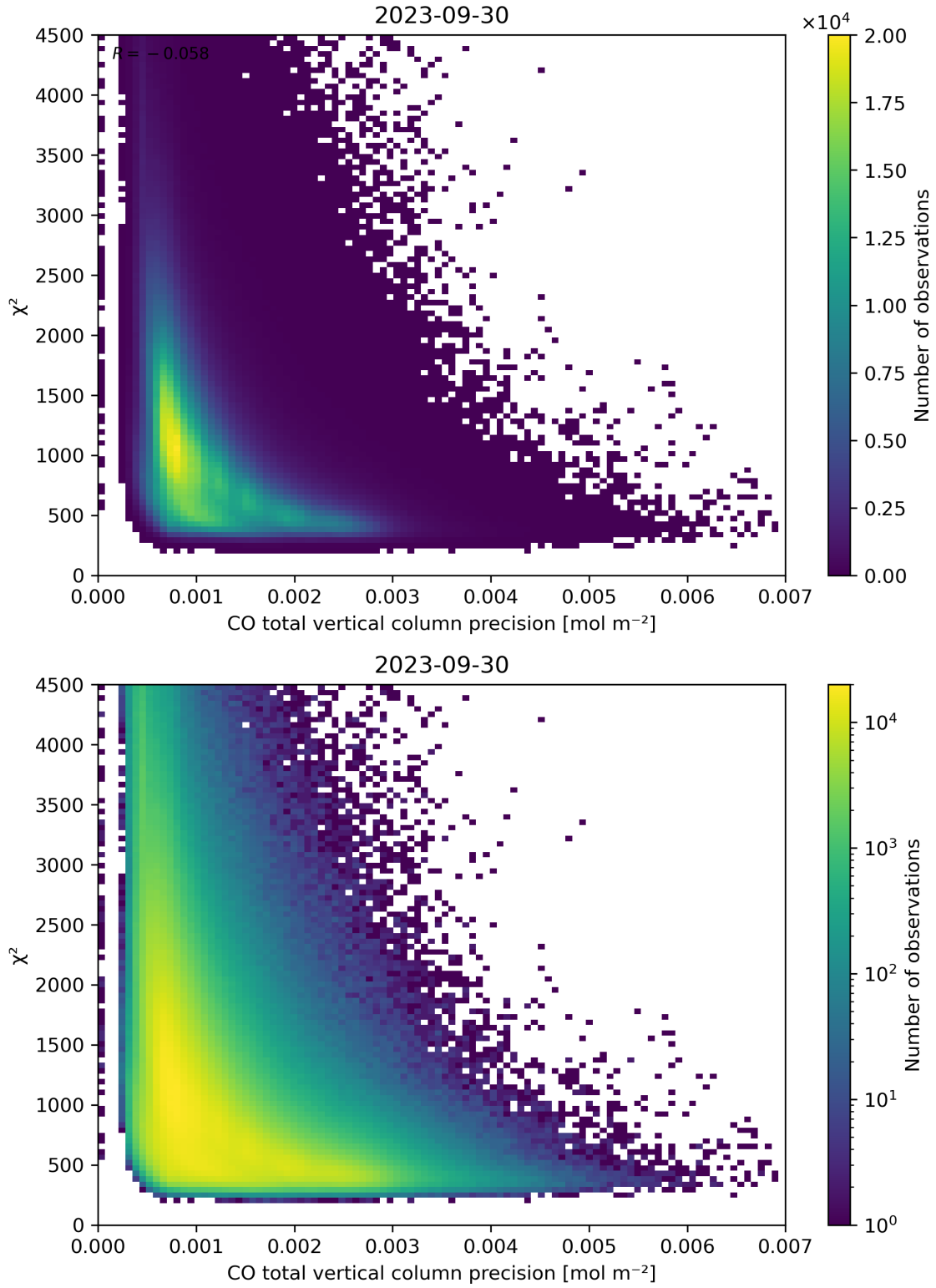
Figure 44: Scatter density plot of “CO total vertical column precision” against “ \chi^2 ” for 2023-09-29 to 2023-10-01.
