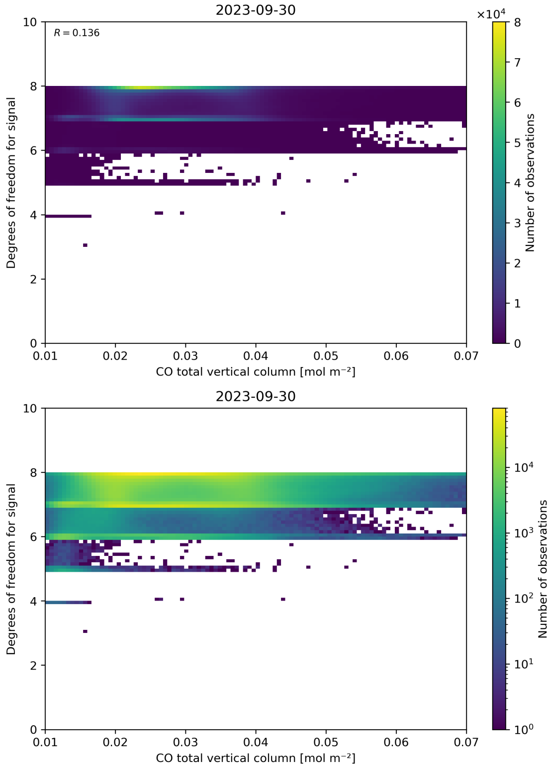
Figure 41: Scatter density plot of “CO total vertical column” against “Degrees of freedom for signal” for 2023-09-29 to 2023-10-01.
