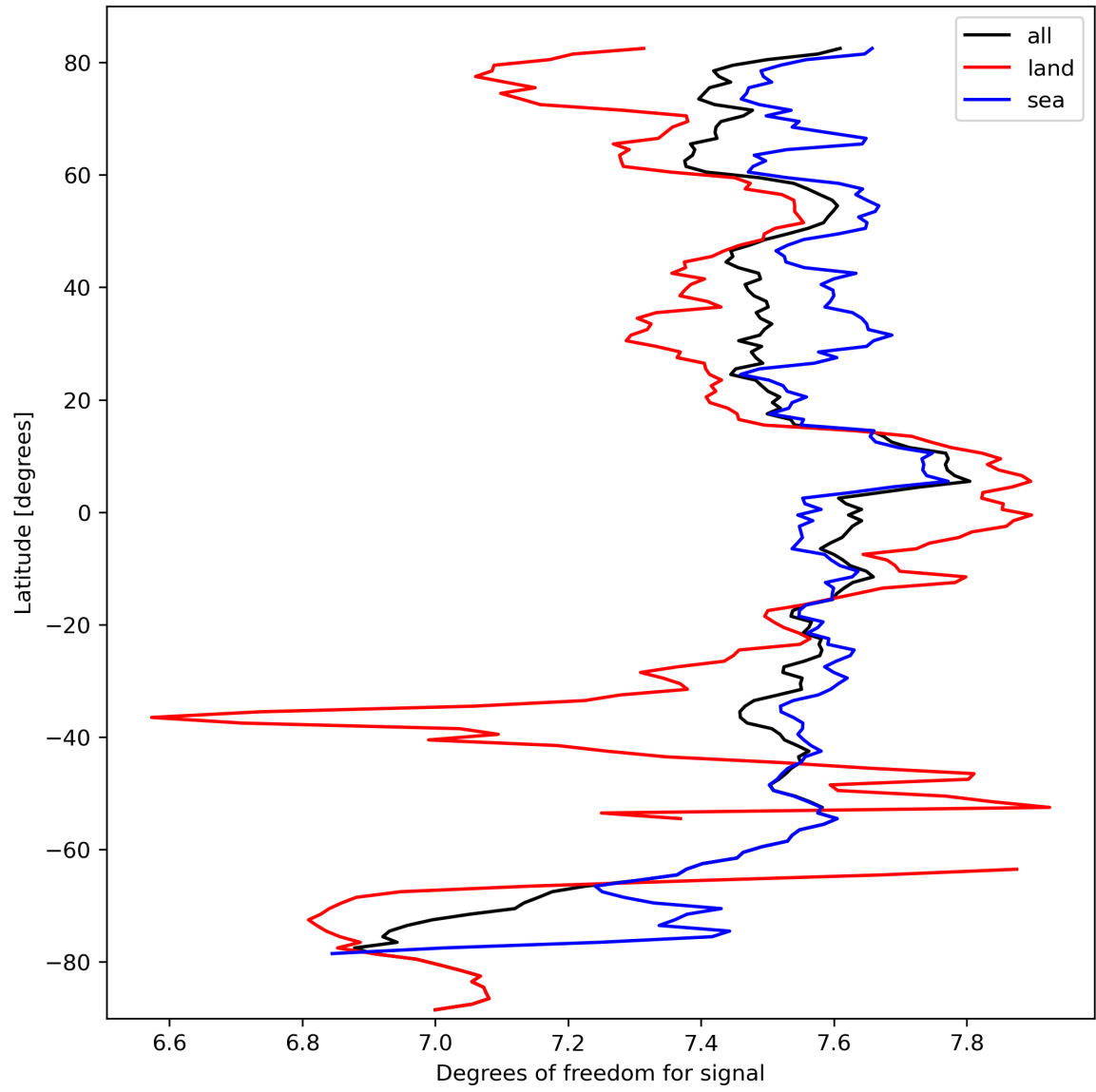
Figure 15: Zonal average of “Degrees of freedom for signal” for 2023-09-29 to 2023-10-01.
