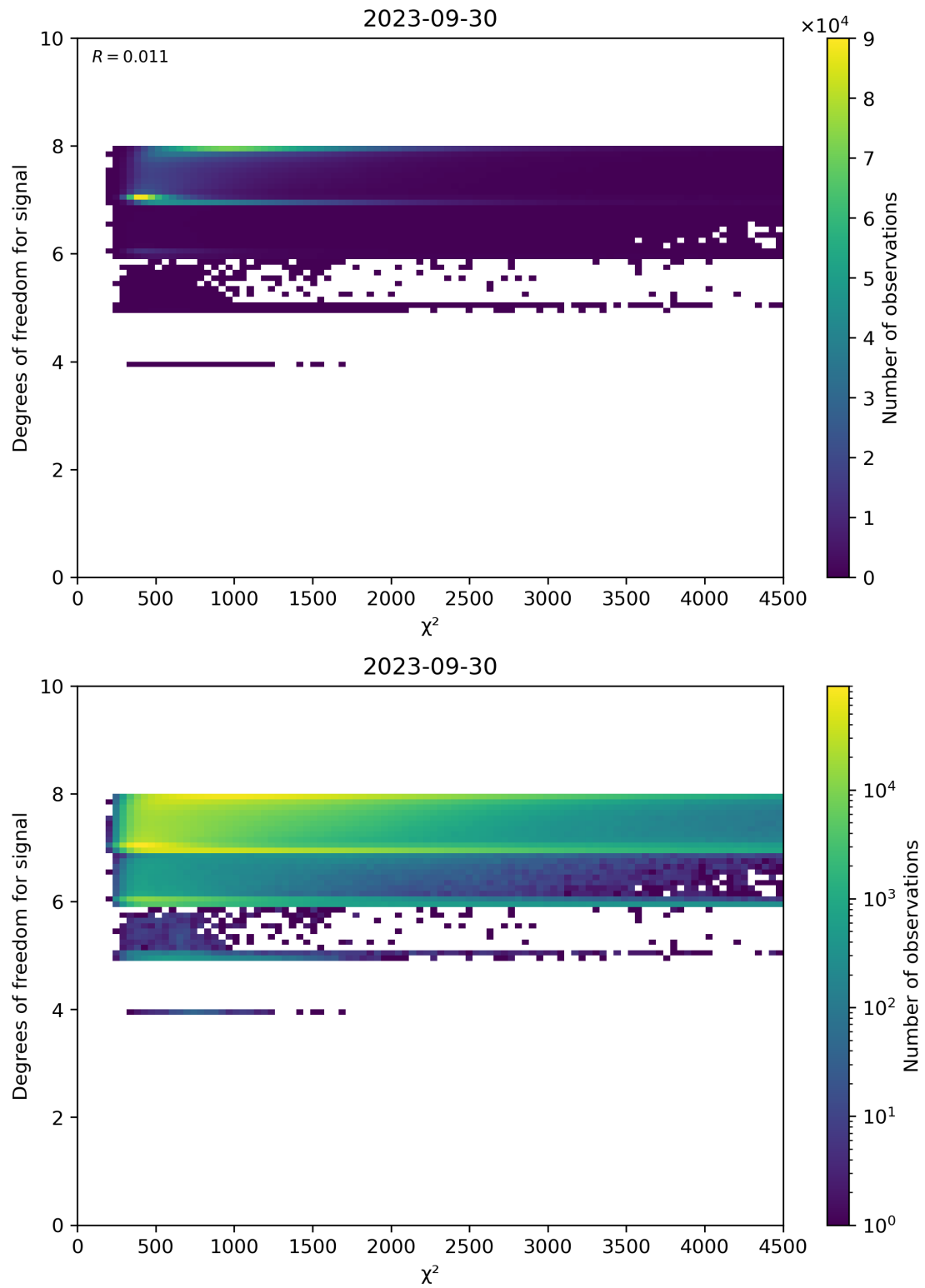
Figure 48: Scatter density plot of “ \chi^2 ” against “Degrees of freedom for signal” for 2023-09-29 to 2023-10-01.
