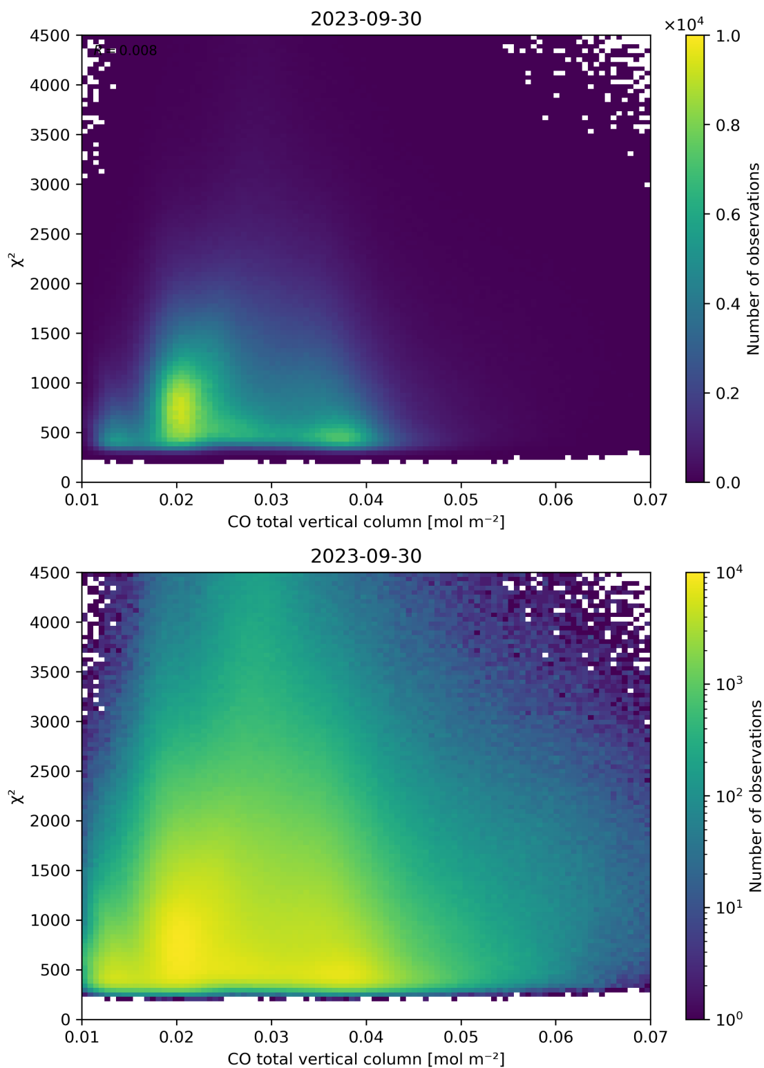
Figure 35: Scatter density plot of “CO total vertical column” against “ \chi^2 ” for 2023-09-29 to 2023-10-01.
