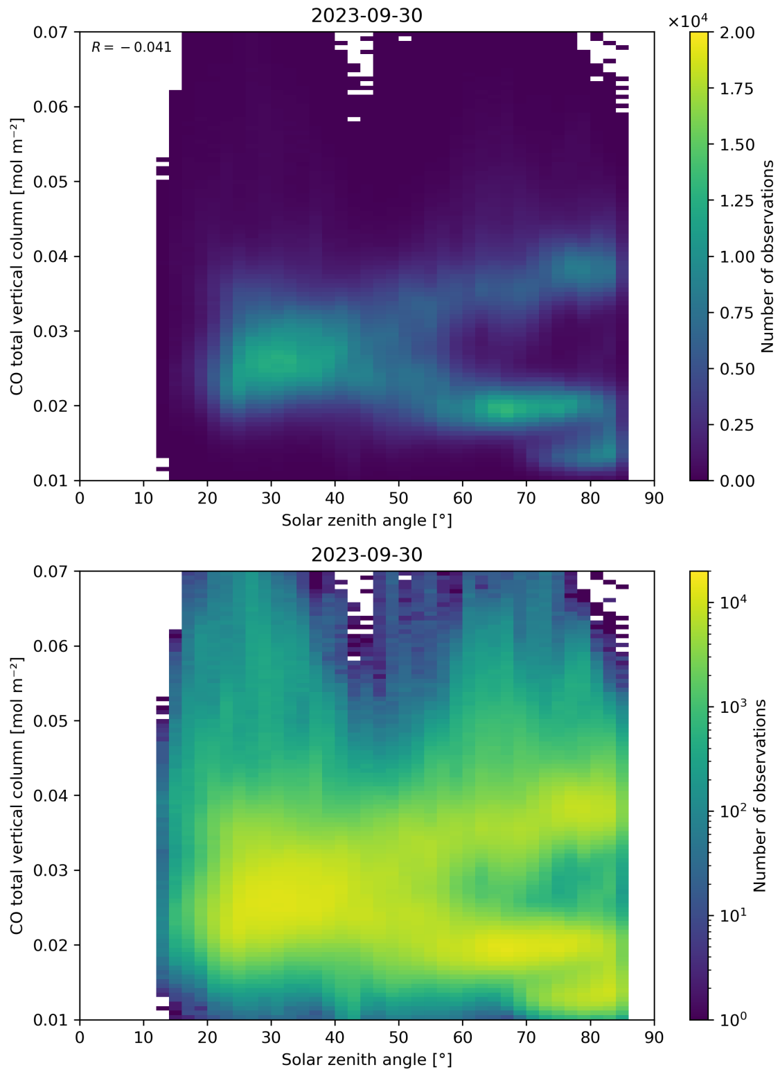
Figure 61: Scatter density plot of “Solar zenith angle” against “CO total vertical column” for 2023-09-29 to 2023-10-01.
