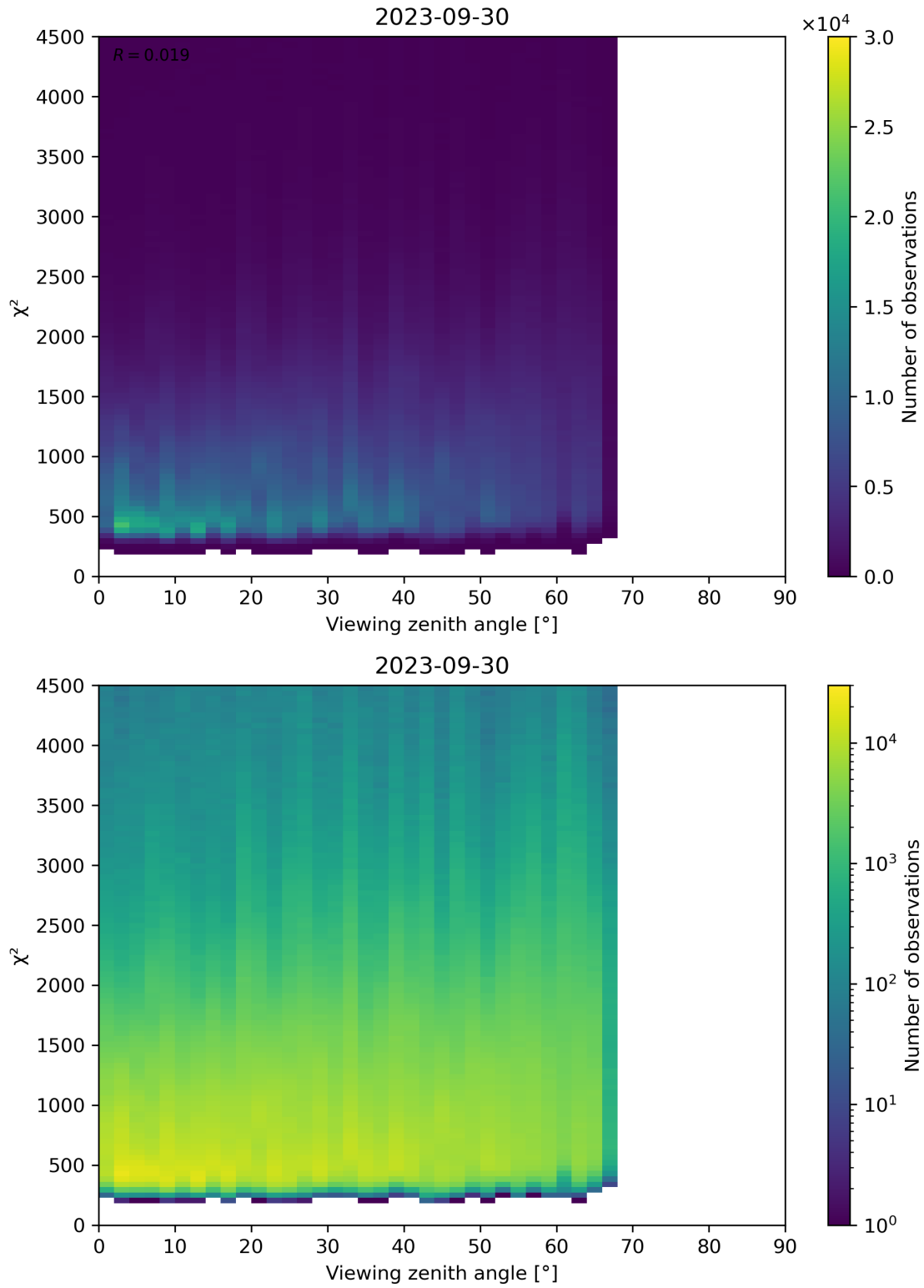
Figure 72: Scatter density plot of “Viewing zenith angle” against “ \chi^2 ” for 2023-09-29 to 2023-10-01.
