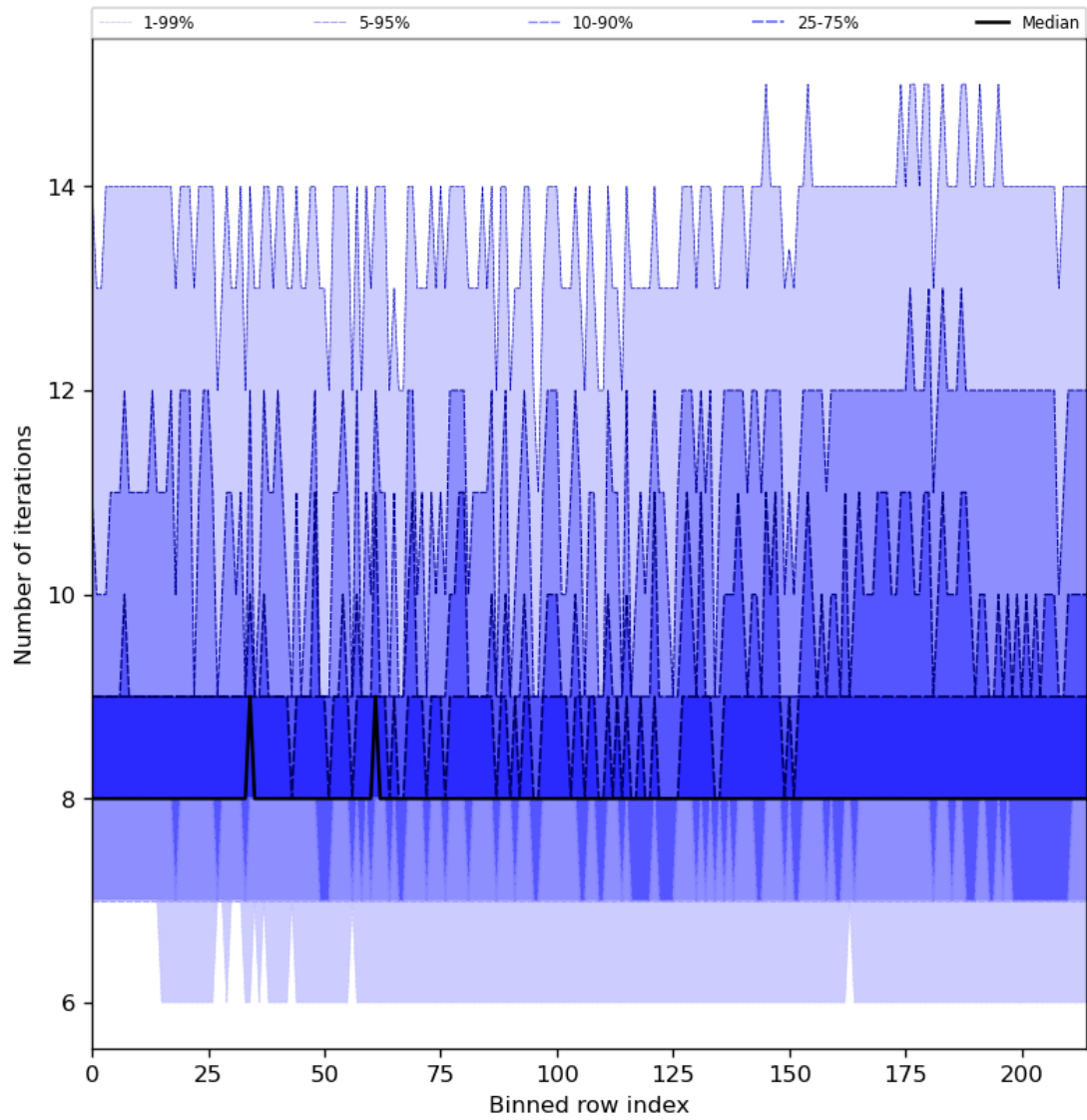
Figure 32: Along track statistics of “Number of iterations” for 2023-09-29 to 2023-10-01
