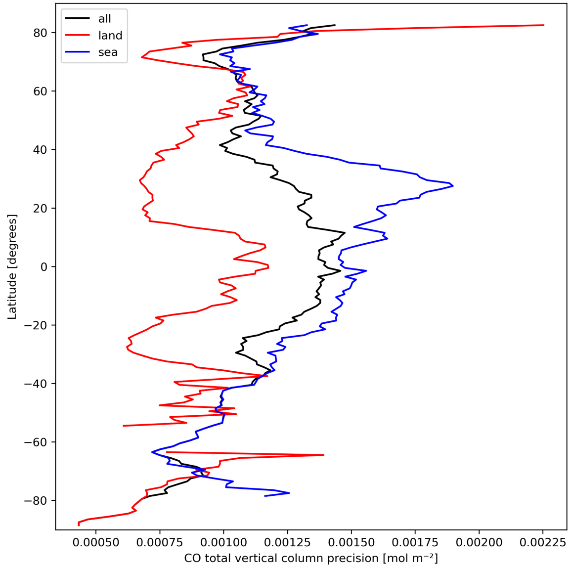
Figure 12: Zonal average of “CO total vertical column precision” for 2023-09-29 to 2023-10-01.
