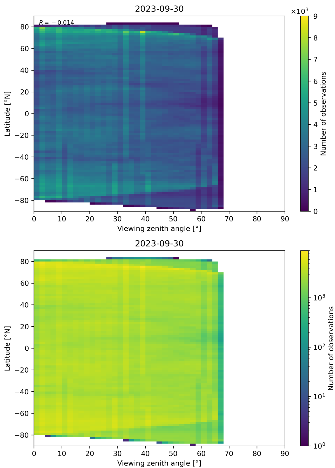
Figure 74: Scatter density plot of “Viewing zenith angle” against “Latitude” for 2023-09-29 to 2023-10-01.
