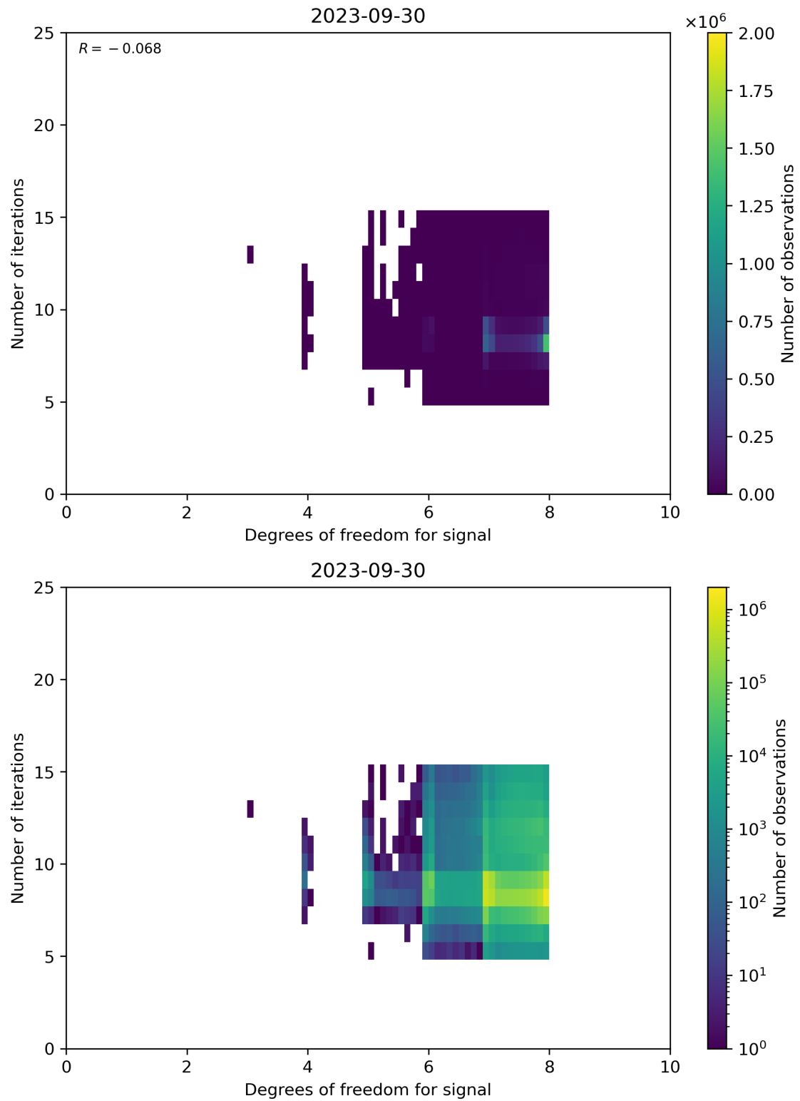
Figure 50: Scatter density plot of “Degrees of freedom for signal” against “Number of iterations” for 2023-09-29 to 2023-10-01.
