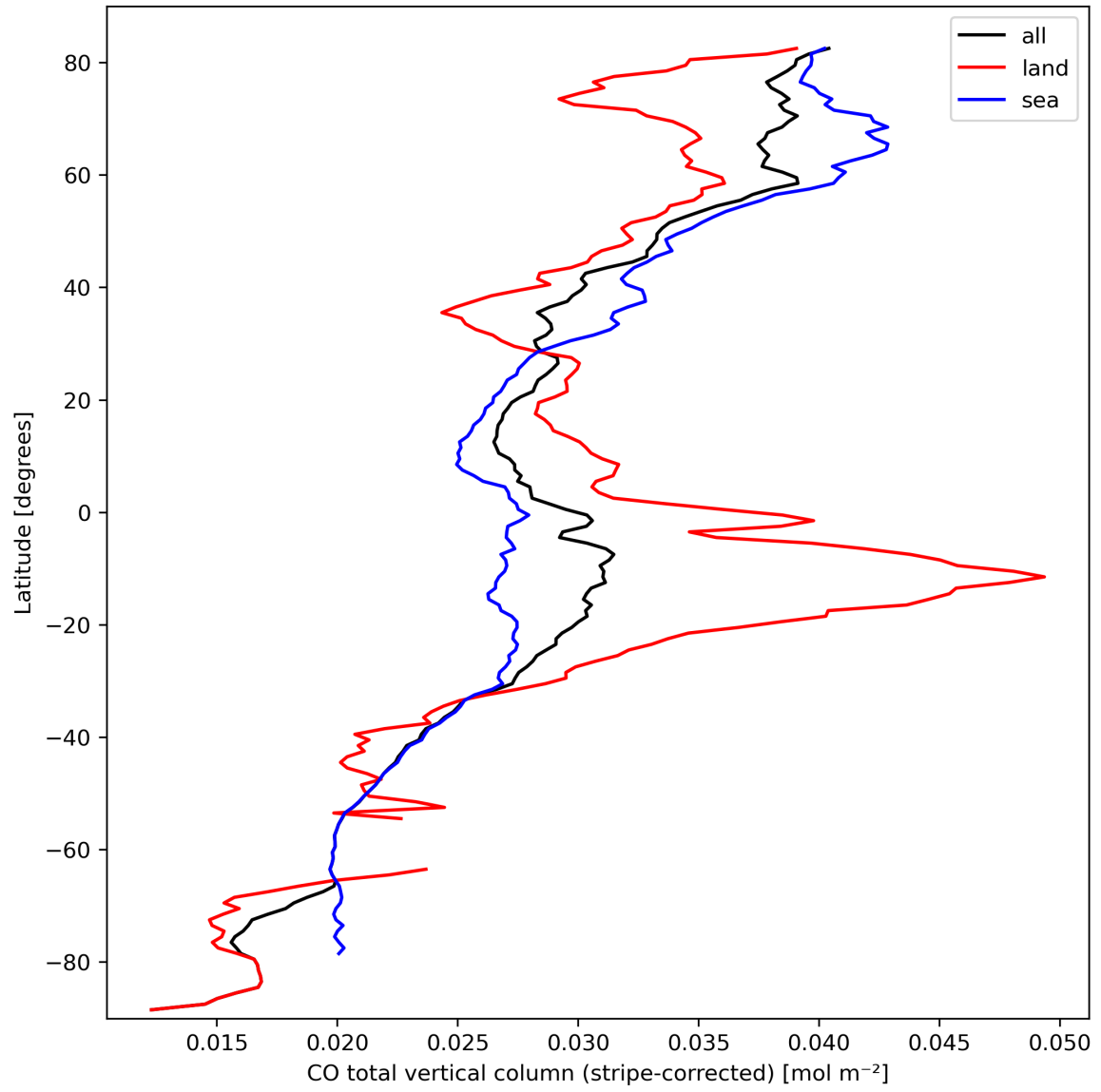
Figure 11: Zonal average of “CO total vertical column (stripe-corrected)” for 2023-09-29 to 2023-10-01.
