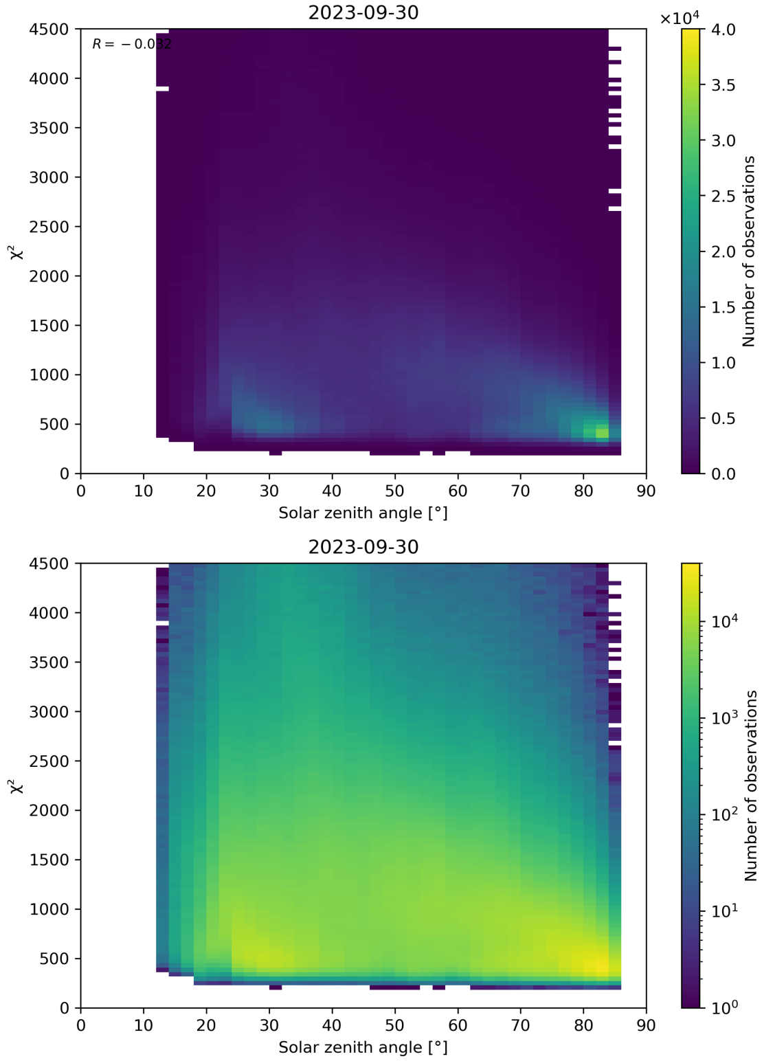
Figure 64: Scatter density plot of “Solar zenith angle” against “ \chi^2 ” for 2023-09-29 to 2023-10-01.
