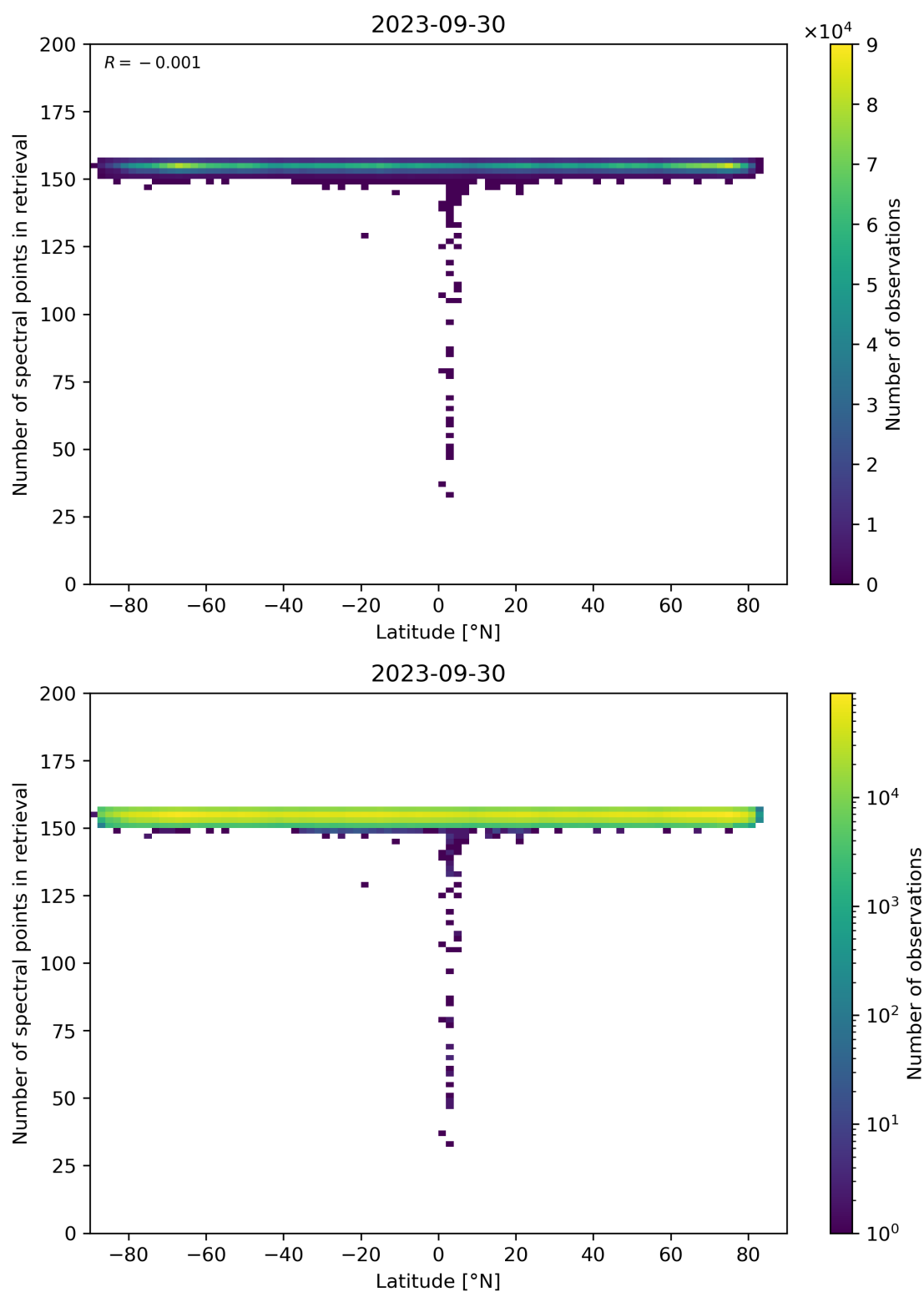
Figure 57: Scatter density plot of “Latitude” against “Number of spectral points in retrieval” for 2023-09-29 to 2023-10-01.
