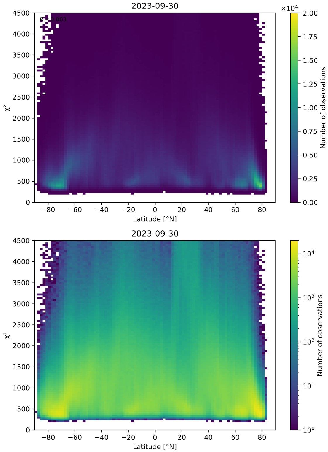
Figure 54: Scatter density plot of “Latitude” against “ \chi^2 ” for 2023-09-29 to 2023-10-01.
