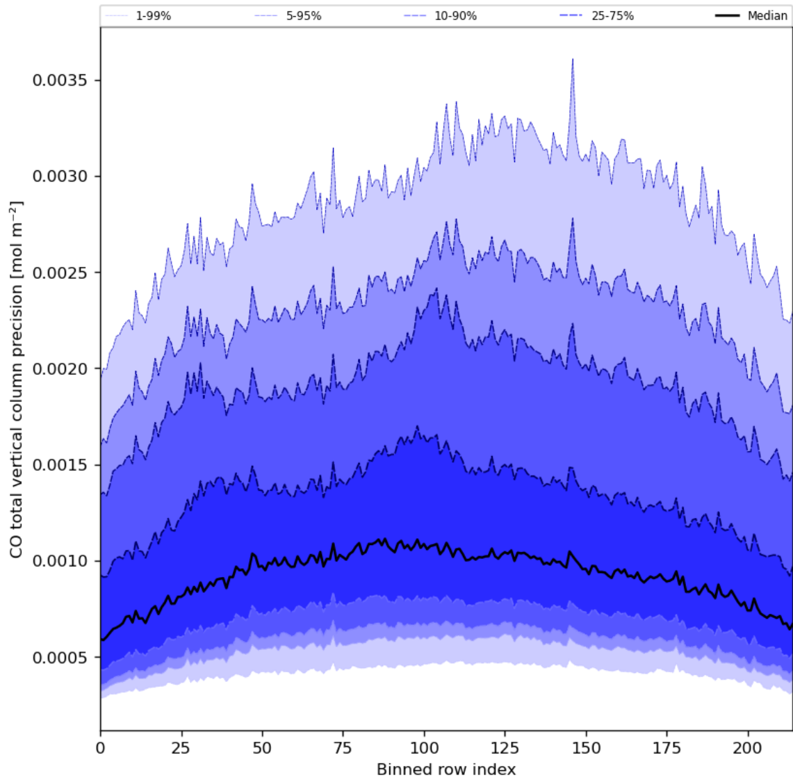
Figure 28: Along track statistics of “CO total vertical column precision” for 2023-09-29 to 2023-10-01
