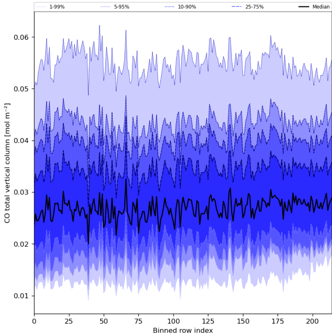
Figure 26: Along track statistics of “CO total vertical column” for 2023-09-29 to 2023-10-01
