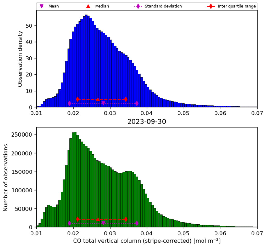
Figure 19: Histogram of “CO total vertical column (stripe-corrected)” for 2023-09-29 to 2023-10-01
