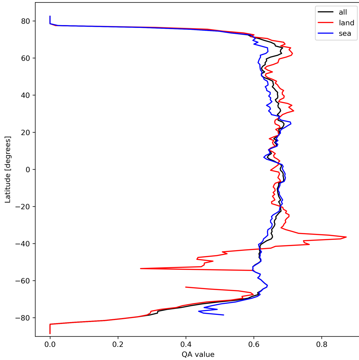
Figure 9: Zonal average of “QA value” for 2023-09-29 to 2023-10-01.
