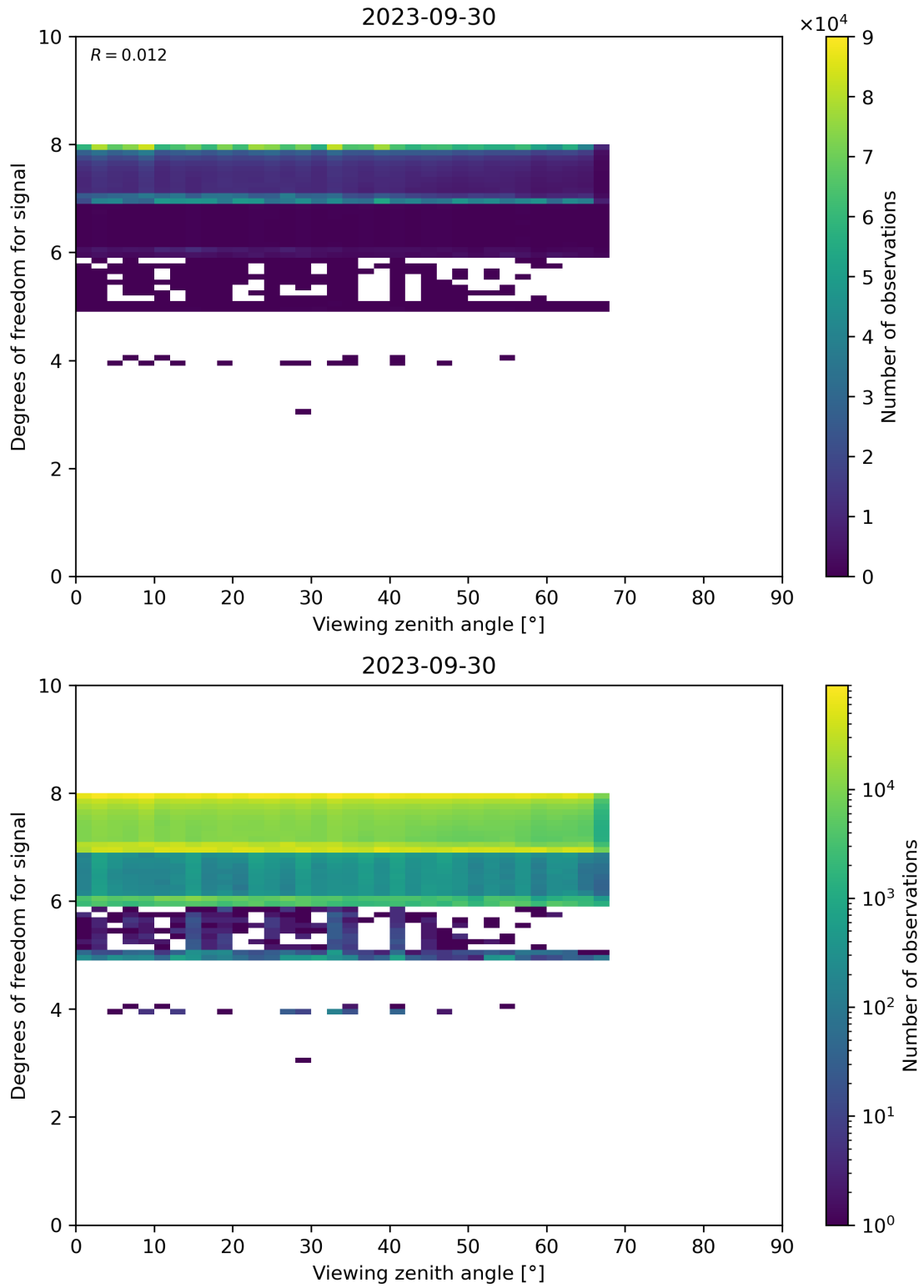
Figure 73: Scatter density plot of “Viewing zenith angle” against “Degrees of freedom for signal” for 2023-09-29 to 2023-10-01.
