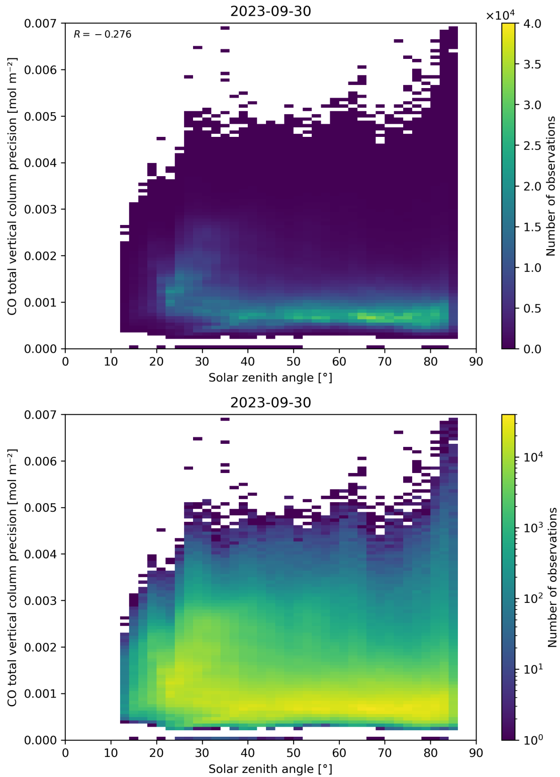
Figure 63: Scatter density plot of “Solar zenith angle” against “CO total vertical column precision” for 2023-09-29 to 2023-10-01.
