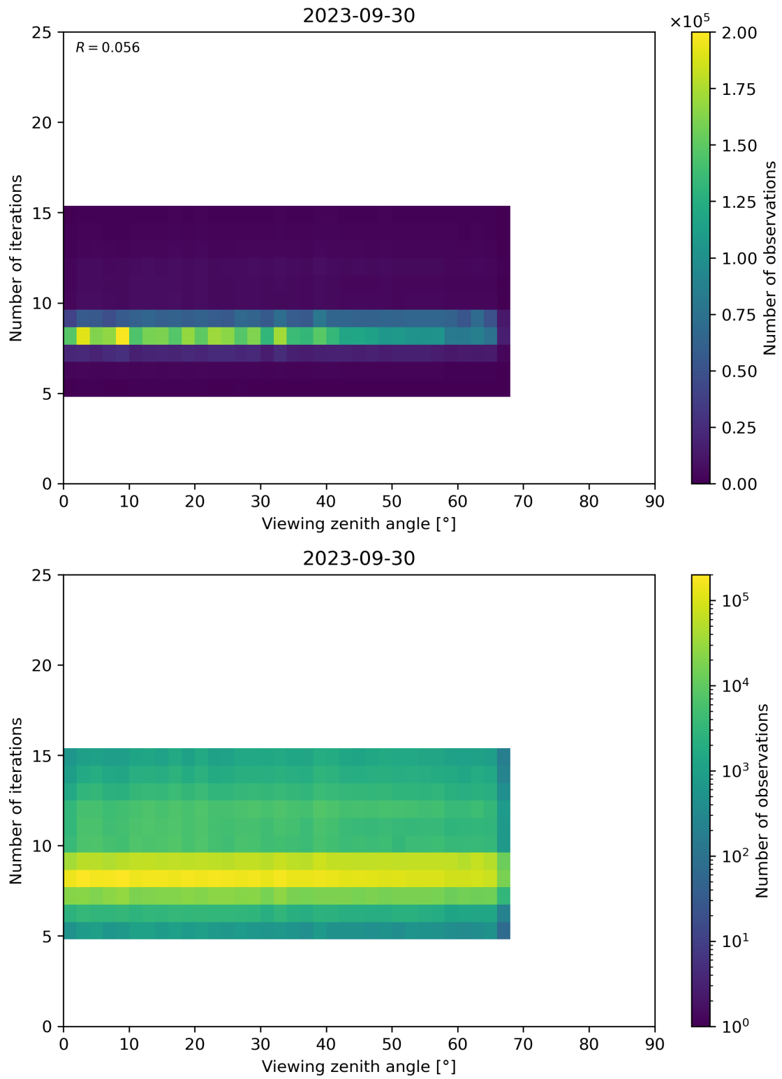
Figure 75: Scatter density plot of “Viewing zenith angle” against “Number of iterations” for 2023-09-29 to 2023-10-01.
