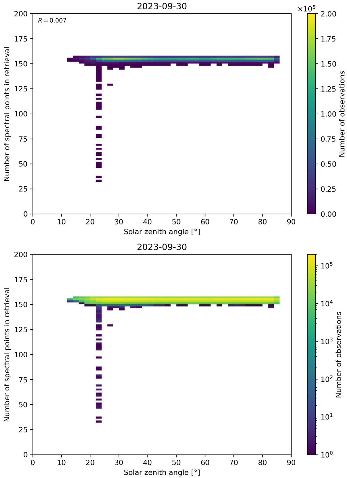
Figure 68: Scatter density plot of “Solar zenith angle” against “Number of spectral points in retrieval” for 2023-09-29 to 2023-10-01.
