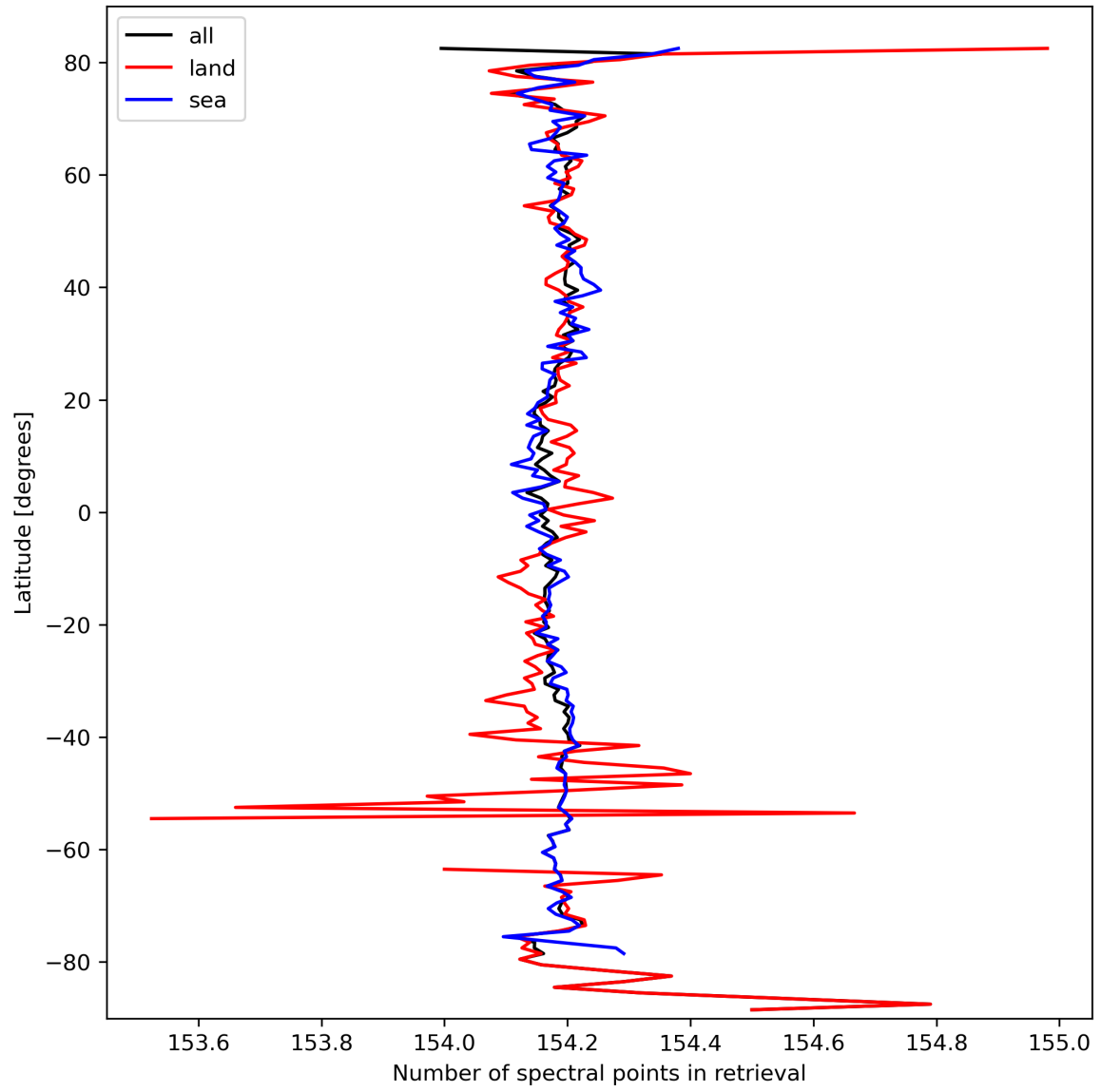
Figure 13: Zonal average of “Number of spectral points in retrieval” for 2023-09-29 to 2023-10-01.
