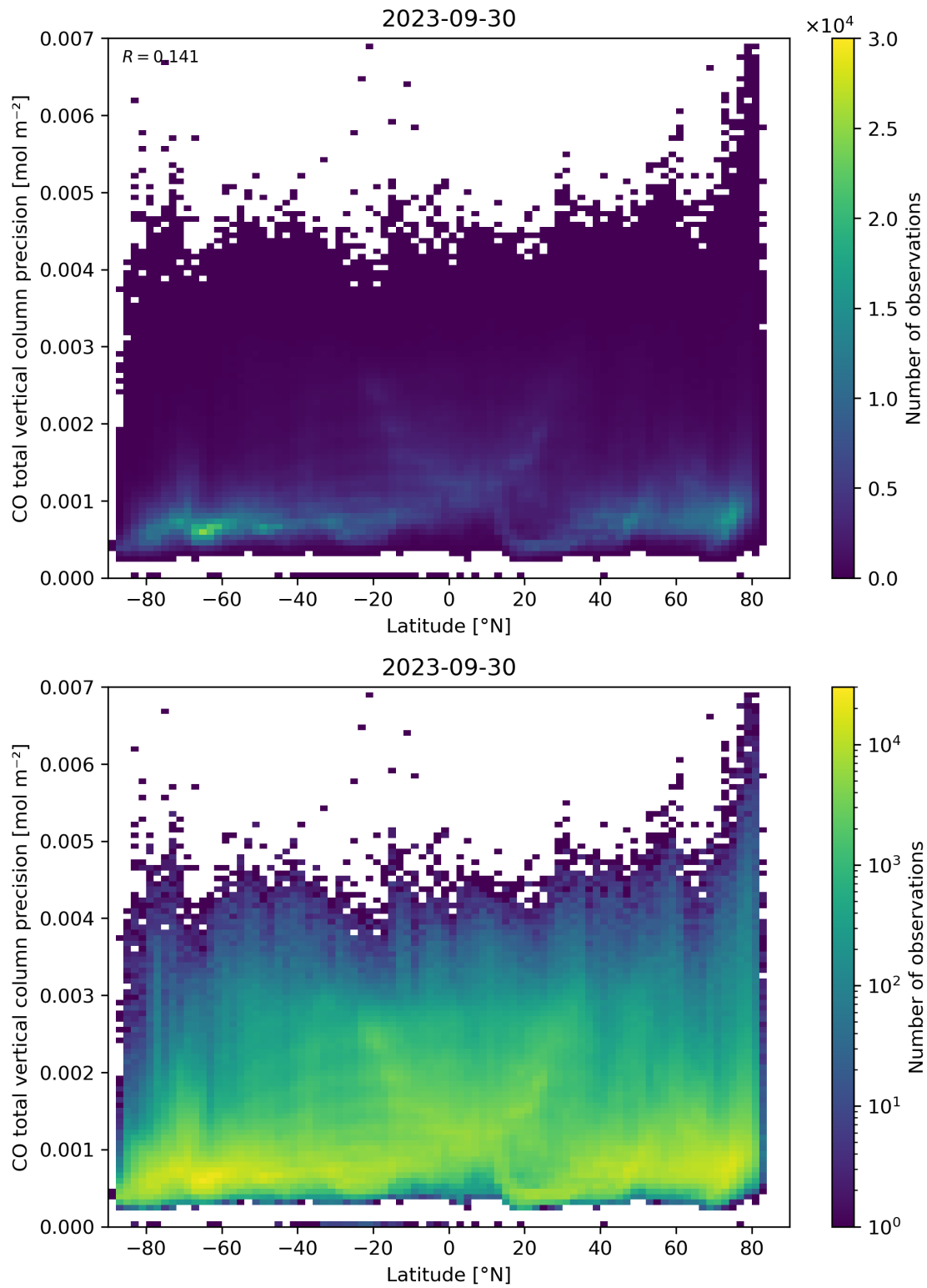
Figure 53: Scatter density plot of “Latitude” against “CO total vertical column precision” for 2023-09-29 to 2023-10-01.
