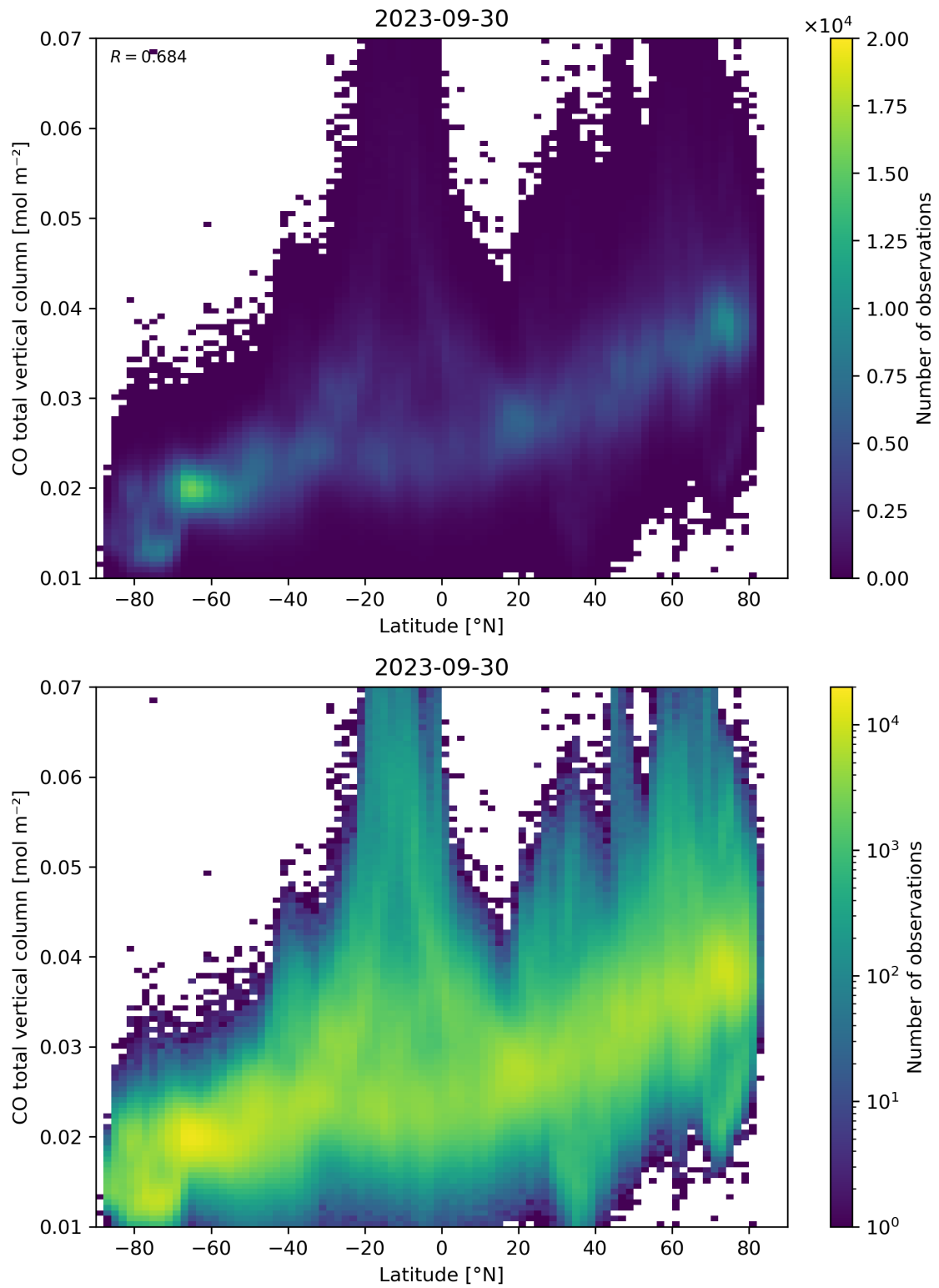
Figure 51: Scatter density plot of “Latitude” against “CO total vertical column” for 2023-09-29 to 2023-10-01.
