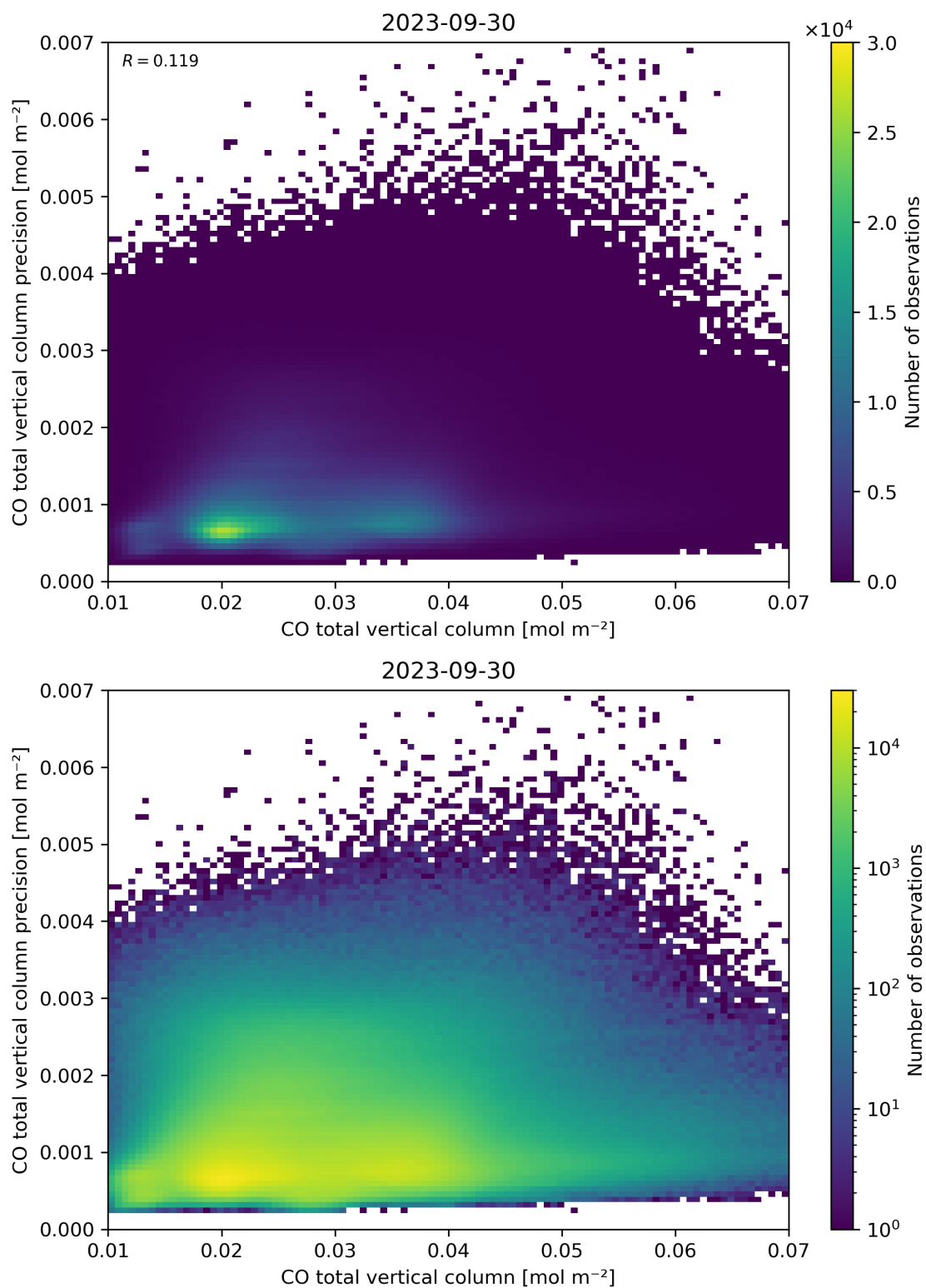
Figure 34: Scatter density plot of “CO total vertical column” against “CO total vertical column precision” for 2023-09-29 to 2023-10-01.
