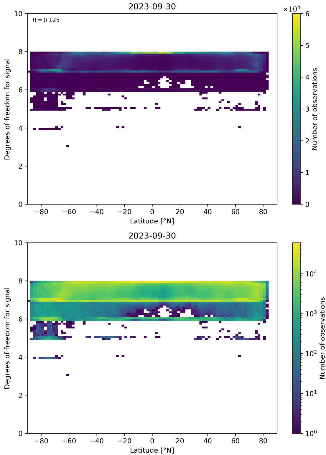
Figure 55: Scatter density plot of “Latitude” against “Degrees of freedom for signal” for 2023-09-29 to 2023-10-01.
