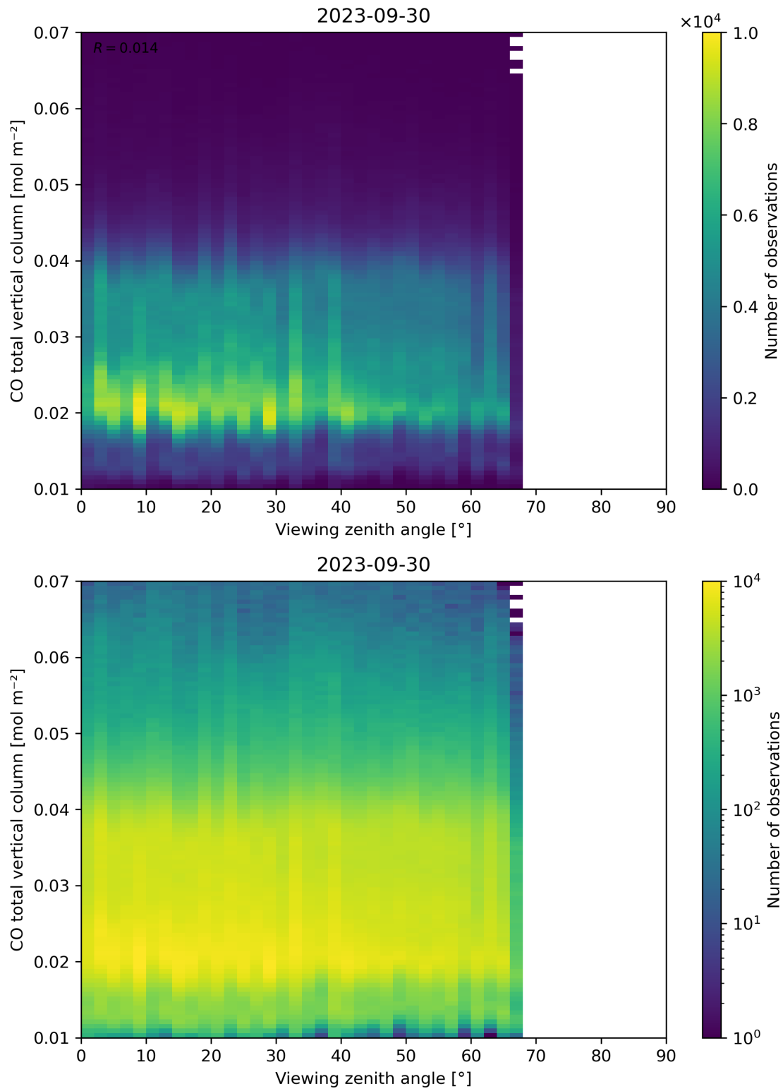
Figure 69: Scatter density plot of “Viewing zenith angle” against “CO total vertical column” for 2023-09-29 to 2023-10-01.
