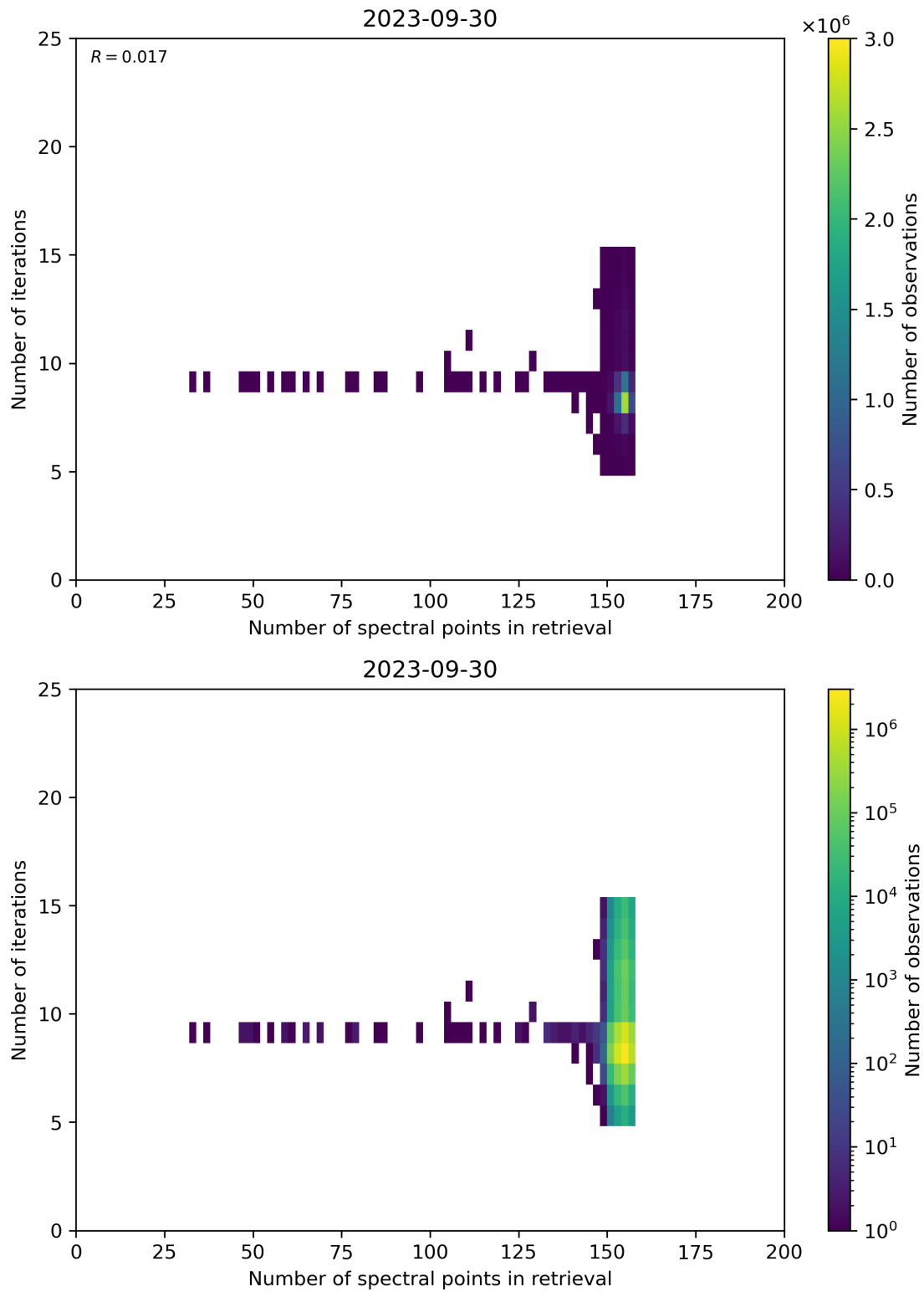
Figure 60: Scatter density plot of “Number of spectral points in retrieval” against “Number of iterations” for 2023-09-29 to 2023-10-01.
