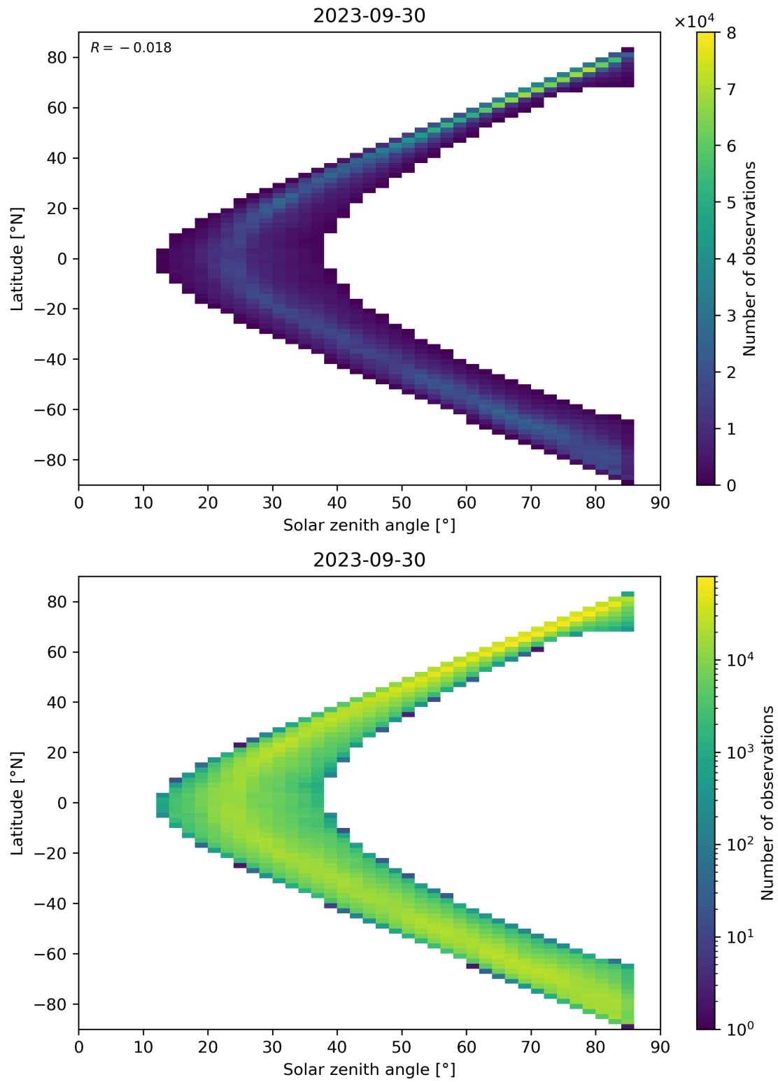
Figure 66: Scatter density plot of “Solar zenith angle” against “Latitude” for 2023-09-29 to 2023-10-01.
