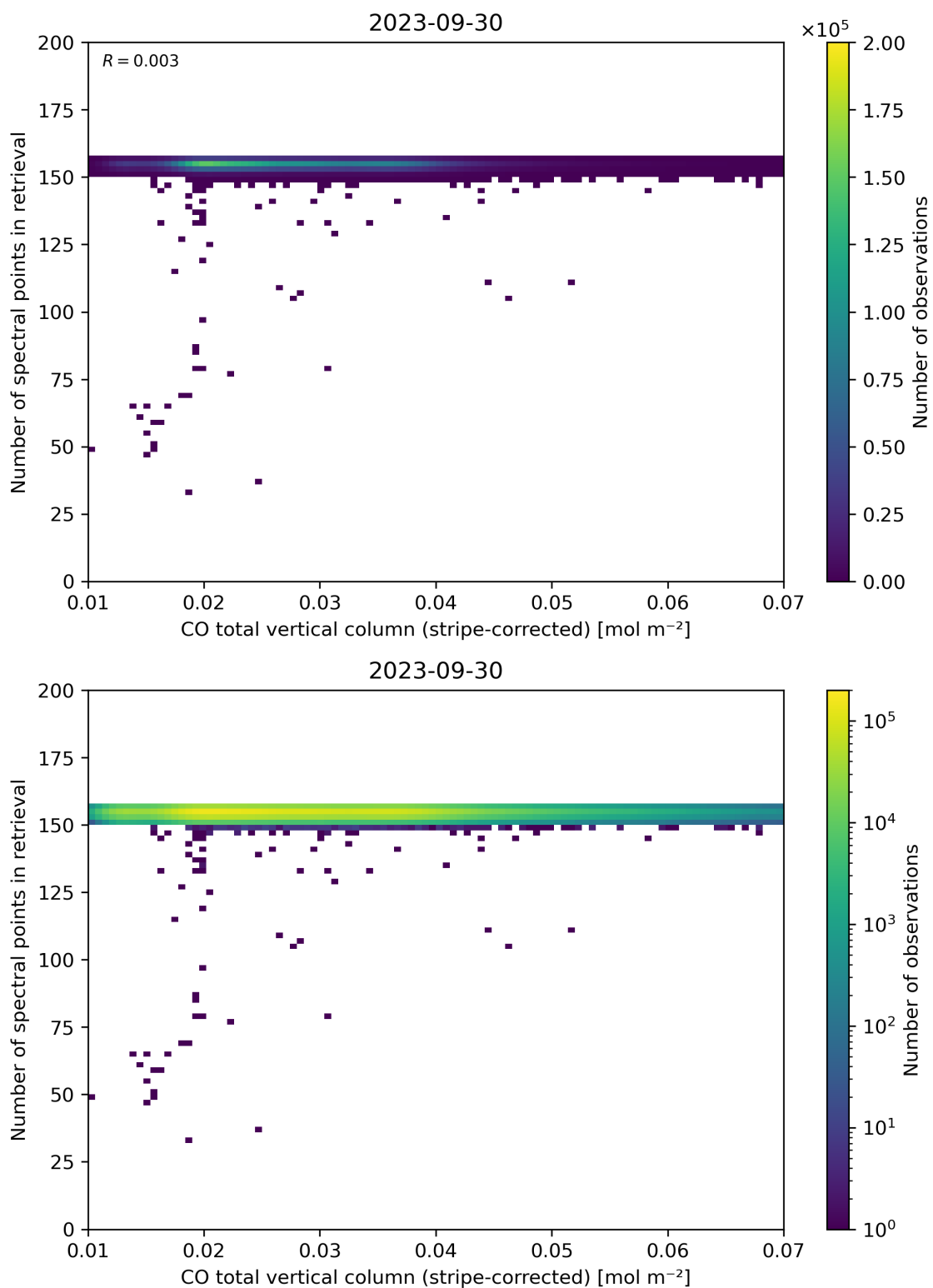
Figure 40: Scatter density plot of “CO total vertical column (stripe-corrected)” against “Number of spectral points in retrieval” for 2023-09-29 to 2023-10-01.
