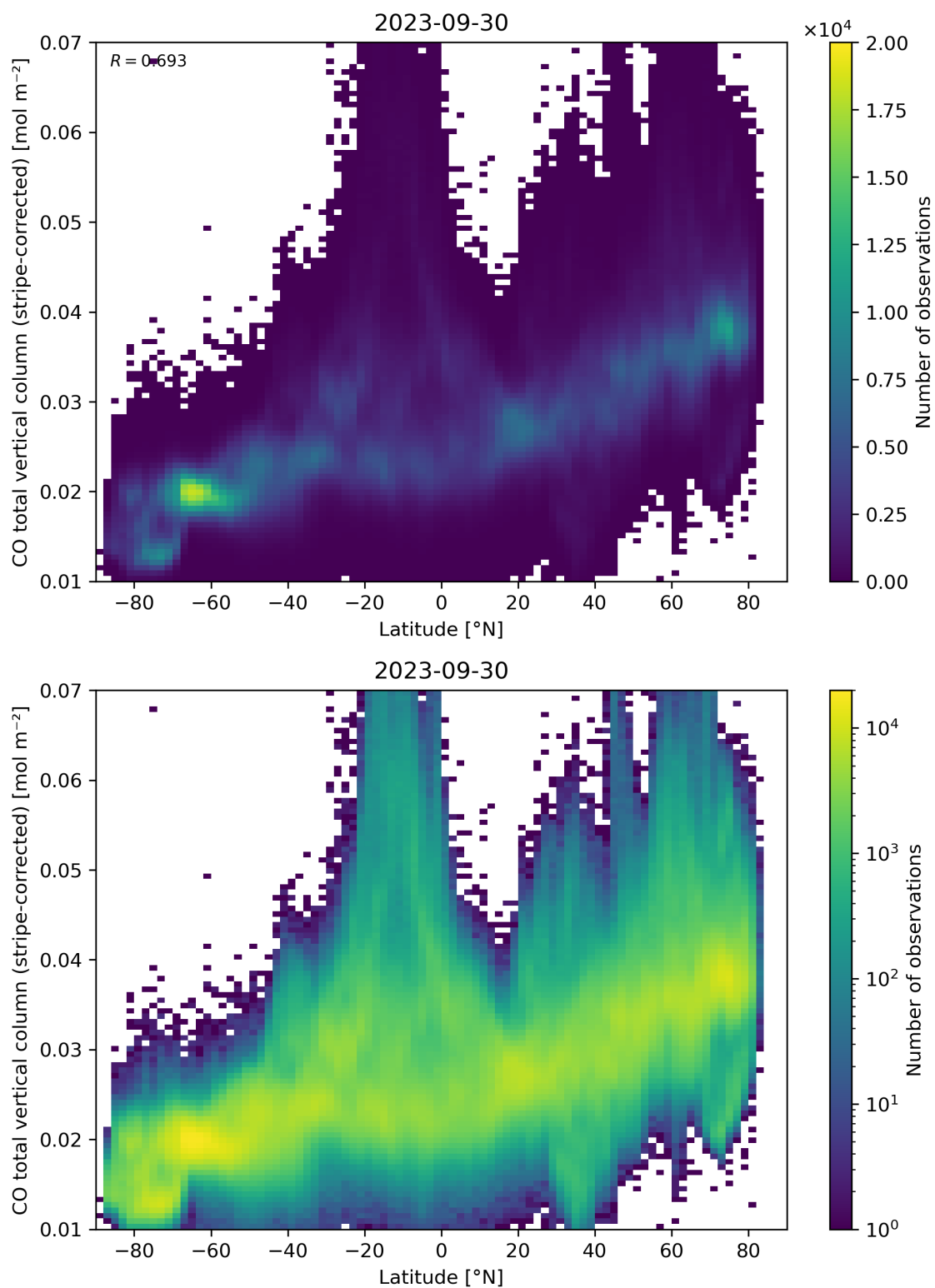
Figure 52: Scatter density plot of “Latitude” against “CO total vertical column (stripe-corrected)” for 2023-09-29 to 2023-10-01.
