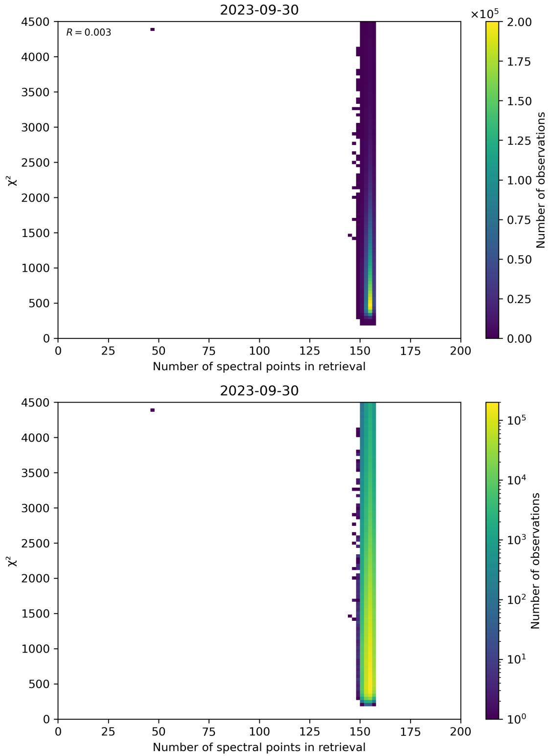
Figure 58: Scatter density plot of “Number of spectral points in retrieval” against “ \chi^2 ” for 2023-09-29 to 2023-10-01.
