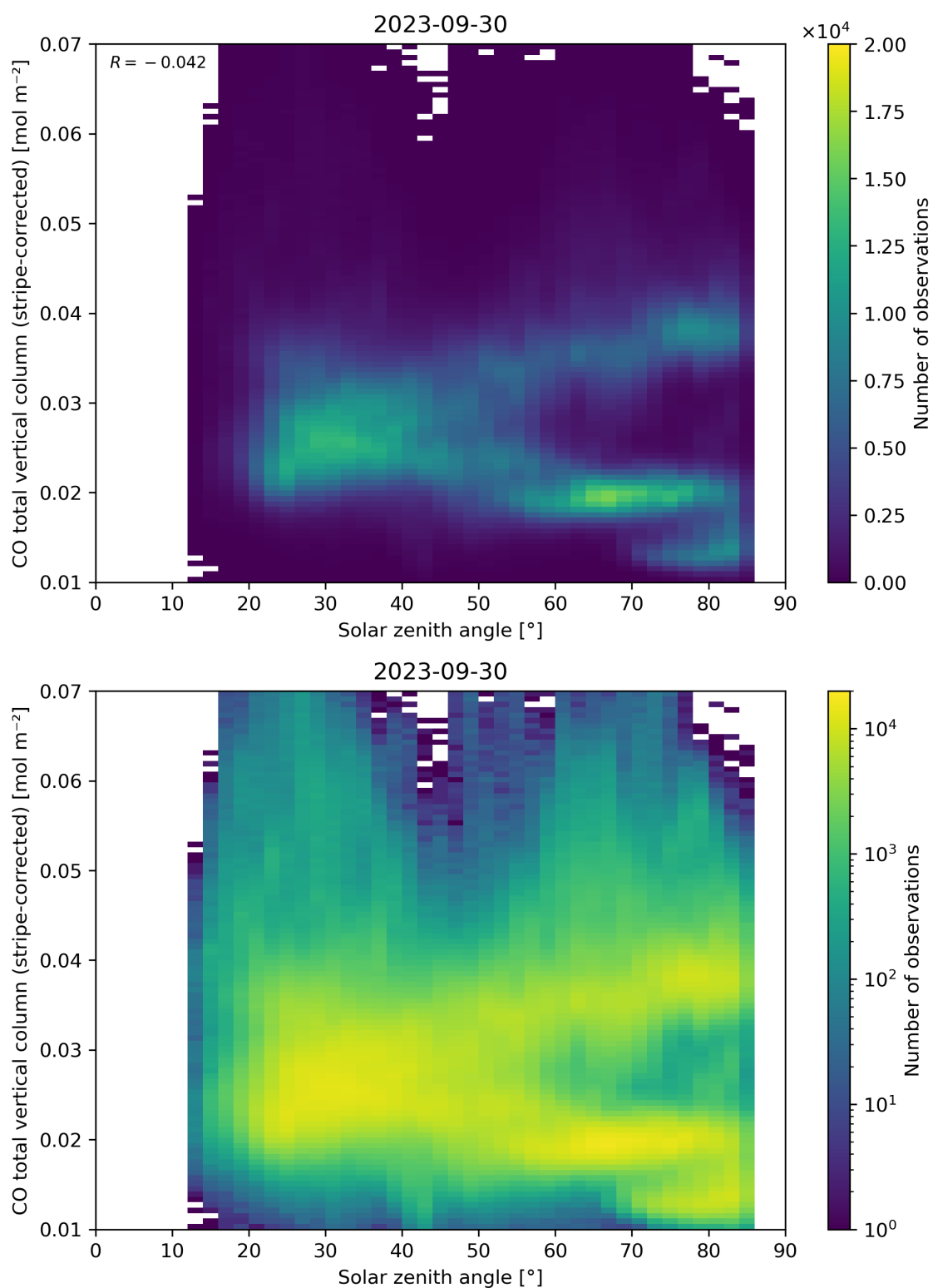
Figure 62: Scatter density plot of “Solar zenith angle” against “CO total vertical column (stripe-corrected)” for 2023-09-29 to 2023-10-01.
