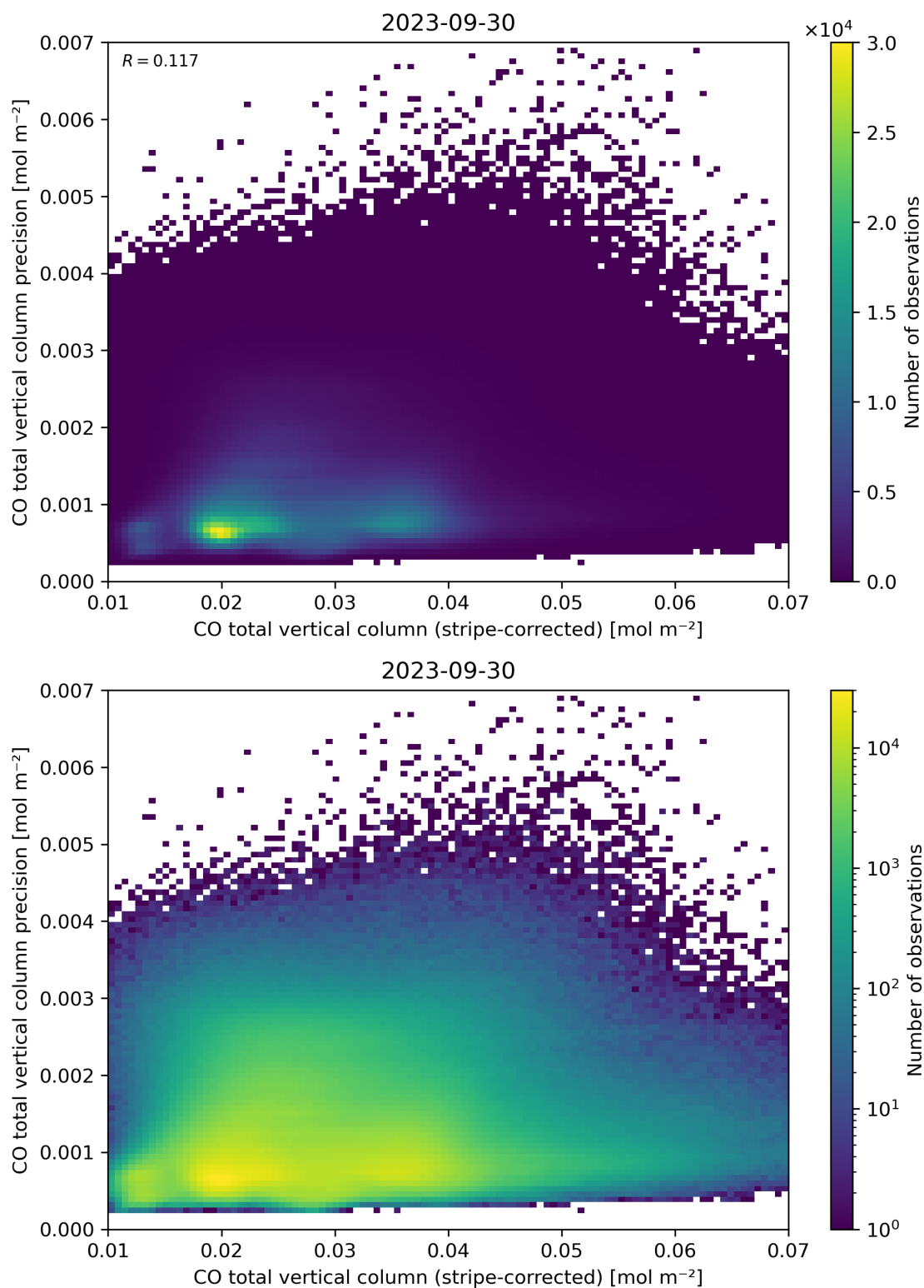
Figure 36: Scatter density plot of “CO total vertical column (stripe-corrected)” against “CO total vertical column precision” for 2023-09-29 to 2023-10-01.
