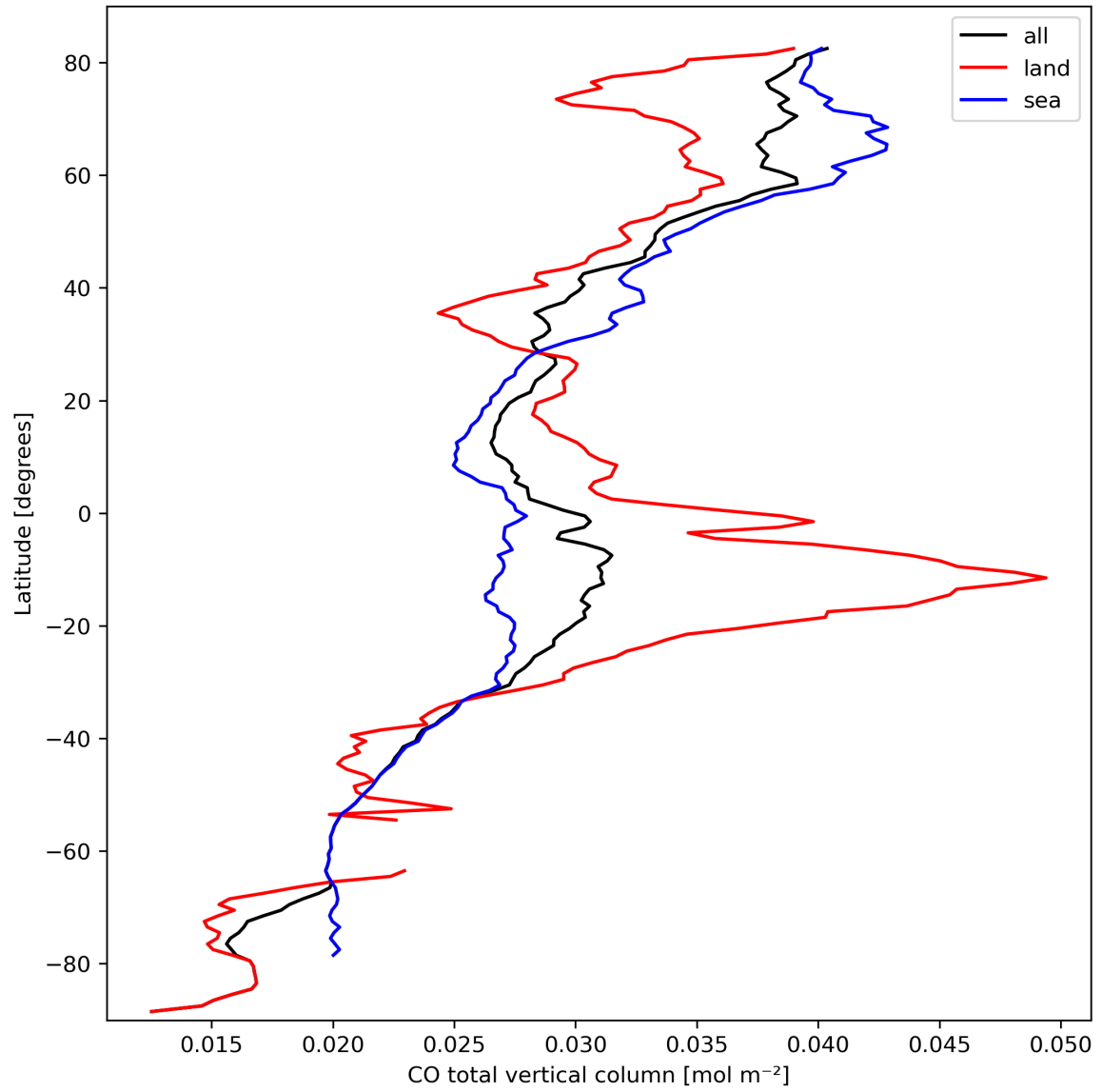
Figure 10: Zonal average of “CO total vertical column” for 2023-09-29 to 2023-10-01.
