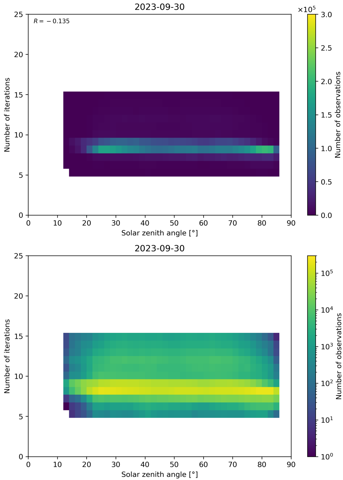
Figure 67: Scatter density plot of “Solar zenith angle” against “Number of iterations” for 2023-09-29 to 2023-10-01.
