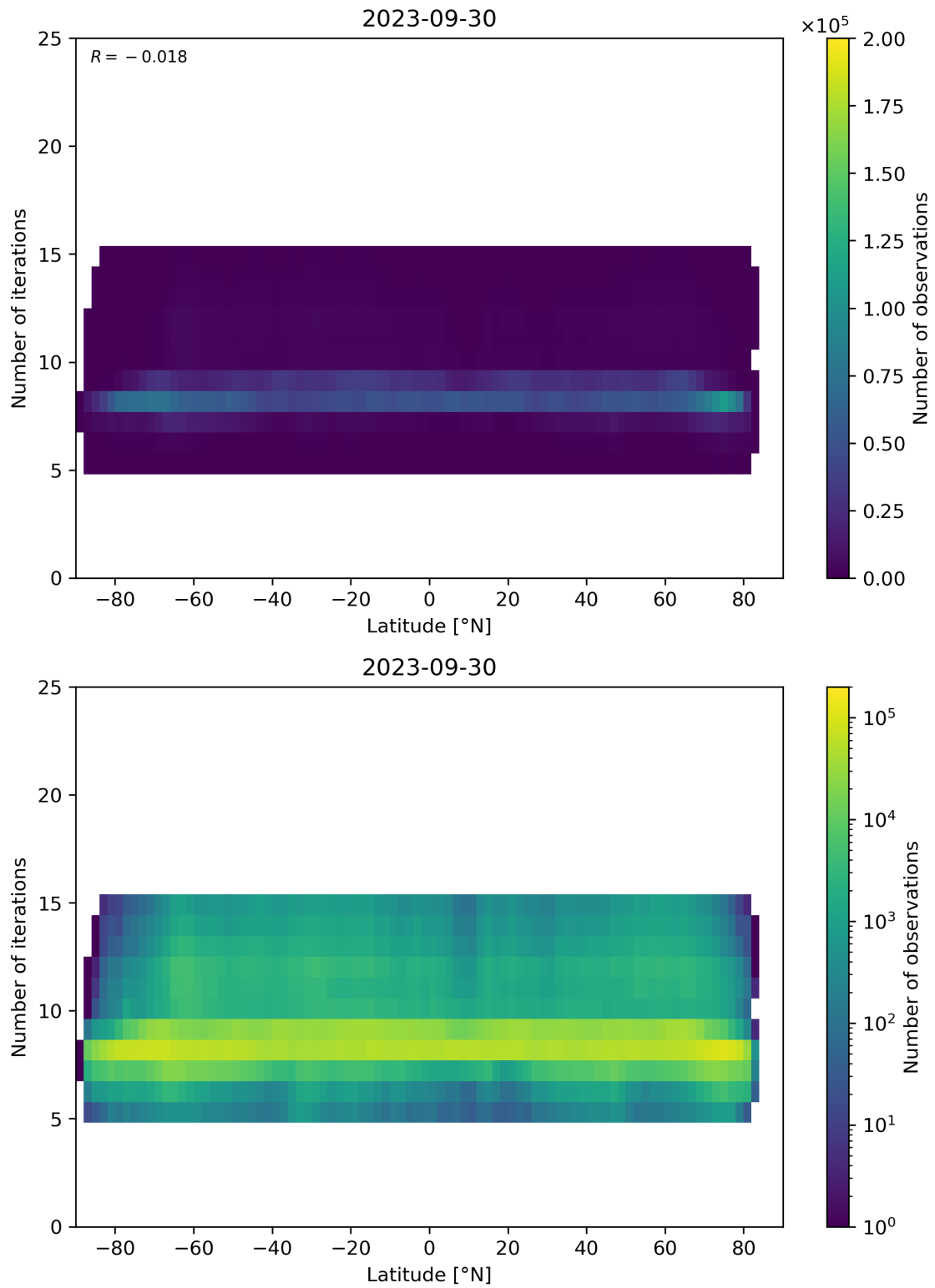
Figure 56: Scatter density plot of “Latitude” against “Number of iterations” for 2023-09-29 to 2023-10-01.
