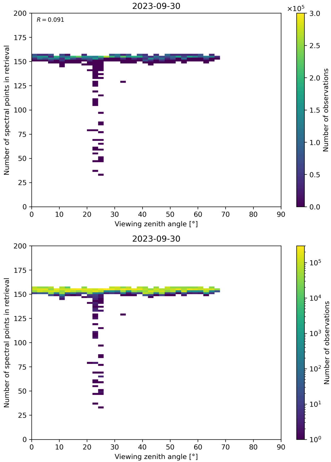
Figure 76: Scatter density plot of “Viewing zenith angle” against “Number of spectral points in retrieval” for 2023-09-29 to 2023-10-01.
