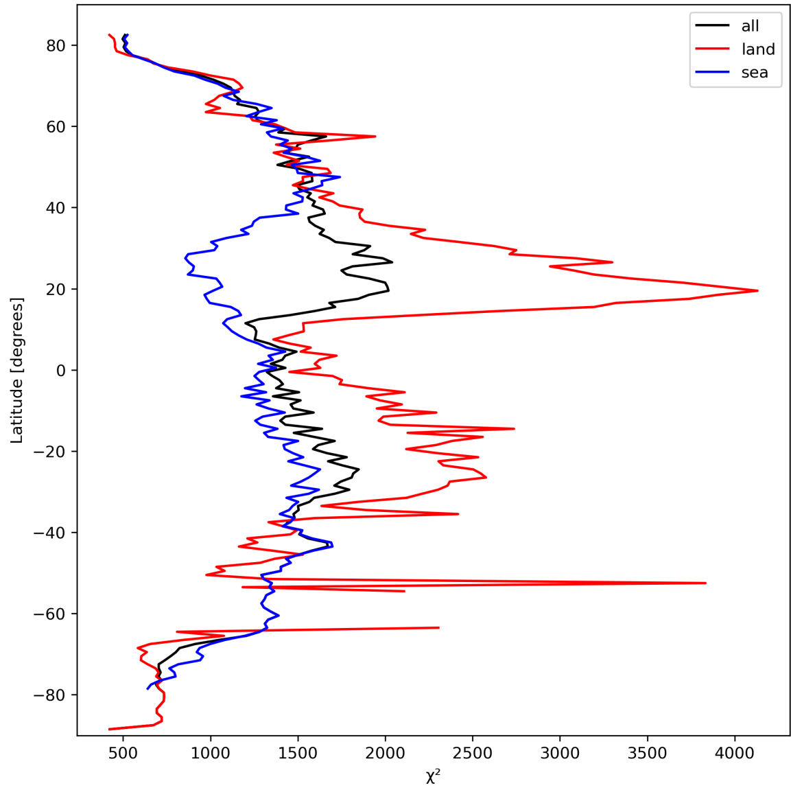
Figure 14: Zonal average of “ \chi^2 ” for 2023-09-29 to 2023-10-01.
