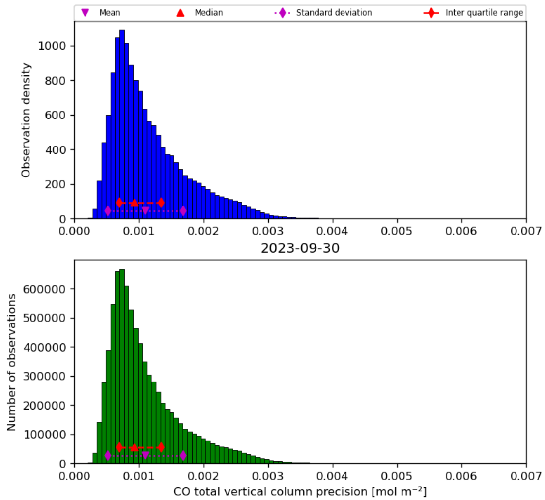
Figure 20: Histogram of “CO total vertical column precision” for 2023-09-29 to 2023-10-01
