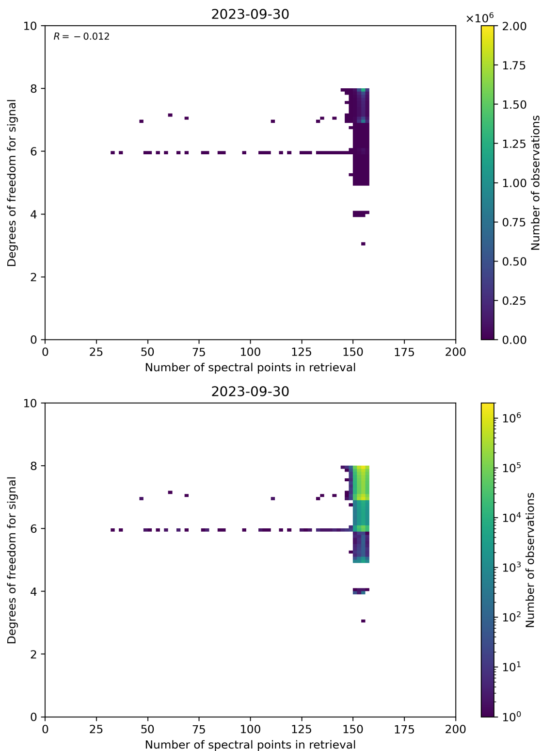
Figure 59: Scatter density plot of “Number of spectral points in retrieval” against “Degrees of freedom for signal” for 2023-09-29 to 2023-10-01.
