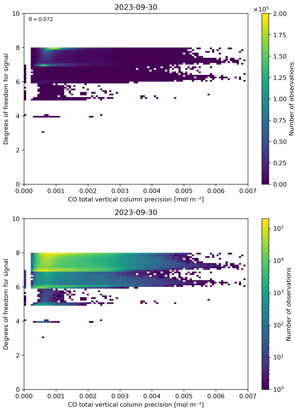
Figure 45: Scatter density plot of “CO total vertical column precision” against “Degrees of freedom for signal” for 2023-09-29 to 2023-10-01.
