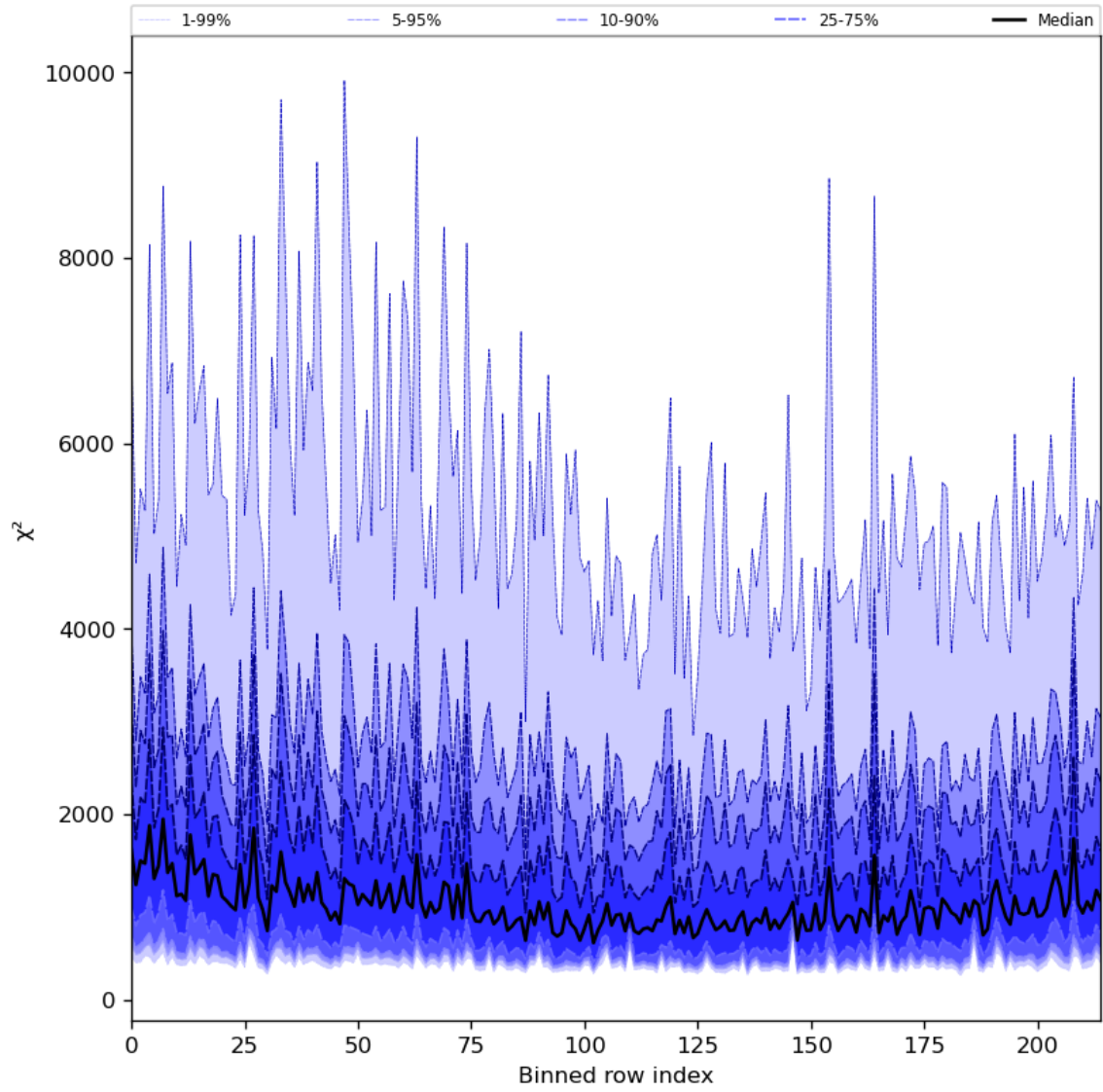
Figure 30: Along track statistics of “ \chi^2 ” for 2023-09-29 to 2023-10-01
