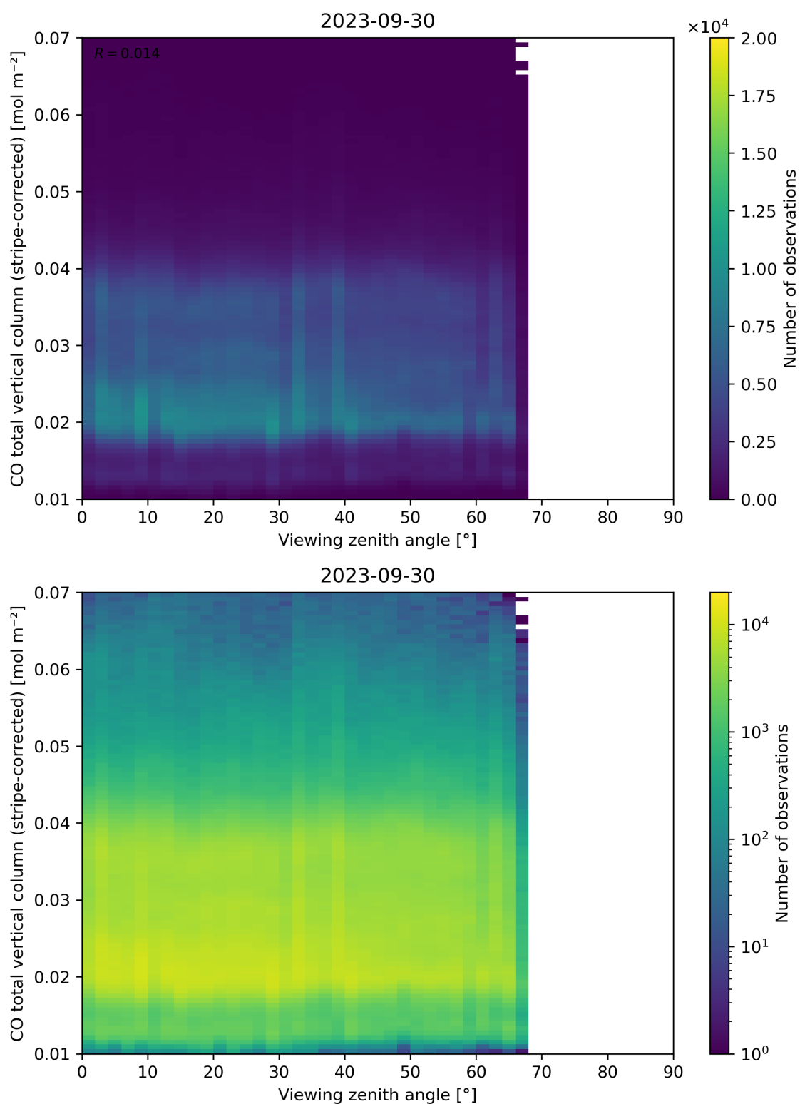
Figure 70: Scatter density plot of “Viewing zenith angle” against “CO total vertical column (stripe-corrected)” for 2023-09-29 to 2023-10-01.
