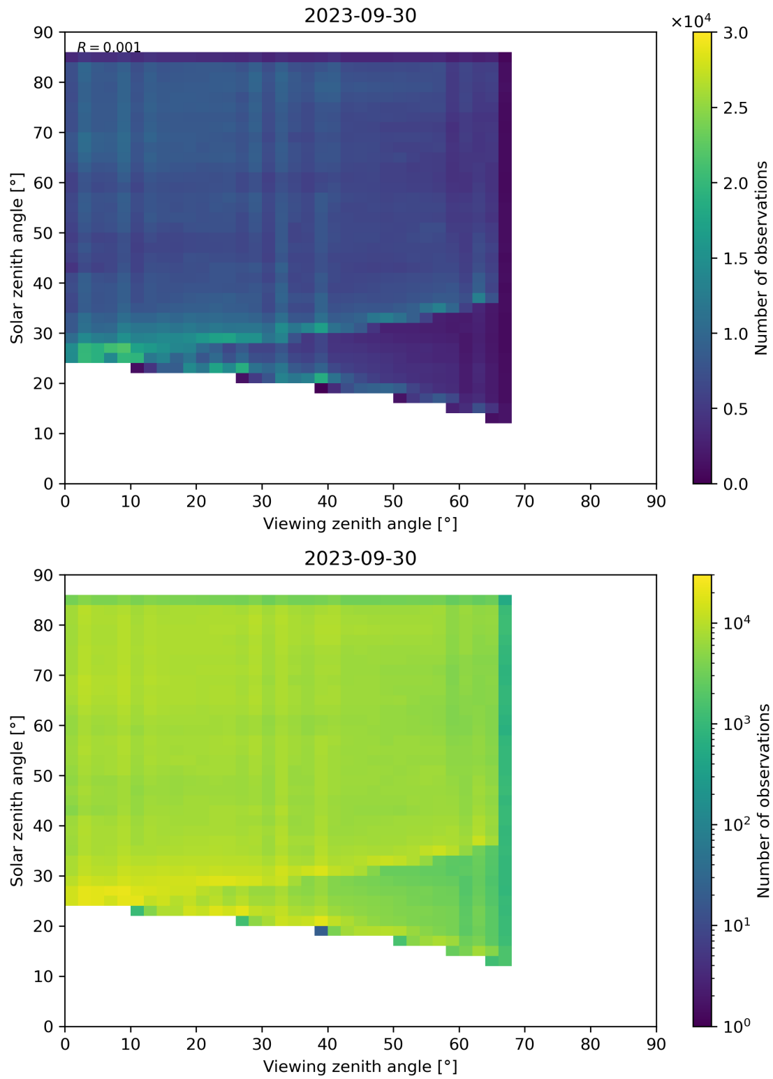
Figure 77: Scatter density plot of “Viewing zenith angle” against “Solar zenith angle” for 2023-09-29 to 2023-10-01.
