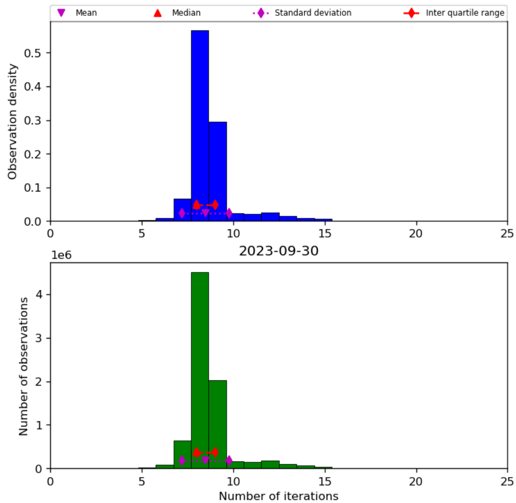
Figure 24: Histogram of “Number of iterations” for 2023-09-29 to 2023-10-01
