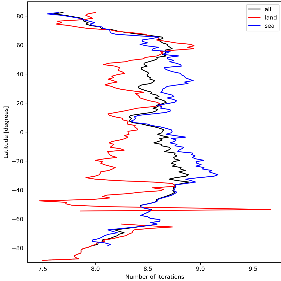
Figure 16: Zonal average of “Number of iterations” for 2023-09-29 to 2023-10-01.
