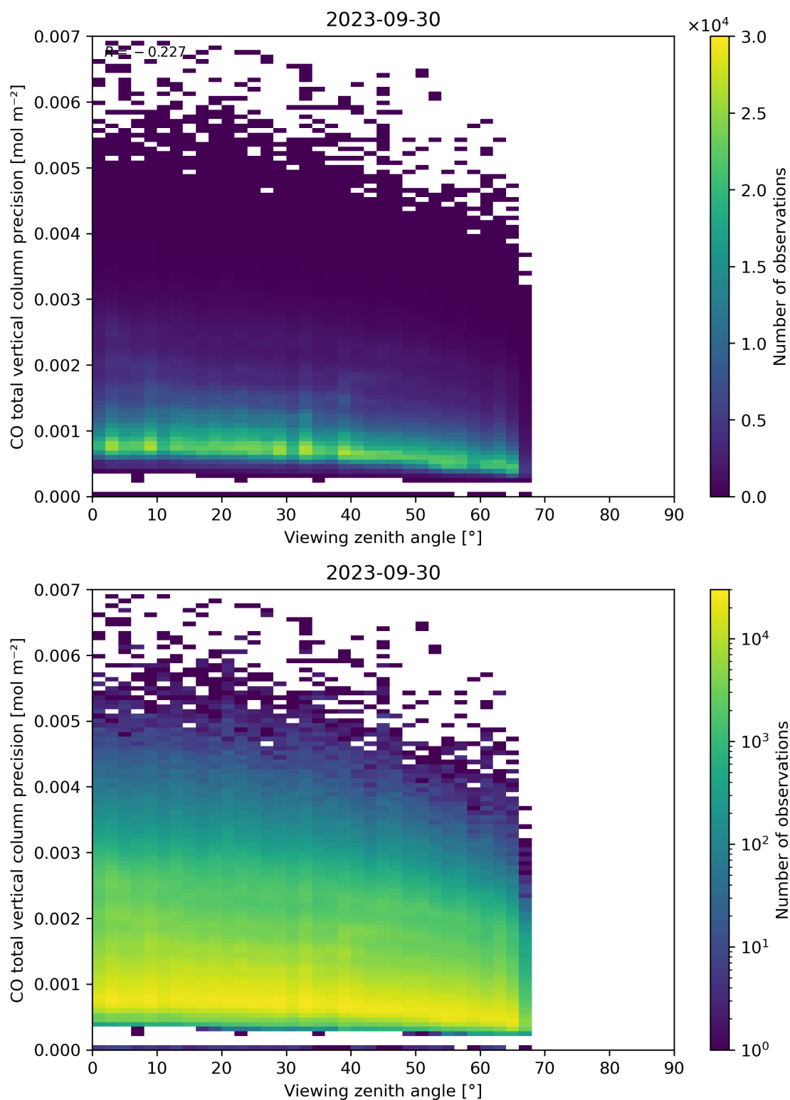
Figure 71: Scatter density plot of “Viewing zenith angle” against “CO total vertical column precision” for 2023-09-29 to 2023-10-01.
