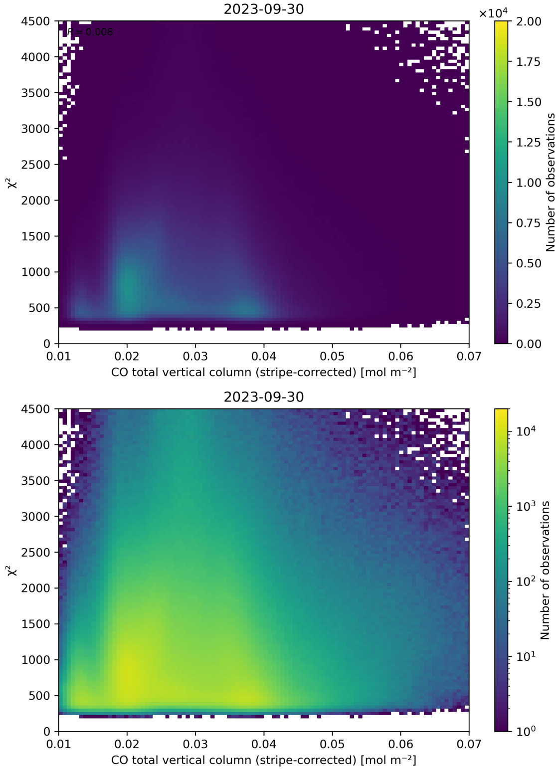
Figure 37: Scatter density plot of “CO total vertical column (stripe-corrected)” against “ \chi^2 ” for 2023-09-29 to 2023-10-01.
