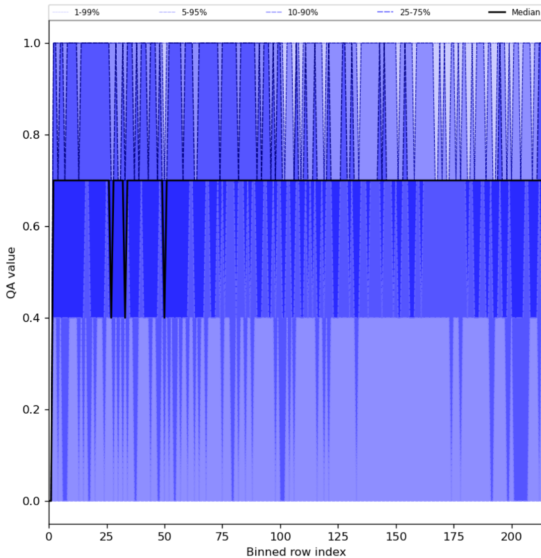
Figure 25: Along track statistics of “QA value” for 2023-09-29 to 2023-10-01
