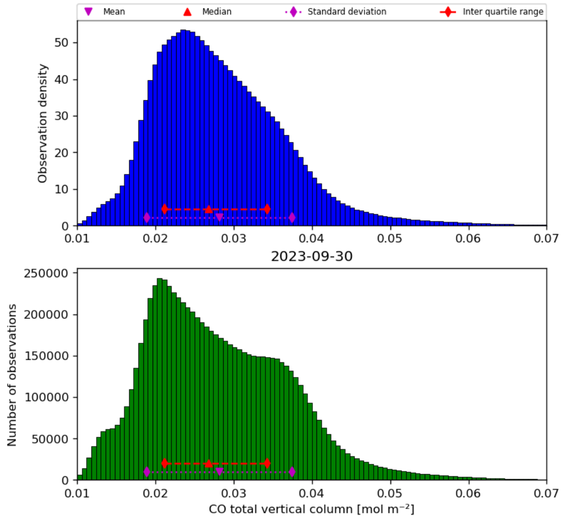
Figure 18: Histogram of “CO total vertical column” for 2023-09-29 to 2023-10-01
