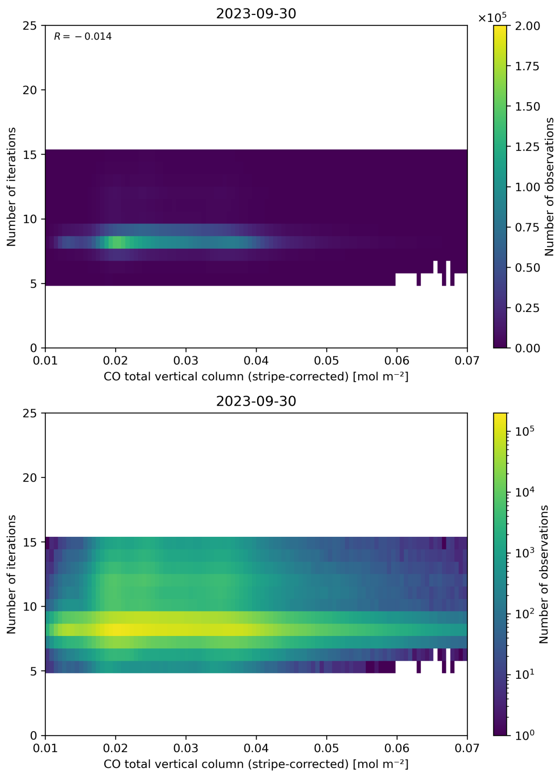
Figure 39: Scatter density plot of “CO total vertical column (stripe-corrected)” against “Number of iterations” for 2023-09-29 to 2023-10-01.
