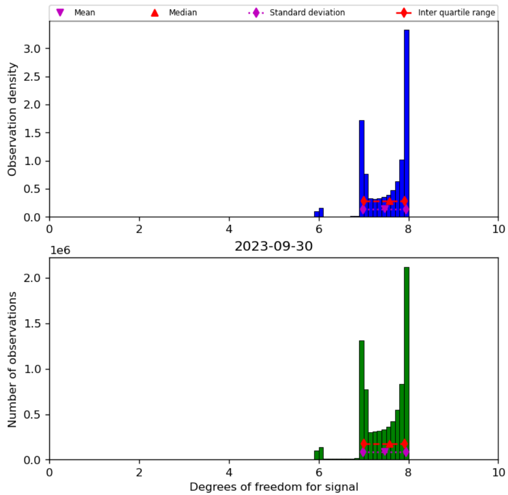
Figure 23: Histogram of “Degrees of freedom for signal” for 2023-09-29 to 2023-10-01
