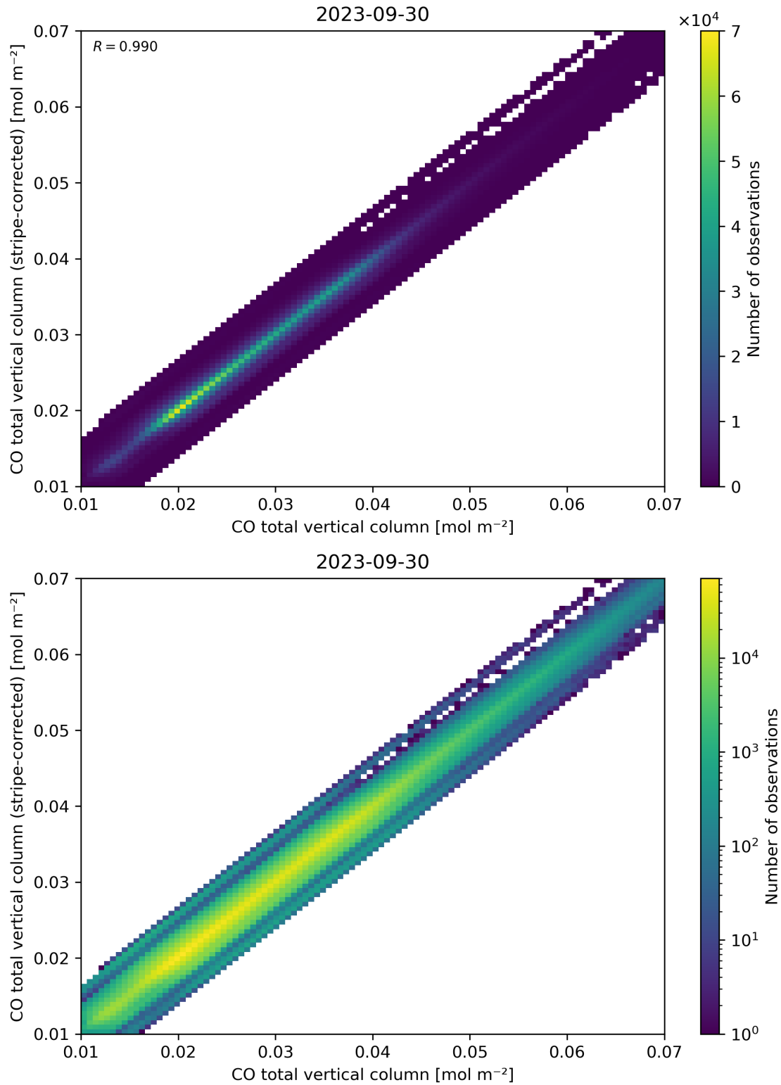
Figure 33: Scatter density plot of “CO total vertical column” against “CO total vertical column (stripe-corrected)” for 2023-09-29 to 2023-10-01.
