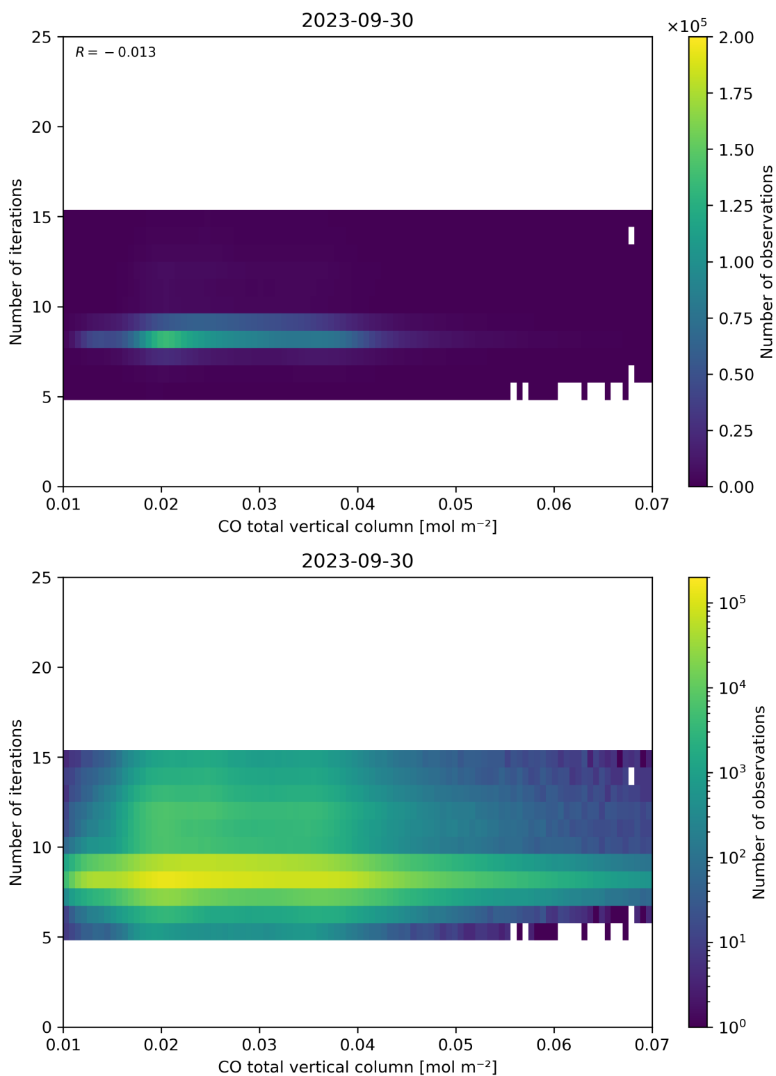
Figure 42: Scatter density plot of “CO total vertical column” against “Number of iterations” for 2023-09-29 to 2023-10-01.
