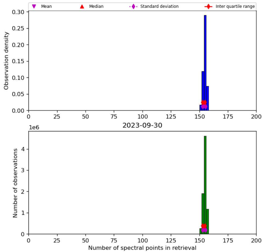
Figure 21: Histogram of “Number of spectral points in retrieval” for 2023-09-29 to 2023-10-01
