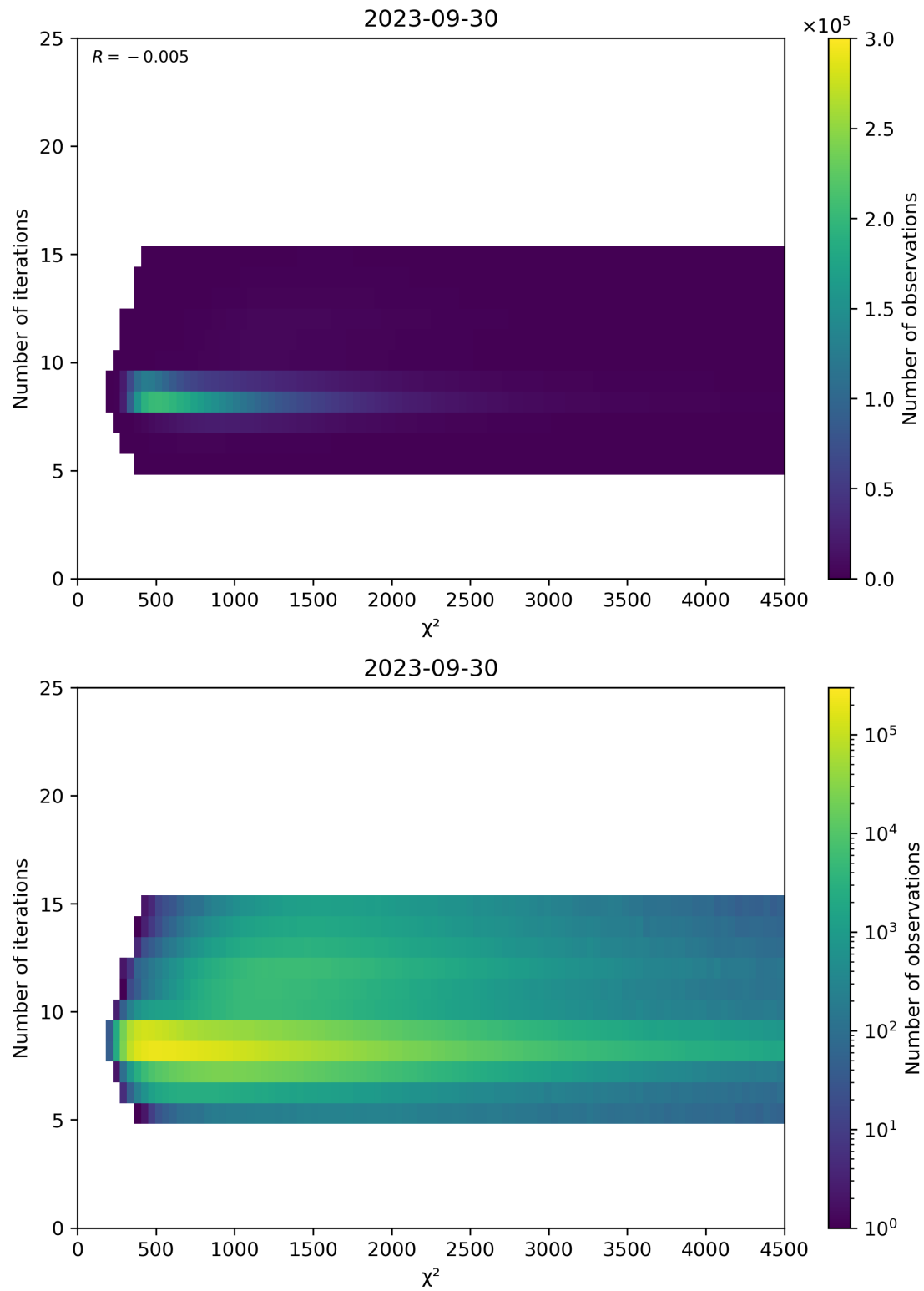
Figure 49: Scatter density plot of “ \chi^2 ” against “Number of iterations” for 2023-09-29 to 2023-10-01.
