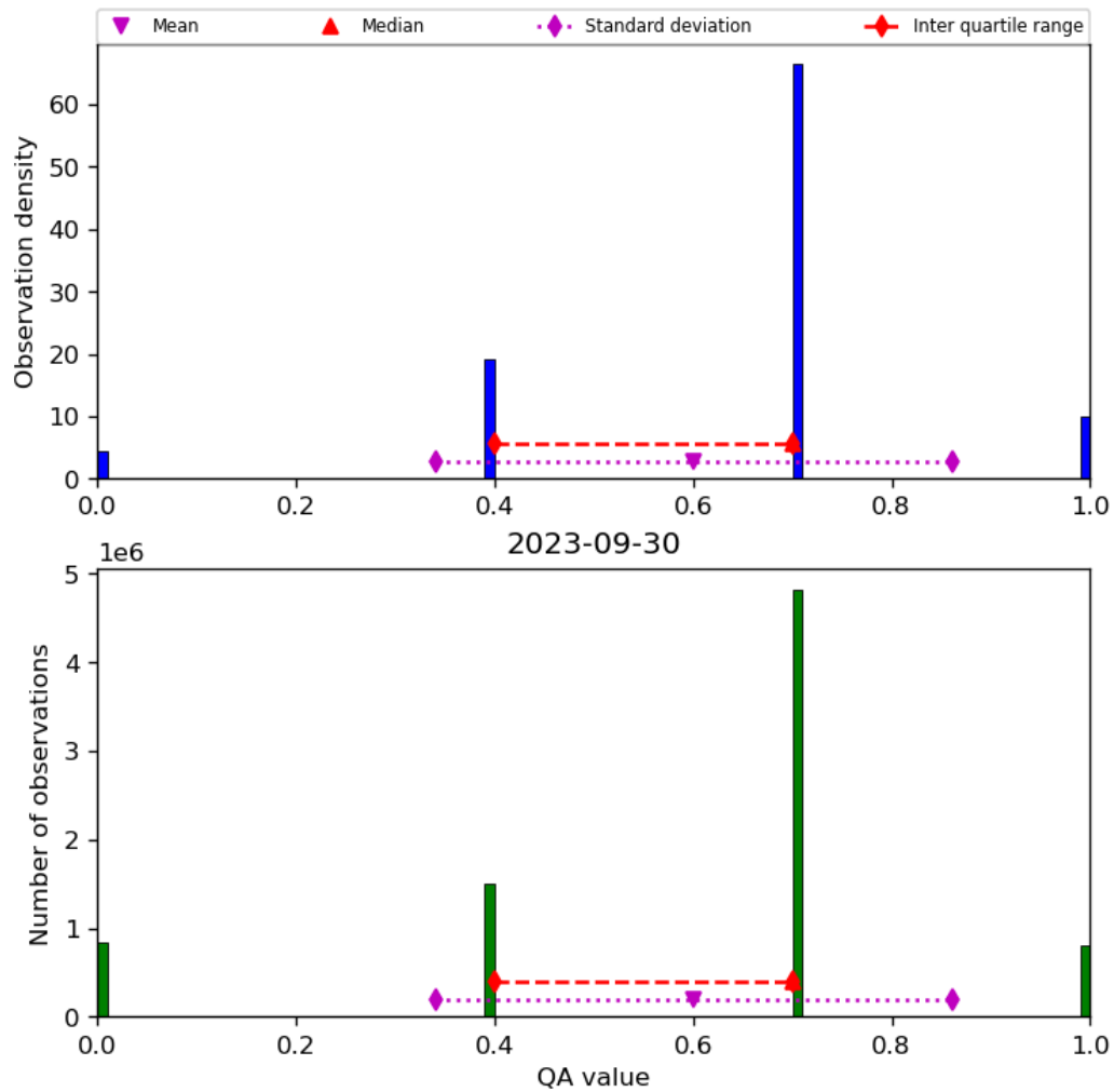
Figure 17: Histogram of “QA value” for 2023-09-29 to 2023-10-01
