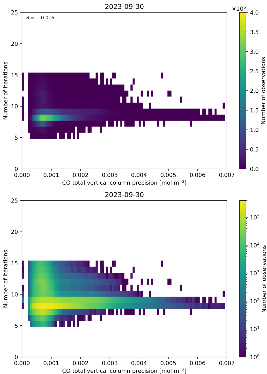
Figure 46: Scatter density plot of “CO total vertical column precision” against “Number of iterations” for 2023-09-29 to 2023-10-01.
