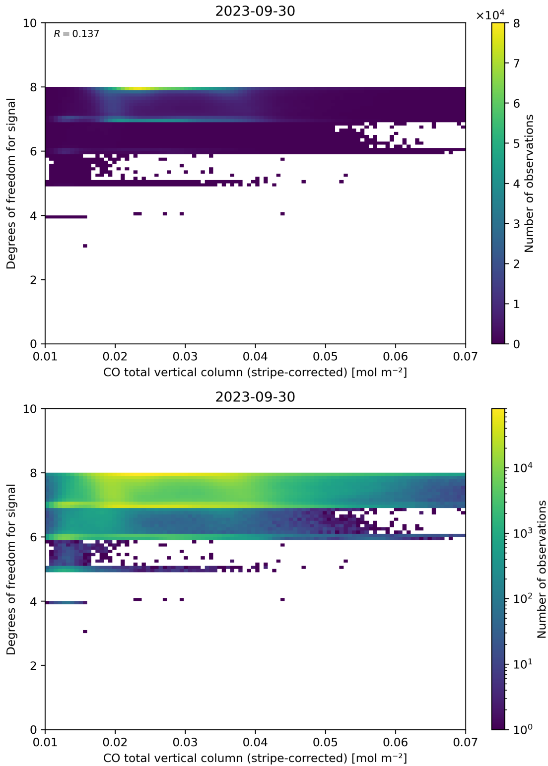
Figure 38: Scatter density plot of “CO total vertical column (stripe-corrected)” against “Degrees of freedom for signal” for 2023-09-29 to 2023-10-01.
