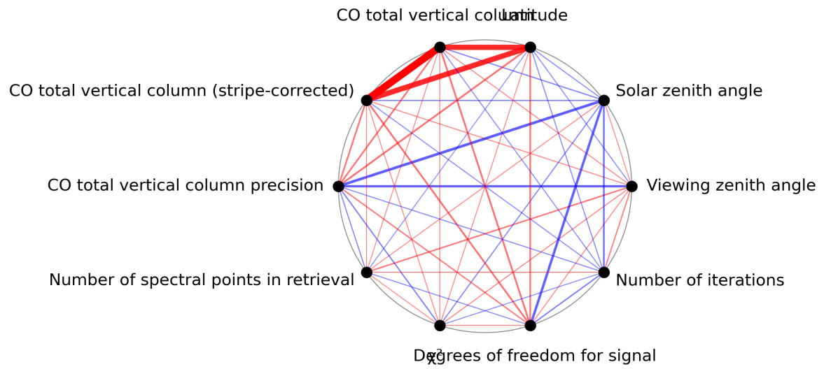
Figure 1: Map of correlation graph for 2023-09-29 to 2023-10-01.
