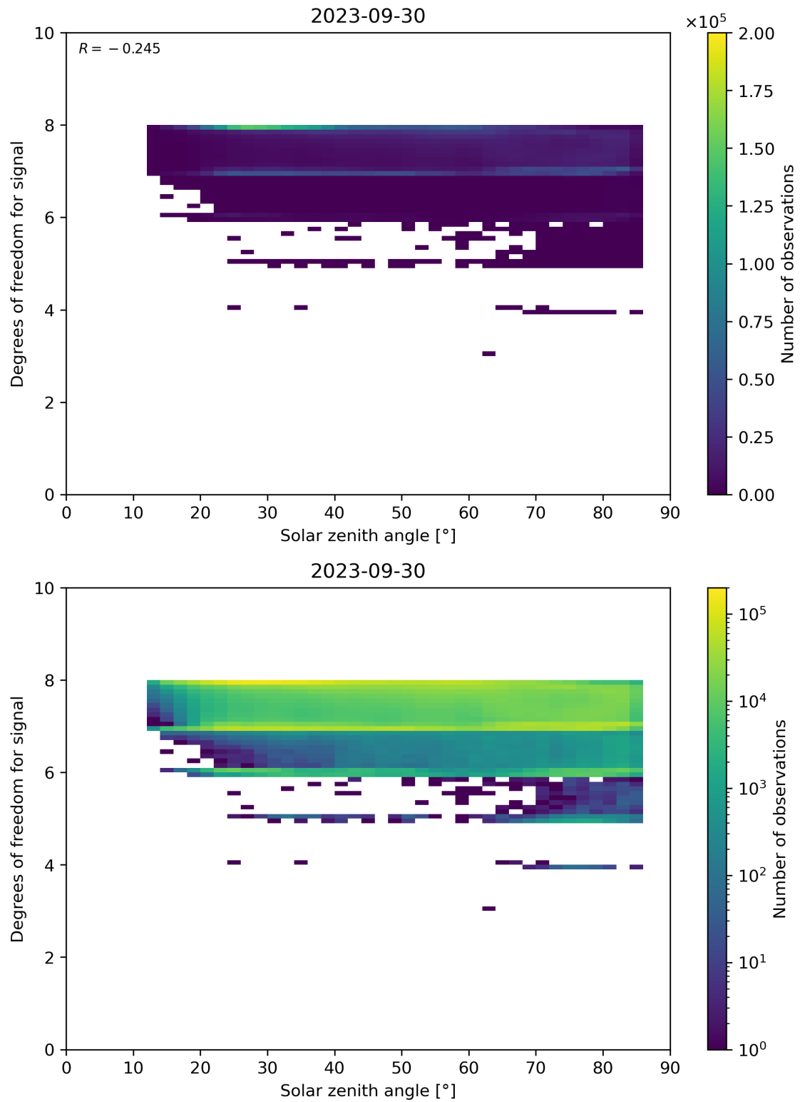
Figure 65: Scatter density plot of “Solar zenith angle” against “Degrees of freedom for signal” for 2023-09-29 to 2023-10-01.
