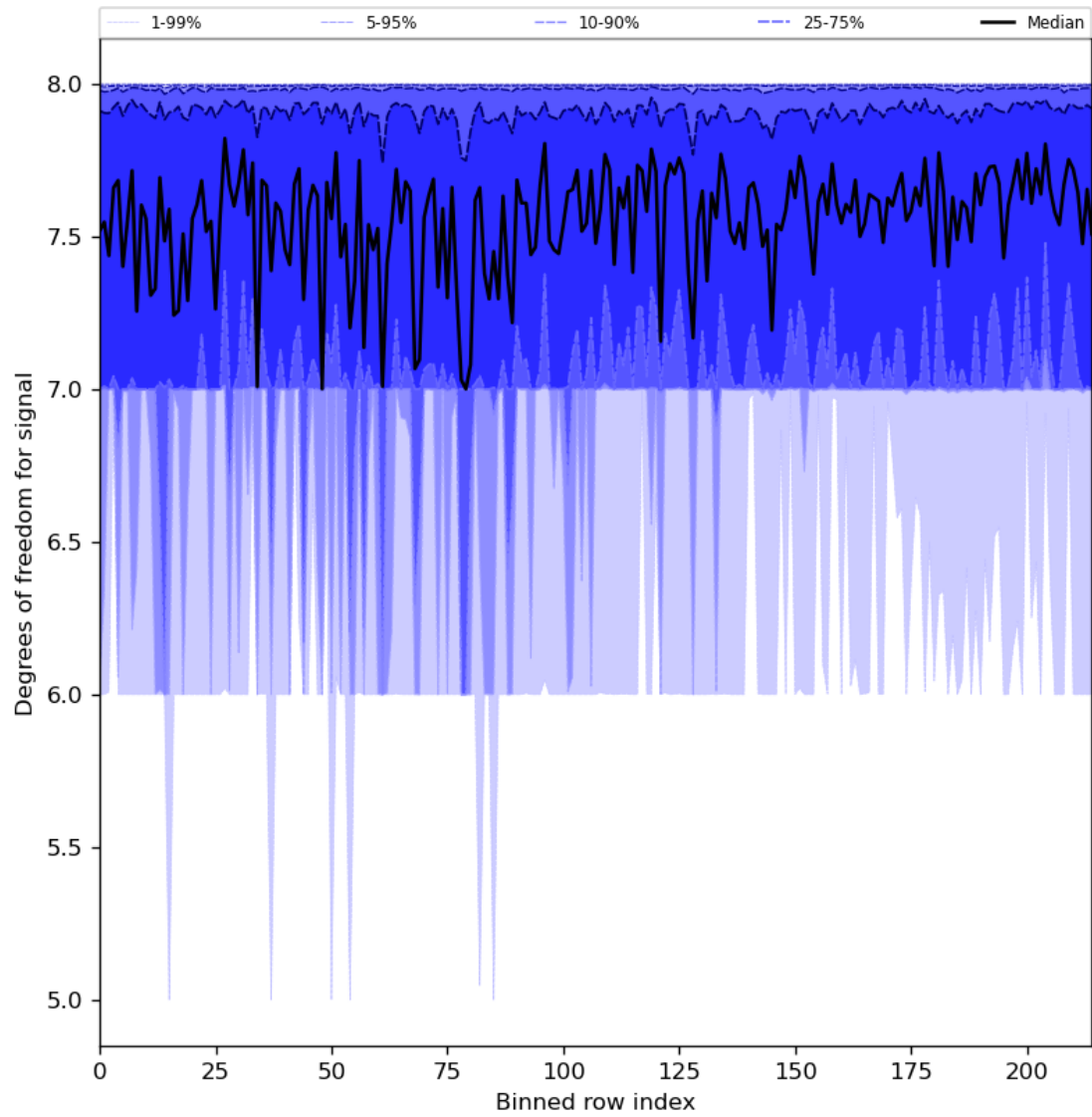
Figure 31: Along track statistics of “Degrees of freedom for signal” for 2023-09-29 to 2023-10-01
