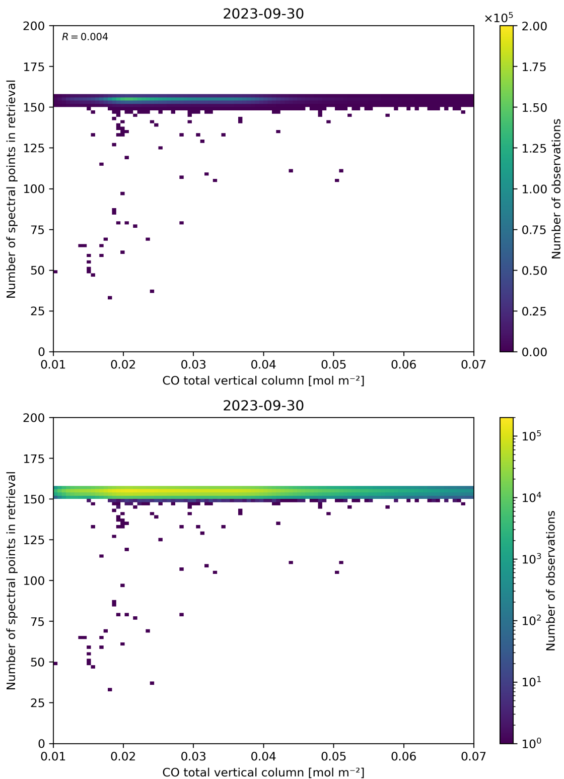
Figure 43: Scatter density plot of “CO total vertical column” against “Number of spectral points in retrieval” for 2023-09-29 to 2023-10-01.
