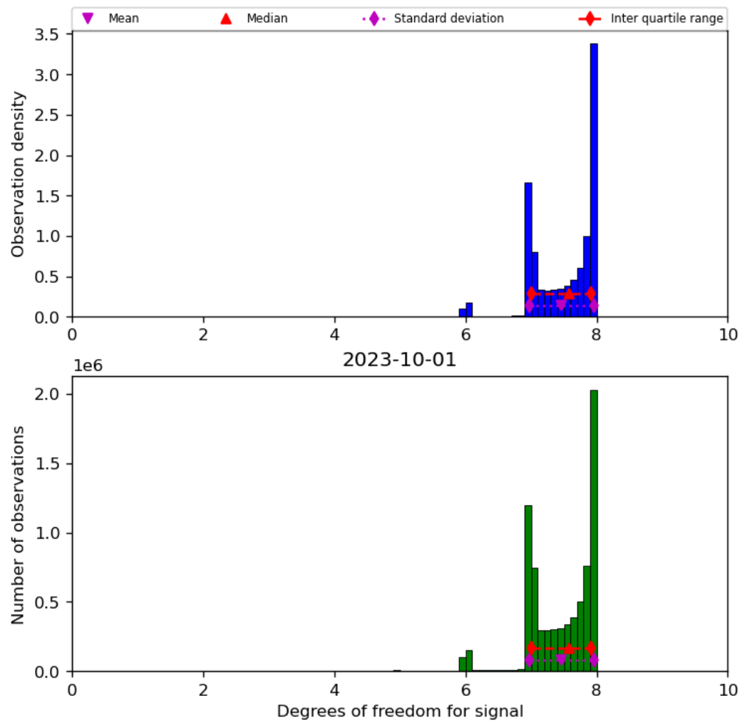
Figure 23: Histogram of “Degrees of freedom for signal” for 2023-10-01 to 2023-10-02
