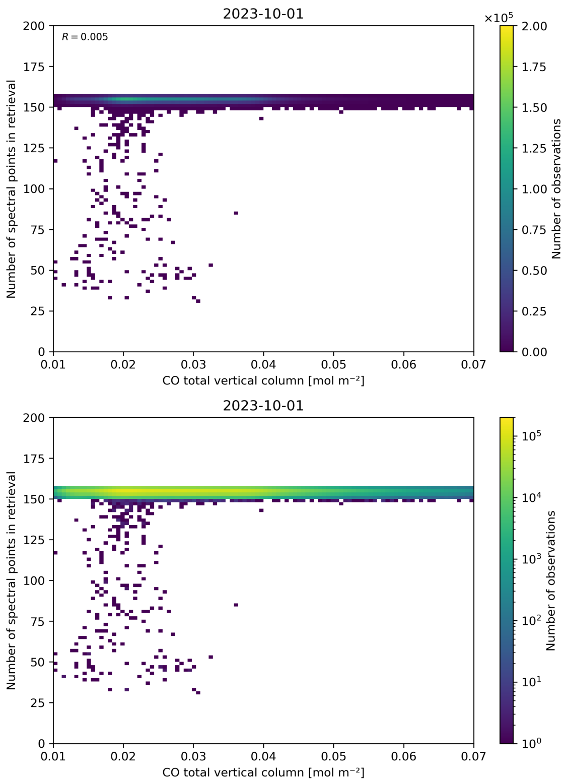
Figure 43: Scatter density plot of “CO total vertical column” against “Number of spectral points in retrieval” for 2023-10-01 to 2023-10-02.
