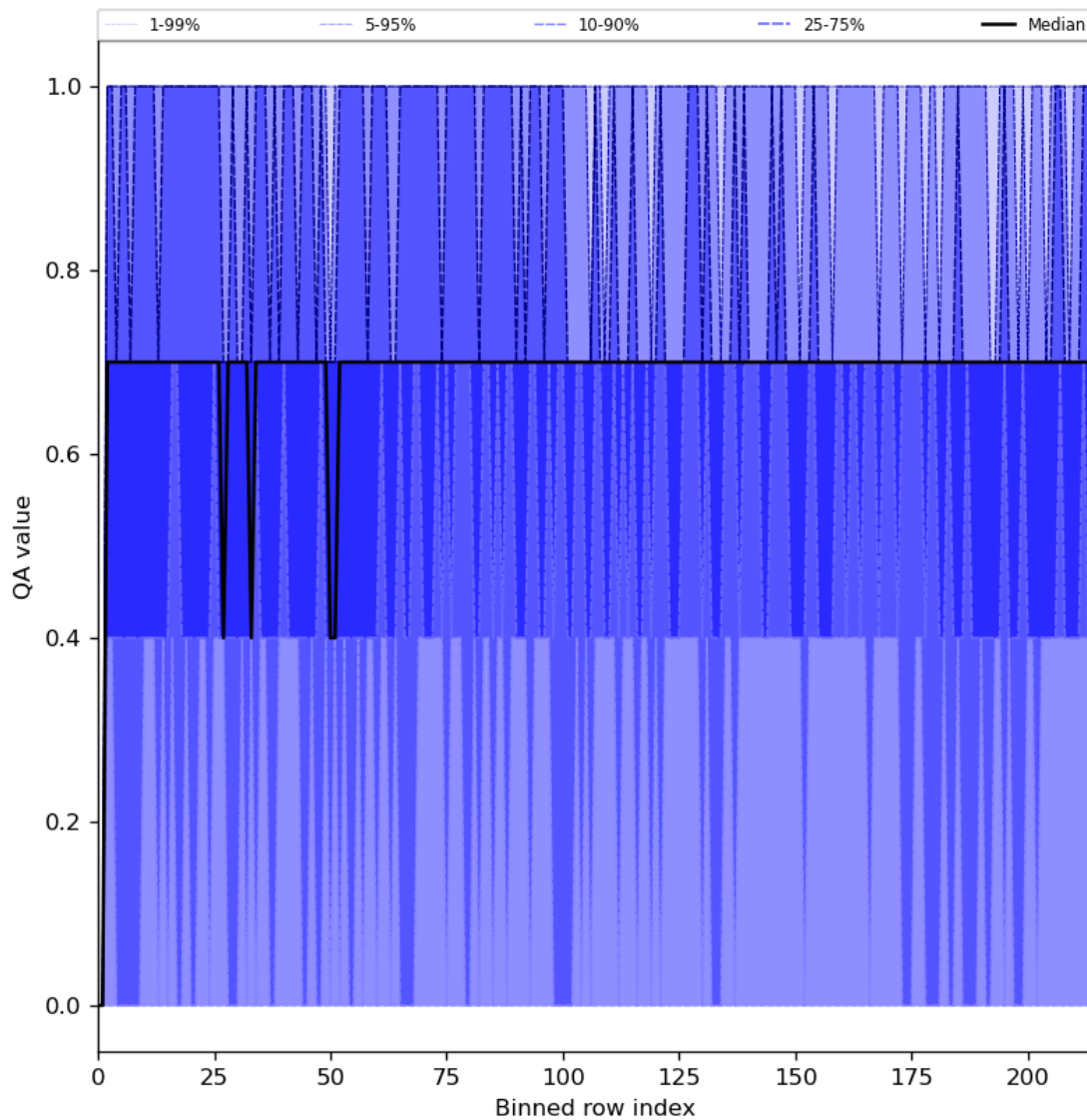
Figure 25: Along track statistics of “QA value” for 2023-10-01 to 2023-10-02
