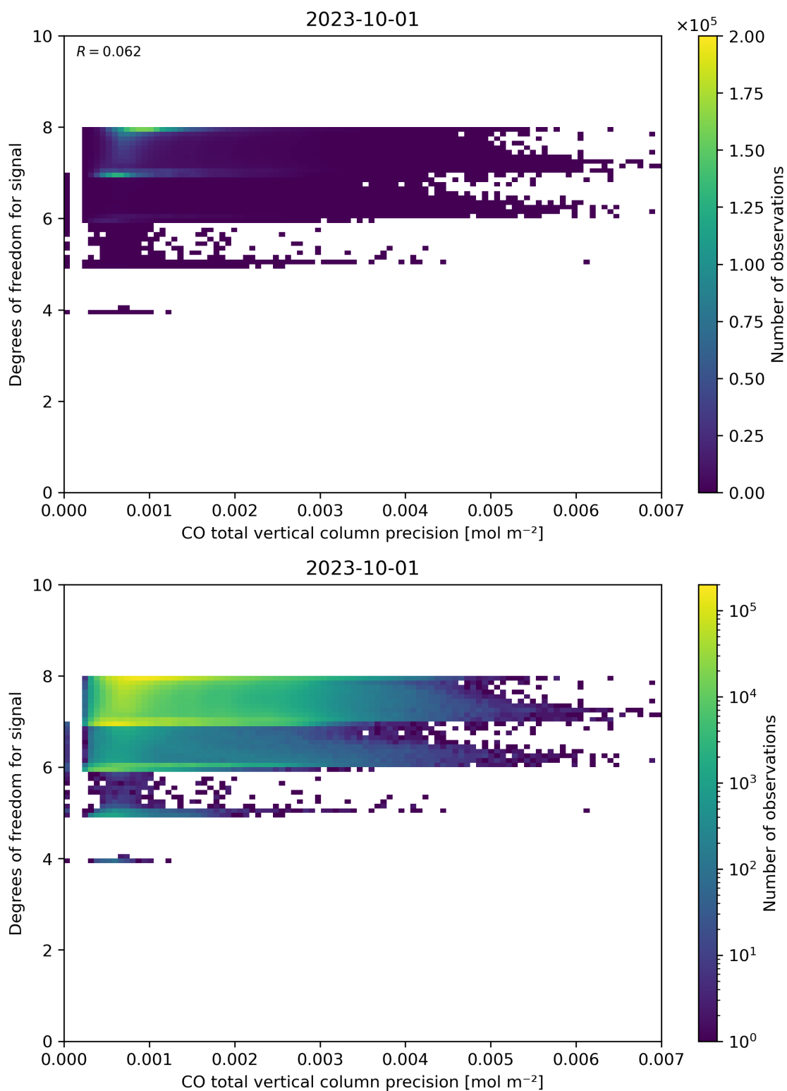
Figure 45: Scatter density plot of “CO total vertical column precision” against “Degrees of freedom for signal” for 2023-10-01 to 2023-10-02.
