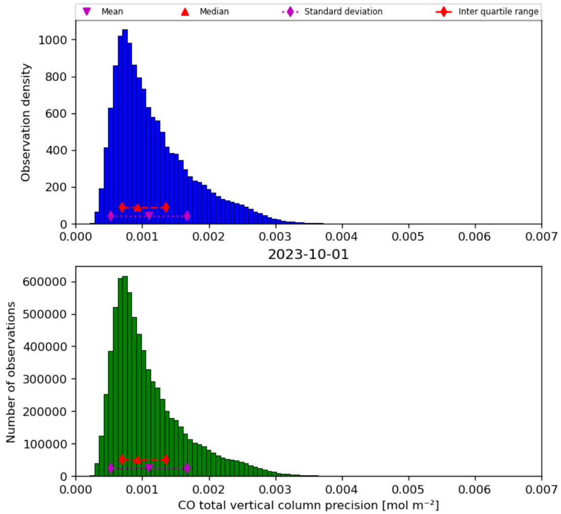
Figure 20: Histogram of “CO total vertical column precision” for 2023-10-01 to 2023-10-02
