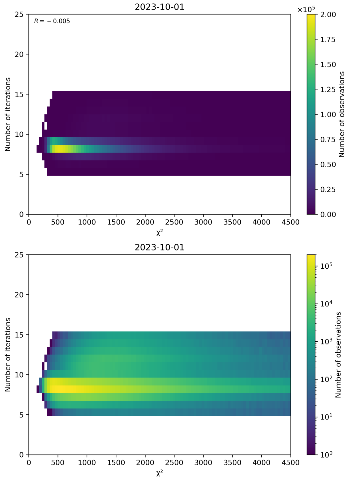
Figure 49: Scatter density plot of “ \chi^2 ” against “Number of iterations” for 2023-10-01 to 2023-10-02.
