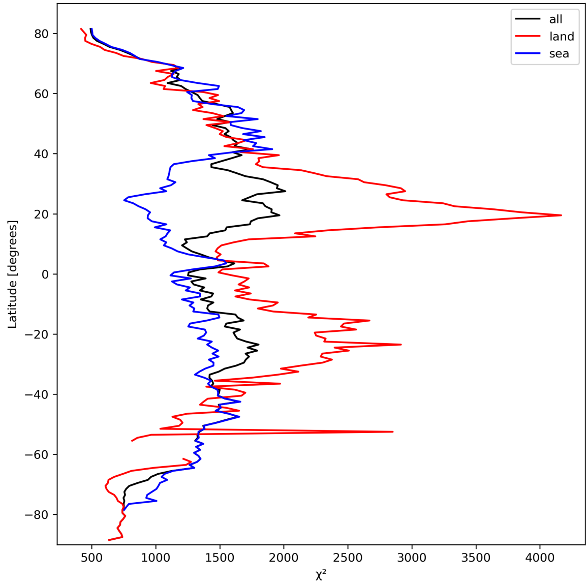
Figure 14: Zonal average of “ \chi^2 ” for 2023-10-01 to 2023-10-02.
