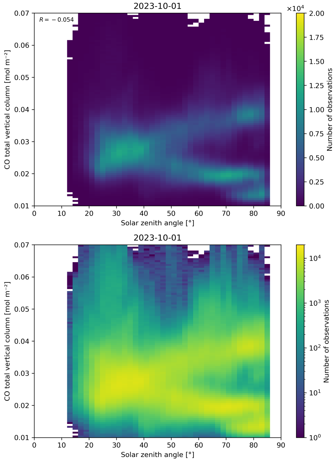
Figure 61: Scatter density plot of “Solar zenith angle” against “CO total vertical column” for 2023-10-01 to 2023-10-02.
