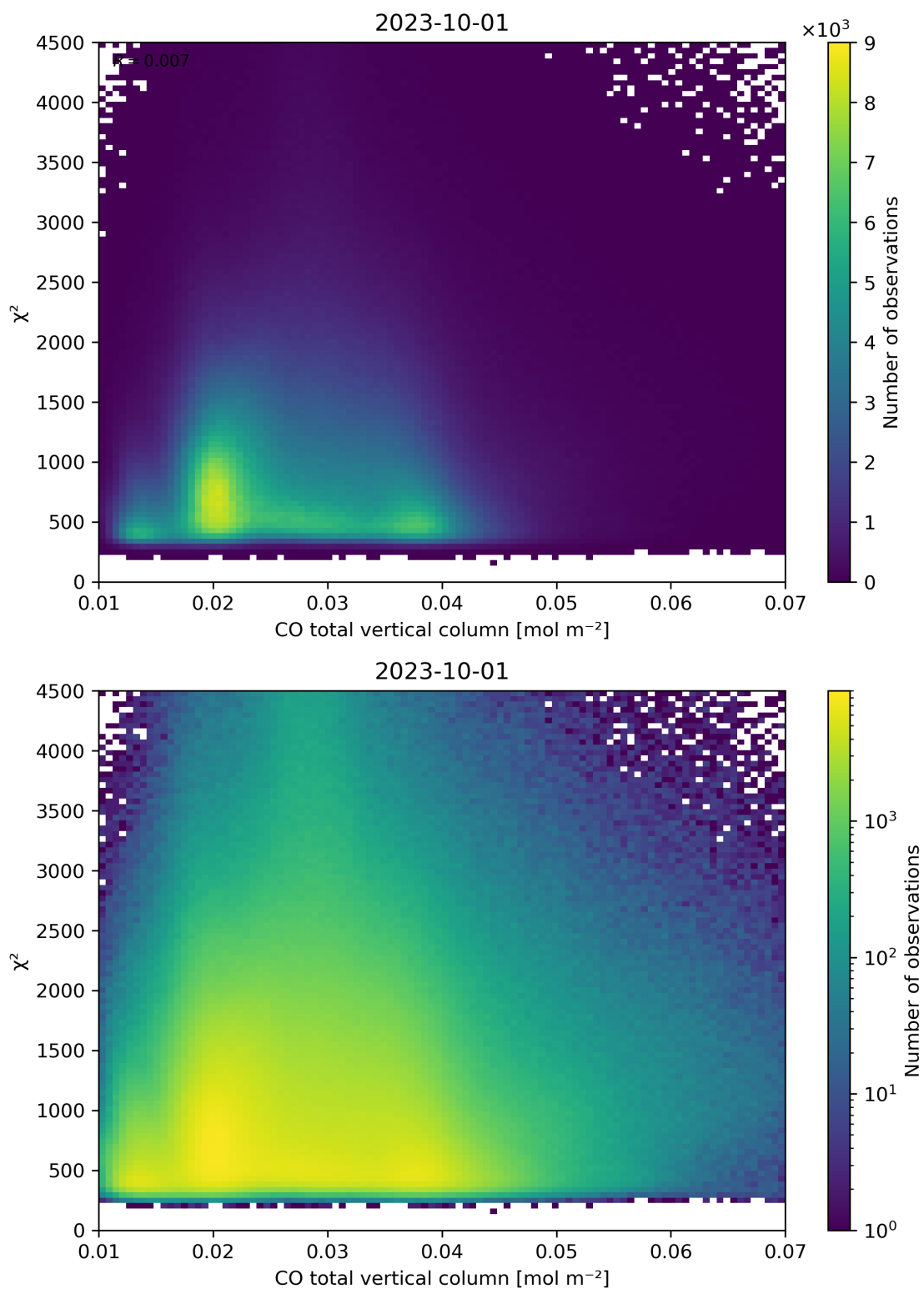
Figure 35: Scatter density plot of “CO total vertical column” against “ \chi^2 ” for 2023-10-01 to 2023-10-02.
