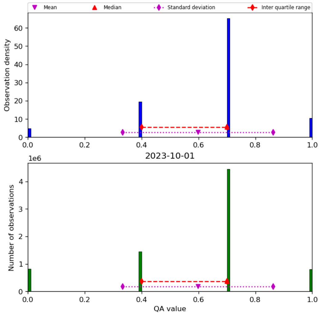
Figure 17: Histogram of “QA value” for 2023-10-01 to 2023-10-02
