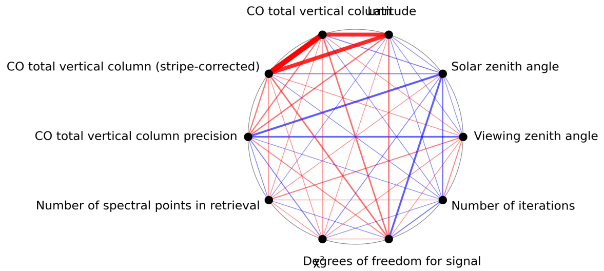
Figure 1: Map of correlation graph for 2023-10-01 to 2023-10-02.
