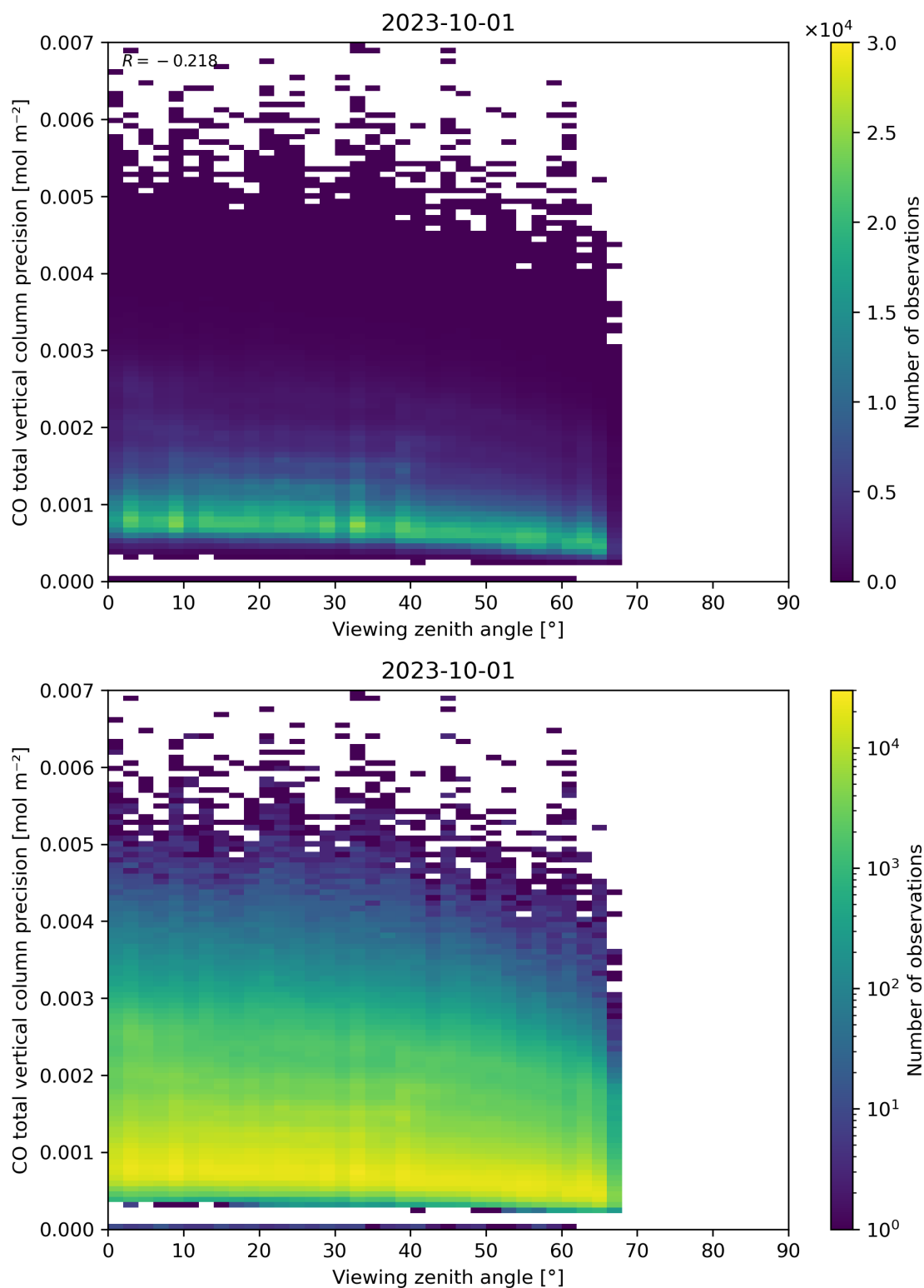
Figure 71: Scatter density plot of “Viewing zenith angle” against “CO total vertical column precision” for 2023-10-01 to 2023-10-02.
