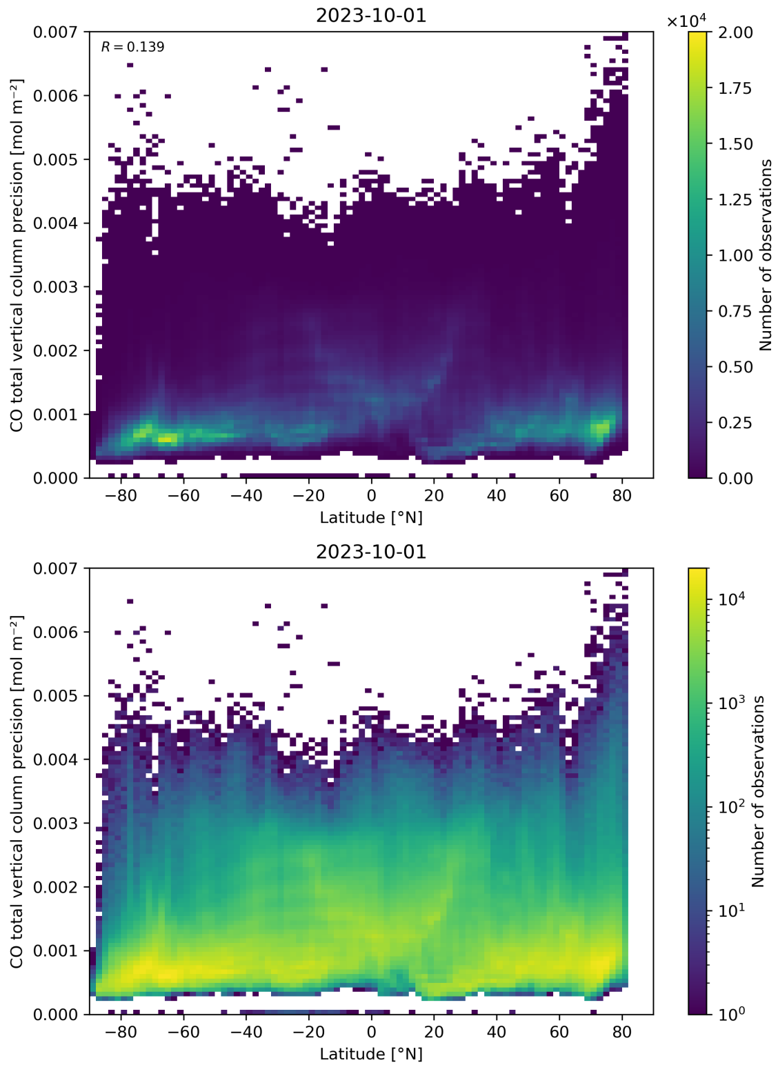
Figure 53: Scatter density plot of “Latitude” against “CO total vertical column precision” for 2023-10-01 to 2023-10-02.
