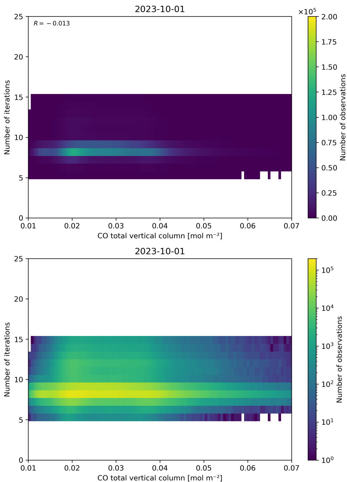
Figure 42: Scatter density plot of “CO total vertical column” against “Number of iterations” for 2023-10-01 to 2023-10-02.
