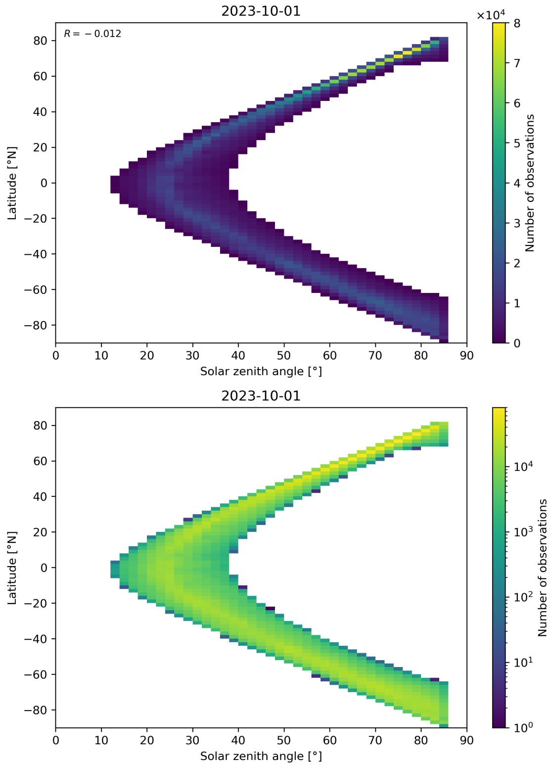
Figure 66: Scatter density plot of “Solar zenith angle” against “Latitude” for 2023-10-01 to 2023-10-02.
