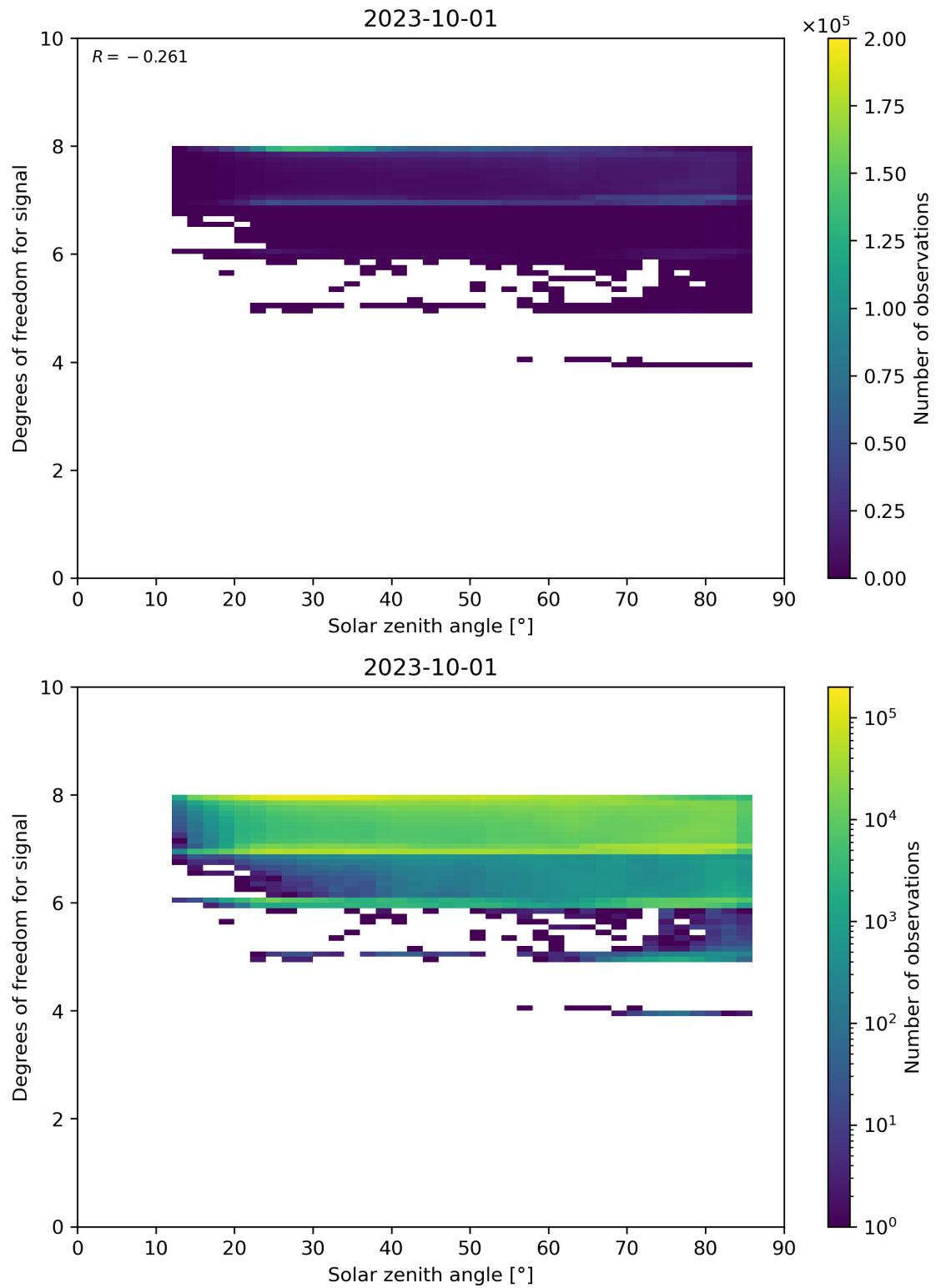
Figure 65: Scatter density plot of “Solar zenith angle” against “Degrees of freedom for signal” for 2023-10-01 to 2023-10-02.
