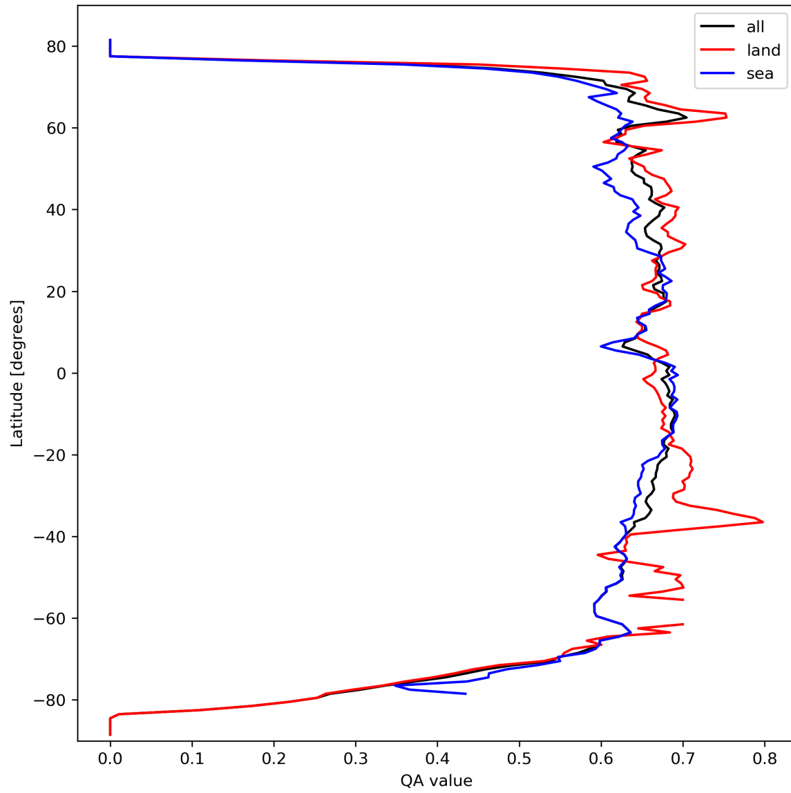
Figure 9: Zonal average of “QA value” for 2023-10-01 to 2023-10-02.
