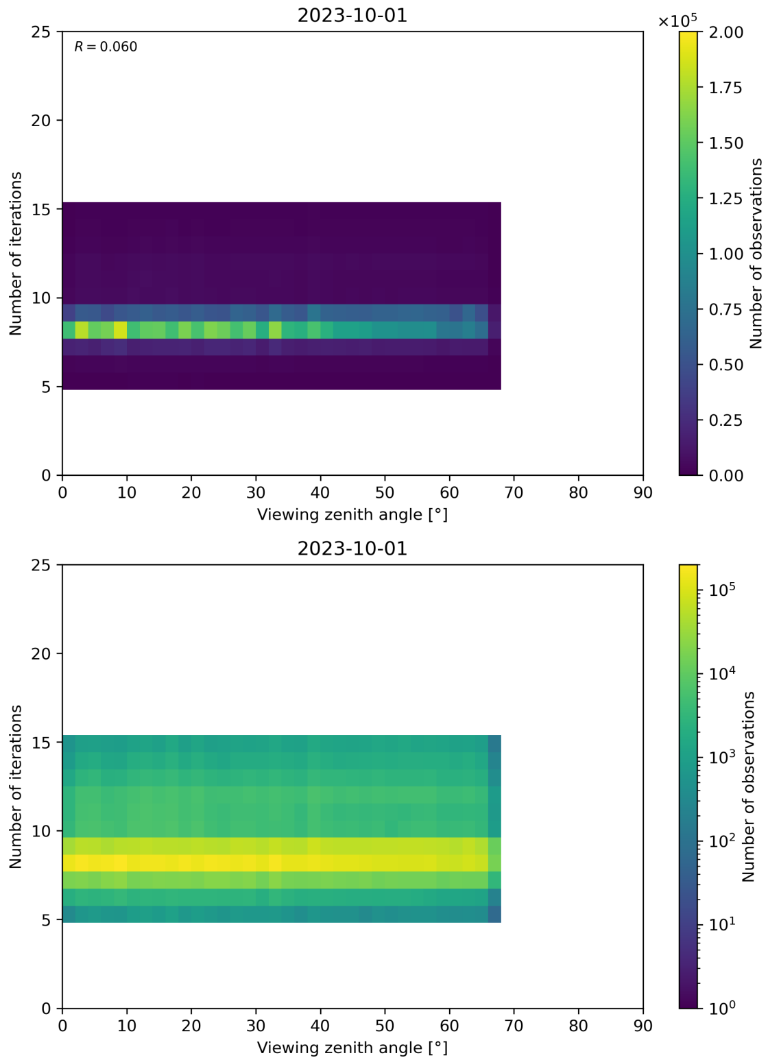
Figure 75: Scatter density plot of “Viewing zenith angle” against “Number of iterations” for 2023-10-01 to 2023-10-02.
