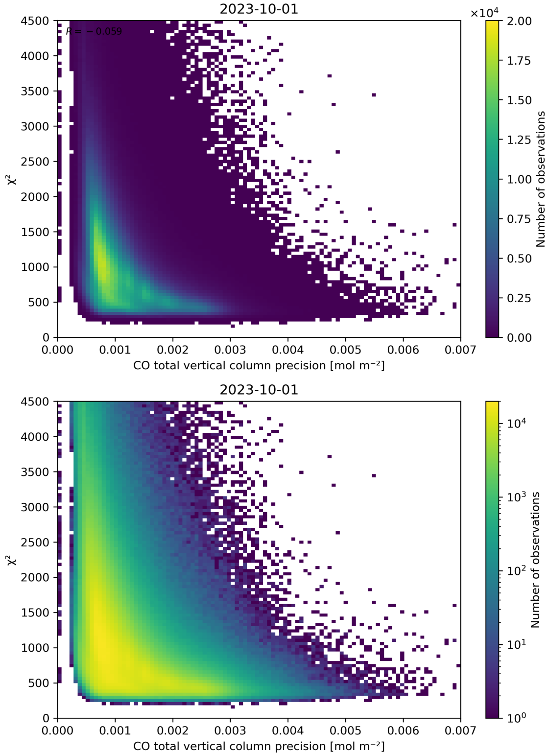
Figure 44: Scatter density plot of “CO total vertical column precision” against “ \chi^2 ” for 2023-10-01 to 2023-10-02.
