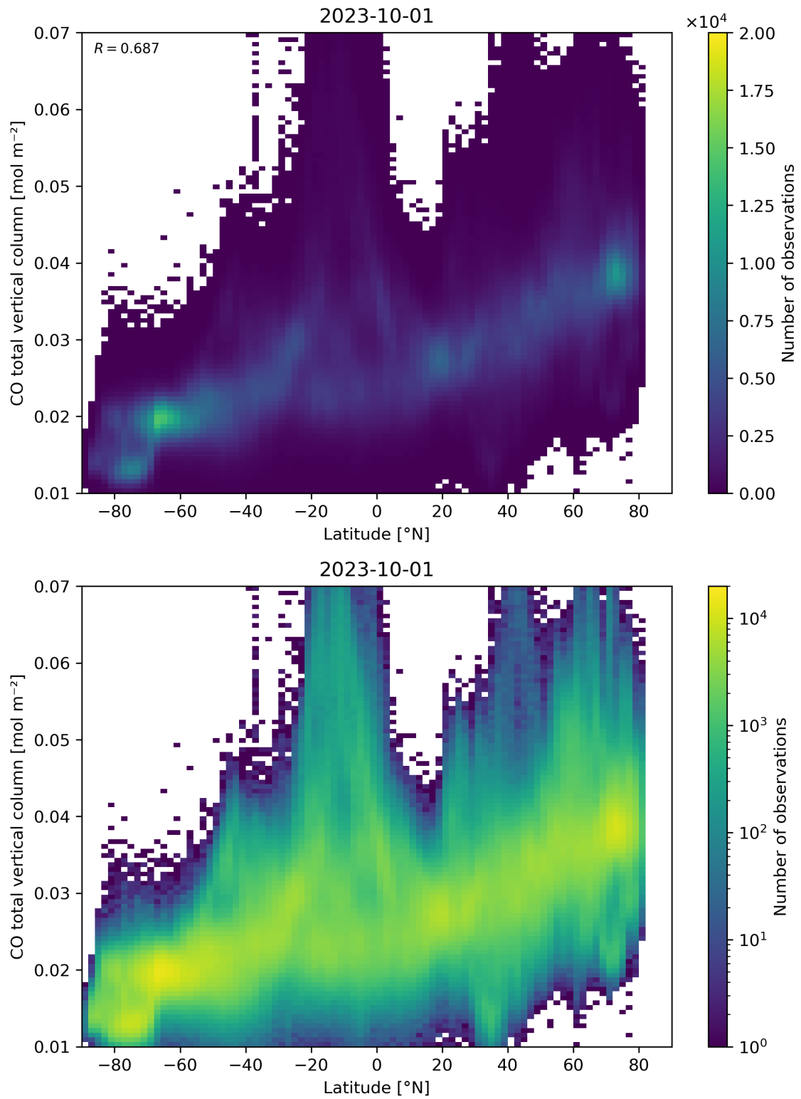
Figure 51: Scatter density plot of “Latitude” against “CO total vertical column” for 2023-10-01 to 2023-10-02.
