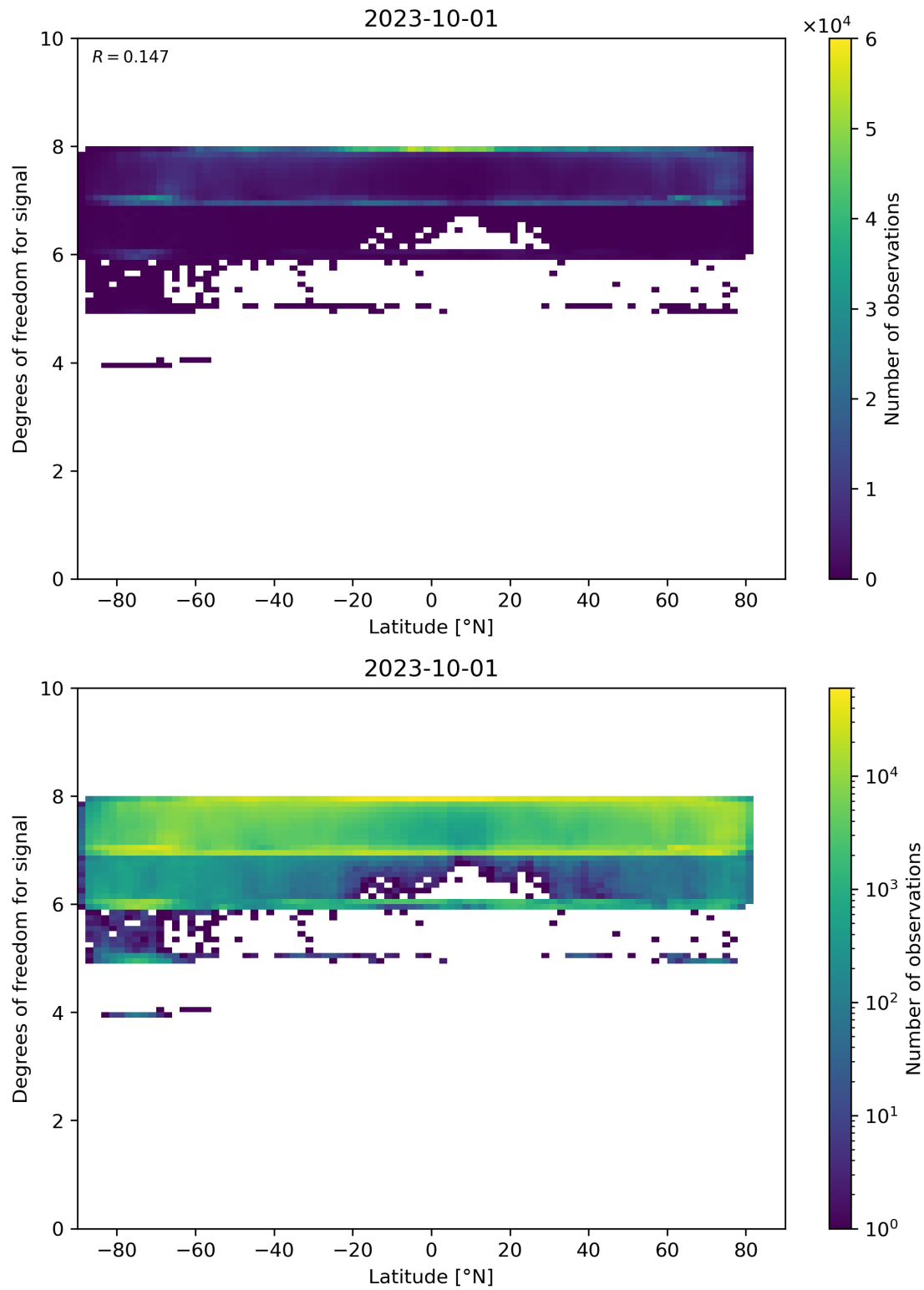
Figure 55: Scatter density plot of “Latitude” against “Degrees of freedom for signal” for 2023-10-01 to 2023-10-02.
