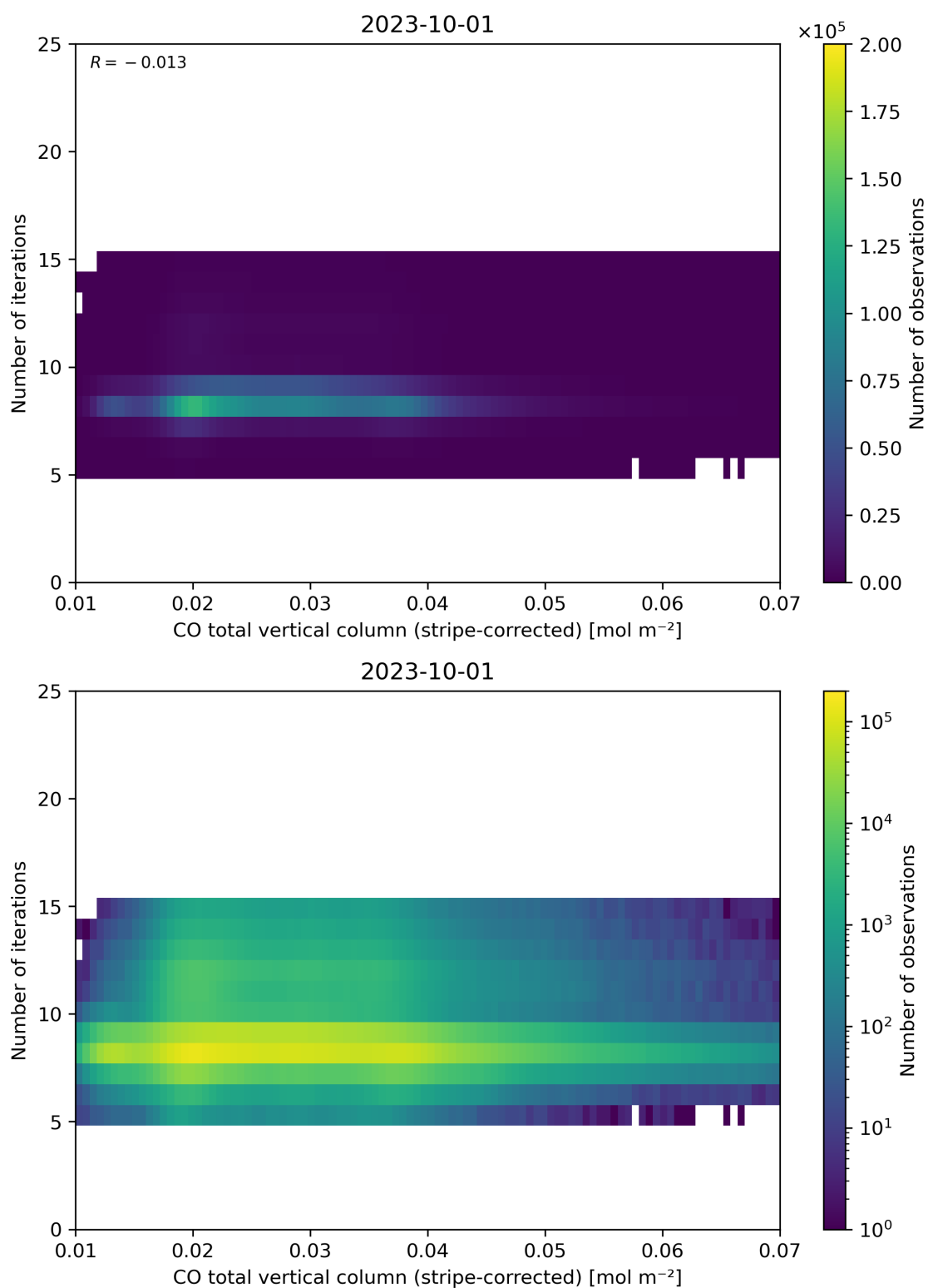
Figure 39: Scatter density plot of “CO total vertical column (stripe-corrected)” against “Number of iterations” for 2023-10-01 to 2023-10-02.
