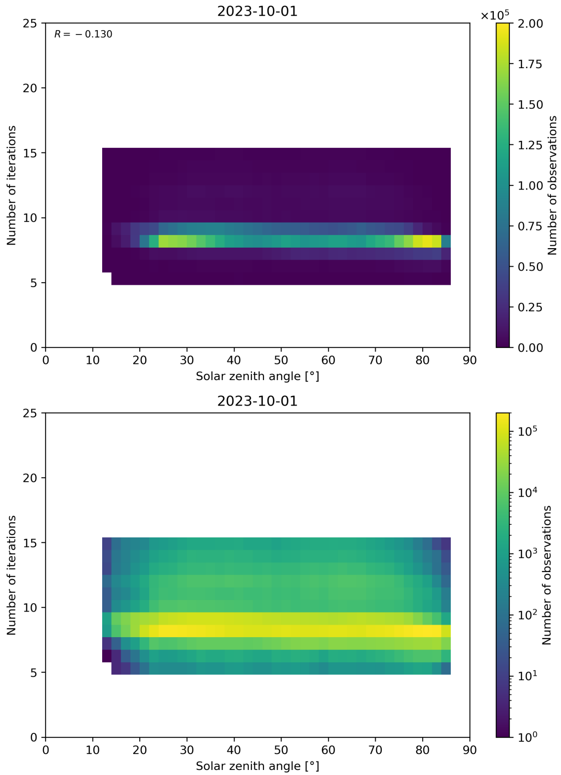
Figure 67: Scatter density plot of “Solar zenith angle” against “Number of iterations” for 2023-10-01 to 2023-10-02.
