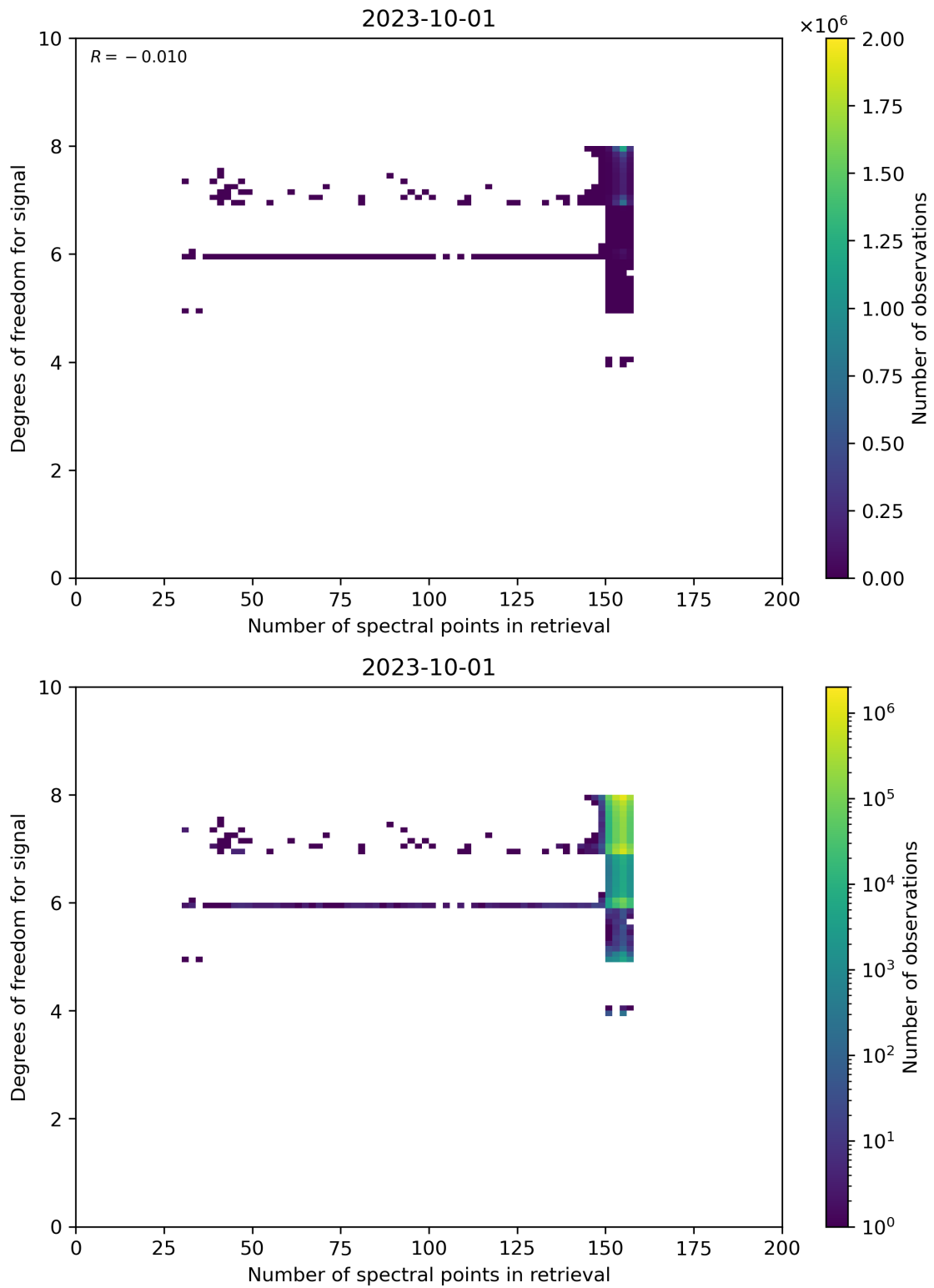
Figure 59: Scatter density plot of “Number of spectral points in retrieval” against “Degrees of freedom for signal” for 2023-10-01 to 2023-10-02.
