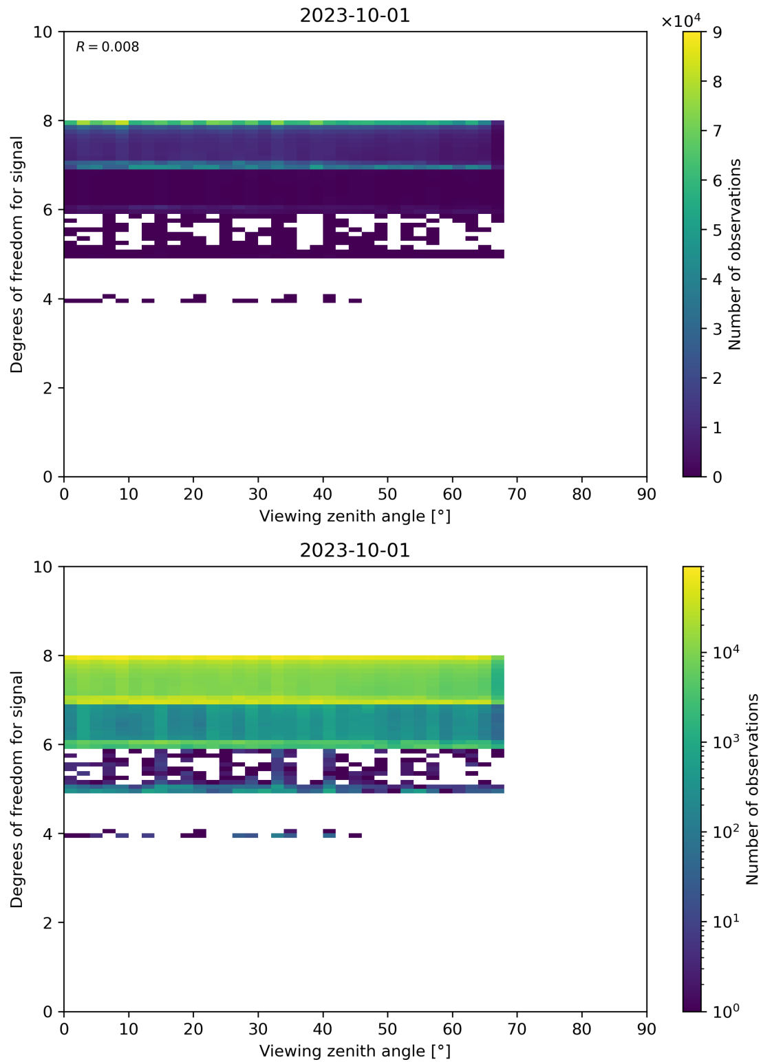
Figure 73: Scatter density plot of “Viewing zenith angle” against “Degrees of freedom for signal” for 2023-10-01 to 2023-10-02.
