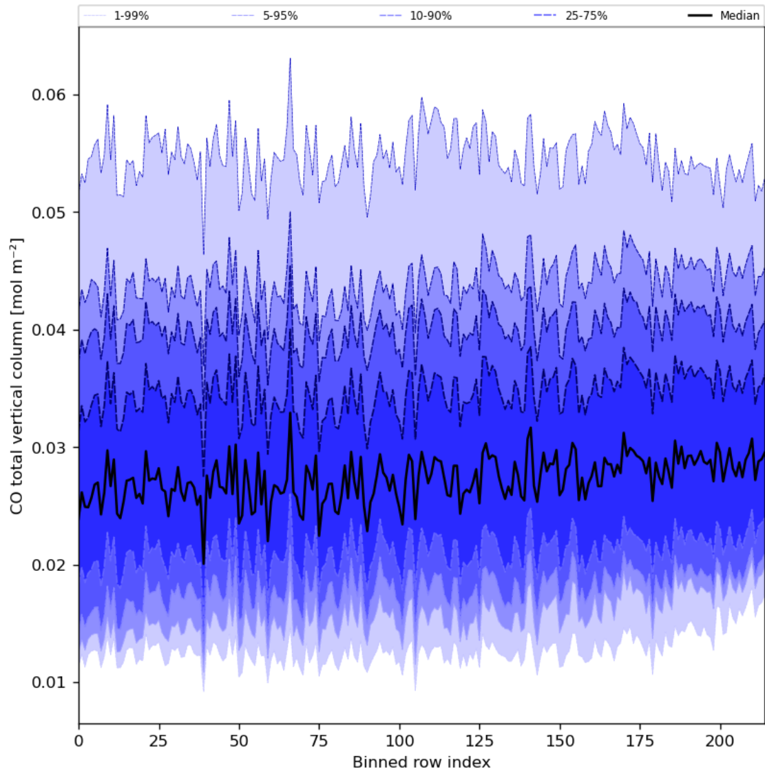
Figure 26: Along track statistics of “CO total vertical column” for 2023-10-01 to 2023-10-02
