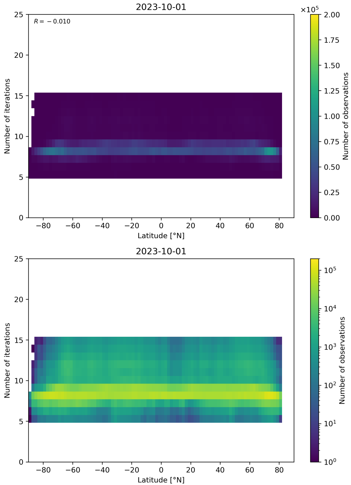
Figure 56: Scatter density plot of “Latitude” against “Number of iterations” for 2023-10-01 to 2023-10-02.
