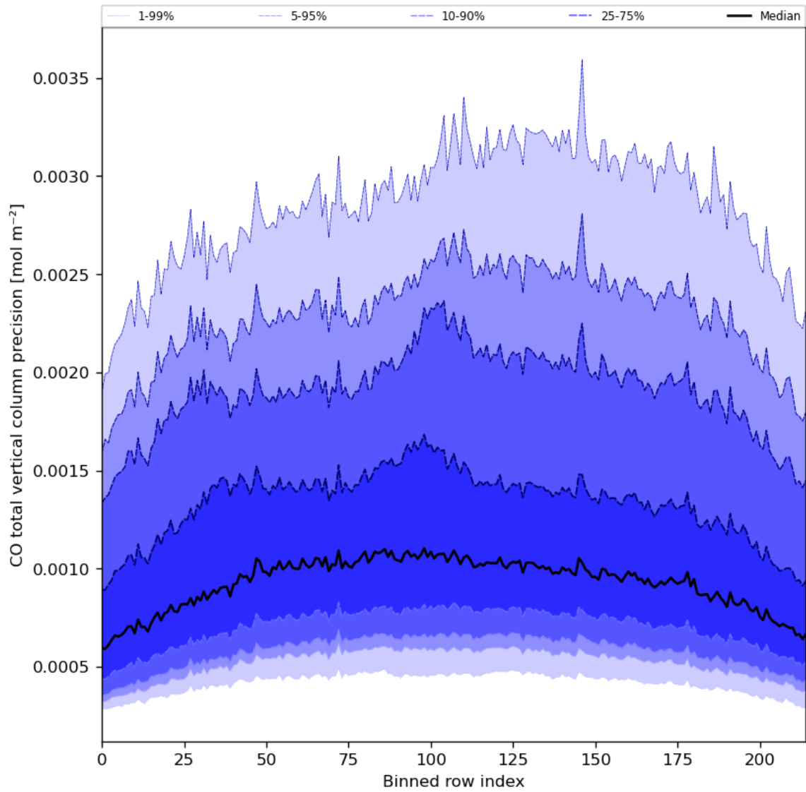
Figure 28: Along track statistics of “CO total vertical column precision” for 2023-10-01 to 2023-10-02
