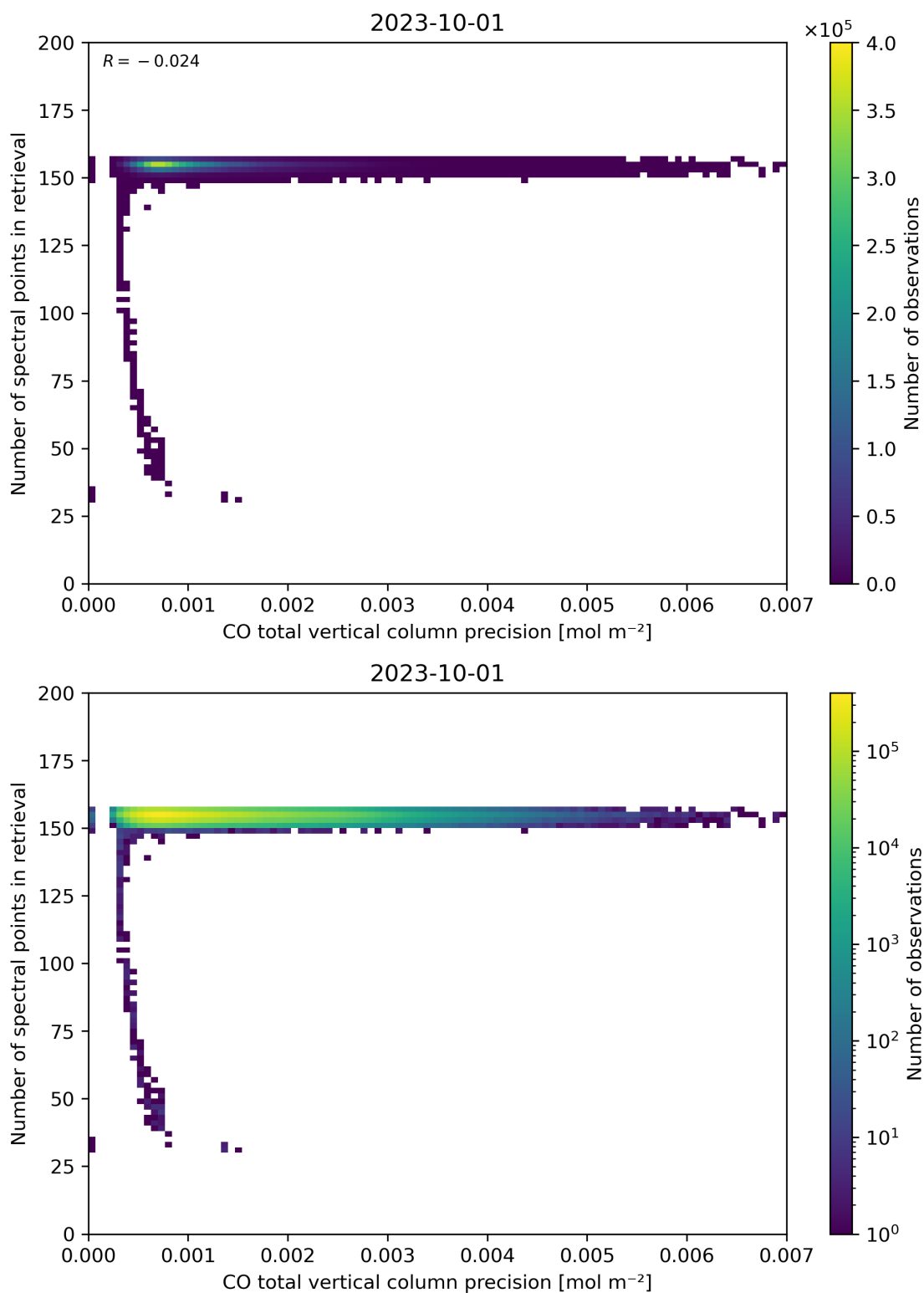
Figure 47: Scatter density plot of “CO total vertical column precision” against “Number of spectral points in retrieval” for 2023-10-01 to 2023-10-02.
