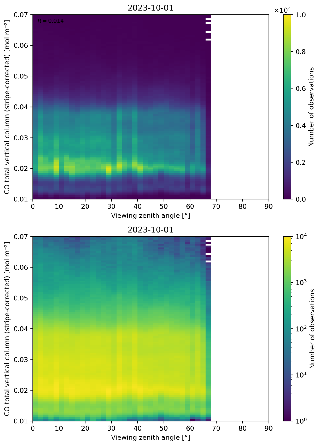
Figure 70: Scatter density plot of “Viewing zenith angle” against “CO total vertical column (stripe-corrected)” for 2023-10-01 to 2023-10-02.
