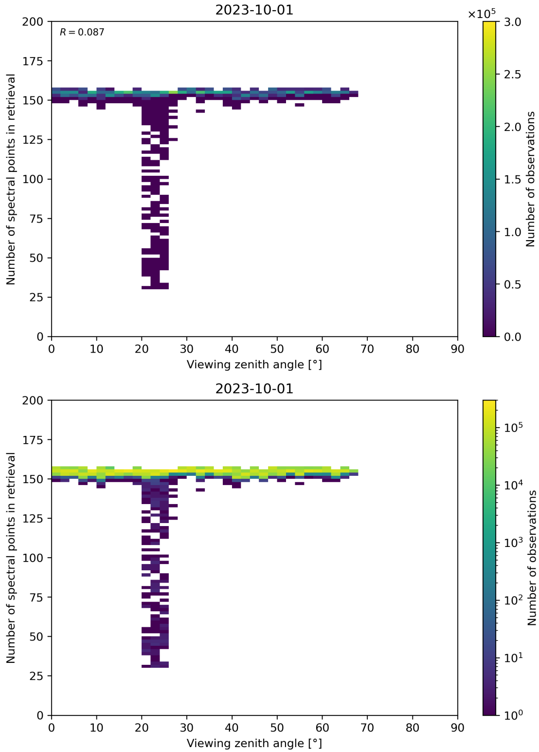
Figure 76: Scatter density plot of “Viewing zenith angle” against “Number of spectral points in retrieval” for 2023-10-01 to 2023-10-02.
