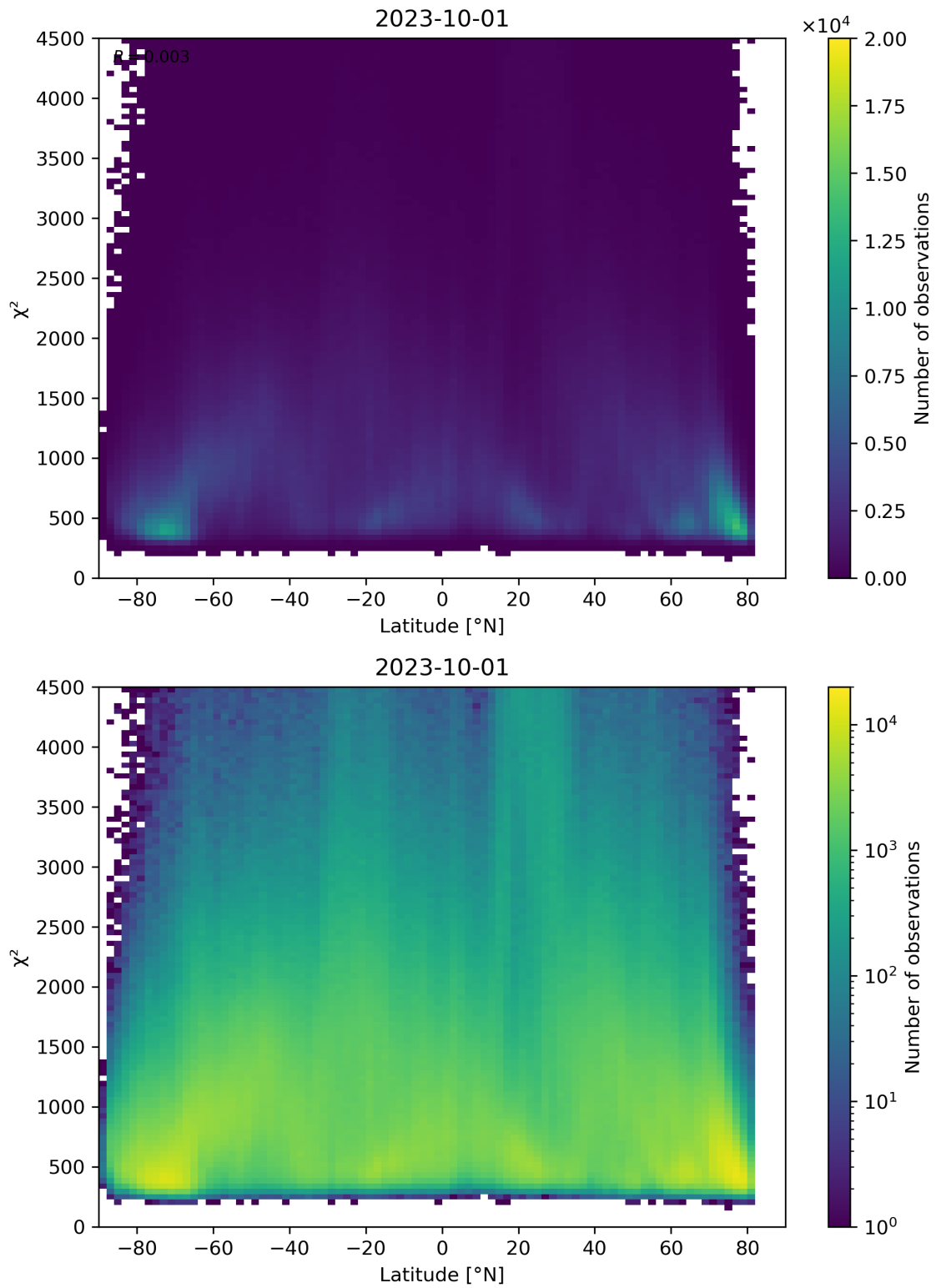
Figure 54: Scatter density plot of “Latitude” against “ \chi^2 ” for 2023-10-01 to 2023-10-02.
