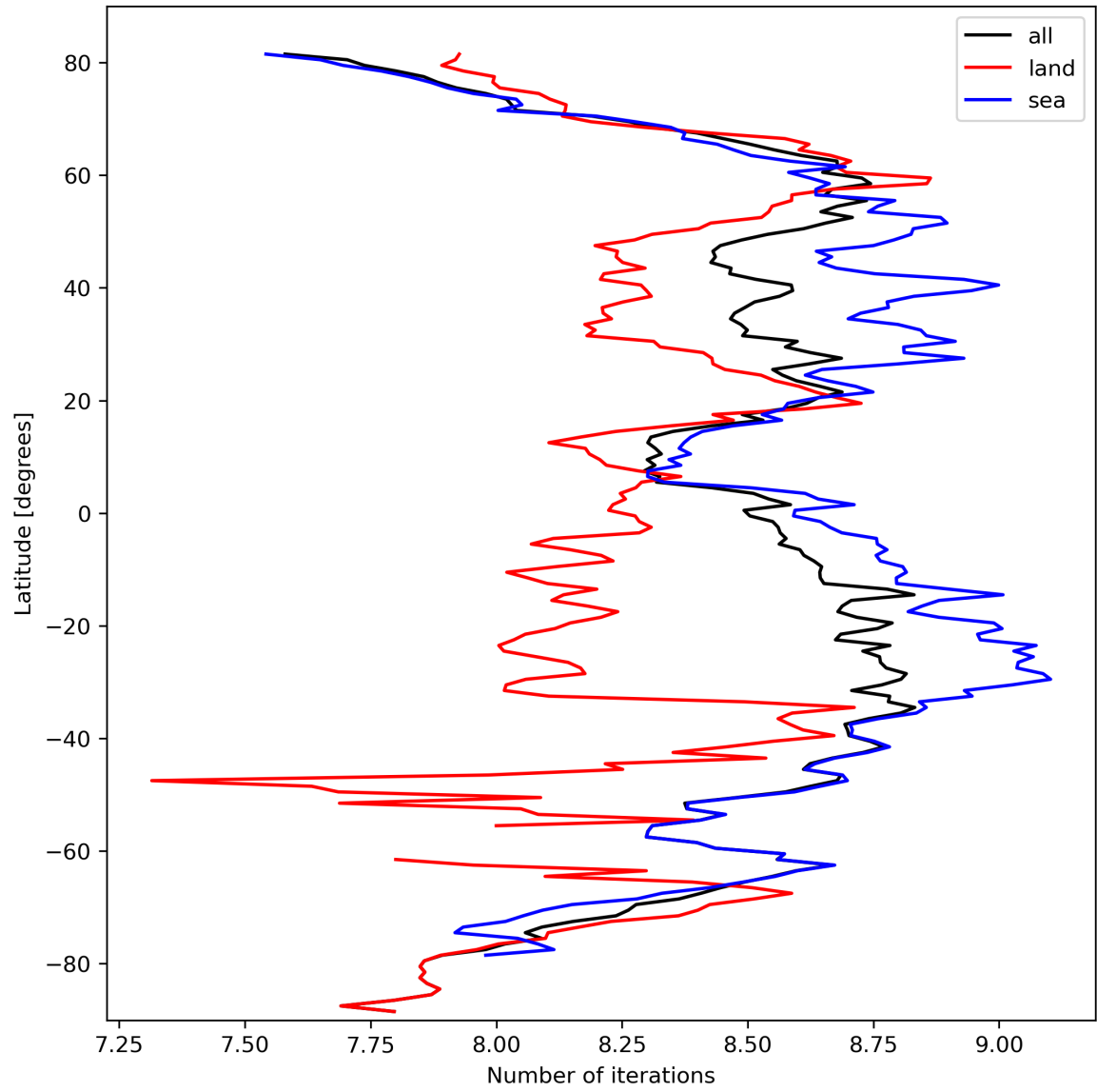
Figure 16: Zonal average of “Number of iterations” for 2023-10-01 to 2023-10-02.
