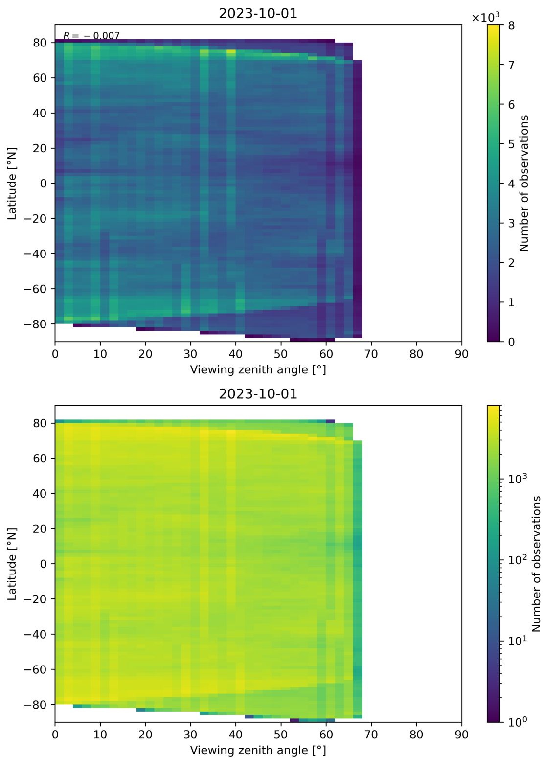
Figure 74: Scatter density plot of “Viewing zenith angle” against “Latitude” for 2023-10-01 to 2023-10-02.
