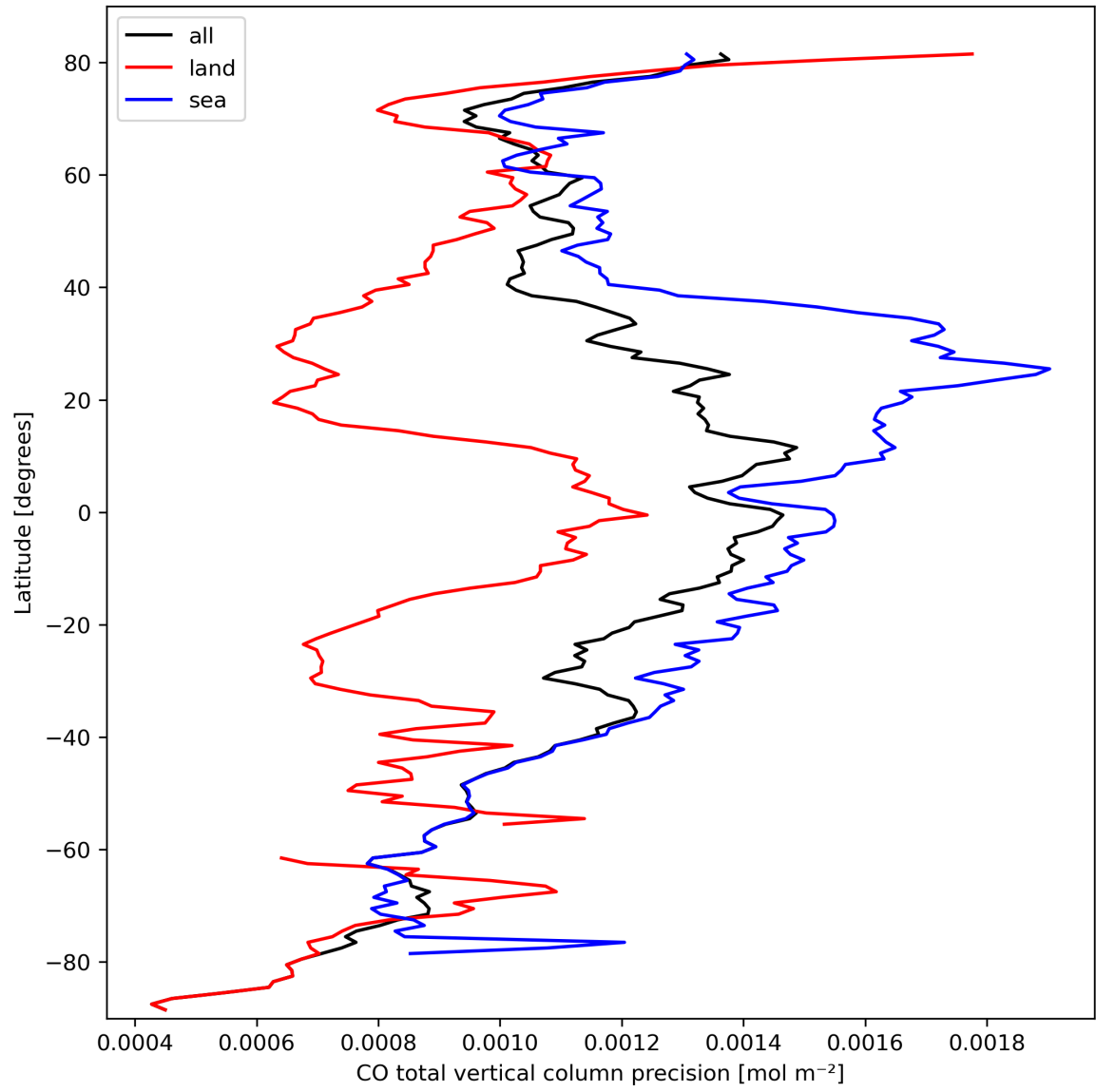
Figure 12: Zonal average of “CO total vertical column precision” for 2023-10-01 to 2023-10-02.
