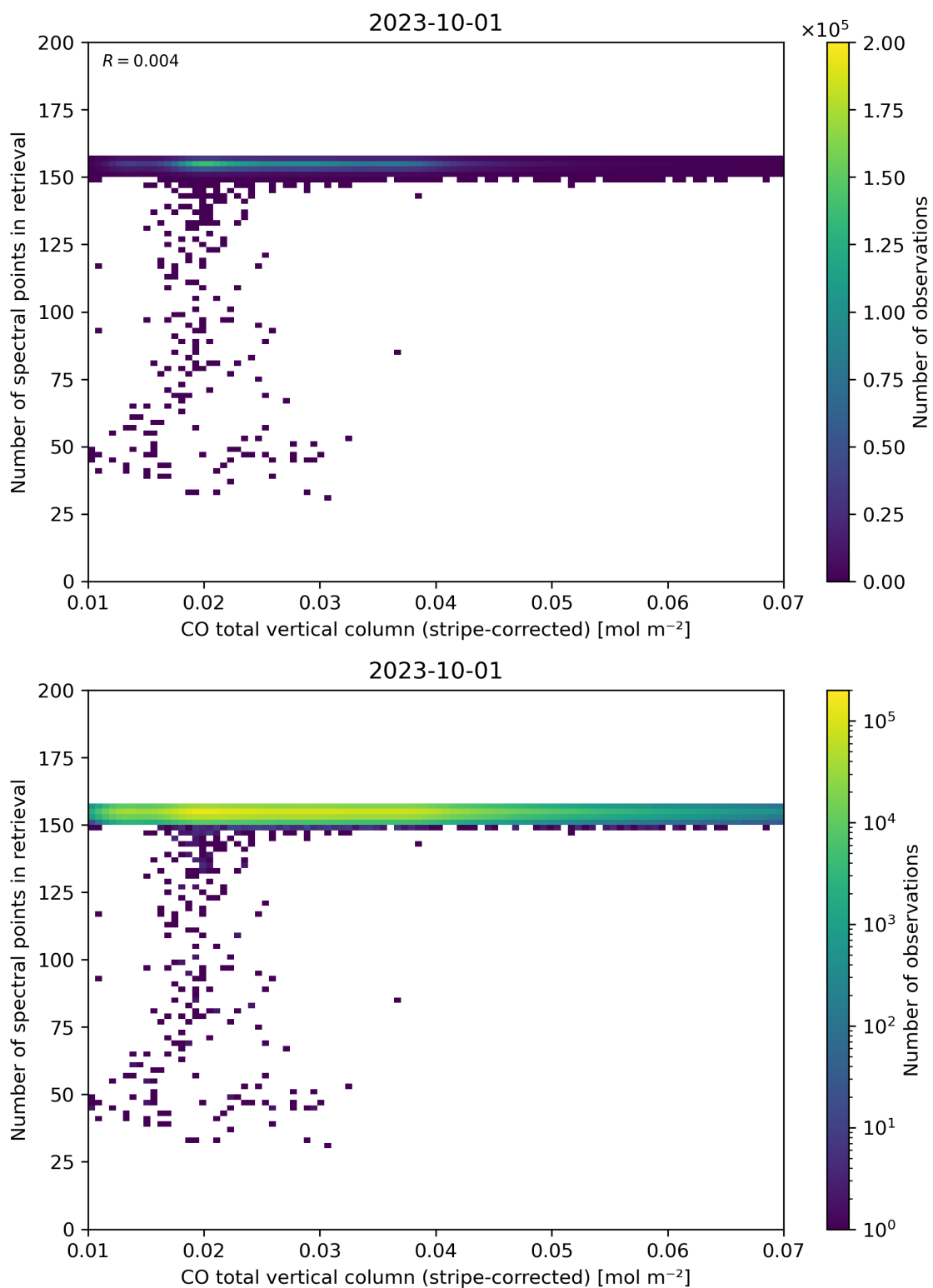
Figure 40: Scatter density plot of “CO total vertical column (stripe-corrected)” against “Number of spectral points in retrieval” for 2023-10-01 to 2023-10-02.
