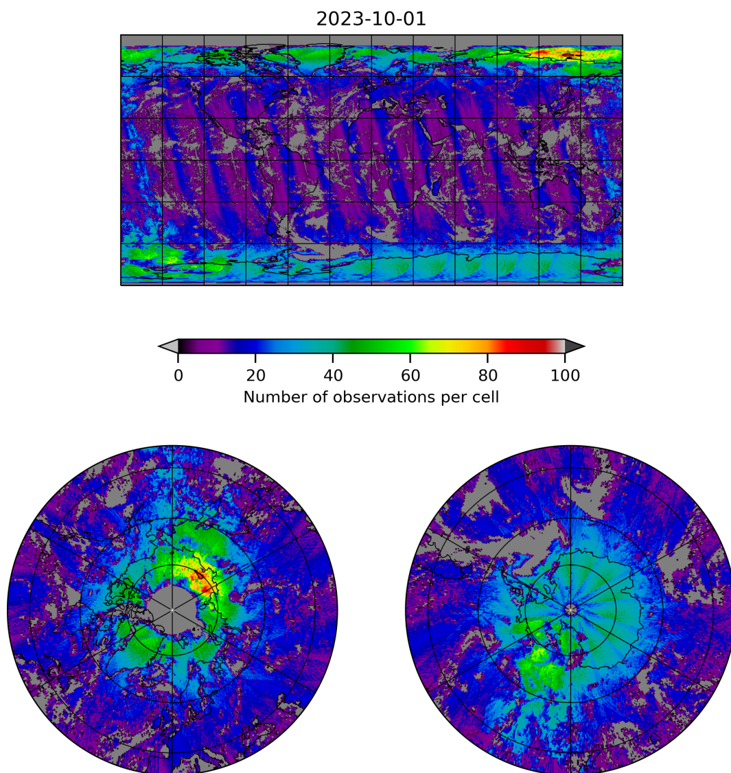
Figure 8: Map of the number of observations for 2023-10-01 to 2023-10-02
