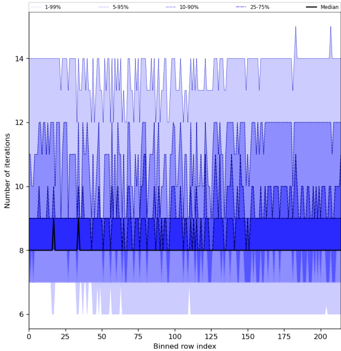
Figure 32: Along track statistics of “Number of iterations” for 2023-10-01 to 2023-10-02
