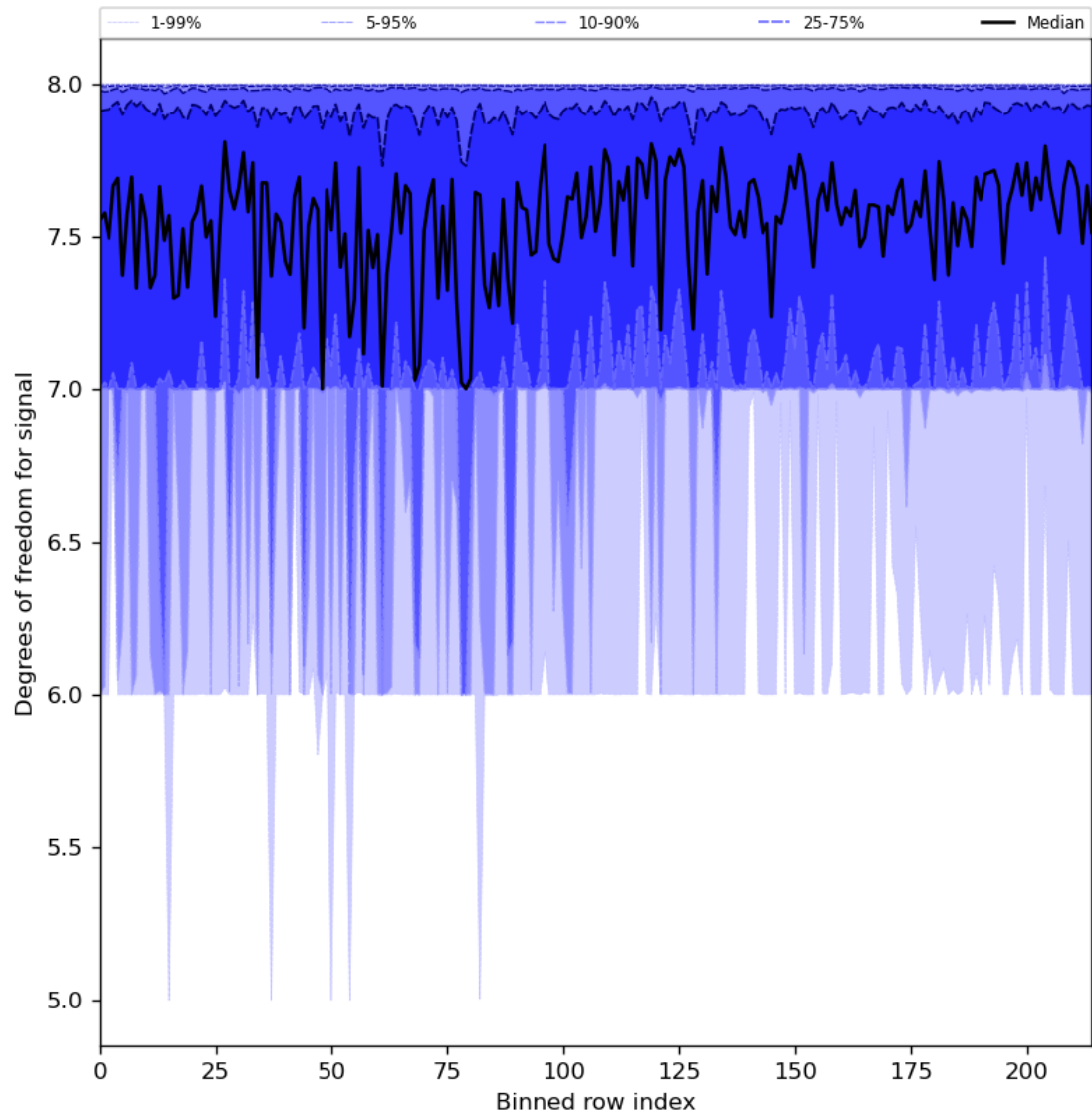
Figure 31: Along track statistics of “Degrees of freedom for signal” for 2023-10-01 to 2023-10-02
