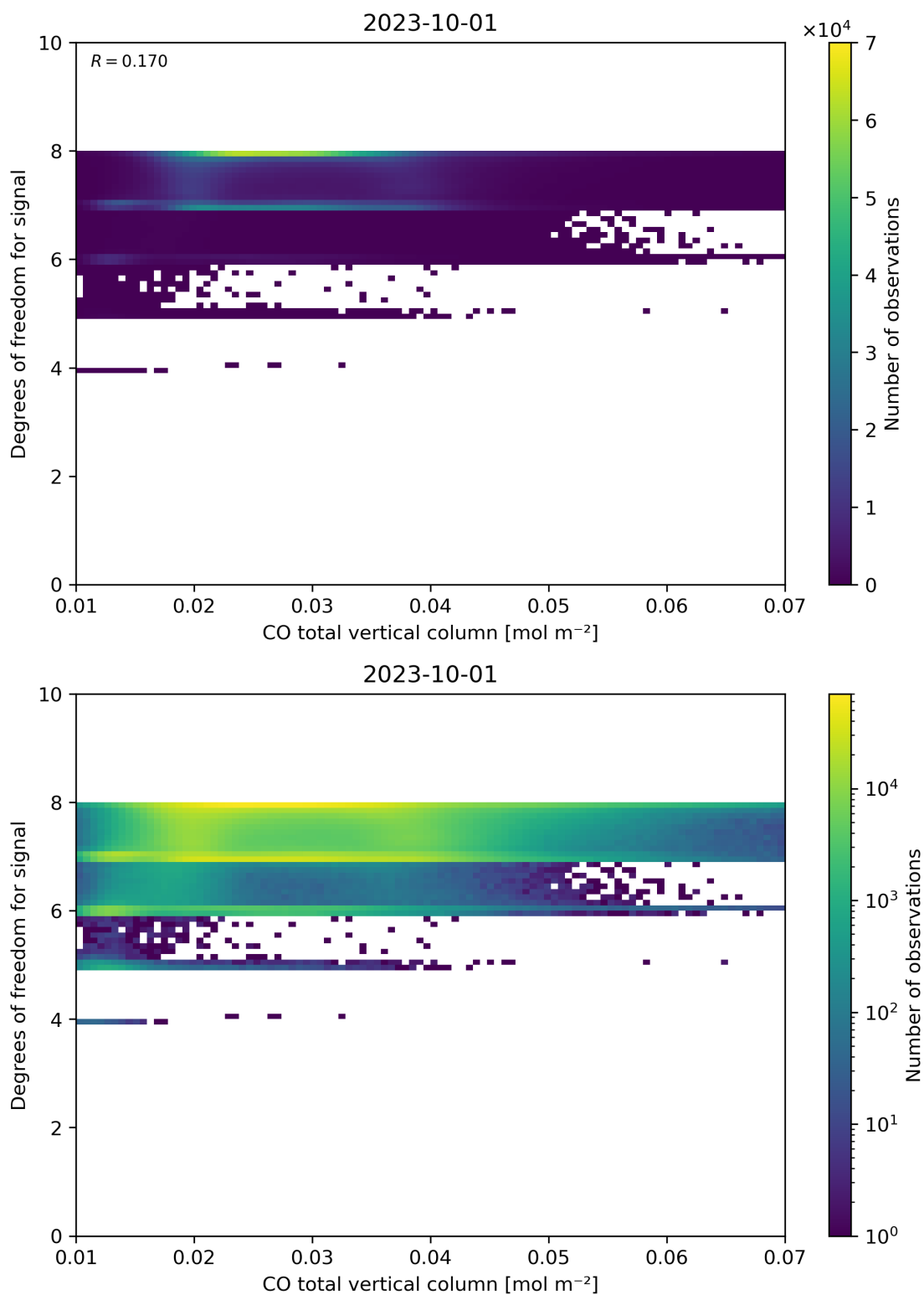
Figure 41: Scatter density plot of “CO total vertical column” against “Degrees of freedom for signal” for 2023-10-01 to 2023-10-02.
