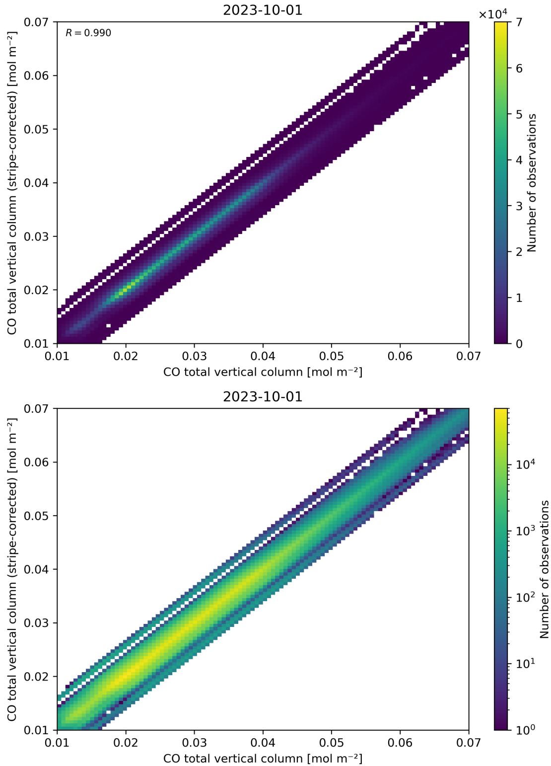
Figure 33: Scatter density plot of “CO total vertical column” against “CO total vertical column (stripe-corrected)” for 2023-10-01 to 2023-10-02.
