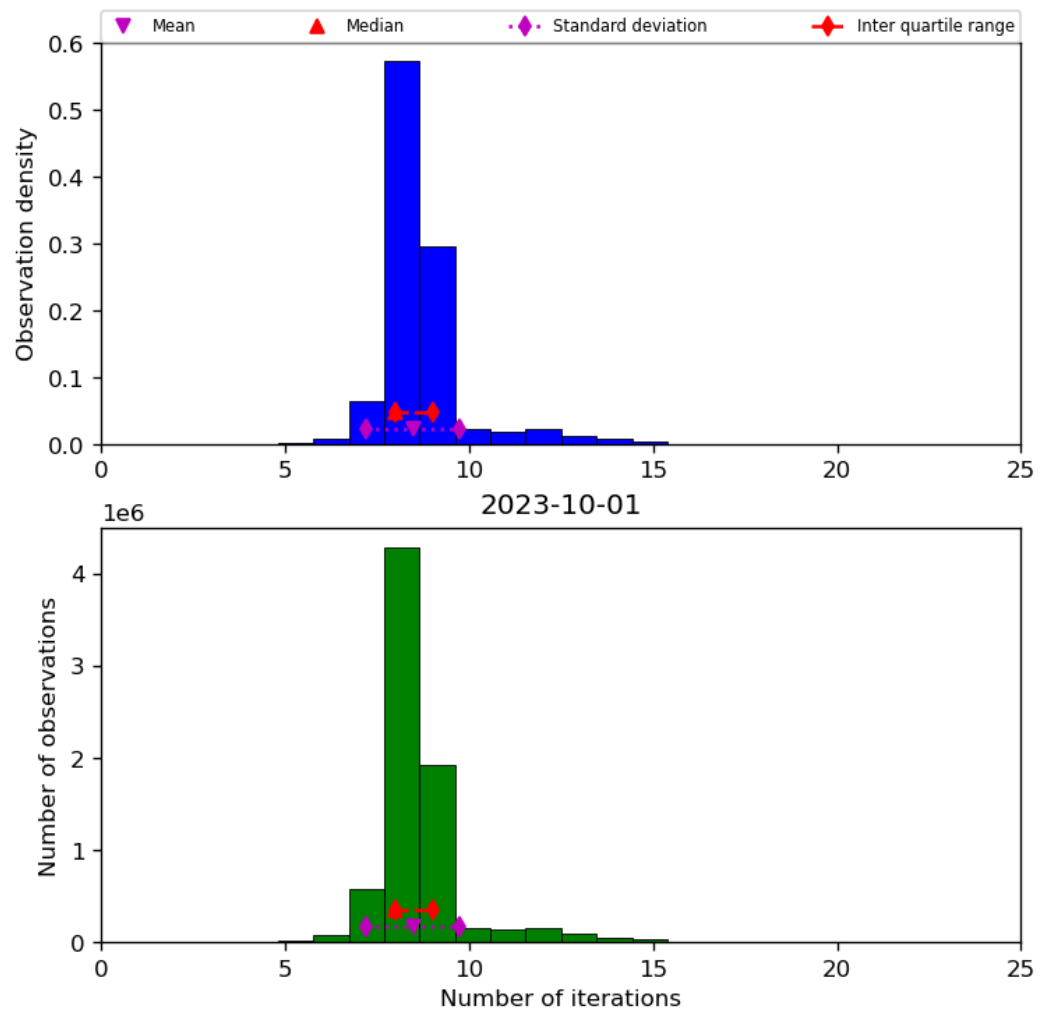
Figure 24: Histogram of “Number of iterations” for 2023-10-01 to 2023-10-02
