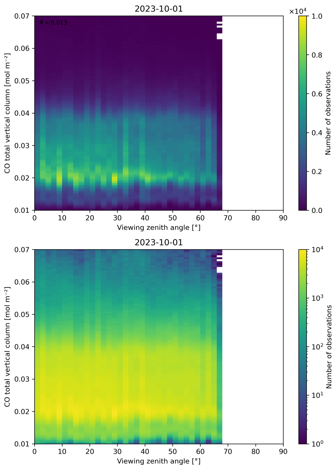
Figure 69: Scatter density plot of “Viewing zenith angle” against “CO total vertical column” for 2023-10-01 to 2023-10-02.
