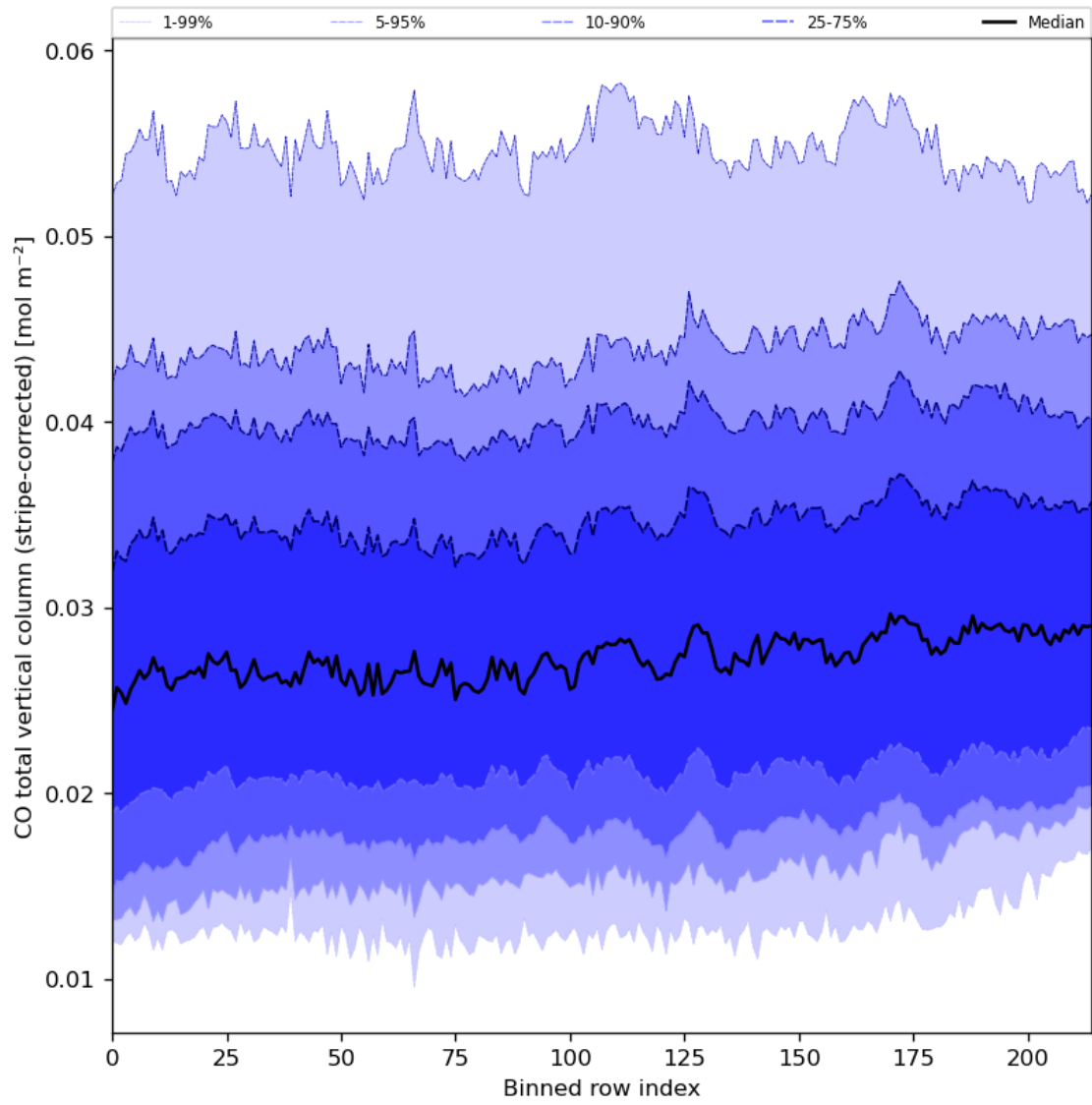
Figure 27: Along track statistics of “CO total vertical column (stripe-corrected)” for 2023-10-01 to 2023-10-02
