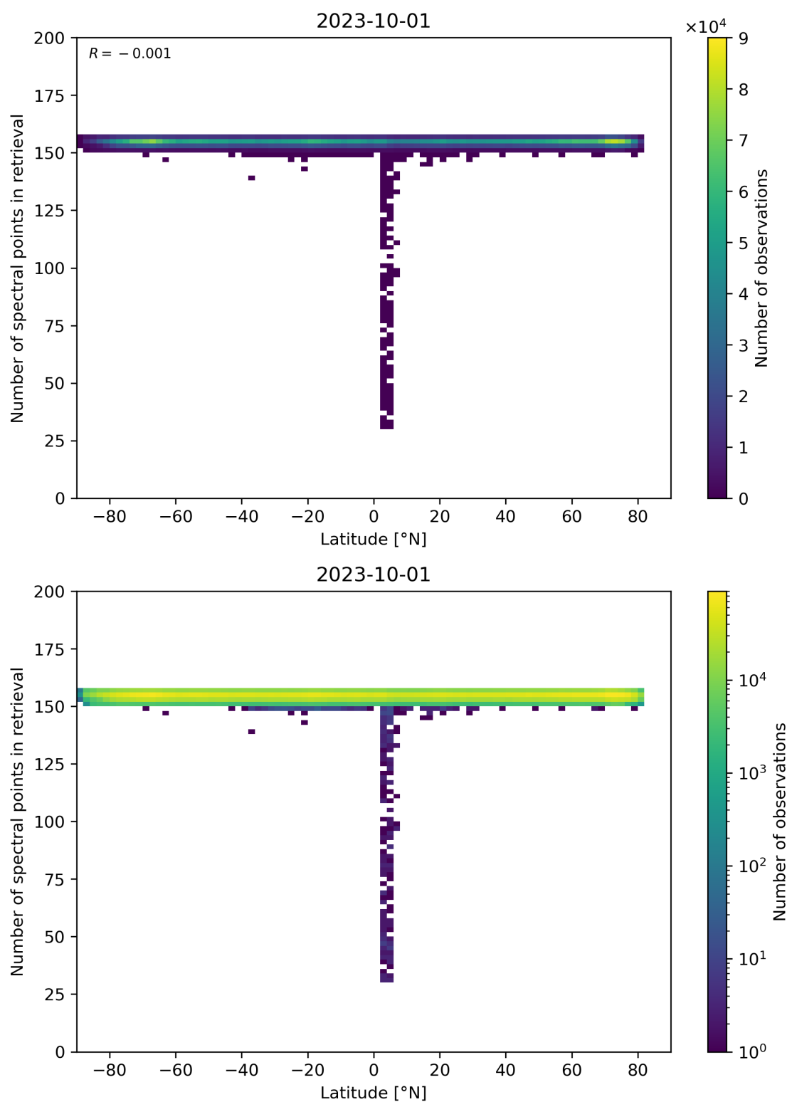
Figure 57: Scatter density plot of “Latitude” against “Number of spectral points in retrieval” for 2023-10-01 to 2023-10-02.
