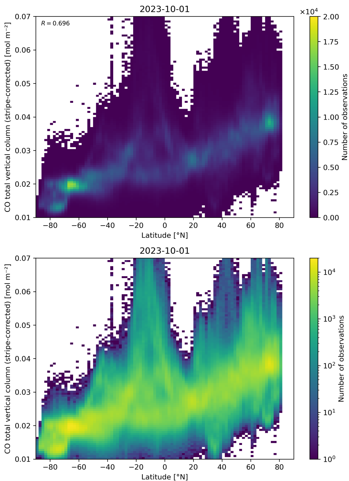
Figure 52: Scatter density plot of “Latitude” against “CO total vertical column (stripe-corrected)” for 2023-10-01 to 2023-10-02.
