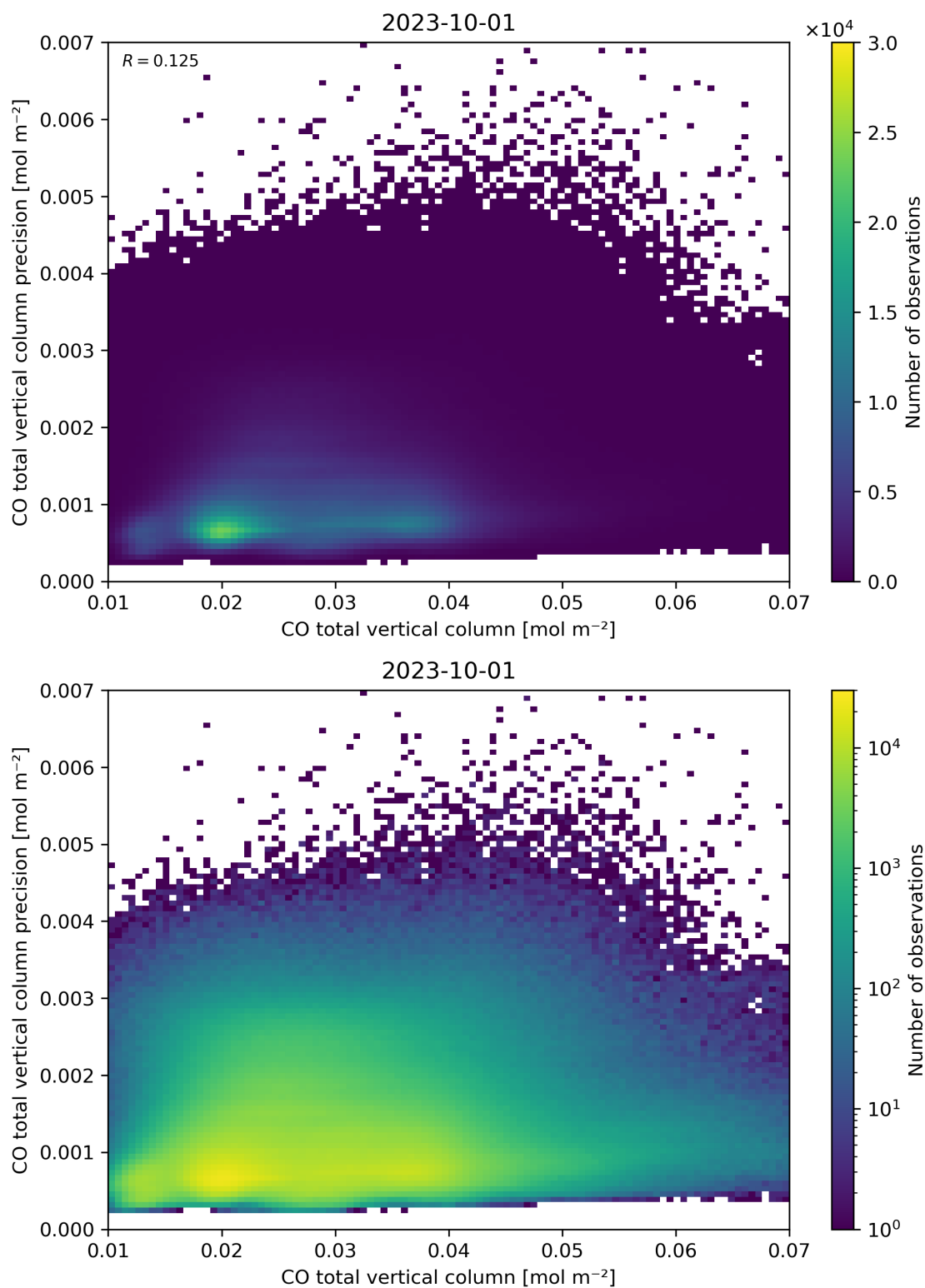
Figure 34: Scatter density plot of “CO total vertical column” against “CO total vertical column precision” for 2023-10-01 to 2023-10-02.
