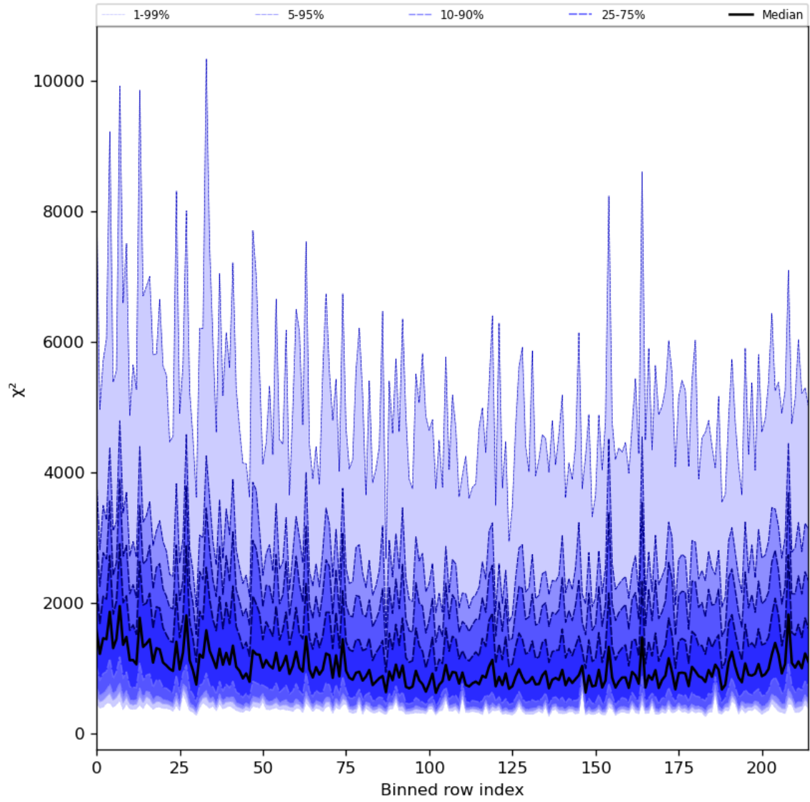
Figure 30: Along track statistics of “ \chi^2 ” for 2023-10-01 to 2023-10-02
