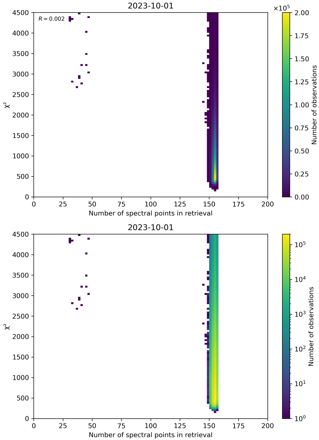
Figure 58: Scatter density plot of “Number of spectral points in retrieval” against “ \chi^2 ” for 2023-10-01 to 2023-10-02.
