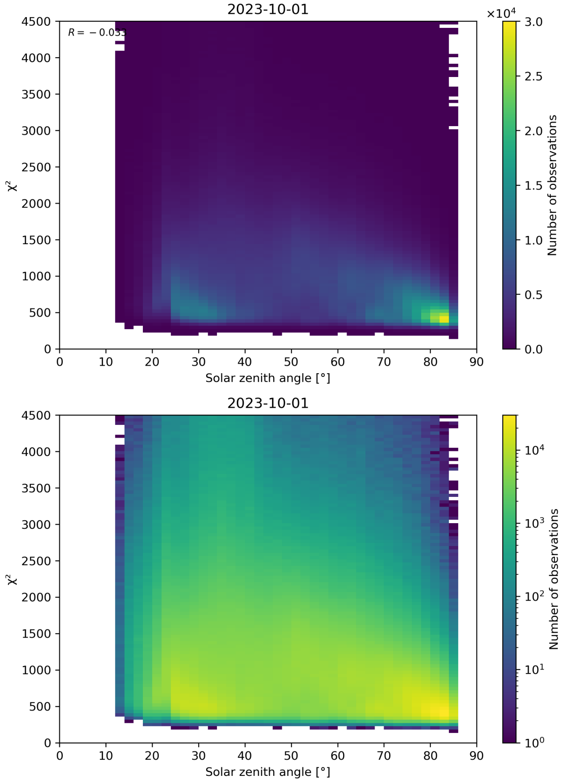
Figure 64: Scatter density plot of “Solar zenith angle” against “ \chi^2 ” for 2023-10-01 to 2023-10-02.
