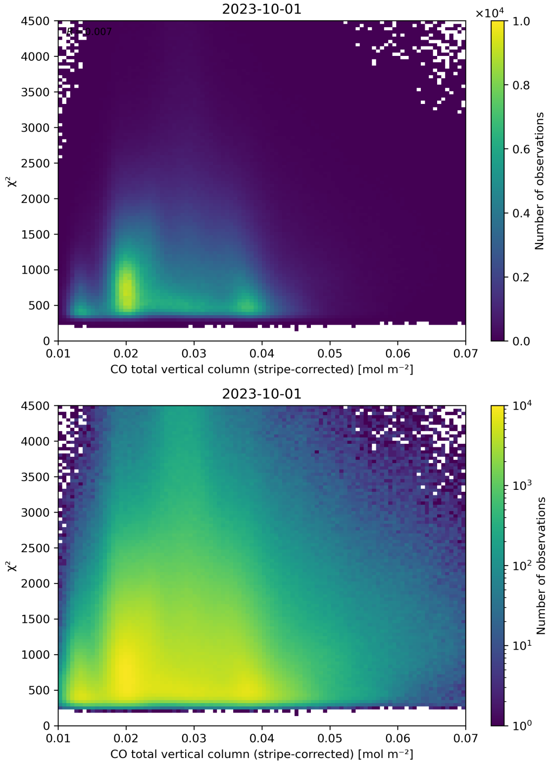
Figure 37: Scatter density plot of “CO total vertical column (stripe-corrected)” against “ \chi^2 ” for 2023-10-01 to 2023-10-02.
