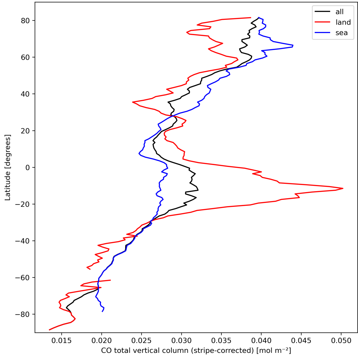
Figure 11: Zonal average of “CO total vertical column (stripe-corrected)” for 2023-10-01 to 2023-10-02.
