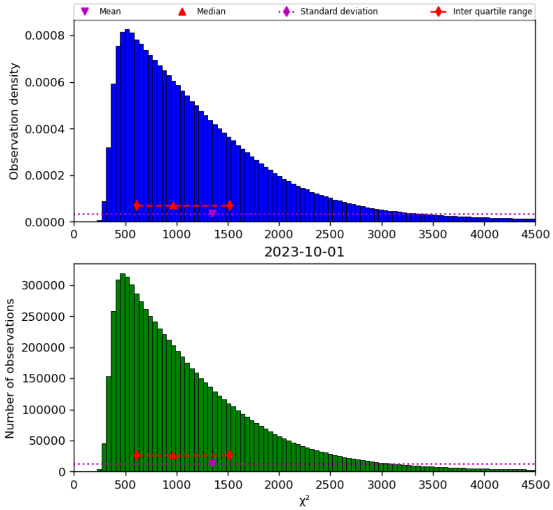
Figure 22: Histogram of “ \chi^2 ” for 2023-10-01 to 2023-10-02
