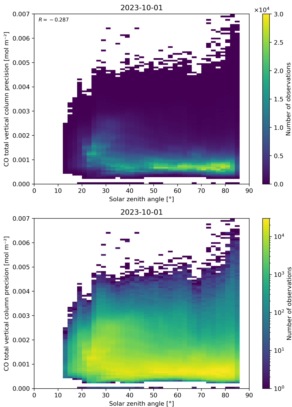
Figure 63: Scatter density plot of “Solar zenith angle” against “CO total vertical column precision” for 2023-10-01 to 2023-10-02.
