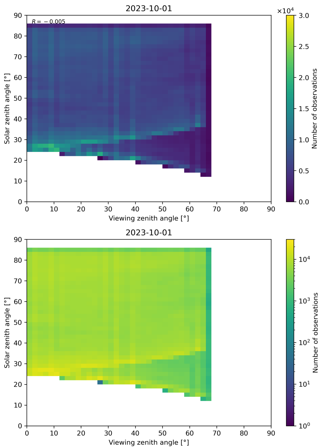
Figure 77: Scatter density plot of “Viewing zenith angle” against “Solar zenith angle” for 2023-10-01 to 2023-10-02.
