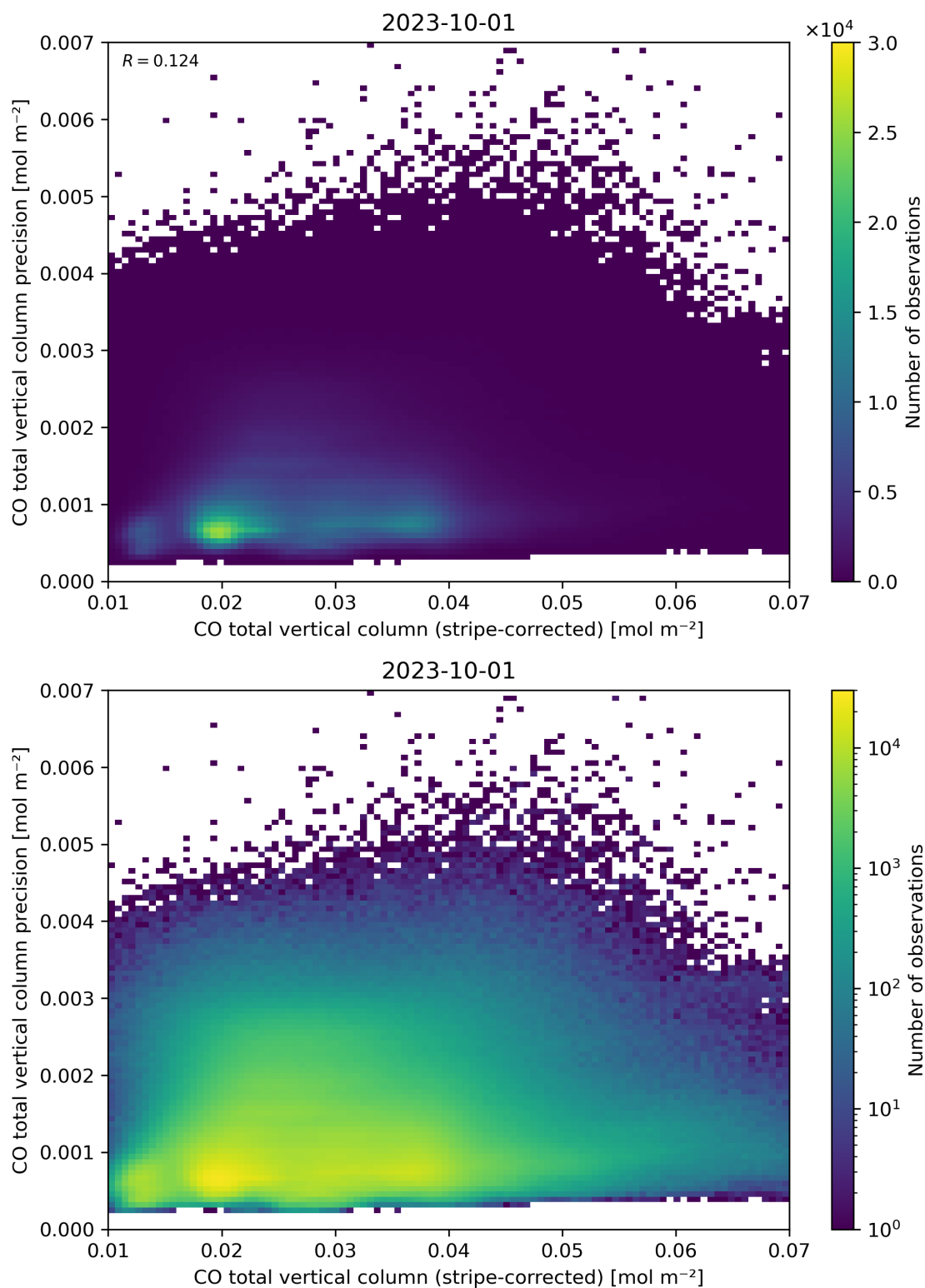
Figure 36: Scatter density plot of “CO total vertical column (stripe-corrected)” against “CO total vertical column precision” for 2023-10-01 to 2023-10-02.
