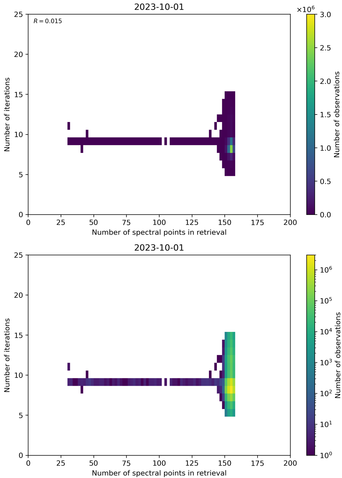
Figure 60: Scatter density plot of “Number of spectral points in retrieval” against “Number of iterations” for 2023-10-01 to 2023-10-02.
