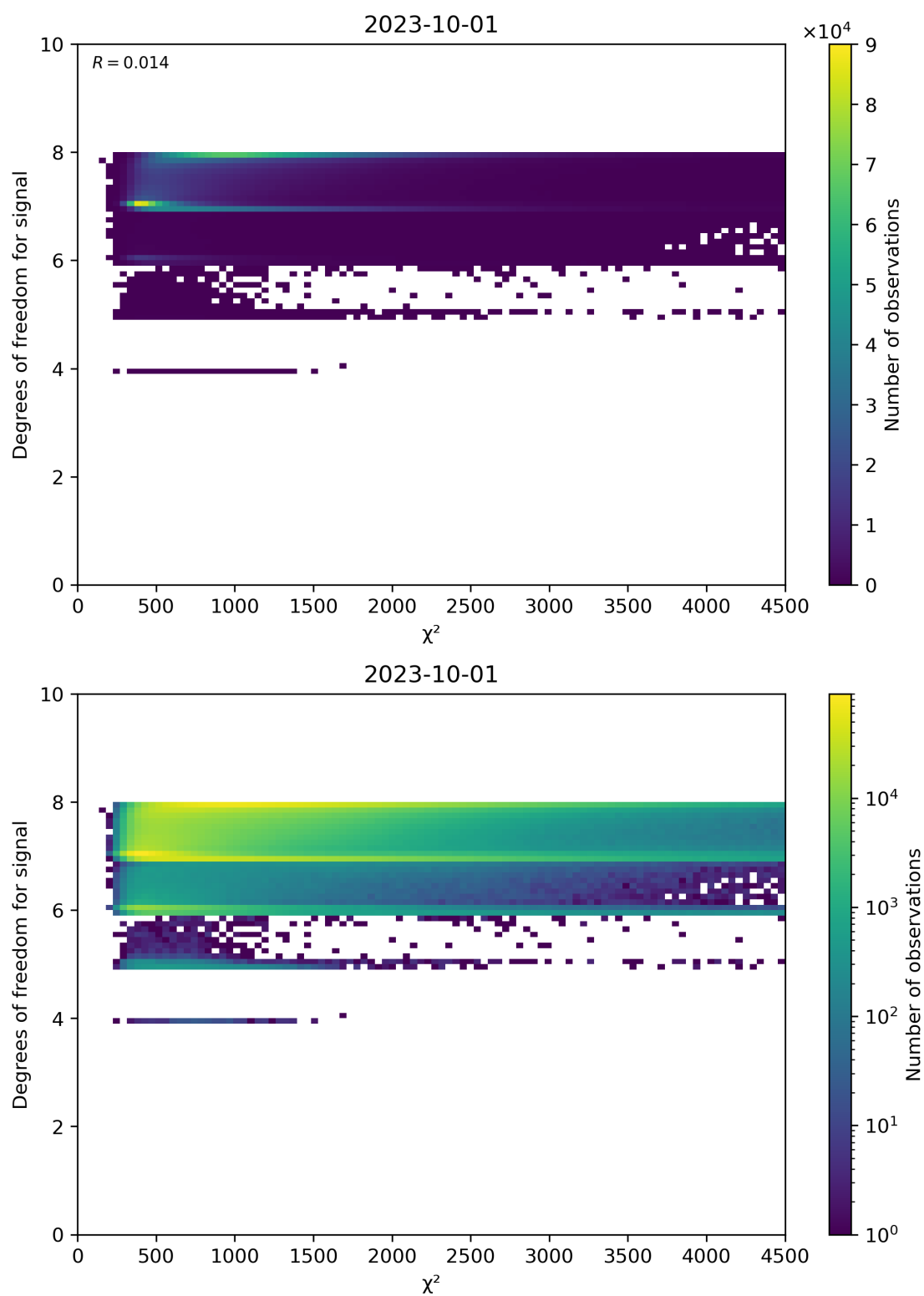
Figure 48: Scatter density plot of " \chi^2 " against "Degrees of freedom for signal" for 2023-10-01 to 2023-10-02.
