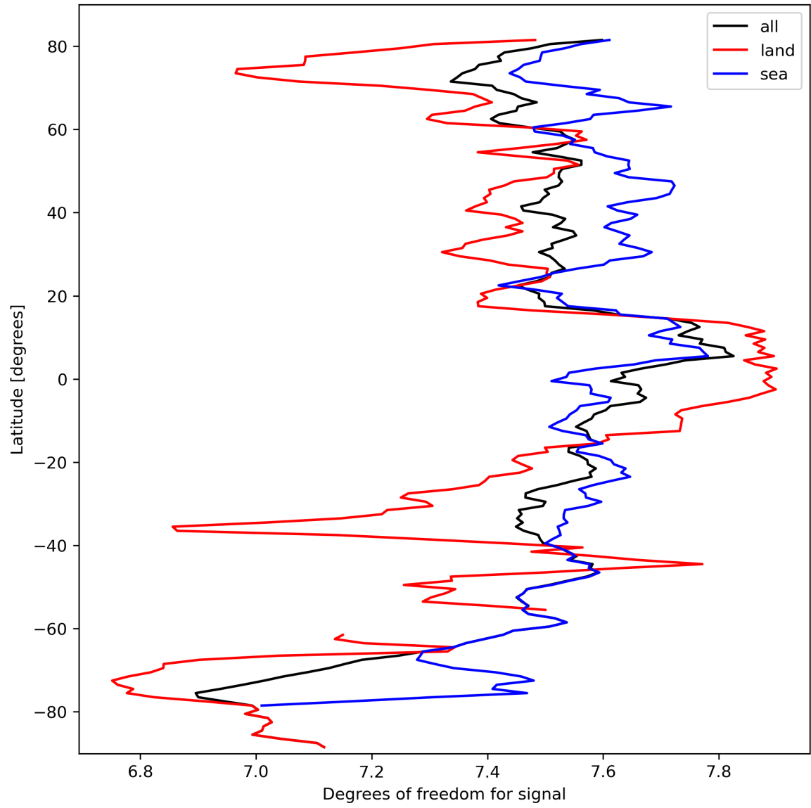
Figure 15: Zonal average of “Degrees of freedom for signal” for 2023-10-01 to 2023-10-02.
