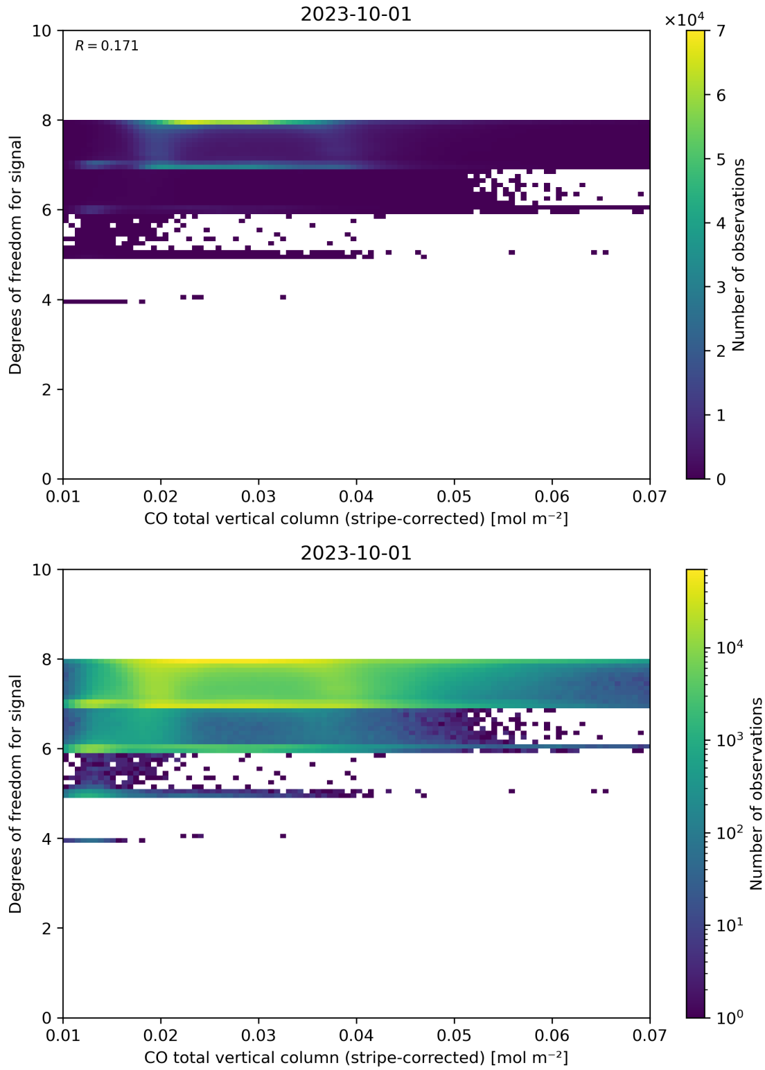
Figure 38: Scatter density plot of “CO total vertical column (stripe-corrected)” against “Degrees of freedom for signal” for 2023-10-01 to 2023-10-02.
