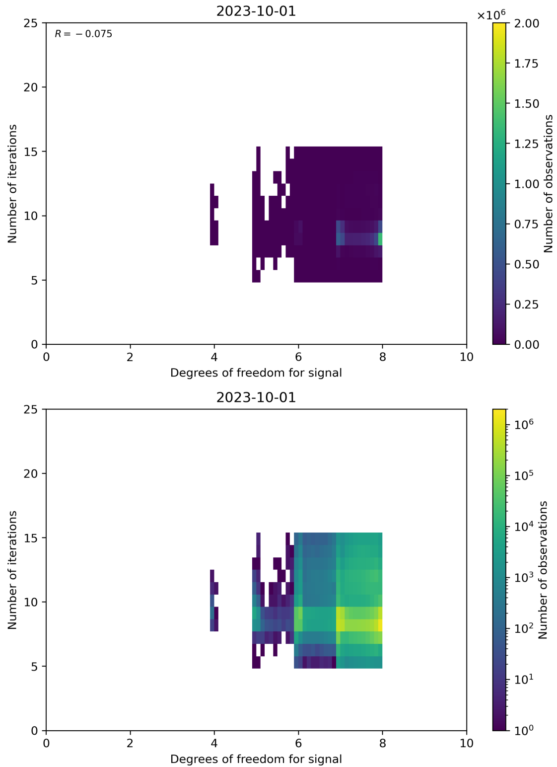
Figure 50: Scatter density plot of “Degrees of freedom for signal” against “Number of iterations” for 2023-10-01 to 2023-10-02.
