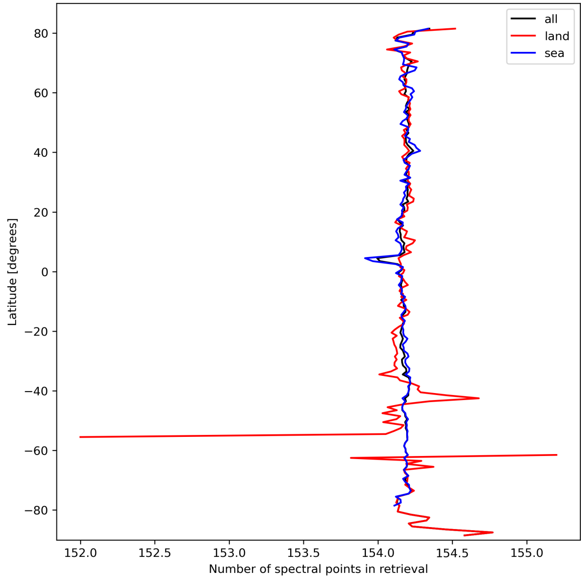
Figure 13: Zonal average of “Number of spectral points in retrieval” for 2023-10-01 to 2023-10-02.
