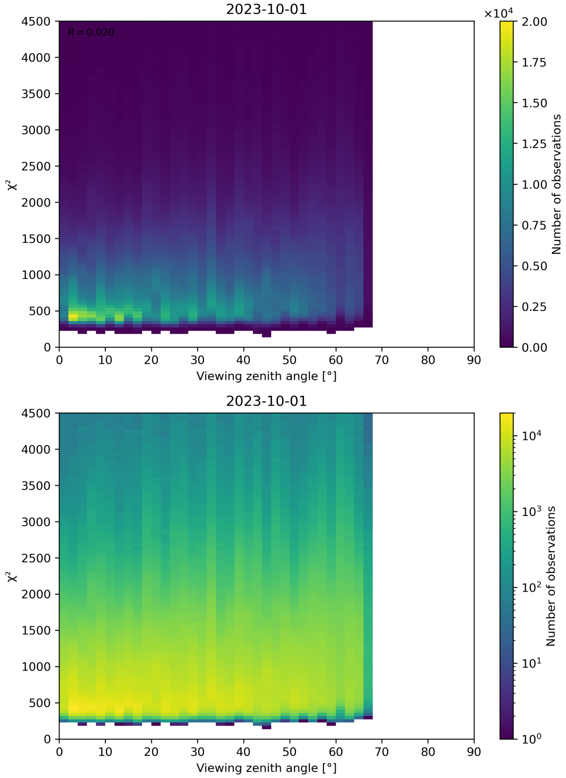
Figure 72: Scatter density plot of “Viewing zenith angle” against “ \chi^2 ” for 2023-10-01 to 2023-10-02.
