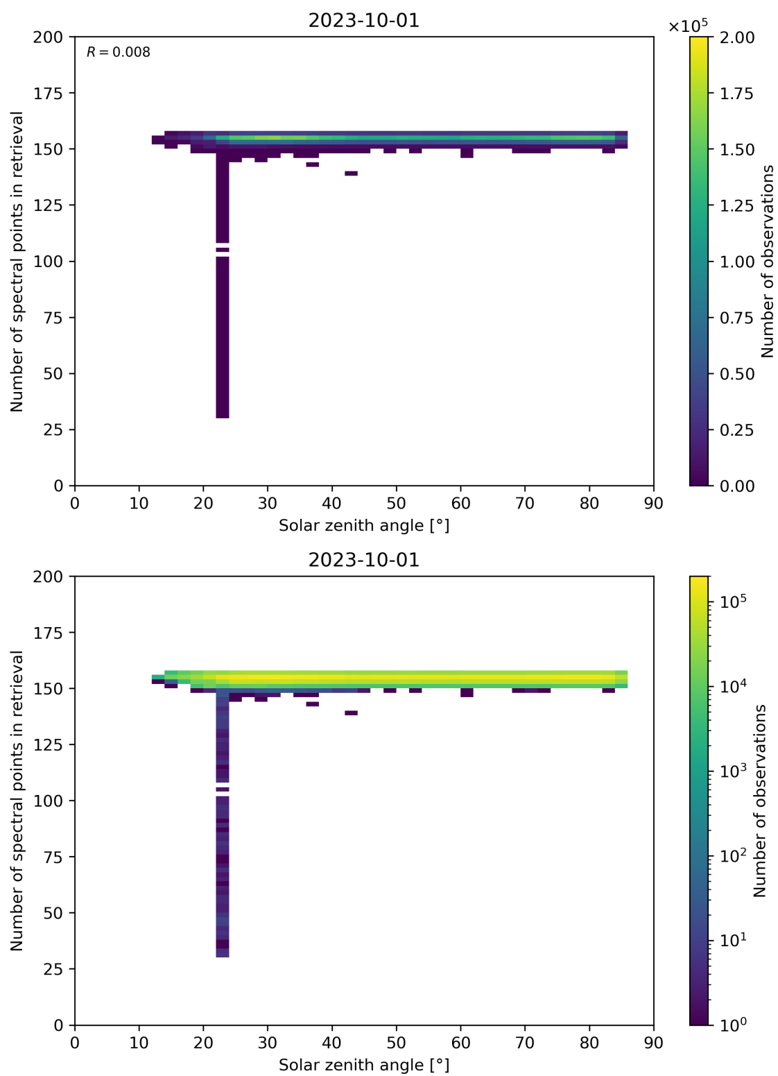
Figure 68: Scatter density plot of “Solar zenith angle” against “Number of spectral points in retrieval” for 2023-10-01 to 2023-10-02.
