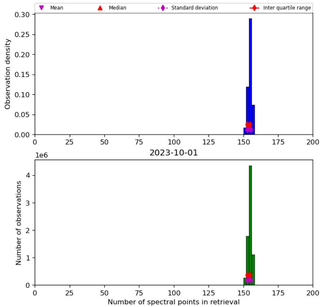
Figure 21: Histogram of “Number of spectral points in retrieval” for 2023-10-01 to 2023-10-02
