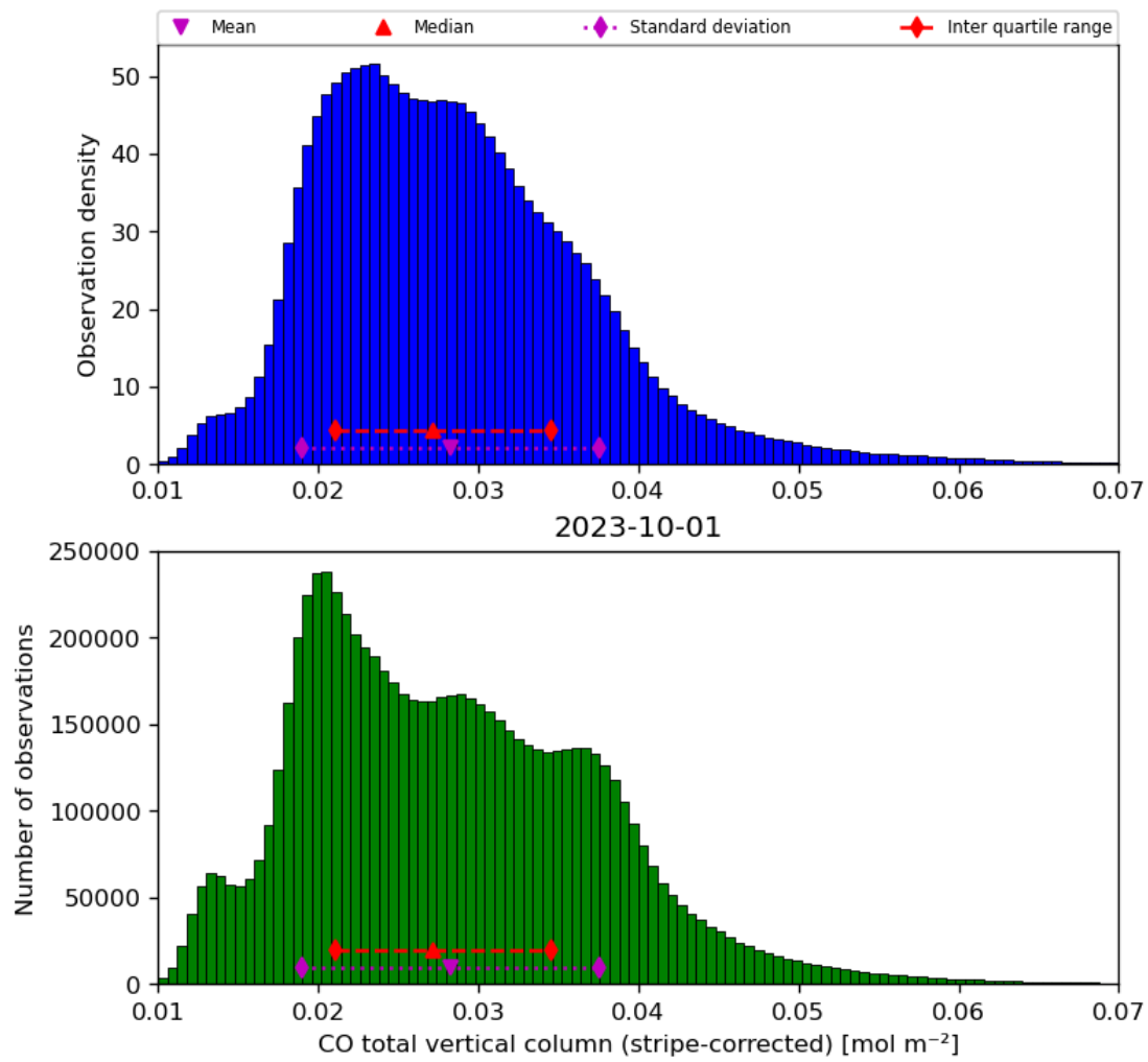
Figure 19: Histogram of “CO total vertical column (stripe-corrected)” for 2023-10-01 to 2023-10-02
