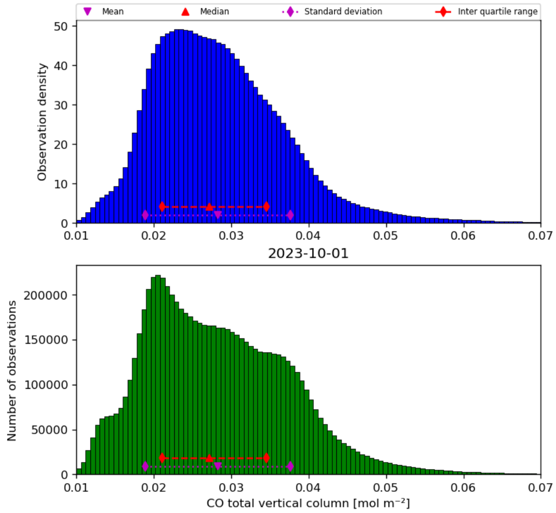
Figure 18: Histogram of “CO total vertical column” for 2023-10-01 to 2023-10-02
