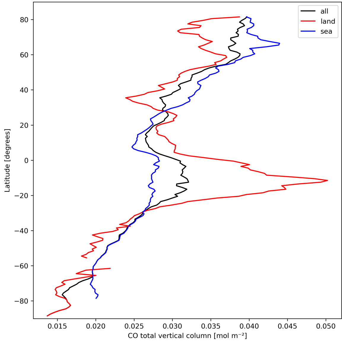
Figure 10: Zonal average of “CO total vertical column” for 2023-10-01 to 2023-10-02.
