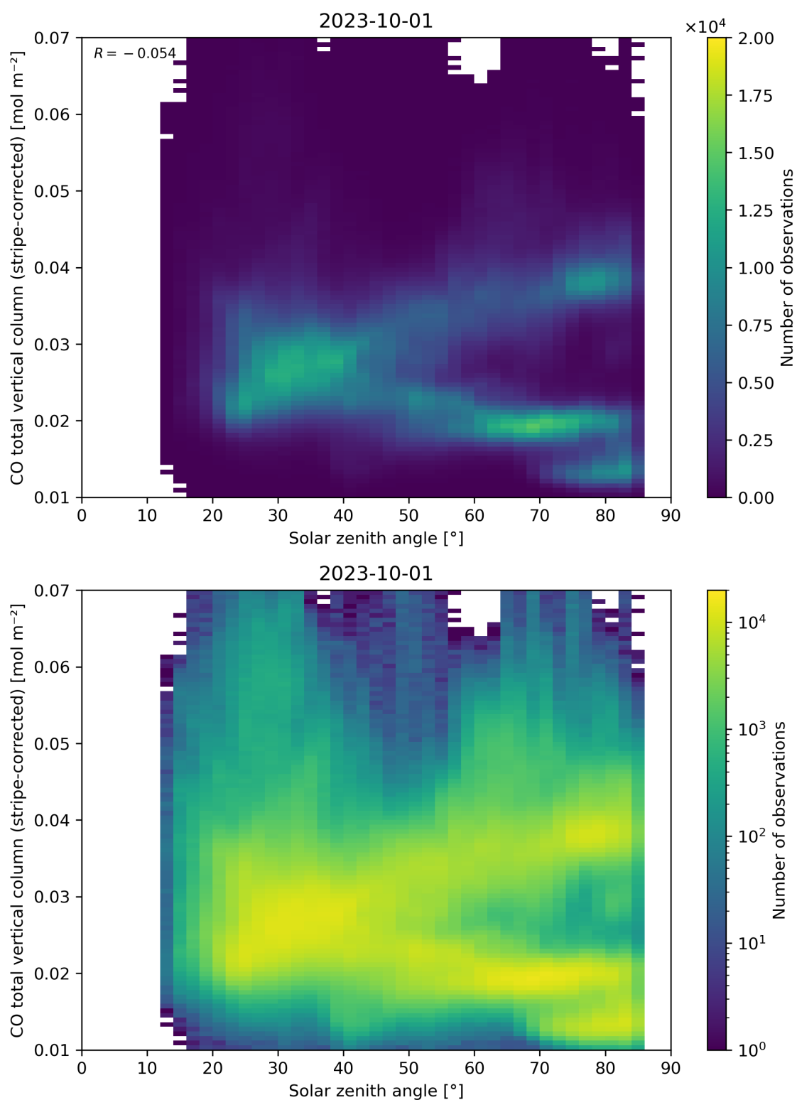
Figure 62: Scatter density plot of “Solar zenith angle” against “CO total vertical column (stripe-corrected)” for 2023-10-01 to 2023-10-02.
