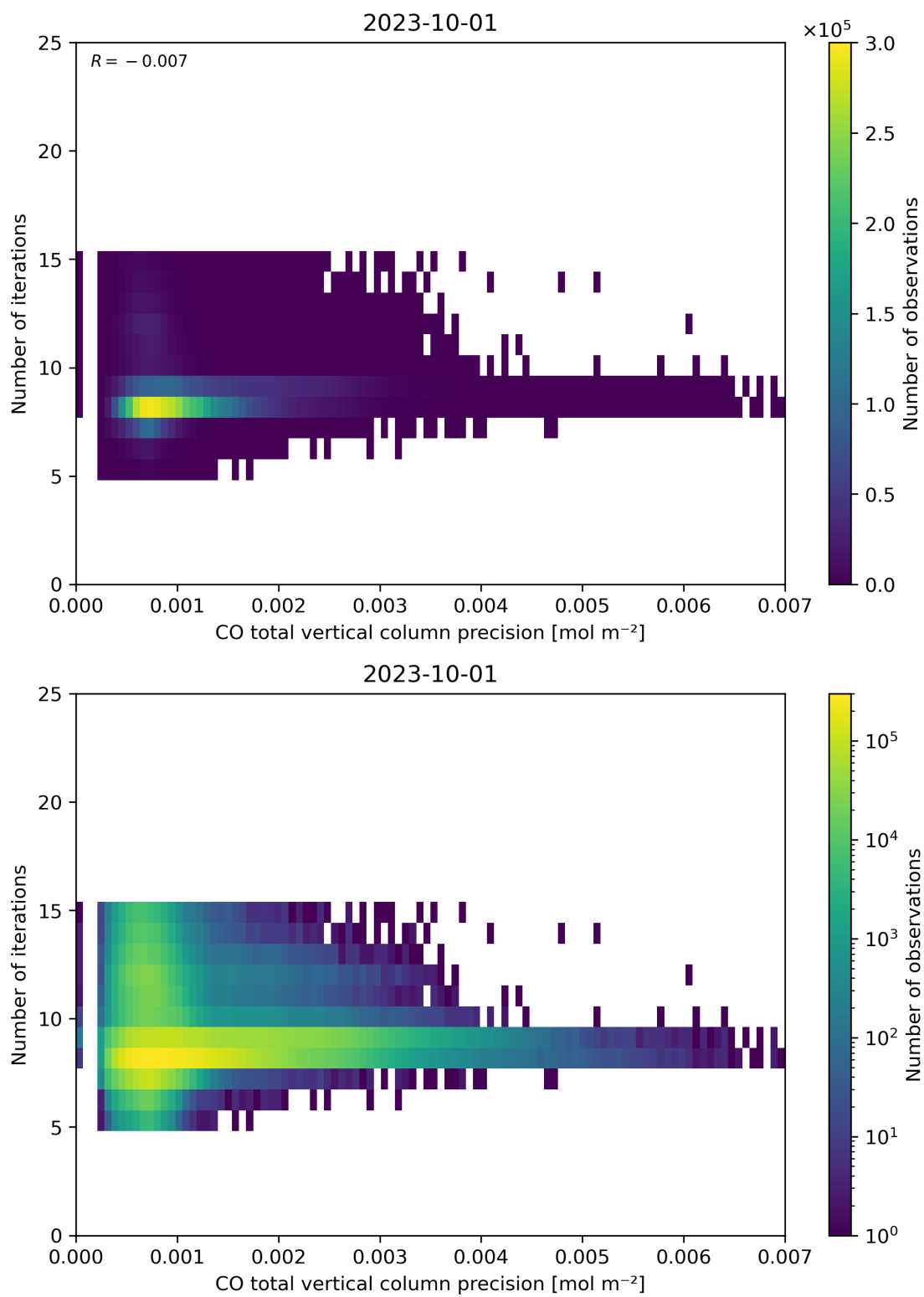
Figure 46: Scatter density plot of “CO total vertical column precision” against “Number of iterations” for 2023-10-01 to 2023-10-02.
